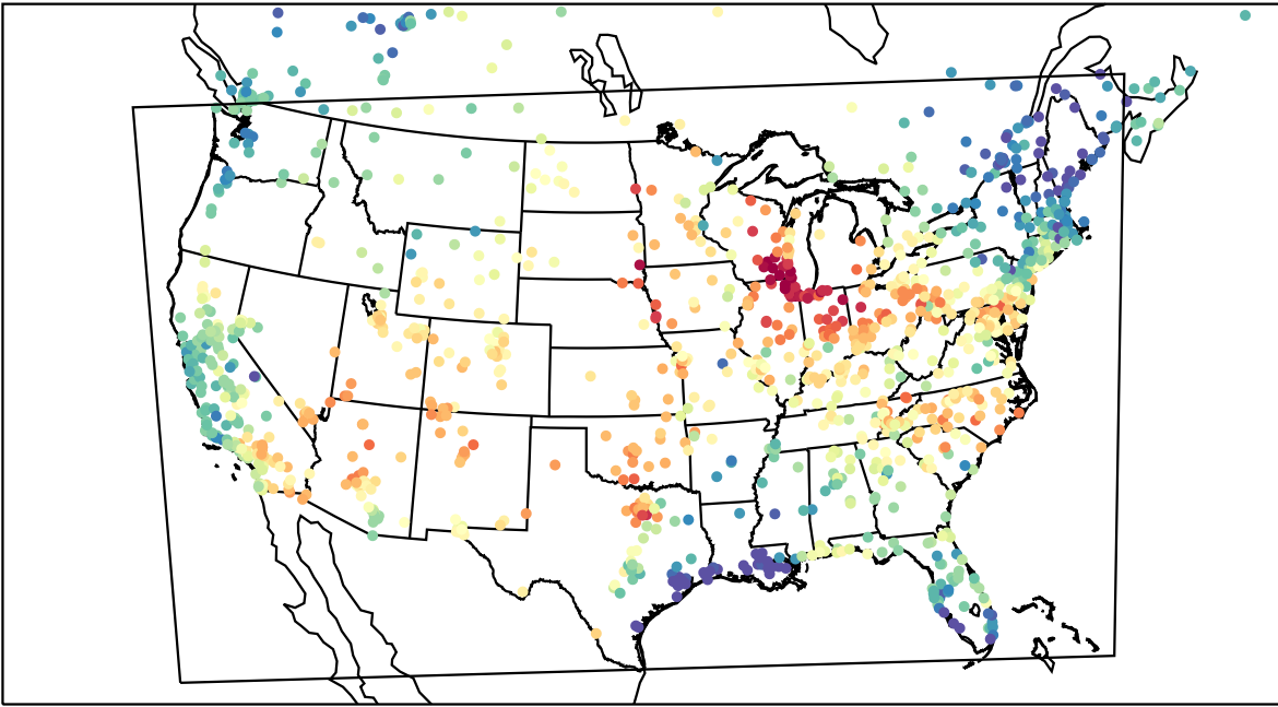
AirNOW (2023-06-18_23:00:00)
