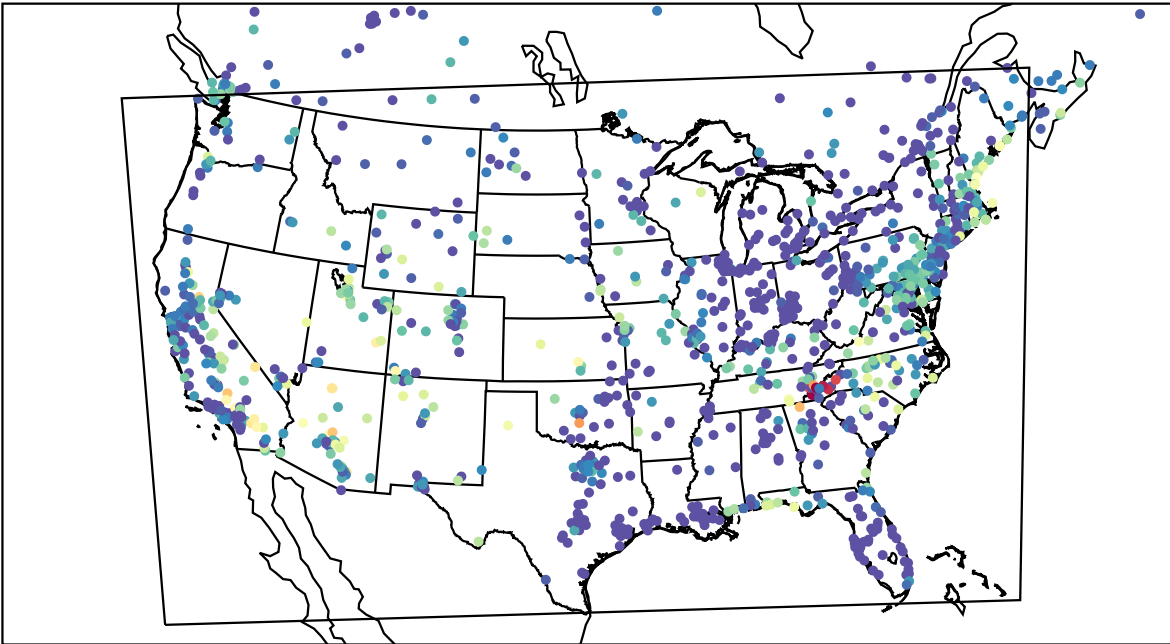
AirNOW (2023-06-17_10:00:00)
