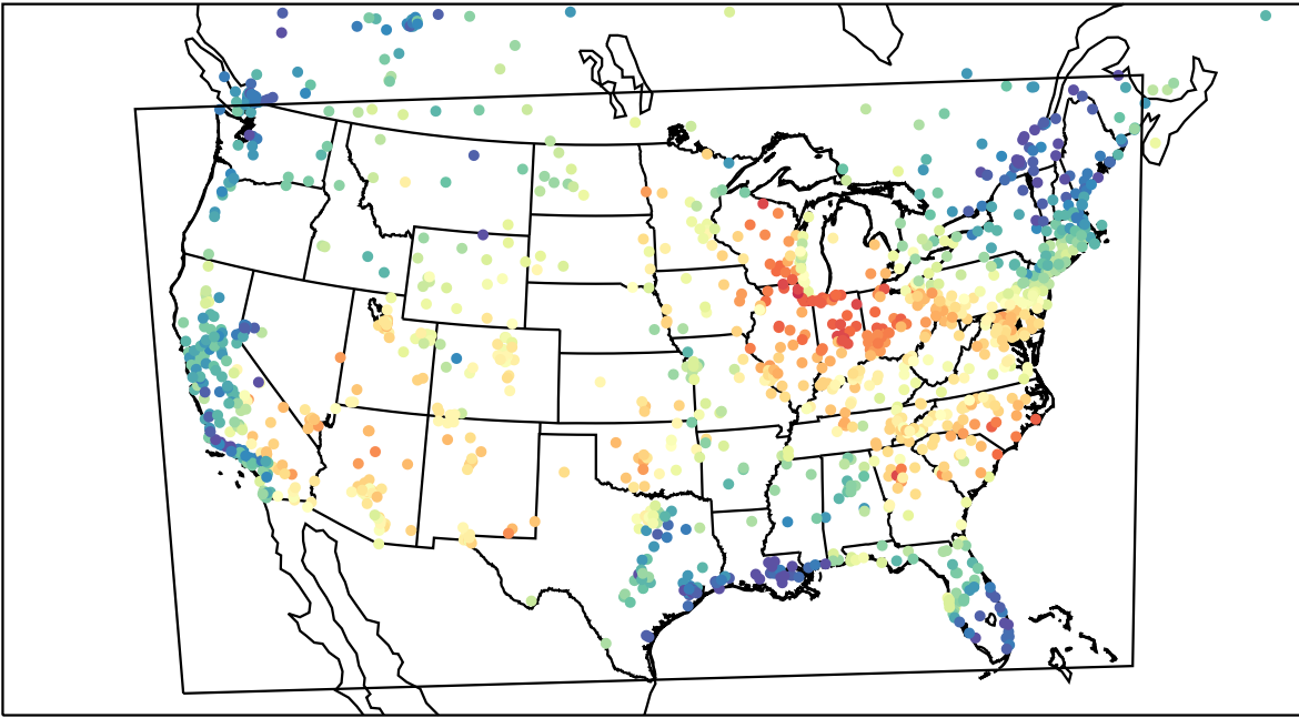
AirNOW (2023-06-18_16:00:00)
