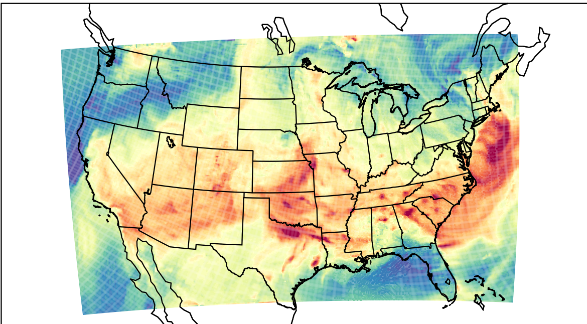
WRF (2023-06-17_19:00:00)
