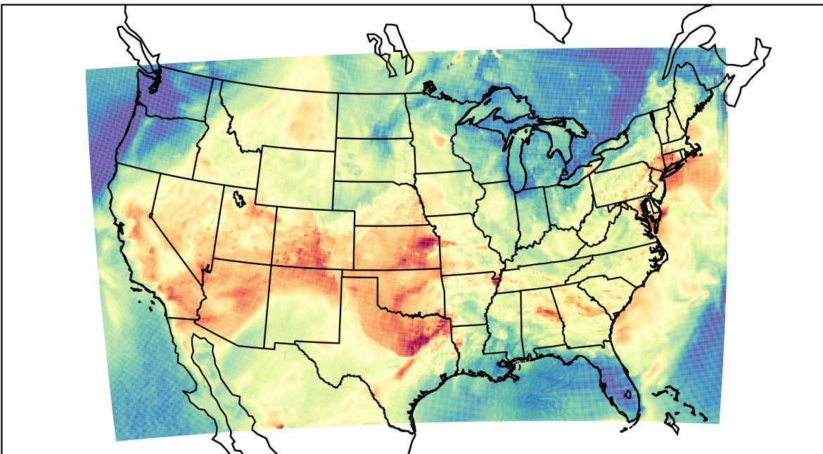
WRF (2023-06-17_00:00:00)
