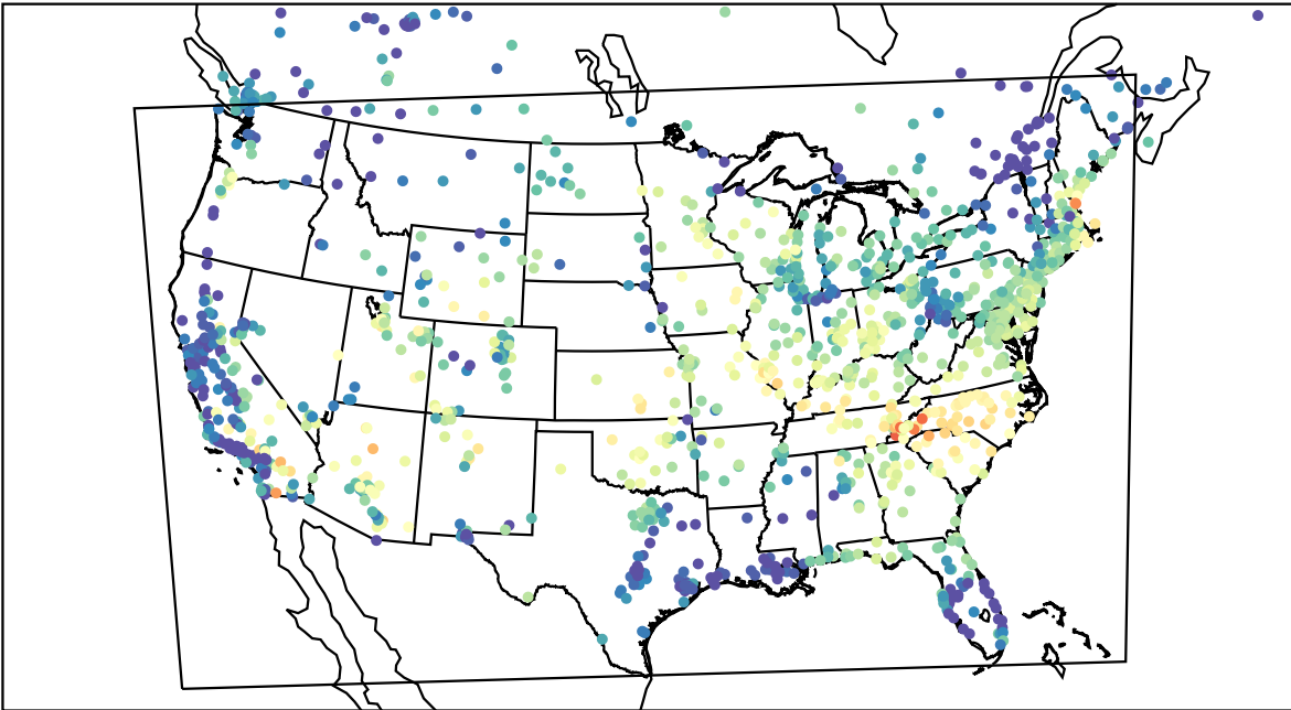
AirNOW (2023-06-17_14:00:00)
