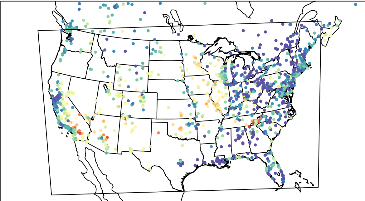
AirNOW (2023-06-18_04:00:00)
