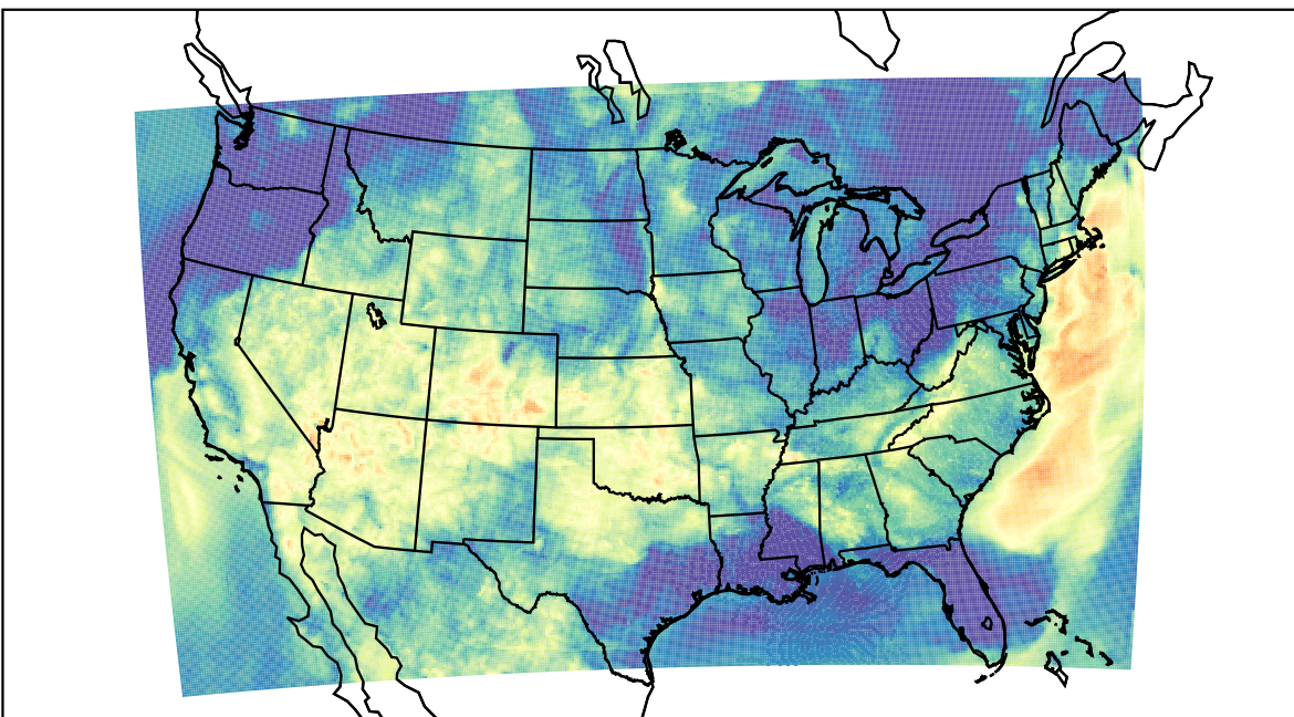
WRF (2023-06-17_09:00:00)
