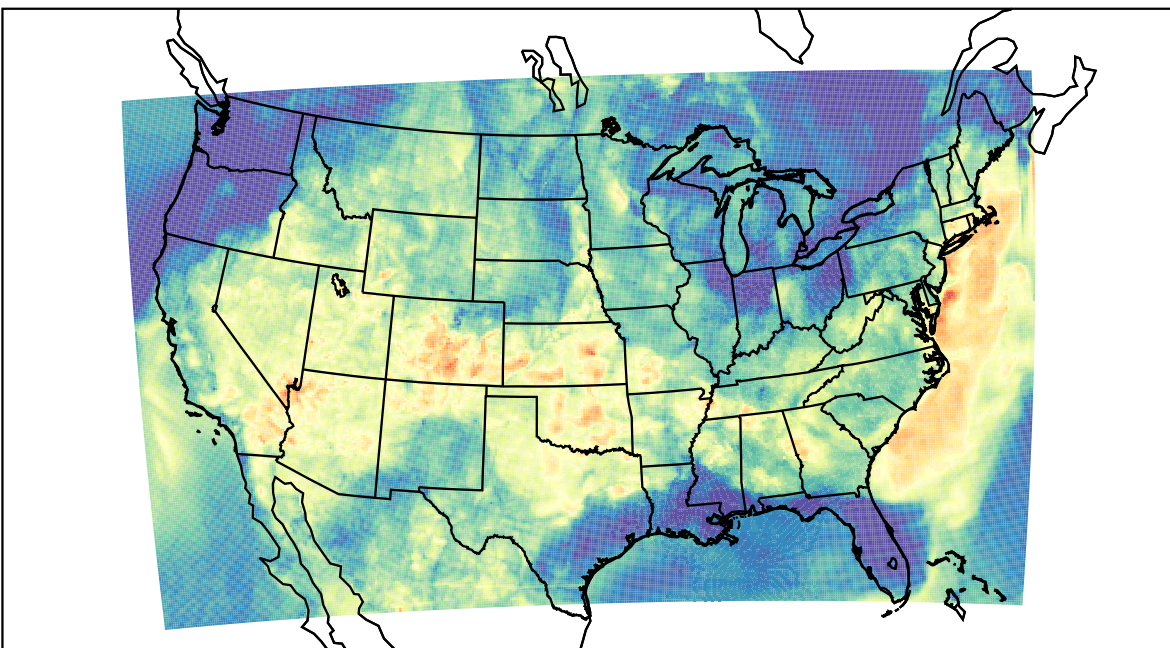
WRF (2023-06-17_05:00:00)
