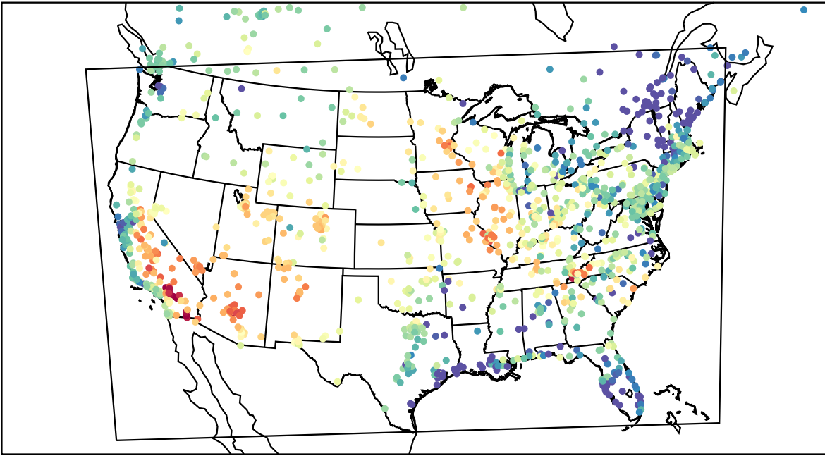
AirNOW (2023-06-18_01:00:00)
