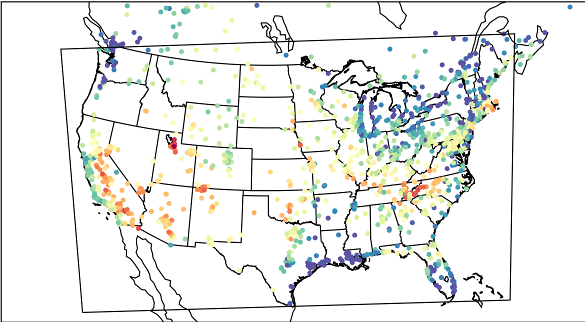
AirNOW (2023-06-17_01:00:00)
