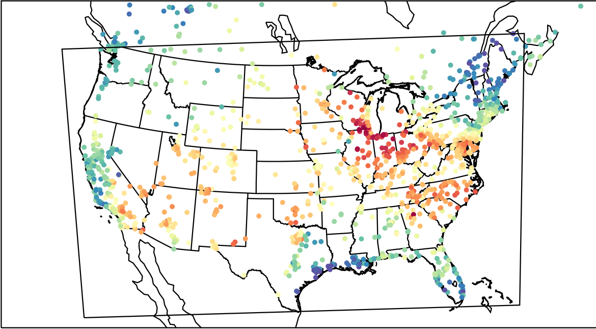
AirNOW (2023-06-18_19:00:00)
