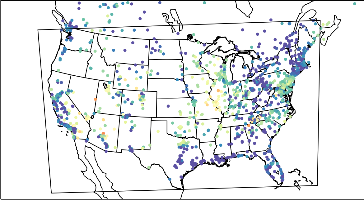
AirNOW (2023-06-18_12:00:00)
