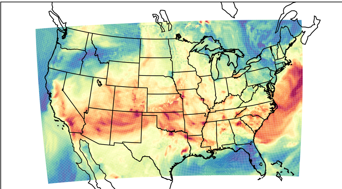
WRF (2023-06-17_23:00:00)
