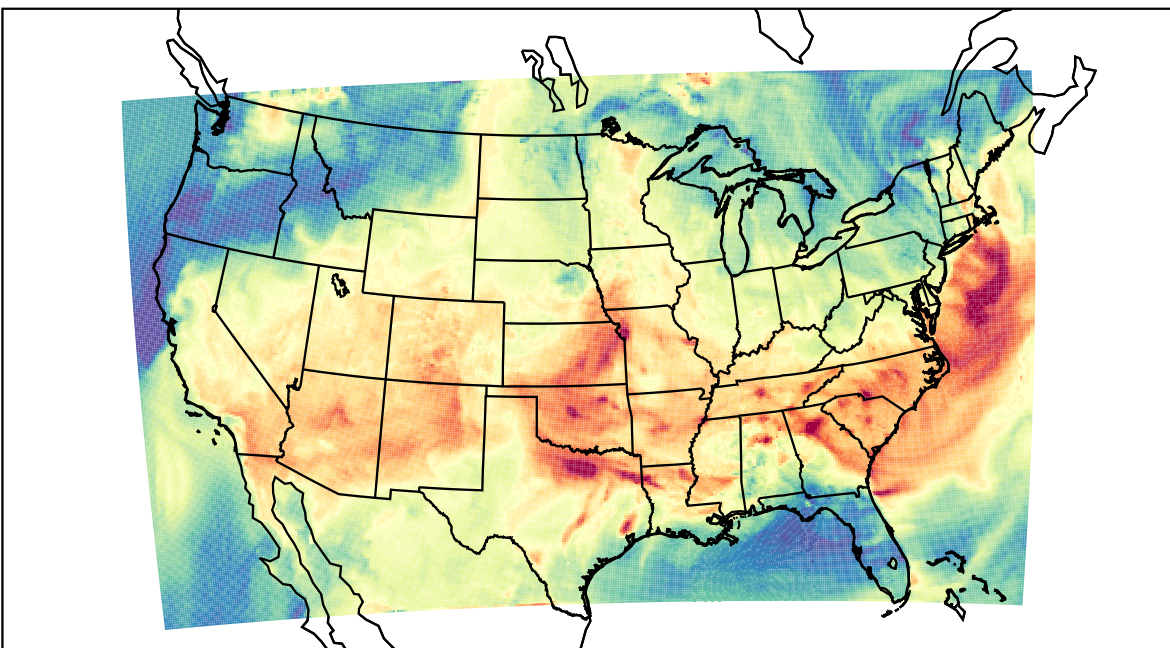
WRF (2023-06-17_18:00:00)
