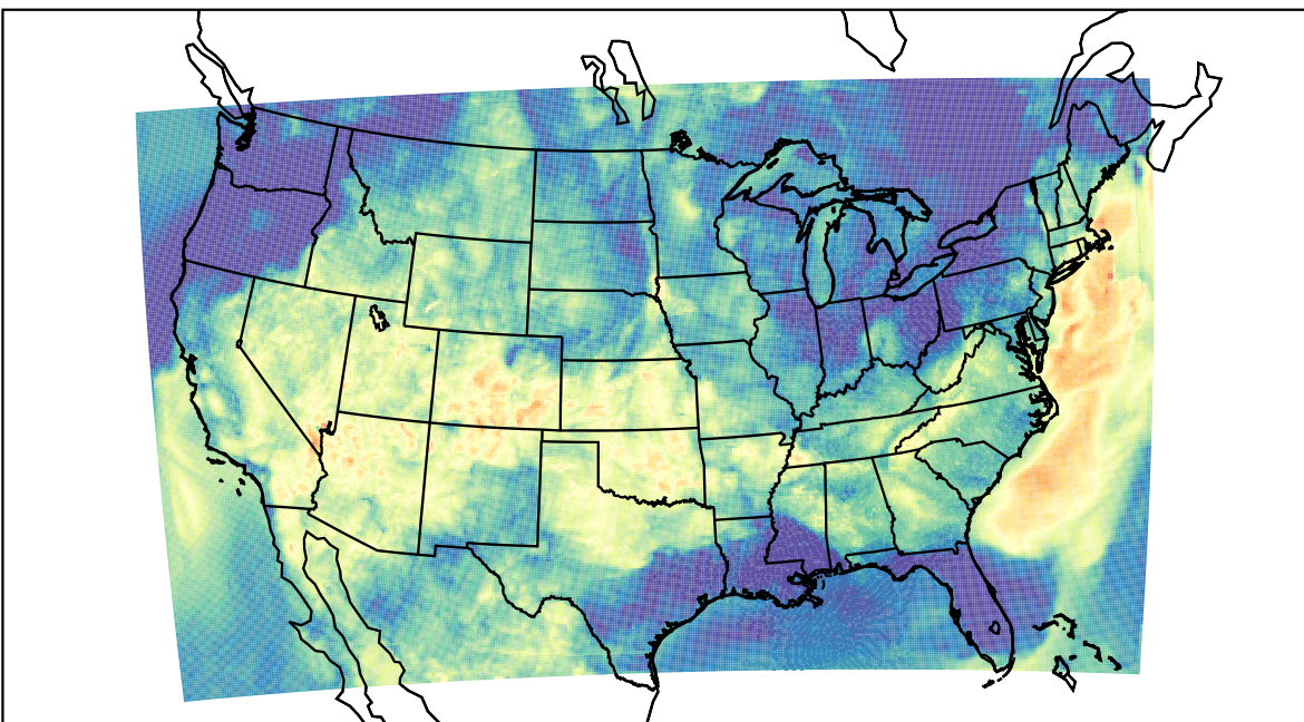
WRF (2023-06-17_08:00:00)
