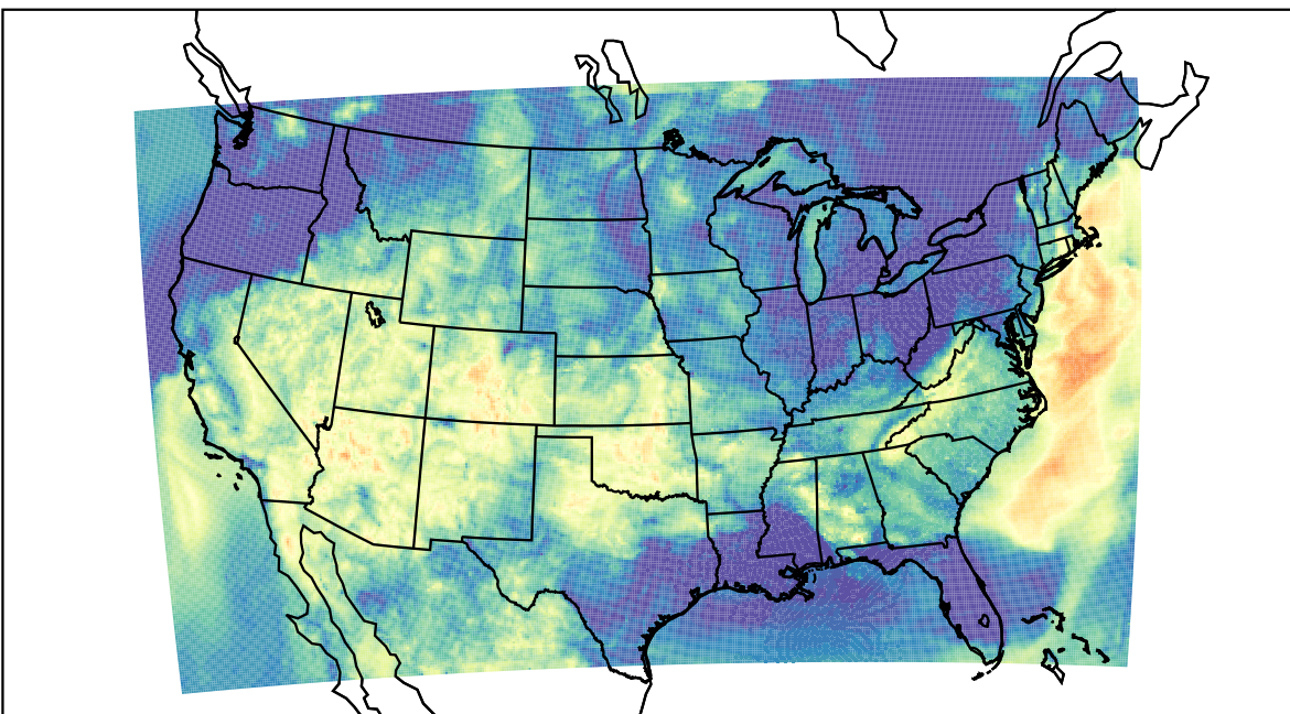
WRF (2023-06-17_11:00:00)
