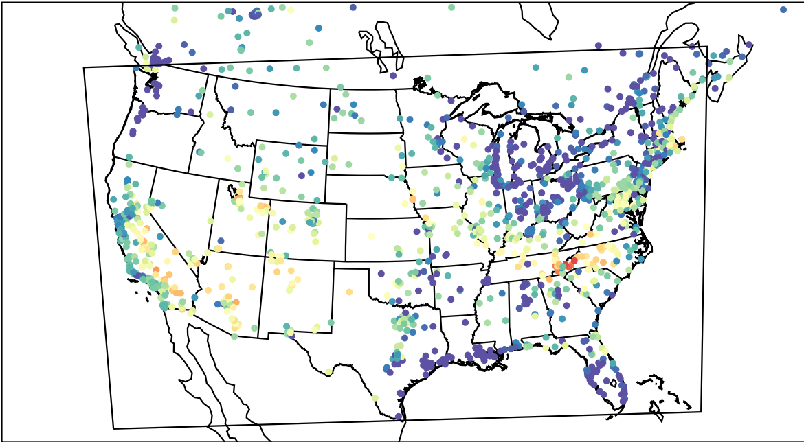
AirNOW (2023-06-17_04:00:00)
