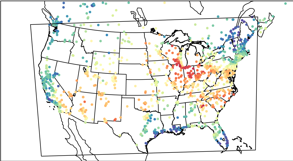
AirNOW (2023-06-18_17:00:00)
