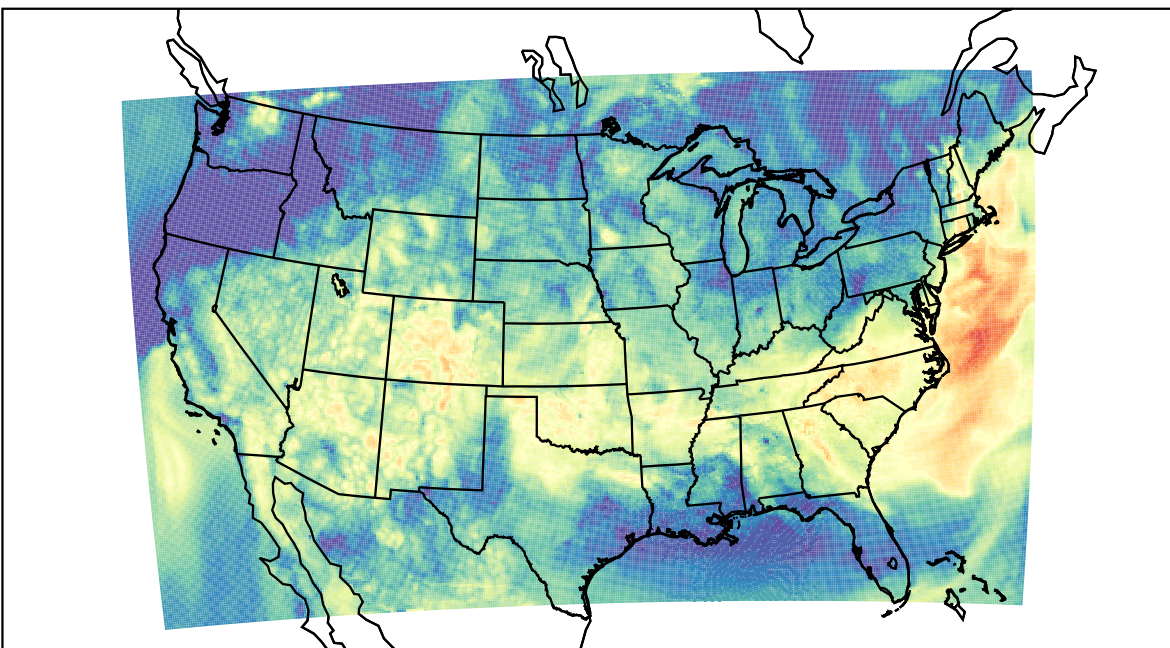
WRF (2023-06-17_14:00:00)
