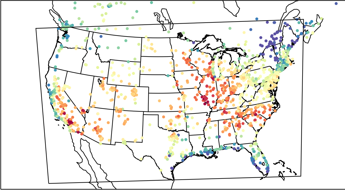
AirNOW (2023-06-17_21:00:00)
