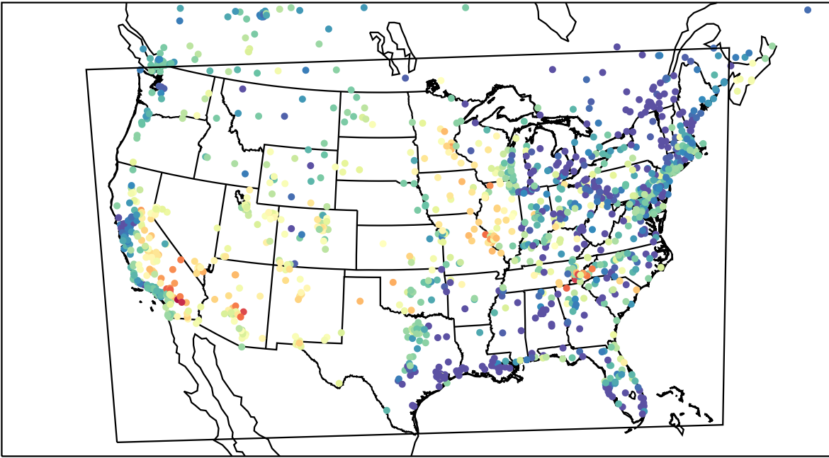
AirNOW (2023-06-18_03:00:00)
