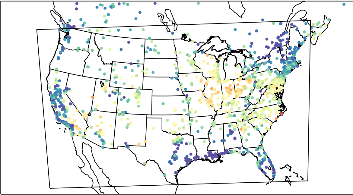
AirNOW (2023-06-18_14:00:00)
