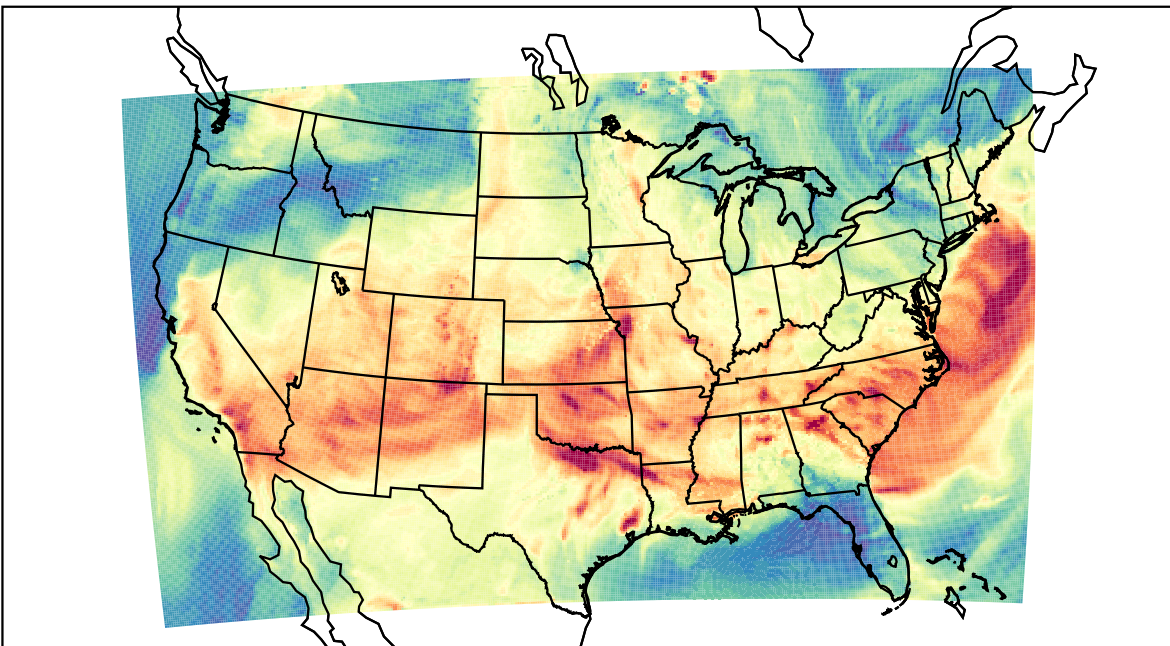
WRF (2023-06-17_21:00:00)
