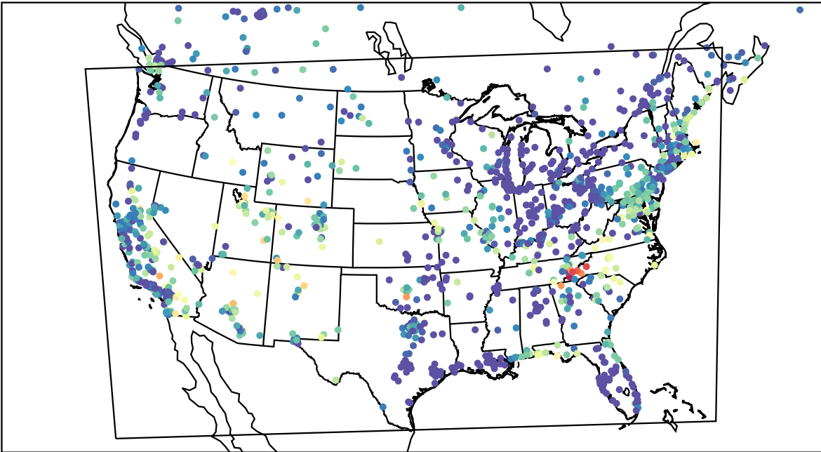
AirNOW (2023-06-17_08:00:00)
