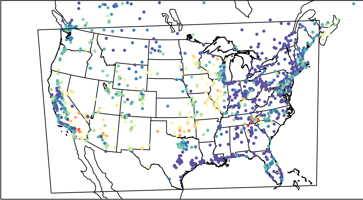
AirNOW (2023-06-18_07:00:00)
