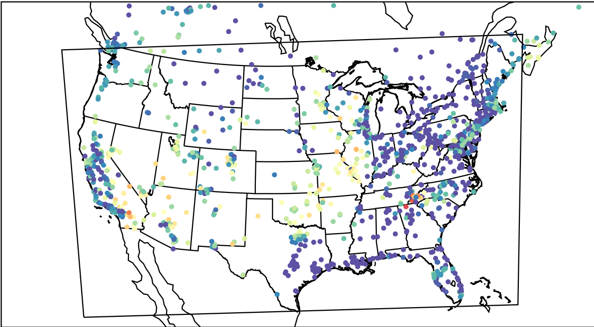
AirNOW (2023-06-18_09:00:00)
