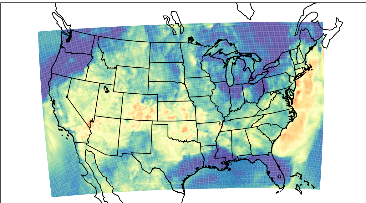
WRF (2023-06-17_06:00:00)
