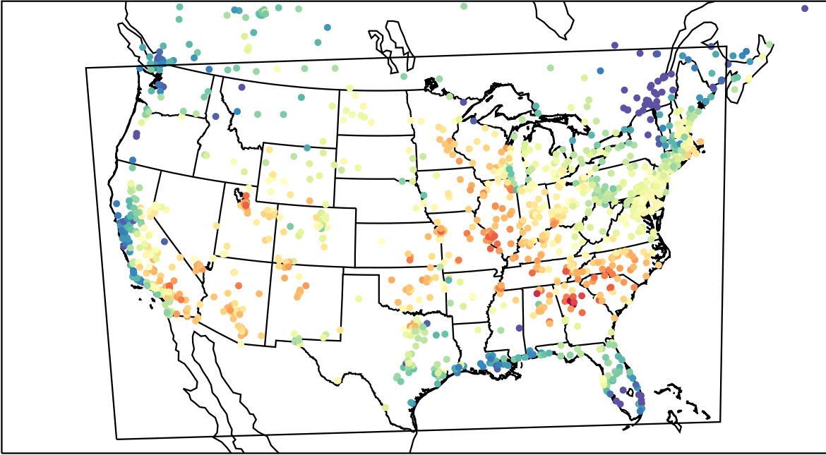
AirNOW (2023-06-17_17:00:00)
