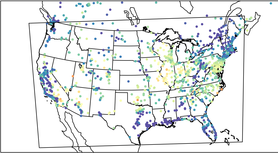
AirNOW (2023-06-18_13:00:00)
