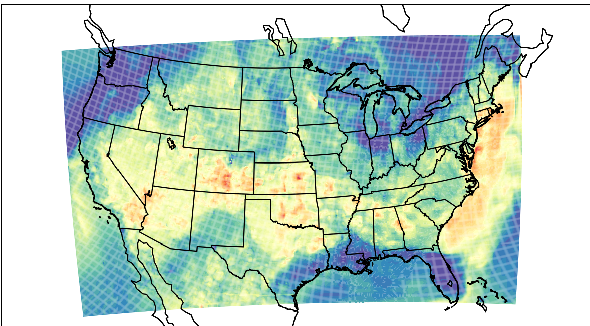
WRF (2023-06-17_04:00:00)
