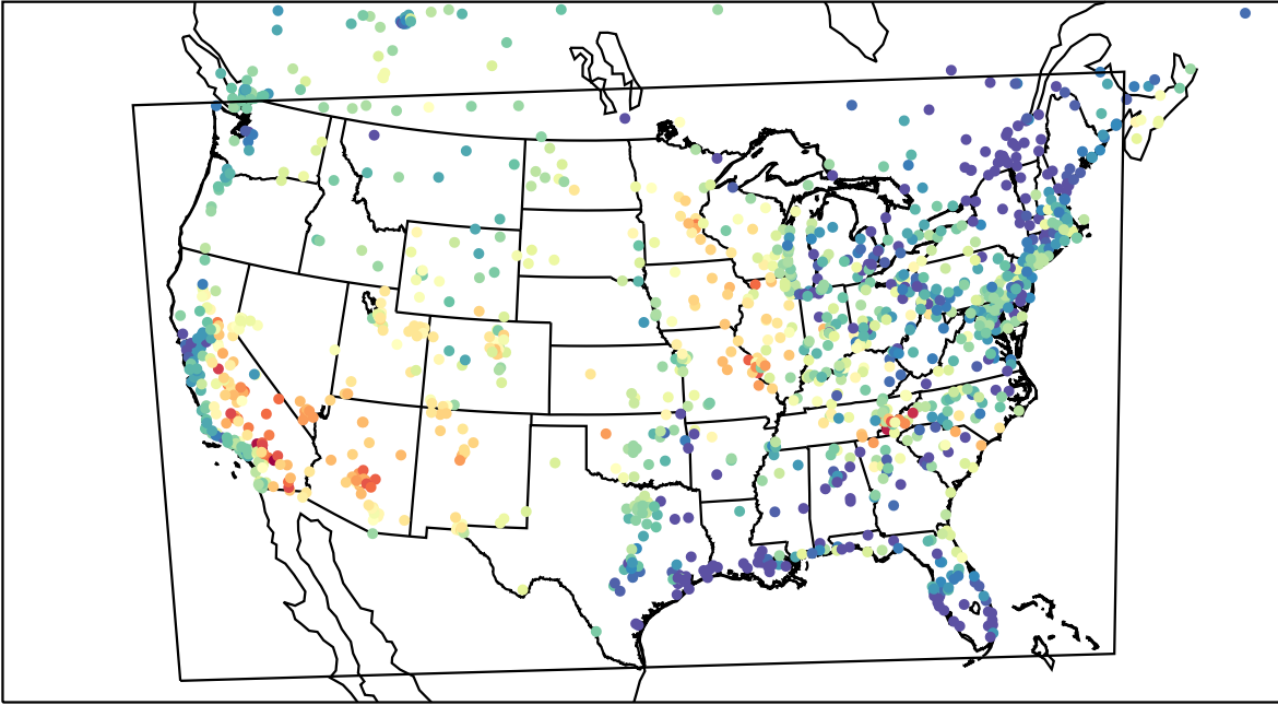
AirNOW (2023-06-18_02:00:00)
