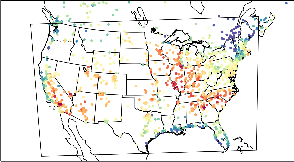
AirNOW (2023-06-17_20:00:00)
