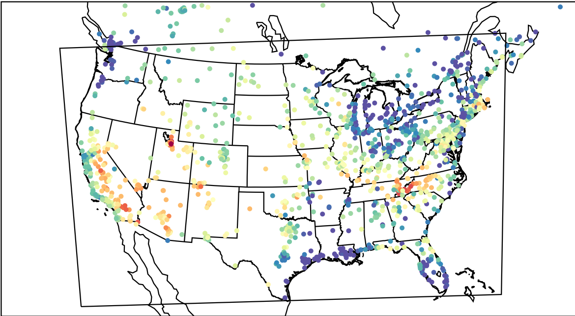
AirNOW (2023-06-17_02:00:00)
