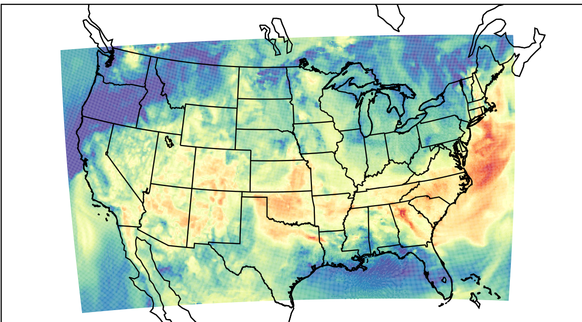
WRF (2023-06-17_15:00:00)
