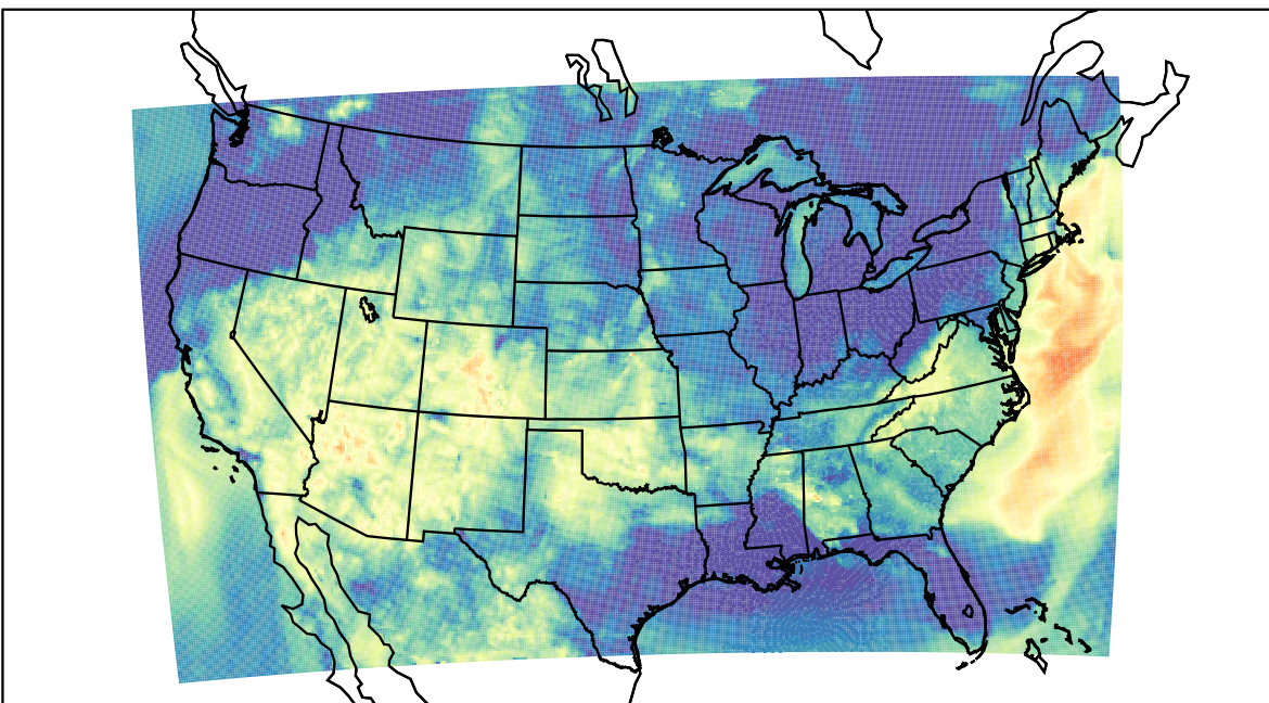
WRF (2023-06-17_12:00:00)
