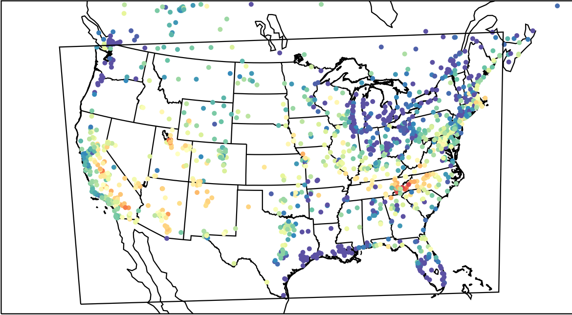
AirNOW (2023-06-17_03:00:00)
