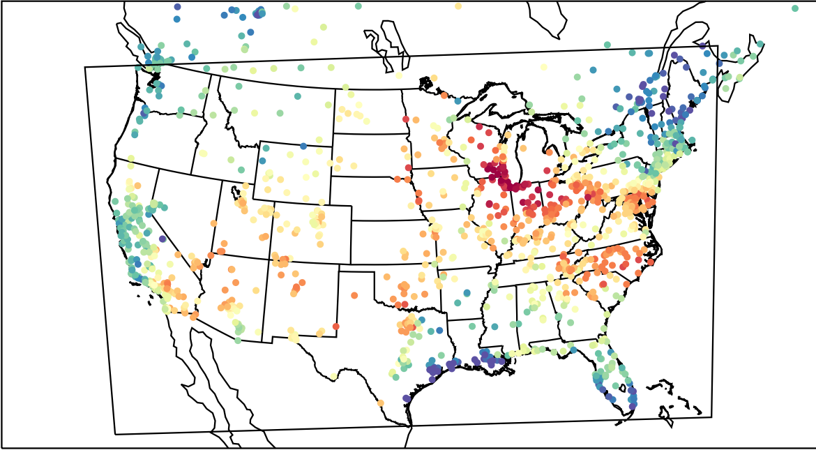
AirNOW (2023-06-18_21:00:00)
