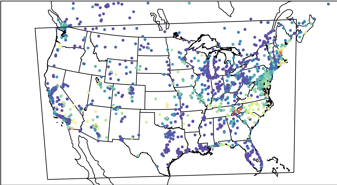
AirNOW (2023-06-17_12:00:00)
