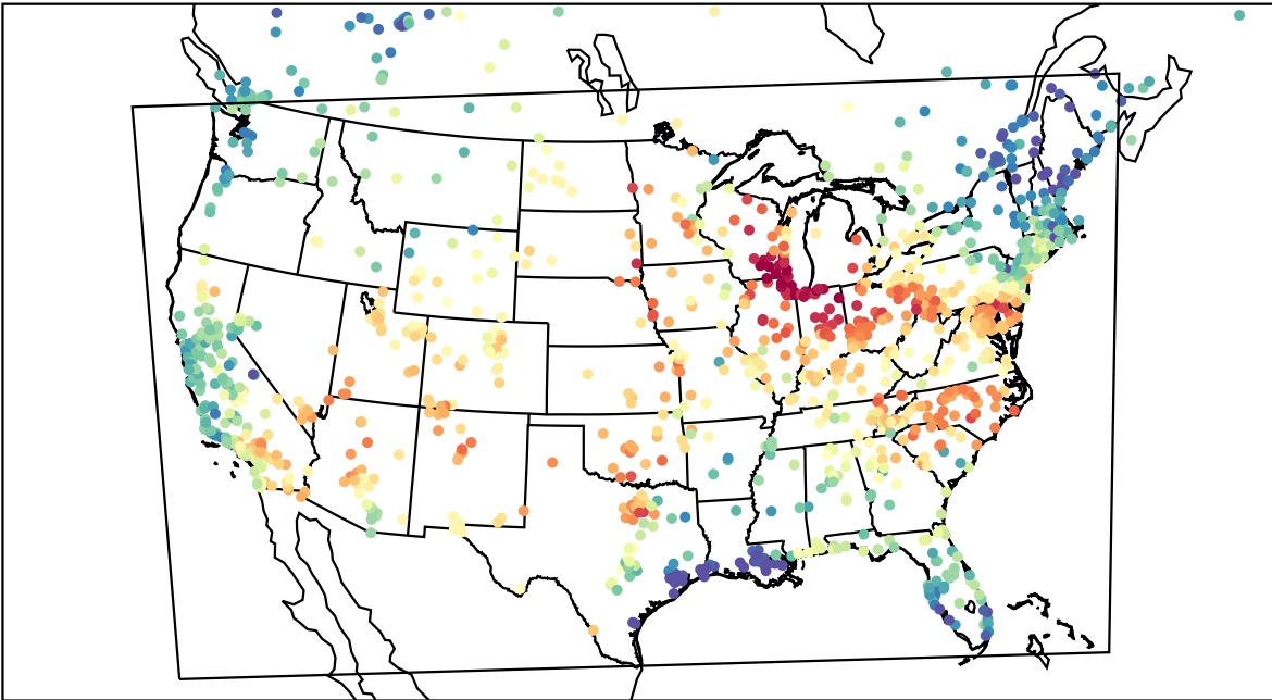
AirNOW (2023-06-18_22:00:00)
