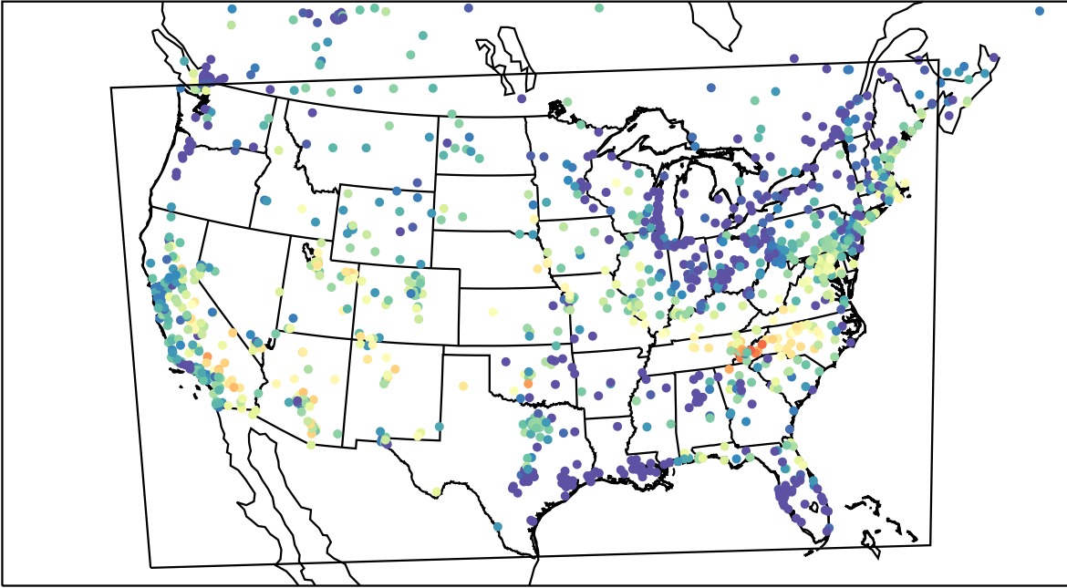
AirNOW (2023-06-17_05:00:00)
