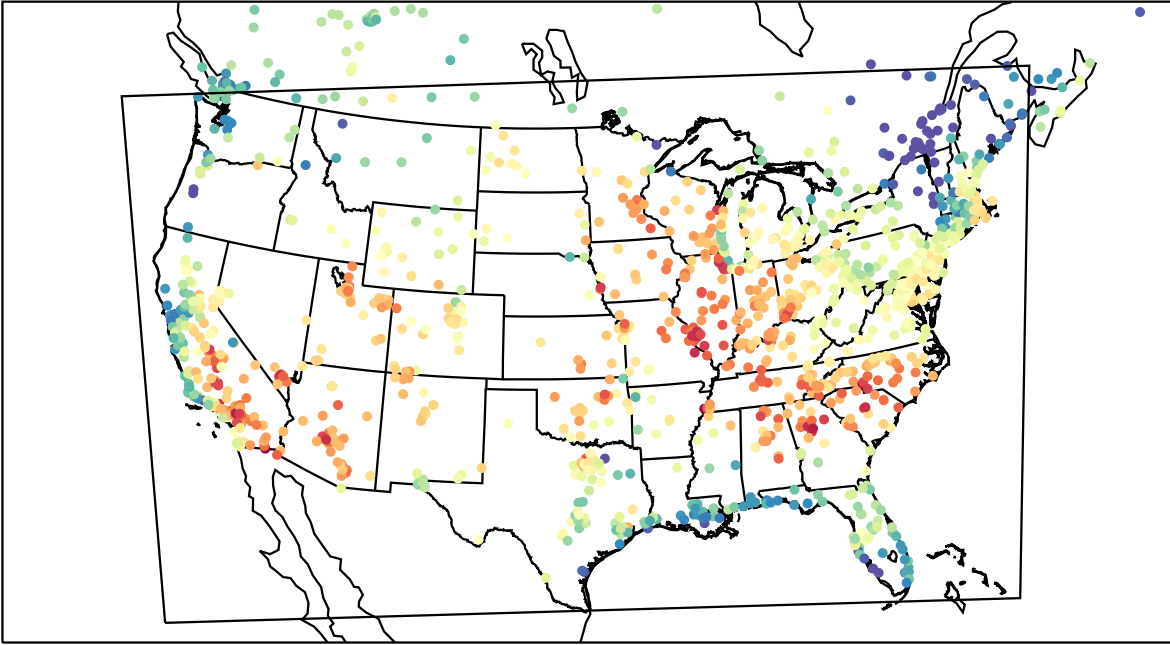
AirNOW (2023-06-17_19:00:00)
