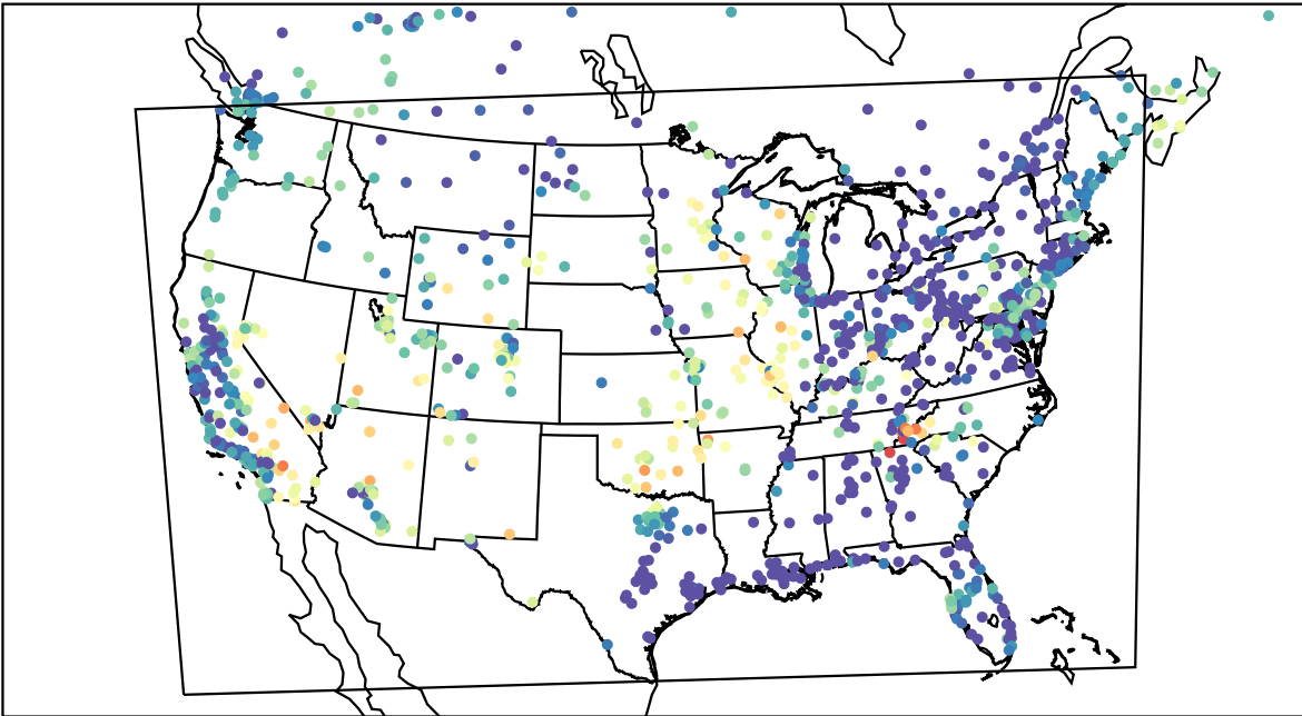
AirNOW (2023-06-18_08:00:00)
