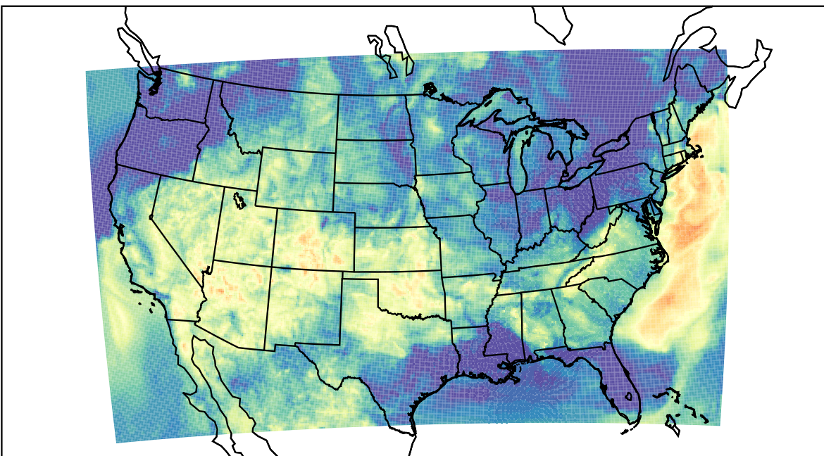
WRF (2023-06-17_10:00:00)
