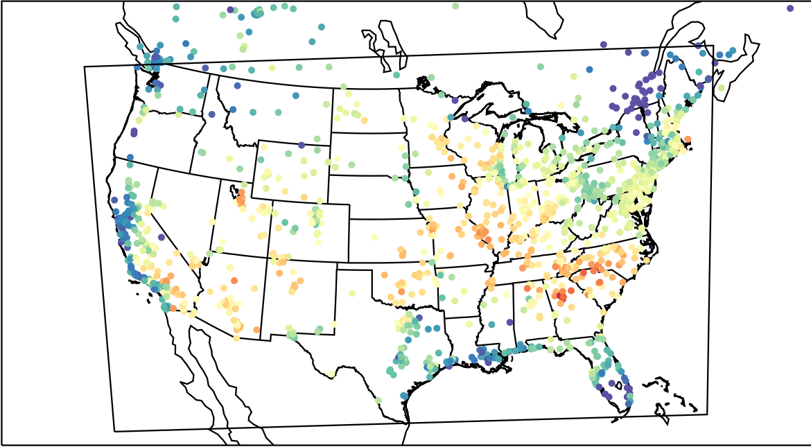
AirNOW (2023-06-17_16:00:00)
