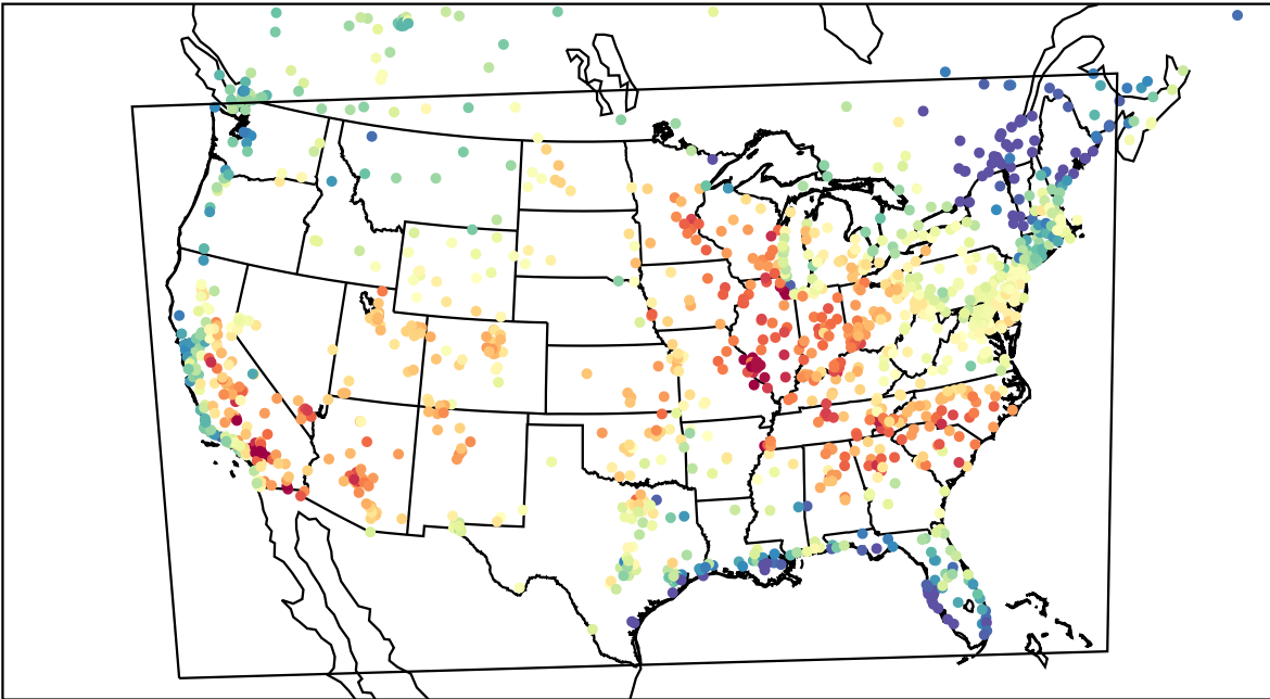
AirNOW (2023-06-17_22:00:00)
