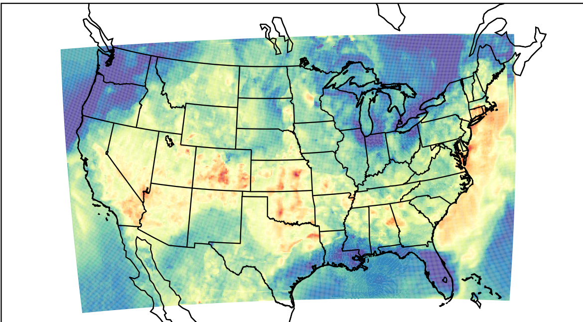
WRF (2023-06-17_03:00:00)
