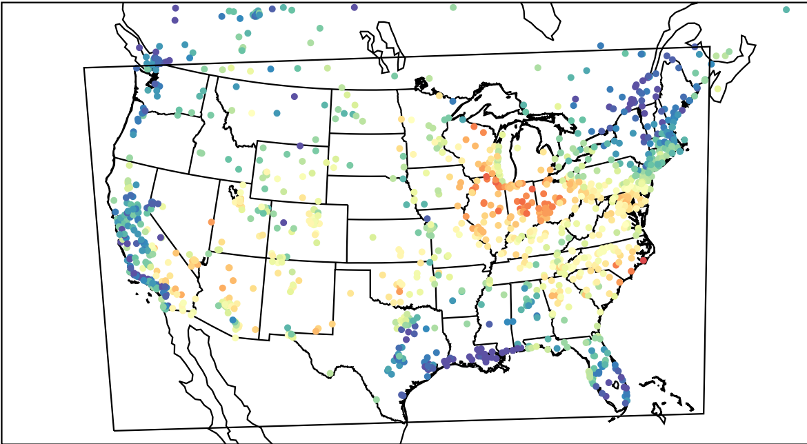
AirNOW (2023-06-18_15:00:00)
