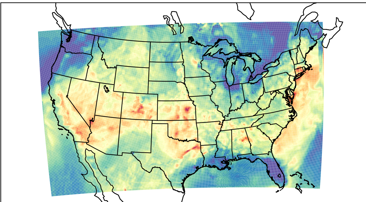
WRF (2023-06-17_02:00:00)
