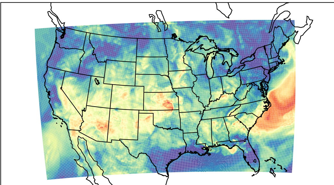
WRF (2023-06-18_08:00:00)
