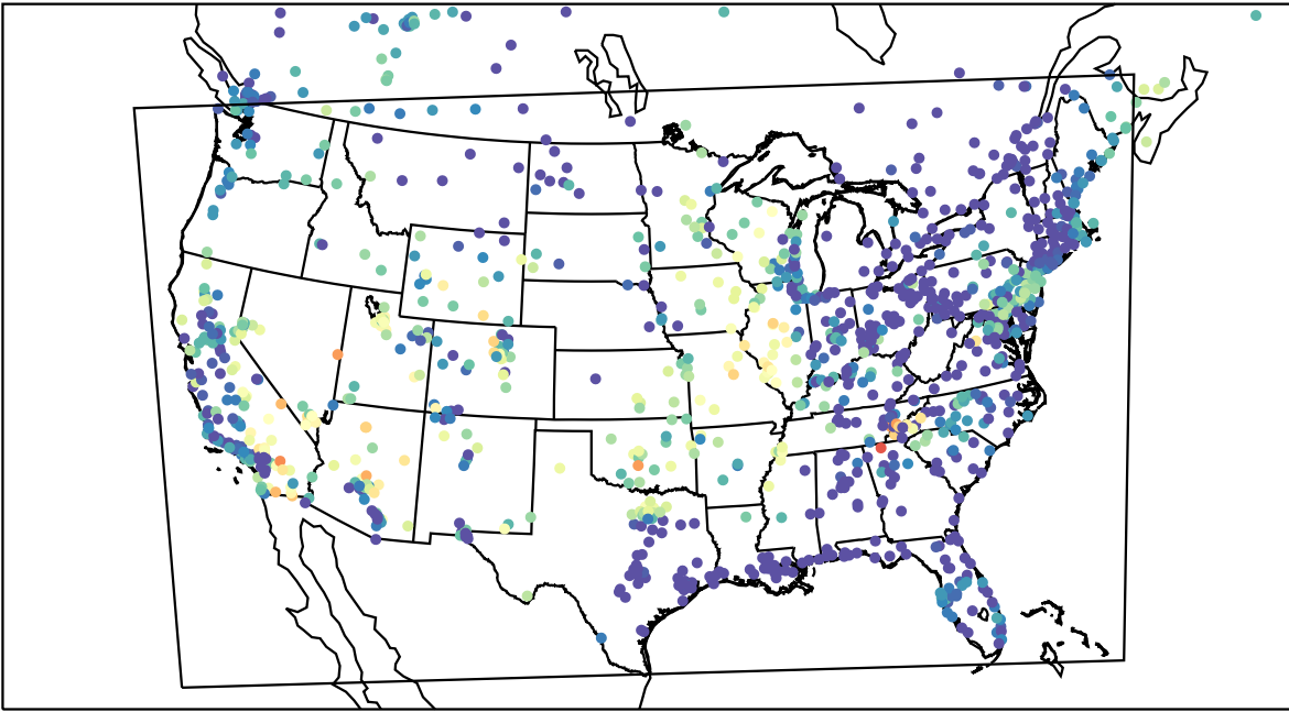
AirNOW (2023-06-18_11:00:00)
