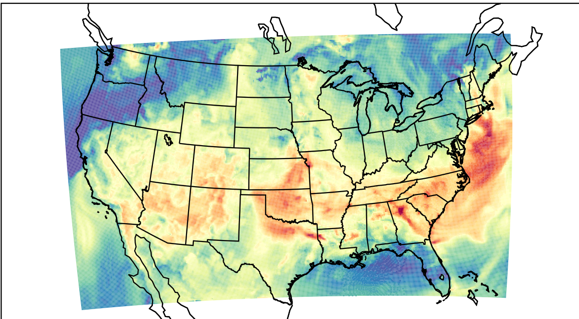
WRF (2023-06-17_16:00:00)
