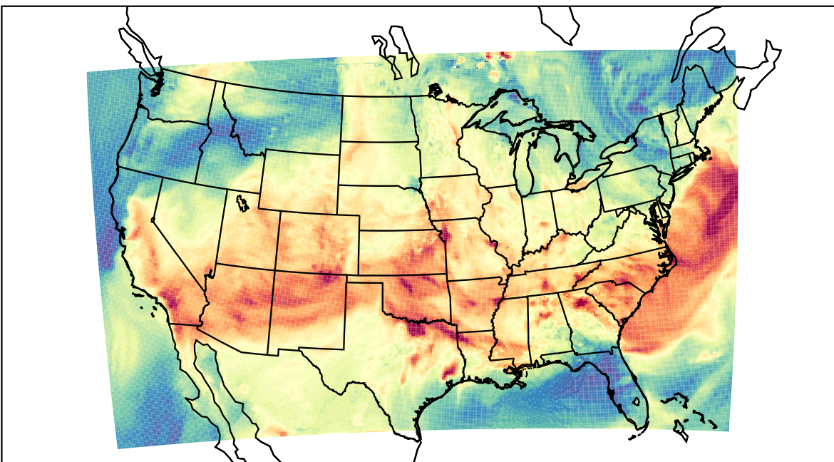
WRF (2023-06-17_22:00:00)
