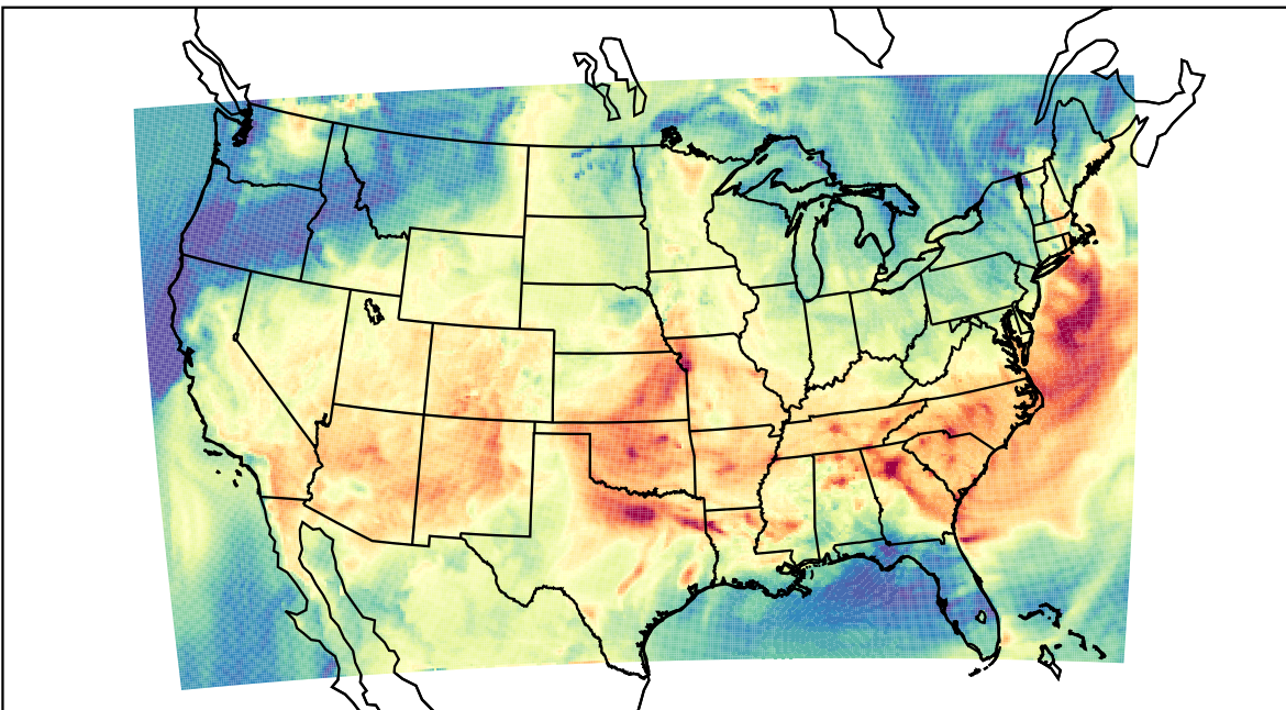
WRF (2023-06-17_17:00:00)
