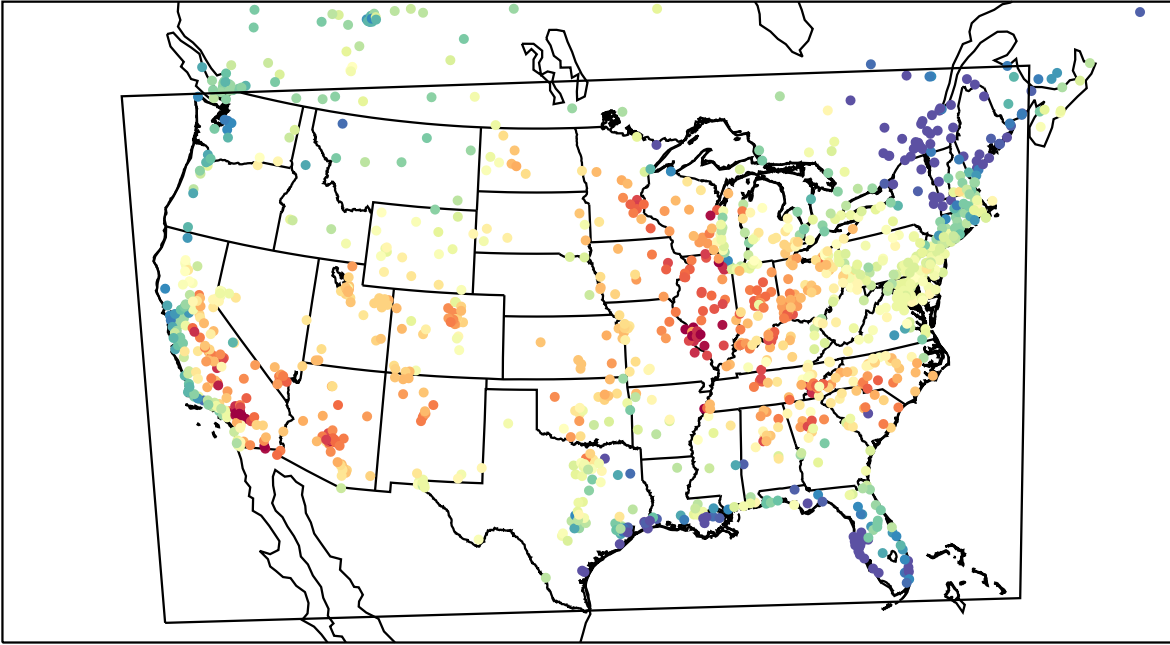
AirNOW (2023-06-17_23:00:00)
