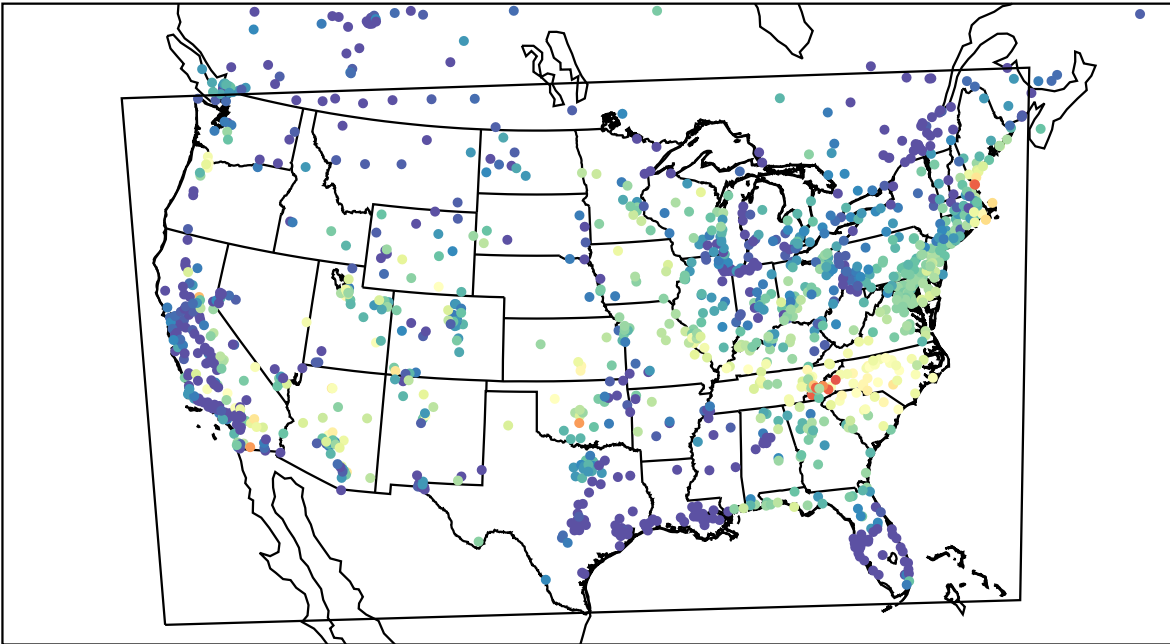
AirNOW (2023-06-17_13:00:00)
