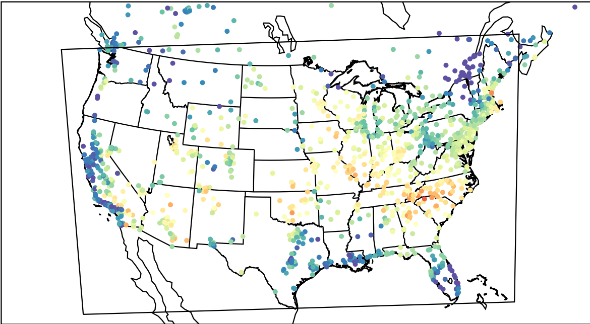
AirNOW (2023-06-17_15:00:00)
