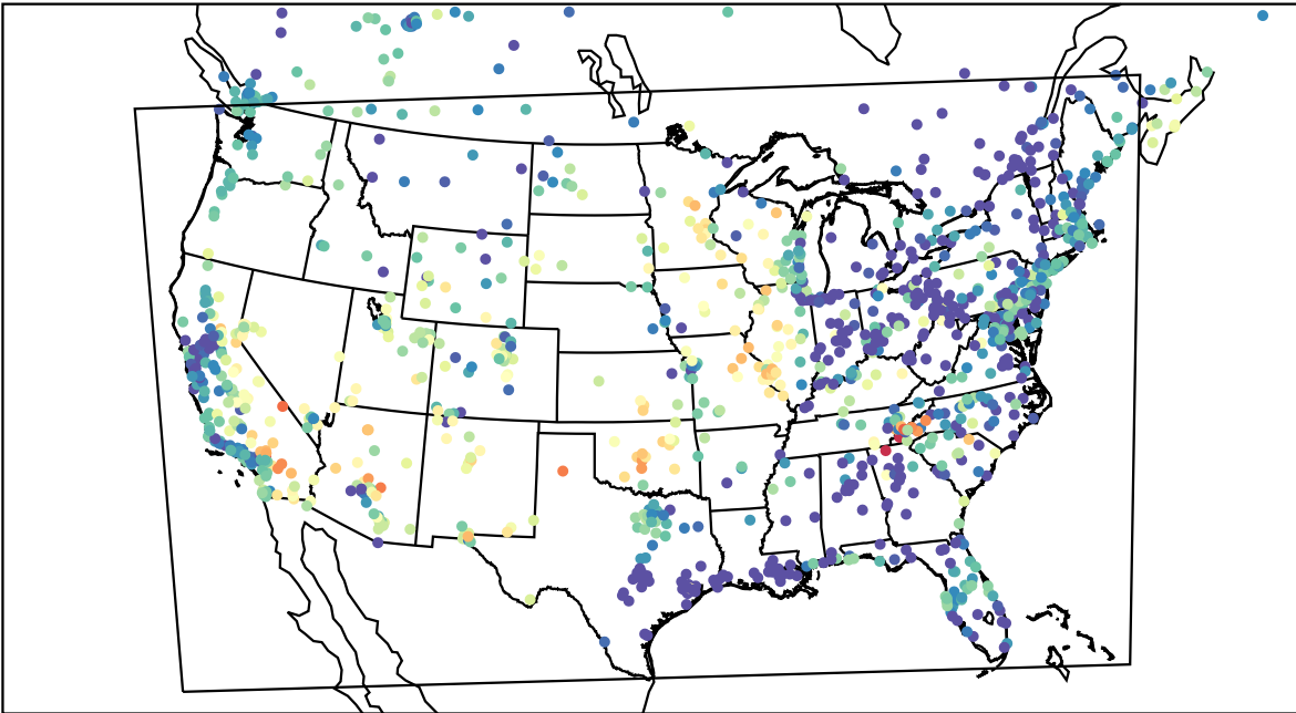
AirNOW (2023-06-18_05:00:00)
