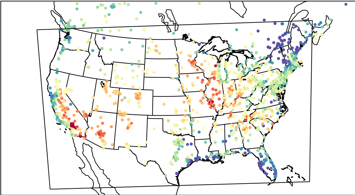
AirNOW (2023-06-18_00:00:00)
