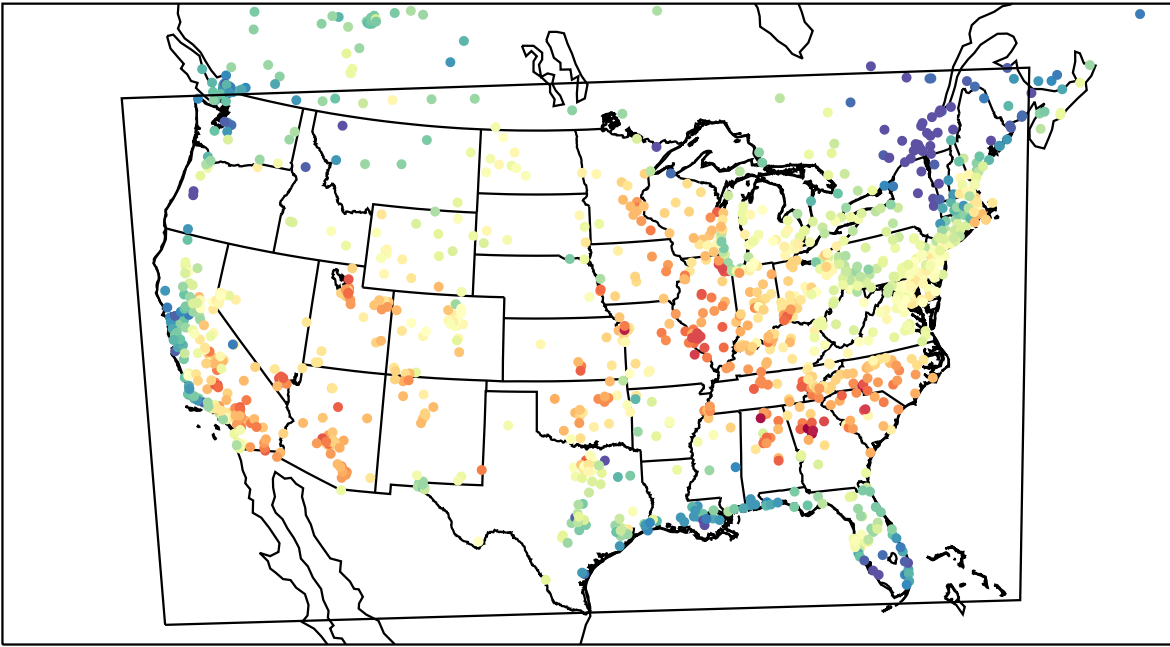
AirNOW (2023-06-17_18:00:00)
