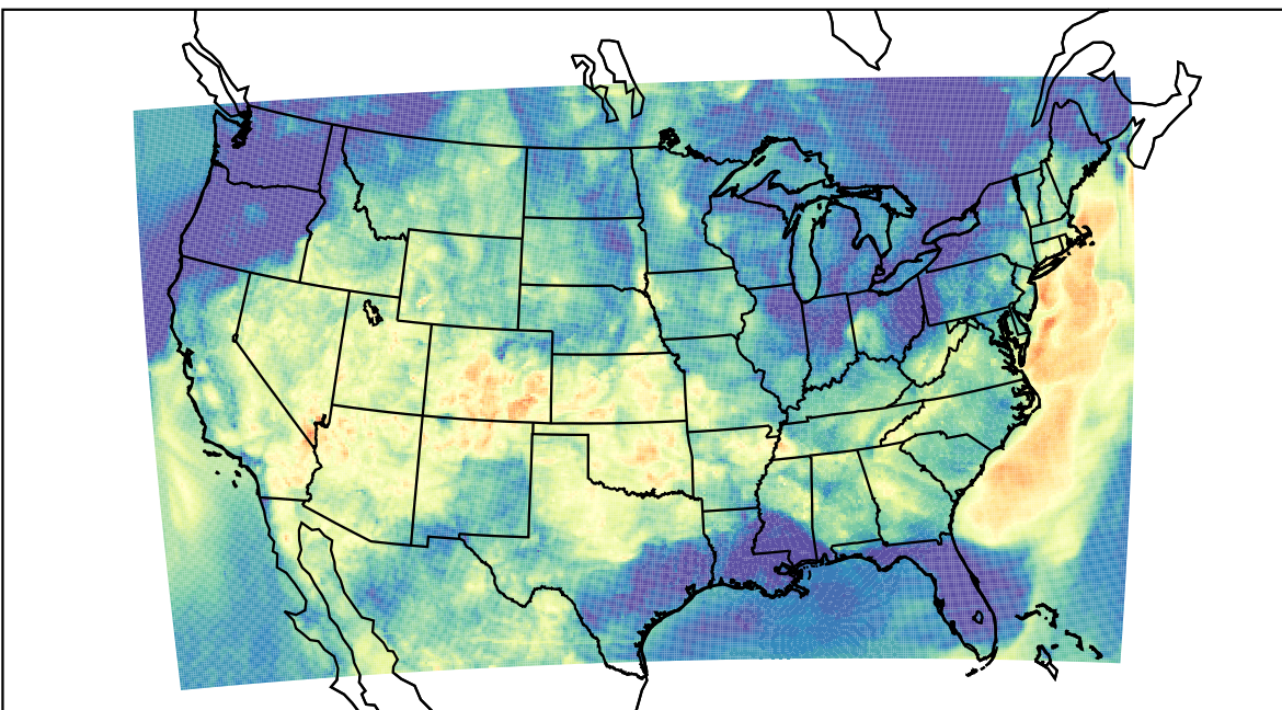
WRF (2023-06-17_07:00:00)
