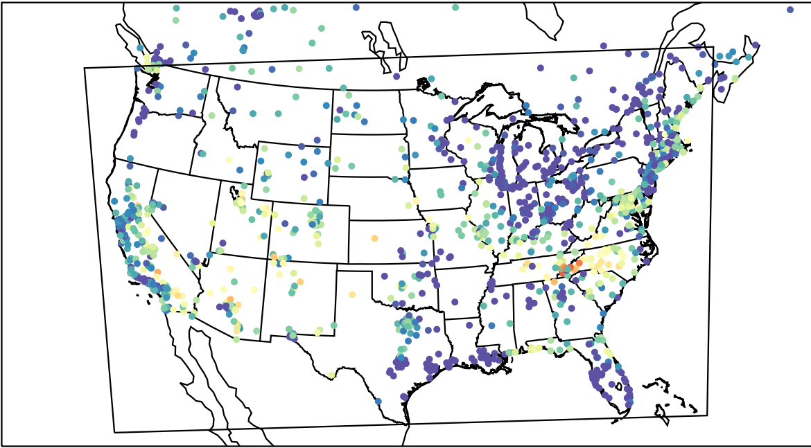
AirNOW (2023-06-17_06:00:00)
