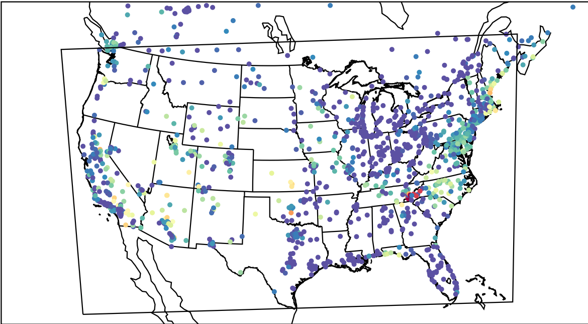
AirNOW (2023-06-17_11:00:00)
