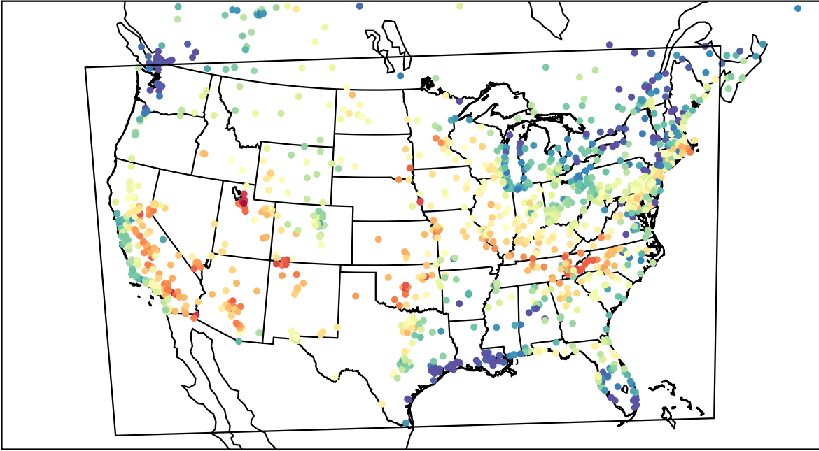
AirNOW (2023-06-17_00:00:00)
