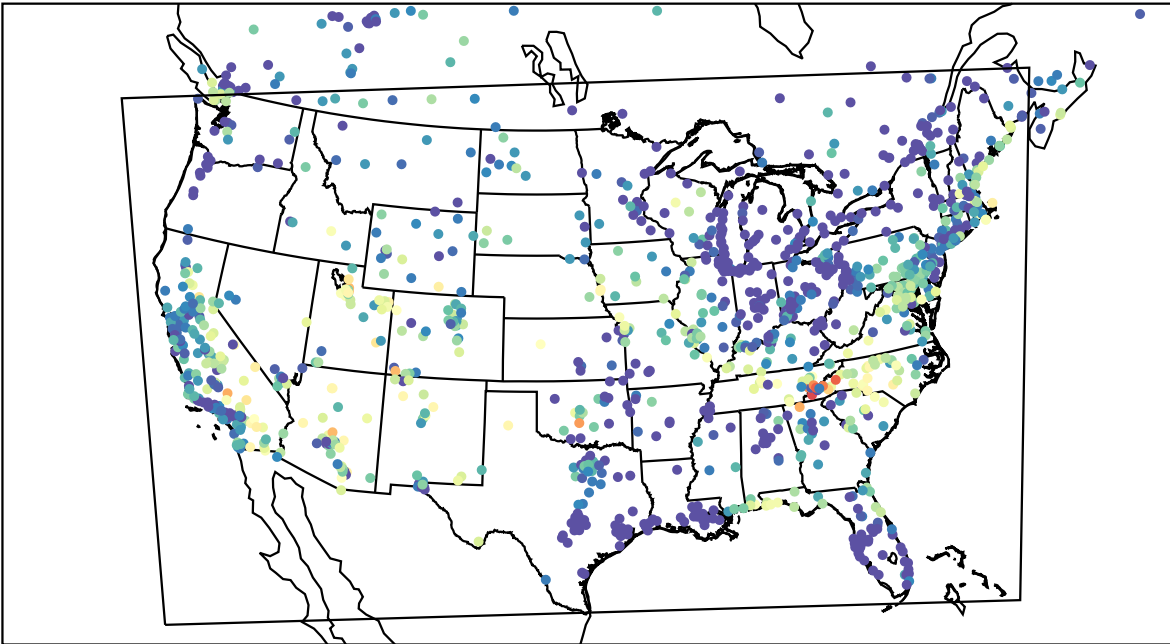
AirNOW (2023-06-17_07:00:00)
