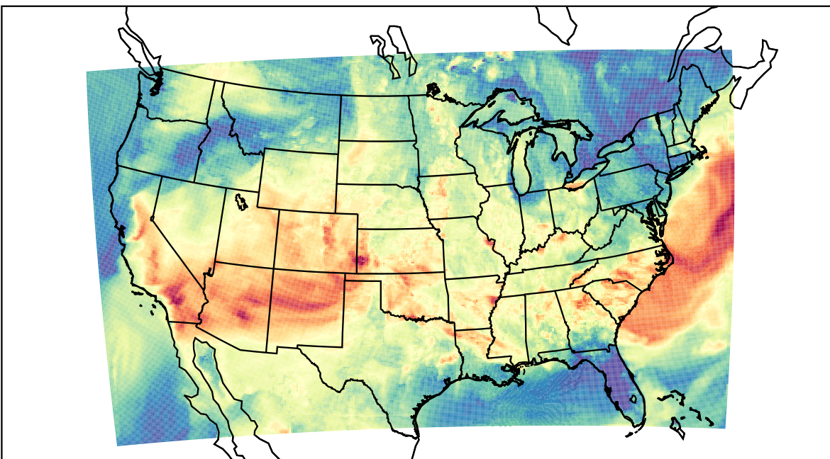
WRF (2023-06-18_01:00:00)
