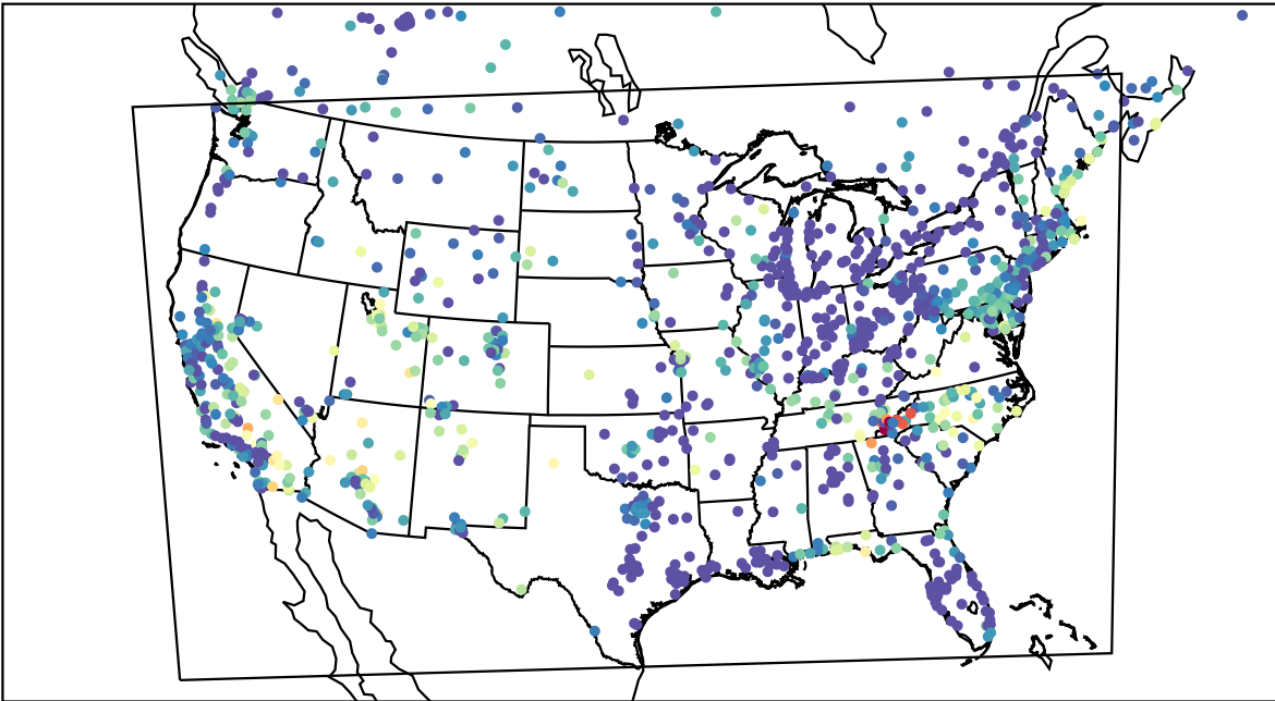
AirNOW (2023-06-17_09:00:00)
