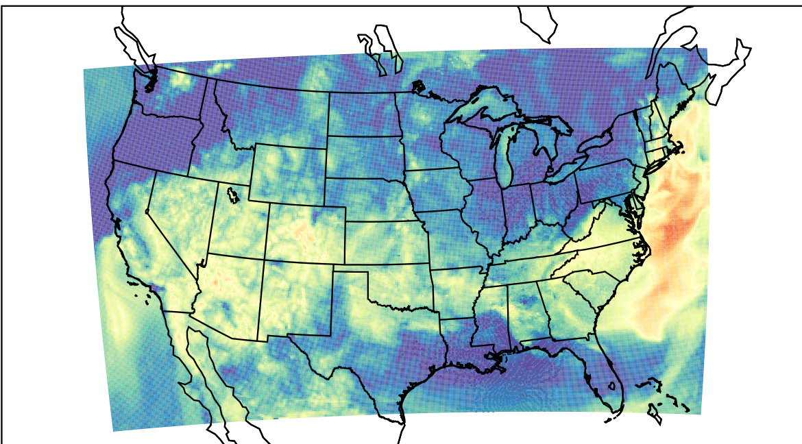
WRF (2023-06-17_13:00:00)
