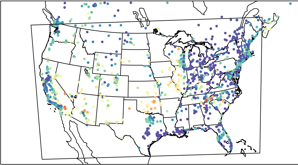
AirNOW (2023-06-18_06:00:00)
