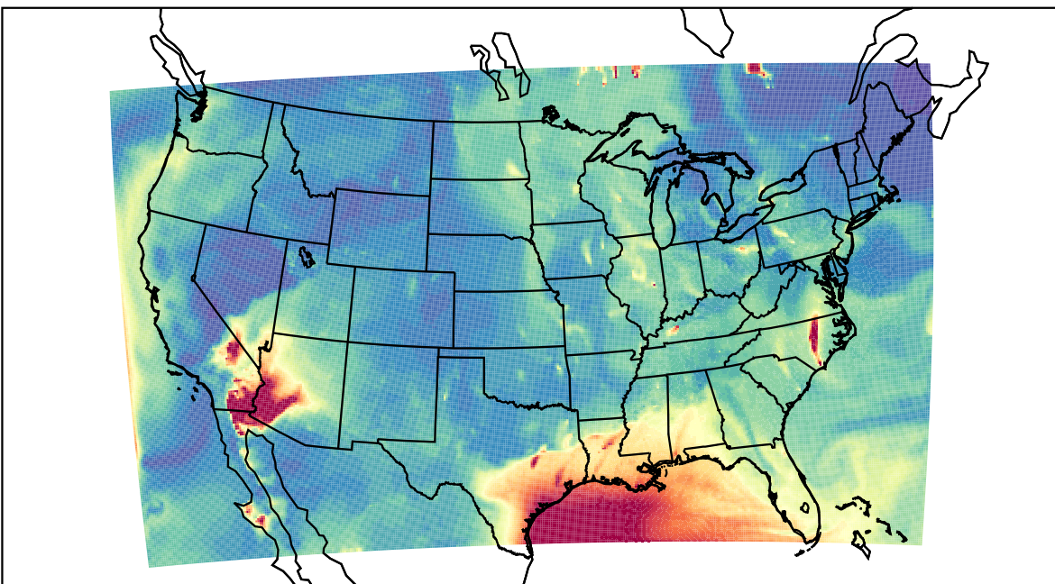
WRF 2023-06-19_07:00:00
