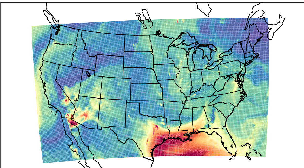
WRF 2023-06-19_15:00:00
