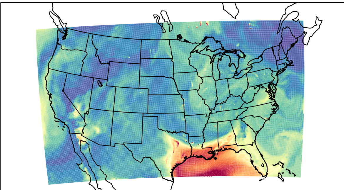
WRF 2023-06-19_18:00:00
