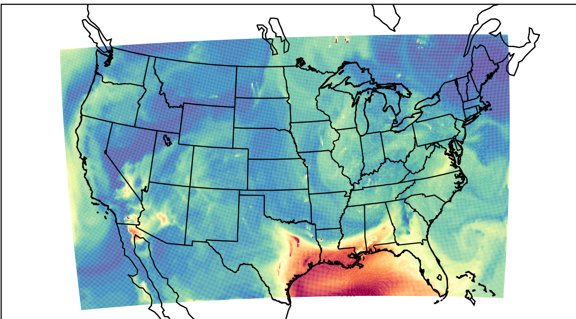
WRF 2023-06-19_17:00:00
