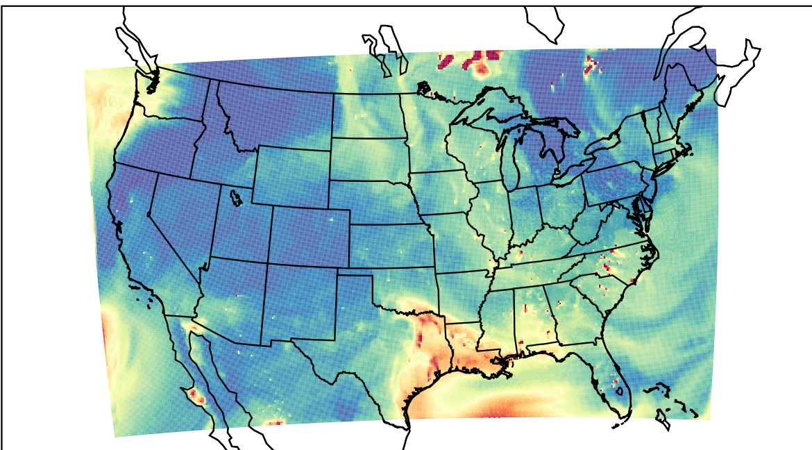
WRF 2023-06-18_00:00:00
