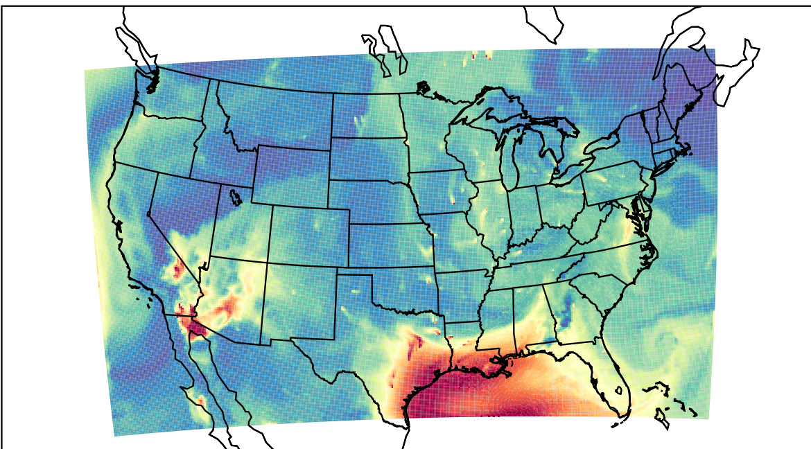
WRF 2023-06-19_14:00:00
