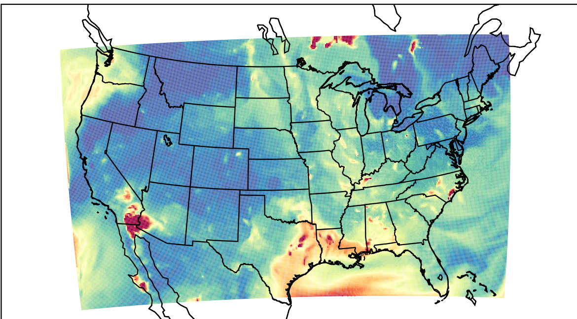
WRF 2023-06-18_05:00:00
