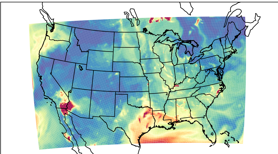
WRF 2023-06-18_07:00:00
