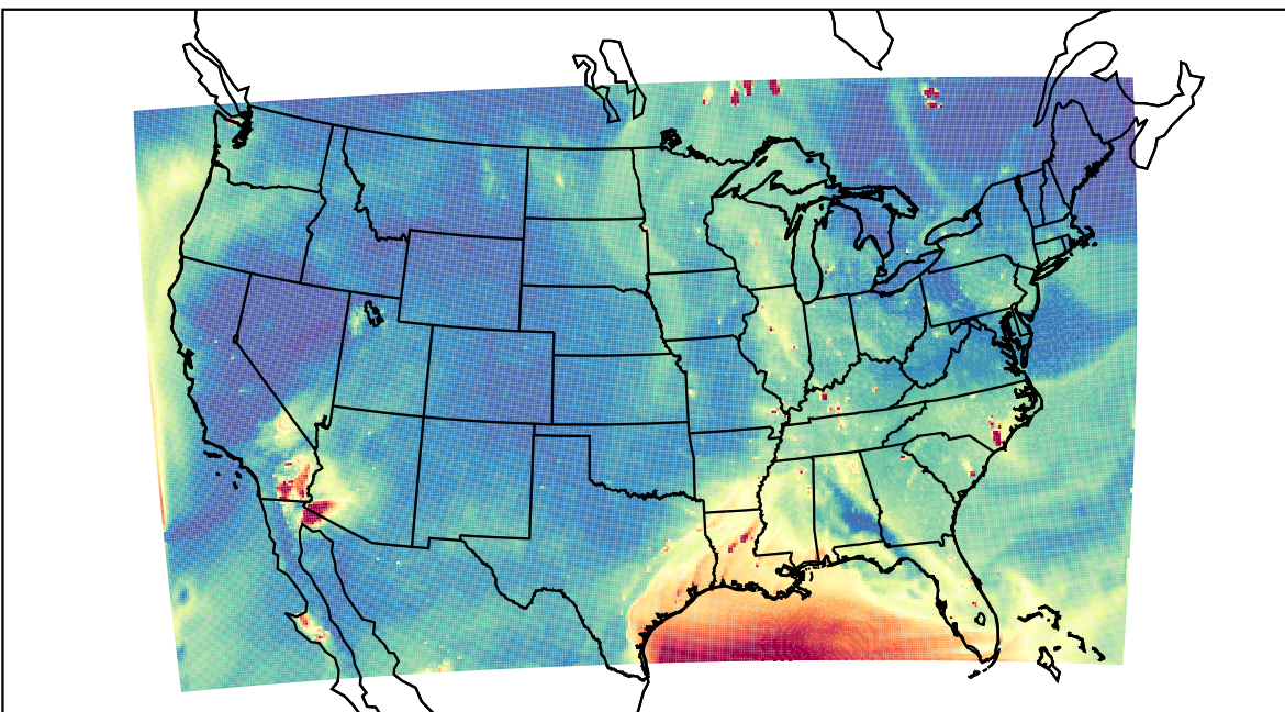
WRF 2023-06-19_00:00:00
