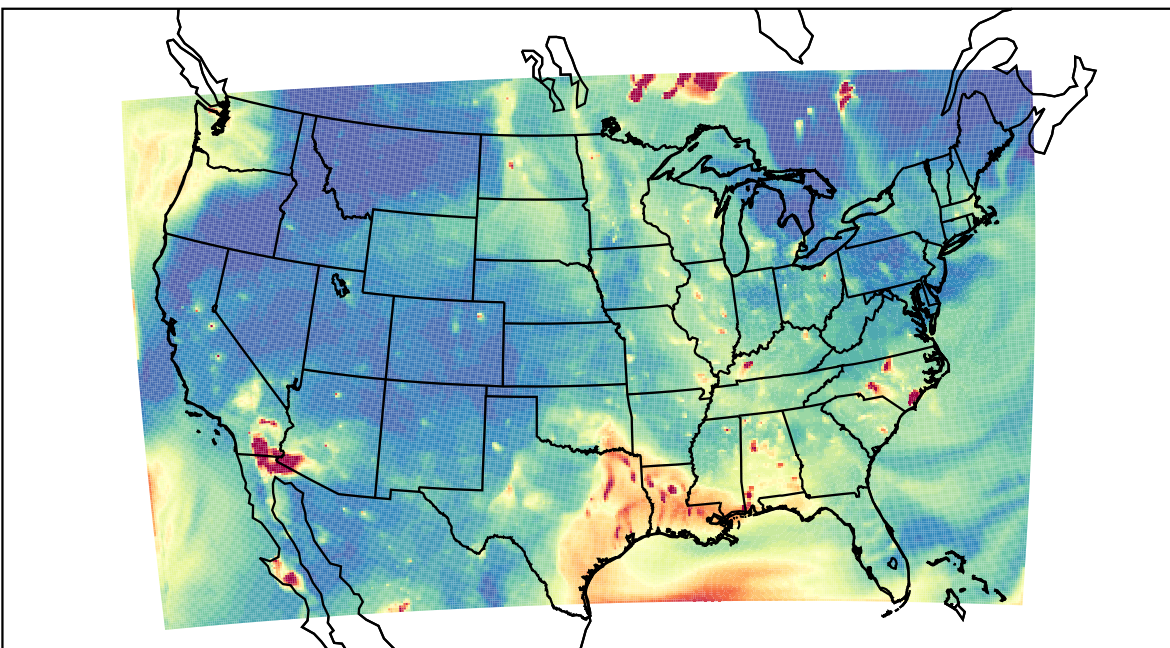
WRF 2023-06-18_03:00:00
