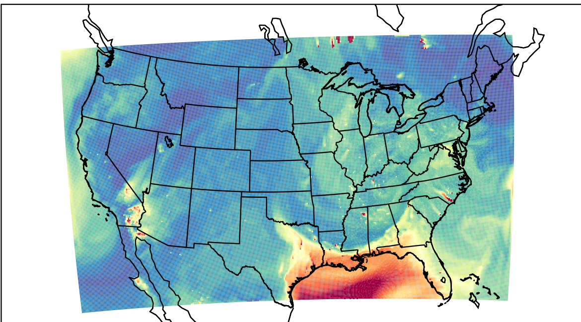
WRF 2023-06-19_23:00:00
