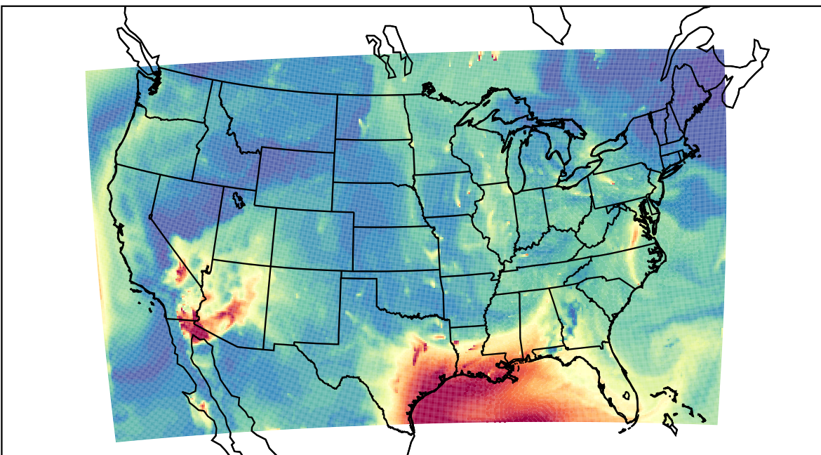
WRF 2023-06-19_13:00:00
