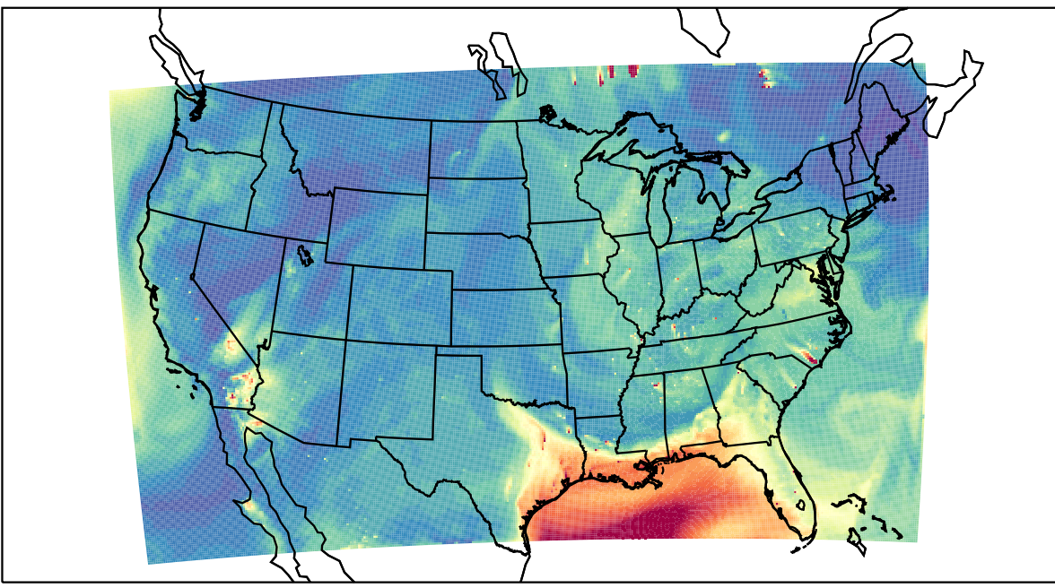
WRF 2023-06-19_22:00:00
