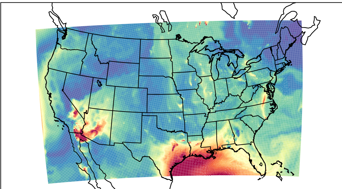
WRF 2023-06-19_12:00:00
