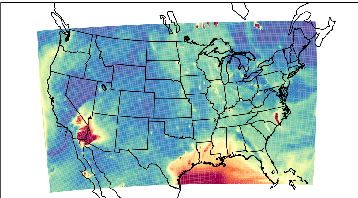
WRF 2023-06-19_04:00:00
