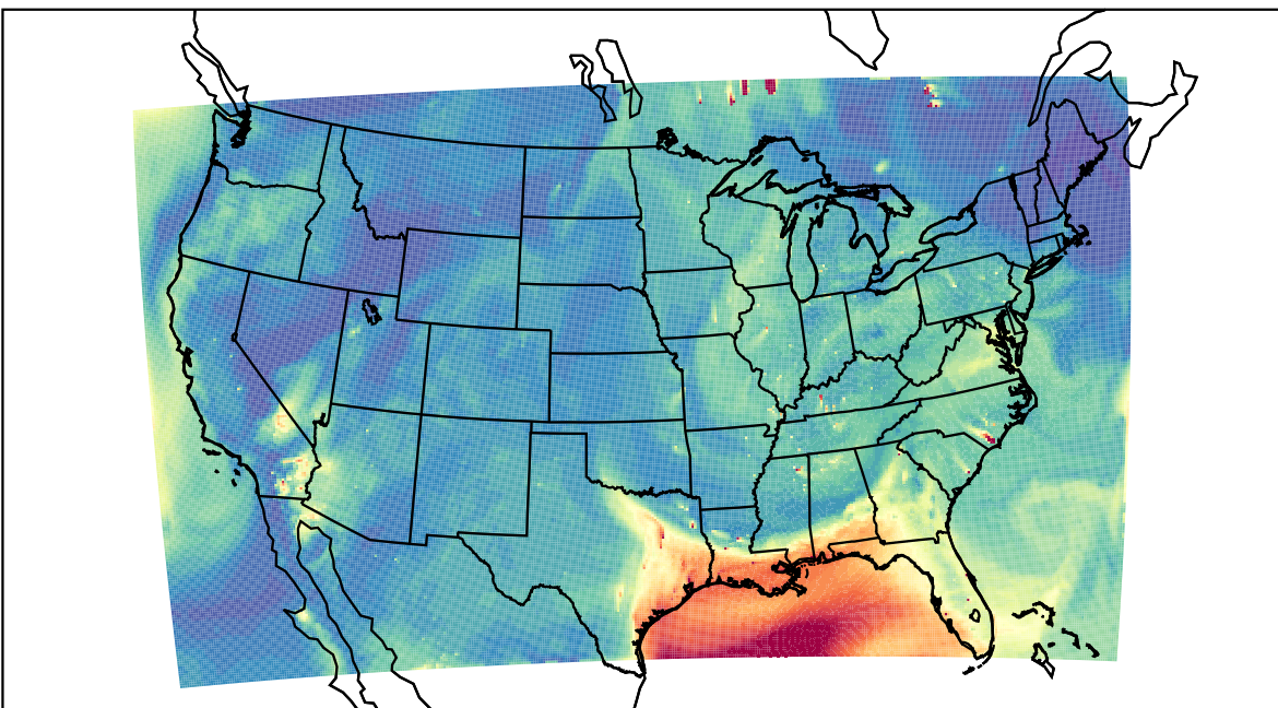
WRF 2023-06-19_21:00:00
