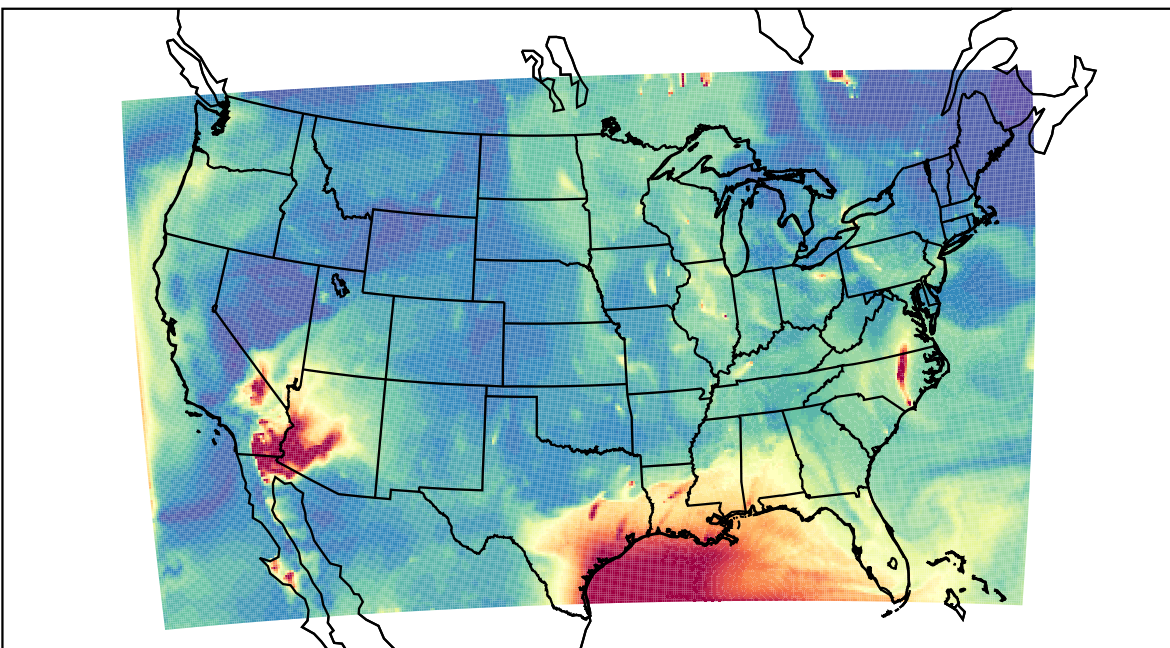
WRF 2023-06-19_08:00:00
