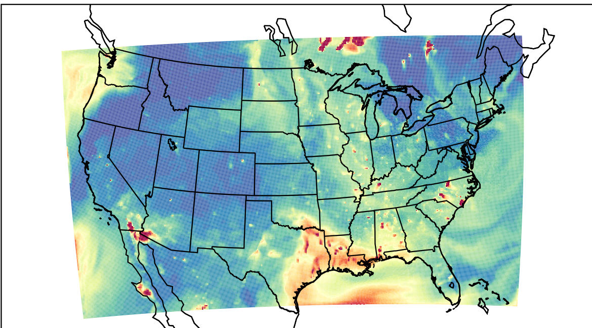
WRF 2023-06-18_02:00:00
