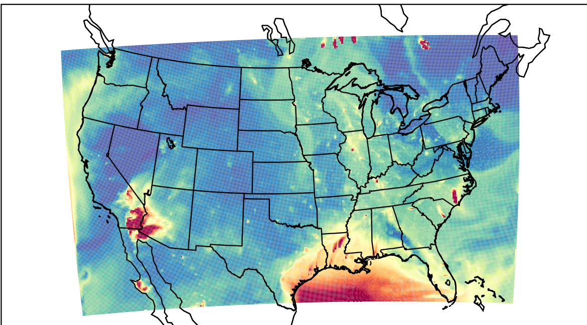
WRF 2023-06-19_02:00:00
