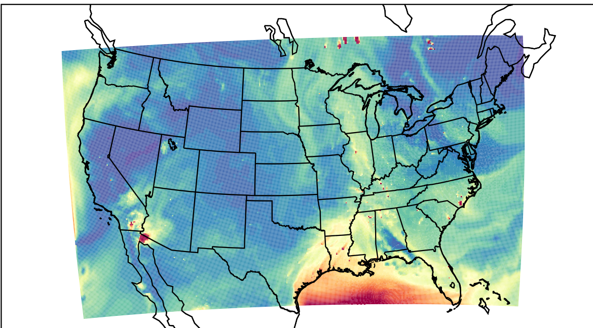
WRF 2023-06-18_22:00:00
