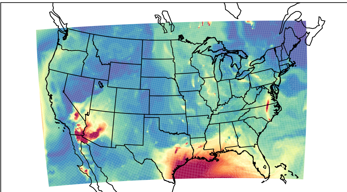
WRF 2023-06-19_10:00:00
