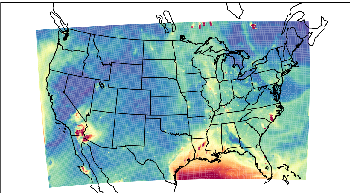
WRF 2023-06-19_01:00:00
