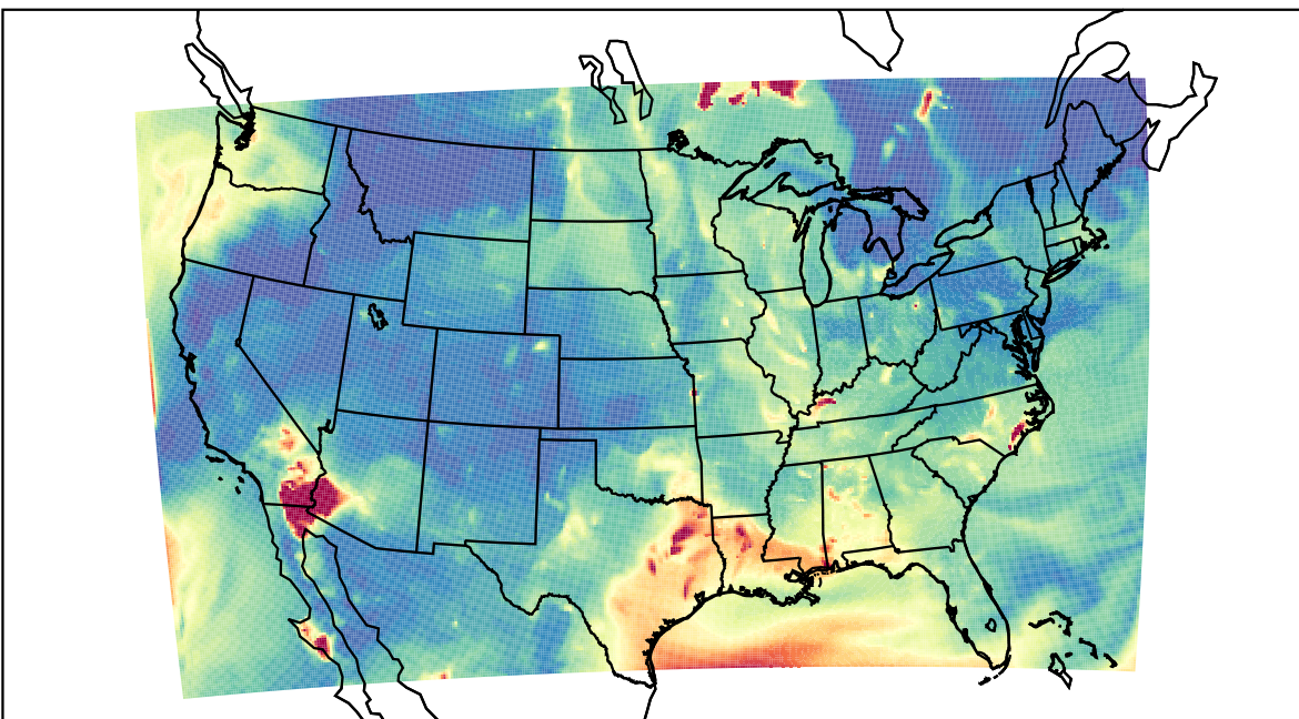
WRF 2023-06-18_06:00:00
