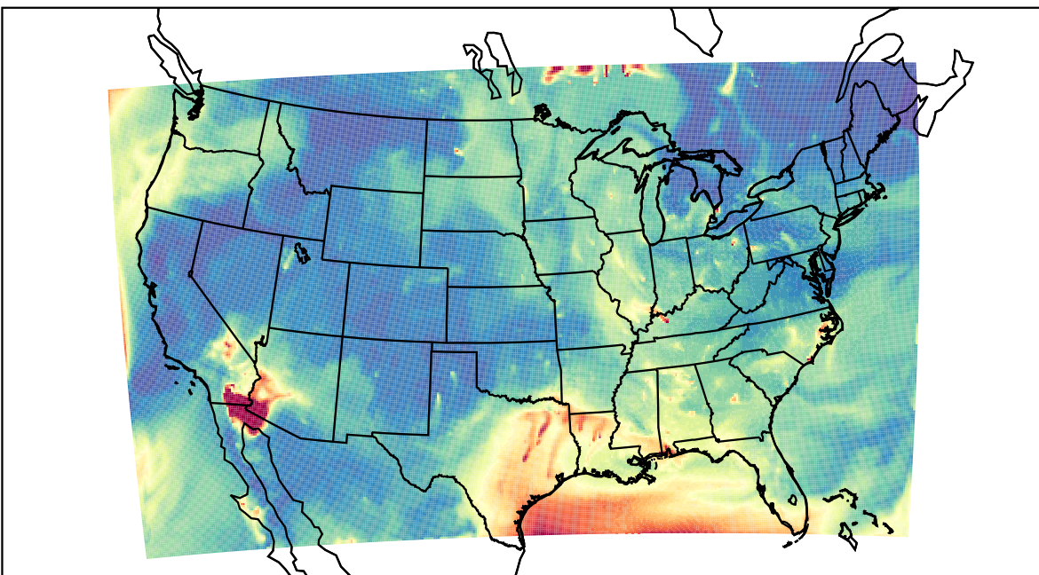
WRF 2023-06-18_12:00:00
