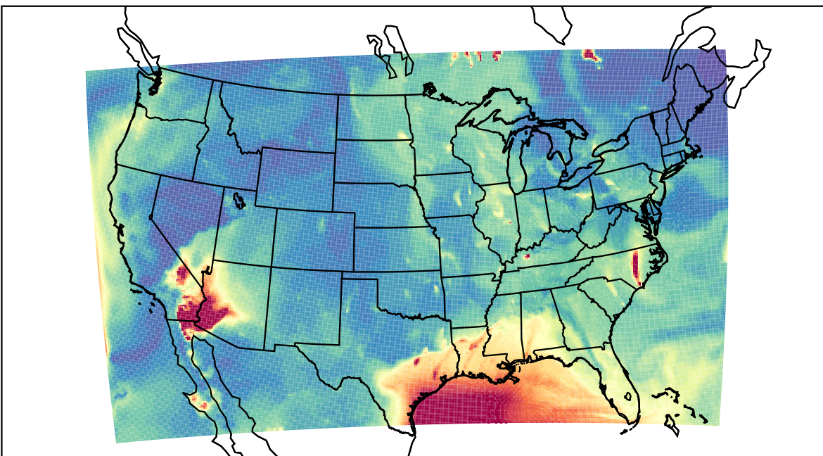
WRF 2023-06-19_06:00:00
