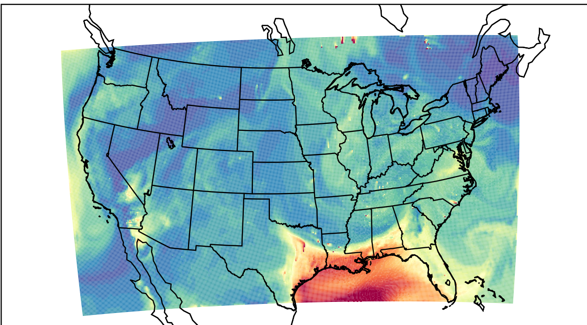
WRF 2023-06-19_19:00:00
