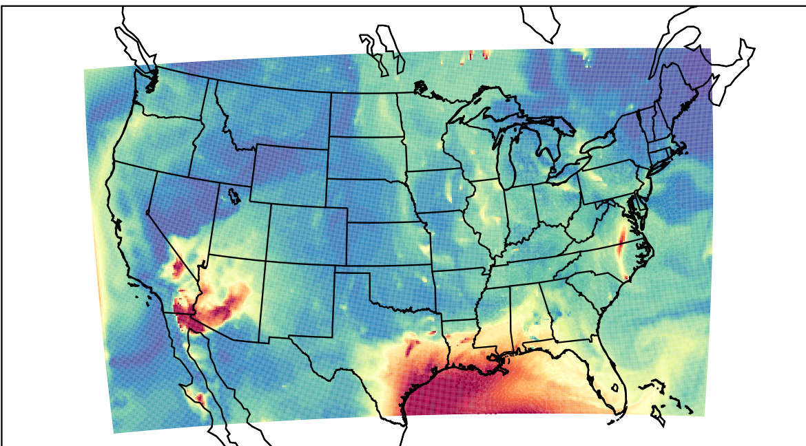
WRF 2023-06-19_11:00:00
