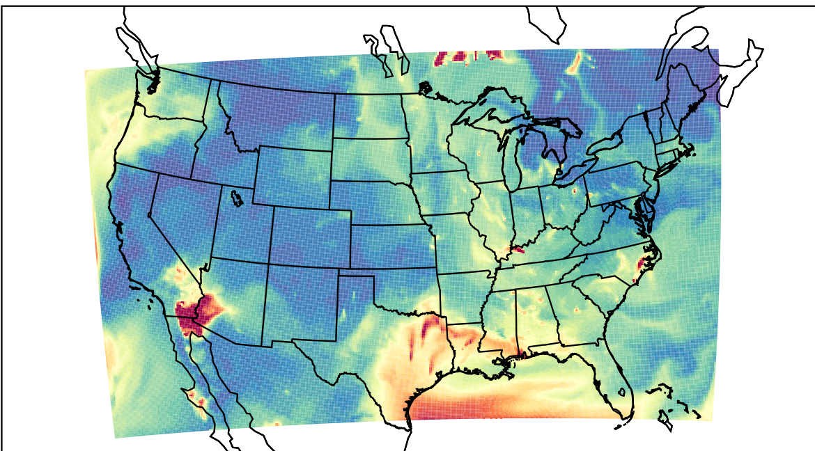
WRF 2023-06-18_09:00:00
