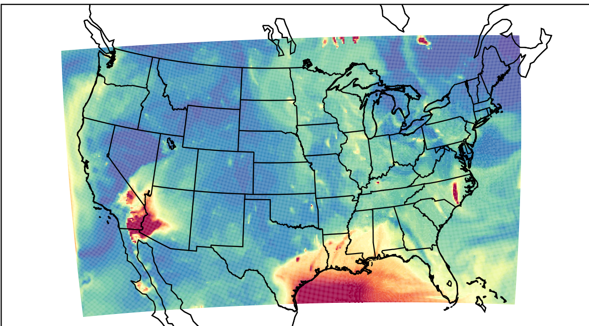
WRF 2023-06-19_05:00:00
