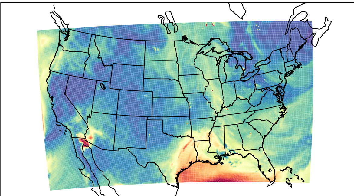
WRF 2023-06-18_17:00:00
