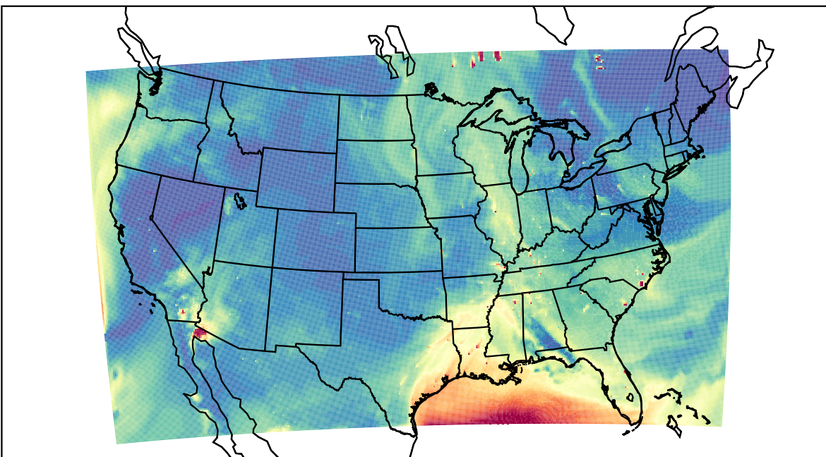
WRF 2023-06-18_21:00:00
