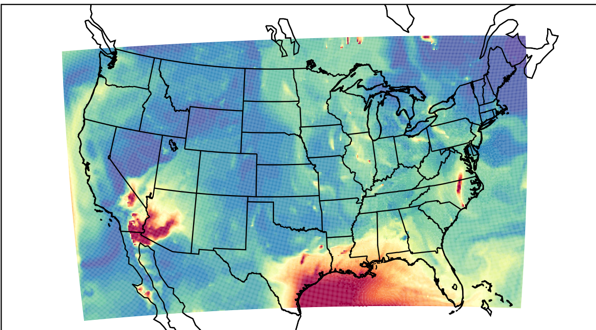
WRF 2023-06-19_09:00:00
