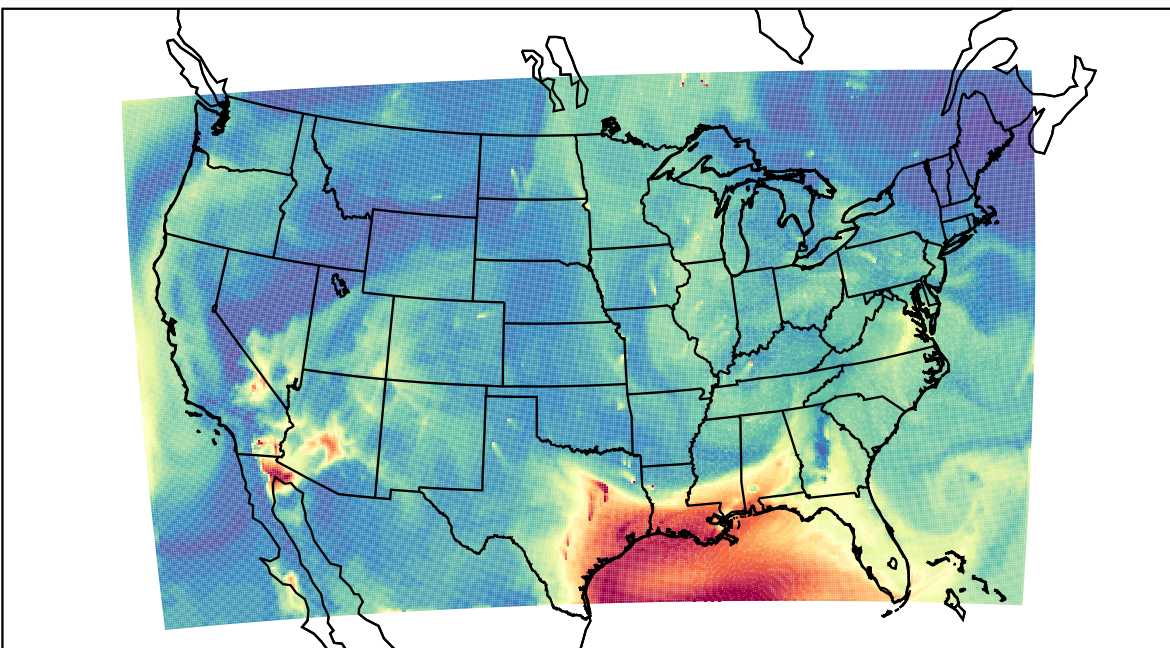
WRF 2023-06-19_16:00:00
