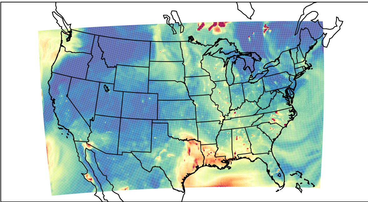
WRF 2023-06-18_01:00:00
