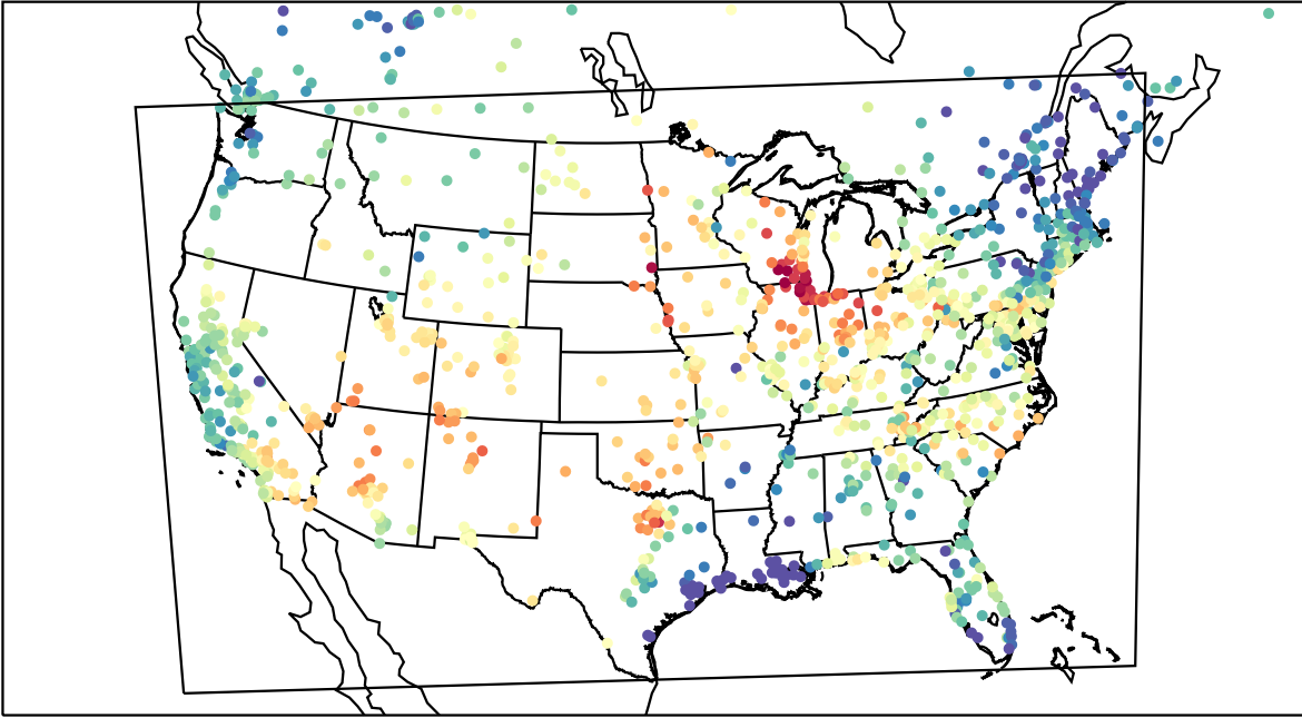
AirNOW (2023-06-19_00:00:00)
