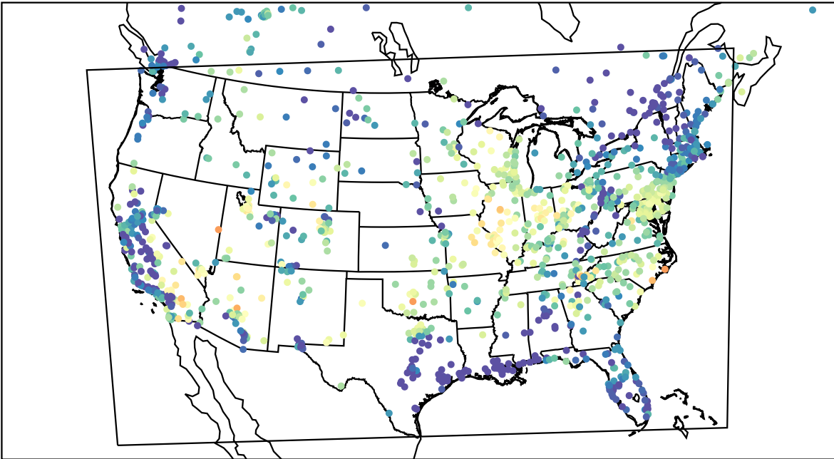
AirNOW (2023-06-18_13:00:00)
