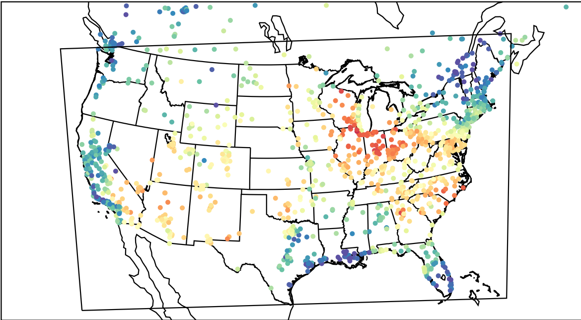
AirNOW (2023-06-18_16:00:00)
