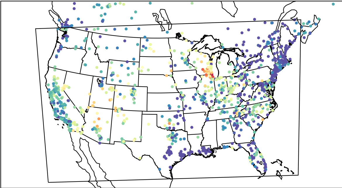
AirNOW (2023-06-19_06:00:00)
