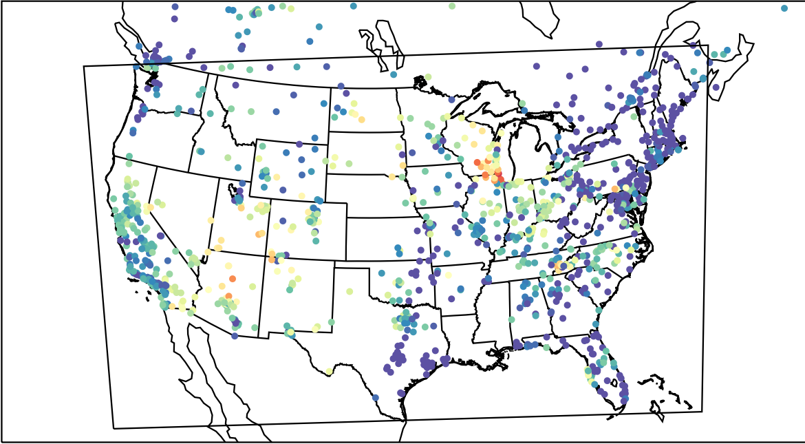
AirNOW (2023-06-19_07:00:00)
