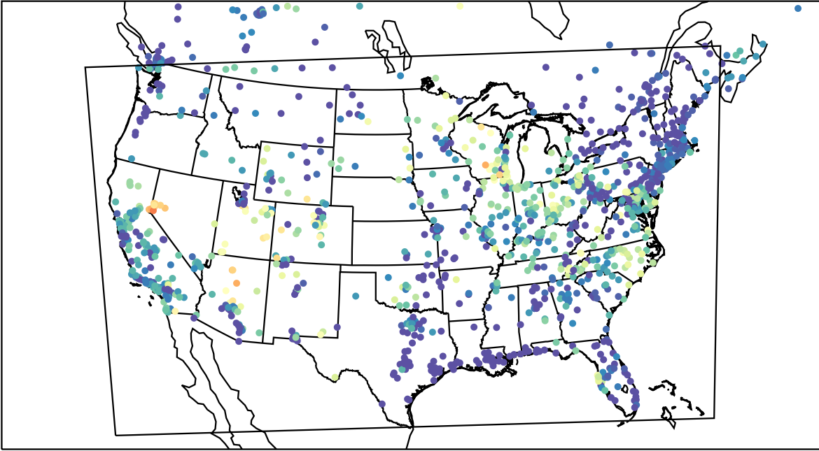
AirNOW (2023-06-19_12:00:00)
