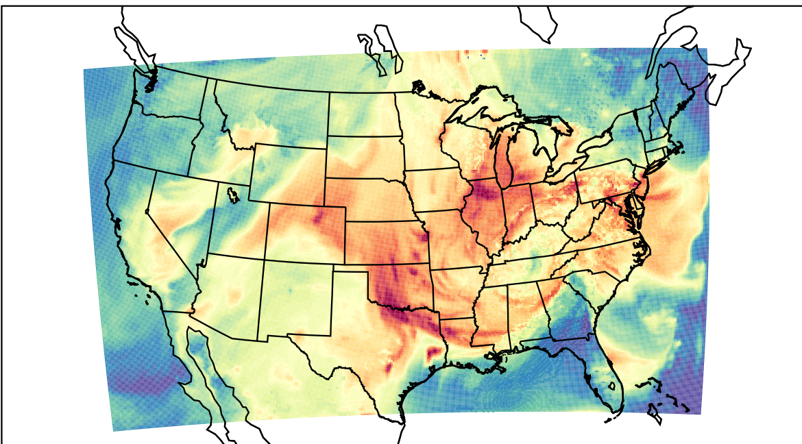
WRF (2023-06-19_22:00:00)
