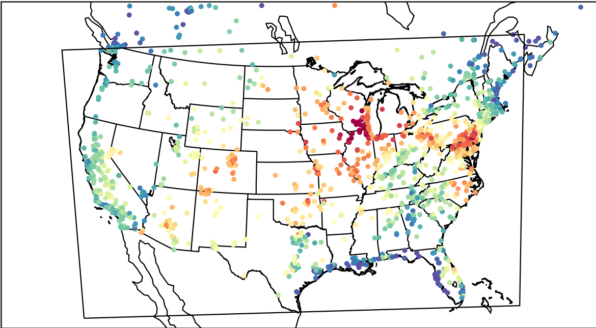
AirNOW (2023-06-19_18:00:00)
