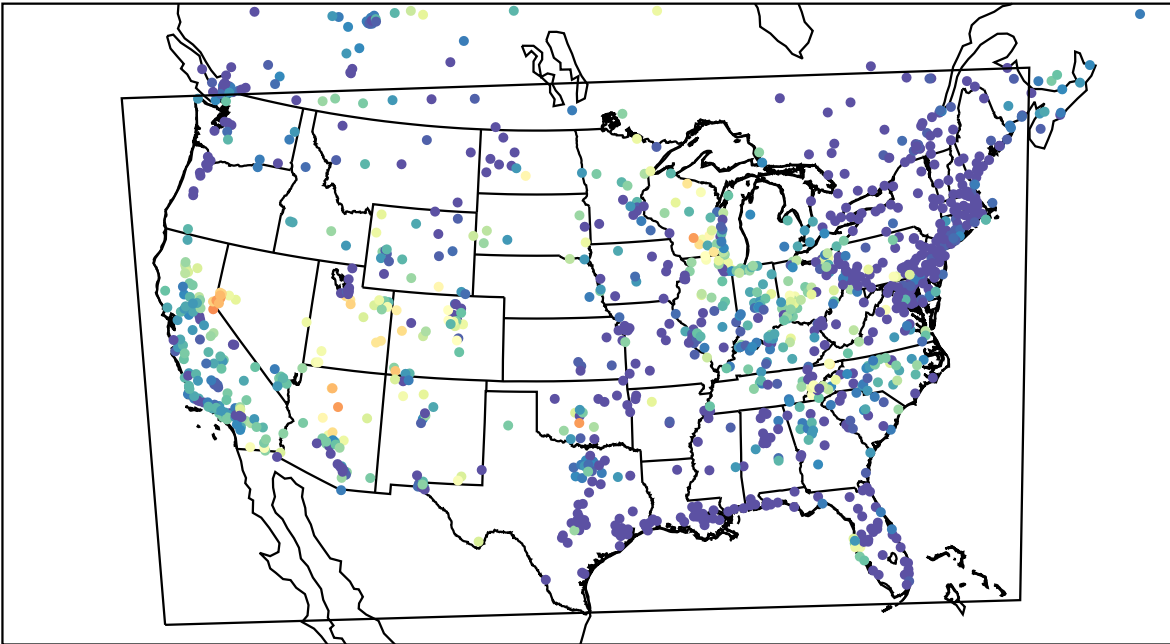
AirNOW (2023-06-19_11:00:00)
