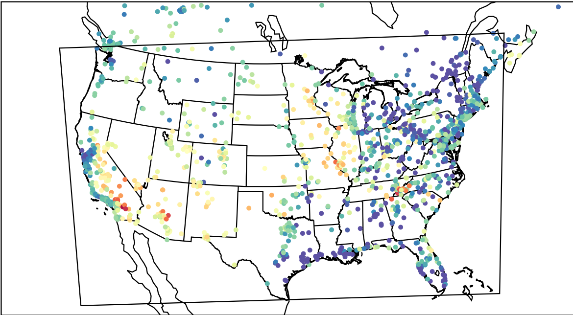
AirNOW (2023-06-18_03:00:00)
