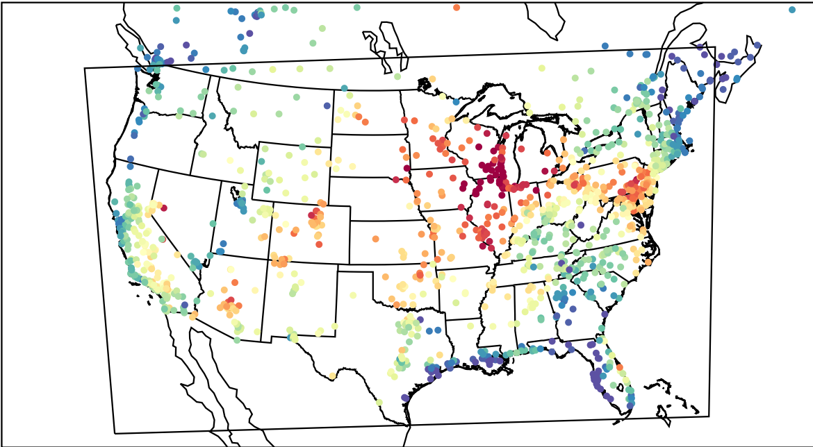
AirNOW (2023-06-19_22:00:00)
