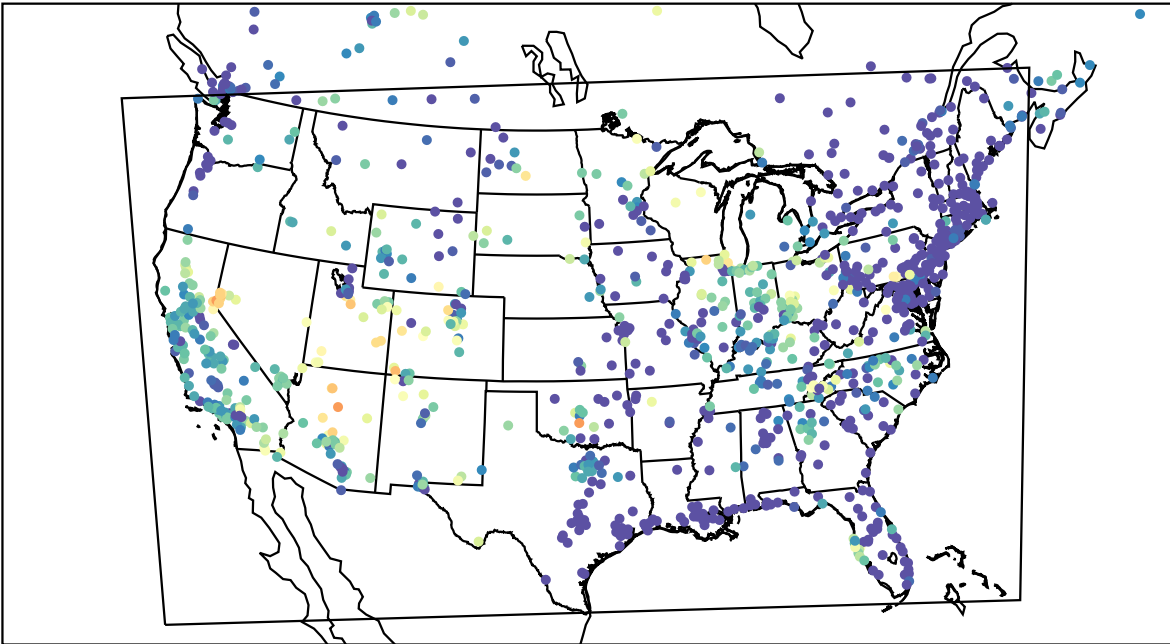
AirNOW (2023-06-19_10:00:00)
