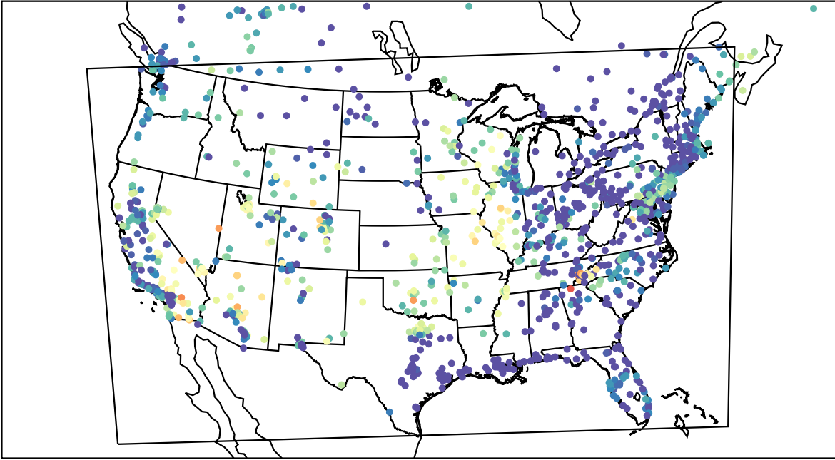
AirNOW (2023-06-18_11:00:00)
