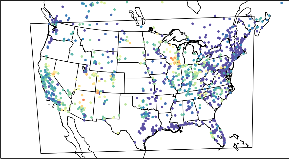
AirNOW (2023-06-19_09:00:00)
