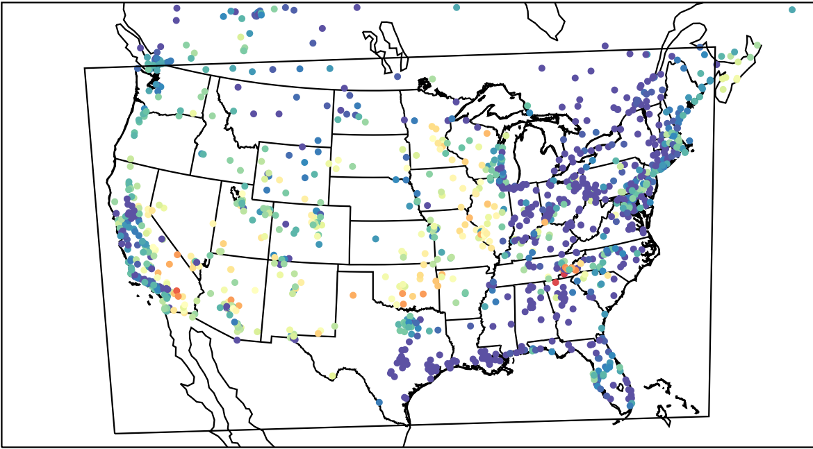
AirNOW (2023-06-18_07:00:00)
