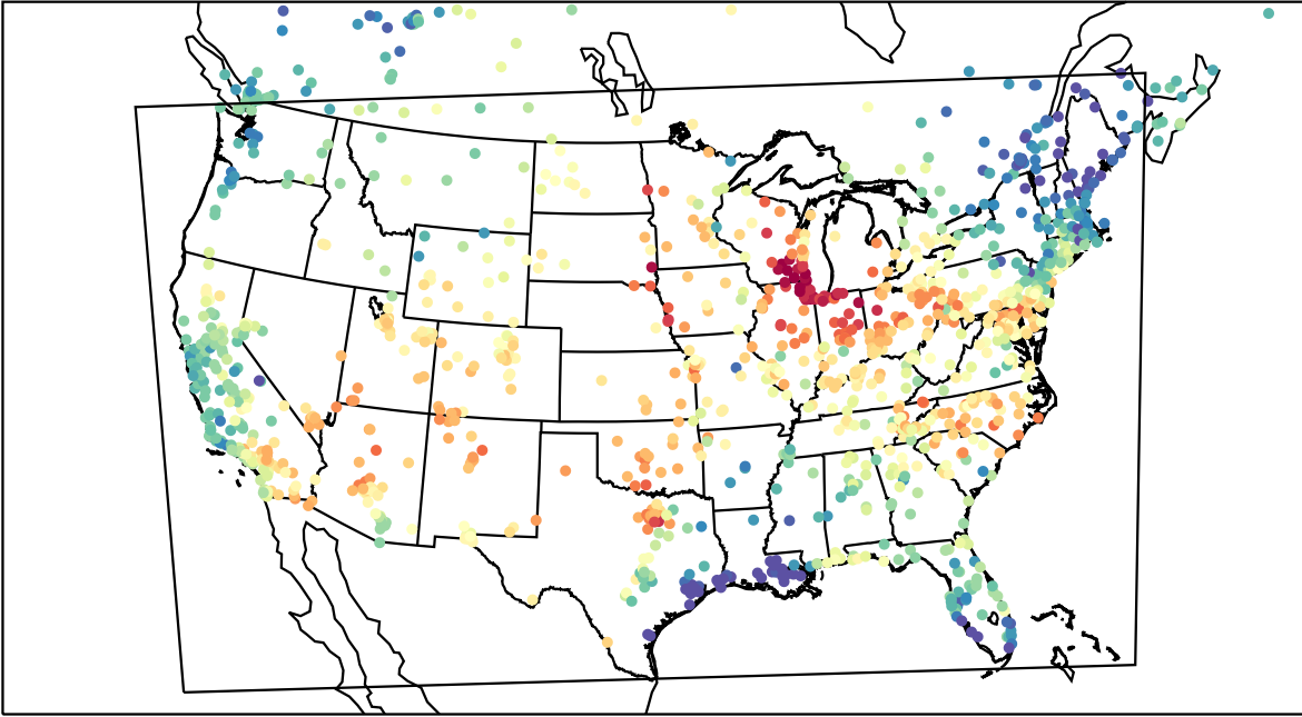
AirNOW (2023-06-18_23:00:00)
