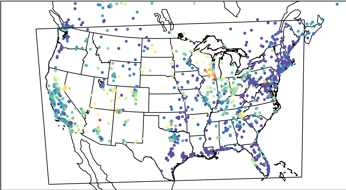
AirNOW (2023-06-19_08:00:00)
