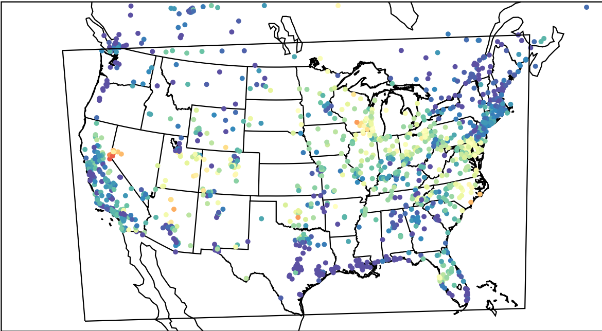
AirNOW (2023-06-19_13:00:00)
