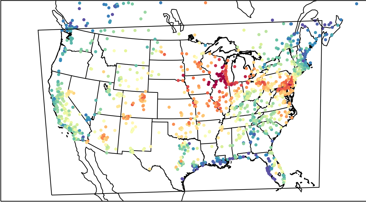
AirNOW (2023-06-19_19:00:00)
