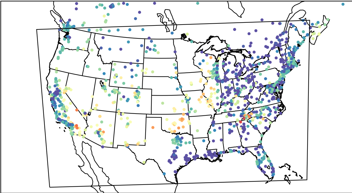
AirNOW (2023-06-18_06:00:00)
