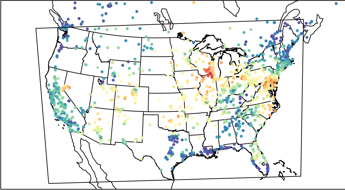
AirNOW (2023-06-19_15:00:00)
