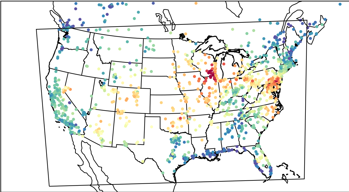
AirNOW (2023-06-19_16:00:00)
