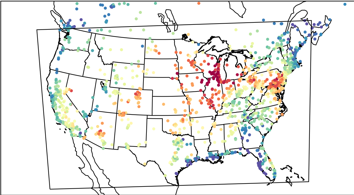
AirNOW (2023-06-19_21:00:00)
