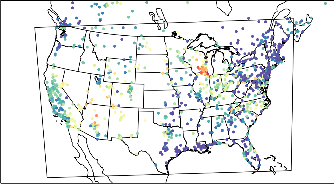
AirNOW (2023-06-19_05:00:00)
