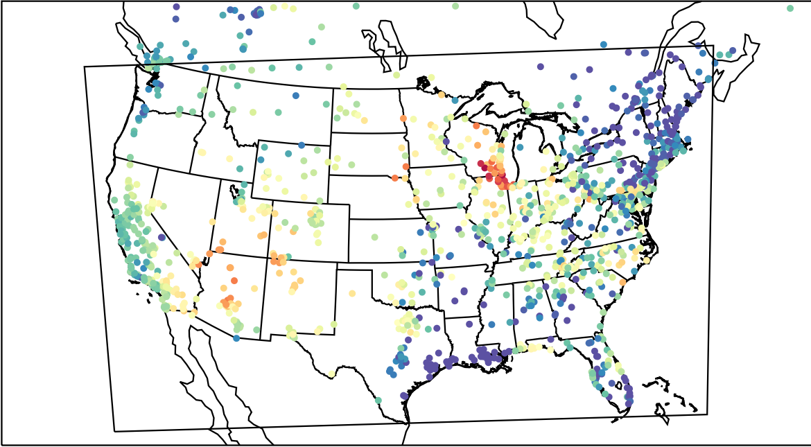
AirNOW (2023-06-19_02:00:00)
