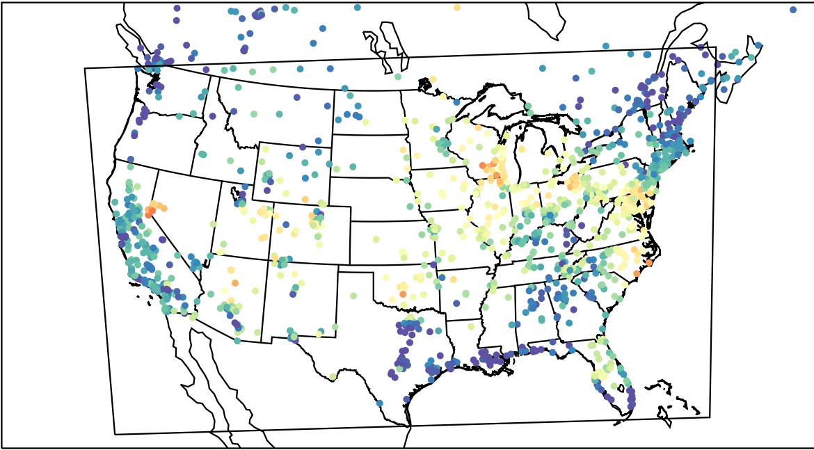
AirNOW (2023-06-19_14:00:00)
