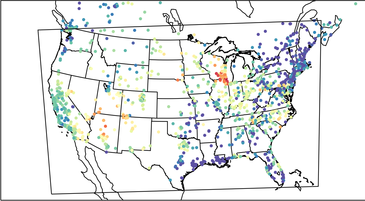
AirNOW (2023-06-19_03:00:00)
