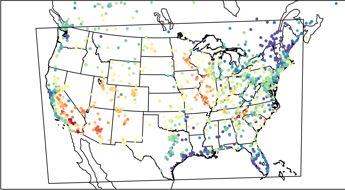
AirNOW (2023-06-18_01:00:00)
