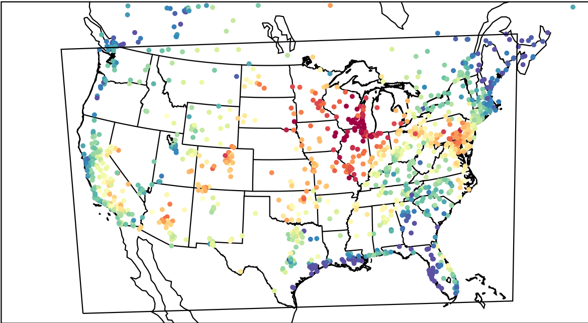
AirNOW (2023-06-19_23:00:00)
