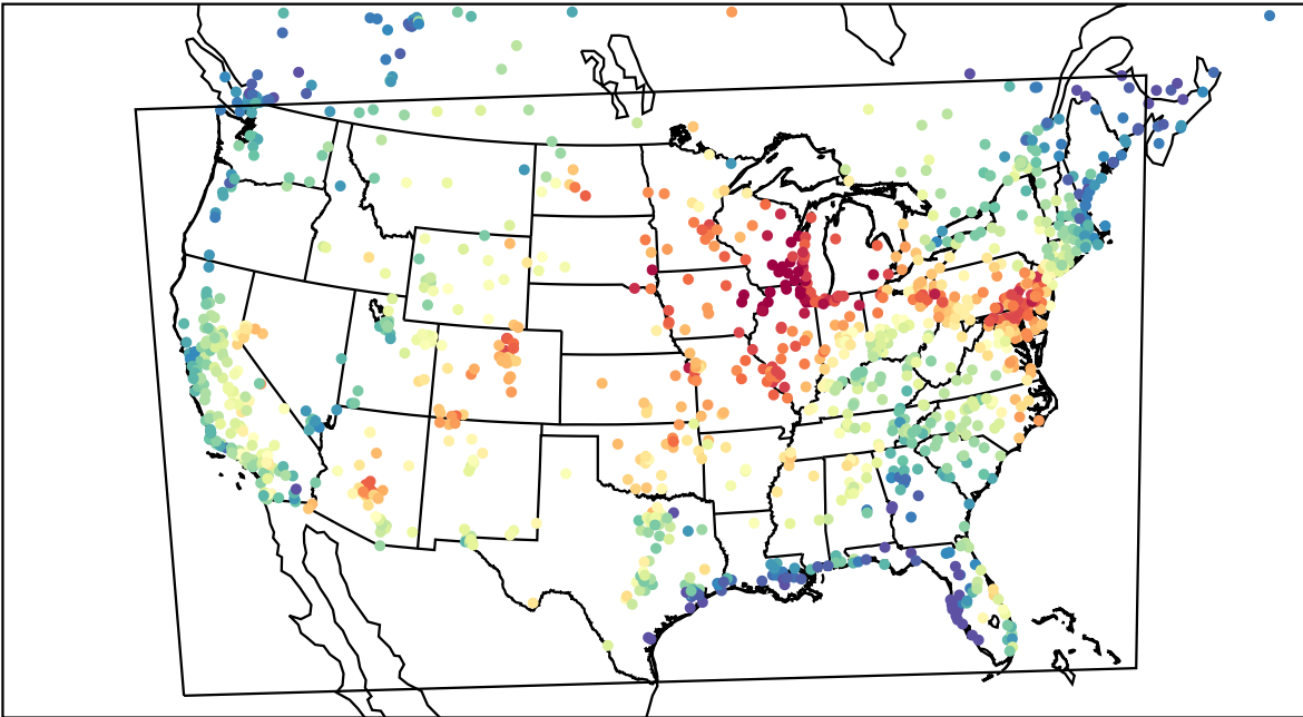
AirNOW (2023-06-19_20:00:00)
