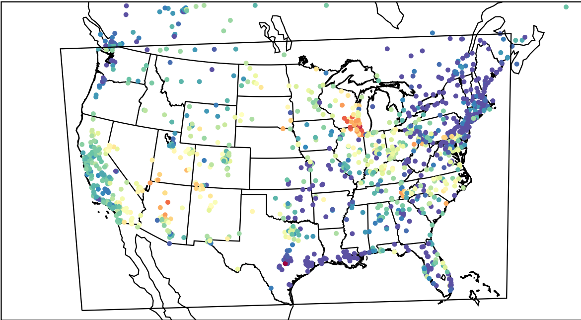
AirNOW (2023-06-19_04:00:00)
