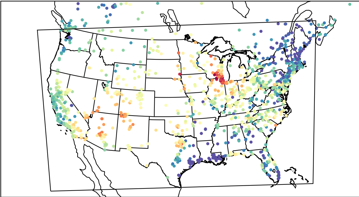
AirNOW (2023-06-19_01:00:00)
