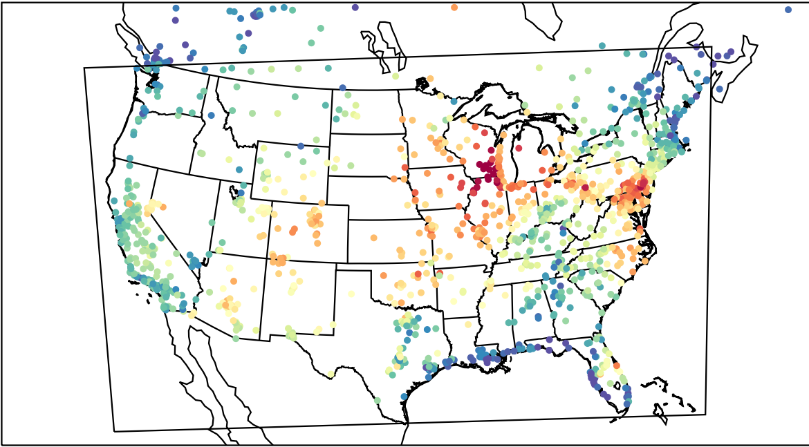
AirNOW (2023-06-19_17:00:00)
