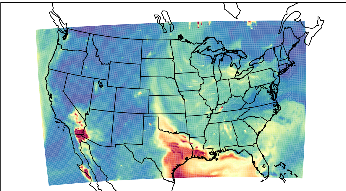
WRF 2023-06-21_05:00:00
