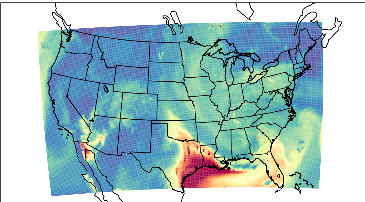
WRF 2023-06-20_17:00:00
