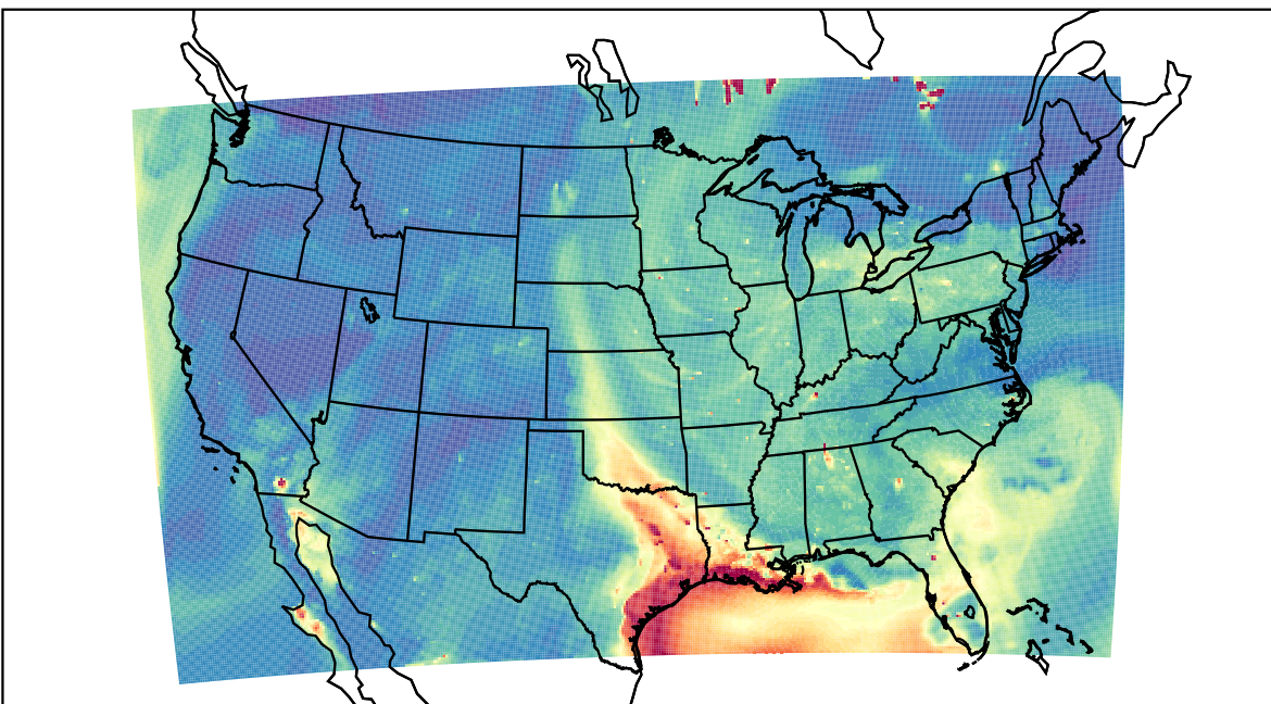
WRF 2023-06-21_00:00:00
