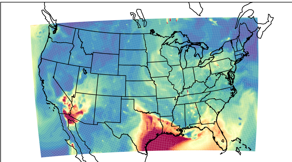
WRF 2023-06-20_12:00:00
