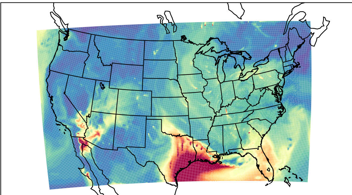
WRF 2023-06-20_15:00:00
