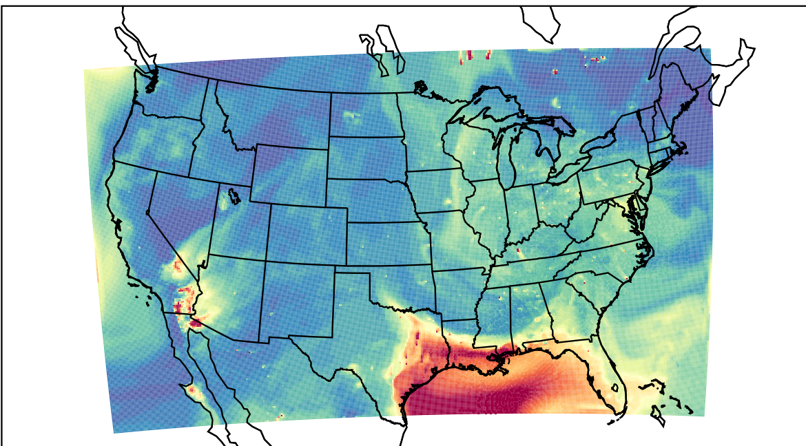
WRF 2023-06-20_00:00:00
