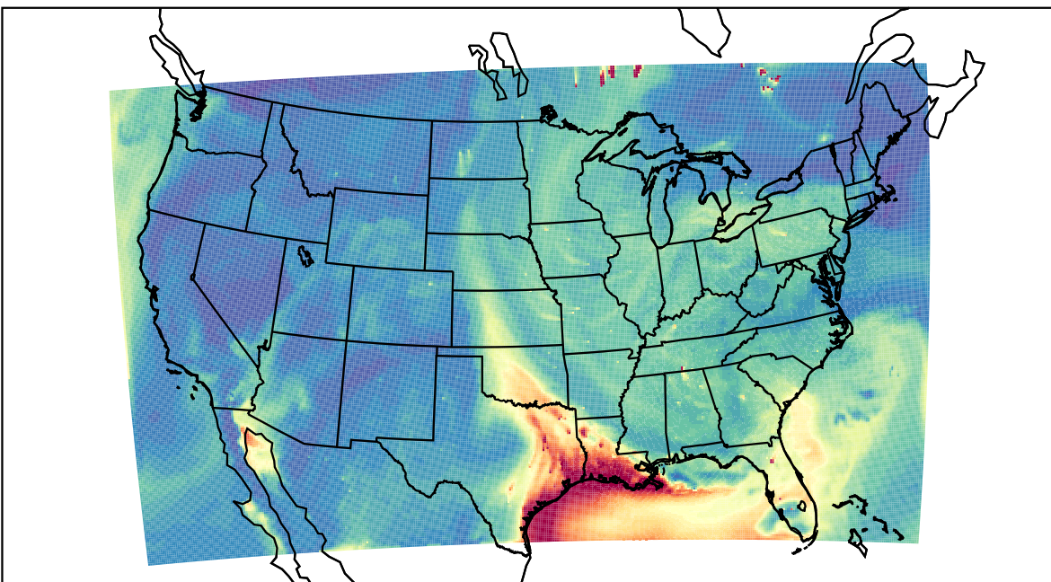
WRF 2023-06-20_21:00:00
