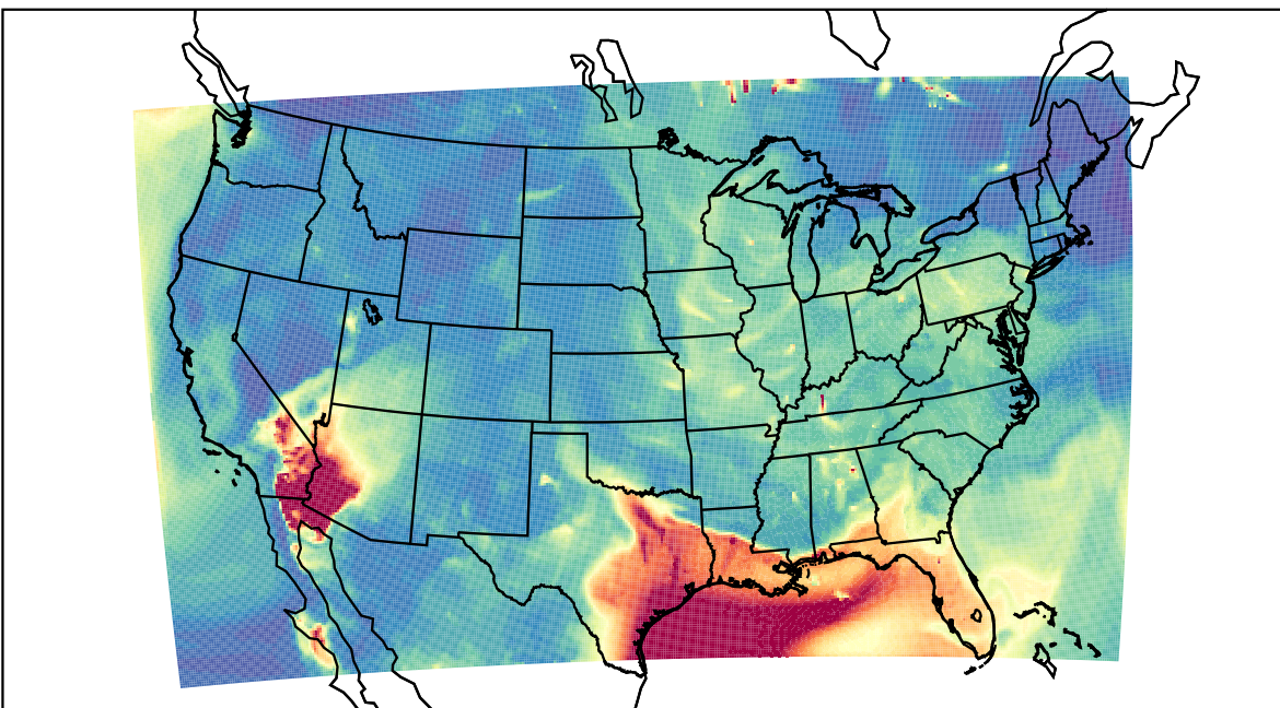
WRF 2023-06-20_07:00:00
