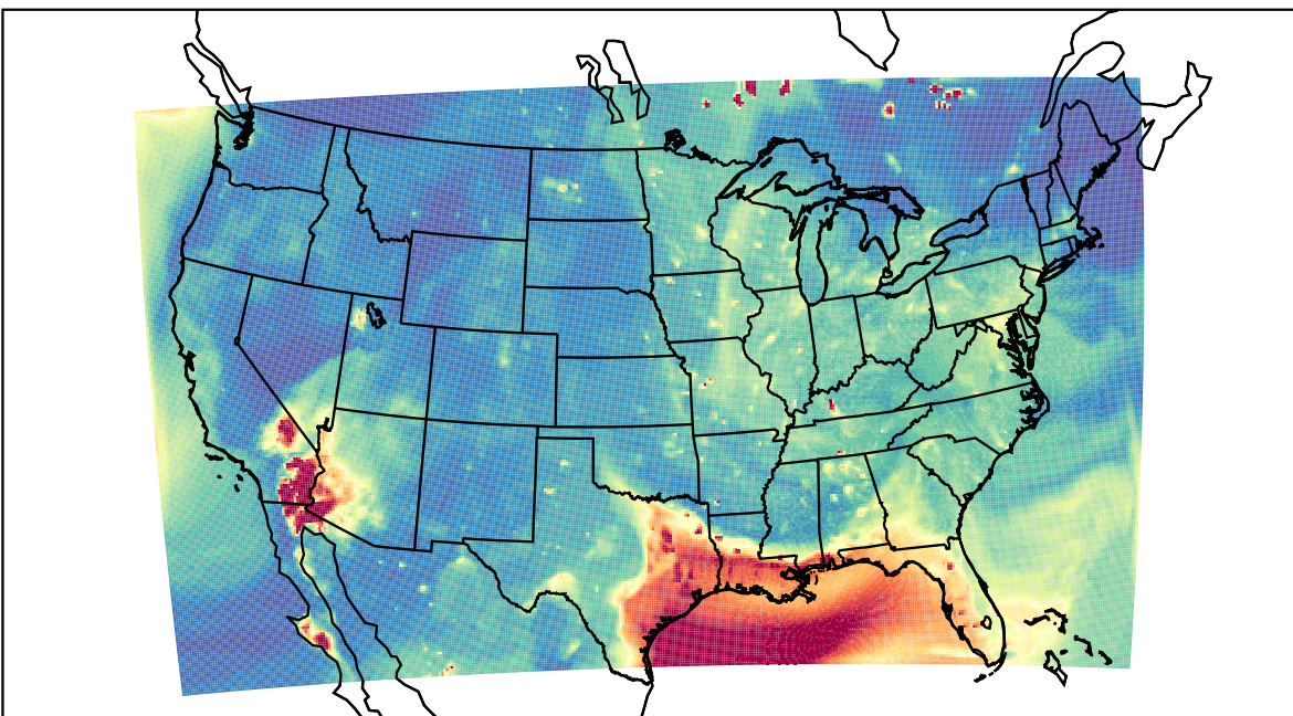
WRF 2023-06-20_02:00:00
