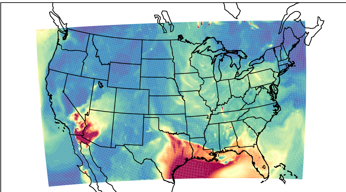
WRF 2023-06-20_09:00:00
