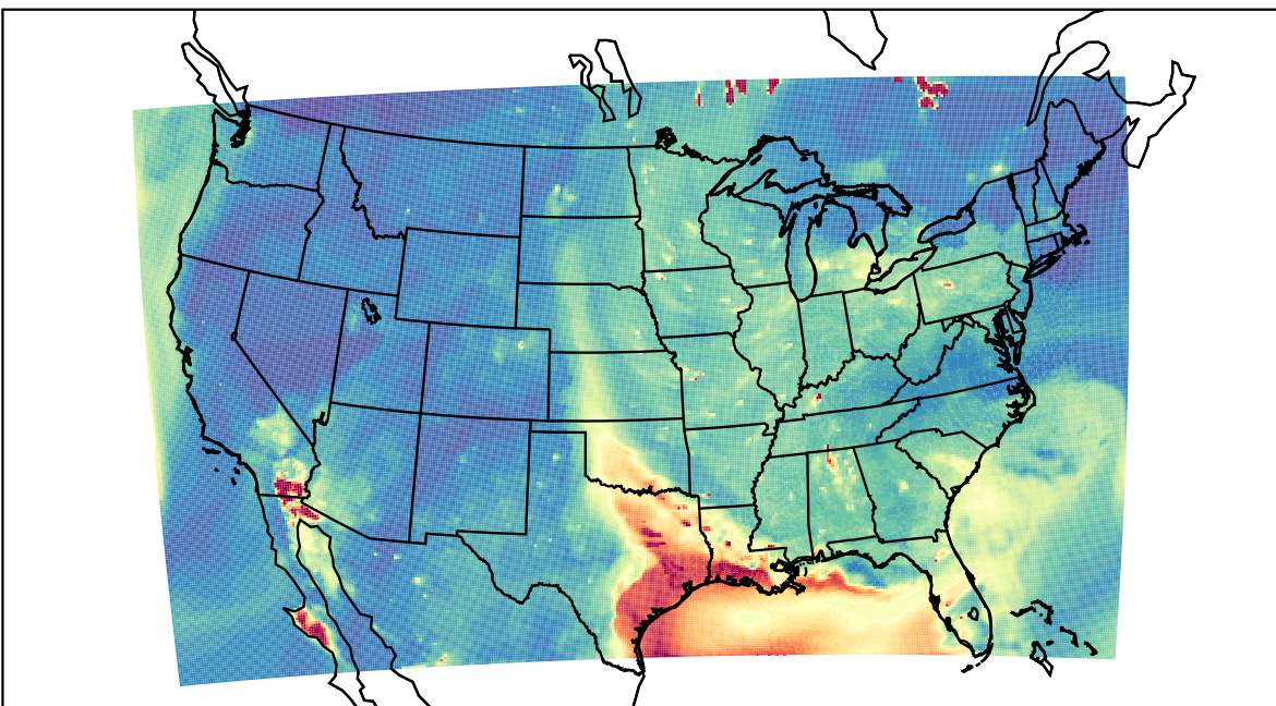
WRF 2023-06-21_02:00:00
