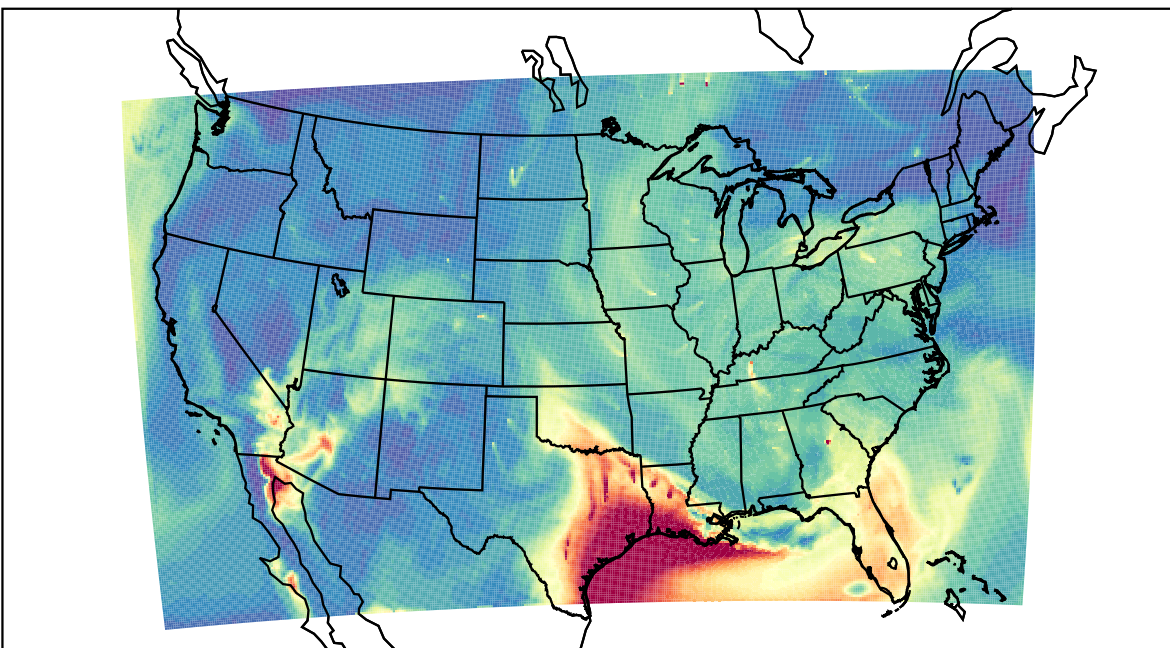
WRF 2023-06-20_16:00:00
