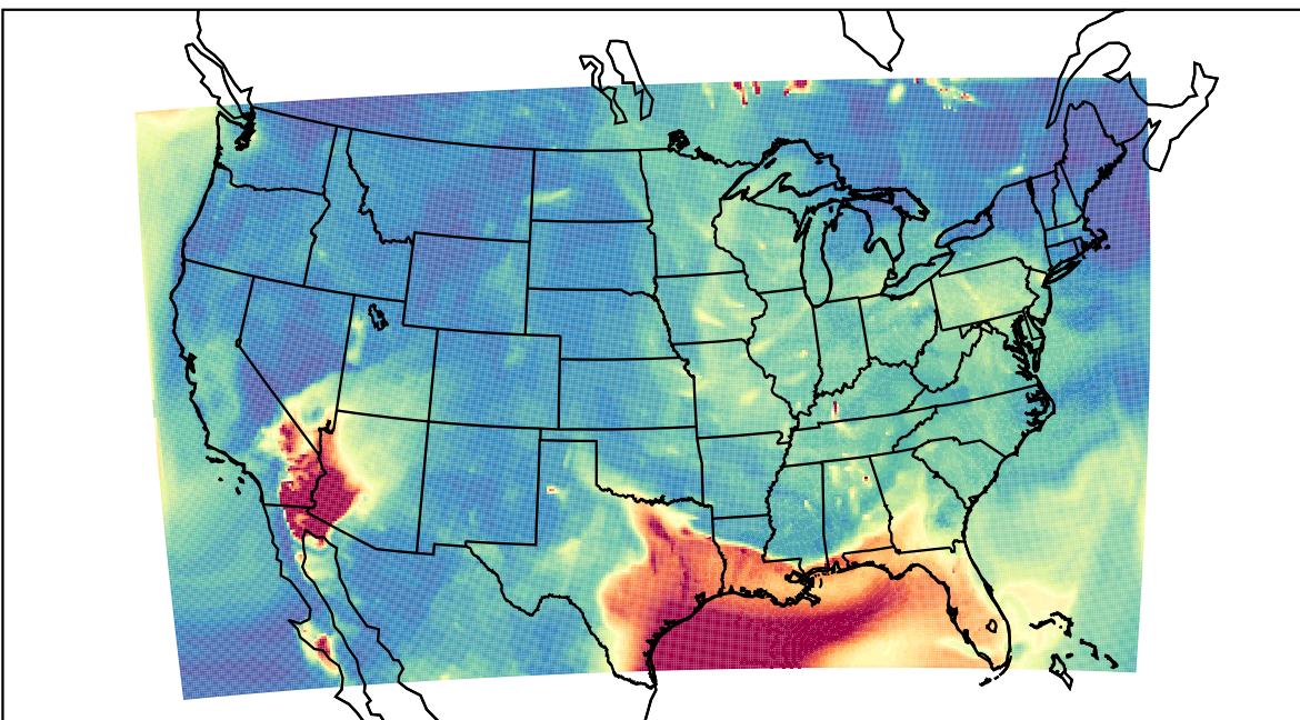
WRF 2023-06-20_06:00:00
