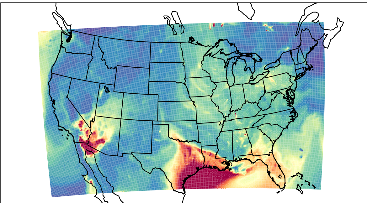
WRF 2023-06-20_11:00:00
