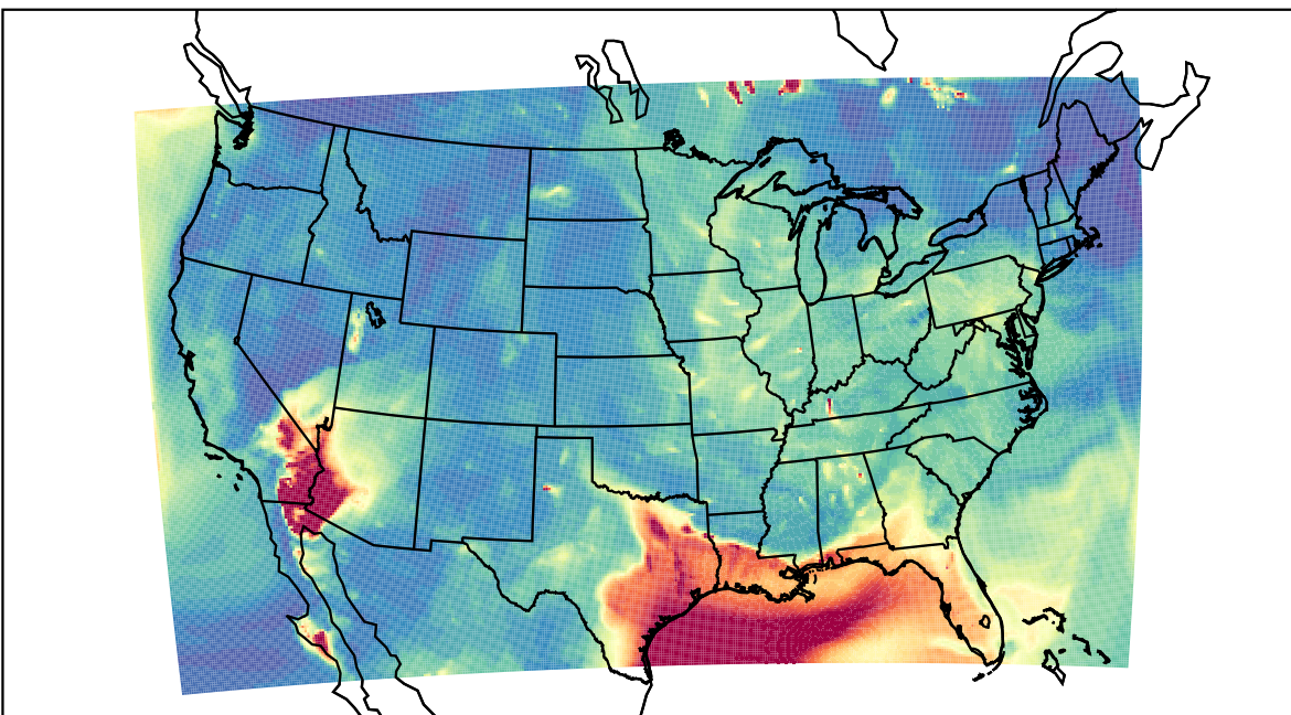
WRF 2023-06-20_05:00:00
