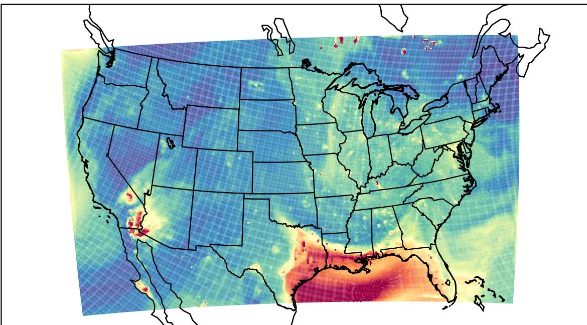
WRF 2023-06-20_01:00:00
