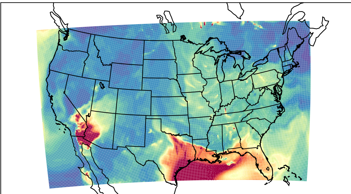
WRF 2023-06-20_08:00:00
