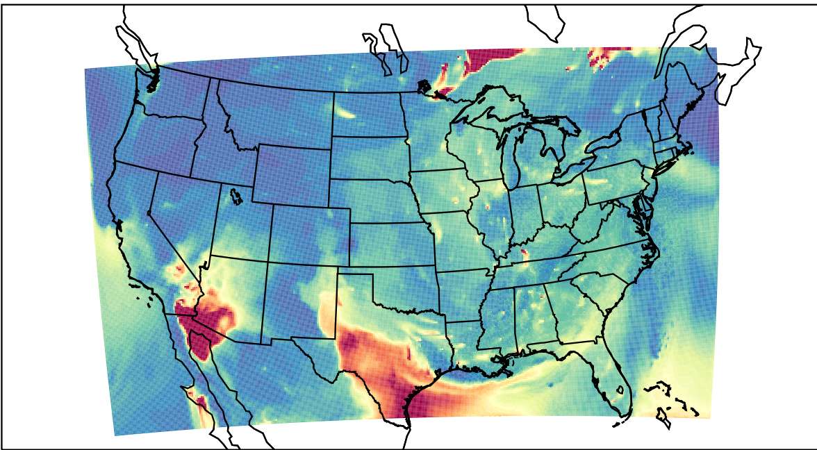
WRF 2023-06-23_11:00:00
