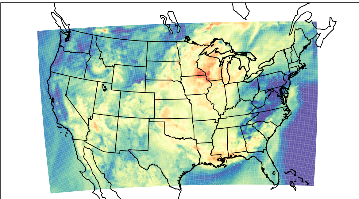
WRF (2023-06-22_15:00:00)
