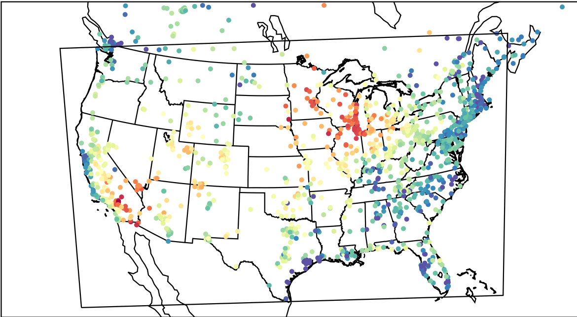
AirNOW (2023-06-22_01:00:00)
