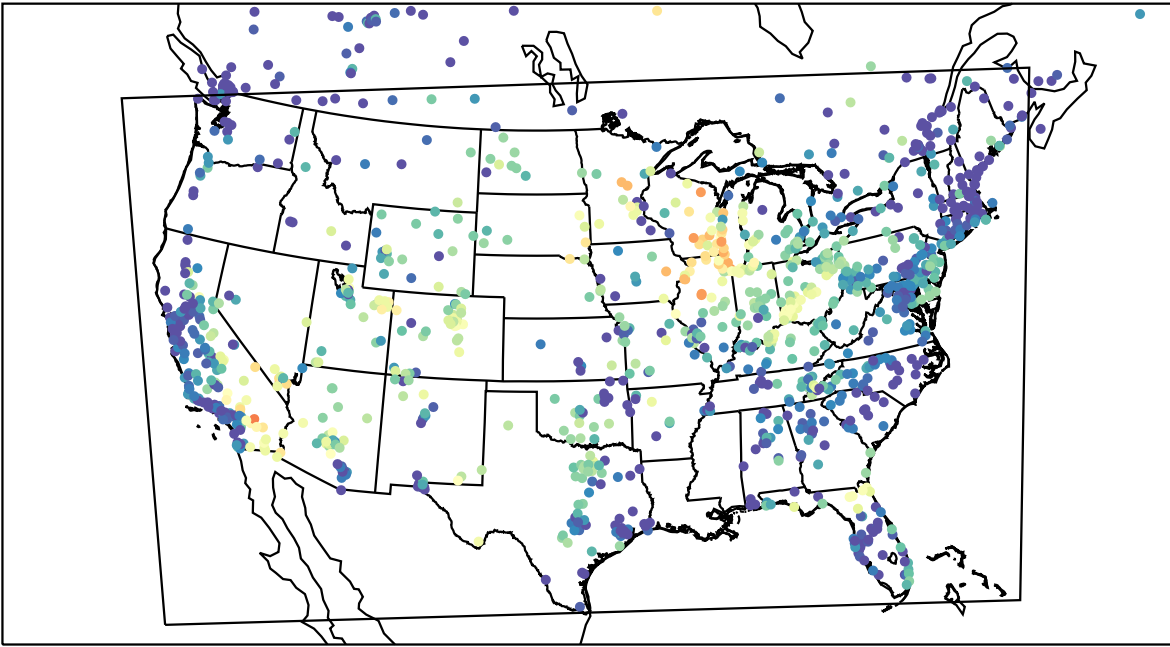
AirNOW (2023-06-22_07:00:00)
