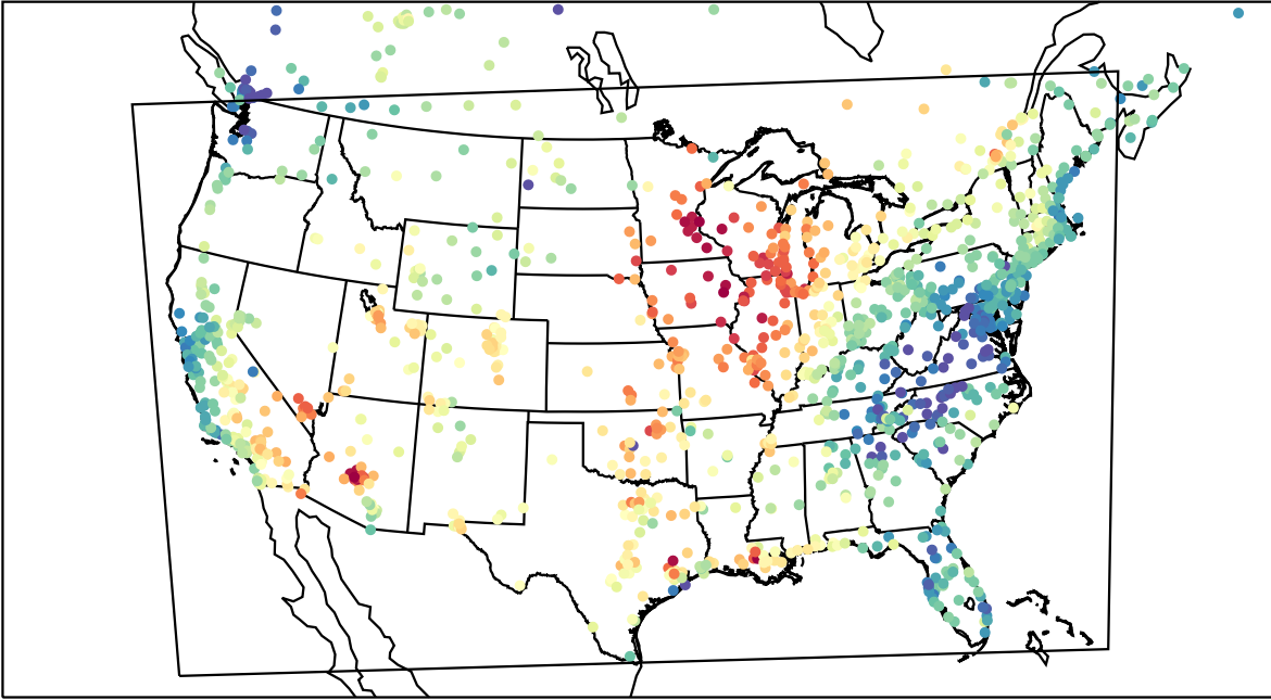
AirNOW (2023-06-22_19:00:00)
