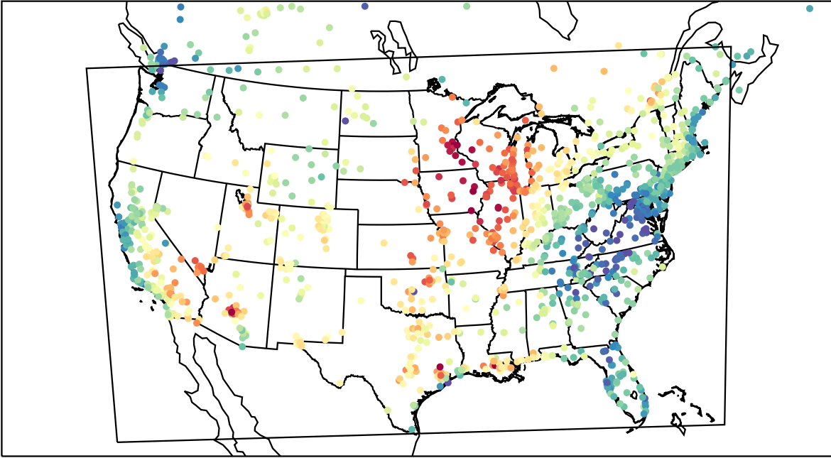
AirNOW (2023-06-22_20:00:00)
