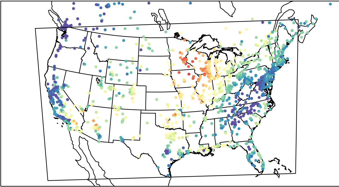
AirNOW (2023-06-22_15:00:00)
