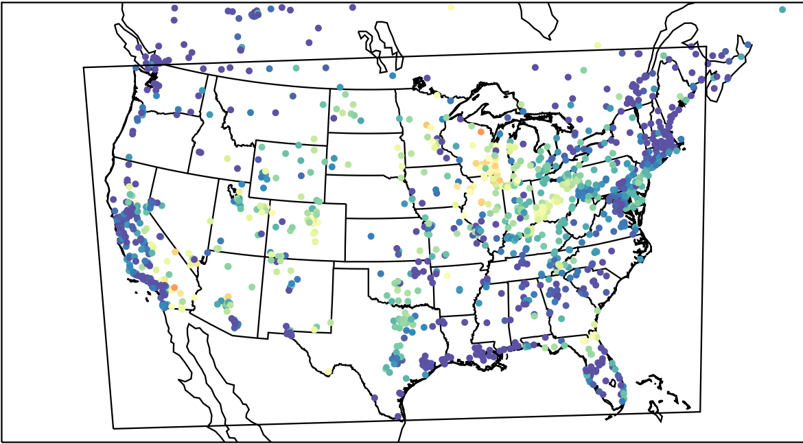
AirNOW (2023-06-22_08:00:00)
