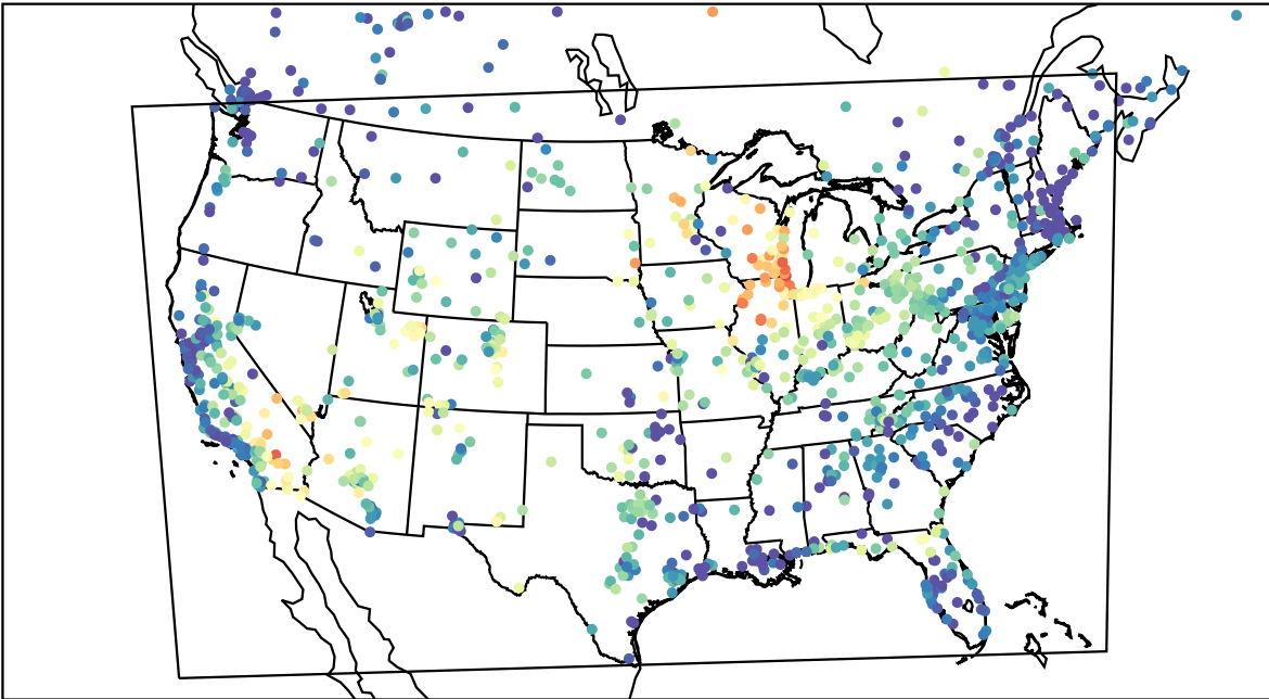
AirNOW (2023-06-22_05:00:00)
