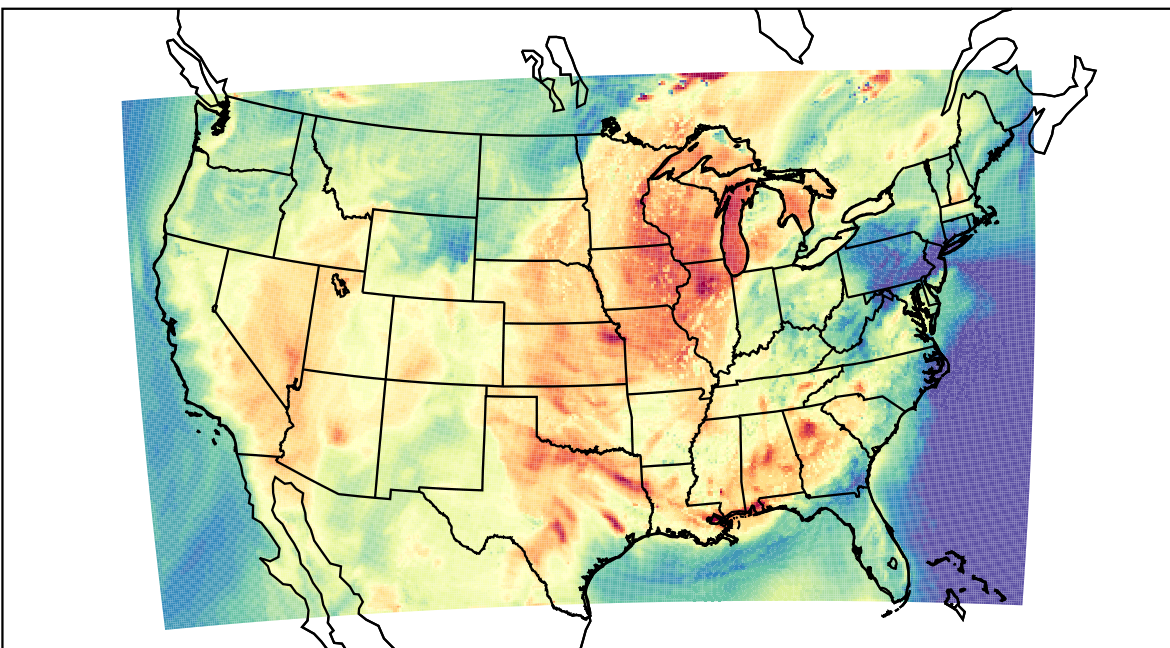
WRF (2023-06-22_22:00:00)
