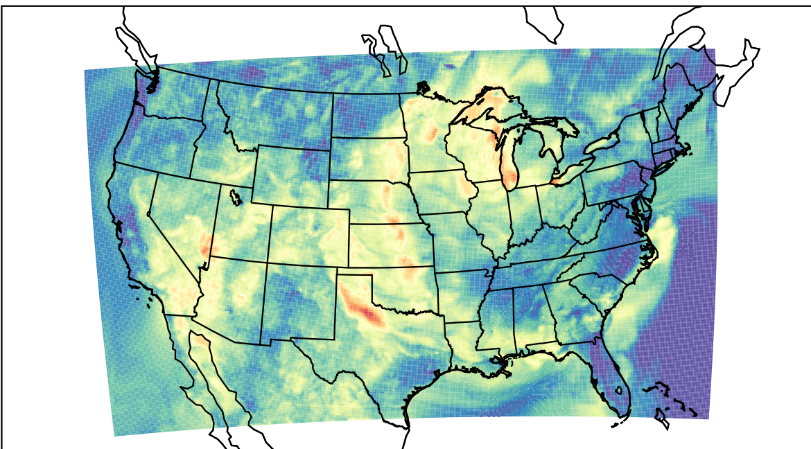
WRF (2023-06-22_05:00:00)
