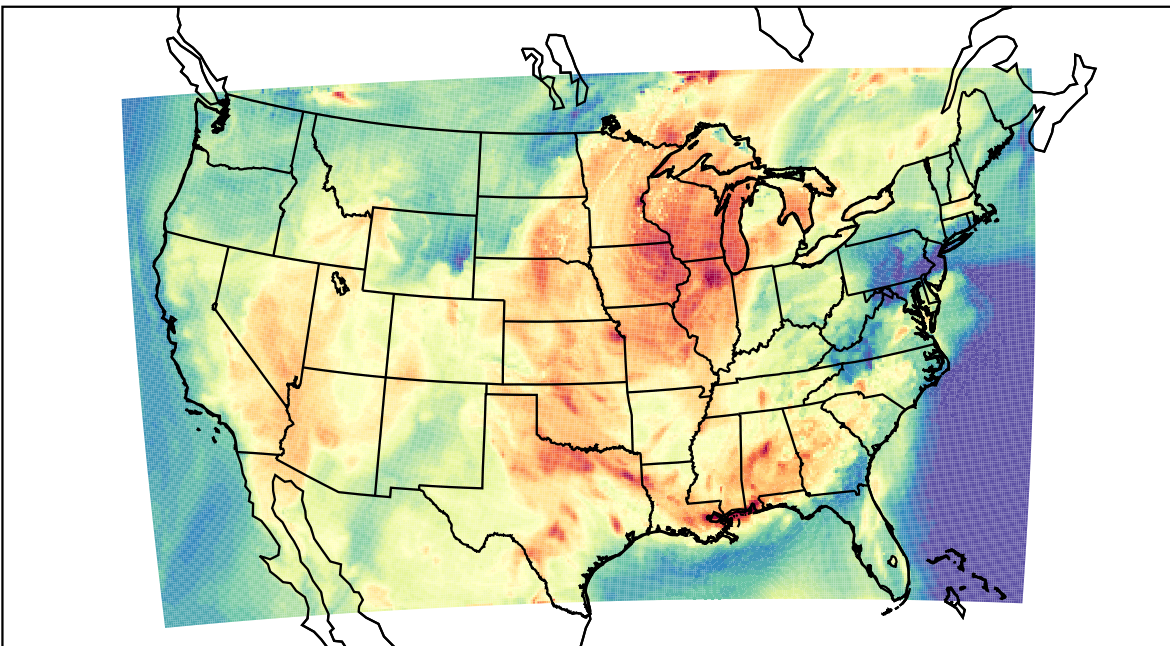
WRF (2023-06-22_19:00:00)
