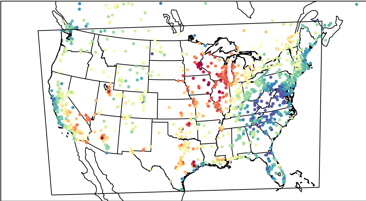
AirNOW (2023-06-22_22:00:00)
