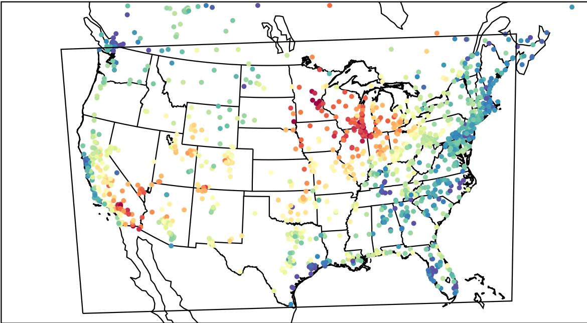
AirNOW (2023-06-22_00:00:00)
