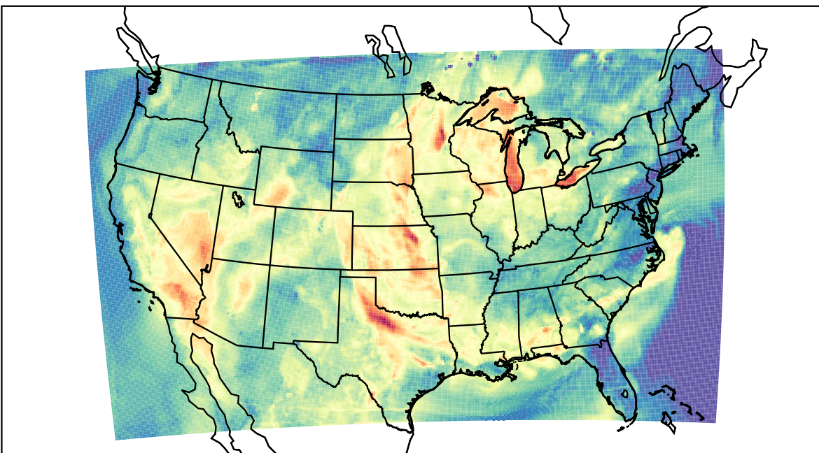
WRF (2023-06-22_02:00:00)
