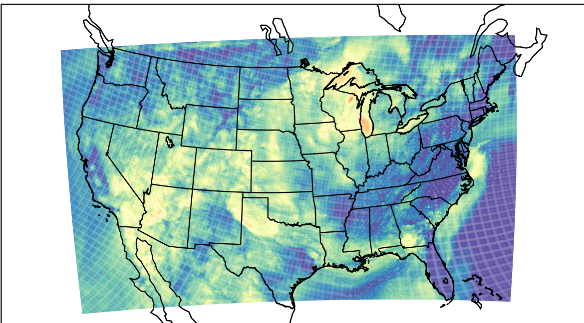
WRF (2023-06-22_09:00:00)
