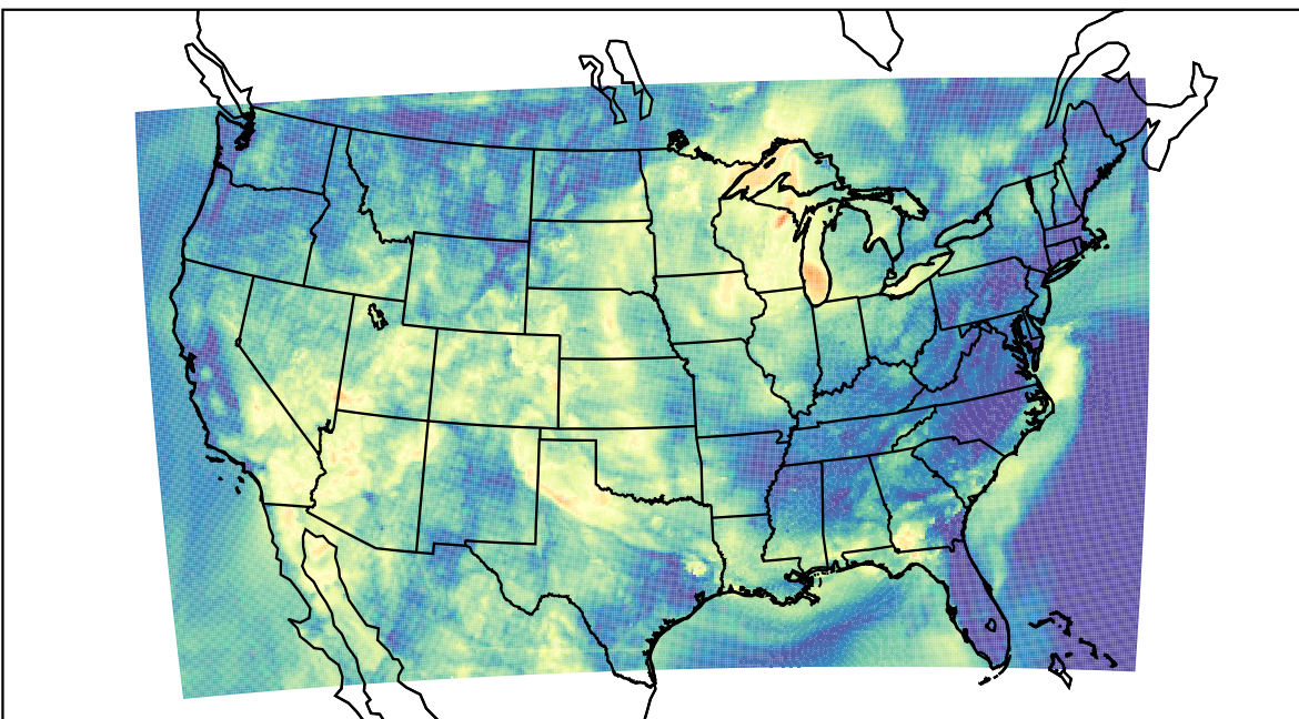
WRF (2023-06-22_08:00:00)
