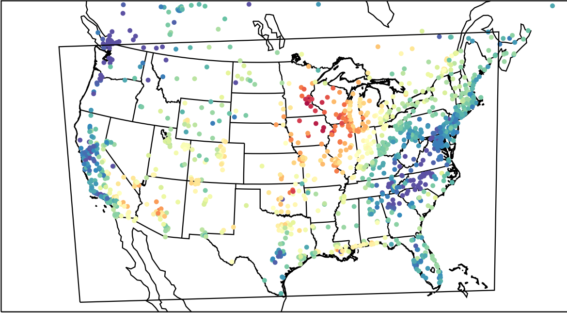
AirNOW (2023-06-22_16:00:00)
