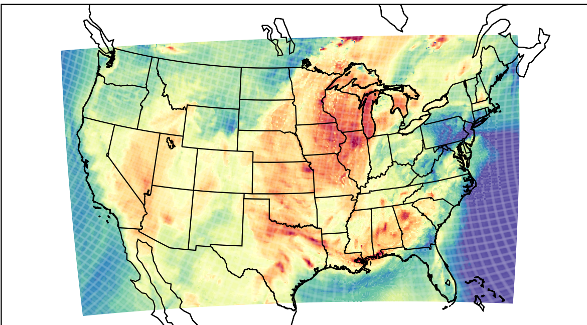
WRF (2023-06-22_21:00:00)
