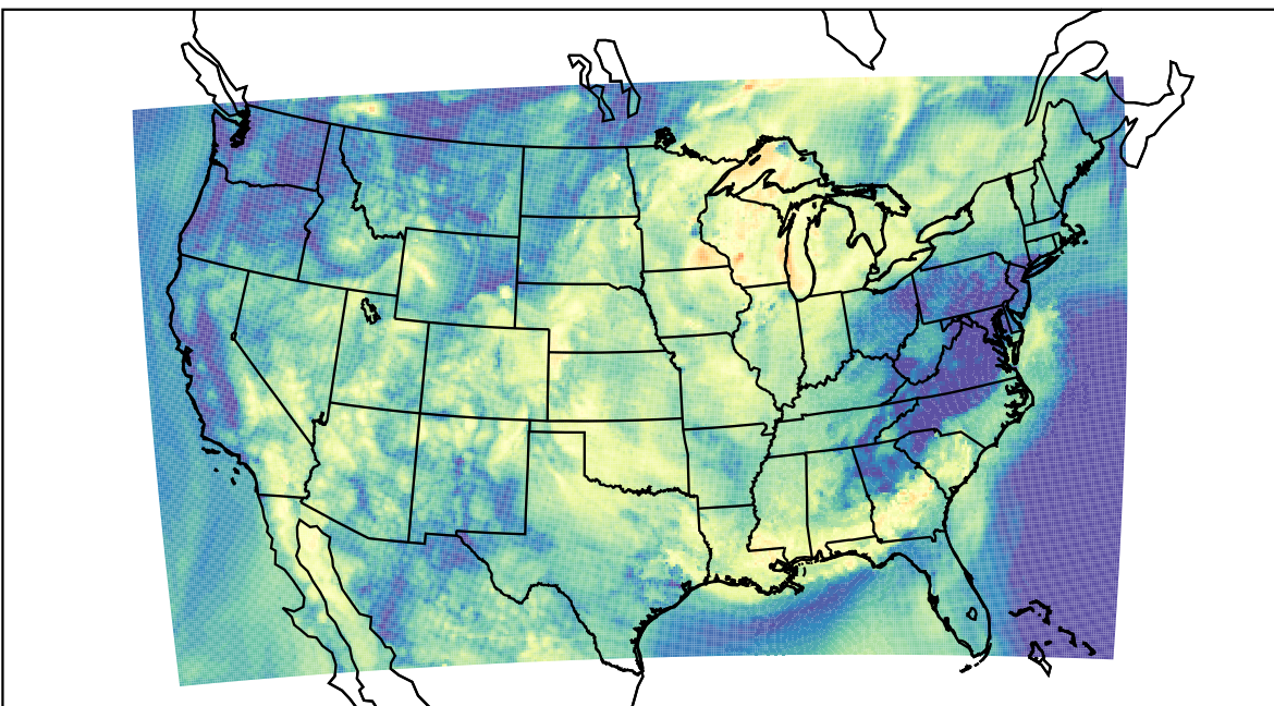
WRF (2023-06-22_14:00:00)
