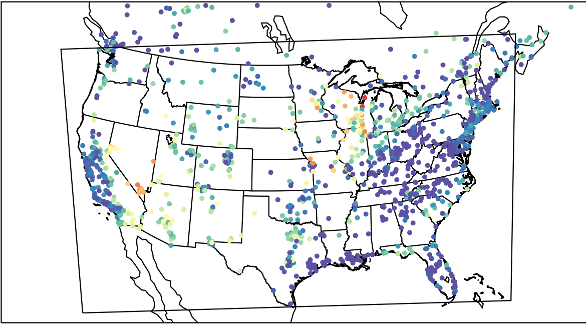
AirNOW (2023-06-23_06:00:00)
