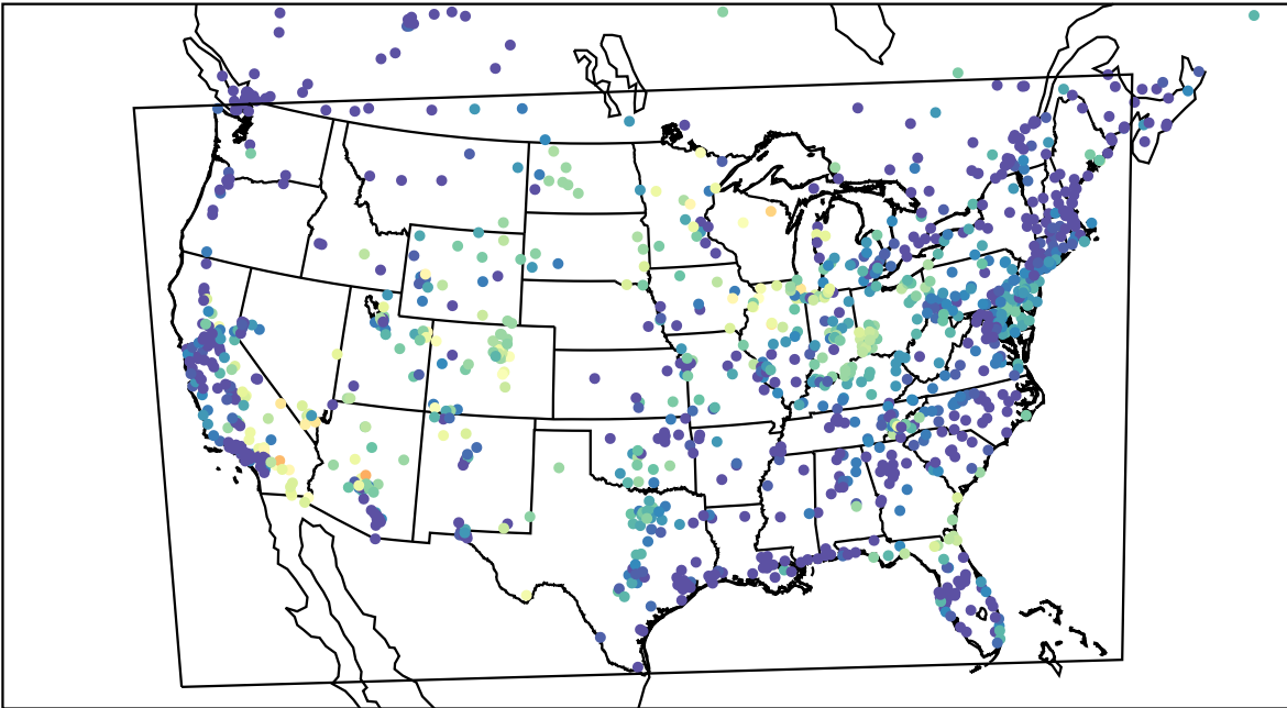
AirNOW (2023-06-22_10:00:00)
