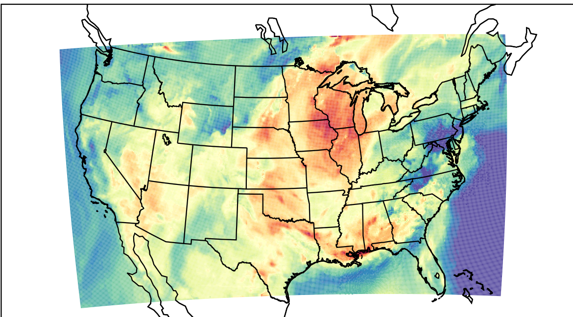
WRF (2023-06-22_17:00:00)
