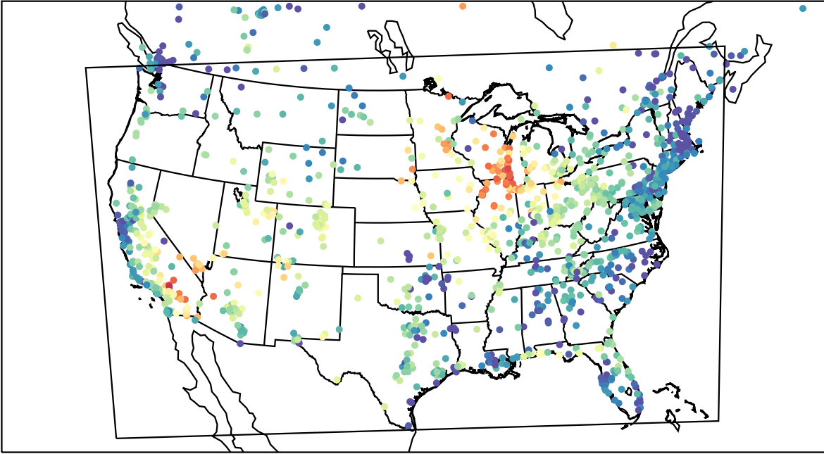
AirNOW (2023-06-22_03:00:00)
