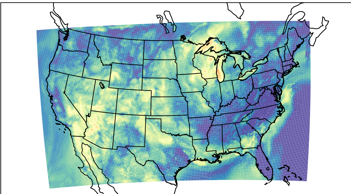
WRF (2023-06-22_11:00:00)
