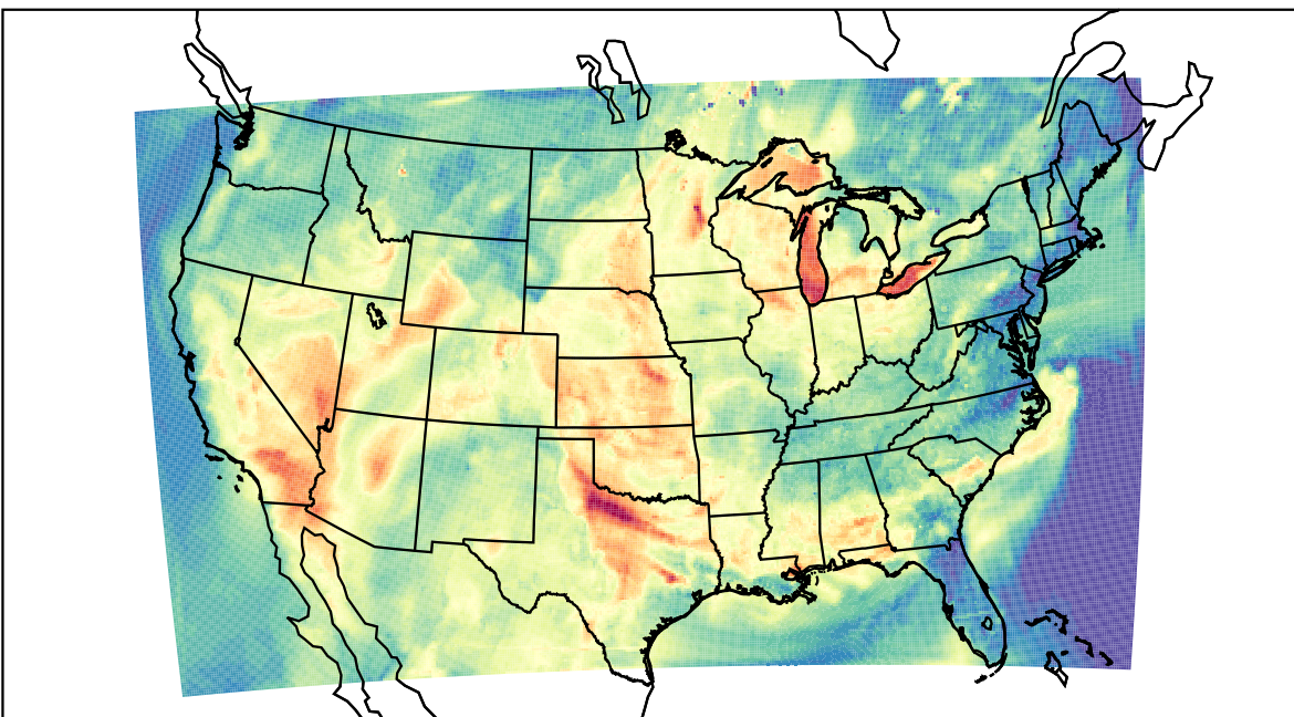
WRF (2023-06-22_01:00:00)
