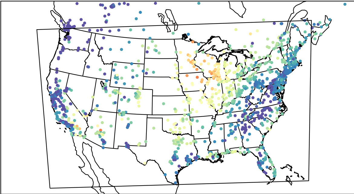
AirNOW (2023-06-22_14:00:00)
