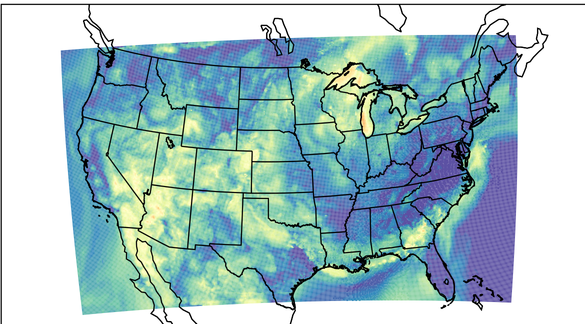
WRF (2023-06-22_12:00:00)
