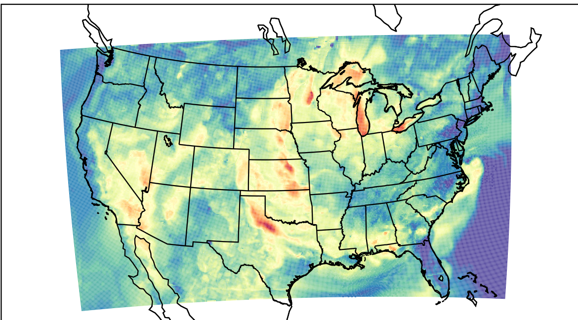
WRF (2023-06-22_03:00:00)
