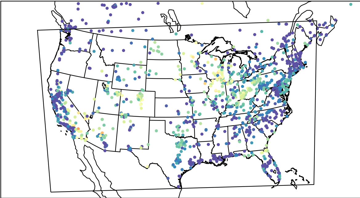
AirNOW (2023-06-22_09:00:00)
