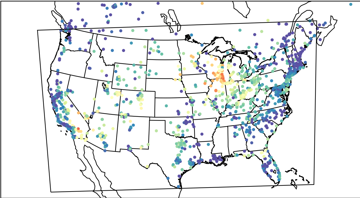
AirNOW (2023-06-22_06:00:00)
