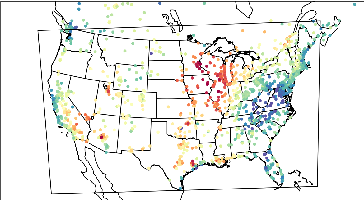
AirNOW (2023-06-22_21:00:00)
