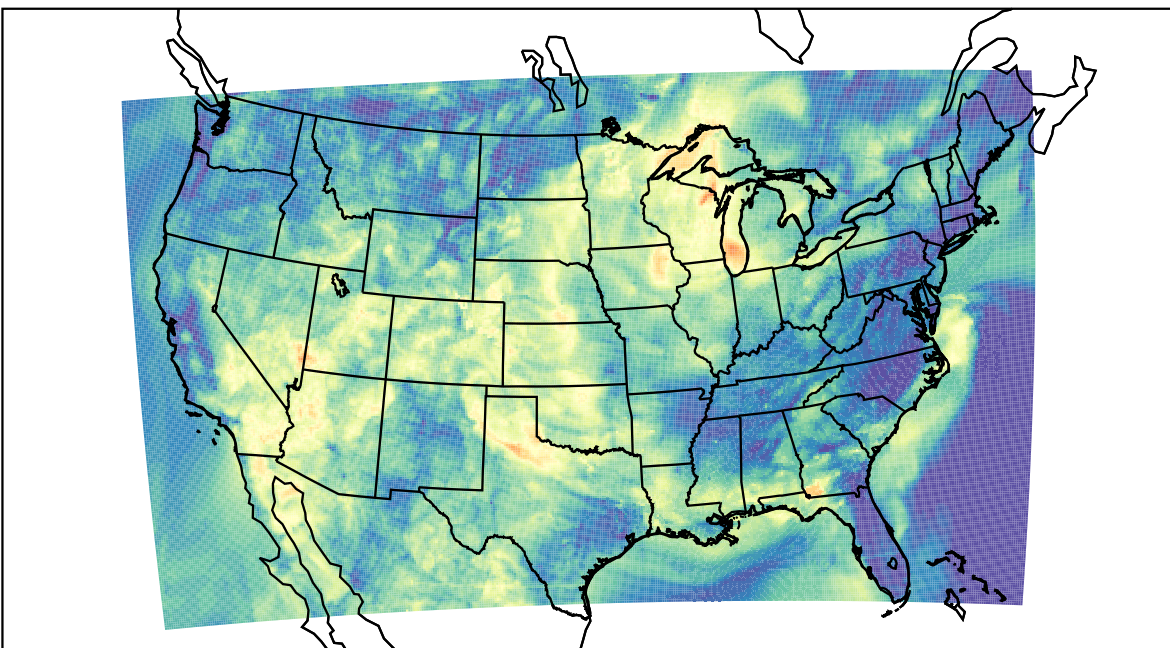
WRF (2023-06-22_07:00:00)
