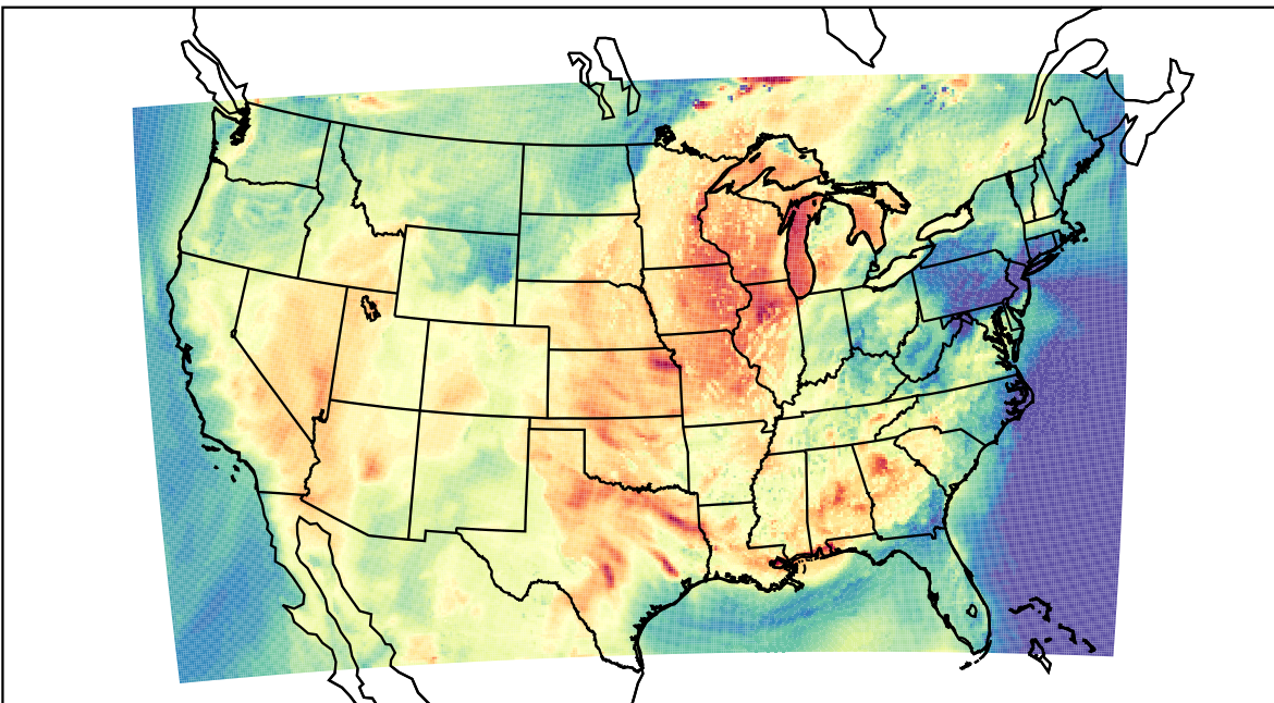
WRF (2023-06-22_23:00:00)
