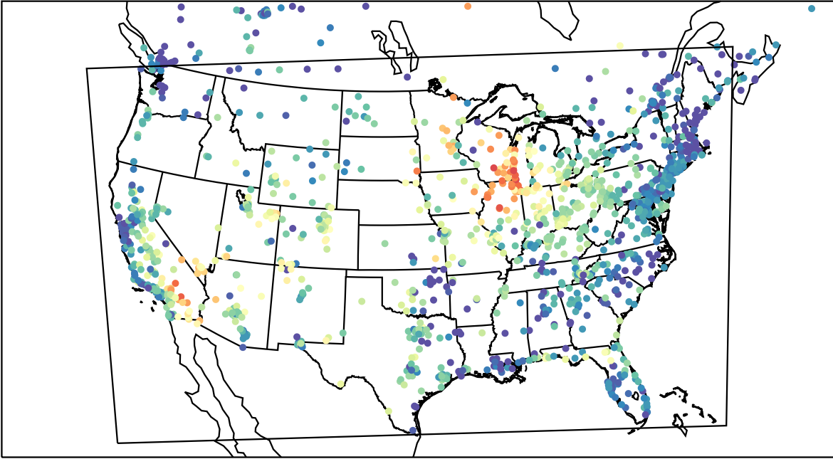
AirNOW (2023-06-22_04:00:00)
