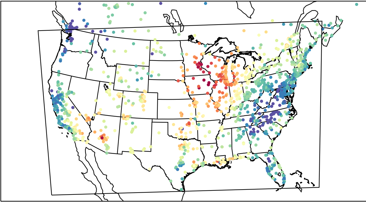
AirNOW (2023-06-22_17:00:00)
