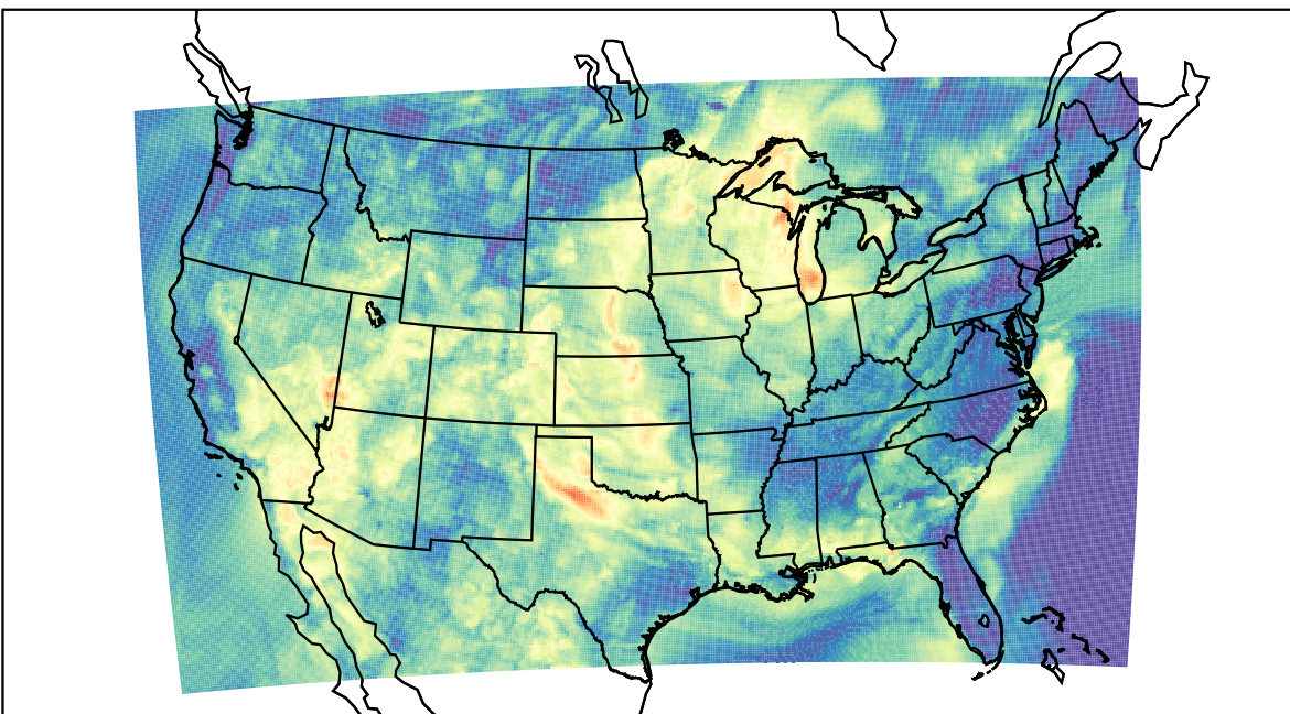
WRF (2023-06-22_06:00:00)
