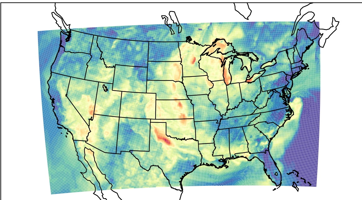
WRF (2023-06-22_04:00:00)
