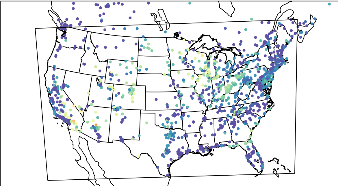
AirNOW (2023-06-22_11:00:00)
