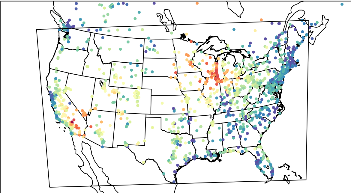
AirNOW (2023-06-22_02:00:00)
