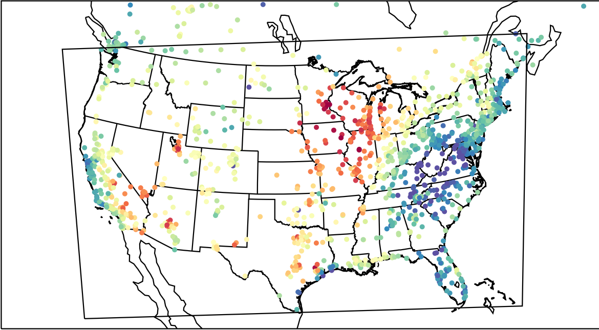
AirNOW (2023-06-22_23:00:00)
