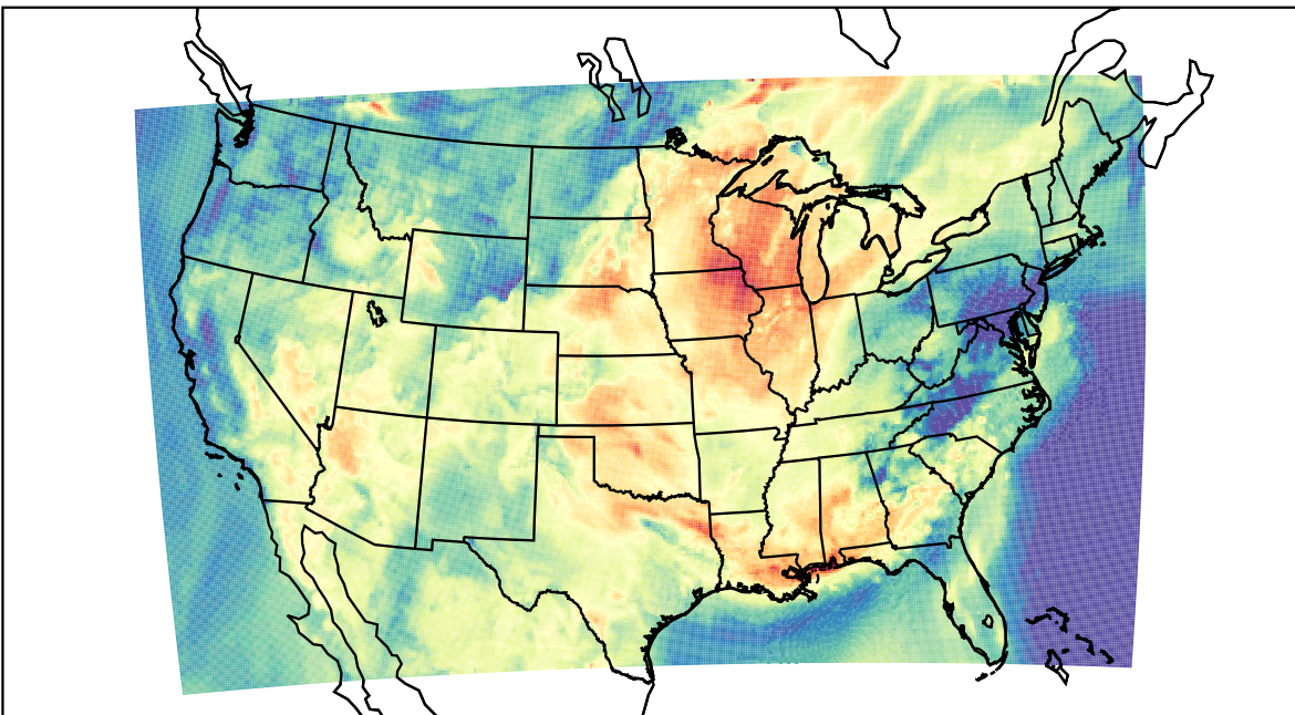
WRF (2023-06-22_16:00:00)
