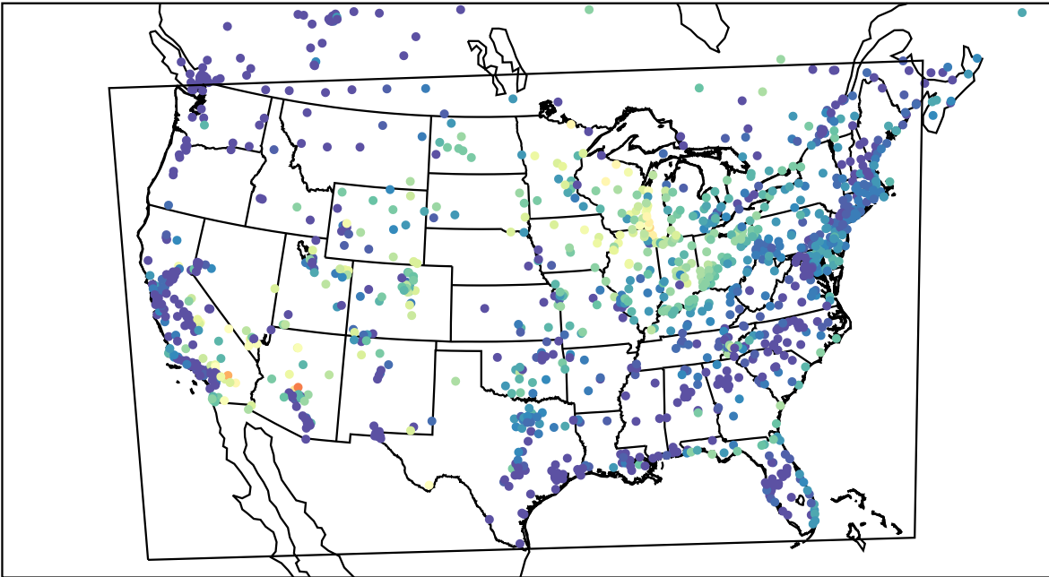
AirNOW (2023-06-22_12:00:00)
