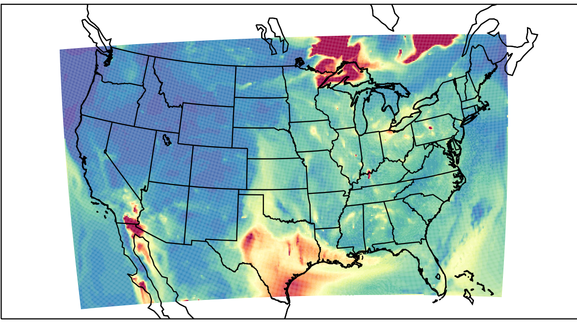
WRF 2023-06-24_10:00:00
