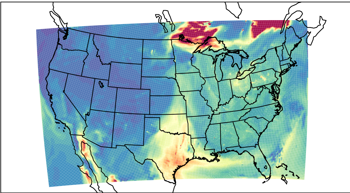
WRF 2023-06-24_17:00:00
