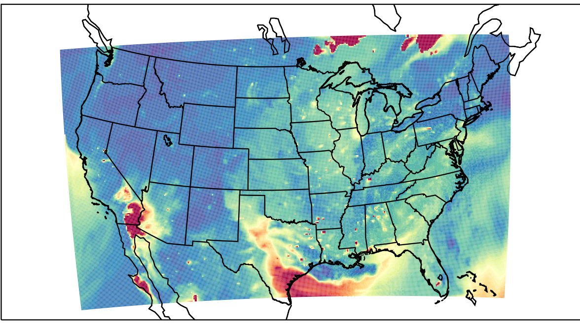
WRF 2023-06-23_02:00:00
