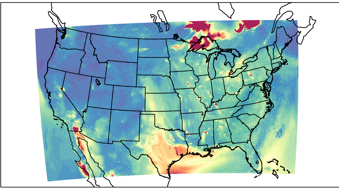
WRF 2023-06-24_05:00:00
