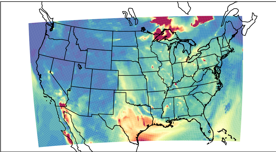
WRF 2023-06-24_06:00:00
