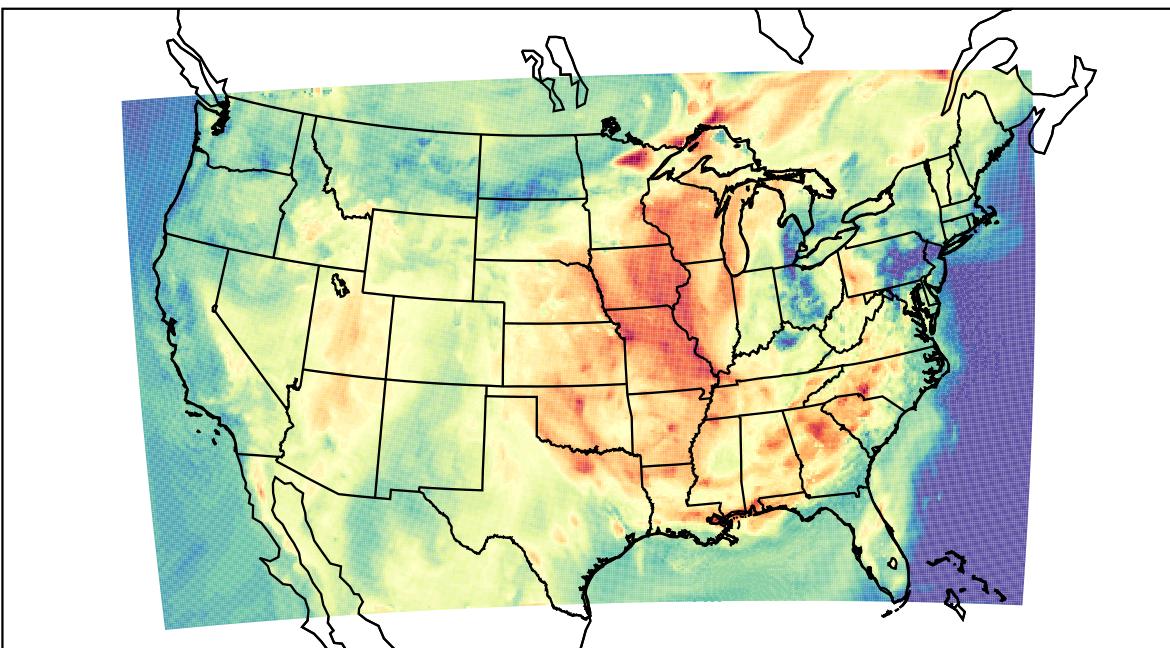
WRF (2023-06-23_17:00:00)
