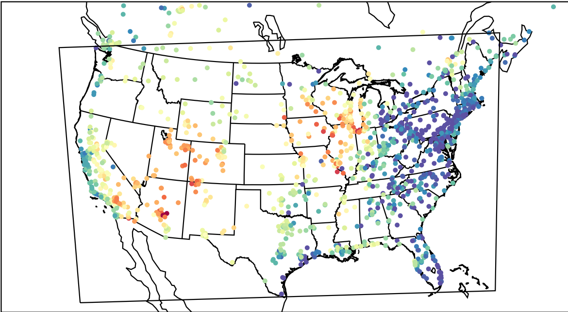
AirNOW (2023-06-24_01:00:00)
