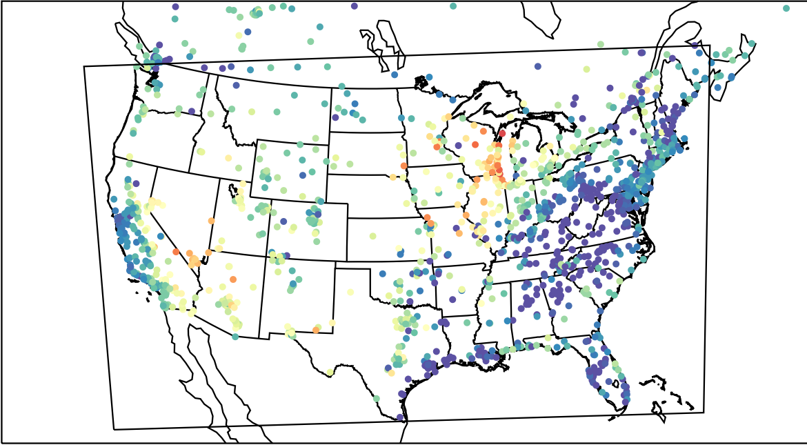
AirNOW (2023-06-23_03:00:00)
