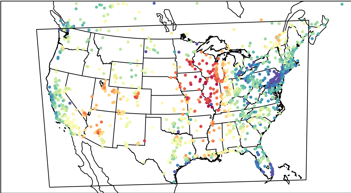
AirNOW (2023-06-23_20:00:00)
