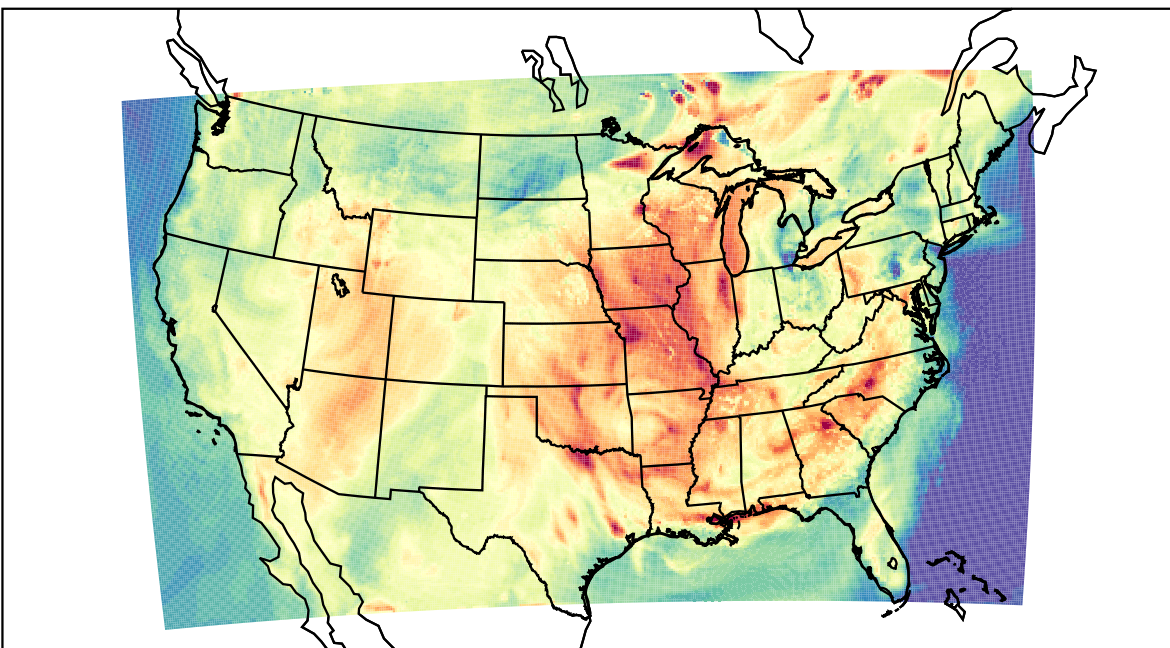
WRF (2023-06-23_20:00:00)
