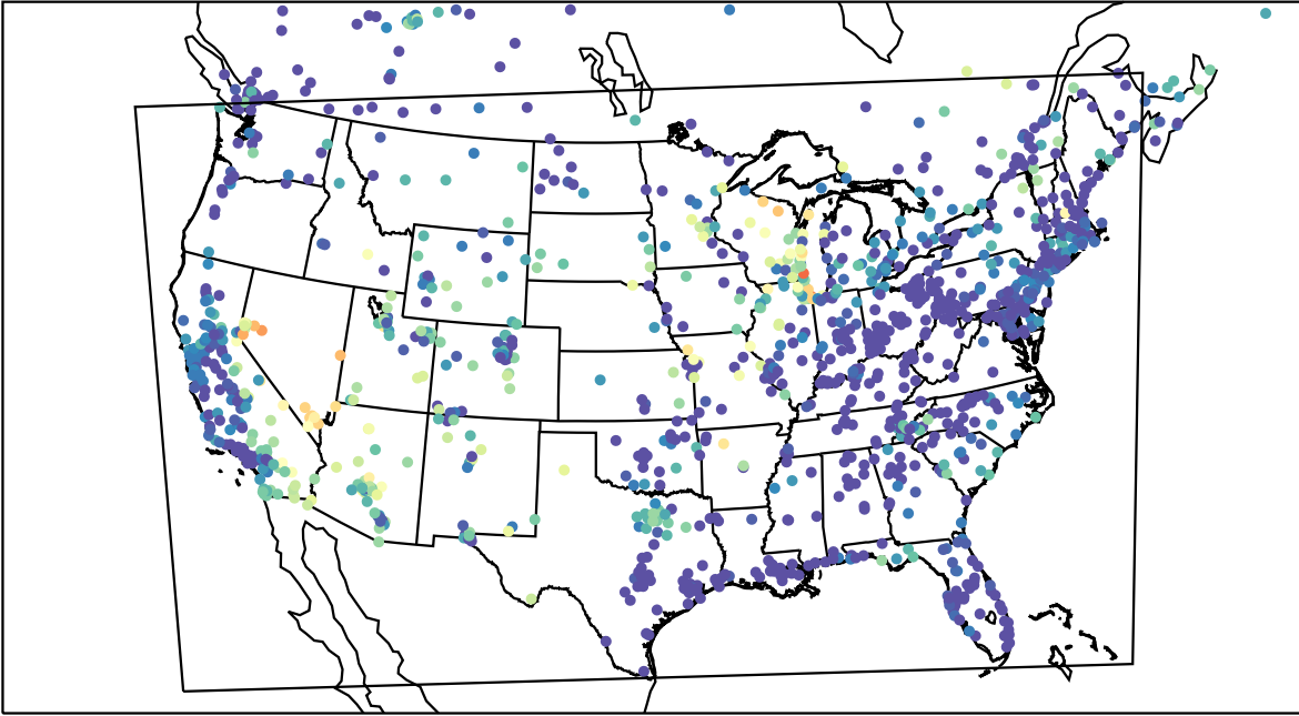
AirNOW (2023-06-23_09:00:00)
