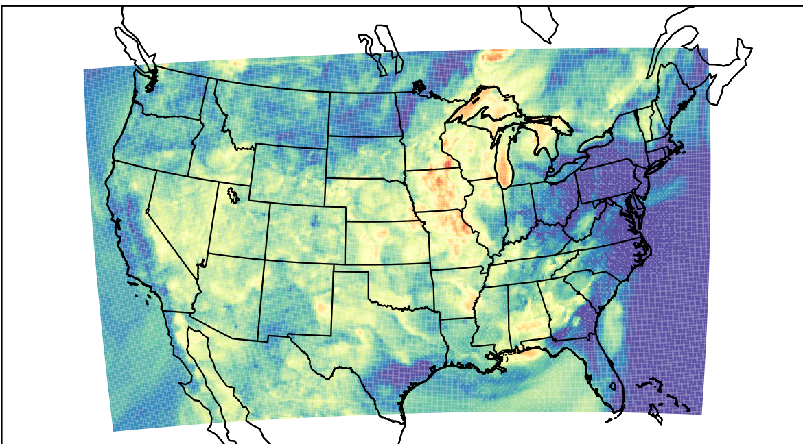
WRF (2023-06-23_06:00:00)
