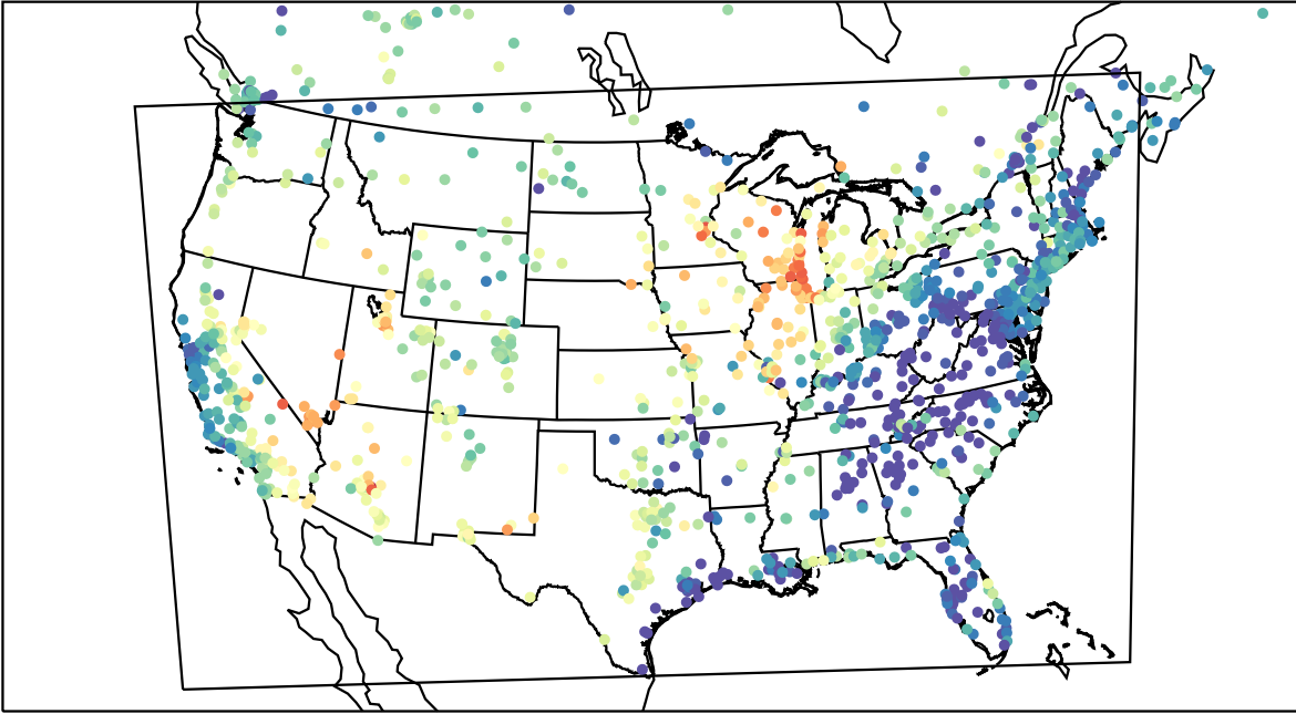
AirNOW (2023-06-23_02:00:00)
