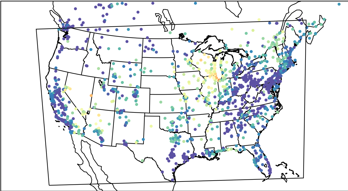
AirNOW (2023-06-23_13:00:00)
