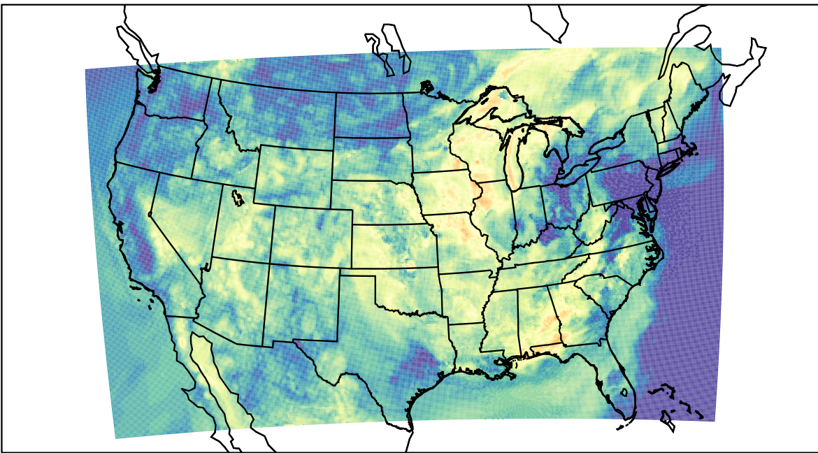
WRF (2023-06-23_14:00:00)
