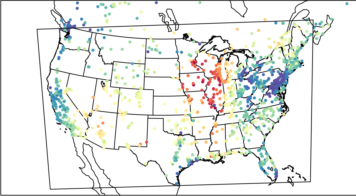
AirNOW (2023-06-23_17:00:00)
