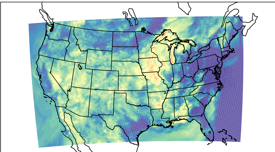
WRF (2023-06-23_10:00:00)
