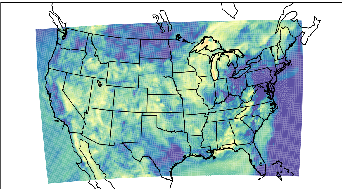
WRF (2023-06-23_13:00:00)
