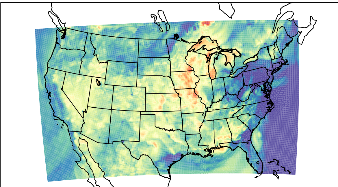
WRF (2023-06-23_04:00:00)
