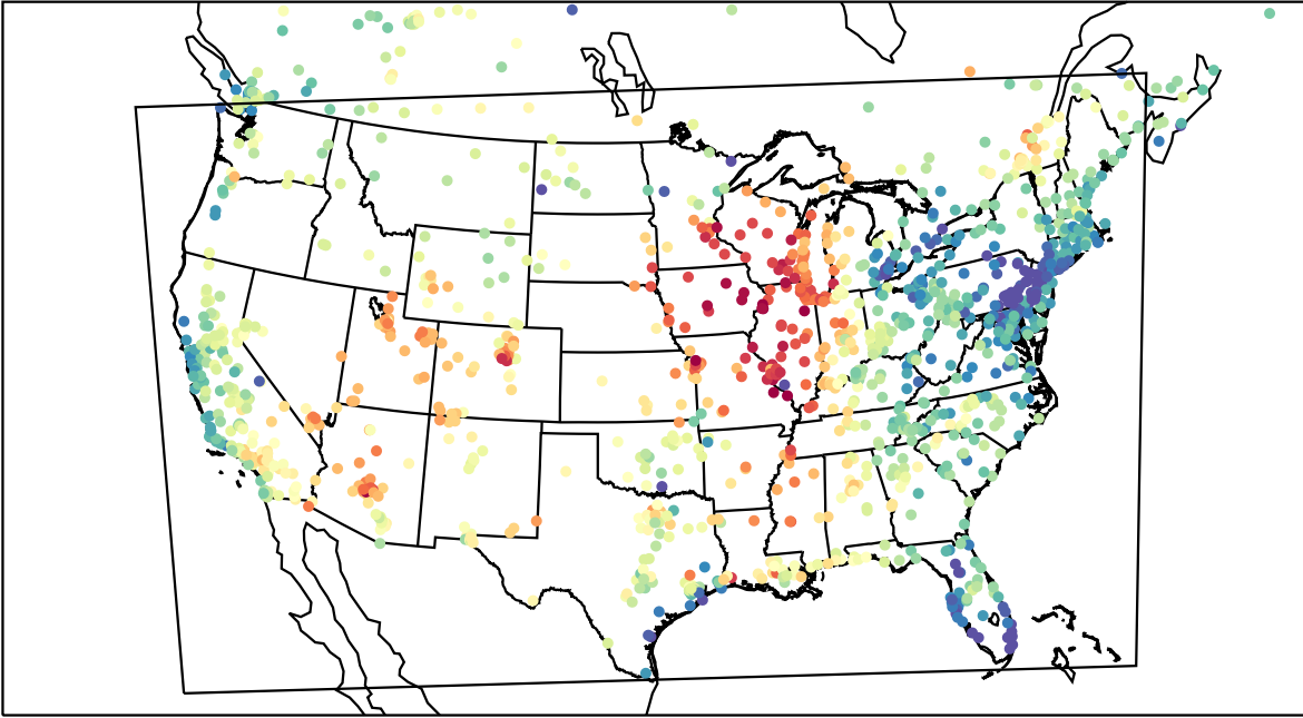
AirNOW (2023-06-23_21:00:00)
