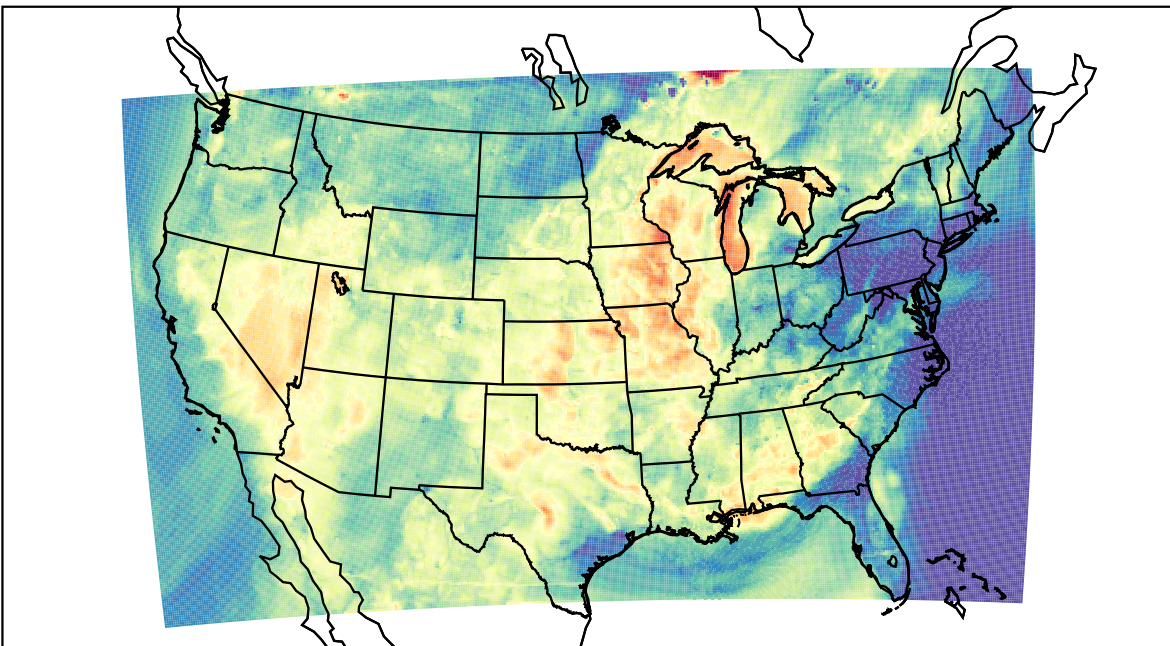
WRF (2023-06-23_02:00:00)
