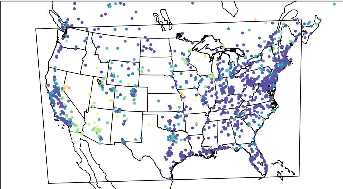
AirNOW (2023-06-23_10:00:00)
