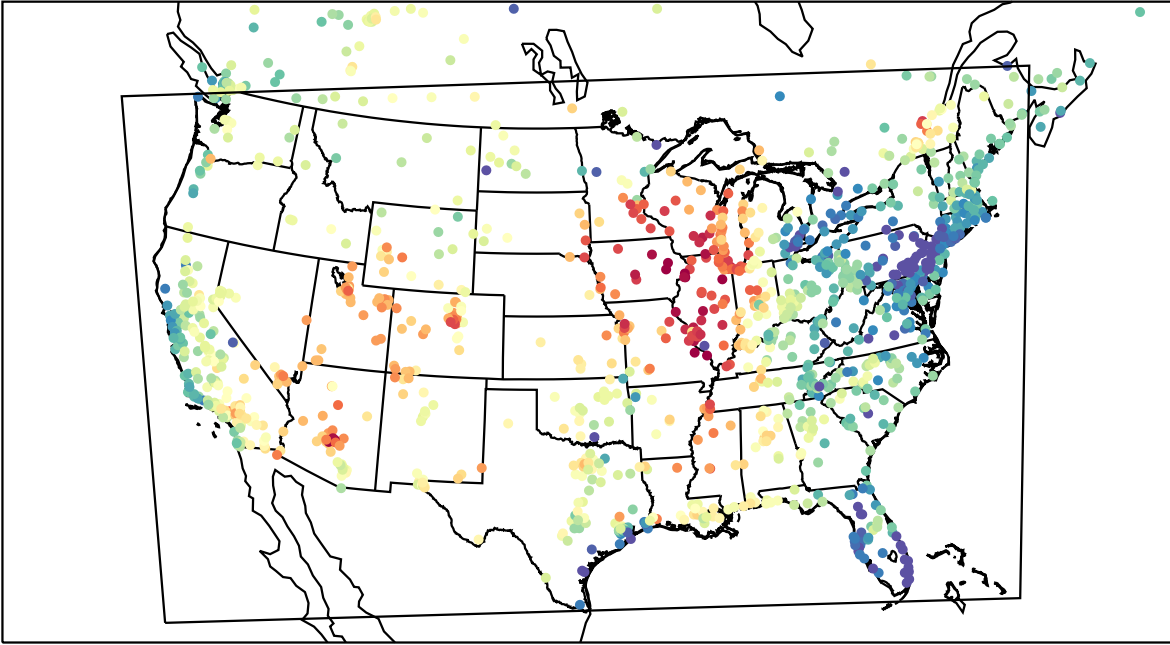
AirNOW (2023-06-23_22:00:00)
