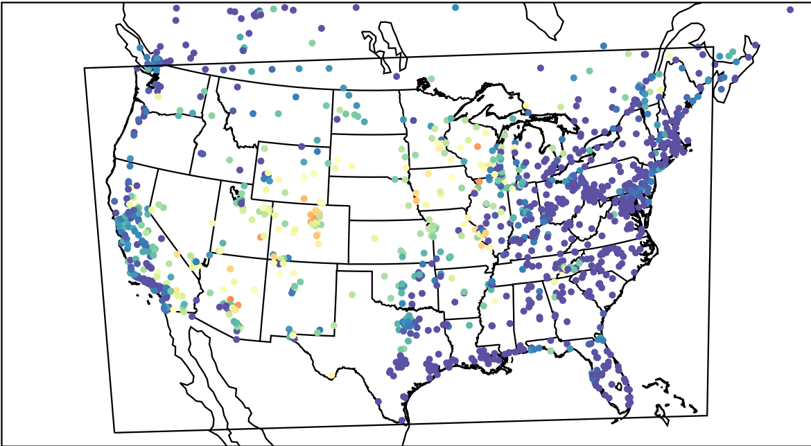
AirNOW (2023-06-24_07:00:00)
