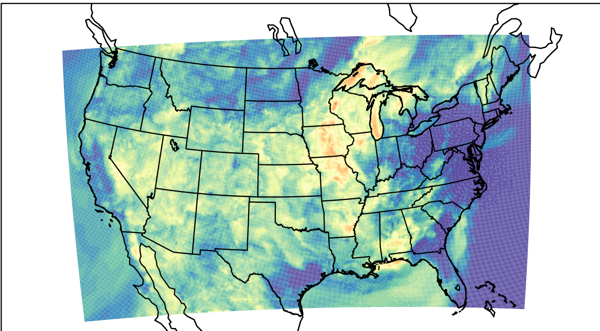
WRF (2023-06-23_08:00:00)
