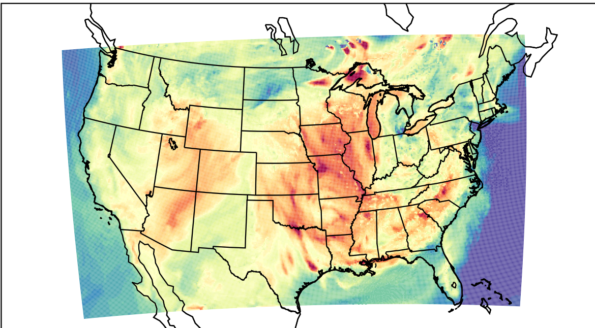
WRF (2023-06-23_22:00:00)
