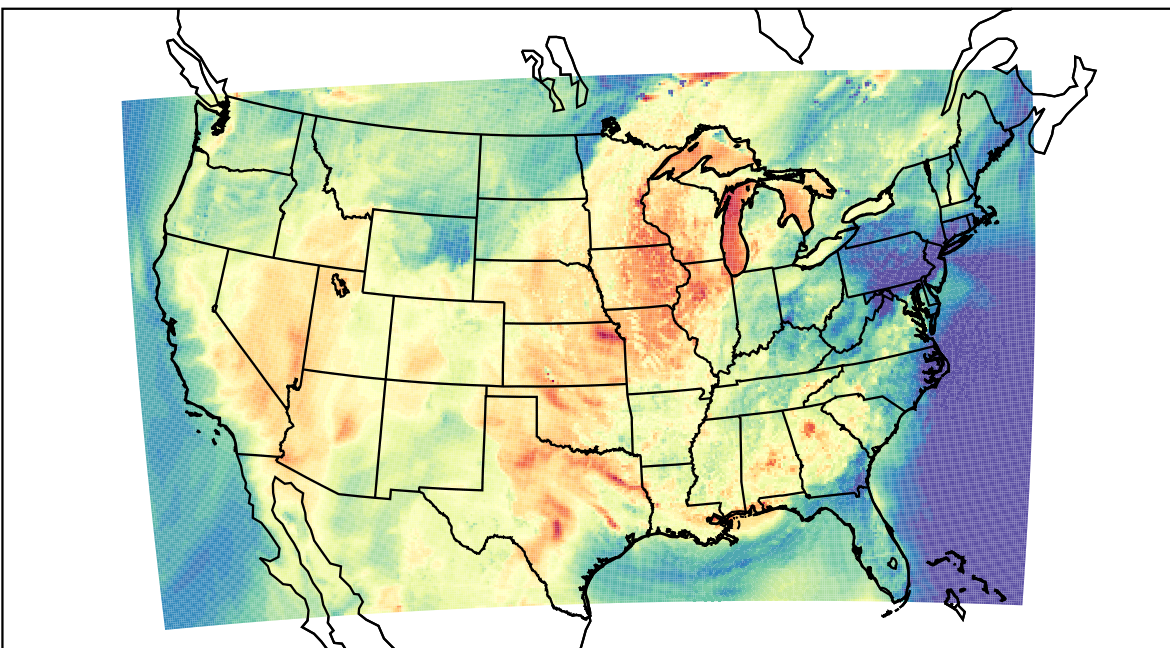
WRF (2023-06-23_00:00:00)
