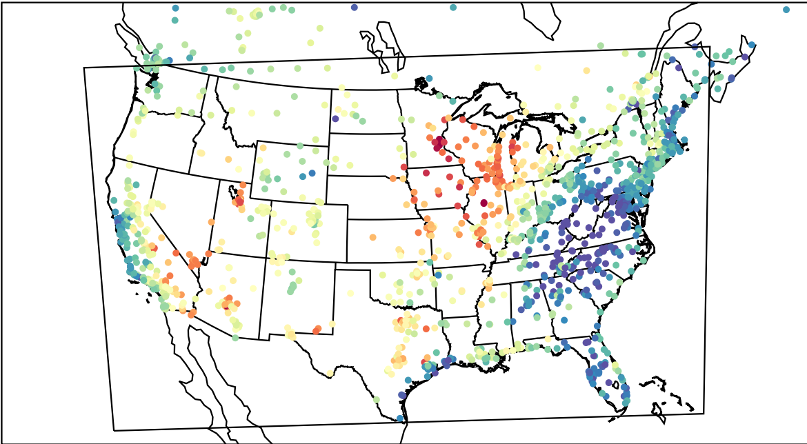
AirNOW (2023-06-23_00:00:00)
