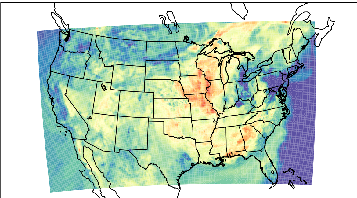
WRF (2023-06-23_15:00:00)
