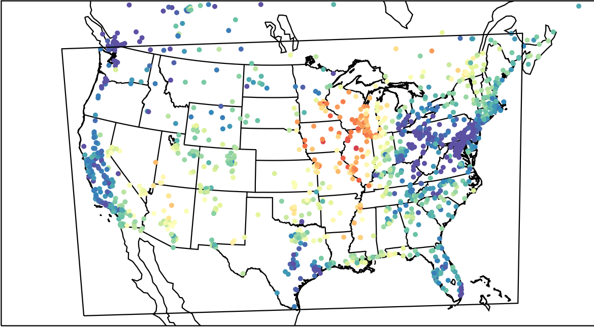
AirNOW (2023-06-23_15:00:00)
