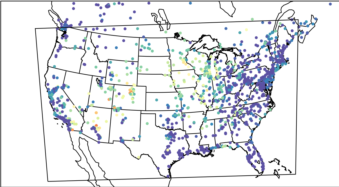
AirNOW (2023-06-24_12:00:00)
