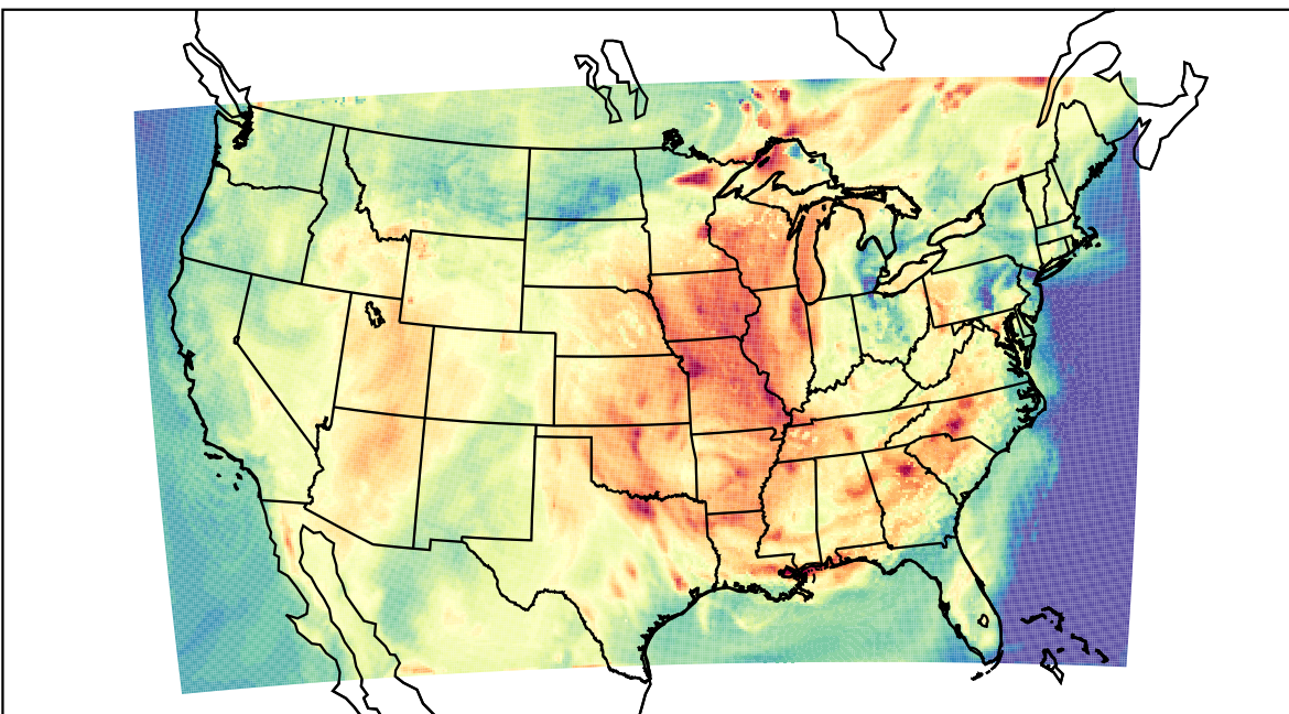
WRF (2023-06-23_19:00:00)
