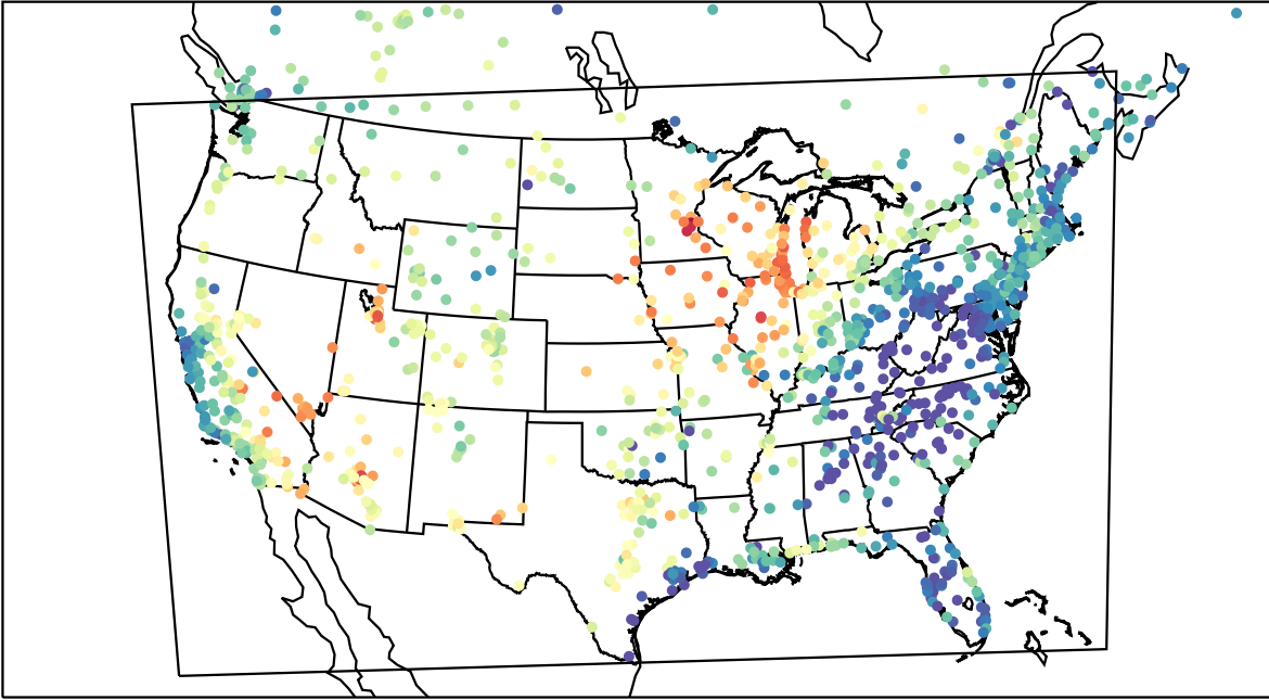
AirNOW (2023-06-23_01:00:00)
