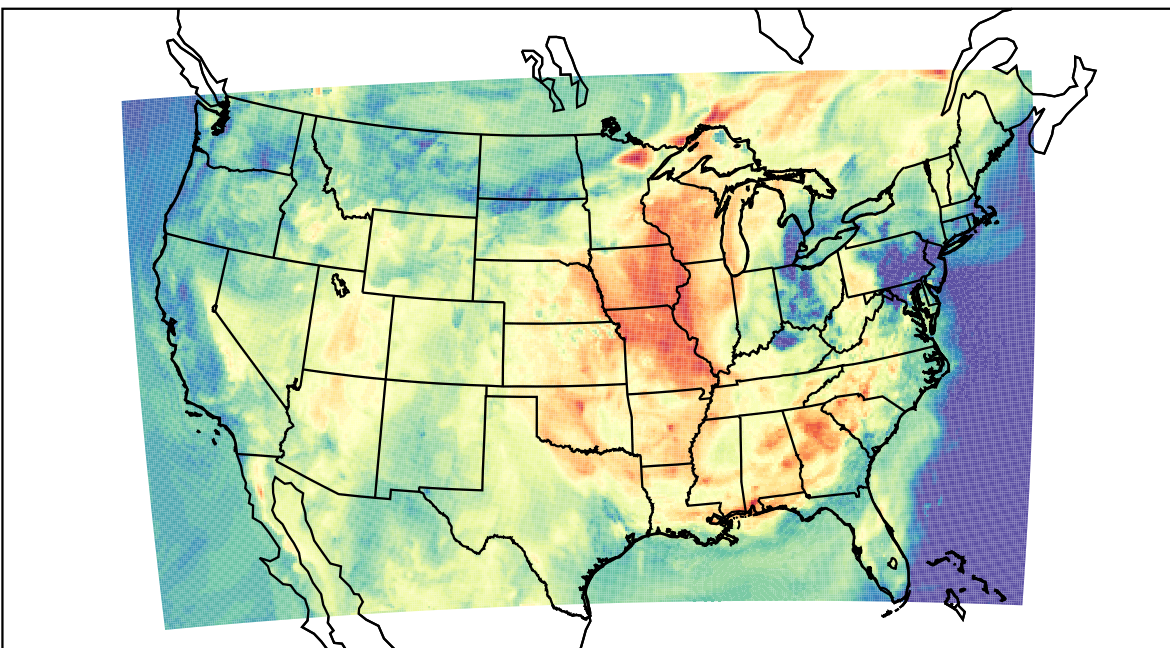
WRF (2023-06-23_16:00:00)
