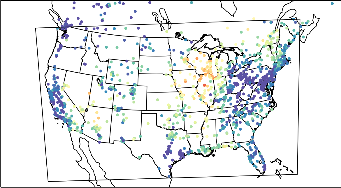
AirNOW (2023-06-23_14:00:00)
