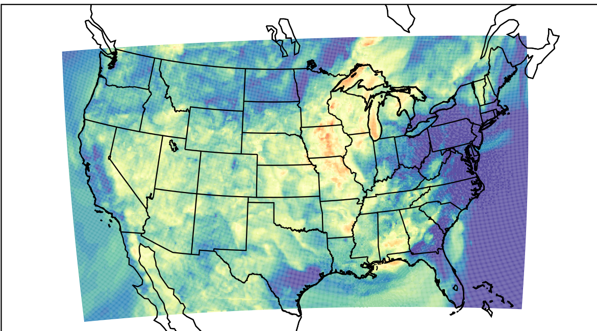
WRF (2023-06-23_07:00:00)
