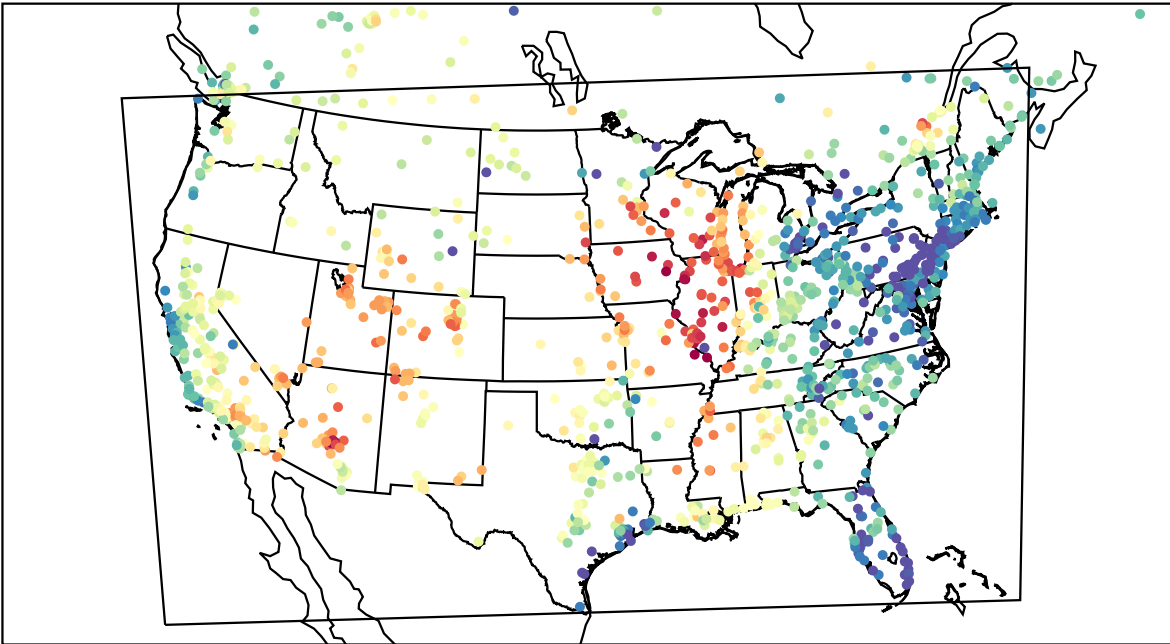
AirNOW (2023-06-23_23:00:00)
