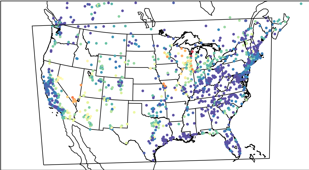
AirNOW (2023-06-23_06:00:00)
