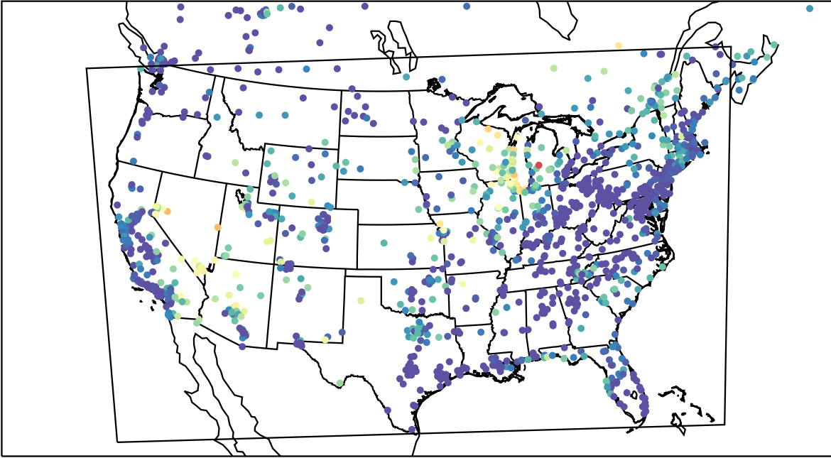
AirNOW (2023-06-23_12:00:00)
