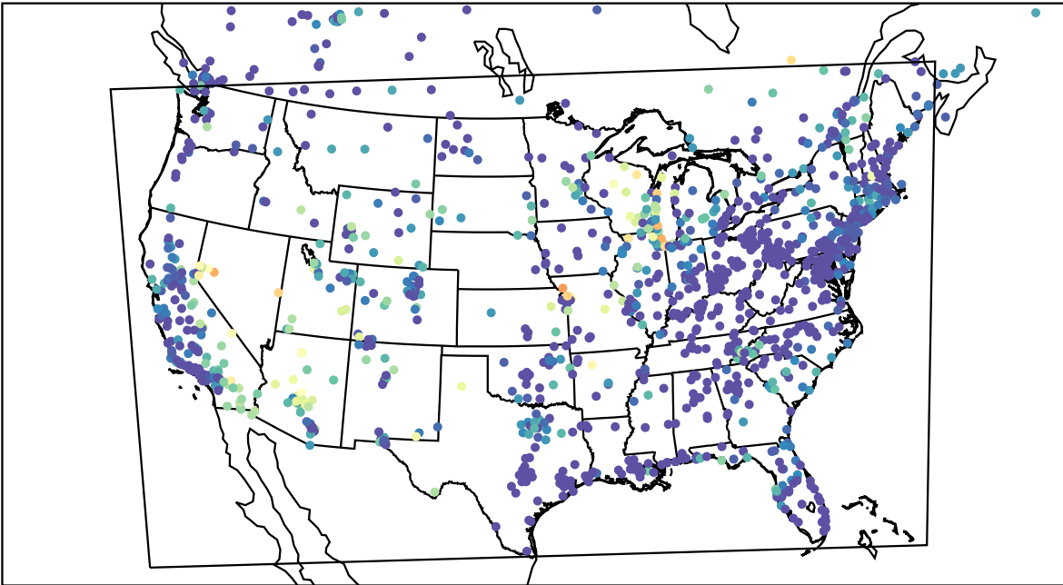
AirNOW (2023-06-23_11:00:00)
