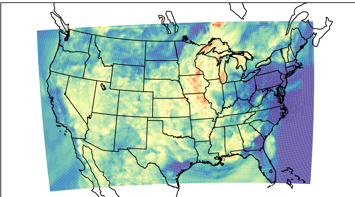
WRF (2023-06-23_05:00:00)
