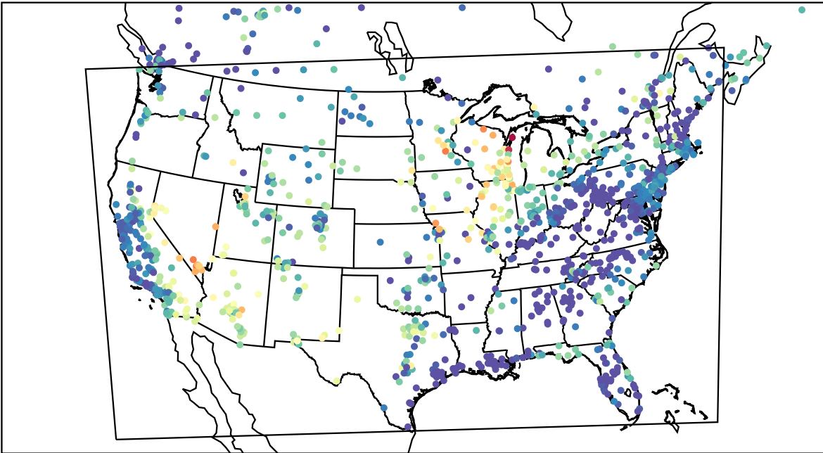
AirNOW (2023-06-23_05:00:00)
