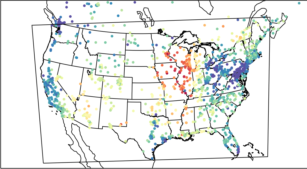
AirNOW (2023-06-23_16:00:00)
