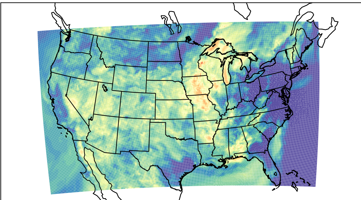
WRF (2023-06-23_09:00:00)
