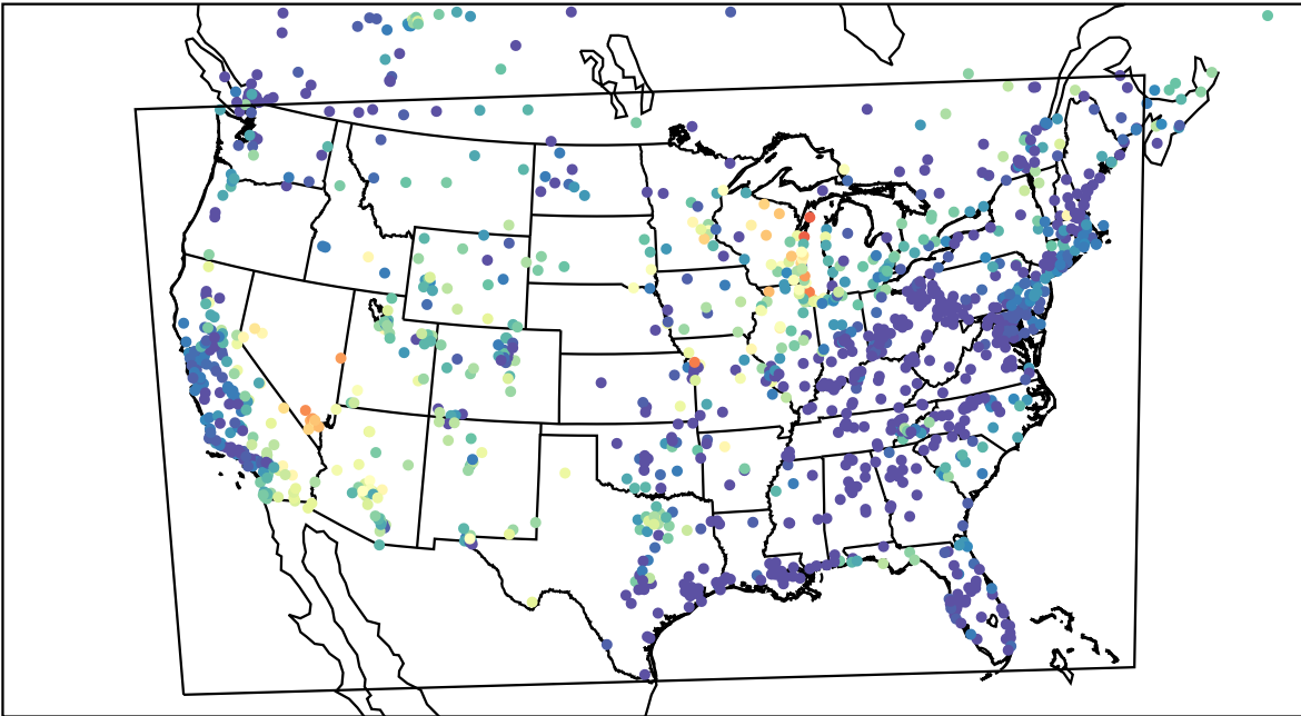
AirNOW (2023-06-23_07:00:00)
