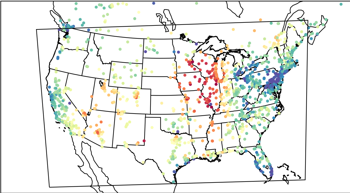
AirNOW (2023-06-23_19:00:00)
