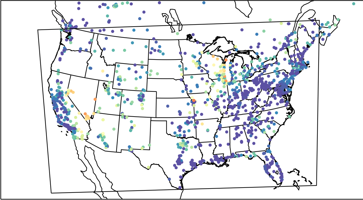
AirNOW (2023-06-23_08:00:00)
