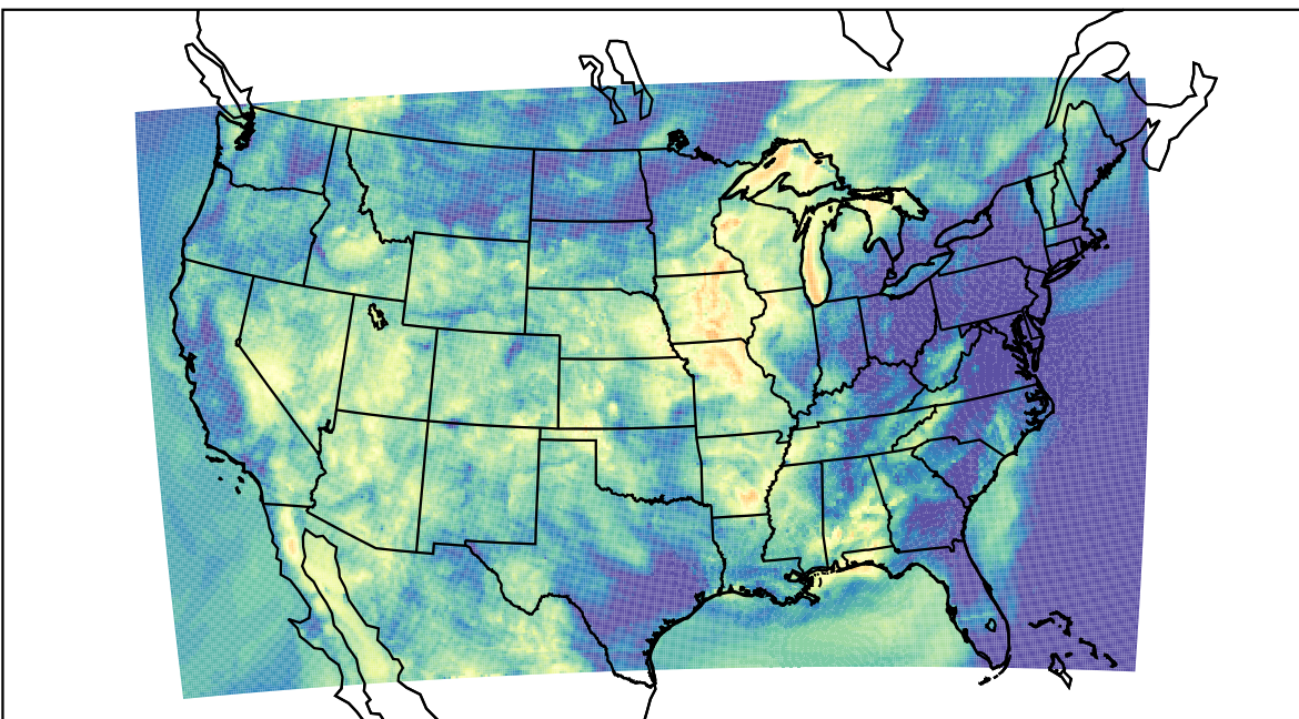
WRF (2023-06-23_11:00:00)
