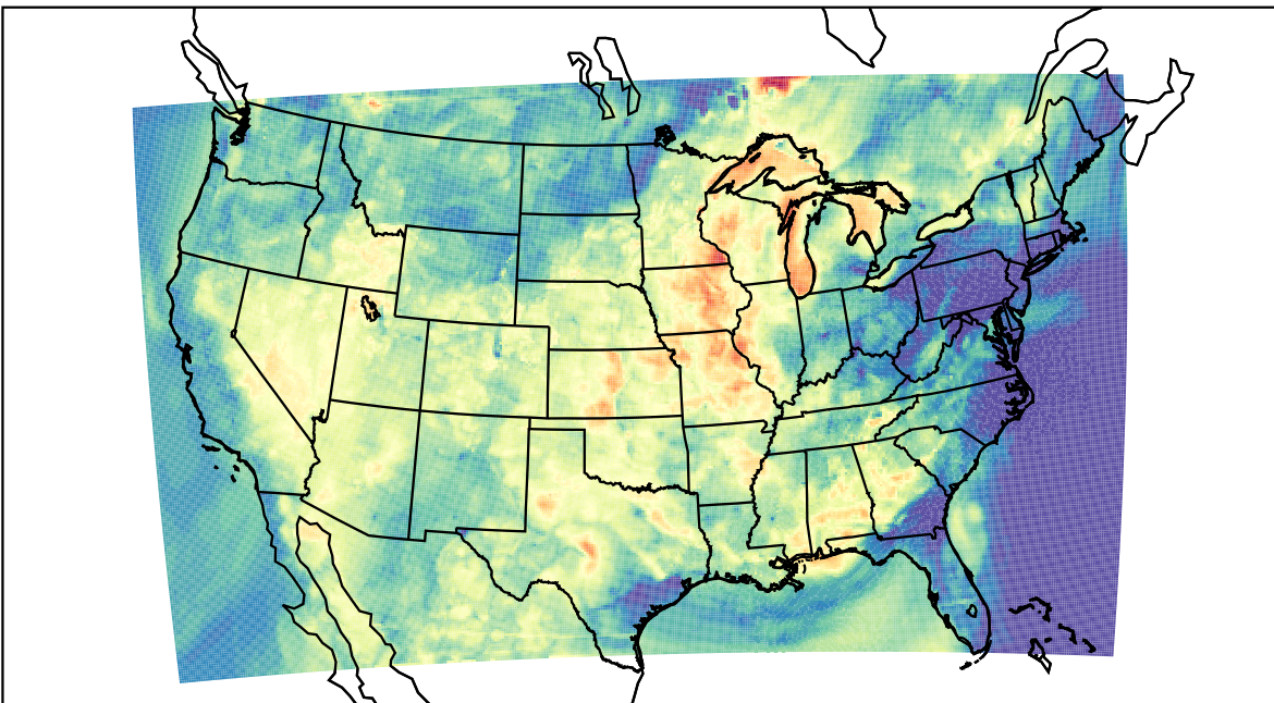
WRF (2023-06-23_03:00:00)
