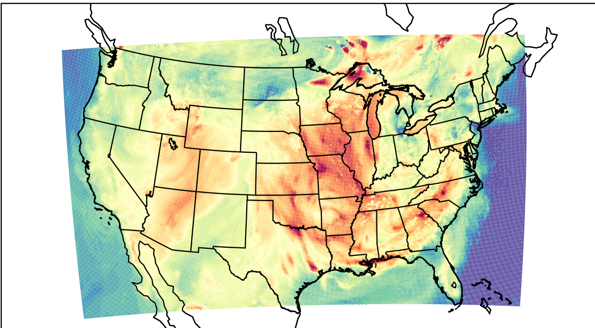
WRF (2023-06-23_21:00:00)
