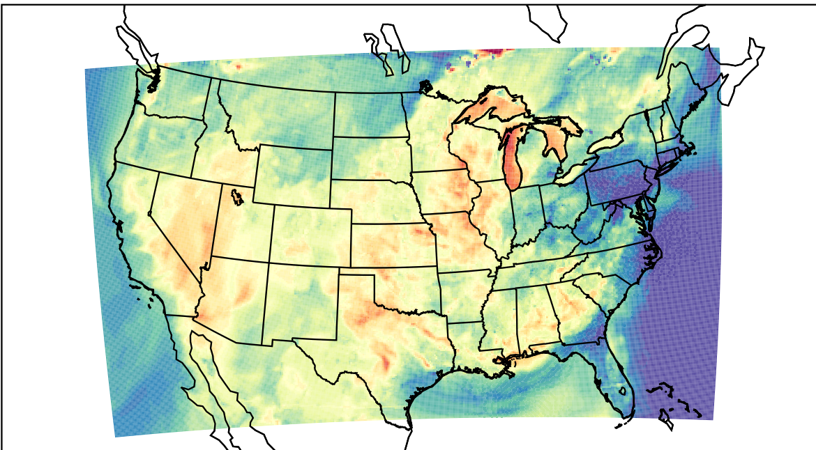
WRF (2023-06-23_01:00:00)
