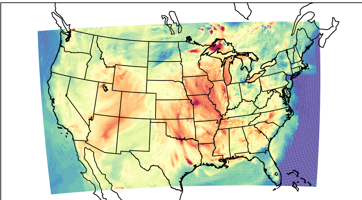
WRF (2023-06-23_23:00:00)
