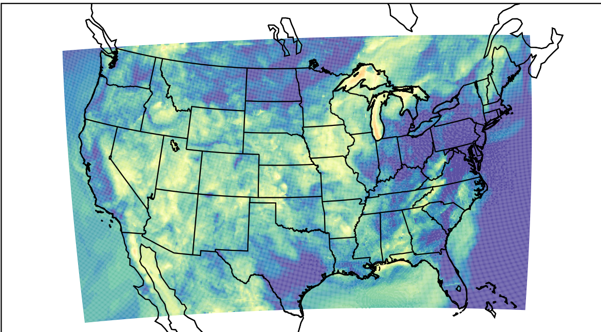
WRF (2023-06-23_12:00:00)
