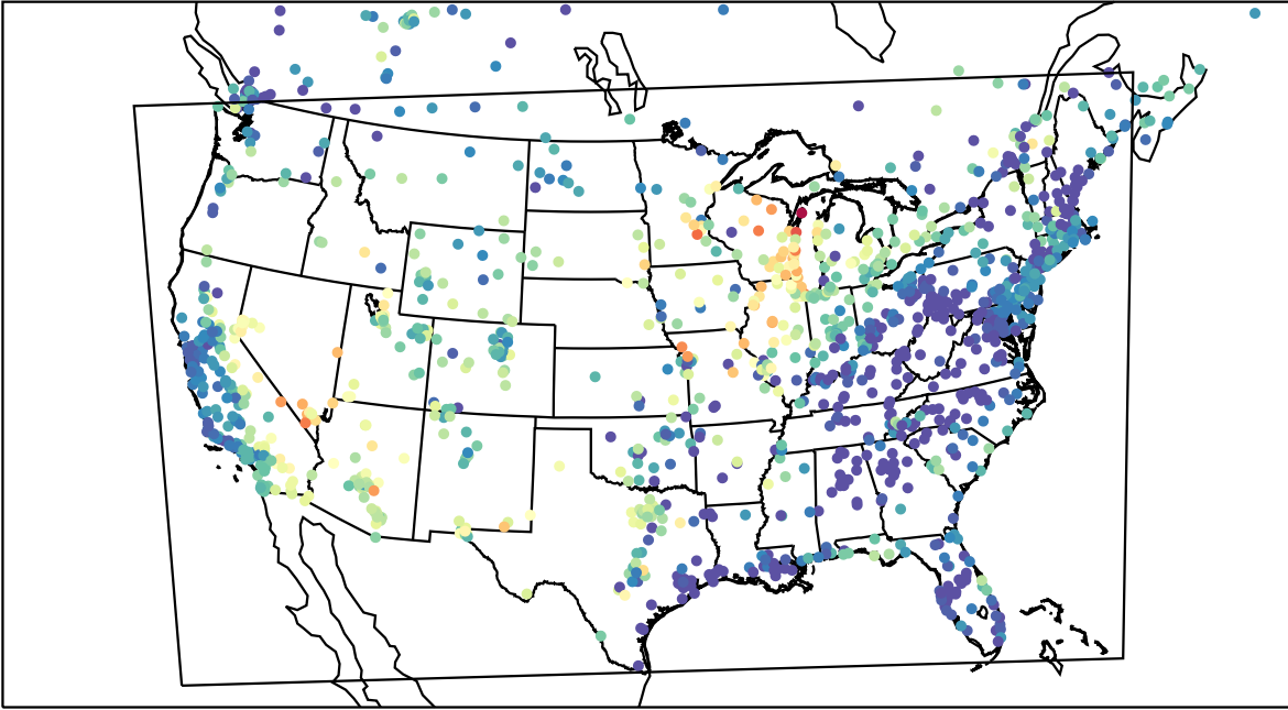
AirNOW (2023-06-23_04:00:00)
