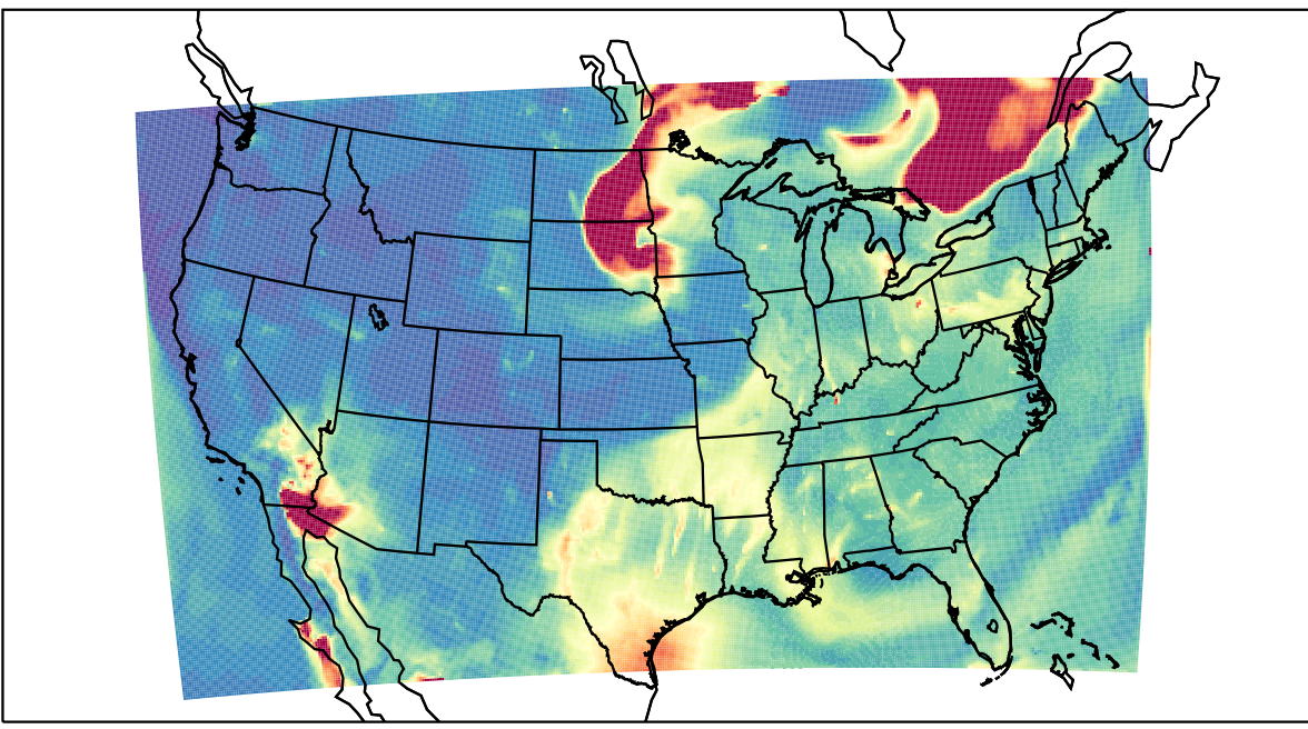
WRF 2023-06-25_09:00:00
