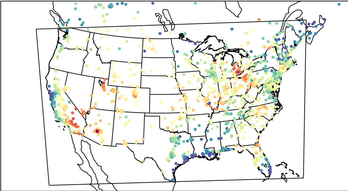
AirNOW (2023-06-25_22:00:00)
