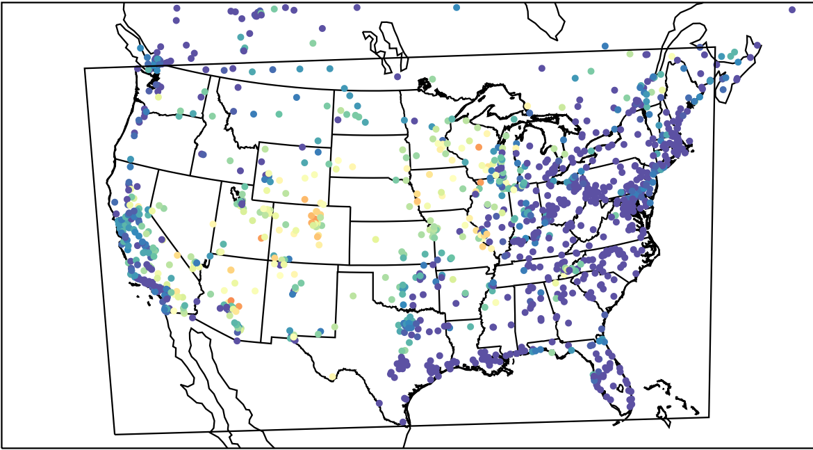
AirNOW (2023-06-24_07:00:00)
