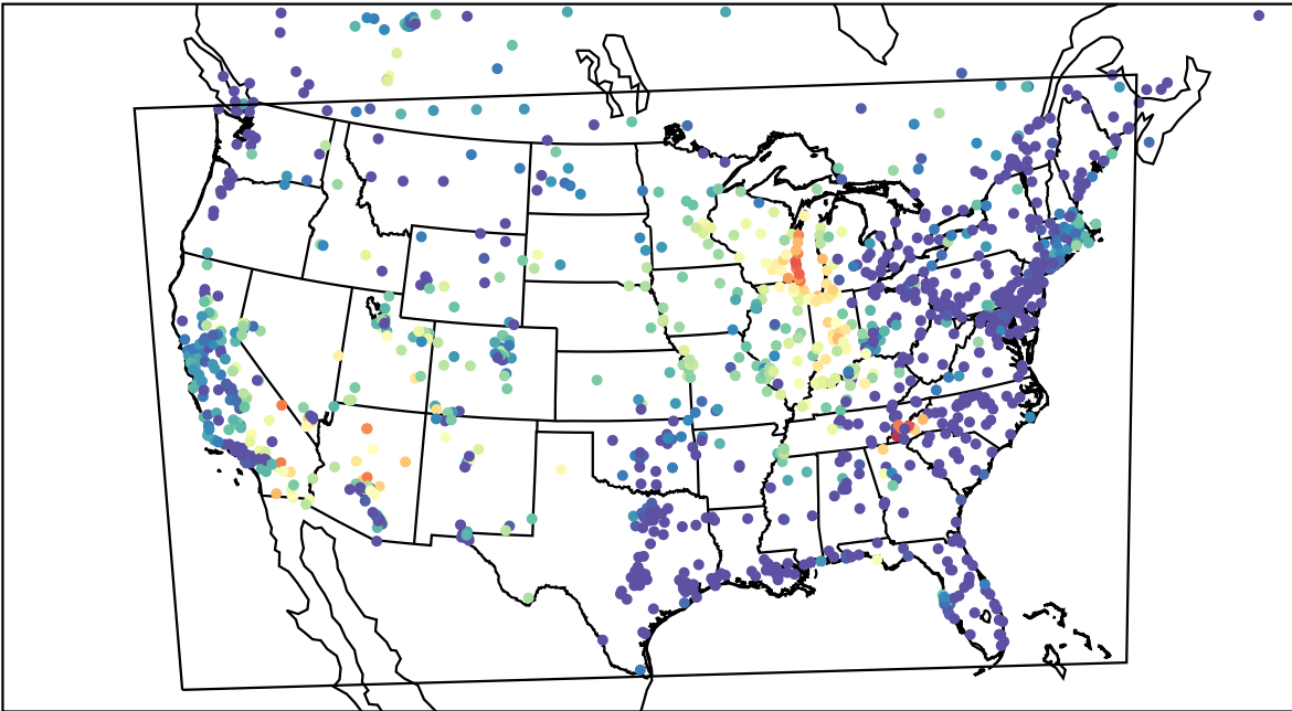
AirNOW (2023-06-25_09:00:00)
