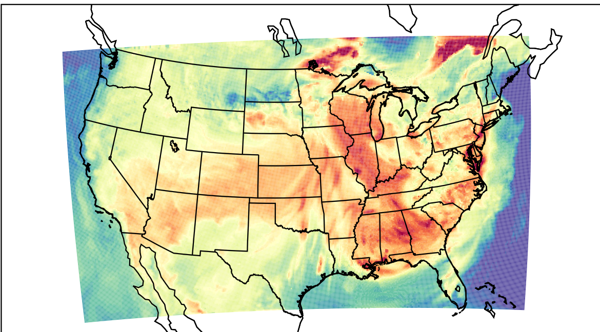
WRF (2023-06-24_19:00:00)
