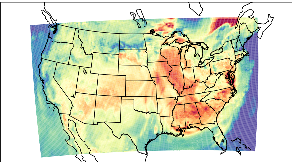
WRF (2023-06-24_17:00:00)
