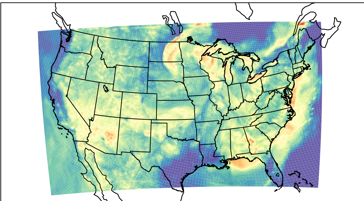
WRF (2023-06-25_06:00:00)
