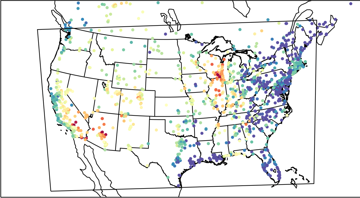
AirNOW (2023-06-25_02:00:00)
