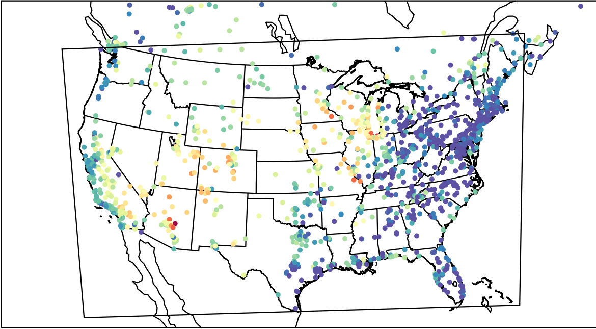
AirNOW (2023-06-24_03:00:00)
