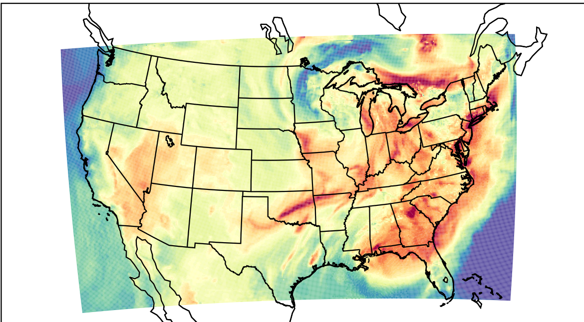
WRF (2023-06-25_19:00:00)
