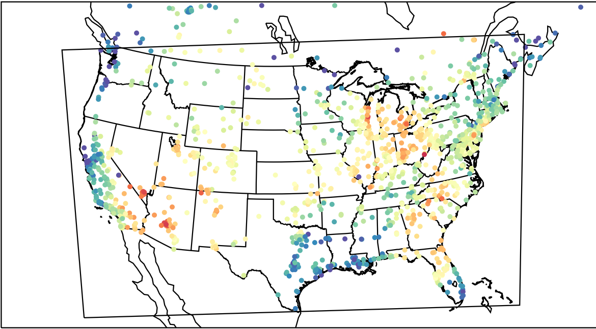
AirNOW (2023-06-25_17:00:00)
