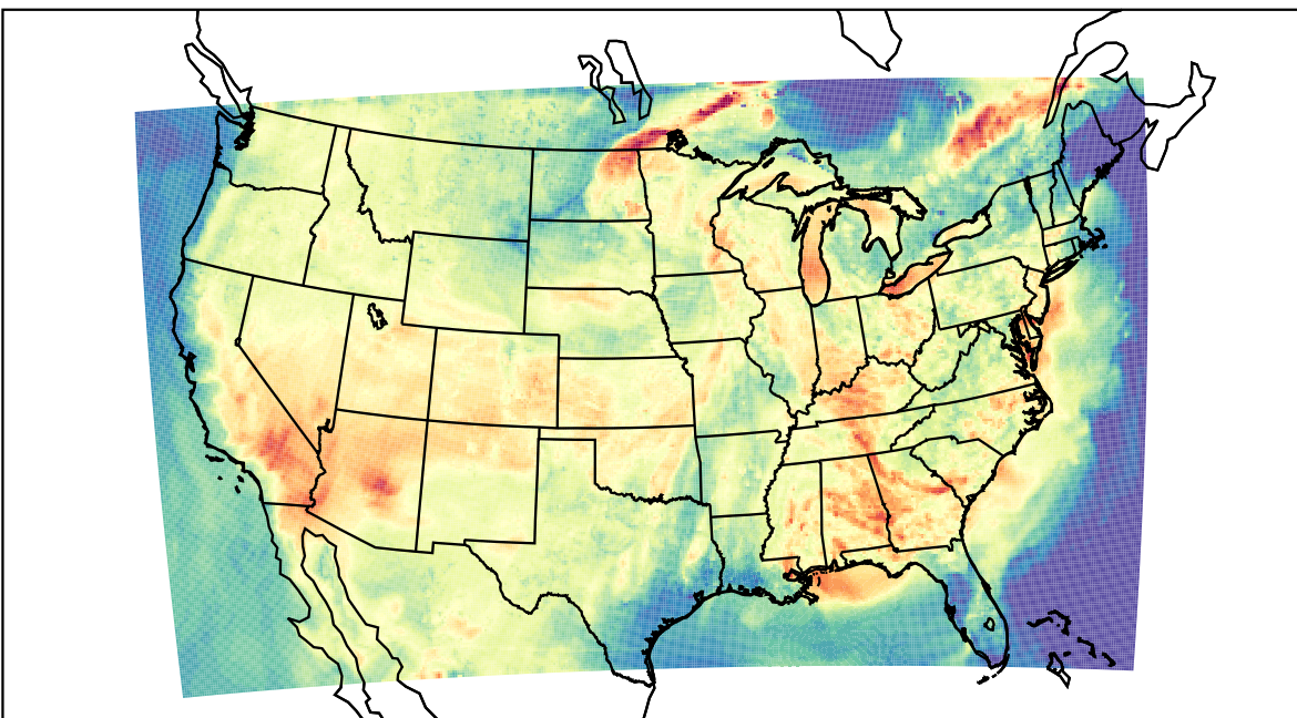
WRF (2023-06-25_01:00:00)
