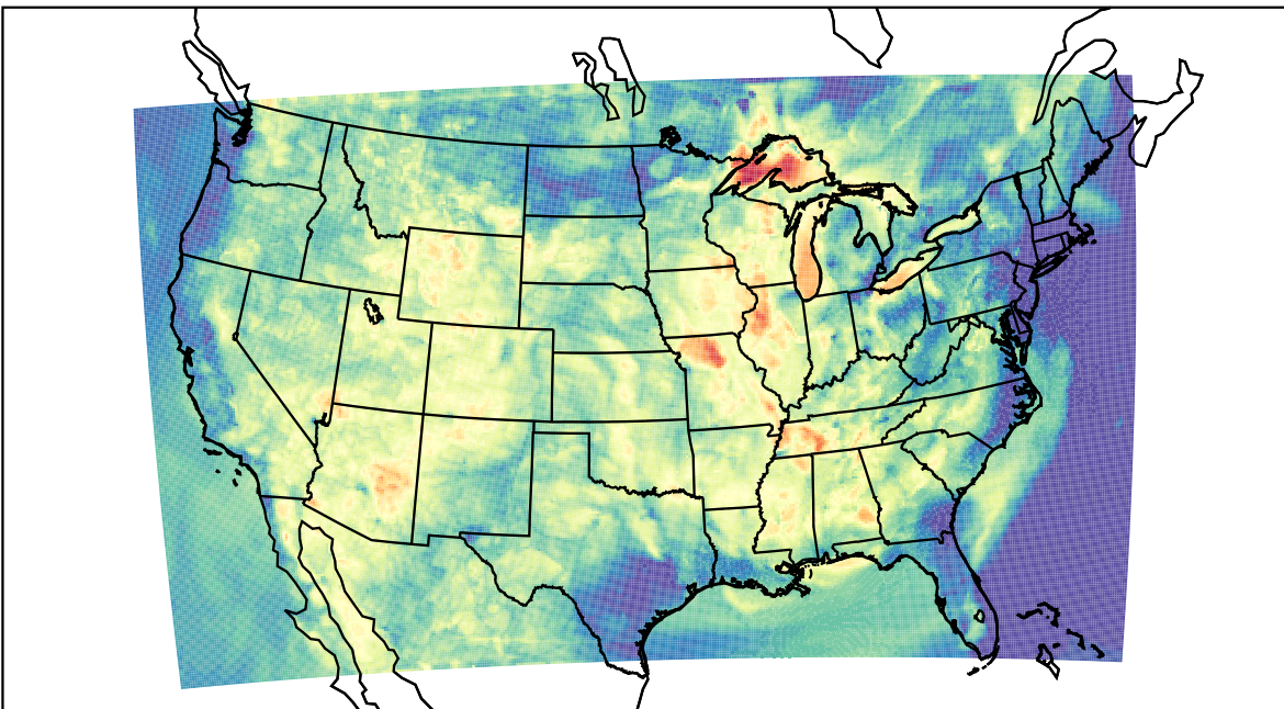
WRF (2023-06-24_05:00:00)
