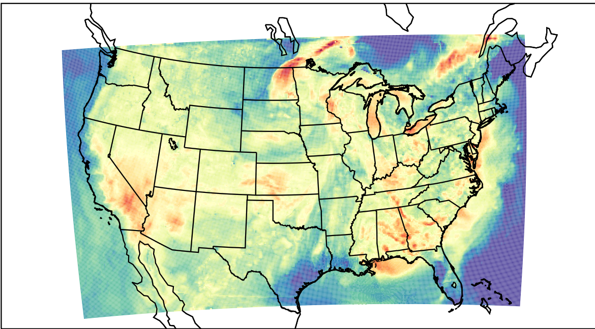
WRF (2023-06-25_02:00:00)
