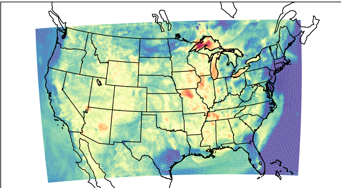
WRF (2023-06-24_04:00:00)
