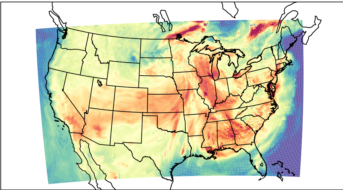
WRF (2023-06-24_22:00:00)
