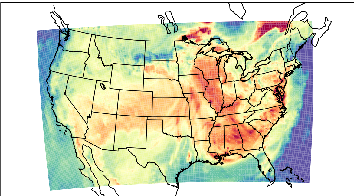
WRF (2023-06-24_18:00:00)
