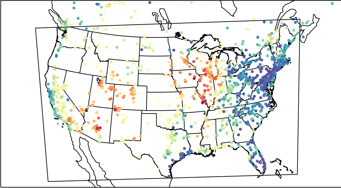
AirNOW (2023-06-24_00:00:00)
