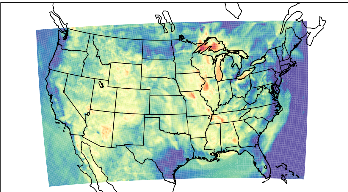
WRF (2023-06-24_06:00:00)
