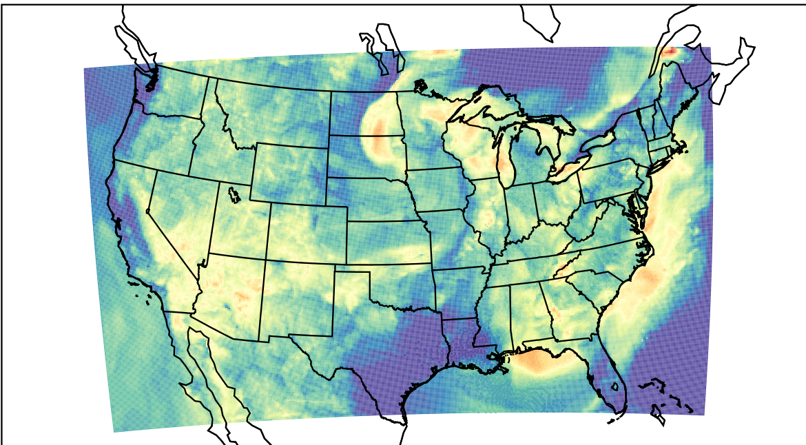
WRF (2023-06-25_08:00:00)
