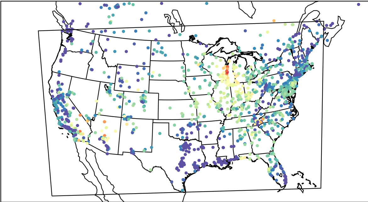
AirNOW (2023-06-25_13:00:00)
