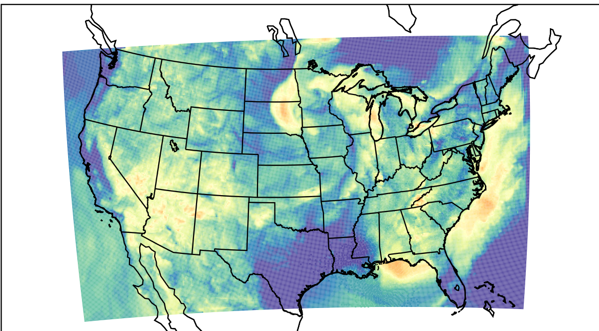
WRF (2023-06-25_10:00:00)
