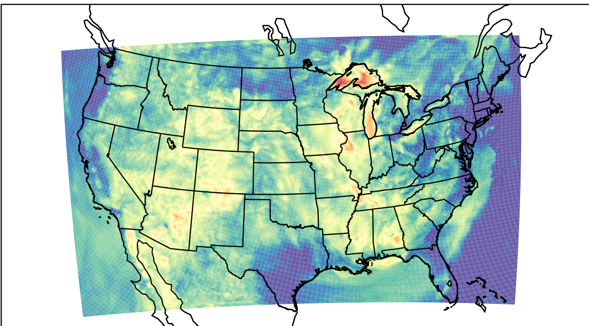
WRF (2023-06-24_08:00:00)
