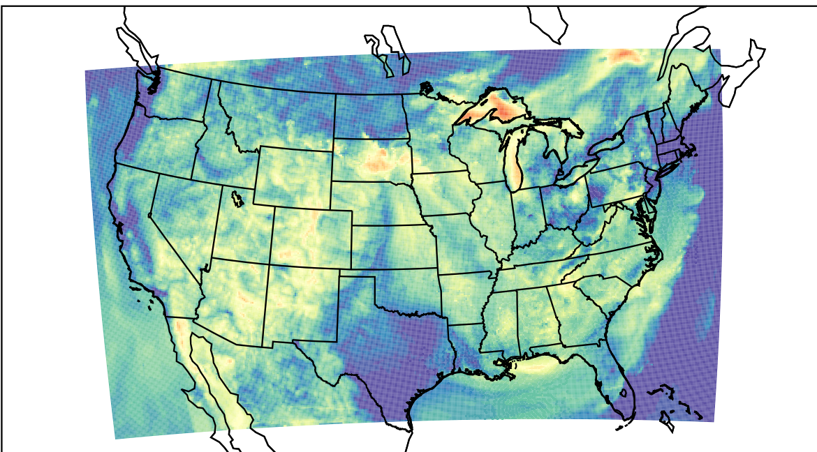
WRF (2023-06-24_13:00:00)
