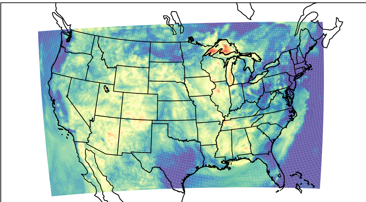
WRF (2023-06-24_09:00:00)
