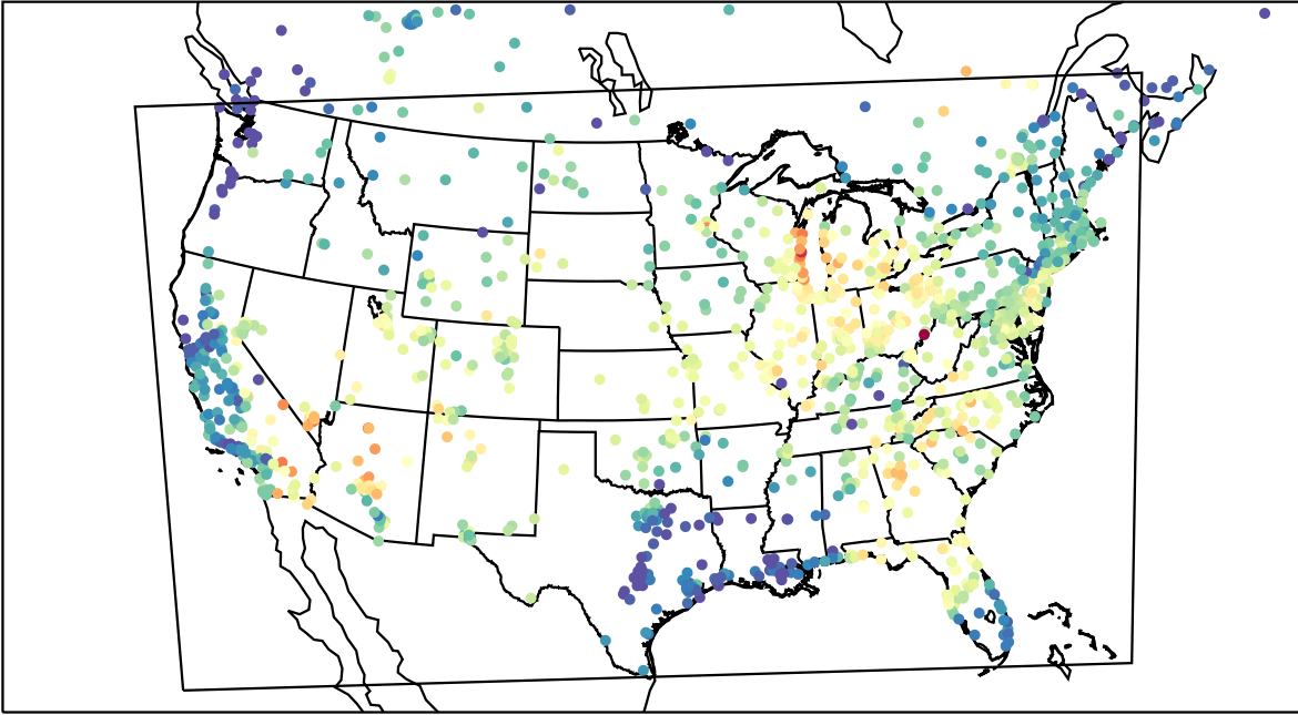
AirNOW (2023-06-25_15:00:00)
