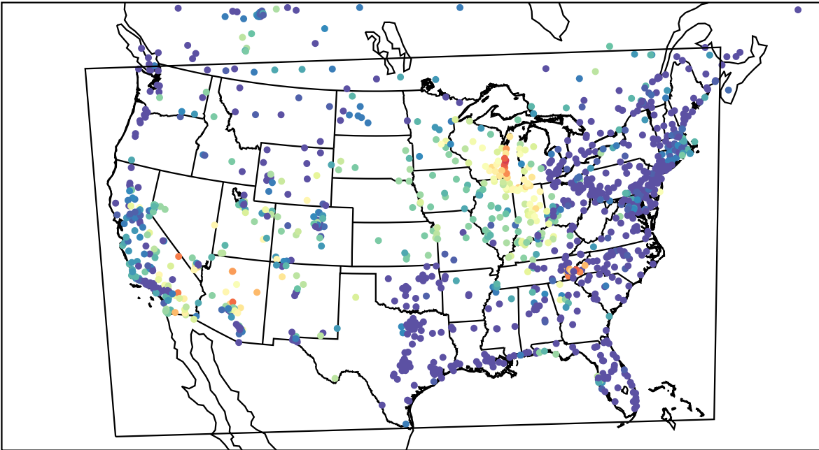
AirNOW (2023-06-25_11:00:00)
