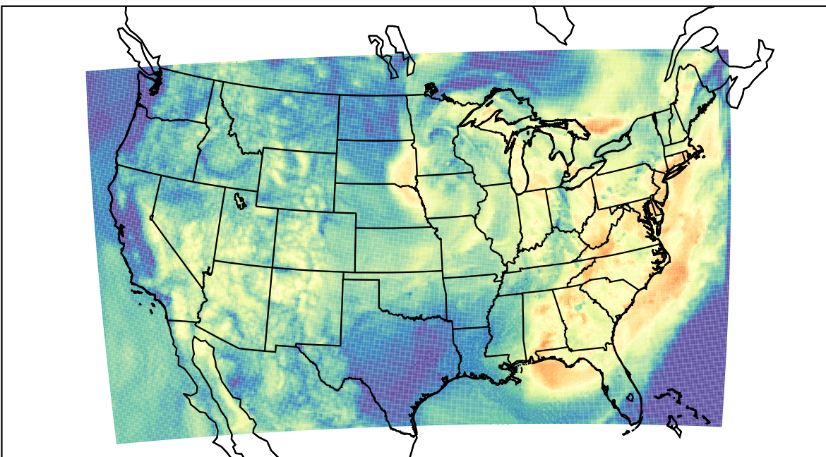
WRF (2023-06-25_14:00:00)
