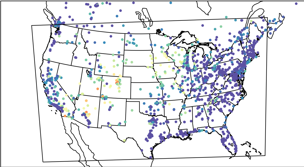
AirNOW (2023-06-24_11:00:00)
