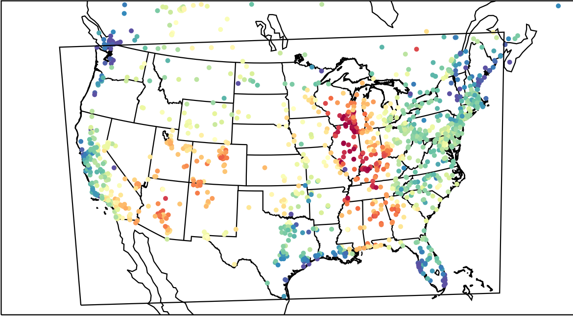
AirNOW (2023-06-24_18:00:00)
