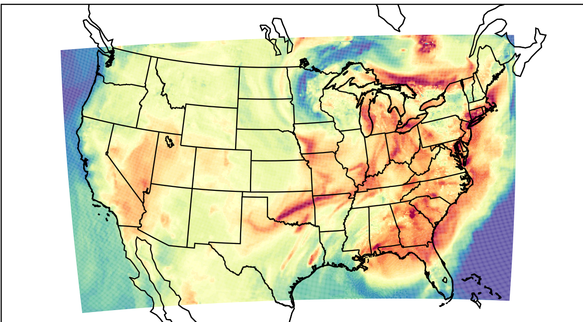
WRF (2023-06-25_20:00:00)
