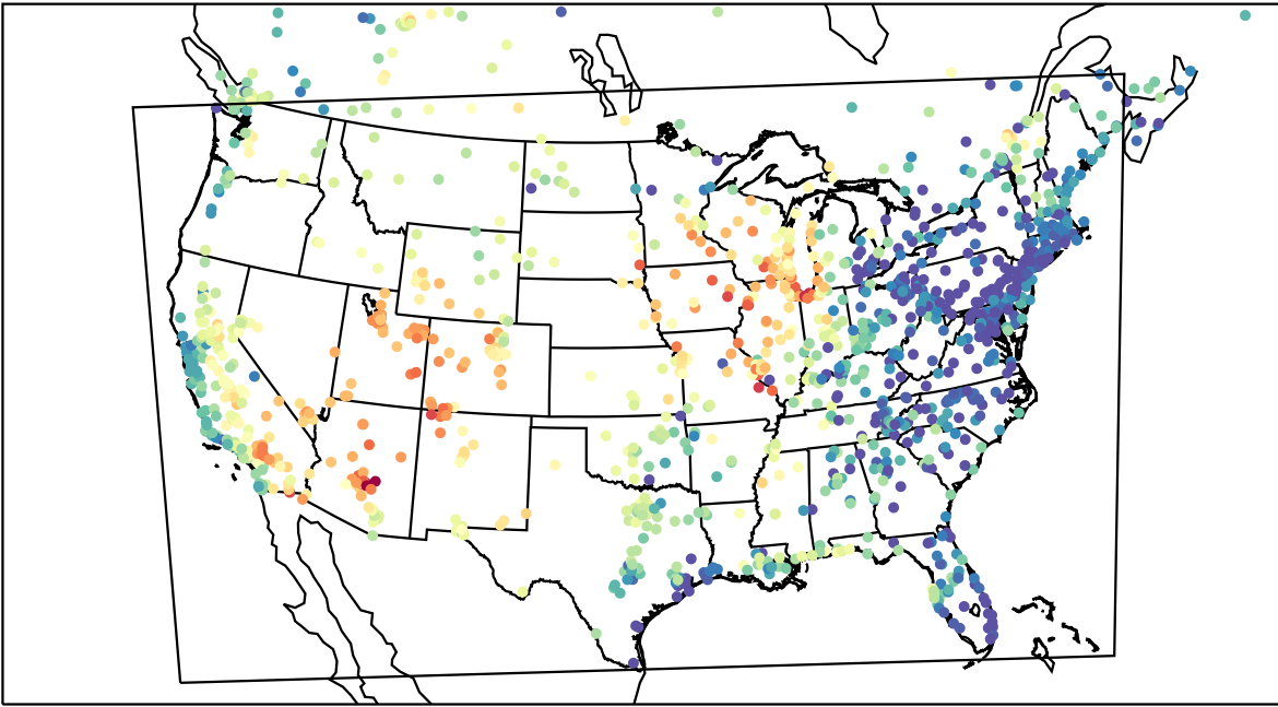
AirNOW (2023-06-24_01:00:00)
