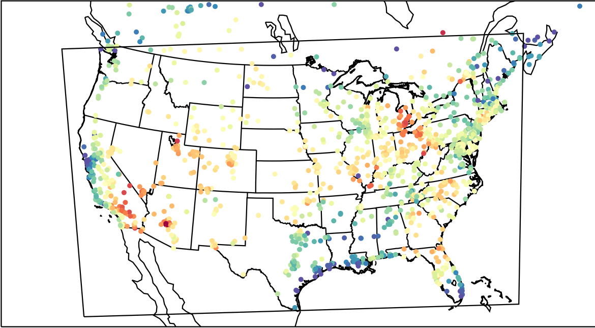
AirNOW (2023-06-25_21:00:00)
