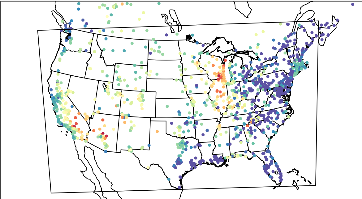
AirNOW (2023-06-25_03:00:00)
