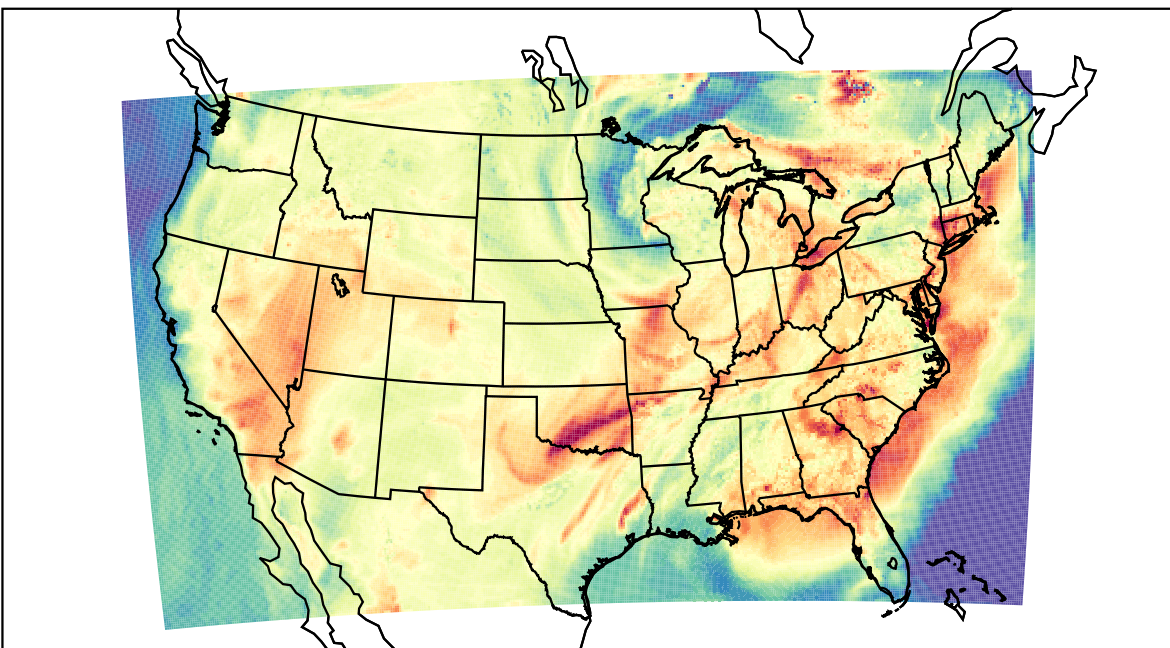
WRF (2023-06-25_23:00:00)
