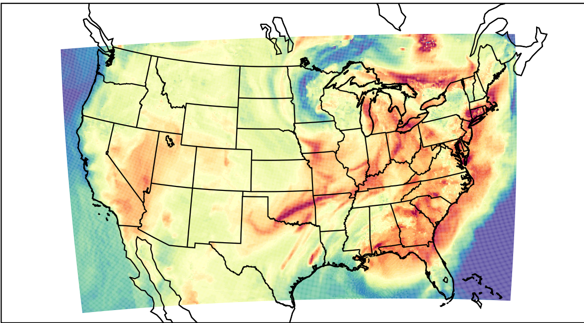
WRF (2023-06-25_21:00:00)
