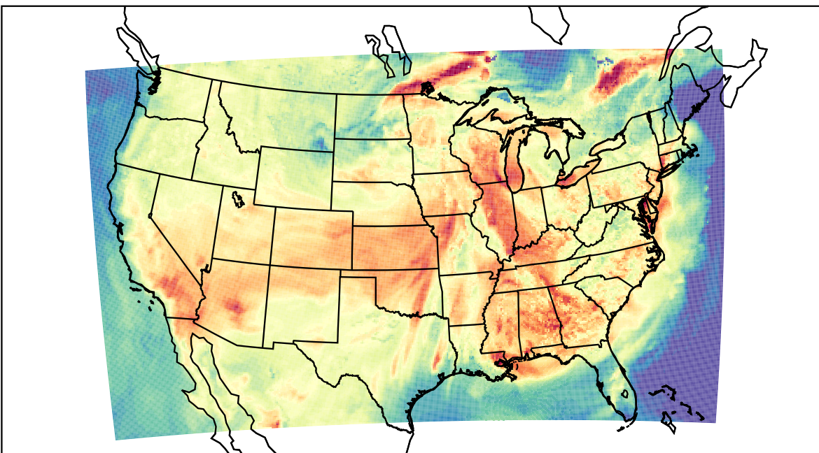
WRF (2023-06-24_23:00:00)
