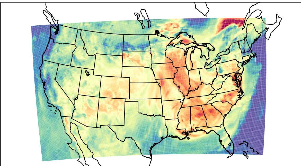
WRF (2023-06-24_16:00:00)
