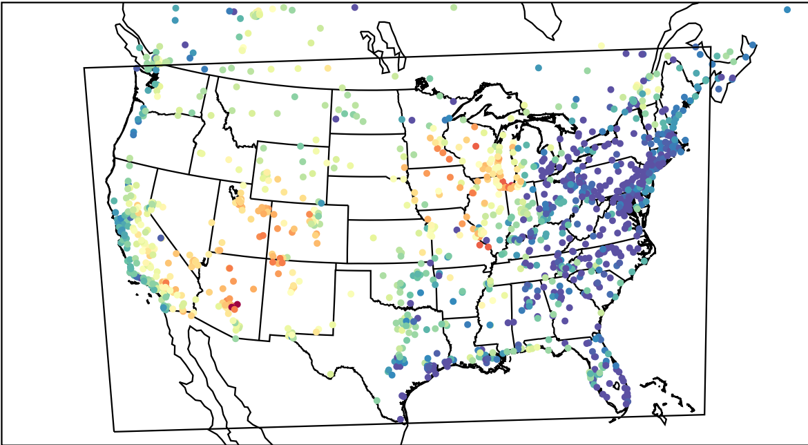
AirNOW (2023-06-24_02:00:00)
