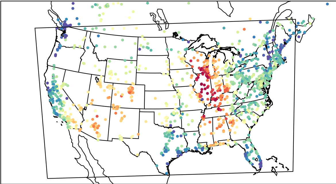
AirNOW (2023-06-24_17:00:00)
