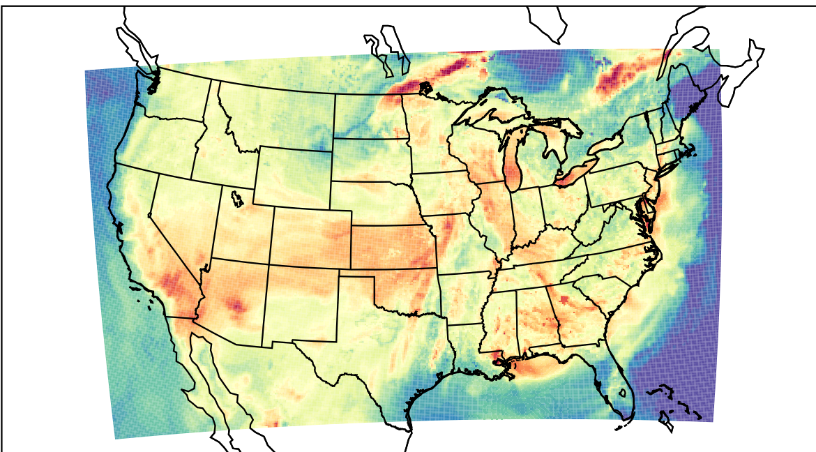
WRF (2023-06-25_00:00:00)
