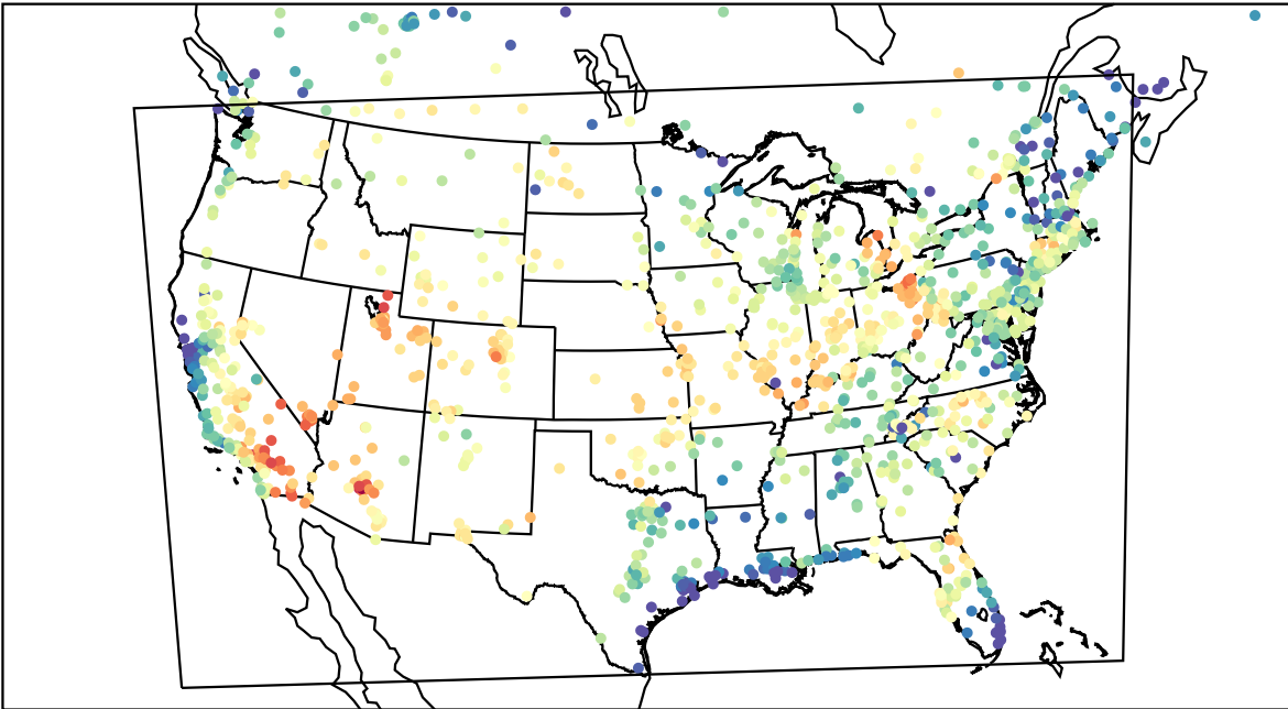
AirNOW (2023-06-25_23:00:00)
