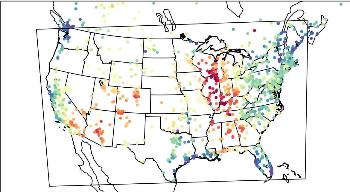
AirNOW (2023-06-24_19:00:00)
