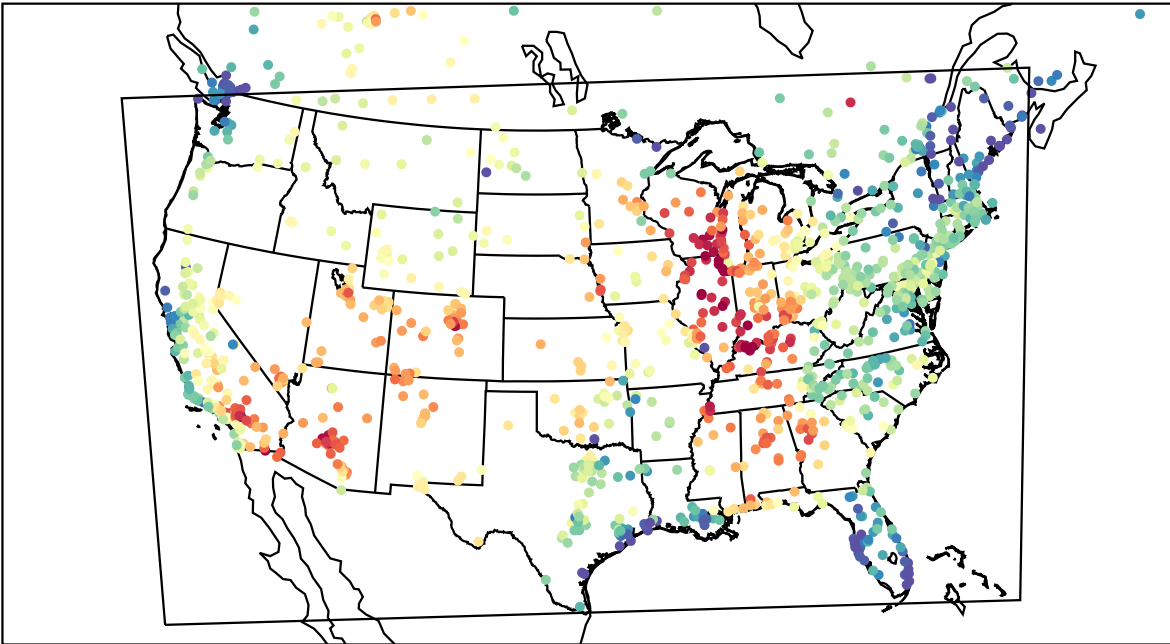
AirNOW (2023-06-24_21:00:00)
