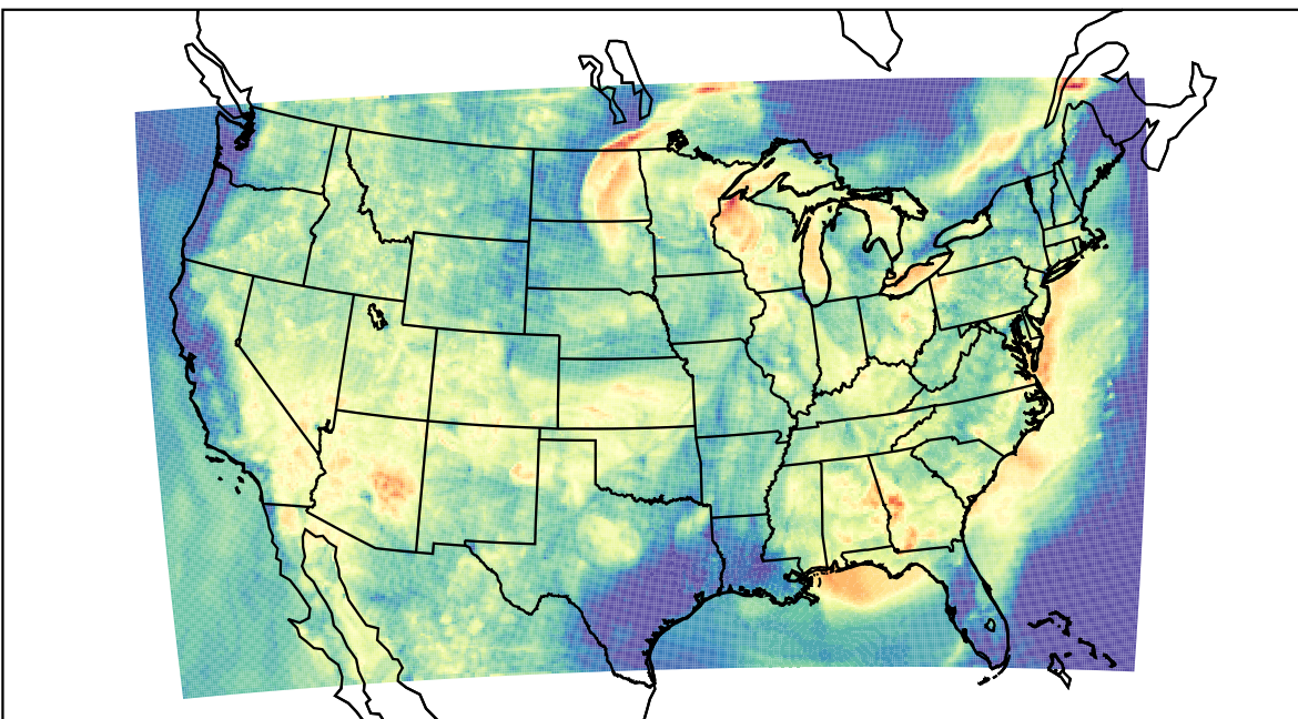
WRF (2023-06-25_05:00:00)
