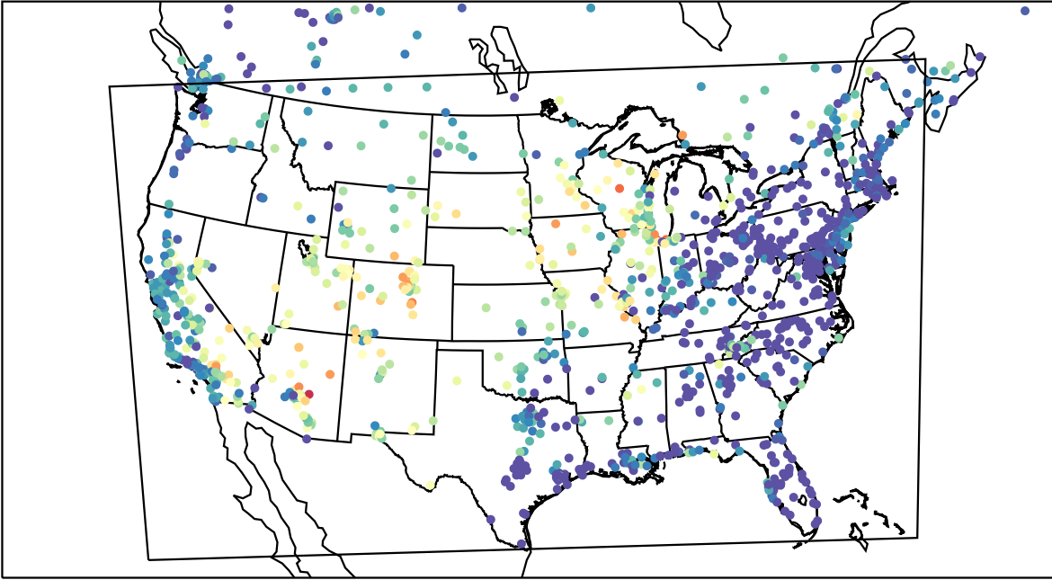
AirNOW (2023-06-24_05:00:00)
