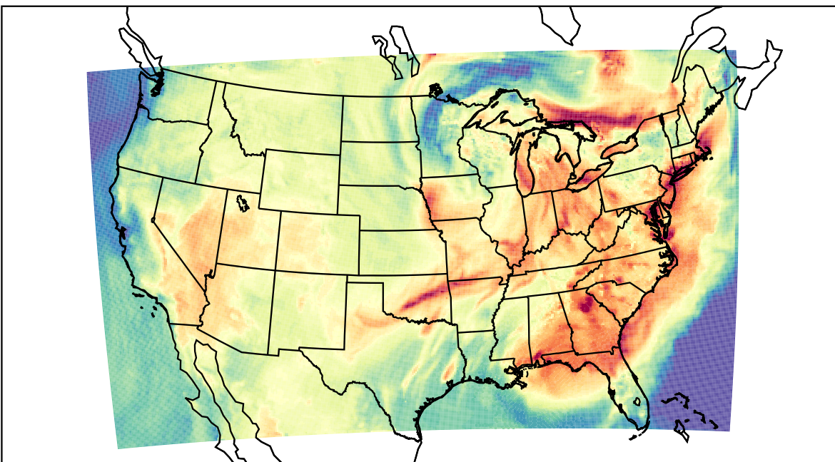
WRF (2023-06-25_18:00:00)
