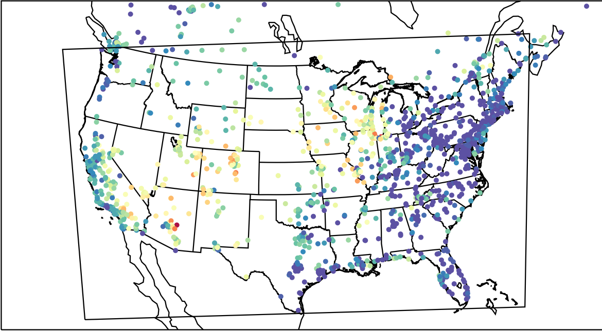
AirNOW (2023-06-24_04:00:00)
