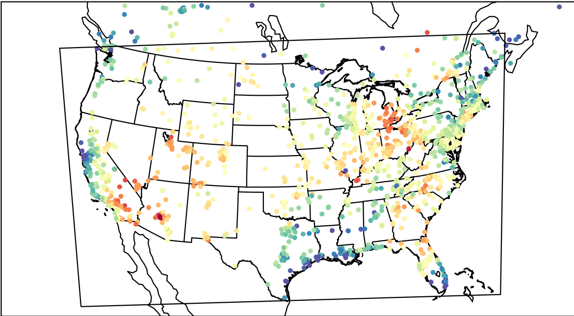
AirNOW (2023-06-25_20:00:00)
