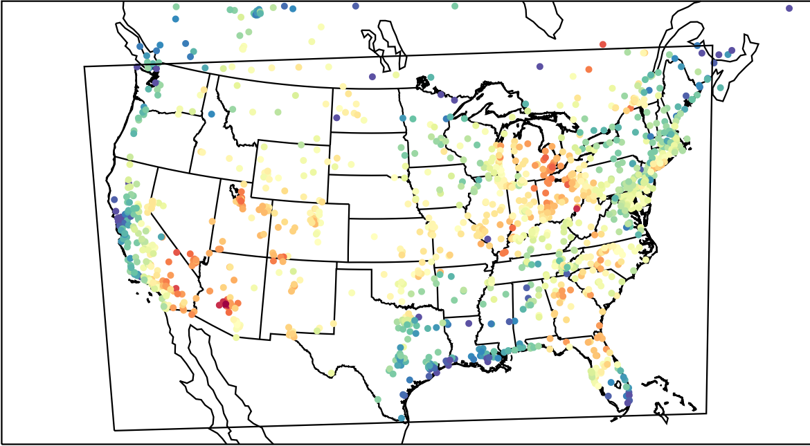
AirNOW (2023-06-25_19:00:00)
