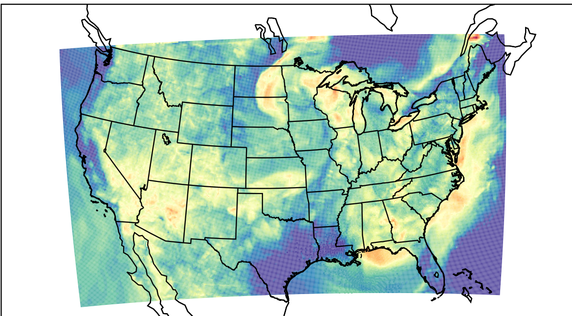
WRF (2023-06-25_07:00:00)
