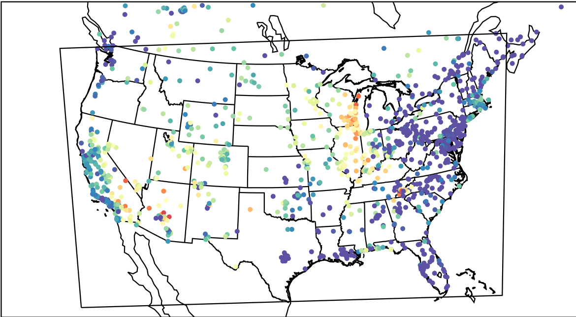
AirNOW (2023-06-25_05:00:00)
