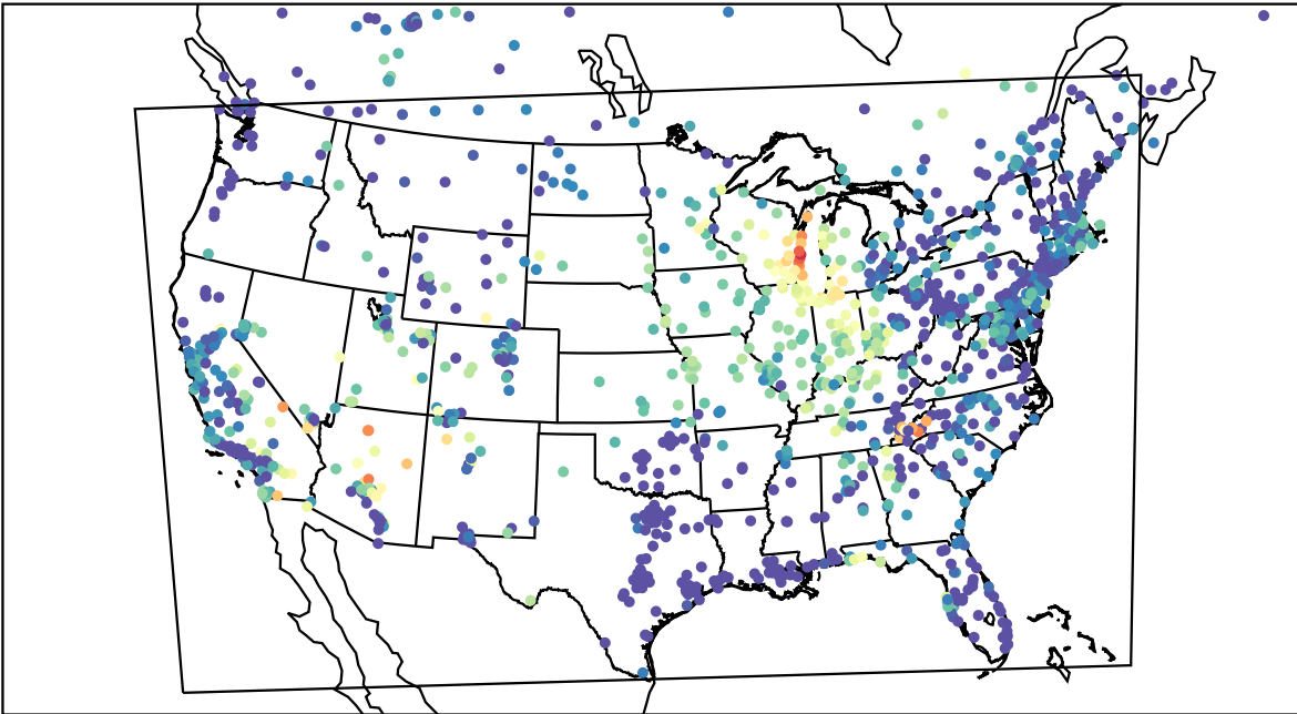
AirNOW (2023-06-25_12:00:00)
