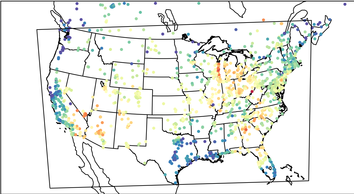
AirNOW (2023-06-25_16:00:00)
