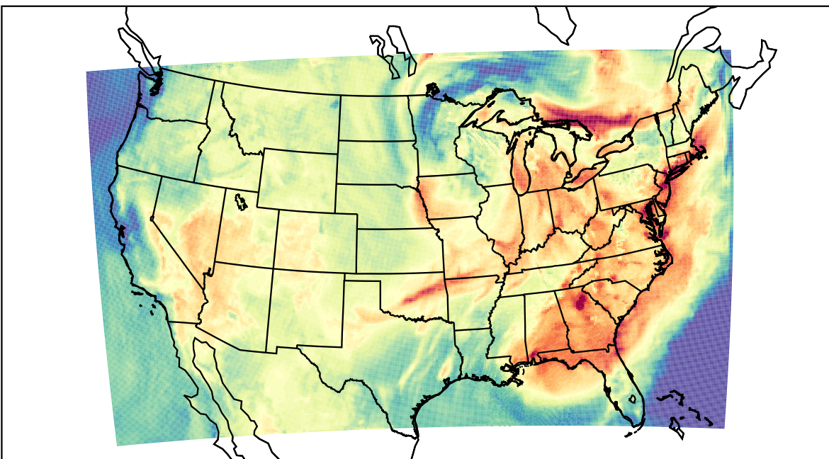
WRF (2023-06-25_17:00:00)
