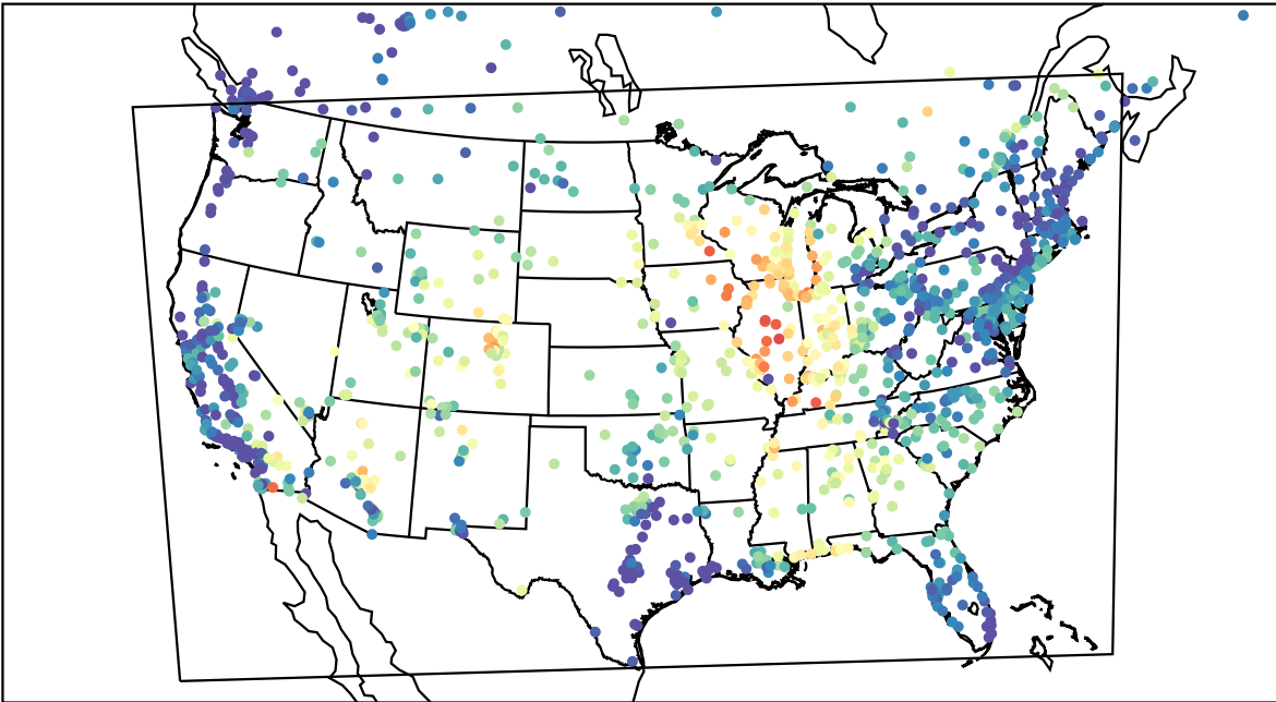
AirNOW (2023-06-24_14:00:00)
