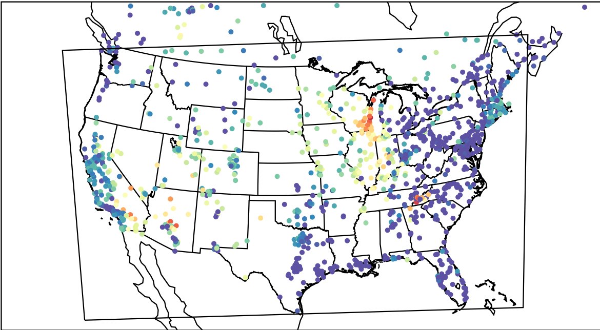
AirNOW (2023-06-25_07:00:00)
