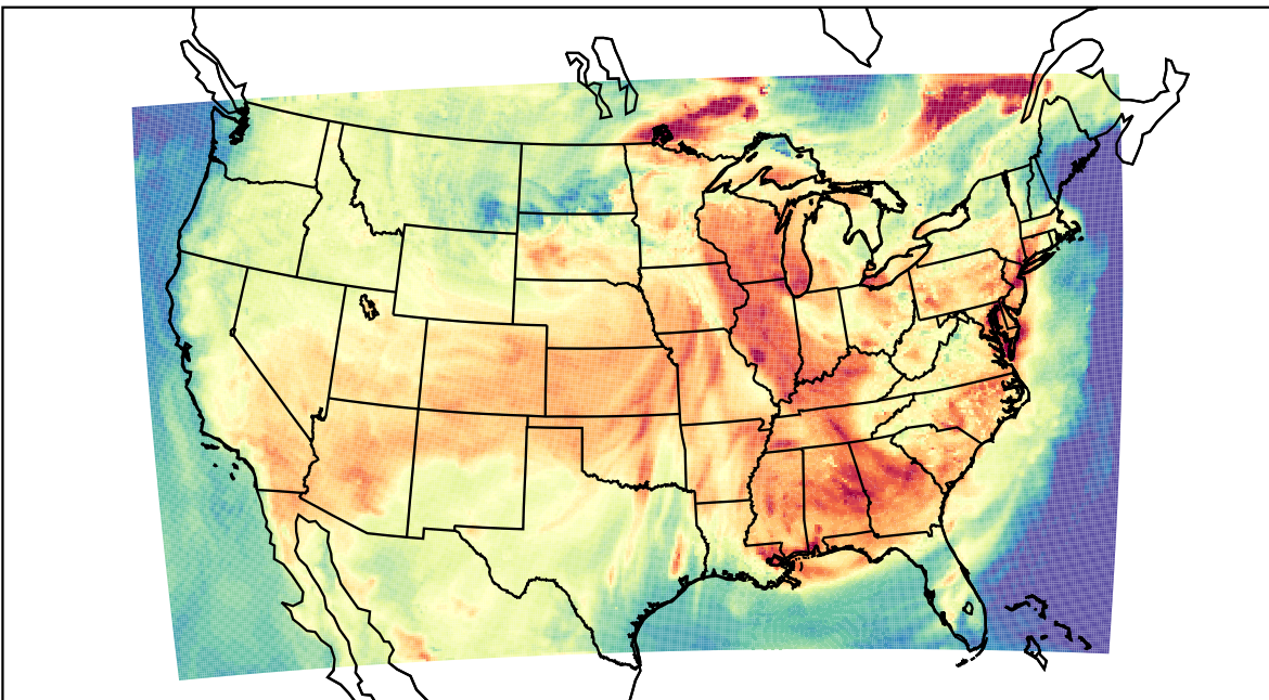
WRF (2023-06-24_20:00:00)
