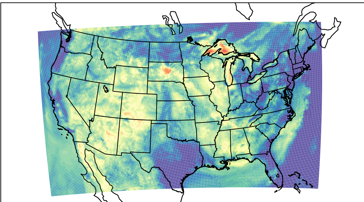
WRF (2023-06-24_11:00:00)
