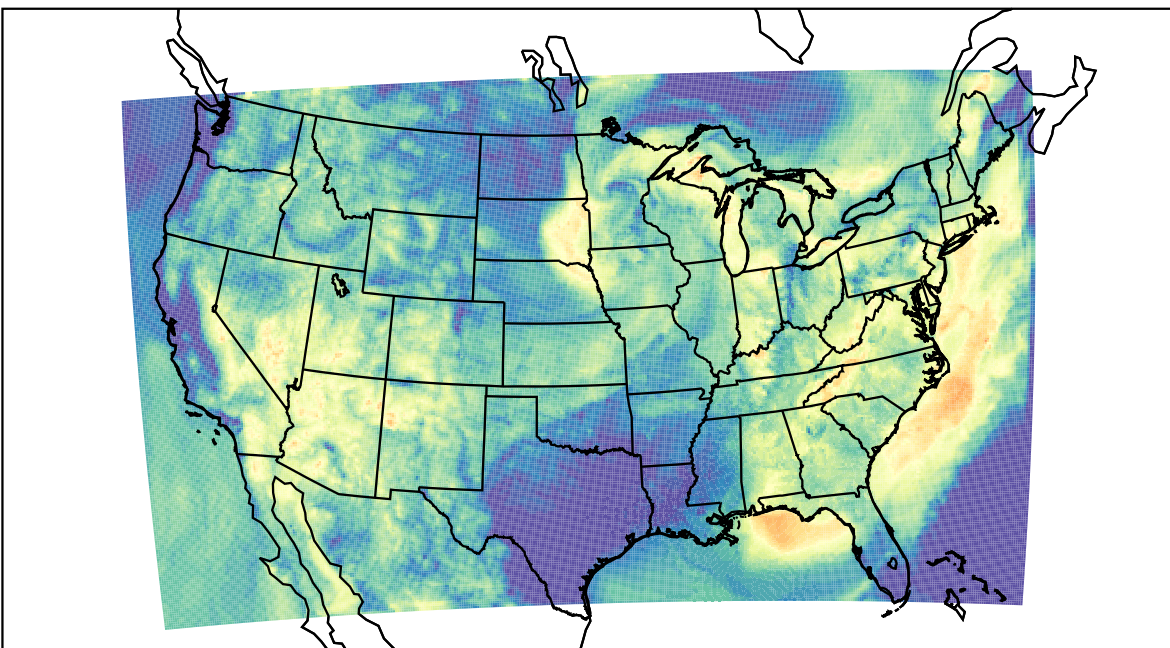
WRF (2023-06-25_13:00:00)
