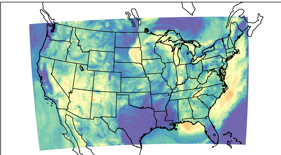
WRF (2023-06-25_12:00:00)
