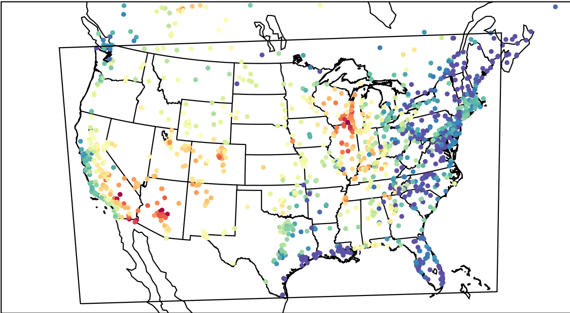
AirNOW (2023-06-25_01:00:00)
