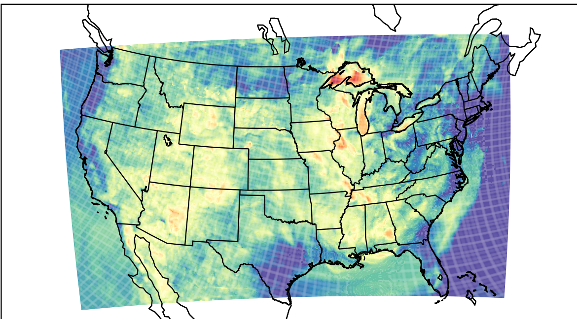
WRF (2023-06-24_07:00:00)
