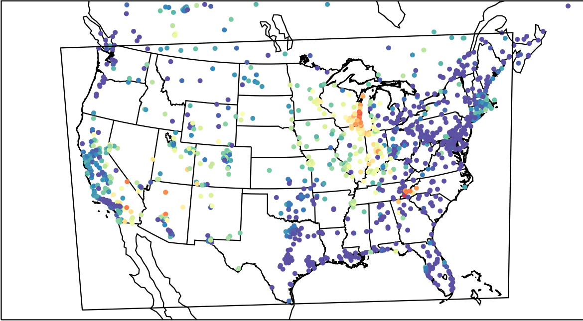
AirNOW (2023-06-25_08:00:00)
