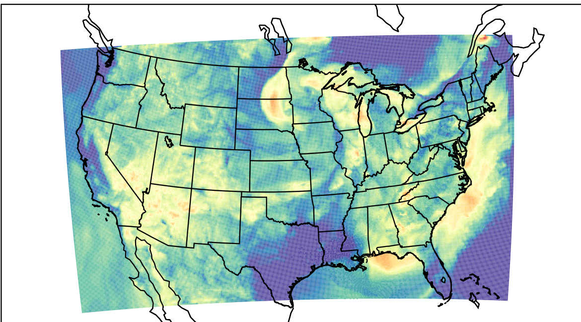
WRF (2023-06-25_09:00:00)
