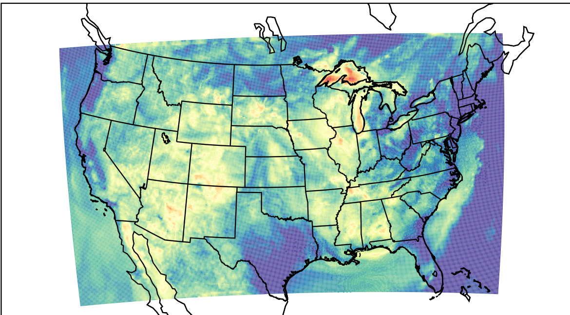
WRF (2023-06-24_10:00:00)
