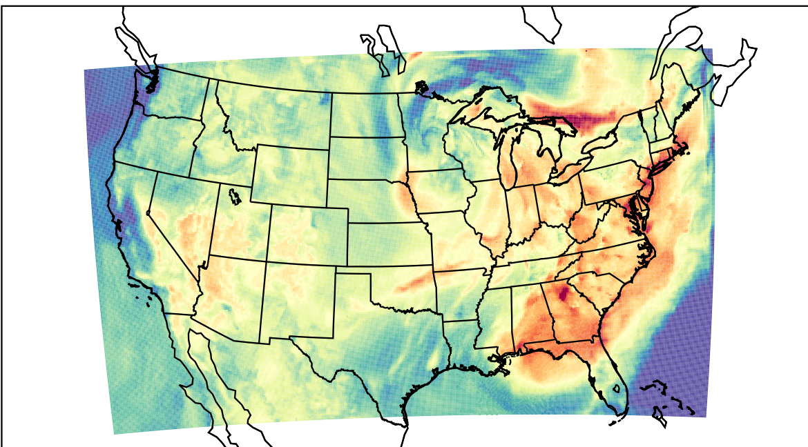
WRF (2023-06-25_16:00:00)
