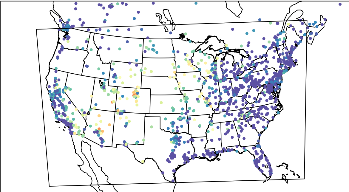
AirNOW (2023-06-24_09:00:00)
