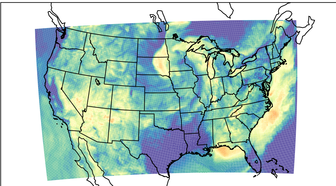
WRF (2023-06-25_11:00:00)
