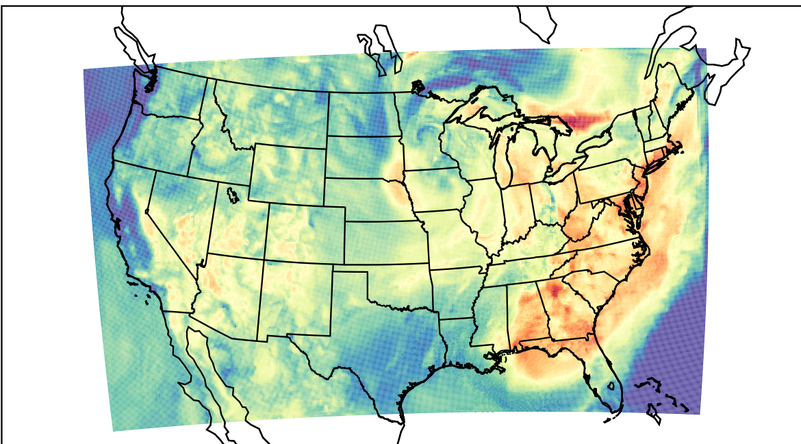
WRF (2023-06-25_15:00:00)
