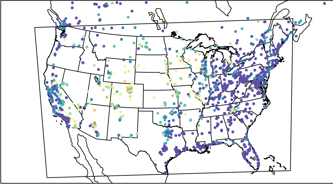
AirNOW (2023-06-24_08:00:00)
