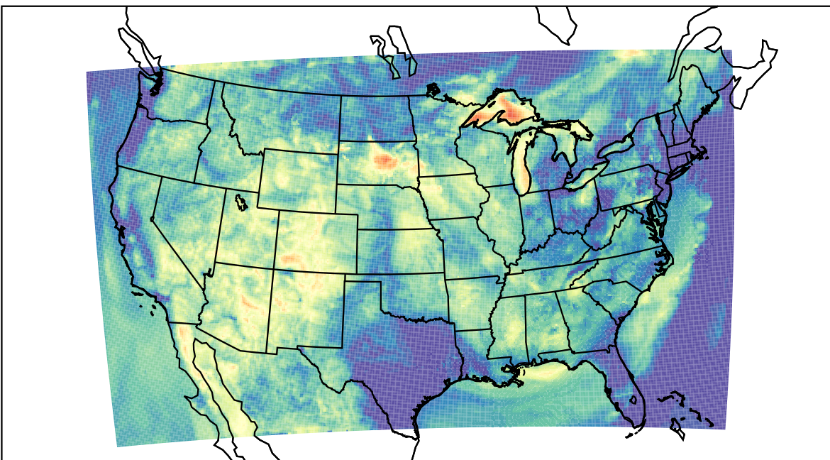
WRF (2023-06-24_12:00:00)
