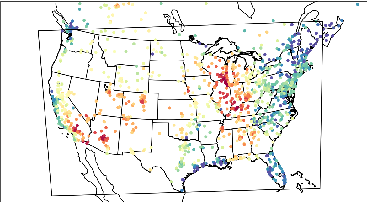
AirNOW (2023-06-24_23:00:00)
