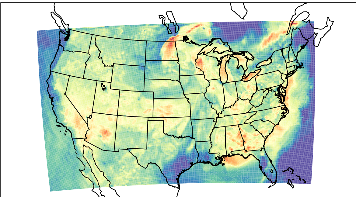
WRF (2023-06-25_03:00:00)
