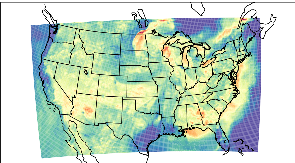
WRF (2023-06-25_04:00:00)
