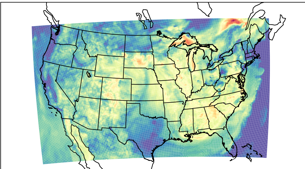
WRF (2023-06-24_14:00:00)
