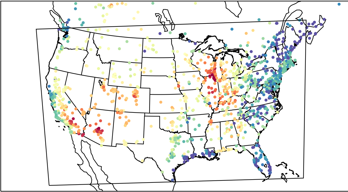
AirNOW (2023-06-25_00:00:00)
