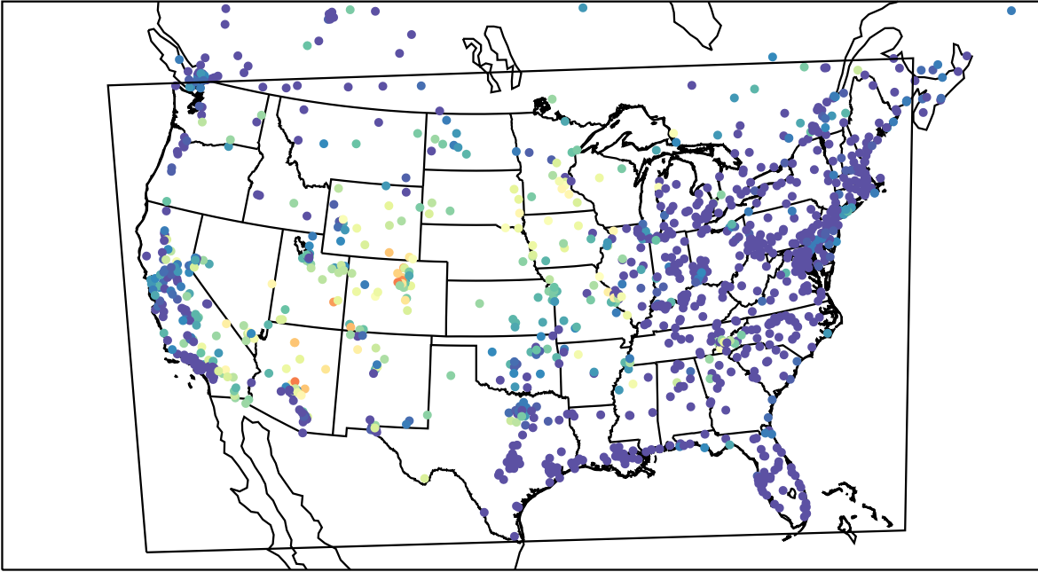
AirNOW (2023-06-24_10:00:00)
