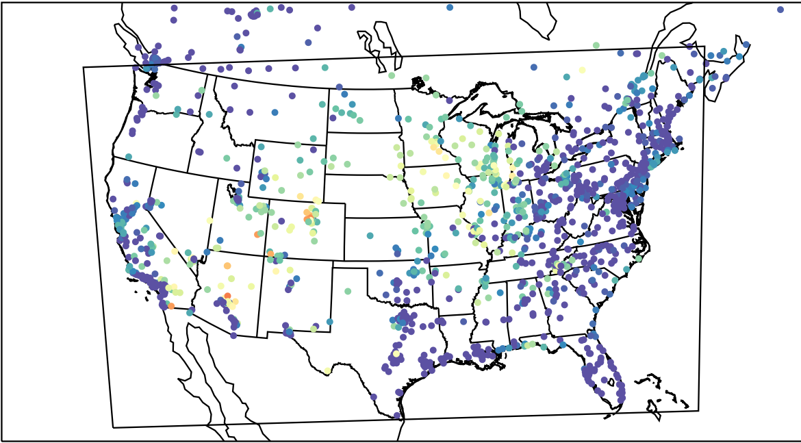
AirNOW (2023-06-24_12:00:00)
