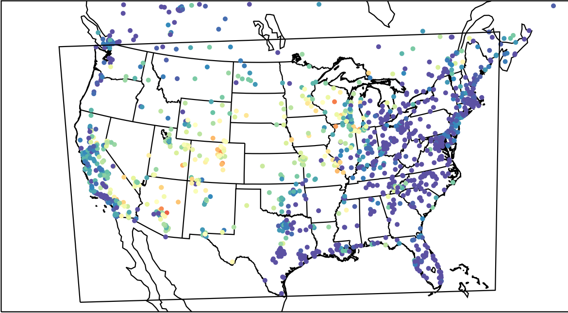
AirNOW (2023-06-24_06:00:00)
