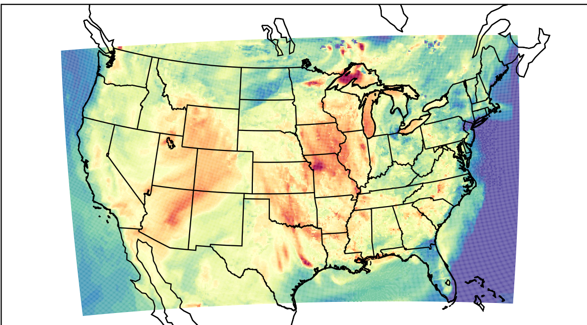
WRF (2023-06-24_00:00:00)
