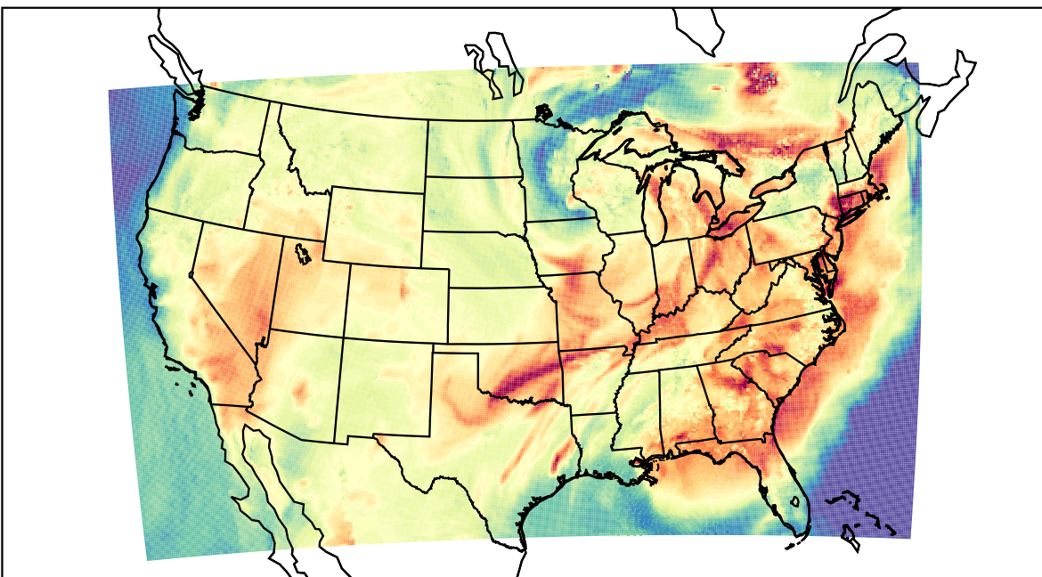
WRF (2023-06-25_22:00:00)
