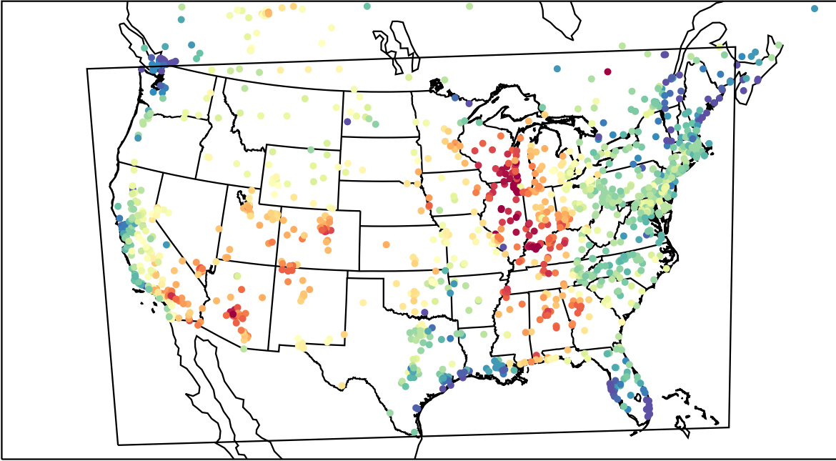
AirNOW (2023-06-24_20:00:00)
