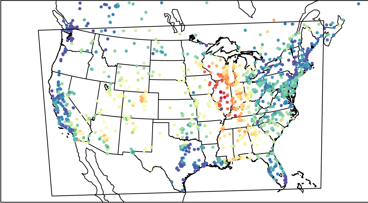
AirNOW (2023-06-24_15:00:00)
