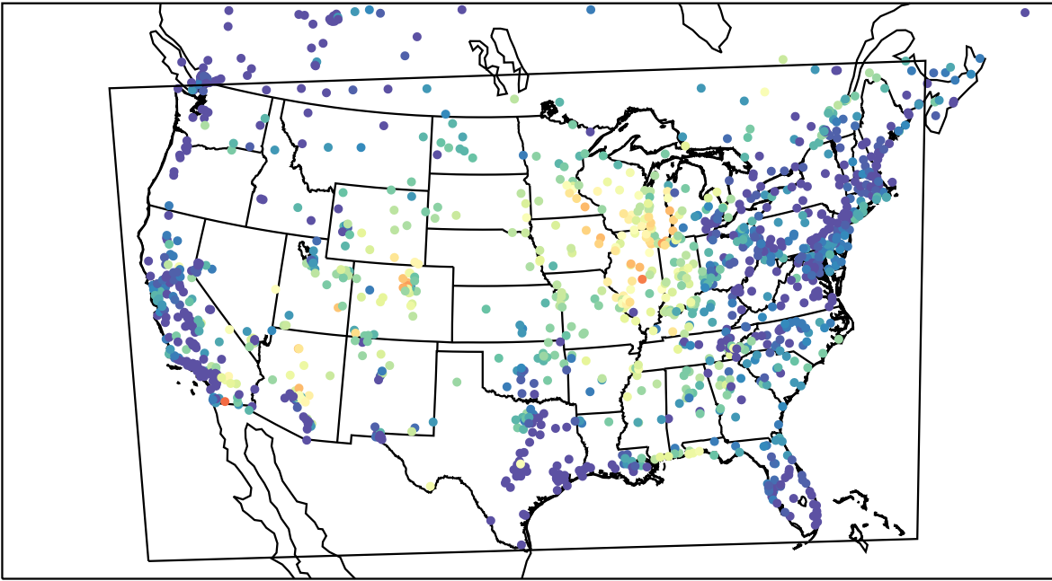
AirNOW (2023-06-24_13:00:00)
