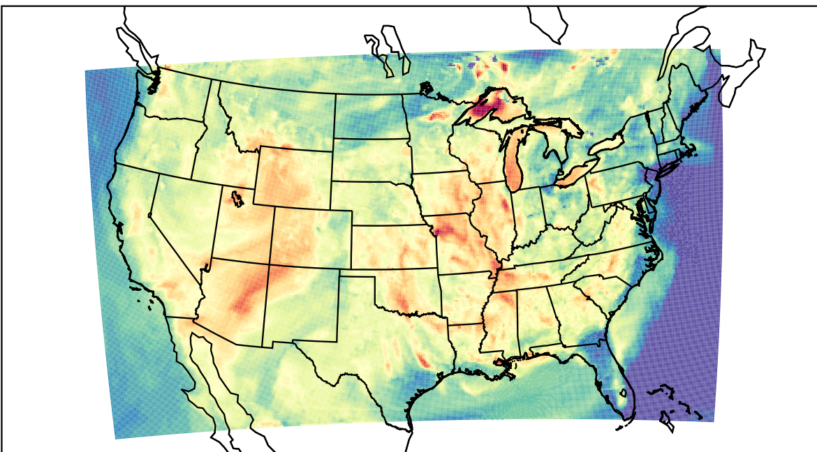
WRF (2023-06-24_01:00:00)
