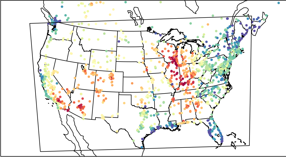
AirNOW (2023-06-24_22:00:00)
