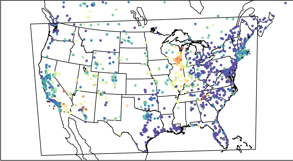
AirNOW (2023-06-25_06:00:00)
