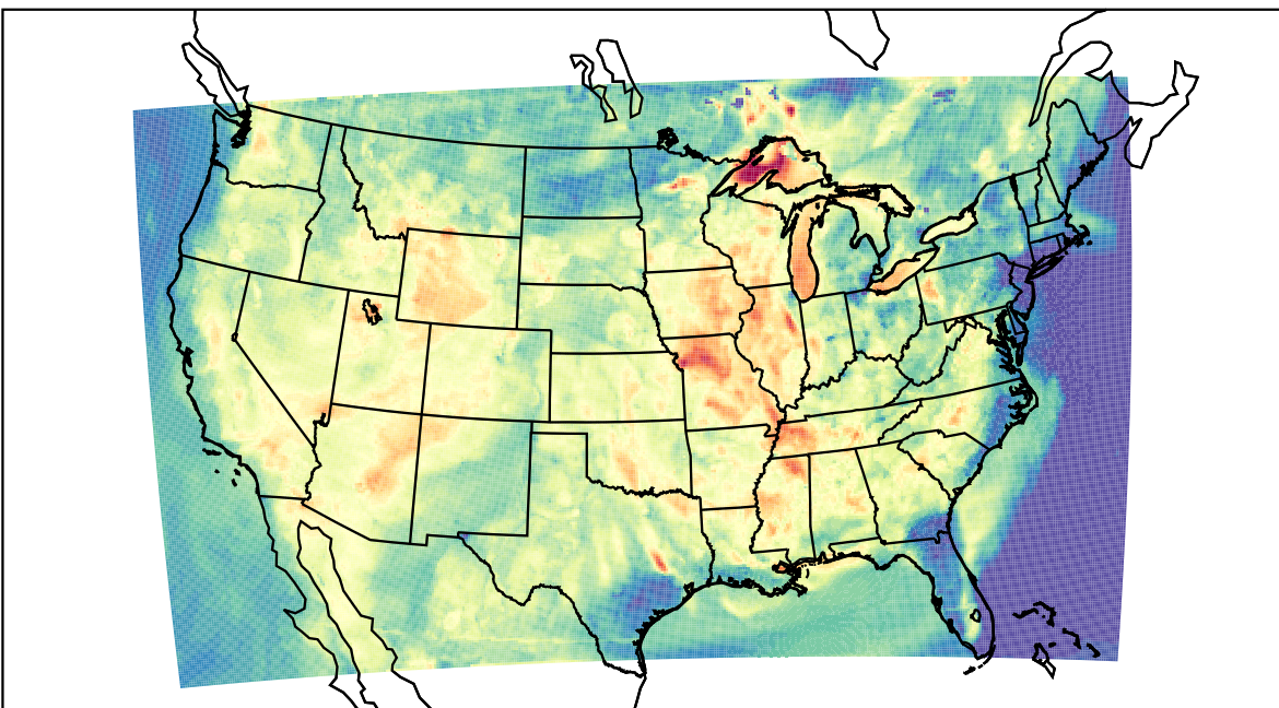
WRF (2023-06-24_02:00:00)
