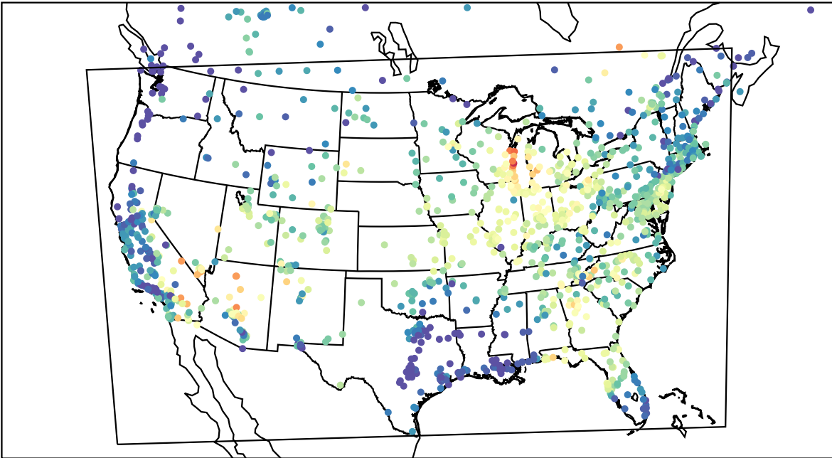
AirNOW (2023-06-25_14:00:00)
