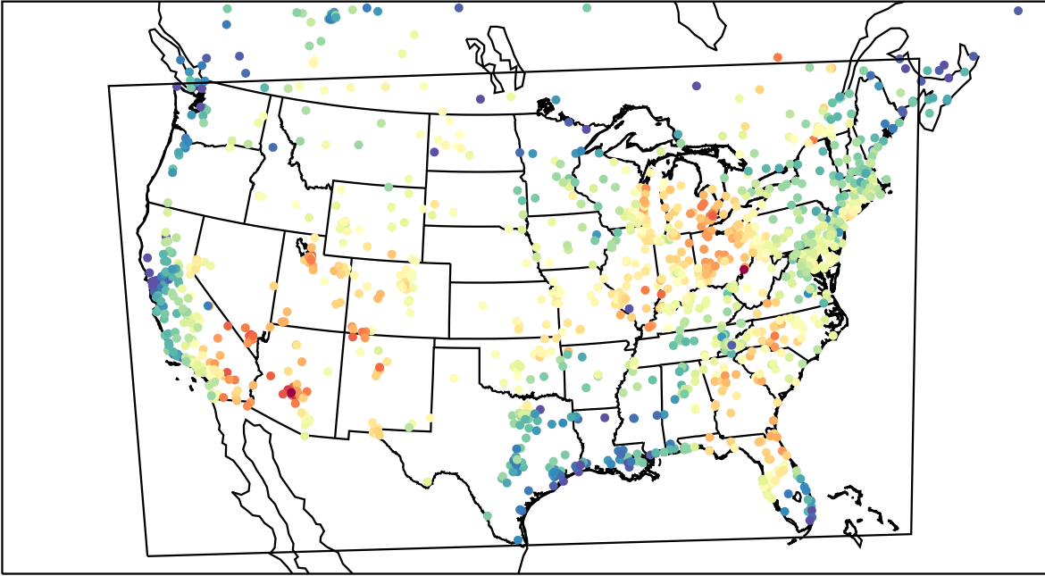
AirNOW (2023-06-25_18:00:00)
