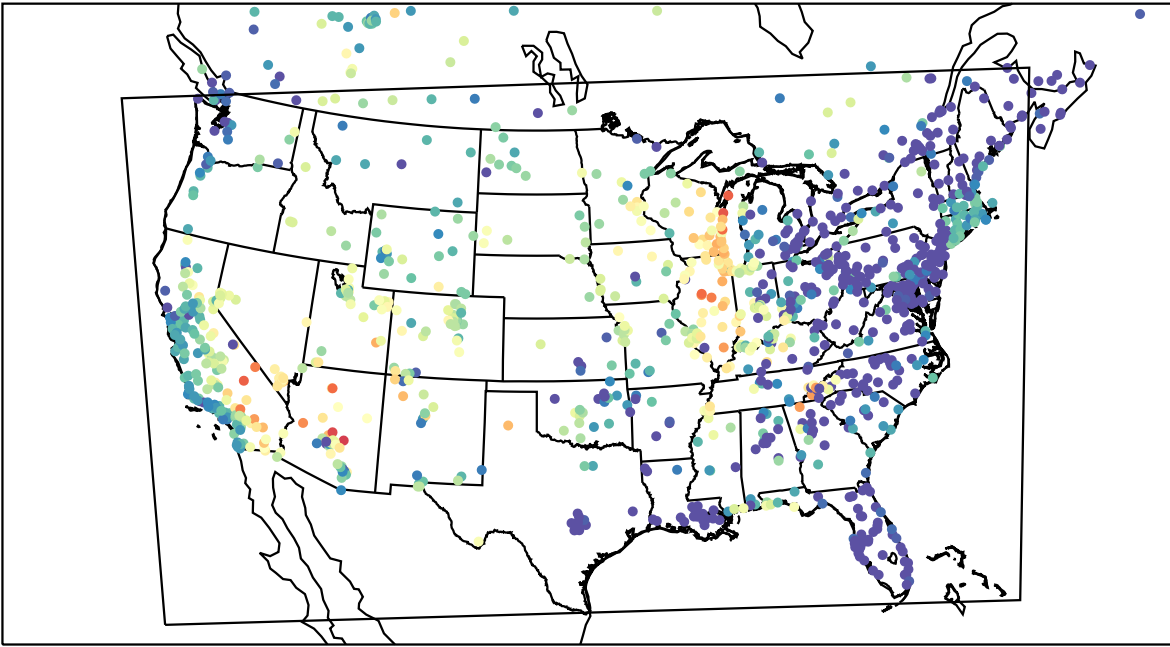
AirNOW (2023-06-25_04:00:00)
