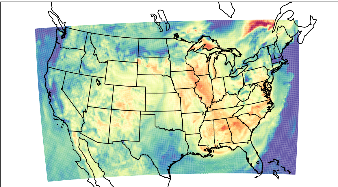
WRF (2023-06-24_15:00:00)
