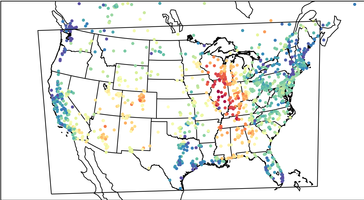
AirNOW (2023-06-24_16:00:00)
