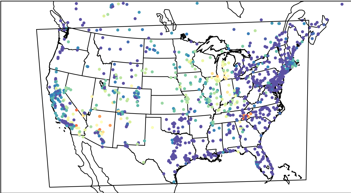
AirNOW (2023-06-25_10:00:00)
