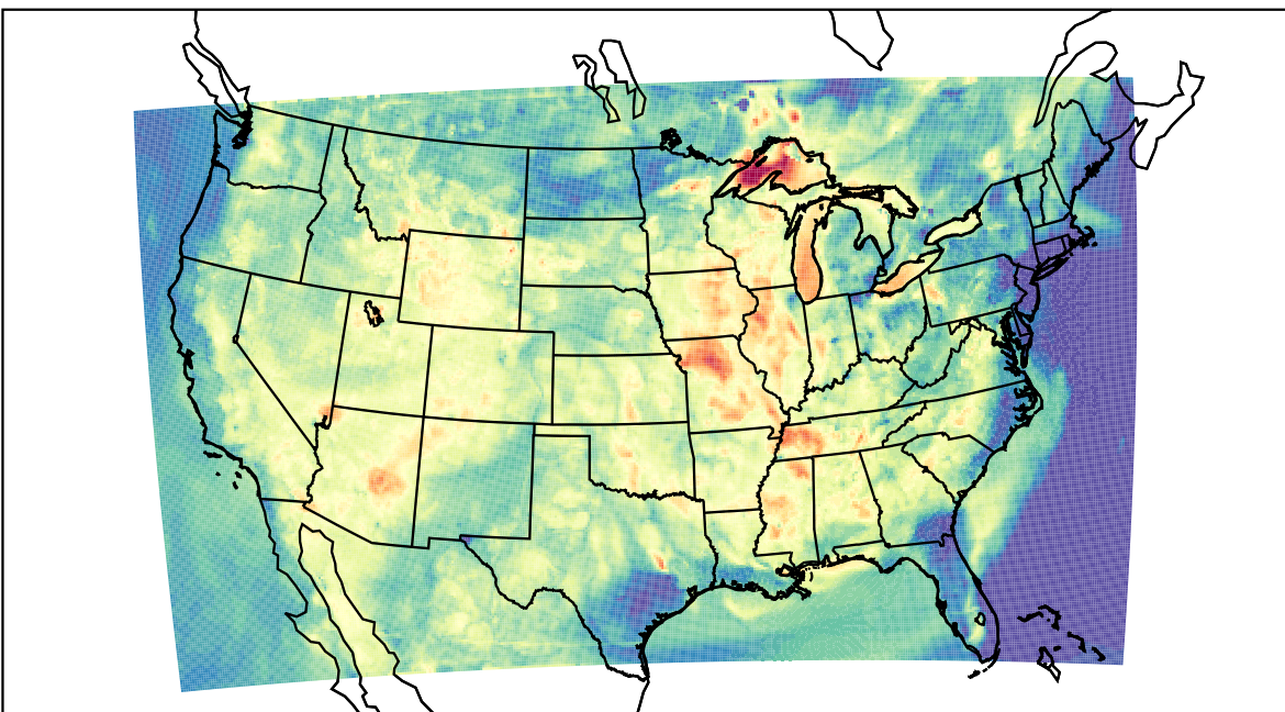
WRF (2023-06-24_03:00:00)
