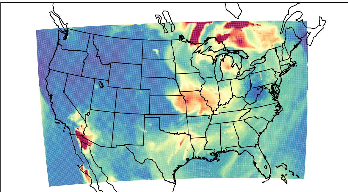
WRF 2023-06-26_12:00:00
