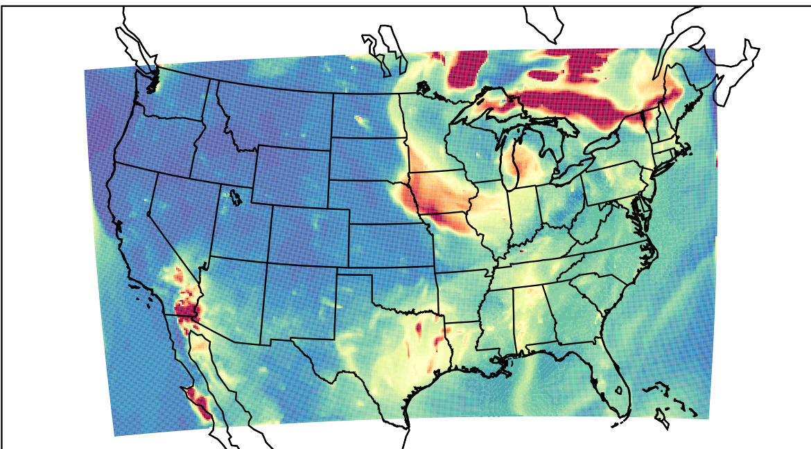
WRF 2023-06-26_05:00:00
