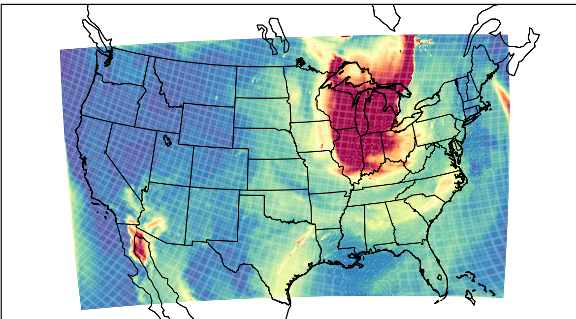
WRF 2023-06-27_16:00:00
