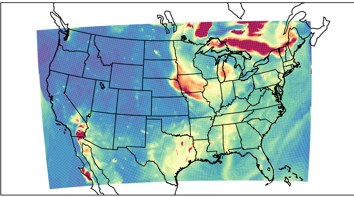
WRF 2023-06-26_04:00:00
