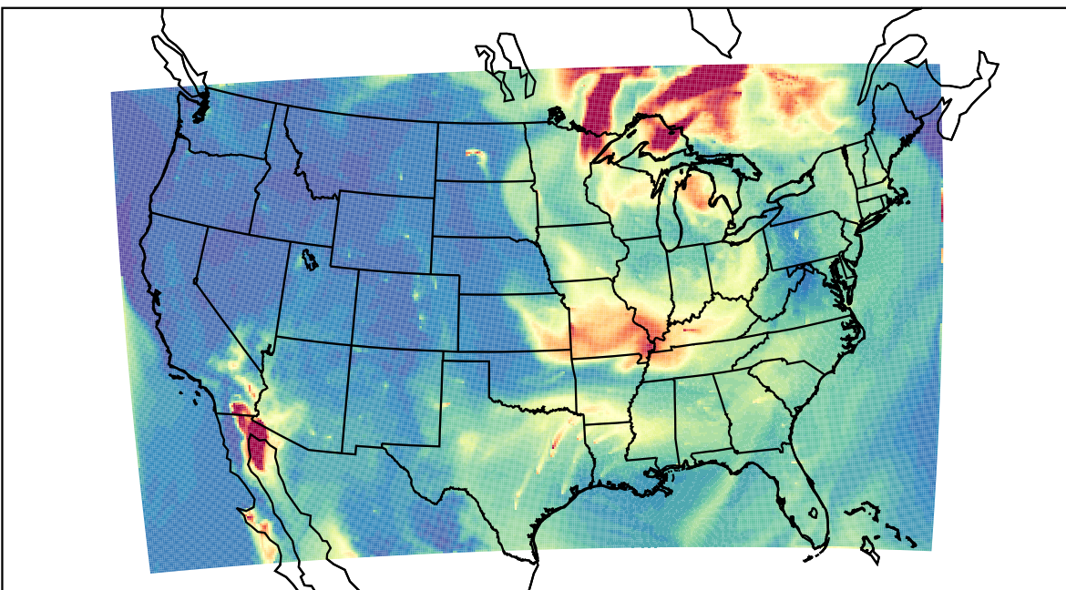
WRF 2023-06-26_15:00:00
