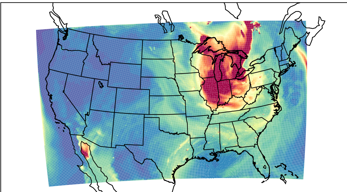
WRF 2023-06-27_20:00:00
