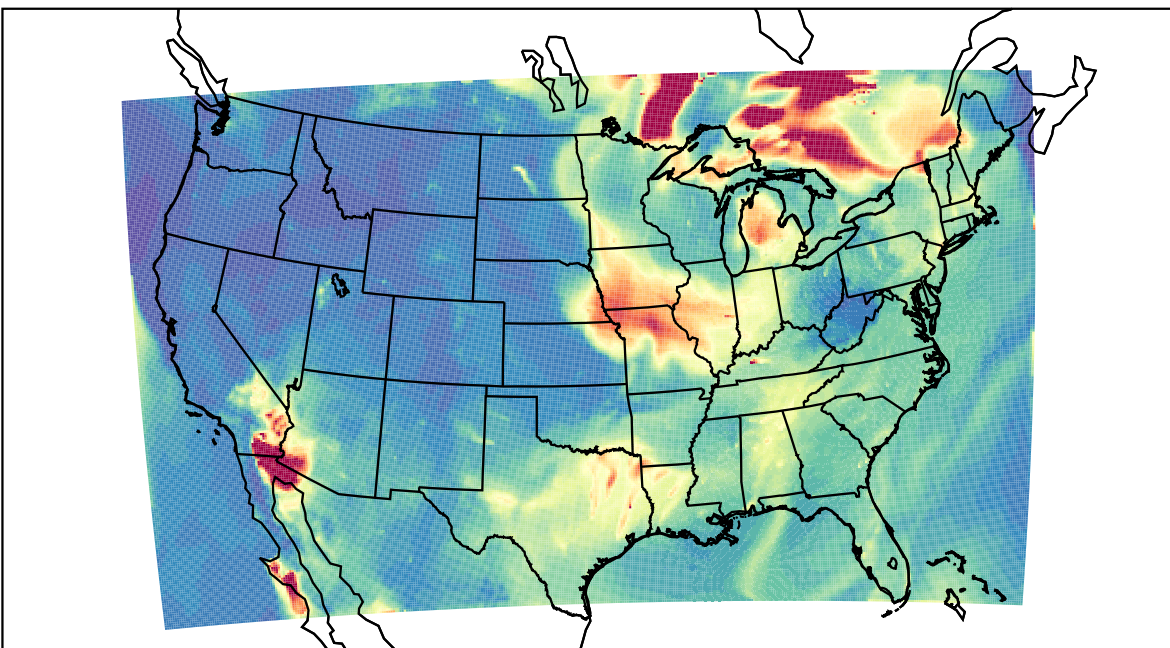
WRF 2023-06-26_09:00:00
