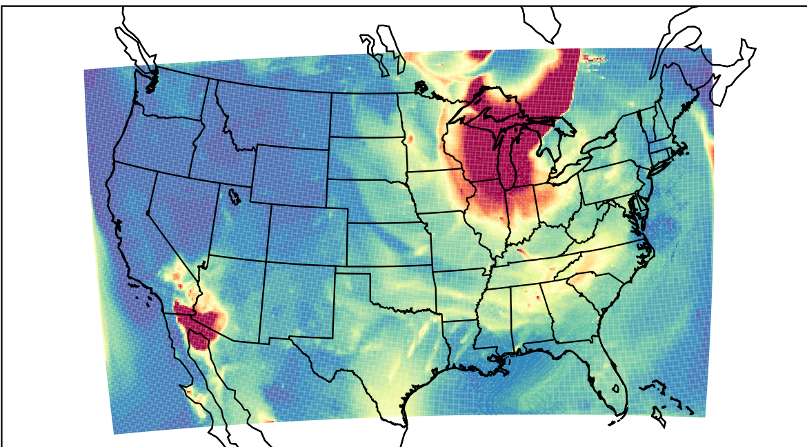
WRF 2023-06-27_10:00:00
