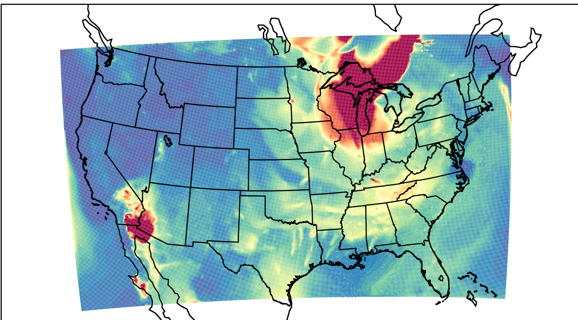
WRF 2023-06-27_07:00:00
