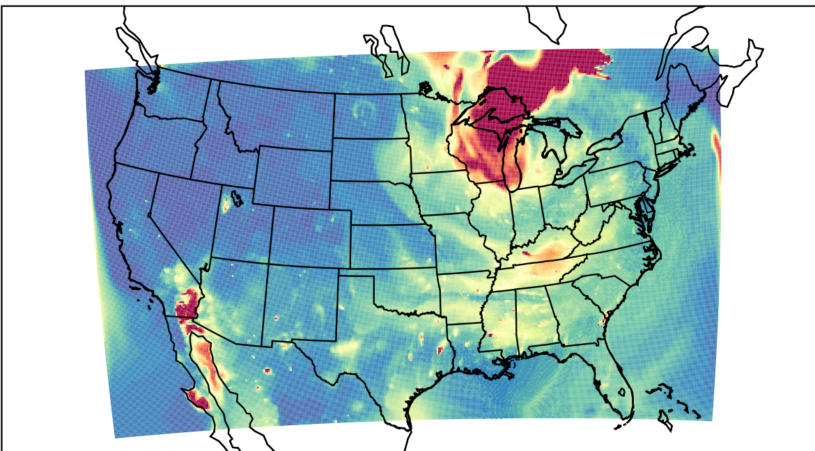
WRF 2023-06-27_02:00:00
