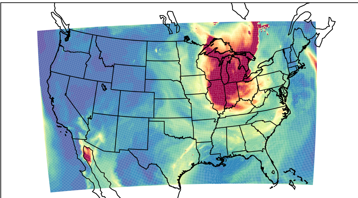
WRF 2023-06-27_18:00:00
