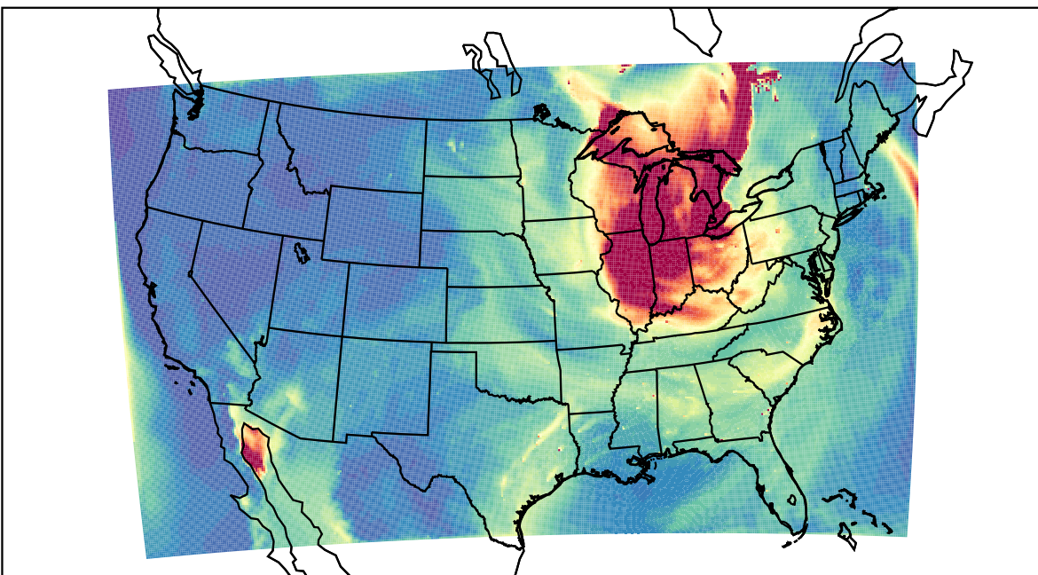
WRF 2023-06-27_19:00:00
