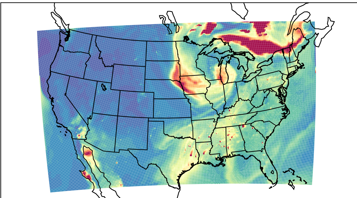
WRF 2023-06-26_00:00:00
