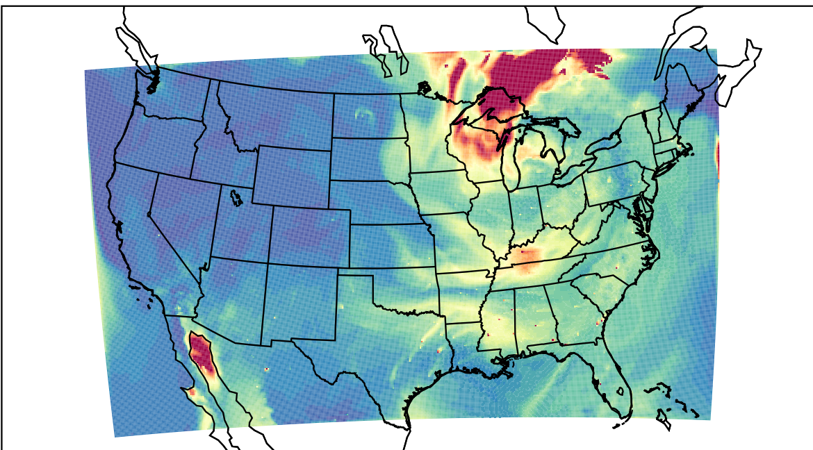
WRF 2023-06-26_21:00:00
