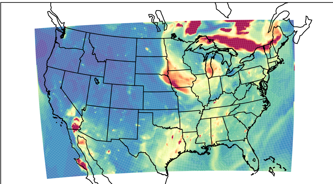
WRF 2023-06-26_03:00:00
