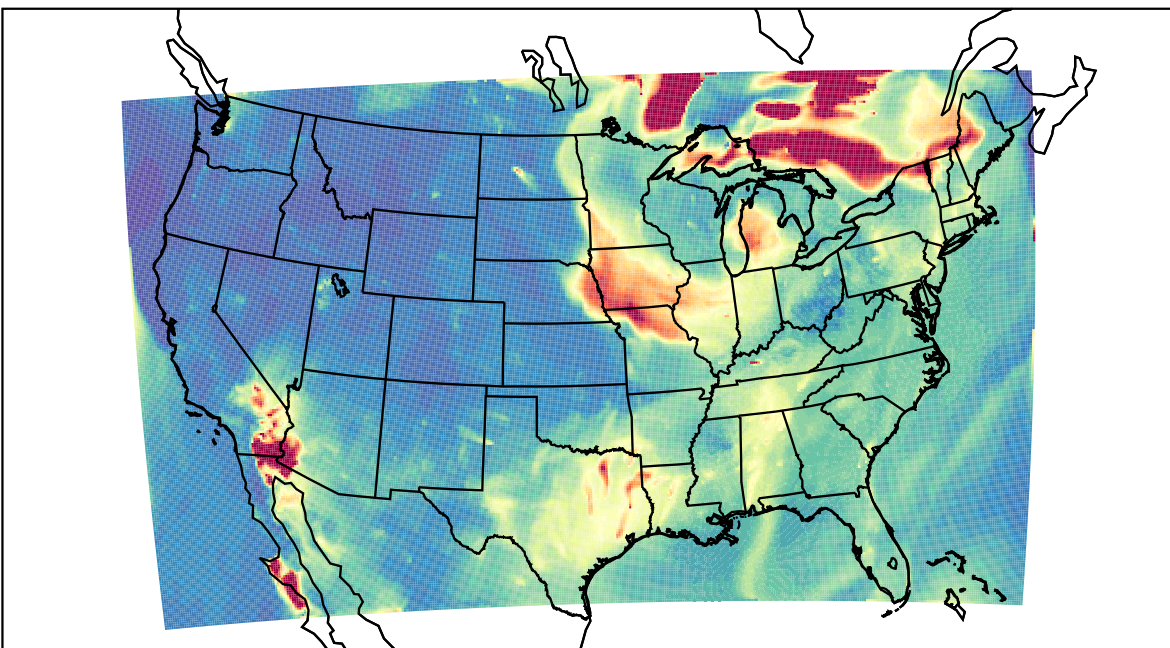
WRF 2023-06-26_06:00:00
