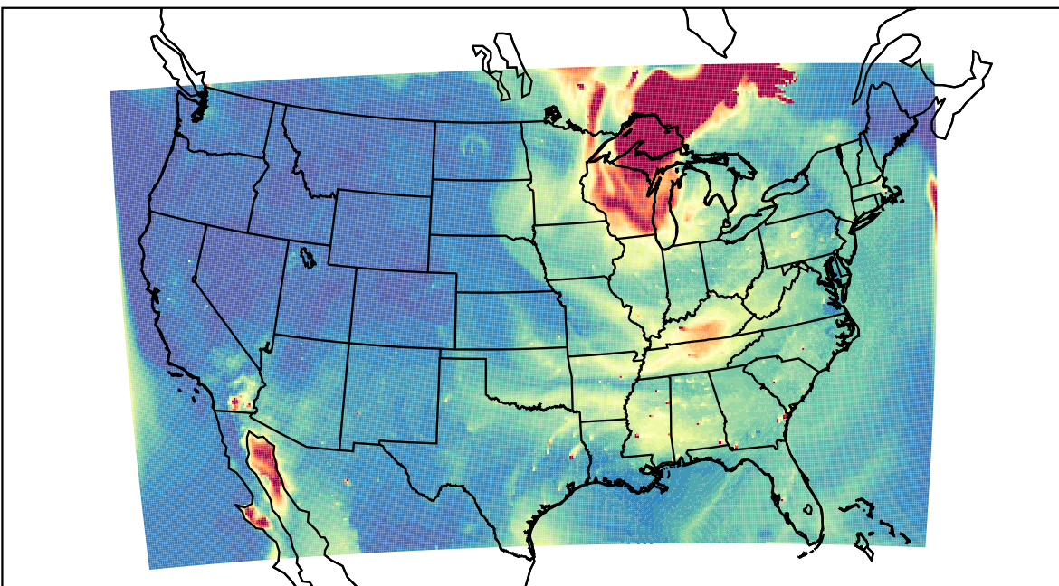
WRF 2023-06-27_00:00:00
