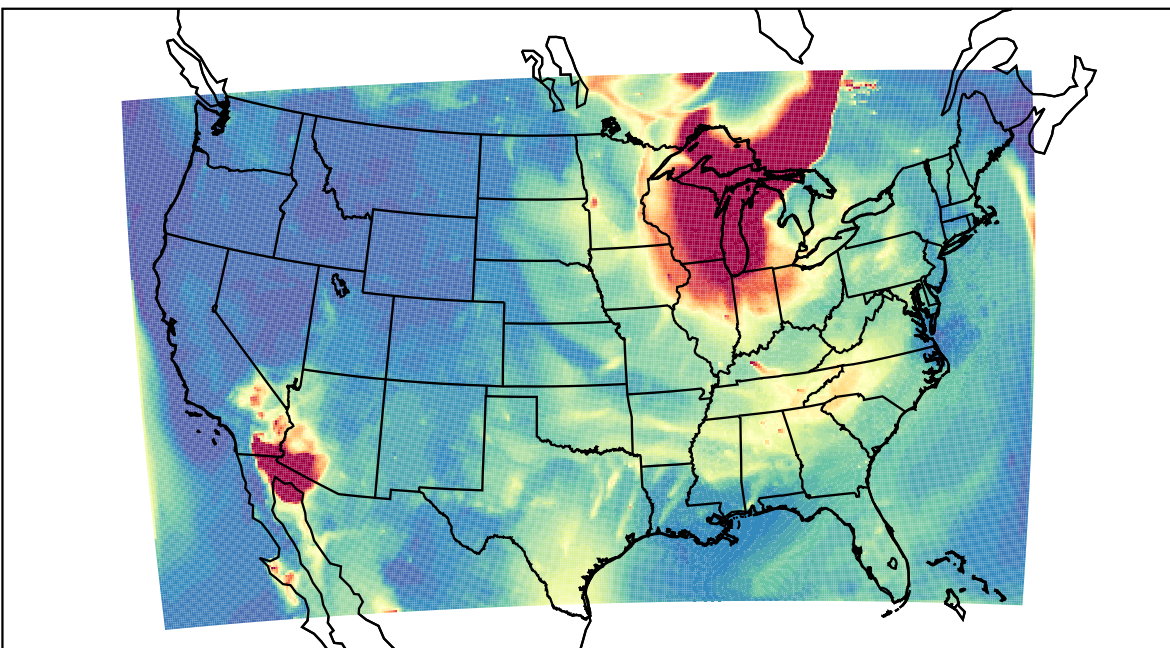
WRF 2023-06-27_09:00:00
