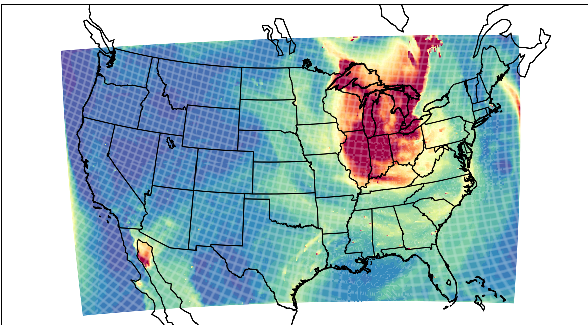
WRF 2023-06-27_21:00:00
