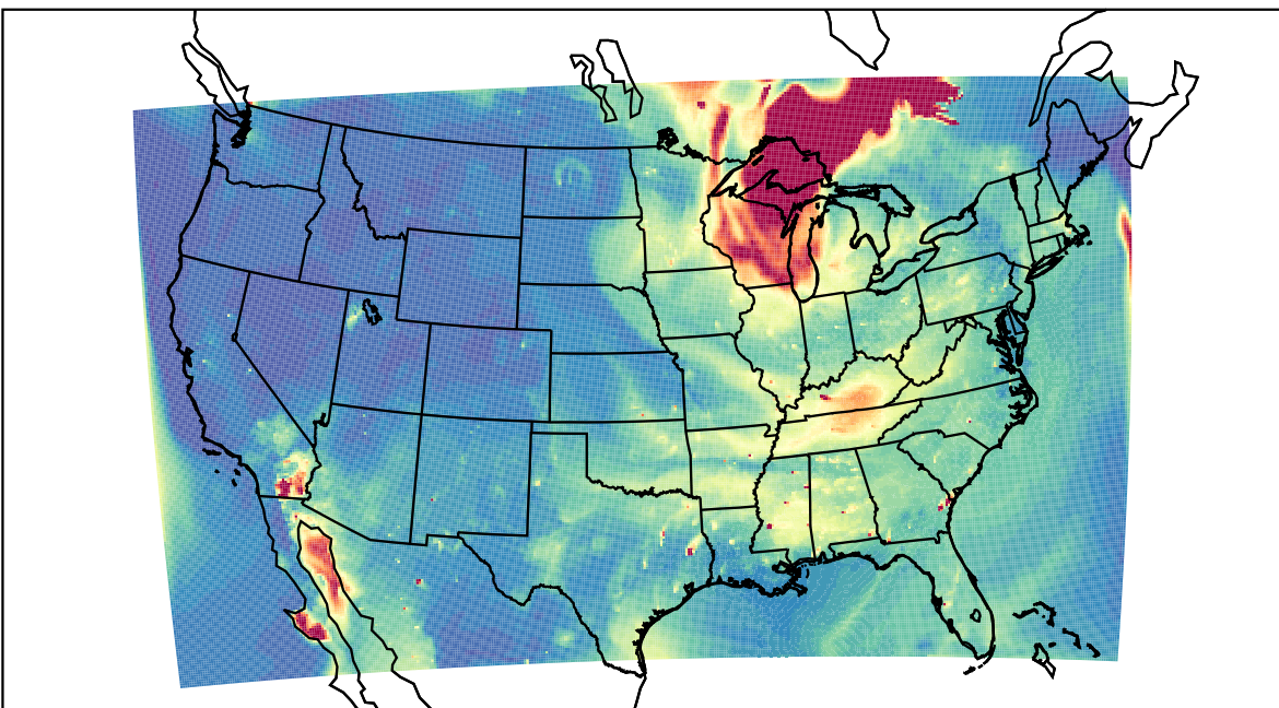
WRF 2023-06-27_01:00:00
