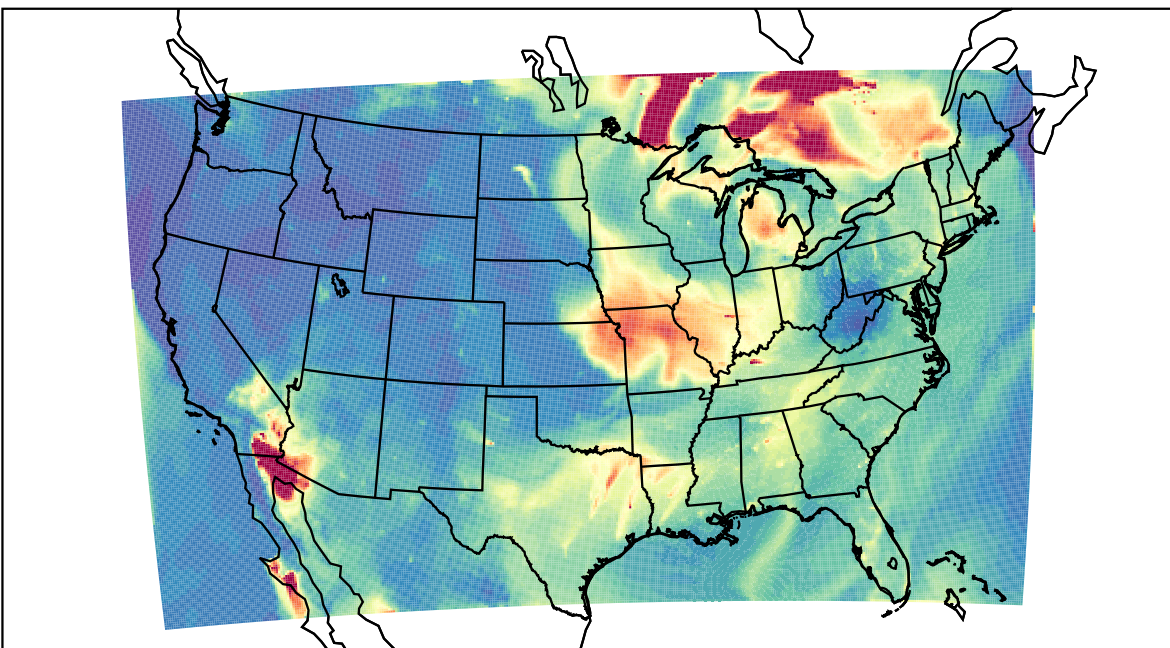
WRF 2023-06-26_11:00:00
