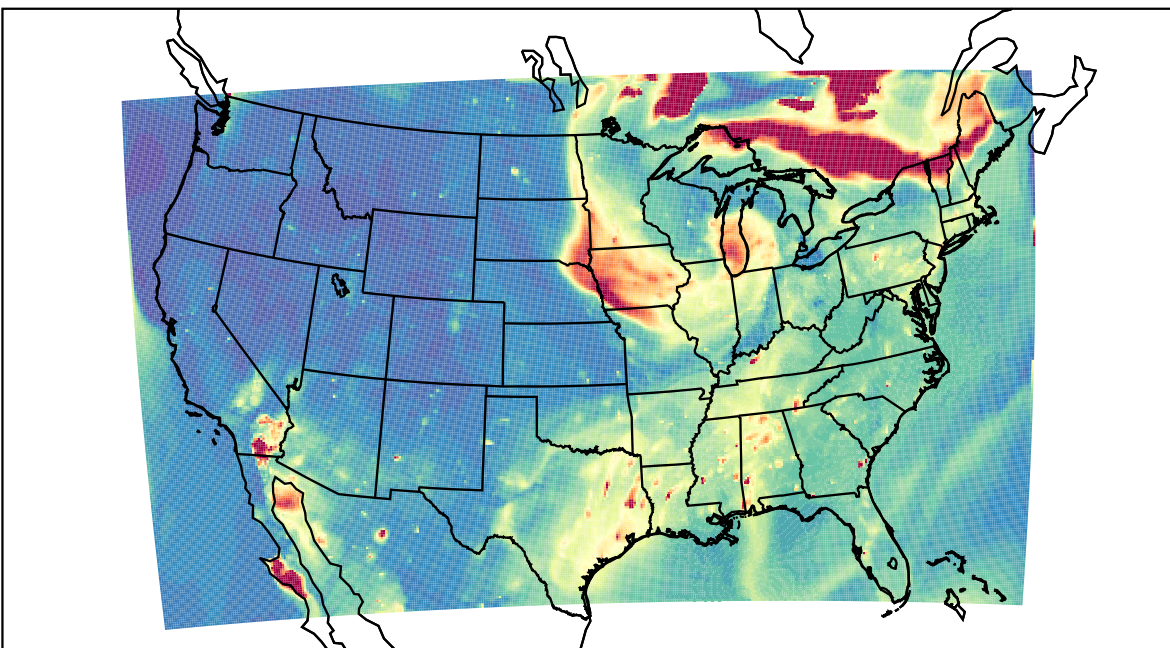
WRF 2023-06-26_02:00:00
