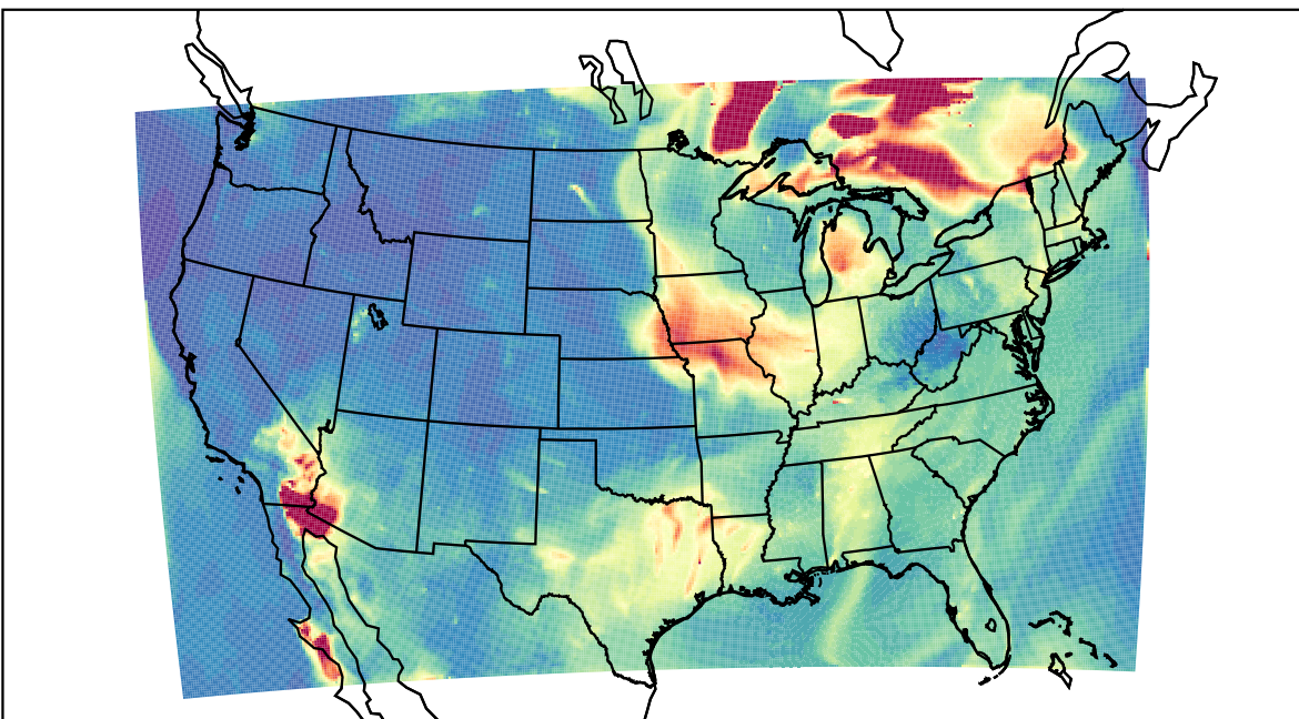
WRF 2023-06-26_08:00:00
