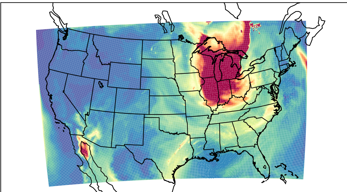
WRF 2023-06-27_17:00:00
