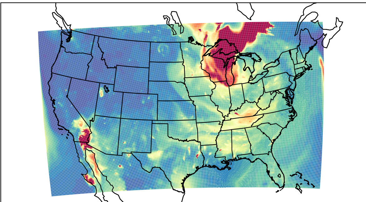
WRF 2023-06-27_03:00:00
