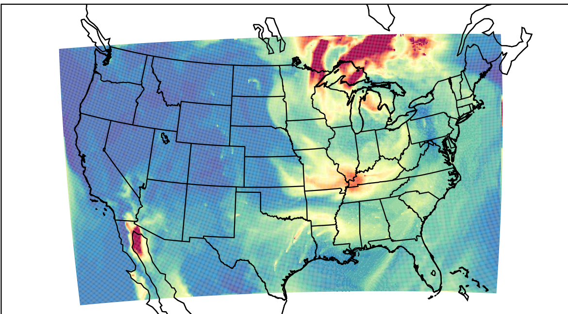
WRF 2023-06-26_17:00:00
