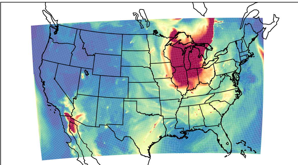
WRF 2023-06-27_14:00:00
