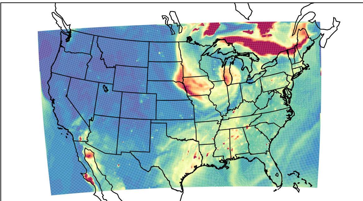
WRF 2023-06-26_01:00:00
