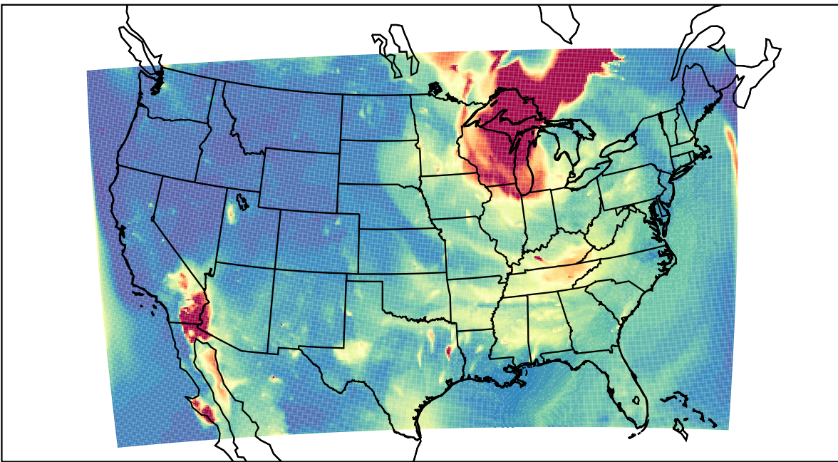
WRF 2023-06-27_04:00:00
