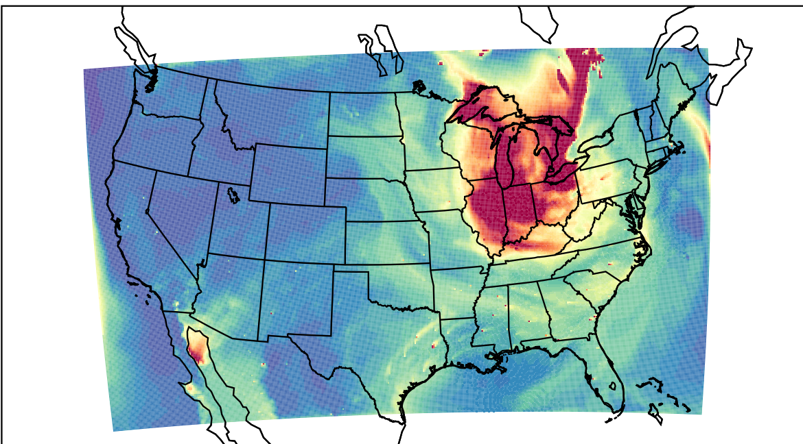
WRF 2023-06-27_22:00:00
