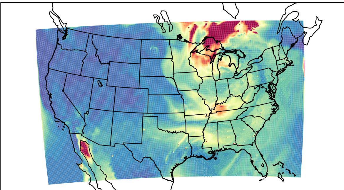
WRF 2023-06-26_20:00:00
