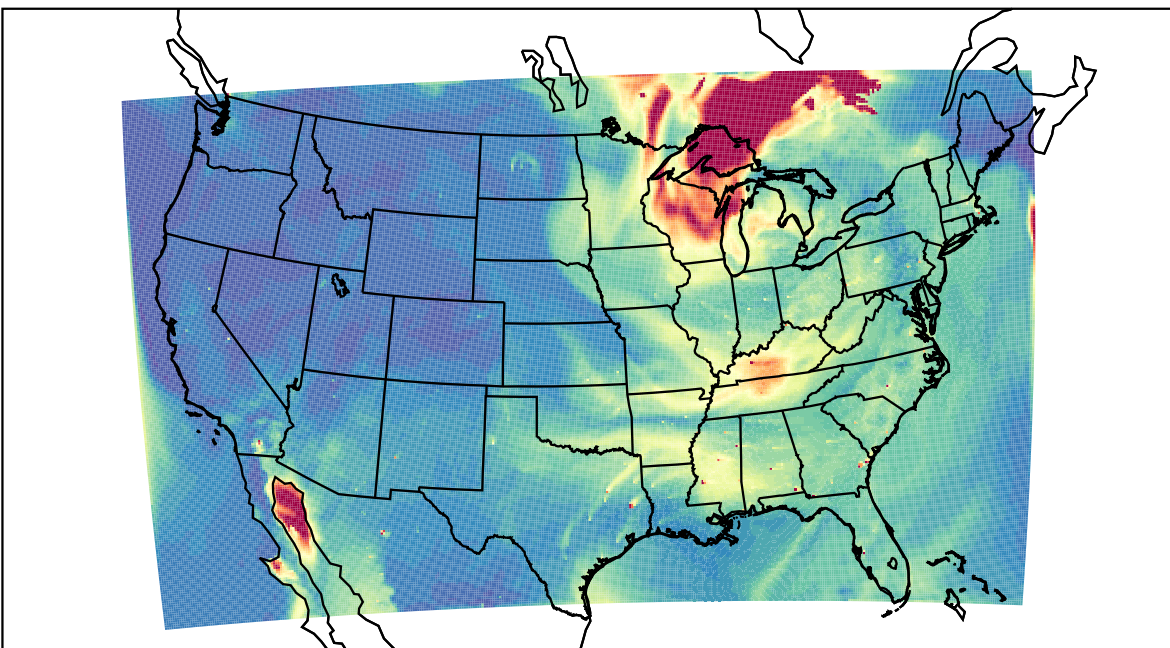
WRF 2023-06-26_22:00:00
