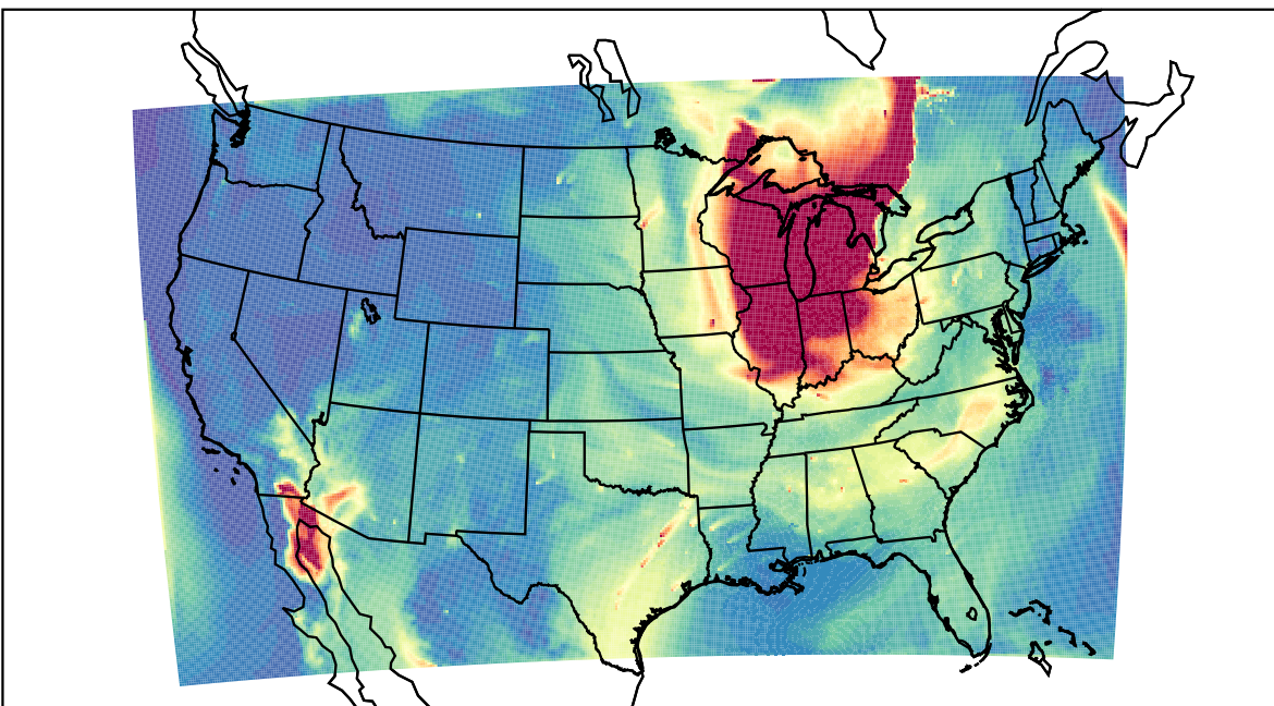
WRF 2023-06-27_15:00:00
