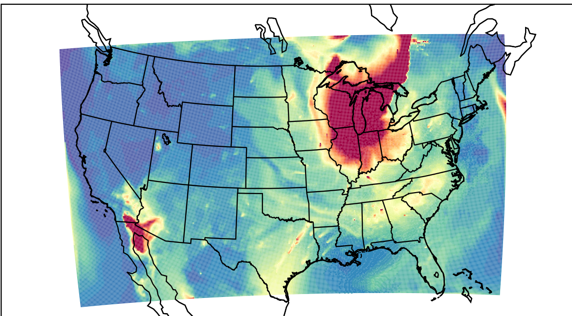
WRF 2023-06-27_13:00:00
