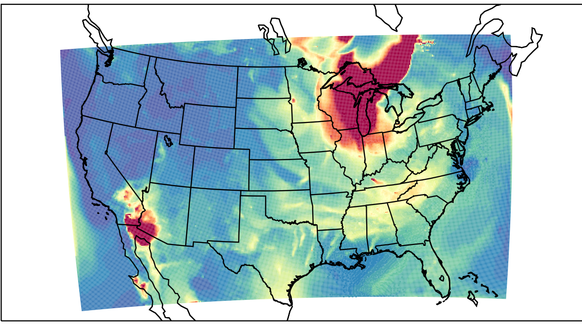
WRF 2023-06-27_08:00:00
