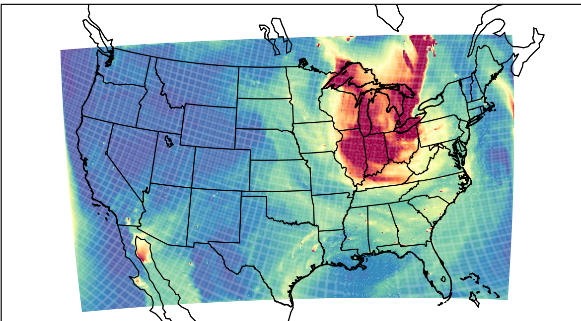
WRF 2023-06-27_23:00:00
