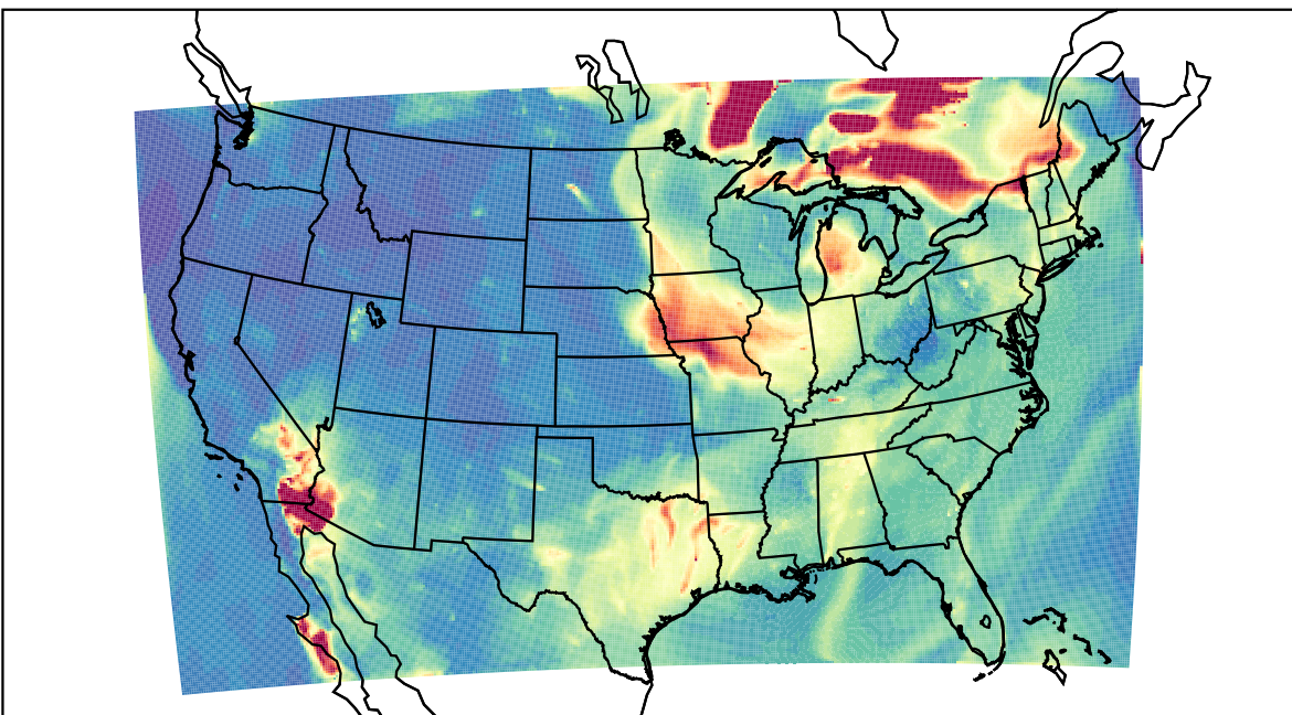
WRF 2023-06-26_07:00:00
