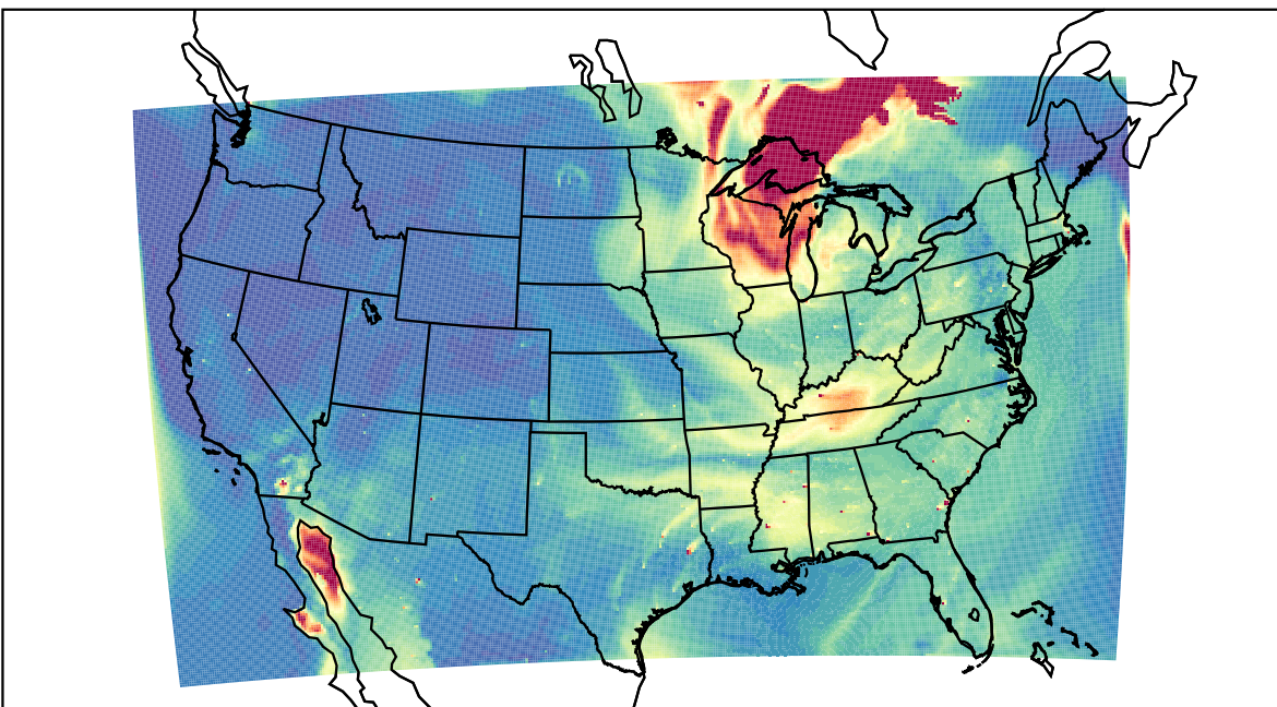
WRF 2023-06-26_23:00:00
