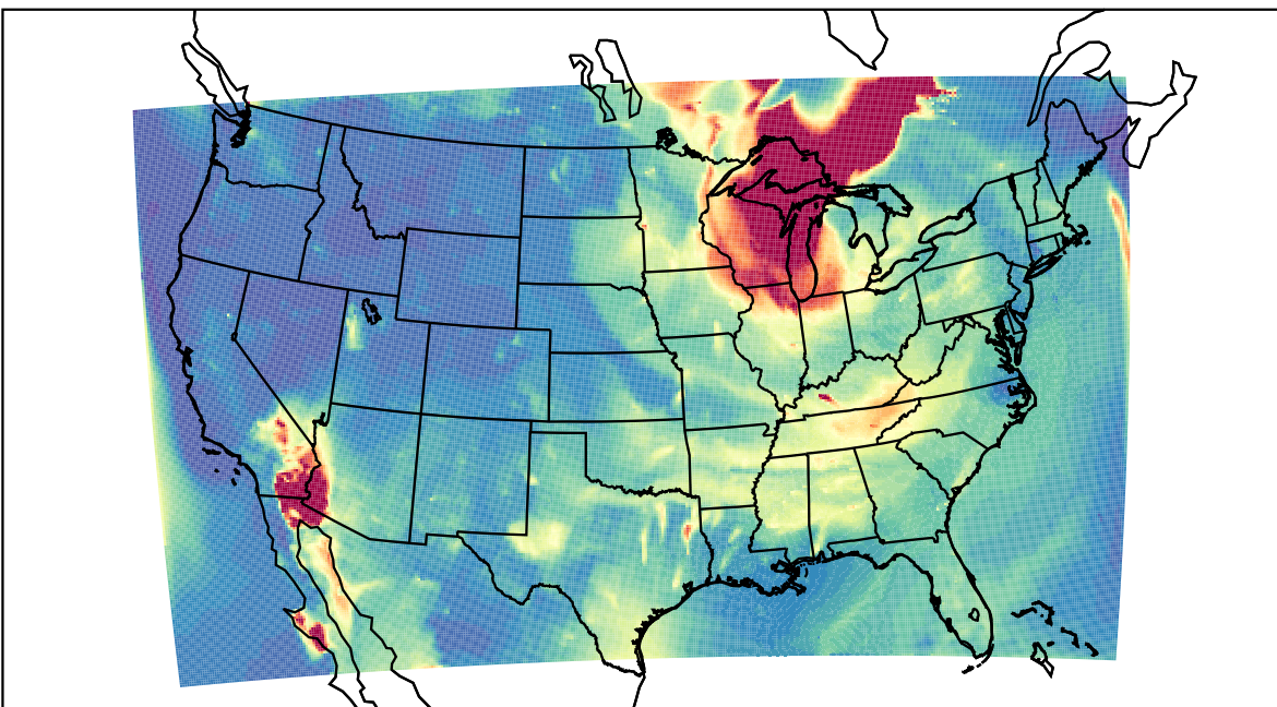
WRF 2023-06-27_05:00:00
