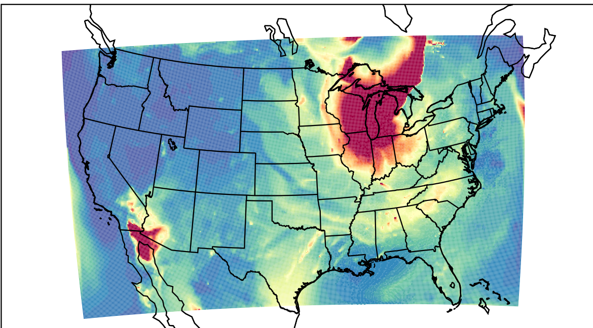
WRF 2023-06-27_12:00:00
