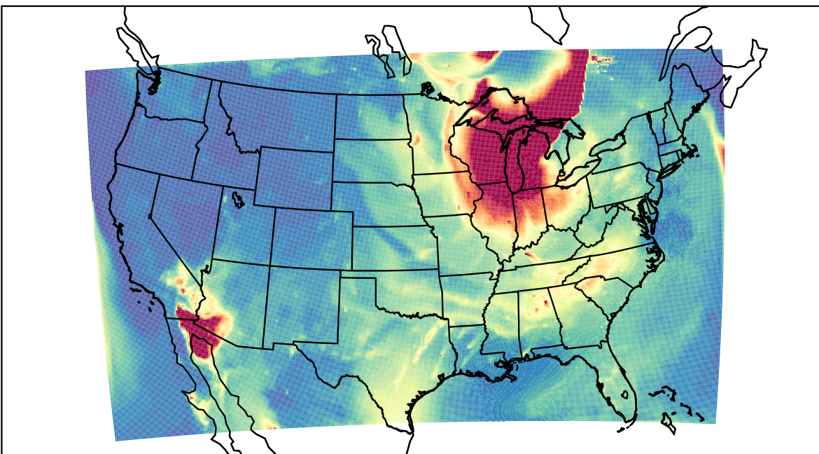
WRF 2023-06-27_11:00:00
