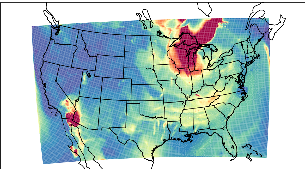
WRF 2023-06-27_06:00:00
