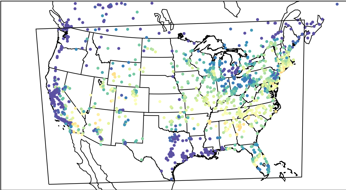
AirNOW (2023-06-27_14:00:00)
