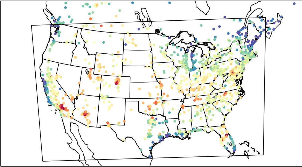
AirNOW (2023-06-26_21:00:00)
