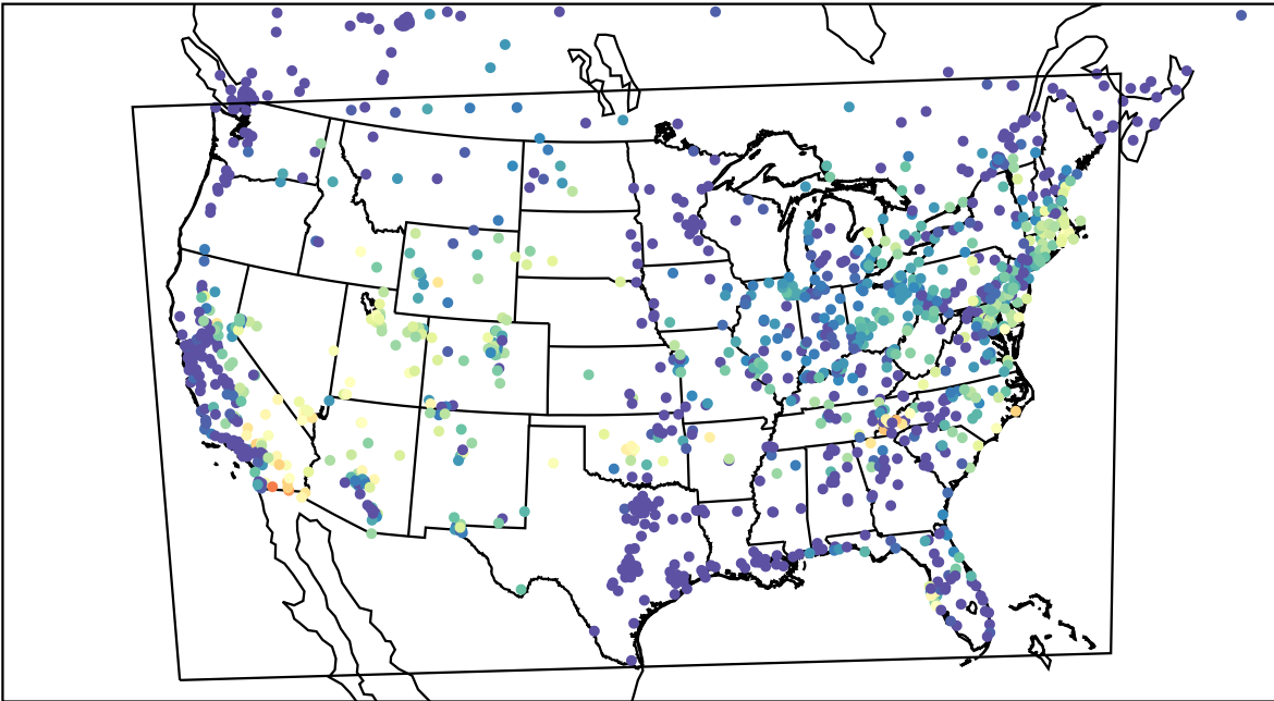
AirNOW (2023-06-27_09:00:00)
