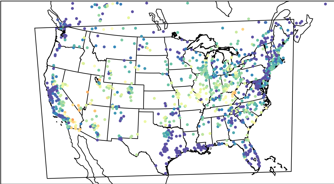
AirNOW (2023-06-26_06:00:00)
