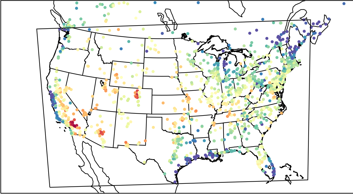
AirNOW (2023-06-27_00:00:00)
