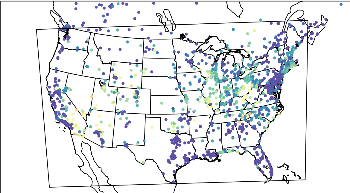
AirNOW (2023-06-26_11:00:00)
