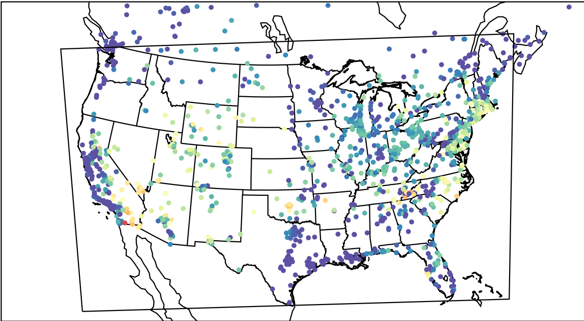
AirNOW (2023-06-27_07:00:00)
