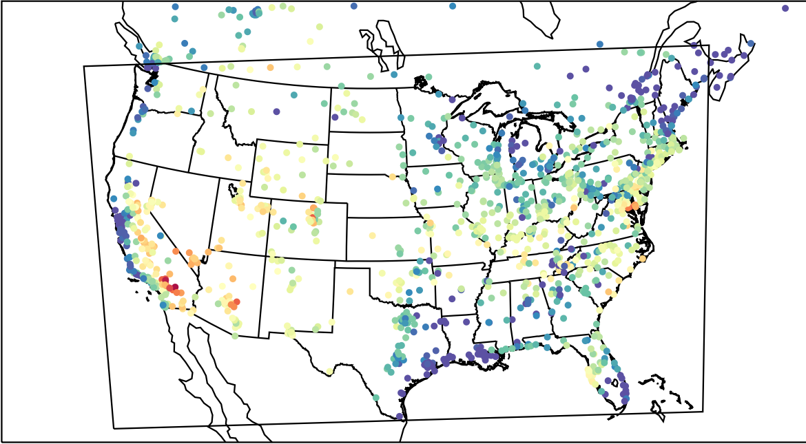
AirNOW (2023-06-27_02:00:00)
