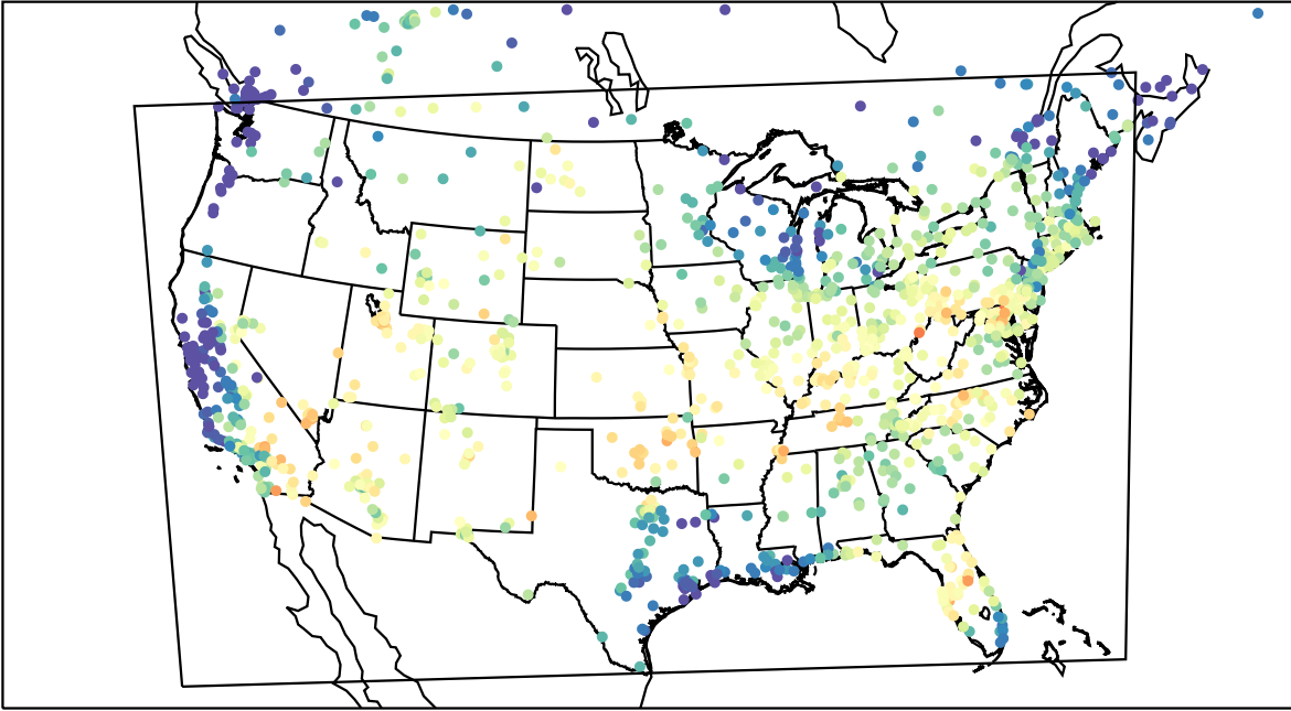
AirNOW (2023-06-26_16:00:00)
