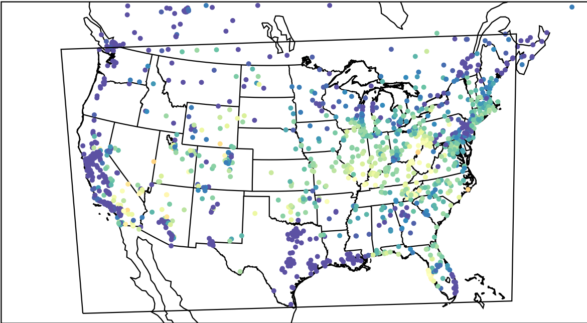
AirNOW (2023-06-26_13:00:00)
