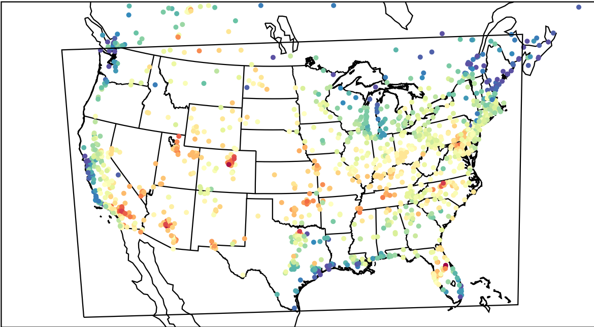
AirNOW (2023-06-26_20:00:00)
