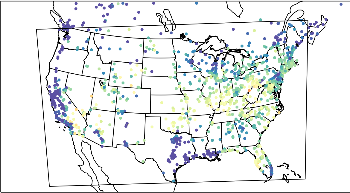
AirNOW (2023-06-26_14:00:00)
