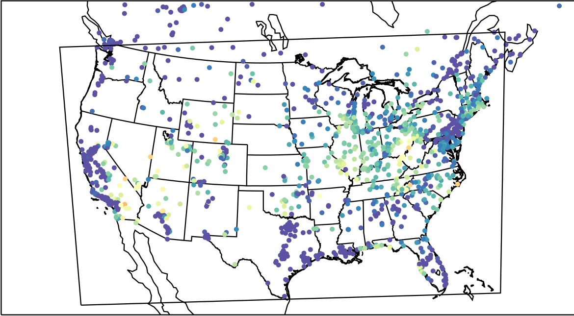
AirNOW (2023-06-26_12:00:00)
