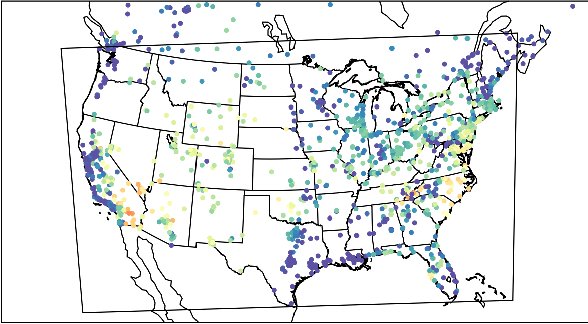
AirNOW (2023-06-27_05:00:00)
