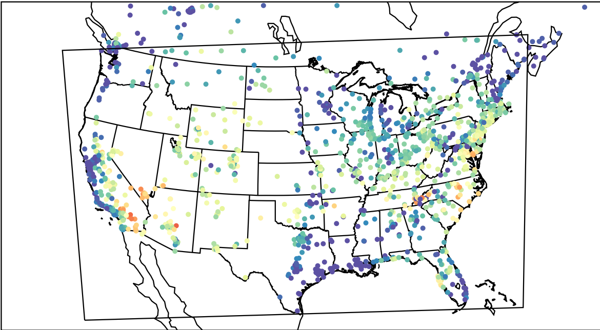
AirNOW (2023-06-27_04:00:00)
