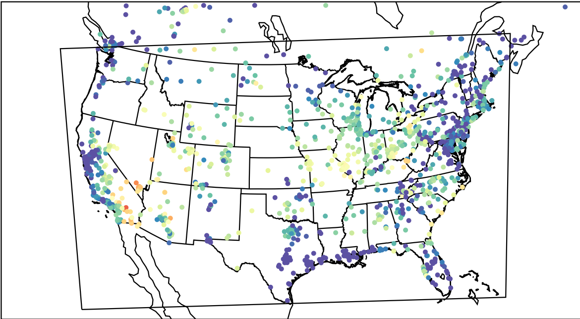
AirNOW (2023-06-26_05:00:00)
