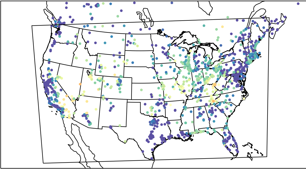
AirNOW (2023-06-26_08:00:00)
