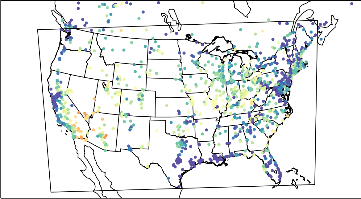
AirNOW (2023-06-26_04:00:00)
