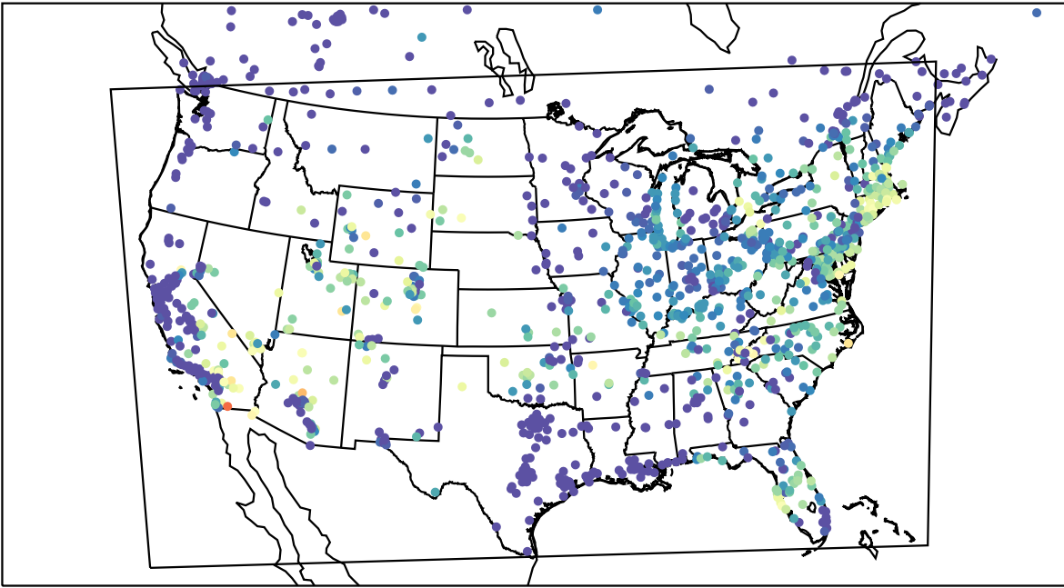
AirNOW (2023-06-27_12:00:00)
