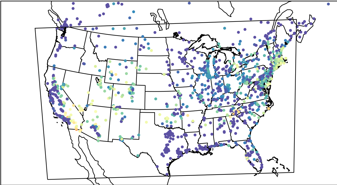
AirNOW (2023-06-27_10:00:00)
