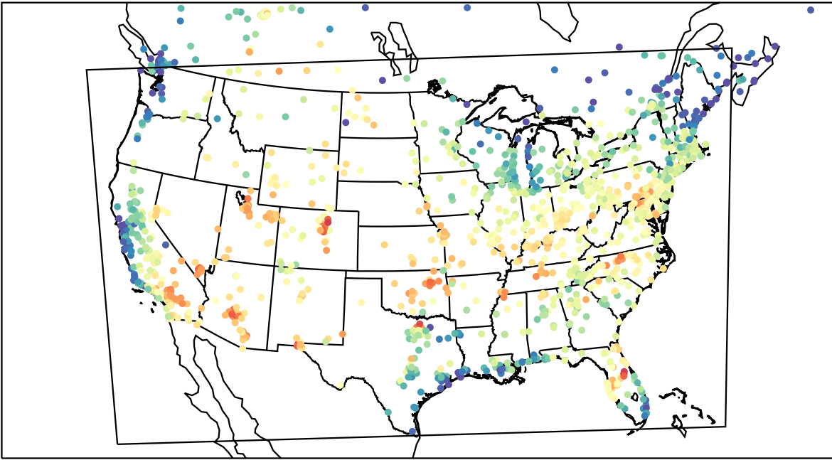
AirNOW (2023-06-26_19:00:00)
