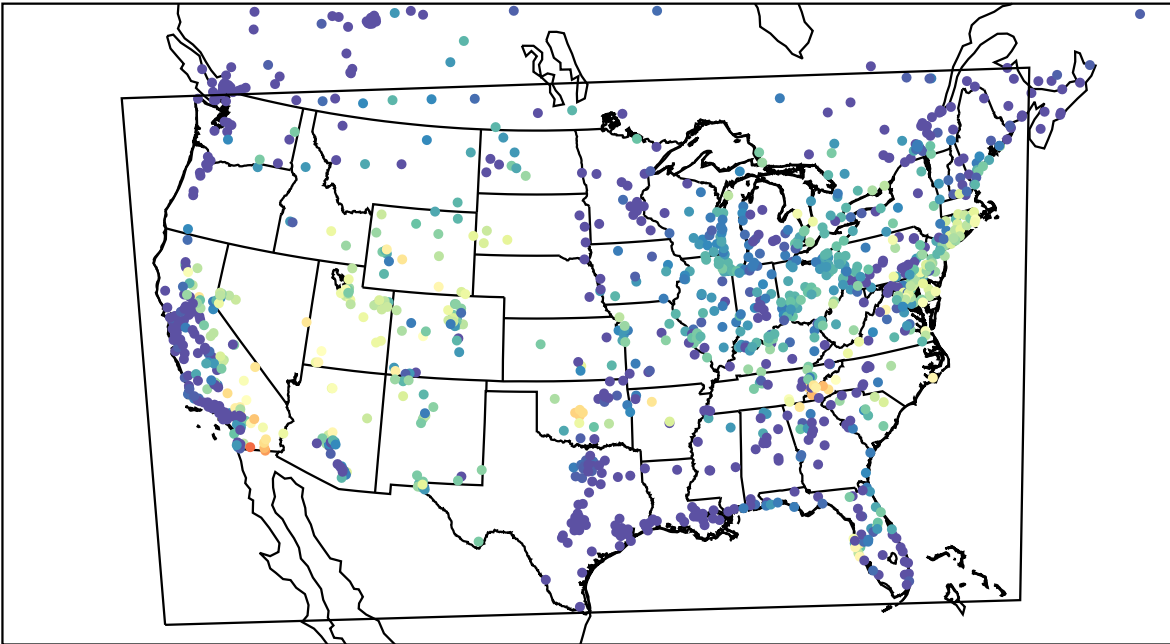
AirNOW (2023-06-27_08:00:00)
