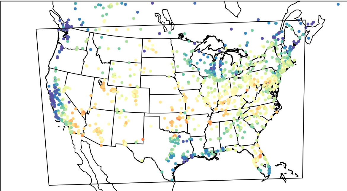
AirNOW (2023-06-26_17:00:00)
