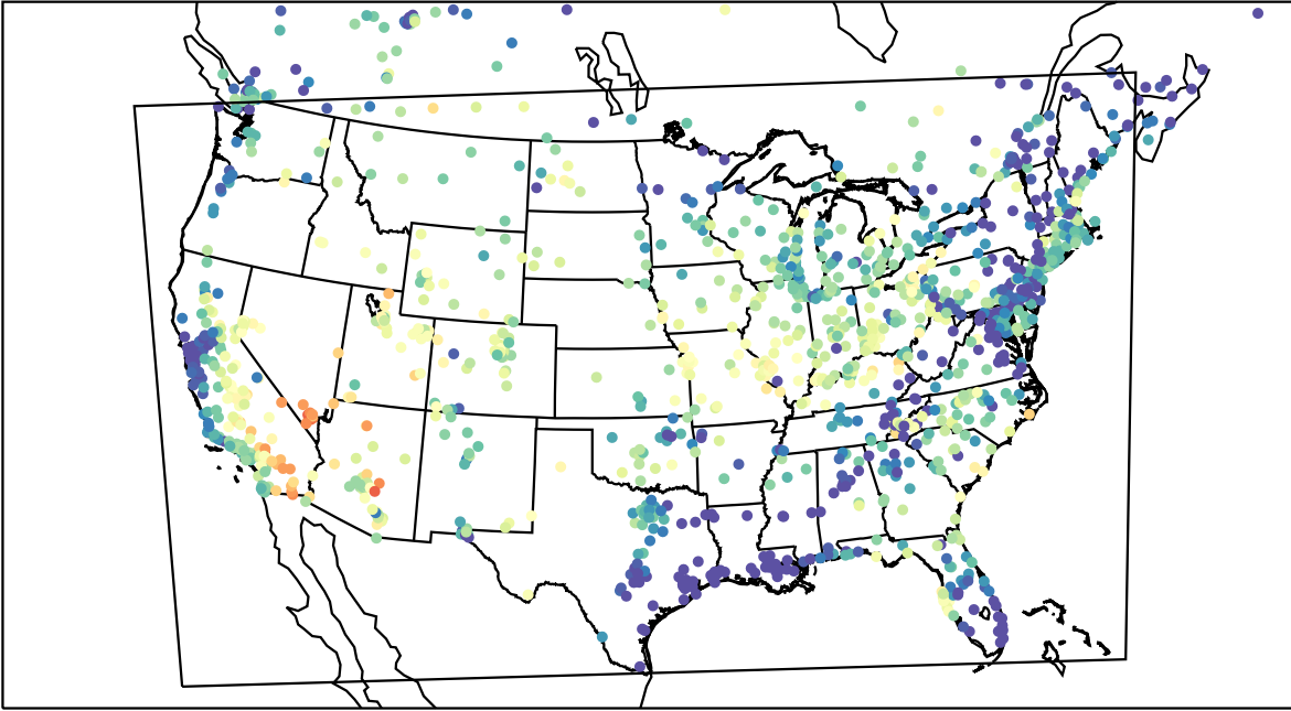
AirNOW (2023-06-26_03:00:00)
