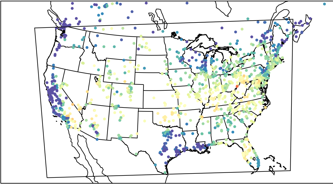
AirNOW (2023-06-26_15:00:00)
