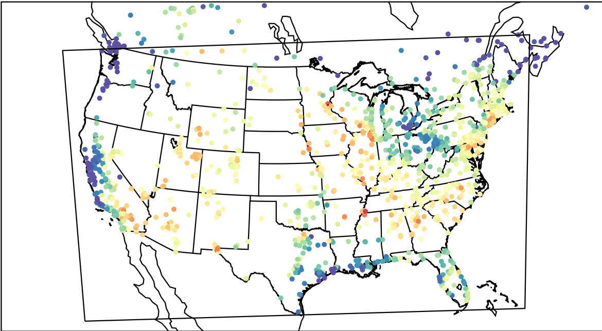
AirNOW (2023-06-27_17:00:00)
