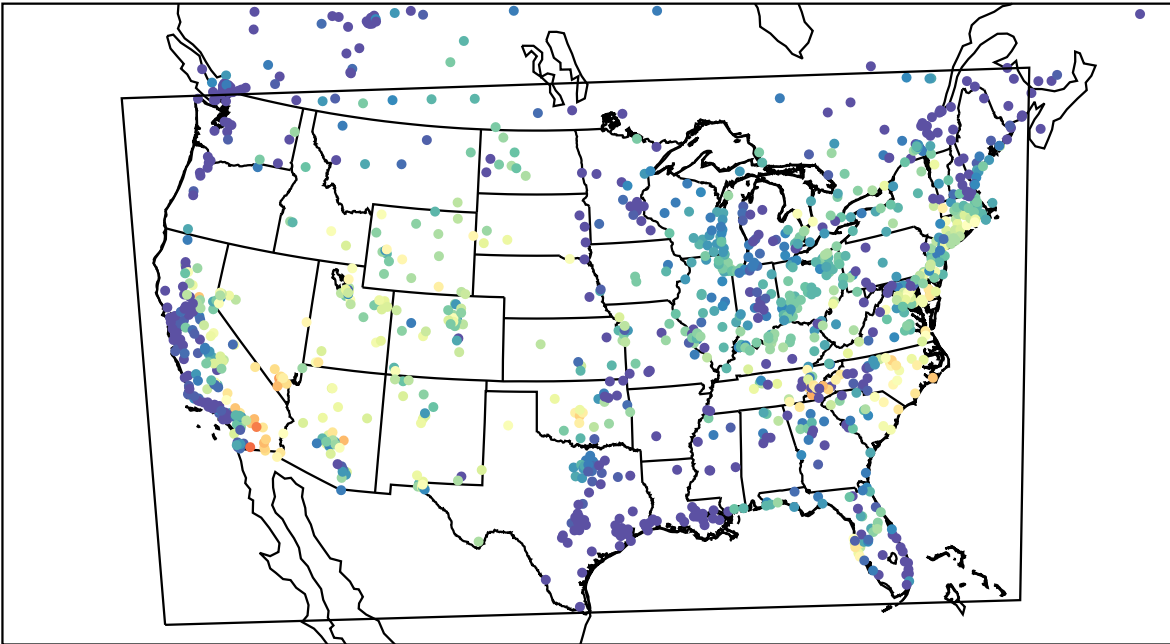
AirNOW (2023-06-27_06:00:00)
