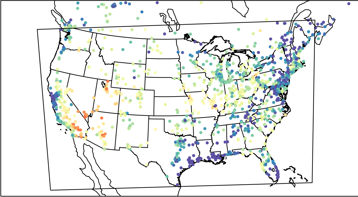
AirNOW (2023-06-26_02:00:00)
