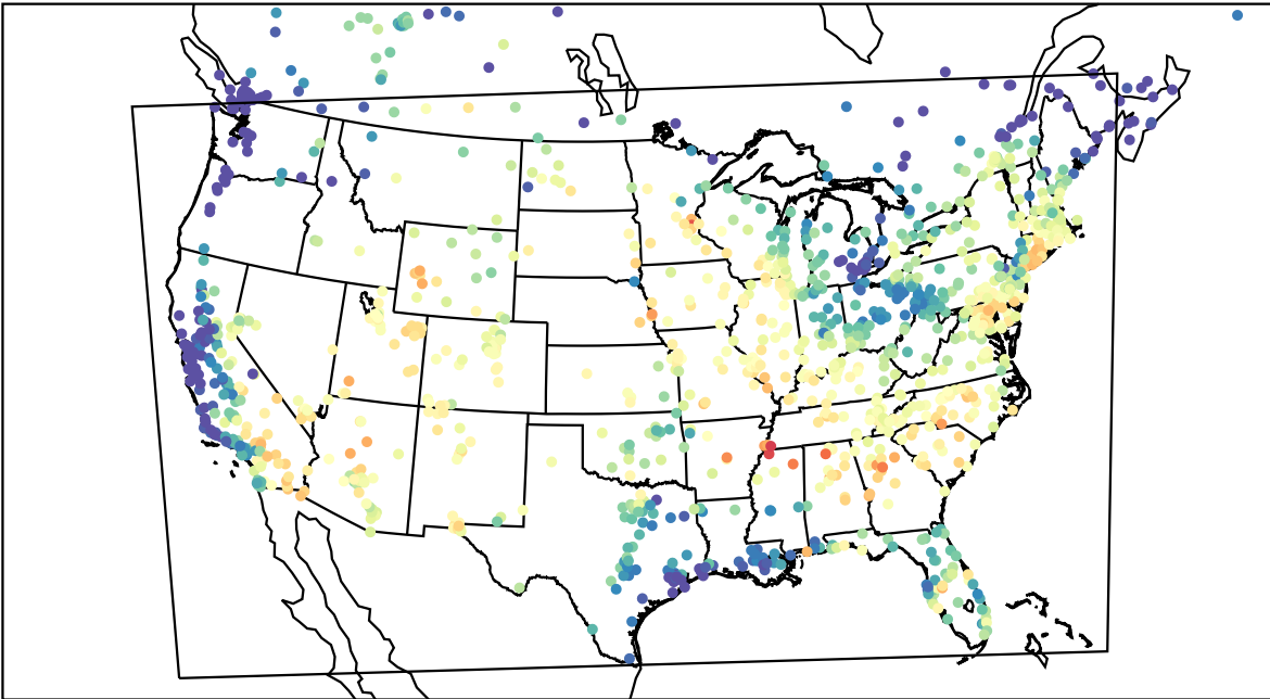
AirNOW (2023-06-27_16:00:00)
