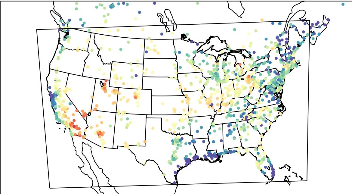
AirNOW (2023-06-26_00:00:00)
