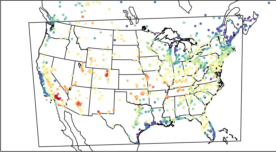
AirNOW (2023-06-26_23:00:00)
