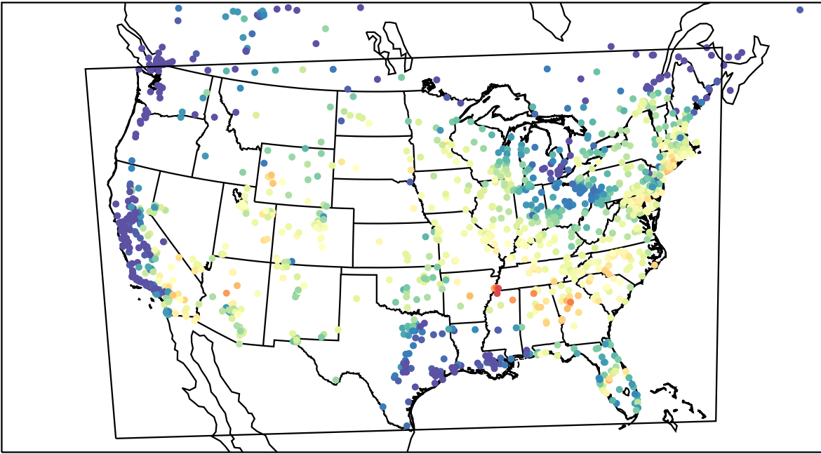
AirNOW (2023-06-27_15:00:00)
