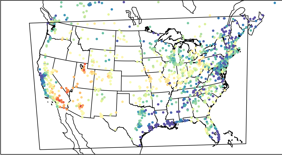
AirNOW (2023-06-26_01:00:00)
