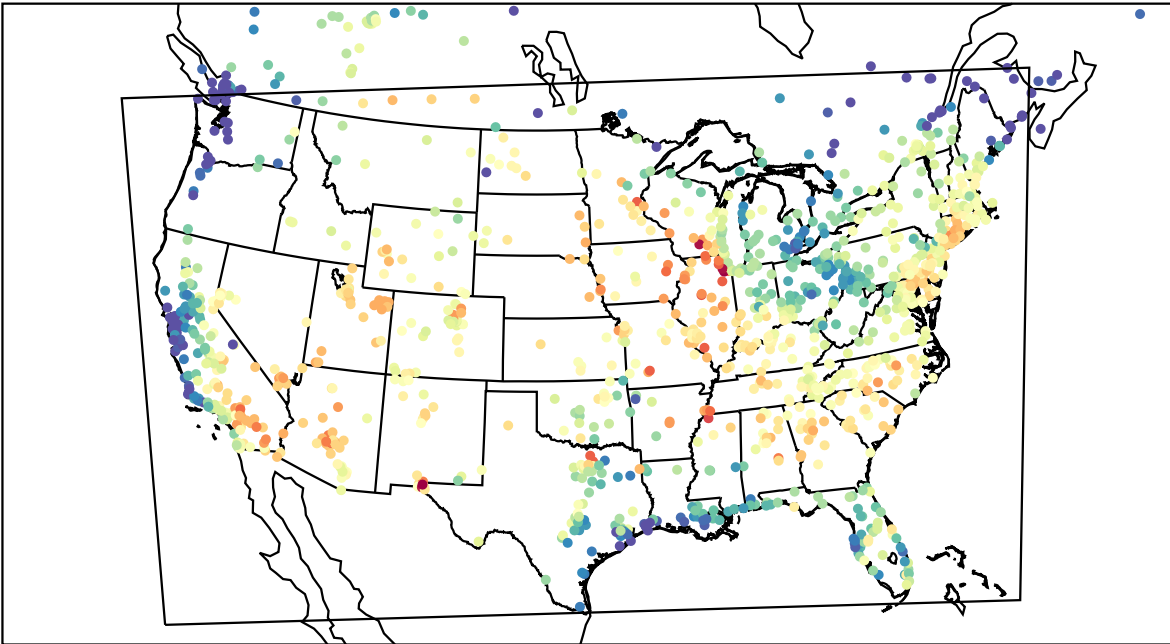
AirNOW (2023-06-27_18:00:00)
