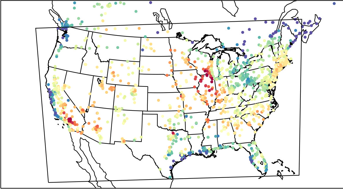
AirNOW (2023-06-27_21:00:00)
