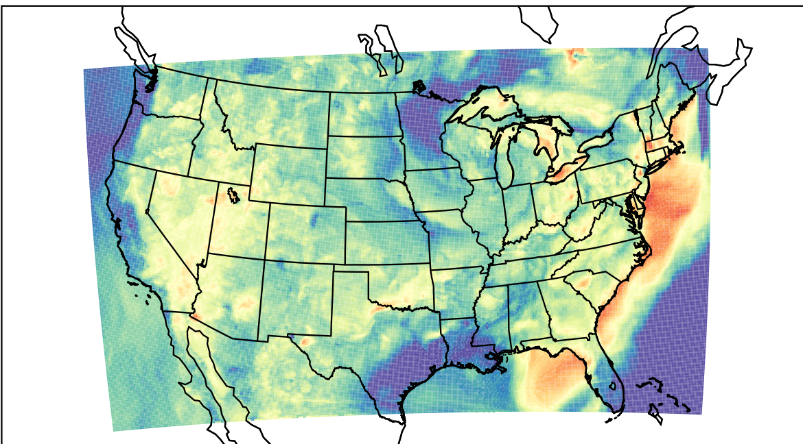
WRF (2023-06-26_04:00:00)
