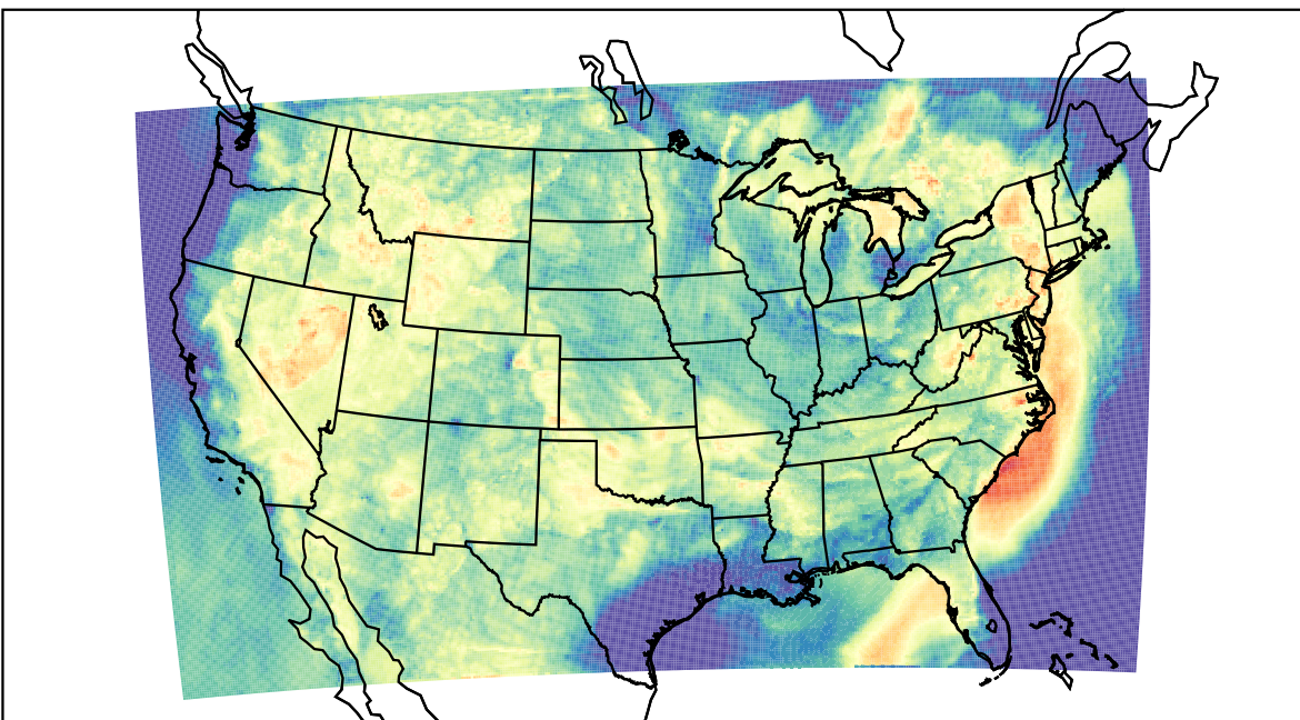
WRF (2023-06-27_04:00:00)
