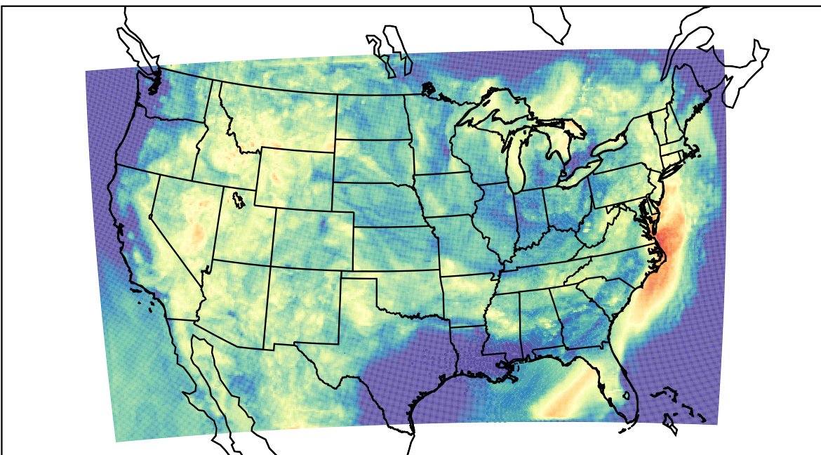
WRF (2023-06-27_08:00:00)
