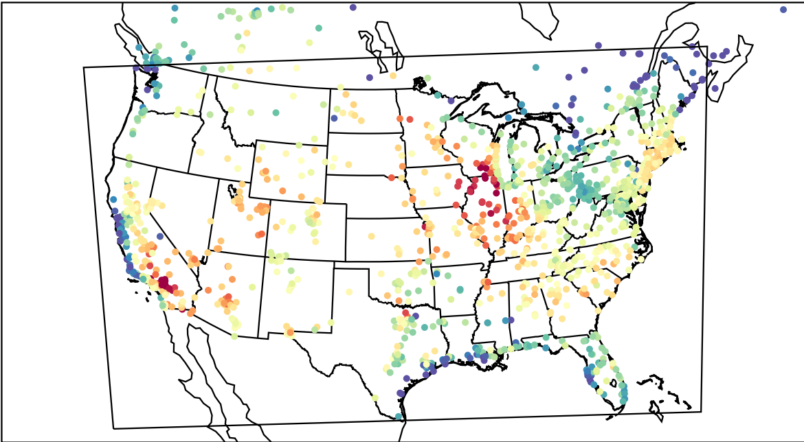
AirNOW (2023-06-27_22:00:00)
