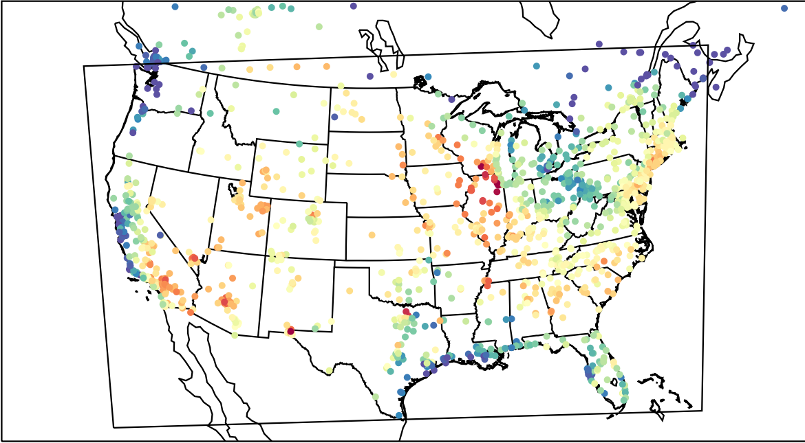
AirNOW (2023-06-27_19:00:00)
