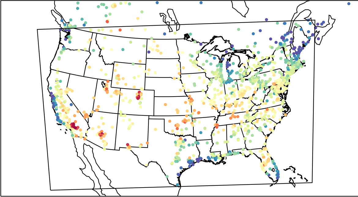
AirNOW (2023-06-26_22:00:00)
