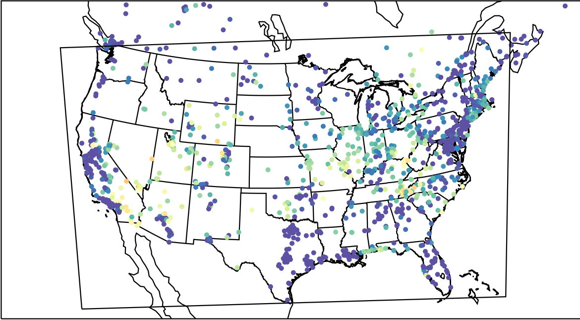
AirNOW (2023-06-26_10:00:00)
