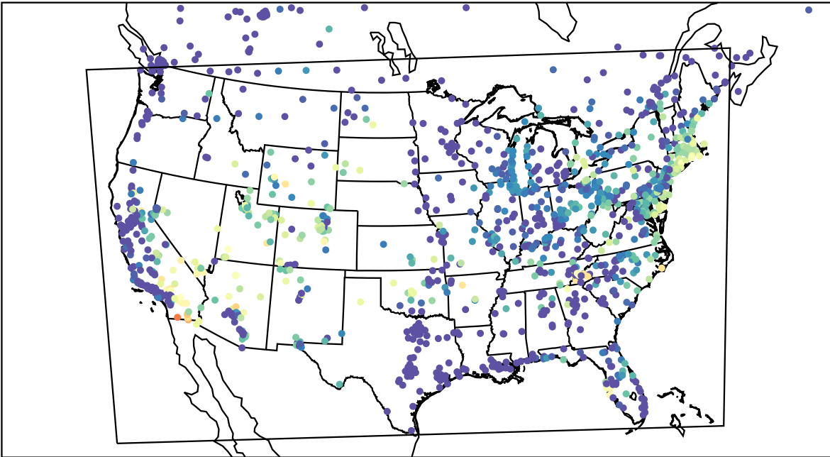
AirNOW (2023-06-27_11:00:00)
