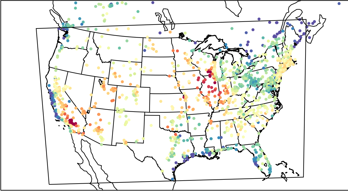
AirNOW (2023-06-27_23:00:00)
