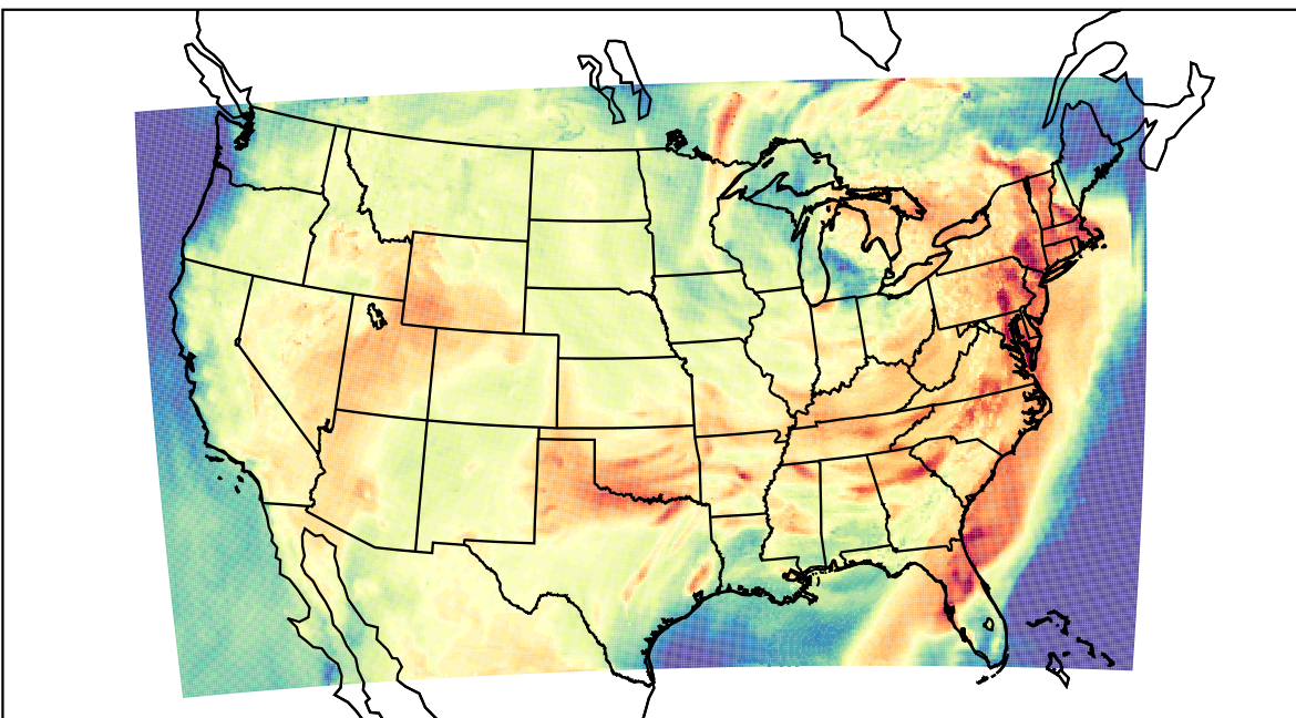
WRF (2023-06-26_19:00:00)
