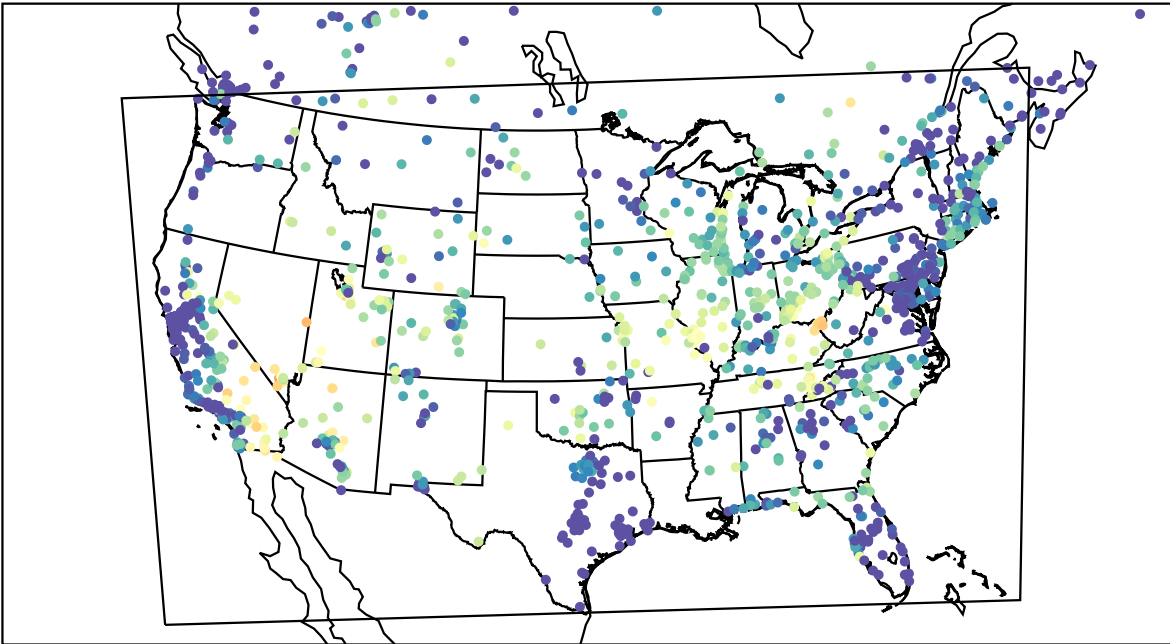
AirNOW (2023-06-26_07:00:00)
