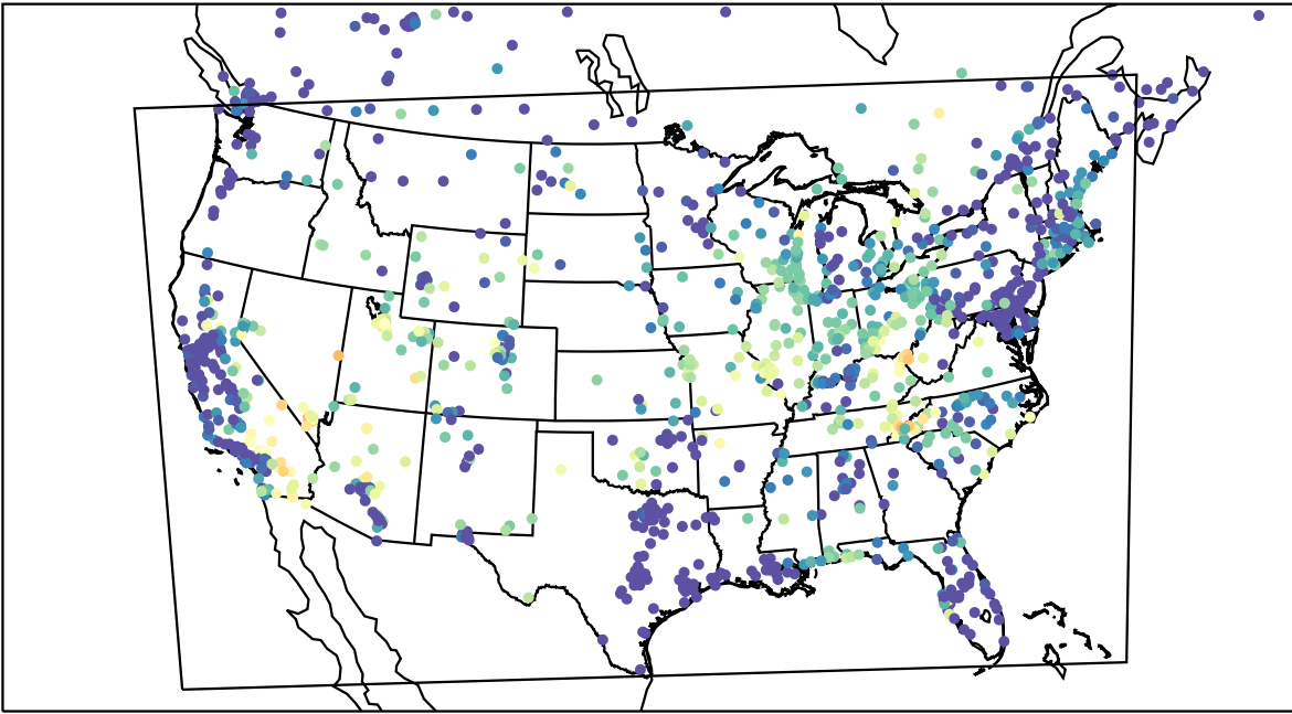
AirNOW (2023-06-26_09:00:00)
