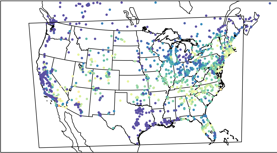
AirNOW (2023-06-27_13:00:00)
