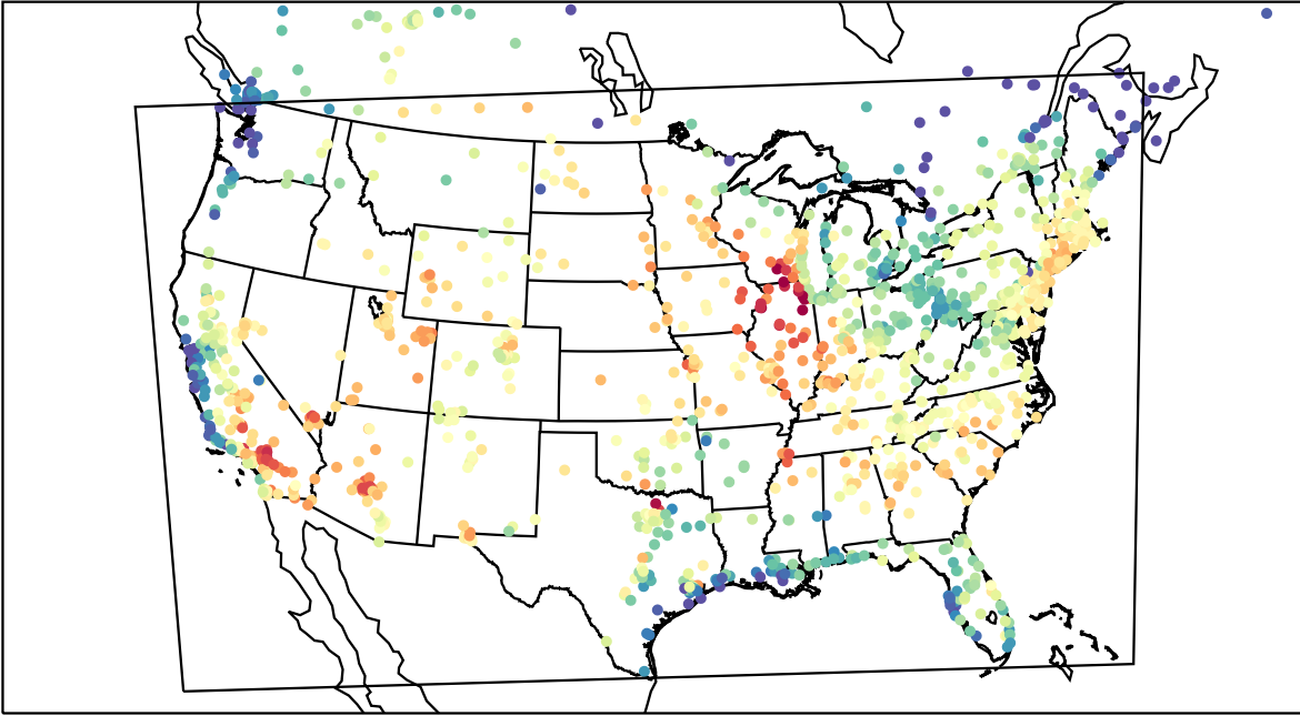
AirNOW (2023-06-27_20:00:00)
