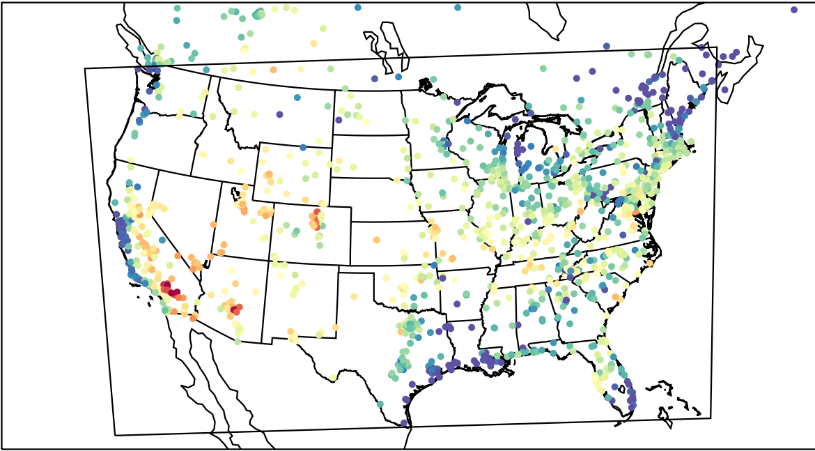
AirNOW (2023-06-27_01:00:00)
