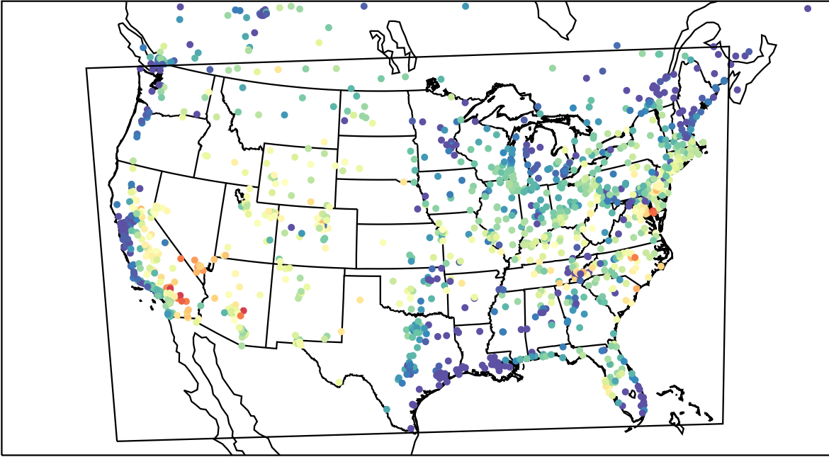
AirNOW (2023-06-27_03:00:00)
