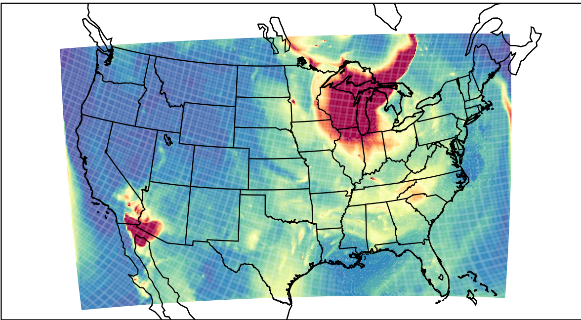
WRF 2023-06-27_10:00:00
