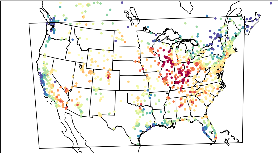
AirNOW (2023-06-28_19:00:00)
