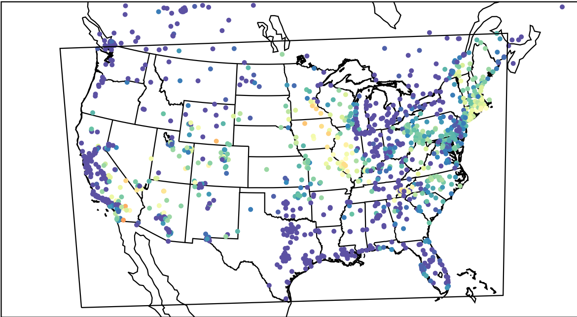
AirNOW (2023-06-28_12:00:00)
