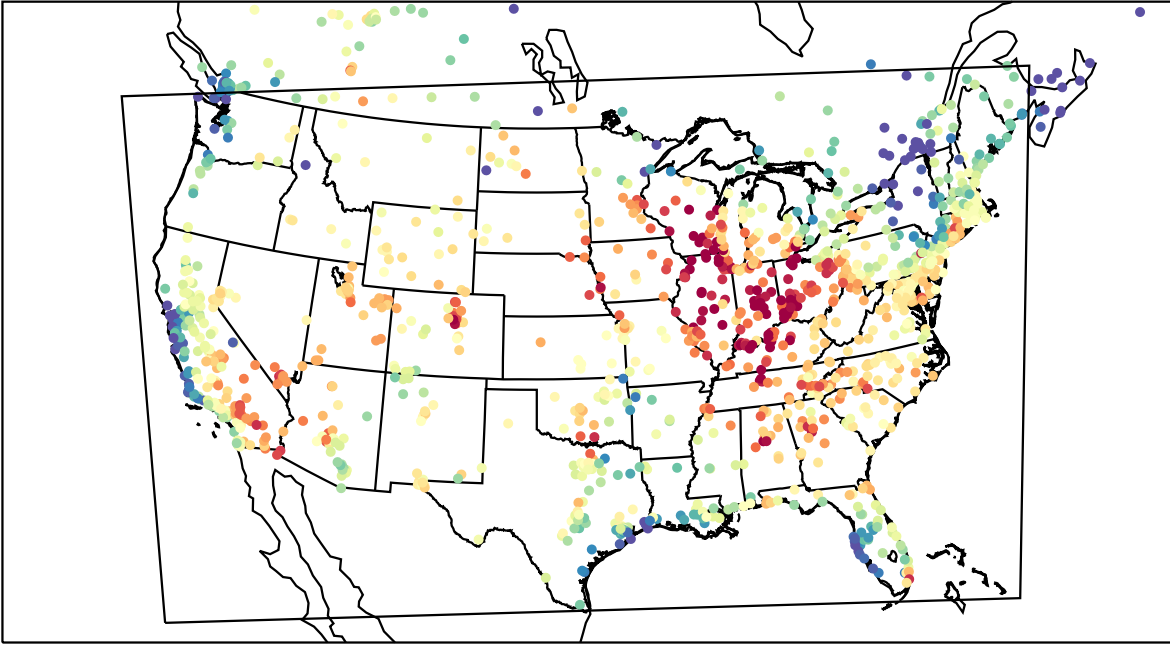
AirNOW (2023-06-28_20:00:00)
