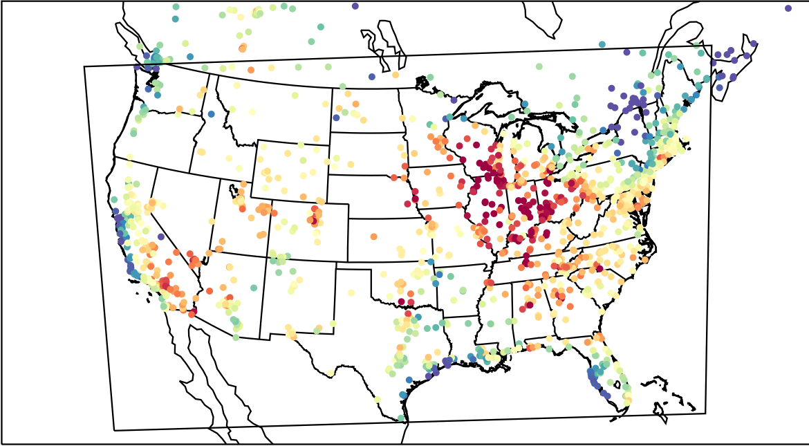
AirNOW (2023-06-28_21:00:00)
