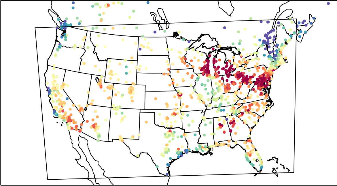
AirNOW (2023-06-29_20:00:00)
