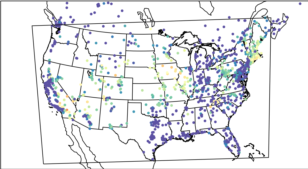
AirNOW (2023-06-28_10:00:00)
