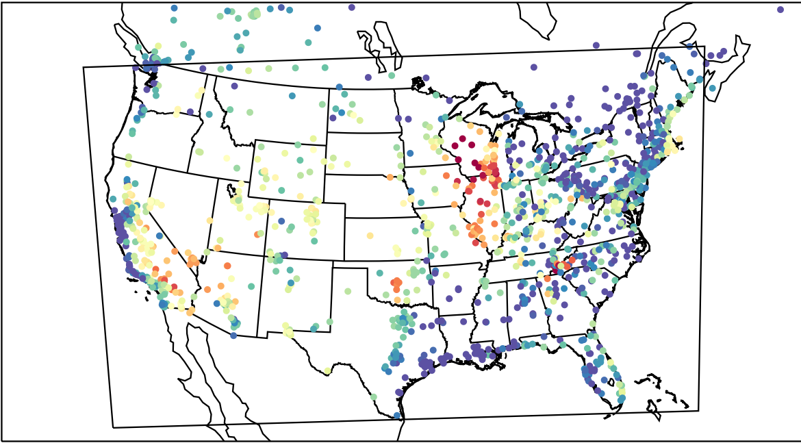
AirNOW (2023-06-29_03:00:00)
