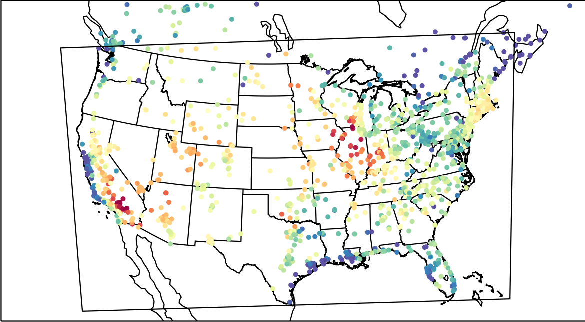
AirNOW (2023-06-28_00:00:00)
