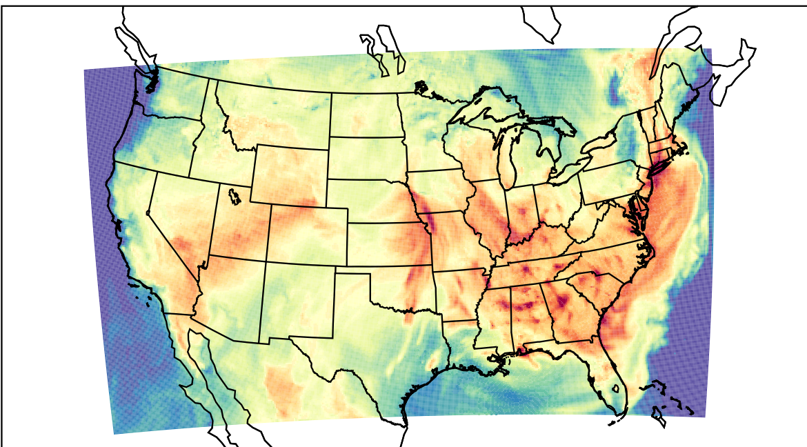
WRF (2023-06-28_18:00:00)
