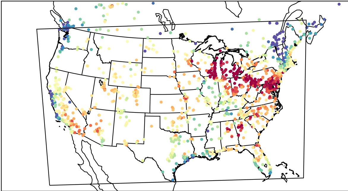
AirNOW (2023-06-29_19:00:00)
