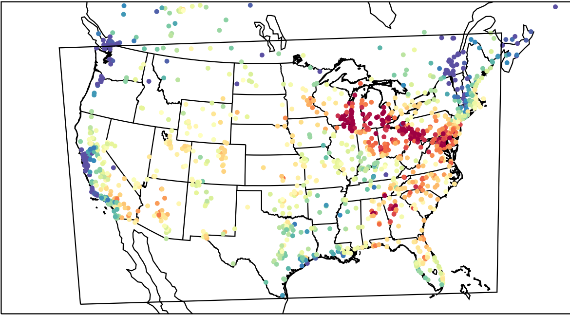
AirNOW (2023-06-29_17:00:00)
