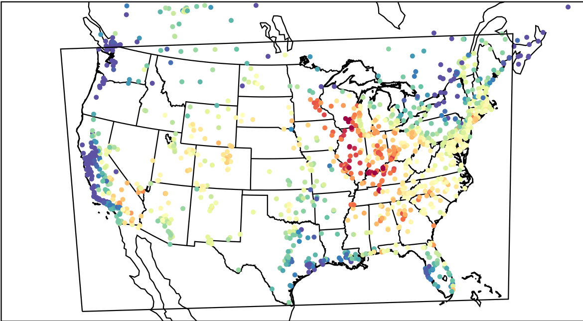
AirNOW (2023-06-28_16:00:00)
