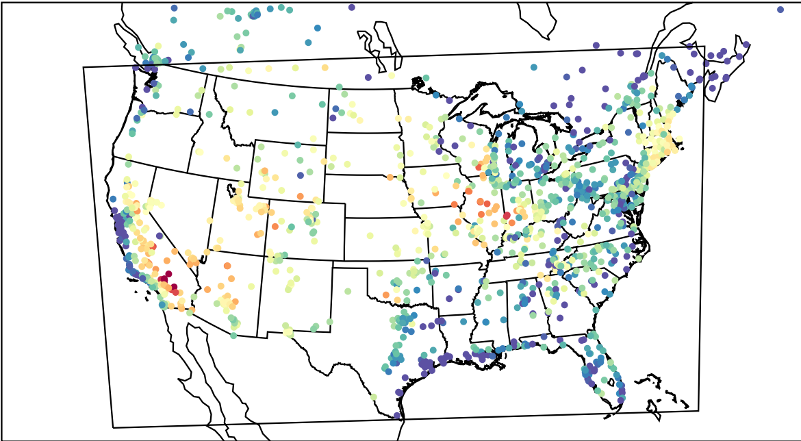
AirNOW (2023-06-28_02:00:00)
