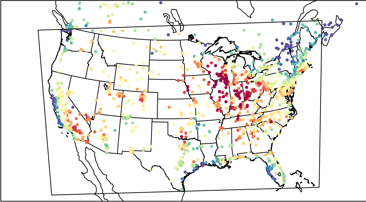
AirNOW (2023-06-28_22:00:00)
