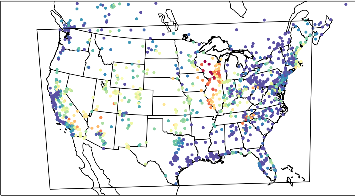
AirNOW (2023-06-29_05:00:00)
