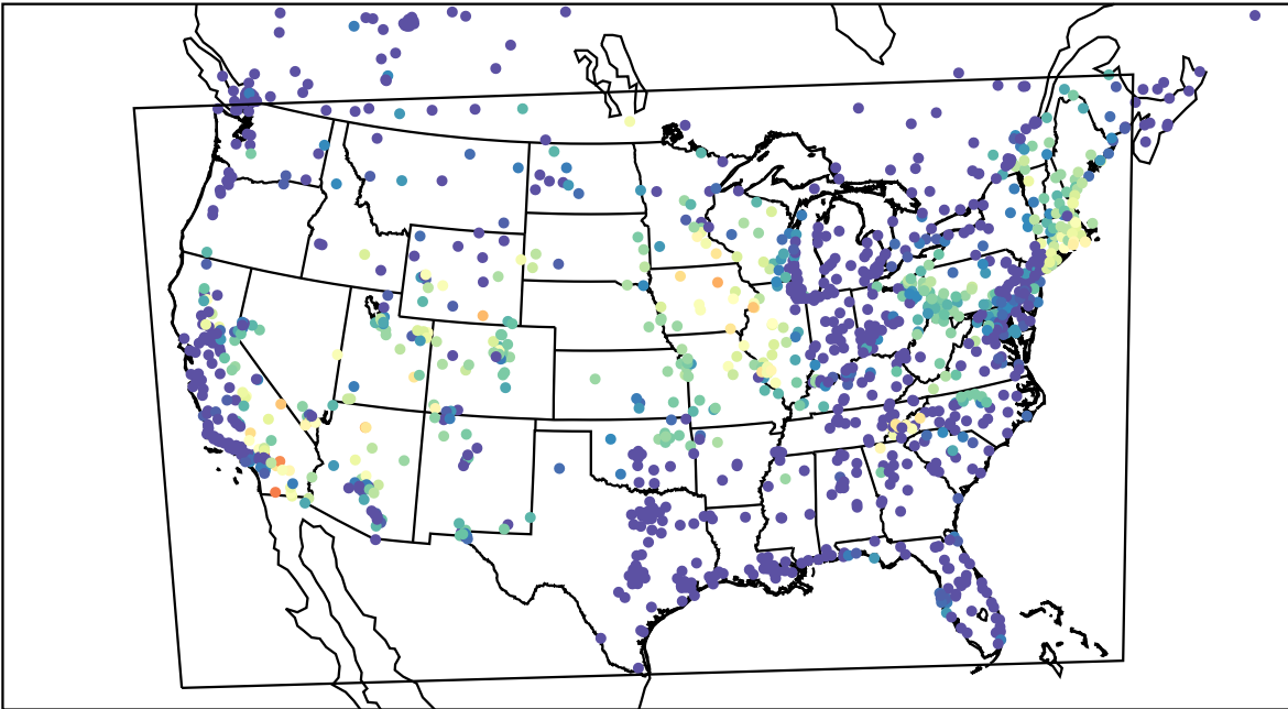
AirNOW (2023-06-28_11:00:00)
