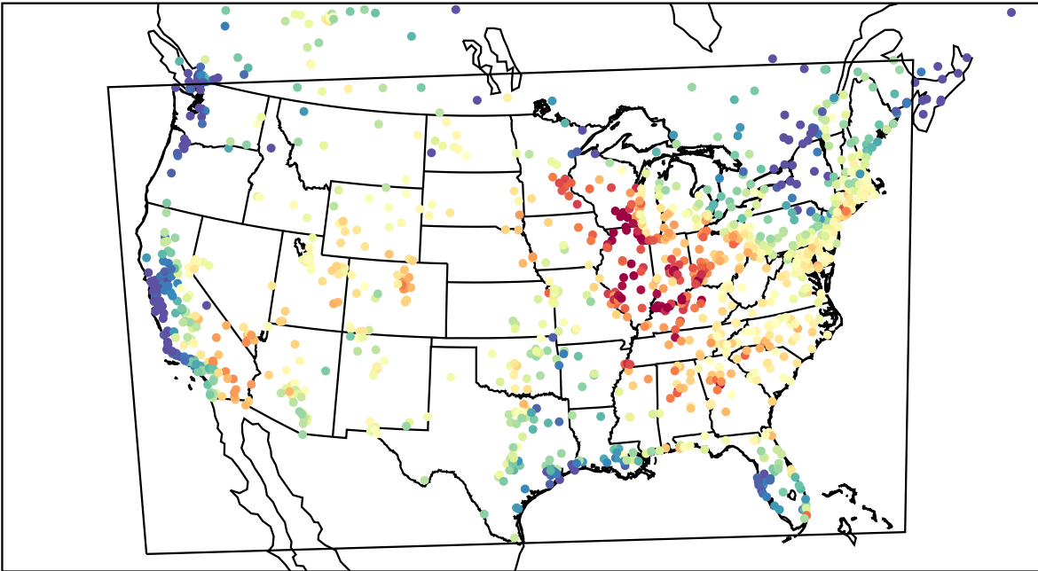
AirNOW (2023-06-28_17:00:00)
