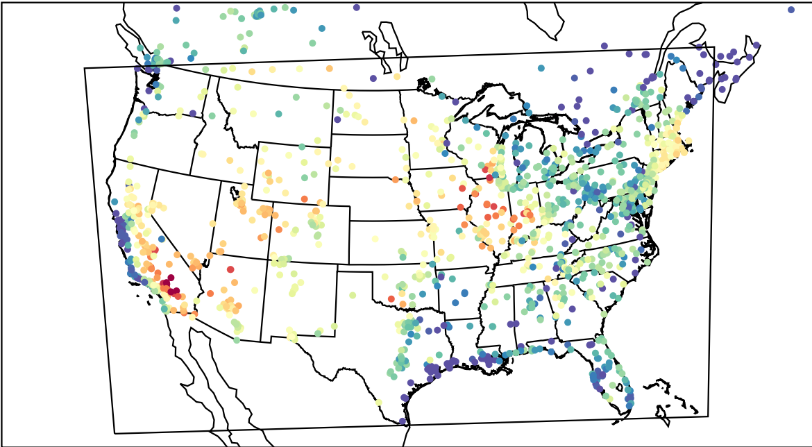
AirNOW (2023-06-28_01:00:00)
