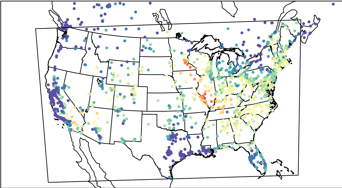
AirNOW (2023-06-28_14:00:00)
