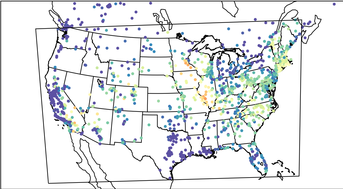
AirNOW (2023-06-28_13:00:00)
