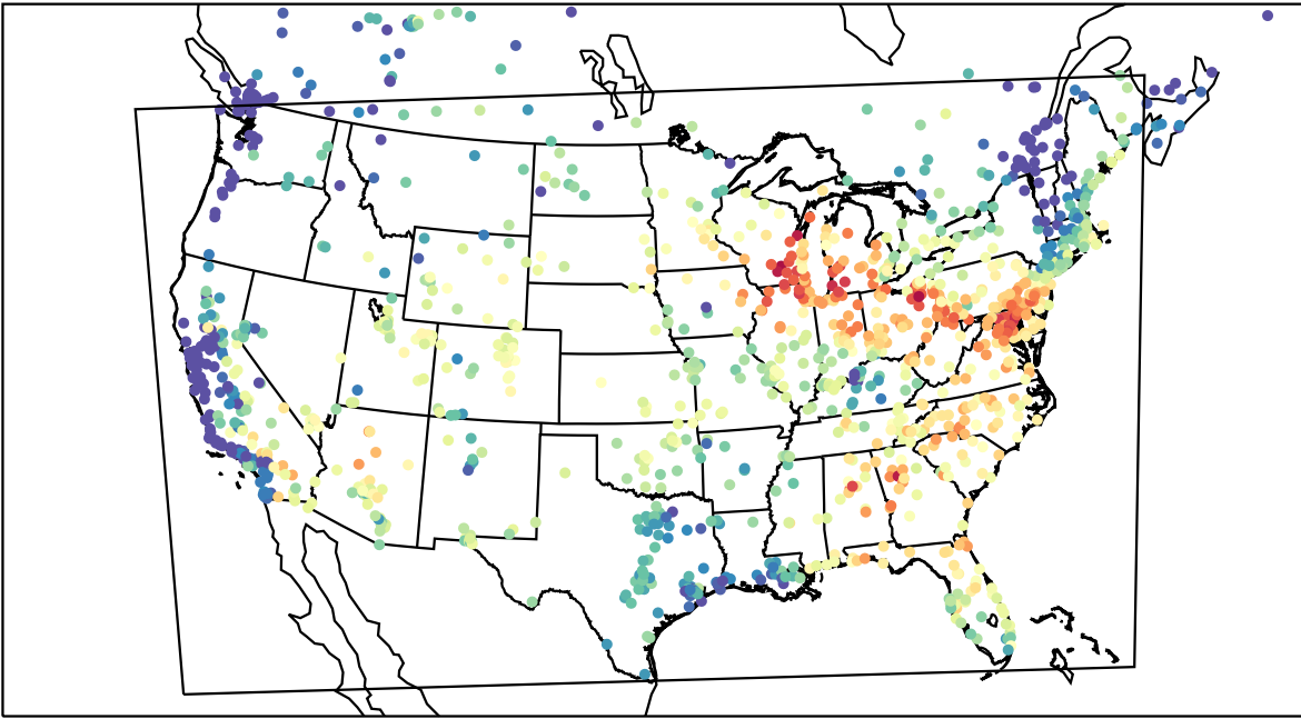
AirNOW (2023-06-29_15:00:00)
