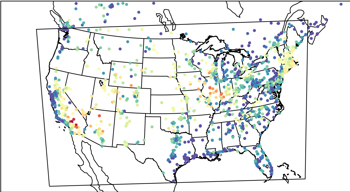
AirNOW (2023-06-28_03:00:00)
