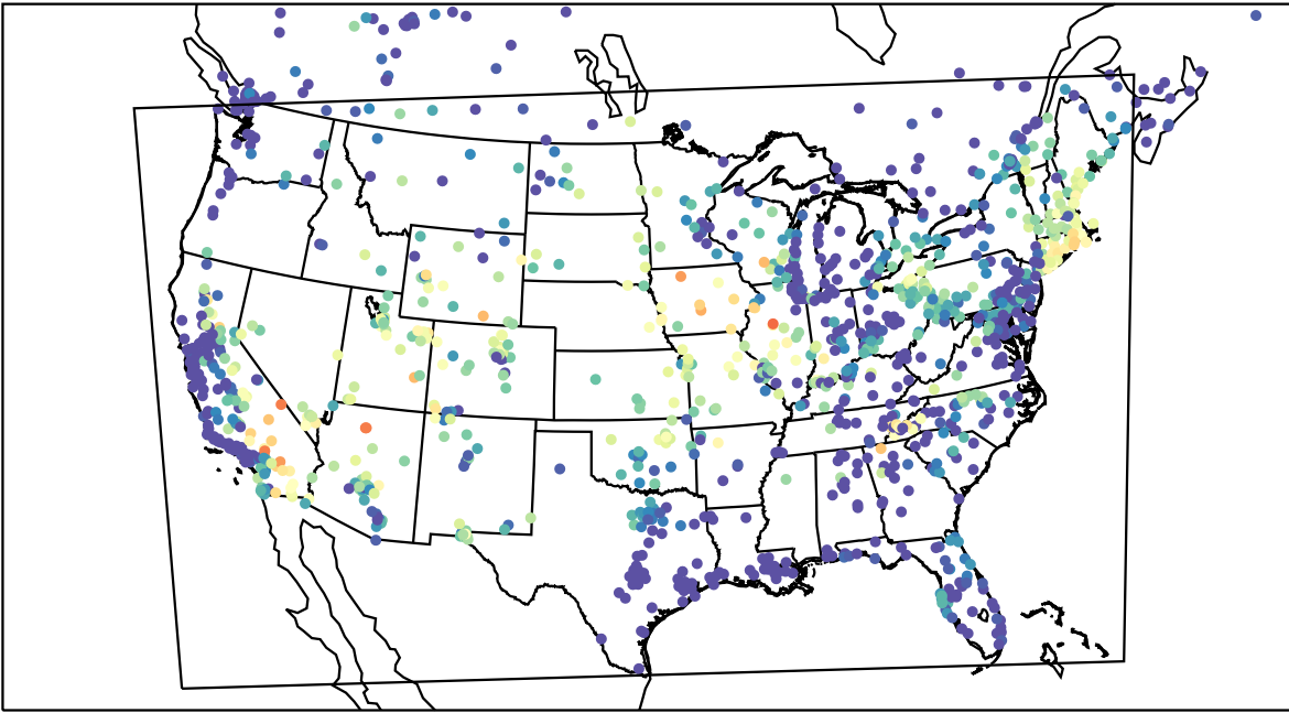
AirNOW (2023-06-28_07:00:00)
