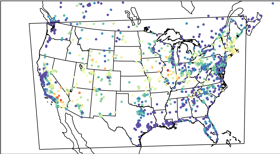
AirNOW (2023-06-28_05:00:00)
