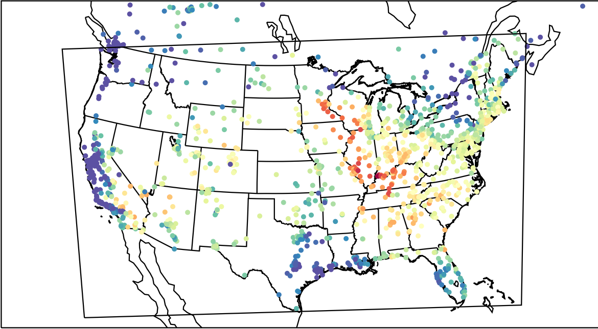
AirNOW (2023-06-28_15:00:00)
