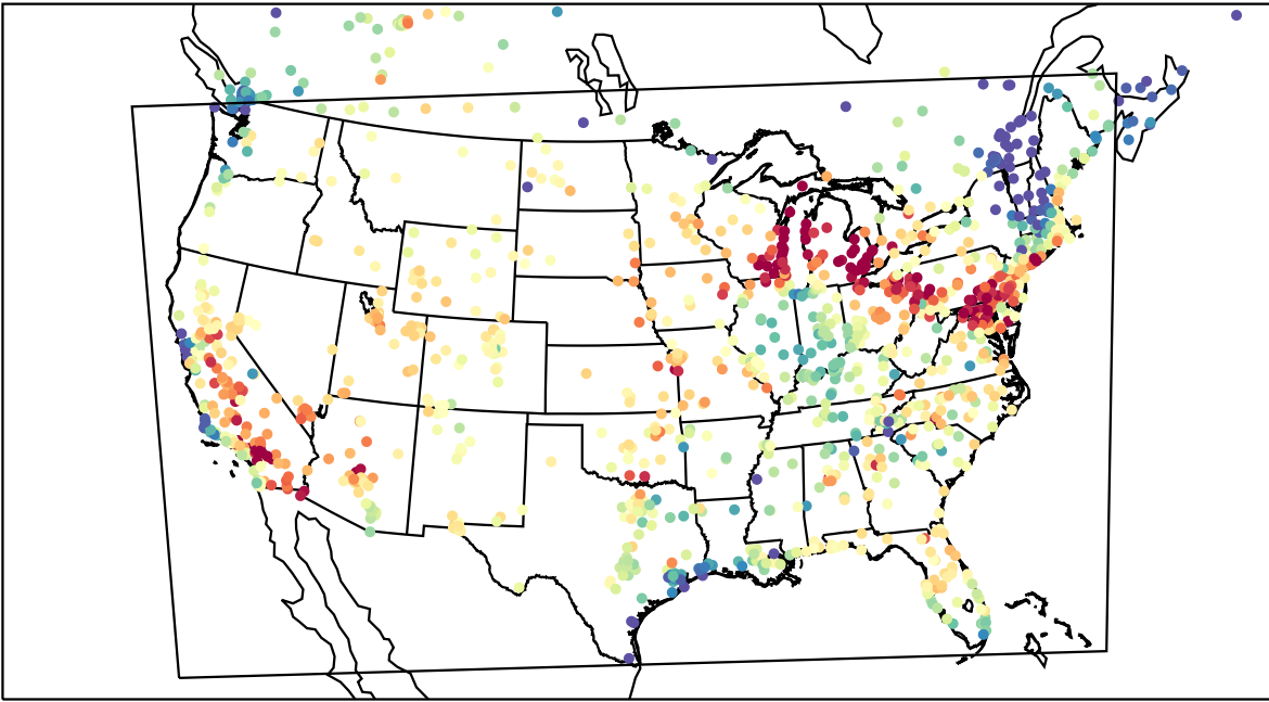
AirNOW (2023-06-29_23:00:00)
