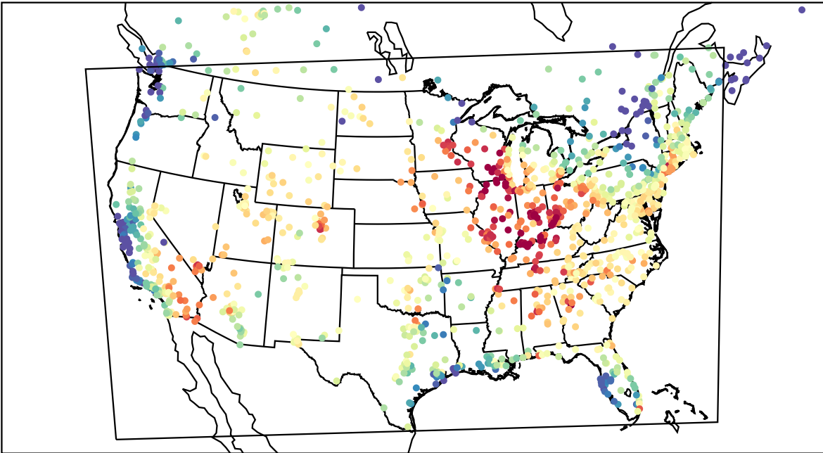
AirNOW (2023-06-28_18:00:00)
