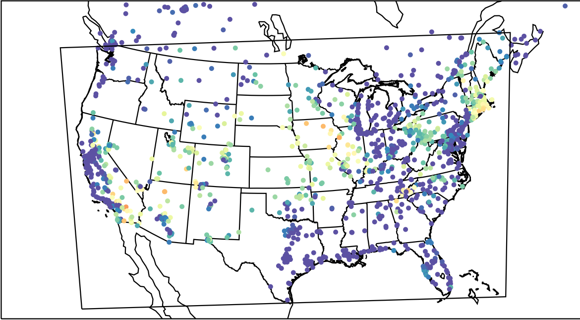
AirNOW (2023-06-28_09:00:00)
