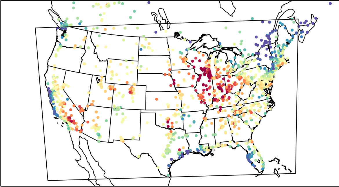
AirNOW (2023-06-28_23:00:00)
