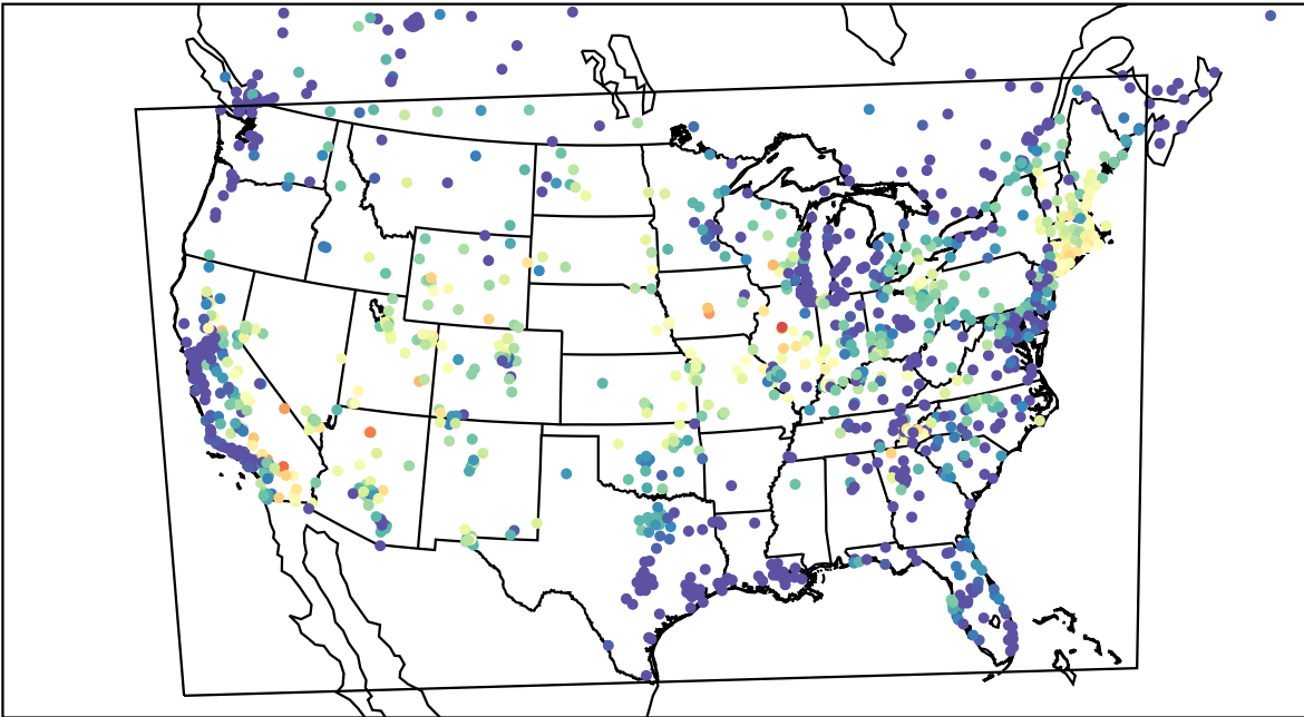
AirNOW (2023-06-28_06:00:00)
