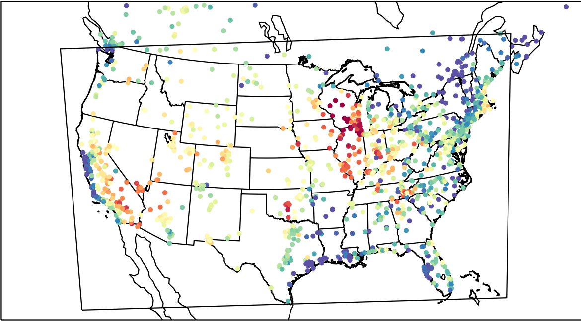
AirNOW (2023-06-29_01:00:00)
