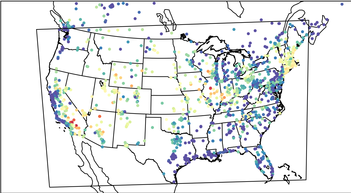
AirNOW (2023-06-28_04:00:00)
