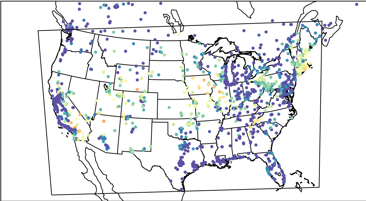
AirNOW (2023-06-28_08:00:00)
