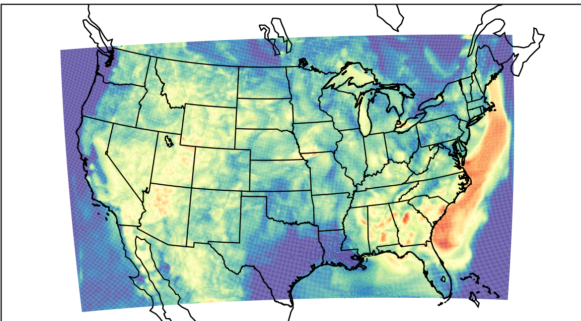
WRF (2023-06-29_08:00:00)
