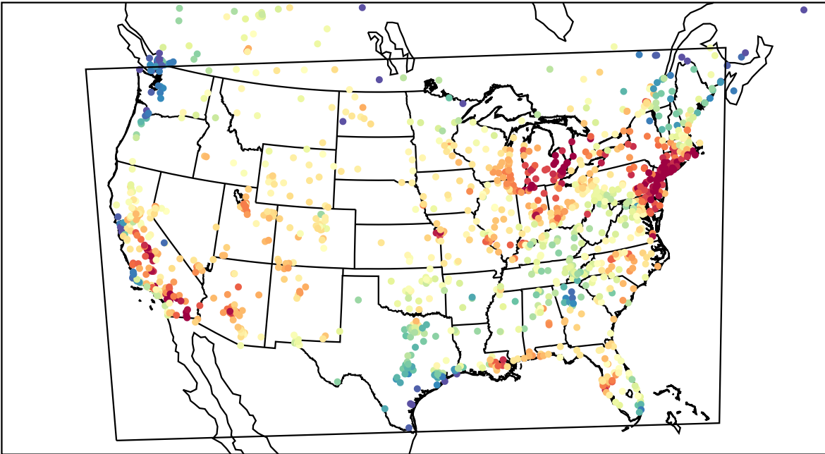
AirNOW (2023-06-30_19:00:00)
