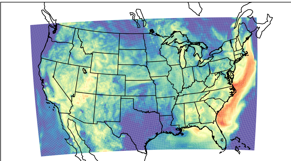
WRF (2023-06-29_13:00:00)
