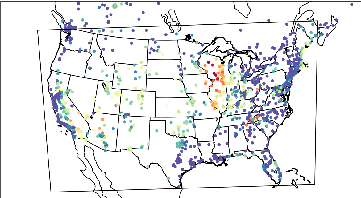
AirNOW (2023-06-29_06:00:00)
