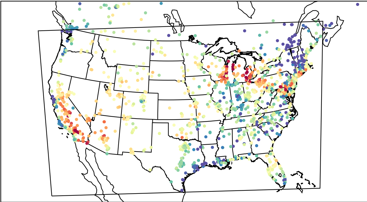
AirNOW (2023-06-30_01:00:00)
