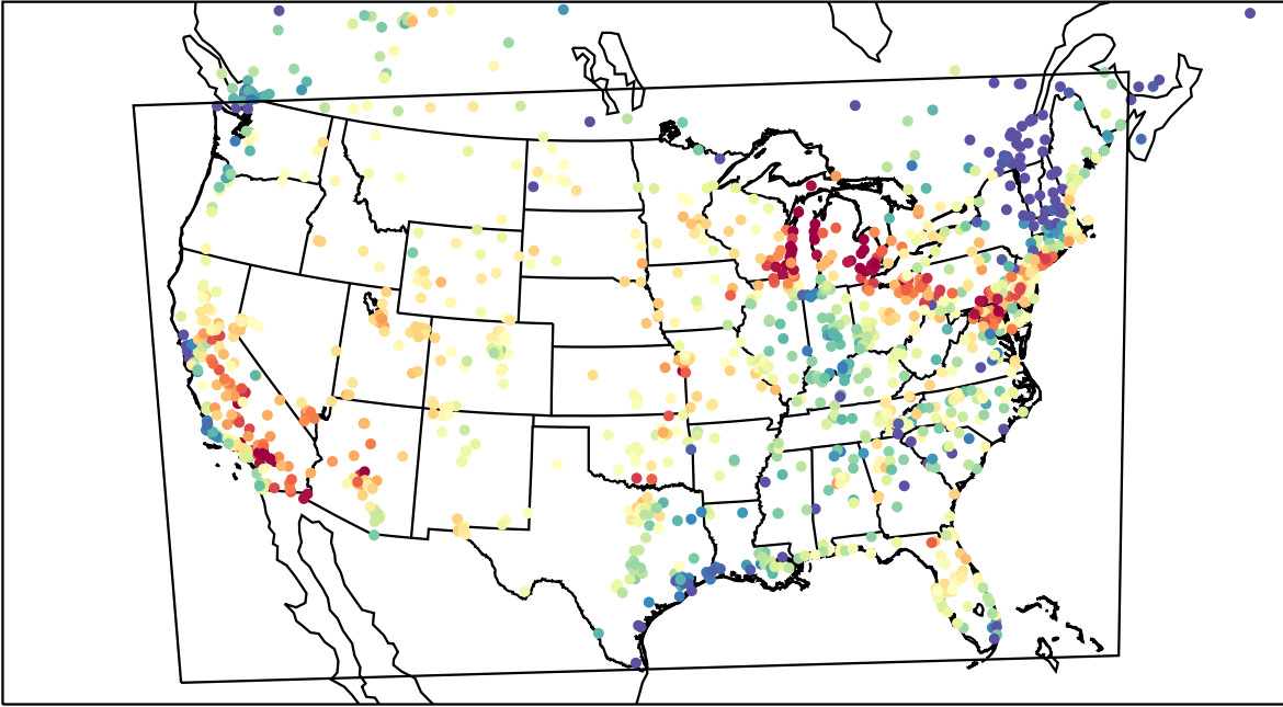
AirNOW (2023-06-30_00:00:00)
