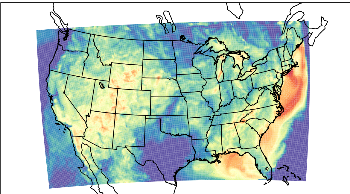
WRF (2023-06-30_09:00:00)
