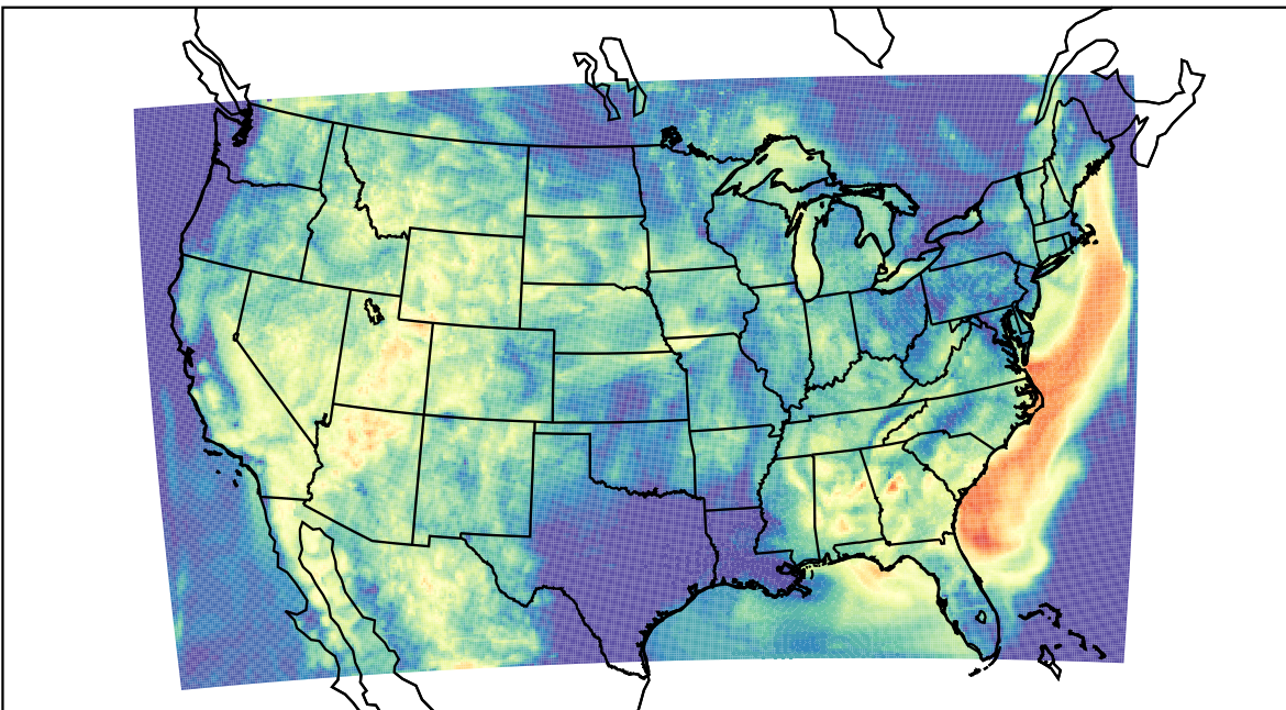
WRF (2023-06-29_11:00:00)
