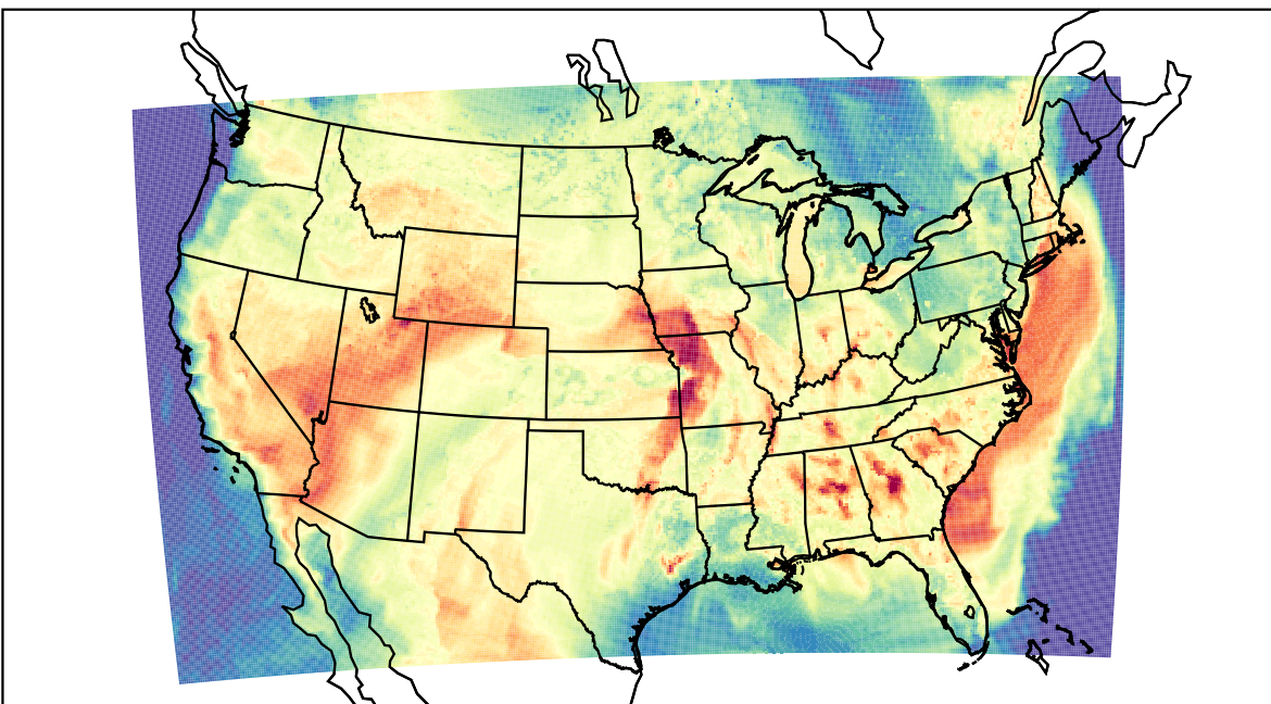
WRF (2023-06-29_00:00:00)
