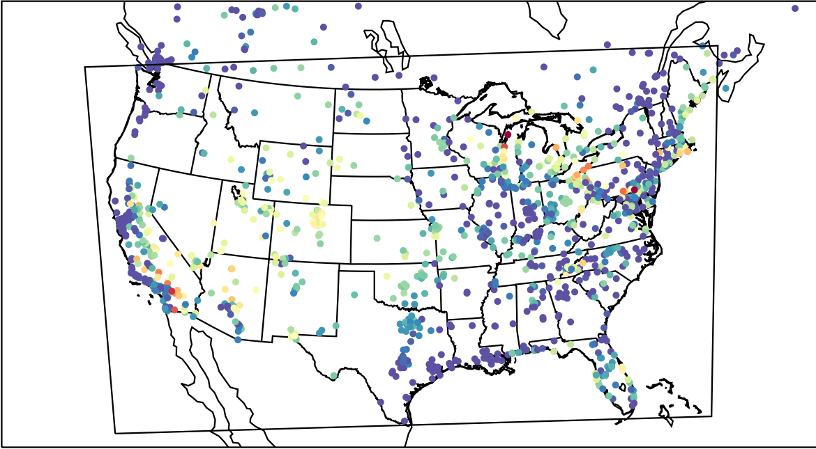
AirNOW (2023-06-30_07:00:00)
