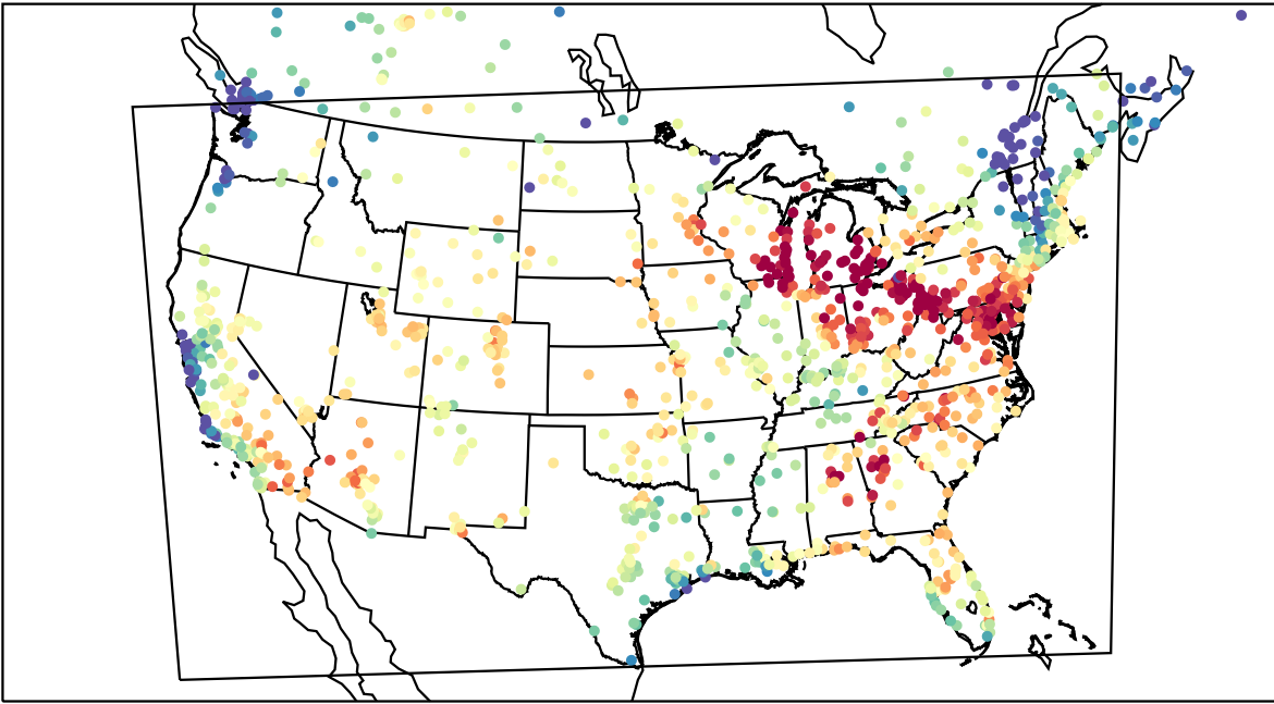
AirNOW (2023-06-29_18:00:00)
