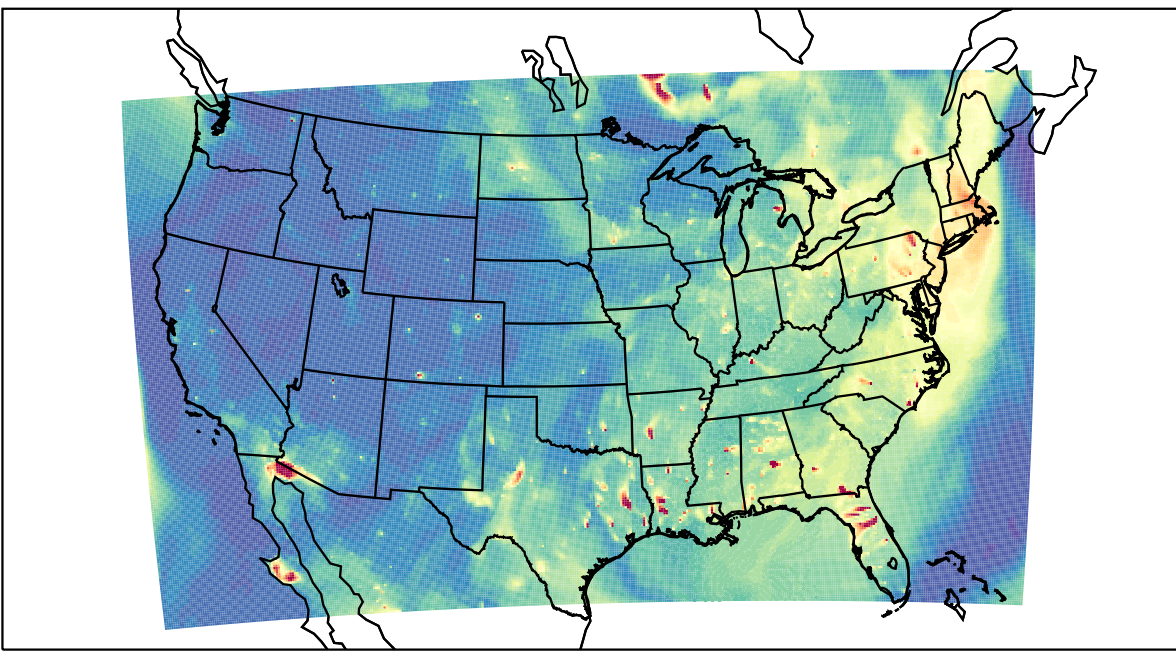
WRF 2023-07-01_02:00:00
