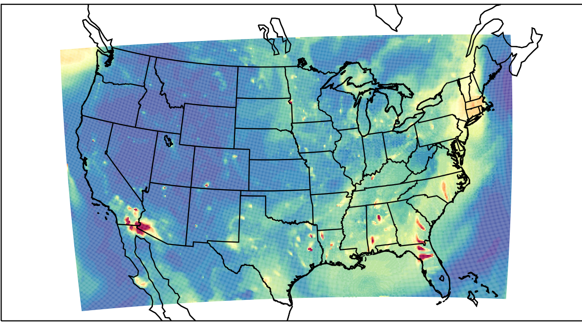
WRF 2023-07-02_03:00:00
