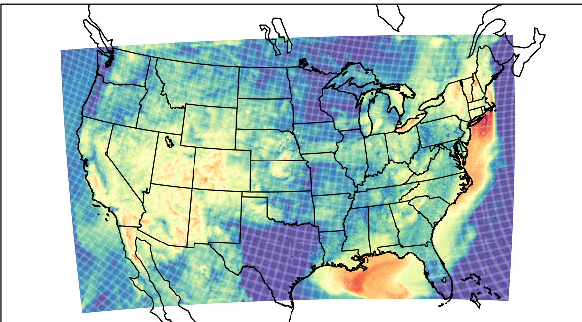
WRF (2023-07-01_12:00:00)
