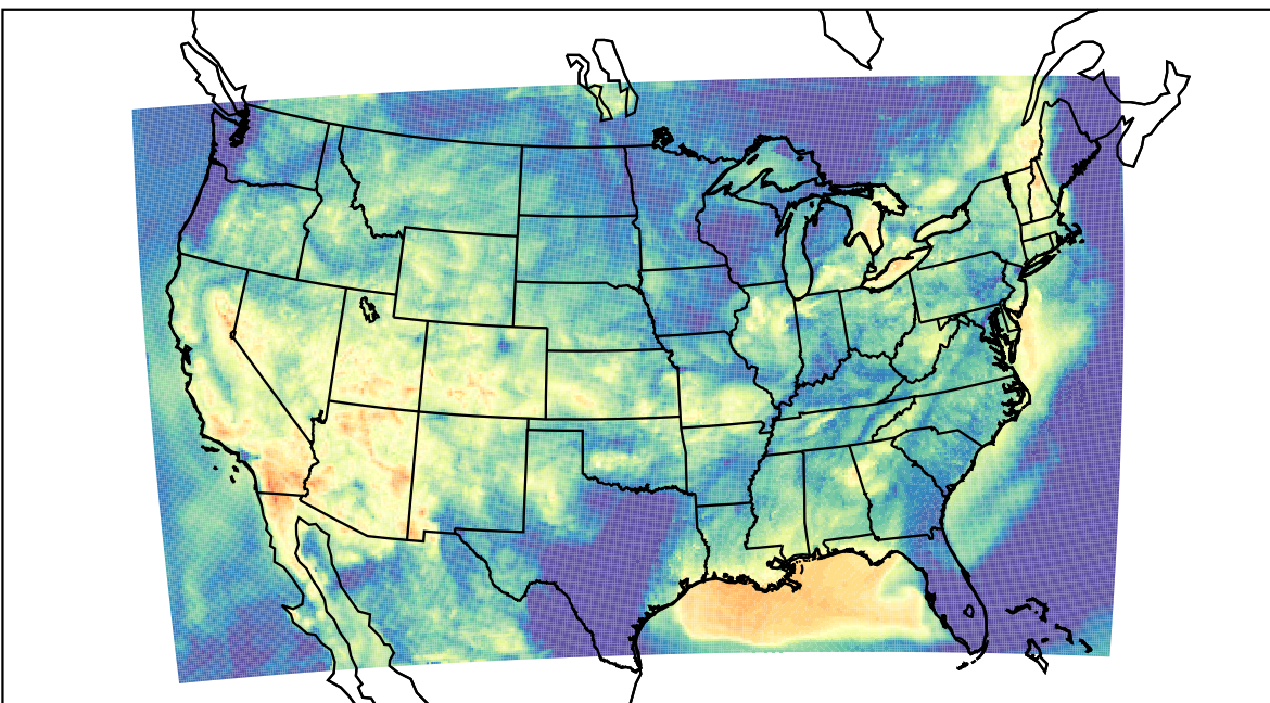
WRF (2023-07-02_11:00:00)
