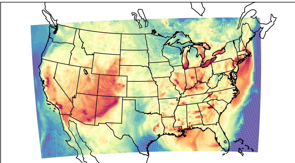
WRF (2023-07-01_00:00:00)
