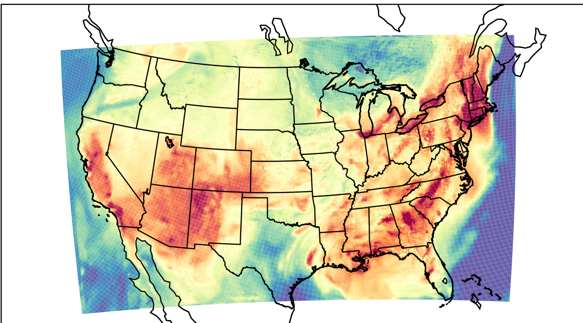
WRF (2023-07-01_21:00:00)
