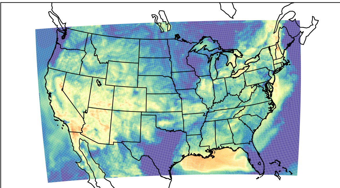
WRF (2023-07-02_12:00:00)
