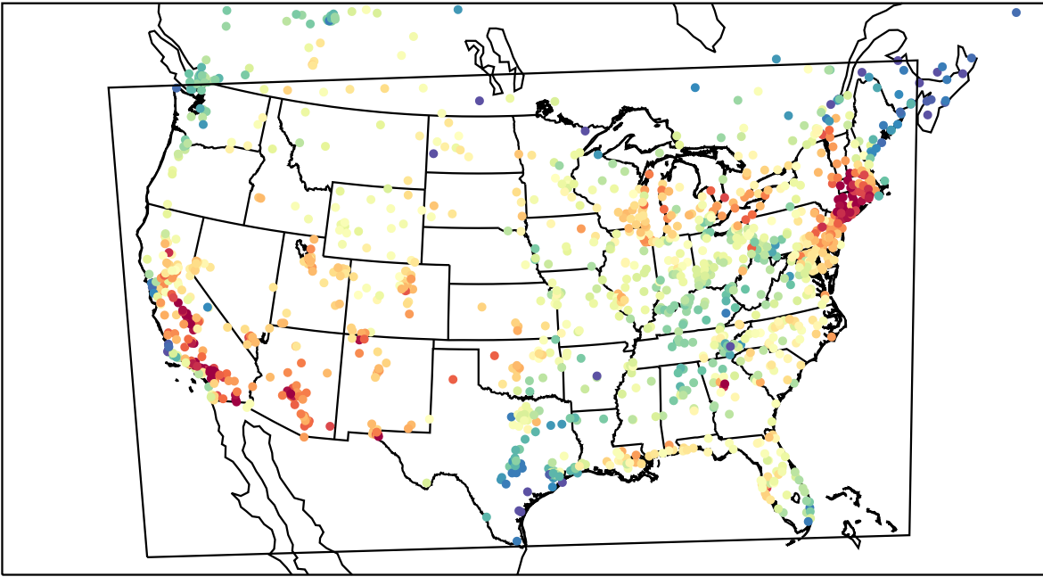
AirNOW (2023-07-01_19:00:00)
