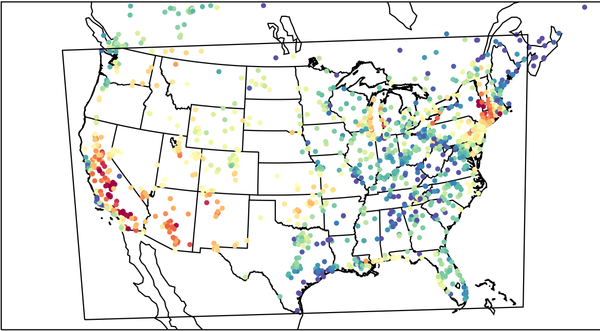
AirNOW (2023-07-02_01:00:00)
