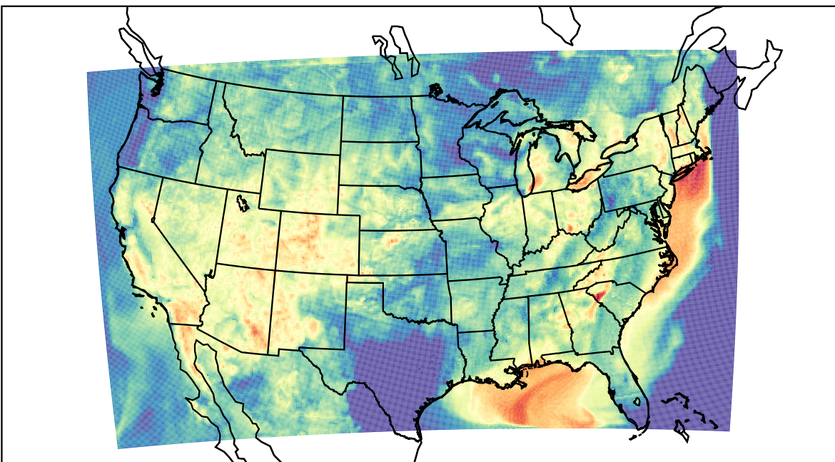
WRF (2023-07-01_09:00:00)
