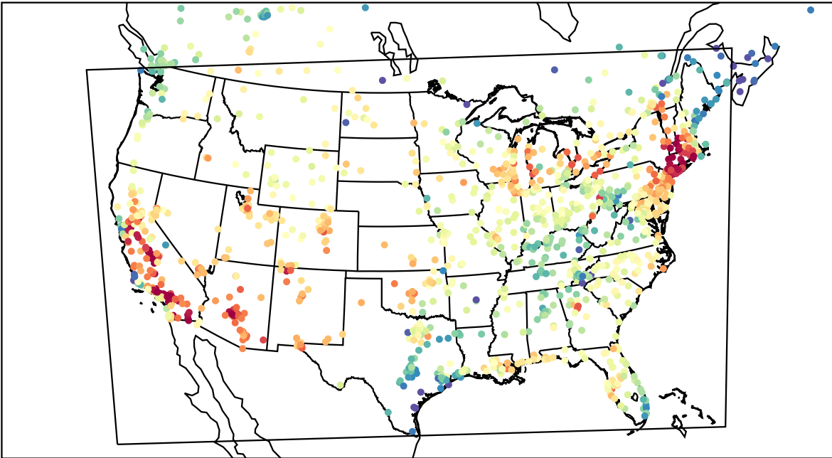
AirNOW (2023-07-01_20:00:00)
