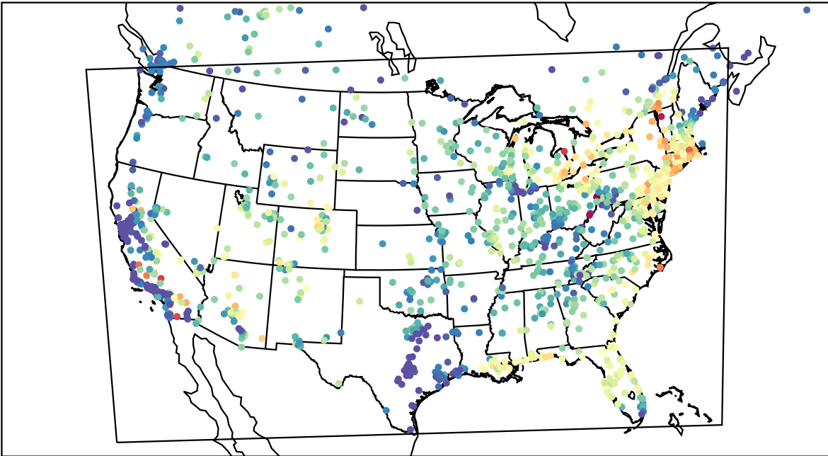
AirNOW (2023-07-01_14:00:00)
