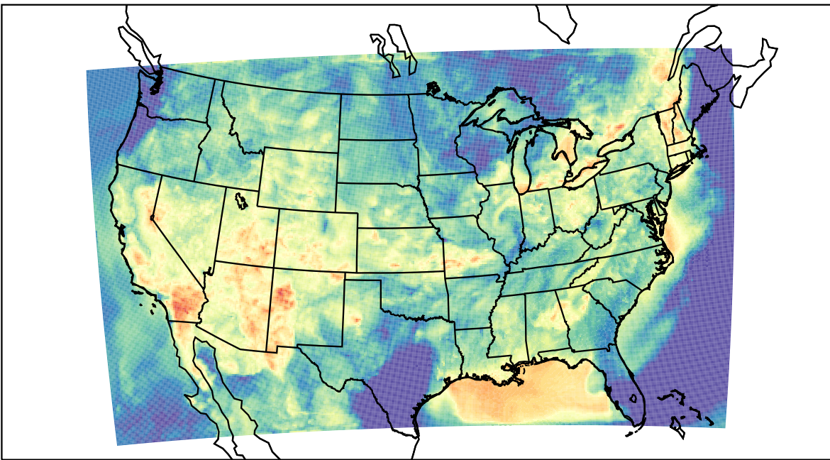
WRF (2023-07-02_07:00:00)
