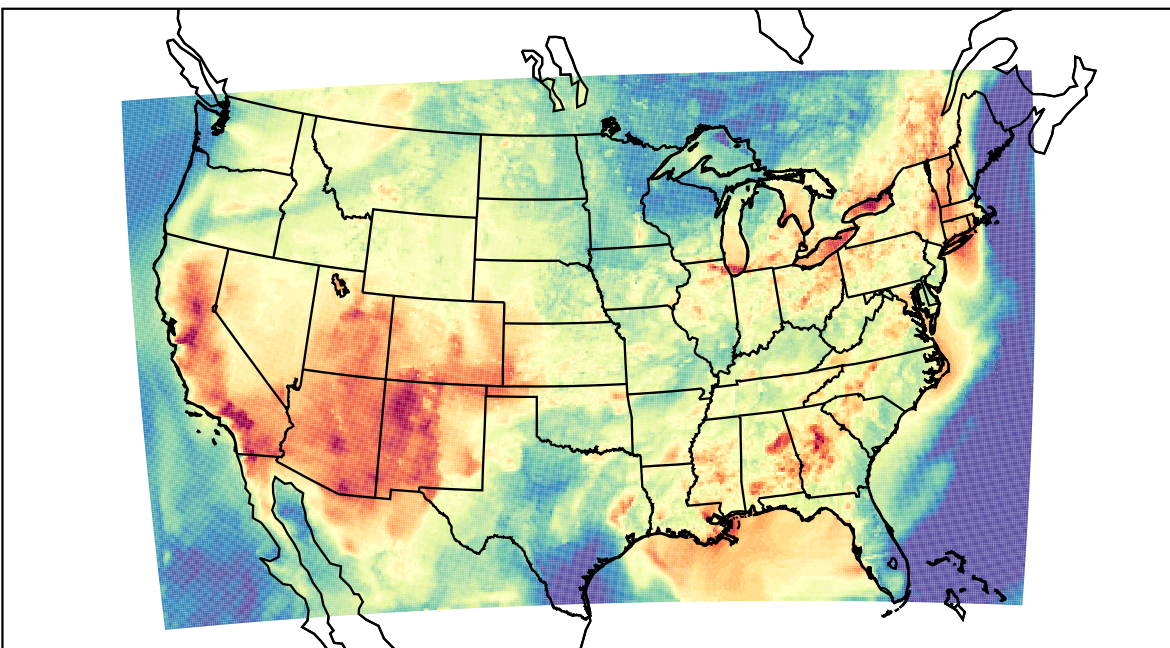
WRF (2023-07-02_01:00:00)
