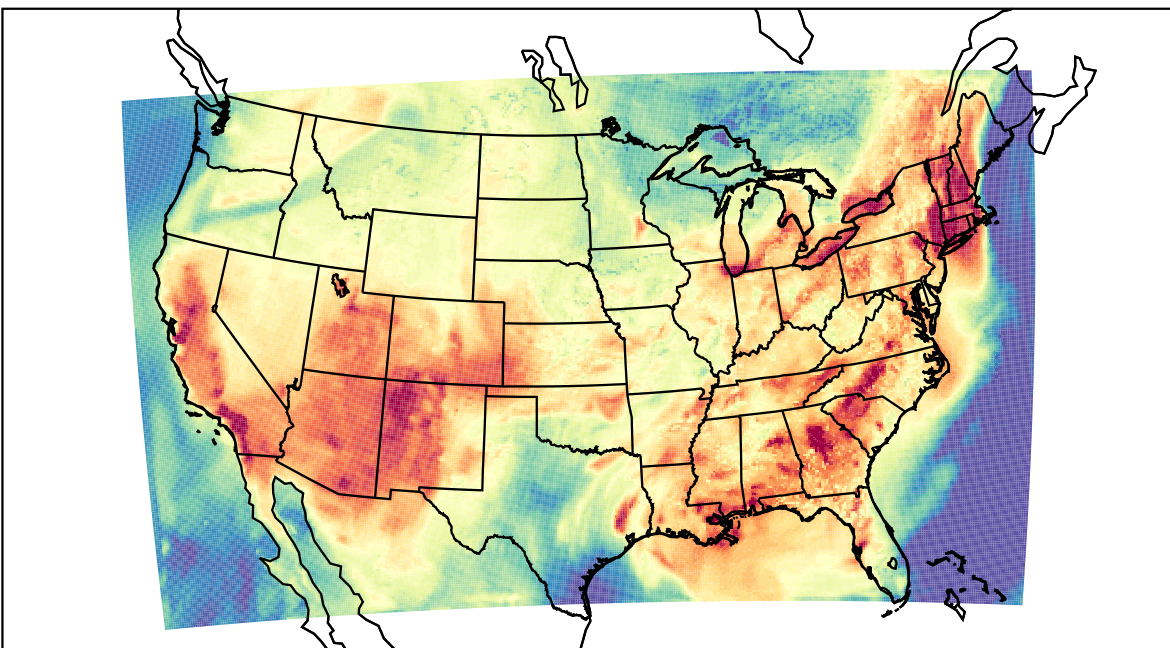
WRF (2023-07-01_22:00:00)
