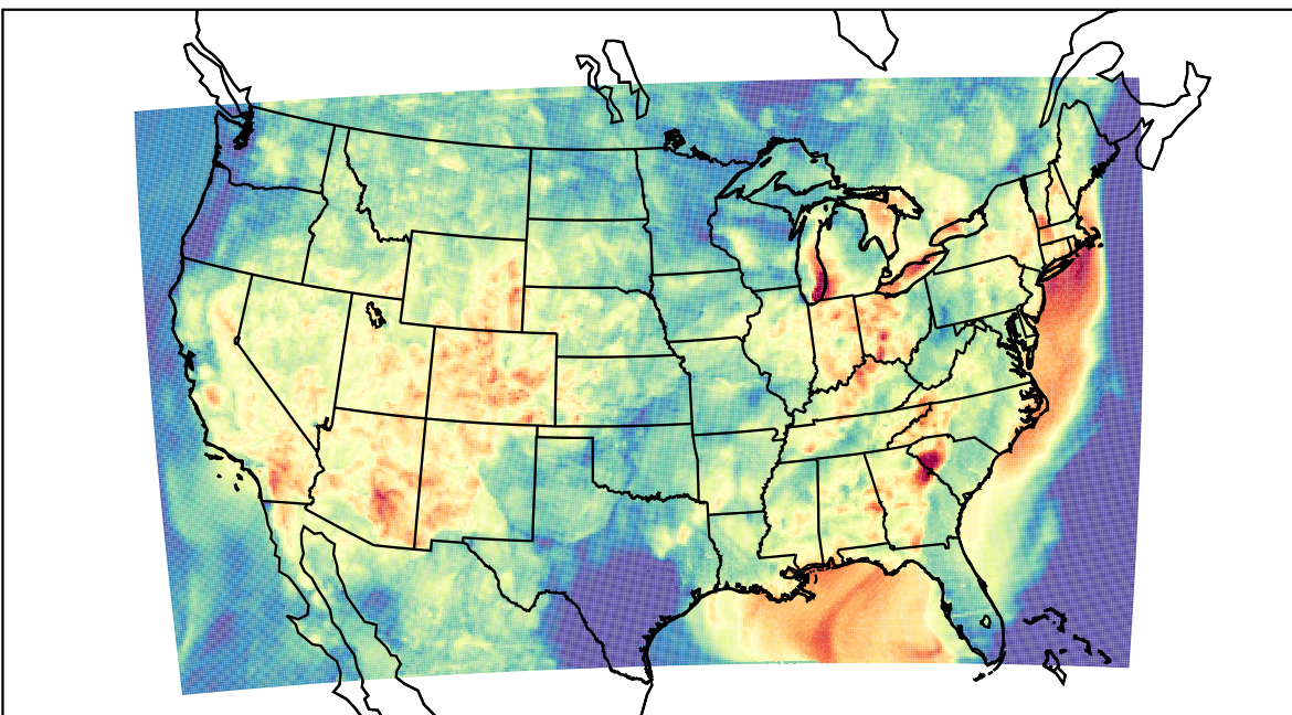
WRF (2023-07-01_05:00:00)
