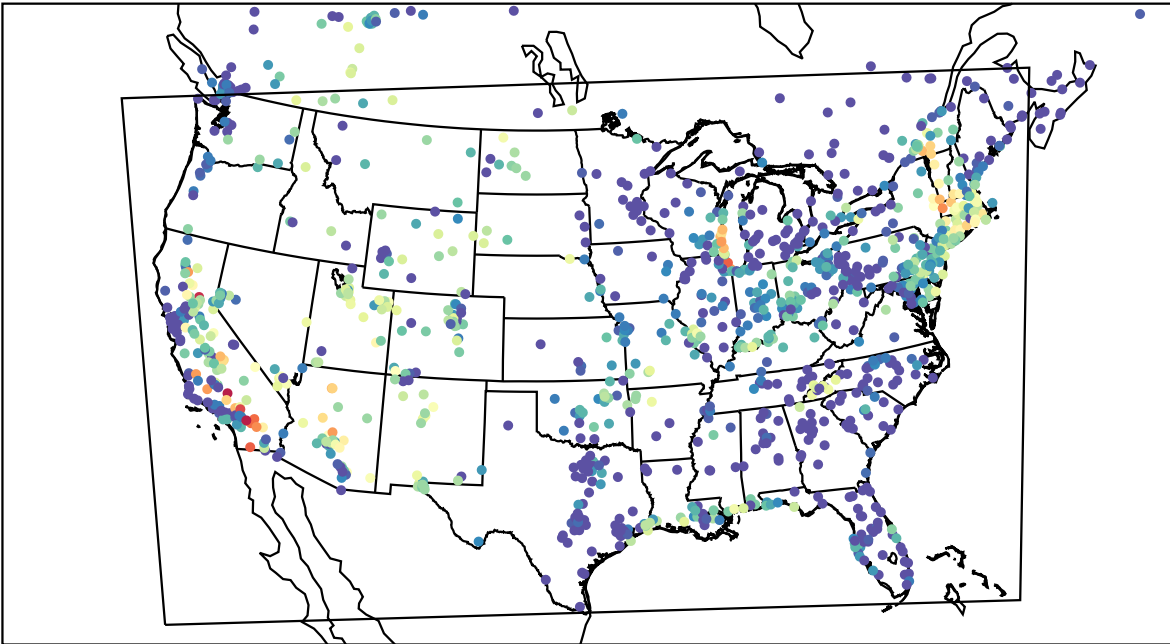
AirNOW (2023-07-02_09:00:00)
