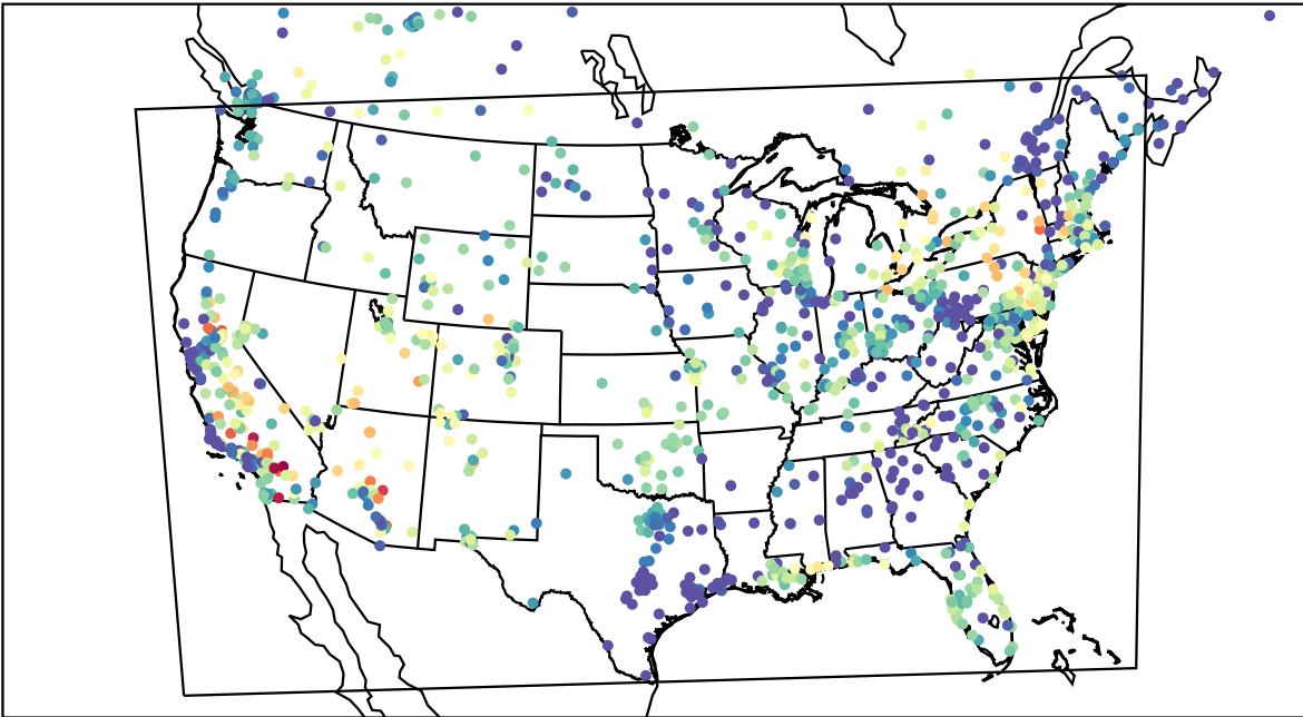
AirNOW (2023-07-01_05:00:00)
