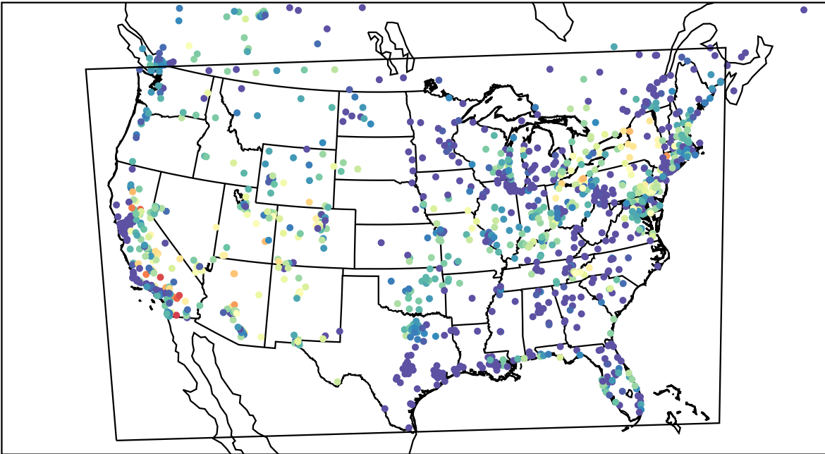
AirNOW (2023-07-01_08:00:00)
