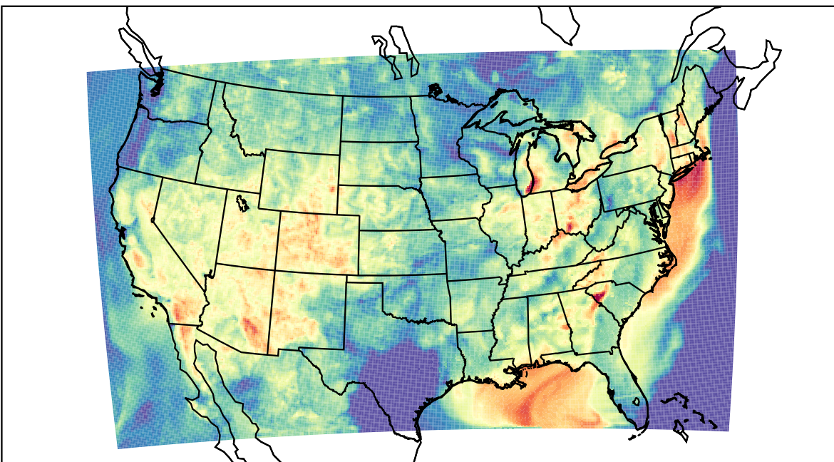
WRF (2023-07-01_07:00:00)
