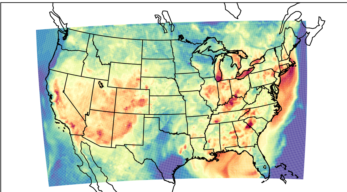
WRF (2023-07-01_02:00:00)
