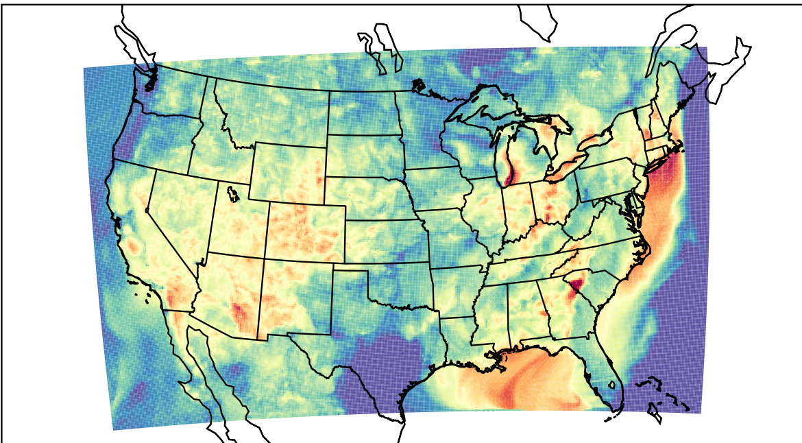
WRF (2023-07-01_06:00:00)
