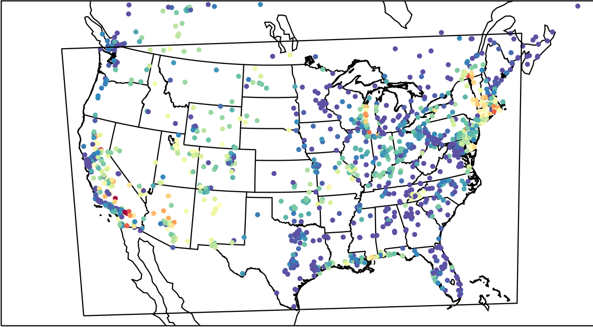
AirNOW (2023-07-02_07:00:00)
