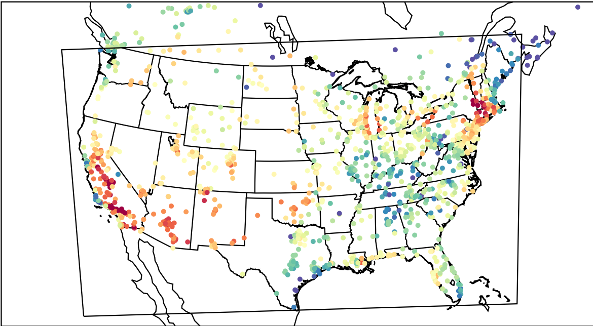
AirNOW (2023-07-01_23:00:00)
