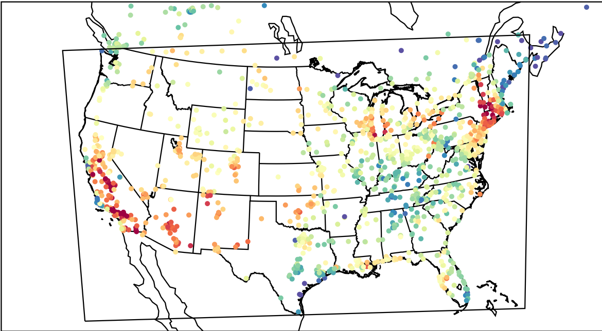
AirNOW (2023-07-01_22:00:00)
