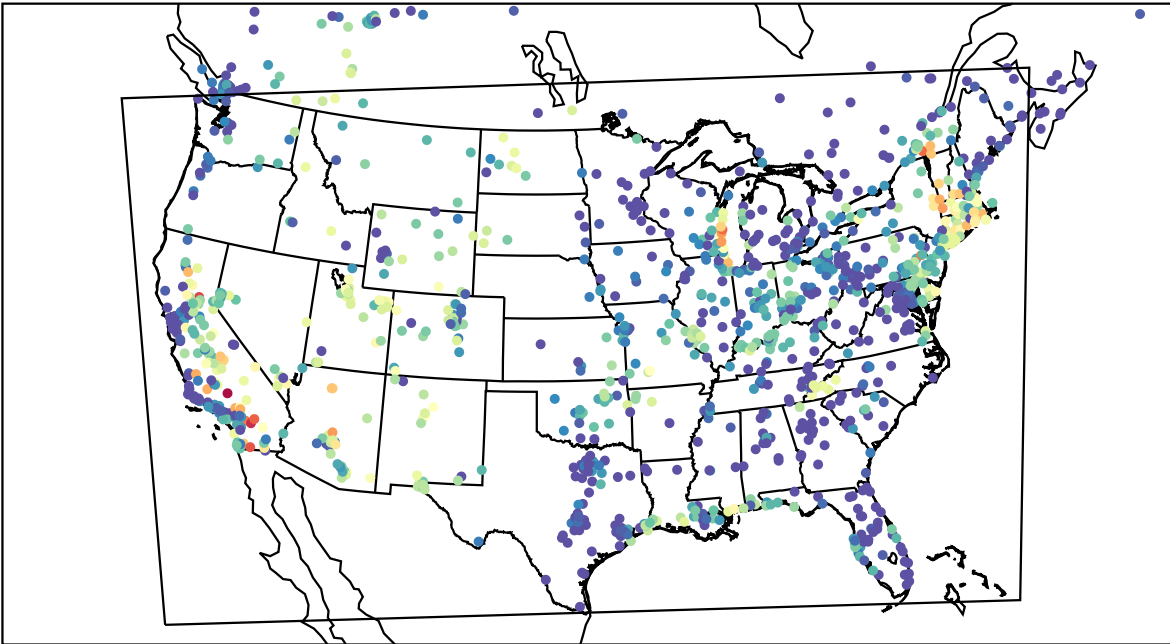
AirNOW (2023-07-02_08:00:00)
