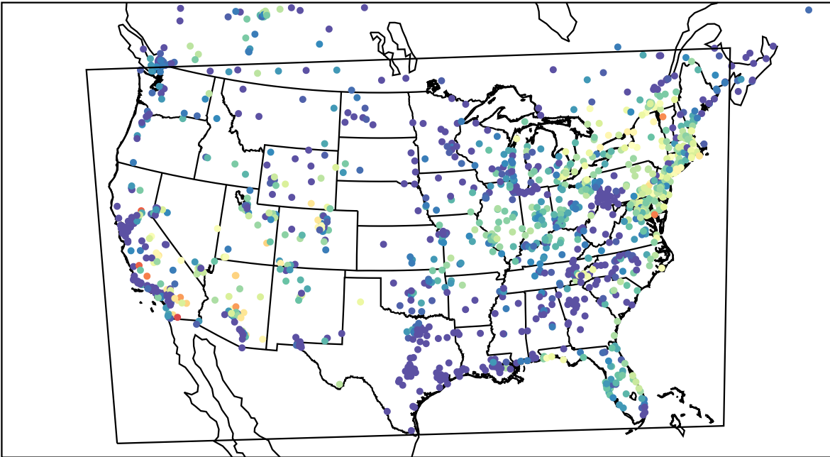
AirNOW (2023-07-01_12:00:00)
