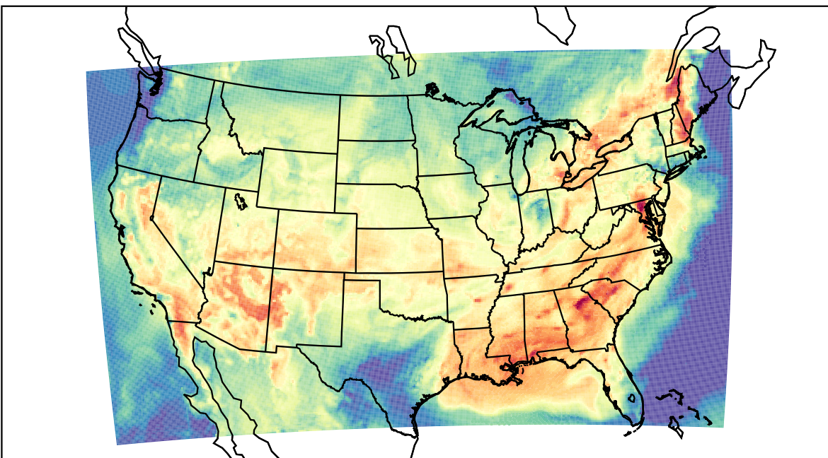
WRF (2023-07-02_16:00:00)
