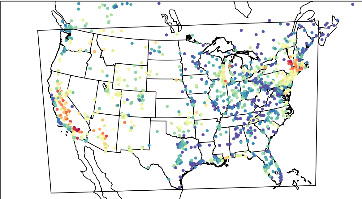
AirNOW (2023-07-02_03:00:00)
