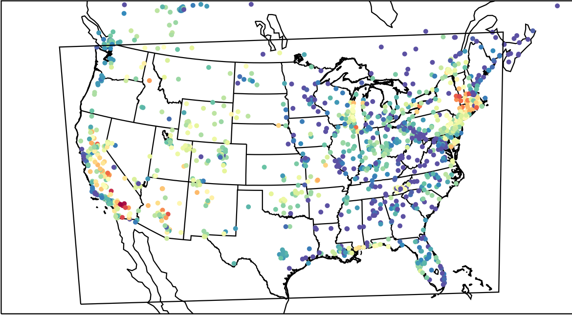
AirNOW (2023-07-02_04:00:00)
