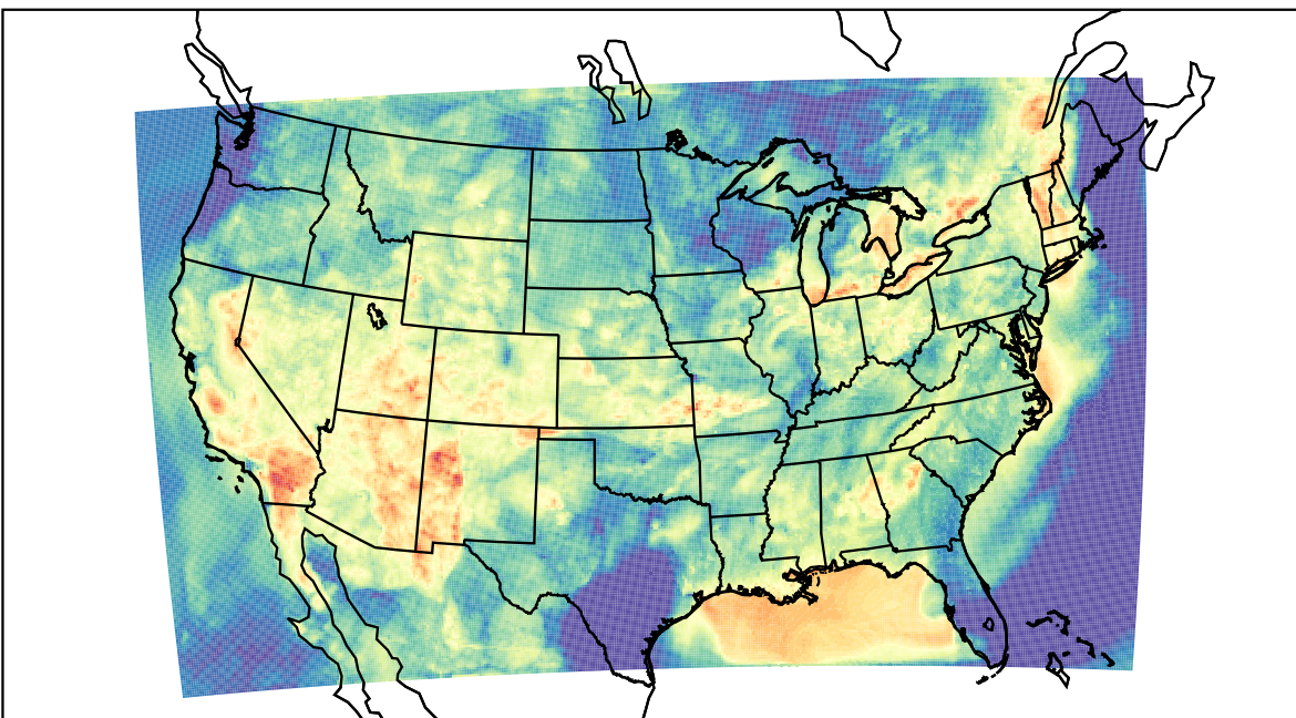
WRF (2023-07-02_06:00:00)
