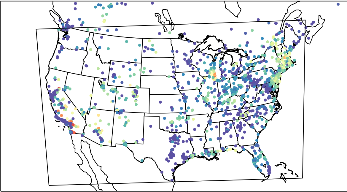
AirNOW (2023-07-02_12:00:00)
