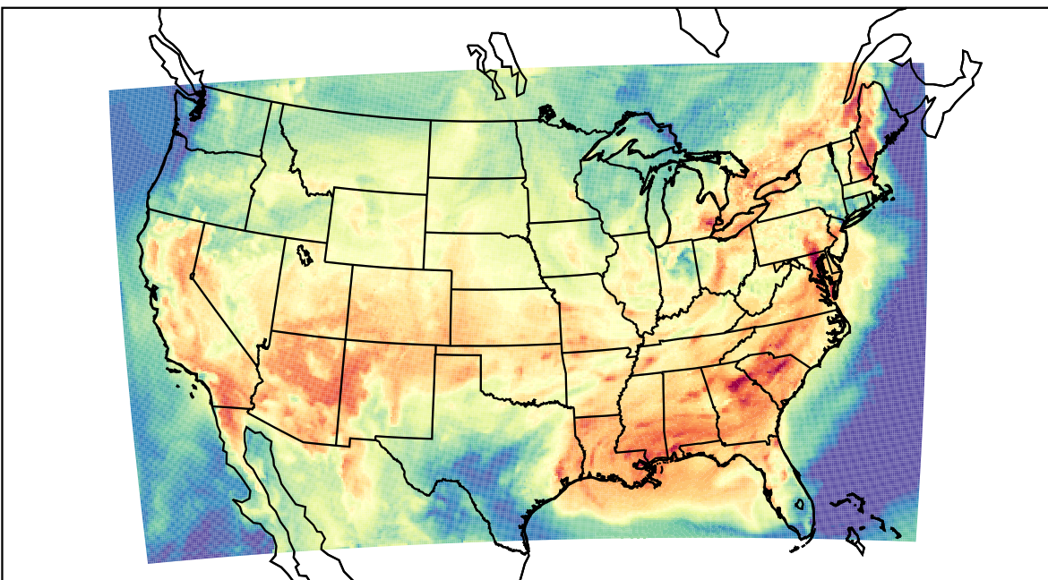
WRF (2023-07-02_17:00:00)
