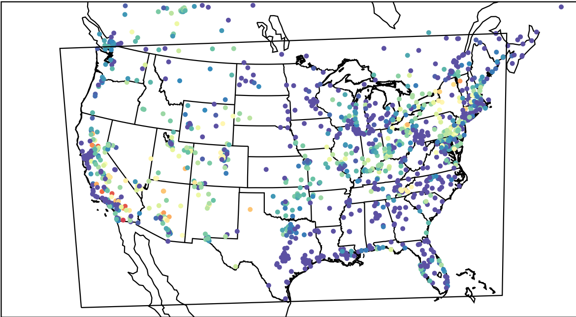
AirNOW (2023-07-01_09:00:00)
