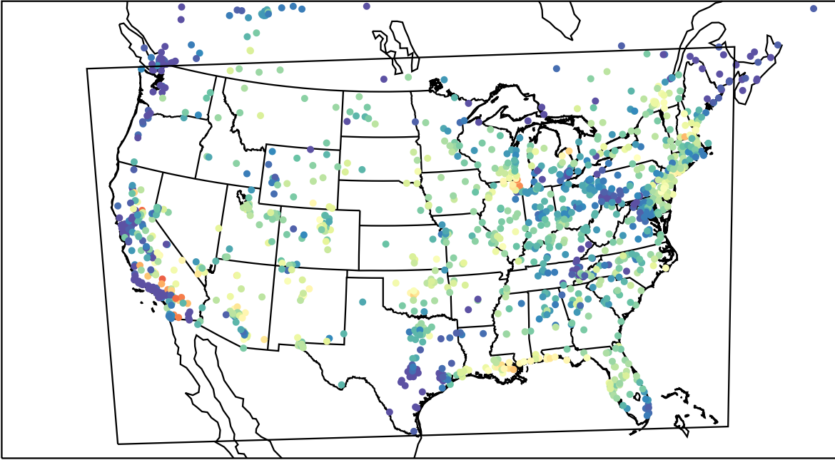
AirNOW (2023-07-02_14:00:00)
