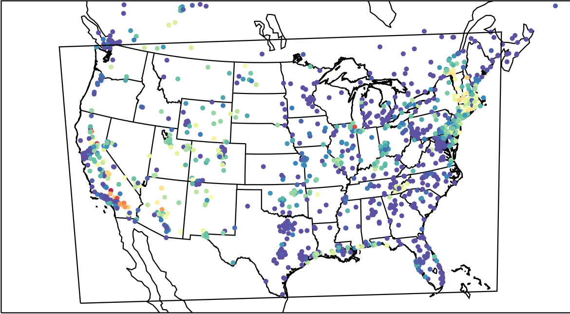
AirNOW (2023-07-02_10:00:00)
