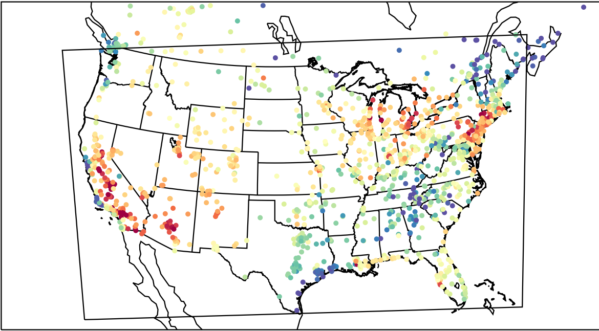
AirNOW (2023-07-01_00:00:00)
