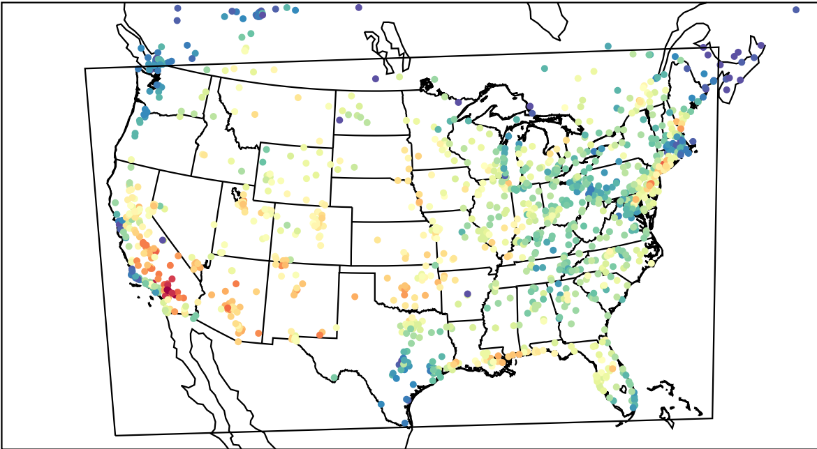
AirNOW (2023-07-02_17:00:00)
