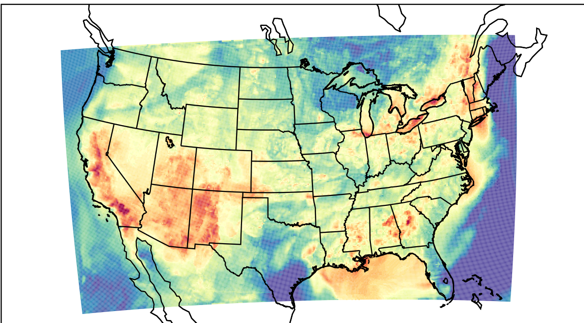
WRF (2023-07-02_02:00:00)
