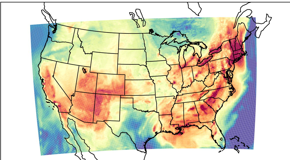
WRF (2023-07-01_19:00:00)
