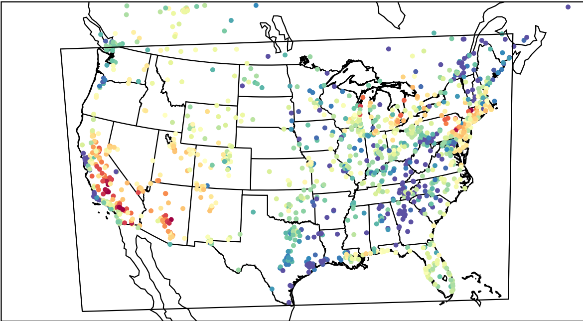
AirNOW (2023-07-01_02:00:00)
