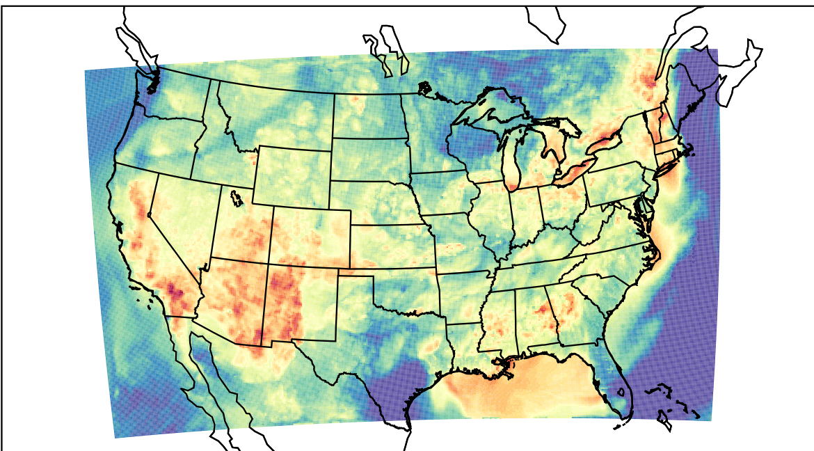
WRF (2023-07-02_03:00:00)
