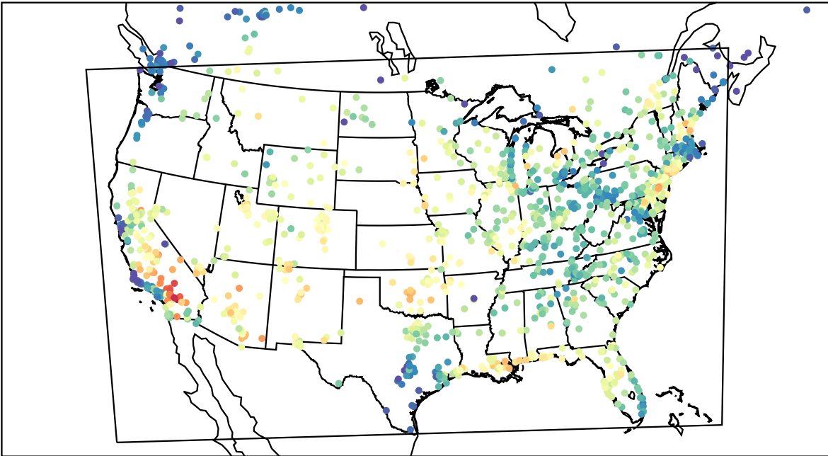
AirNOW (2023-07-02_16:00:00)
