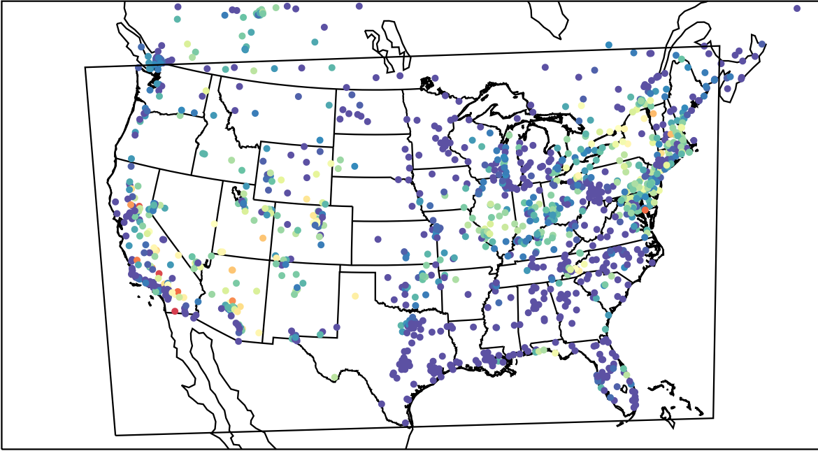
AirNOW (2023-07-01_11:00:00)
