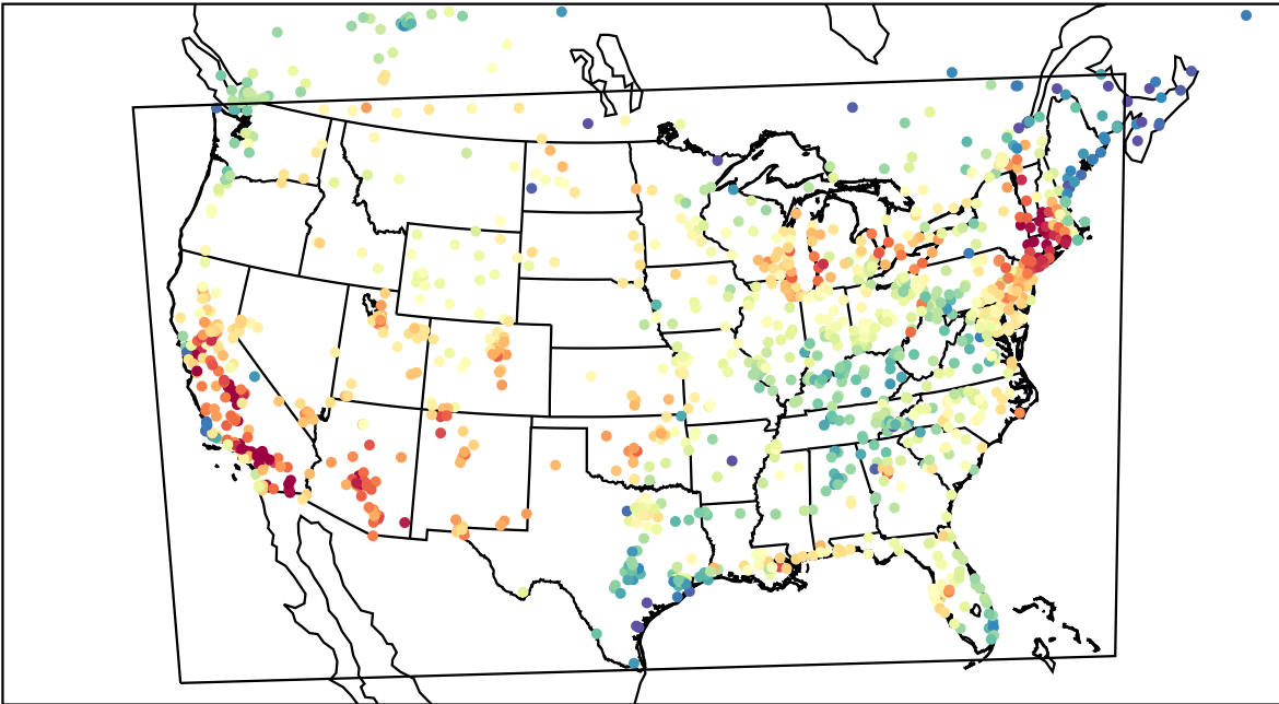
AirNOW (2023-07-01_21:00:00)
