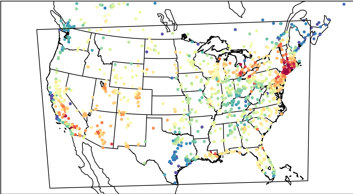
AirNOW (2023-07-01_17:00:00)
