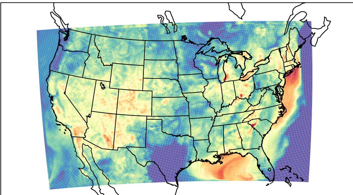
WRF (2023-07-01_08:00:00)
