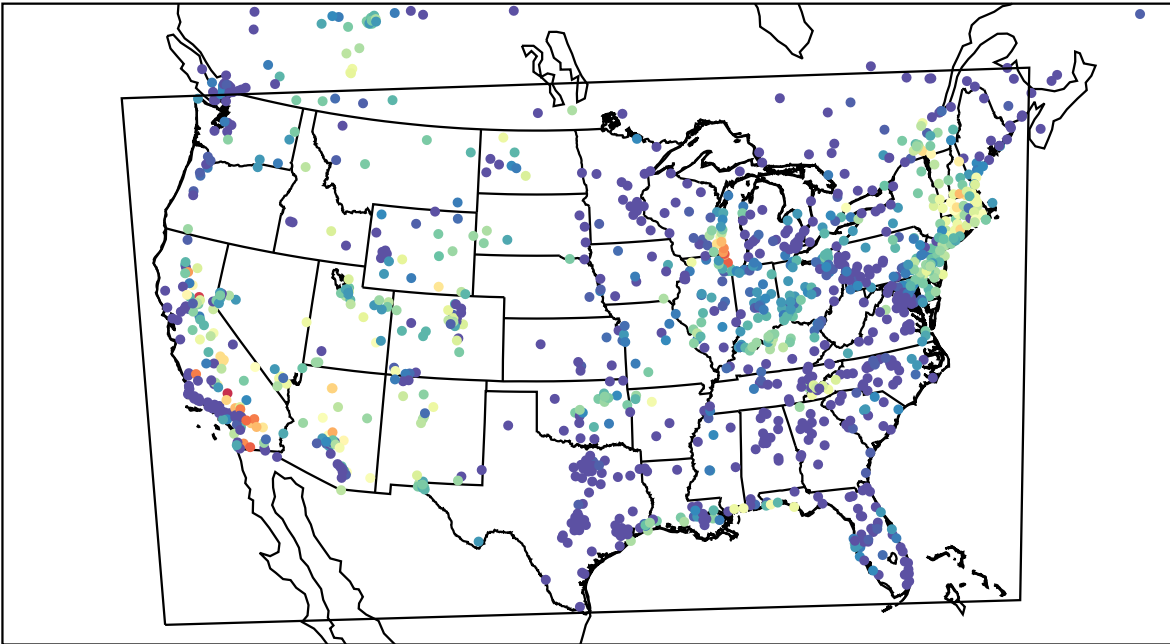
AirNOW (2023-07-02_11:00:00)
