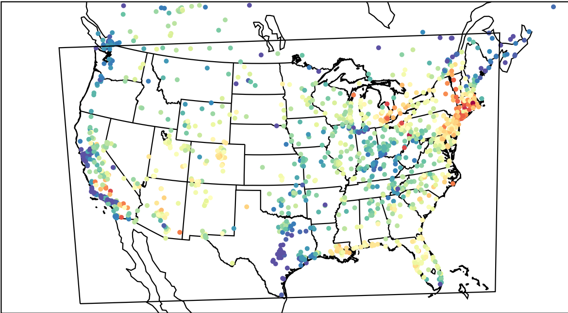
AirNOW (2023-07-01_15:00:00)
