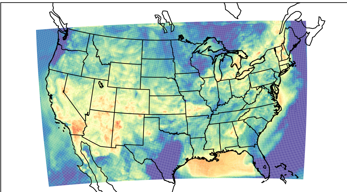
WRF (2023-07-02_08:00:00)
