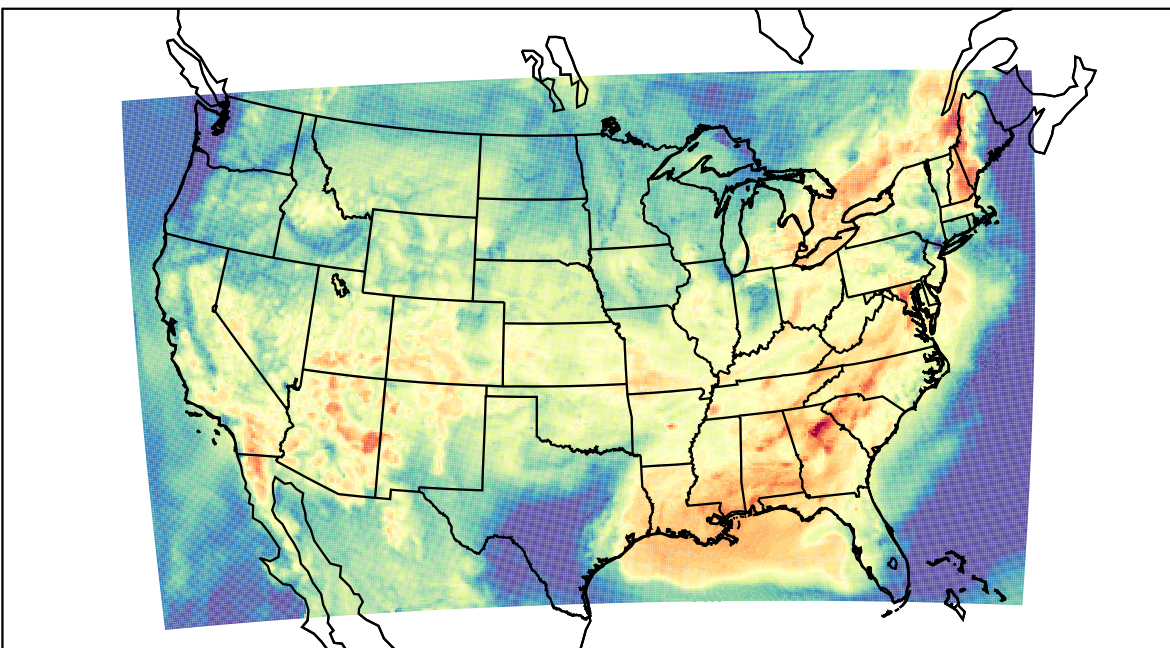
WRF (2023-07-02_15:00:00)
