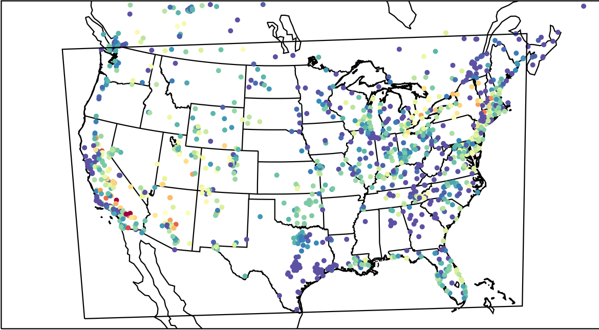
AirNOW (2023-07-01_06:00:00)
