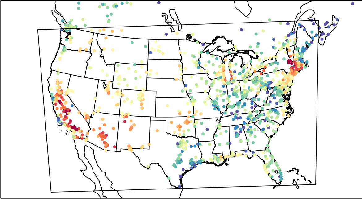
AirNOW (2023-07-02_00:00:00)
