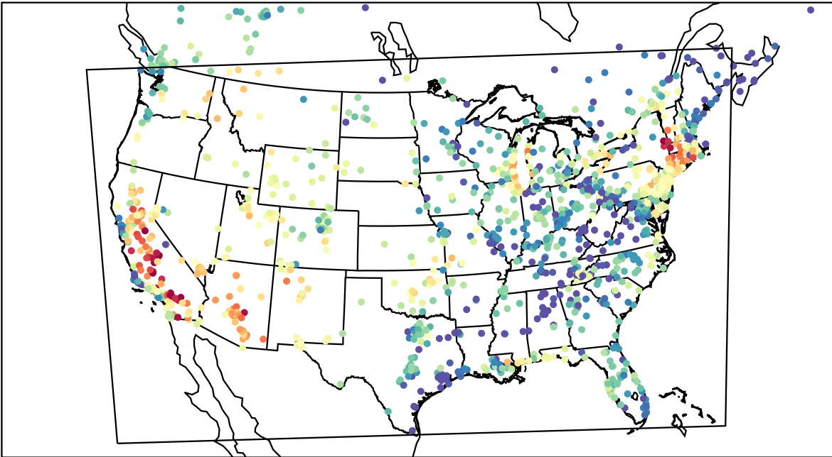
AirNOW (2023-07-02_02:00:00)
