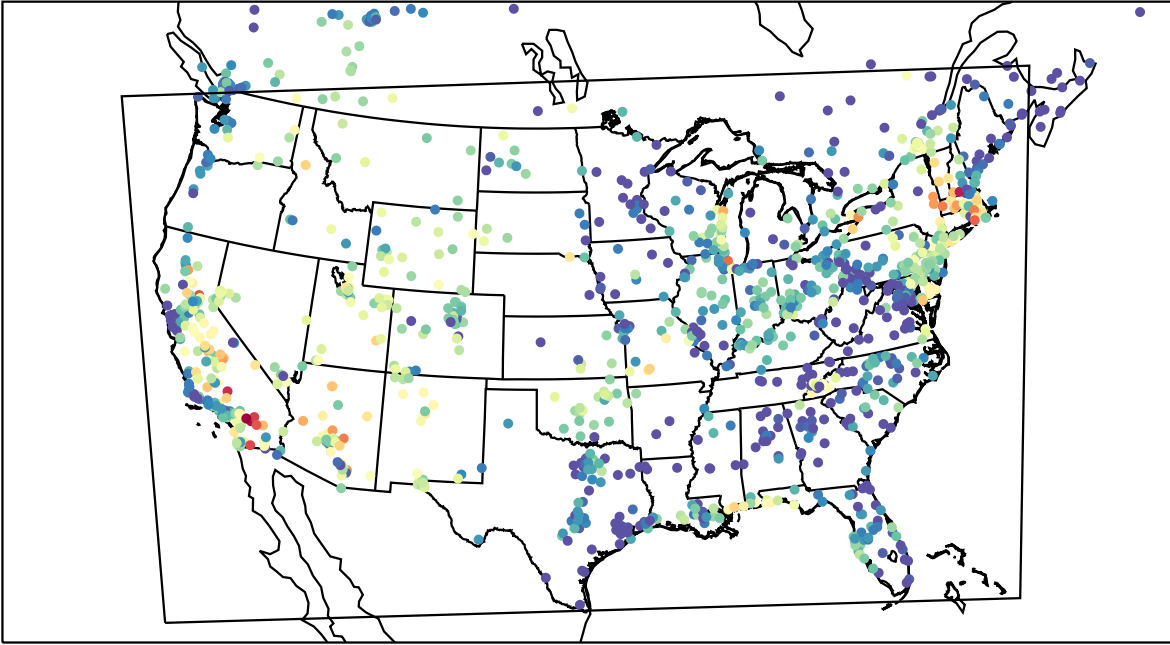
AirNOW (2023-07-02_05:00:00)
