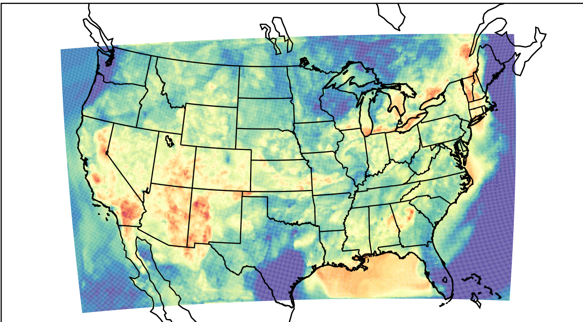
WRF (2023-07-02_05:00:00)
