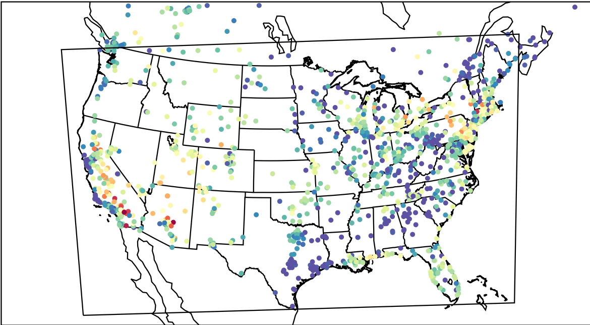
AirNOW (2023-07-01_04:00:00)
