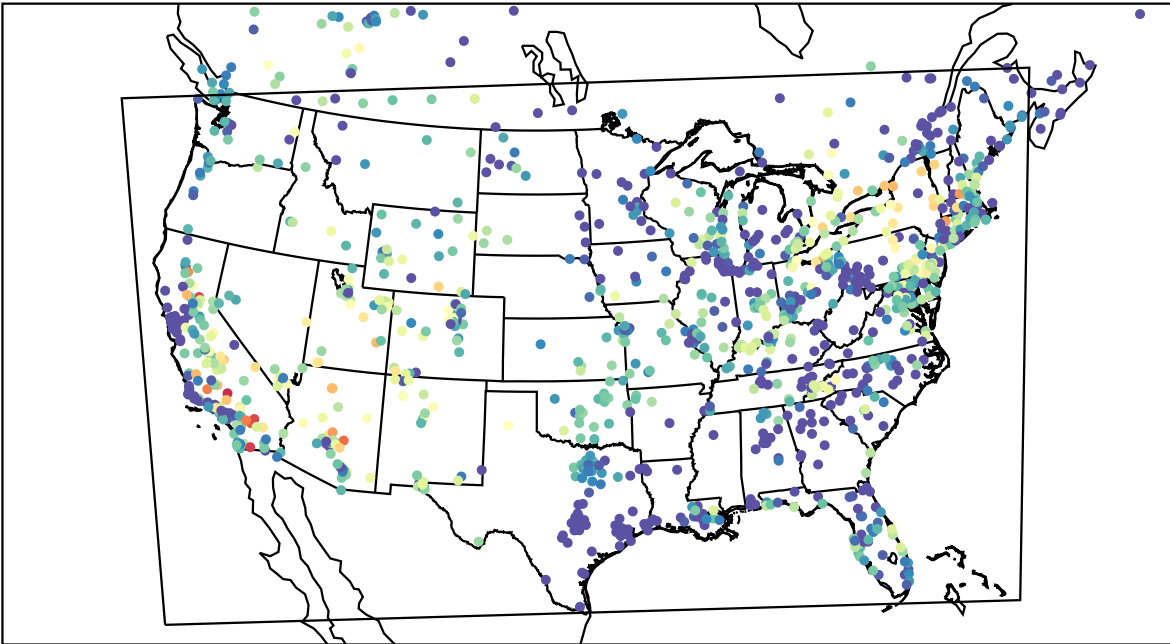
AirNOW (2023-07-01_07:00:00)
