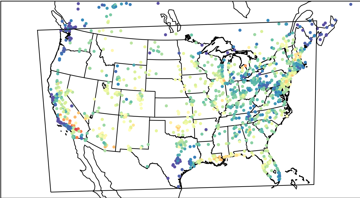
AirNOW (2023-07-02_15:00:00)
