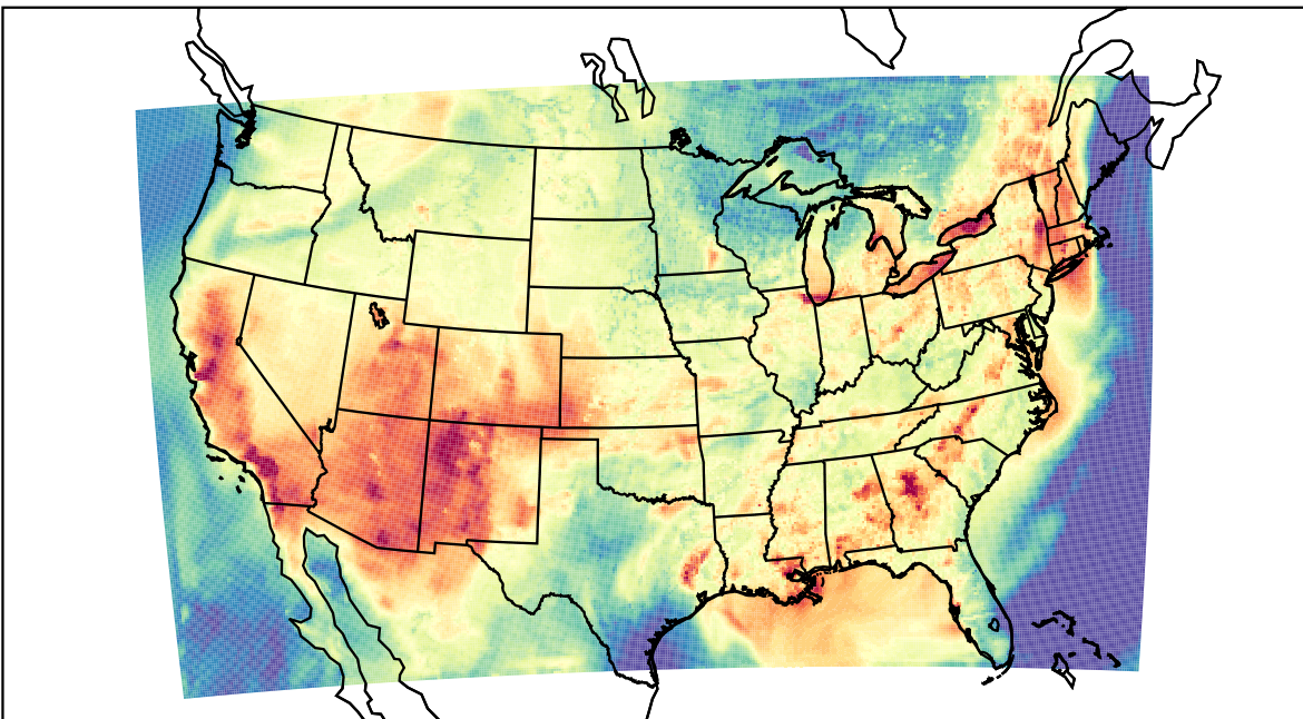
WRF (2023-07-02_00:00:00)
