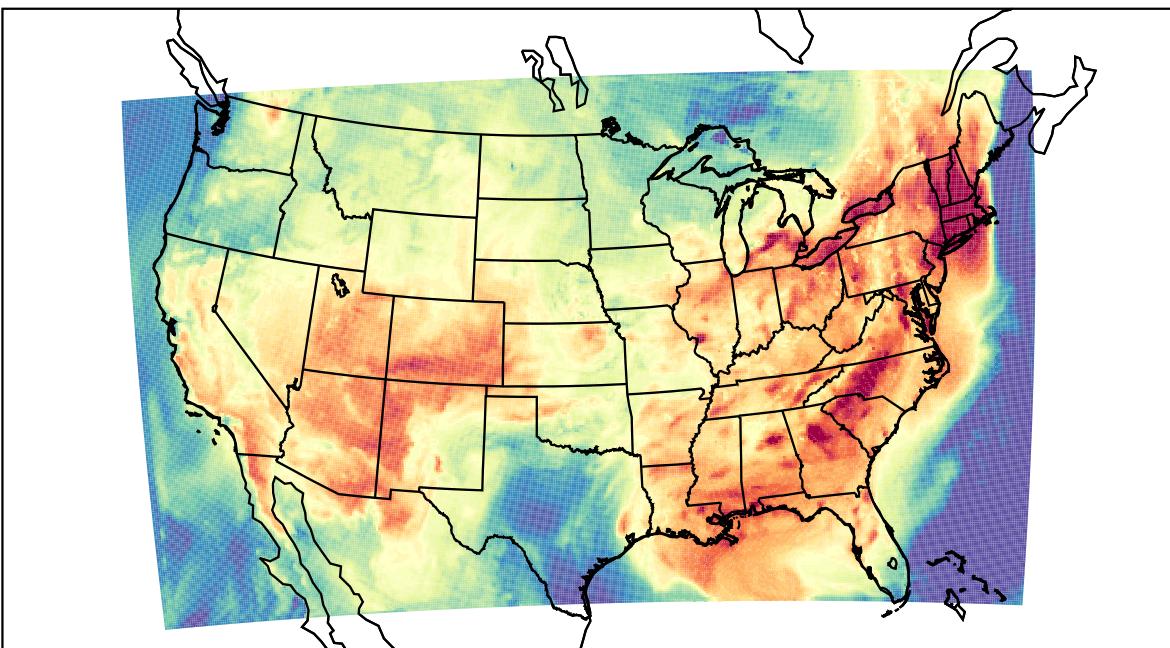
WRF (2023-07-01_17:00:00)
