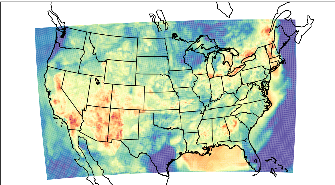
WRF (2023-07-02_04:00:00)
