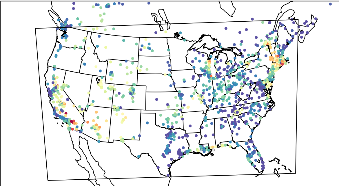
AirNOW (2023-07-02_06:00:00)
