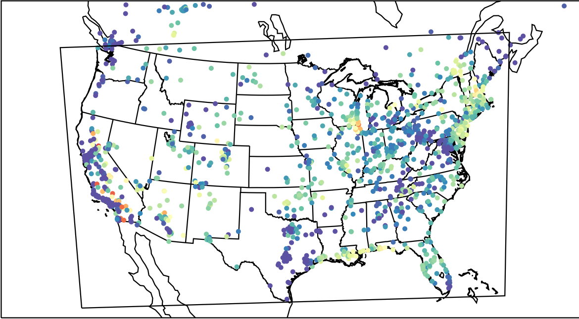
AirNOW (2023-07-02_13:00:00)
