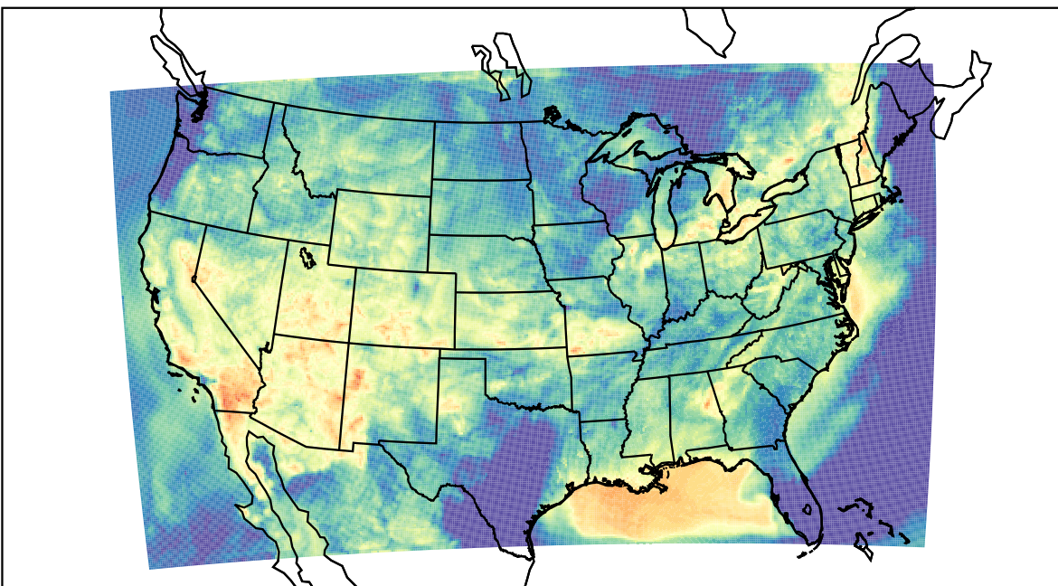
WRF (2023-07-02_09:00:00)
