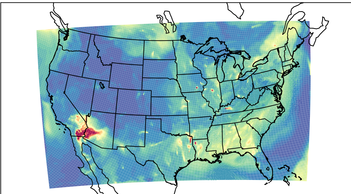
WRF 2023-07-03_07:00:00
