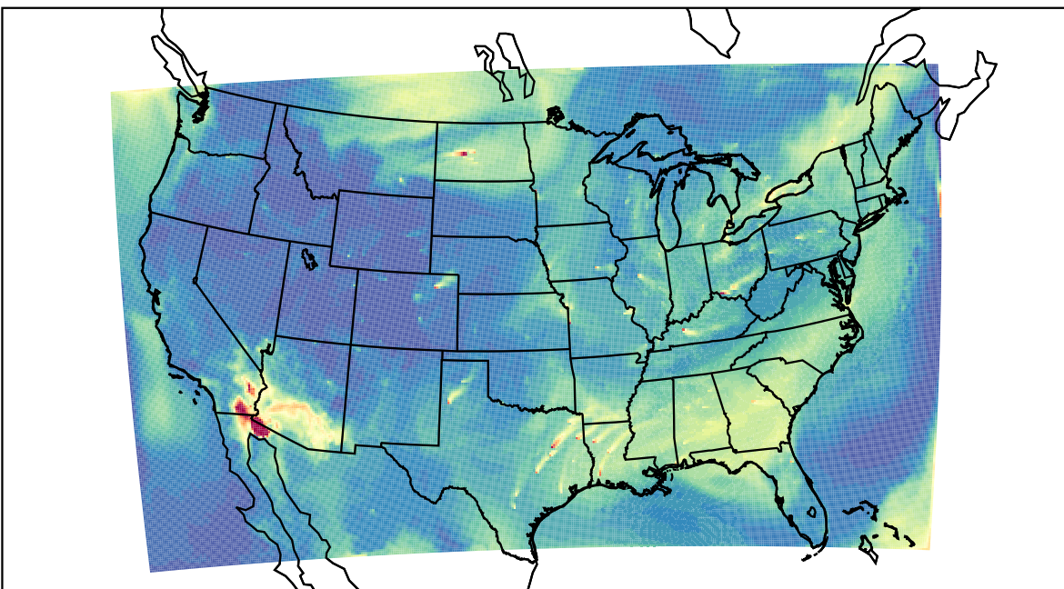
WRF 2023-07-03_15:00:00
