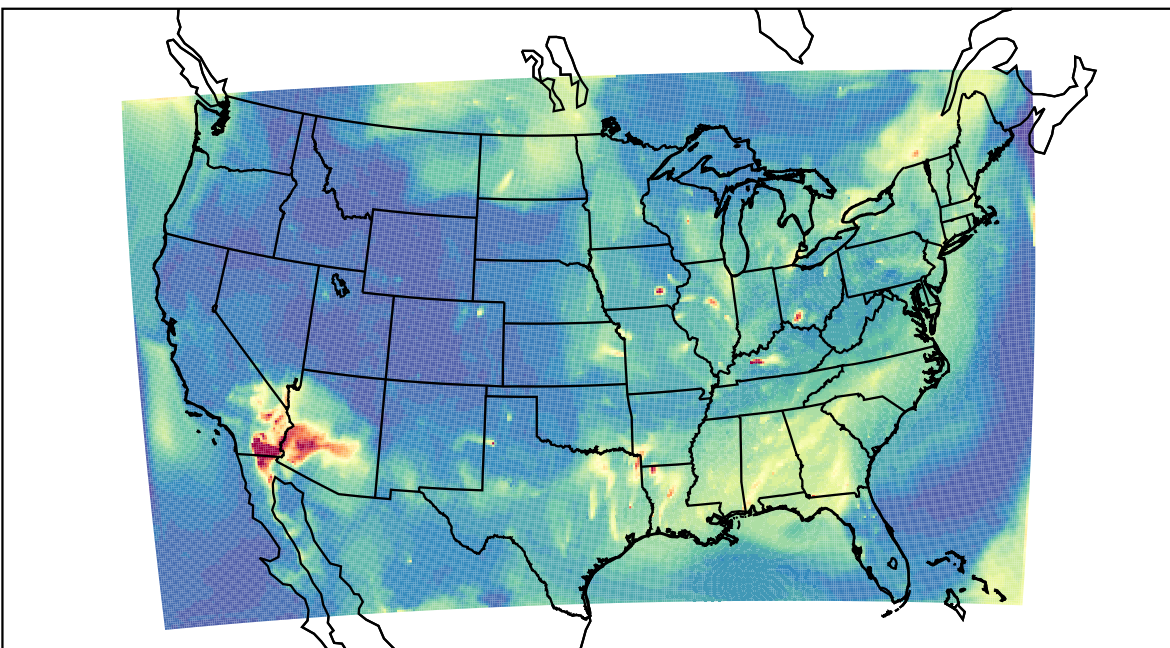
WRF 2023-07-03_09:00:00
