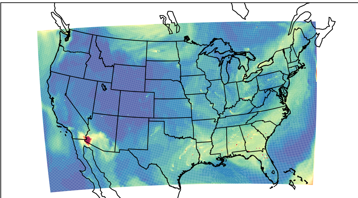
WRF 2023-07-03_19:00:00
