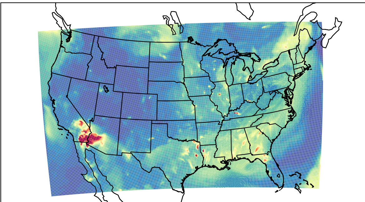
WRF 2023-07-03_05:00:00
