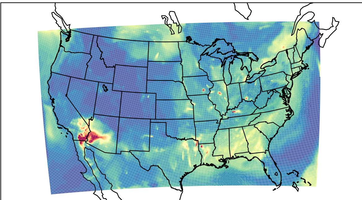
WRF 2023-07-03_08:00:00
