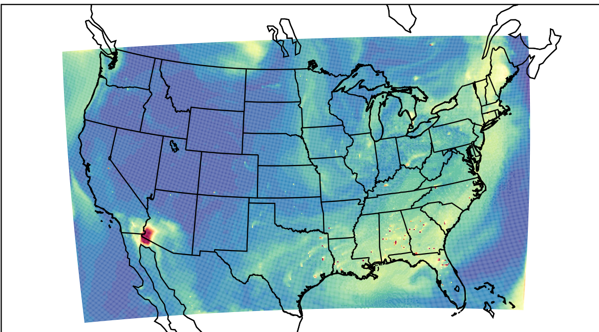
WRF 2023-07-02_21:00:00
