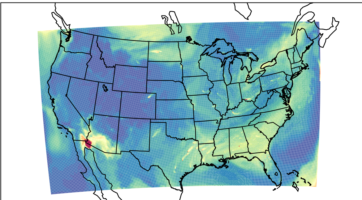
WRF 2023-07-03_17:00:00
