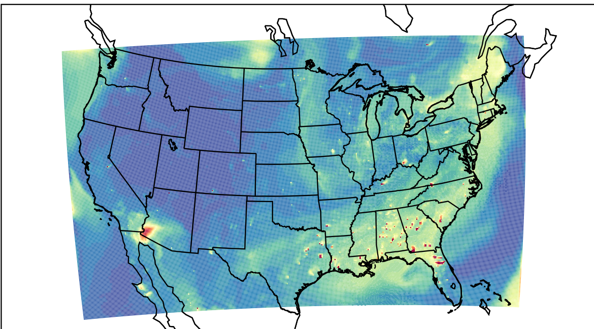
WRF 2023-07-03_00:00:00
