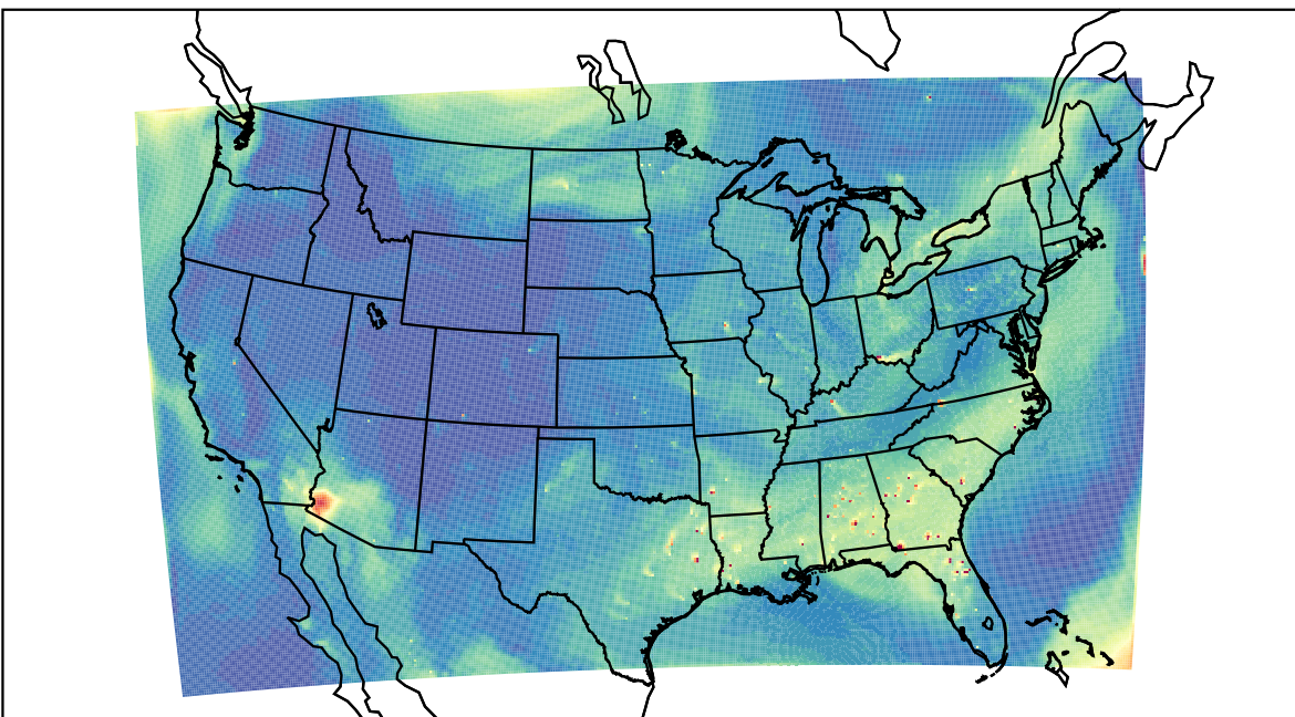
WRF 2023-07-03_21:00:00
