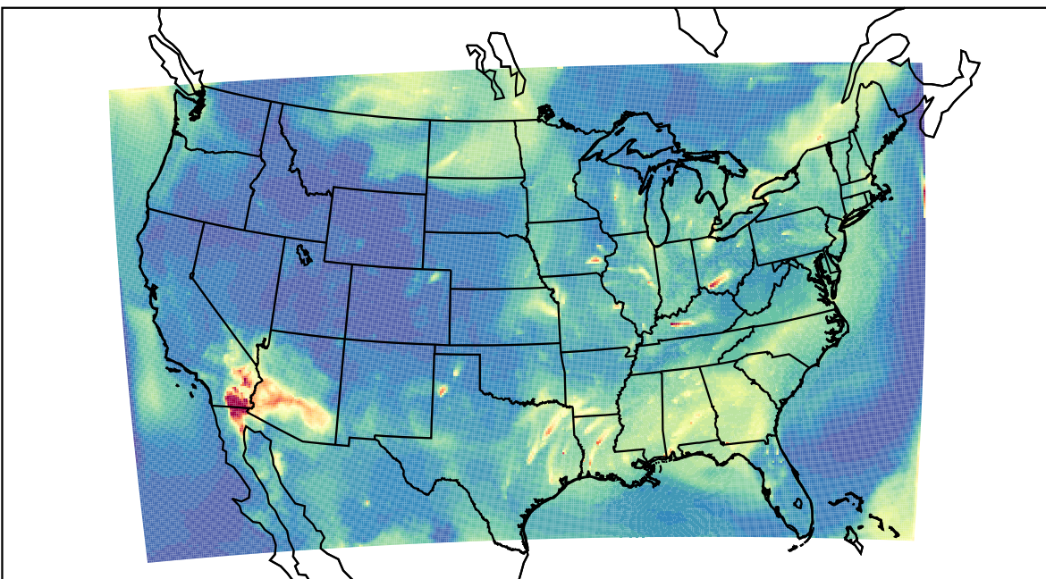
WRF 2023-07-03_12:00:00
