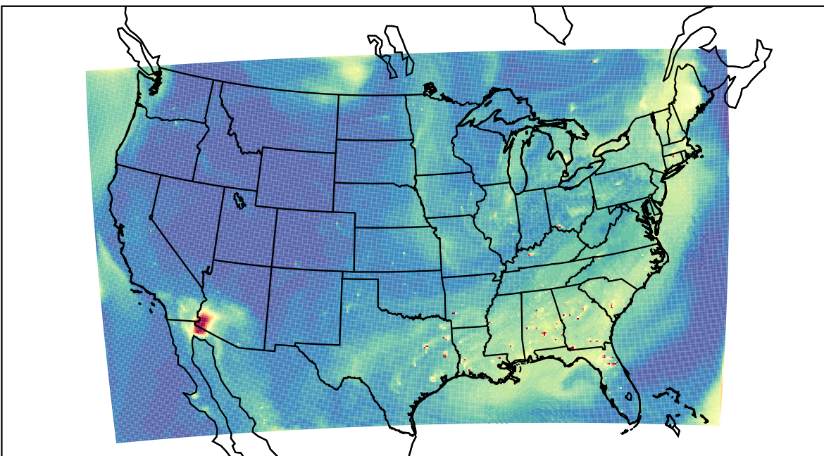
WRF 2023-07-02_22:00:00
