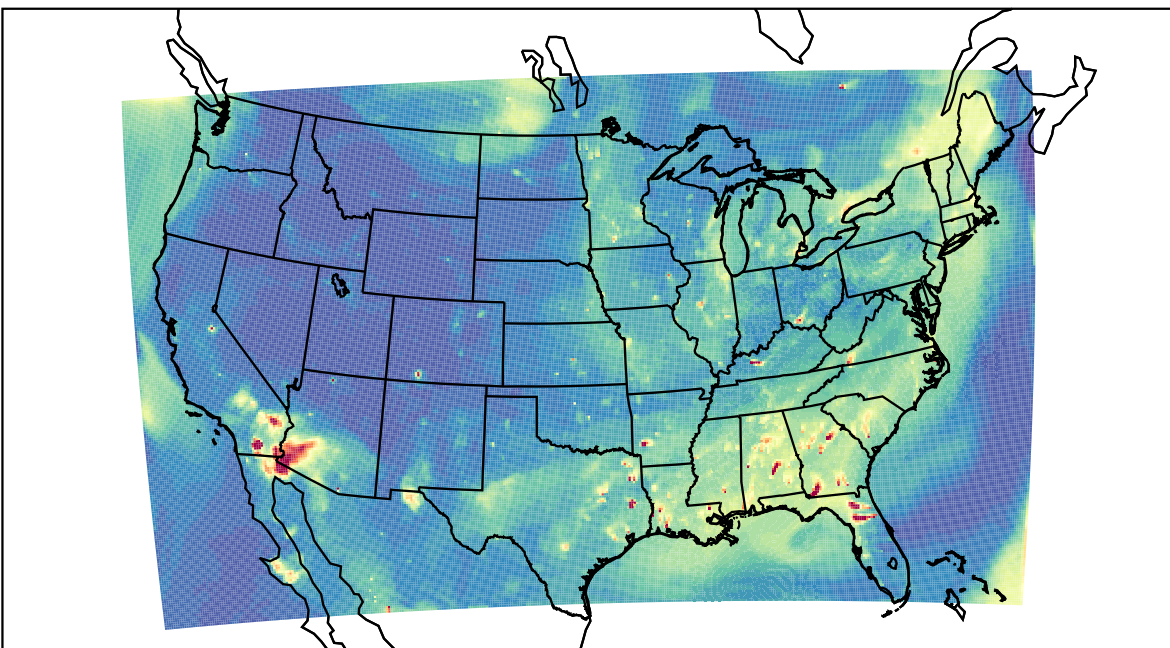
WRF 2023-07-03_02:00:00
