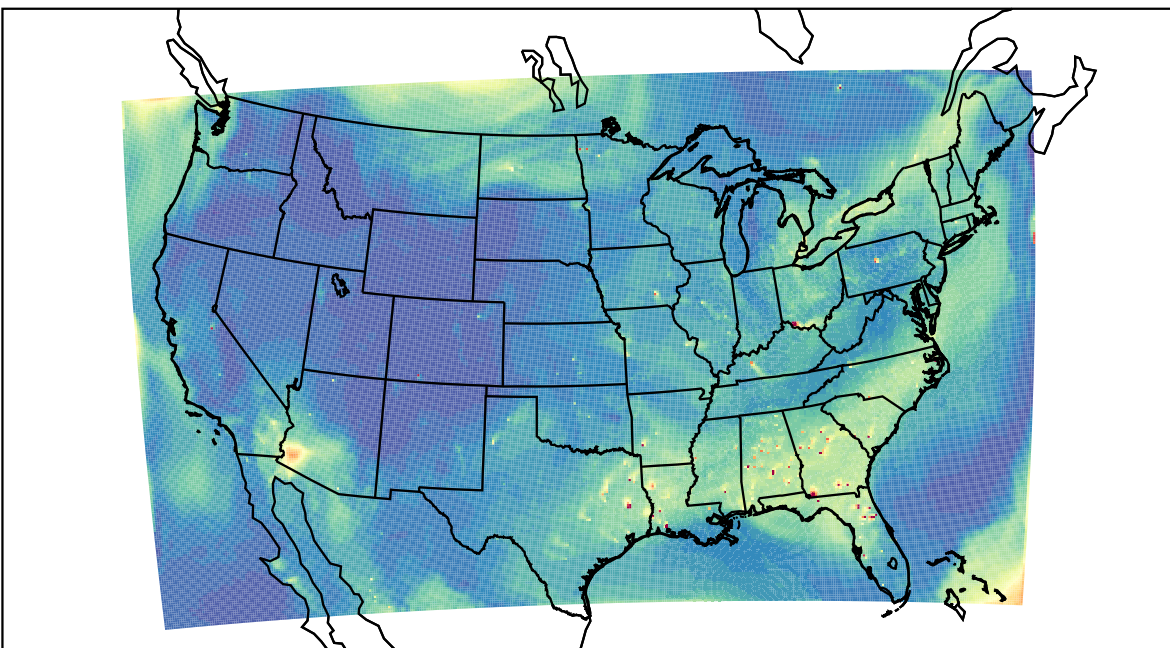
WRF 2023-07-03_22:00:00
