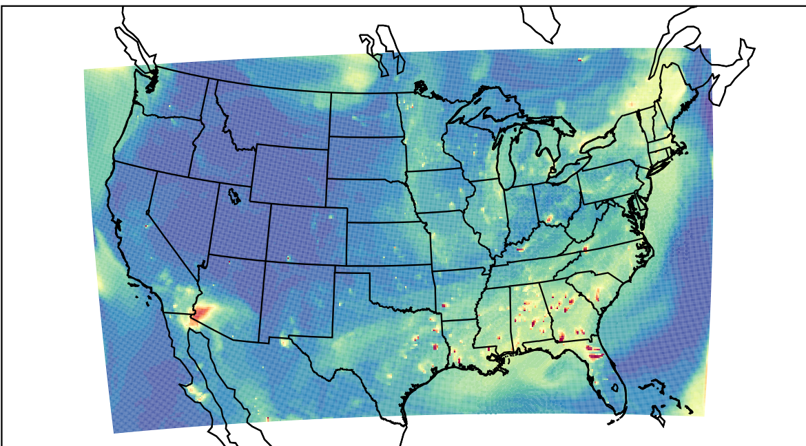
WRF 2023-07-03_01:00:00
