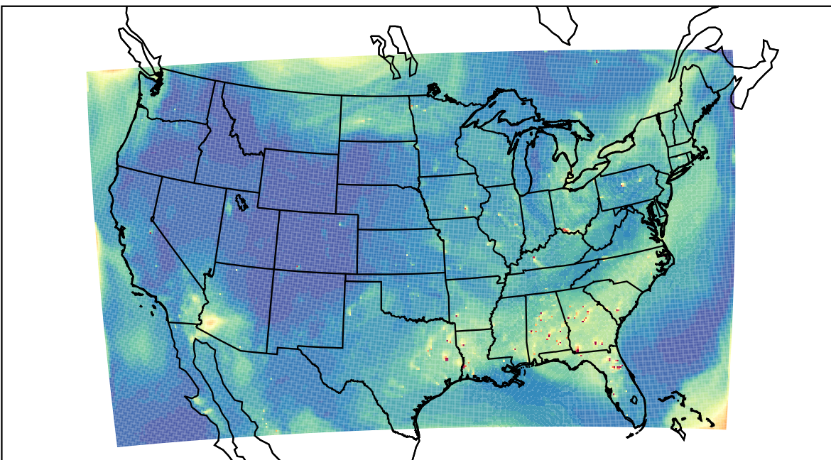
WRF 2023-07-03_23:00:00
