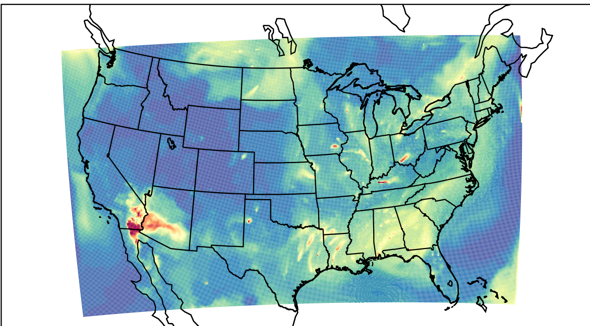
WRF 2023-07-03_11:00:00
