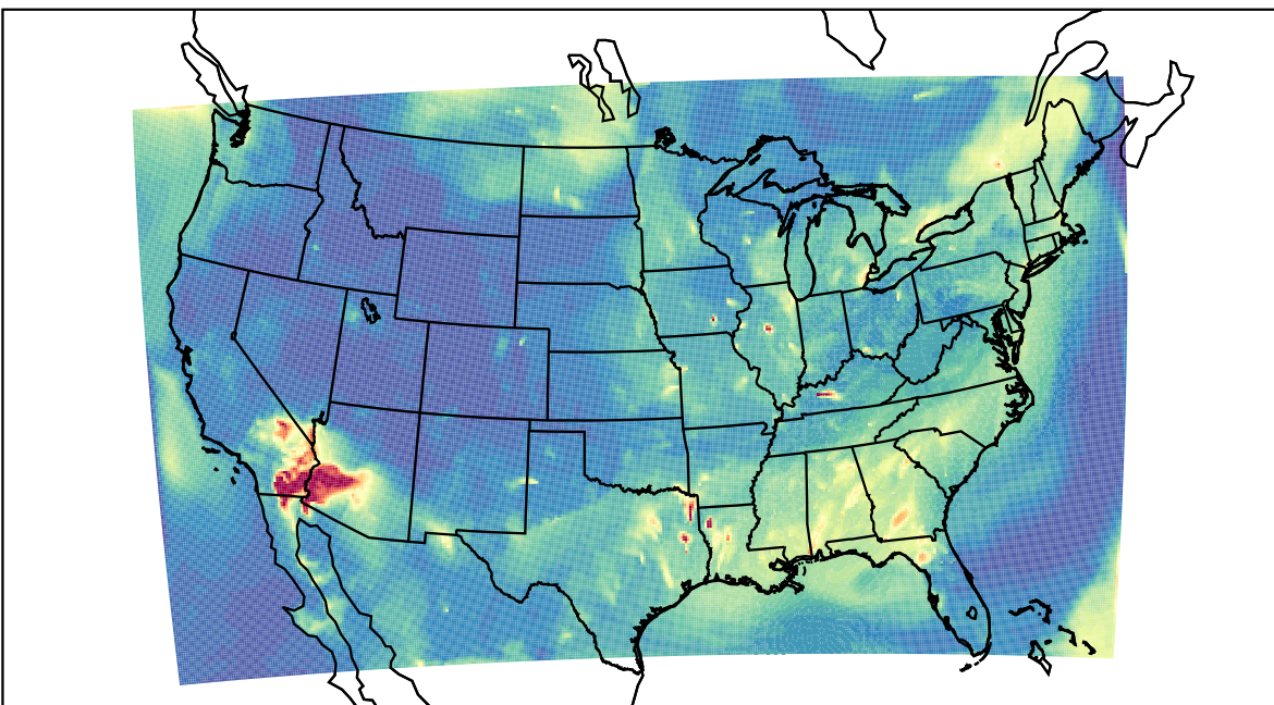
WRF 2023-07-03_06:00:00
