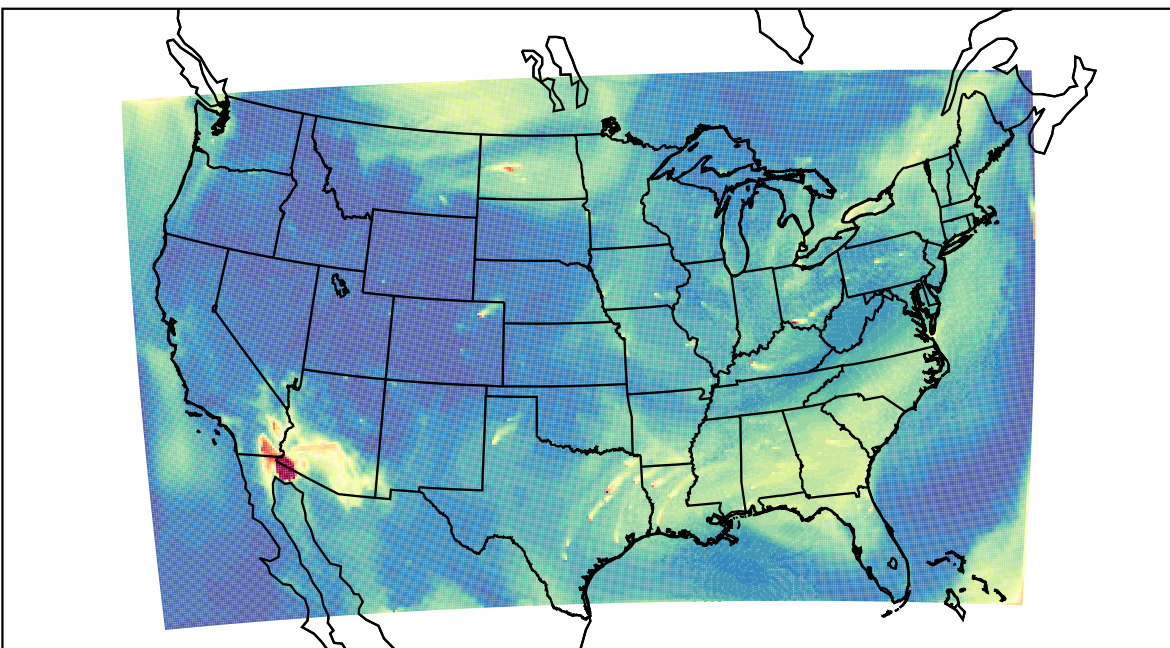
WRF 2023-07-03_16:00:00
