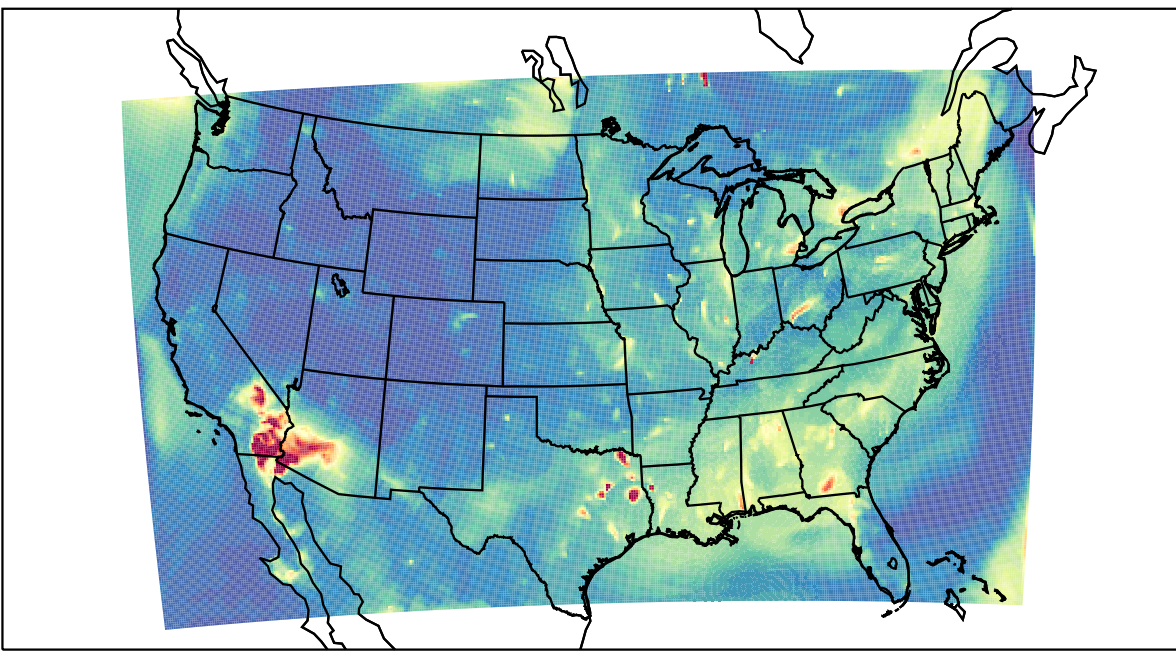
WRF 2023-07-03_05:00:00
