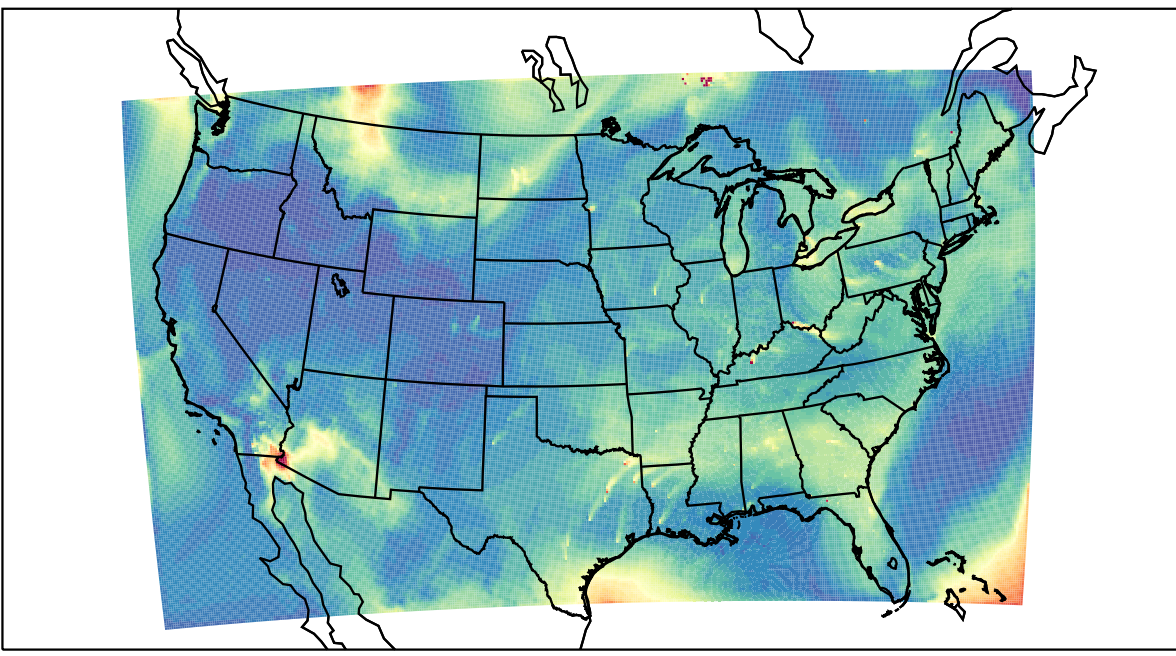
WRF 2023-07-04_17:00:00
