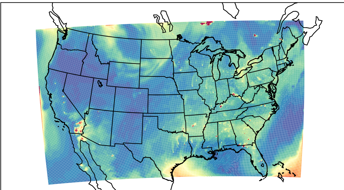
WRF 2023-07-05_00:00:00
