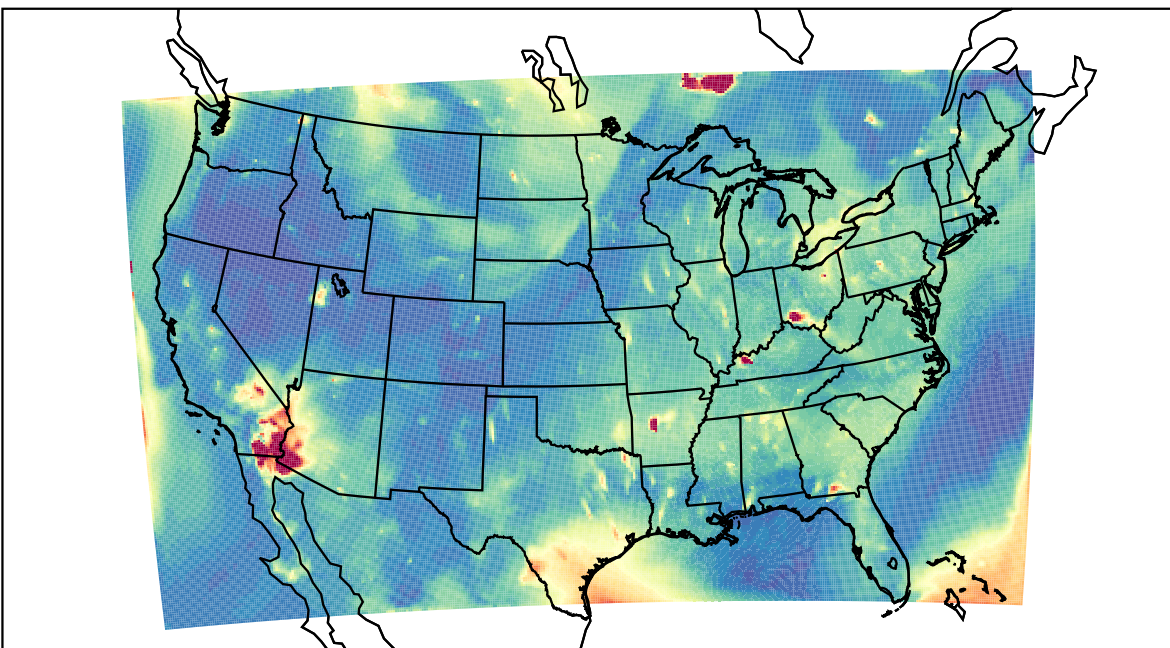
WRF 2023-07-05_04:00:00
