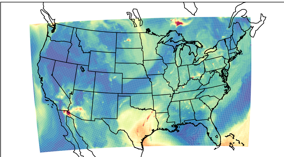
WRF 2023-07-05_15:00:00
