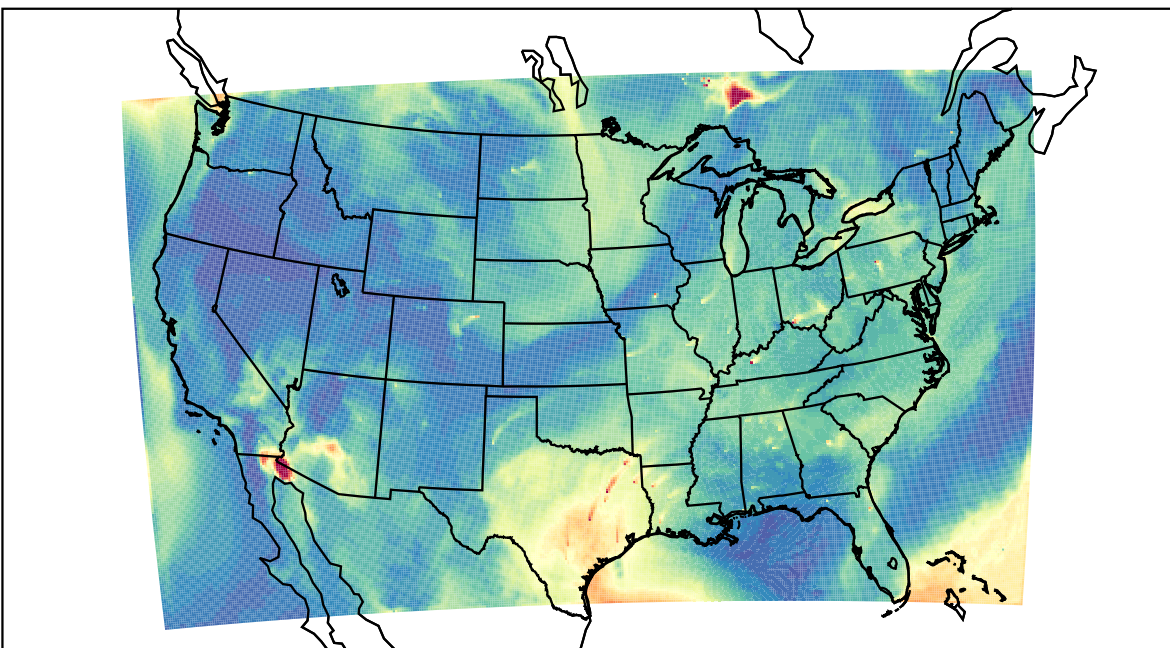
WRF 2023-07-05_16:00:00
