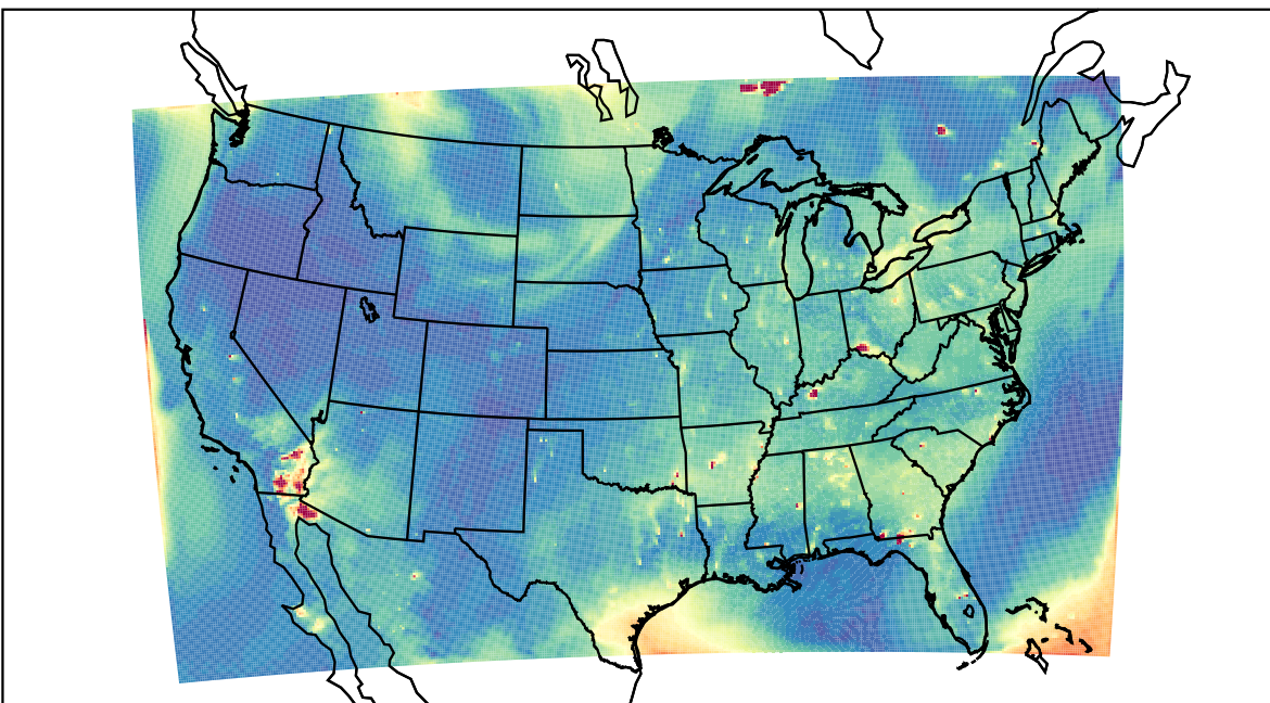
WRF 2023-07-05_01:00:00
