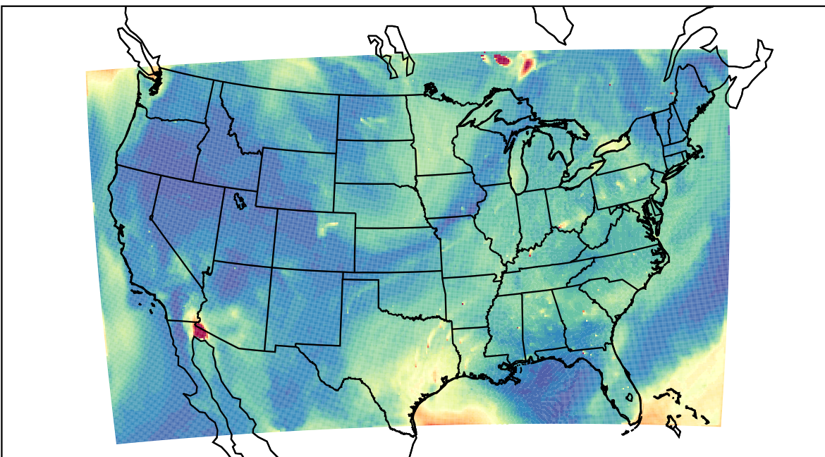
WRF 2023-07-05_19:00:00
