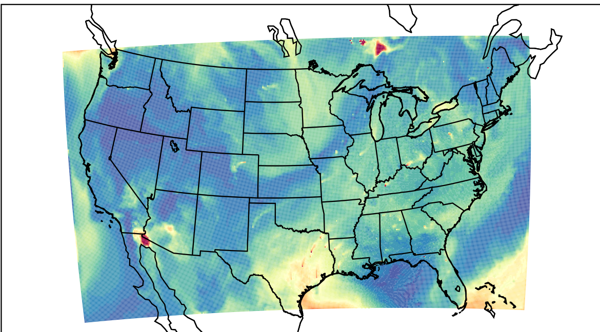
WRF 2023-07-05_17:00:00
