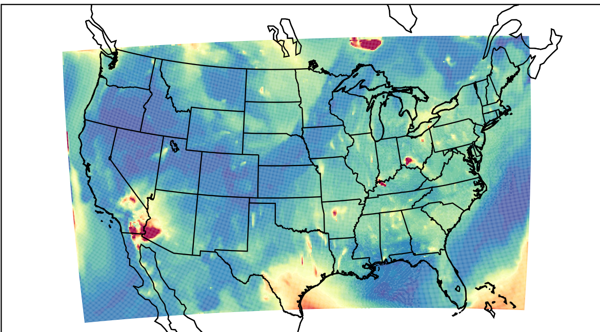
WRF 2023-07-05_06:00:00
