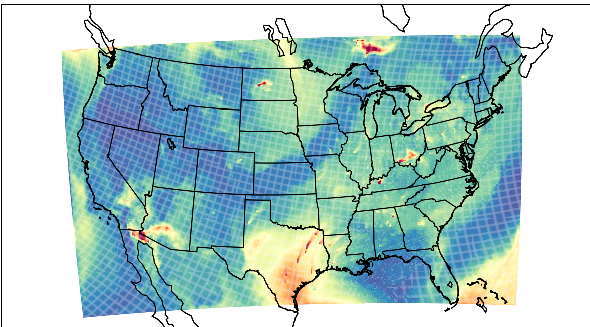
WRF 2023-07-05_14:00:00
