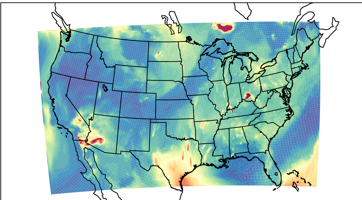
WRF 2023-07-05_09:00:00
