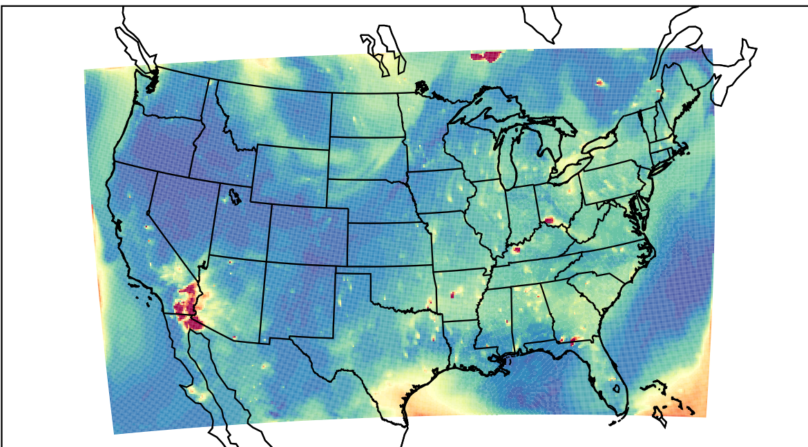
WRF 2023-07-05_02:00:00
