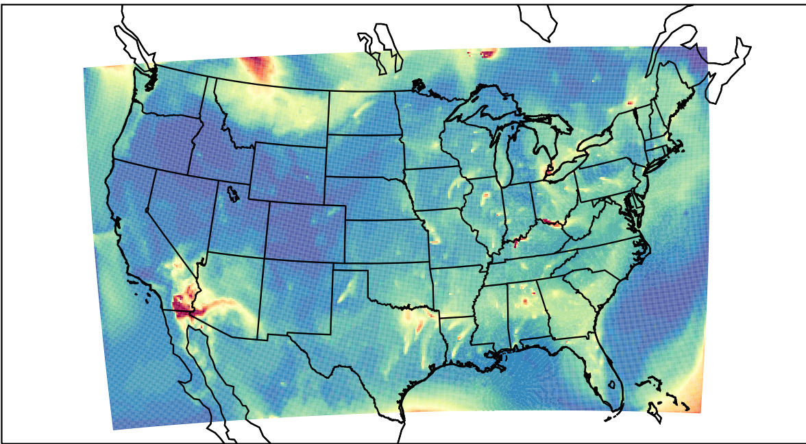
WRF 2023-07-04_12:00:00
