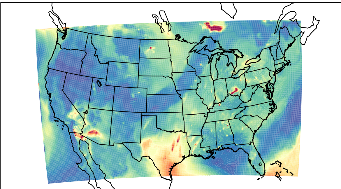
WRF 2023-07-05_12:00:00
