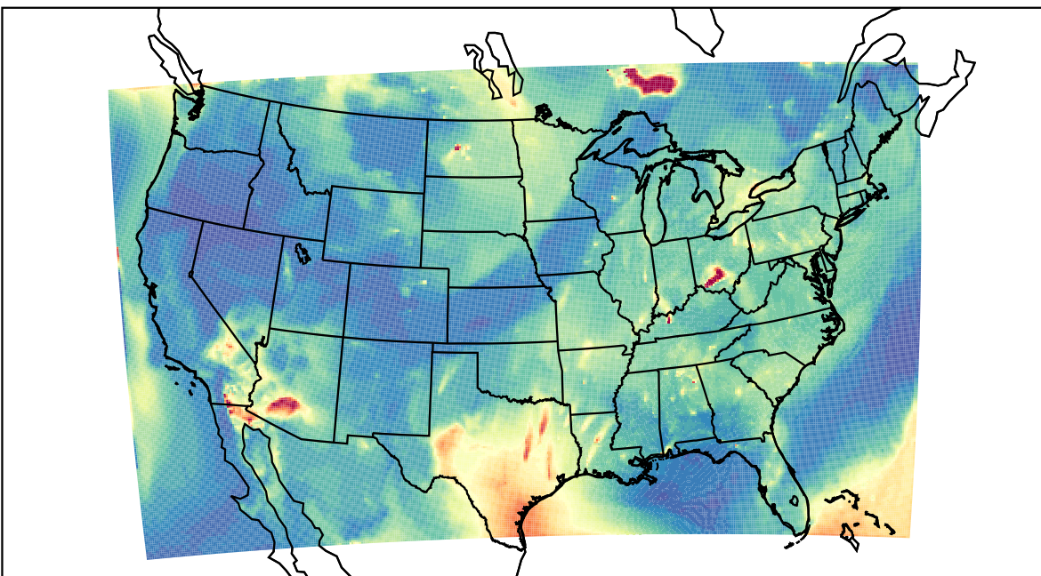
WRF 2023-07-05_11:00:00
