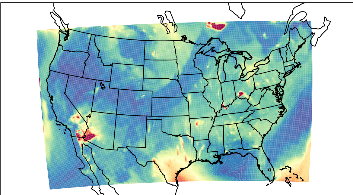
WRF 2023-07-05_07:00:00
