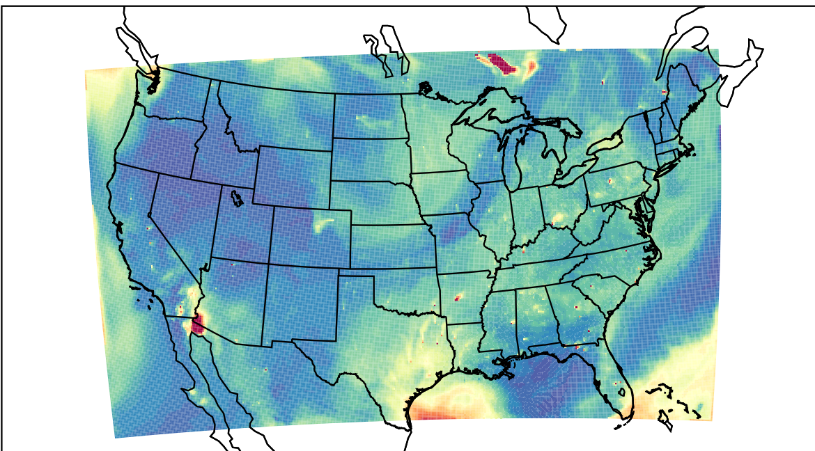
WRF 2023-07-05_23:00:00
