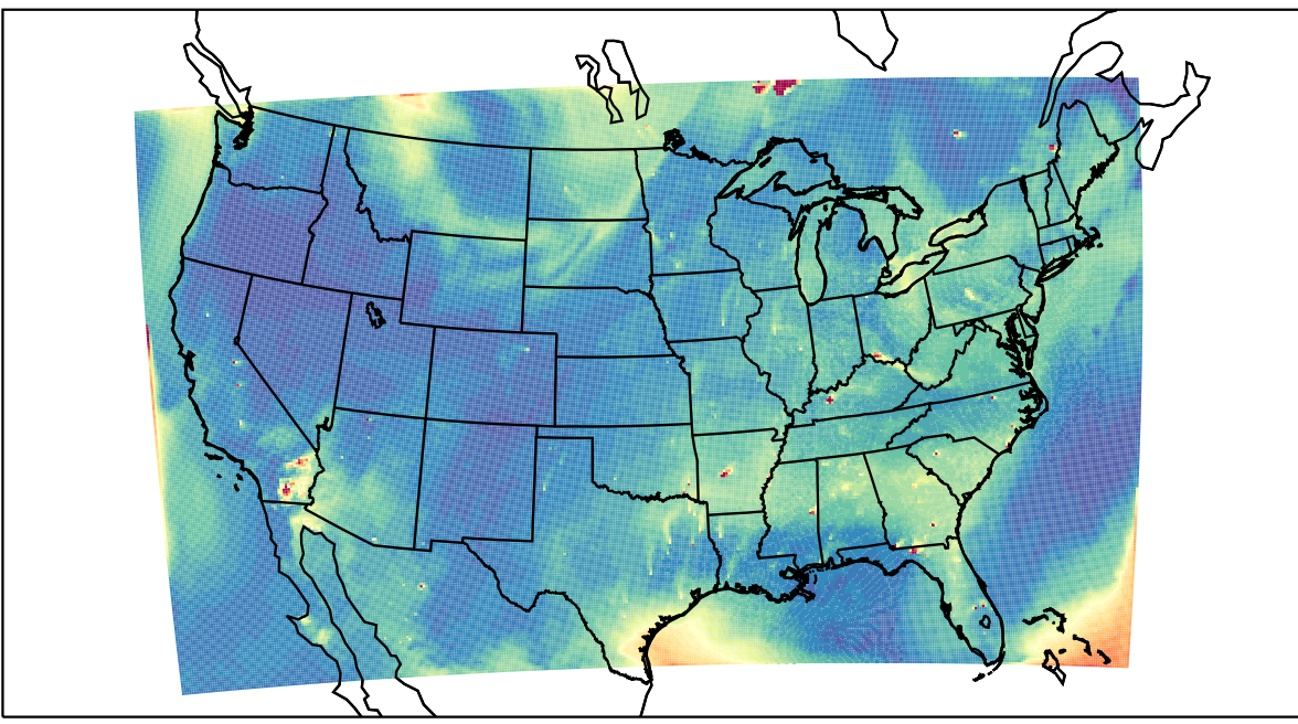
WRF 2023-07-04_23:00:00
