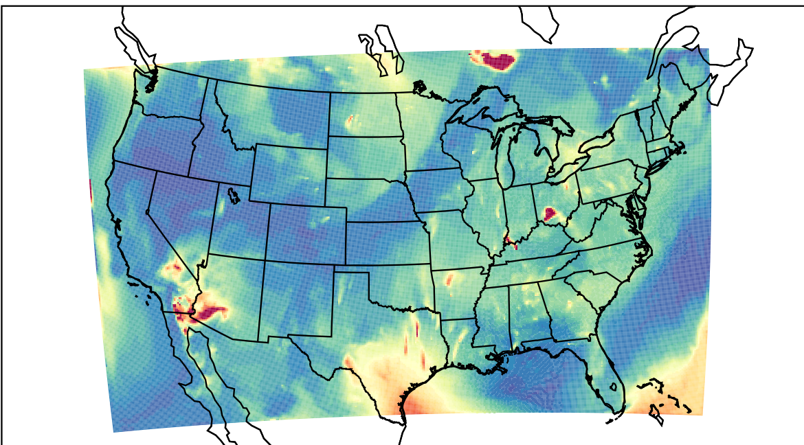
WRF 2023-07-05_08:00:00
