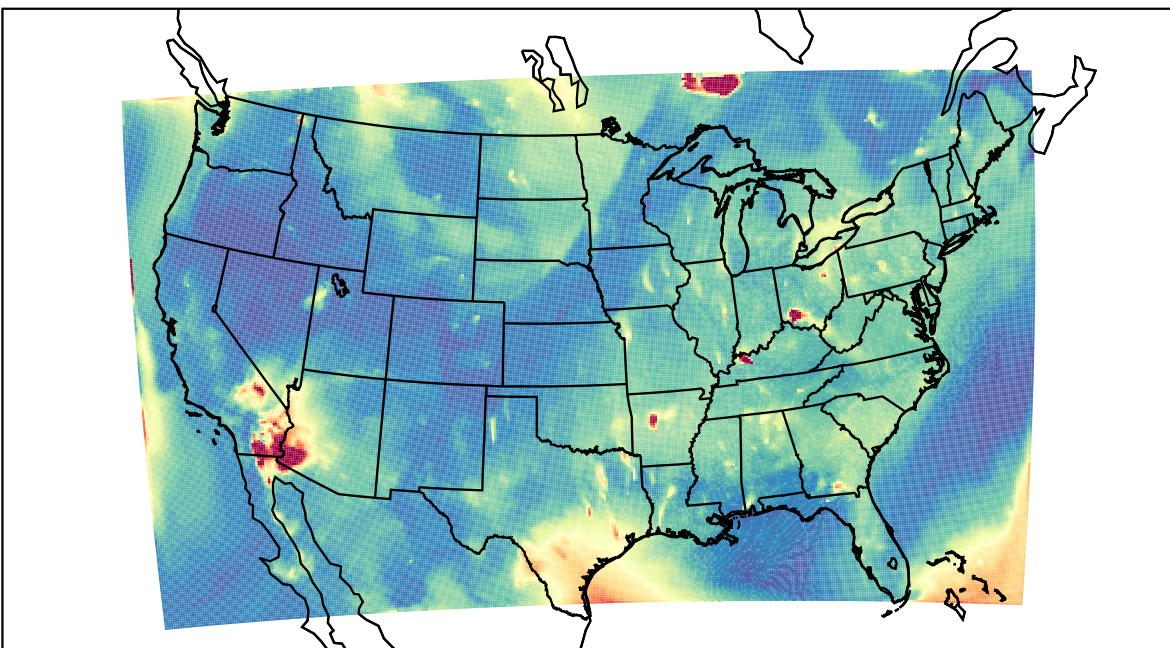
WRF 2023-07-05_05:00:00
