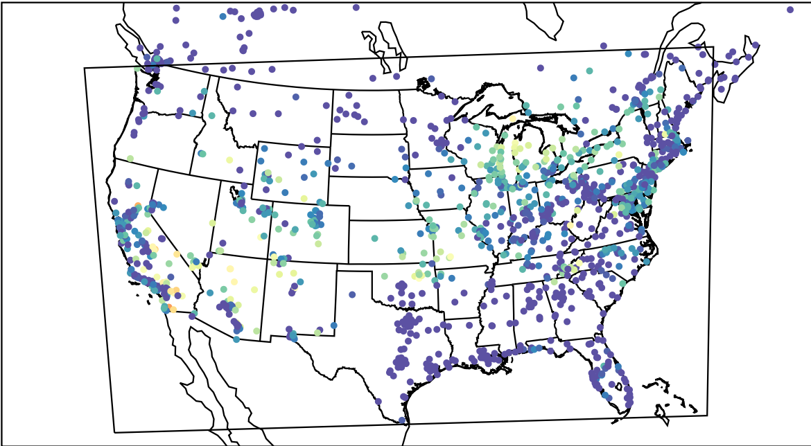
AirNOW (2023-07-05_12:00:00)
