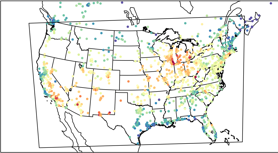
AirNOW (2023-07-04_18:00:00)
