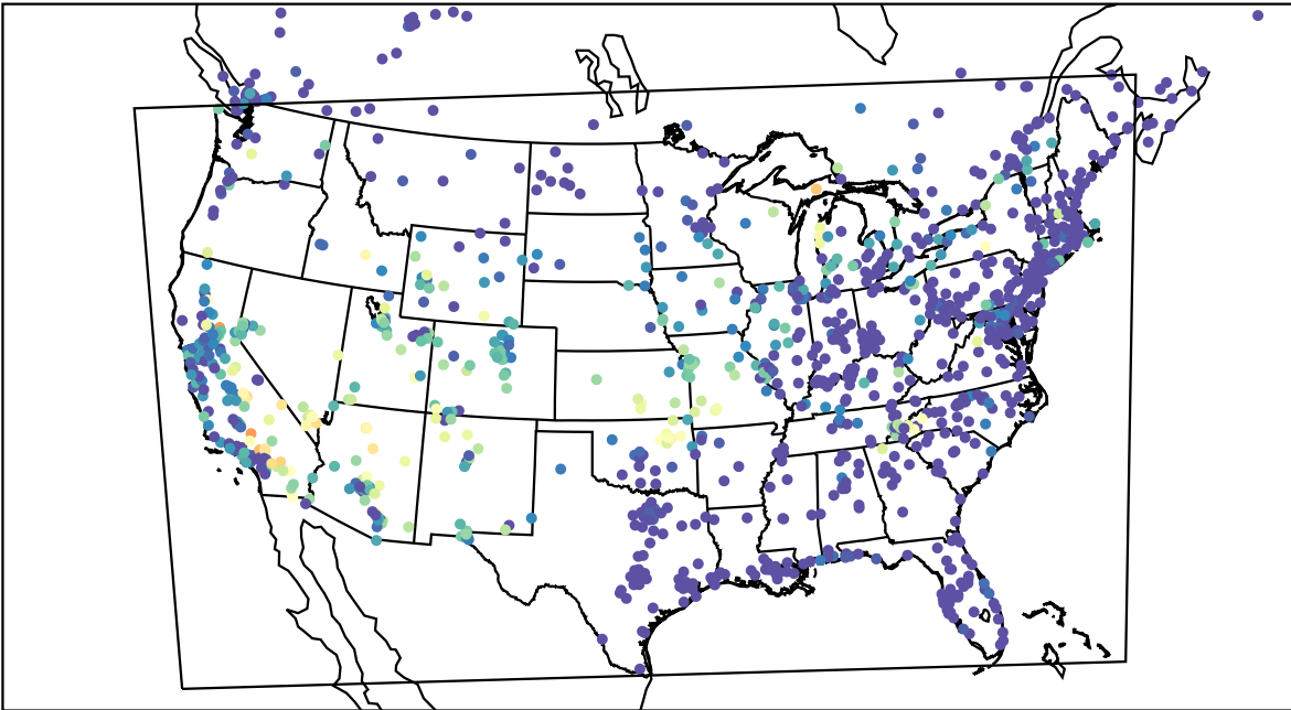
AirNOW (2023-07-05_10:00:00)
