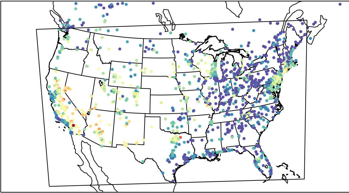
AirNOW (2023-07-04_04:00:00)
