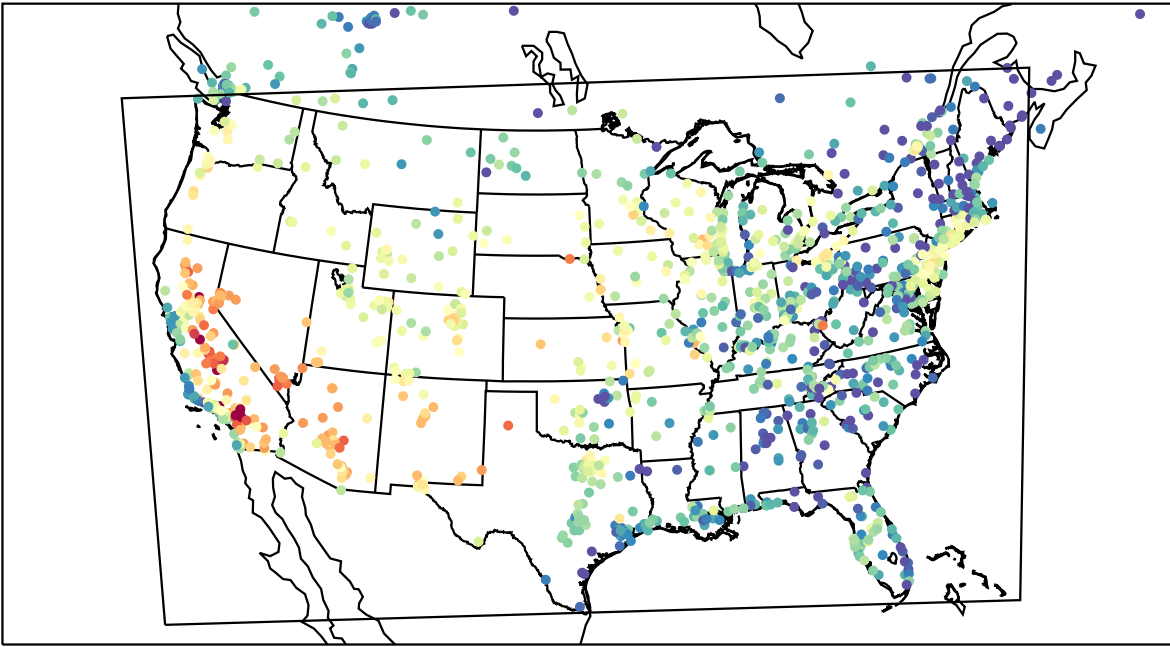
AirNOW (2023-07-04_01:00:00)
