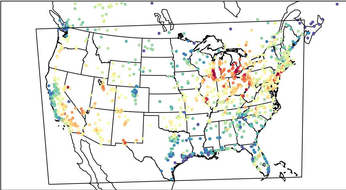
AirNOW (2023-07-05_18:00:00)
