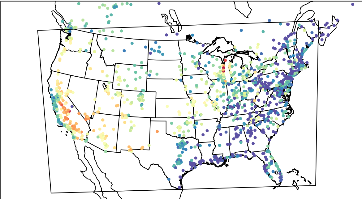
AirNOW (2023-07-05_02:00:00)
