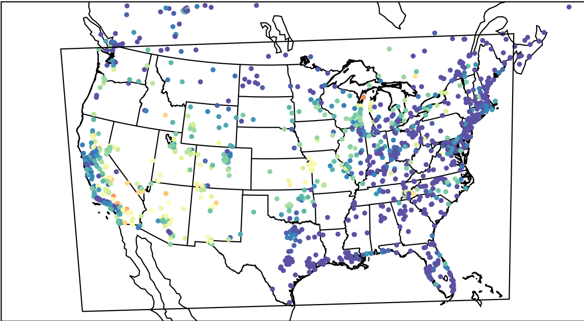
AirNOW (2023-07-05_06:00:00)
