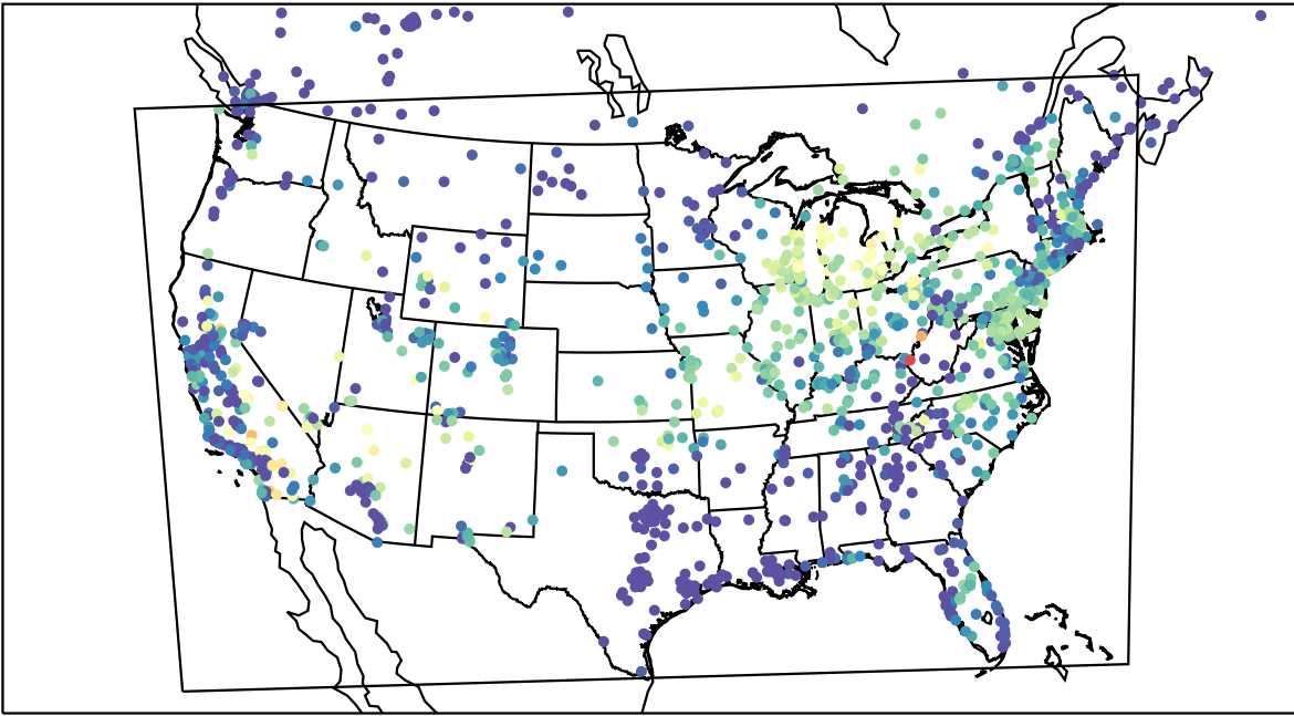
AirNOW (2023-07-05_13:00:00)
