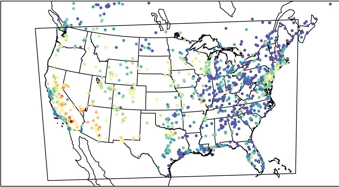
AirNOW (2023-07-04_03:00:00)
