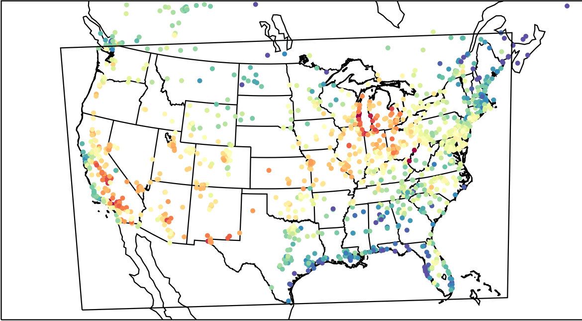
AirNOW (2023-07-04_22:00:00)
