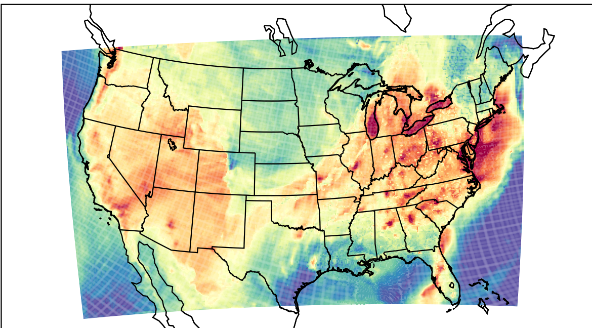
WRF (2023-07-05_21:00:00)
