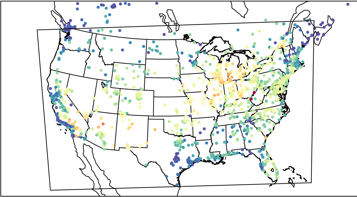
AirNOW (2023-07-04_15:00:00)
