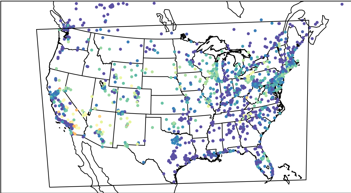
AirNOW (2023-07-04_12:00:00)
