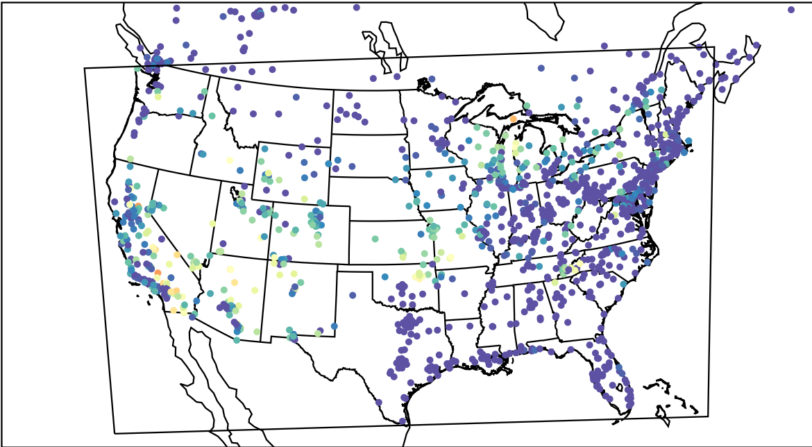
AirNOW (2023-07-05_11:00:00)
