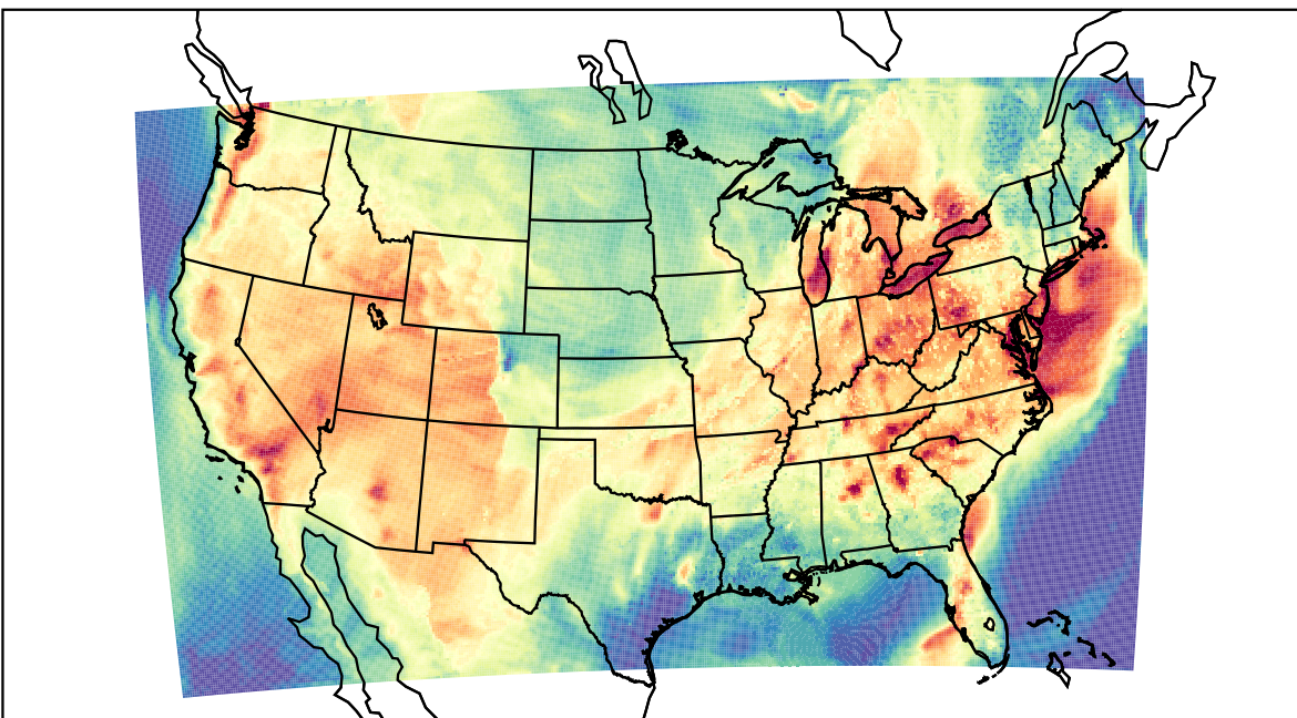
WRF (2023-07-05_22:00:00)
