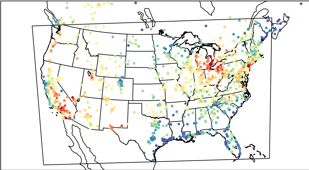
AirNOW (2023-07-05_21:00:00)
