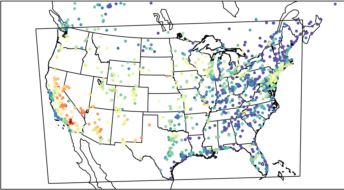
AirNOW (2023-07-04_02:00:00)
