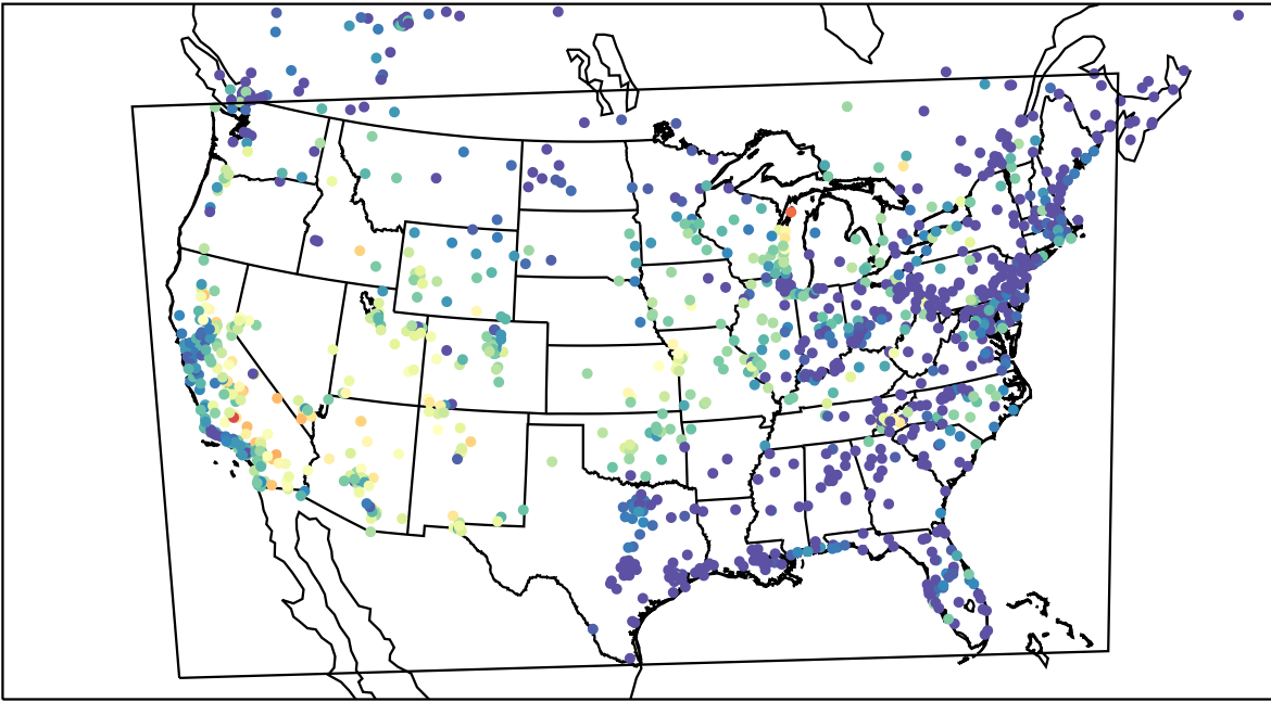
AirNOW (2023-07-05_05:00:00)
