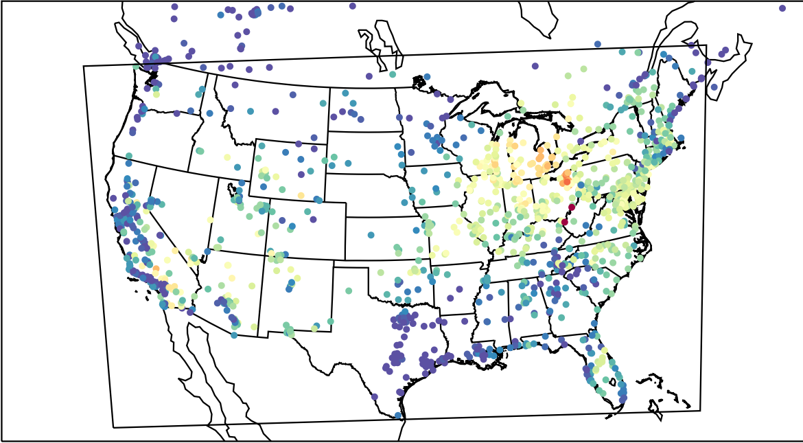
AirNOW (2023-07-05_14:00:00)
