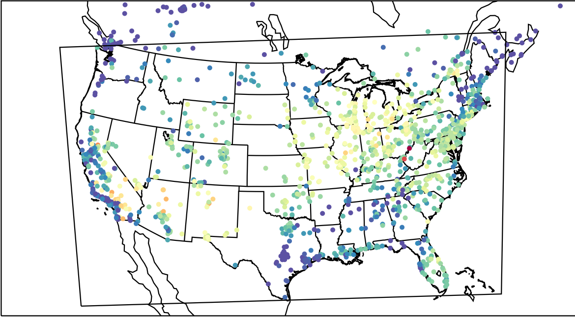
AirNOW (2023-07-04_14:00:00)
