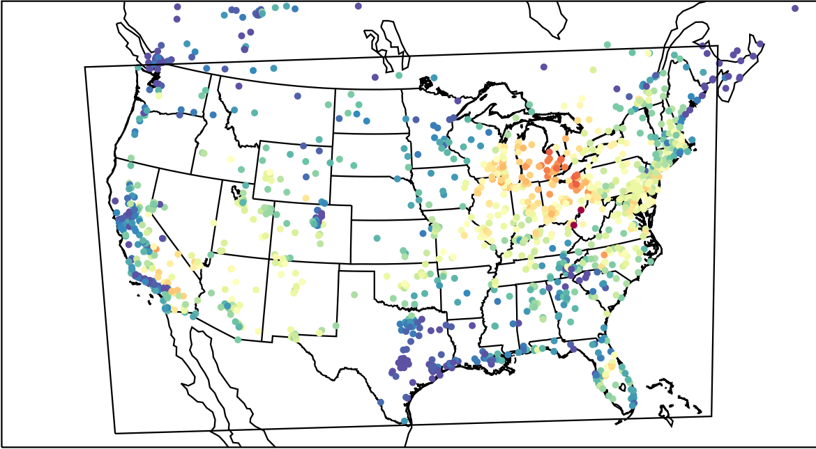
AirNOW (2023-07-05_15:00:00)
