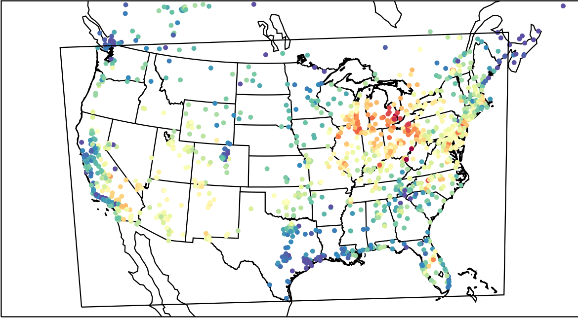
AirNOW (2023-07-05_16:00:00)
