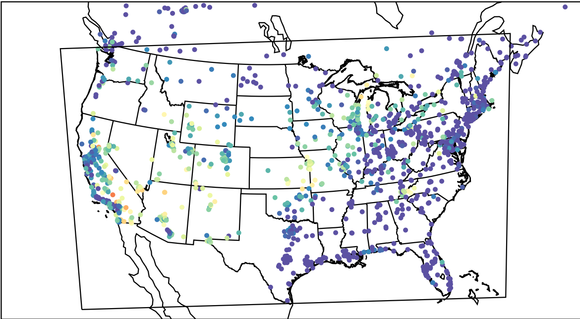
AirNOW (2023-07-05_08:00:00)
