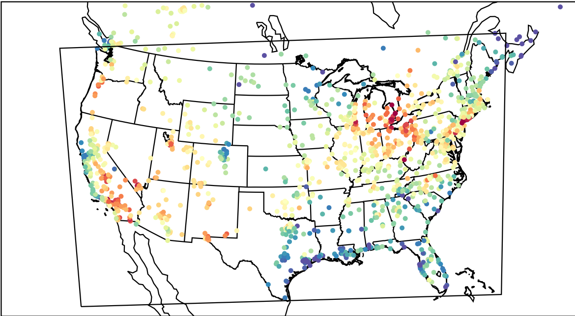
AirNOW (2023-07-05_20:00:00)
