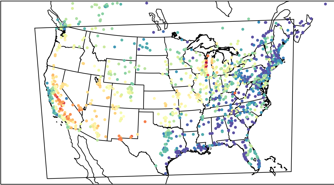
AirNOW (2023-07-05_01:00:00)
