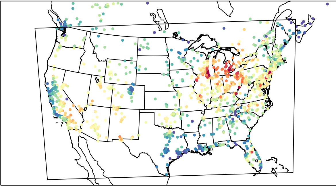
AirNOW (2023-07-05_17:00:00)
