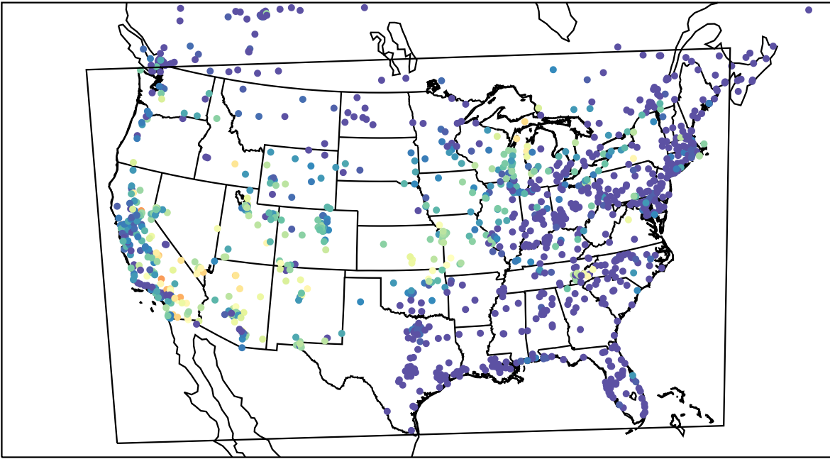
AirNOW (2023-07-05_09:00:00)
