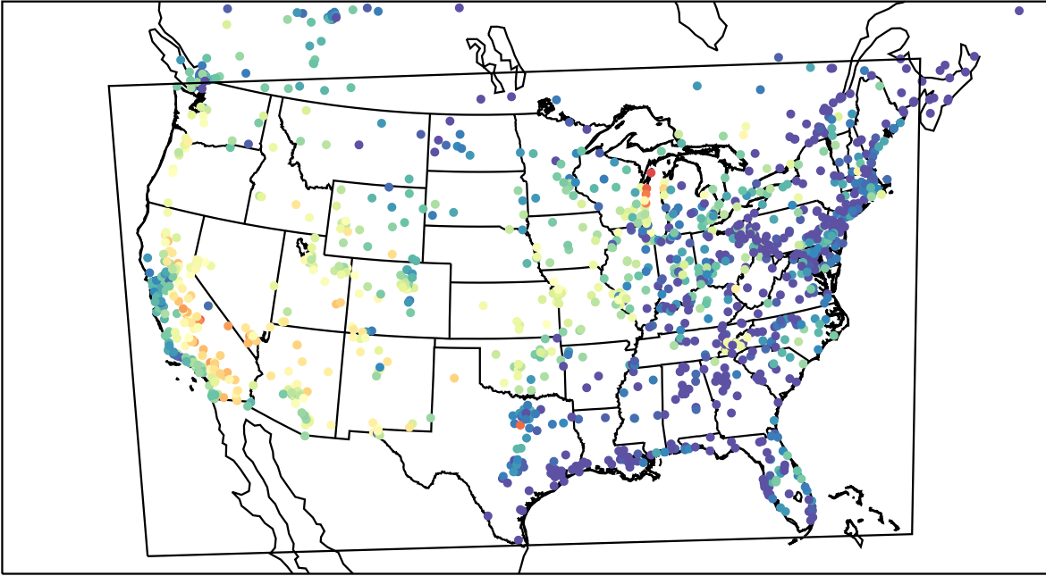
AirNOW (2023-07-05_03:00:00)
