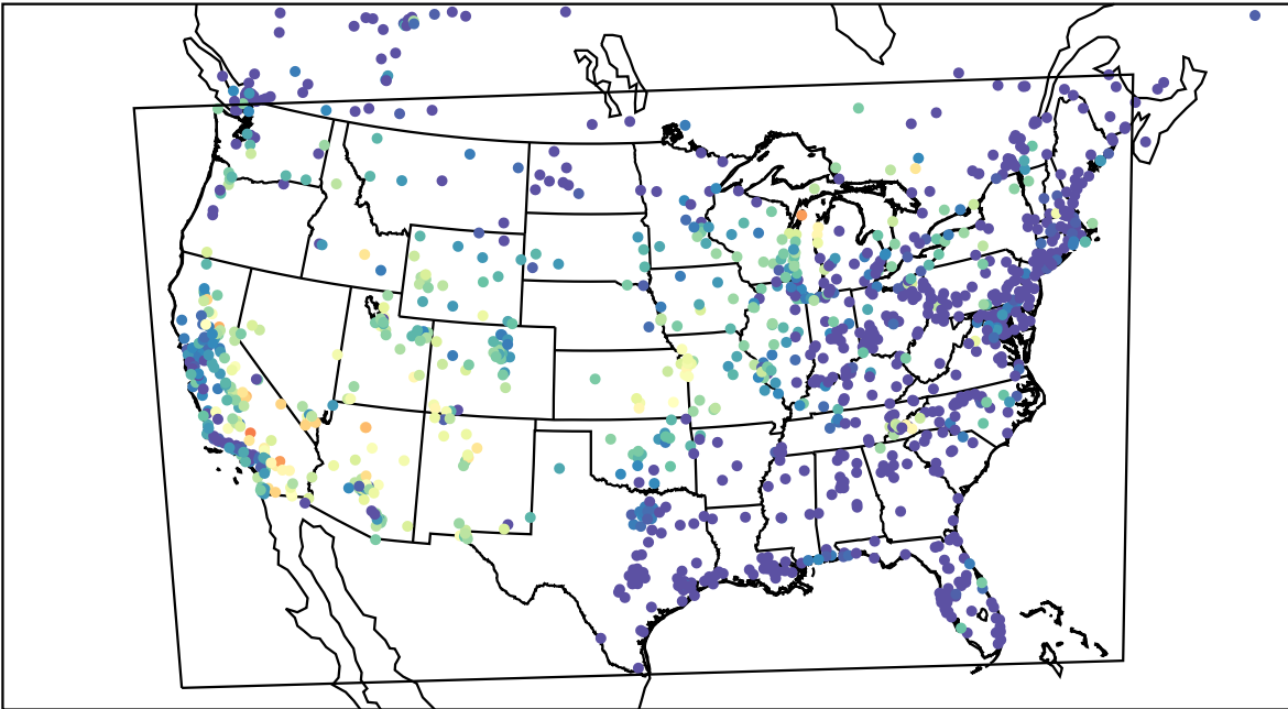
AirNOW (2023-07-05_07:00:00)
