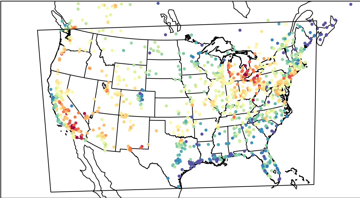
AirNOW (2023-07-05_22:00:00)
