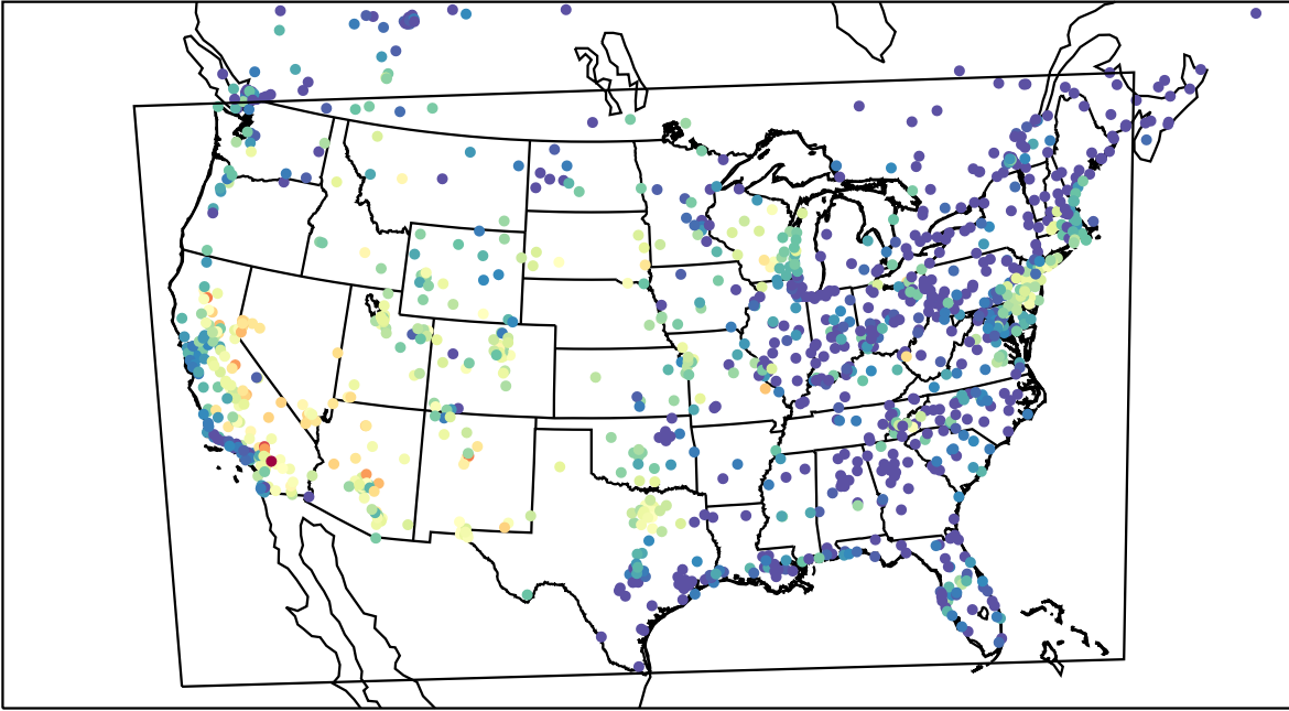
AirNOW (2023-07-04_05:00:00)
