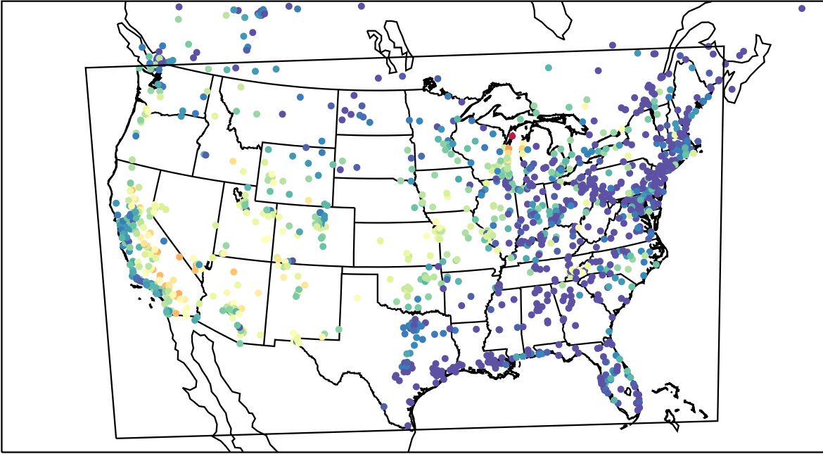
AirNOW (2023-07-05_04:00:00)
