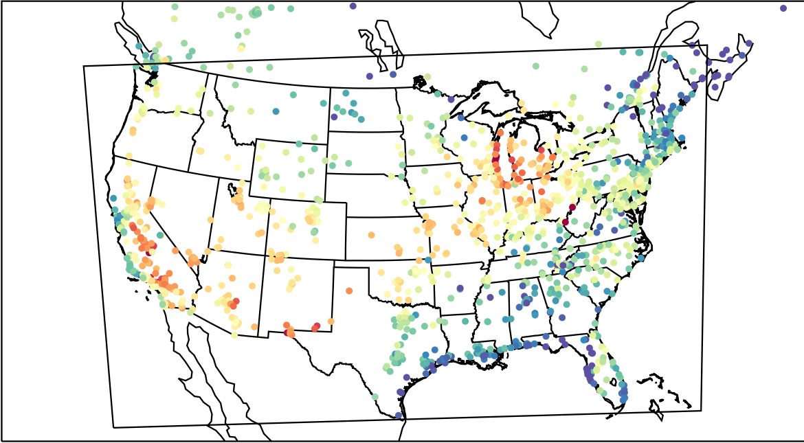
AirNOW (2023-07-04_23:00:00)
