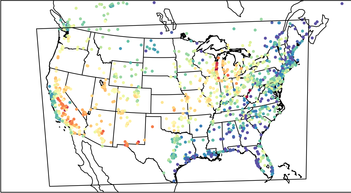
AirNOW (2023-07-05_00:00:00)
