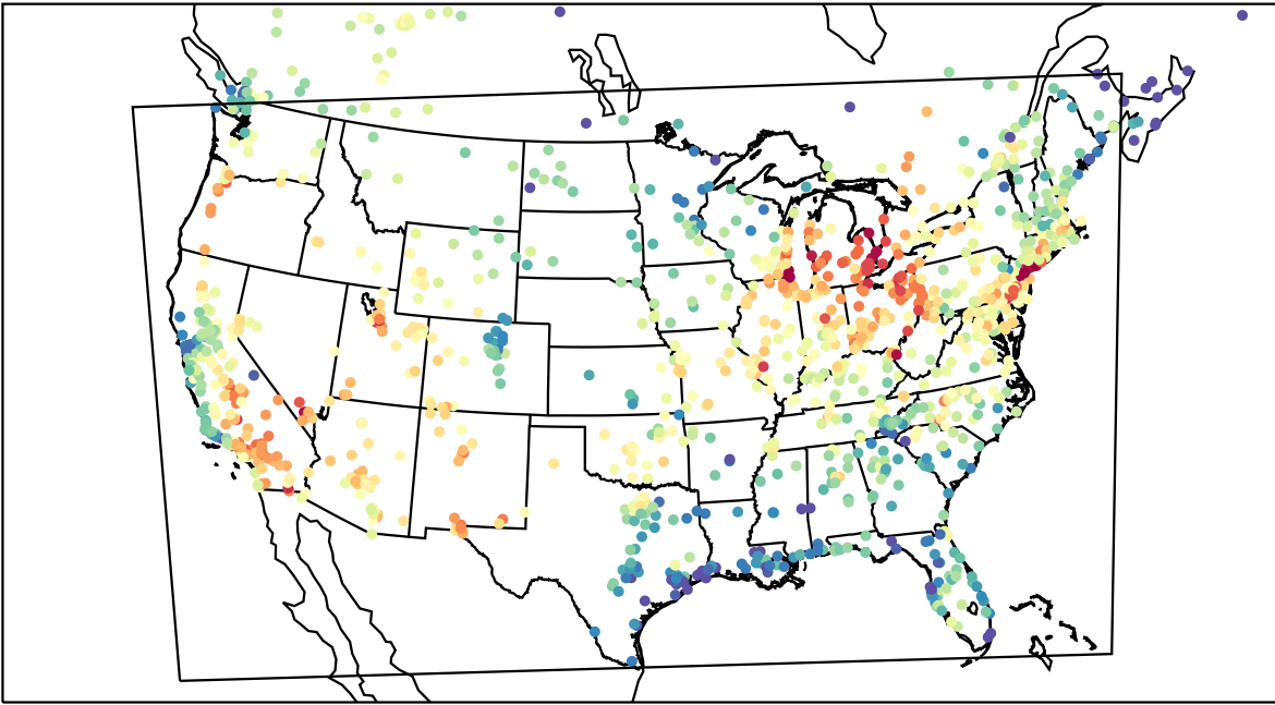
AirNOW (2023-07-05_19:00:00)
