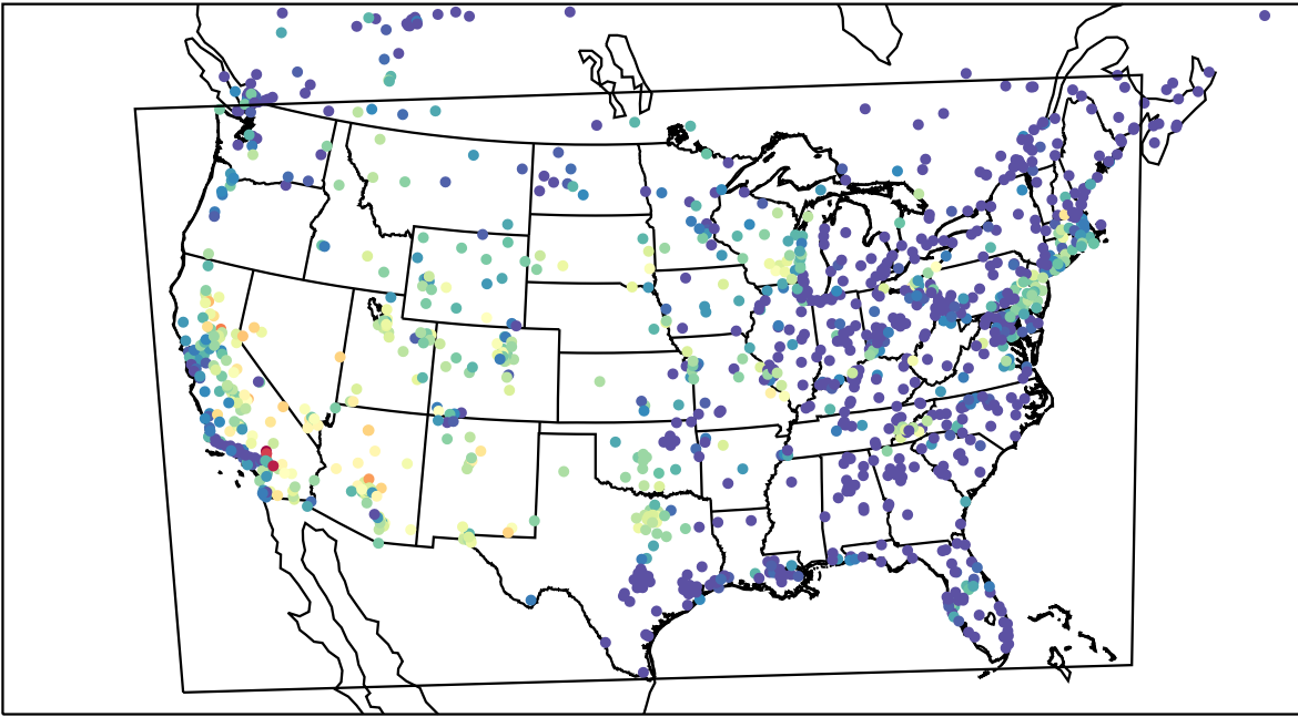
AirNOW (2023-07-04_07:00:00)
