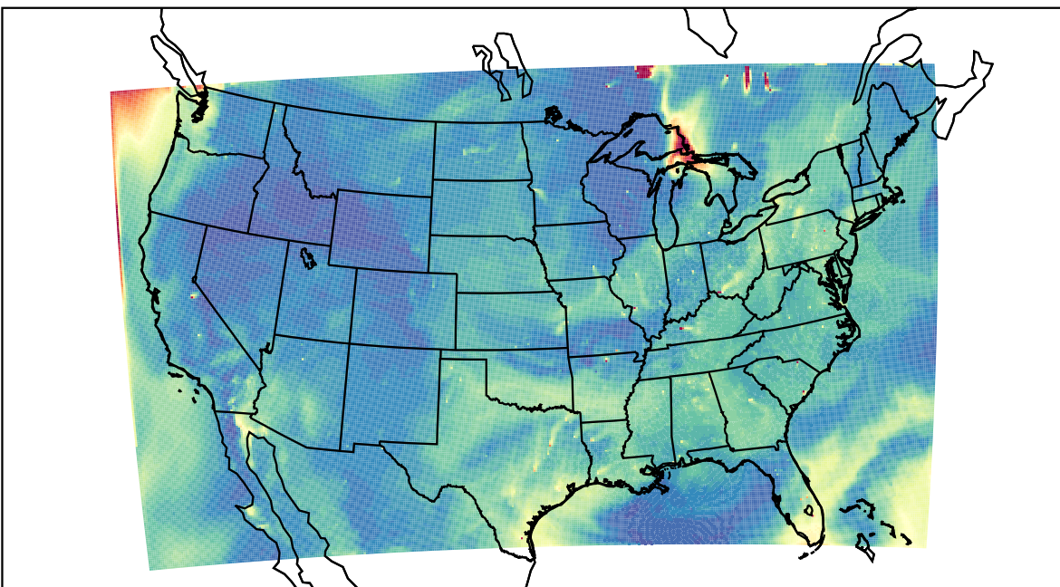
WRF 2023-07-06_22:00:00
