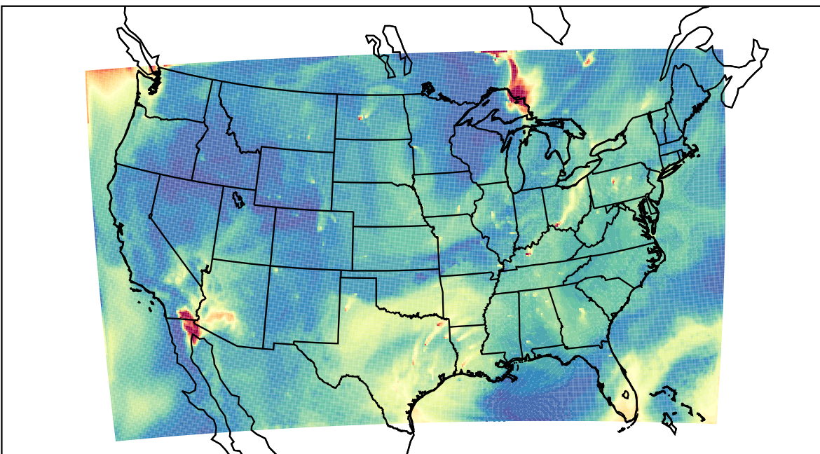
WRF 2023-07-06_15:00:00
