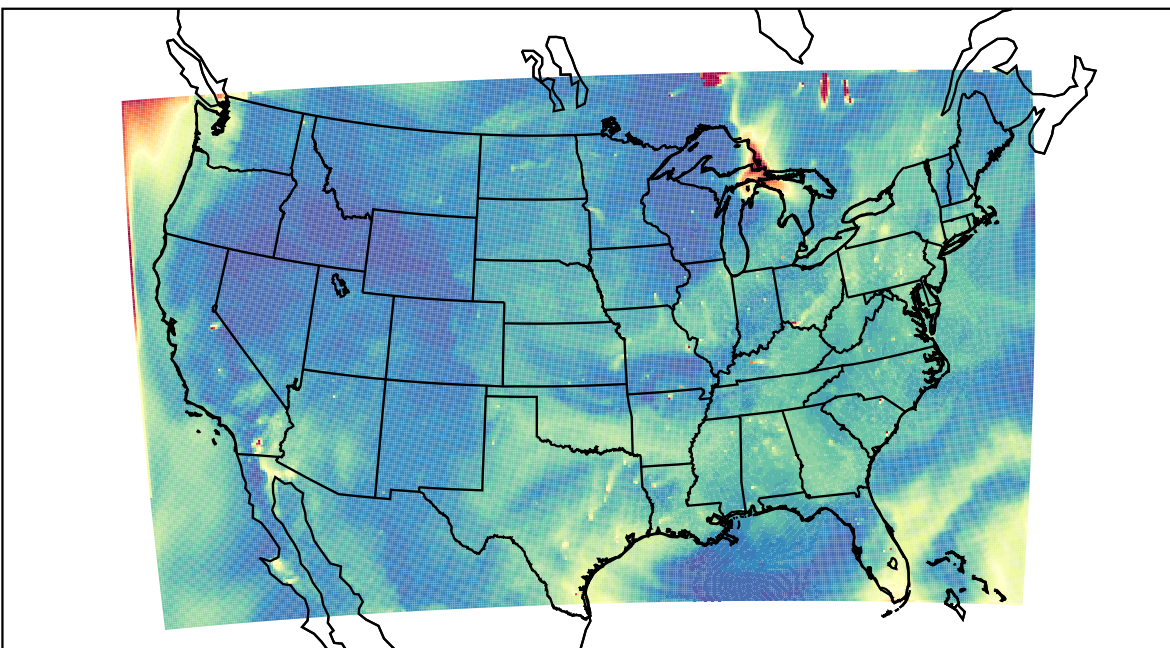
WRF 2023-07-06_23:00:00
