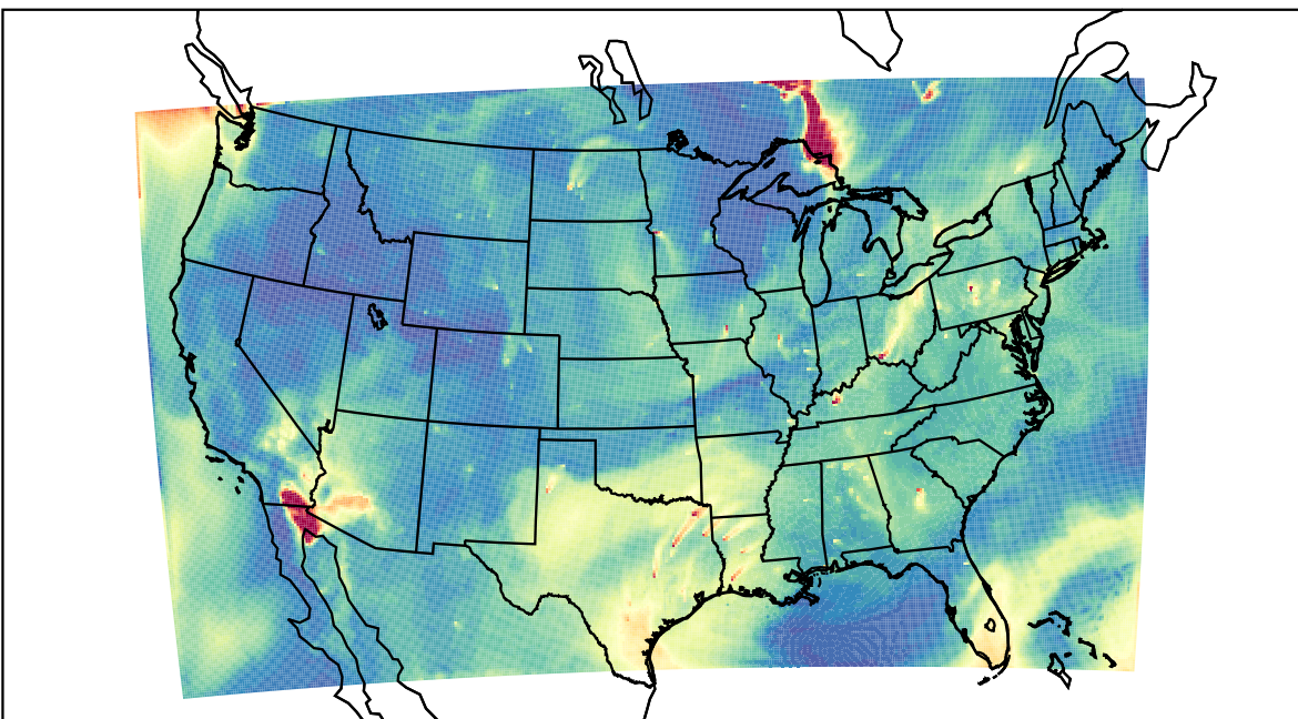
WRF 2023-07-06_14:00:00
