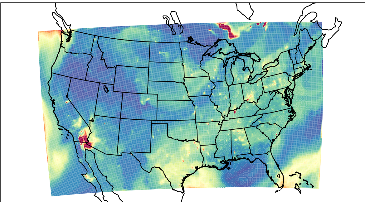
WRF 2023-07-06_02:00:00
