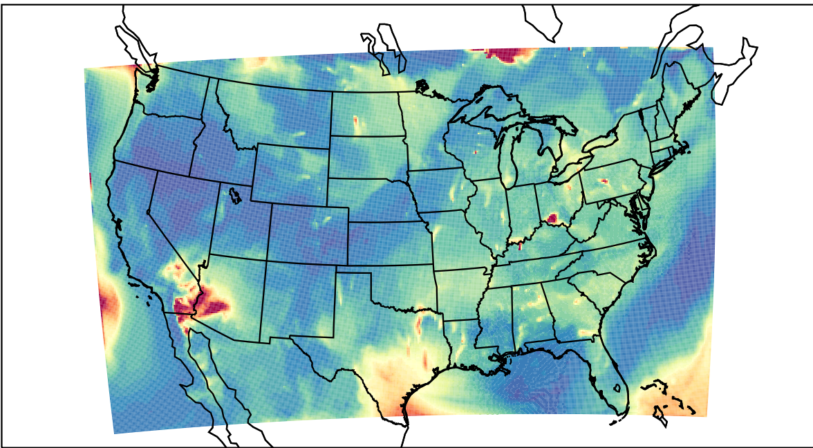
WRF 2023-07-05_08:00:00
