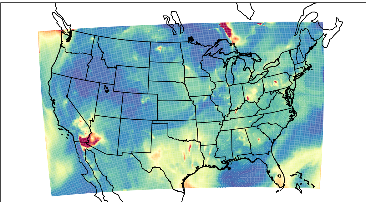
WRF 2023-07-06_08:00:00
