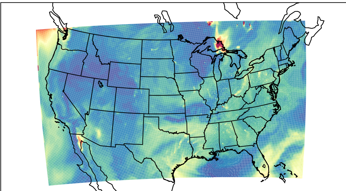
WRF 2023-07-06_19:00:00
