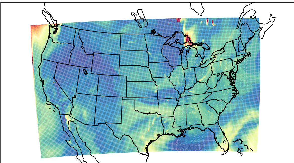
WRF 2023-07-06_21:00:00
