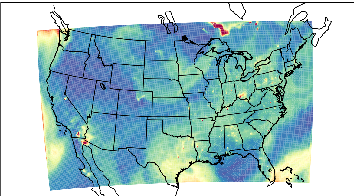
WRF 2023-07-06_00:00:00
