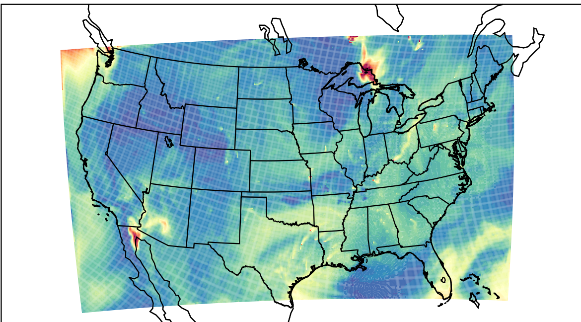
WRF 2023-07-06_17:00:00
