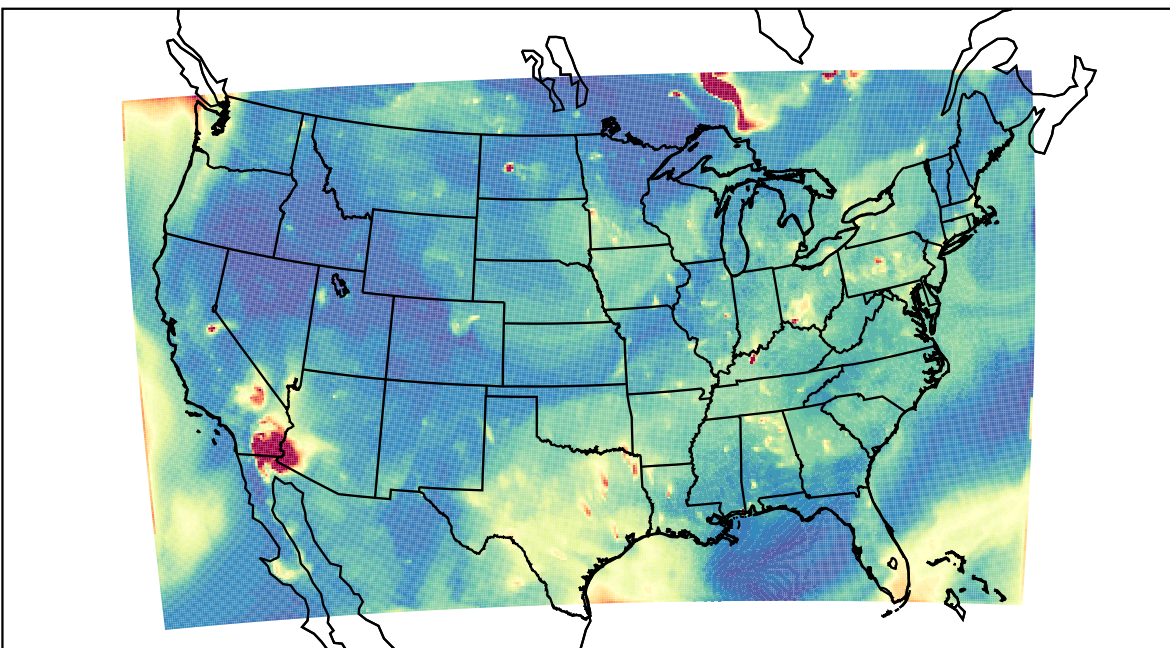
WRF 2023-07-06_04:00:00
