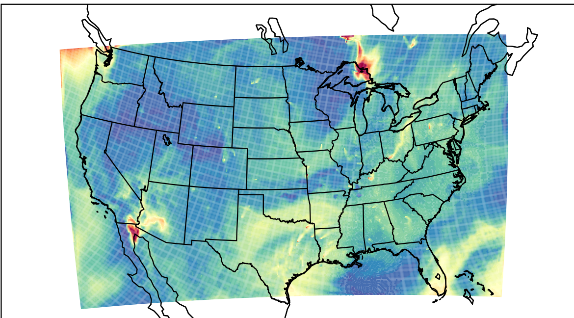
WRF 2023-07-06_16:00:00
