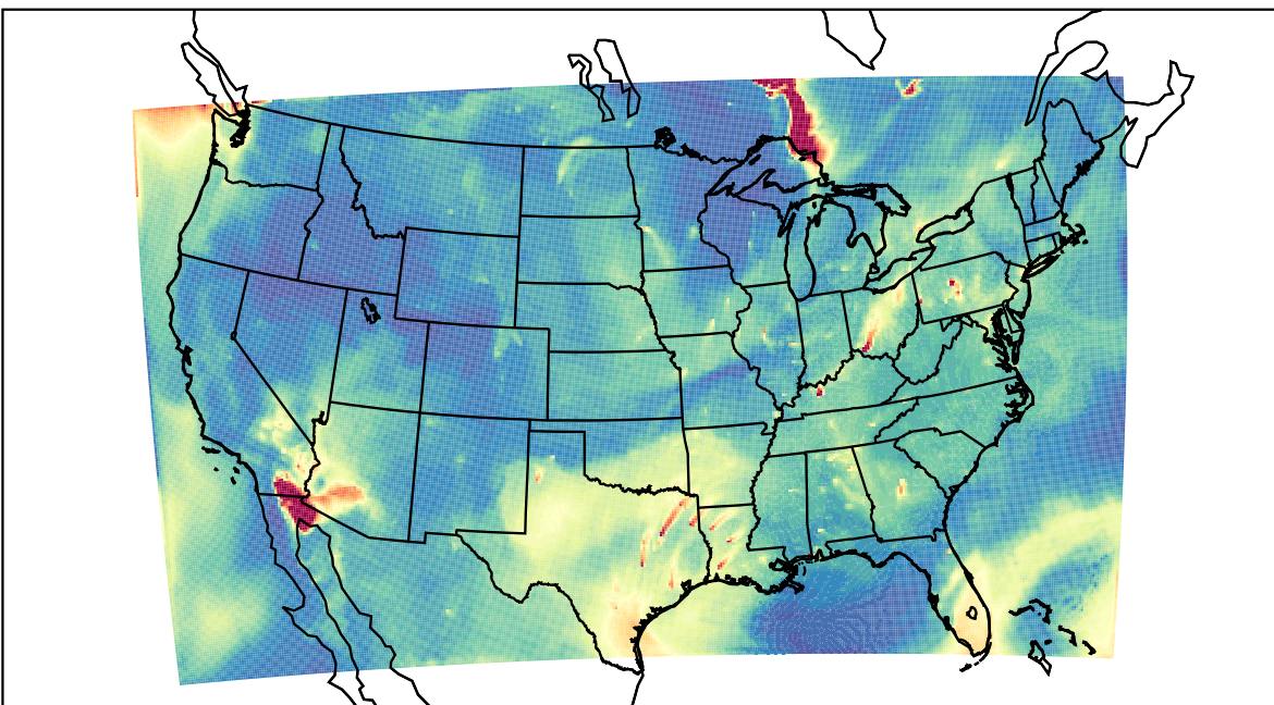
WRF 2023-07-06_13:00:00
