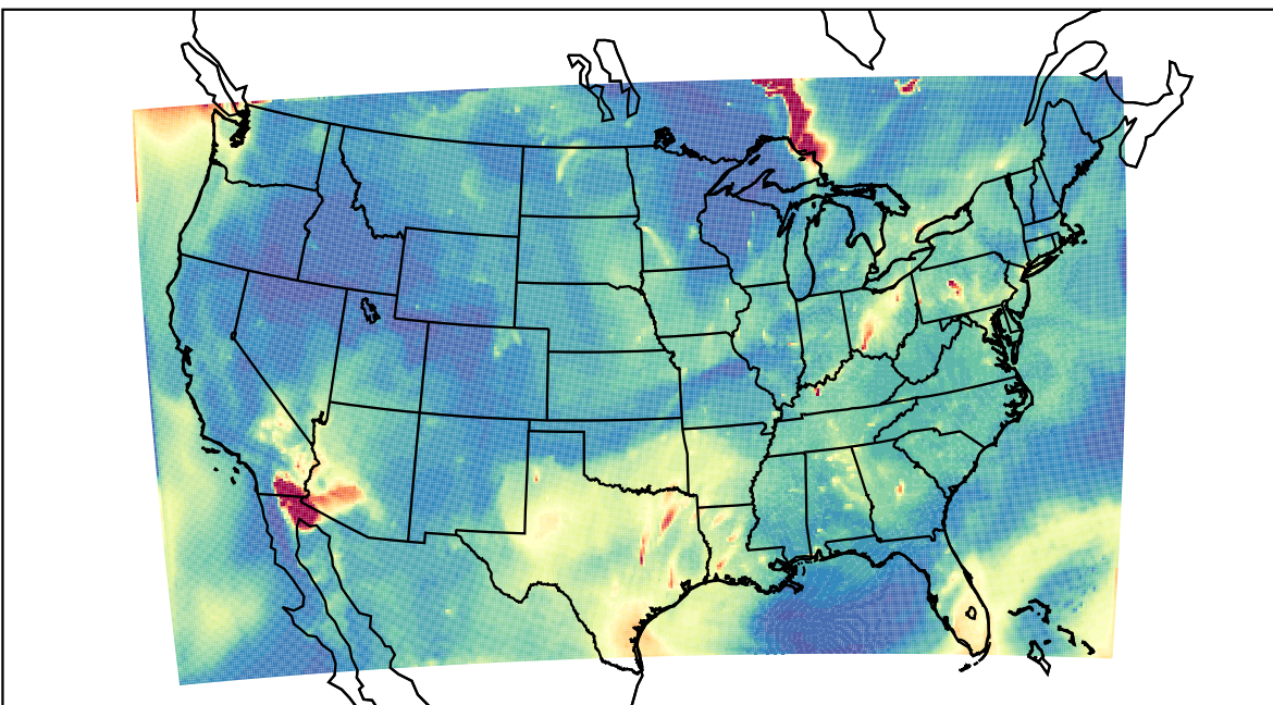
WRF 2023-07-06_12:00:00
