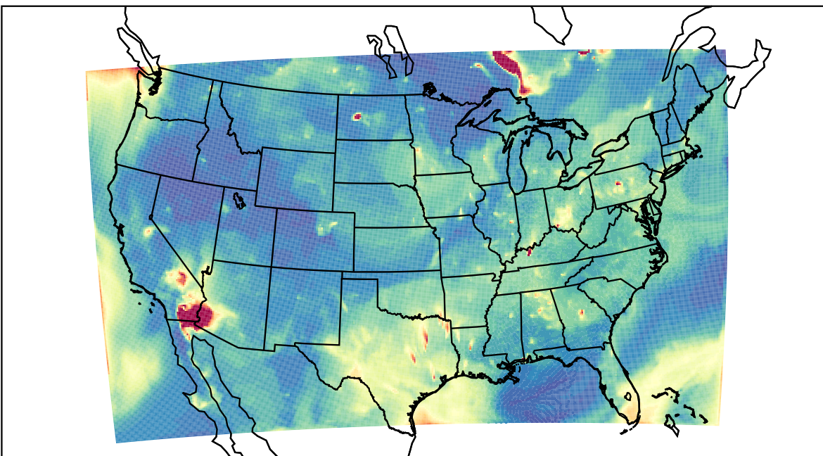
WRF 2023-07-06_05:00:00
