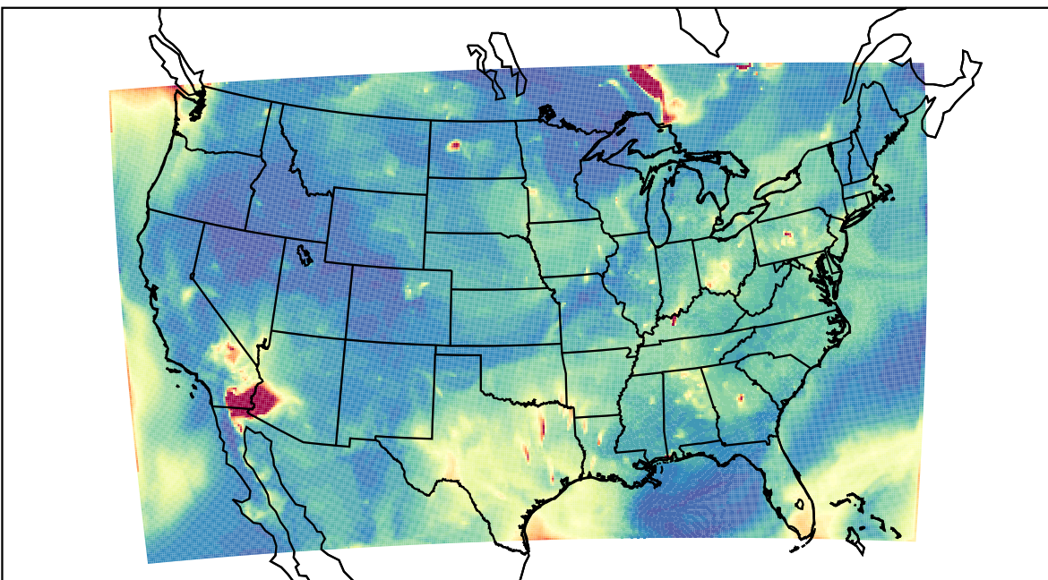
WRF 2023-07-06_06:00:00
