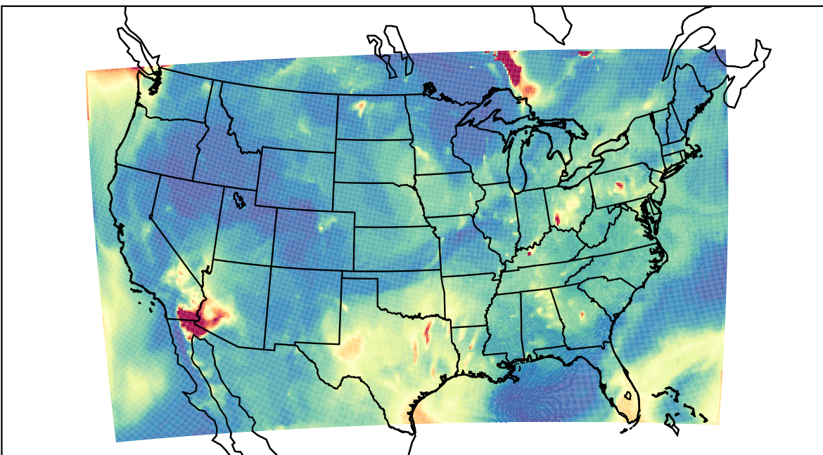
WRF 2023-07-06_09:00:00
