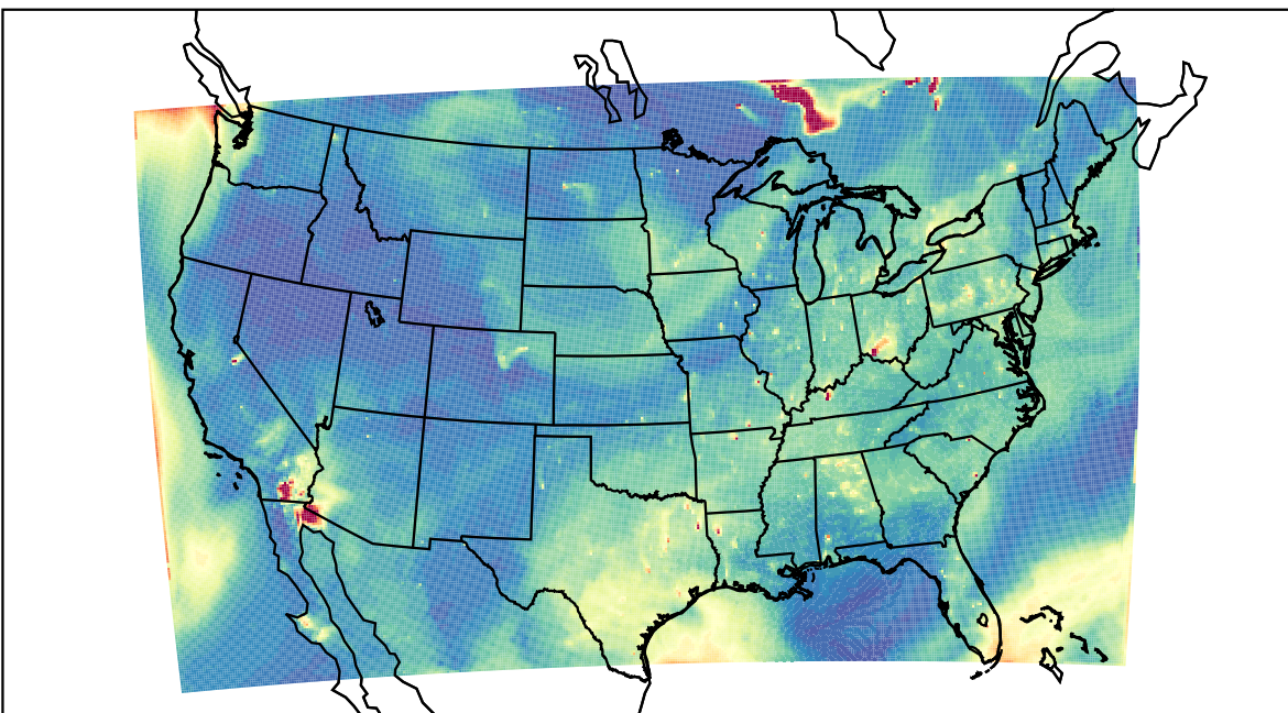
WRF 2023-07-06_01:00:00
