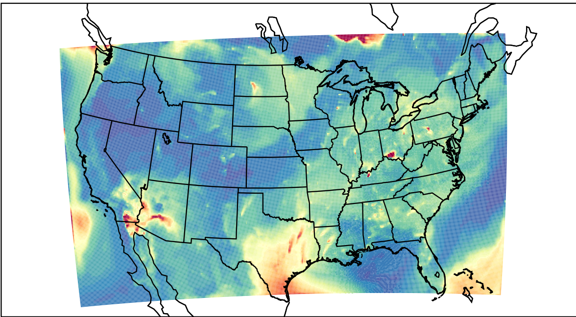
WRF 2023-07-05_12:00:00
