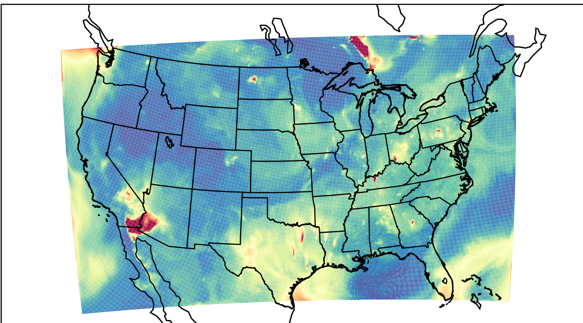
WRF 2023-07-06_07:00:00
