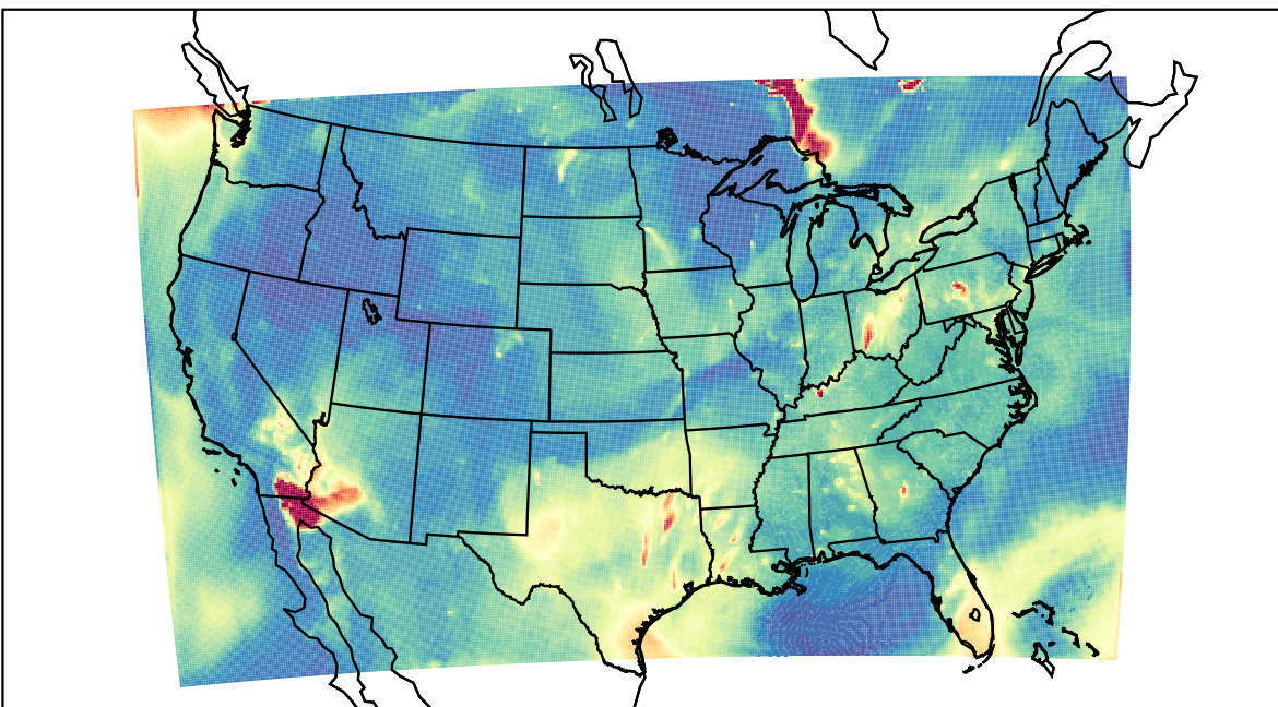
WRF 2023-07-06_11:00:00
