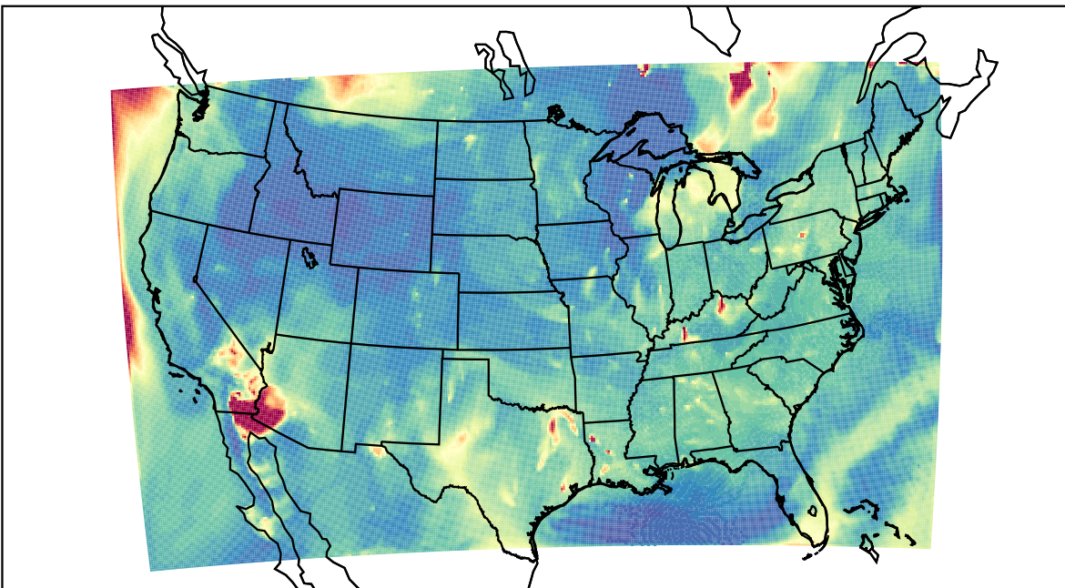
WRF 2023-07-07_08:00:00
