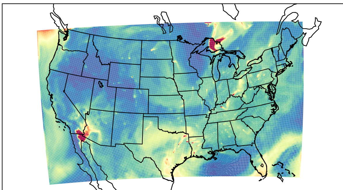
WRF 2023-07-06_15:00:00
