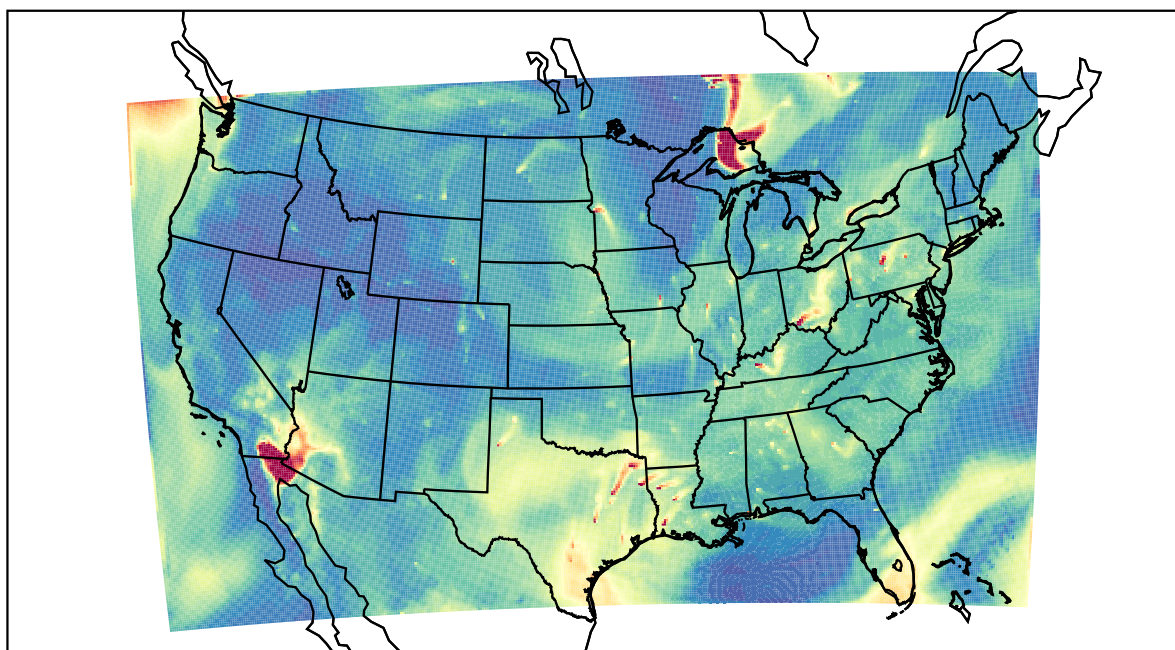
WRF 2023-07-06_14:00:00
