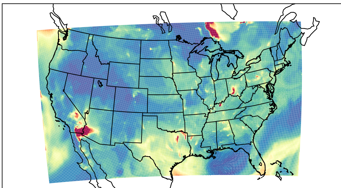
WRF 2023-07-06_06:00:00
