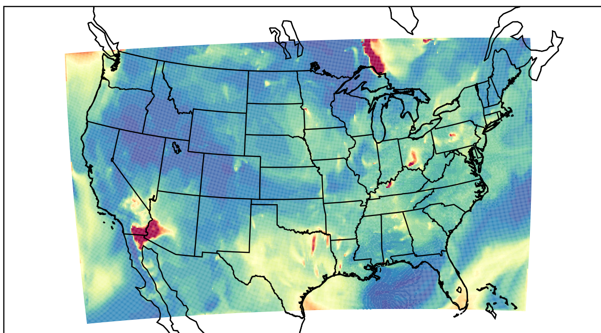
WRF 2023-07-06_08:00:00
