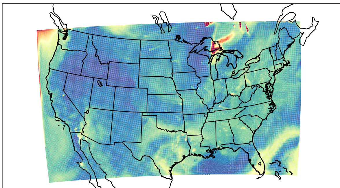
WRF 2023-07-06_22:00:00
