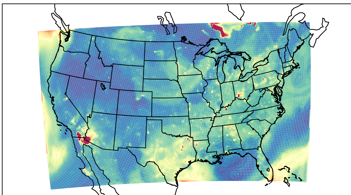
WRF 2023-07-06_02:00:00
