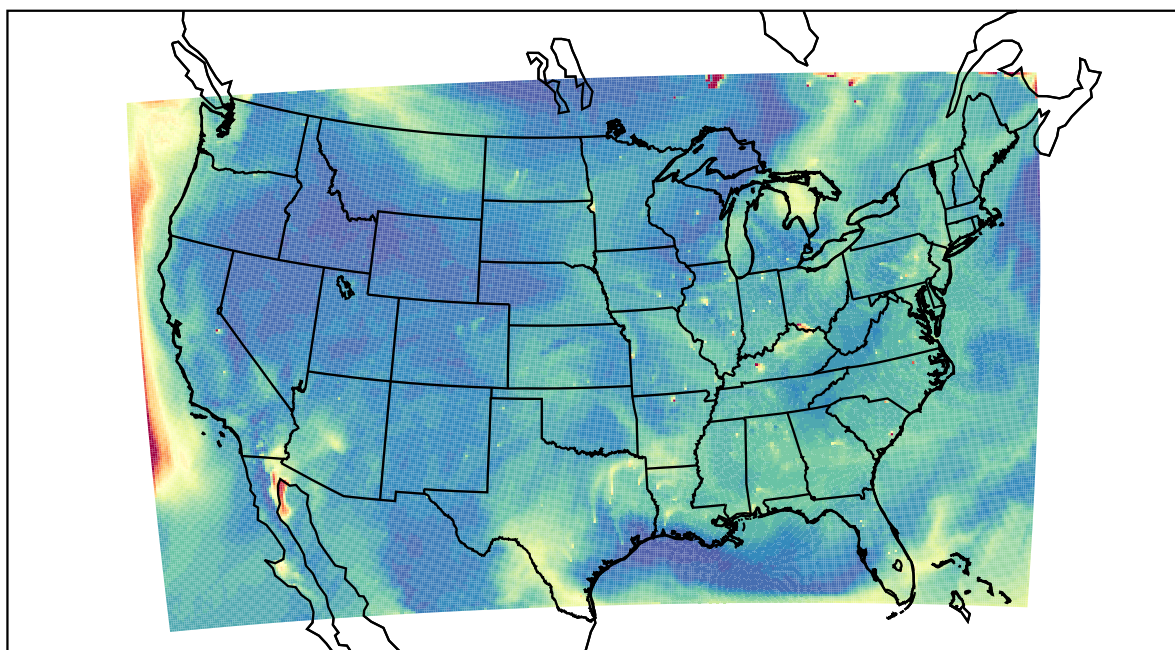
WRF 2023-07-07_21:00:00
