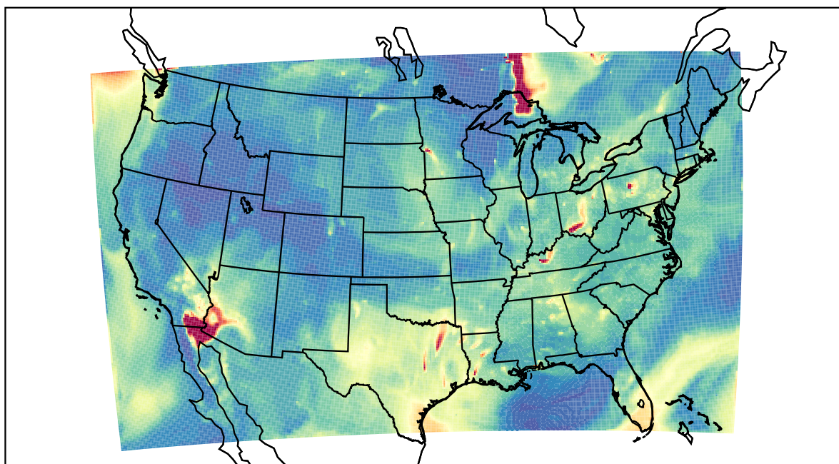
WRF 2023-07-06_11:00:00
