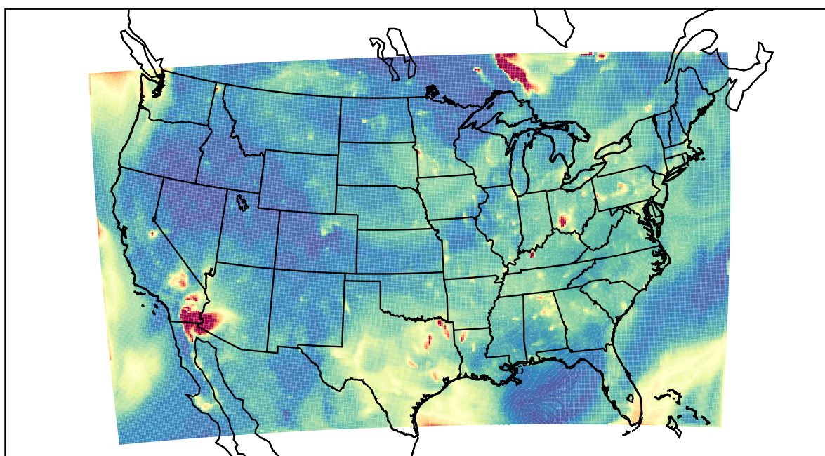
WRF 2023-07-06_04:00:00
