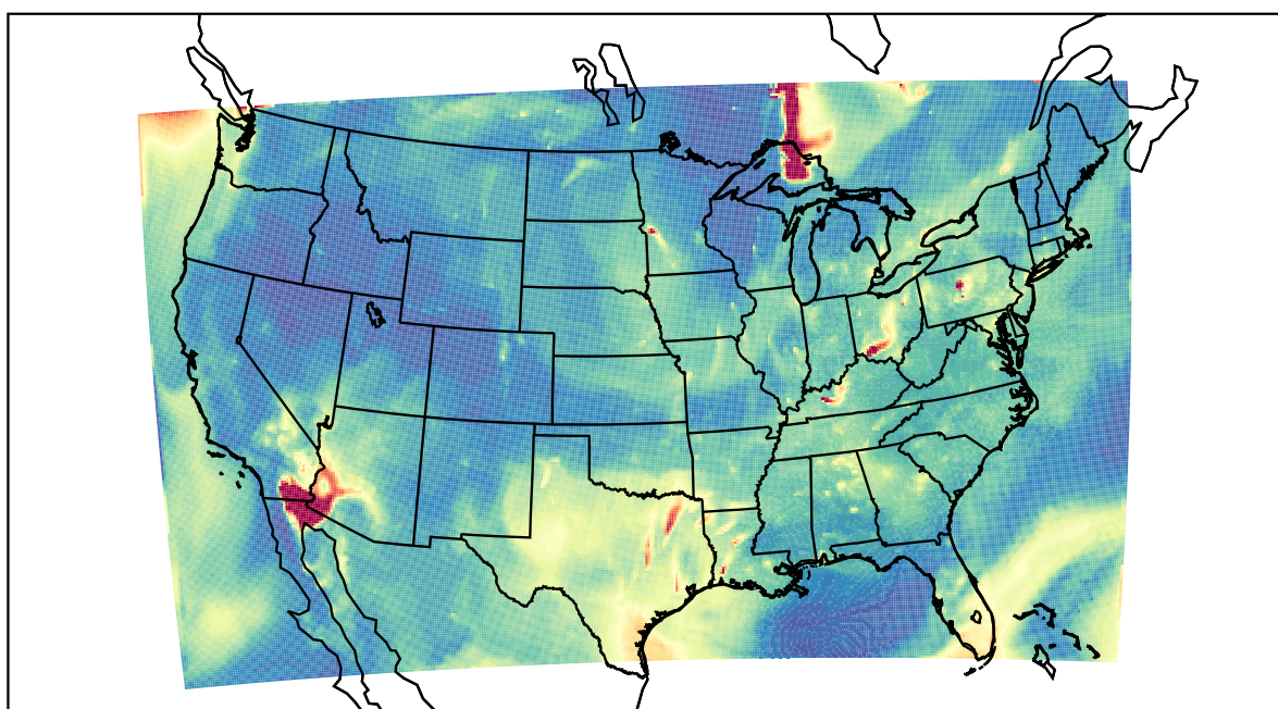
WRF 2023-07-06_12:00:00
