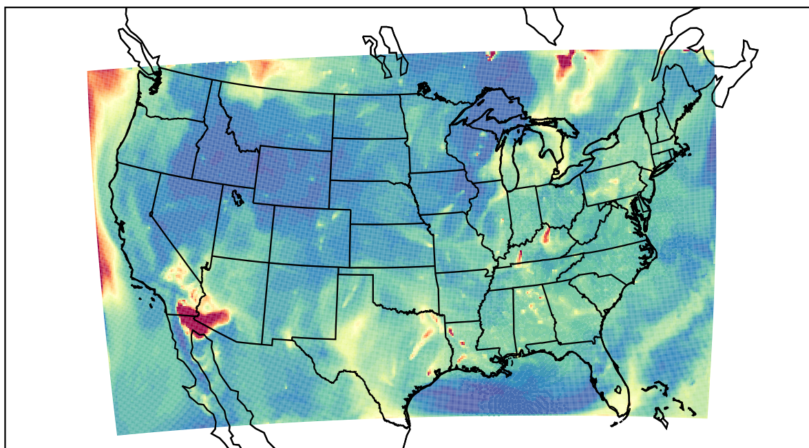
WRF 2023-07-07_11:00:00
