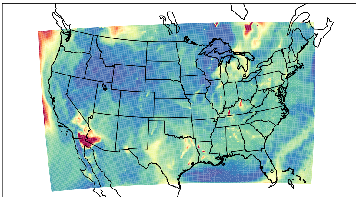
WRF 2023-07-07_10:00:00
