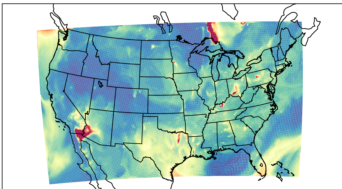
WRF 2023-07-06_09:00:00
