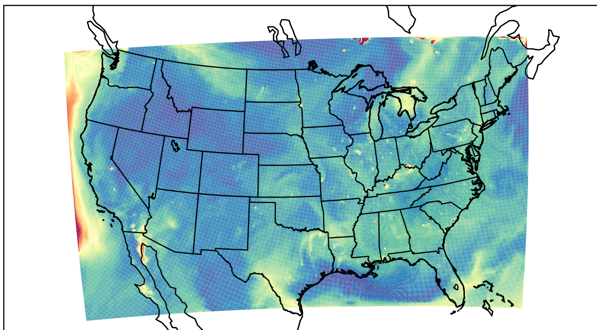
WRF 2023-07-07_22:00:00
