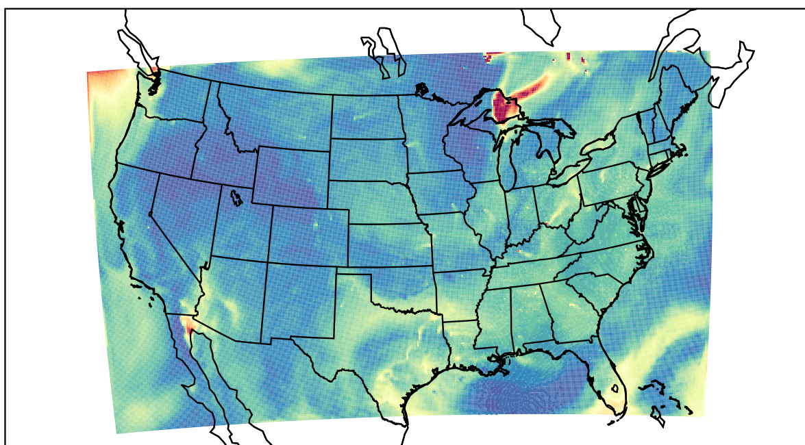
WRF 2023-07-06_19:00:00
