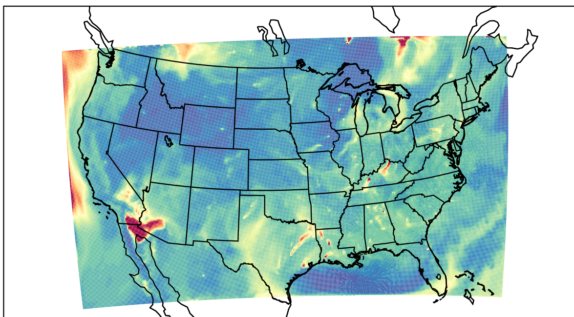
WRF 2023-07-07_13:00:00
