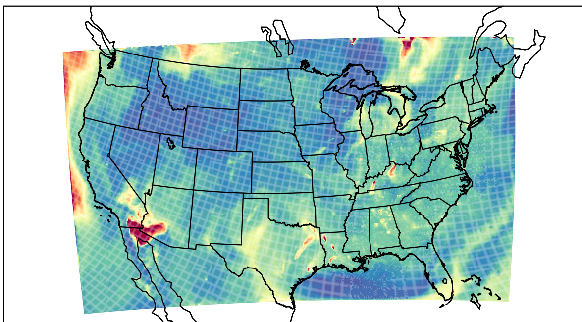
WRF 2023-07-07_12:00:00
