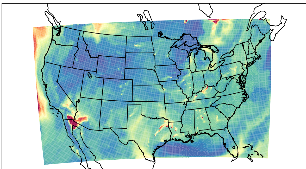
WRF 2023-07-07_14:00:00
