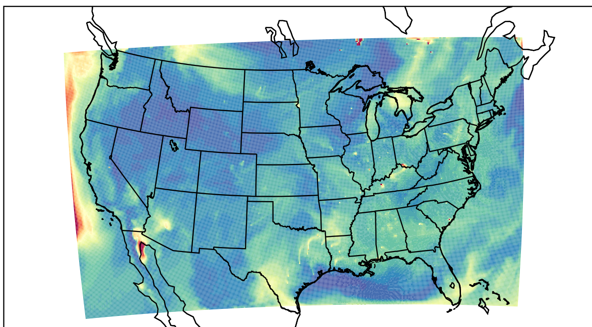
WRF 2023-07-07_19:00:00
