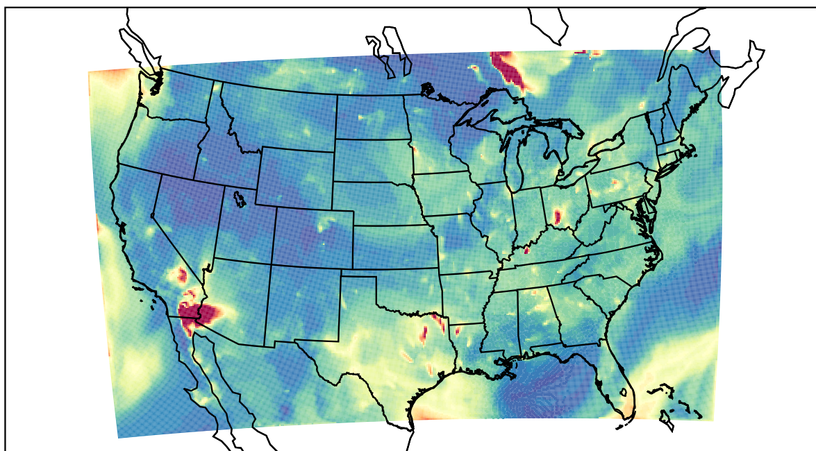
WRF 2023-07-06_05:00:00
