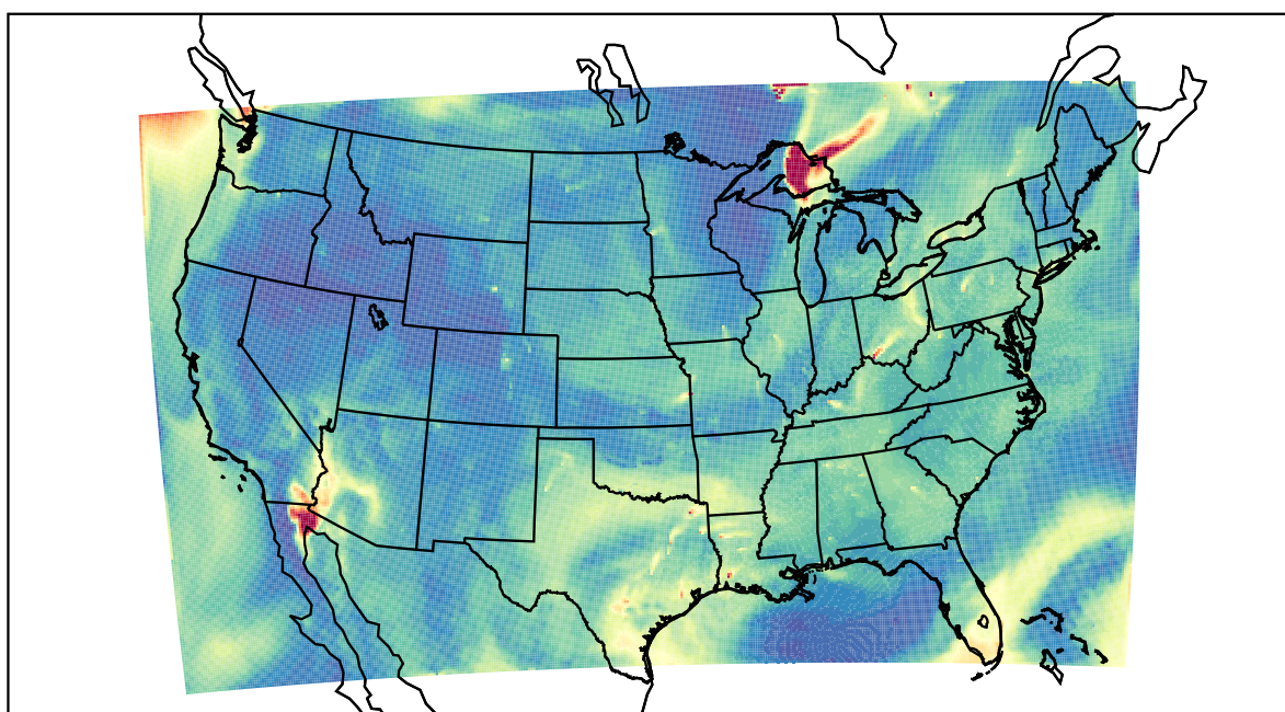
WRF 2023-07-06_17:00:00
