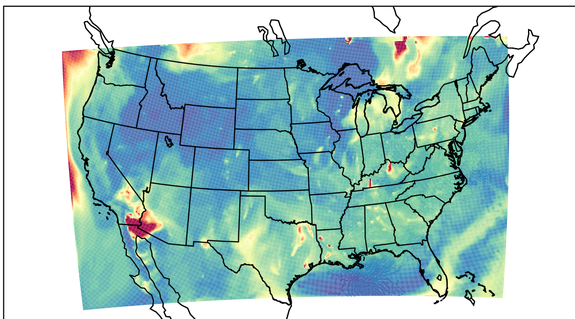
WRF 2023-07-07_09:00:00
