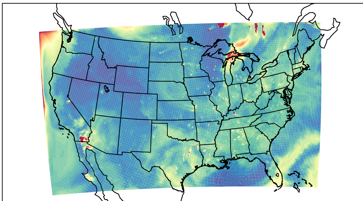
WRF 2023-07-07_01:00:00
