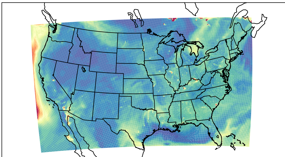
WRF 2023-07-07_23:00:00
