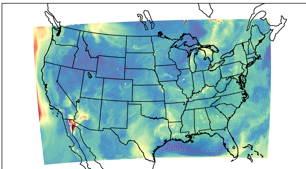
WRF 2023-07-07_17:00:00
