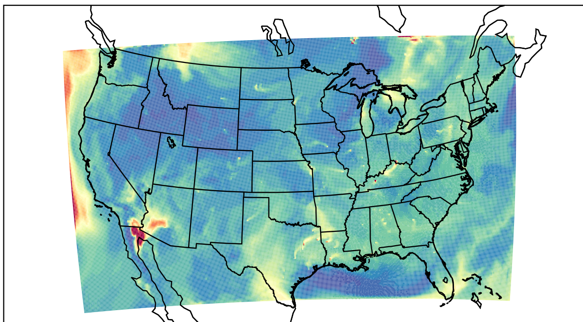
WRF 2023-07-07_16:00:00
