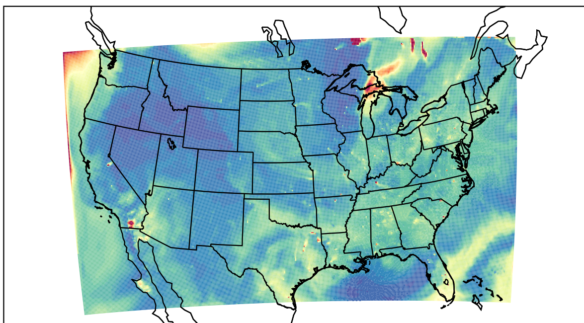
WRF 2023-07-07_00:00:00
