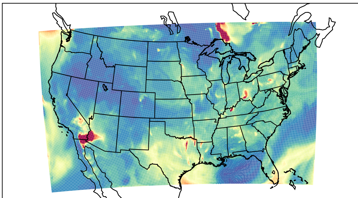
WRF 2023-07-06_07:00:00
