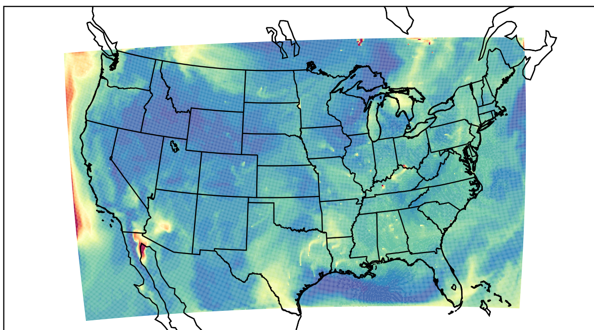
WRF 2023-07-07_18:00:00
