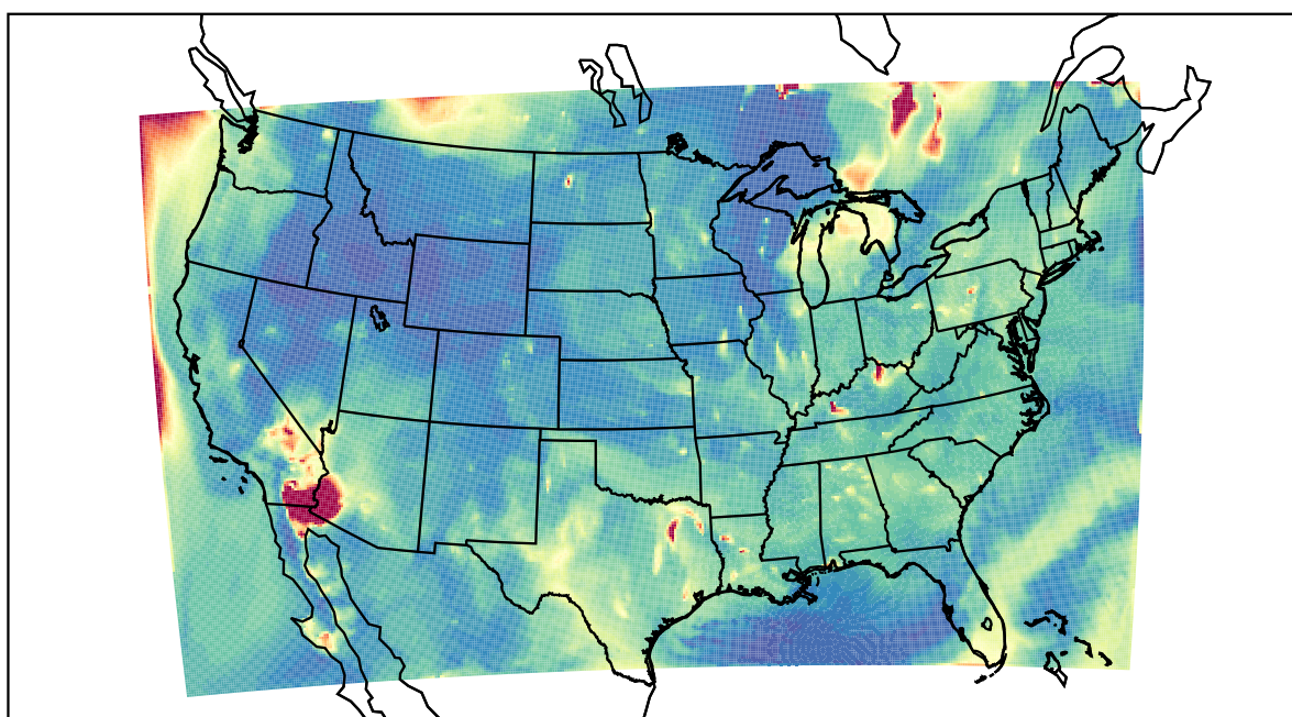
WRF 2023-07-07_06:00:00
