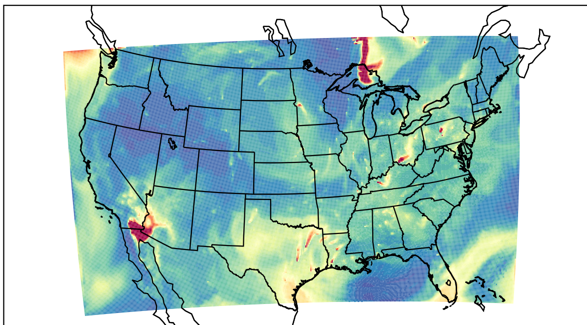
WRF 2023-07-06_13:00:00
