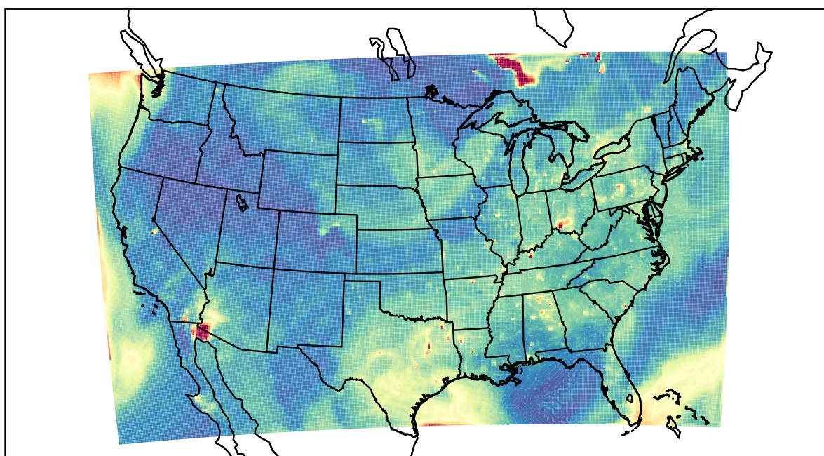
WRF 2023-07-06_01:00:00
