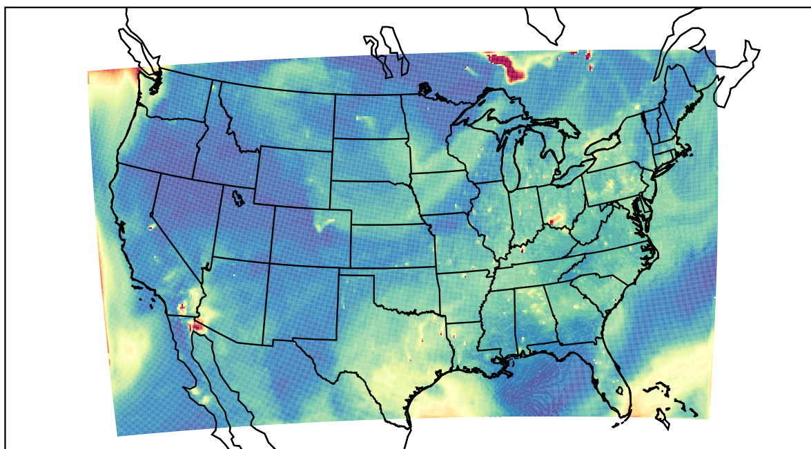
WRF 2023-07-06_00:00:00
