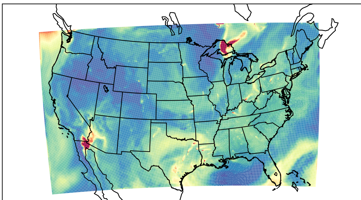
WRF 2023-07-06_16:00:00
