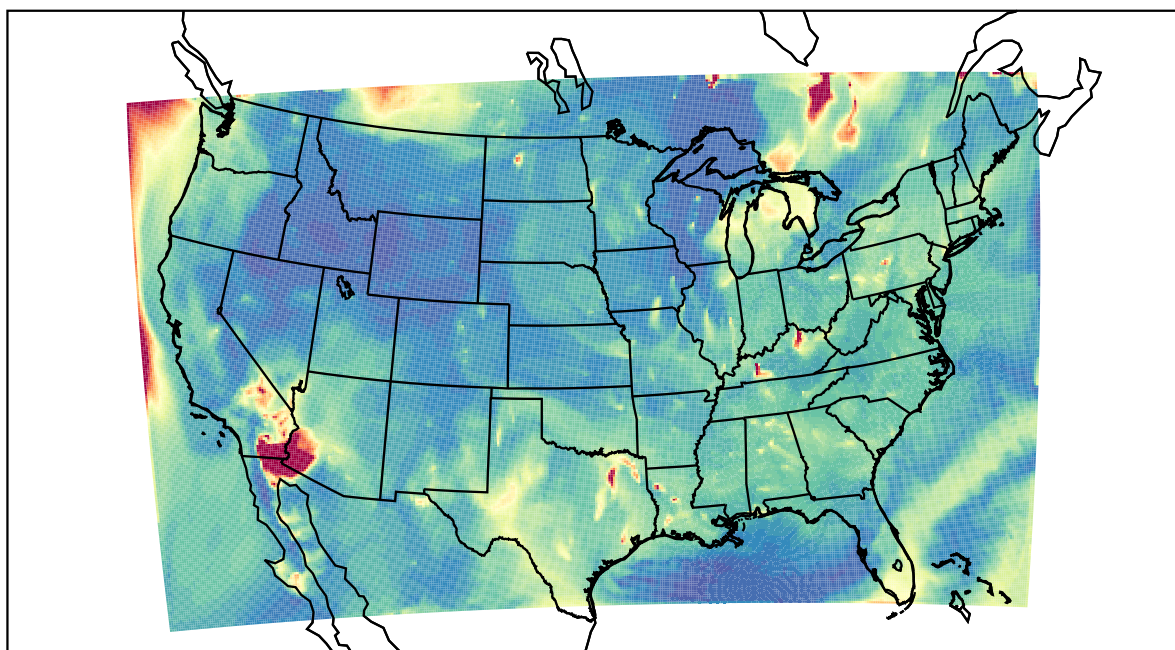
WRF 2023-07-07_07:00:00
