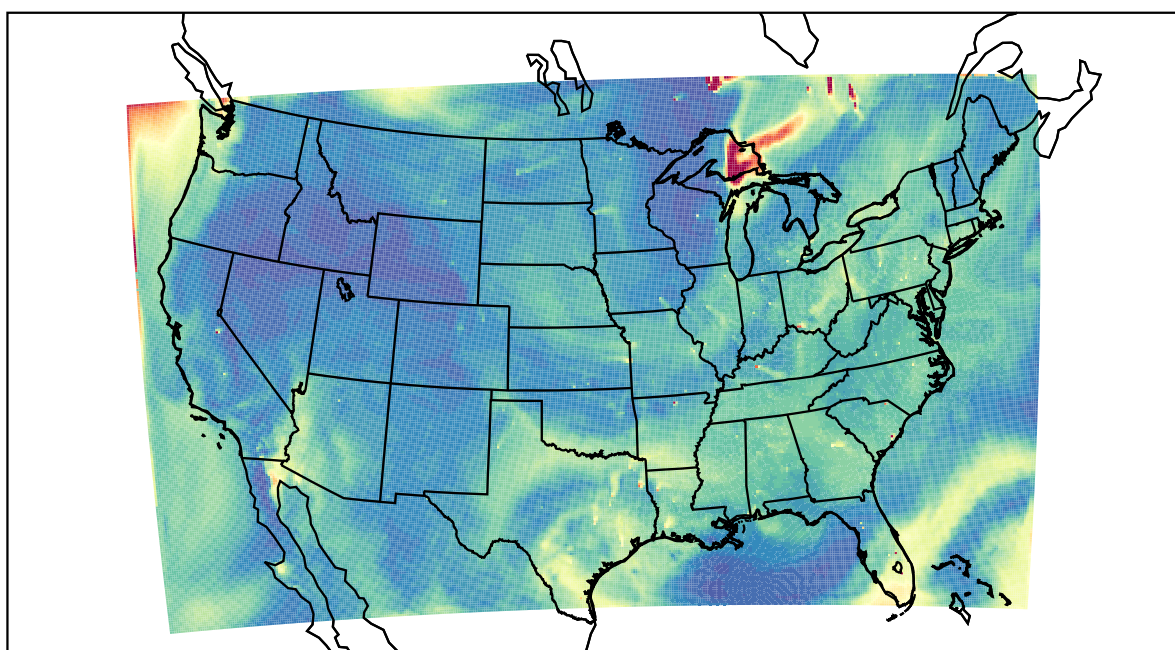
WRF 2023-07-06_21:00:00
