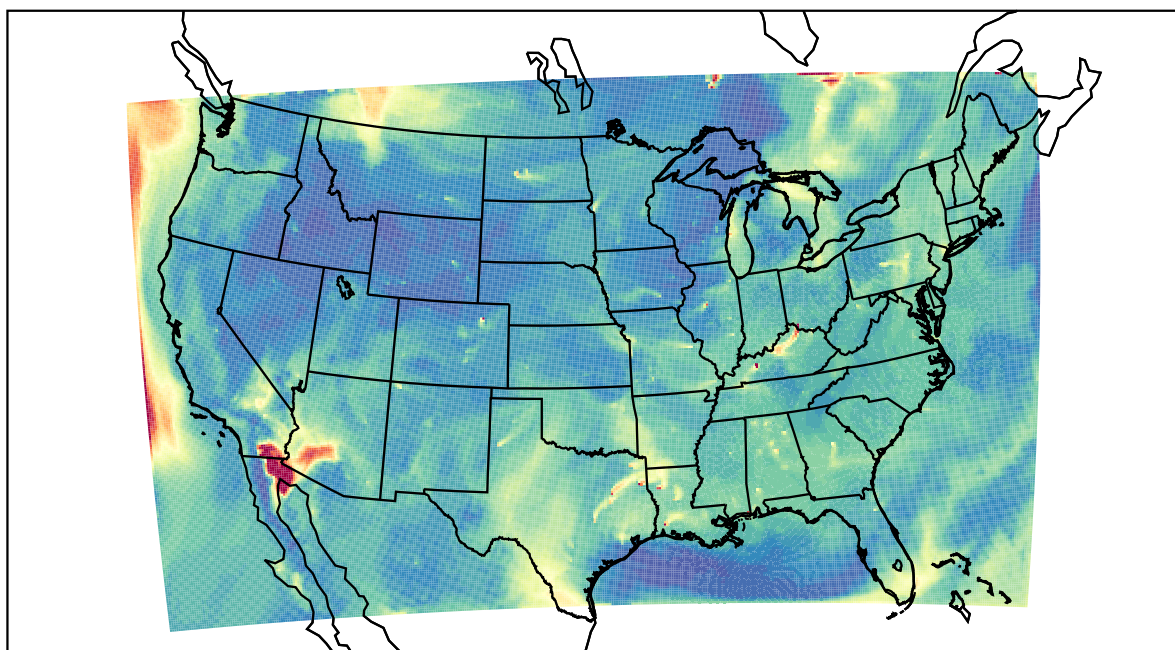
WRF 2023-07-07_15:00:00
