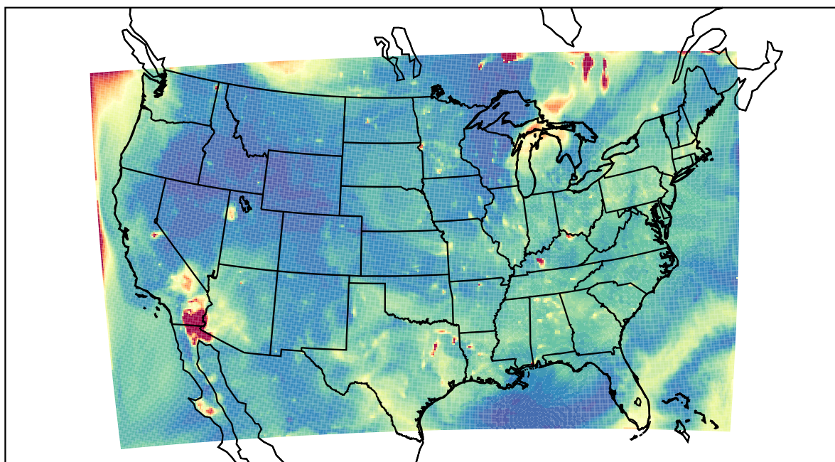
WRF 2023-07-07_03:00:00
