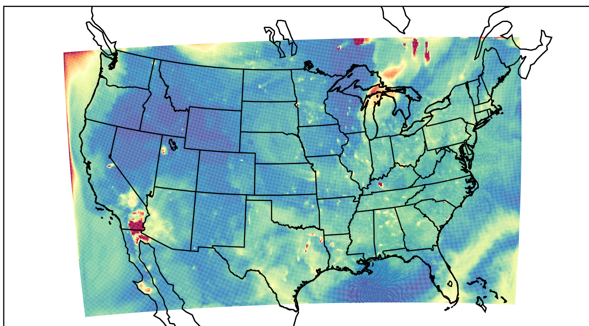
WRF 2023-07-07_02:00:00
