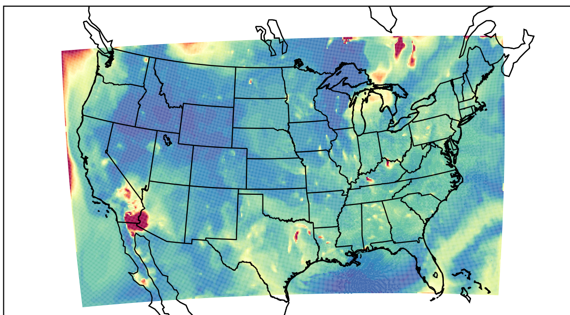
WRF 2023-07-07_05:00:00
