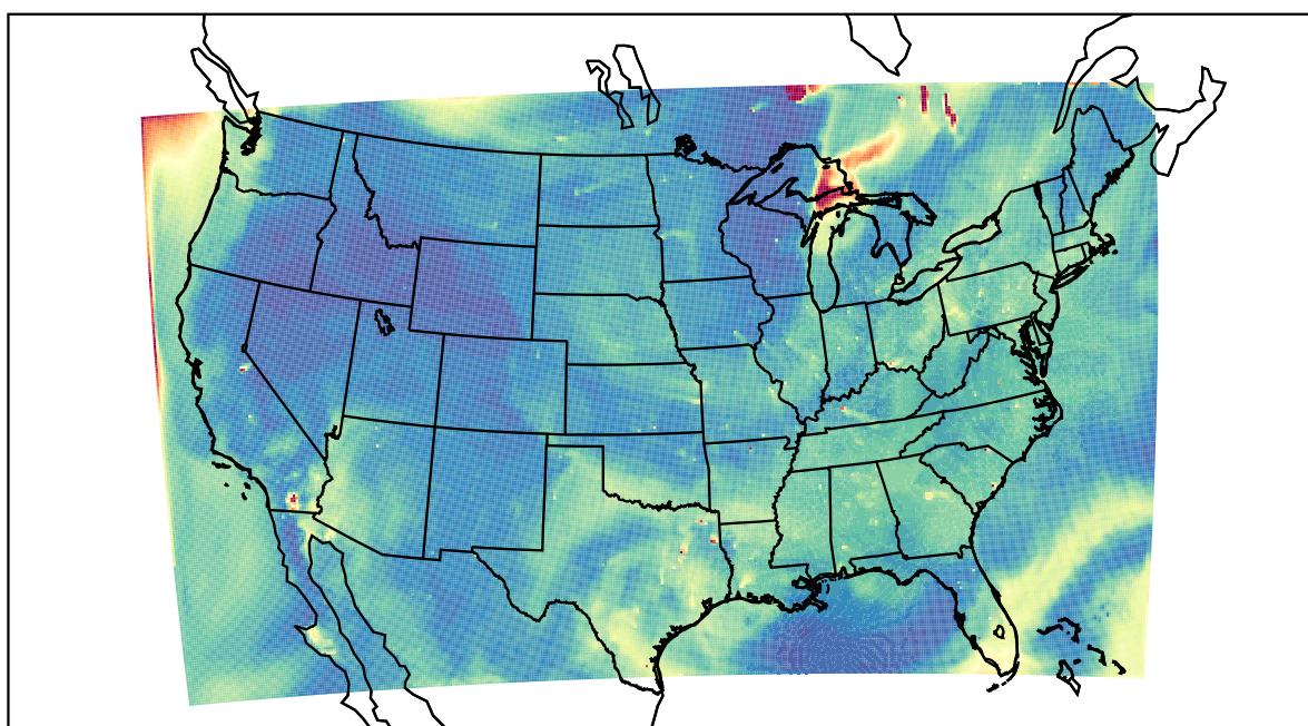
WRF 2023-07-06_23:00:00
