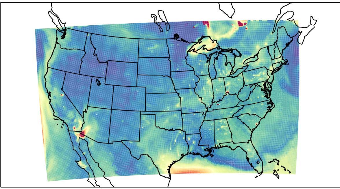
WRF 2023-07-09_01:00:00
