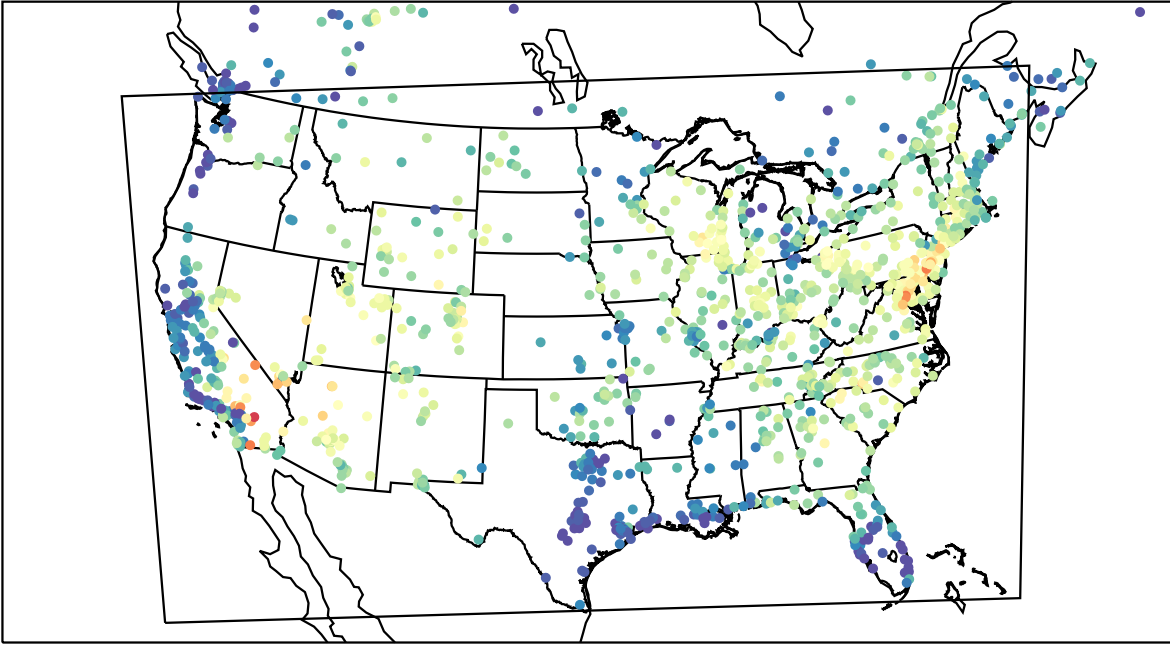
AirNOW (2023-07-08_15:00:00)
