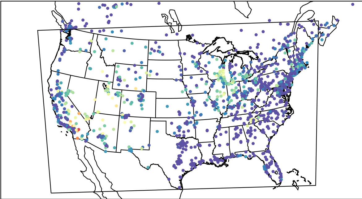
AirNOW (2023-07-08_11:00:00)
