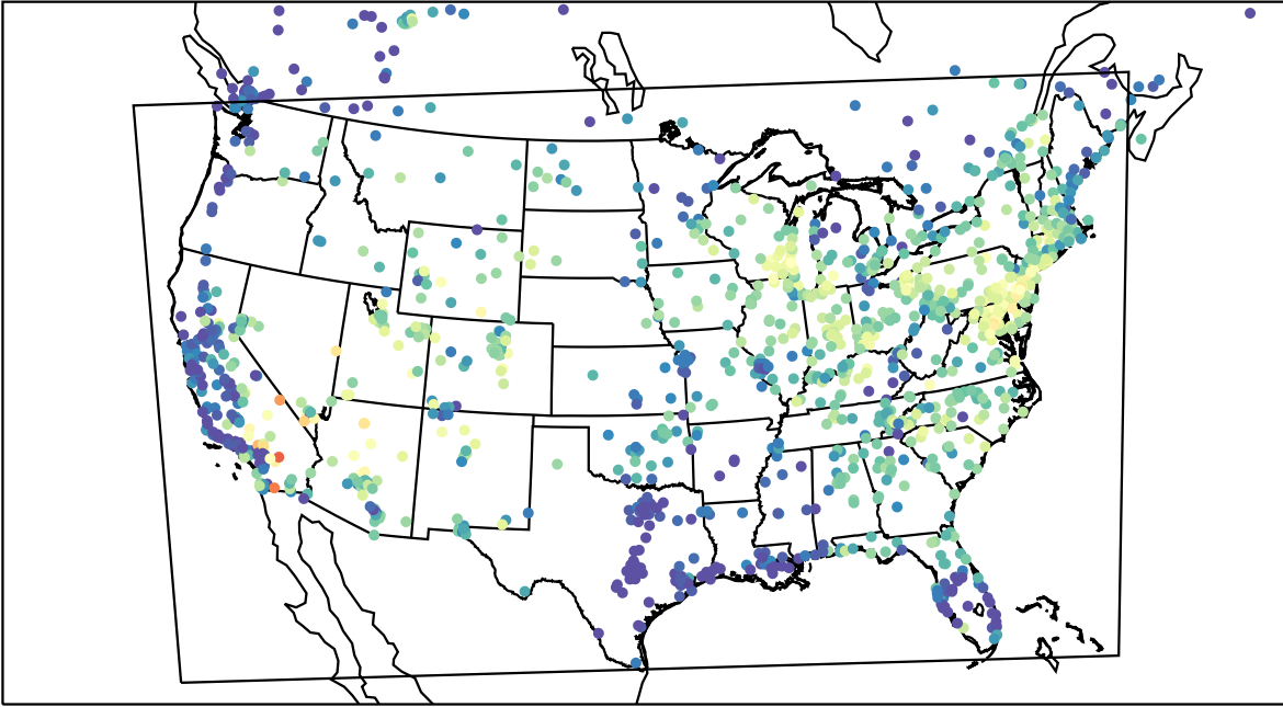
AirNOW (2023-07-08_14:00:00)
