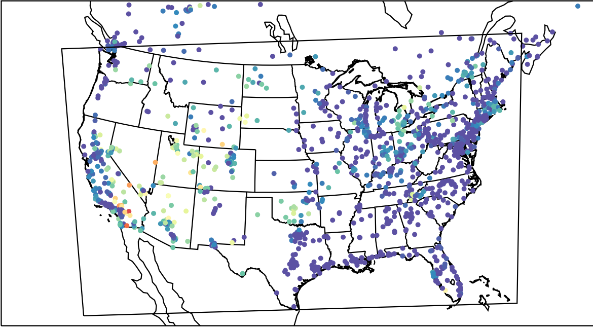
AirNOW (2023-07-09_11:00:00)
