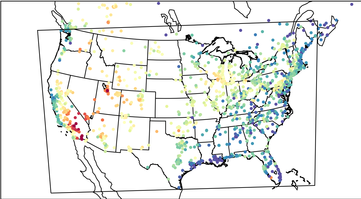
AirNOW (2023-07-09_00:00:00)
