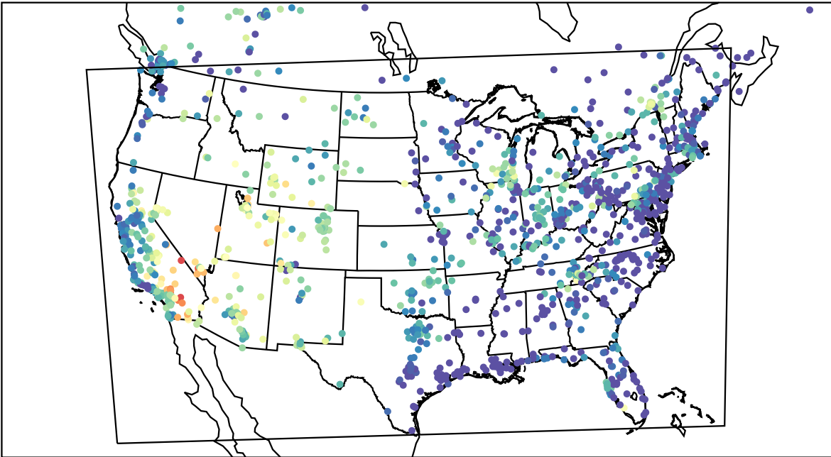
AirNOW (2023-07-09_05:00:00)
