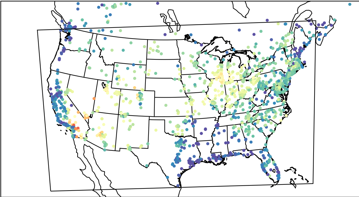
AirNOW (2023-07-09_15:00:00)
