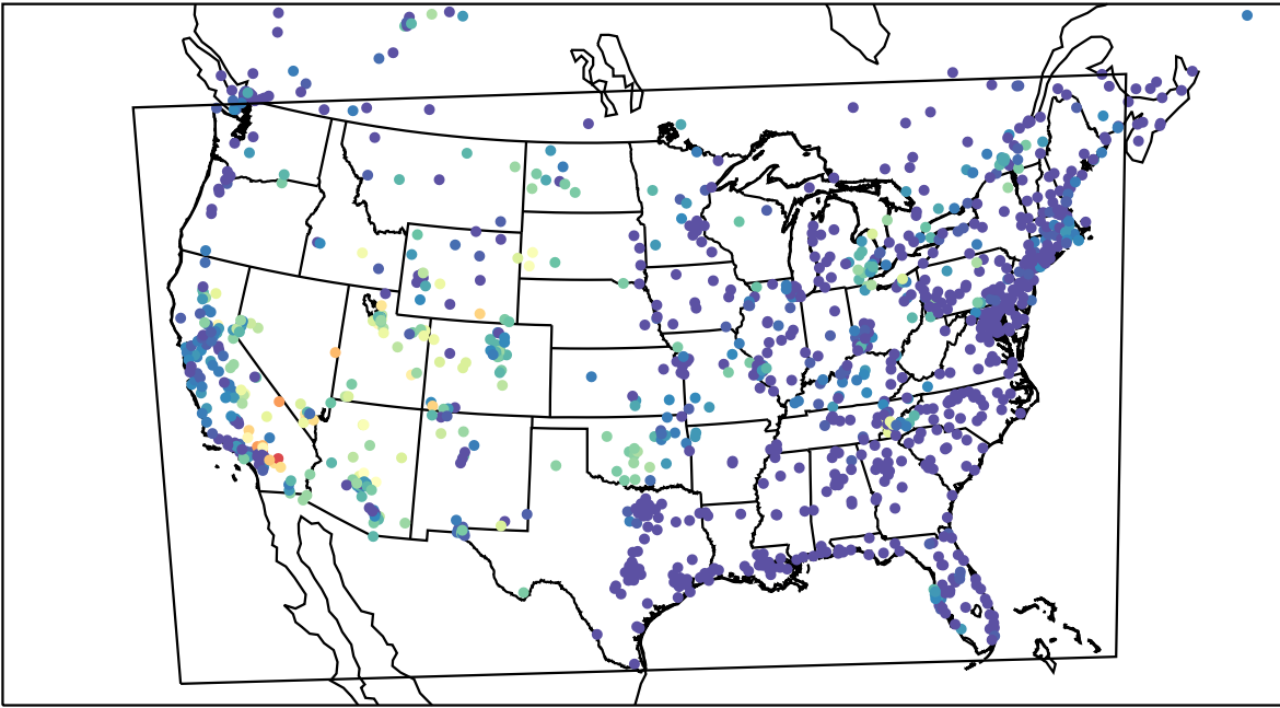
AirNOW (2023-07-09_10:00:00)
