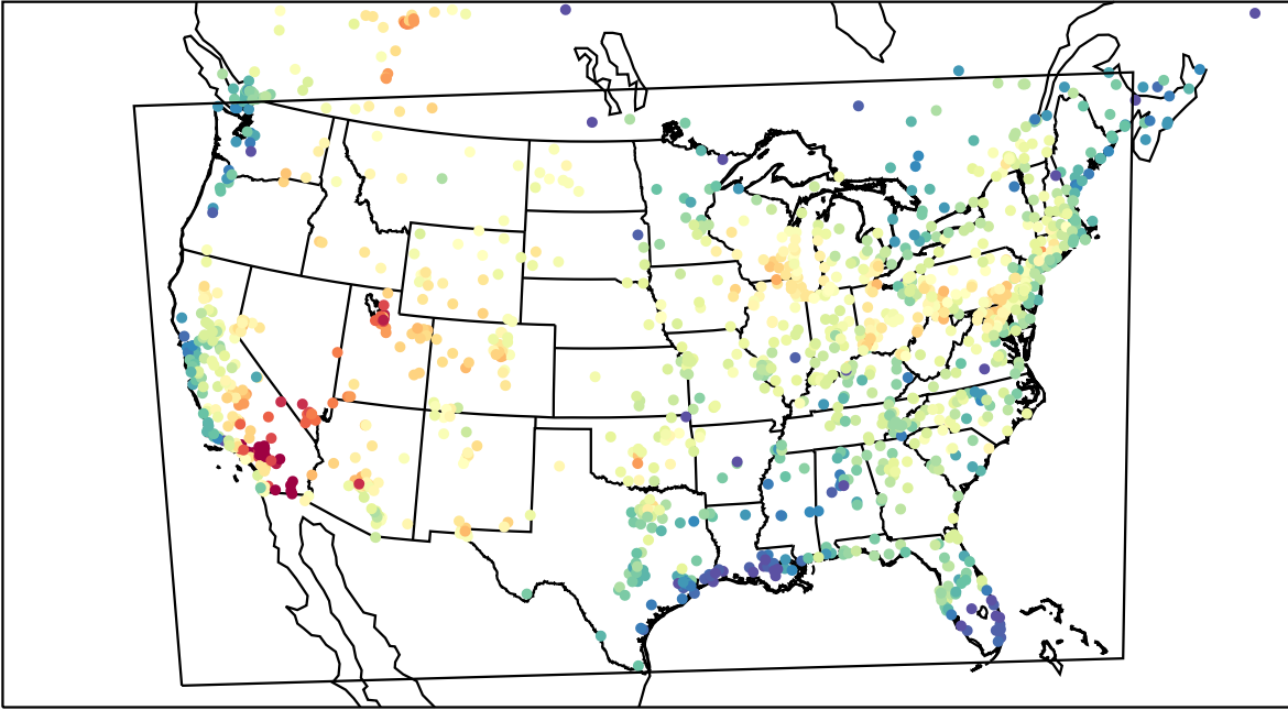
AirNOW (2023-07-08_21:00:00)
