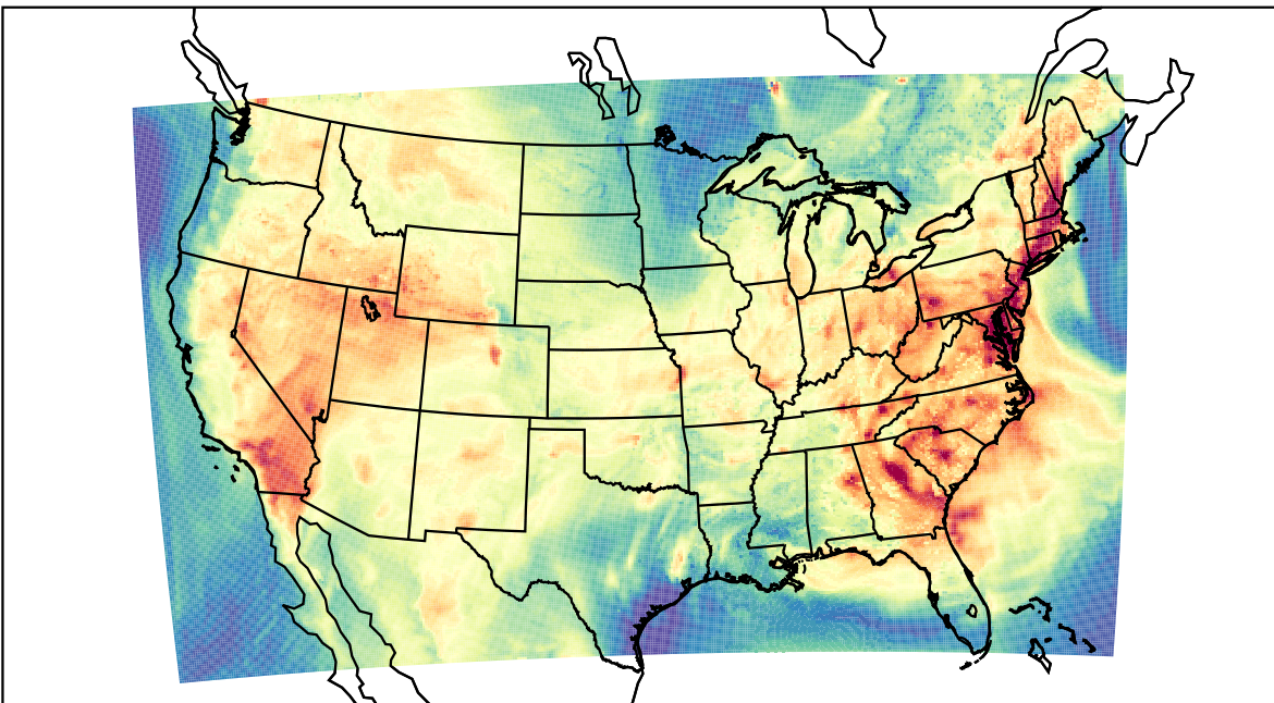
WRF (2023-07-08_21:00:00)
