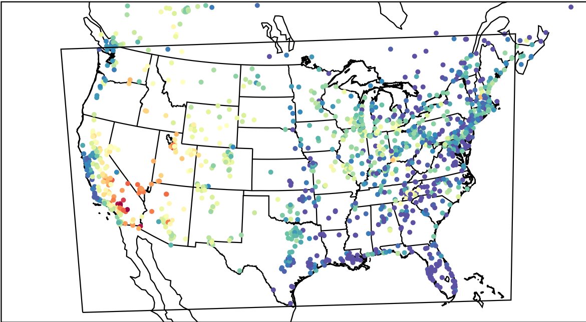
AirNOW (2023-07-08_02:00:00)
