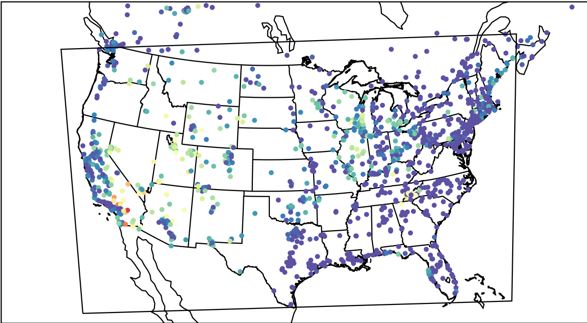
AirNOW (2023-07-08_09:00:00)
