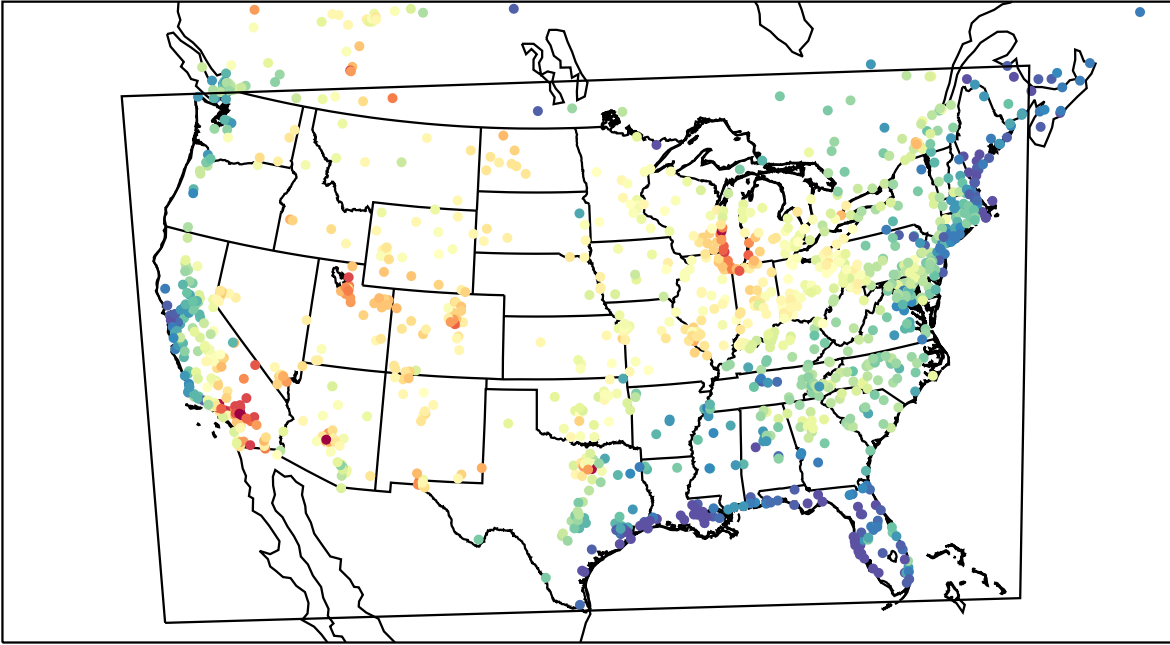
AirNOW (2023-07-09_20:00:00)
