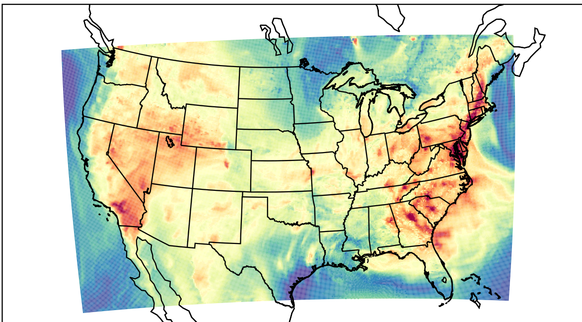
WRF (2023-07-08_22:00:00)
