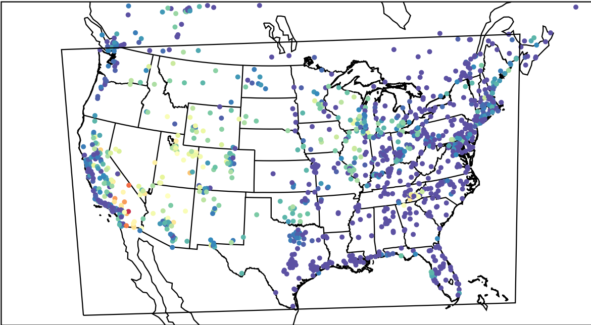
AirNOW (2023-07-08_07:00:00)
