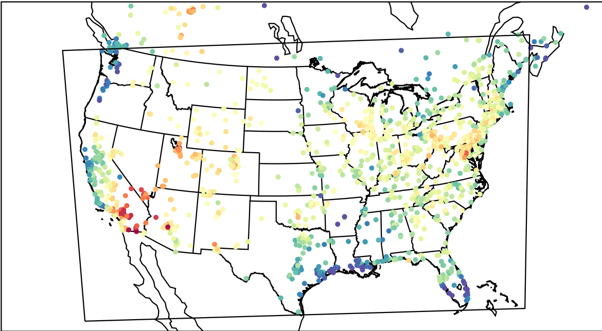
AirNOW (2023-07-08_19:00:00)
