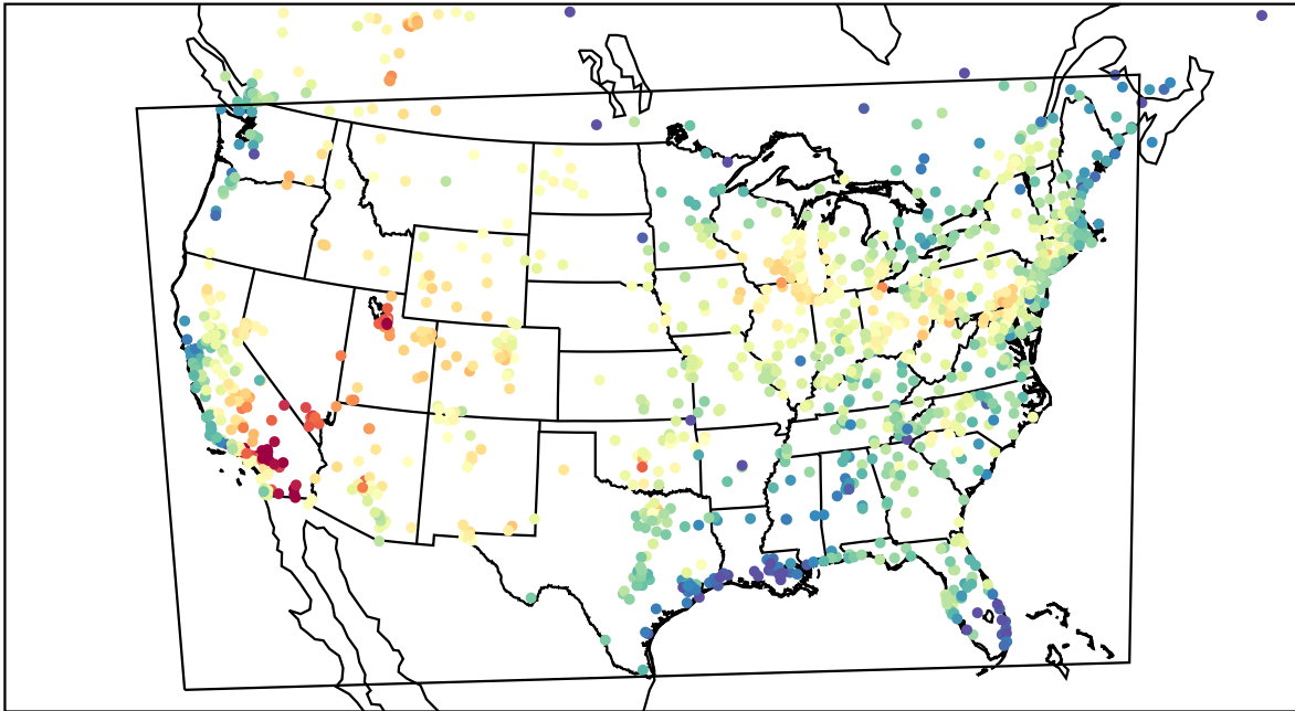
AirNOW (2023-07-08_22:00:00)
