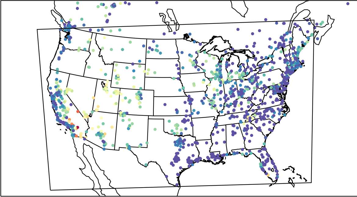
AirNOW (2023-07-08_06:00:00)
