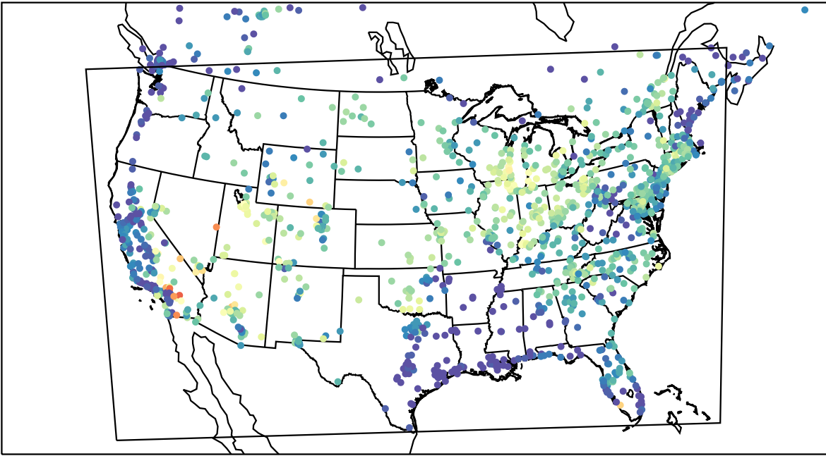
AirNOW (2023-07-09_14:00:00)
