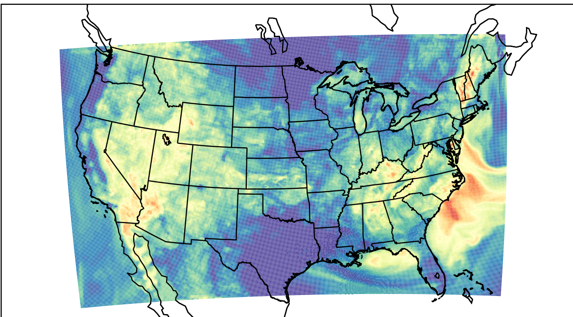
WRF (2023-07-08_09:00:00)
