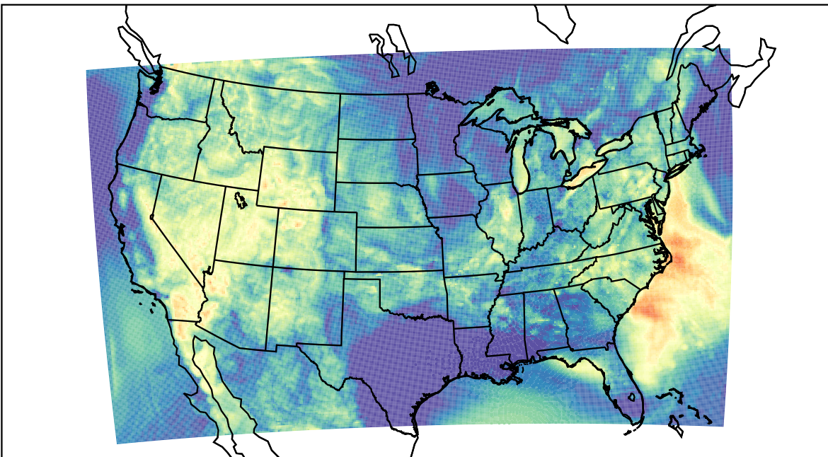
WRF (2023-07-09_11:00:00)
