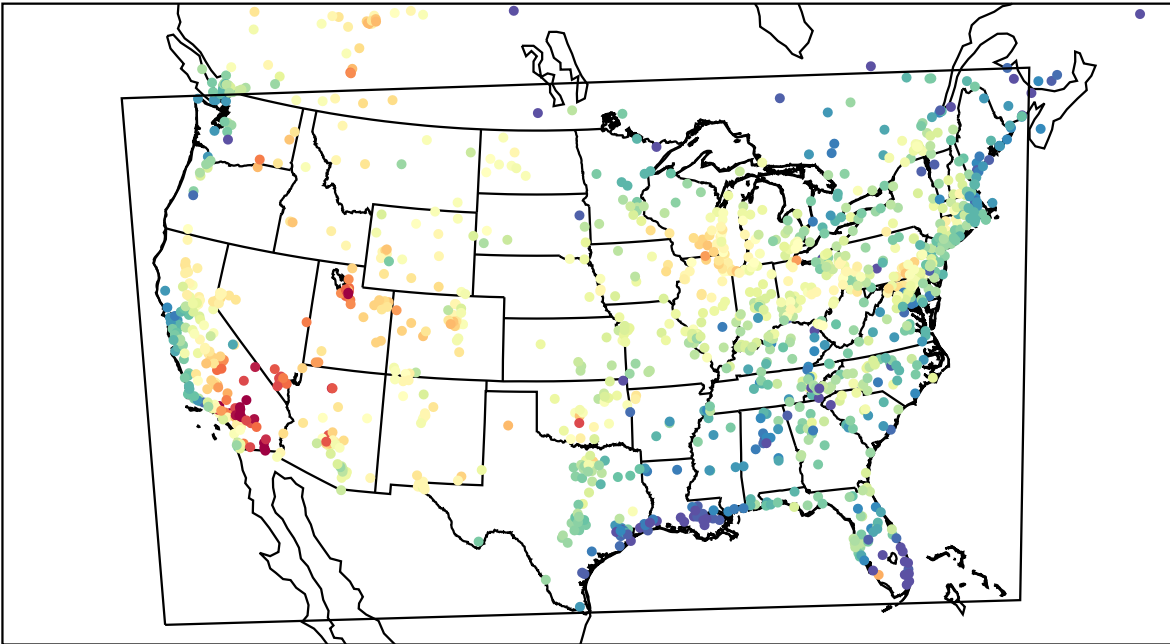
AirNOW (2023-07-08_23:00:00)
