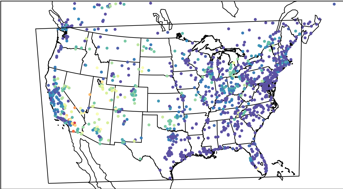
AirNOW (2023-07-09_09:00:00)
