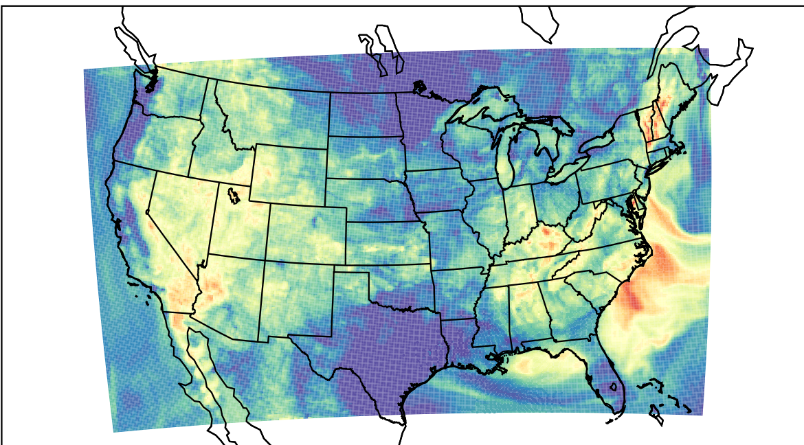
WRF (2023-07-08_08:00:00)
