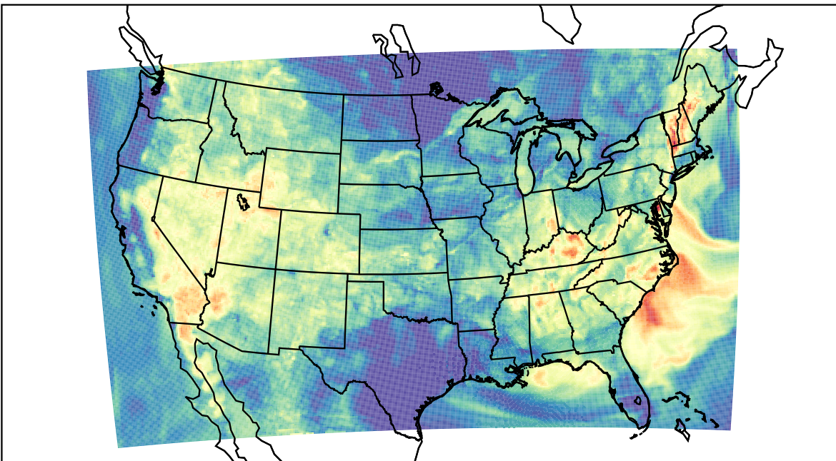
WRF (2023-07-08_06:00:00)
