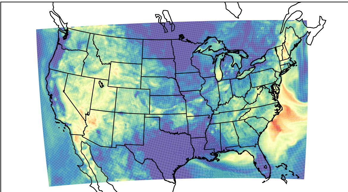
WRF (2023-07-08_12:00:00)
