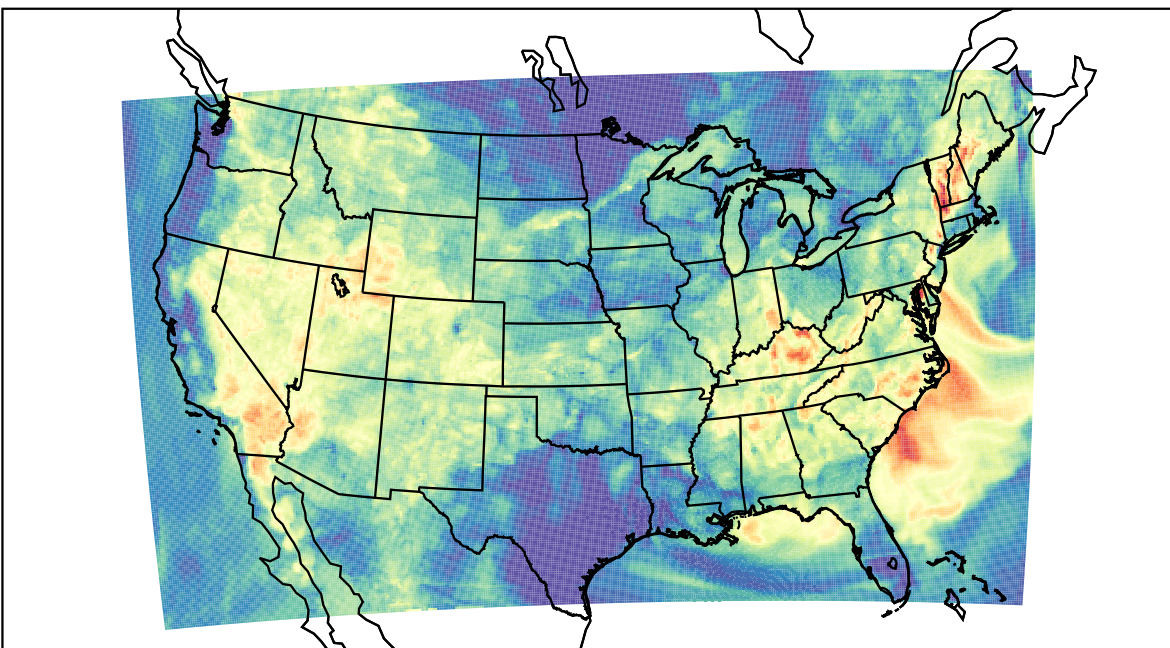
WRF (2023-07-08_05:00:00)
