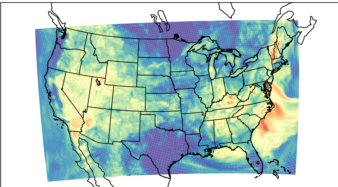
WRF (2023-07-08_07:00:00)
