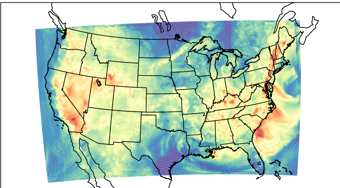
WRF (2023-07-08_02:00:00)
