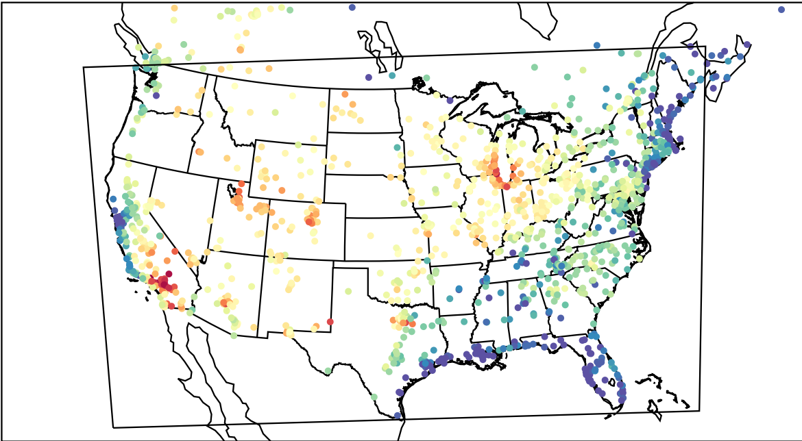
AirNOW (2023-07-09_22:00:00)
