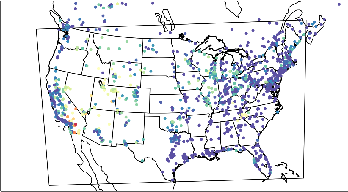
AirNOW (2023-07-08_08:00:00)
