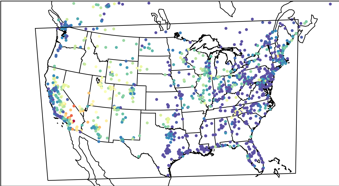
AirNOW (2023-07-08_05:00:00)
