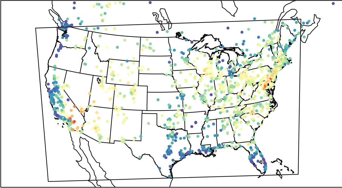
AirNOW (2023-07-08_16:00:00)
