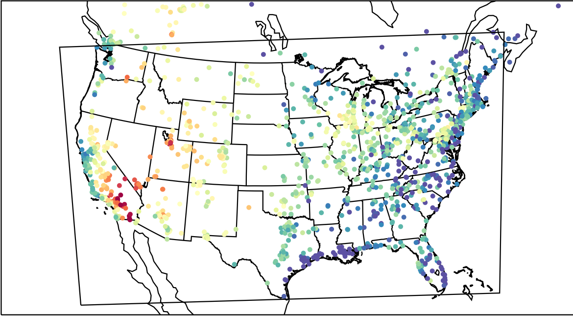
AirNOW (2023-07-09_01:00:00)
