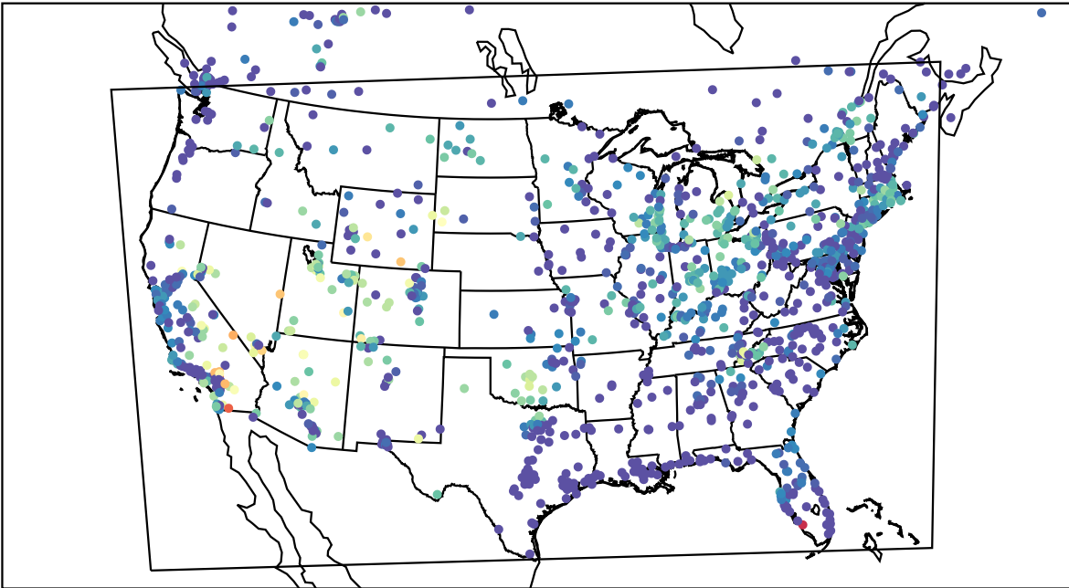
AirNOW (2023-07-09_12:00:00)
