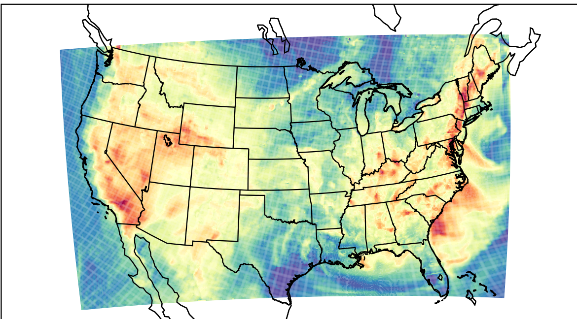
WRF (2023-07-08_01:00:00)
