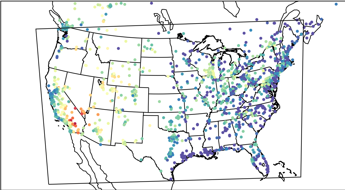
AirNOW (2023-07-09_03:00:00)
