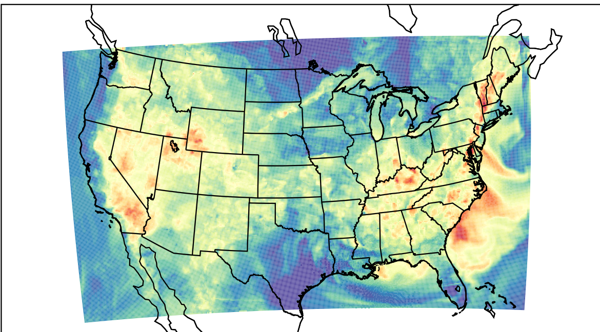
WRF (2023-07-08_03:00:00)
