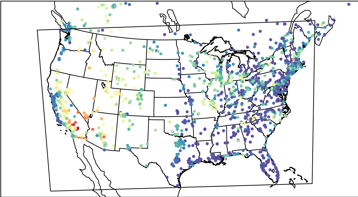
AirNOW (2023-07-08_03:00:00)
