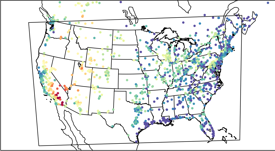
AirNOW (2023-07-09_02:00:00)
