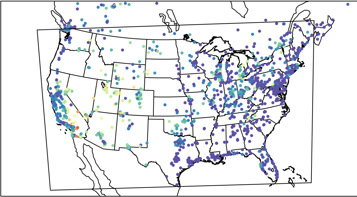
AirNOW (2023-07-09_08:00:00)
