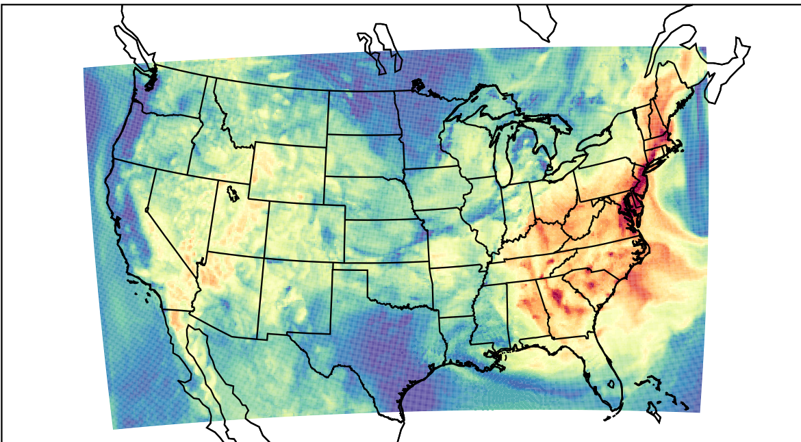
WRF (2023-07-08_15:00:00)
