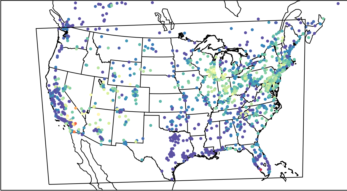
AirNOW (2023-07-08_13:00:00)
