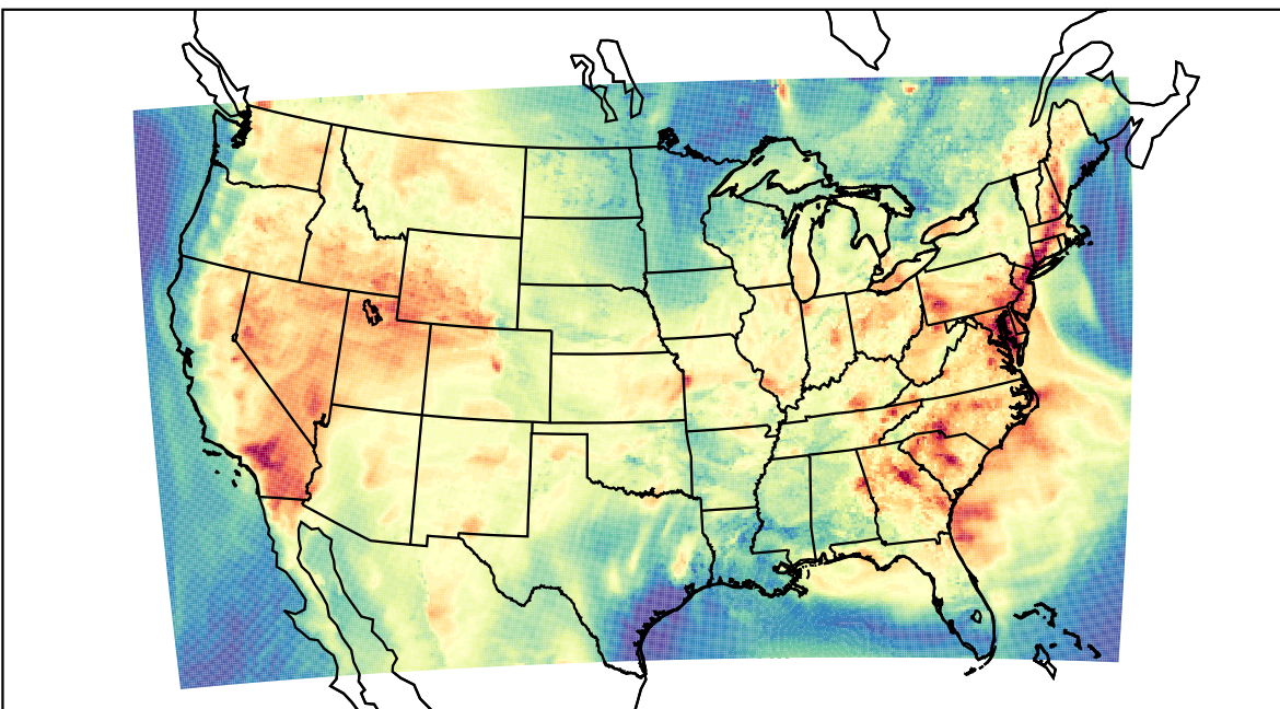
WRF (2023-07-08_23:00:00)
