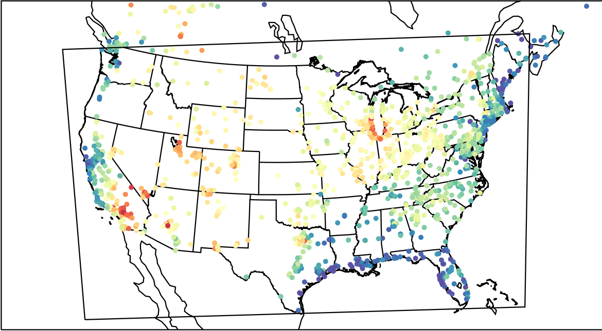
AirNOW (2023-07-09_19:00:00)
