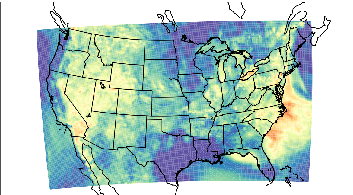
WRF (2023-07-09_07:00:00)
