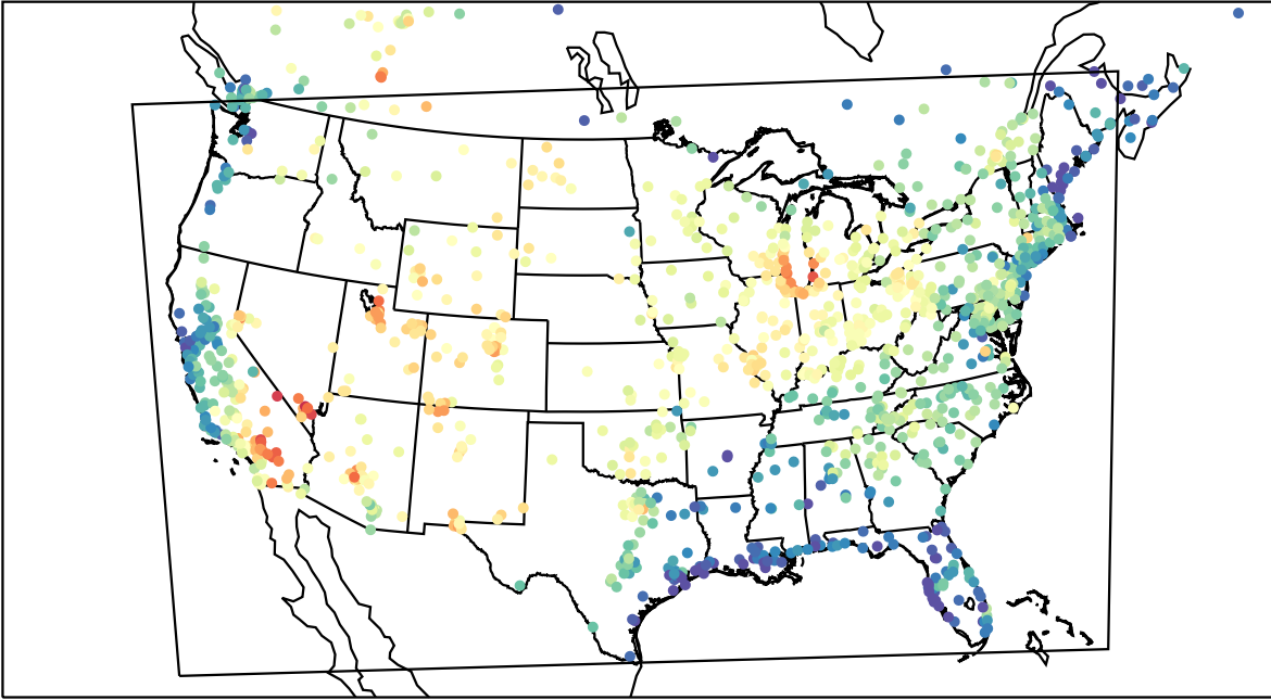
AirNOW (2023-07-09_18:00:00)
