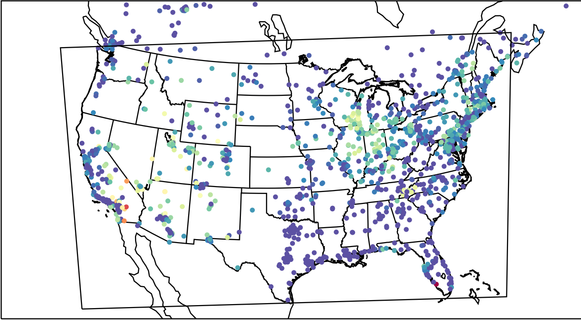
AirNOW (2023-07-08_12:00:00)
