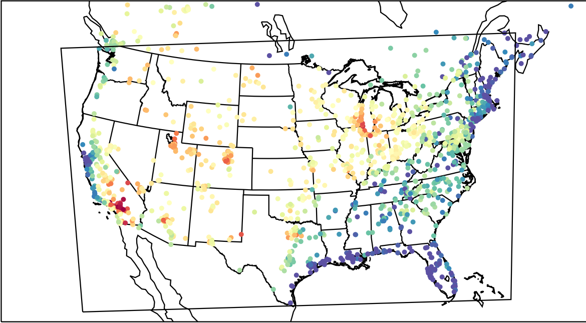
AirNOW (2023-07-09_23:00:00)
