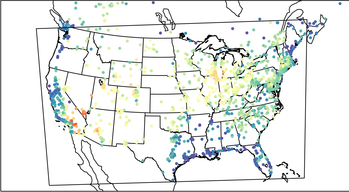
AirNOW (2023-07-09_16:00:00)
