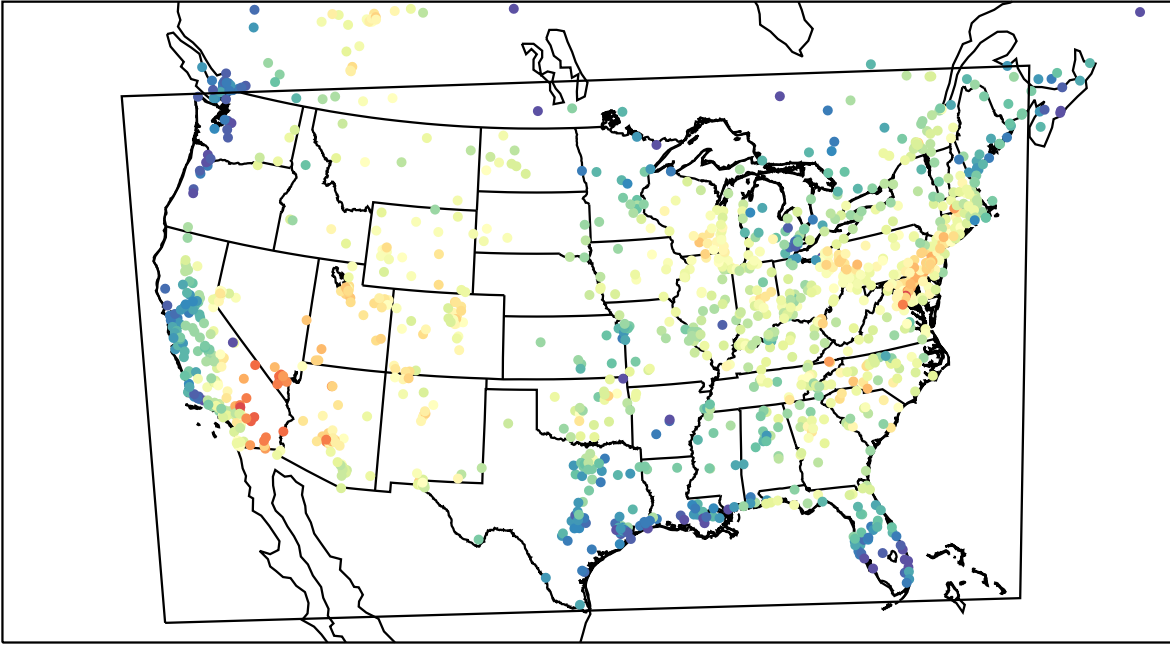
AirNOW (2023-07-08_17:00:00)
