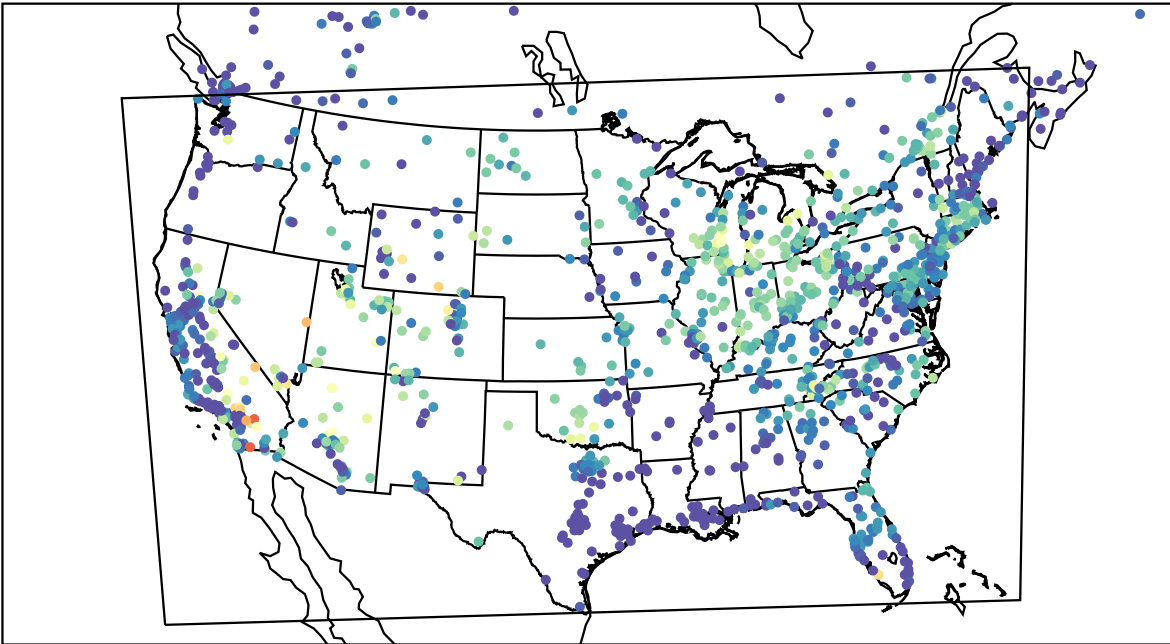
AirNOW (2023-07-09_13:00:00)
