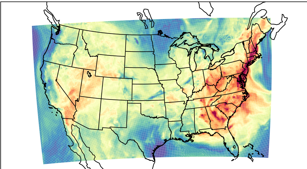
WRF (2023-07-08_17:00:00)
