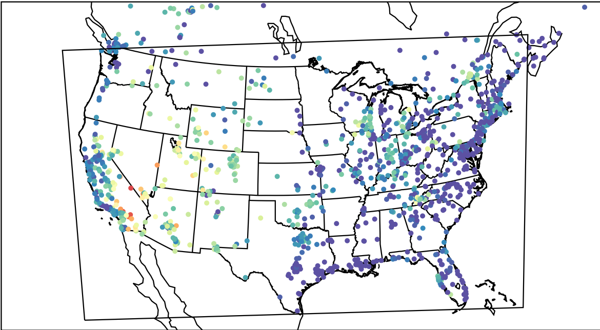
AirNOW (2023-07-09_06:00:00)
