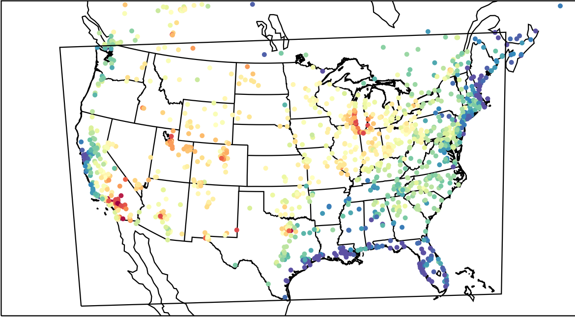
AirNOW (2023-07-09_21:00:00)
