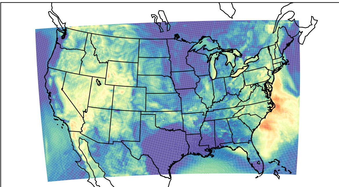
WRF (2023-07-09_12:00:00)
