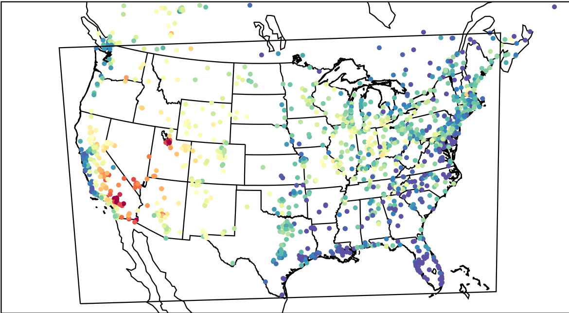
AirNOW (2023-07-08_01:00:00)
