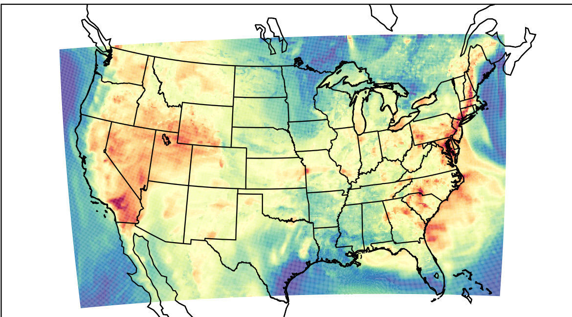
WRF (2023-07-09_00:00:00)
