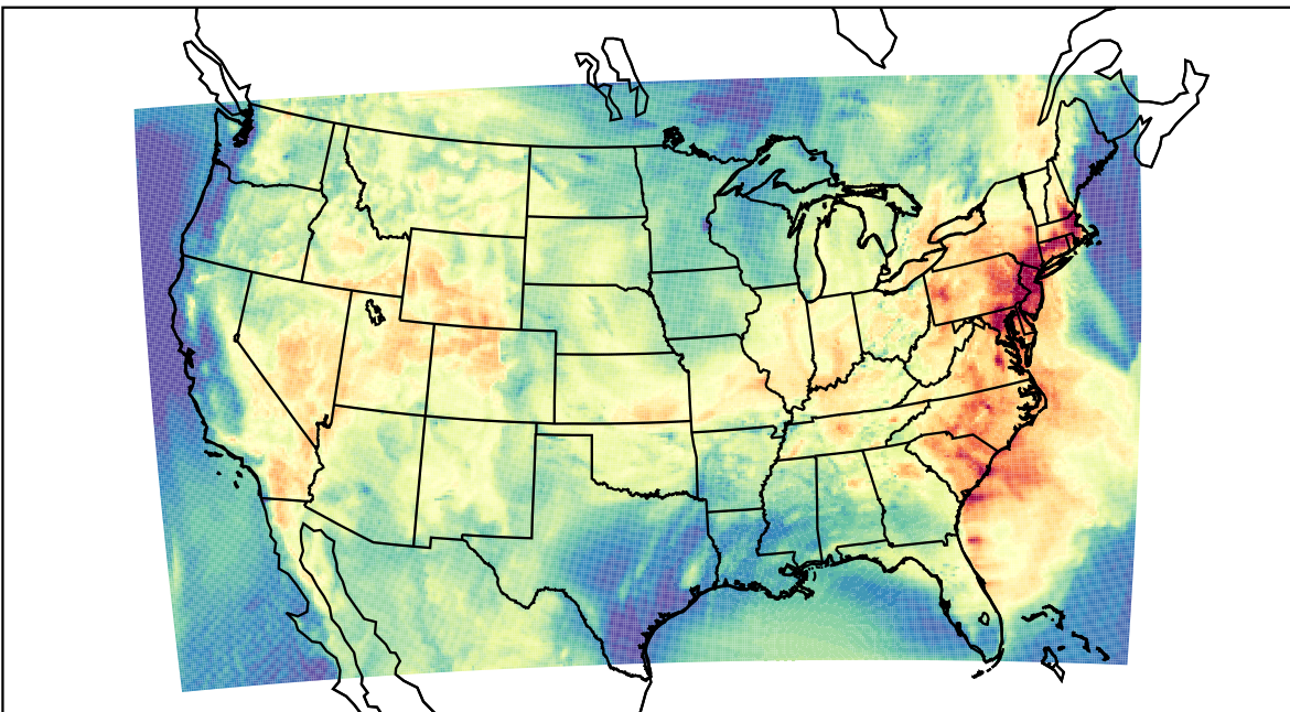
WRF (2023-07-09_16:00:00)
