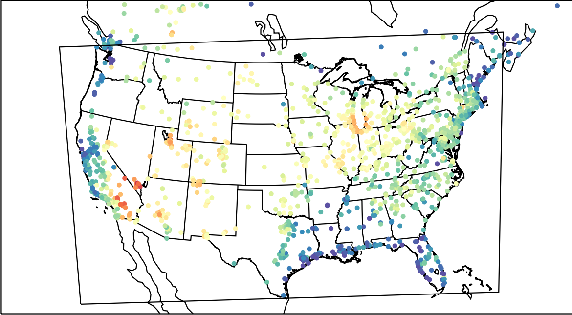
AirNOW (2023-07-09_17:00:00)
