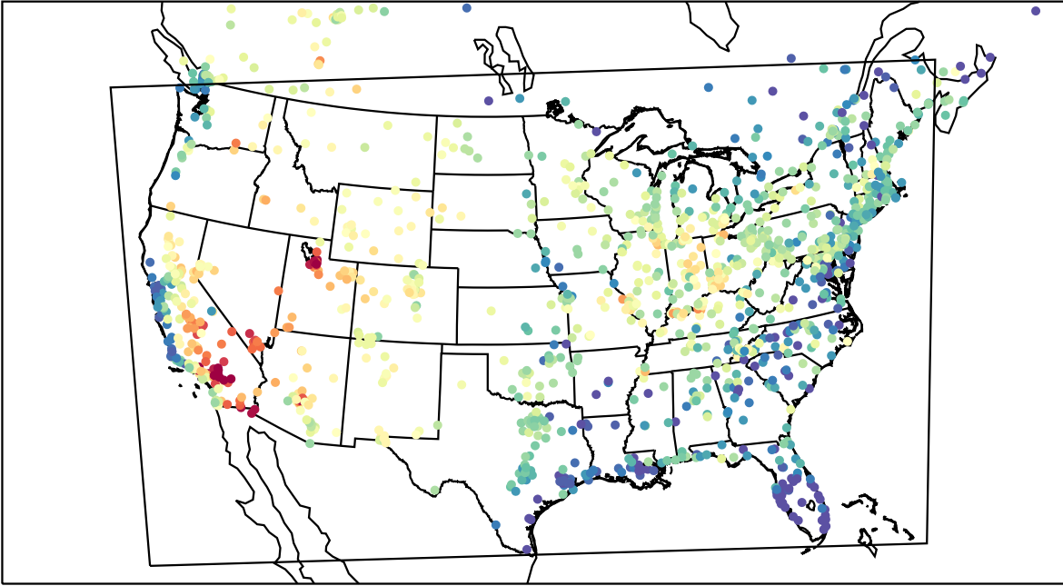
AirNOW (2023-07-08_00:00:00)
