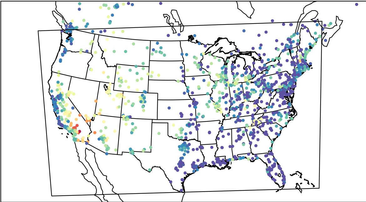
AirNOW (2023-07-08_04:00:00)
