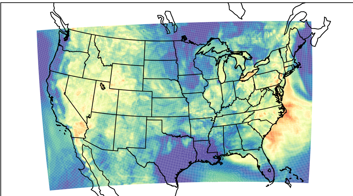
WRF (2023-07-09_06:00:00)
