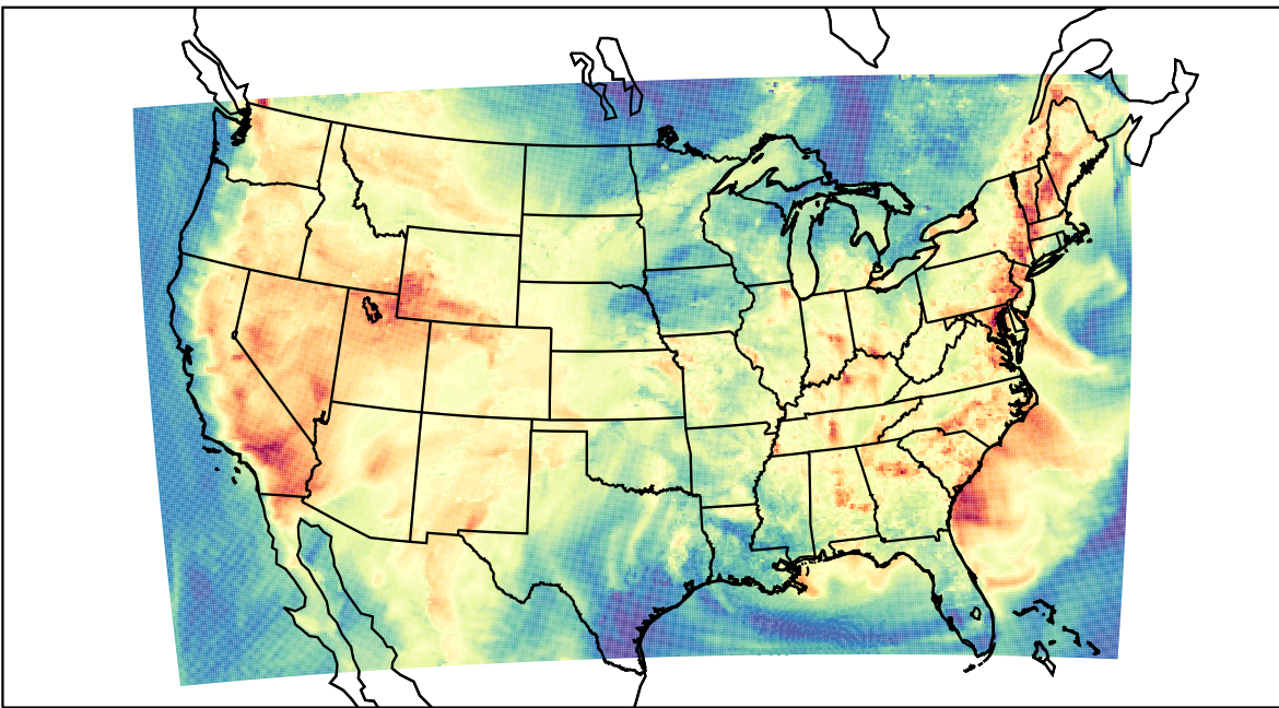
WRF (2023-07-08_00:00:00)
