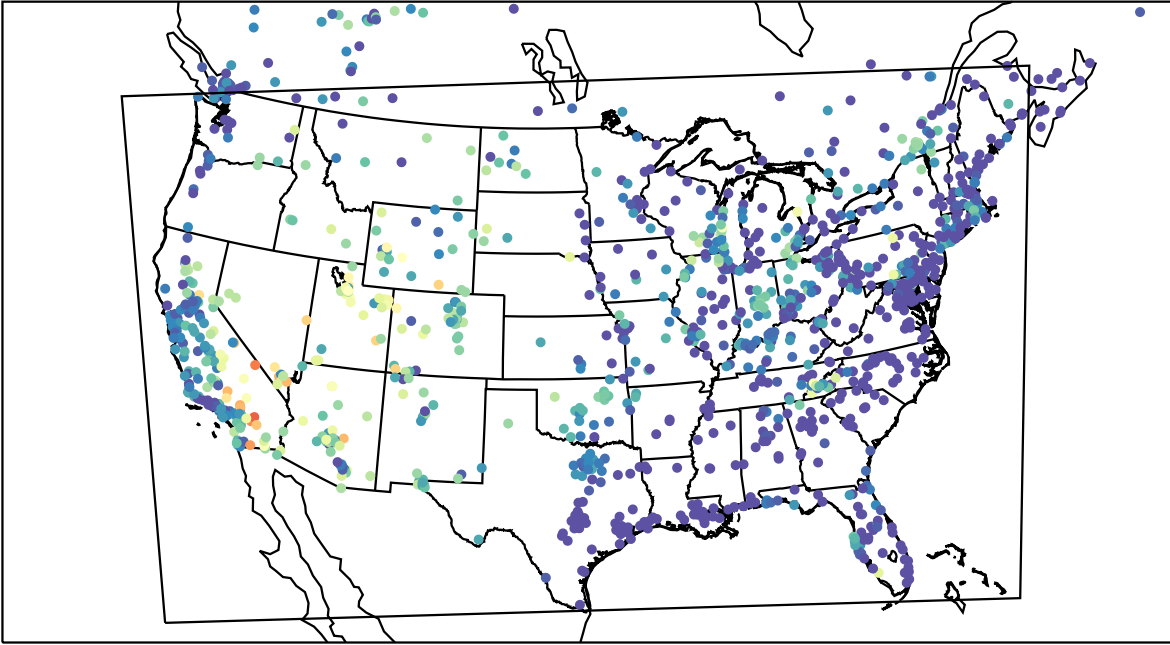
AirNOW (2023-07-09_07:00:00)
