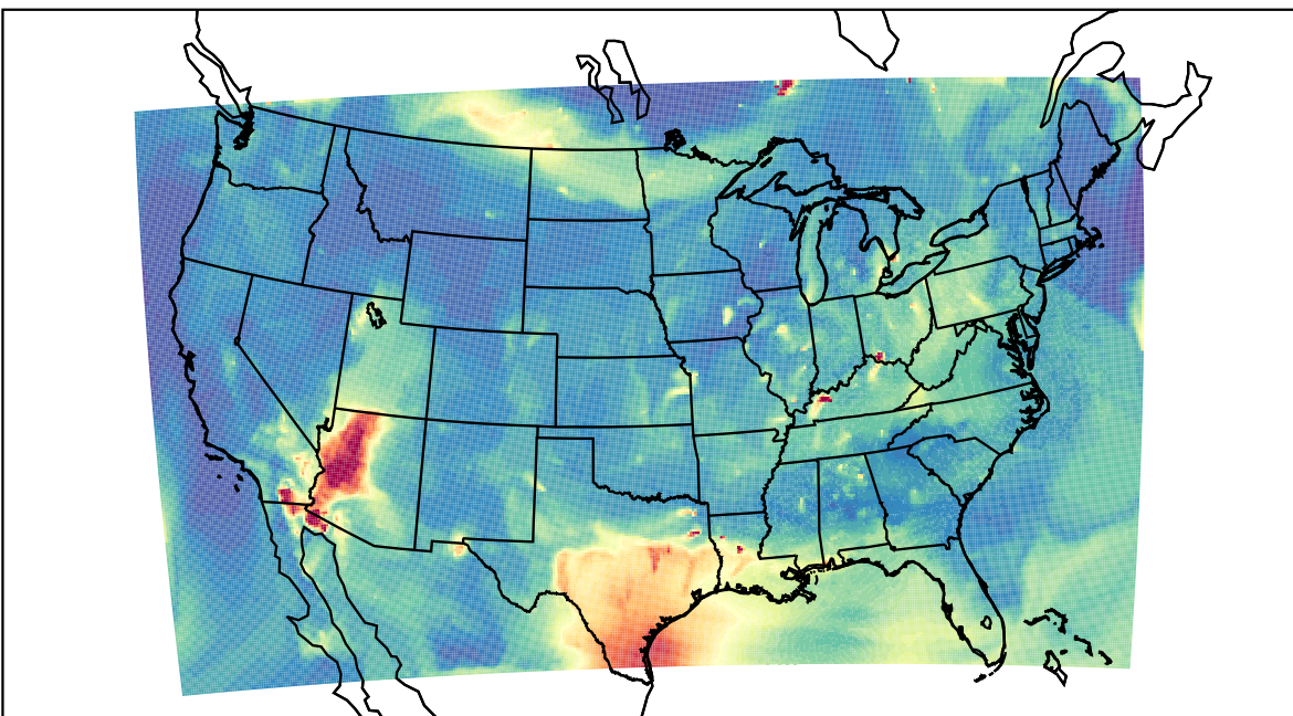
WRF 2023-07-10_09:00:00
