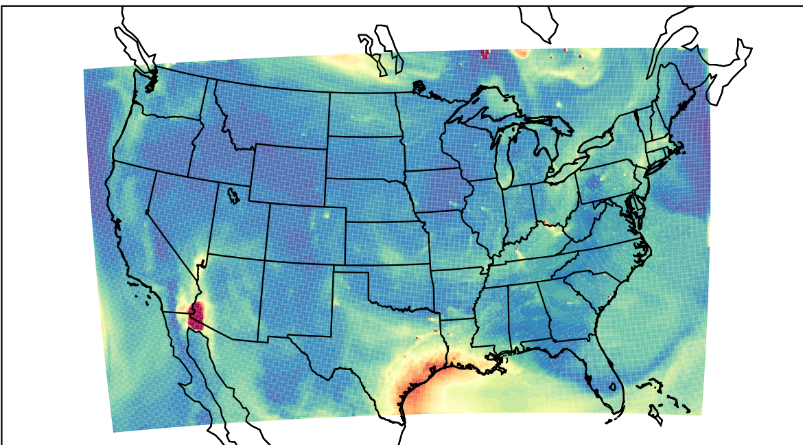
WRF 2023-07-09_19:00:00
