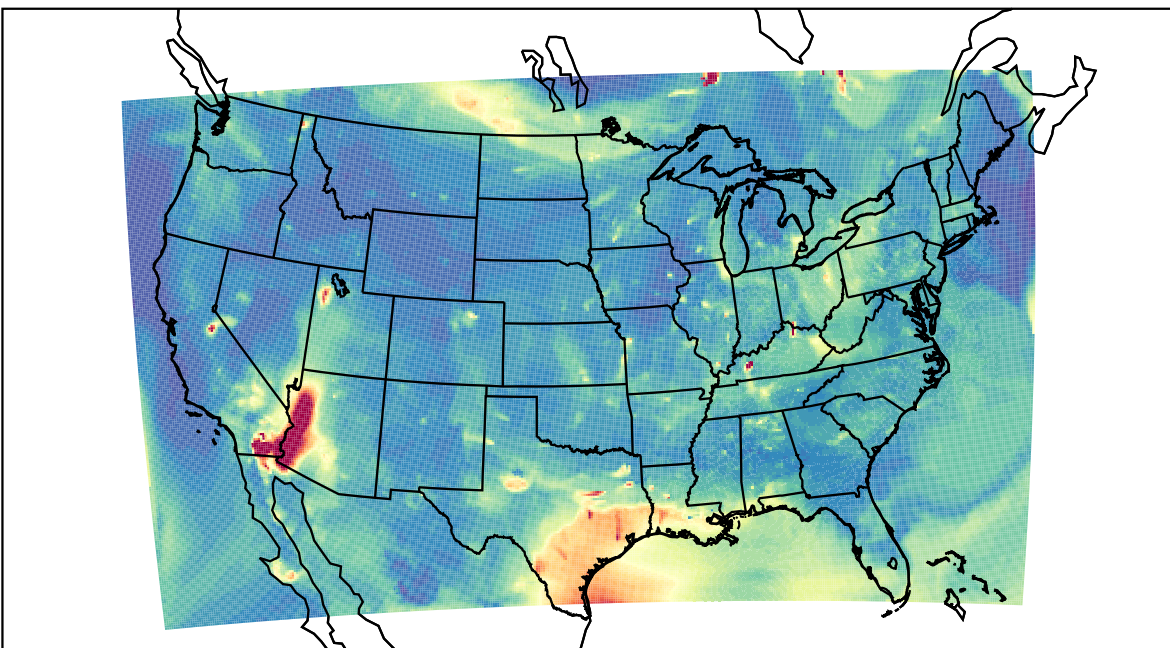
WRF 2023-07-10_04:00:00
