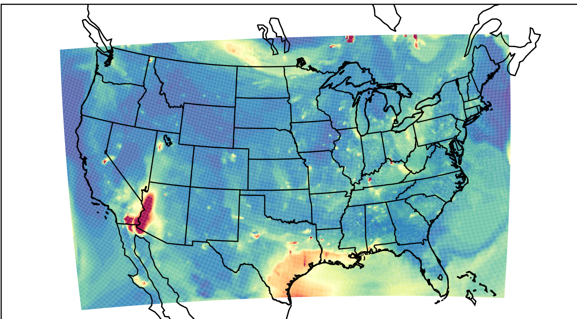
WRF 2023-07-10_03:00:00
