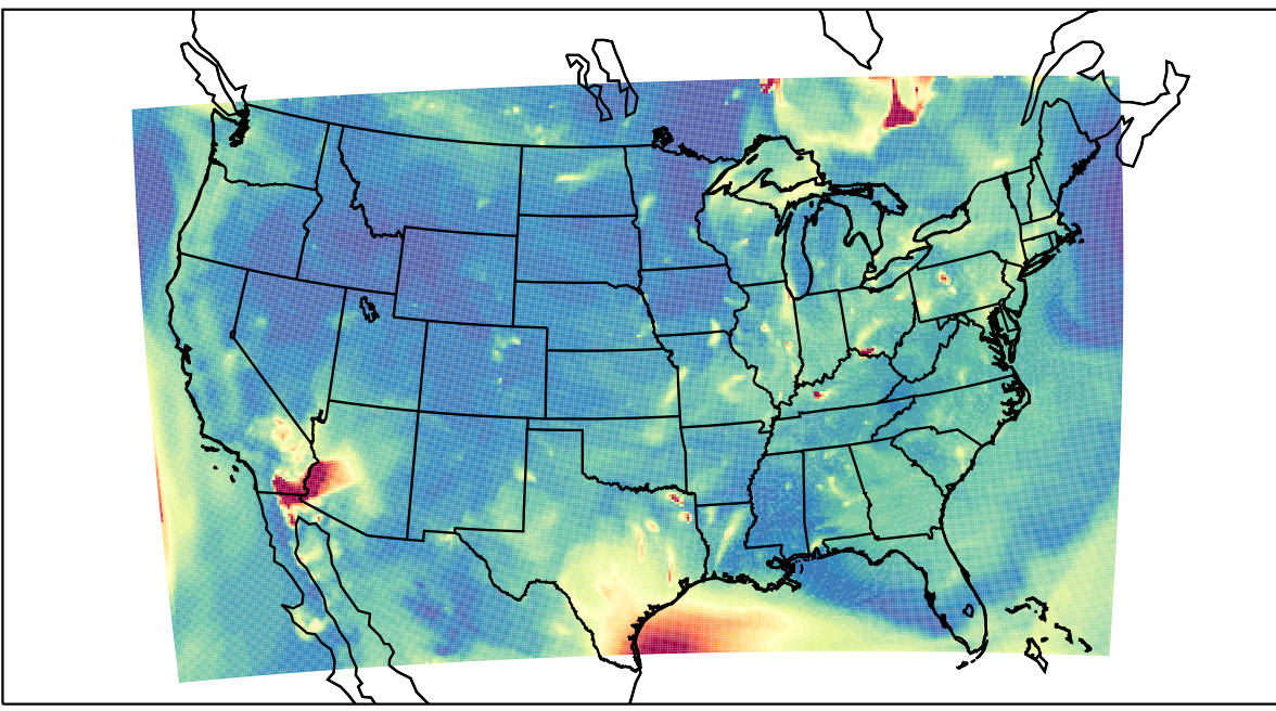
WRF 2023-07-09_07:00:00
