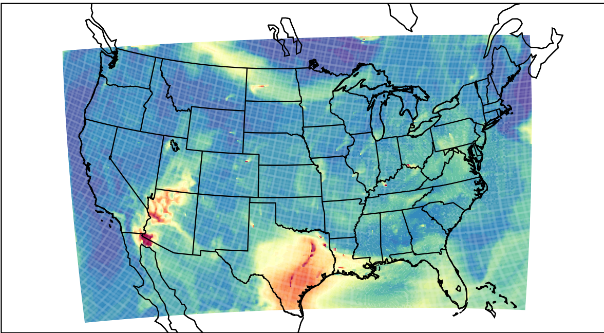
WRF 2023-07-10_15:00:00
