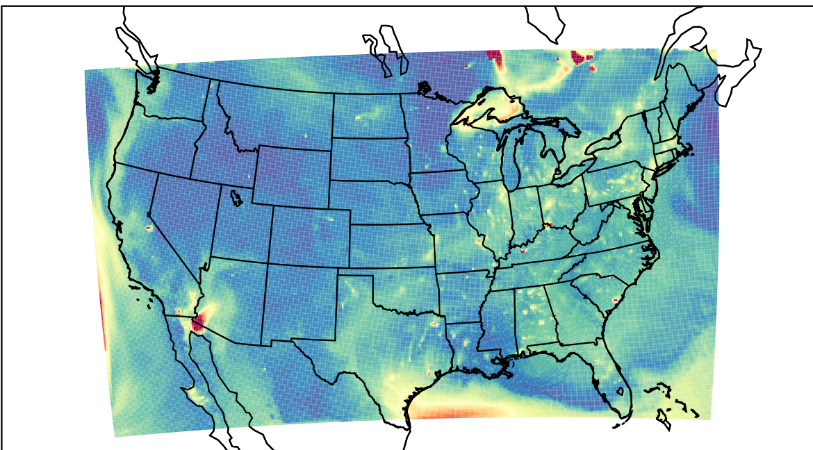
WRF 2023-07-09_01:00:00
