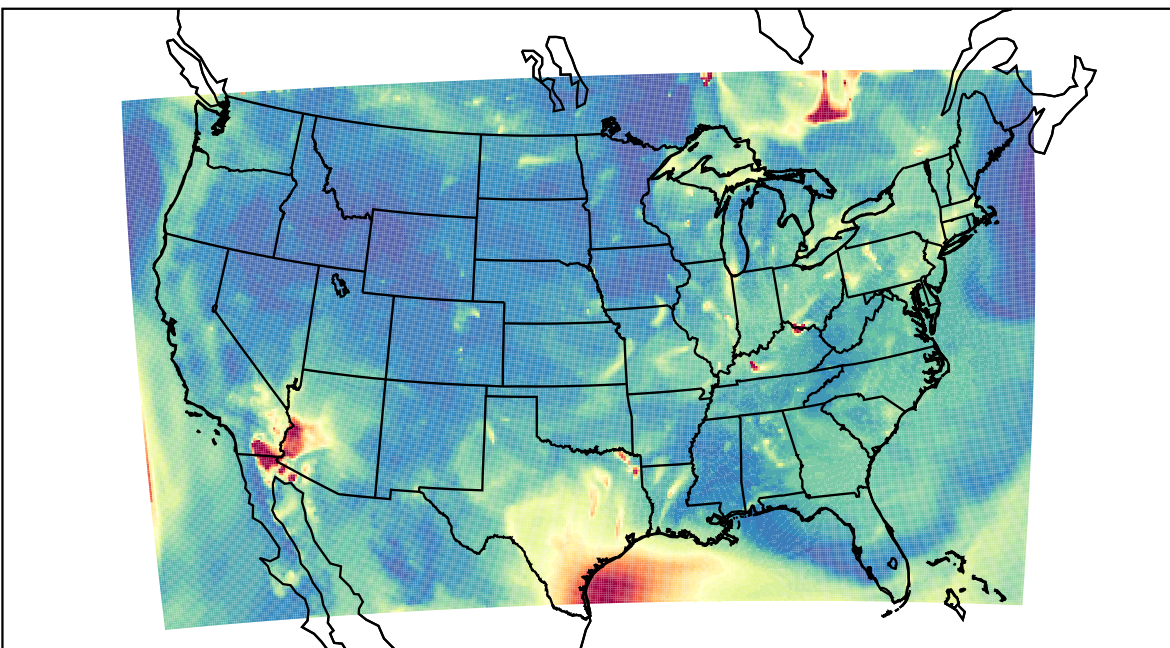
WRF 2023-07-09_09:00:00
