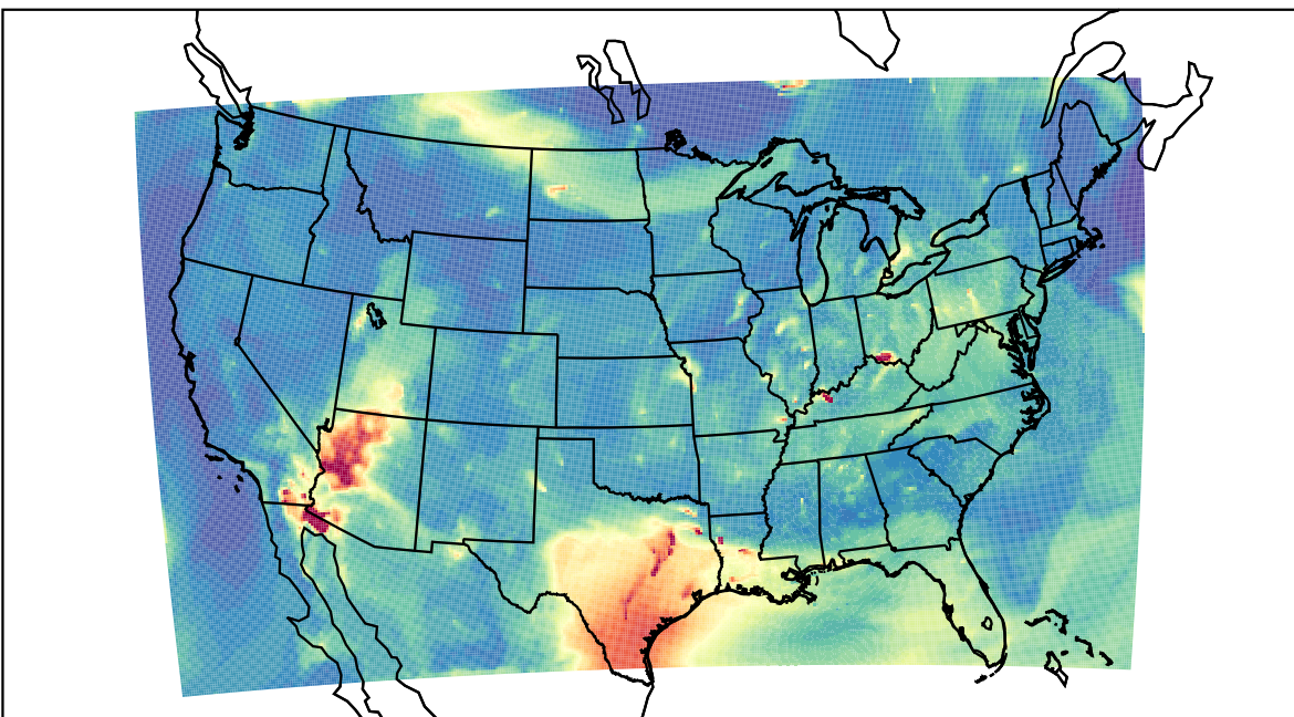
WRF 2023-07-10_13:00:00
