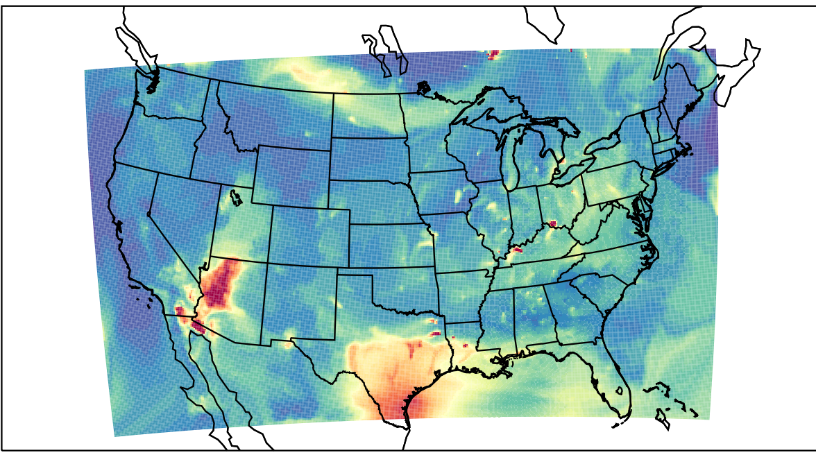
WRF 2023-07-10_10:00:00
