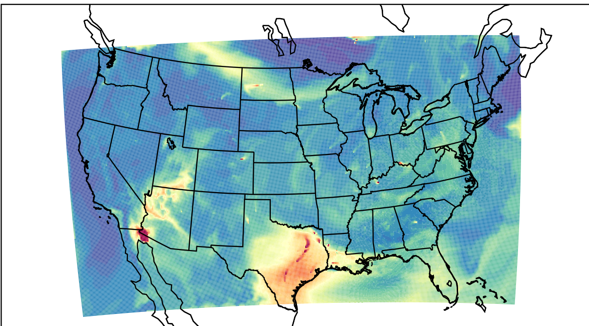
WRF 2023-07-10_16:00:00
