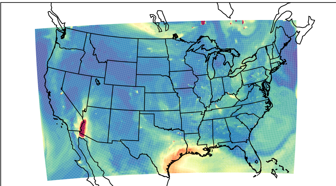
WRF 2023-07-09_23:00:00
