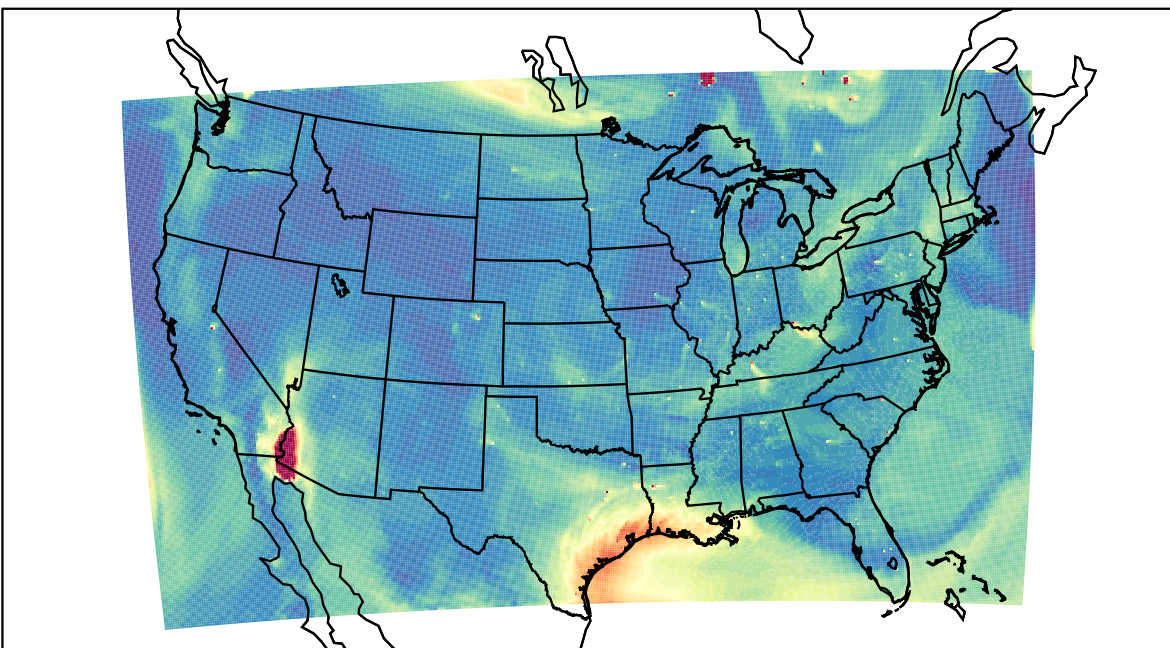
WRF 2023-07-09_21:00:00
