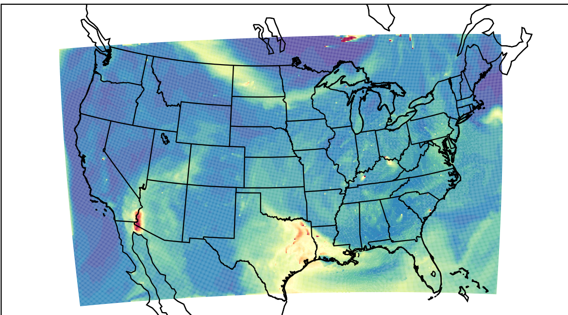
WRF 2023-07-10_21:00:00
