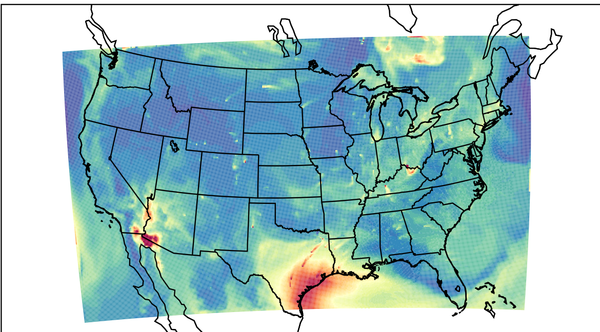
WRF 2023-07-09_15:00:00
