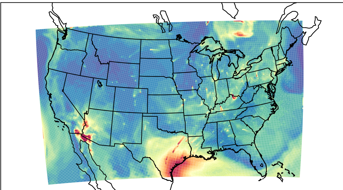
WRF 2023-07-09_14:00:00
