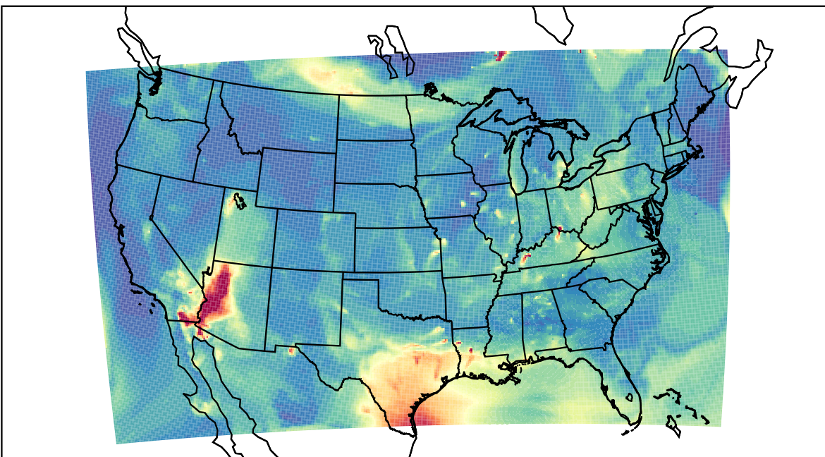
WRF 2023-07-10_07:00:00
