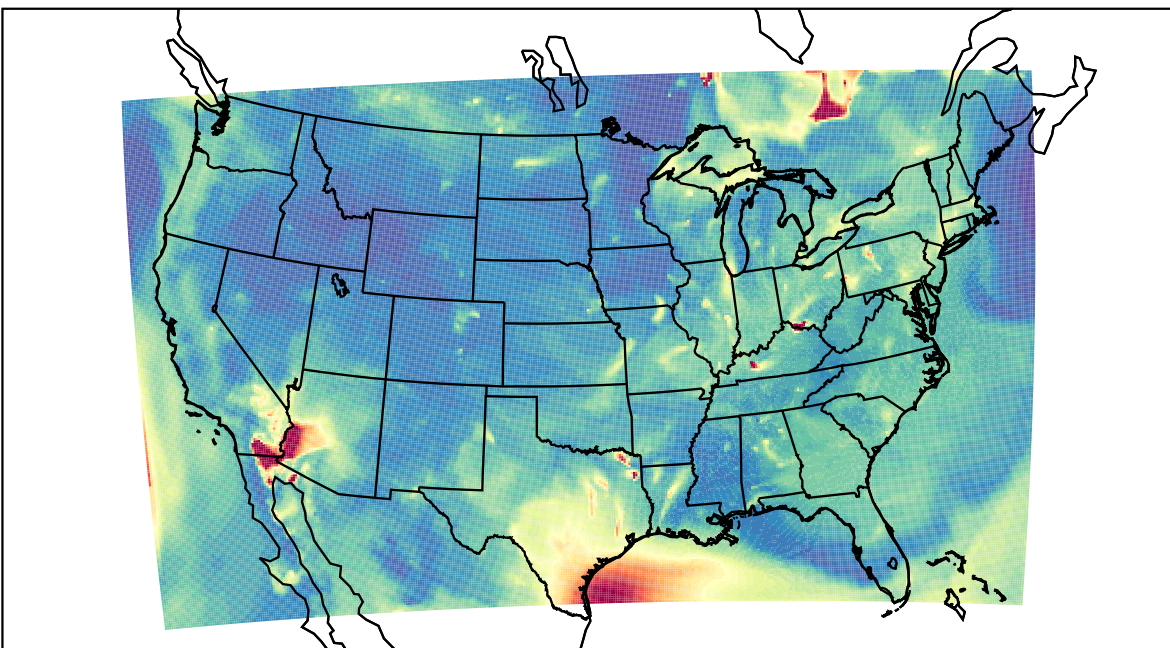
WRF 2023-07-09_08:00:00
