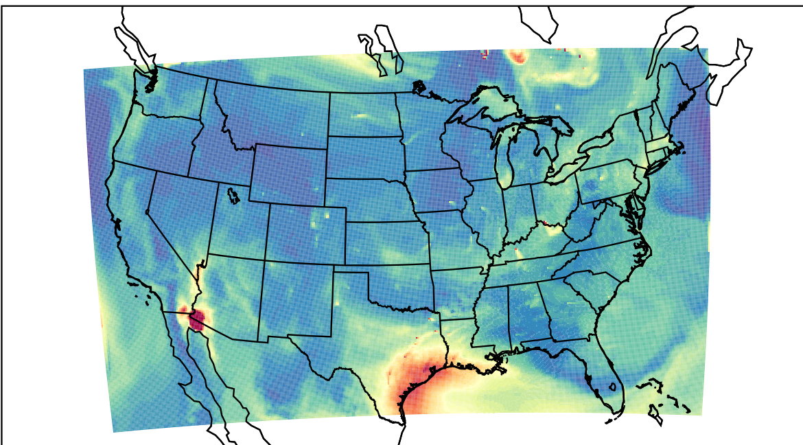
WRF 2023-07-09_17:00:00
