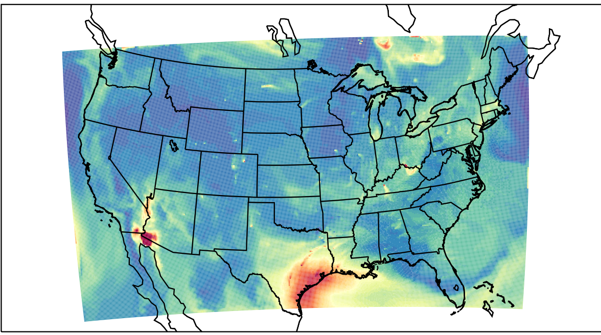
WRF 2023-07-09_16:00:00
