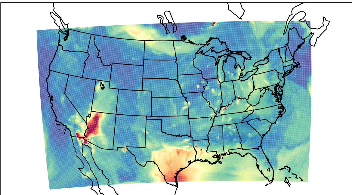
WRF 2023-07-10_08:00:00
