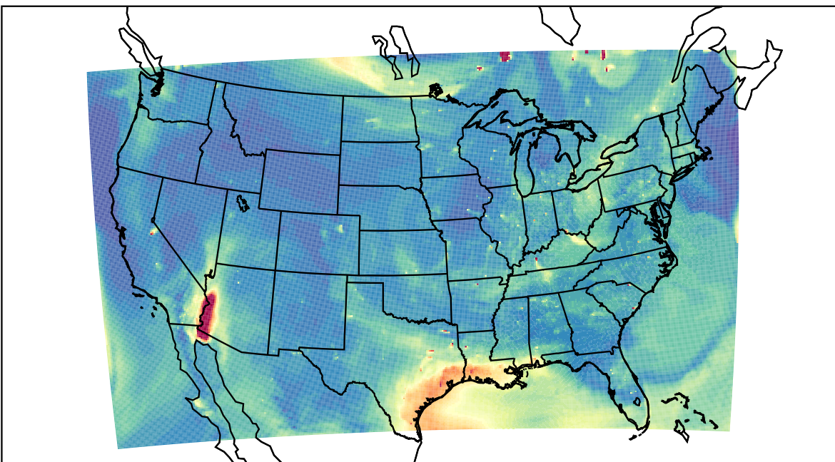
WRF 2023-07-10_00:00:00
