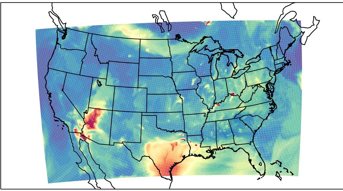
WRF 2023-07-10_11:00:00
