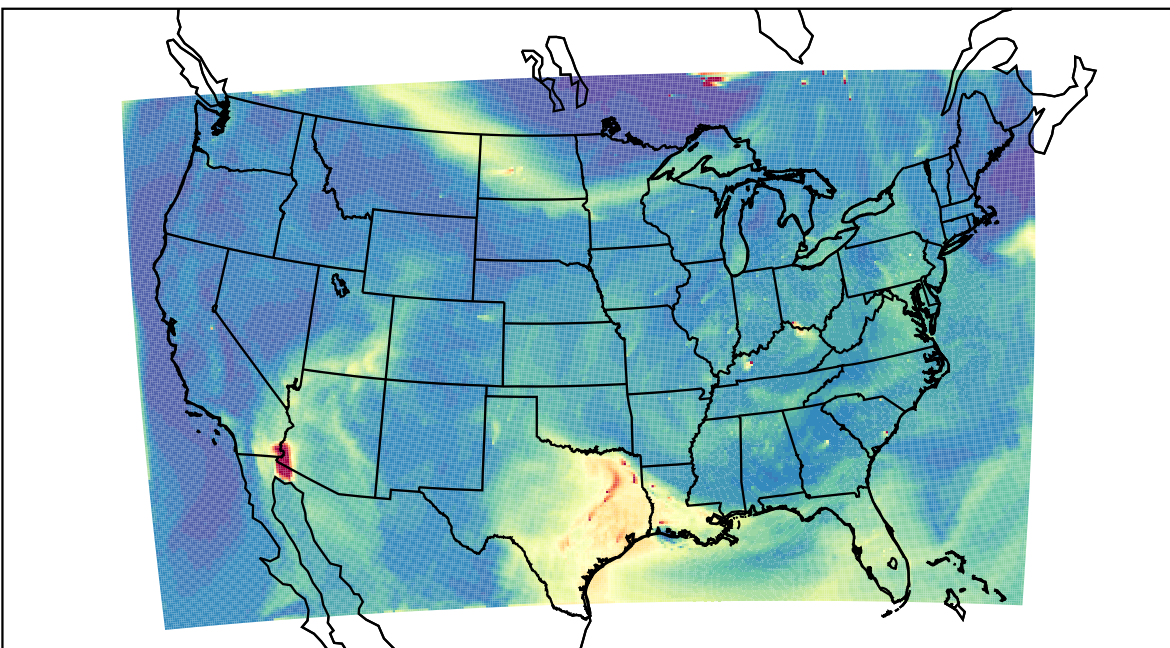
WRF 2023-07-10_19:00:00
