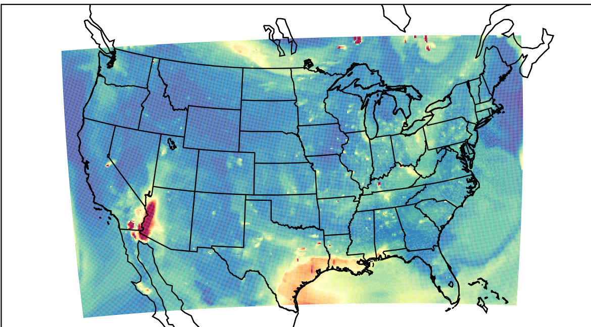
WRF 2023-07-10_02:00:00
