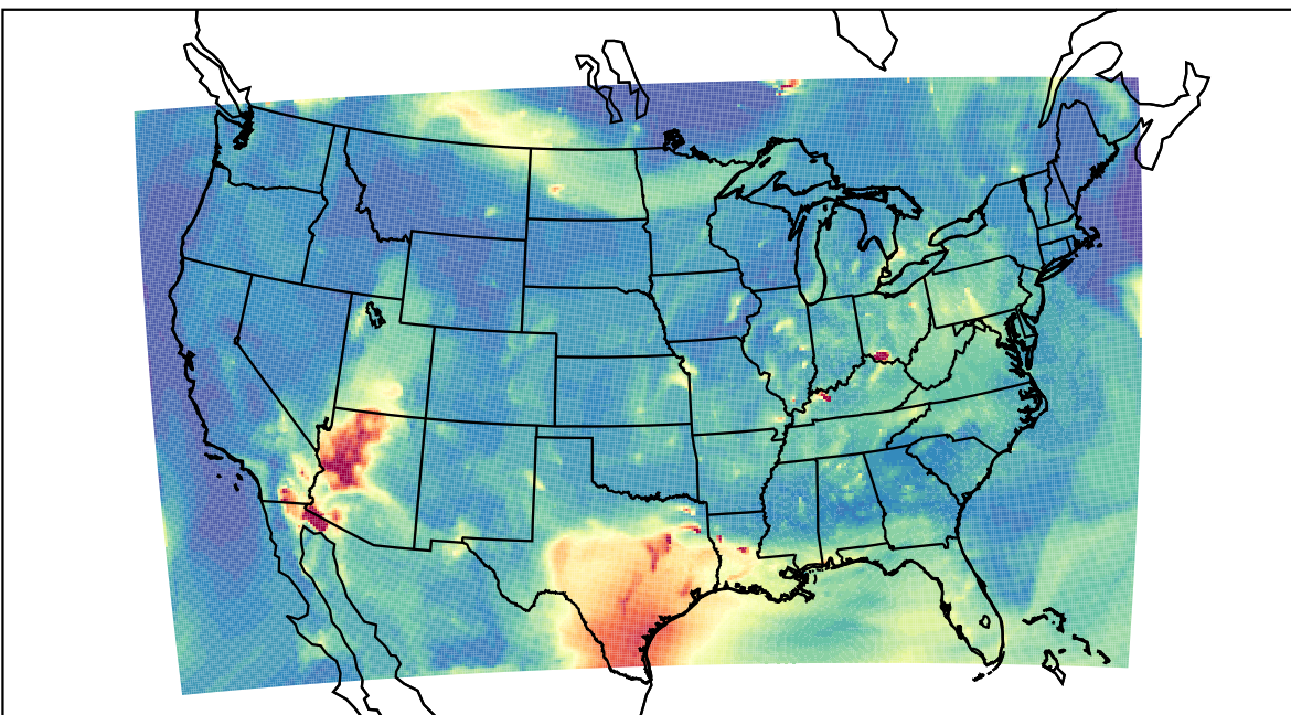
WRF 2023-07-10_12:00:00
