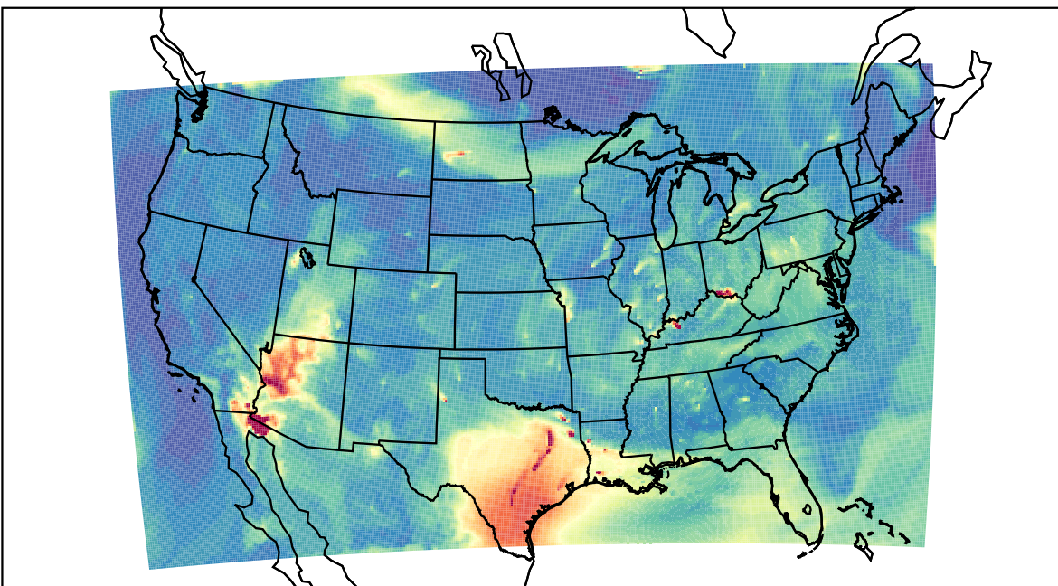
WRF 2023-07-10_14:00:00
