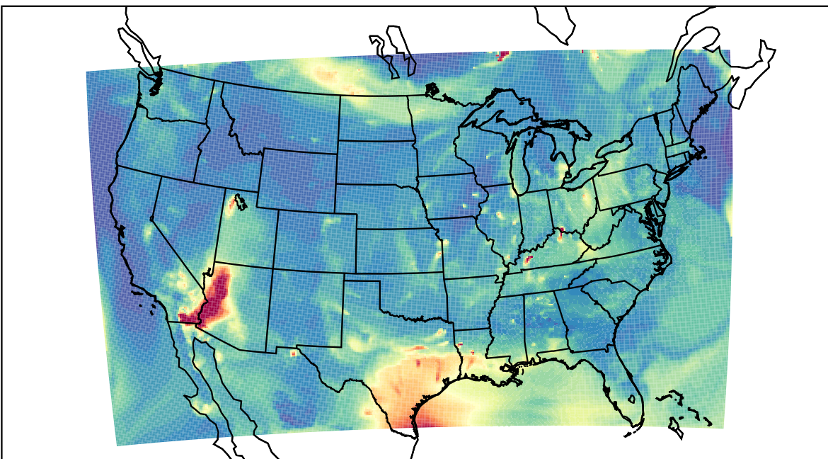
WRF 2023-07-10_06:00:00
