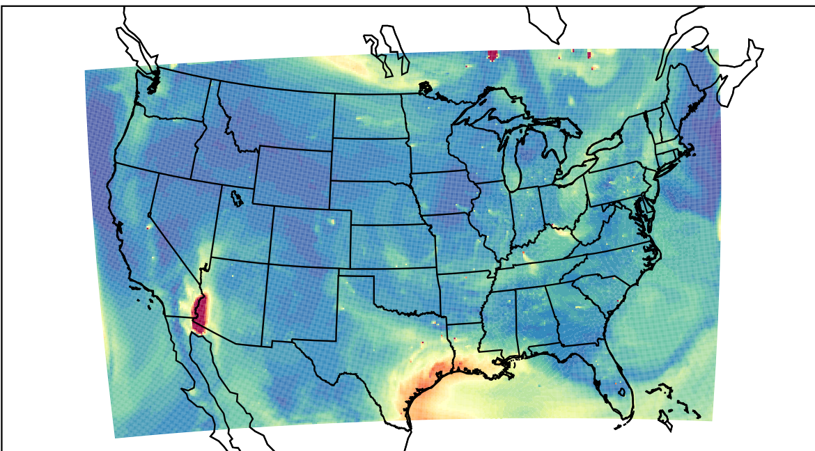
WRF 2023-07-09_22:00:00
