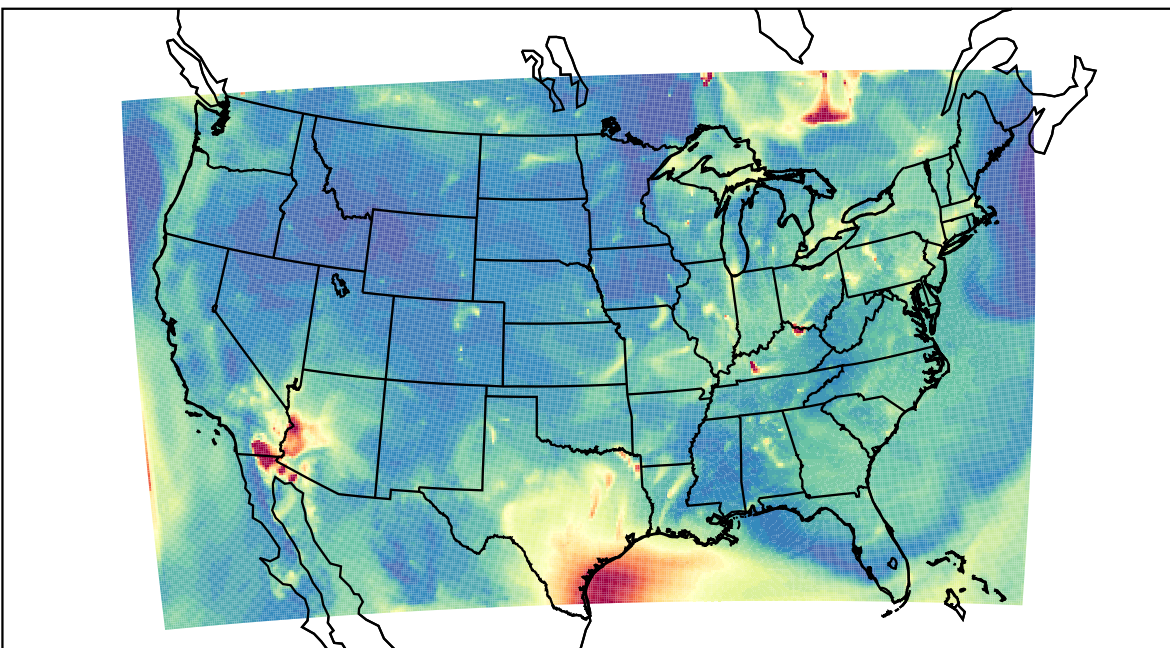
WRF 2023-07-09_10:00:00
