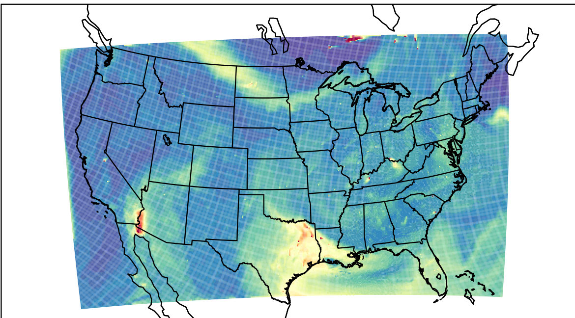
WRF 2023-07-10_22:00:00
