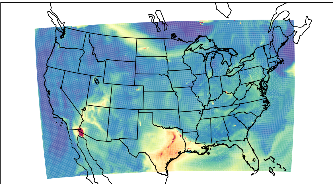
WRF 2023-07-10_17:00:00
