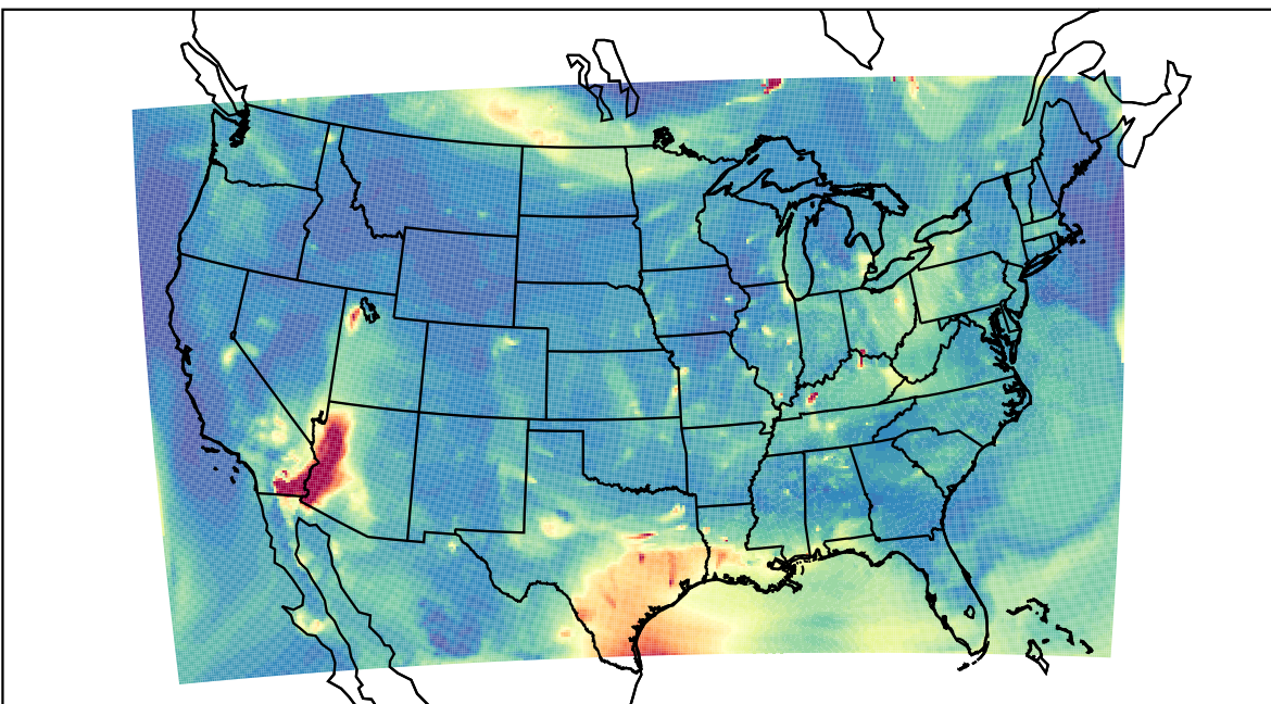
WRF 2023-07-10_05:00:00
