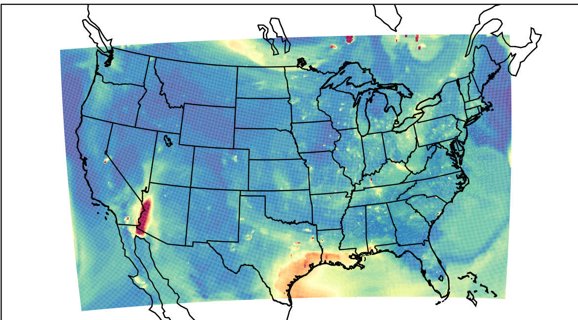
WRF 2023-07-10_01:00:00
