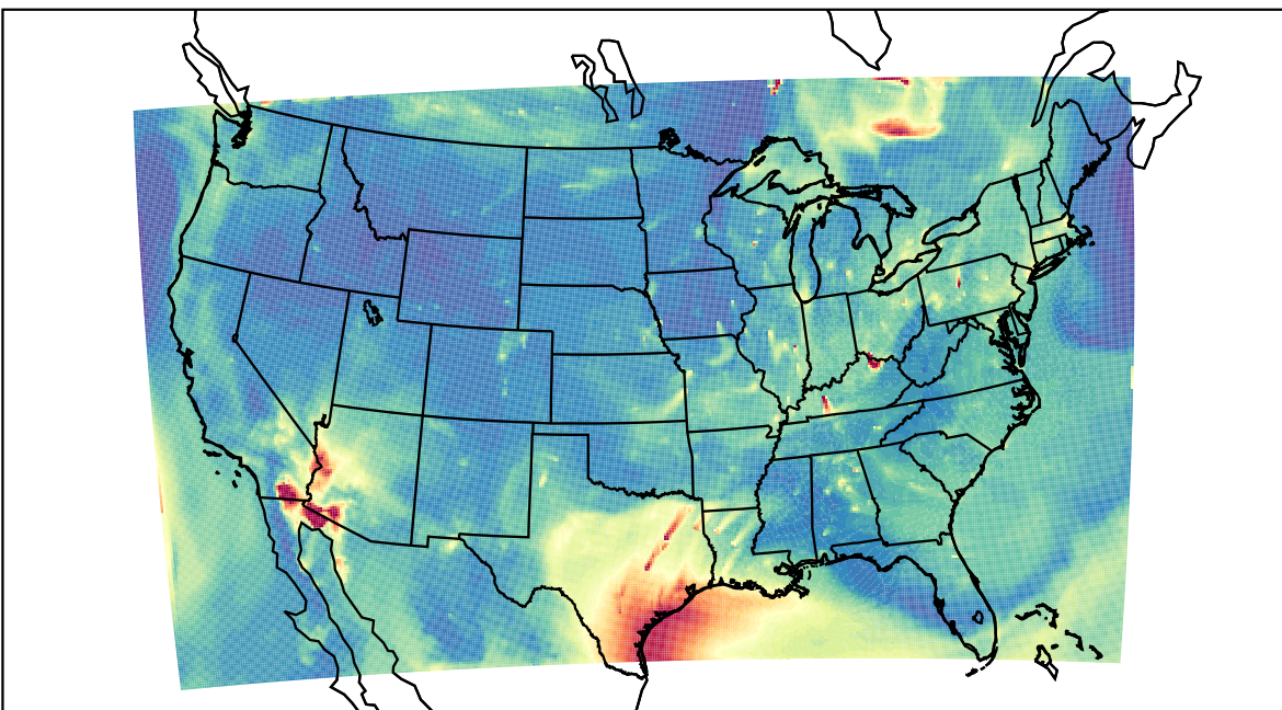
WRF 2023-07-09_13:00:00
