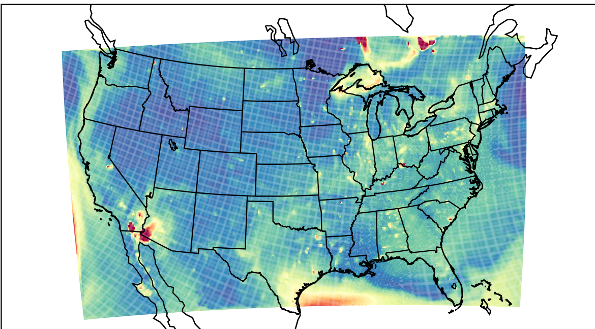
WRF 2023-07-09_02:00:00
