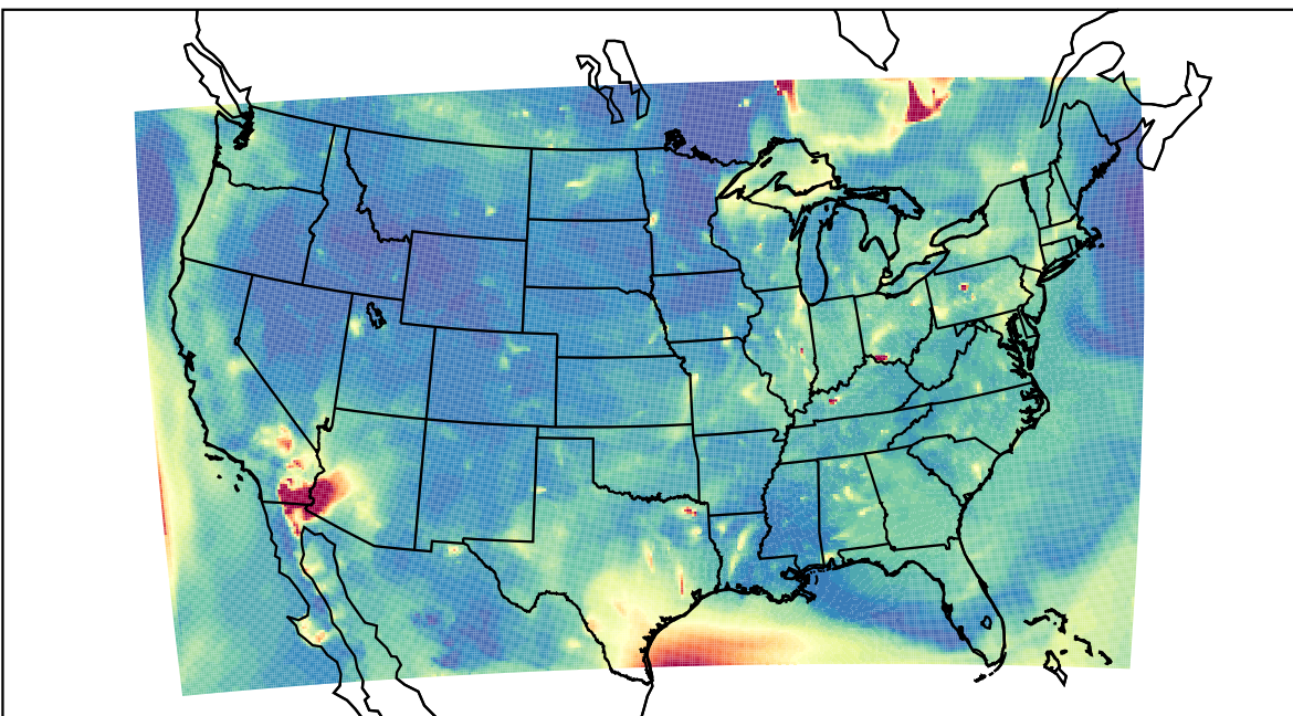
WRF 2023-07-09_05:00:00
