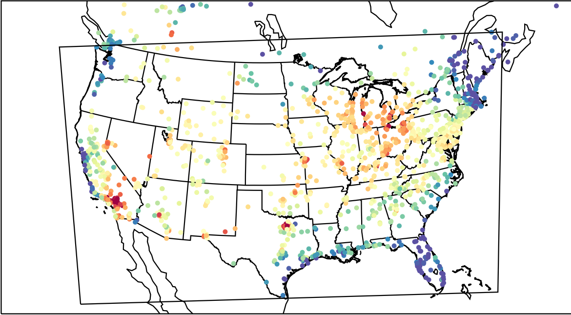
AirNOW (2023-07-10_20:00:00)
