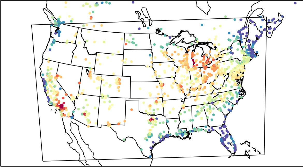
AirNOW (2023-07-10_21:00:00)
