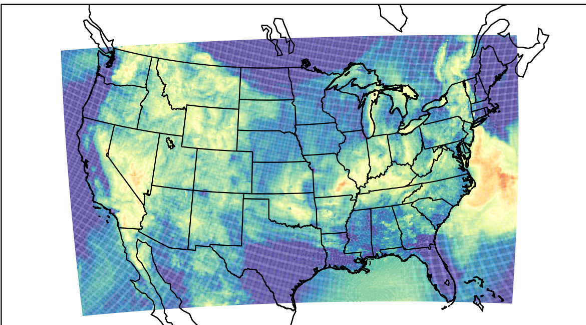
WRF (2023-07-10_11:00:00)
