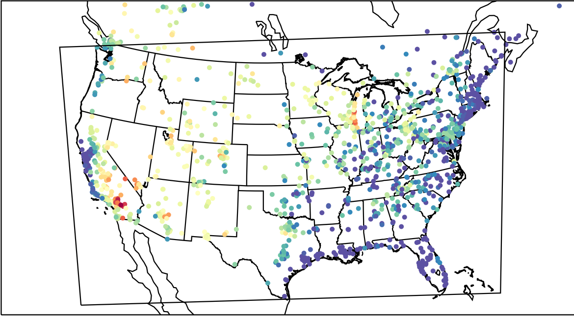
AirNOW (2023-07-10_02:00:00)
