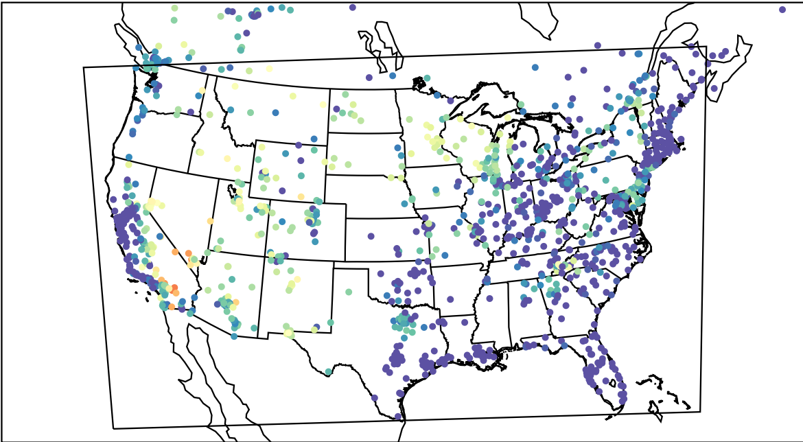
AirNOW (2023-07-10_06:00:00)
