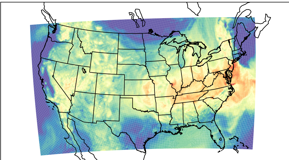
WRF (2023-07-10_15:00:00)
