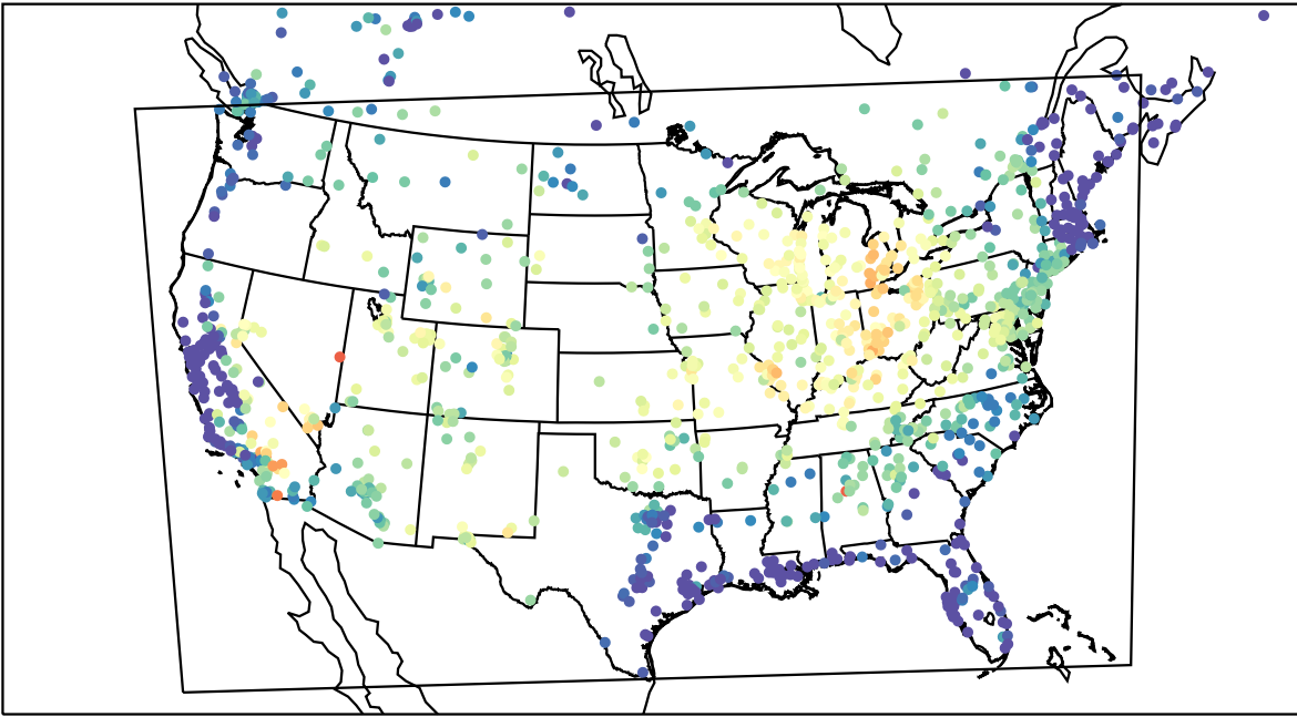
AirNOW (2023-07-10_15:00:00)
