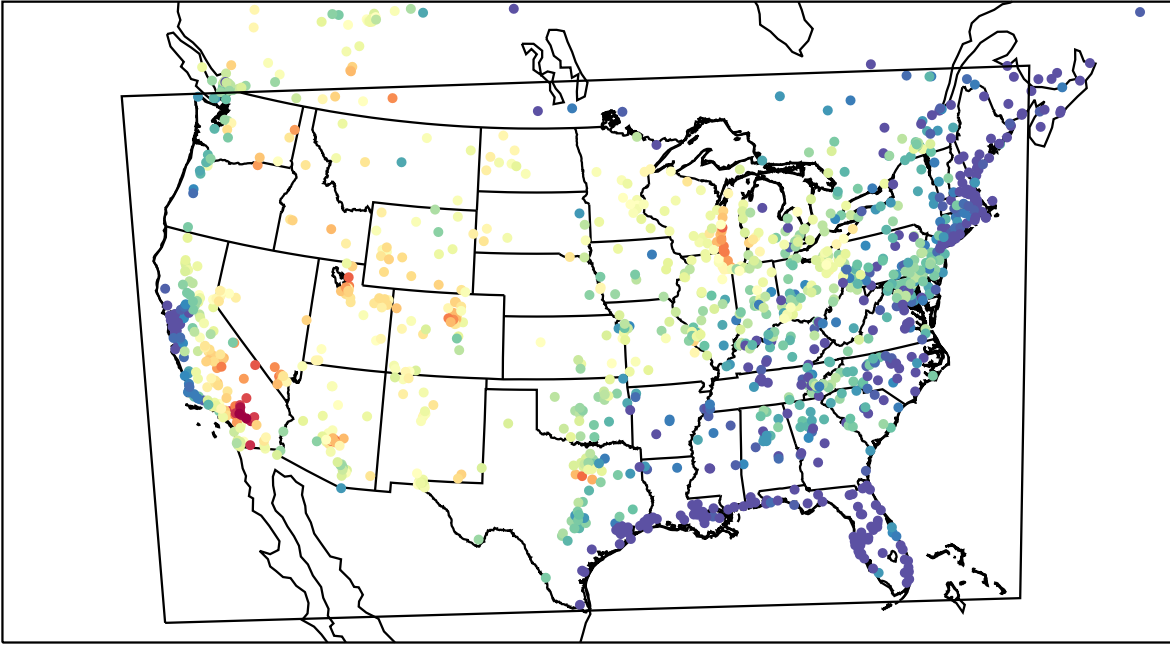
AirNOW (2023-07-10_01:00:00)
