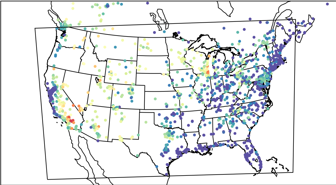
AirNOW (2023-07-10_03:00:00)
