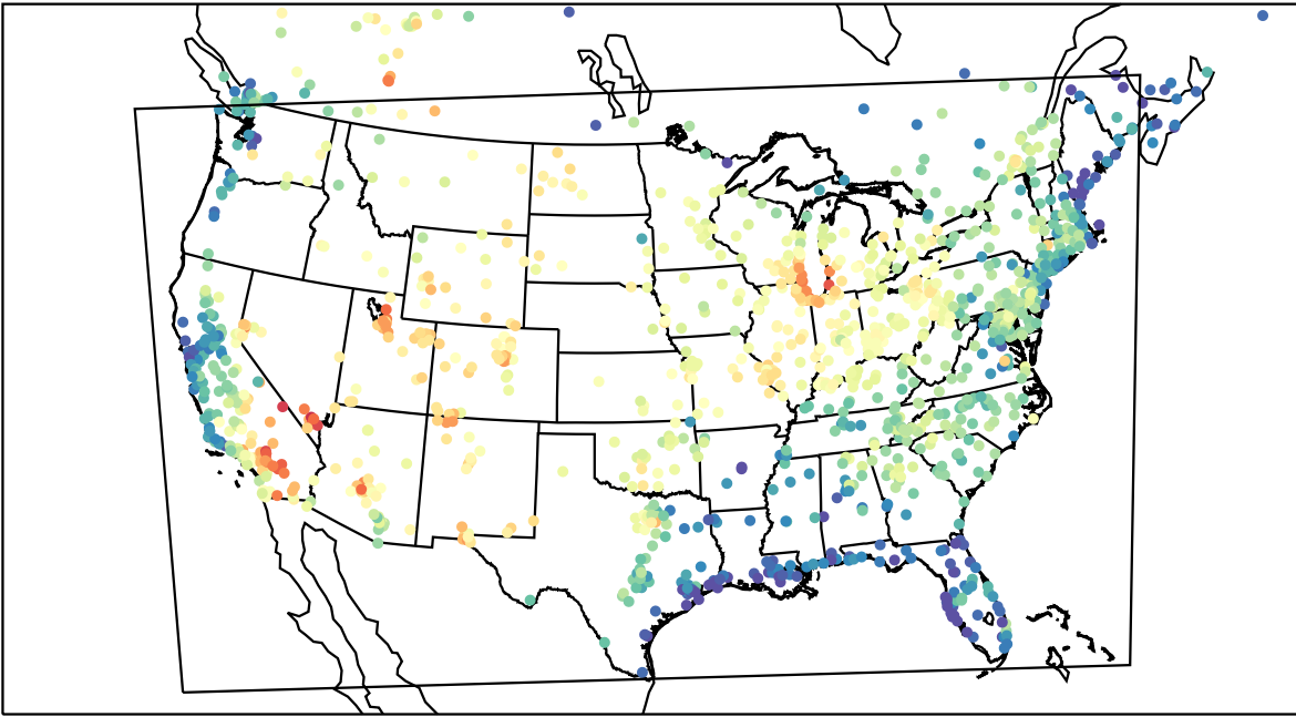
AirNOW (2023-07-09_18:00:00)
