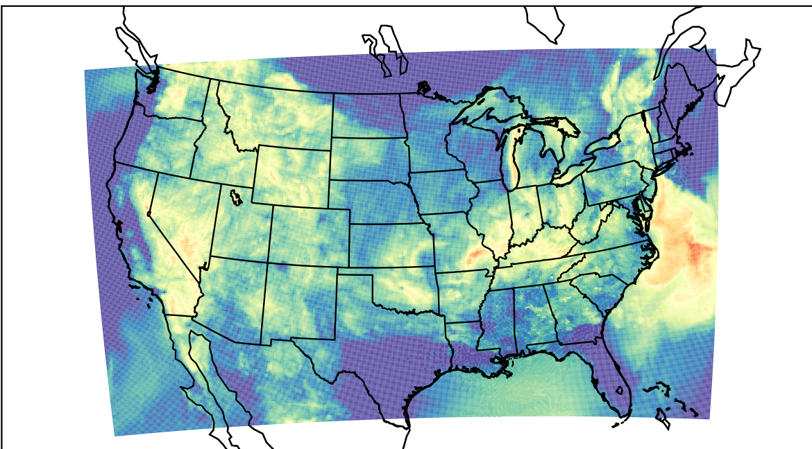
WRF (2023-07-10_10:00:00)
