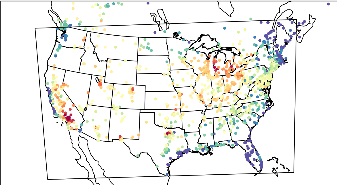
AirNOW (2023-07-10_23:00:00)
