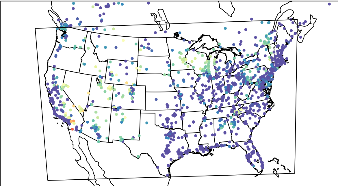
AirNOW (2023-07-10_11:00:00)
