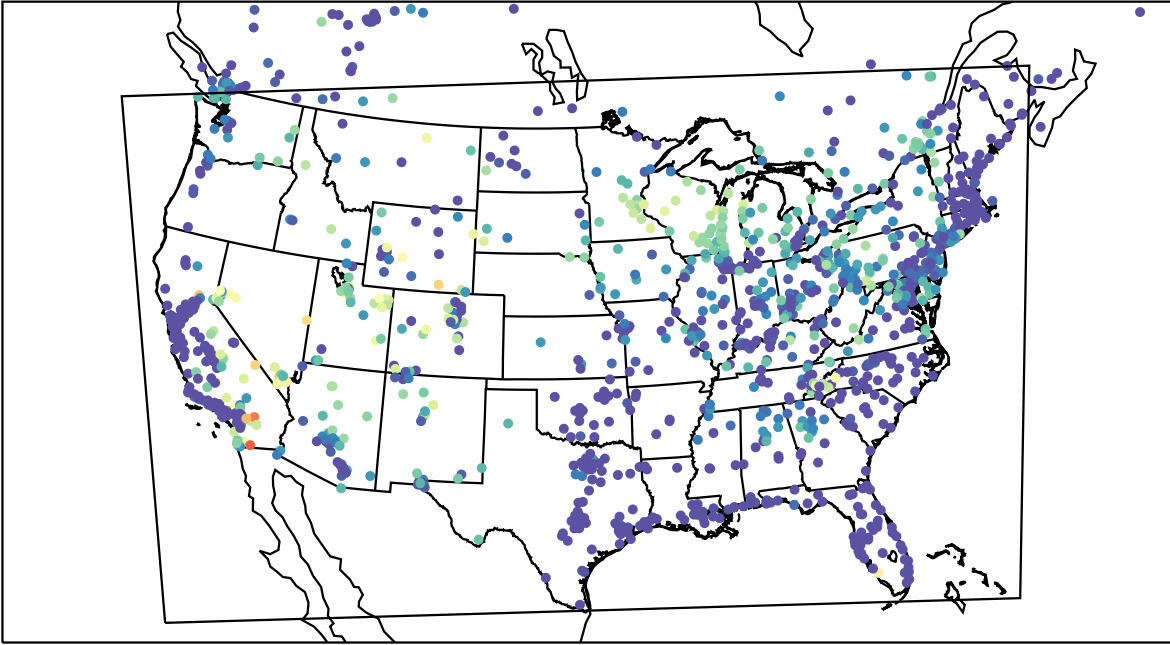
AirNOW (2023-07-10_12:00:00)
