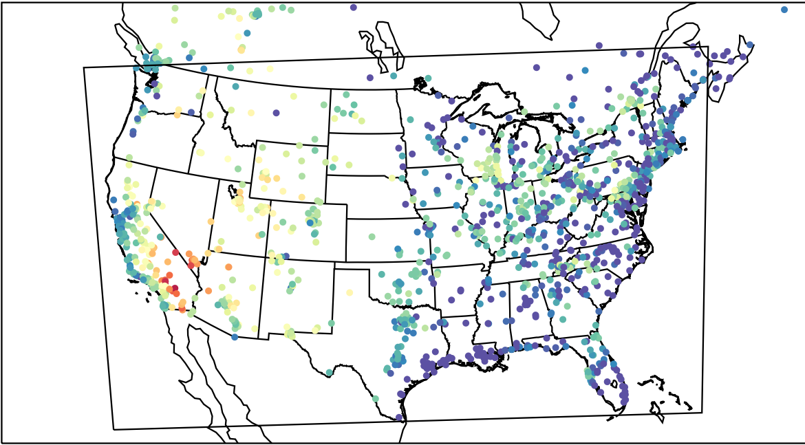
AirNOW (2023-07-09_03:00:00)
