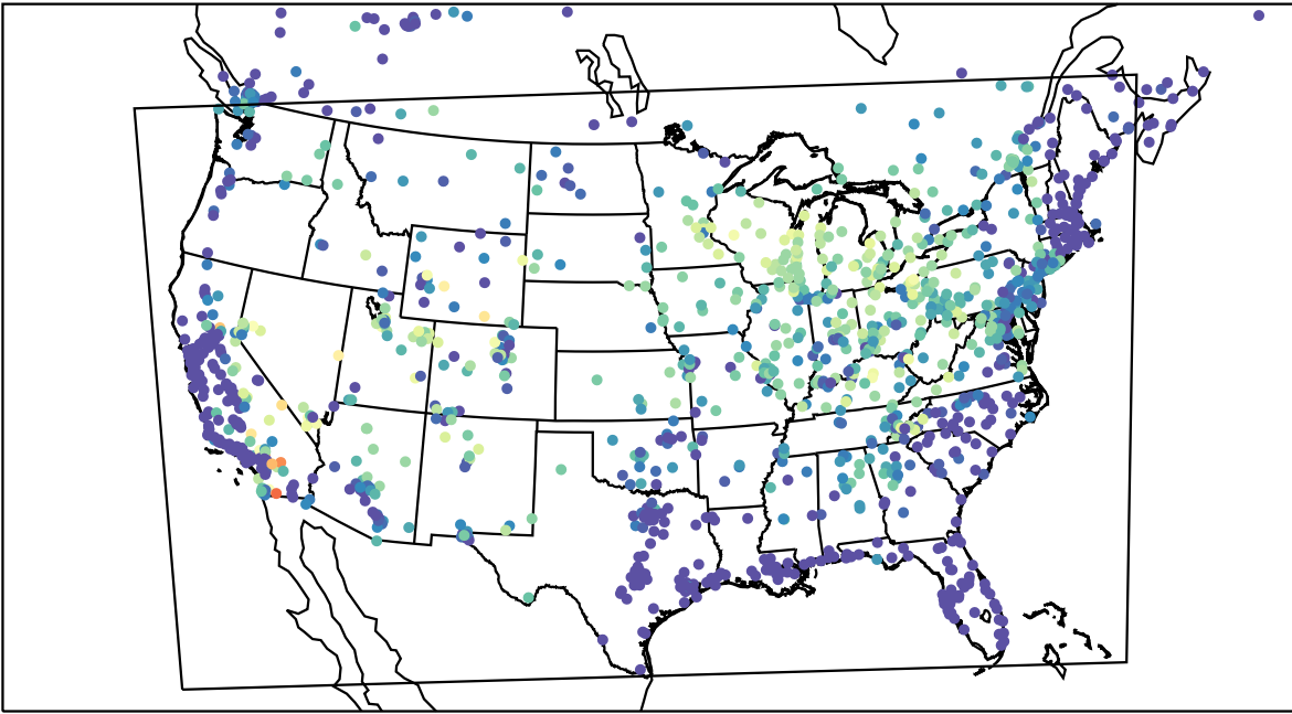
AirNOW (2023-07-10_13:00:00)
