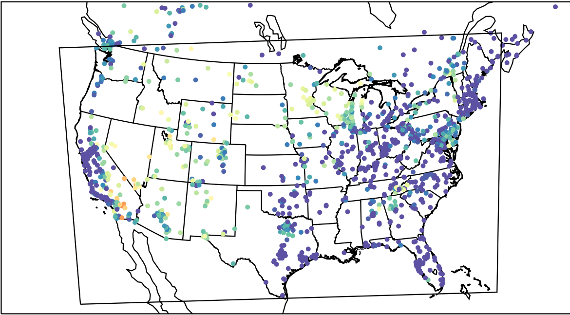
AirNOW (2023-07-10_07:00:00)
