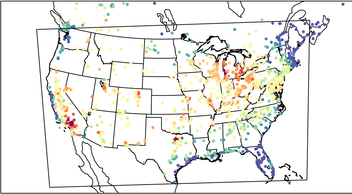
AirNOW (2023-07-10_22:00:00)
