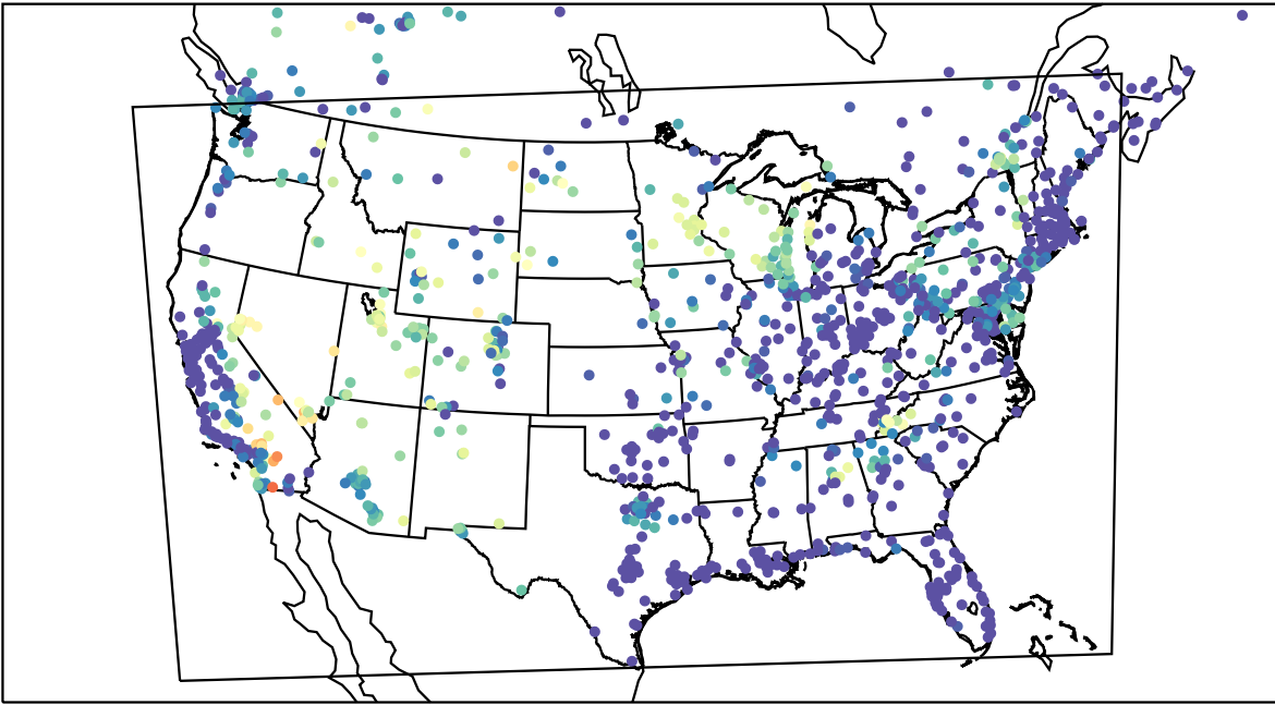
AirNOW (2023-07-10_08:00:00)
