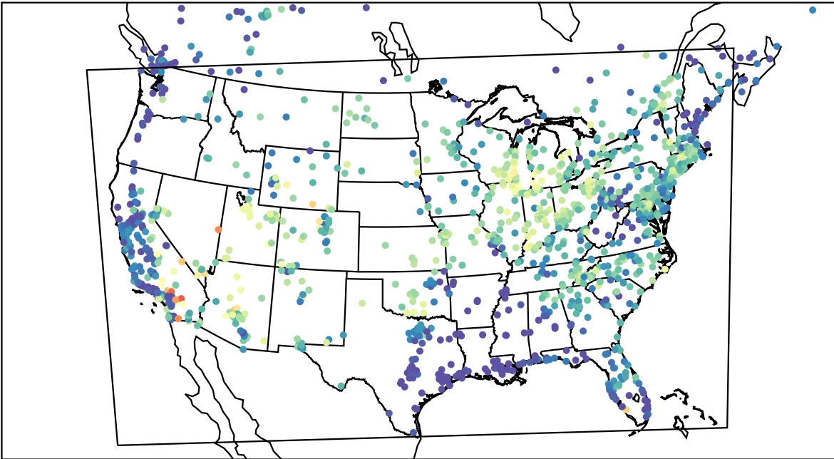
AirNOW (2023-07-09_14:00:00)
