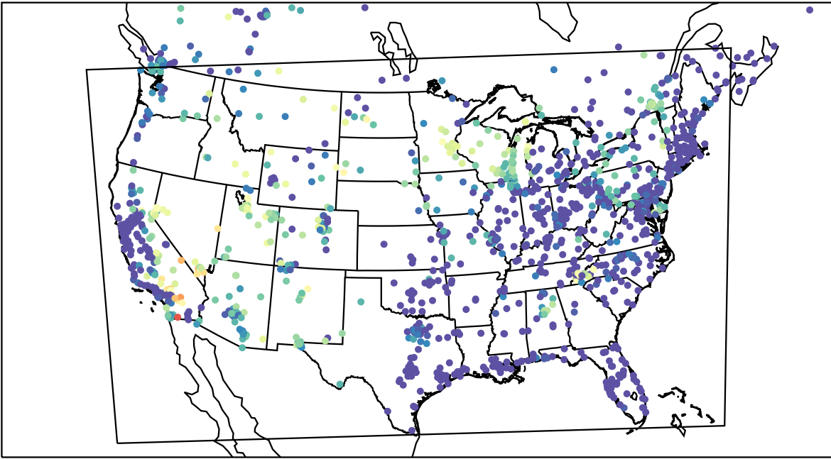
AirNOW (2023-07-10_09:00:00)
