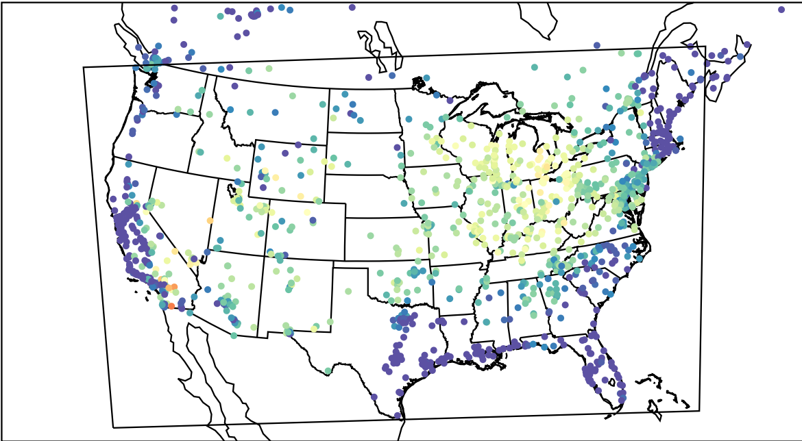
AirNOW (2023-07-10_14:00:00)
