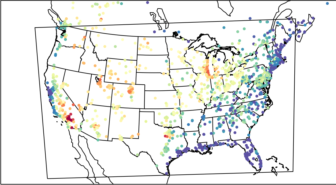
AirNOW (2023-07-10_00:00:00)
