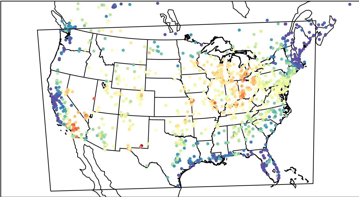
AirNOW (2023-07-10_17:00:00)
