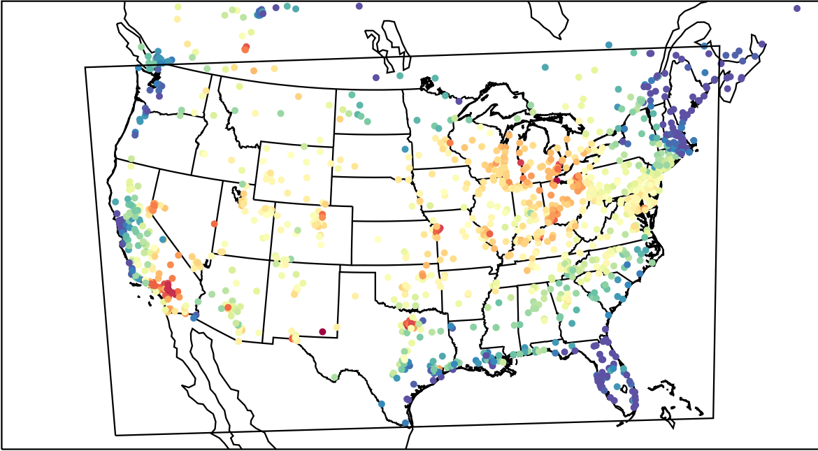
AirNOW (2023-07-10_19:00:00)
