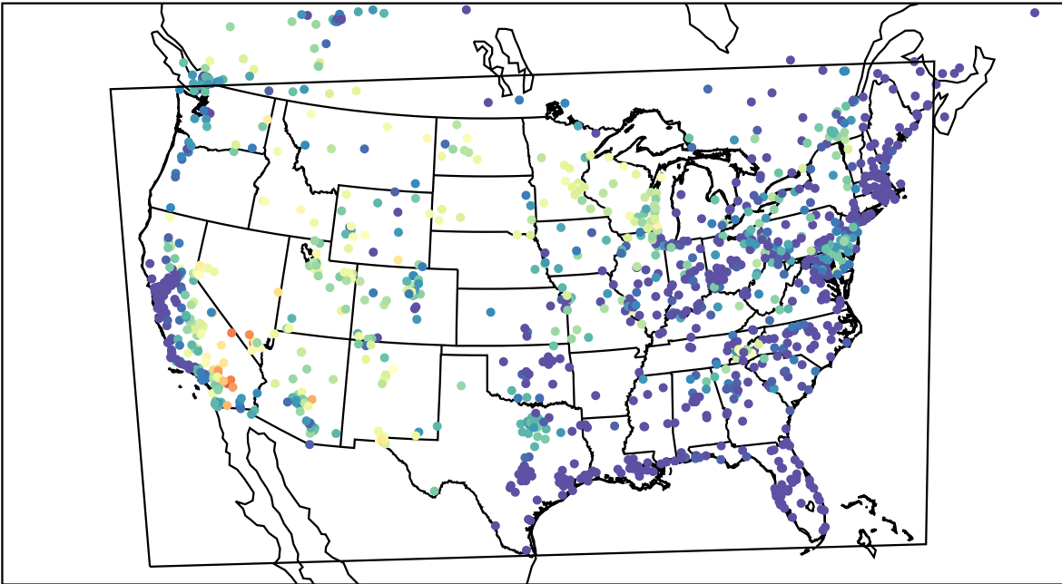
AirNOW (2023-07-10_05:00:00)
