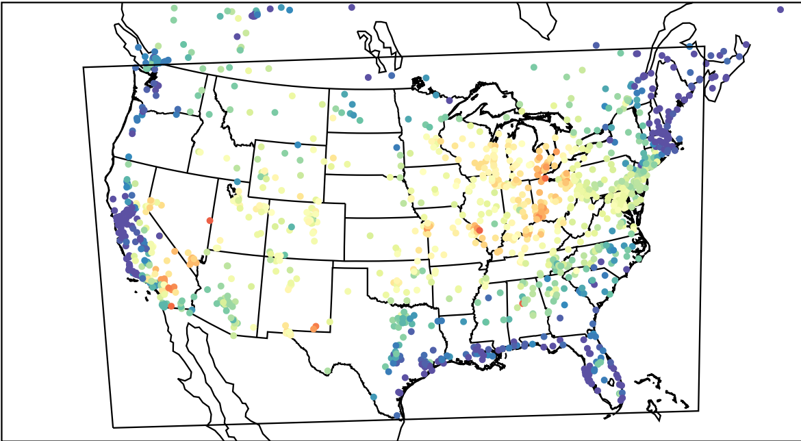
AirNOW (2023-07-10_16:00:00)
