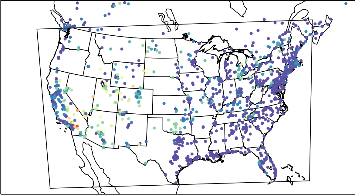
AirNOW (2023-07-09_10:00:00)
