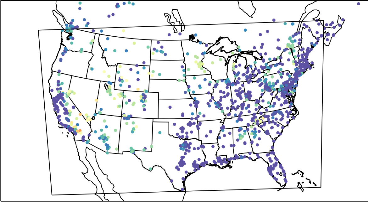
AirNOW (2023-07-10_10:00:00)
