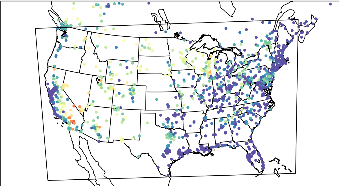
AirNOW (2023-07-10_04:00:00)
