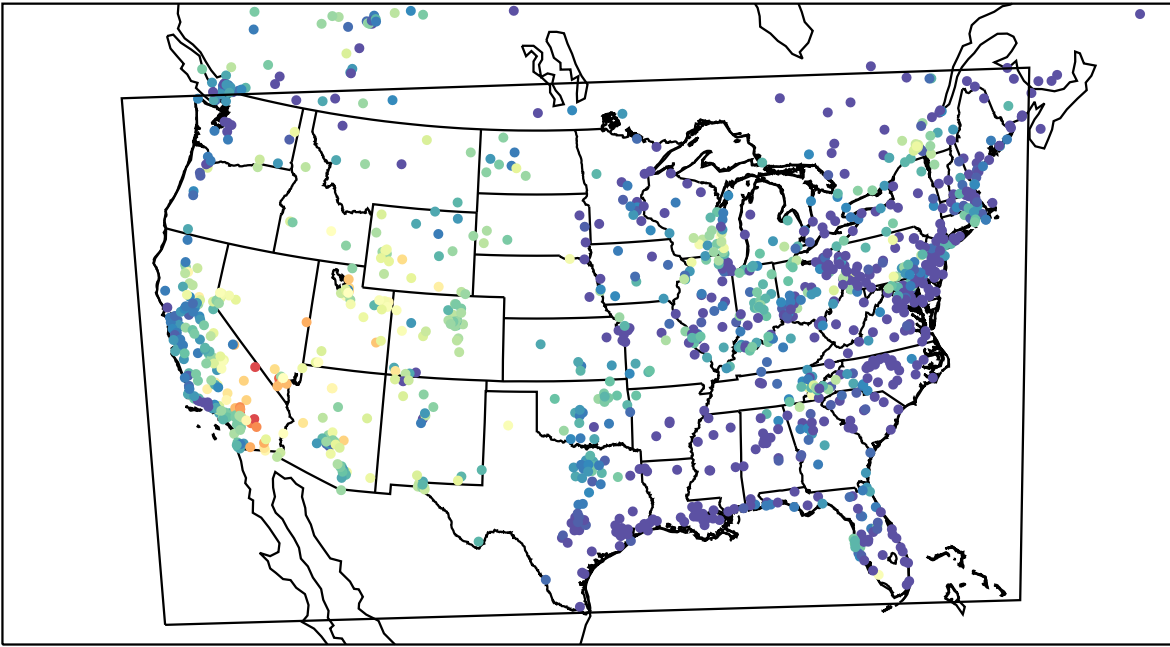
AirNOW (2023-07-09_05:00:00)
