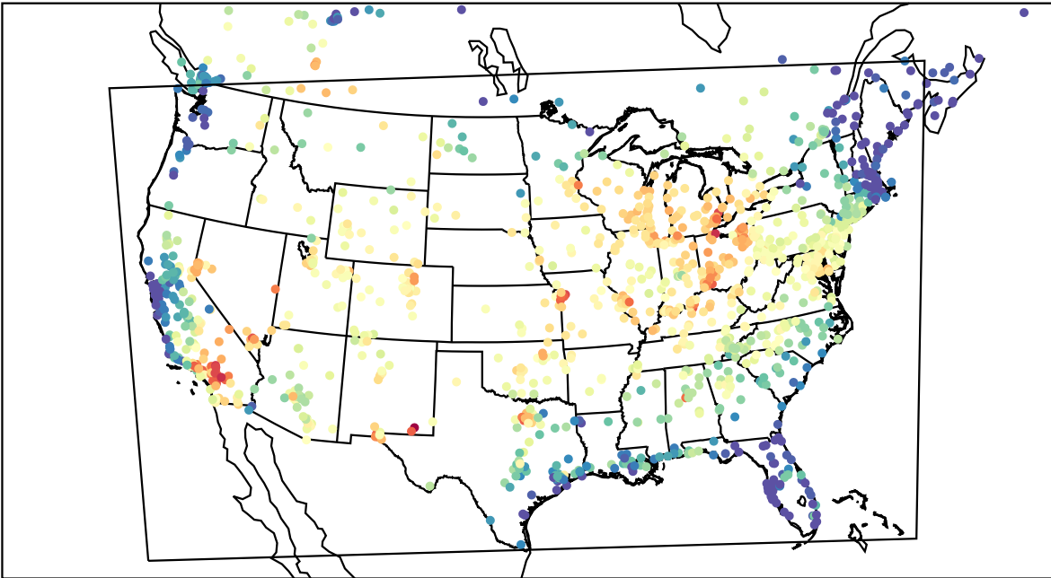
AirNOW (2023-07-10_18:00:00)
