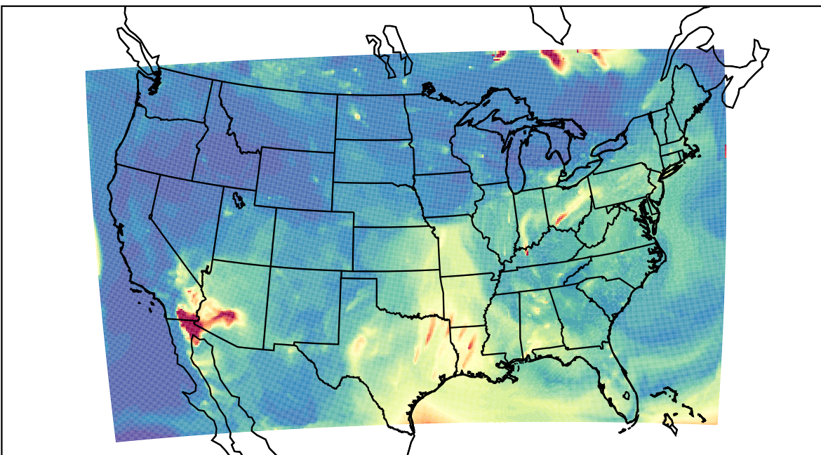
WRF 2023-07-12_11:00:00
