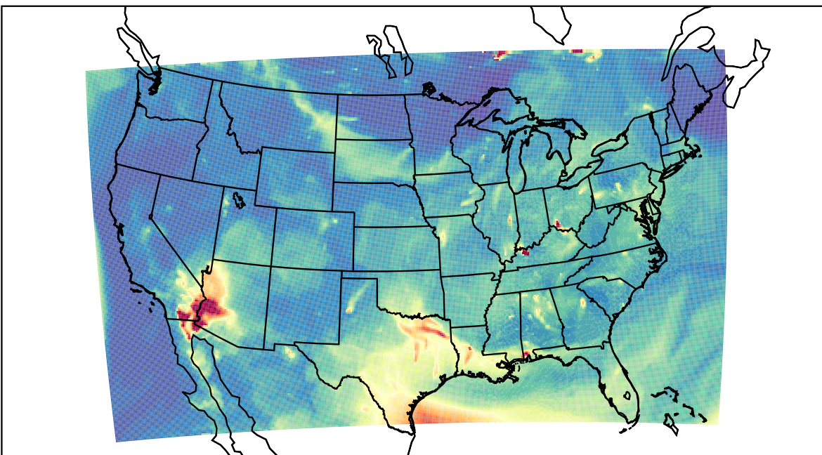
WRF 2023-07-11_07:00:00
