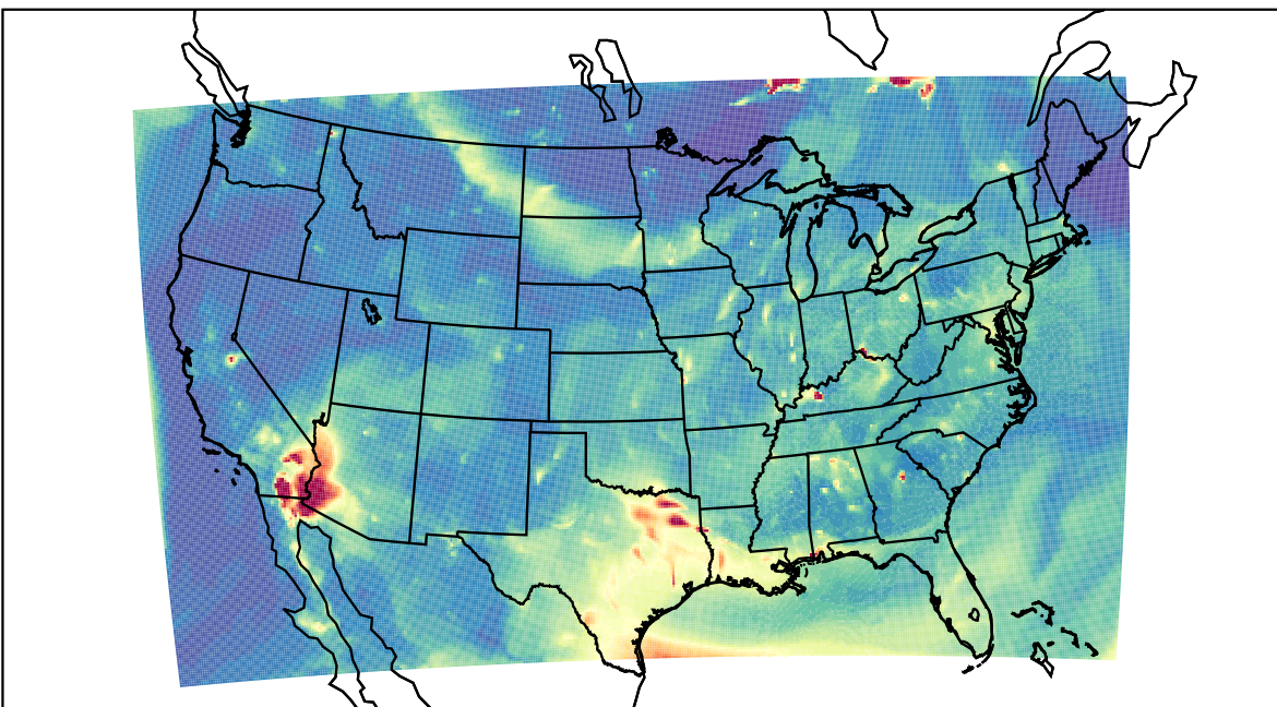
WRF 2023-07-11_04:00:00
