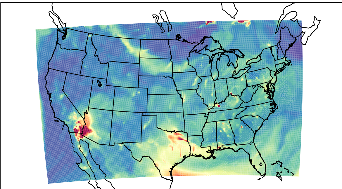
WRF 2023-07-11_05:00:00
