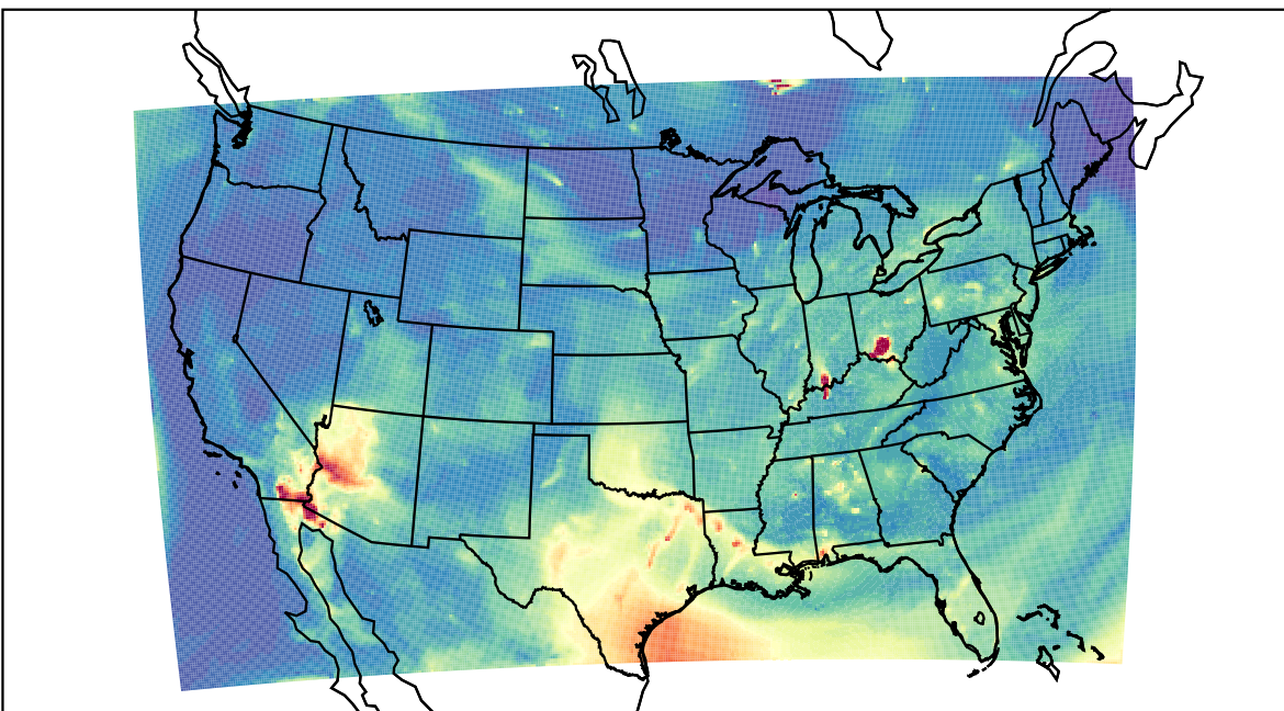
WRF 2023-07-11_12:00:00
