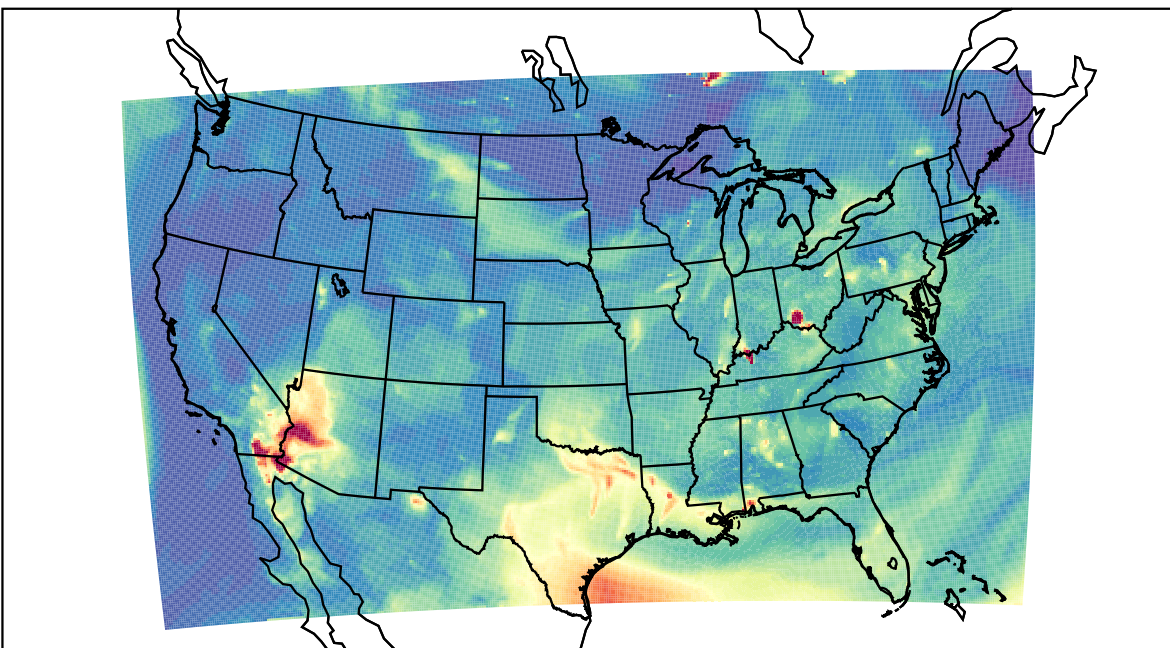
WRF 2023-07-11_09:00:00
