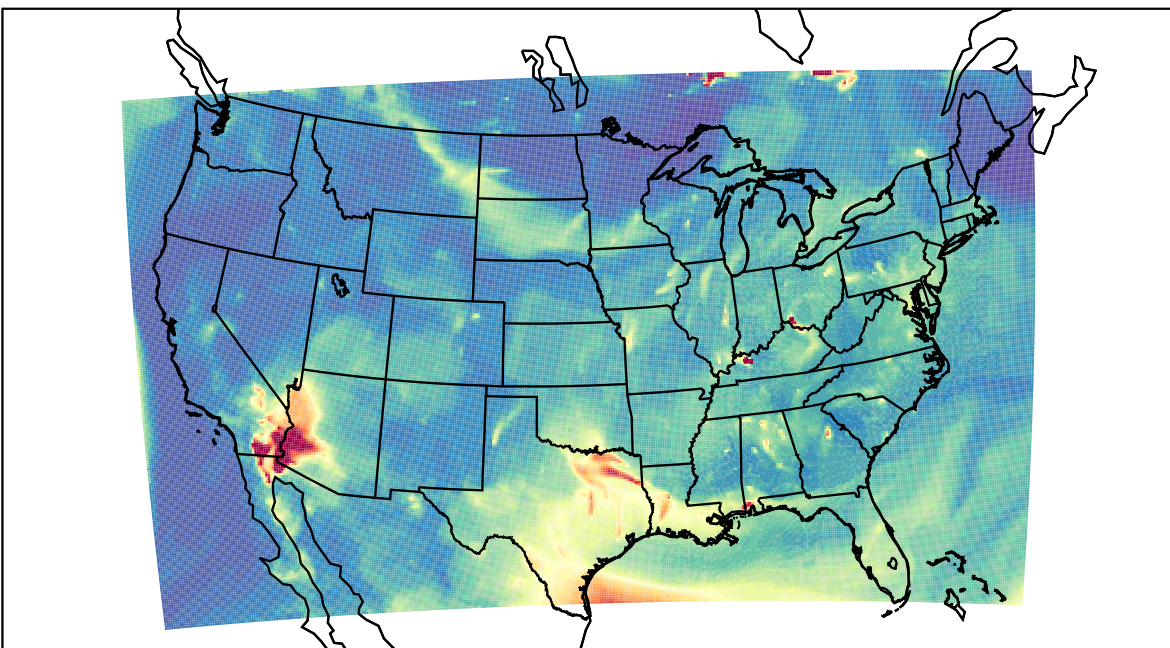
WRF 2023-07-11_06:00:00
