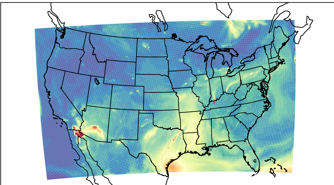
WRF 2023-07-12_15:00:00
