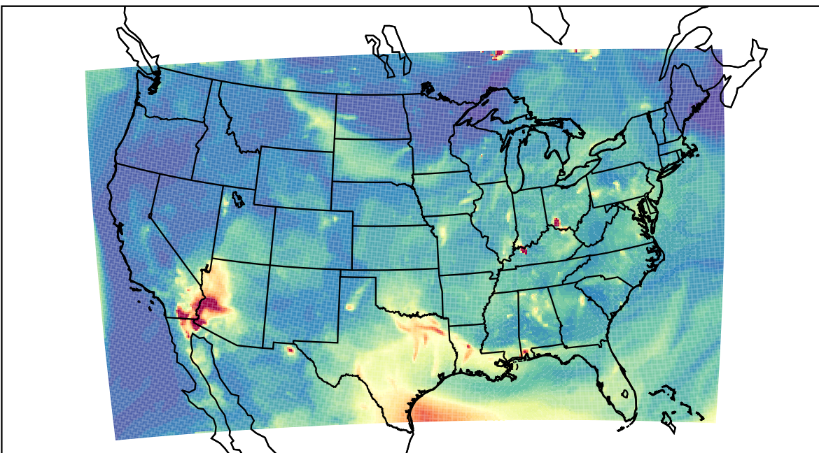
WRF 2023-07-11_08:00:00
