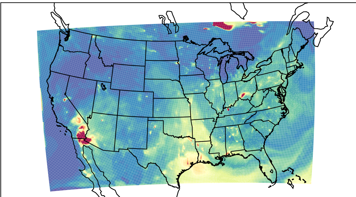
WRF 2023-07-12_03:00:00
