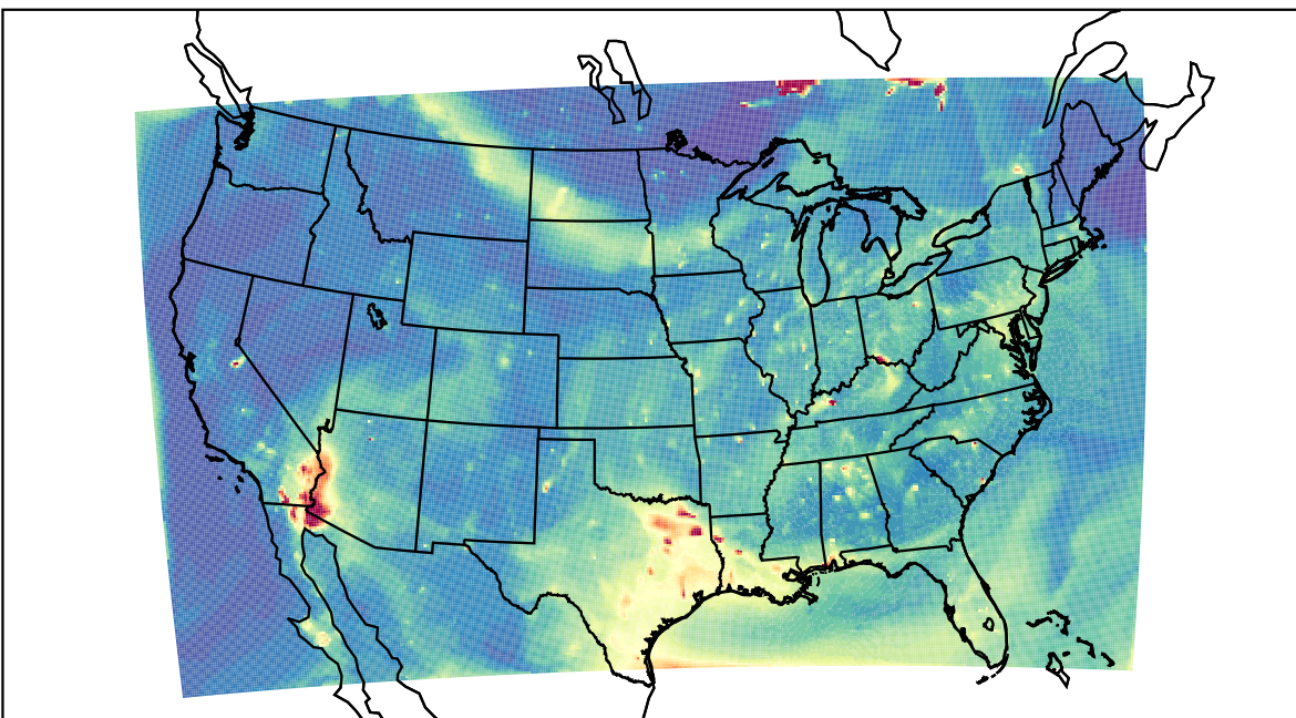
WRF 2023-07-11_02:00:00
