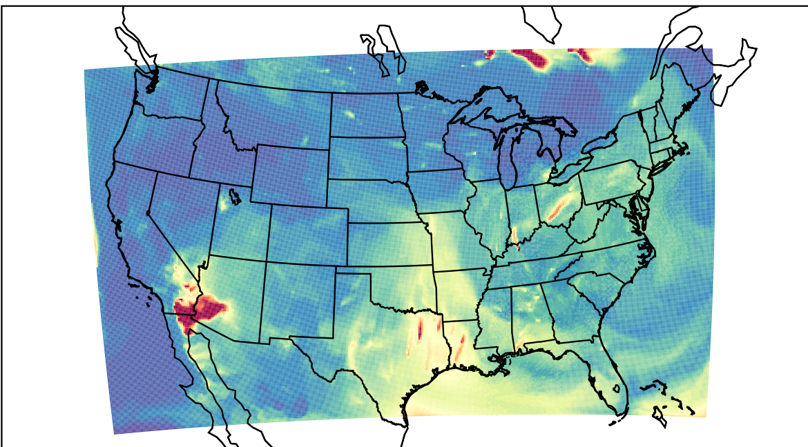
WRF 2023-07-12_08:00:00
