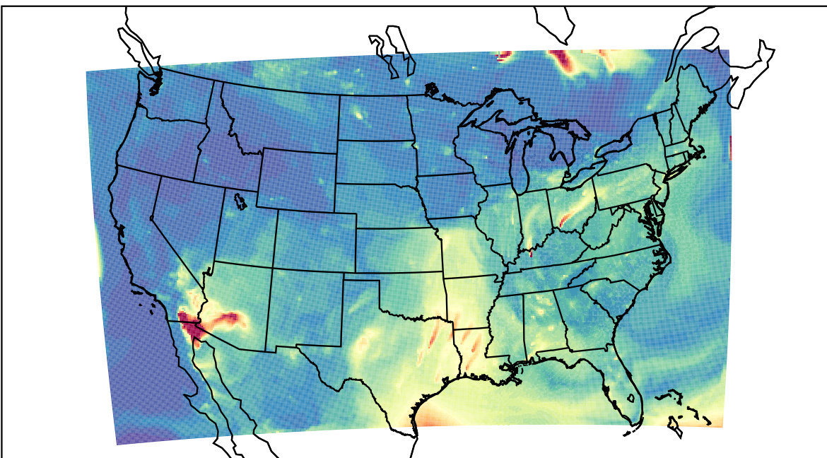
WRF 2023-07-12_12:00:00
