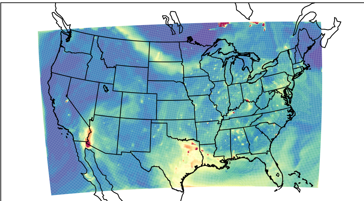
WRF 2023-07-11_01:00:00
