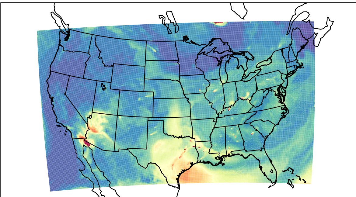
WRF 2023-07-11_15:00:00
