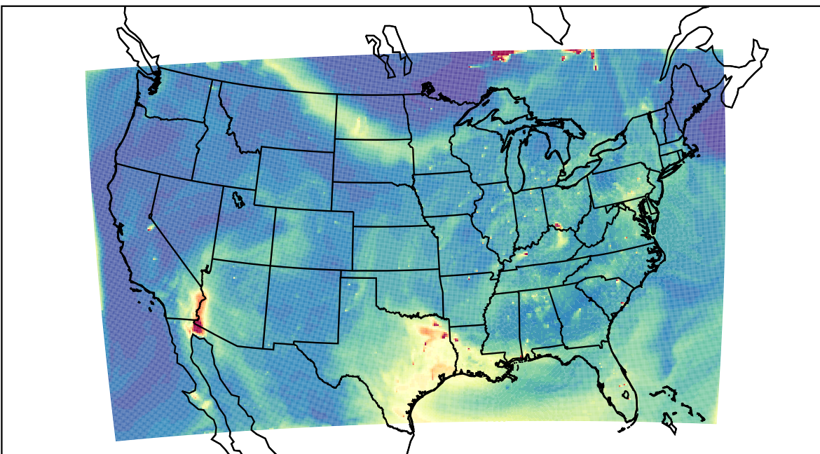
WRF 2023-07-11_00:00:00
