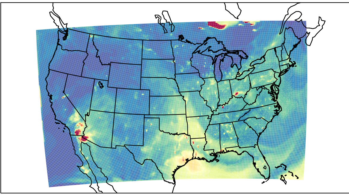
WRF 2023-07-12_02:00:00
