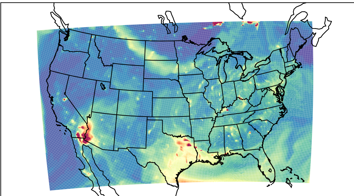
WRF 2023-07-11_03:00:00
