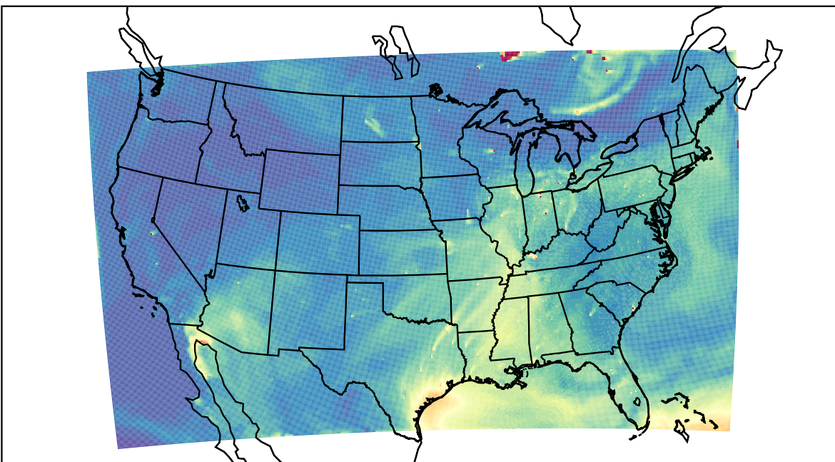
WRF 2023-07-12_21:00:00
