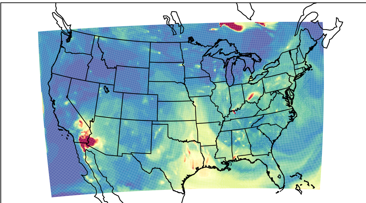
WRF 2023-07-12_05:00:00
