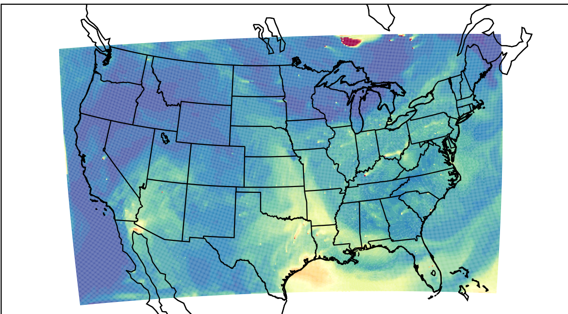
WRF 2023-07-11_22:00:00
