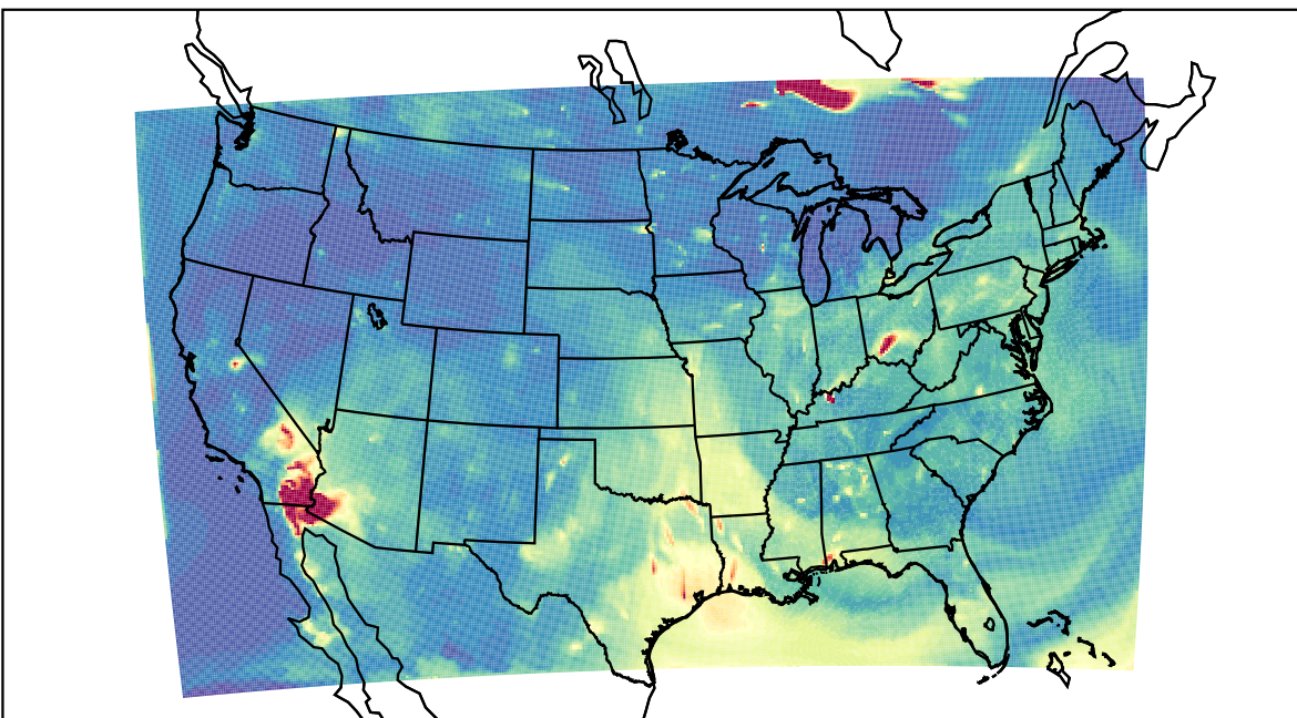
WRF 2023-07-12_04:00:00
