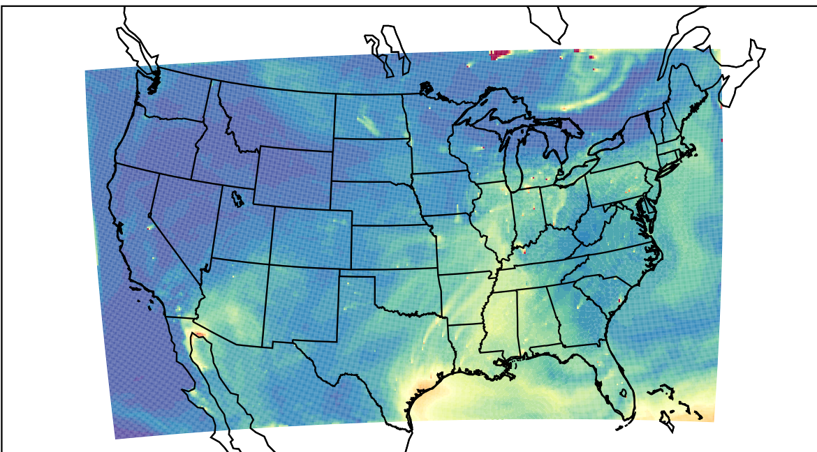
WRF 2023-07-12_22:00:00
