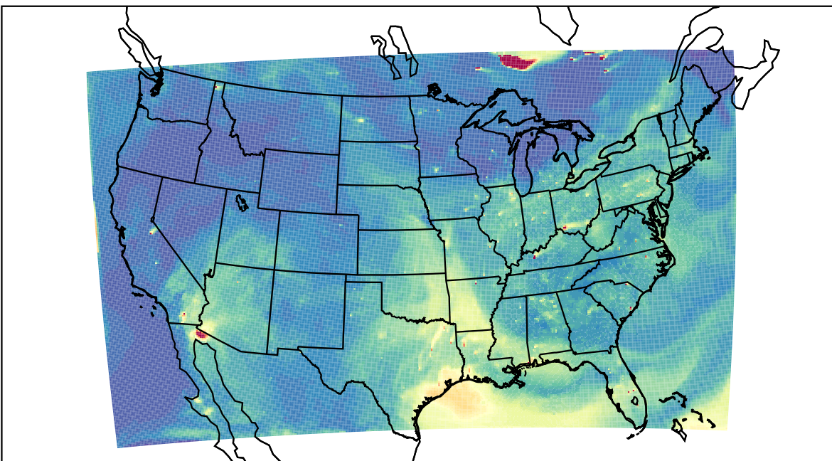
WRF 2023-07-12_00:00:00
