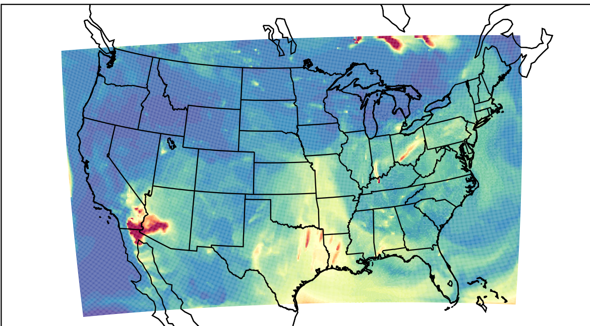
WRF 2023-07-12_09:00:00
