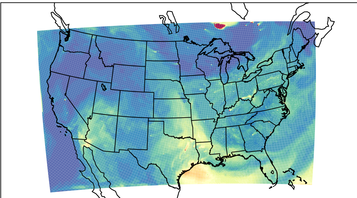
WRF 2023-07-11_21:00:00
