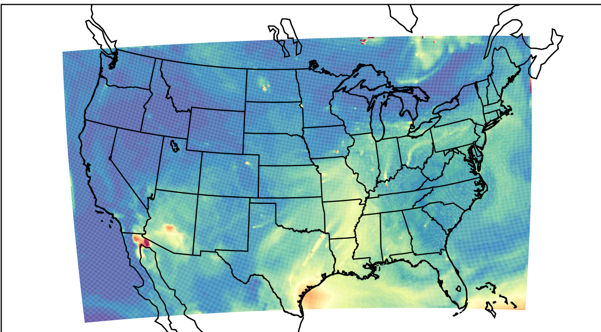
WRF 2023-07-12_17:00:00
