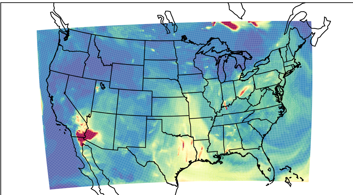
WRF 2023-07-12_07:00:00
