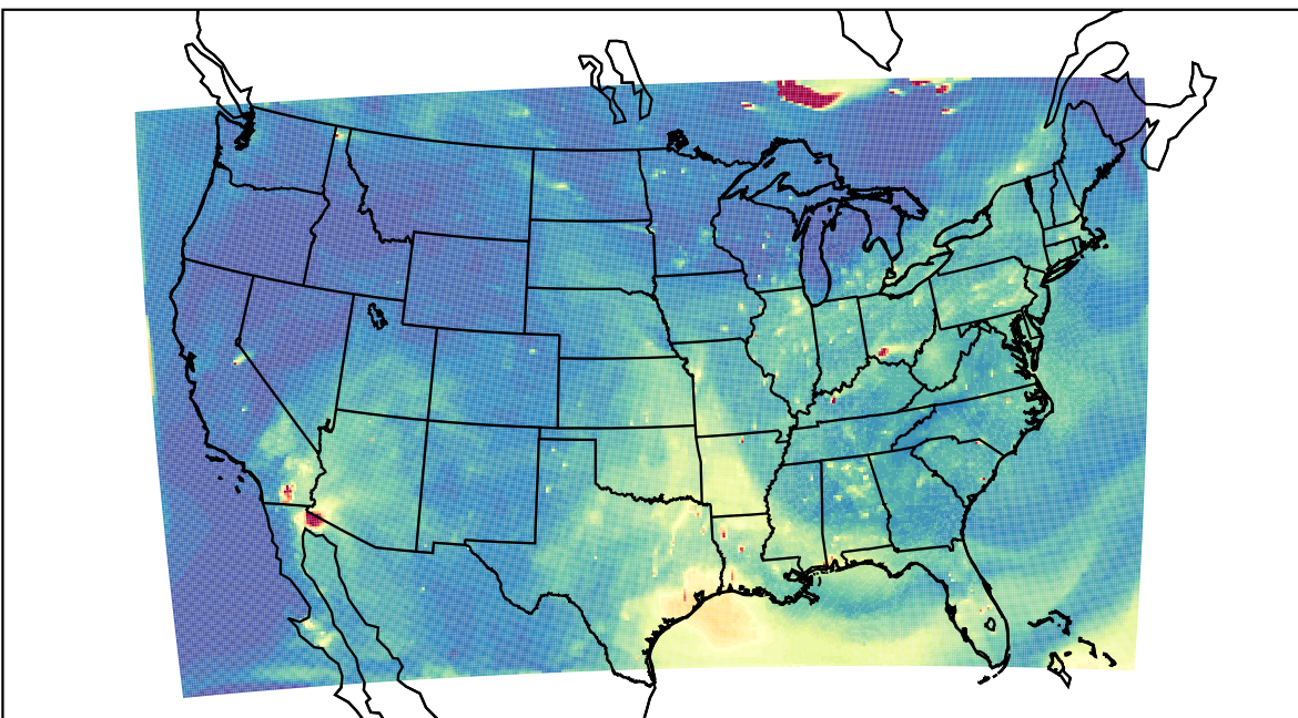
WRF 2023-07-12_01:00:00
