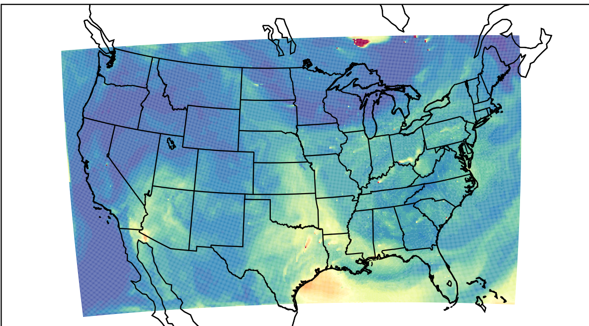
WRF 2023-07-11_20:00:00
