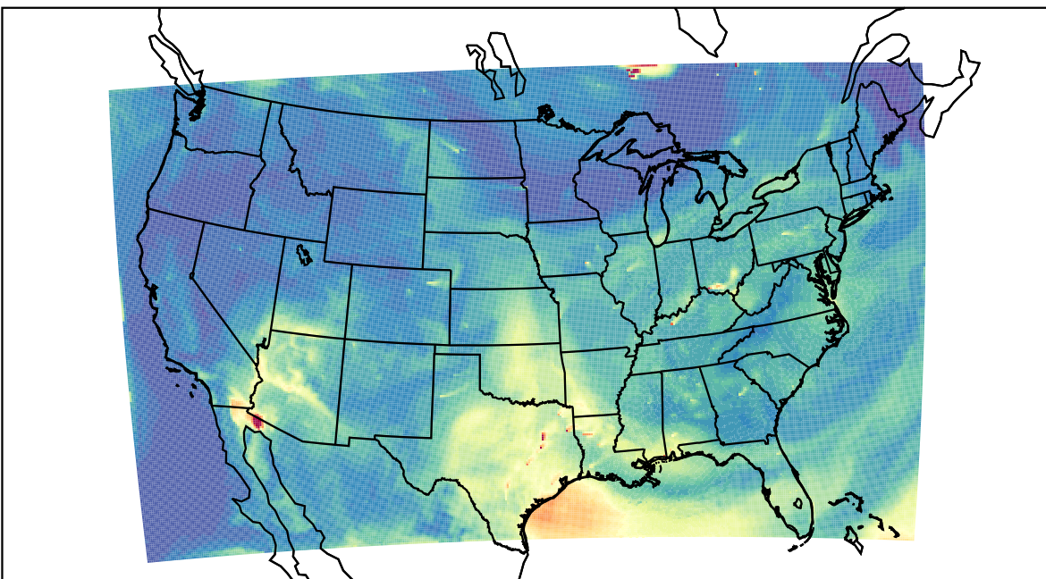
WRF 2023-07-11_17:00:00
