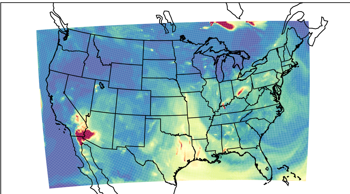
WRF 2023-07-12_06:00:00
