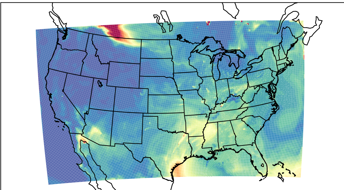
WRF 2023-07-13_19:00:00
