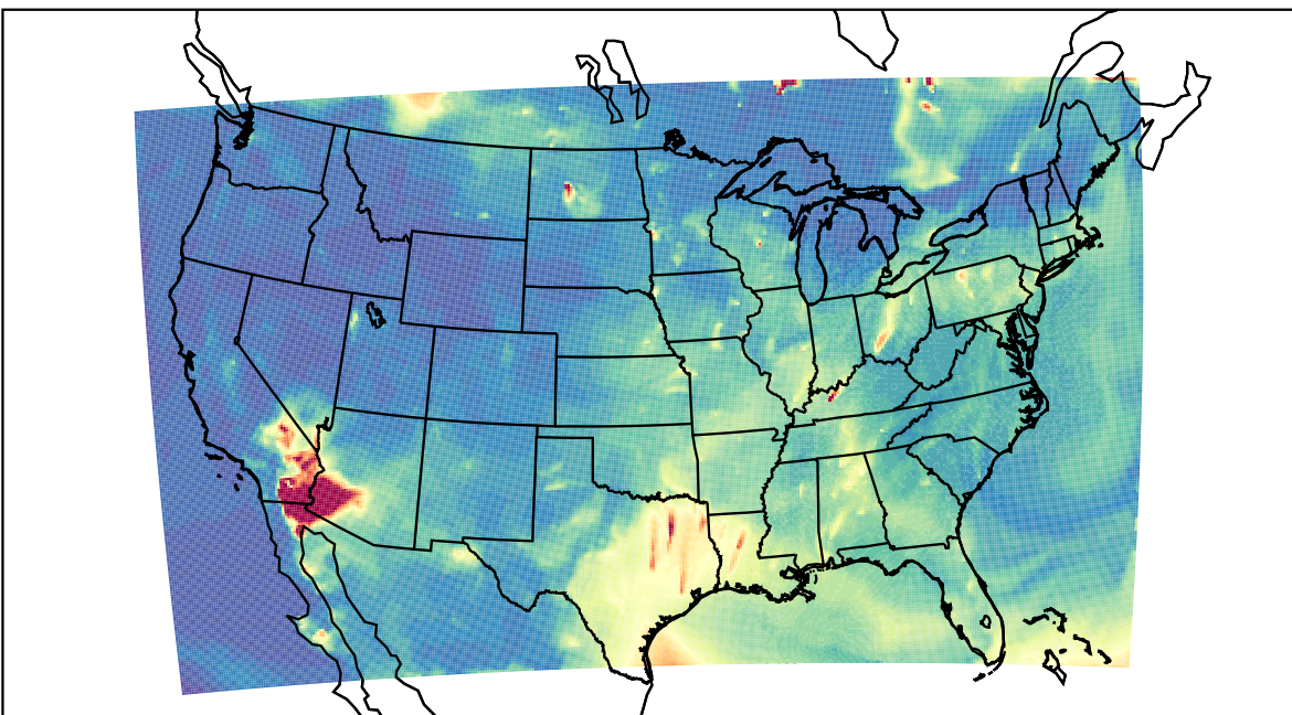
WRF 2023-07-13_07:00:00
