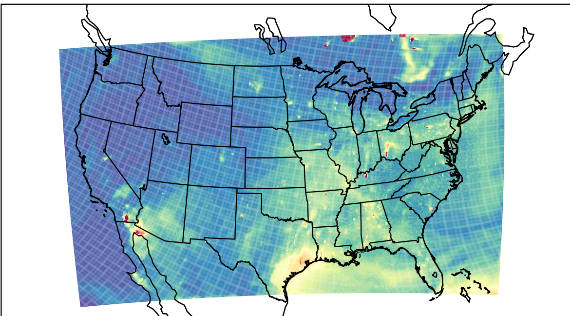
WRF 2023-07-13_01:00:00
