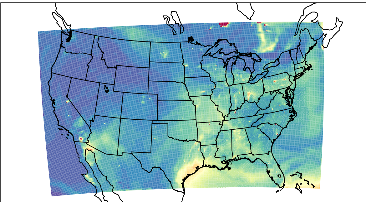
WRF 2023-07-13_00:00:00
