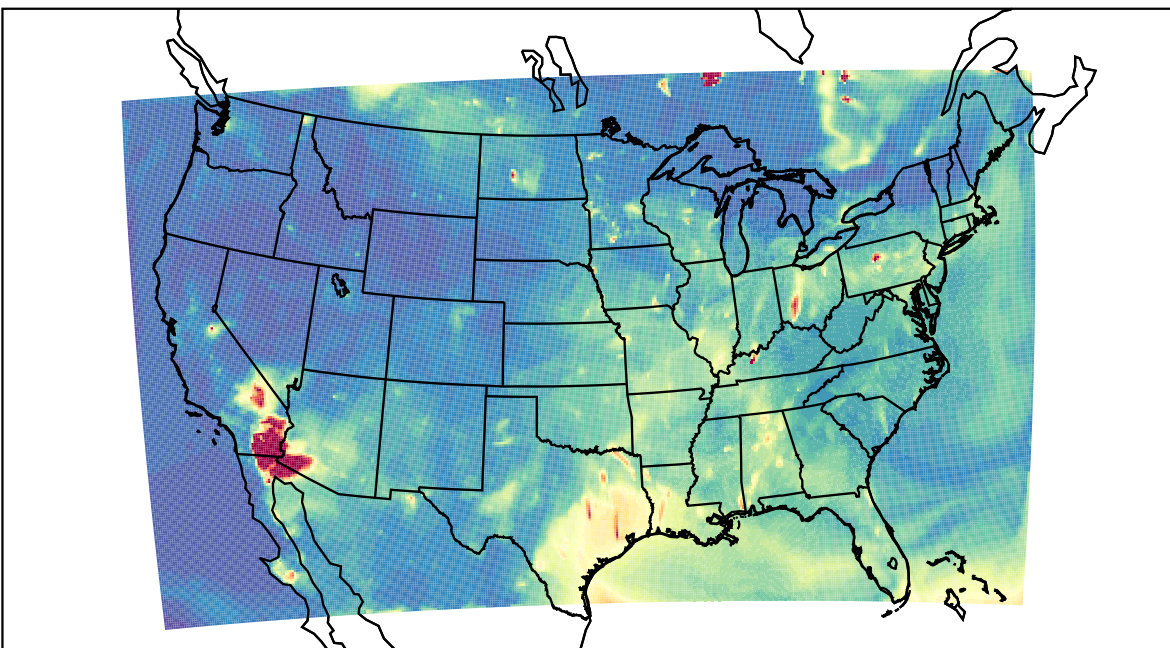
WRF 2023-07-13_04:00:00
