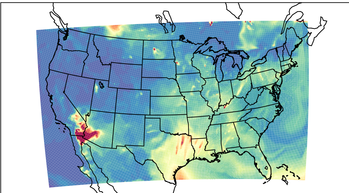
WRF 2023-07-13_09:00:00
