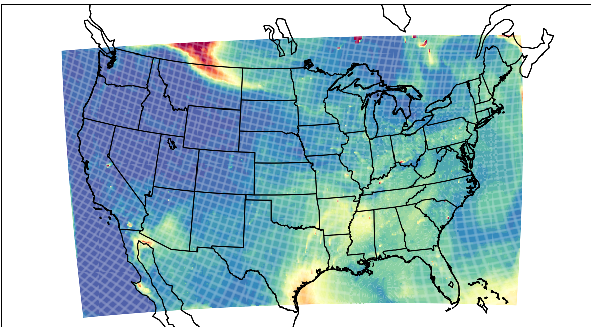
WRF 2023-07-13_23:00:00
