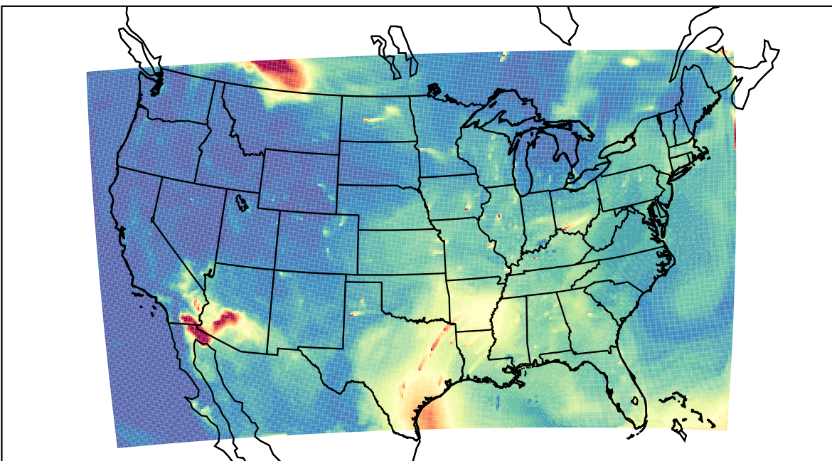
WRF 2023-07-13_15:00:00
