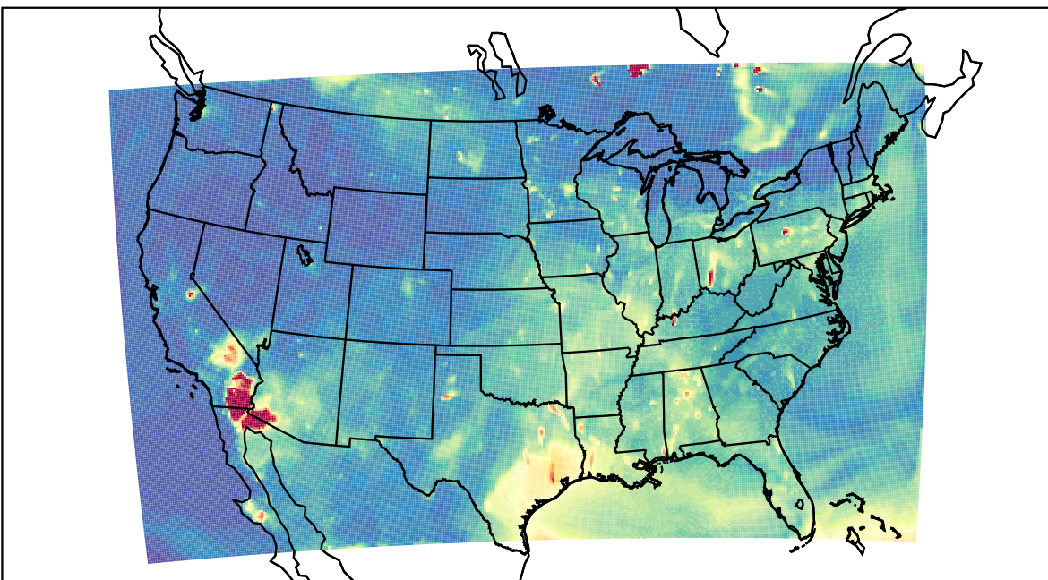
WRF 2023-07-13_03:00:00
