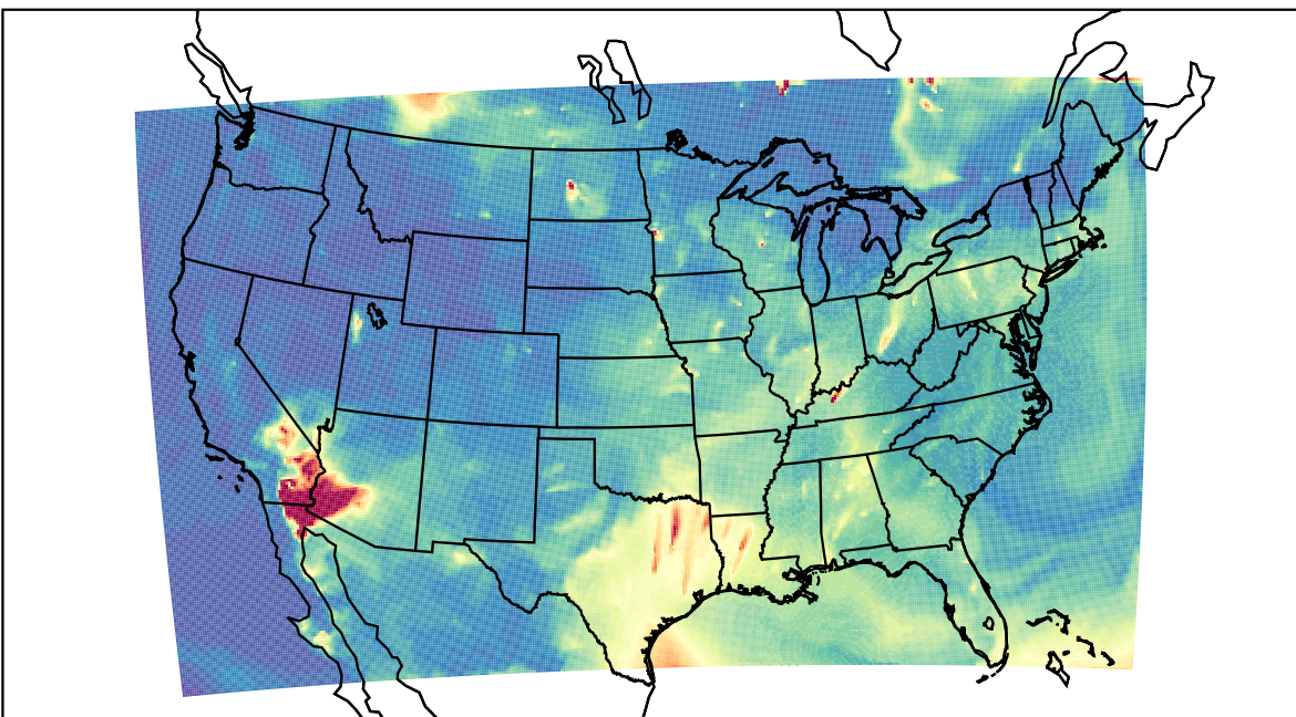
WRF 2023-07-13_08:00:00
