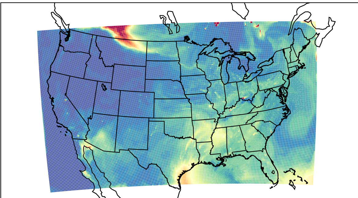
WRF 2023-07-13_22:00:00
