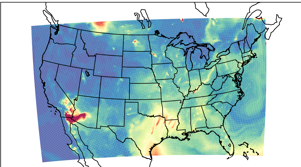
WRF 2023-07-13_11:00:00
