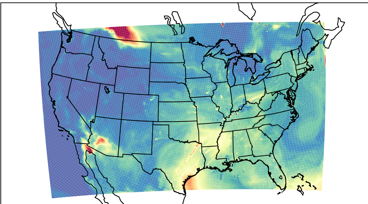
WRF 2023-07-13_17:00:00
