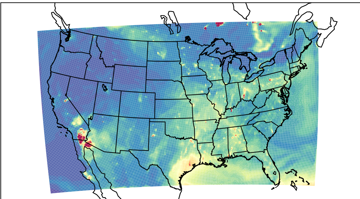
WRF 2023-07-13_02:00:00
