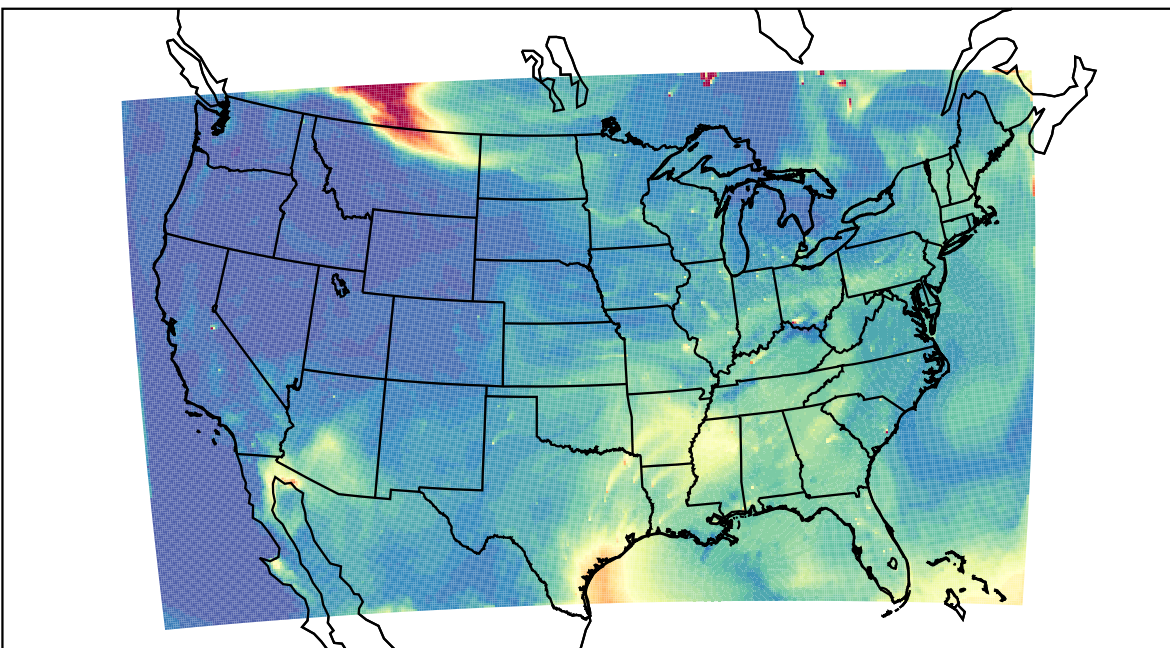
WRF 2023-07-13_21:00:00
