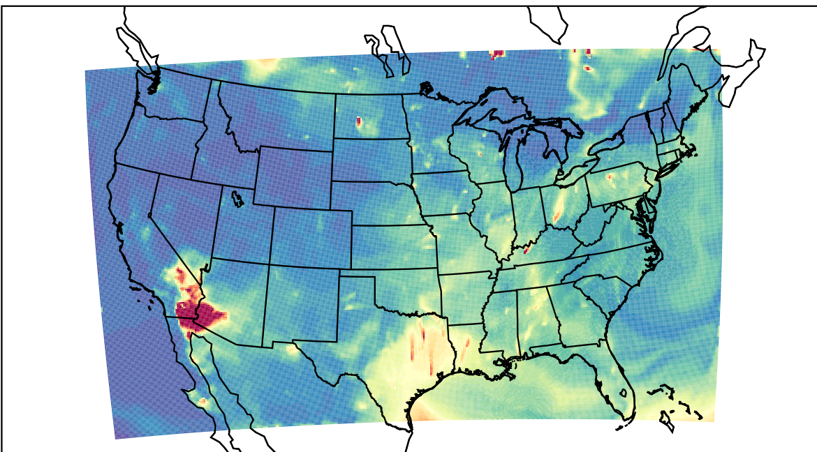
WRF 2023-07-13_06:00:00
