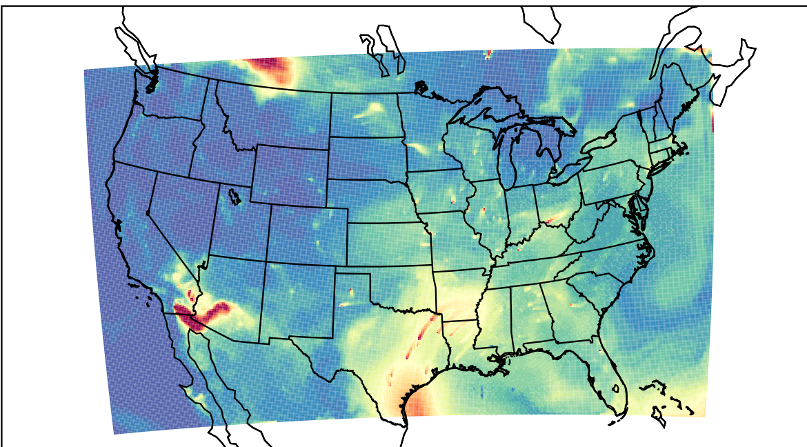
WRF 2023-07-13_14:00:00
