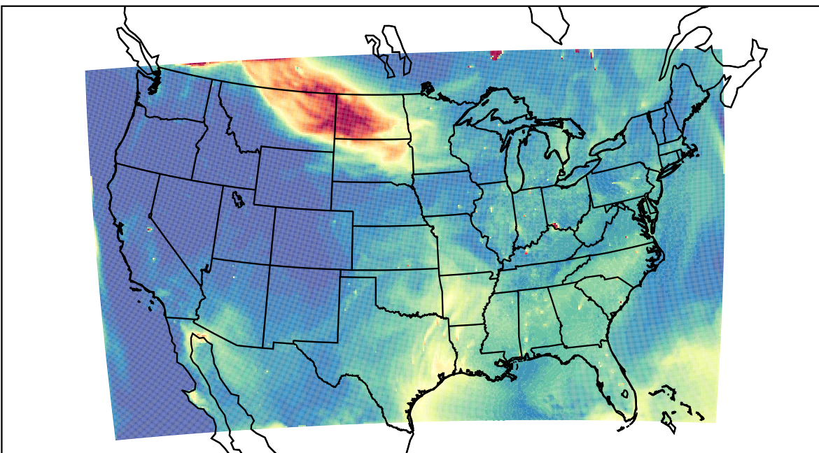
WRF 2023-07-14_22:00:00
