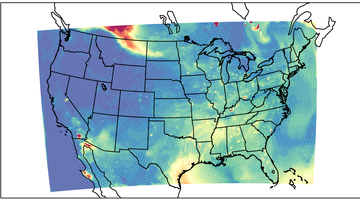
WRF 2023-07-14_01:00:00
