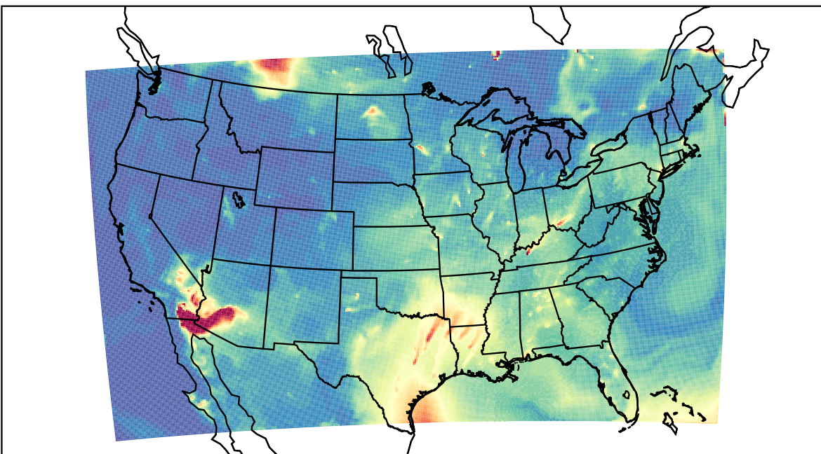
WRF 2023-07-13_12:00:00
