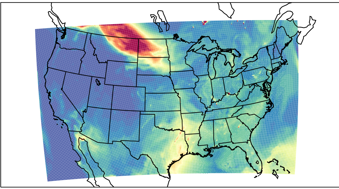
WRF 2023-07-14_19:00:00
