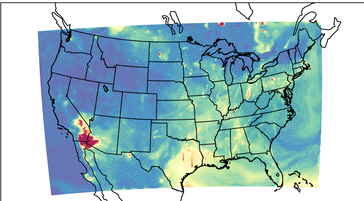
WRF 2023-07-13_05:00:00
