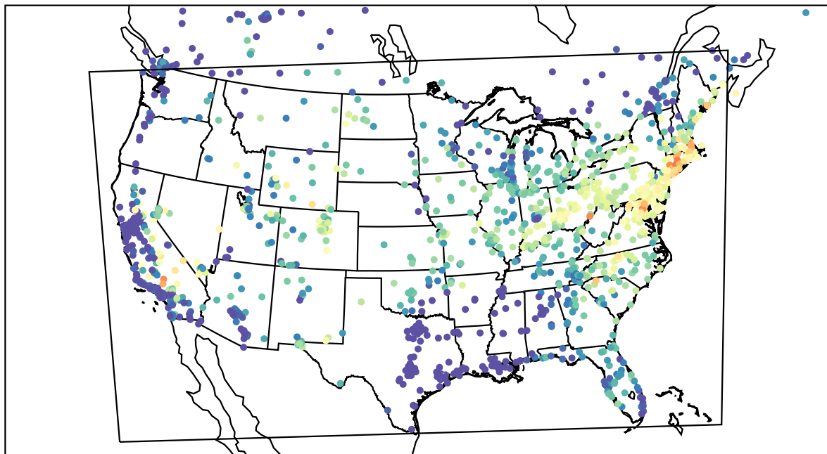
AirNOW (2023-07-13_14:00:00)
