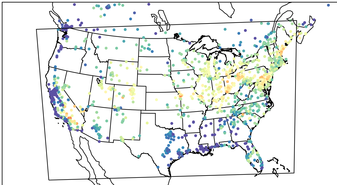
AirNOW (2023-07-14_15:00:00)
