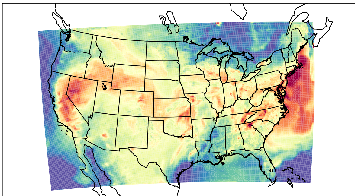
WRF (2023-07-13_00:00:00)
