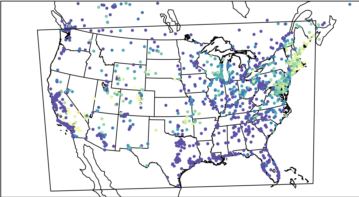
AirNOW (2023-07-14_12:00:00)
