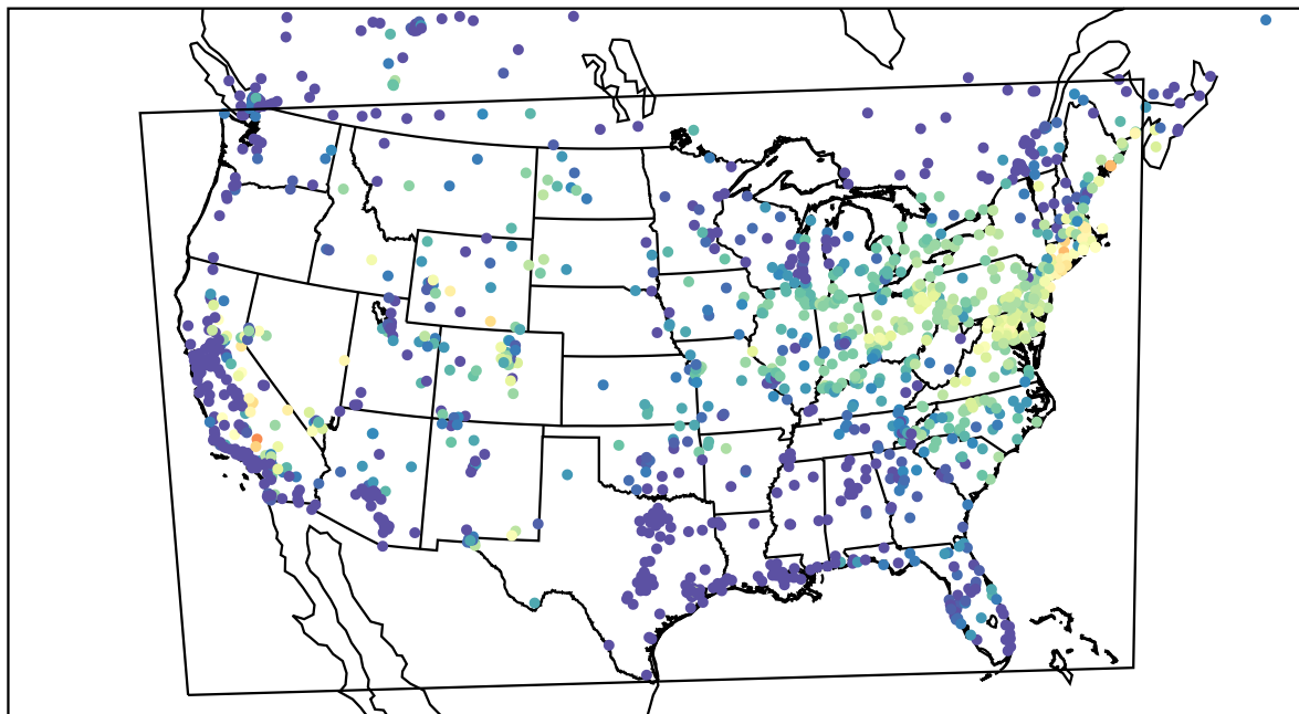
AirNOW (2023-07-13_13:00:00)
