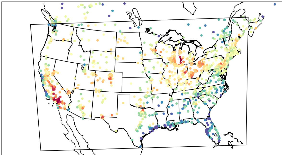
AirNOW (2023-07-14_21:00:00)
