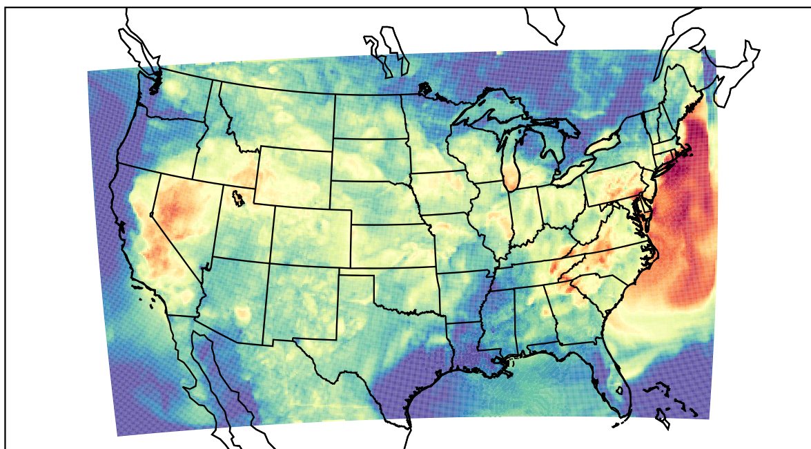
WRF (2023-07-13_03:00:00)
