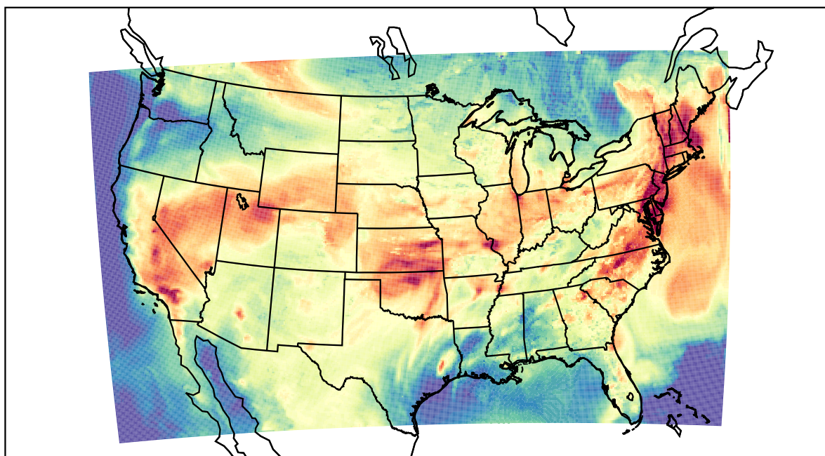
WRF (2023-07-13_22:00:00)
