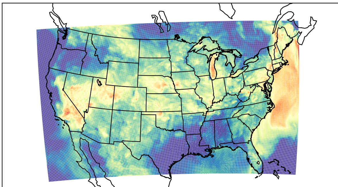
WRF (2023-07-14_05:00:00)
