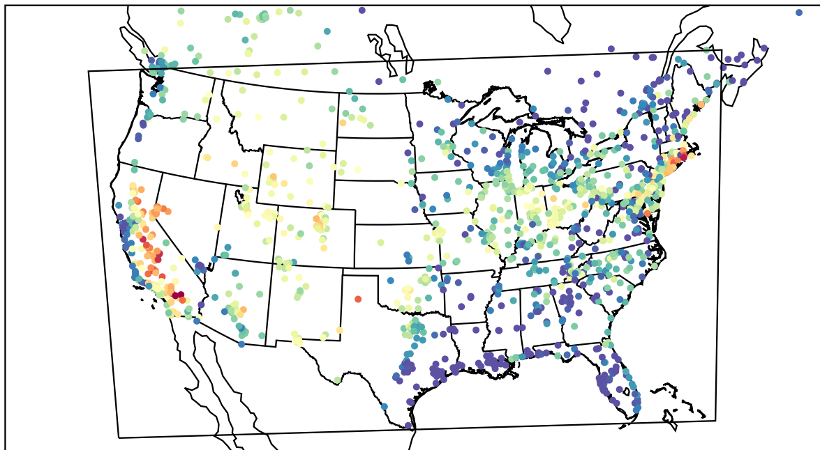
AirNOW (2023-07-13_02:00:00)
