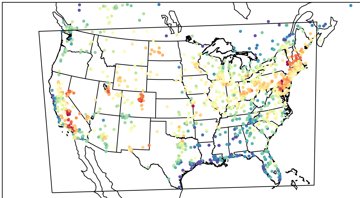
AirNOW (2023-07-13_20:00:00)
