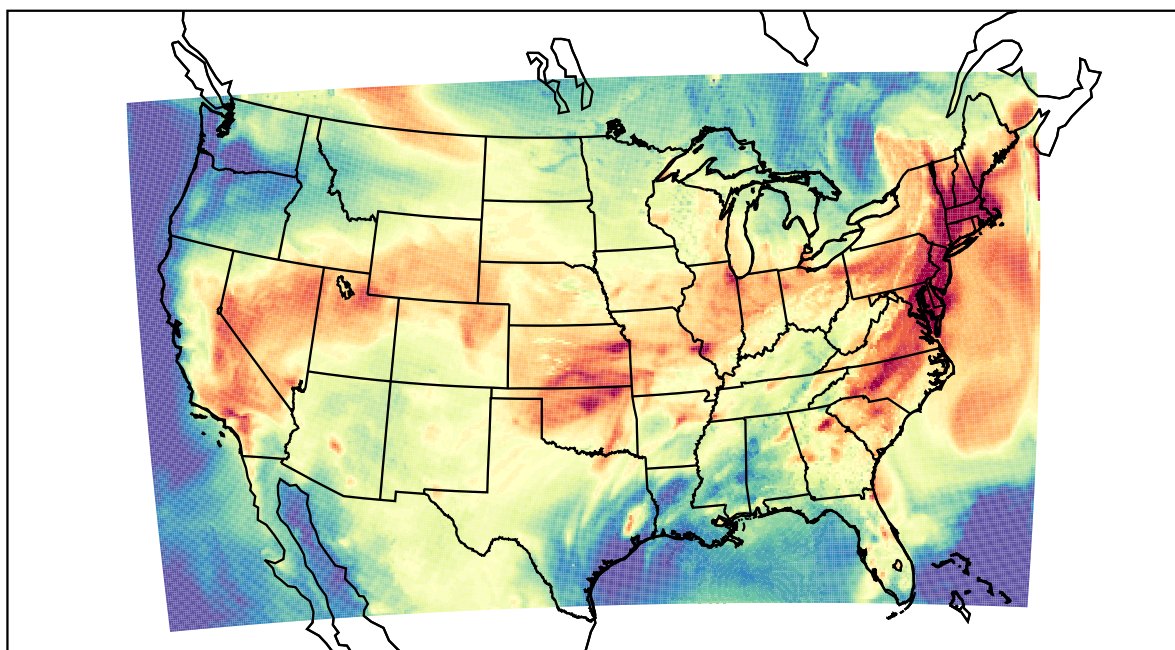
WRF (2023-07-13_20:00:00)
