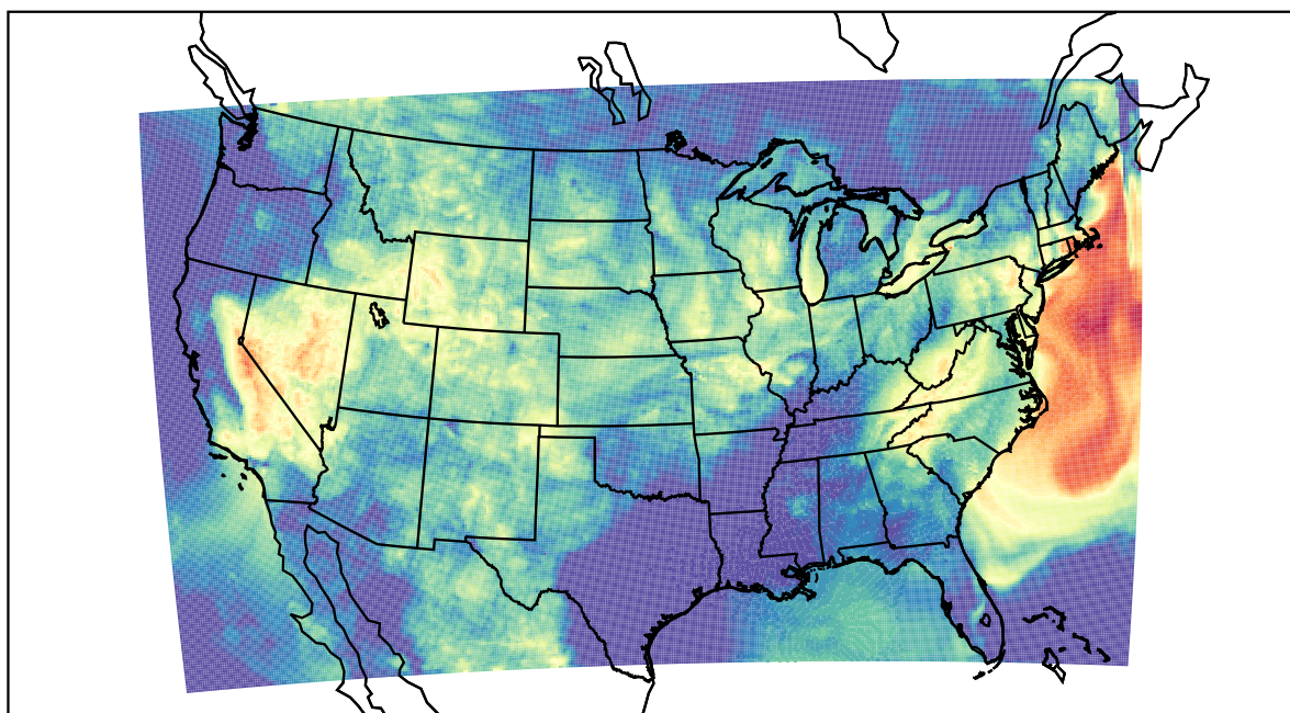
WRF (2023-07-13_09:00:00)
