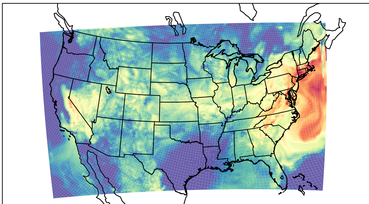
WRF (2023-07-13_14:00:00)
