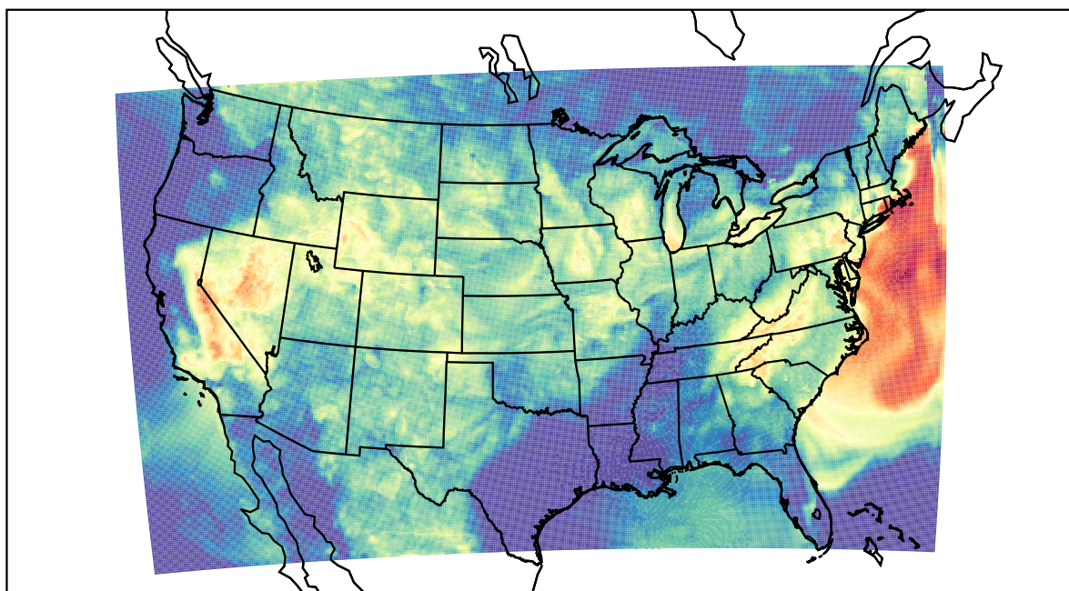
WRF (2023-07-13_07:00:00)
