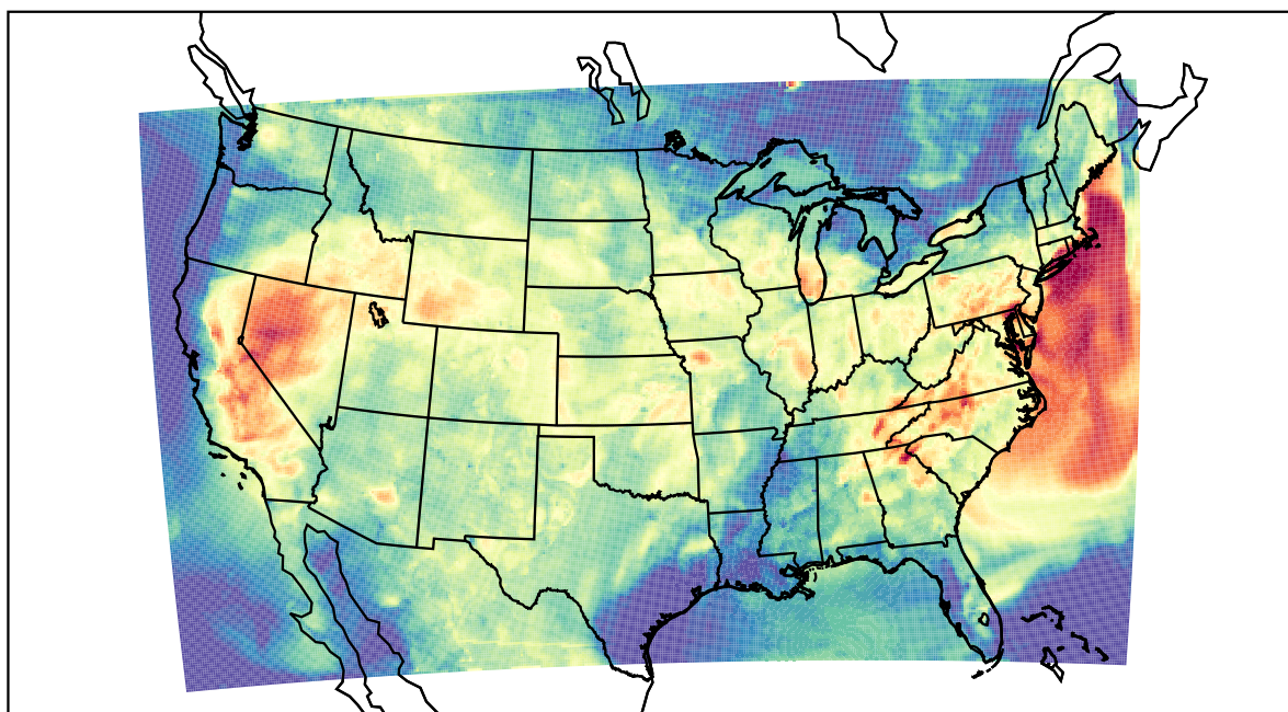
WRF (2023-07-13_02:00:00)
