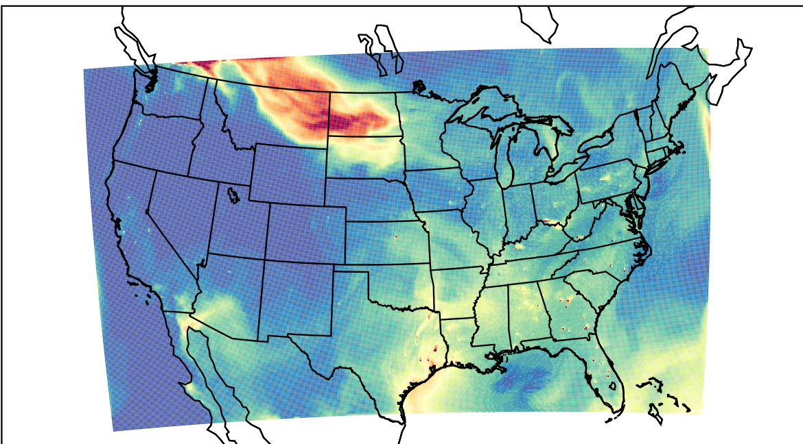
WRF 2023-07-14_21:00:00
