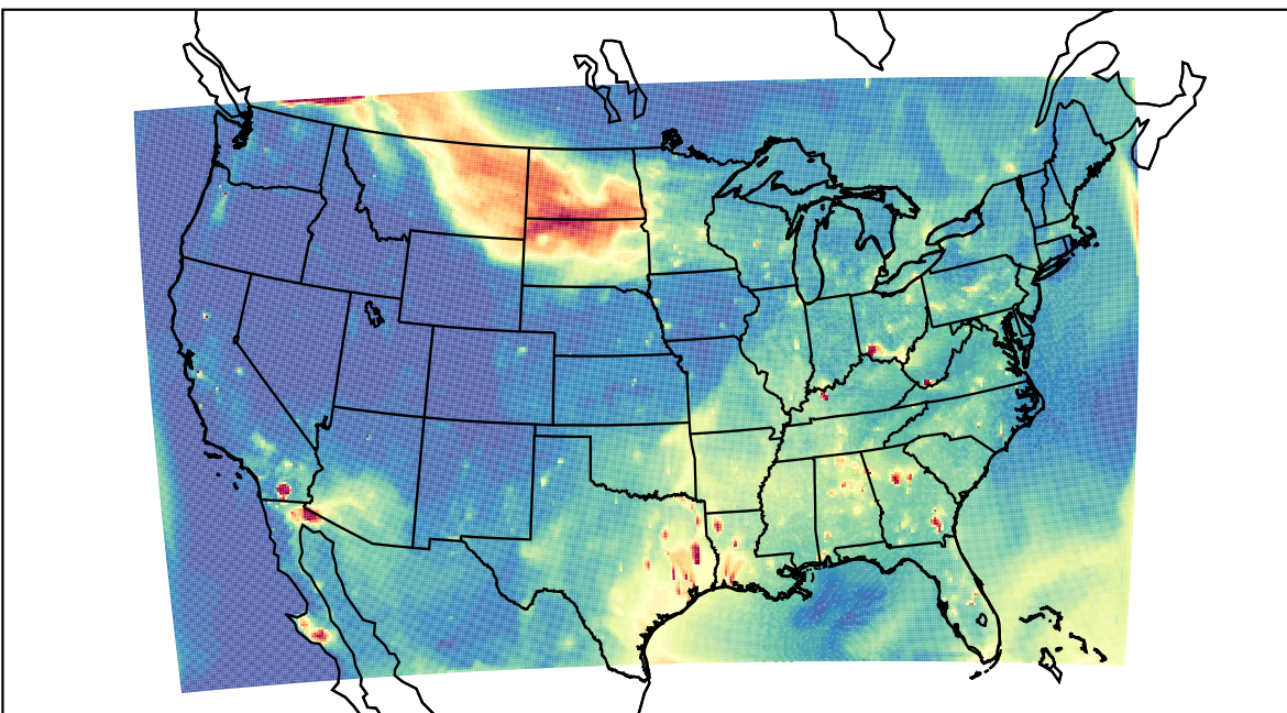
WRF 2023-07-15_02:00:00
