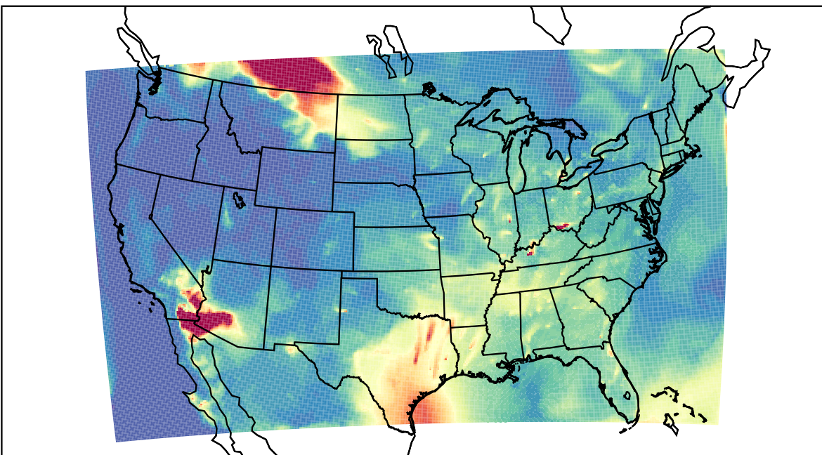
WRF 2023-07-14_09:00:00
