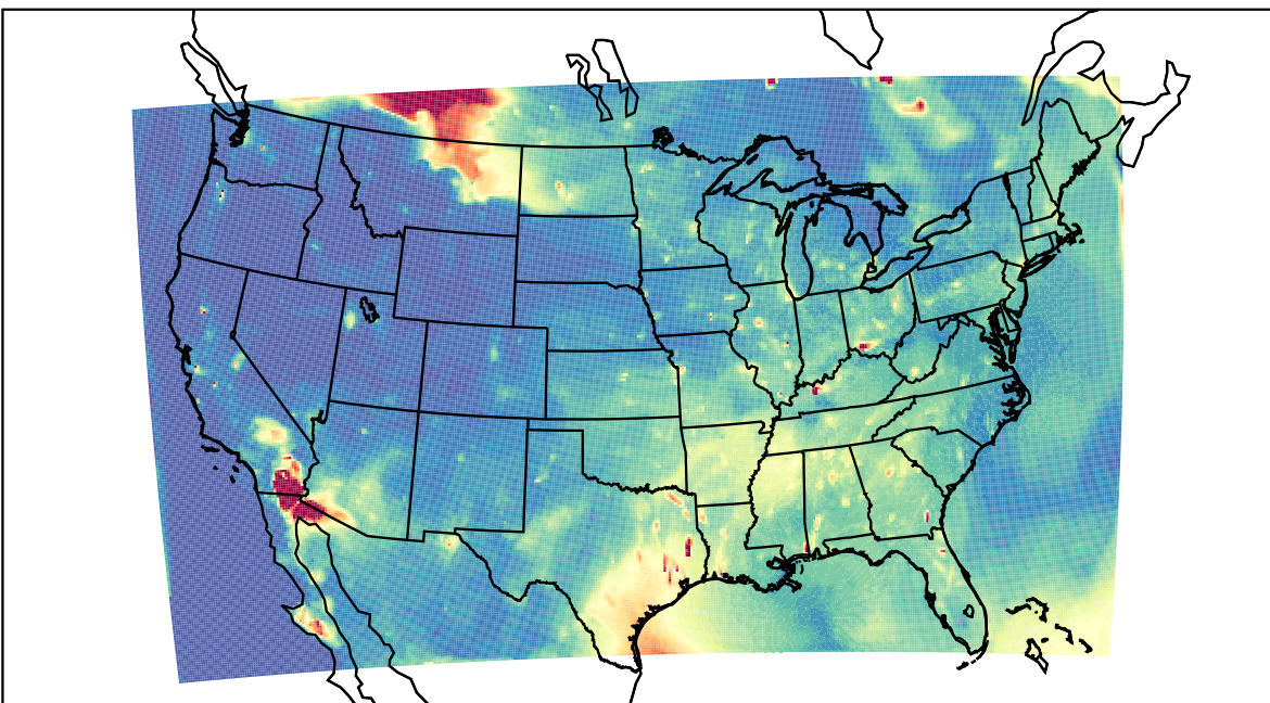
WRF 2023-07-14_03:00:00
