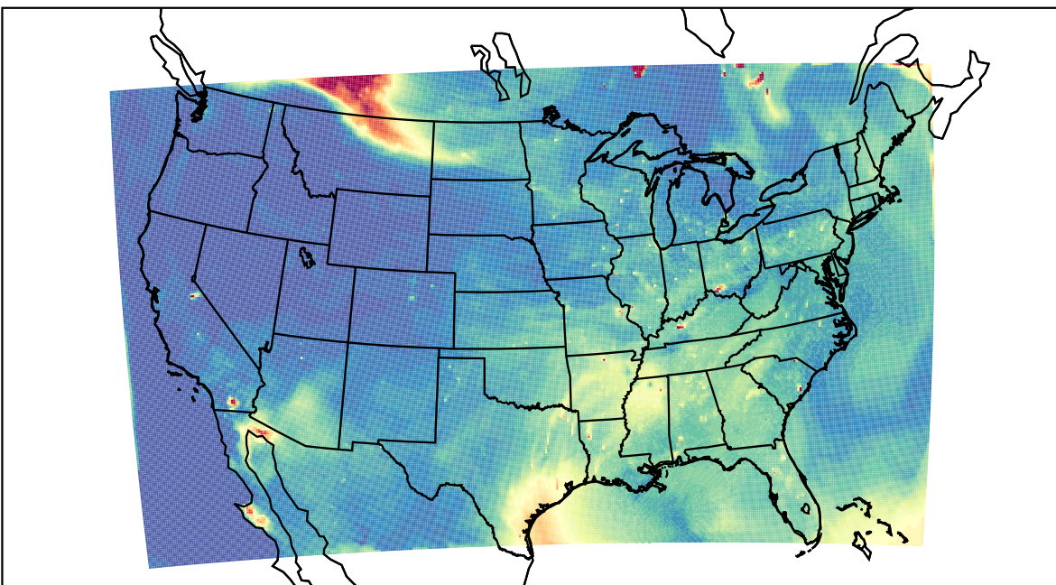
WRF 2023-07-14_00:00:00
