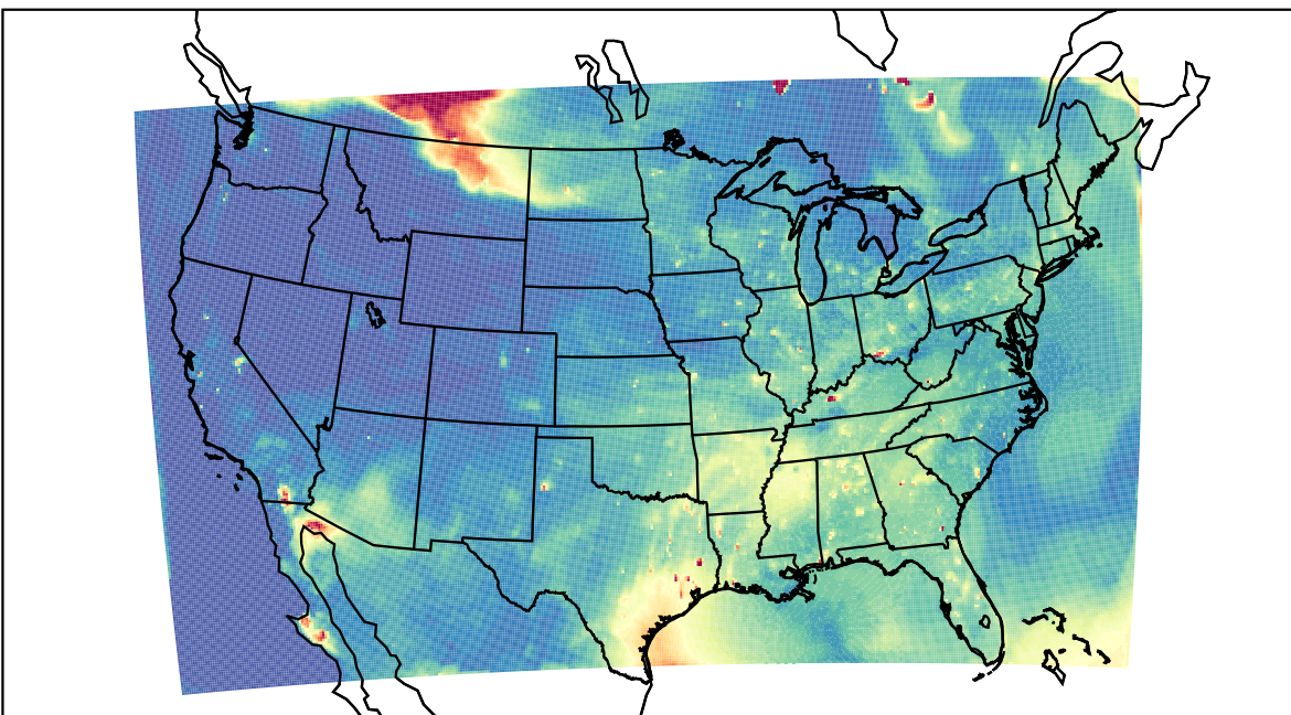
WRF 2023-07-14_01:00:00
