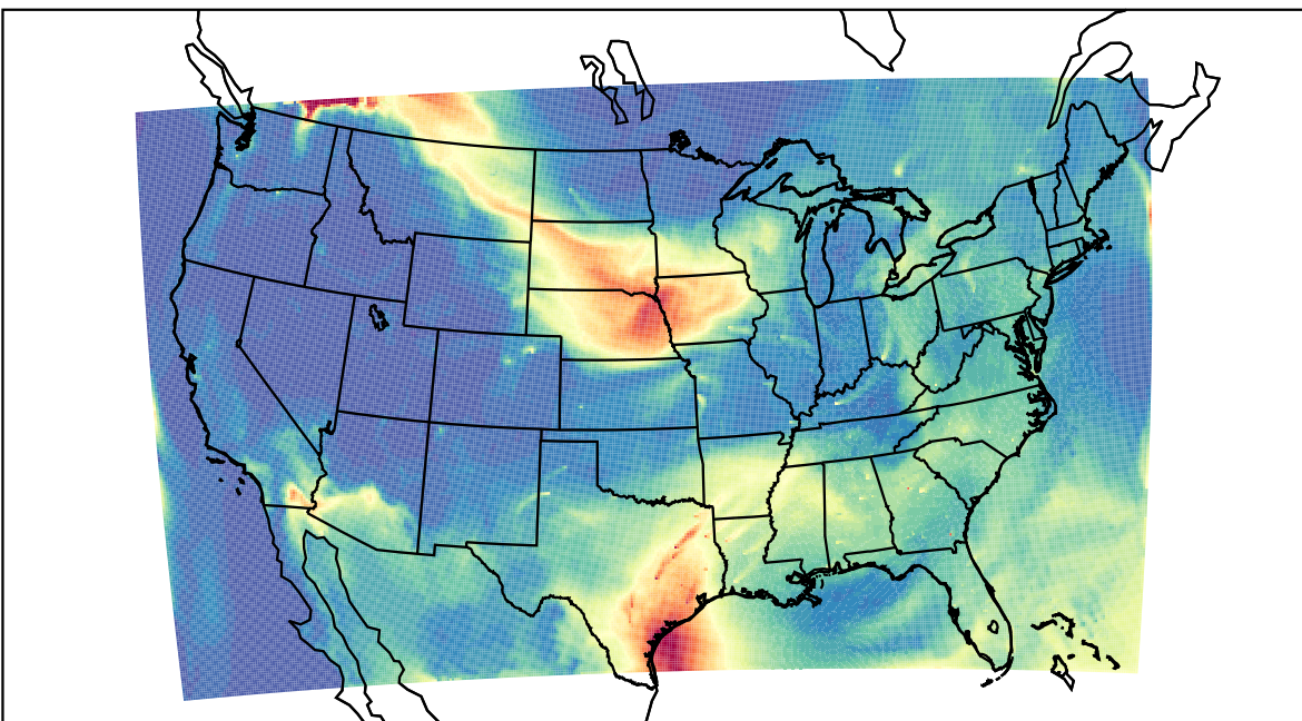
WRF 2023-07-15_17:00:00
