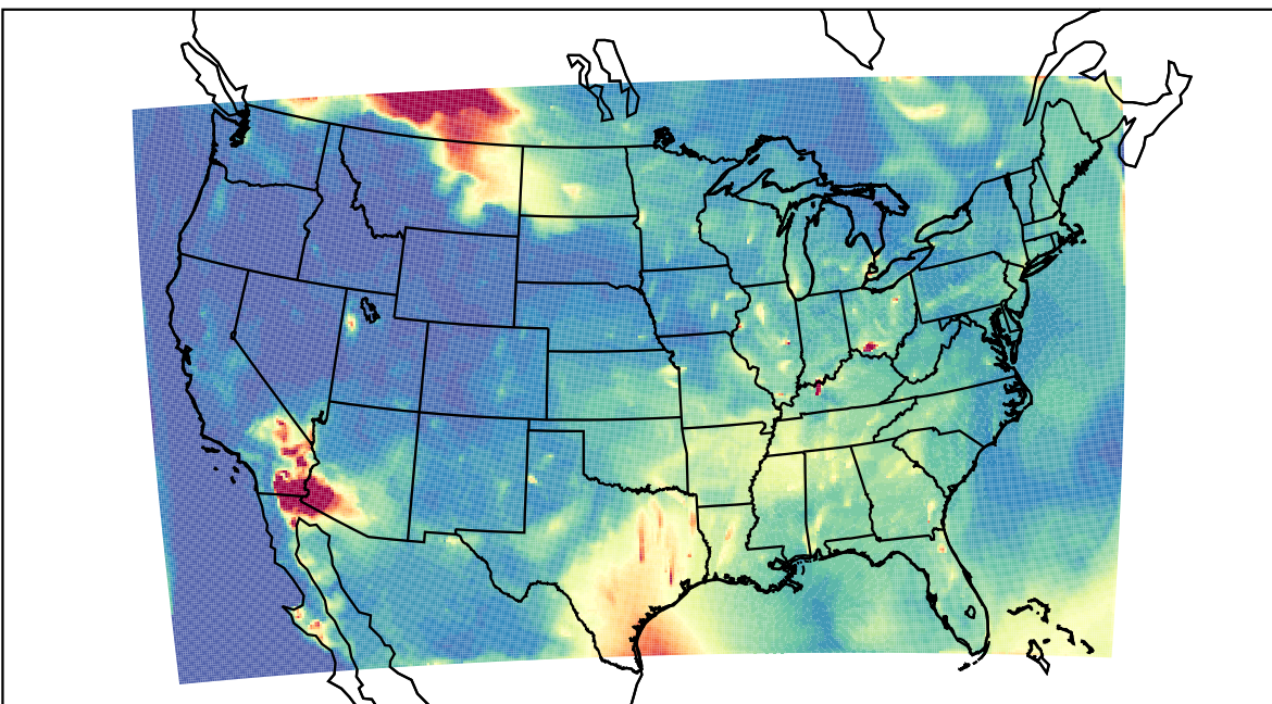
WRF 2023-07-14_06:00:00
