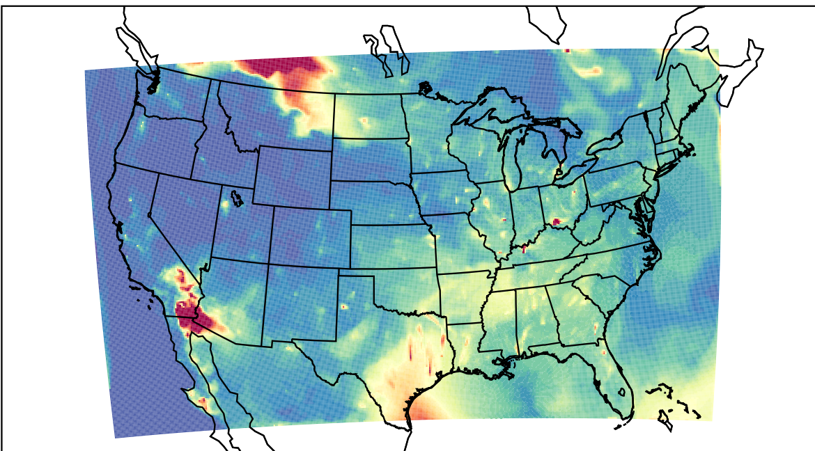
WRF 2023-07-14_05:00:00
