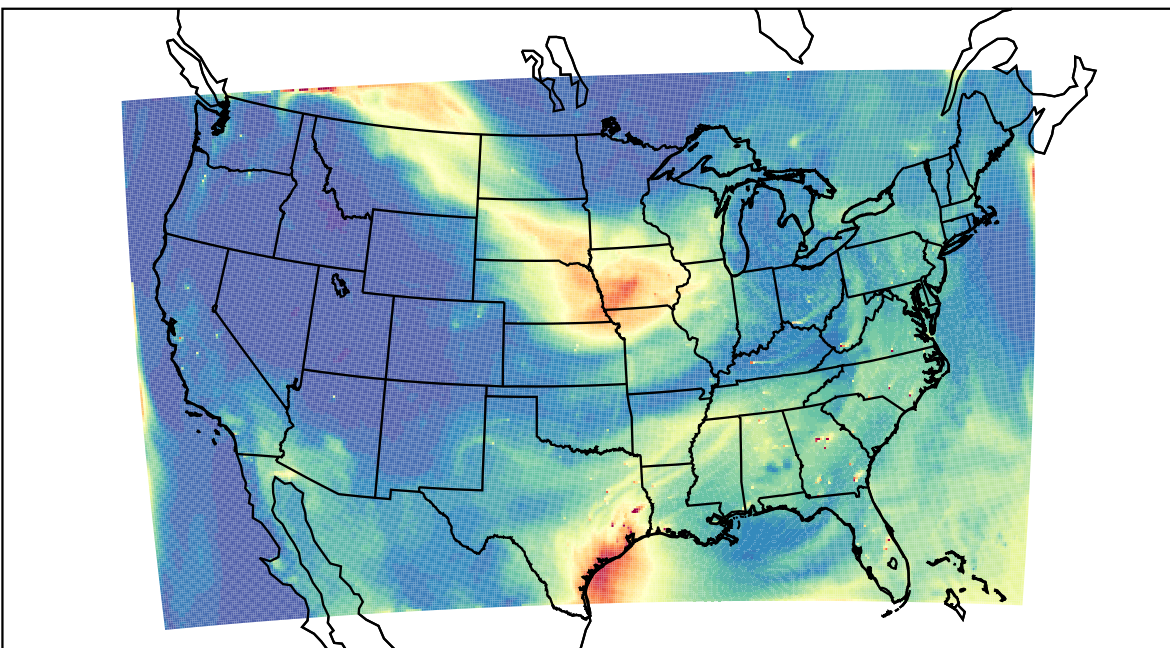
WRF 2023-07-15_22:00:00
