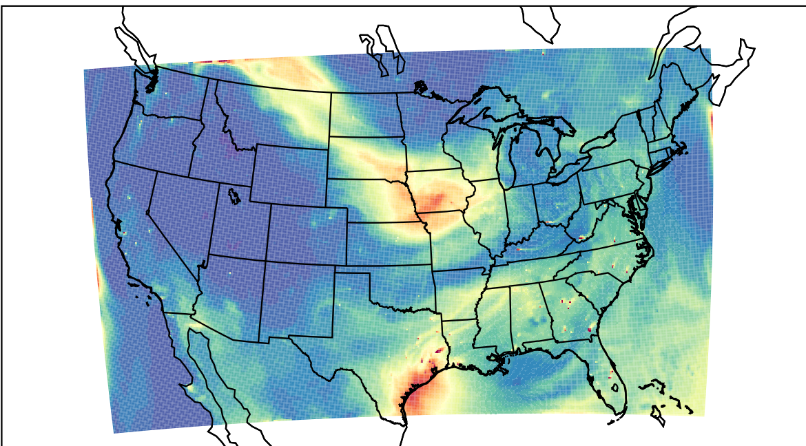
WRF 2023-07-15_23:00:00
