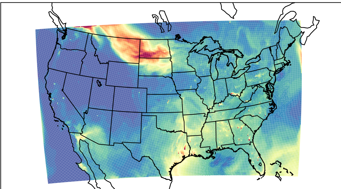
WRF 2023-07-14_23:00:00
