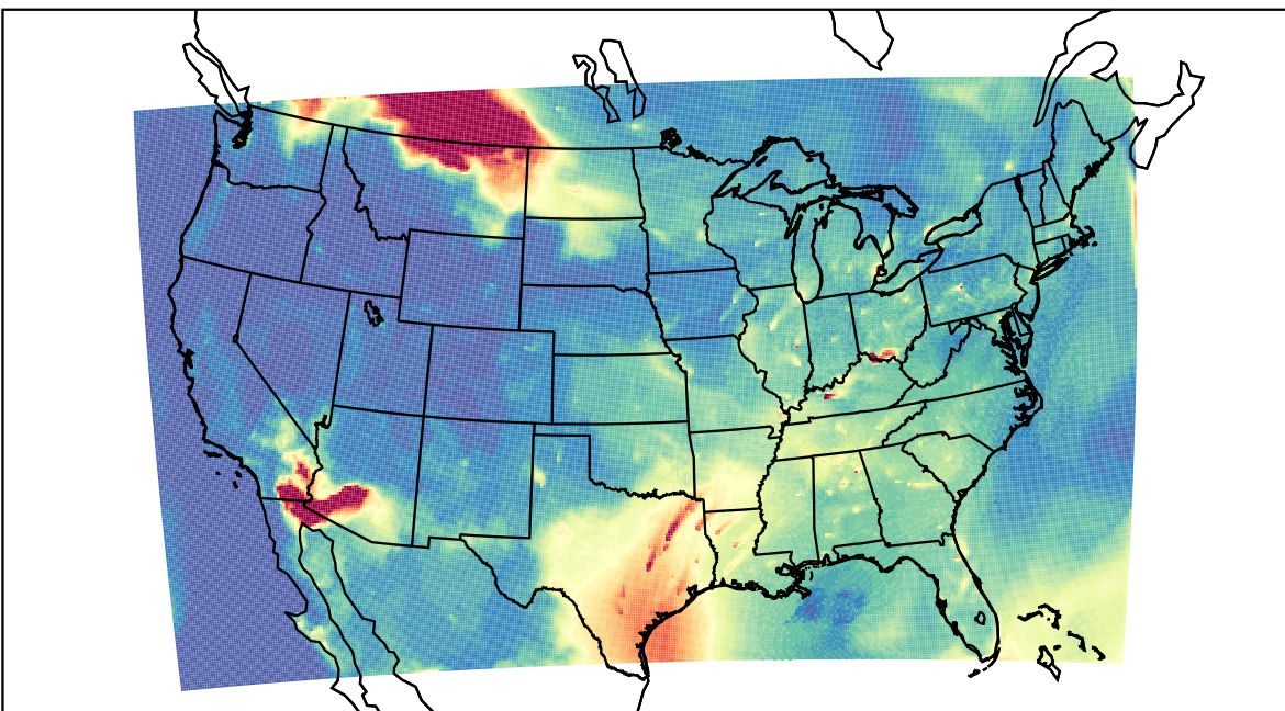
WRF 2023-07-14_13:00:00
