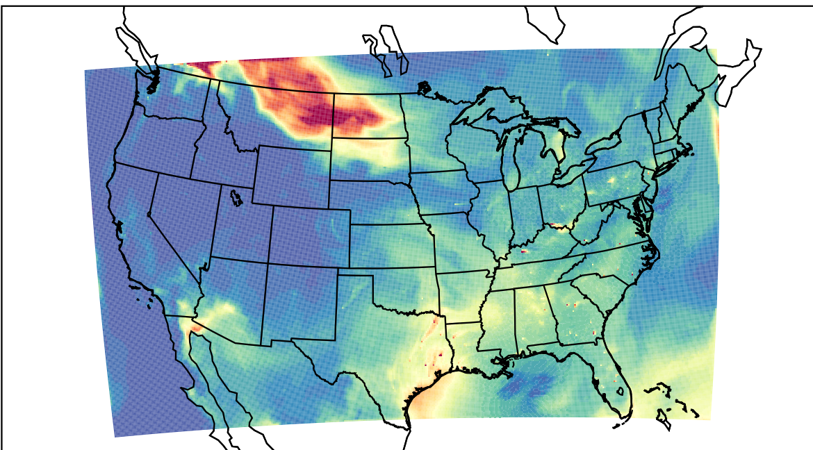
WRF 2023-07-14_19:00:00
