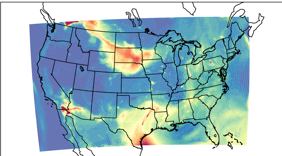
WRF 2023-07-15_12:00:00
