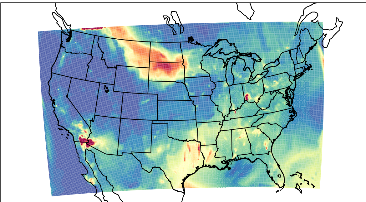
WRF 2023-07-15_05:00:00
