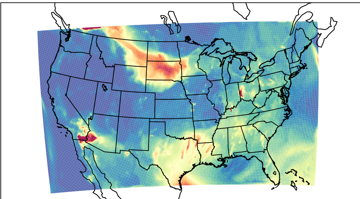
WRF 2023-07-15_08:00:00
