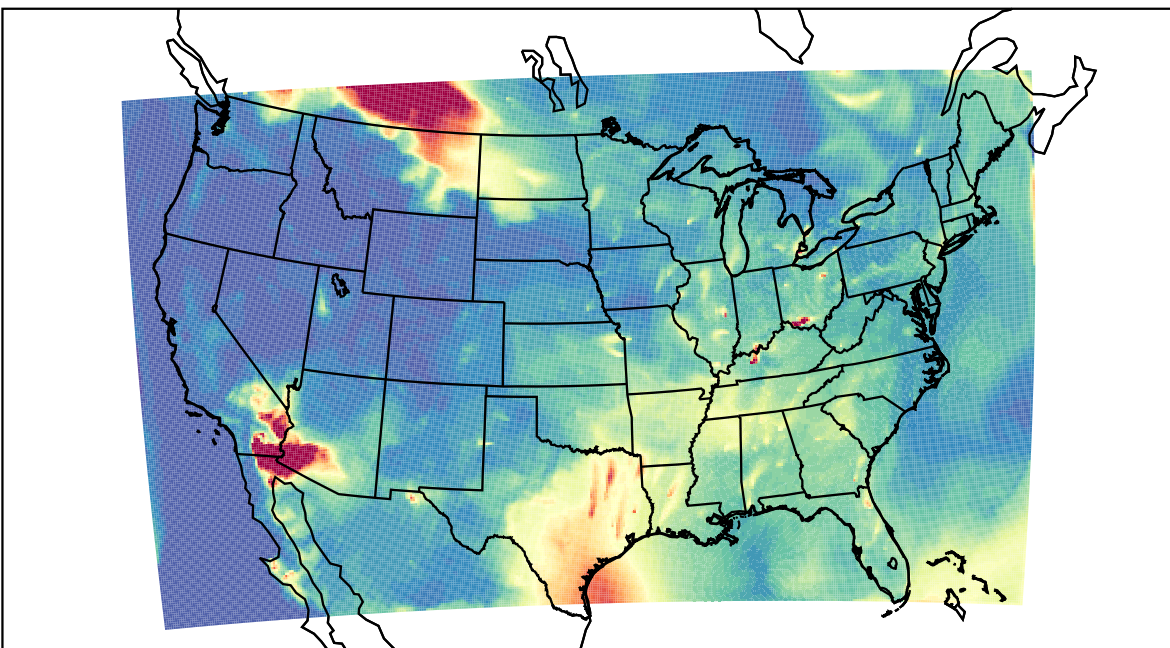
WRF 2023-07-14_08:00:00
