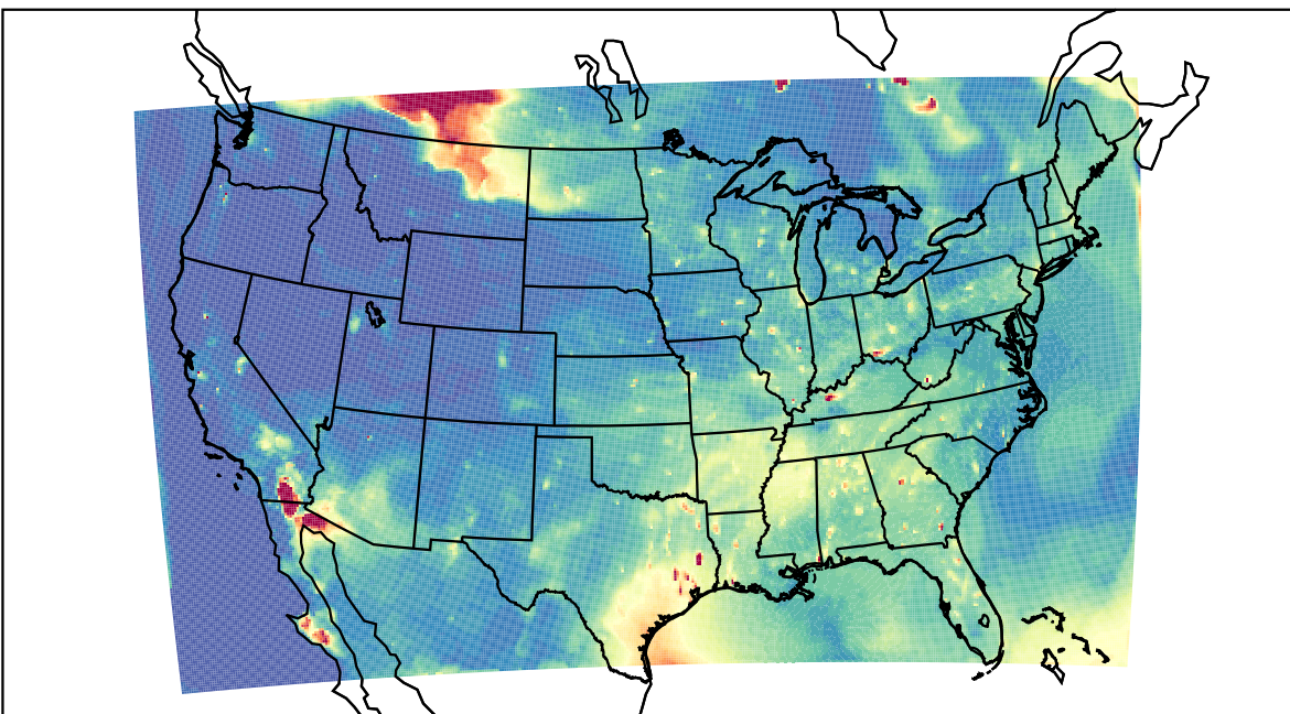
WRF 2023-07-14_02:00:00
