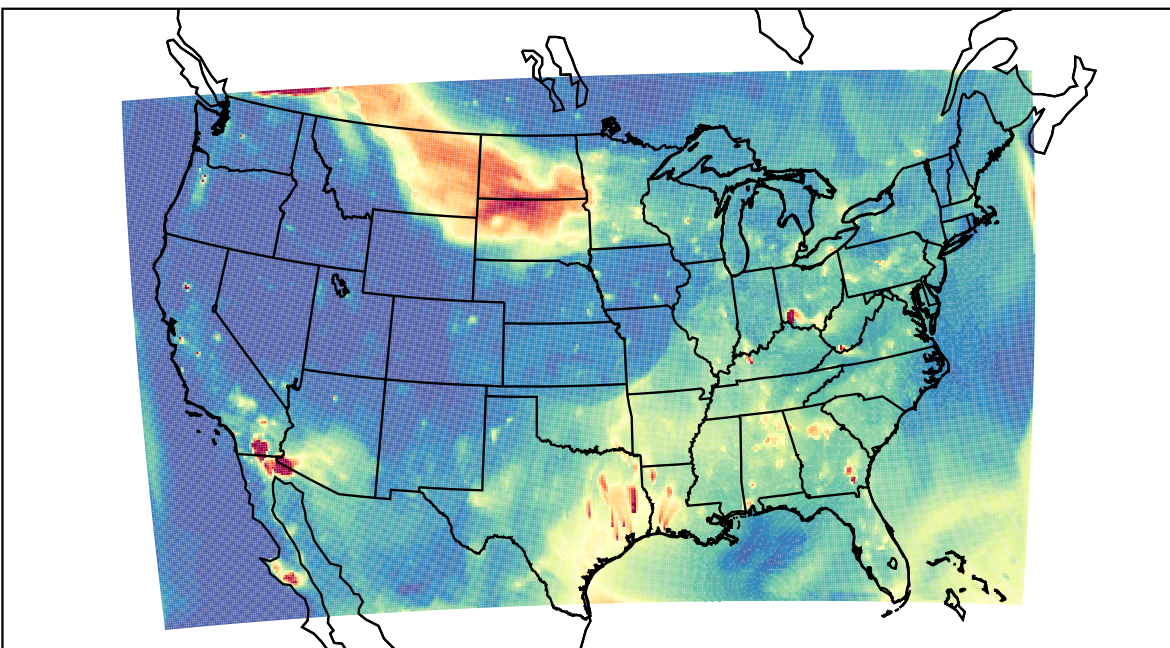
WRF 2023-07-15_03:00:00
