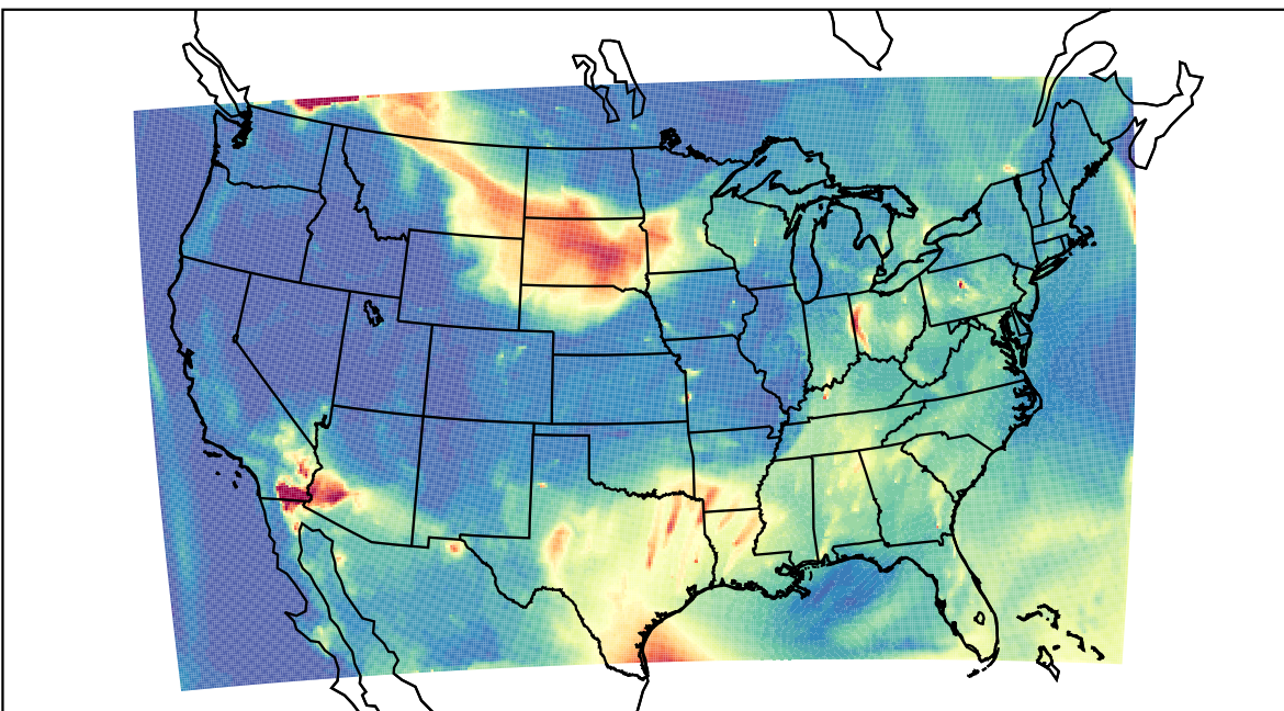
WRF 2023-07-15_09:00:00
