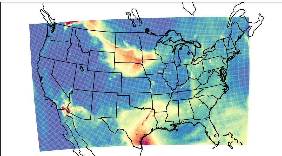
WRF 2023-07-15_14:00:00
