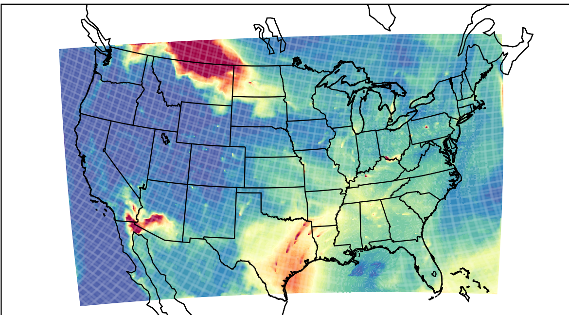
WRF 2023-07-14_15:00:00
