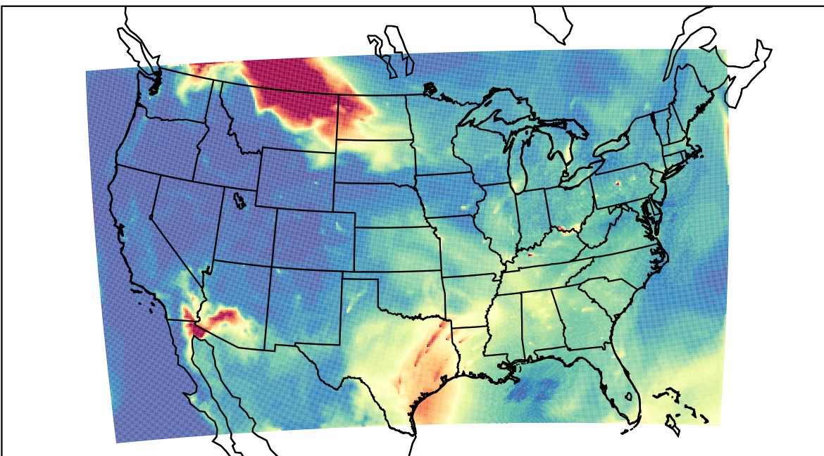
WRF 2023-07-14_16:00:00
