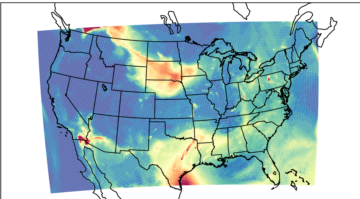
WRF 2023-07-15_13:00:00
