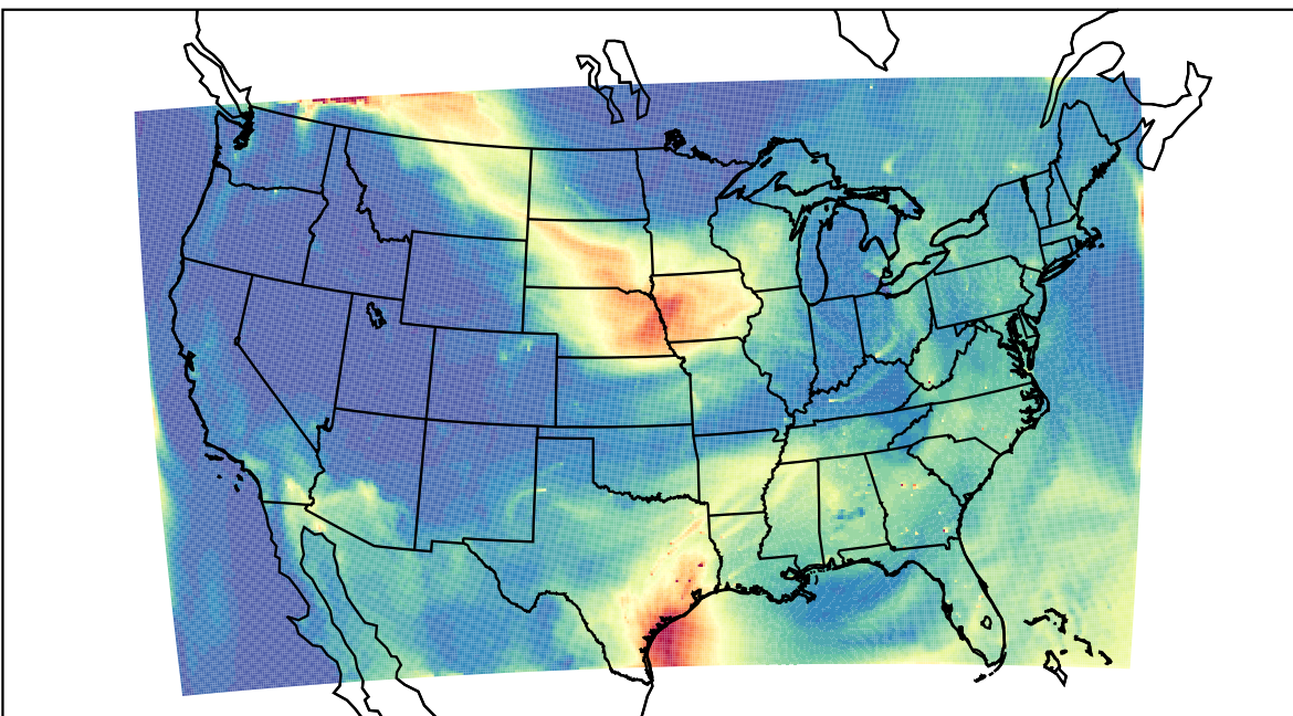
WRF 2023-07-15_19:00:00
