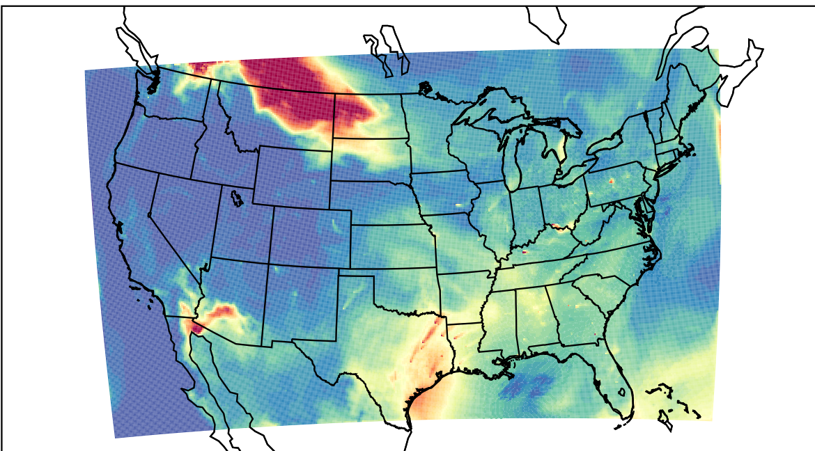
WRF 2023-07-14_17:00:00
