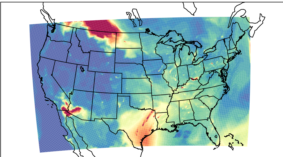
WRF 2023-07-14_14:00:00
