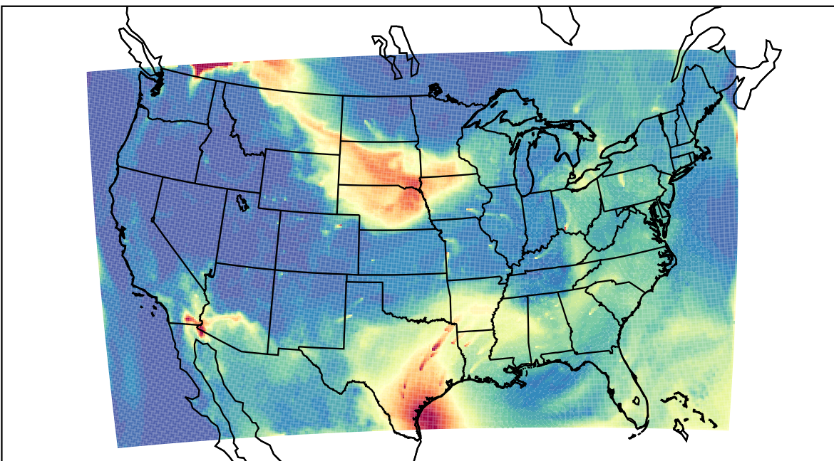
WRF 2023-07-15_15:00:00
