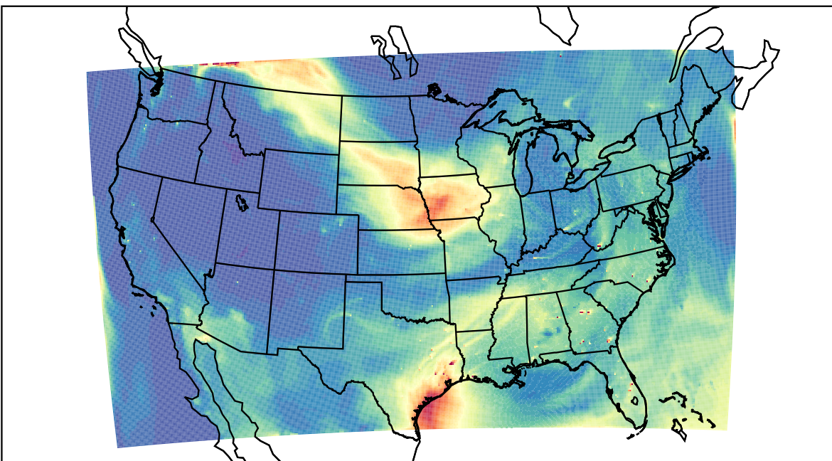
WRF 2023-07-15_21:00:00
