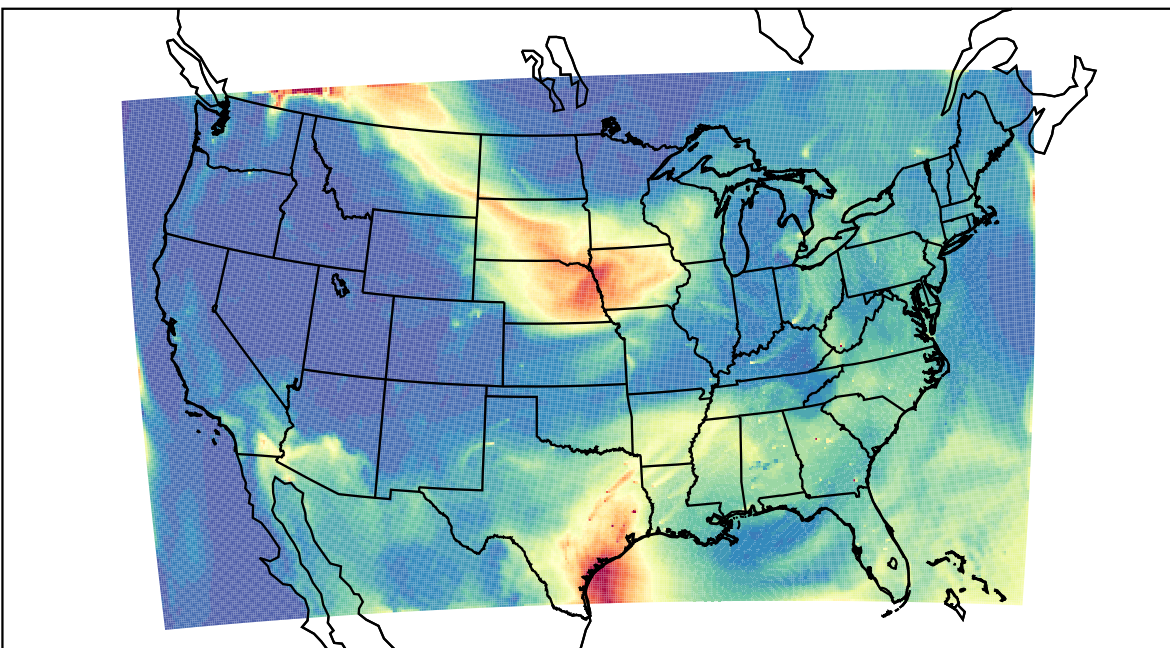
WRF 2023-07-15_18:00:00
