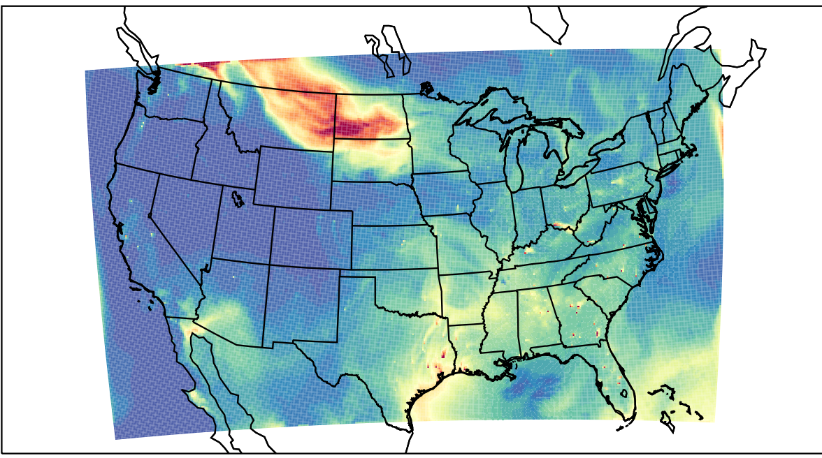
WRF 2023-07-14_22:00:00
