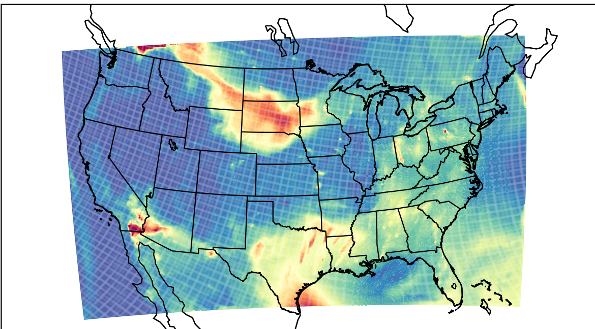
WRF 2023-07-15_10:00:00
