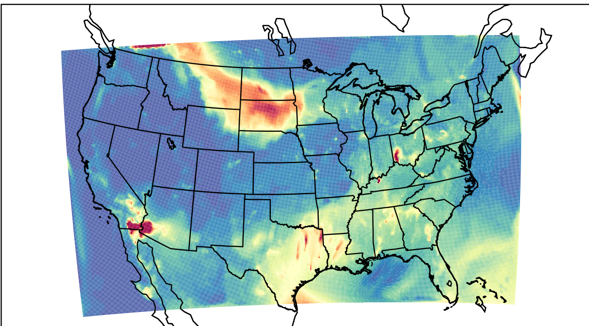
WRF 2023-07-15_06:00:00
