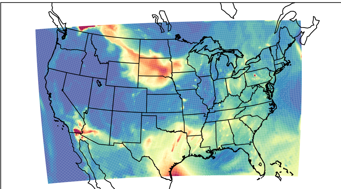
WRF 2023-07-15_11:00:00
