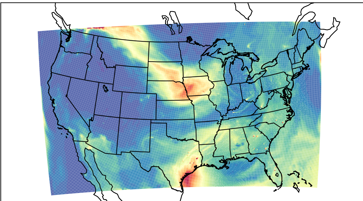
WRF 2023-07-15_20:00:00
