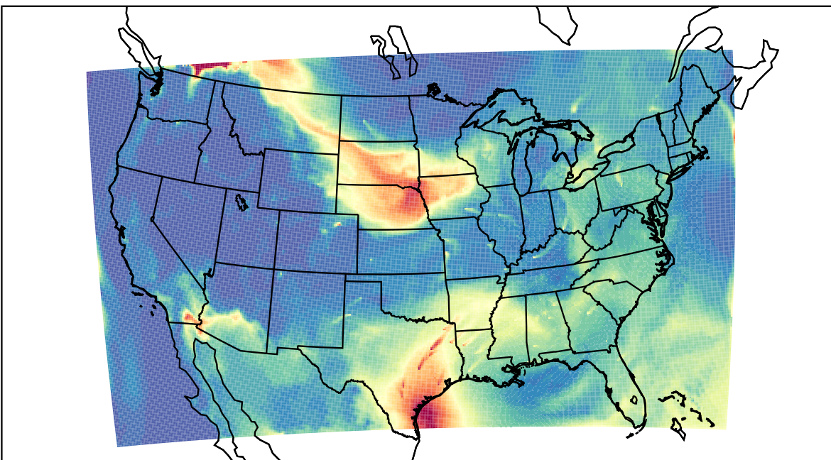
WRF 2023-07-15_16:00:00
