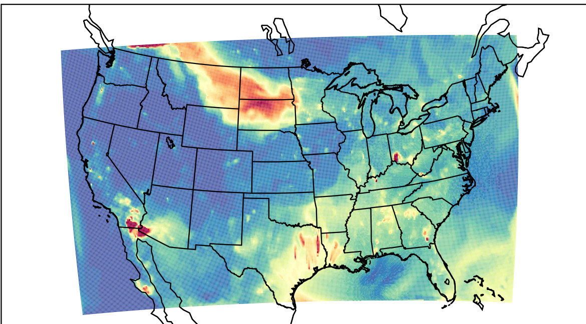
WRF 2023-07-15_04:00:00
