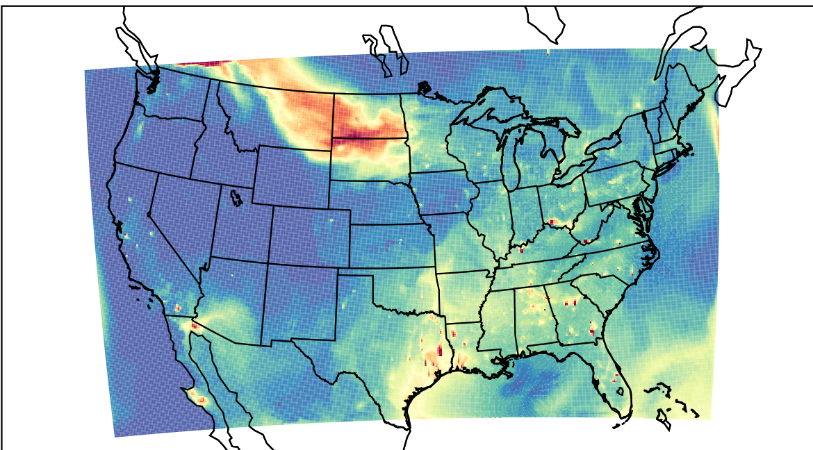
WRF 2023-07-15_01:00:00
