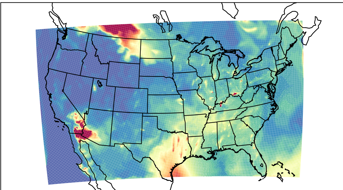
WRF 2023-07-14_07:00:00
