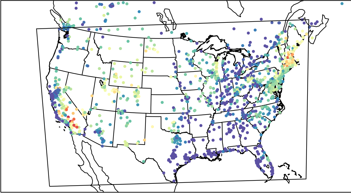
AirNOW (2023-07-14_04:00:00)
