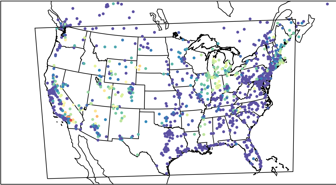
AirNOW (2023-07-15_10:00:00)
