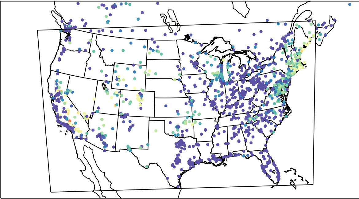
AirNOW (2023-07-14_11:00:00)
