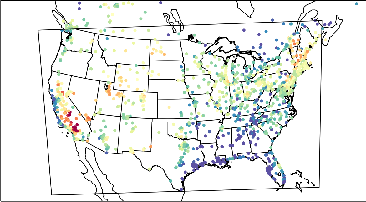
AirNOW (2023-07-14_01:00:00)
