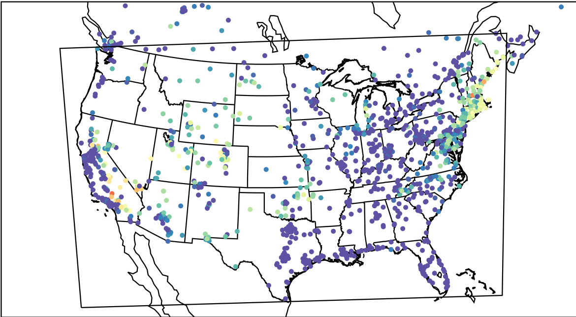
AirNOW (2023-07-14_10:00:00)
