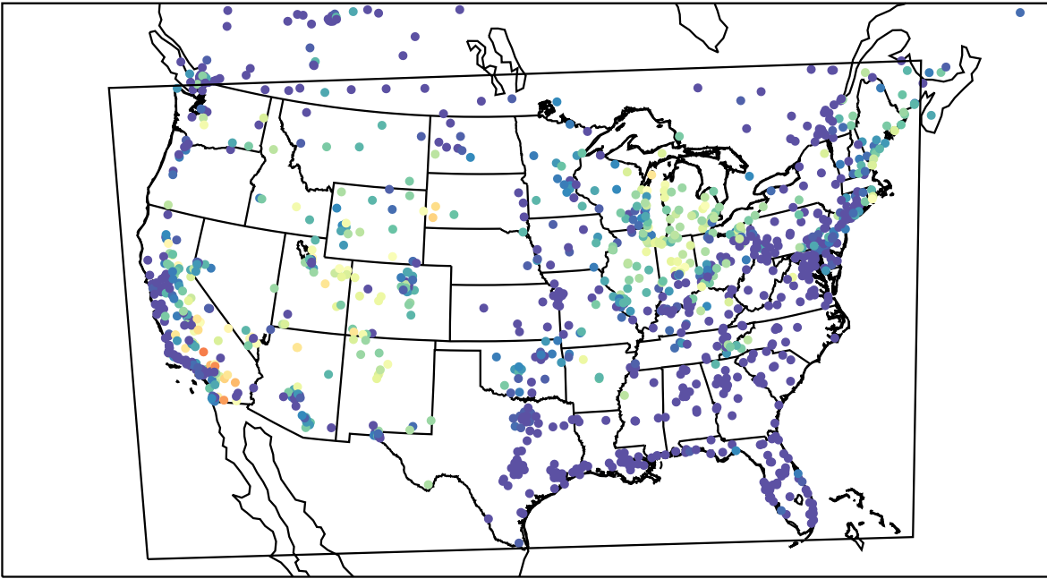
AirNOW (2023-07-15_08:00:00)
