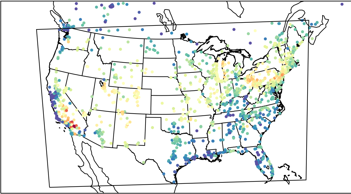
AirNOW (2023-07-15_16:00:00)
