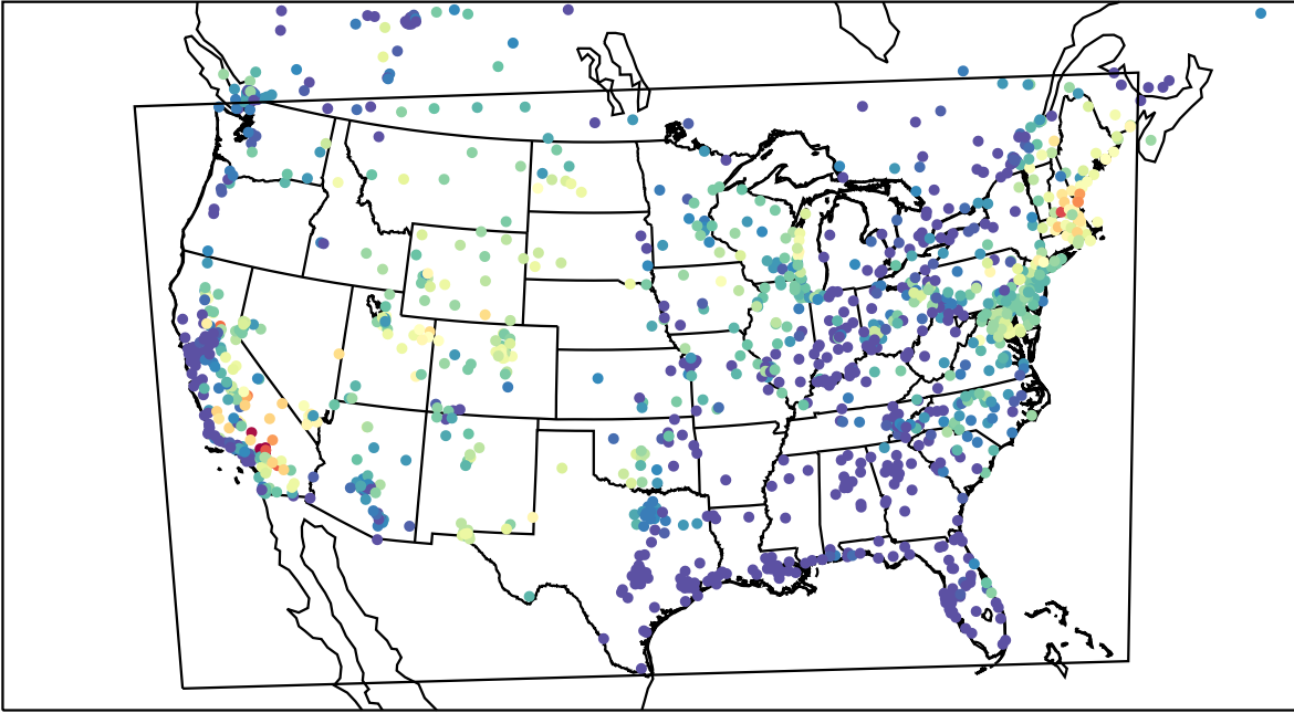
AirNOW (2023-07-14_05:00:00)
