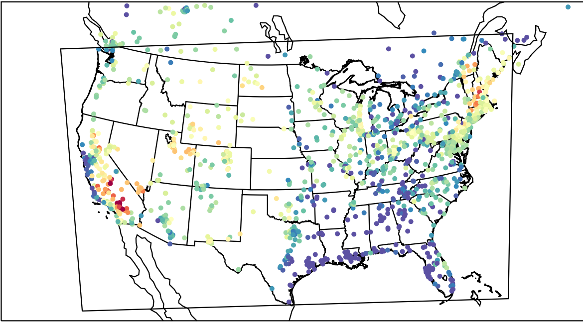
AirNOW (2023-07-14_02:00:00)
