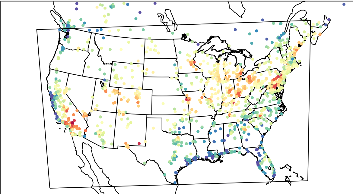
AirNOW (2023-07-14_18:00:00)
