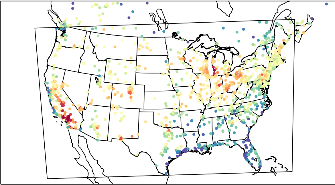
AirNOW (2023-07-14_21:00:00)
