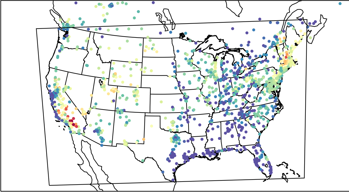
AirNOW (2023-07-14_03:00:00)
