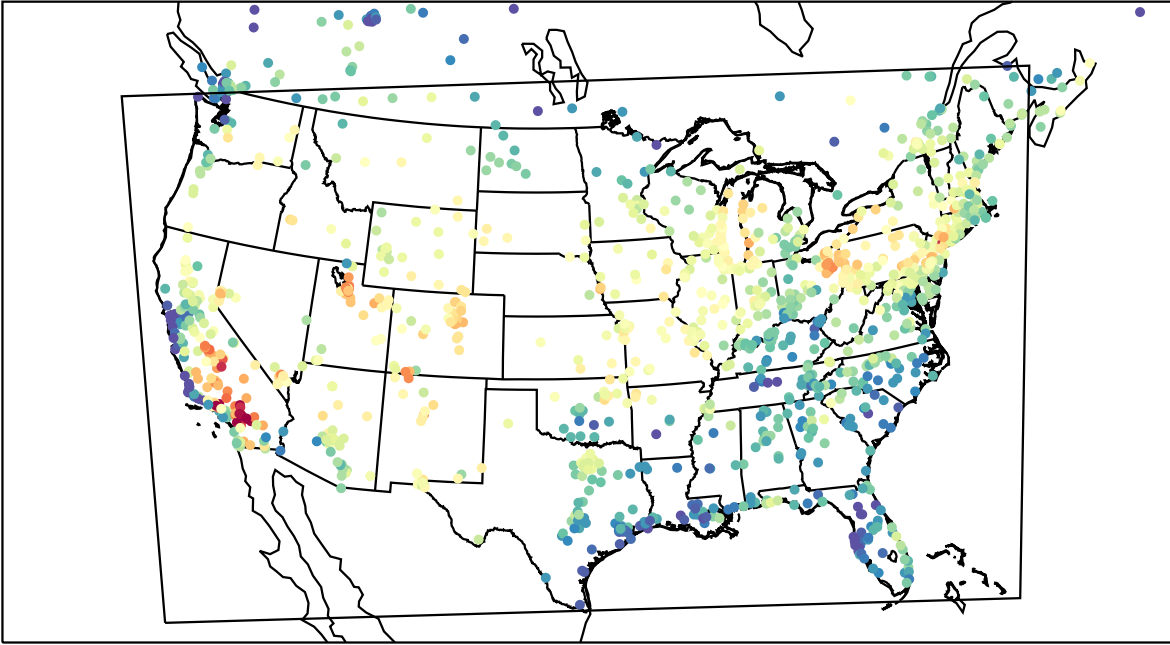
AirNOW (2023-07-15_17:00:00)
