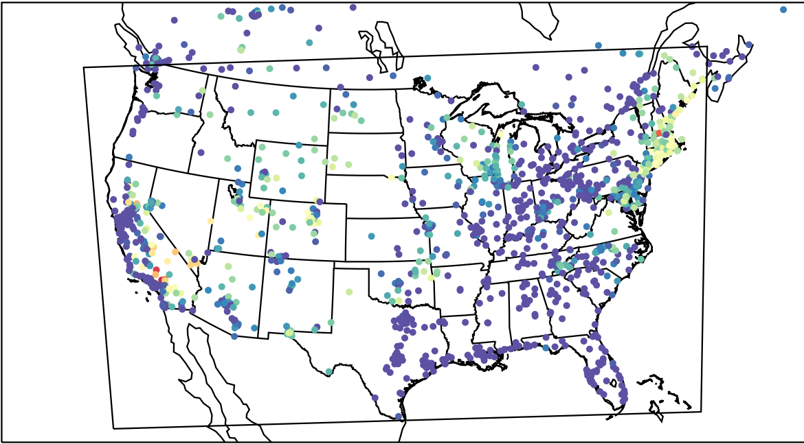
AirNOW (2023-07-14_09:00:00)
