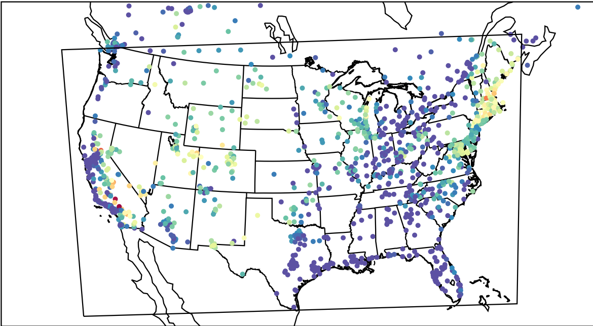
AirNOW (2023-07-14_06:00:00)
