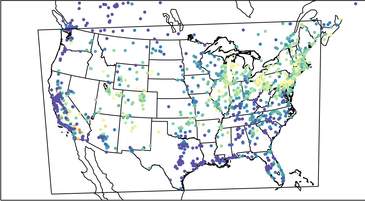
AirNOW (2023-07-15_14:00:00)
