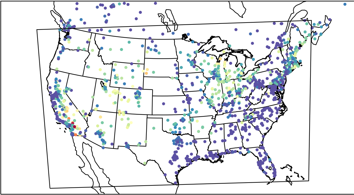
AirNOW (2023-07-15_07:00:00)
