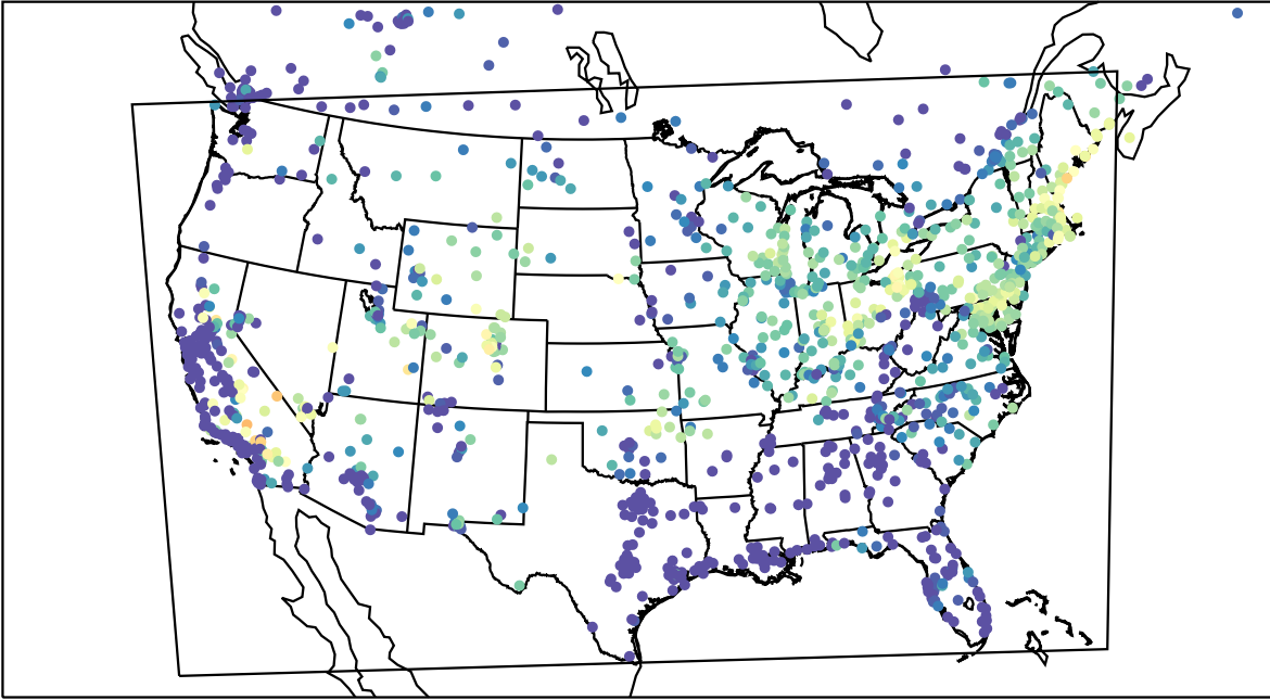
AirNOW (2023-07-14_13:00:00)
