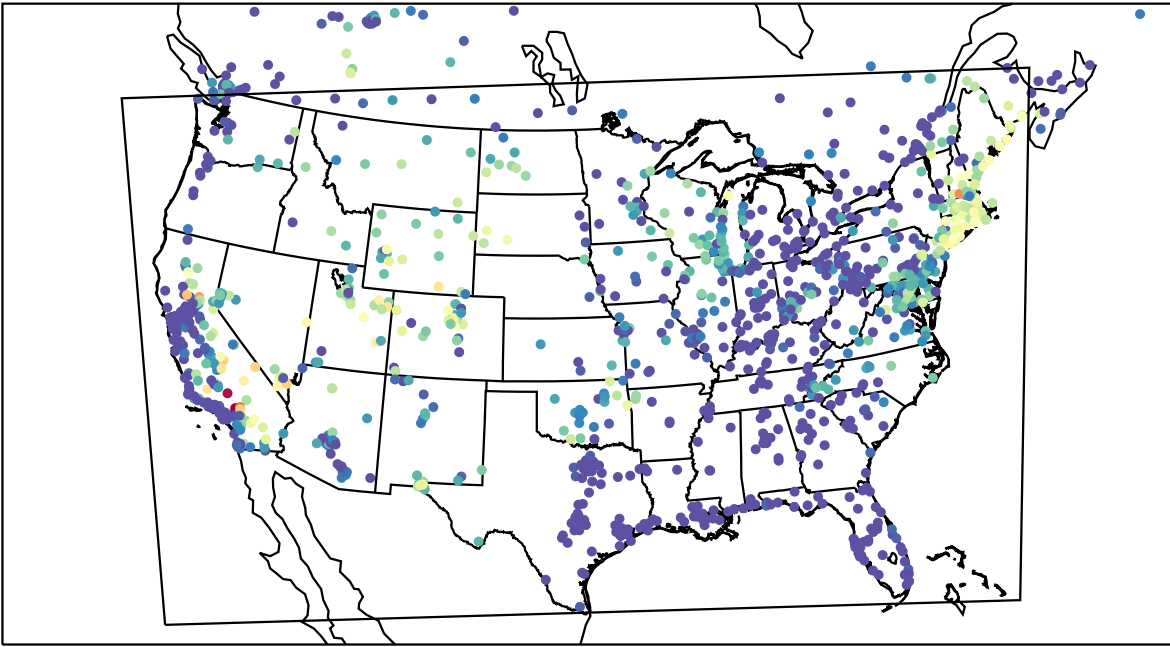
AirNOW (2023-07-14_08:00:00)
