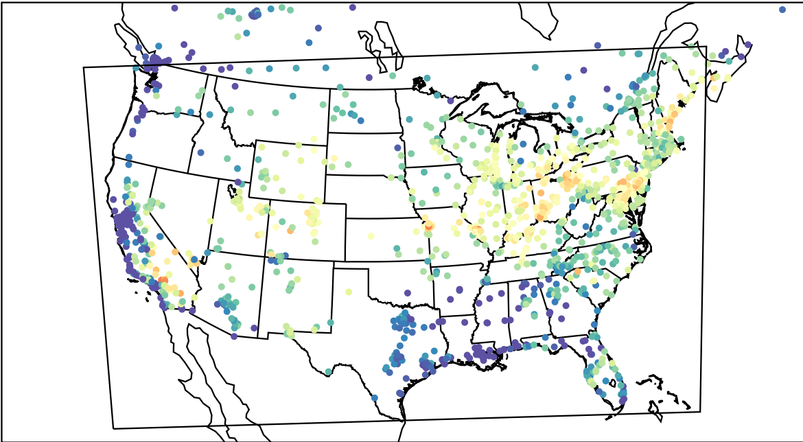
AirNOW (2023-07-14_15:00:00)
