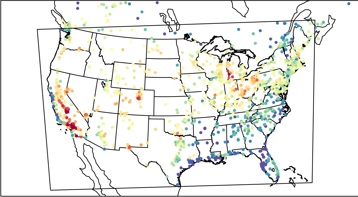
AirNOW (2023-07-14_23:00:00)
