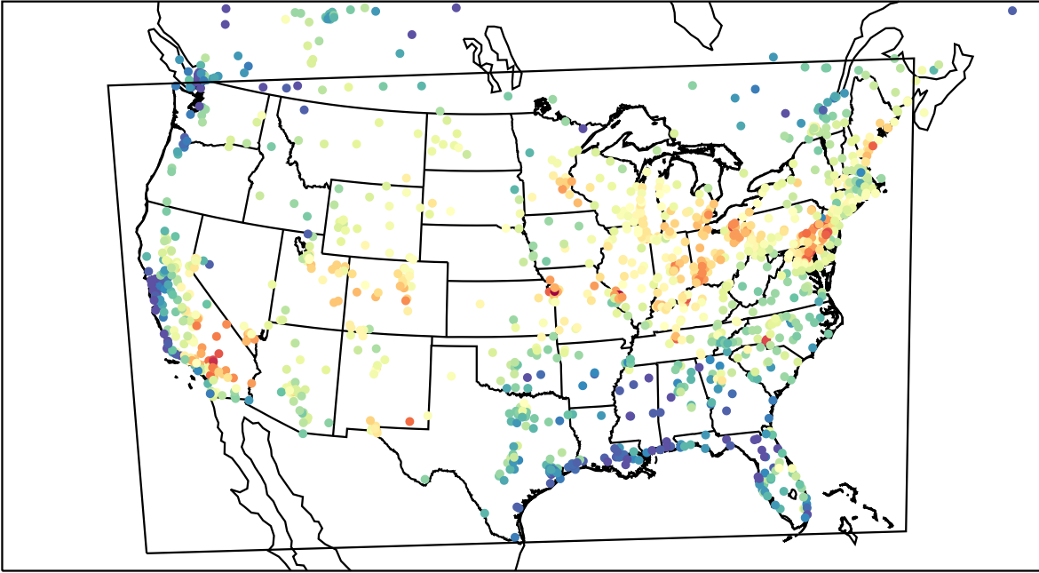
AirNOW (2023-07-14_17:00:00)
