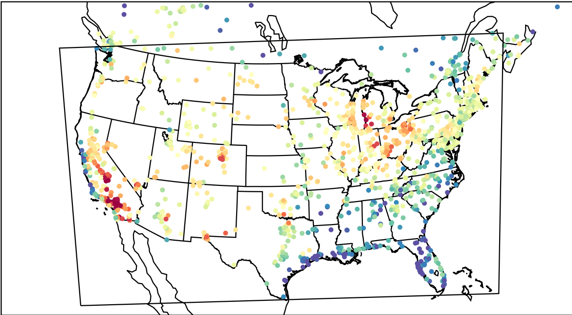
AirNOW (2023-07-14_22:00:00)
