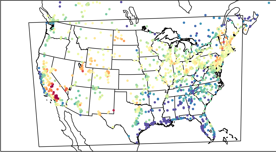
AirNOW (2023-07-14_00:00:00)
