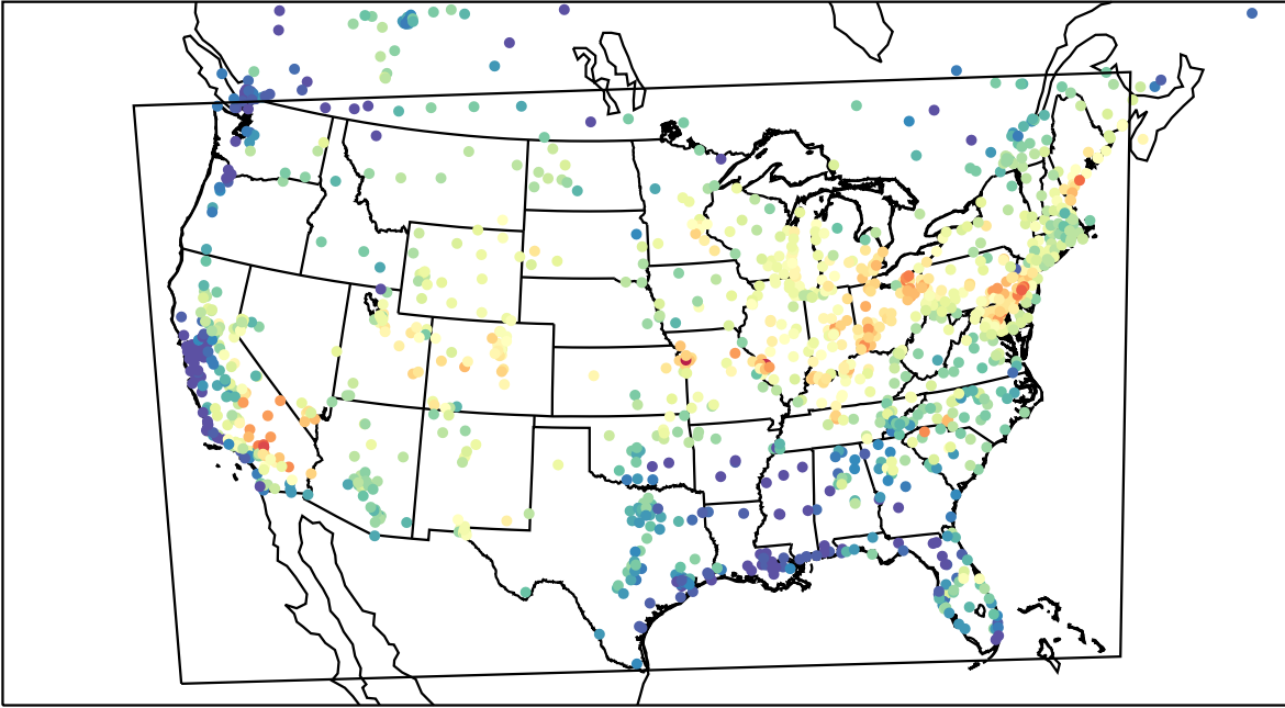
AirNOW (2023-07-14_16:00:00)
