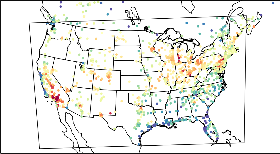
AirNOW (2023-07-14_20:00:00)
