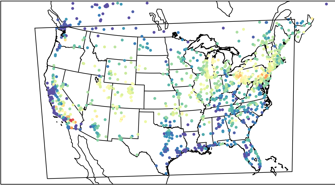
AirNOW (2023-07-15_15:00:00)
