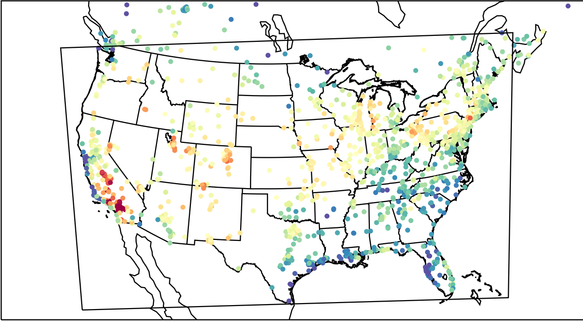
AirNOW (2023-07-15_18:00:00)
