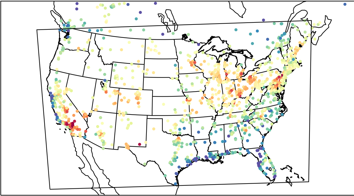
AirNOW (2023-07-14_19:00:00)
