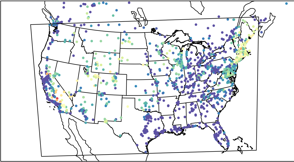
AirNOW (2023-07-14_07:00:00)
