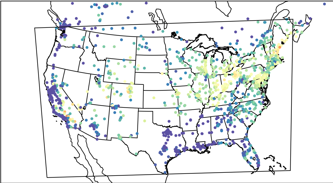
AirNOW (2023-07-14_14:00:00)
