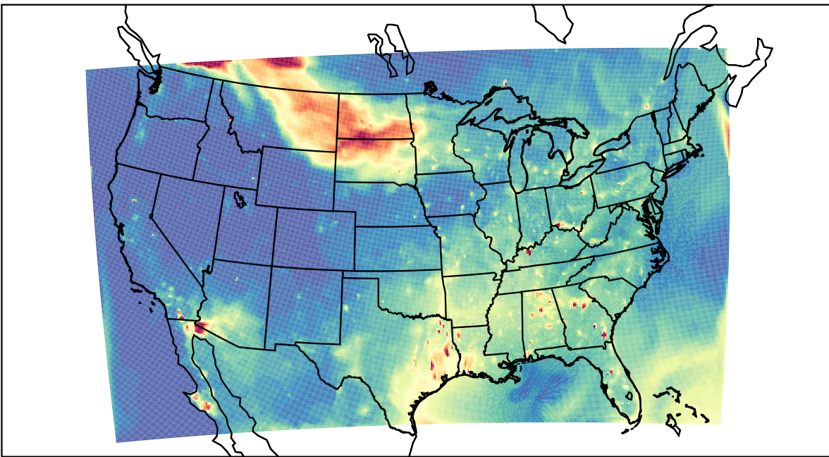
WRF 2023-07-15_02:00:00
