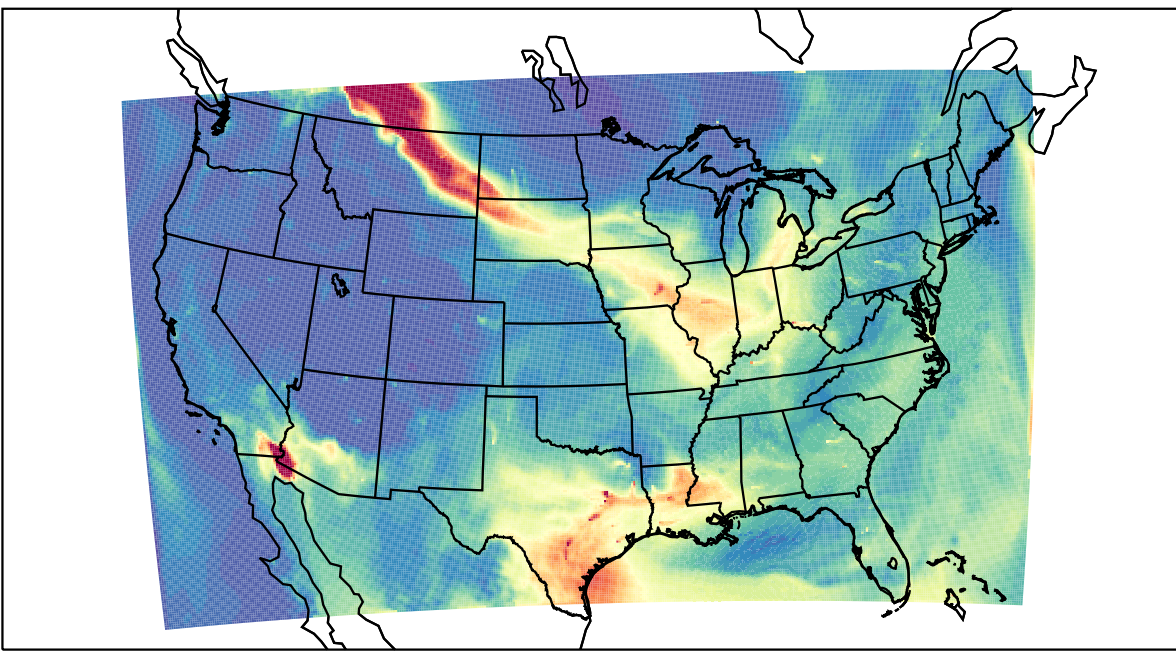
WRF 2023-07-16_17:00:00
