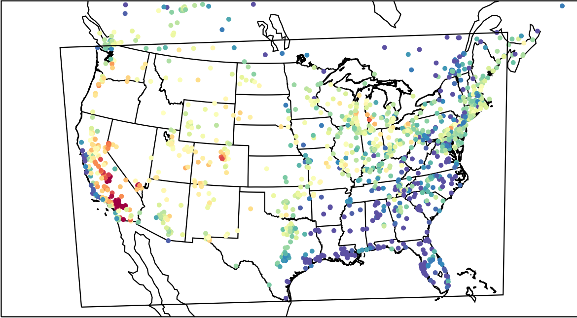
AirNOW (2023-07-15_01:00:00)
