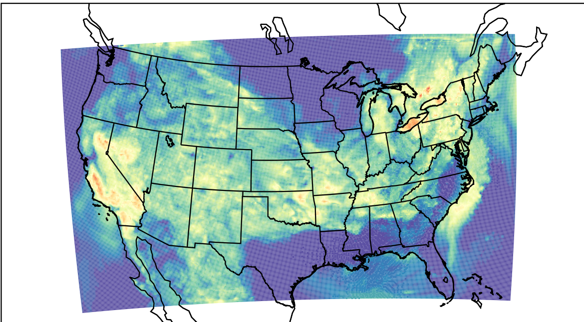
WRF (2023-07-16_10:00:00)
