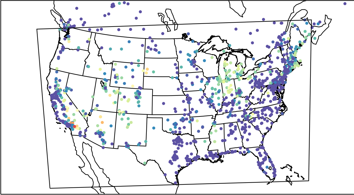
AirNOW (2023-07-15_10:00:00)
