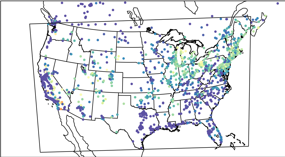
AirNOW (2023-07-15_13:00:00)
