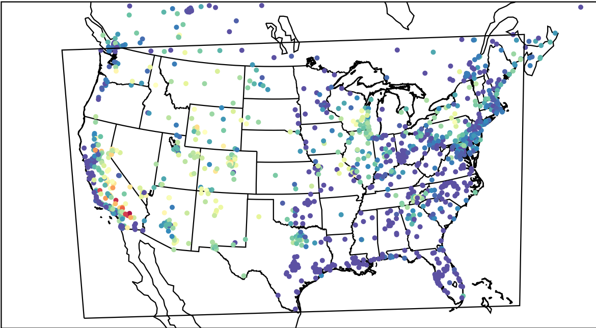
AirNOW (2023-07-16_05:00:00)
