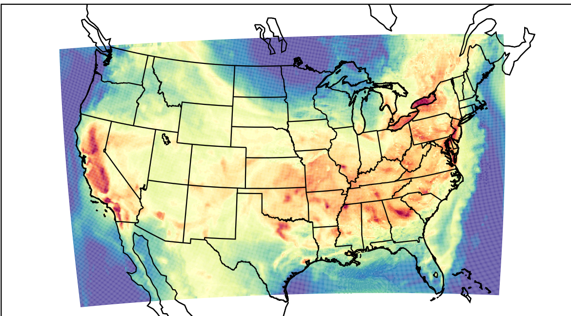
WRF (2023-07-16_19:00:00)
