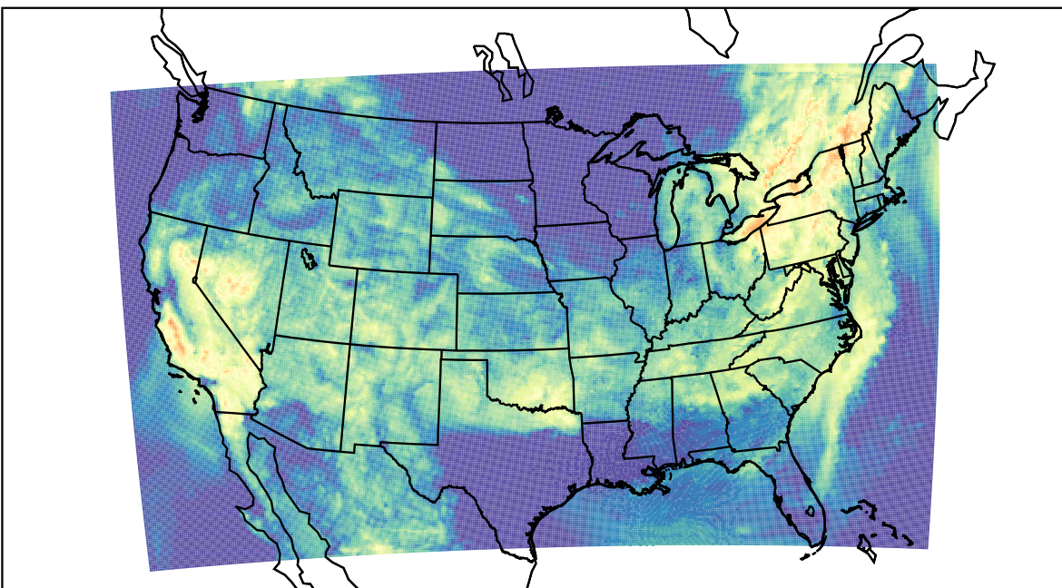
WRF (2023-07-16_13:00:00)
