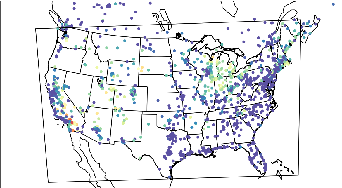
AirNOW (2023-07-15_09:00:00)
