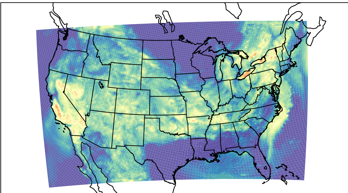
WRF (2023-07-16_11:00:00)
