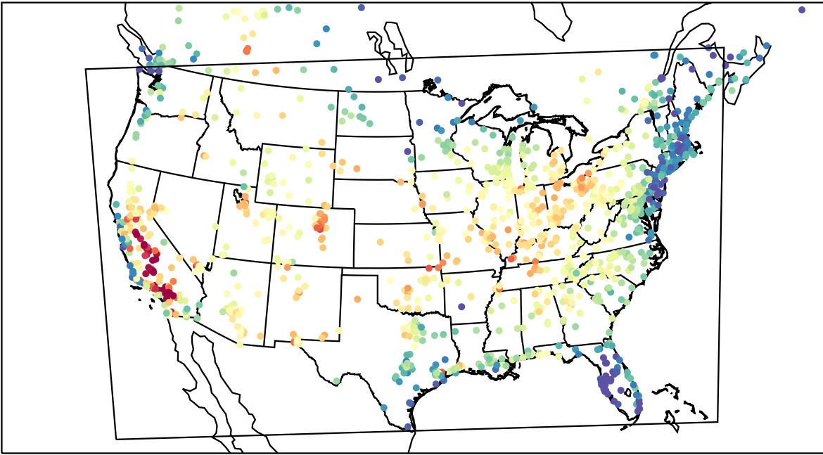
AirNOW (2023-07-16_20:00:00)
