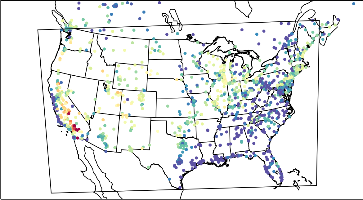
AirNOW (2023-07-15_03:00:00)
