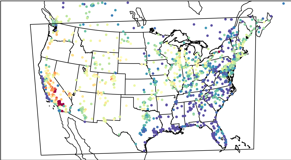
AirNOW (2023-07-15_02:00:00)
