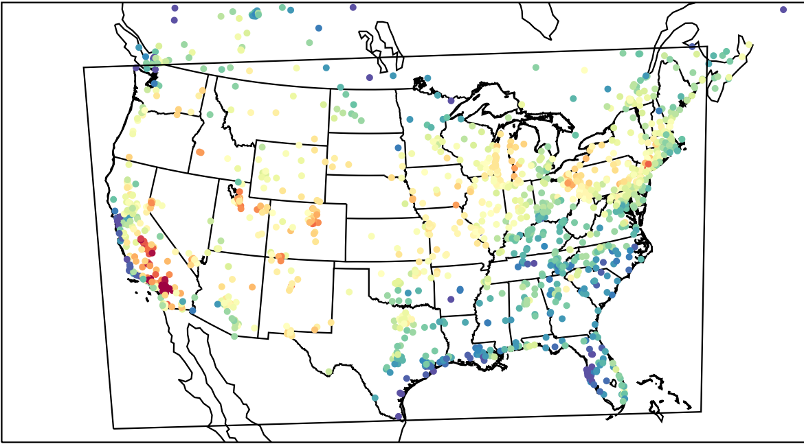
AirNOW (2023-07-15_18:00:00)
