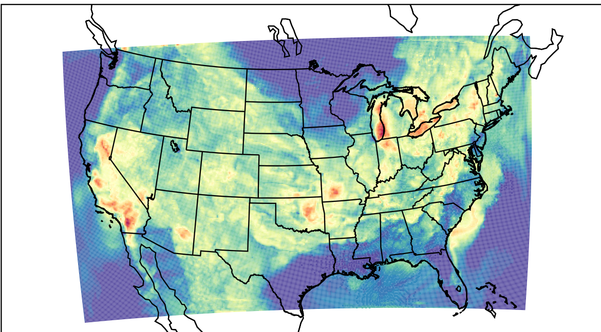
WRF (2023-07-16_05:00:00)
