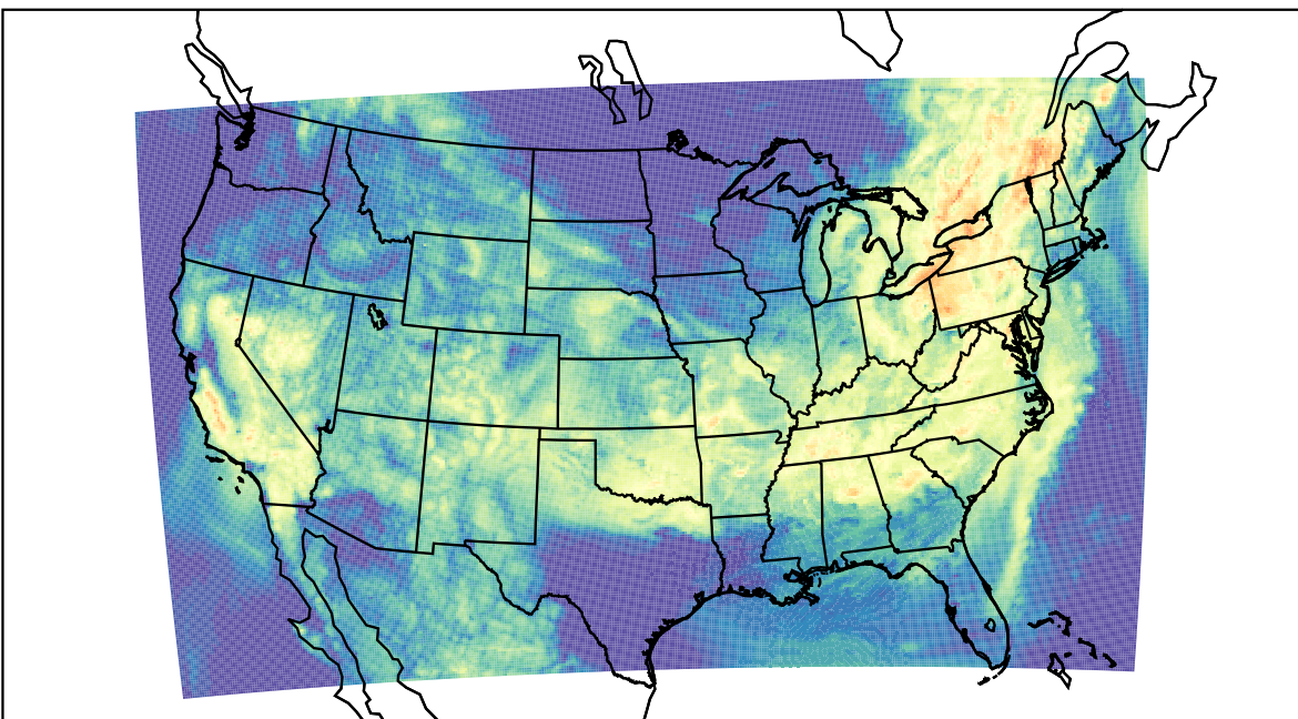
WRF (2023-07-16_14:00:00)
