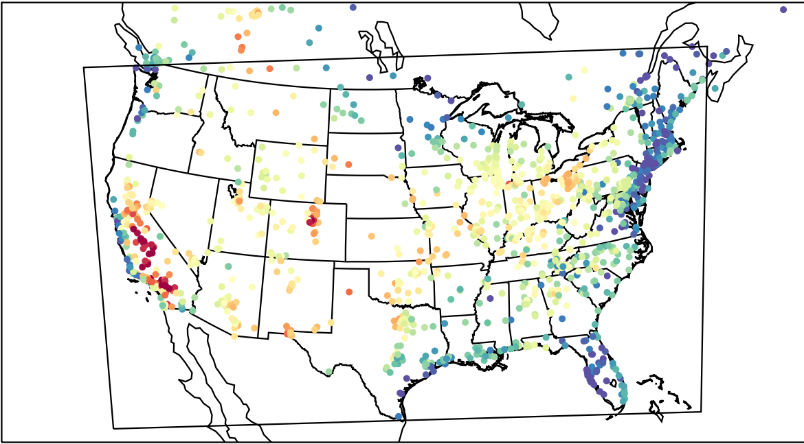
AirNOW (2023-07-16_23:00:00)
