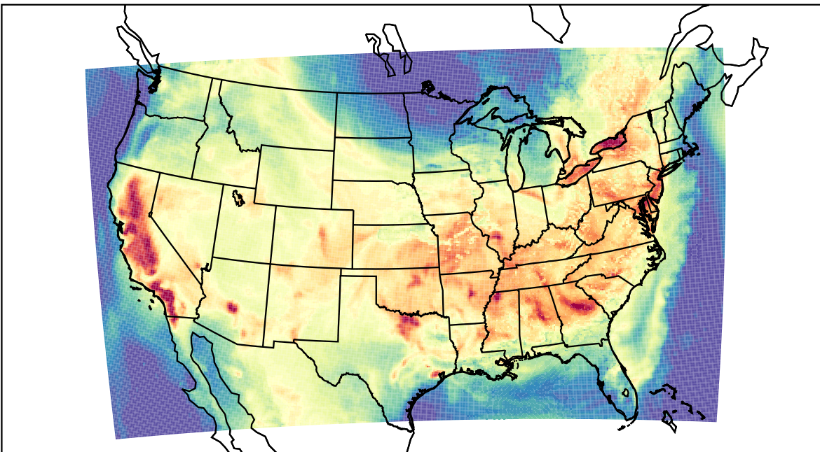
WRF (2023-07-16_21:00:00)
