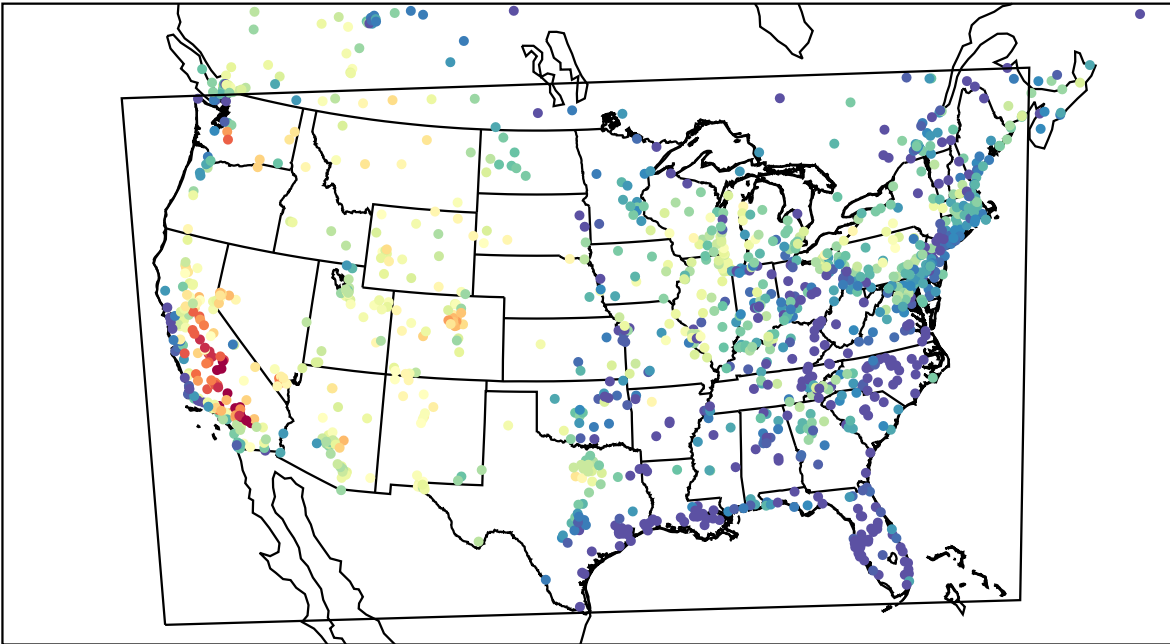
AirNOW (2023-07-16_02:00:00)
