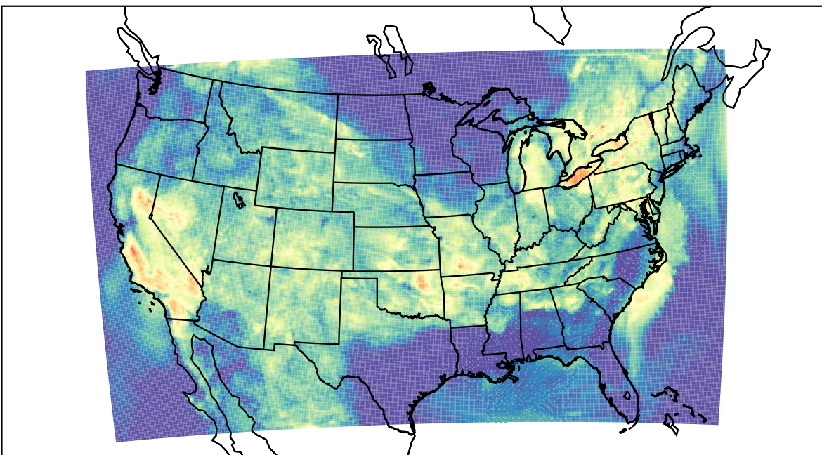
WRF (2023-07-16_09:00:00)
