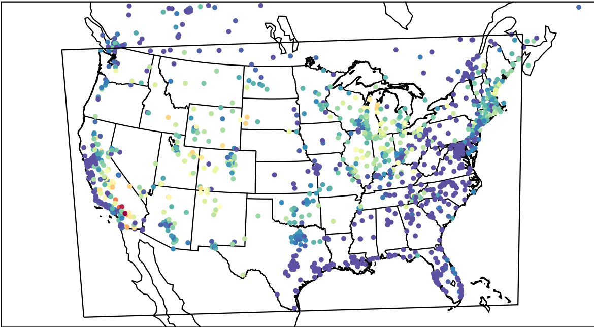
AirNOW (2023-07-15_06:00:00)
