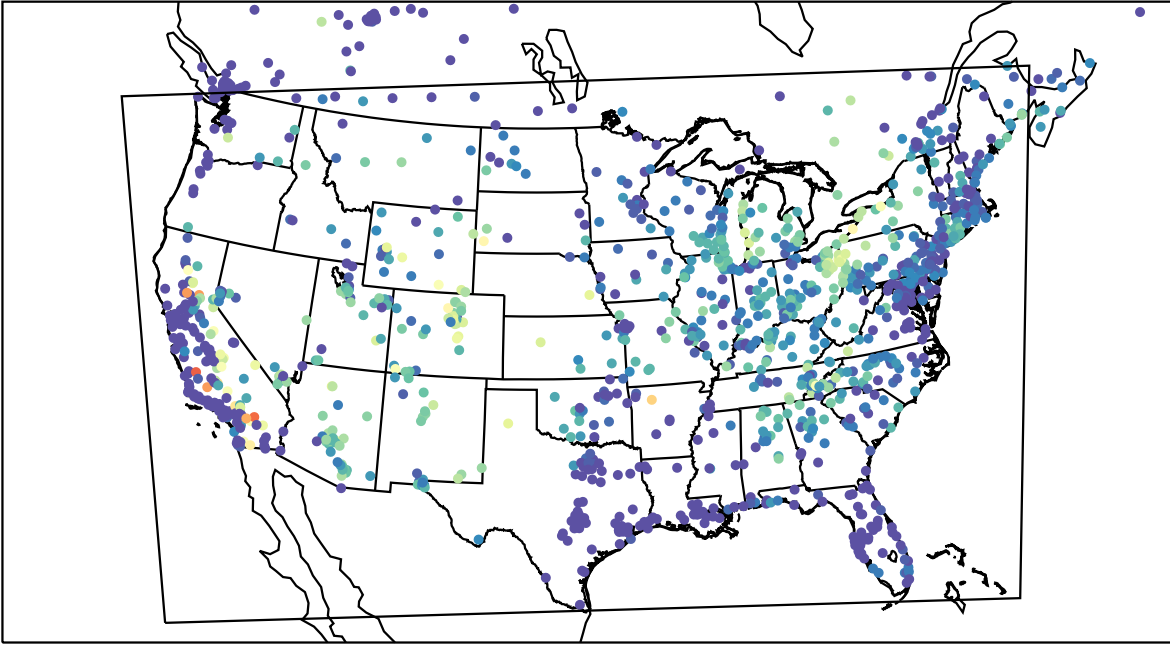
AirNOW (2023-07-16_13:00:00)
