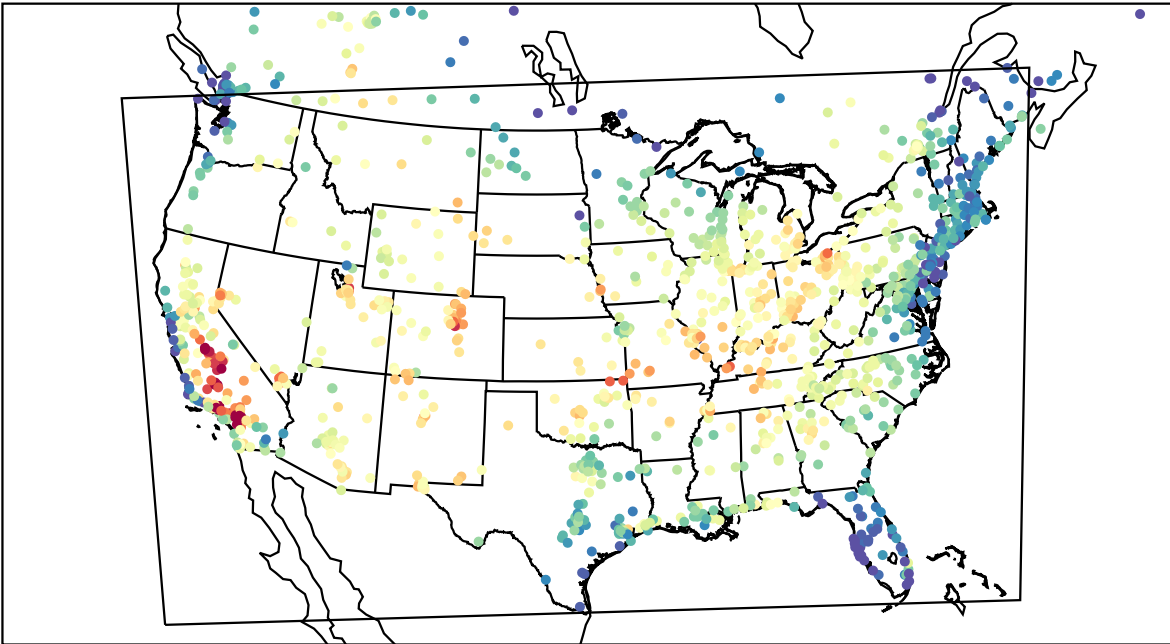
AirNOW (2023-07-16_18:00:00)
