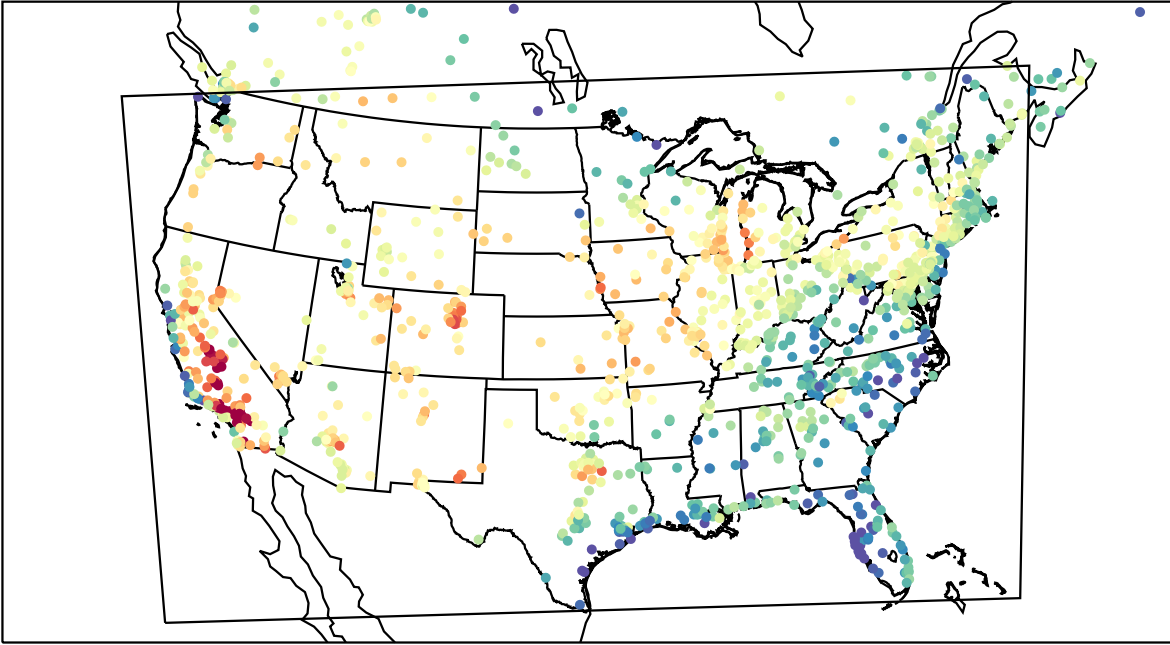
AirNOW (2023-07-15_21:00:00)
