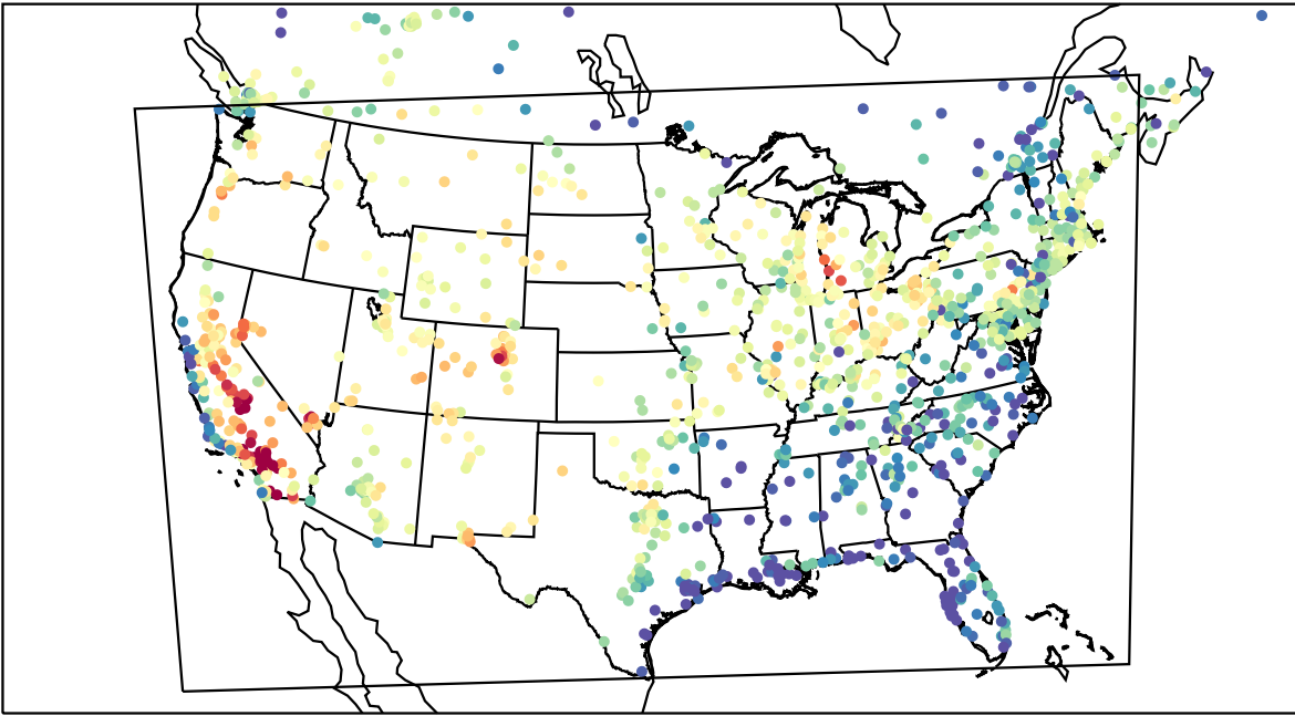
AirNOW (2023-07-15_00:00:00)
