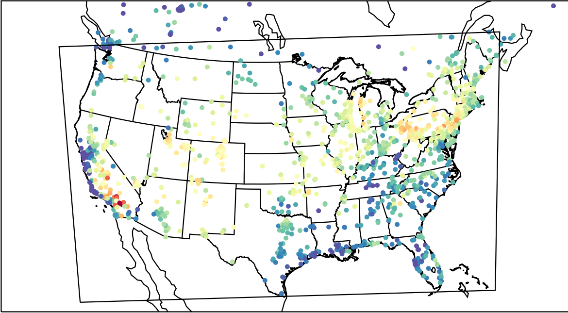
AirNOW (2023-07-15_16:00:00)
