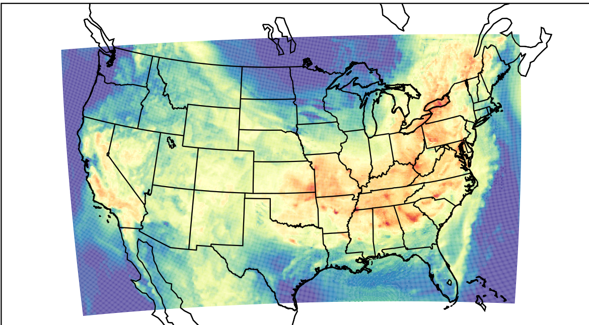
WRF (2023-07-16_16:00:00)
