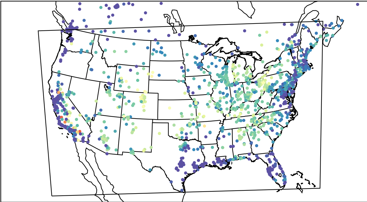
AirNOW (2023-07-16_14:00:00)
