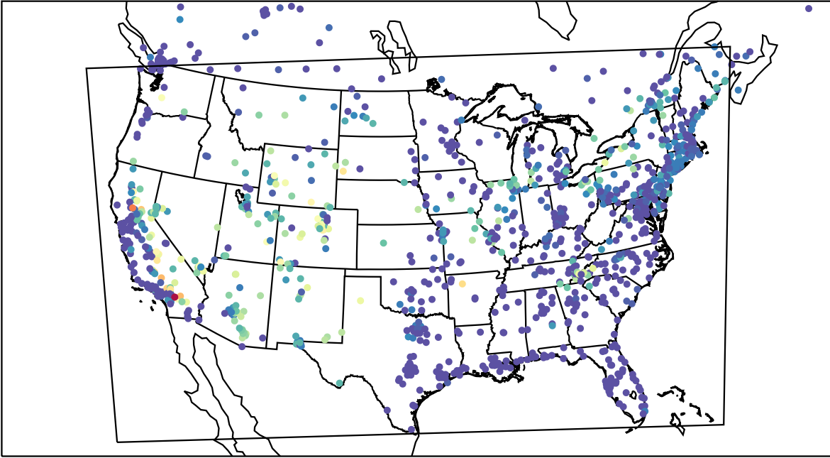
AirNOW (2023-07-16_10:00:00)
