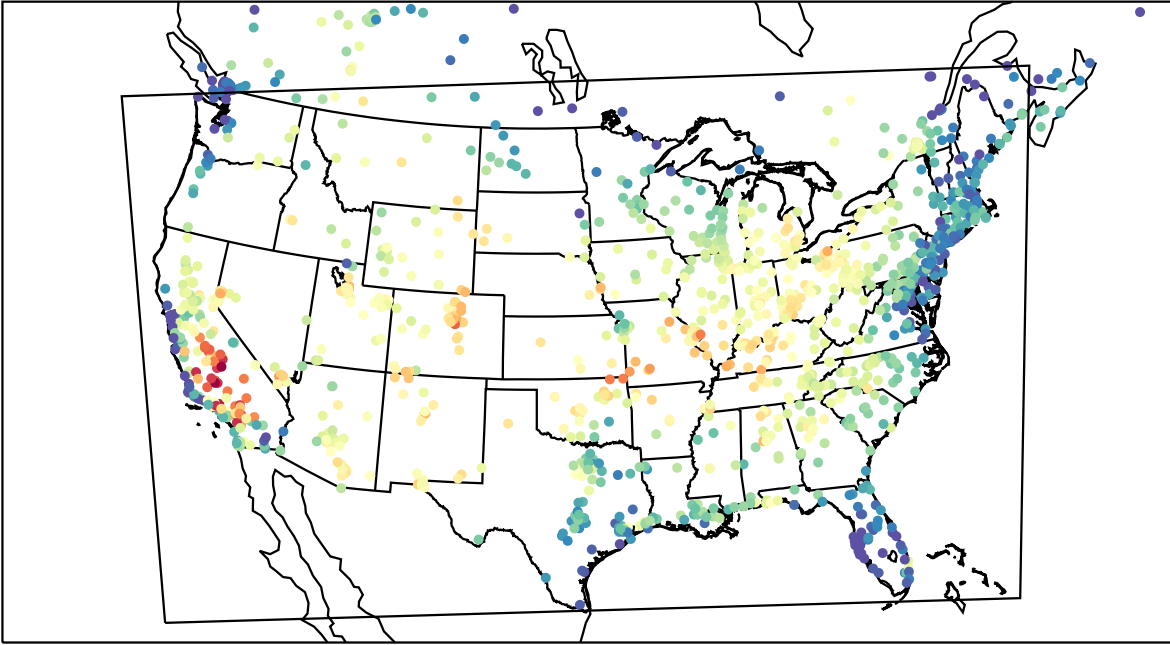
AirNOW (2023-07-16_17:00:00)
