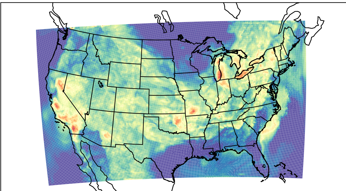
WRF (2023-07-16_06:00:00)
