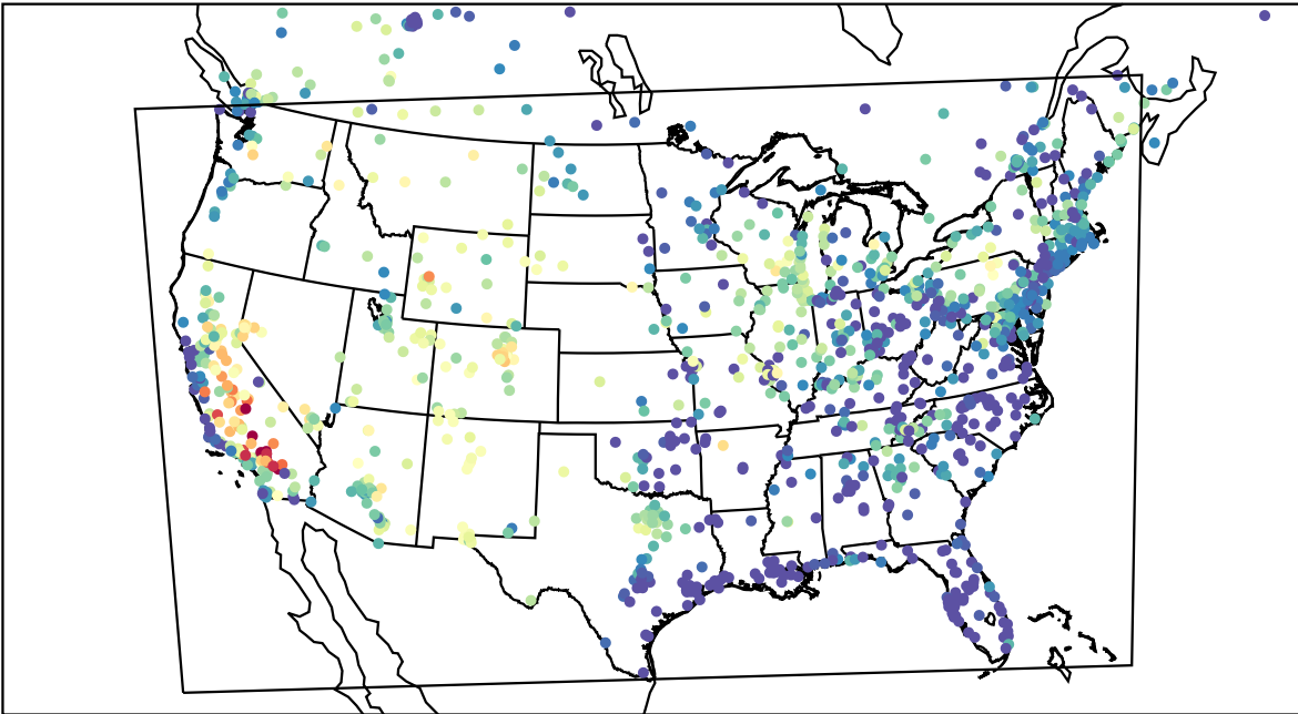
AirNOW (2023-07-16_03:00:00)
