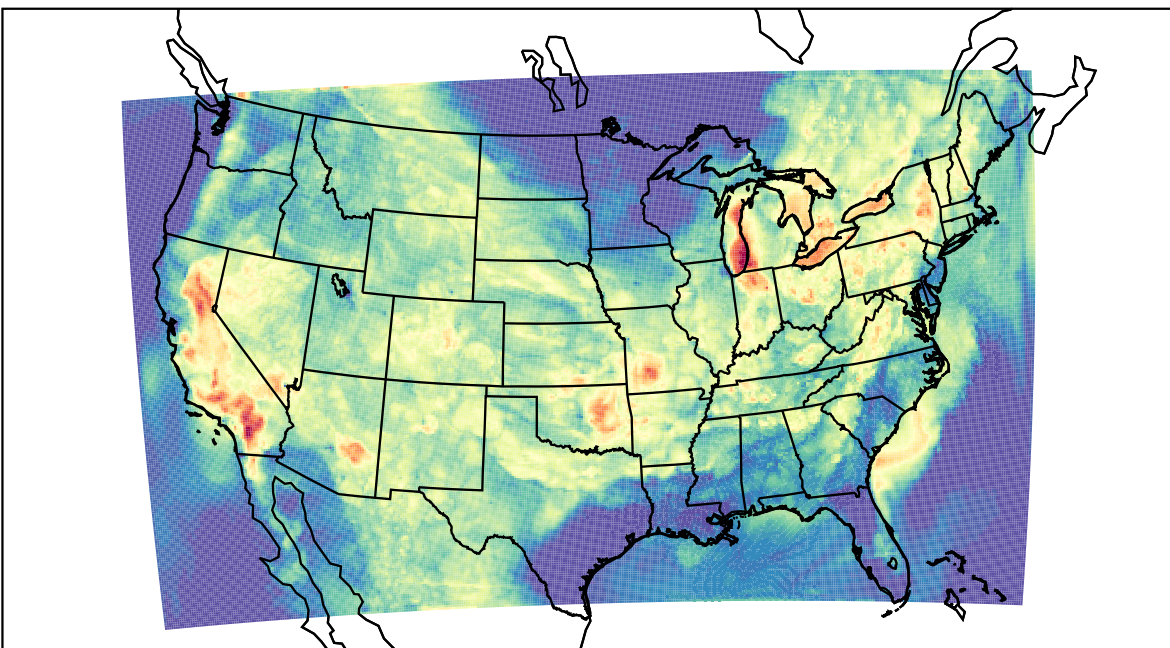
WRF (2023-07-16_04:00:00)
