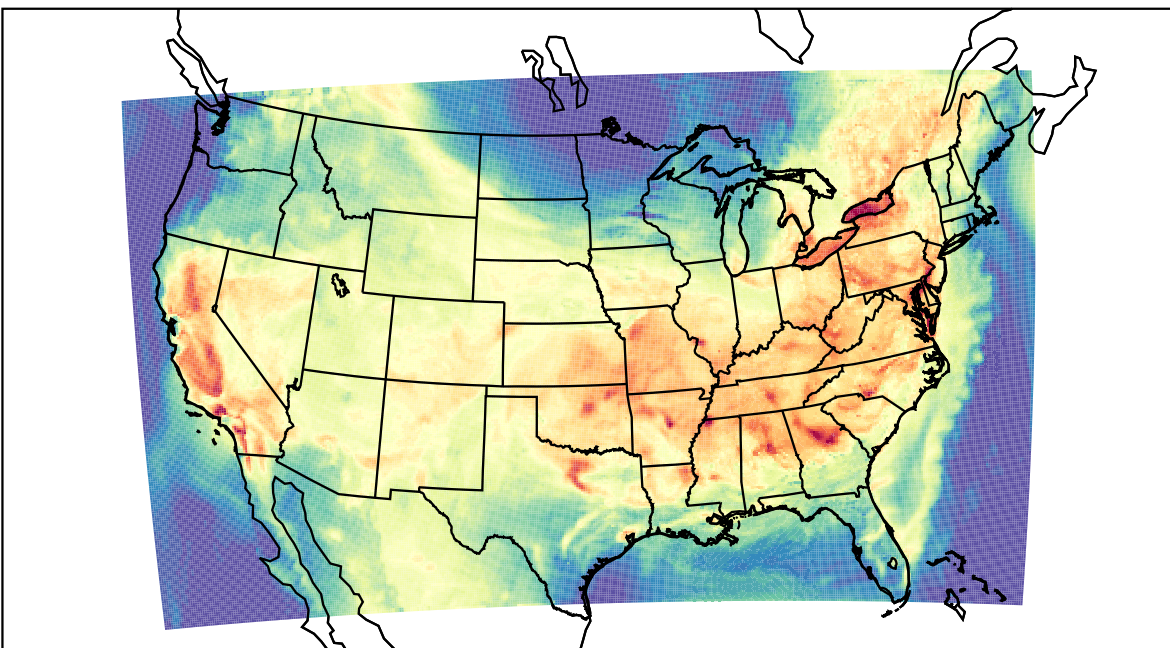
WRF (2023-07-16_18:00:00)
