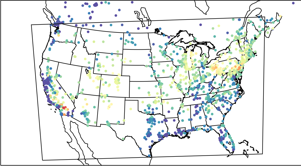
AirNOW (2023-07-15_15:00:00)
