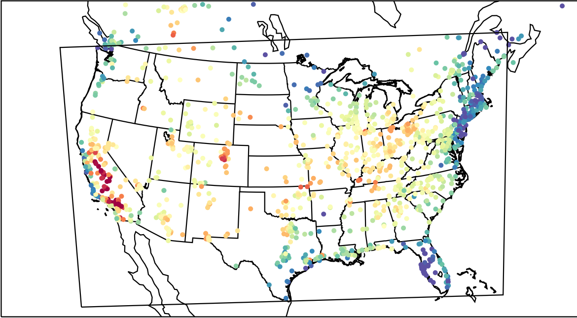
AirNOW (2023-07-16_21:00:00)
