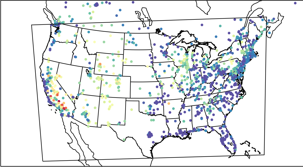
AirNOW (2023-07-16_04:00:00)
