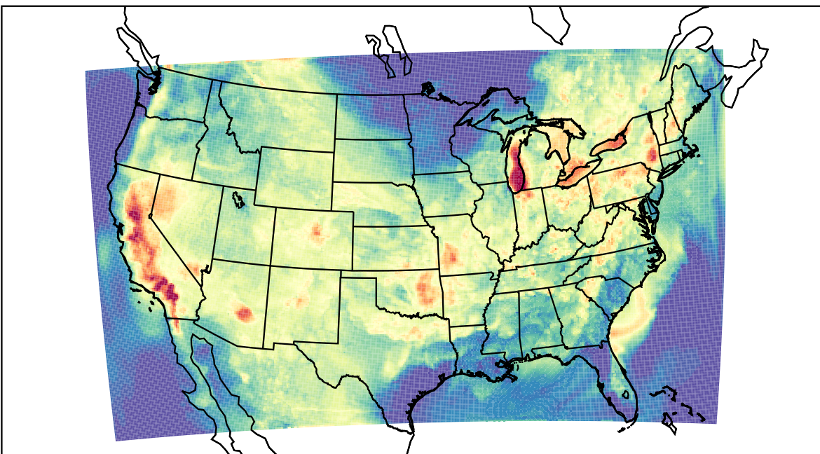
WRF (2023-07-16_02:00:00)
