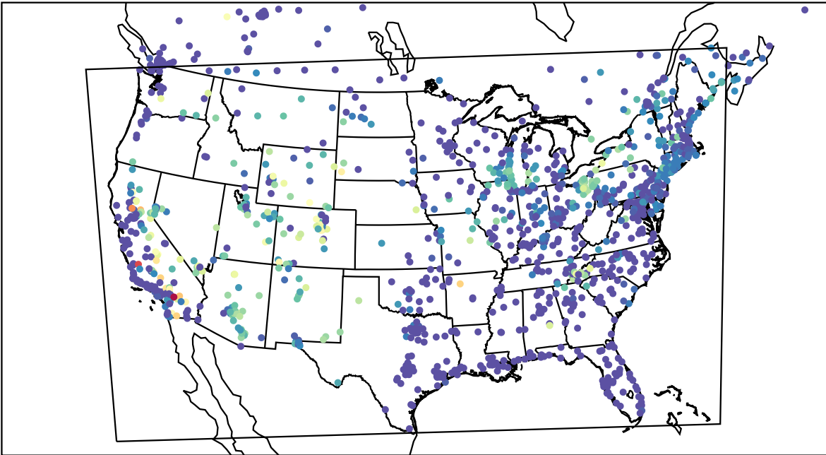
AirNOW (2023-07-16_11:00:00)
