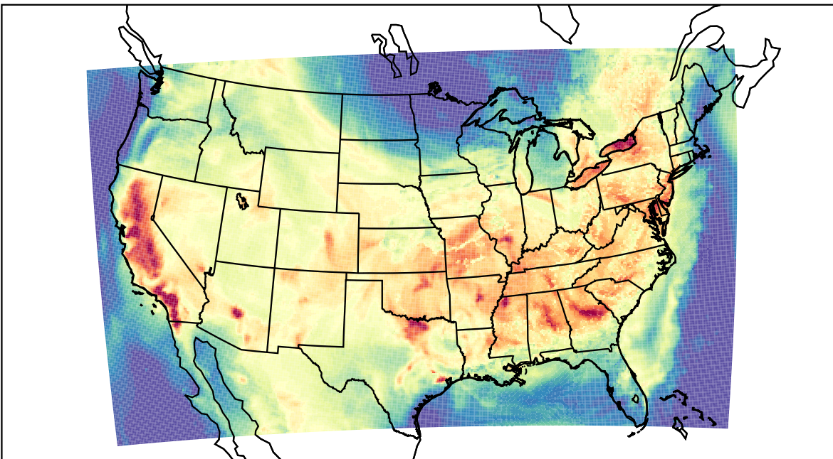
WRF (2023-07-16_22:00:00)
