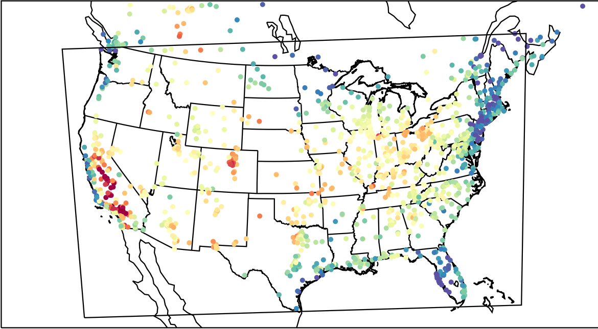
AirNOW (2023-07-16_22:00:00)
