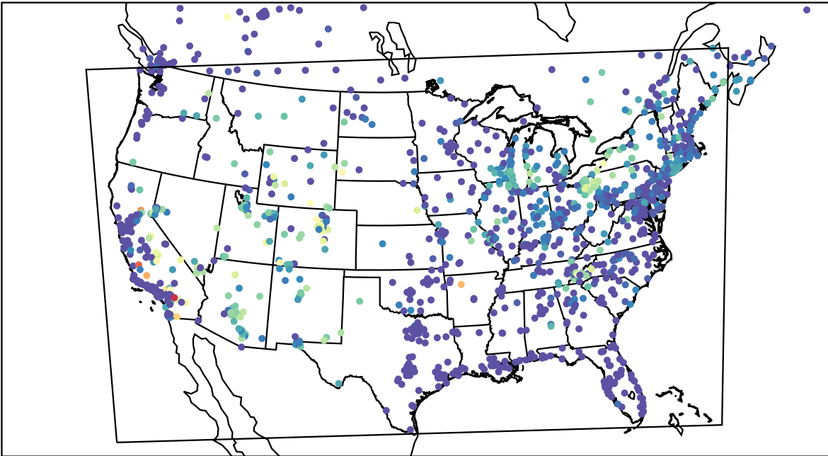
AirNOW (2023-07-16_12:00:00)
