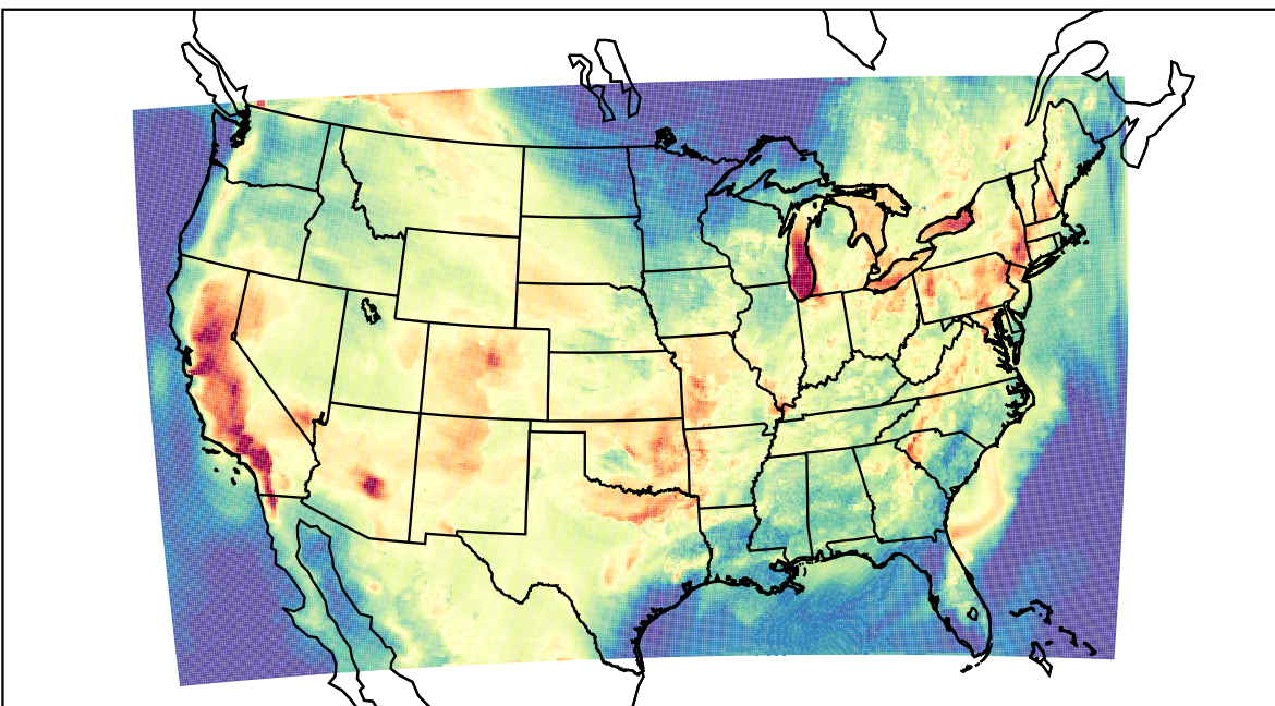
WRF (2023-07-16_00:00:00)
