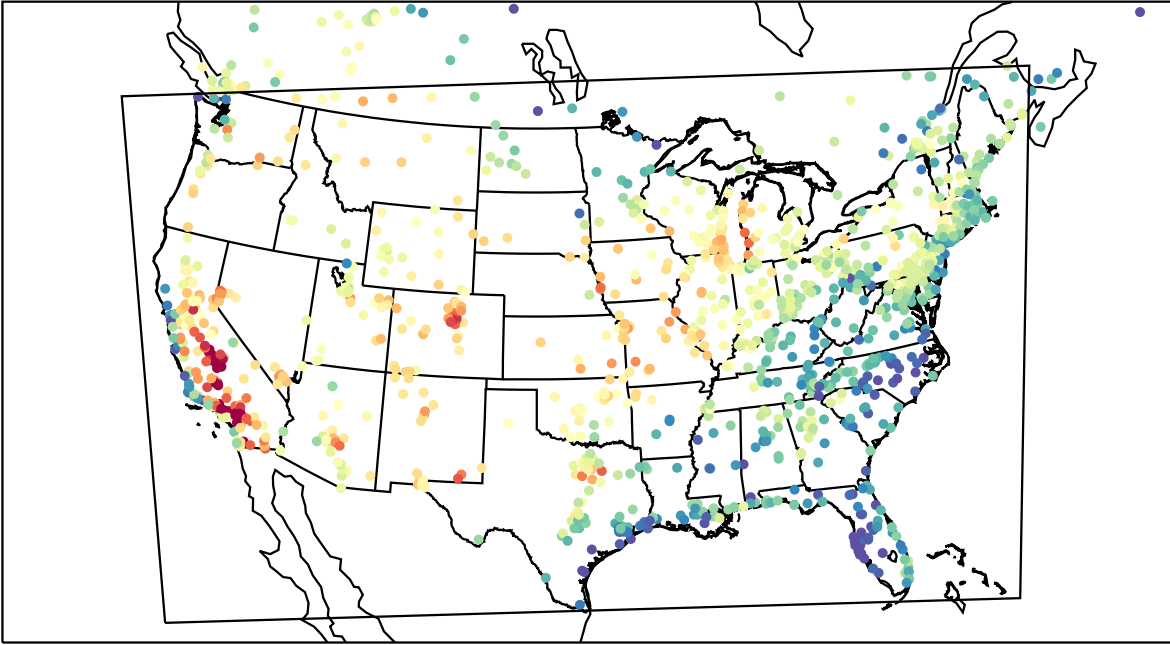
AirNOW (2023-07-15_22:00:00)
