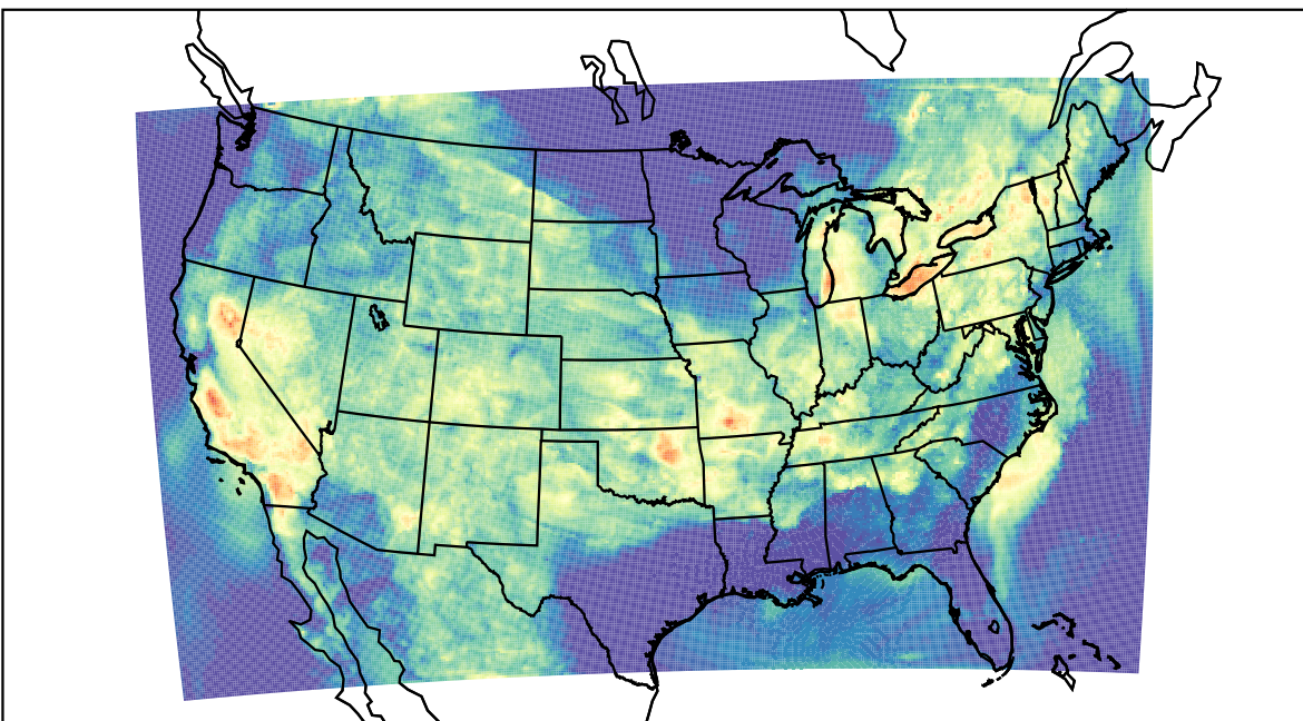
WRF (2023-07-16_08:00:00)
