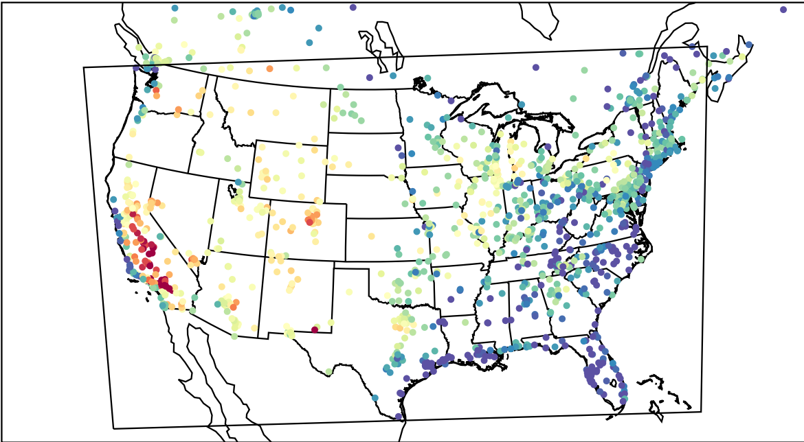
AirNOW (2023-07-16_01:00:00)
