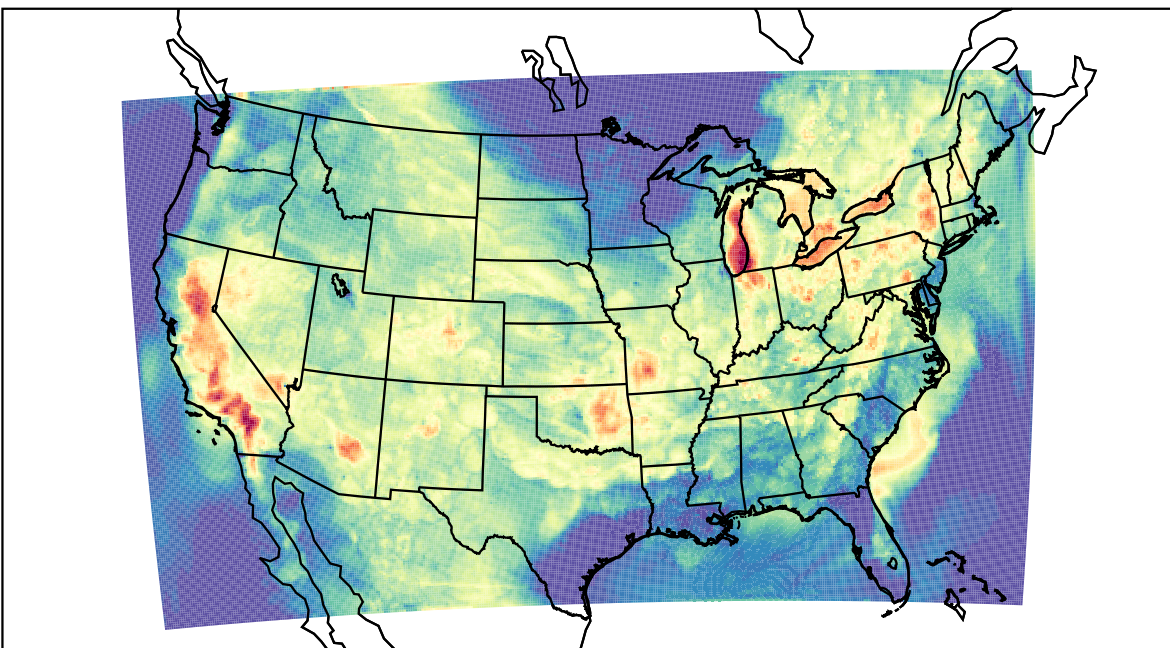
WRF (2023-07-16_03:00:00)
