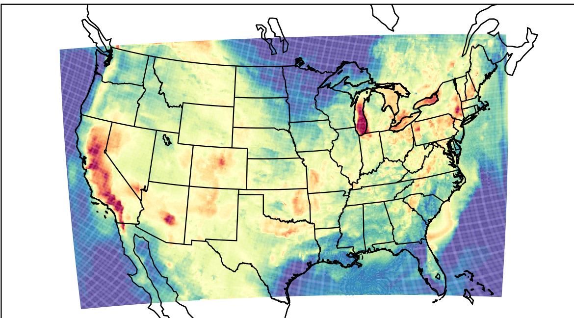
WRF (2023-07-16_01:00:00)
