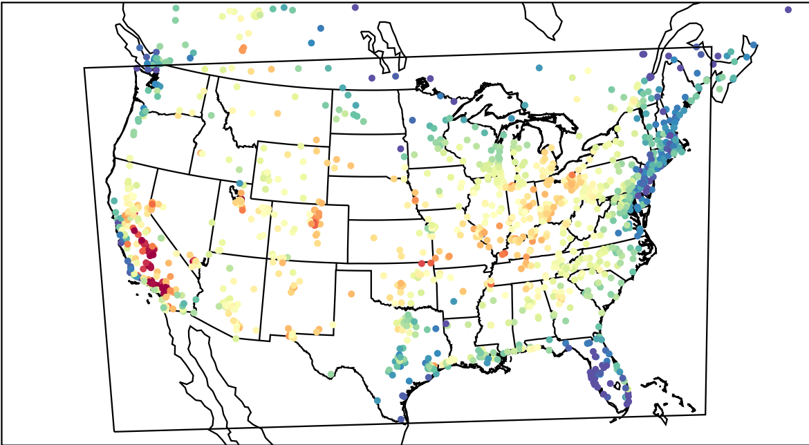
AirNOW (2023-07-16_19:00:00)
