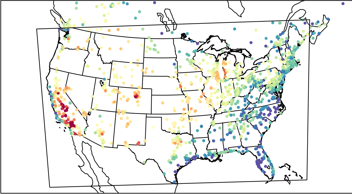
AirNOW (2023-07-15_23:00:00)
