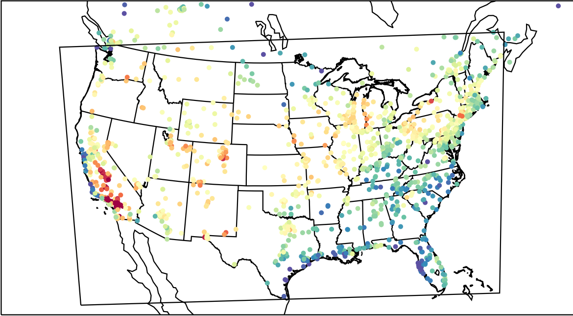
AirNOW (2023-07-15_19:00:00)
