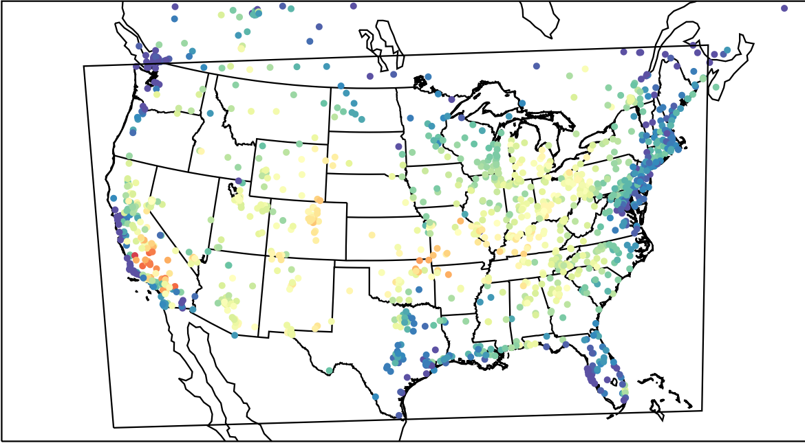
AirNOW (2023-07-16_16:00:00)
