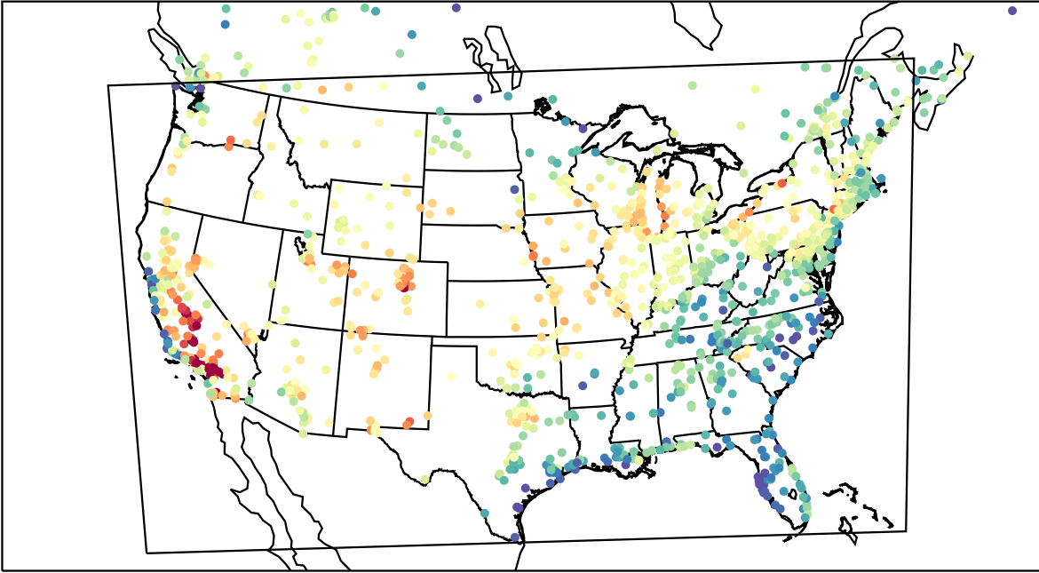
AirNOW (2023-07-15_20:00:00)
