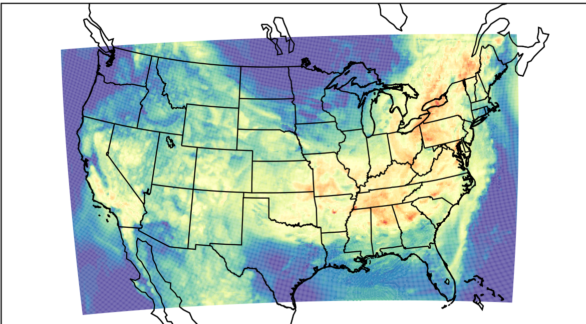
WRF (2023-07-16_15:00:00)
