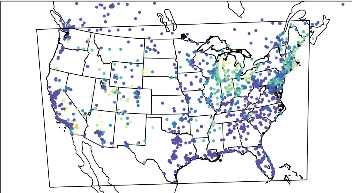
AirNOW (2023-07-15_12:00:00)
