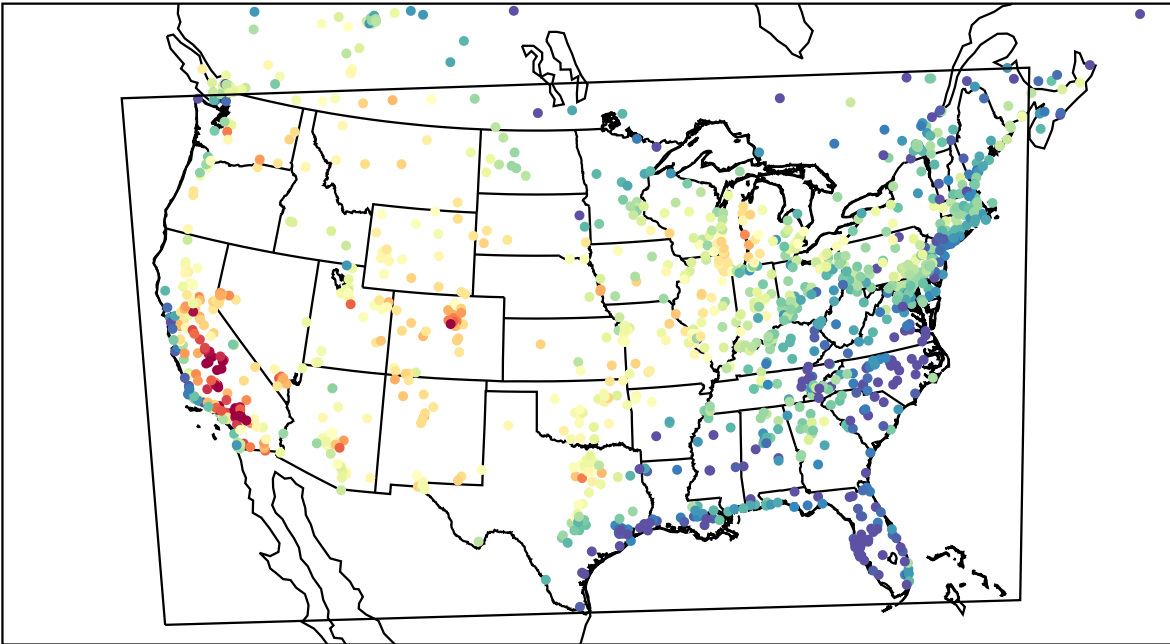
AirNOW (2023-07-16_00:00:00)
