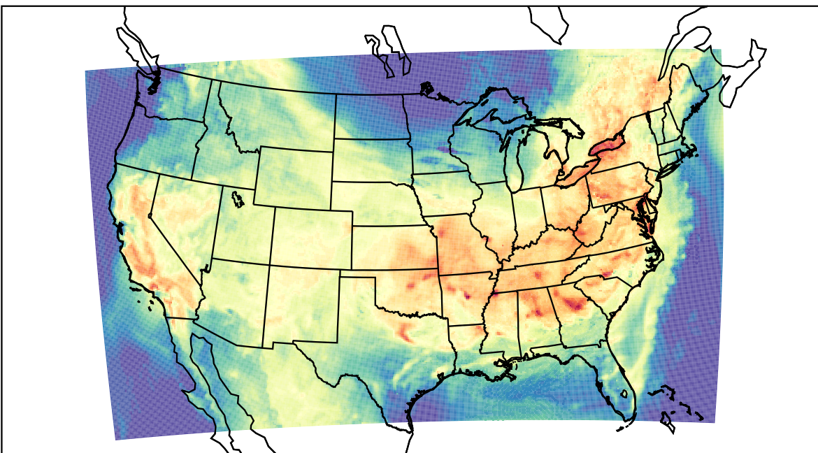
WRF (2023-07-16_17:00:00)
