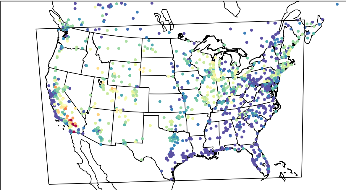
AirNOW (2023-07-15_04:00:00)
