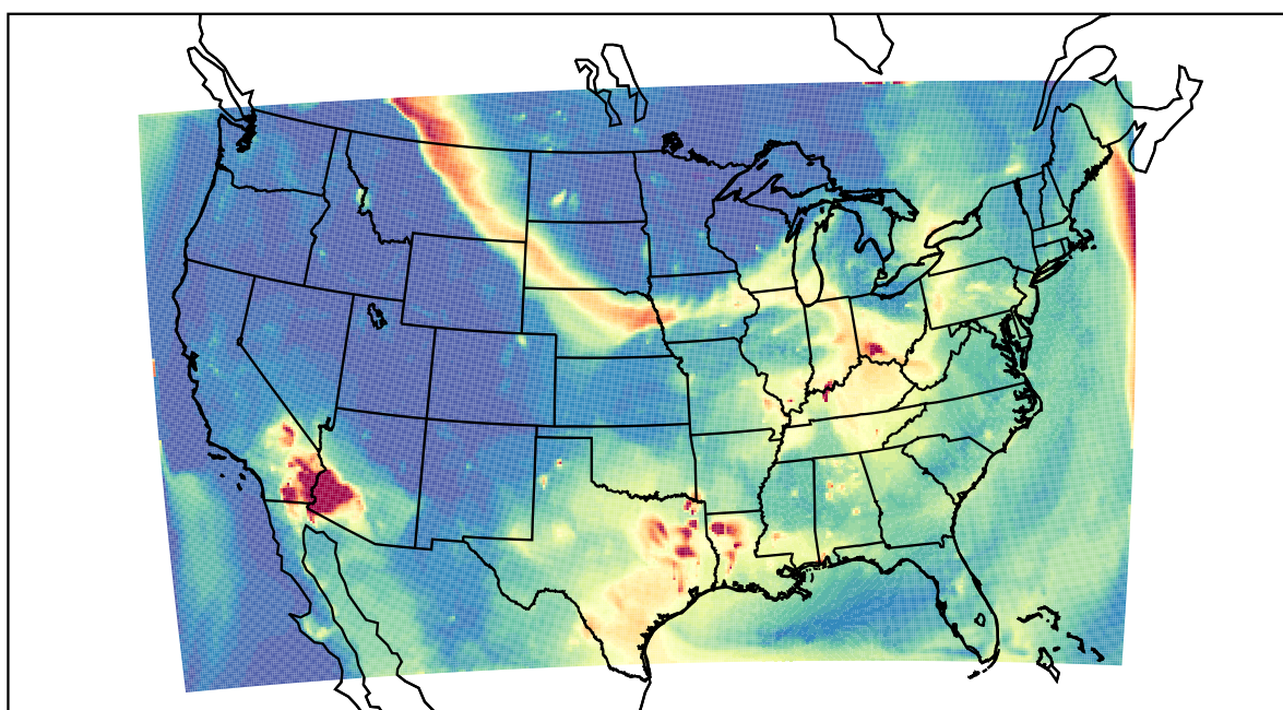
WRF 2023-07-17_05:00:00
