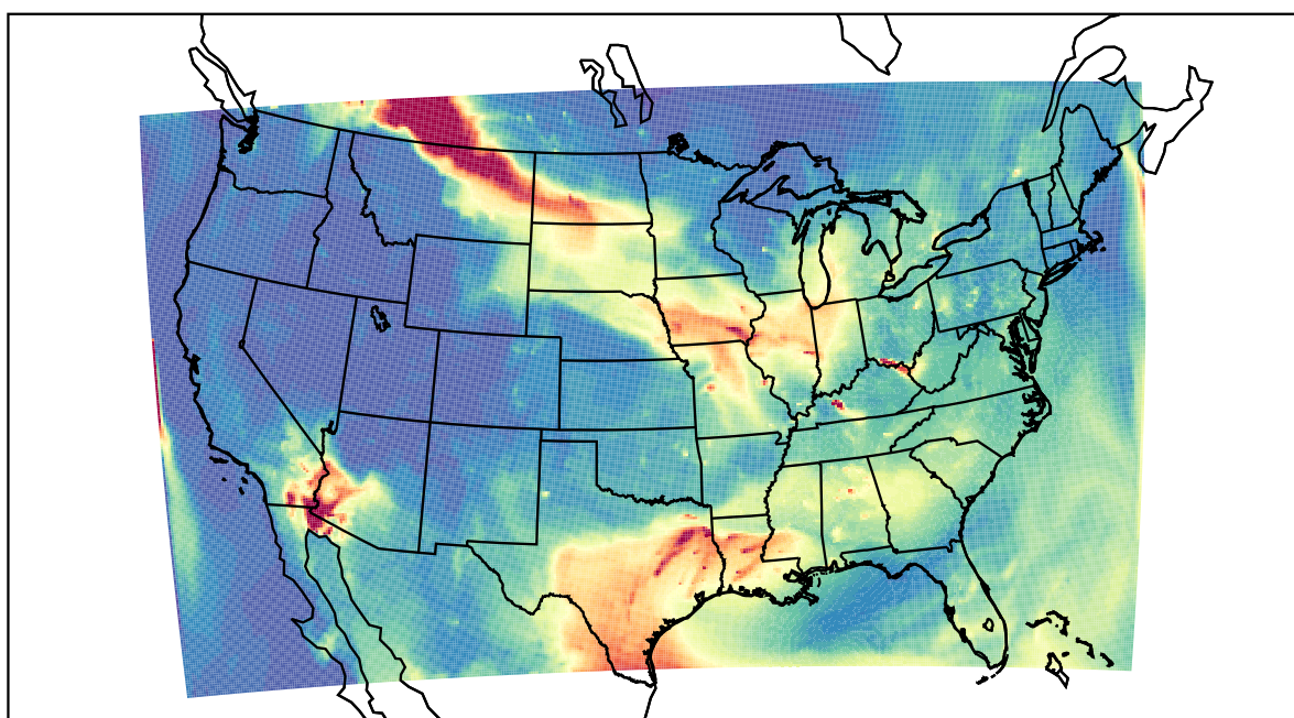
WRF 2023-07-16_11:00:00
