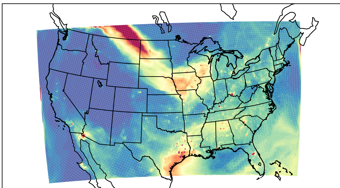
WRF 2023-07-16_01:00:00
