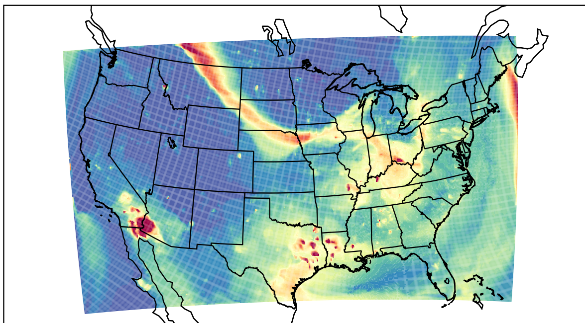
WRF 2023-07-17_03:00:00
