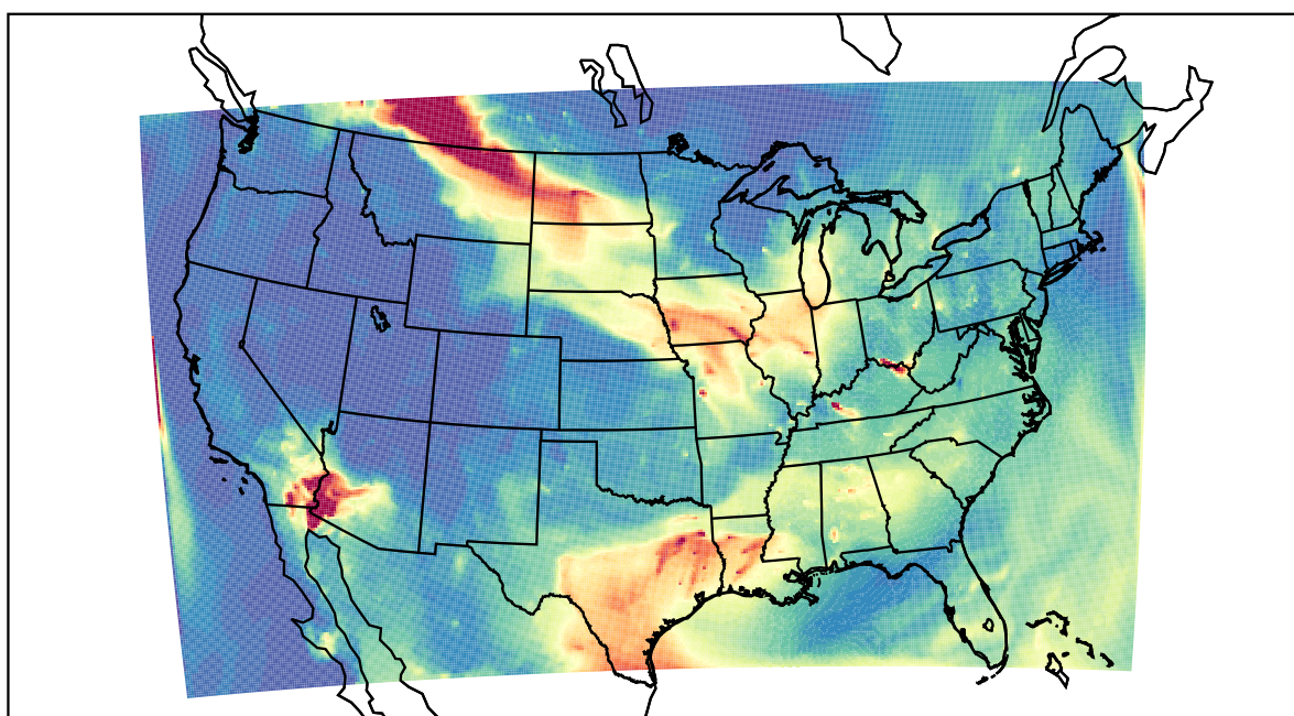
WRF 2023-07-16_09:00:00
