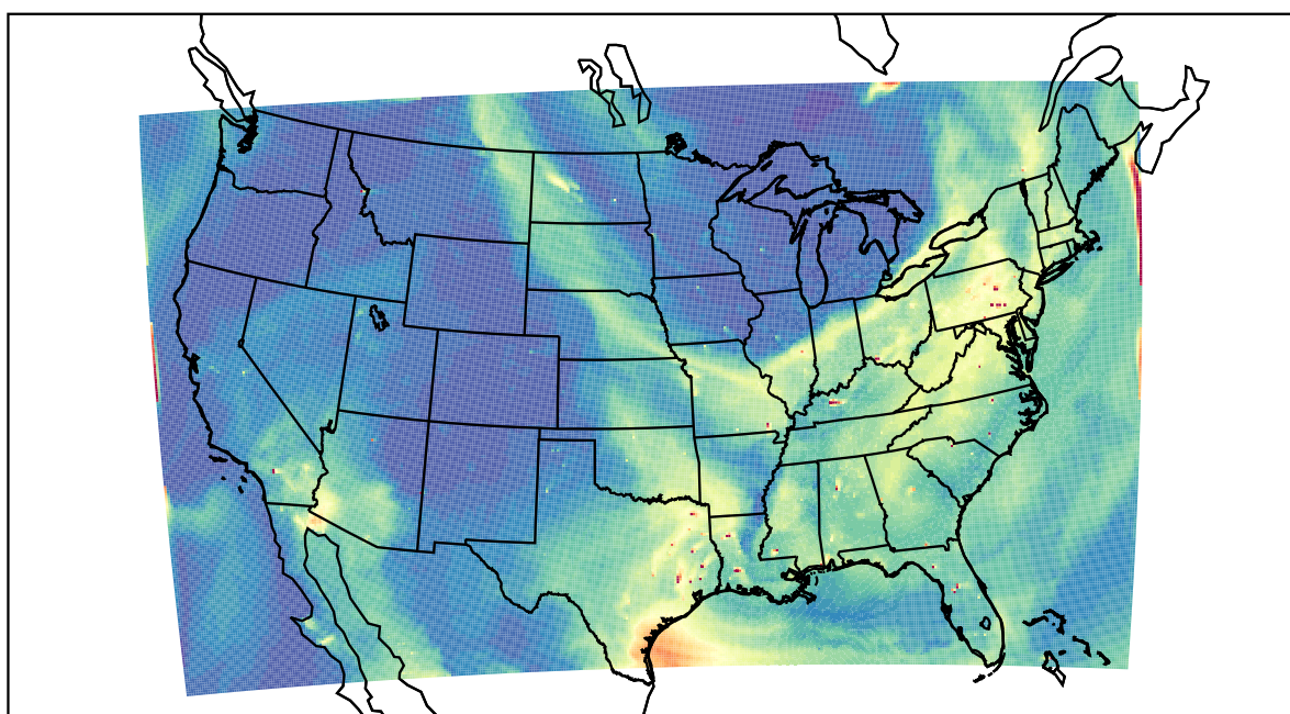
WRF 2023-07-17_23:00:00
