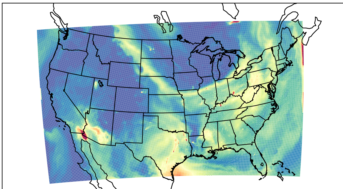
WRF 2023-07-17_17:00:00
