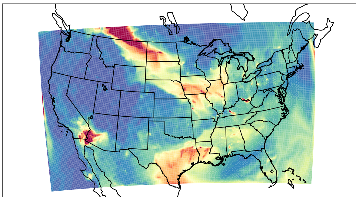
WRF 2023-07-16_08:00:00
