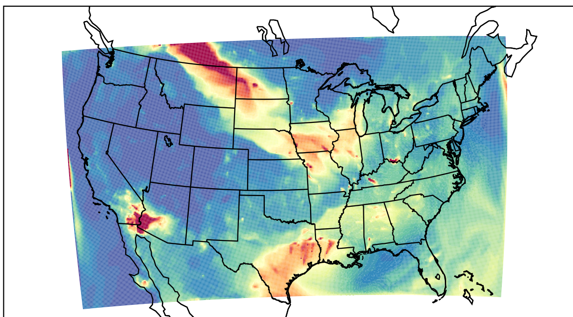
WRF 2023-07-16_06:00:00
