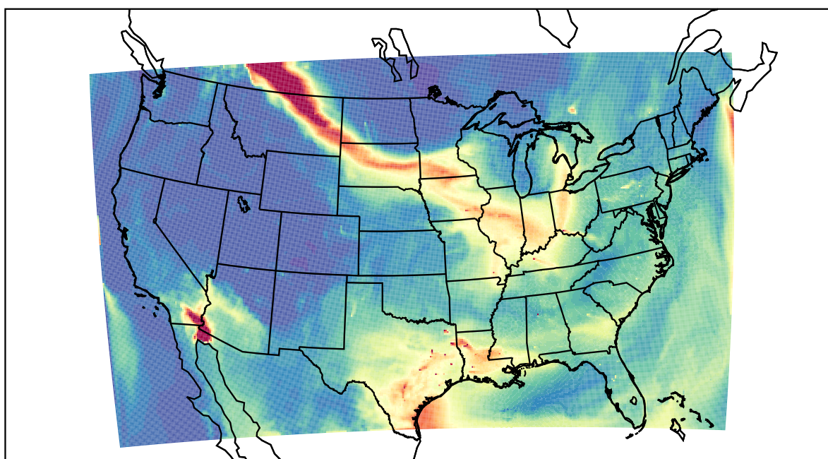
WRF 2023-07-16_18:00:00
