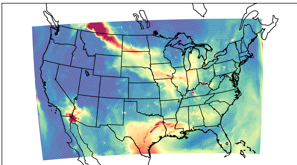
WRF 2023-07-16_13:00:00
