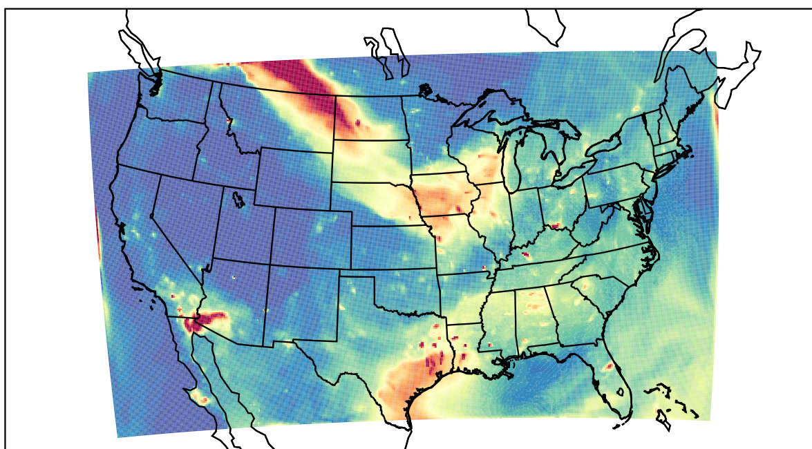
WRF 2023-07-16_03:00:00
