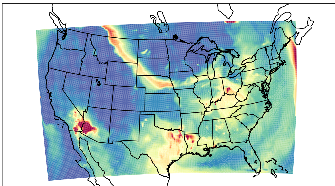
WRF 2023-07-17_07:00:00
