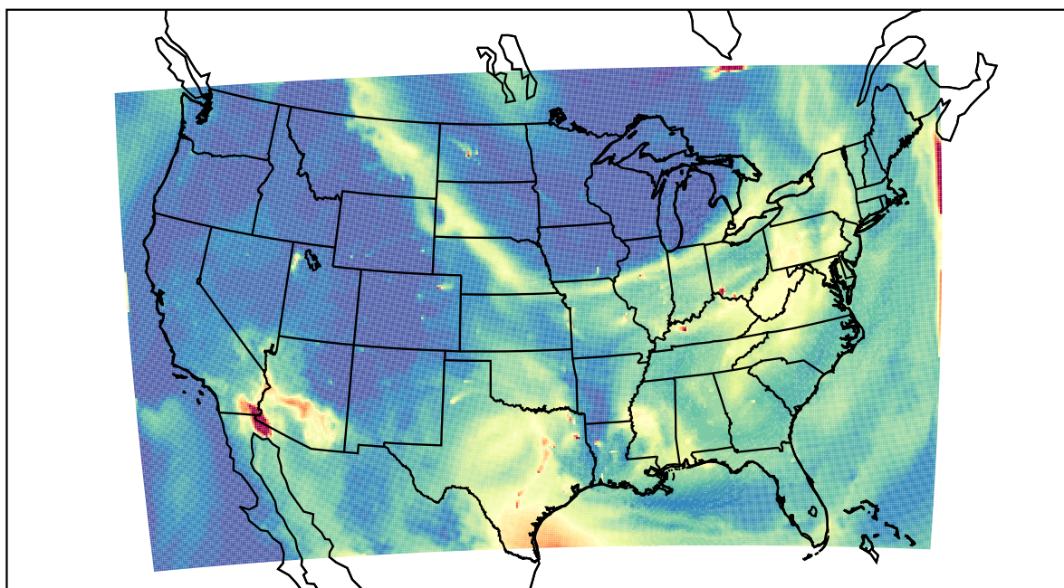
WRF 2023-07-17_16:00:00
