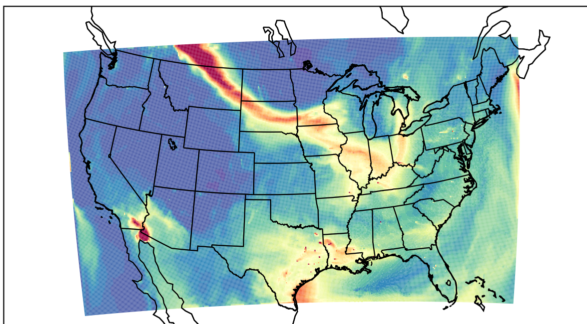
WRF 2023-07-16_19:00:00
