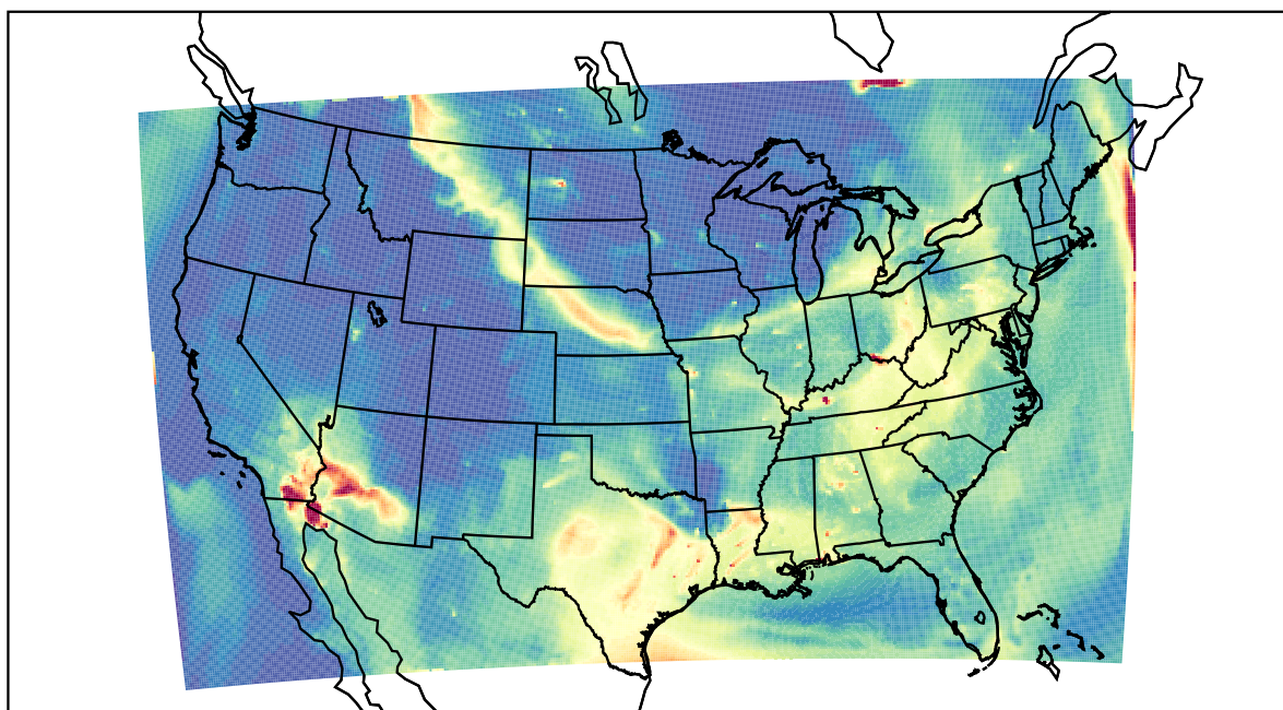
WRF 2023-07-17_12:00:00
