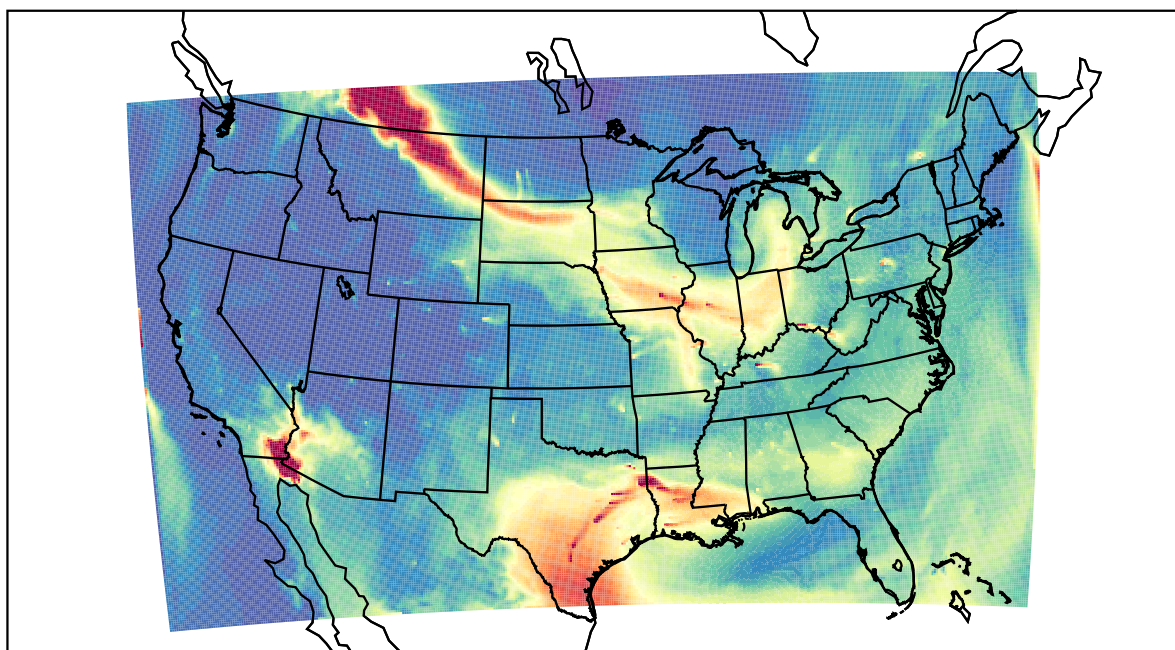
WRF 2023-07-16_15:00:00
