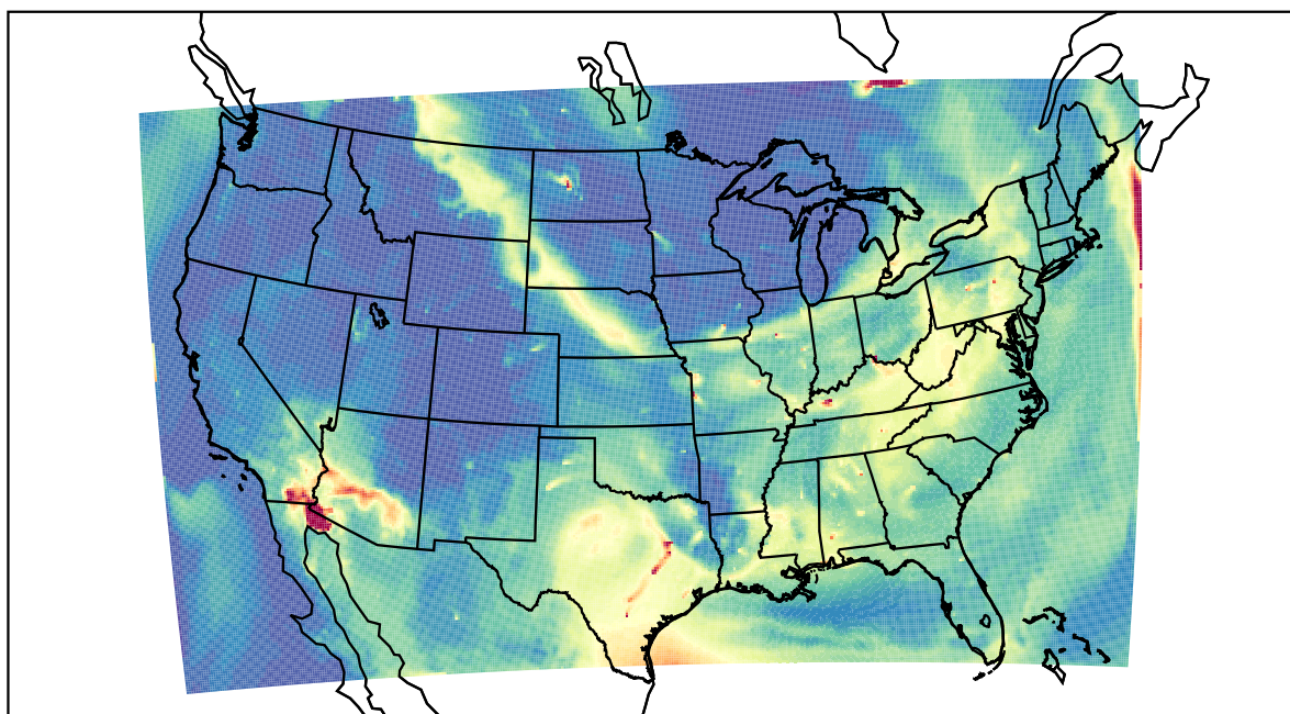
WRF 2023-07-17_14:00:00
