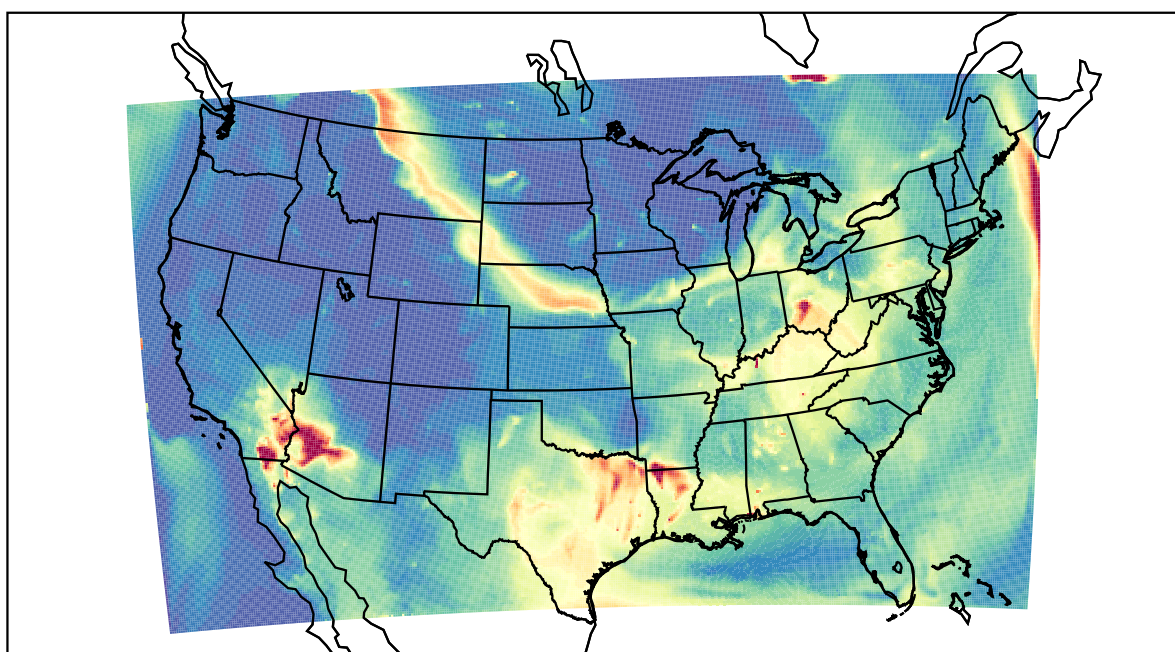
WRF 2023-07-17_09:00:00
