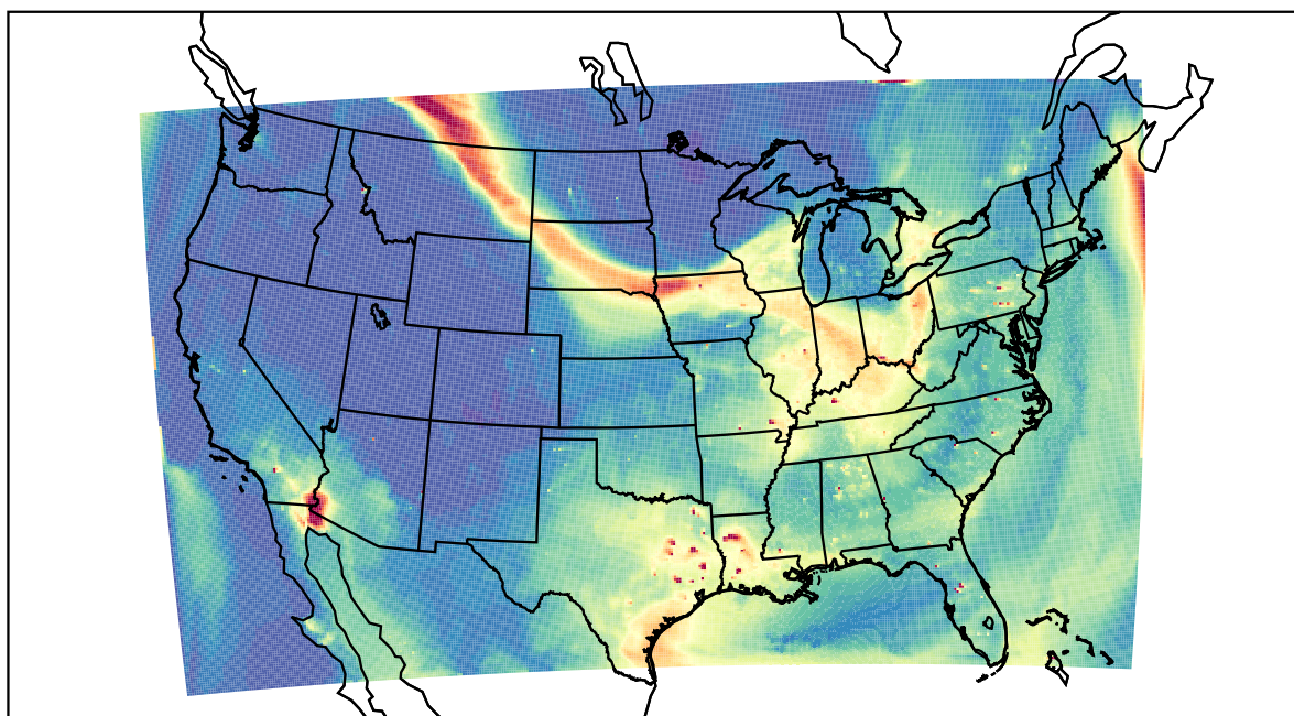
WRF 2023-07-17_00:00:00
