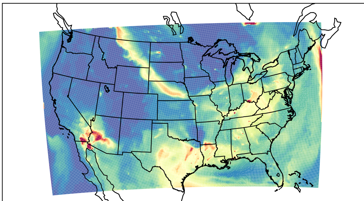
WRF 2023-07-17_11:00:00
