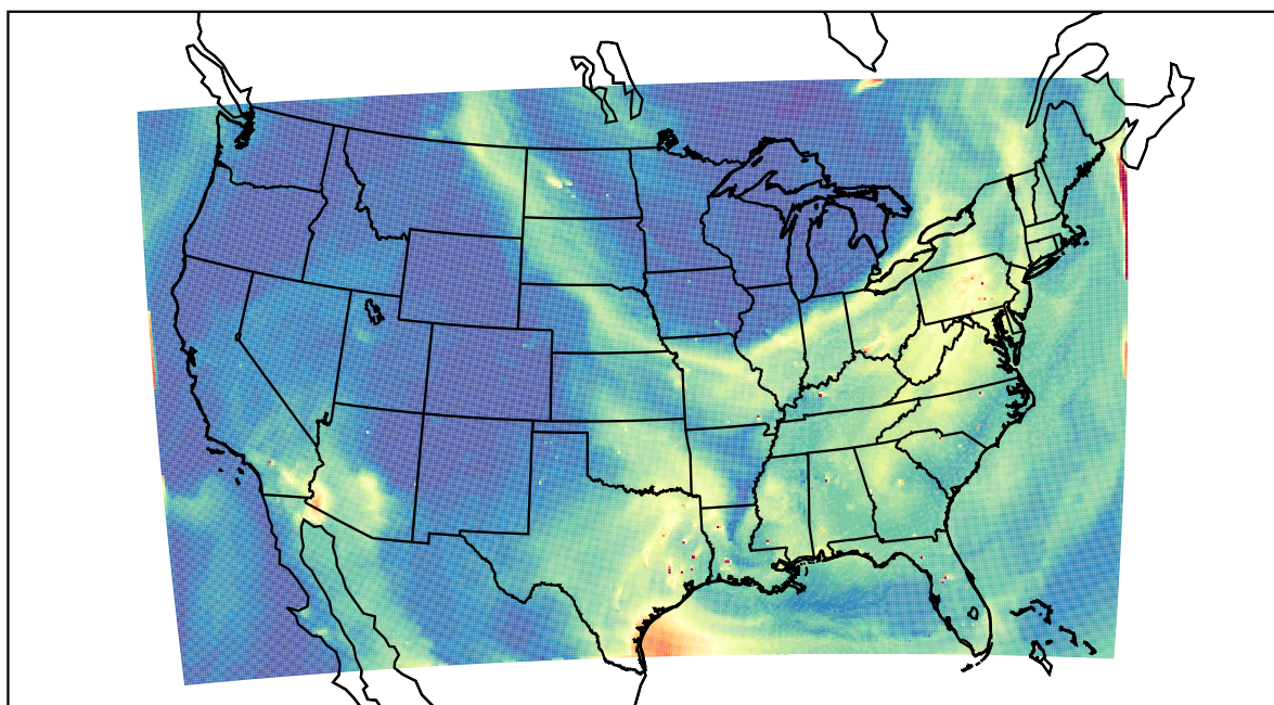
WRF 2023-07-17_21:00:00
