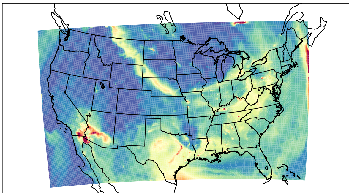
WRF 2023-07-17_13:00:00
