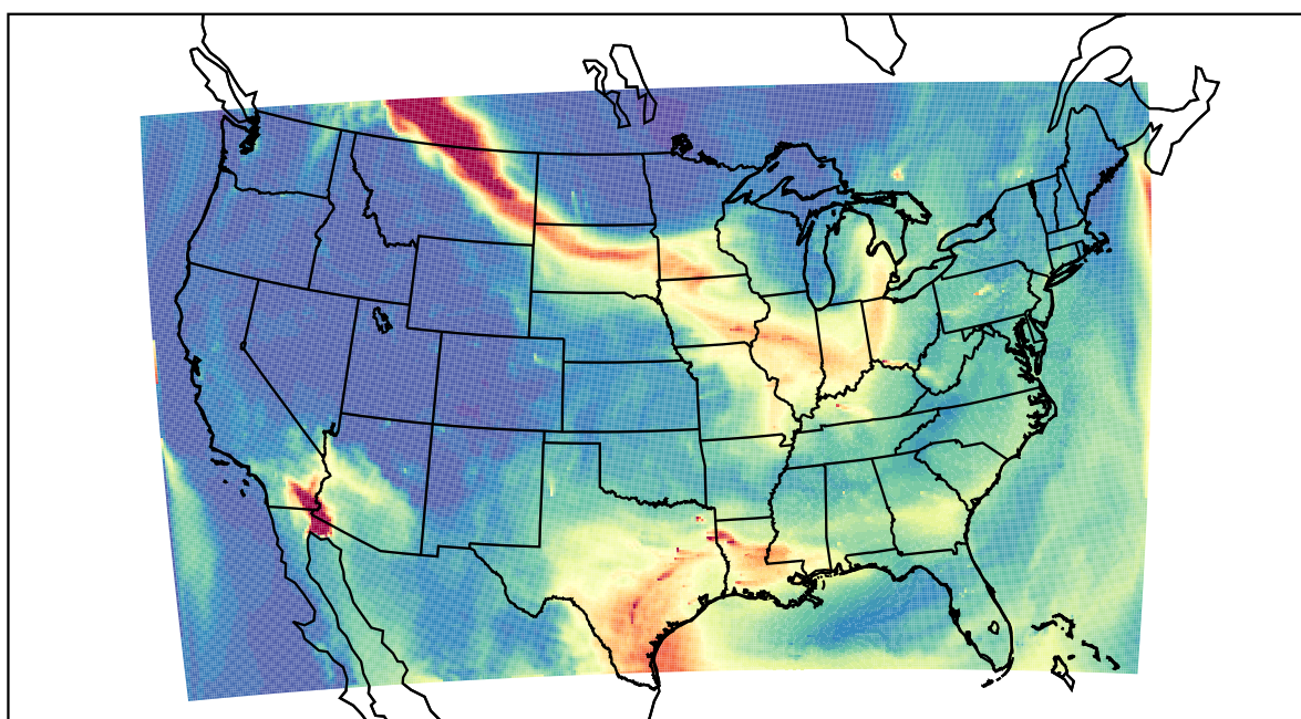
WRF 2023-07-16_17:00:00
