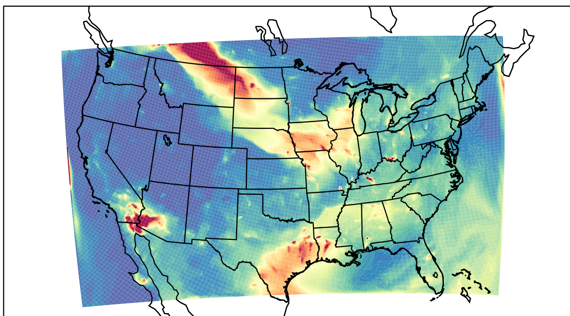
WRF 2023-07-16_05:00:00
