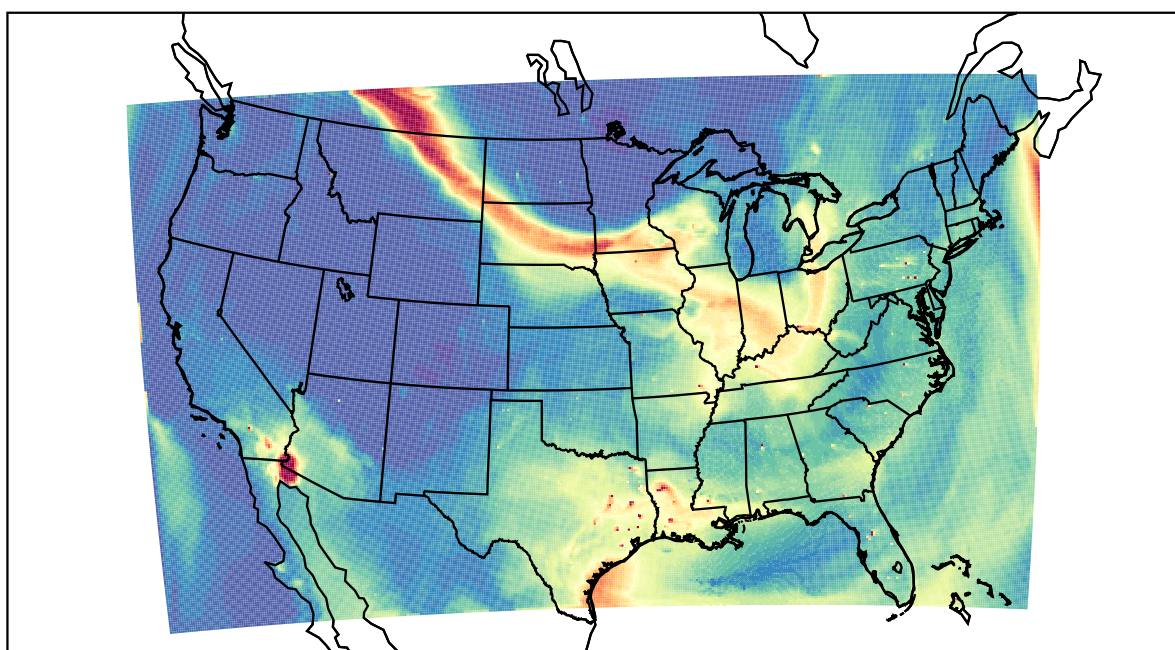
WRF 2023-07-16_21:00:00
