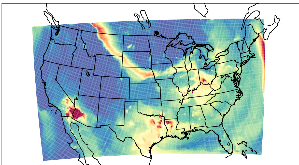
WRF 2023-07-17_06:00:00
