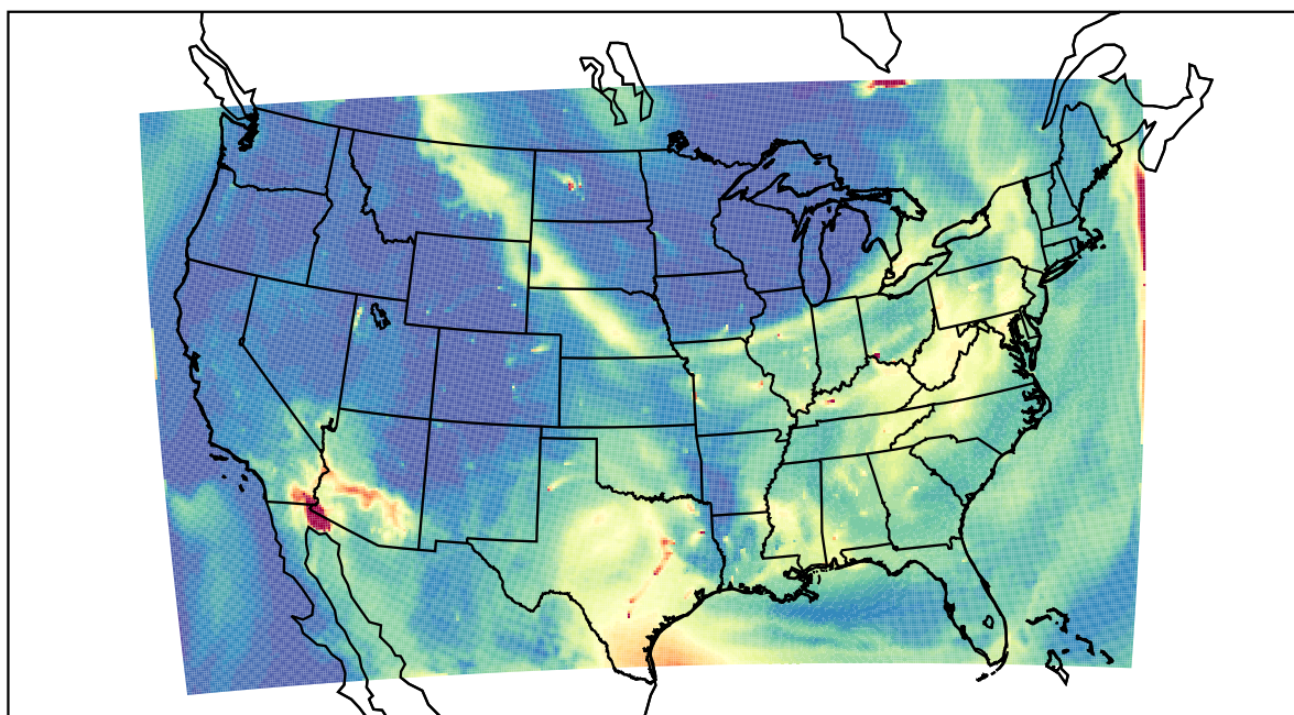
WRF 2023-07-17_15:00:00
