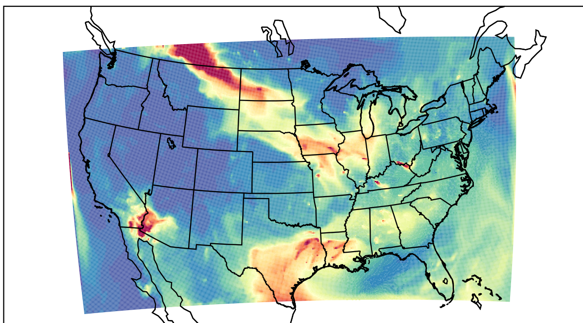
WRF 2023-07-16_10:00:00
