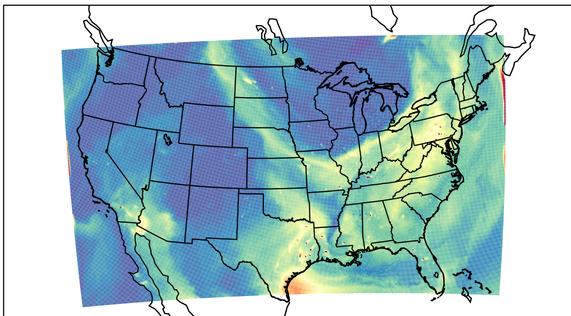
WRF 2023-07-17_22:00:00
