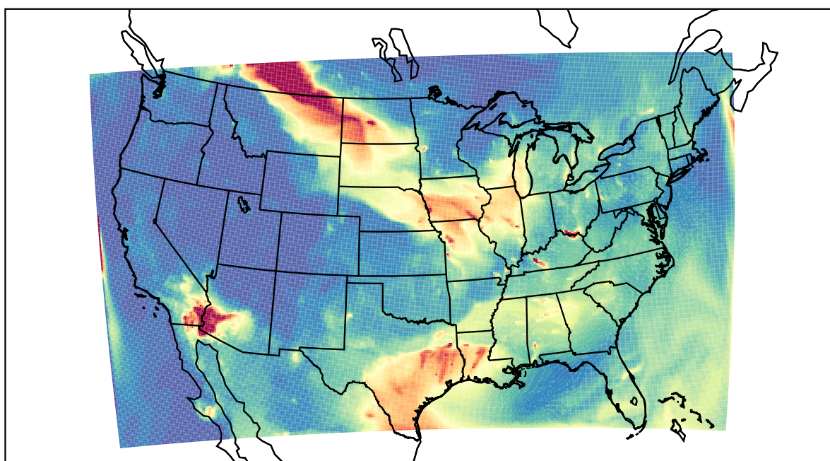
WRF 2023-07-16_07:00:00
