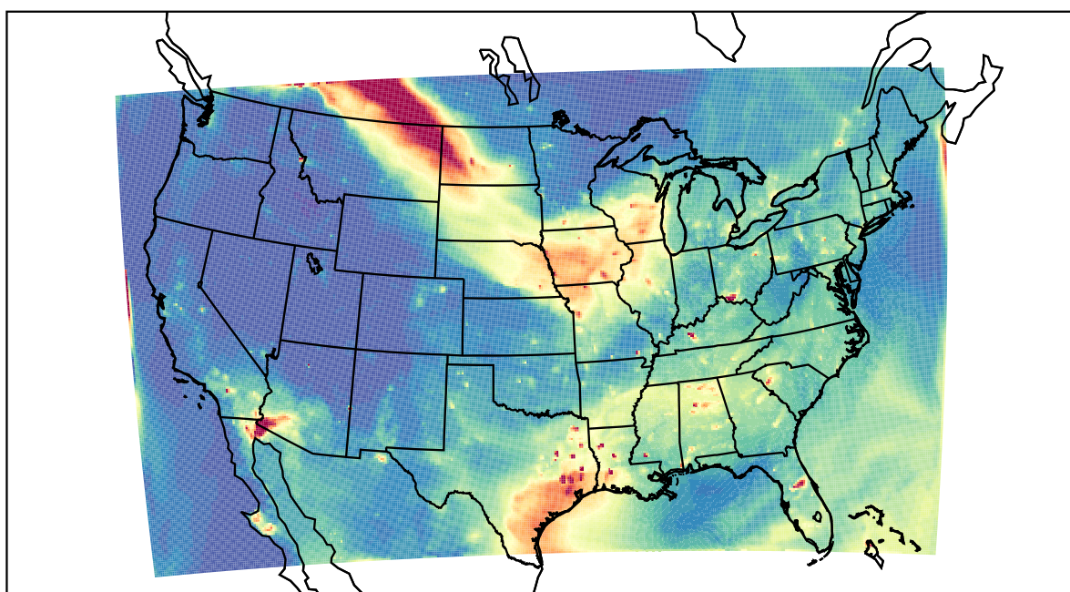
WRF 2023-07-16_02:00:00
