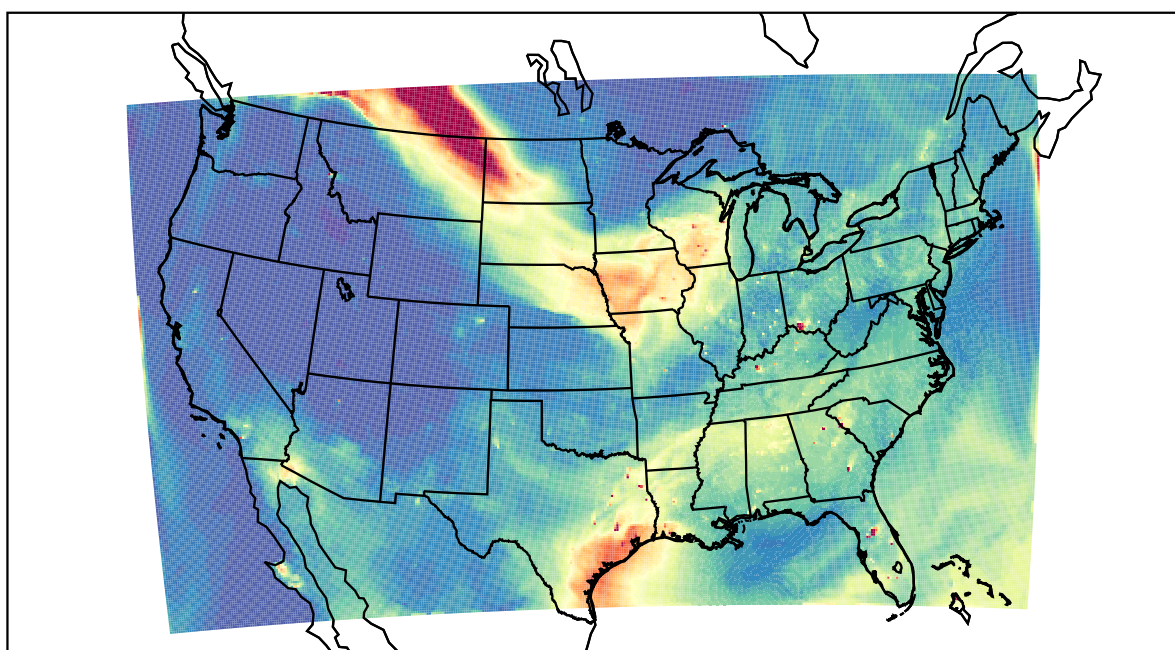
WRF 2023-07-16_00:00:00
