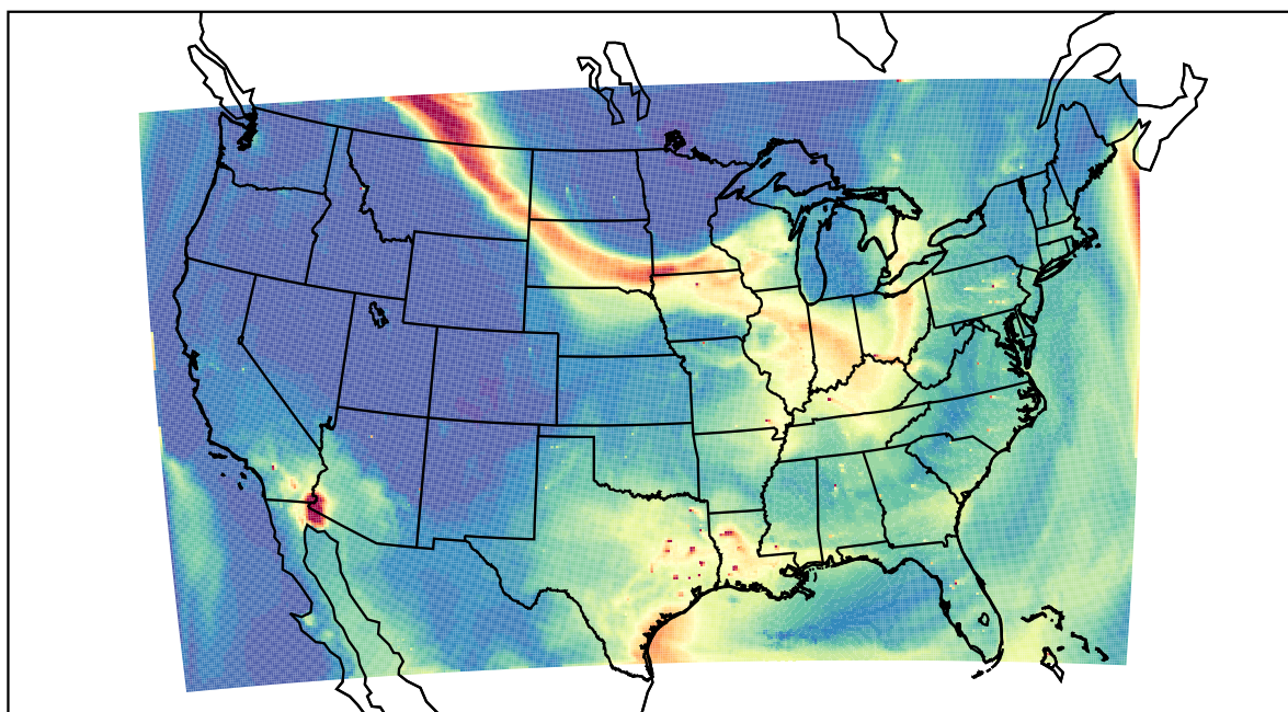
WRF 2023-07-16_22:00:00
