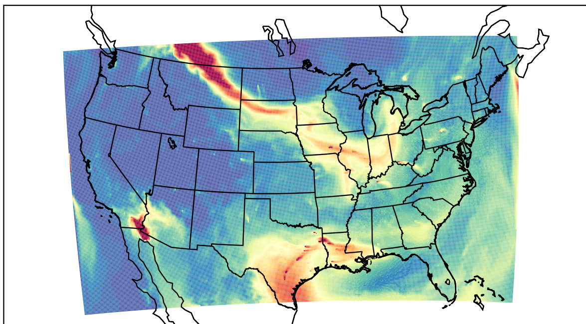
WRF 2023-07-16_16:00:00
