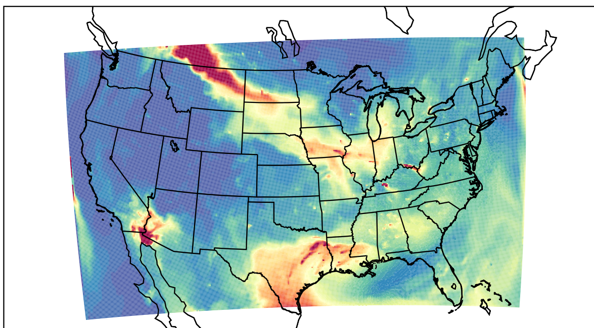
WRF 2023-07-16_12:00:00
