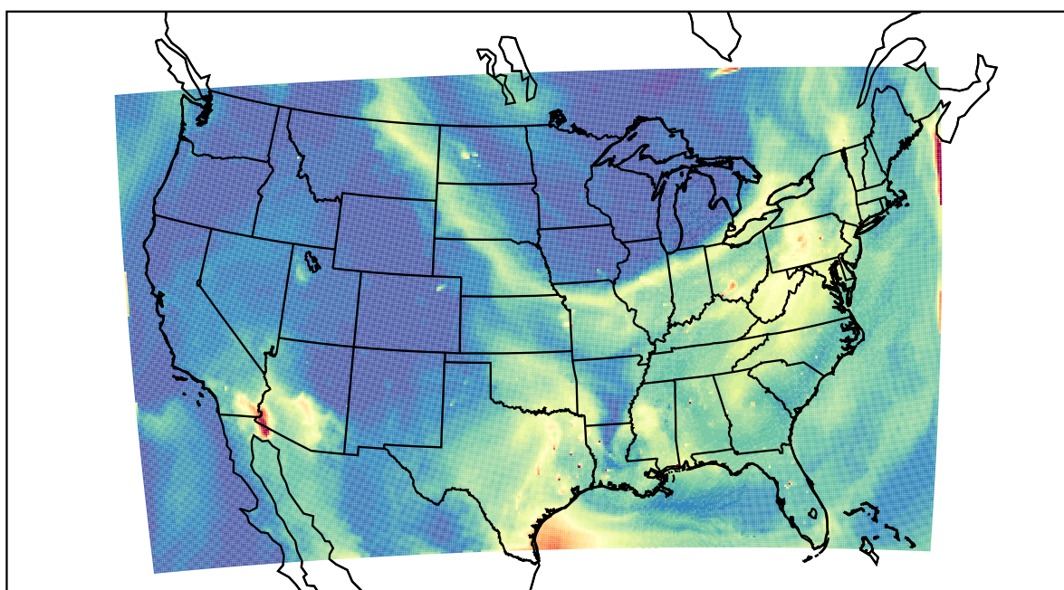
WRF 2023-07-17_19:00:00
