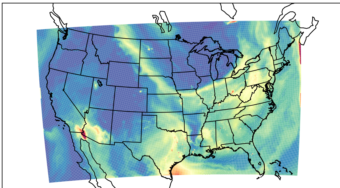
WRF 2023-07-17_18:00:00
