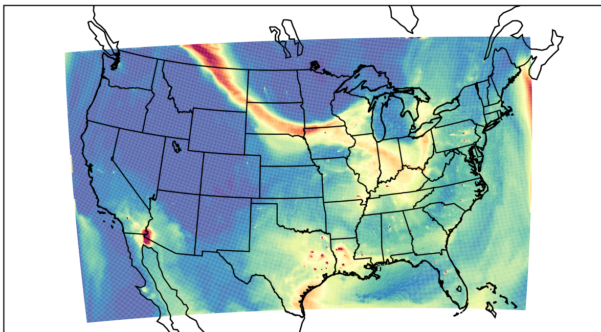
WRF 2023-07-16_23:00:00
