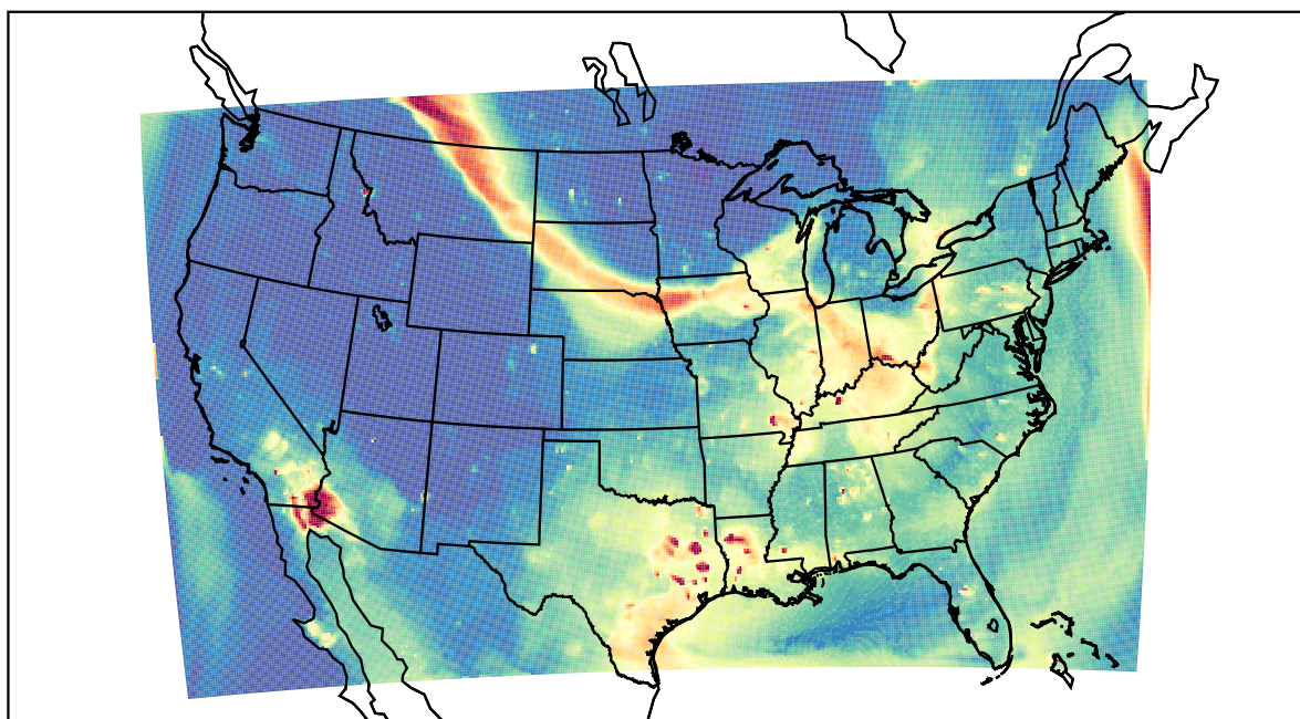
WRF 2023-07-17_02:00:00
