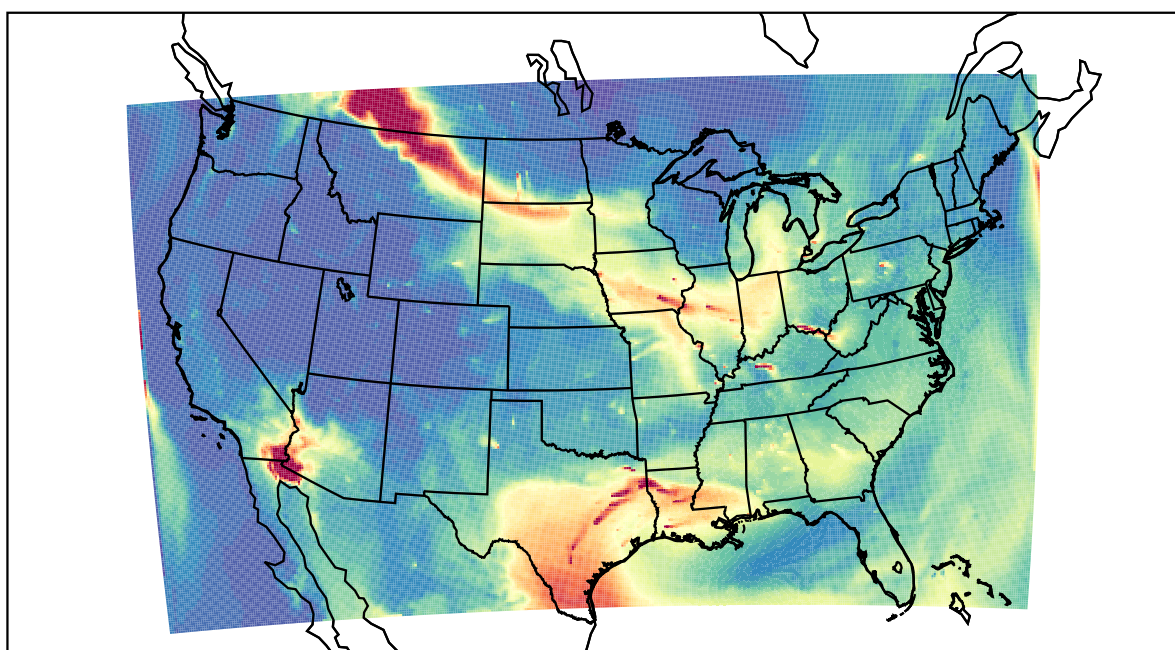
WRF 2023-07-16_14:00:00
