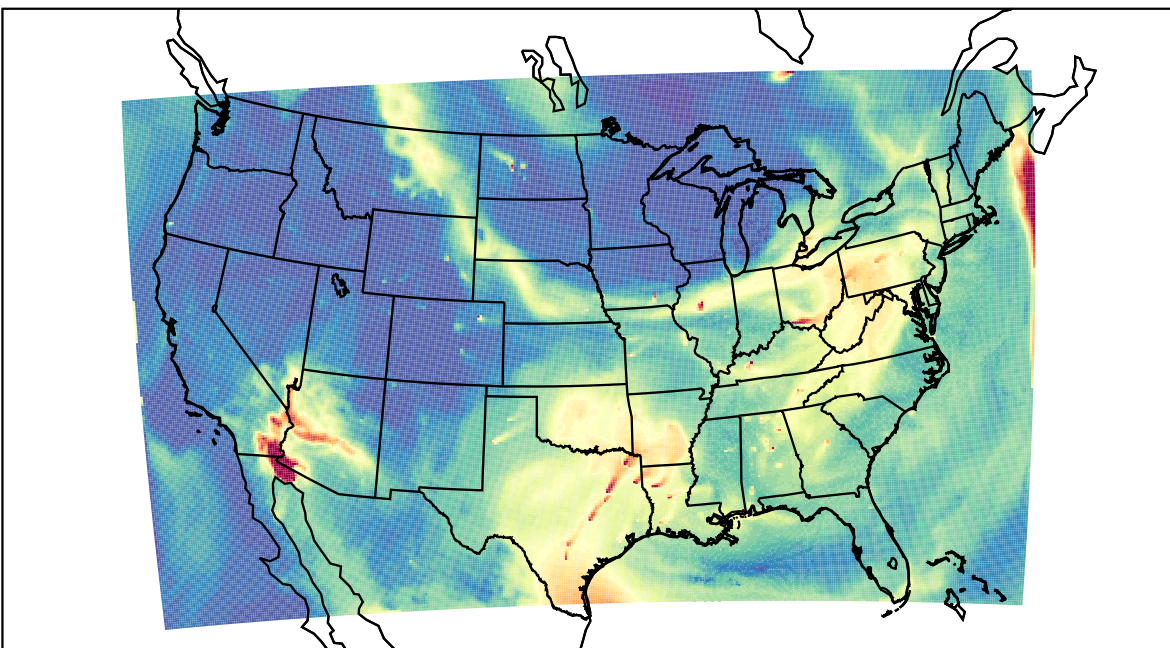
WRF 2023-07-17_15:00:00
