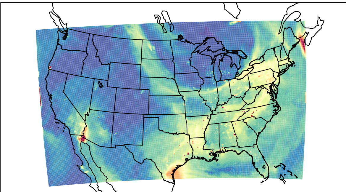
WRF 2023-07-18_00:00:00
