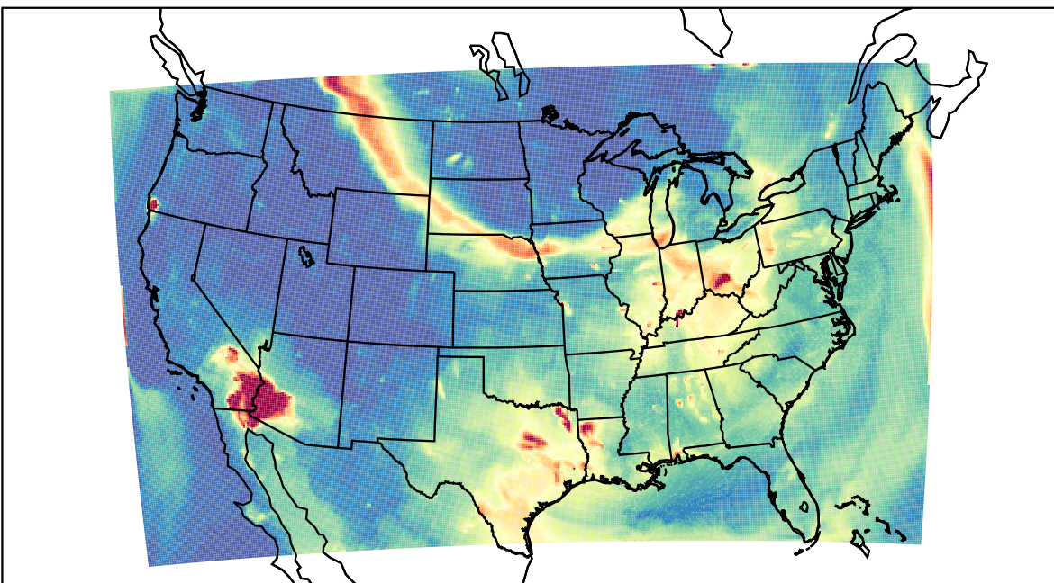
WRF 2023-07-17_05:00:00
