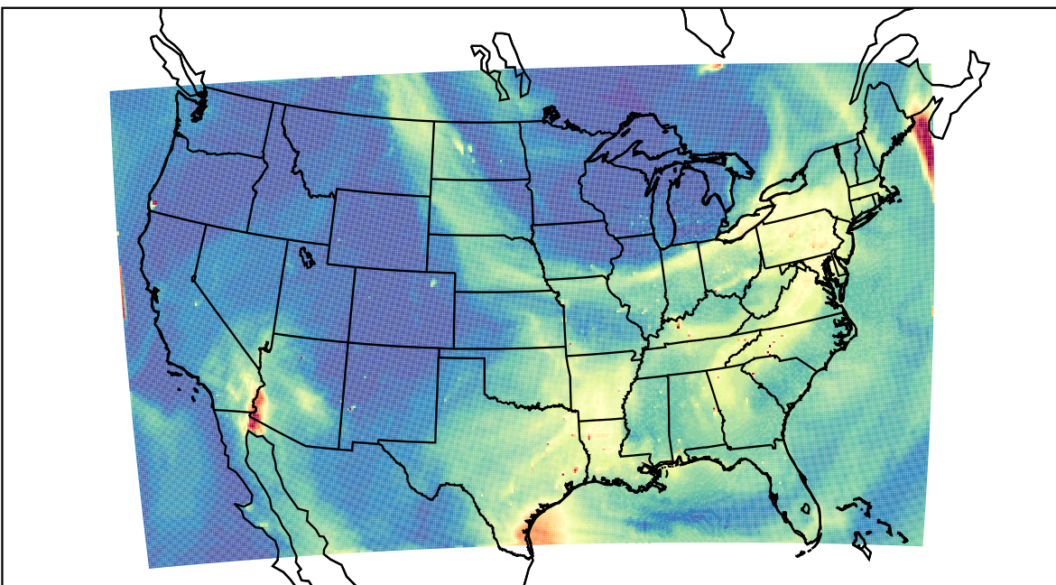
WRF 2023-07-17_22:00:00
