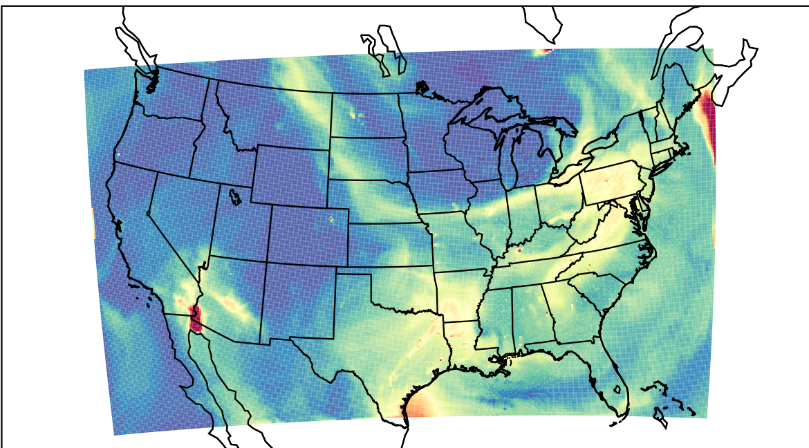
WRF 2023-07-17_19:00:00
