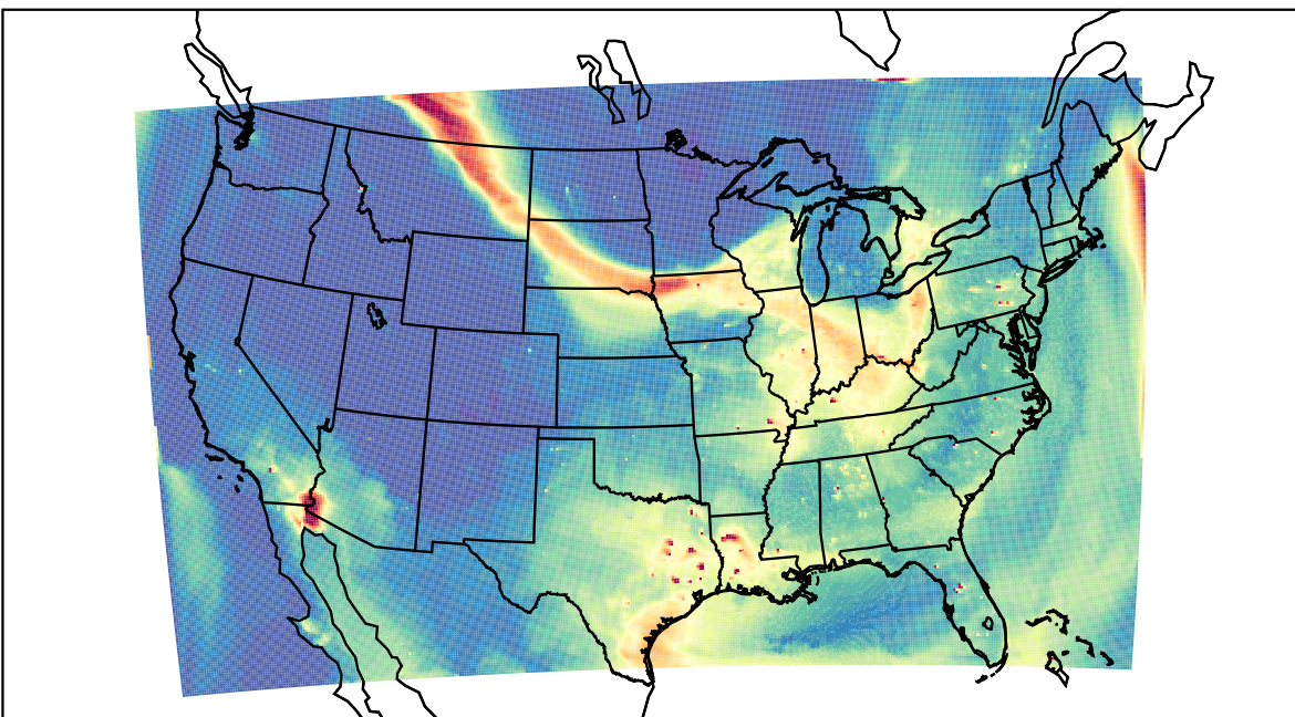
WRF 2023-07-17_00:00:00
