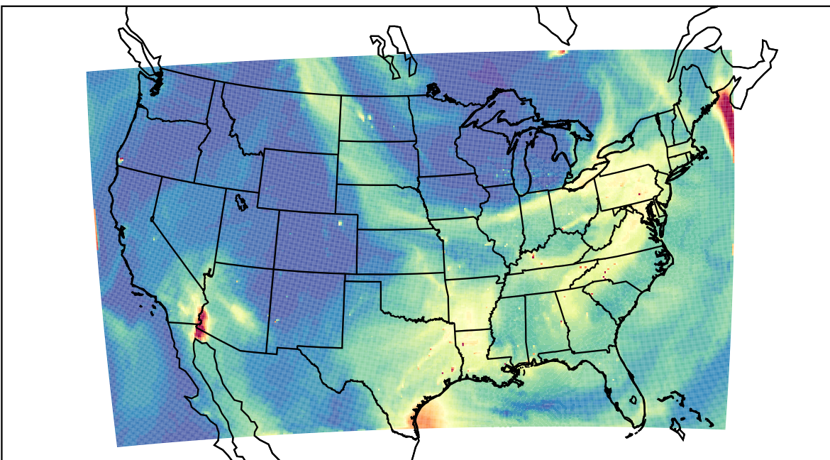
WRF 2023-07-17_21:00:00
