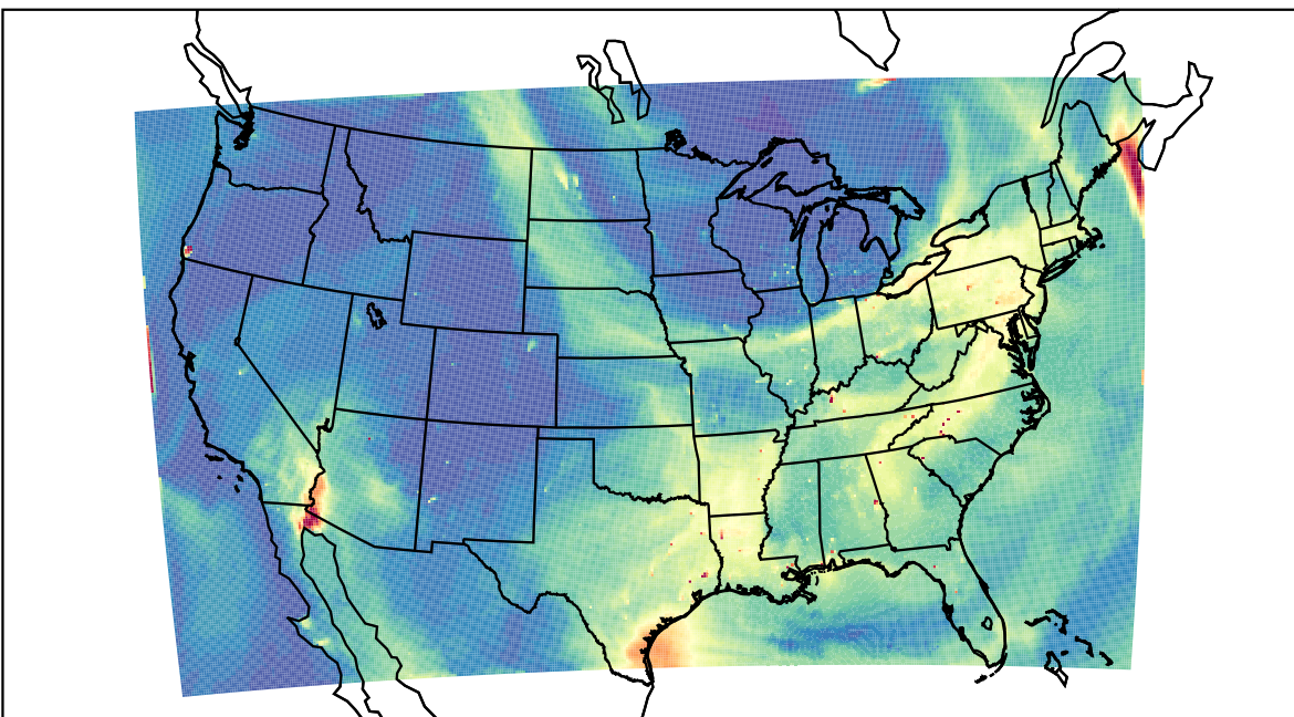
WRF 2023-07-17_23:00:00
