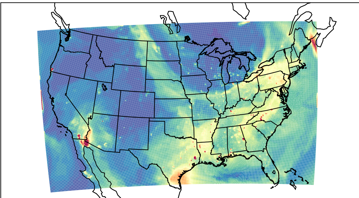
WRF 2023-07-18_01:00:00
