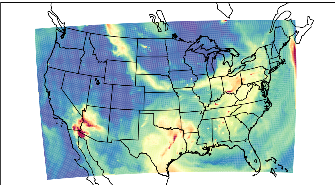
WRF 2023-07-17_13:00:00
