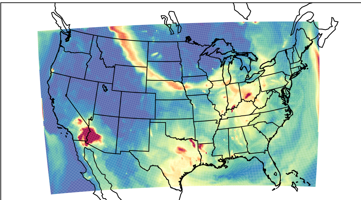
WRF 2023-07-17_06:00:00
