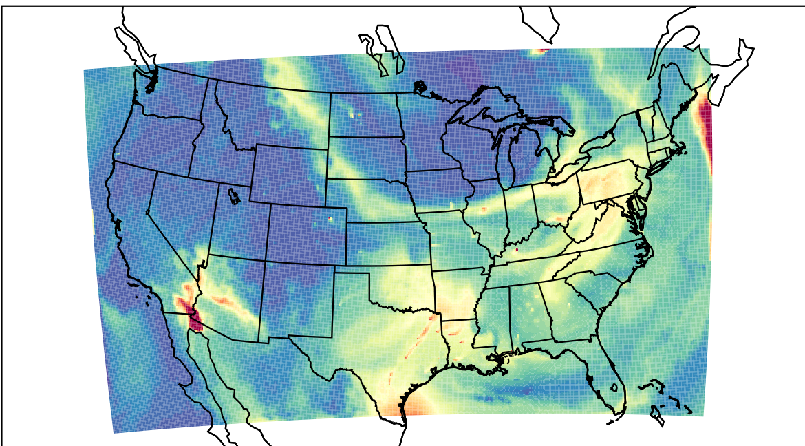
WRF 2023-07-17_17:00:00
