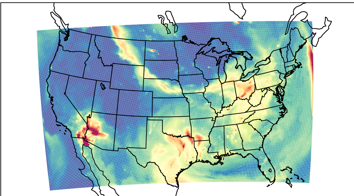
WRF 2023-07-17_11:00:00
