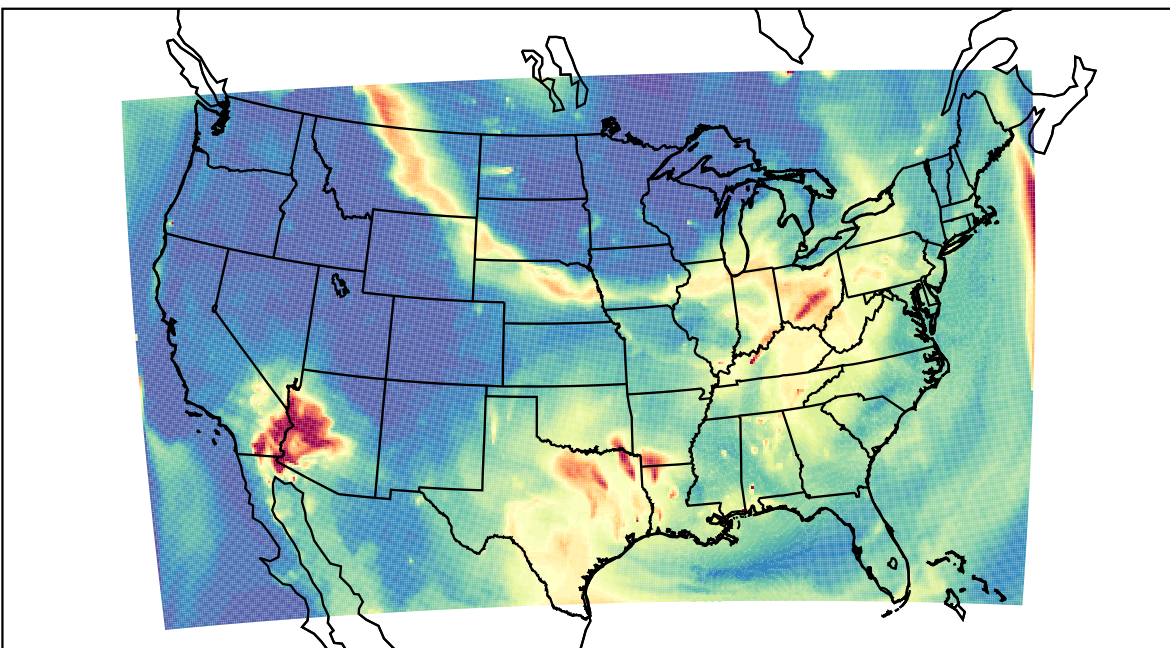
WRF 2023-07-17_09:00:00
