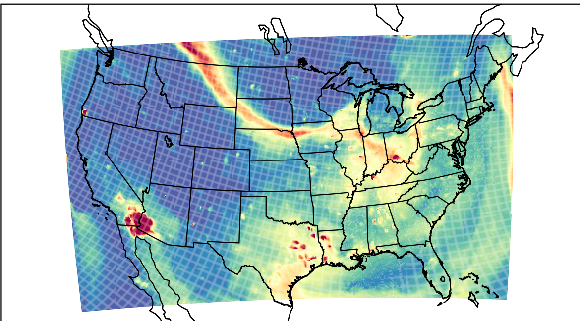
WRF 2023-07-17_03:00:00
