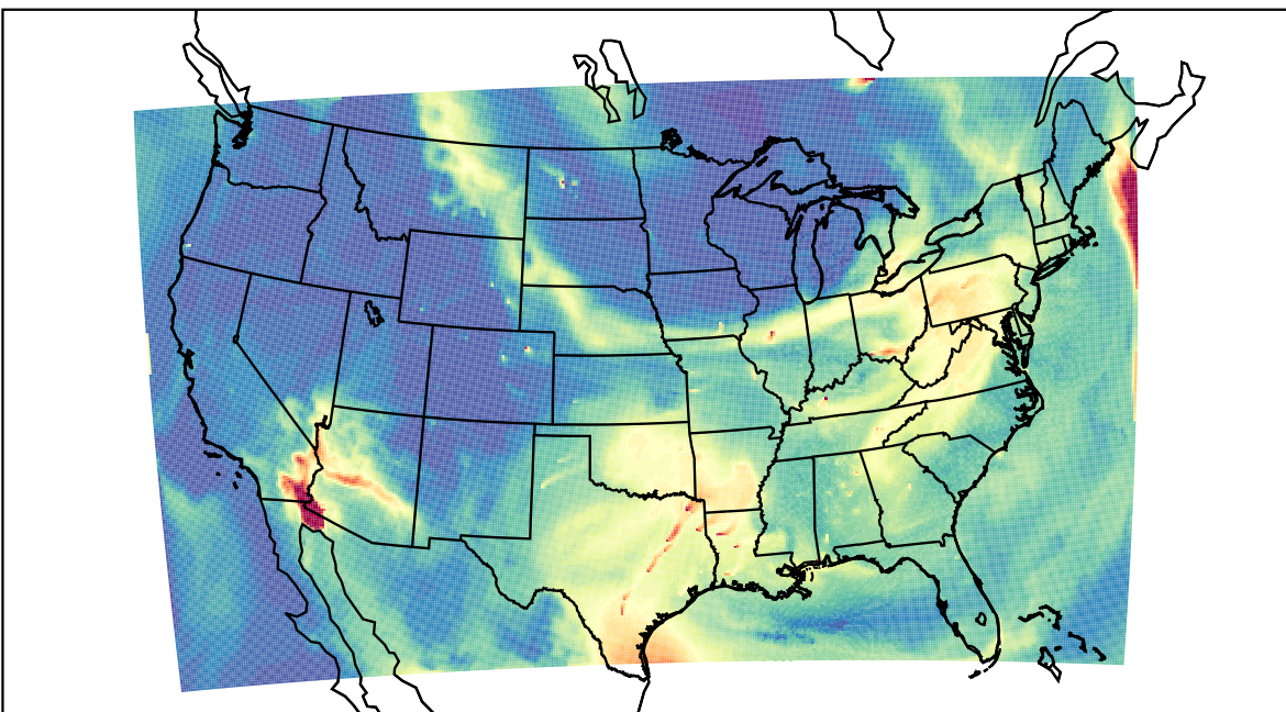
WRF 2023-07-17_16:00:00
