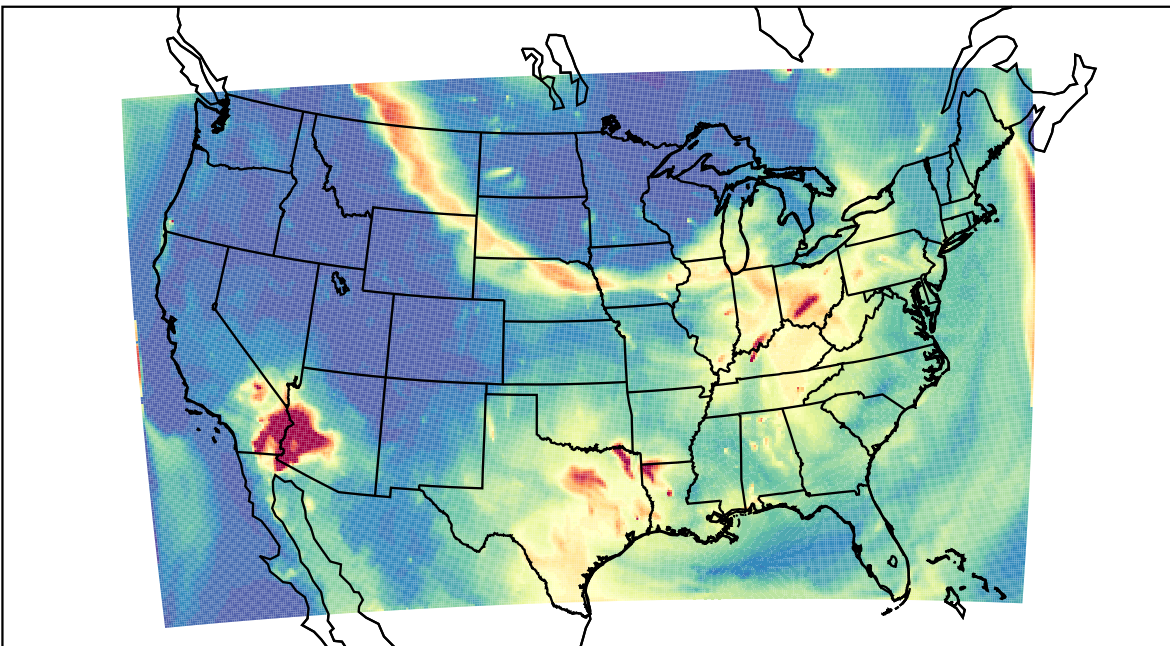
WRF 2023-07-17_07:00:00
