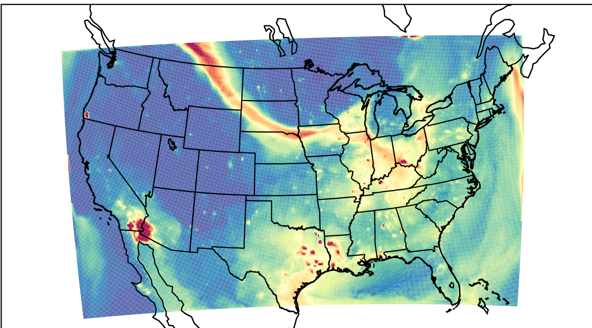
WRF 2023-07-17_02:00:00
