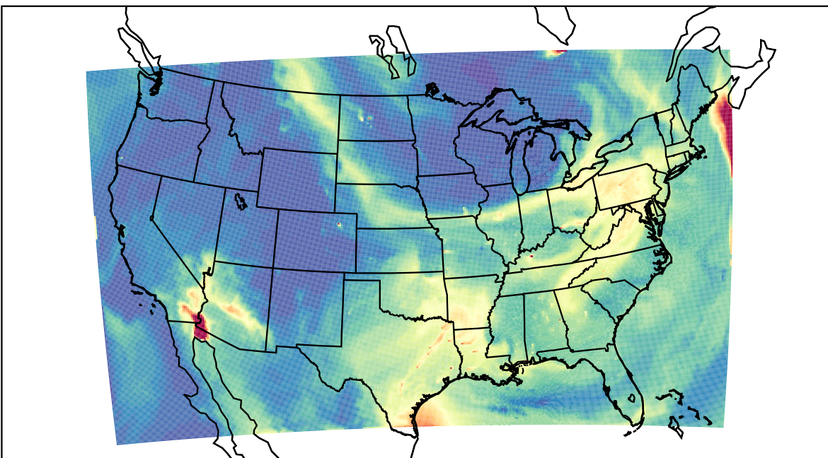
WRF 2023-07-17_18:00:00
