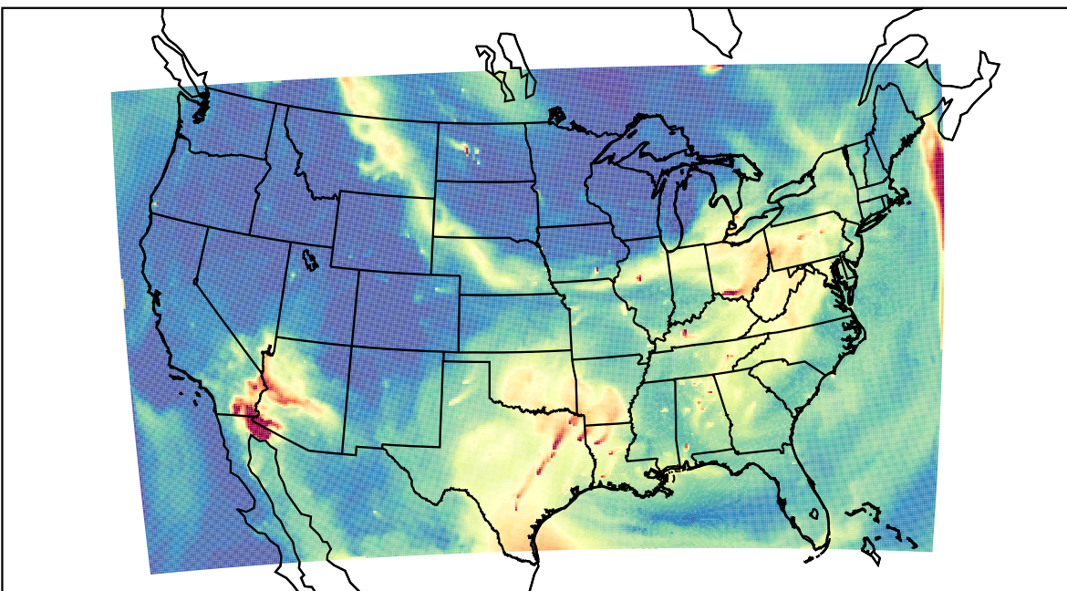
WRF 2023-07-17_14:00:00
