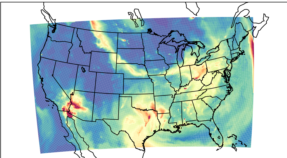
WRF 2023-07-17_12:00:00
