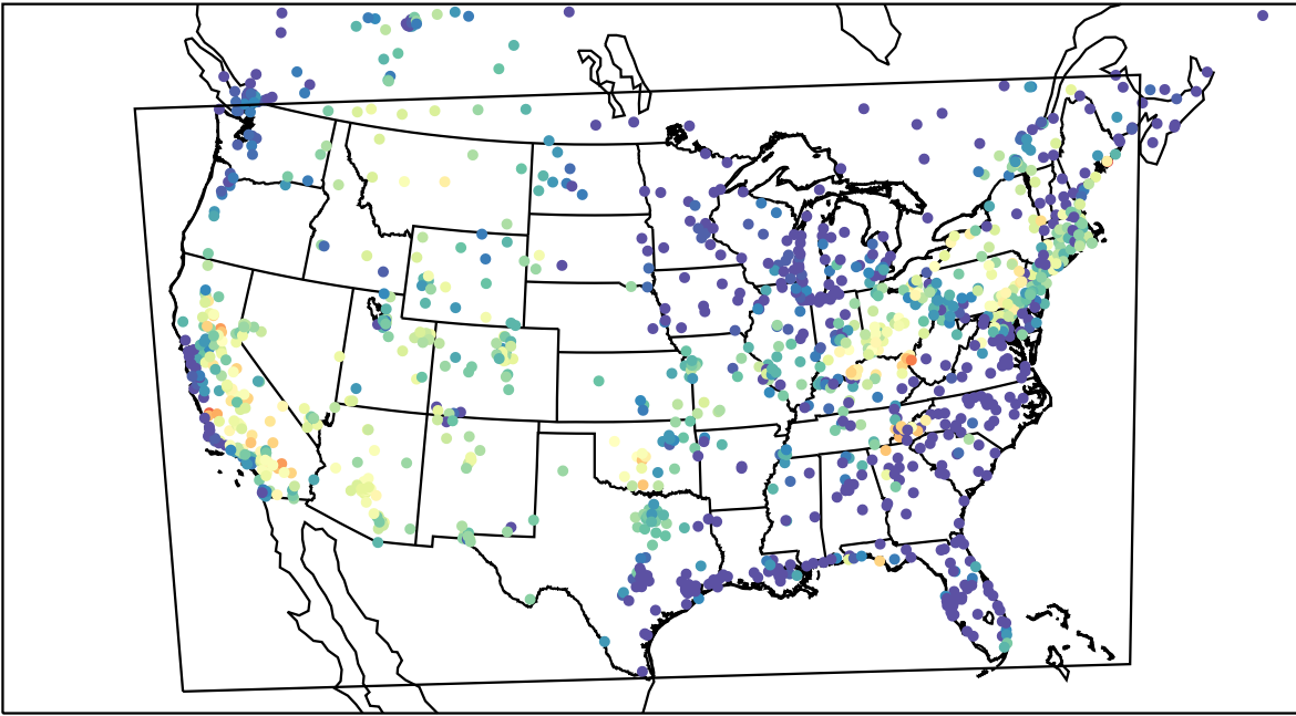
AirNOW (2023-07-18_04:00:00)
