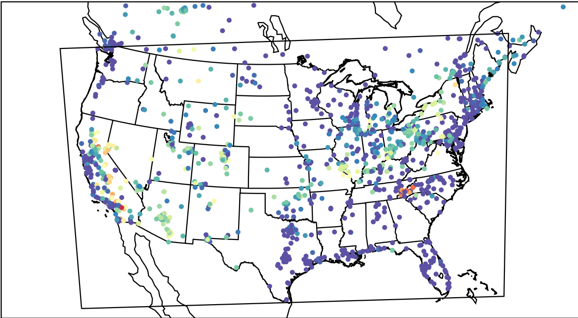
AirNOW (2023-07-17_09:00:00)
