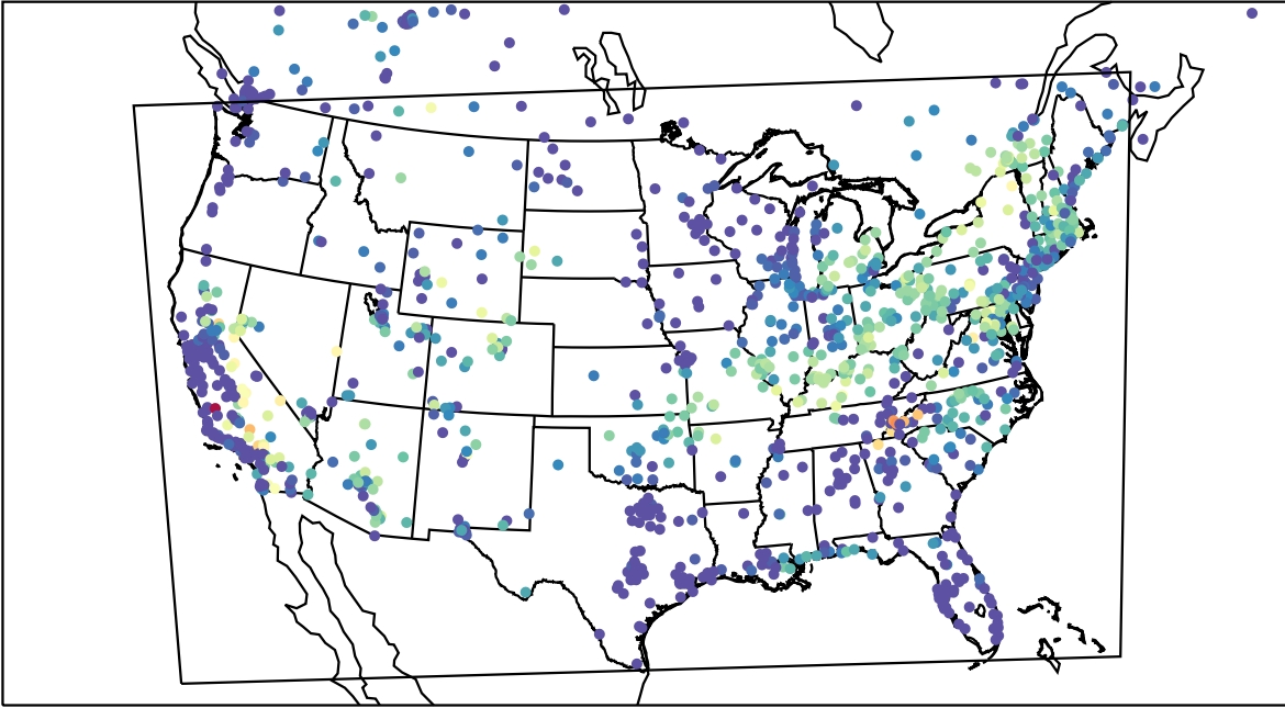
AirNOW (2023-07-17_13:00:00)
