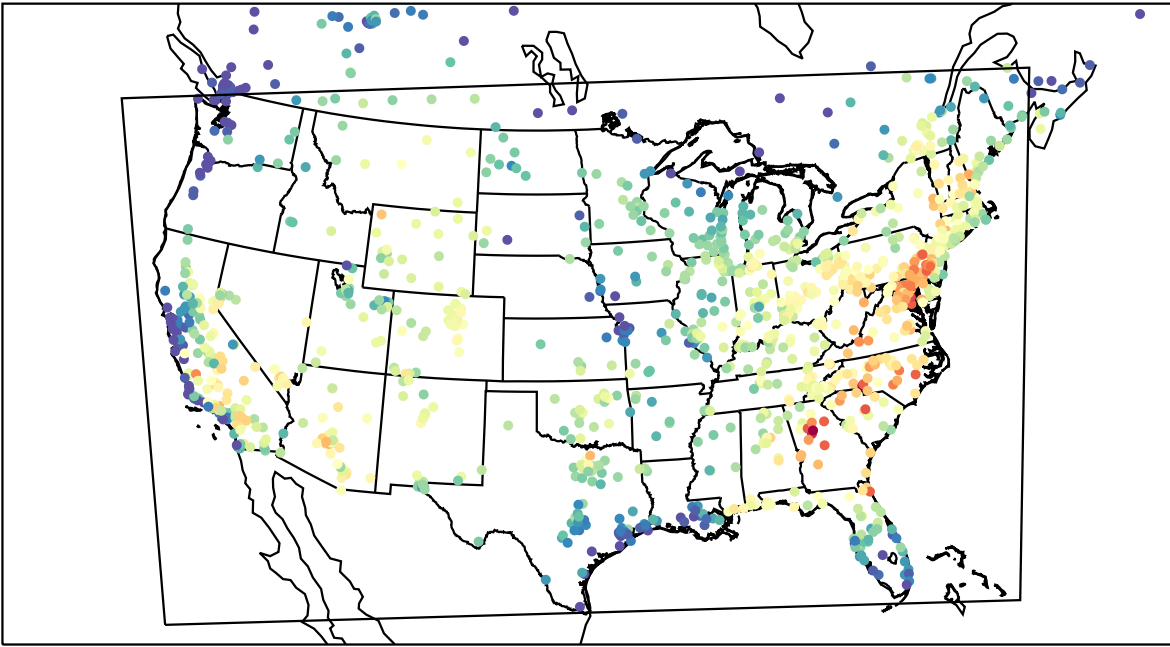
AirNOW (2023-07-18_16:00:00)
