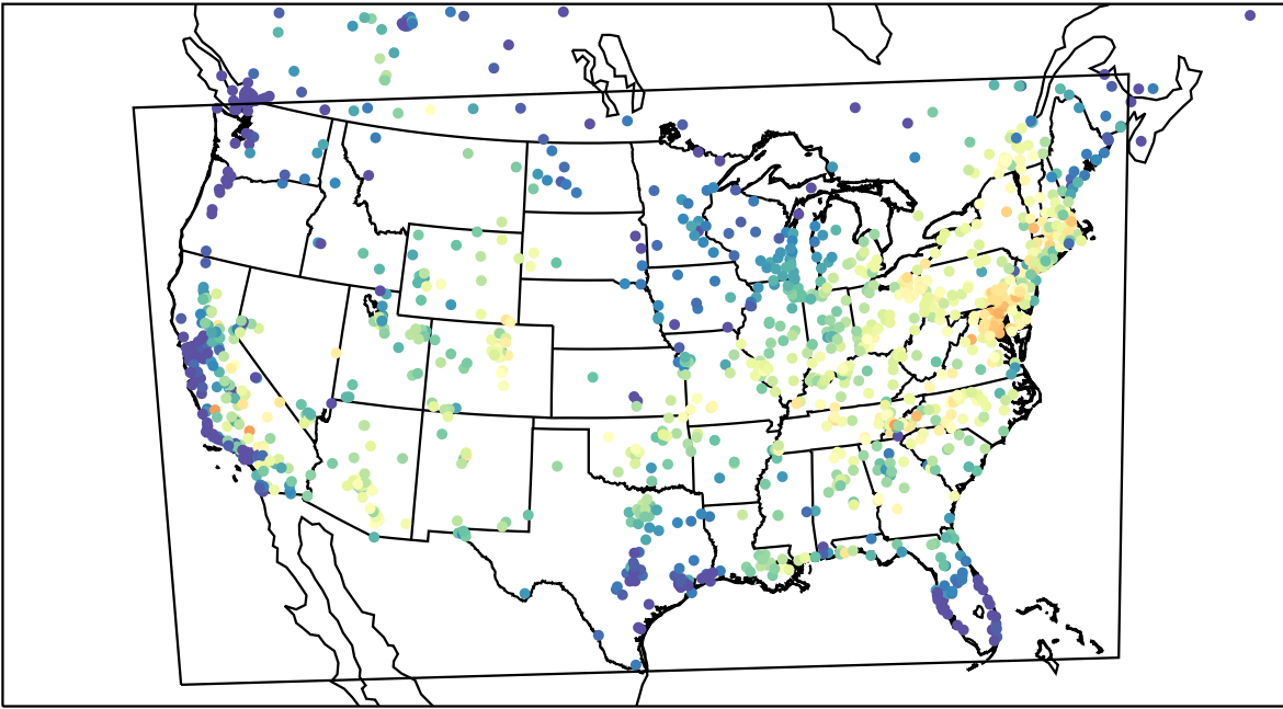
AirNOW (2023-07-17_15:00:00)
