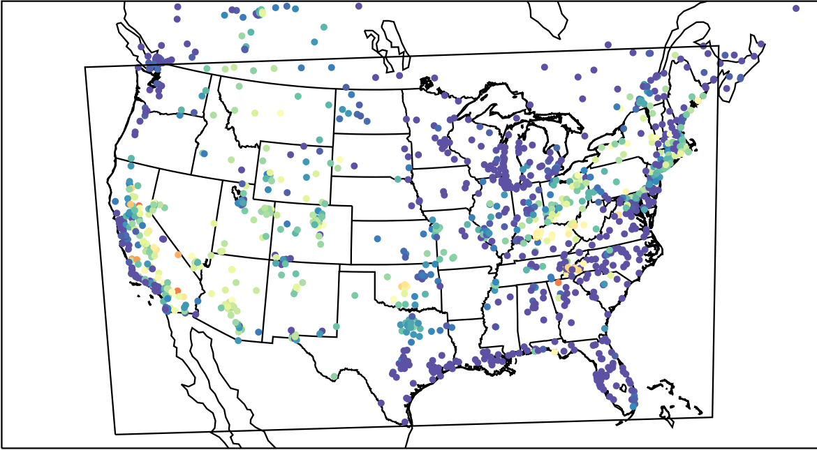
AirNOW (2023-07-18_06:00:00)
