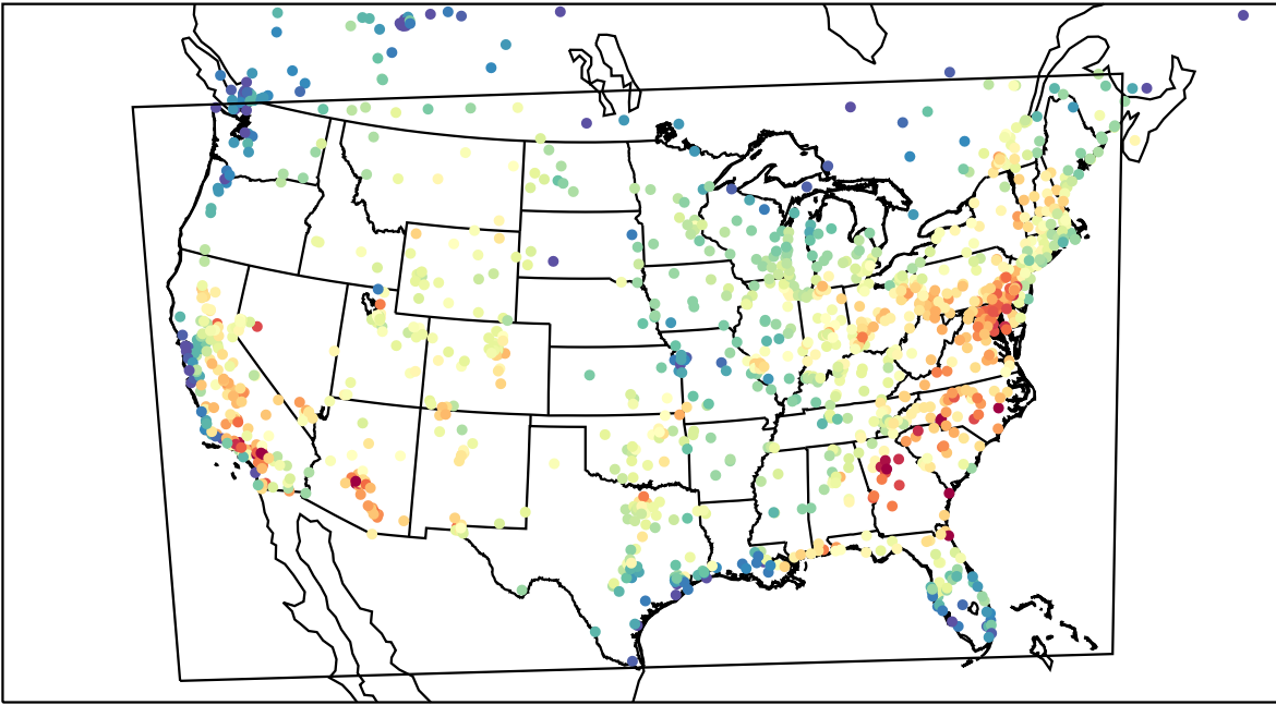
AirNOW (2023-07-18_18:00:00)
