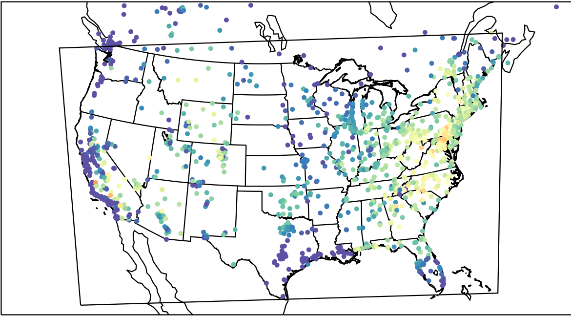
AirNOW (2023-07-18_14:00:00)
