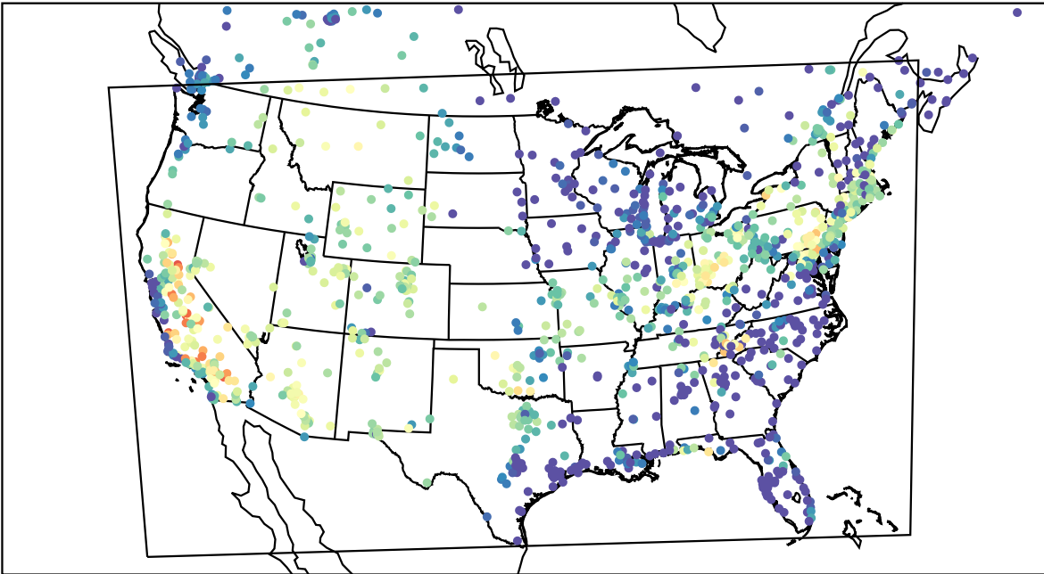
AirNOW (2023-07-18_03:00:00)
