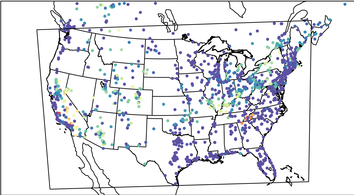
AirNOW (2023-07-17_11:00:00)
