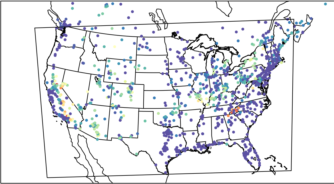
AirNOW (2023-07-17_10:00:00)
