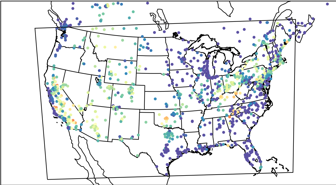
AirNOW (2023-07-18_05:00:00)
