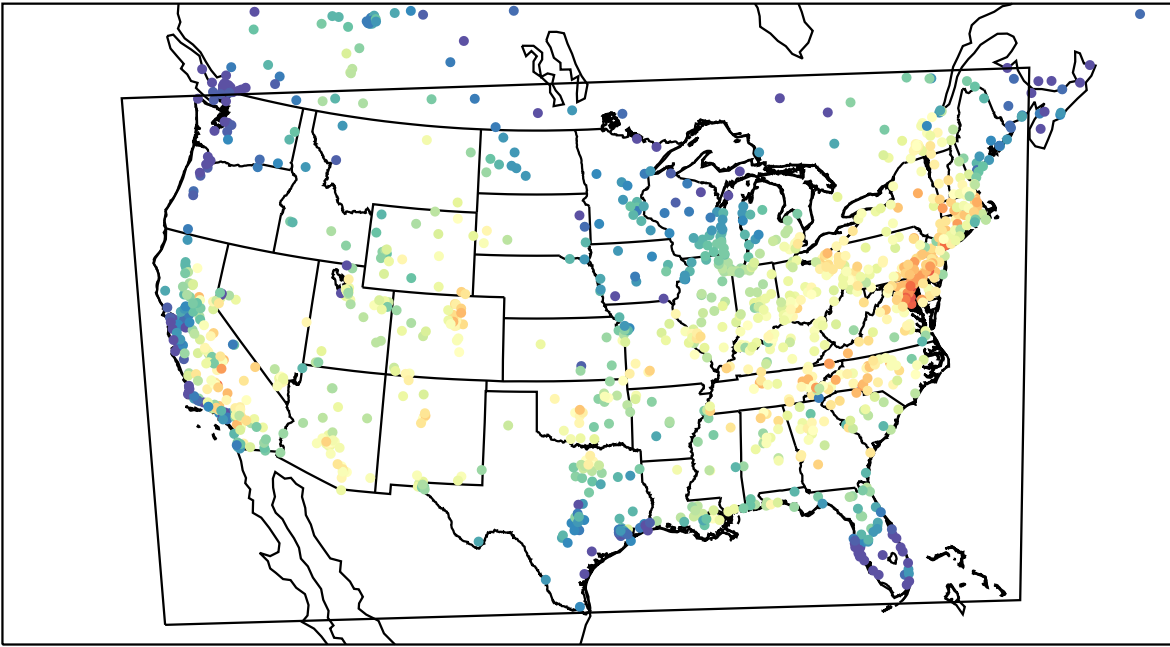
AirNOW (2023-07-17_16:00:00)
