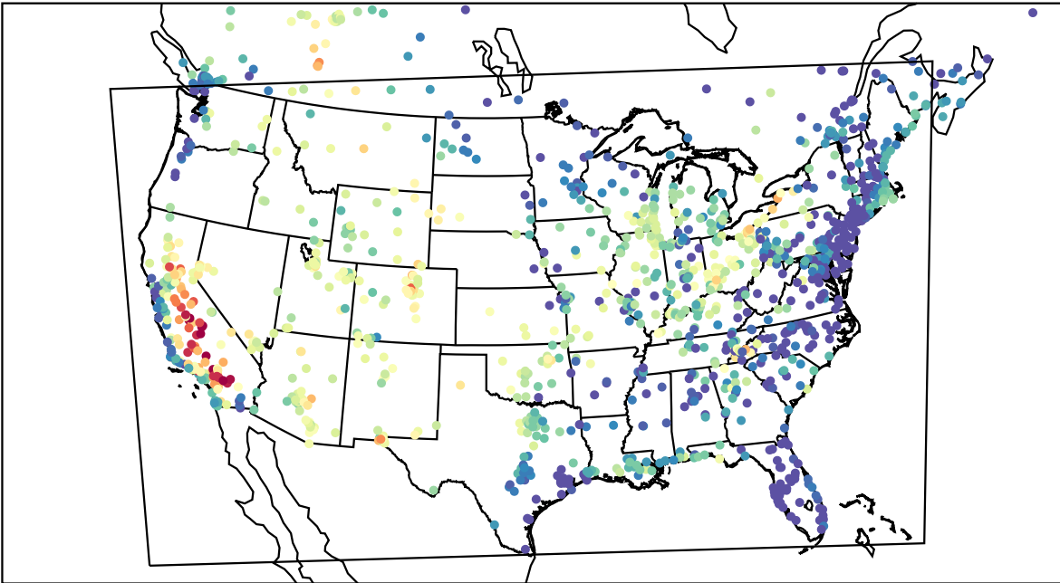
AirNOW (2023-07-17_02:00:00)
