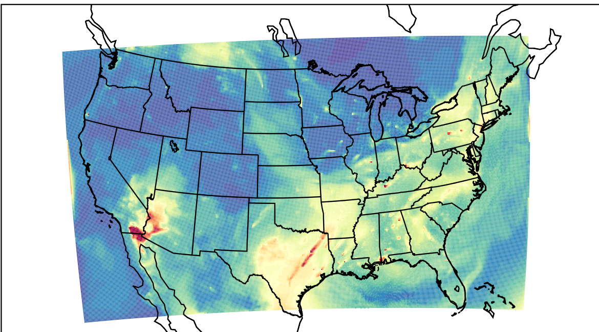
WRF 2023-07-18_13:00:00
