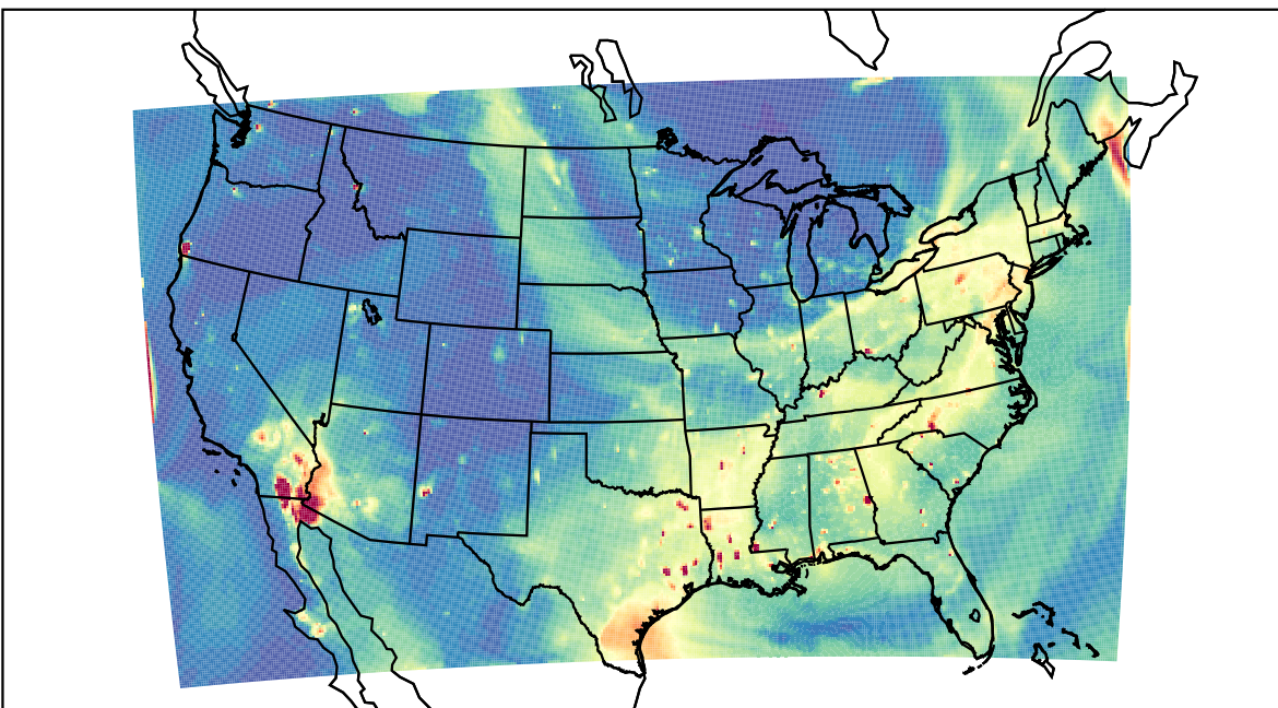
WRF 2023-07-18_02:00:00
