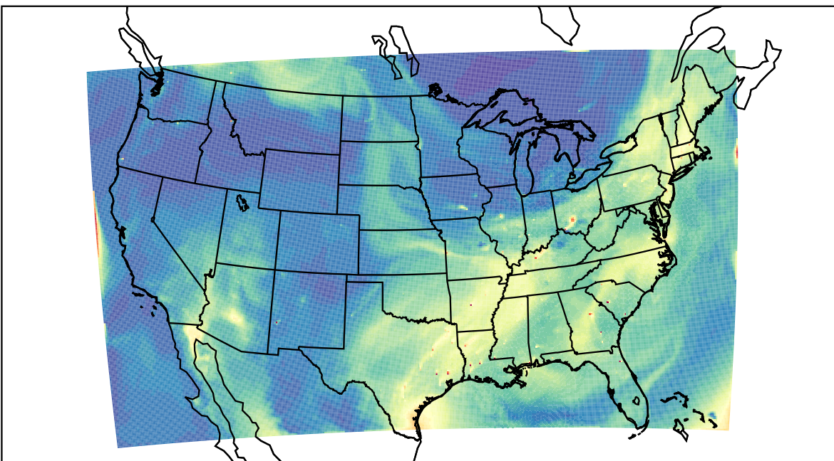
WRF 2023-07-18_19:00:00
