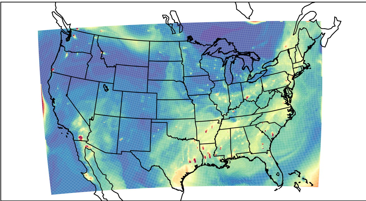
WRF 2023-07-19_01:00:00
