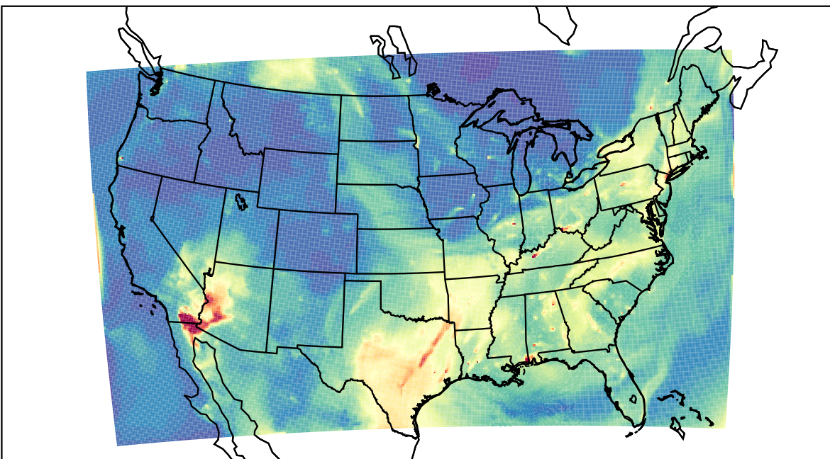
WRF 2023-07-18_12:00:00
