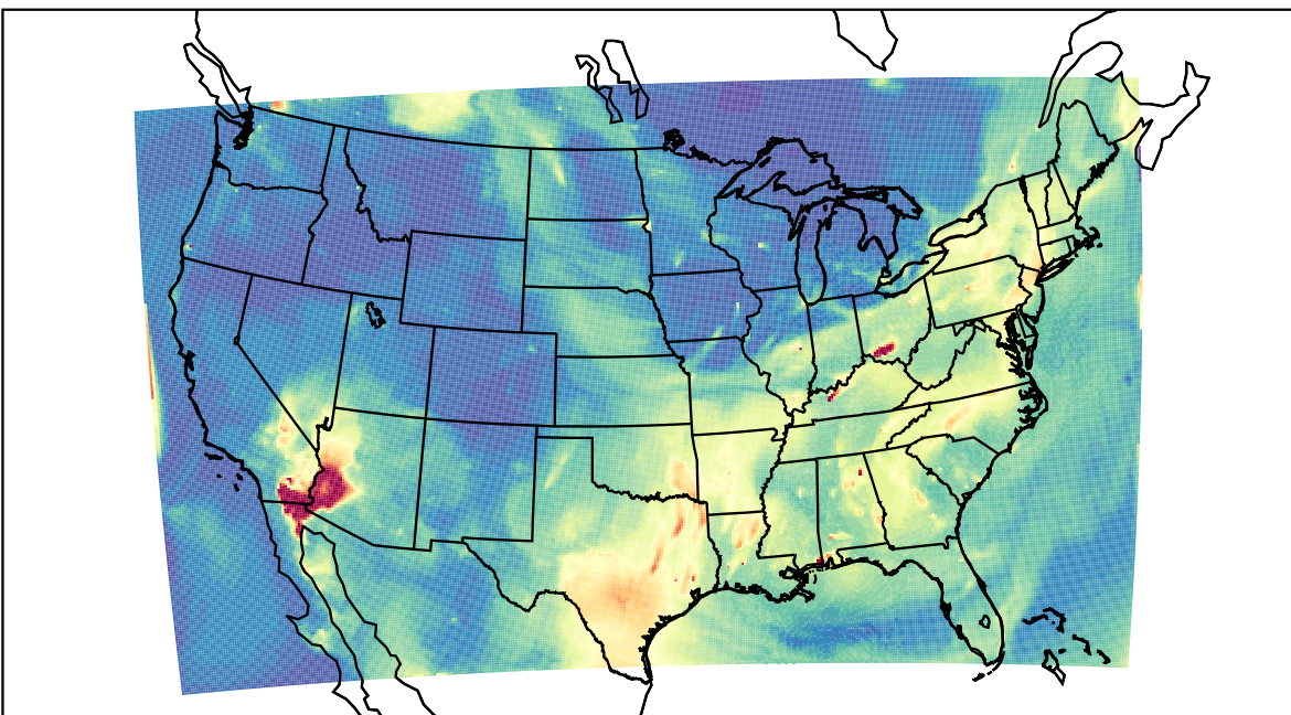
WRF 2023-07-18_09:00:00
