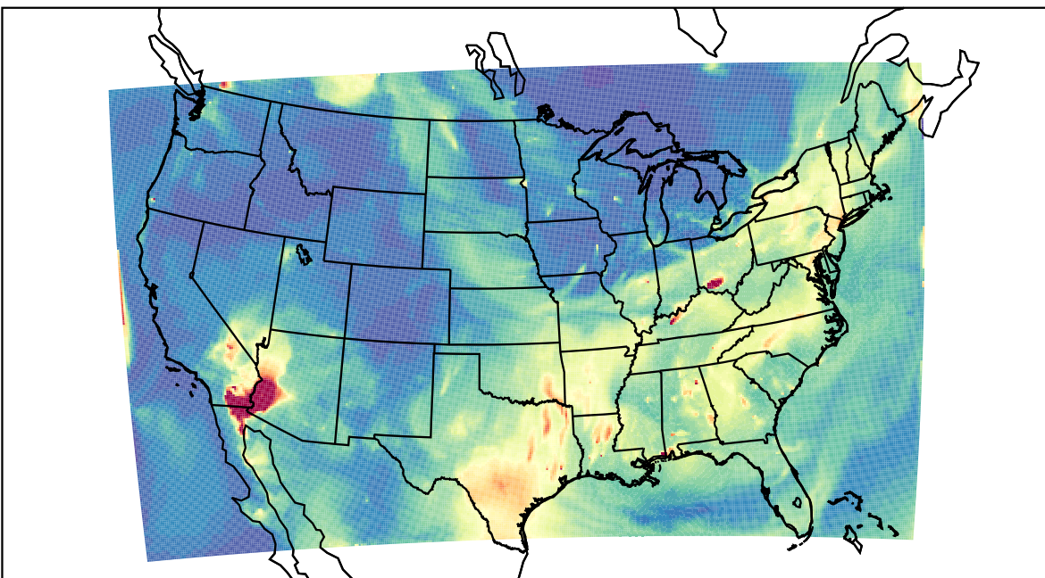
WRF 2023-07-18_08:00:00
