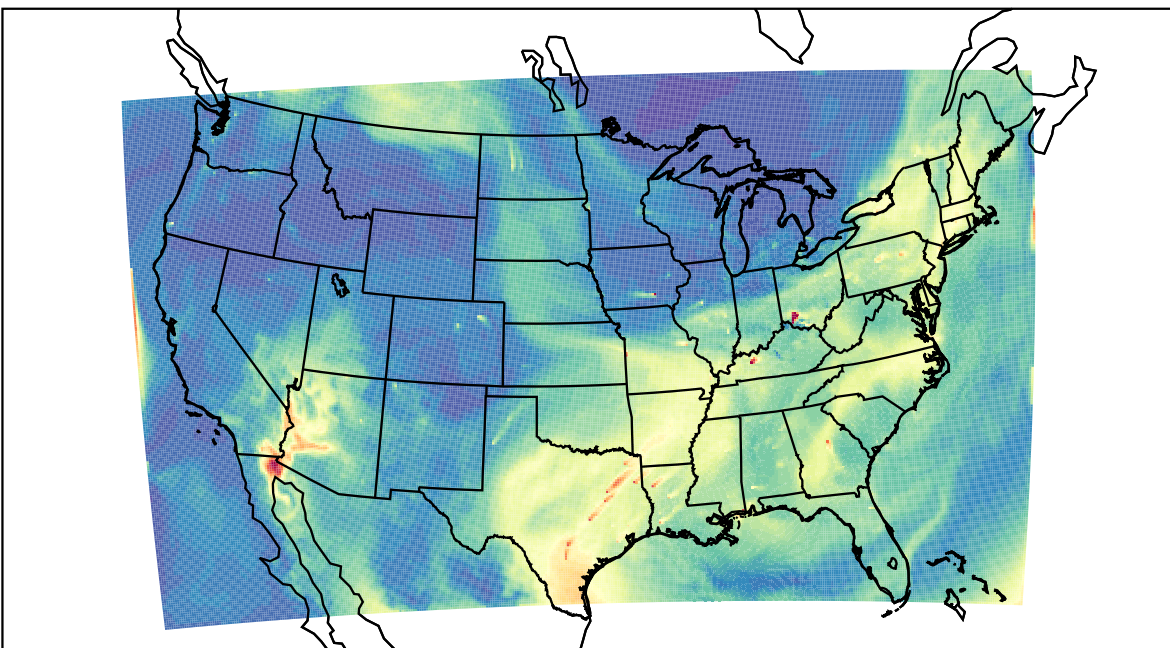
WRF 2023-07-18_16:00:00
