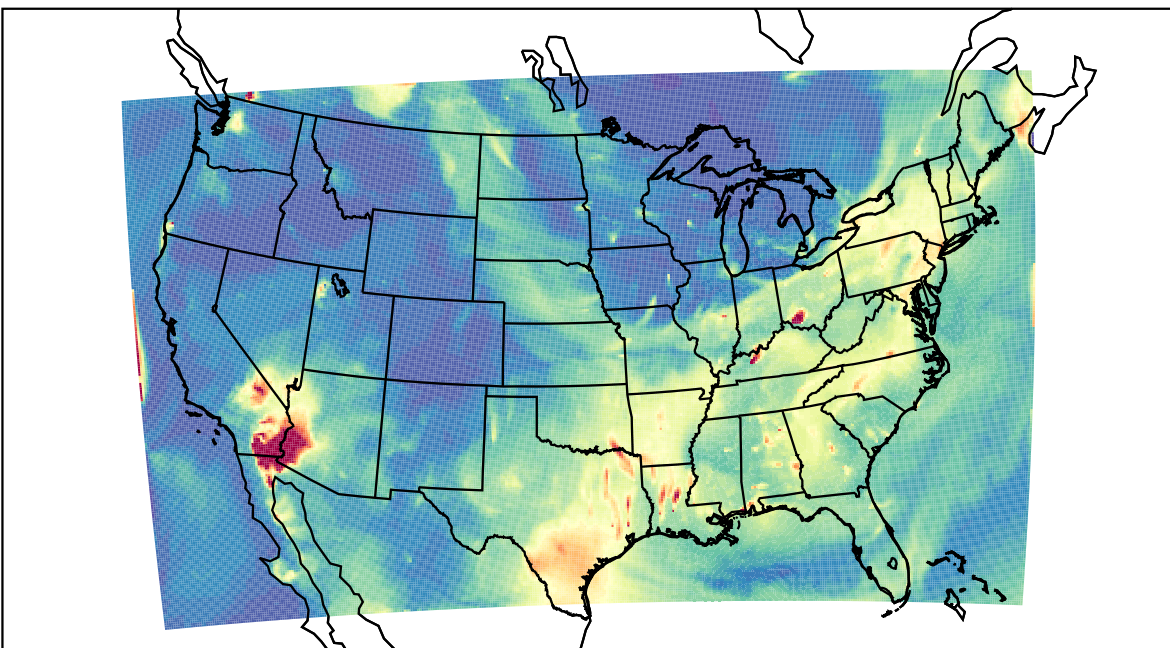
WRF 2023-07-18_06:00:00
