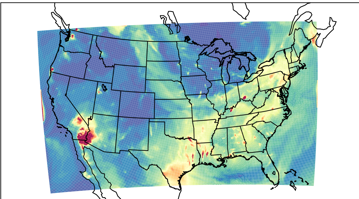
WRF 2023-07-18_05:00:00
