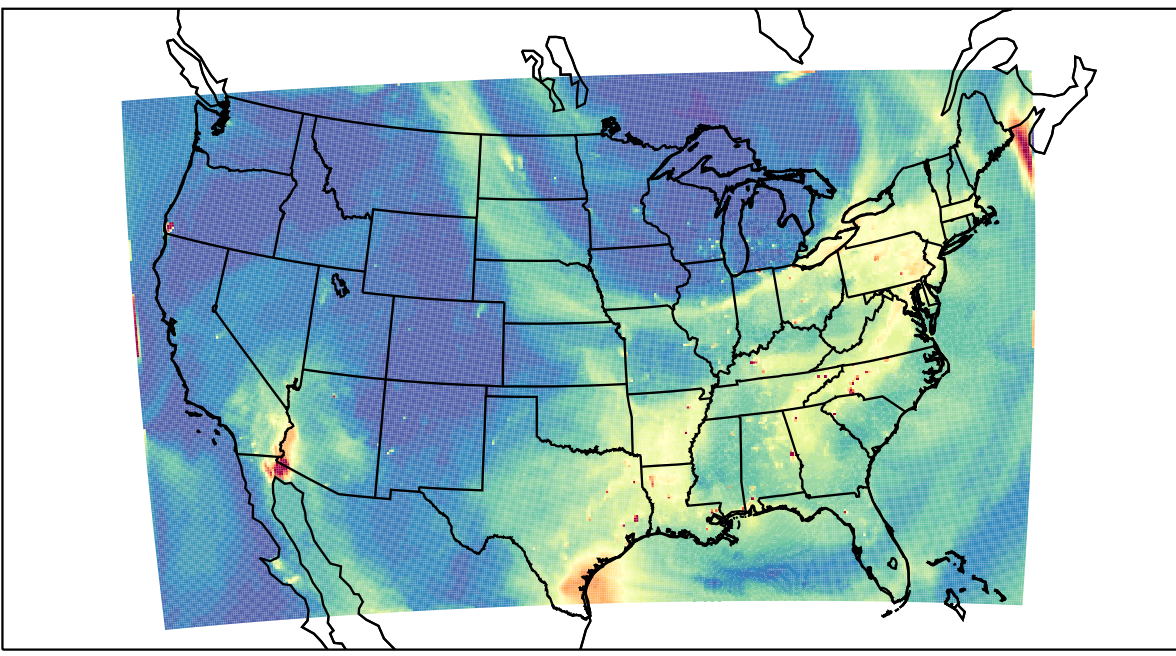
WRF 2023-07-18_00:00:00
