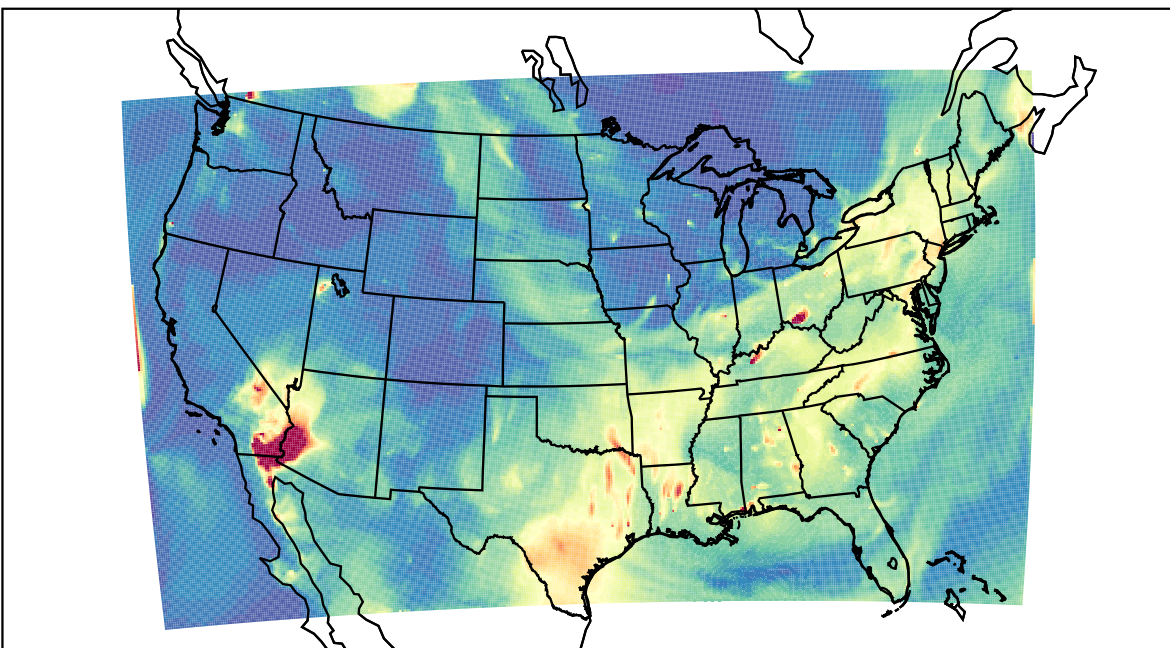
WRF 2023-07-18_07:00:00
