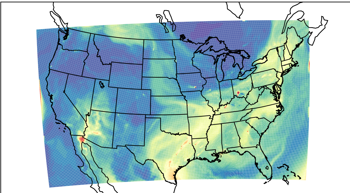
WRF 2023-07-18_17:00:00
