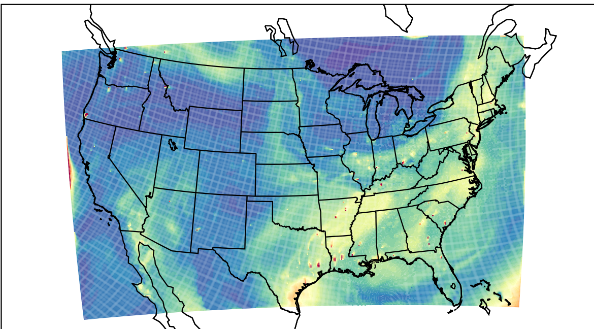
WRF 2023-07-18_23:00:00
