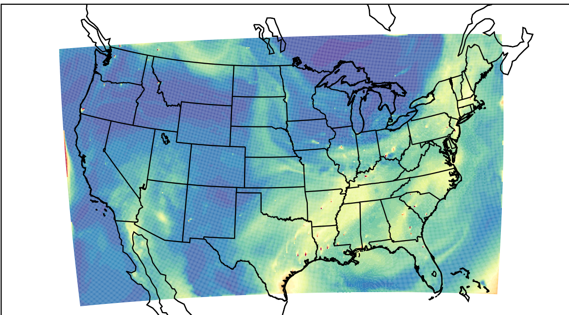
WRF 2023-07-18_21:00:00
