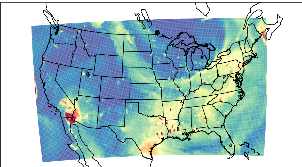
WRF 2023-07-18_03:00:00
