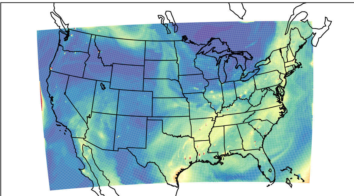
WRF 2023-07-18_22:00:00
