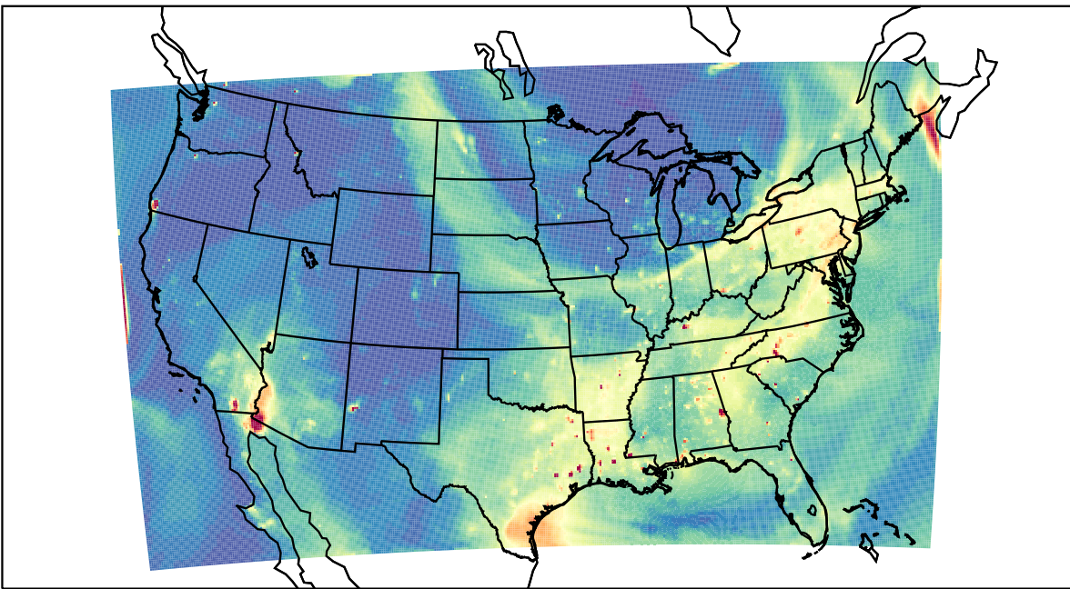
WRF 2023-07-18_01:00:00
