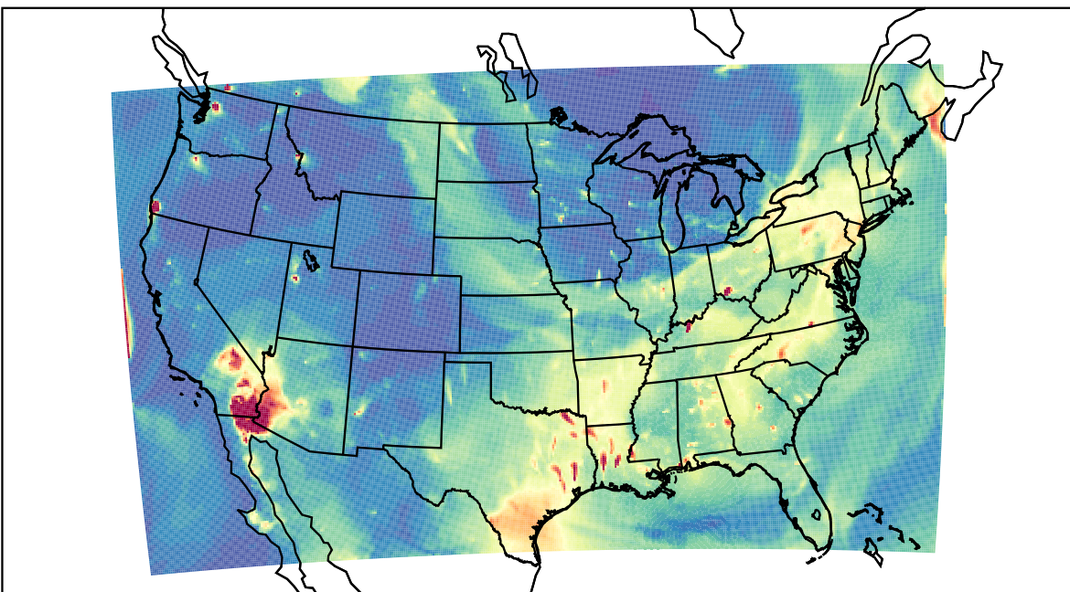
WRF 2023-07-18_04:00:00
