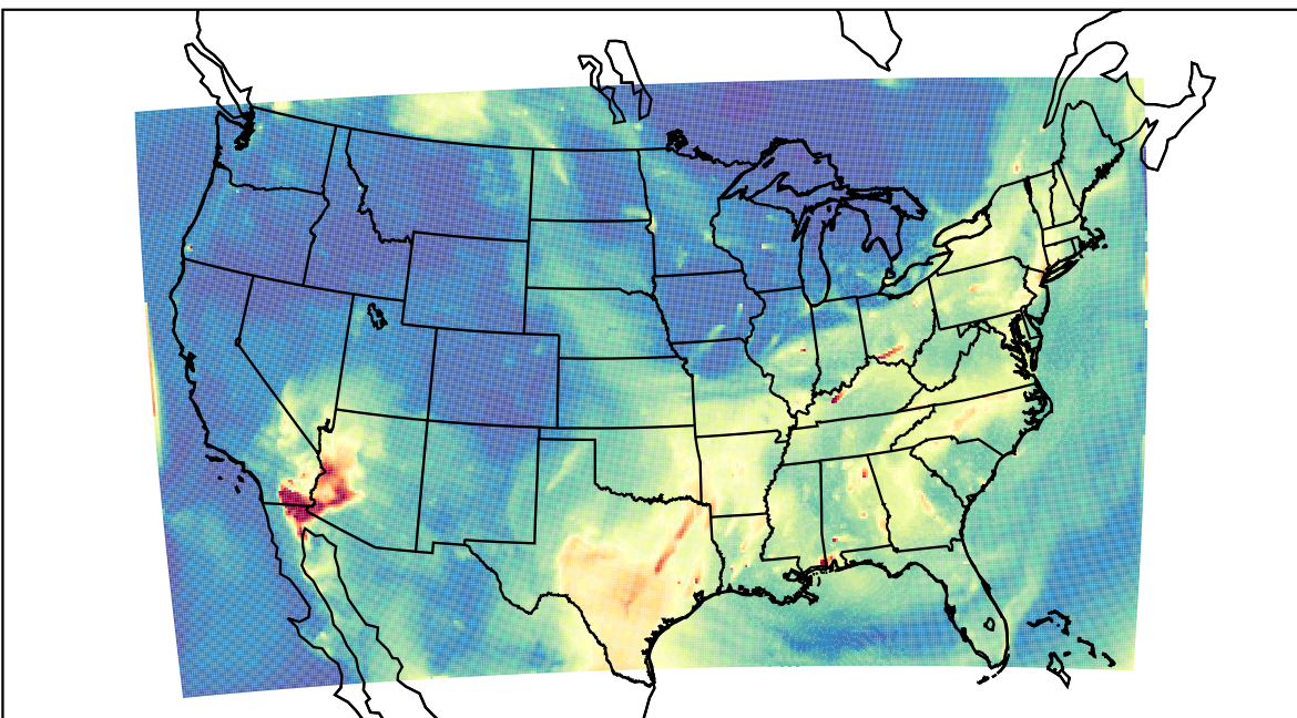
WRF 2023-07-18_11:00:00
