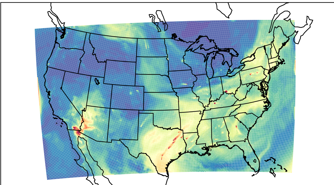
WRF 2023-07-18_15:00:00
