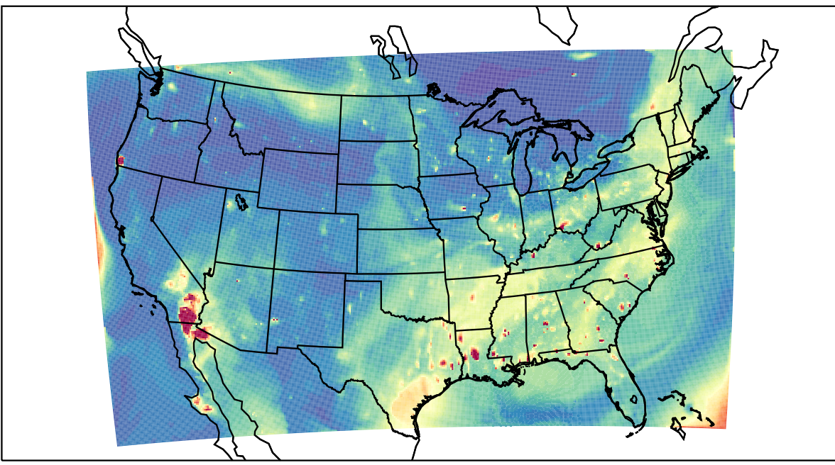
WRF 2023-07-19_02:00:00
