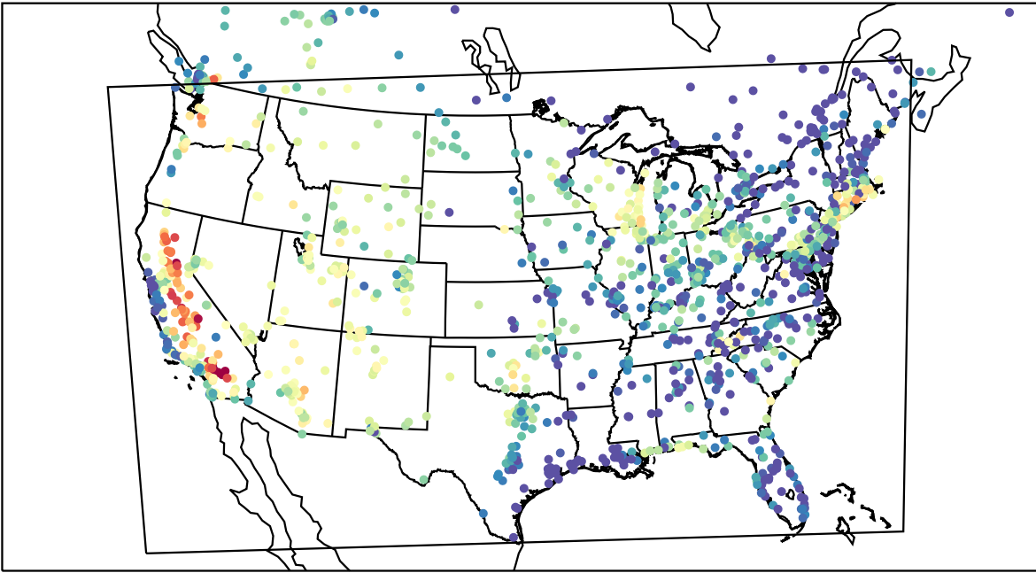
AirNOW (2023-07-20_02:00:00)
