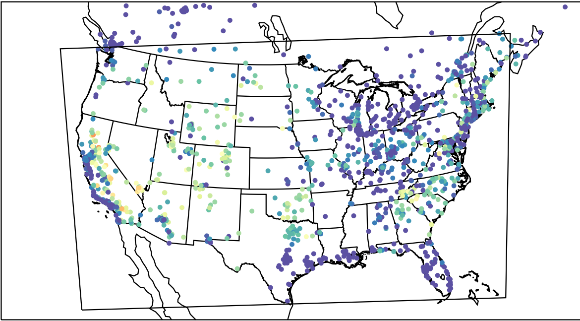
AirNOW (2023-07-19_06:00:00)
