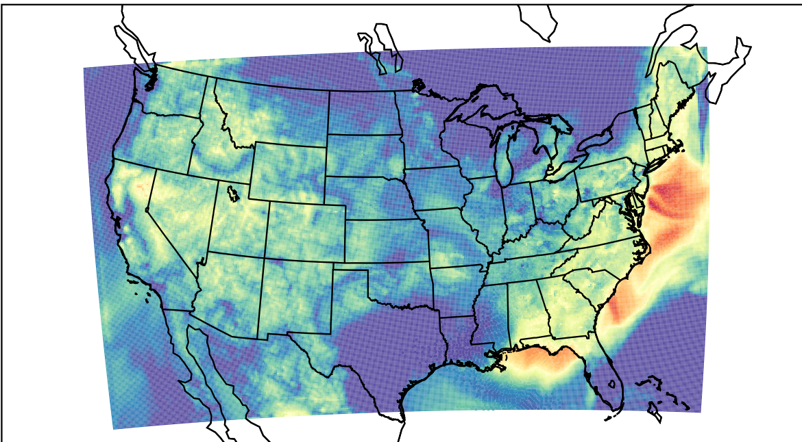
WRF (2023-07-19_13:00:00)
