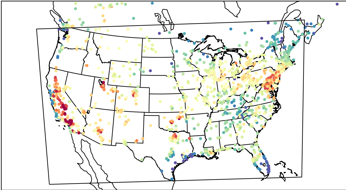
AirNOW (2023-07-20_21:00:00)
