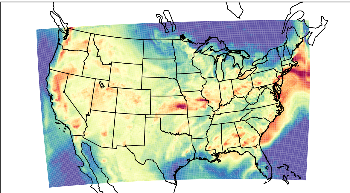
WRF (2023-07-20_01:00:00)
