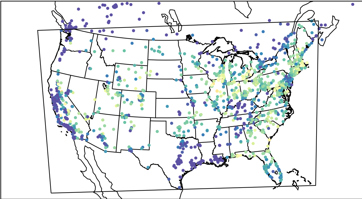
AirNOW (2023-07-19_14:00:00)
