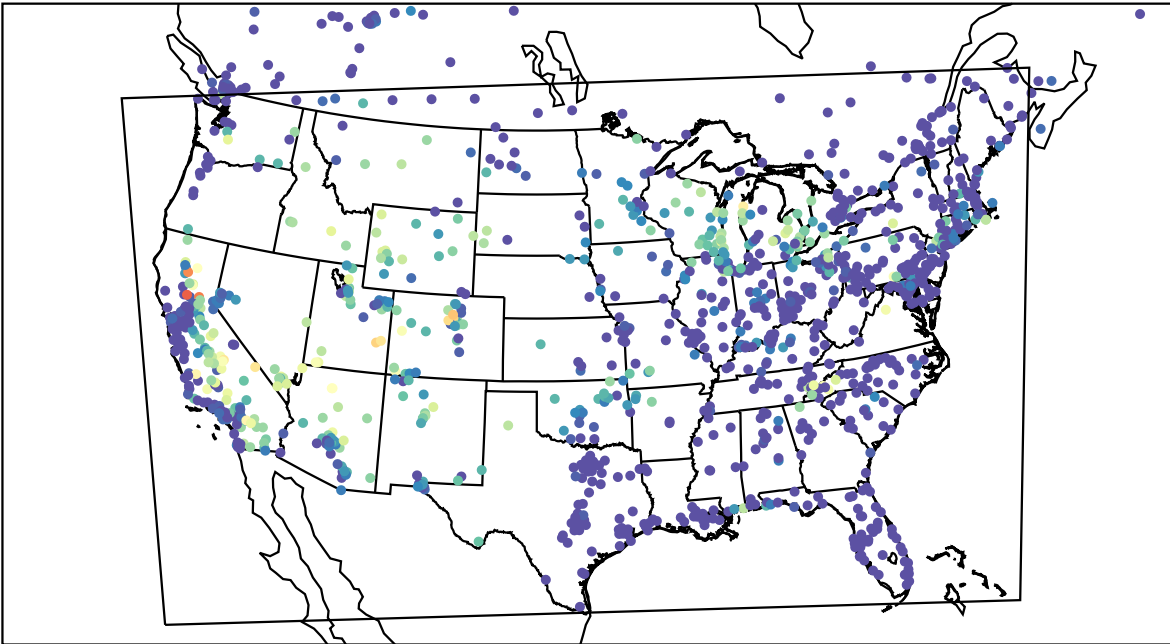
AirNOW (2023-07-20_09:00:00)
