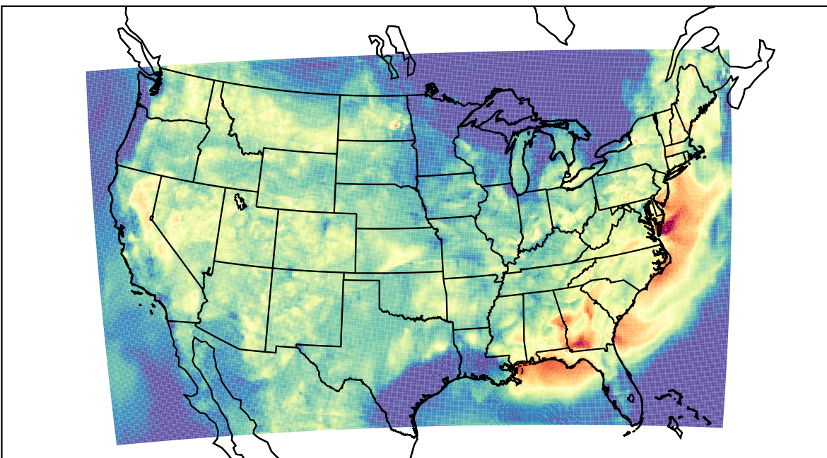
WRF (2023-07-19_04:00:00)
