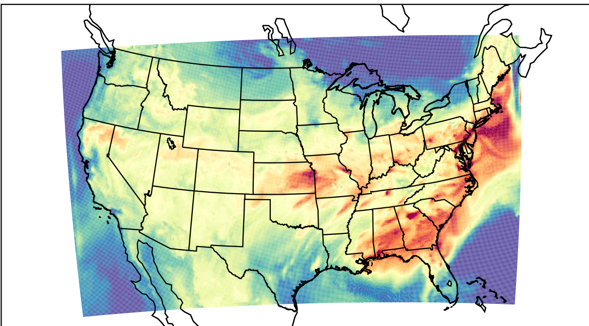
WRF (2023-07-19_17:00:00)
