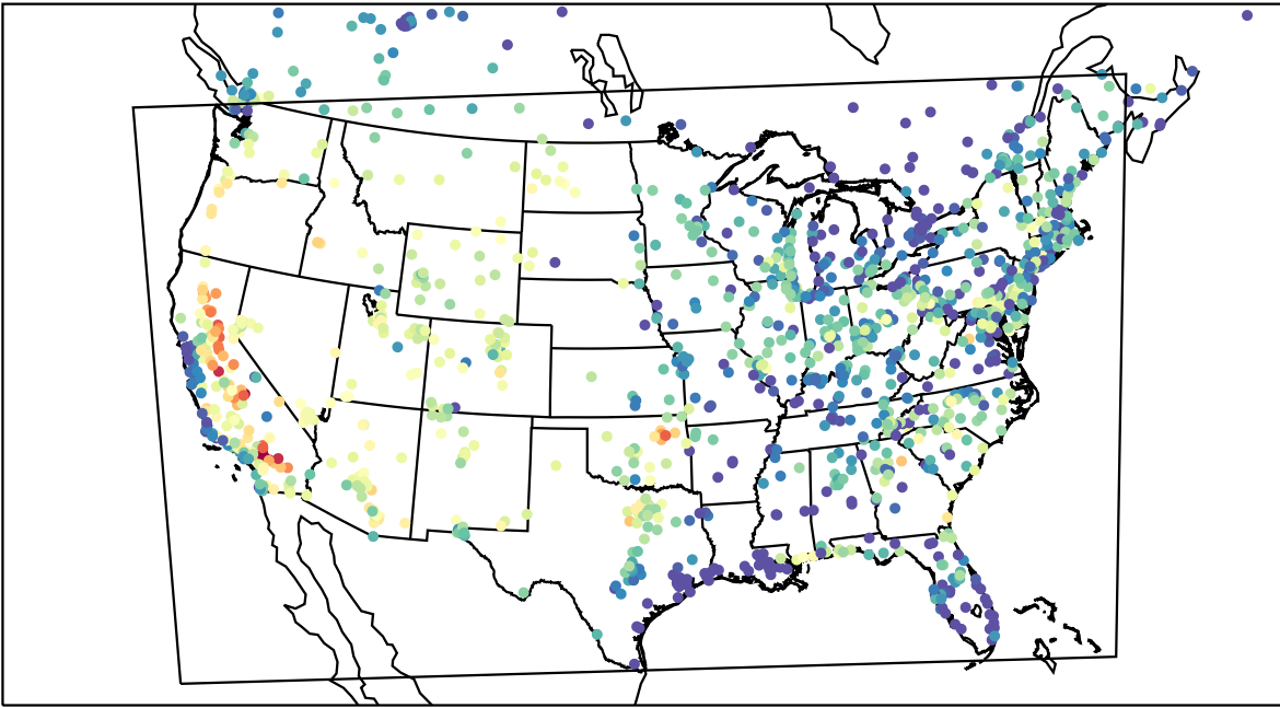
AirNOW (2023-07-19_02:00:00)
