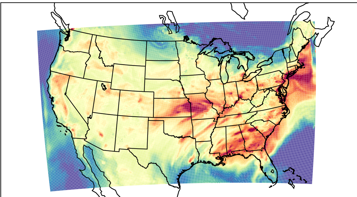
WRF (2023-07-19_20:00:00)
