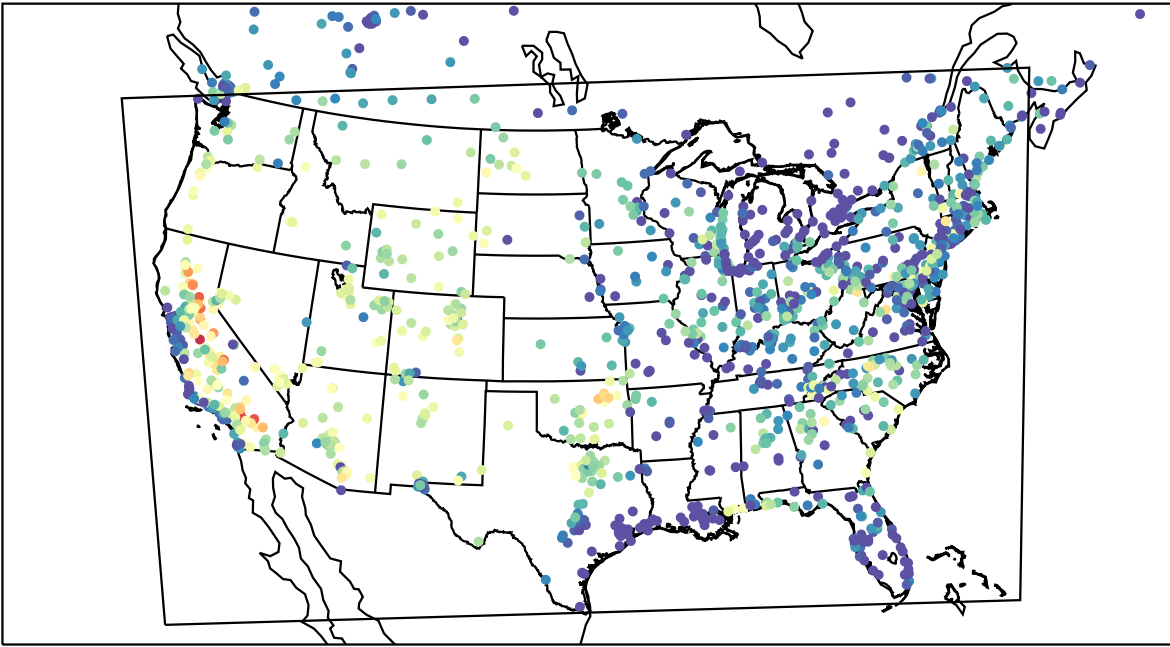
AirNOW (2023-07-19_03:00:00)
