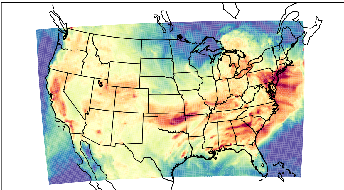
WRF (2023-07-20_21:00:00)
