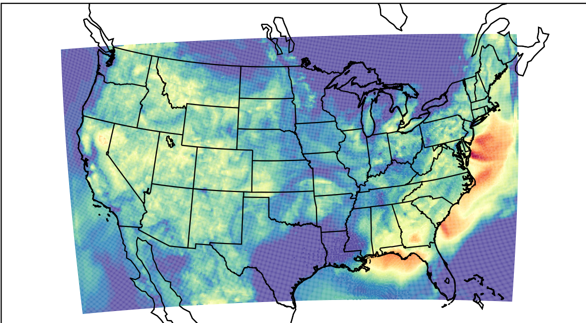
WRF (2023-07-19_10:00:00)
