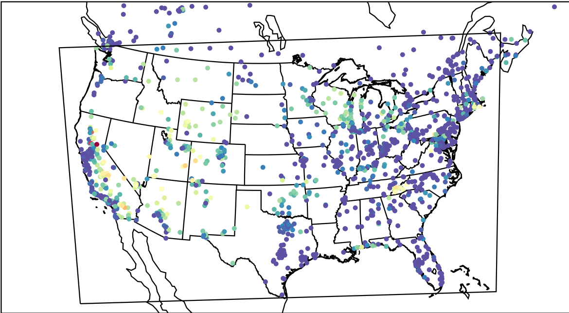
AirNOW (2023-07-20_07:00:00)
