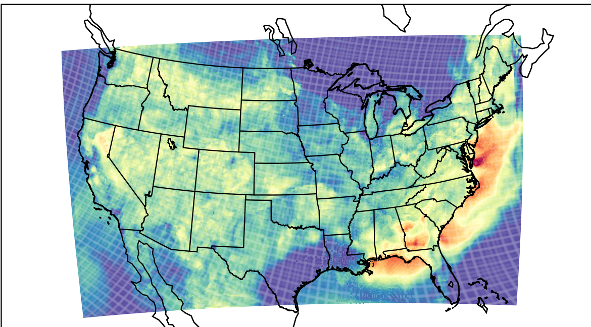
WRF (2023-07-19_06:00:00)
