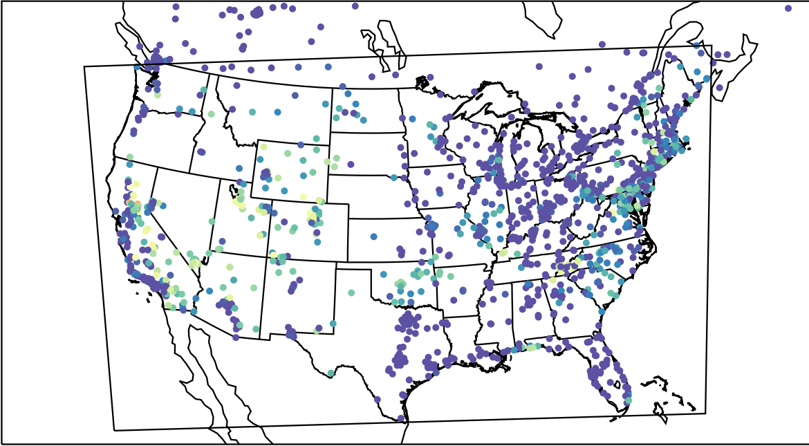
AirNOW (2023-07-19_11:00:00)
