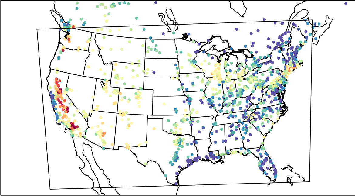
AirNOW (2023-07-20_01:00:00)
