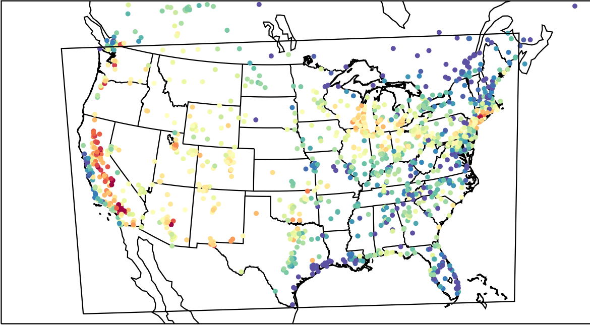
AirNOW (2023-07-20_00:00:00)
