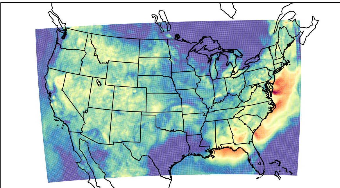
WRF (2023-07-19_08:00:00)
