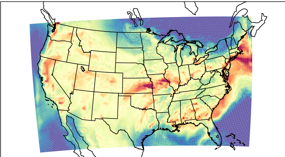
WRF (2023-07-20_00:00:00)
