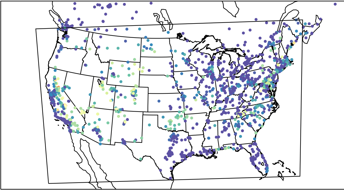
AirNOW (2023-07-19_09:00:00)
