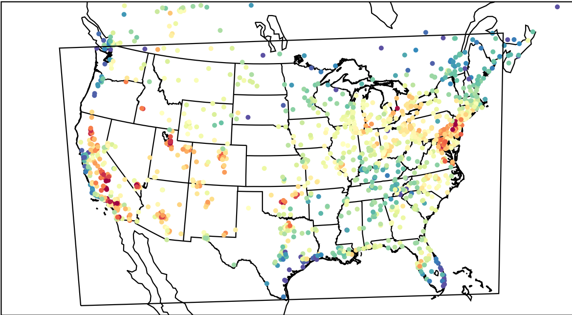
AirNOW (2023-07-20_19:00:00)
