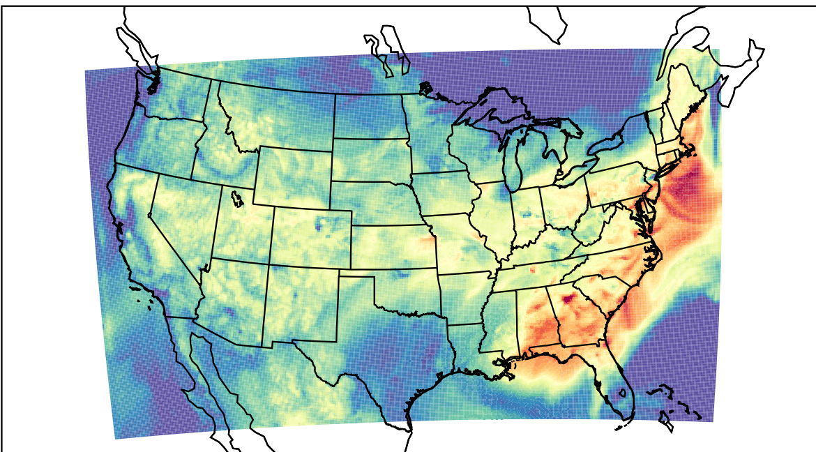
WRF (2023-07-19_15:00:00)
