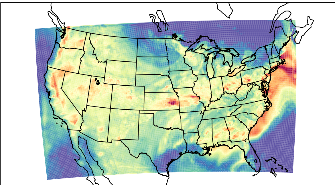
WRF (2023-07-20_02:00:00)
