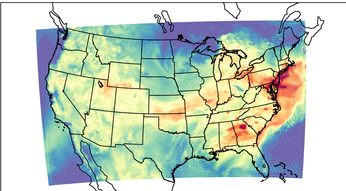
WRF (2023-07-20_16:00:00)
