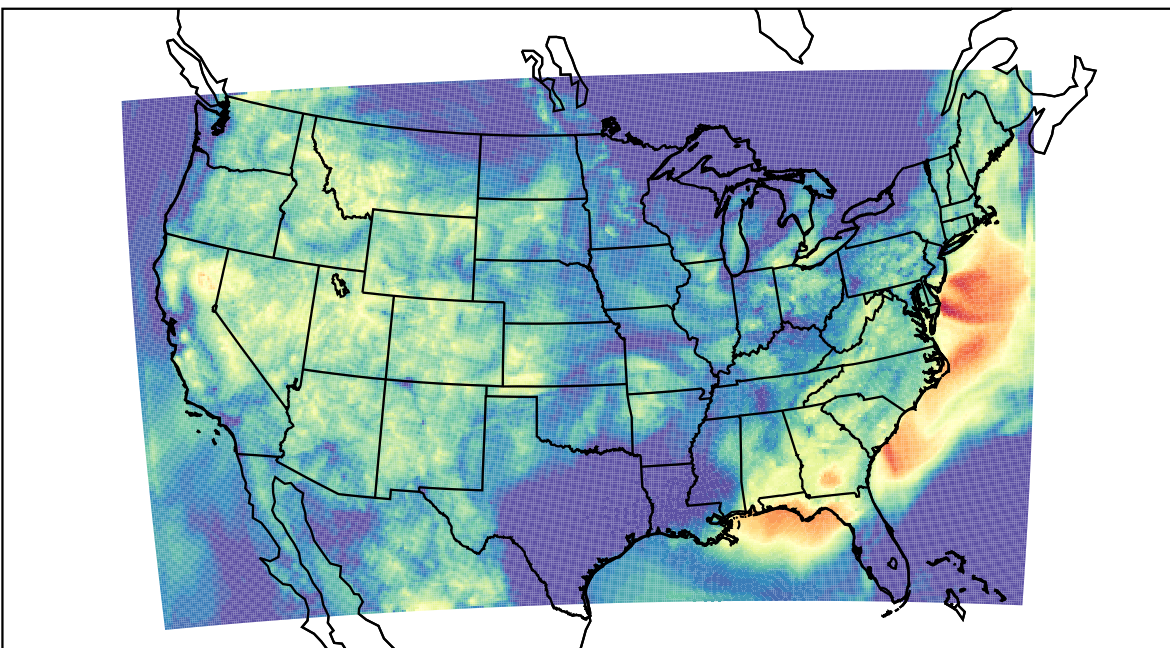
WRF (2023-07-19_11:00:00)
