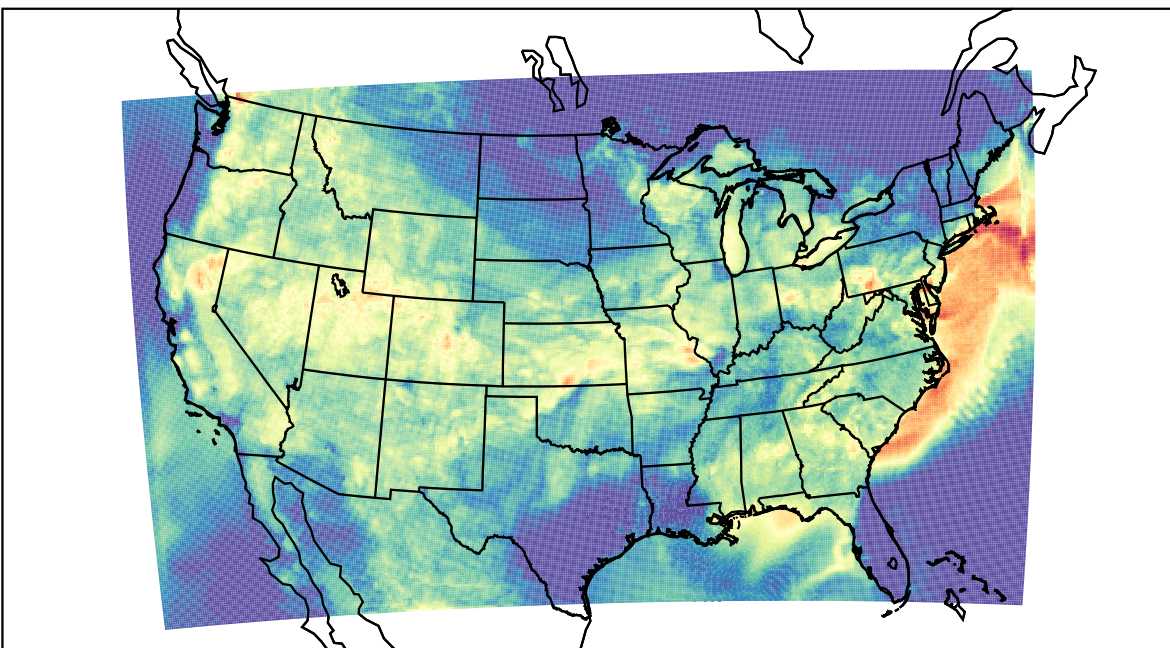
WRF (2023-07-20_06:00:00)
