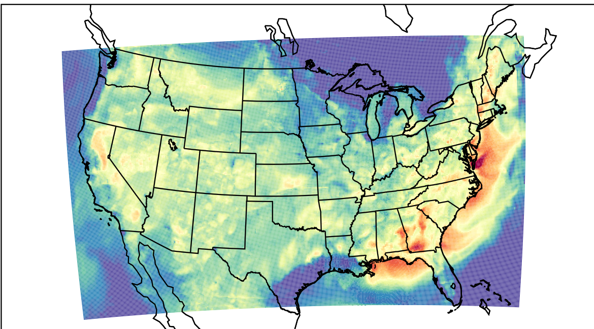
WRF (2023-07-19_03:00:00)
