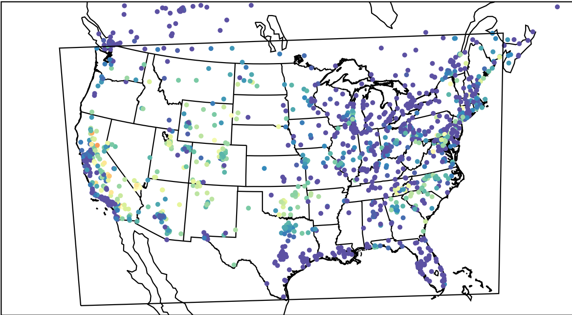
AirNOW (2023-07-19_07:00:00)
