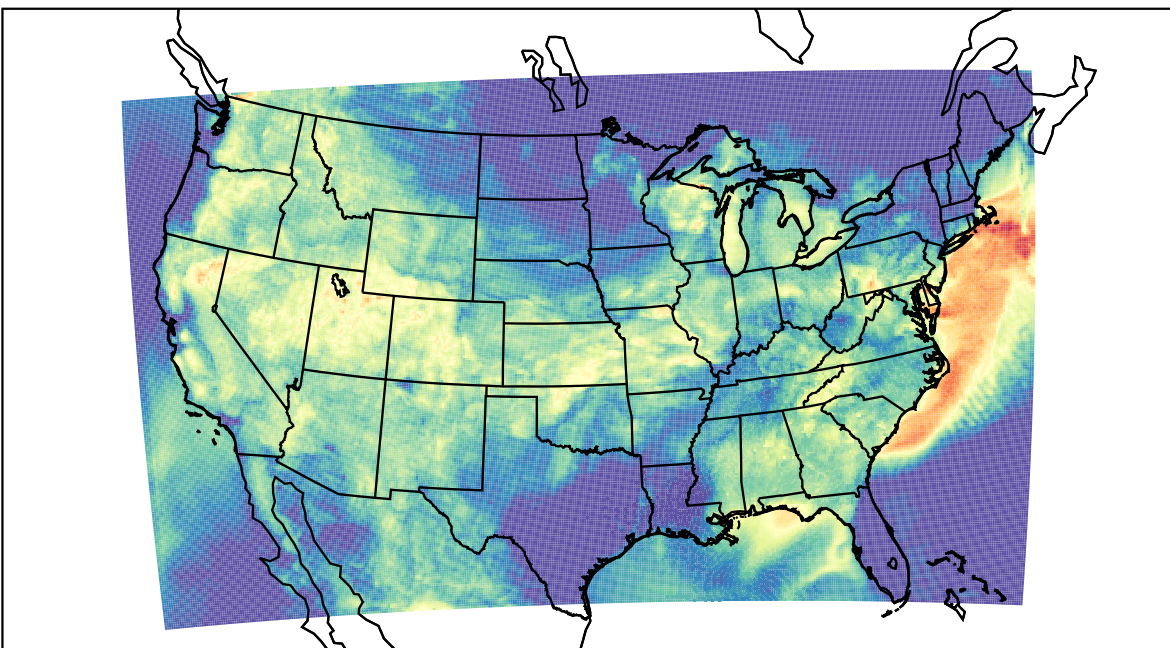
WRF (2023-07-20_08:00:00)
