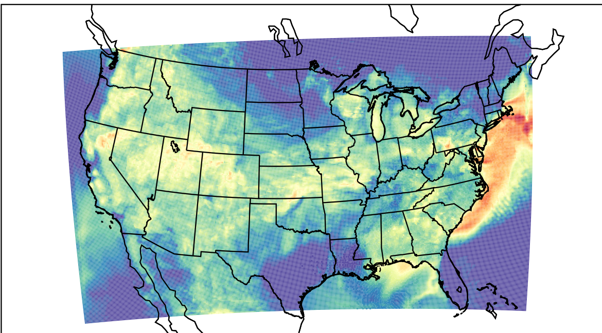
WRF (2023-07-20_07:00:00)
