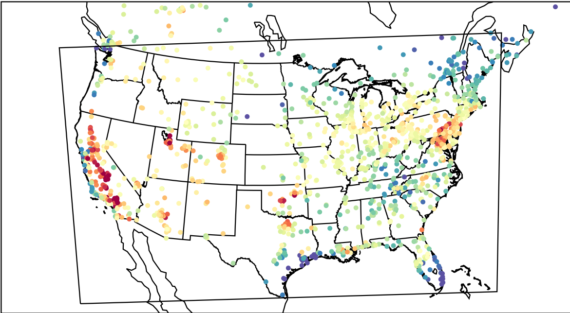
AirNOW (2023-07-20_22:00:00)
