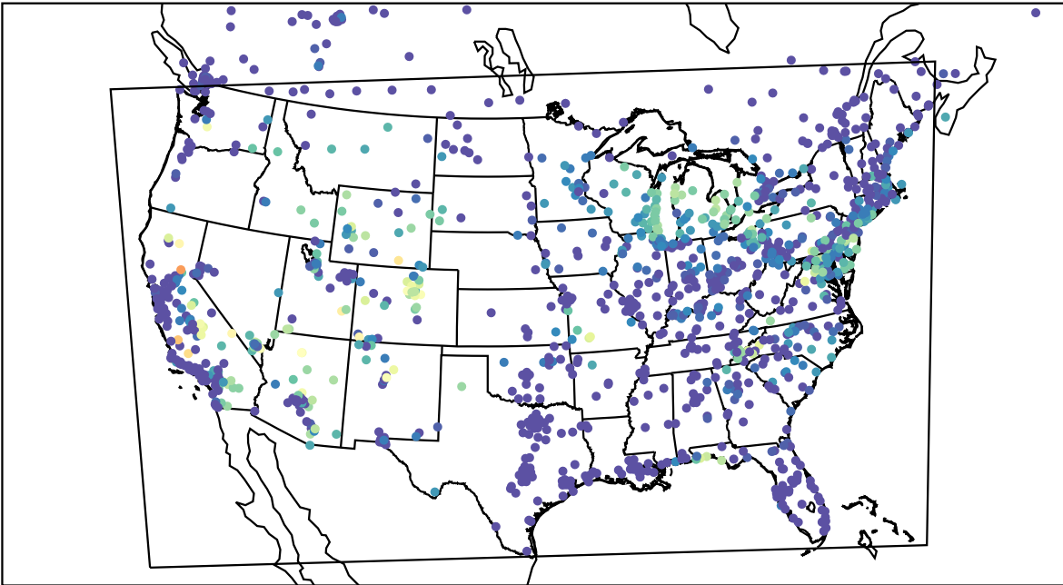
AirNOW (2023-07-20_12:00:00)
