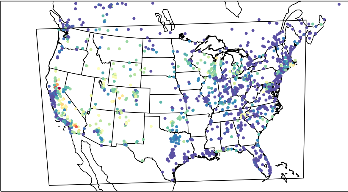
AirNOW (2023-07-20_06:00:00)
