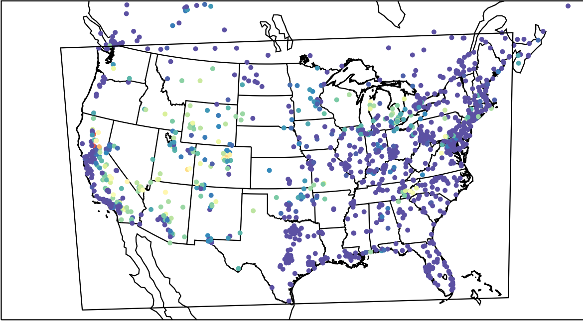
AirNOW (2023-07-20_10:00:00)
