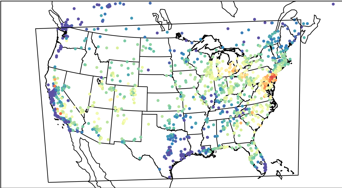
AirNOW (2023-07-20_15:00:00)
