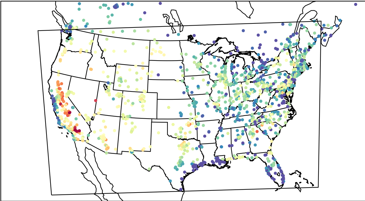
AirNOW (2023-07-19_01:00:00)
