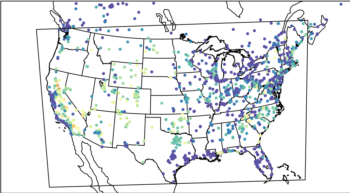
AirNOW (2023-07-19_05:00:00)
