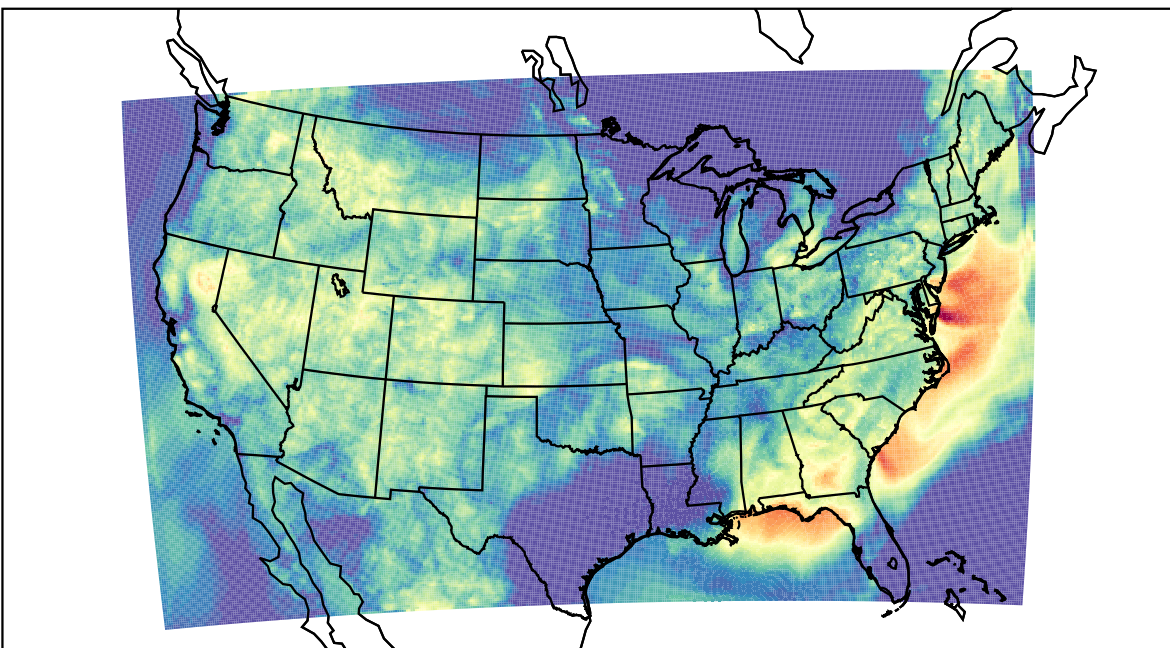
WRF (2023-07-19_09:00:00)
