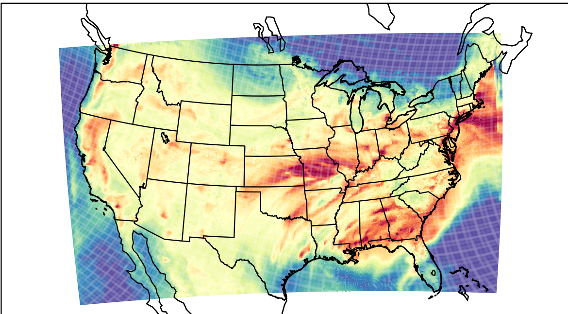
WRF (2023-07-19_22:00:00)
