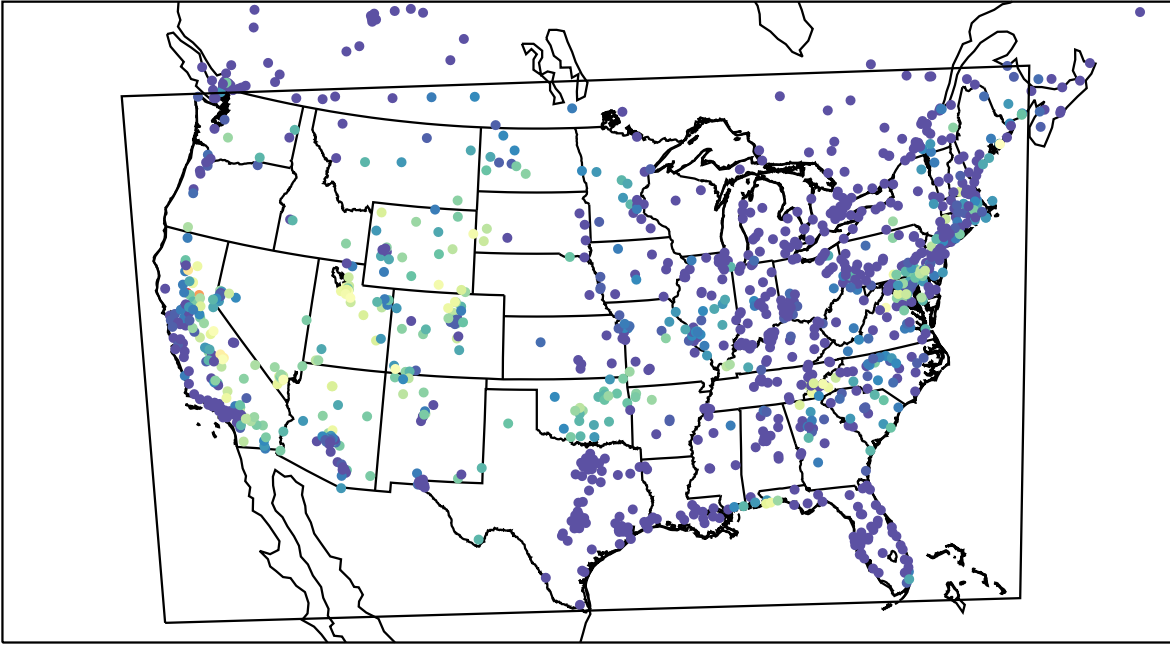
AirNOW (2023-07-19_10:00:00)
