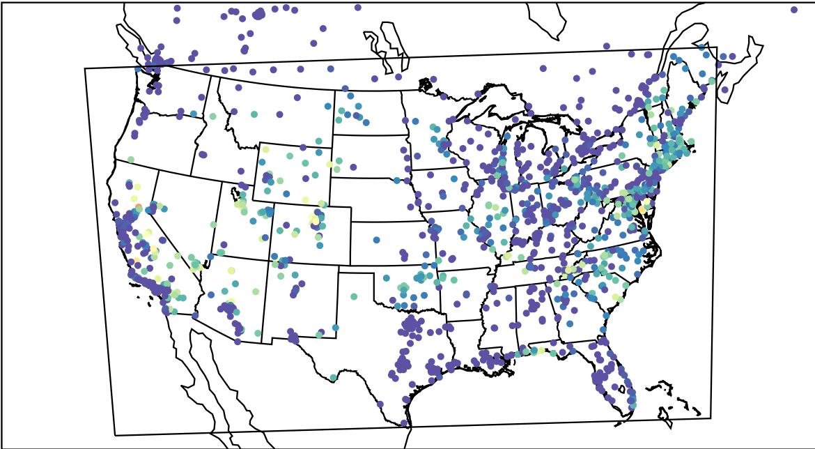
AirNOW (2023-07-19_12:00:00)
