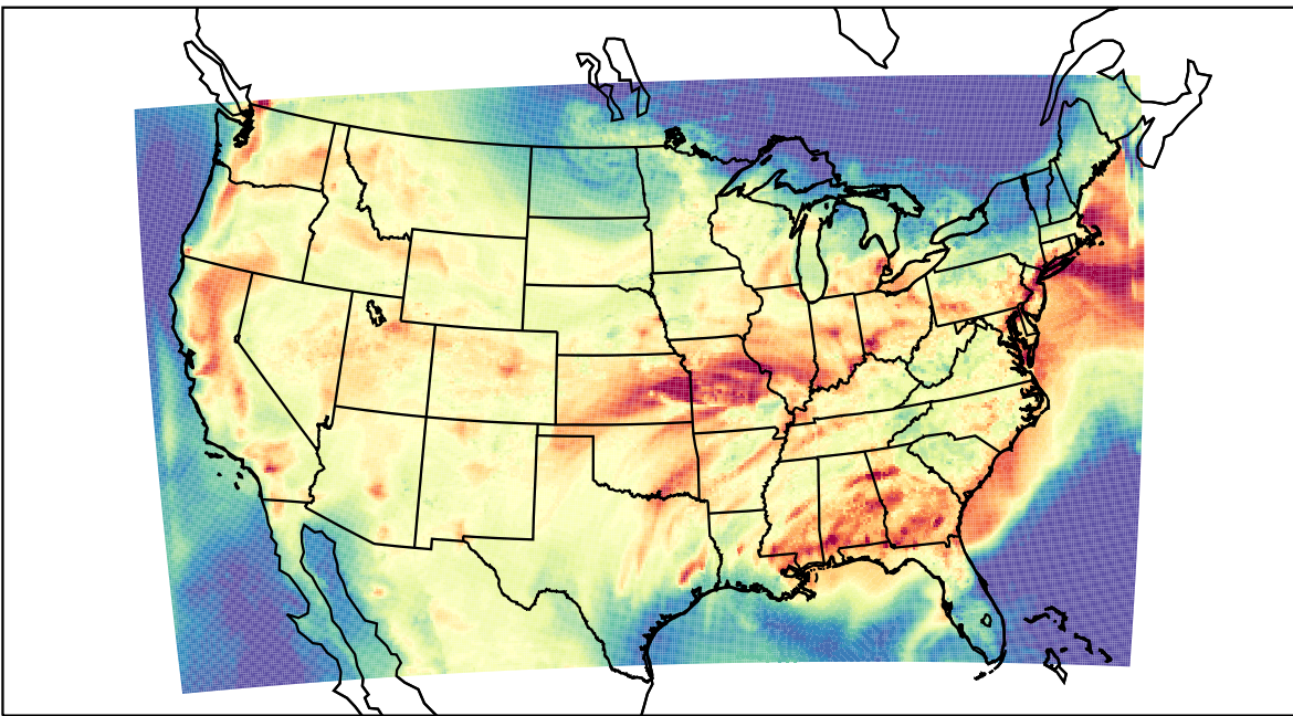
WRF (2023-07-19_23:00:00)
