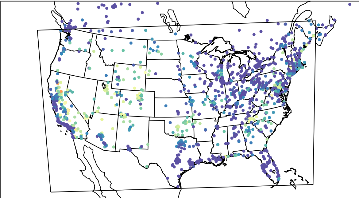
AirNOW (2023-07-19_08:00:00)
