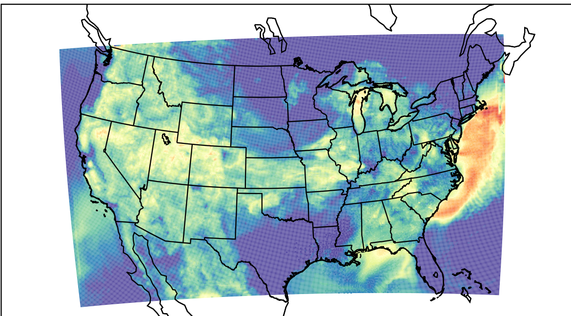
WRF (2023-07-20_11:00:00)
