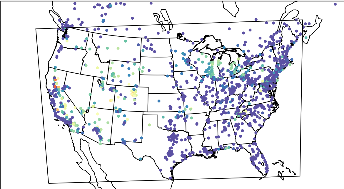
AirNOW (2023-07-20_11:00:00)
