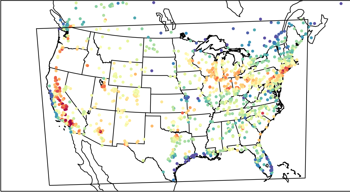
AirNOW (2023-07-19_22:00:00)
