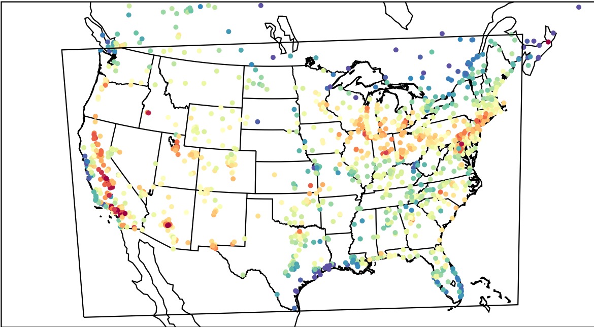
AirNOW (2023-07-19_20:00:00)
