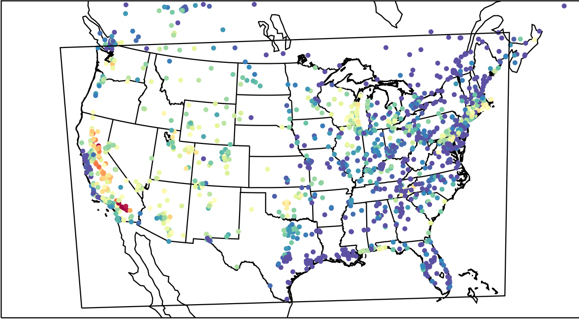
AirNOW (2023-07-20_03:00:00)
