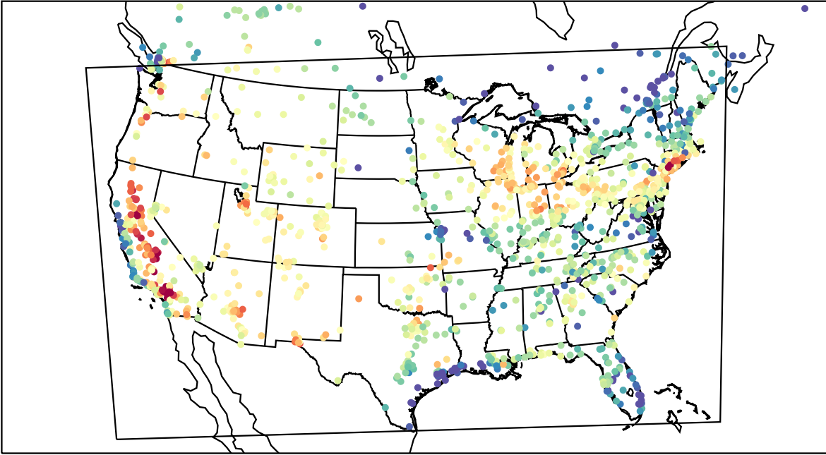
AirNOW (2023-07-19_23:00:00)
