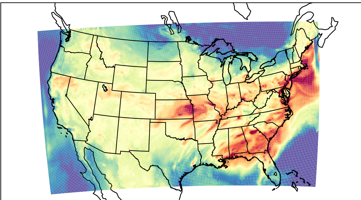
WRF (2023-07-19_18:00:00)
