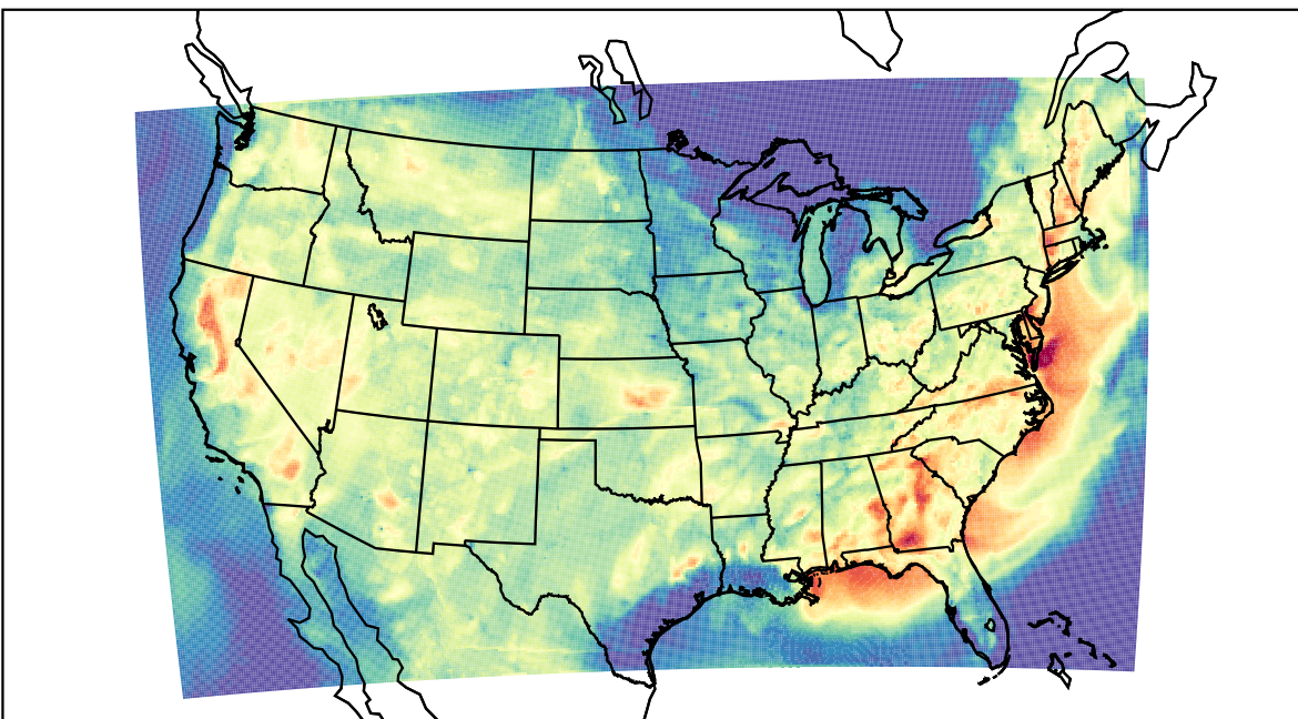
WRF (2023-07-19_02:00:00)
