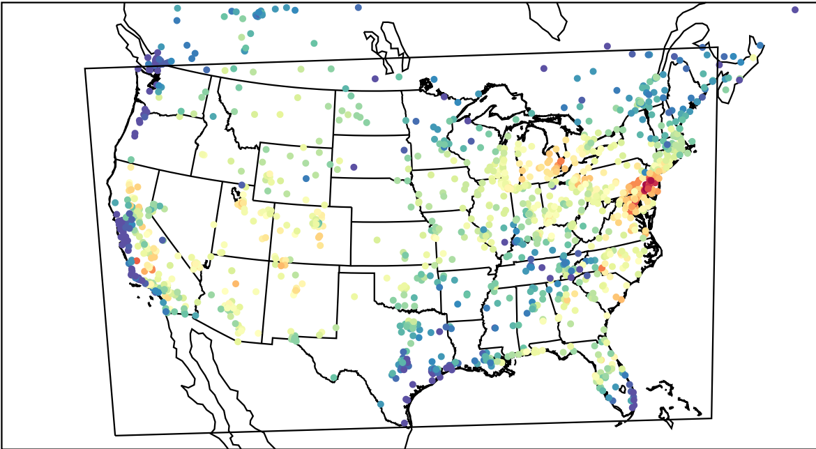
AirNOW (2023-07-20_16:00:00)
