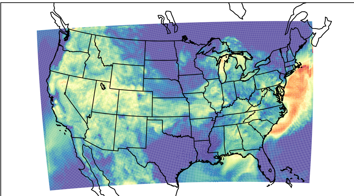
WRF (2023-07-20_12:00:00)
