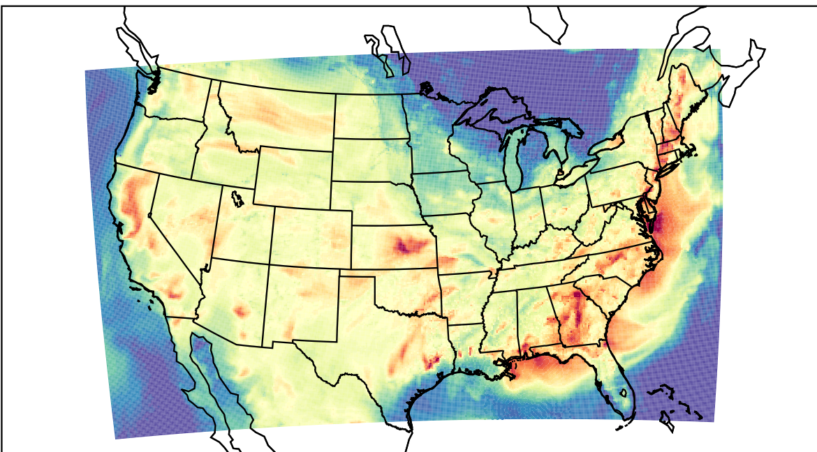
WRF (2023-07-19_00:00:00)
