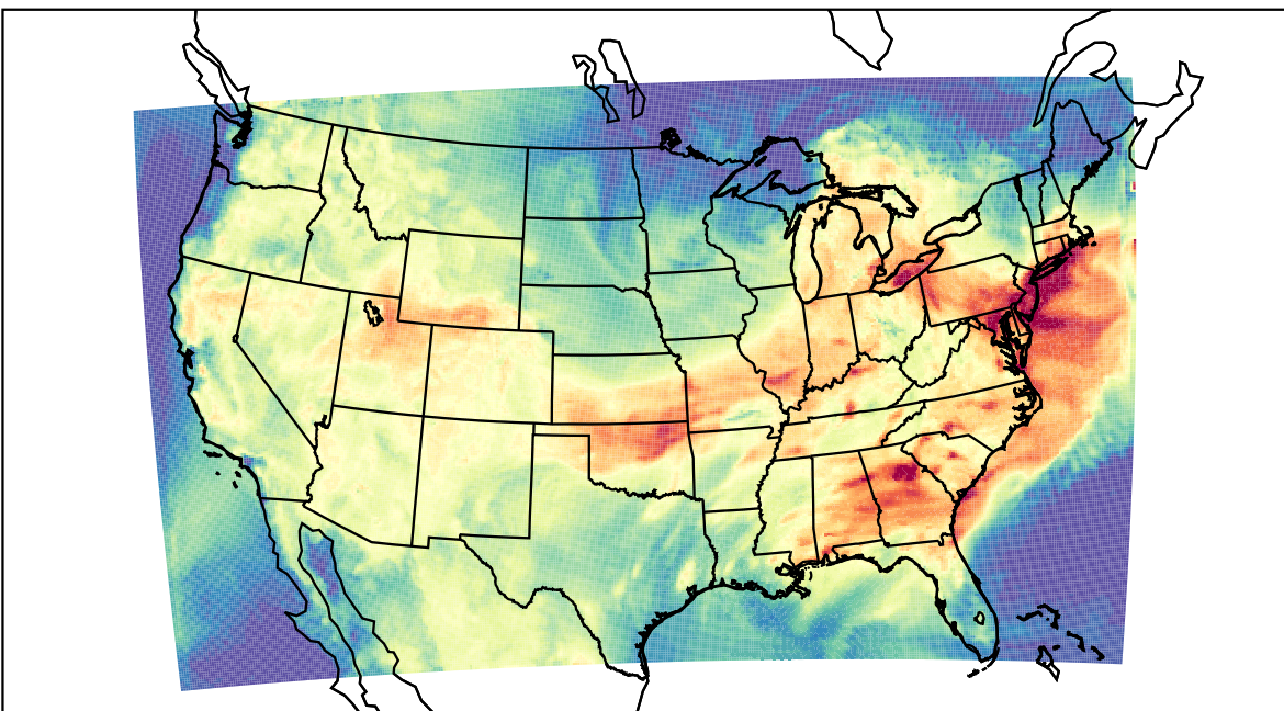
WRF (2023-07-20_17:00:00)
