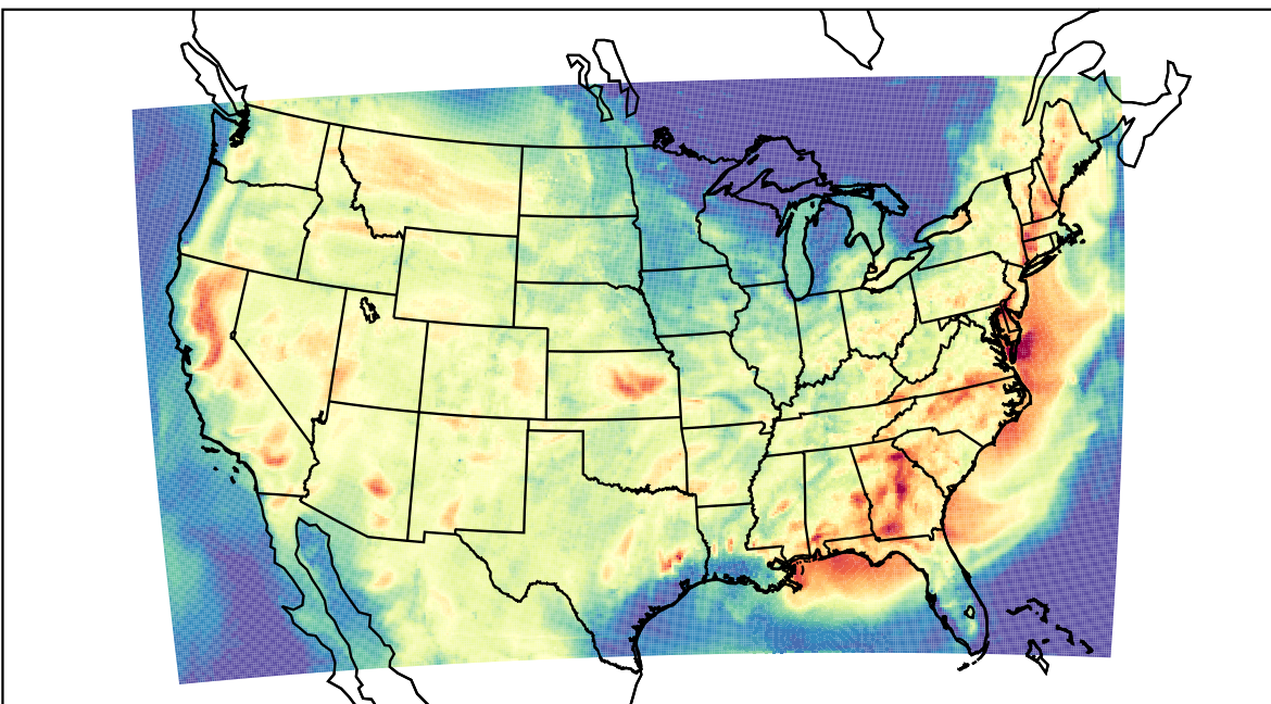
WRF (2023-07-19_01:00:00)
