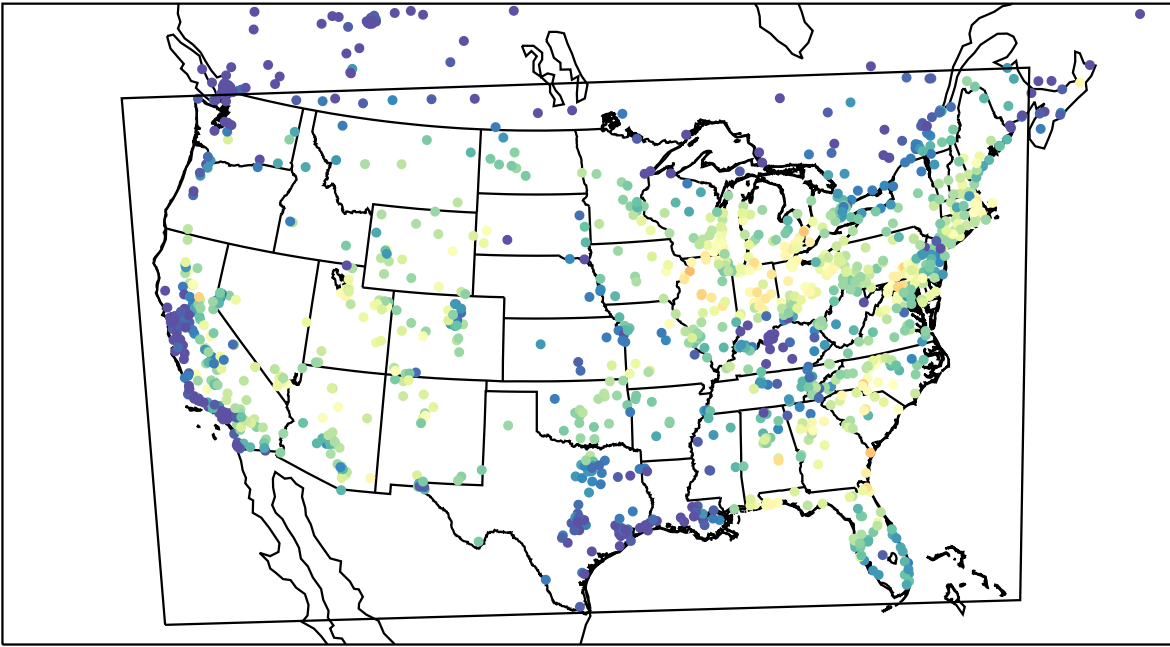
AirNOW (2023-07-19_15:00:00)
