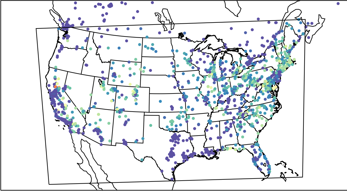
AirNOW (2023-07-19_13:00:00)
