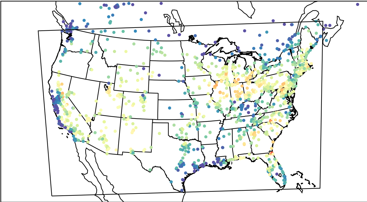
AirNOW (2023-07-19_16:00:00)
