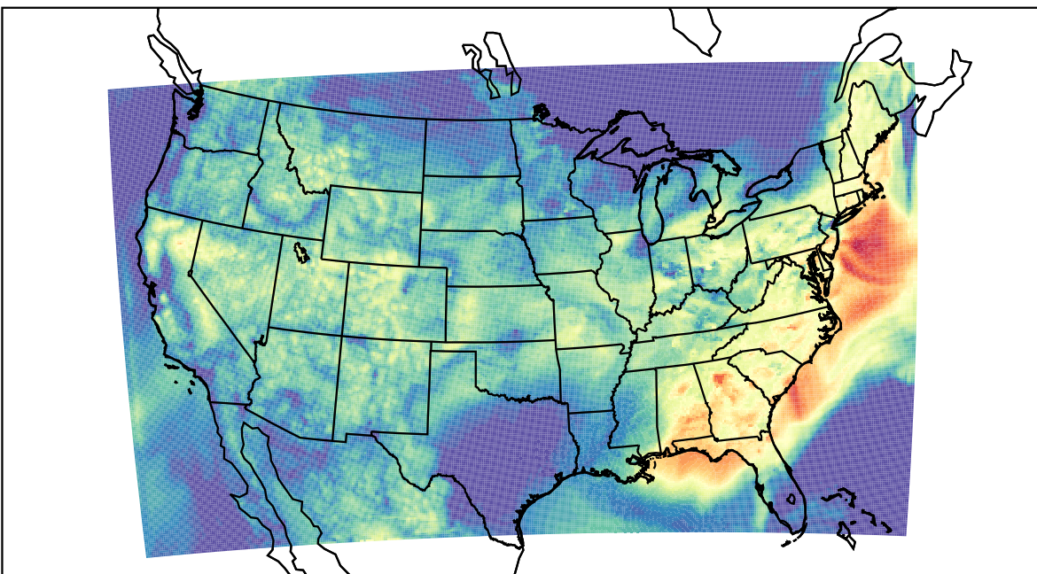
WRF (2023-07-19_14:00:00)
