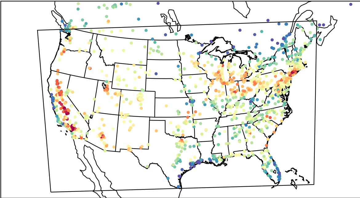
AirNOW (2023-07-19_21:00:00)
