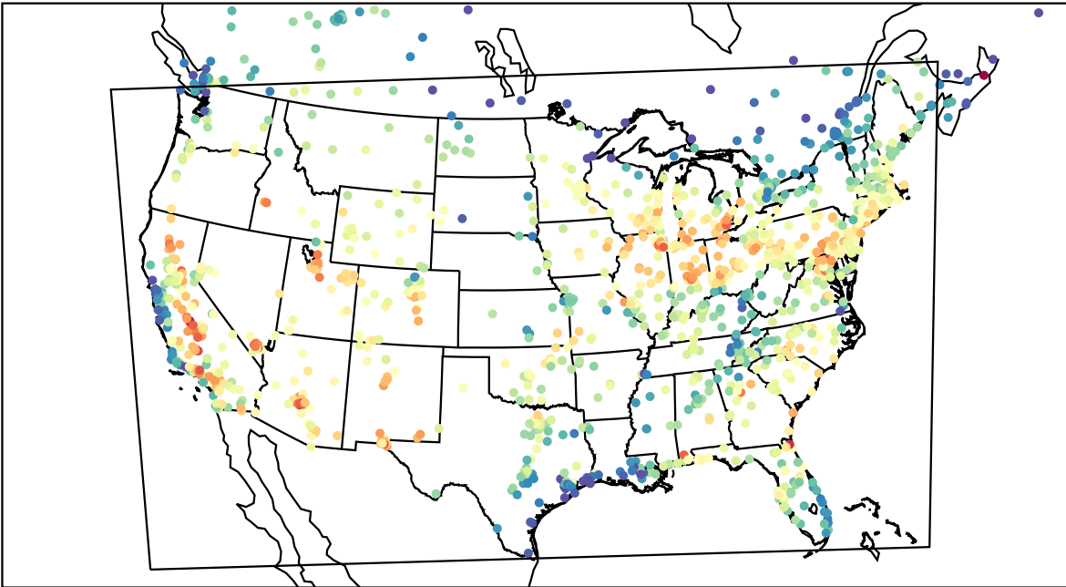
AirNOW (2023-07-19_18:00:00)
