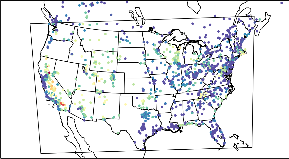
AirNOW (2023-07-20_05:00:00)
