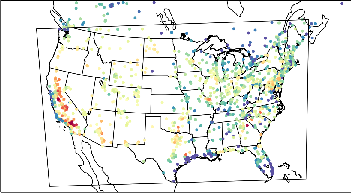
AirNOW (2023-07-19_00:00:00)
