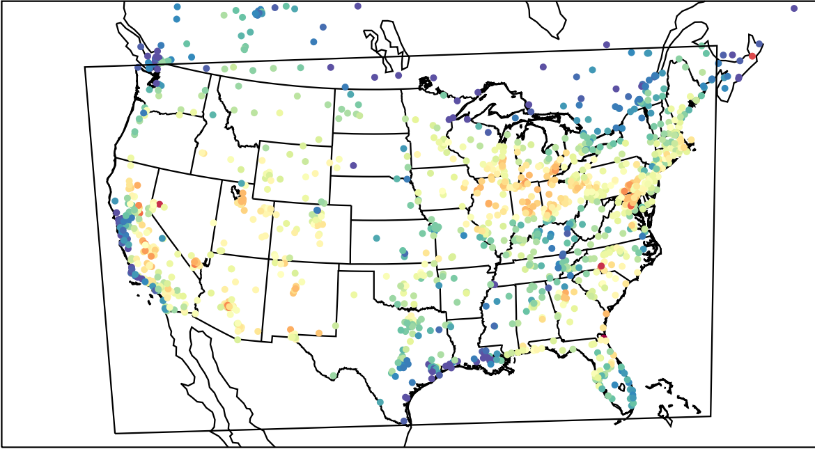
AirNOW (2023-07-19_17:00:00)
