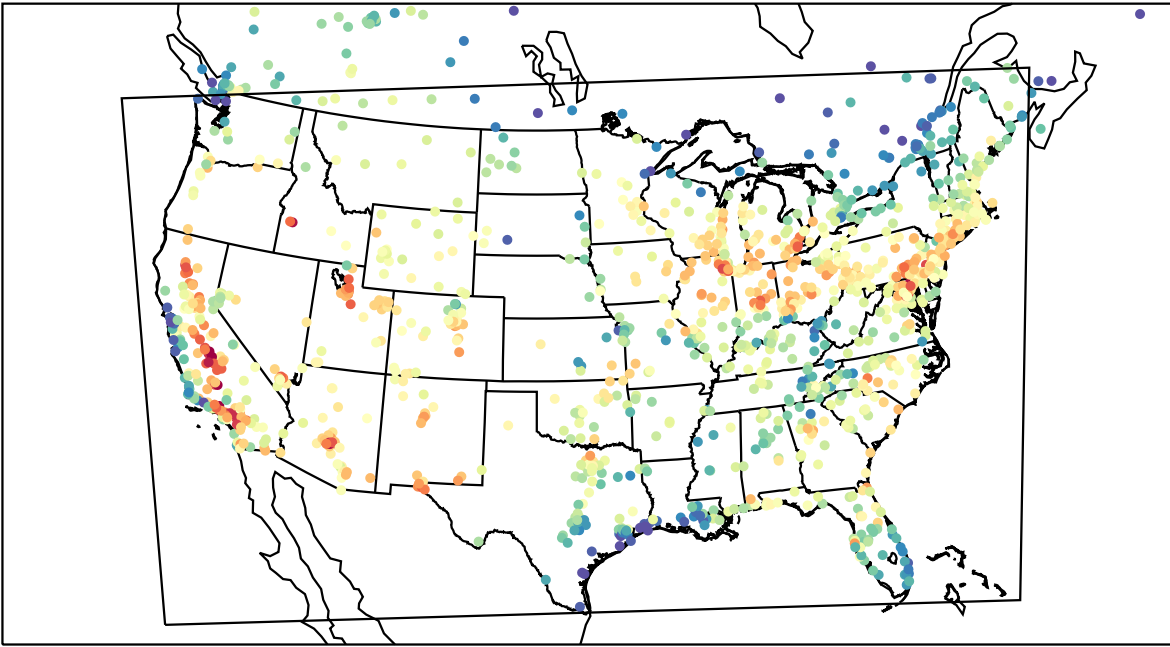
AirNOW (2023-07-19_19:00:00)
