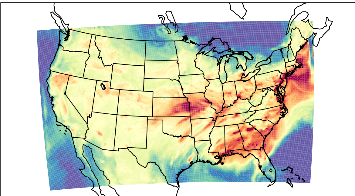
WRF (2023-07-19_19:00:00)
