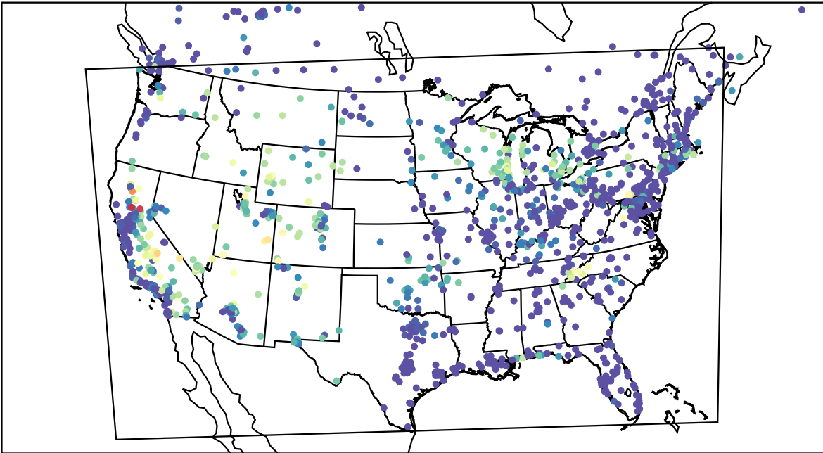
AirNOW (2023-07-20_08:00:00)
