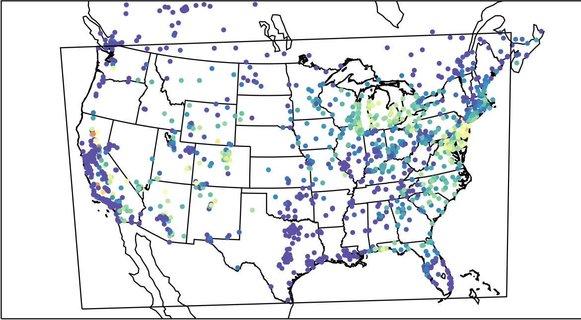
AirNOW (2023-07-20_13:00:00)
