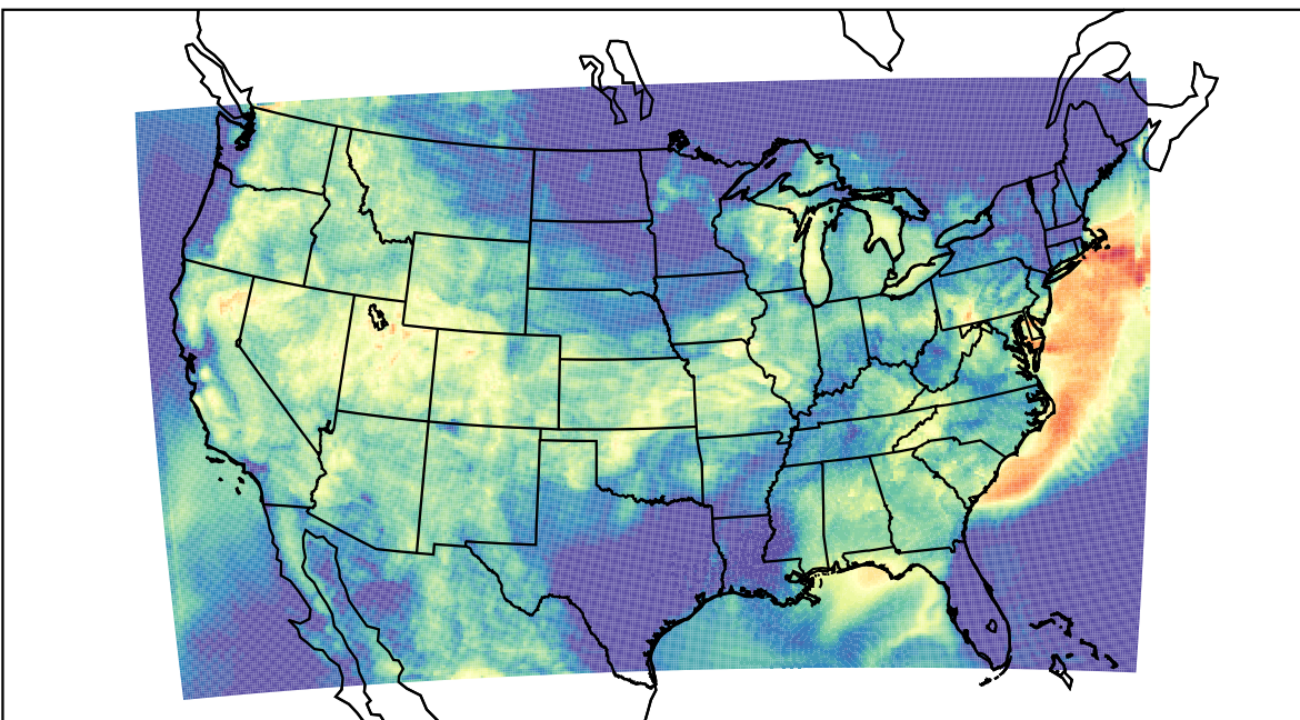
WRF (2023-07-20_09:00:00)
