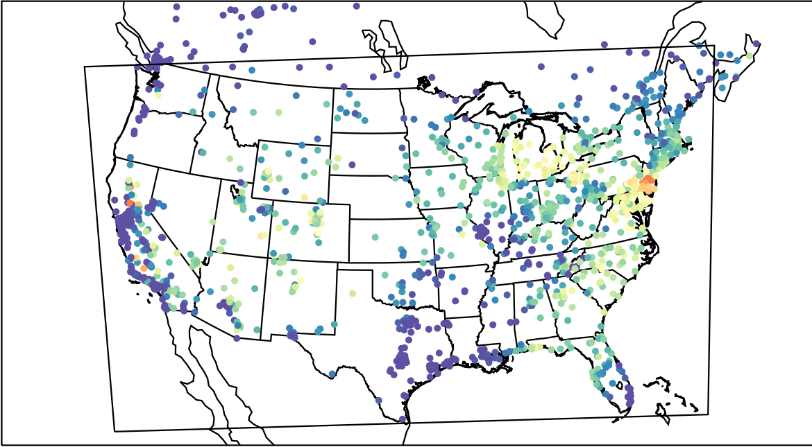
AirNOW (2023-07-20_14:00:00)
