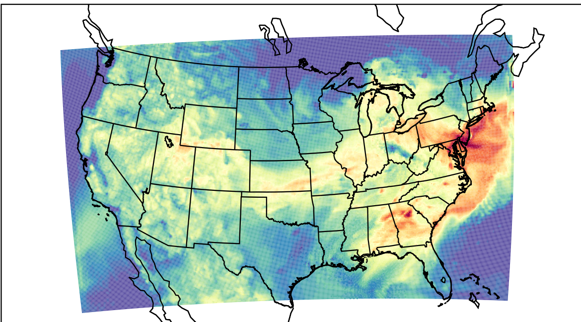
WRF (2023-07-20_15:00:00)
