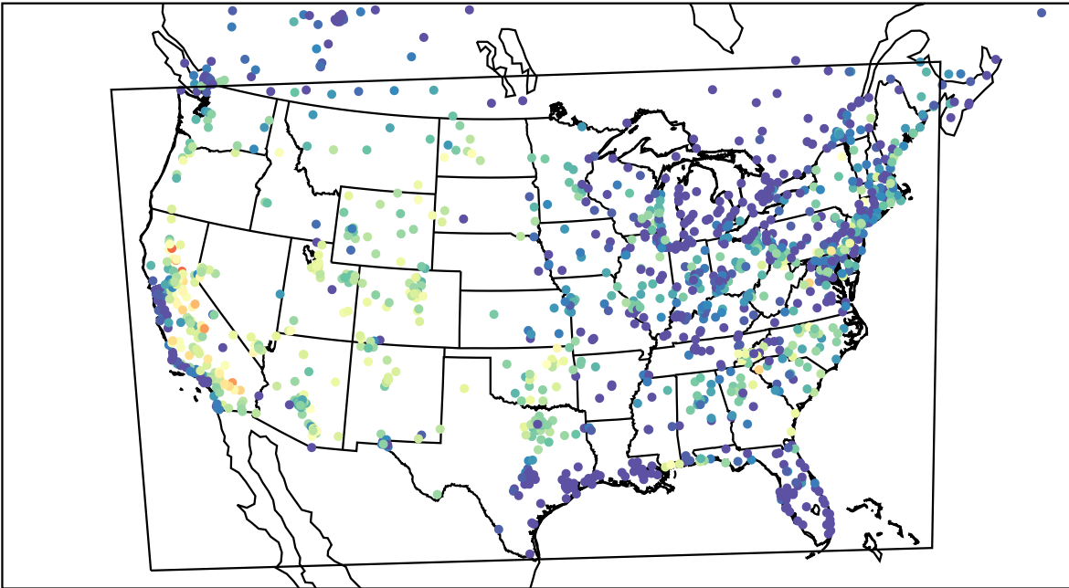
AirNOW (2023-07-19_04:00:00)
