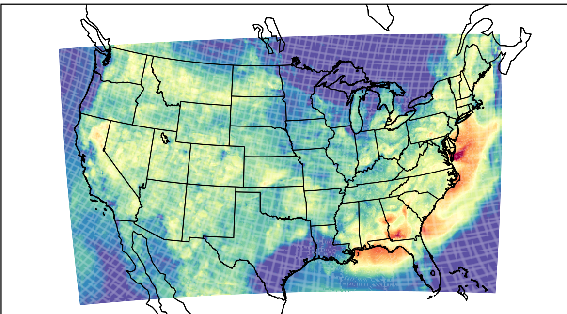
WRF (2023-07-19_05:00:00)
