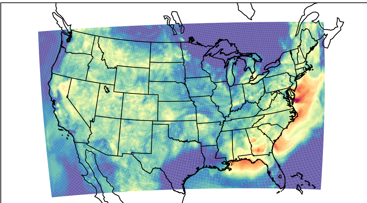
WRF (2023-07-19_07:00:00)
