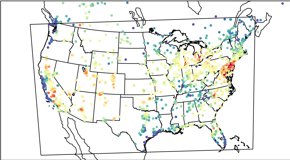
AirNOW (2023-07-20_17:00:00)
