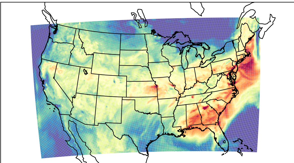
WRF (2023-07-19_16:00:00)
