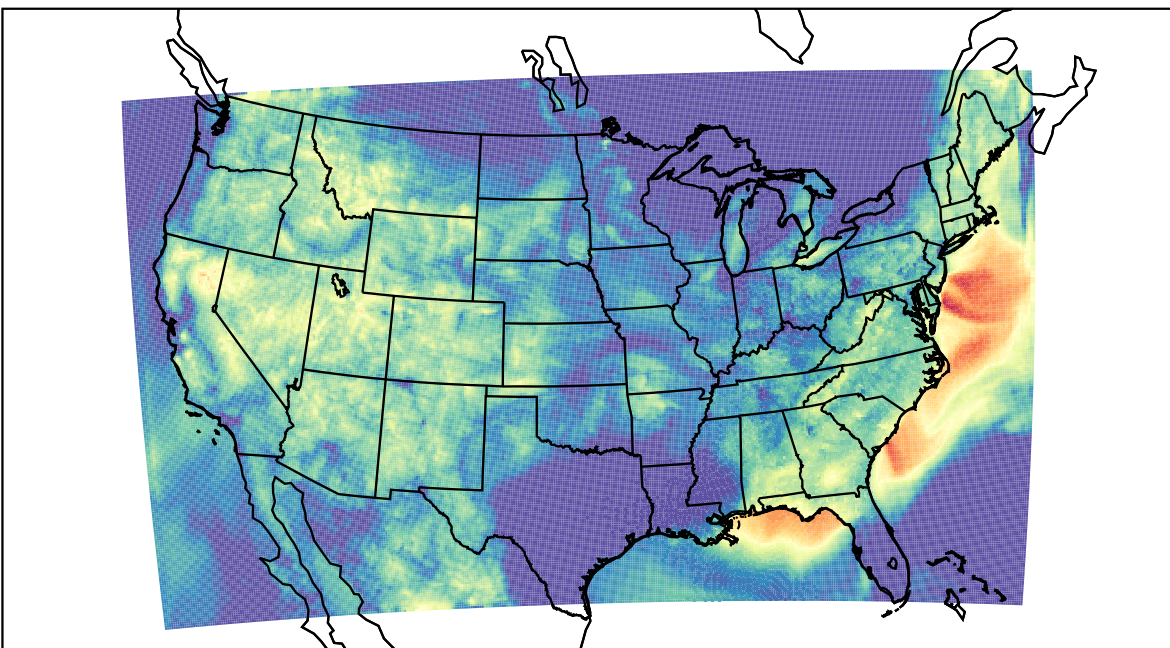
WRF (2023-07-19_12:00:00)
