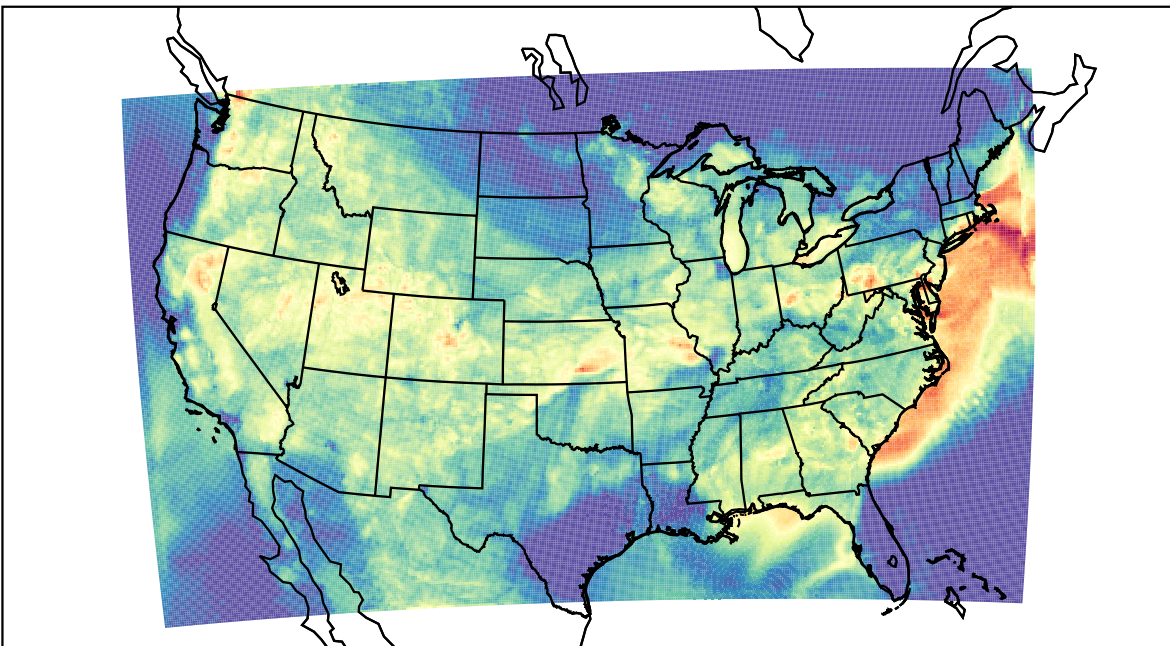
WRF (2023-07-20_05:00:00)
