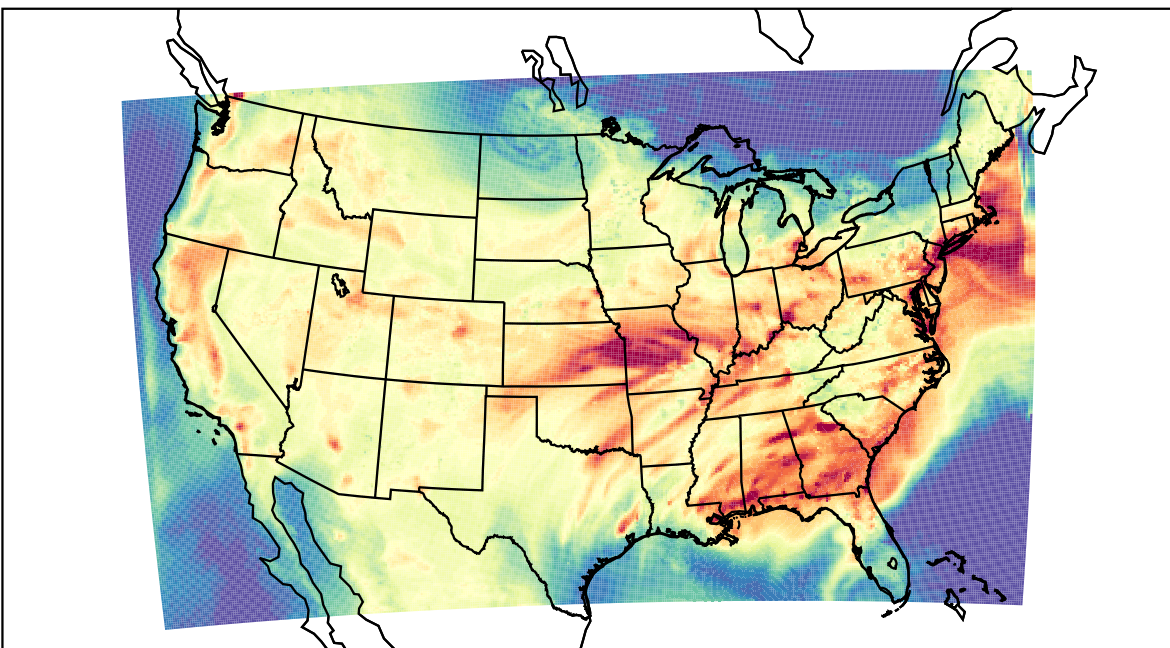
WRF (2023-07-19_21:00:00)
