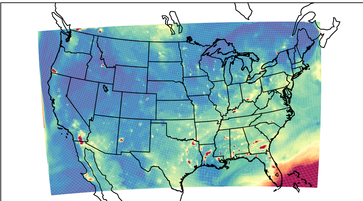
WRF 2023-07-21_02:00:00
