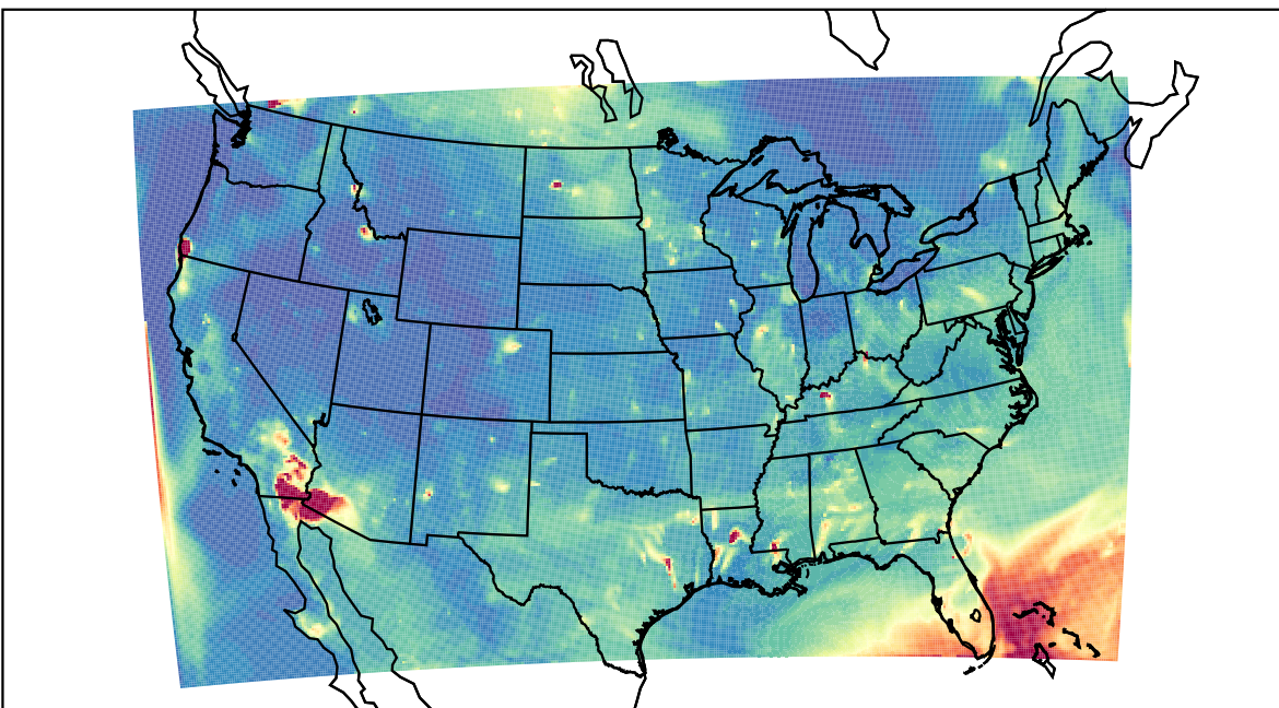
WRF 2023-07-22_04:00:00
