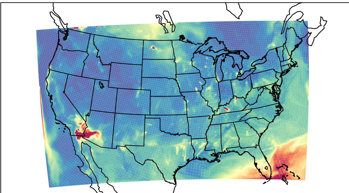
WRF 2023-07-22_08:00:00
