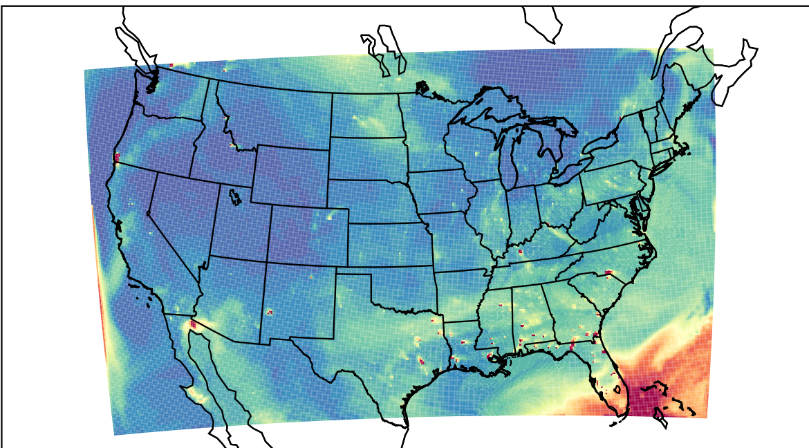
WRF 2023-07-22_00:00:00
