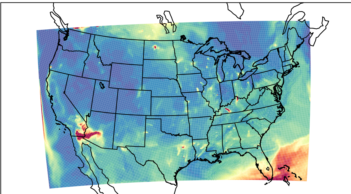
WRF 2023-07-22_09:00:00
