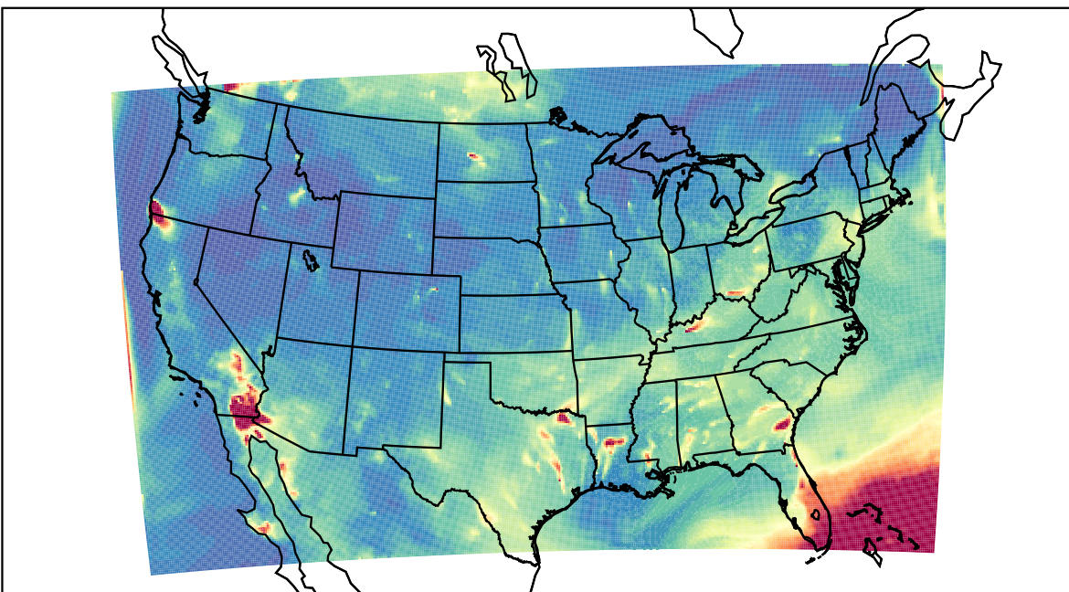
WRF 2023-07-21_05:00:00
