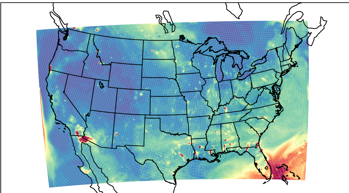
WRF 2023-07-22_02:00:00
