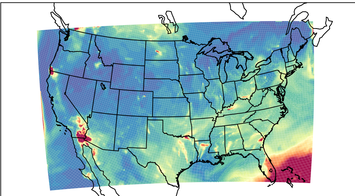
WRF 2023-07-21_06:00:00
