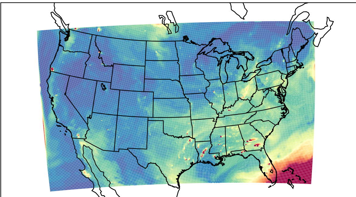
WRF 2023-07-21_00:00:00
