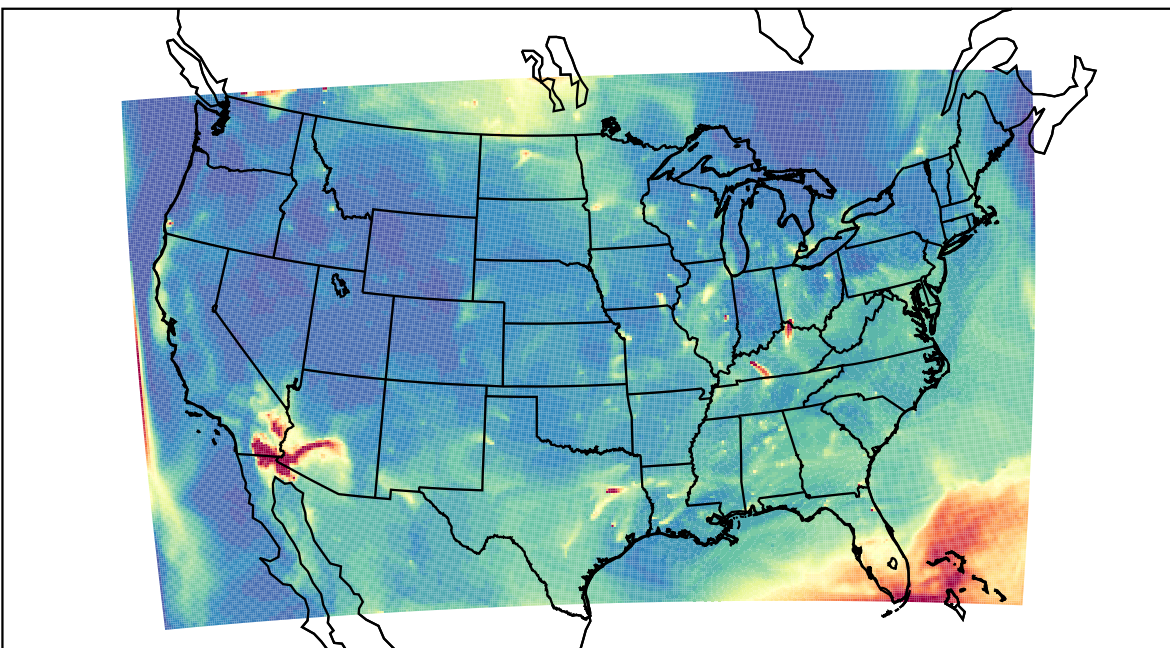
WRF 2023-07-22_11:00:00
