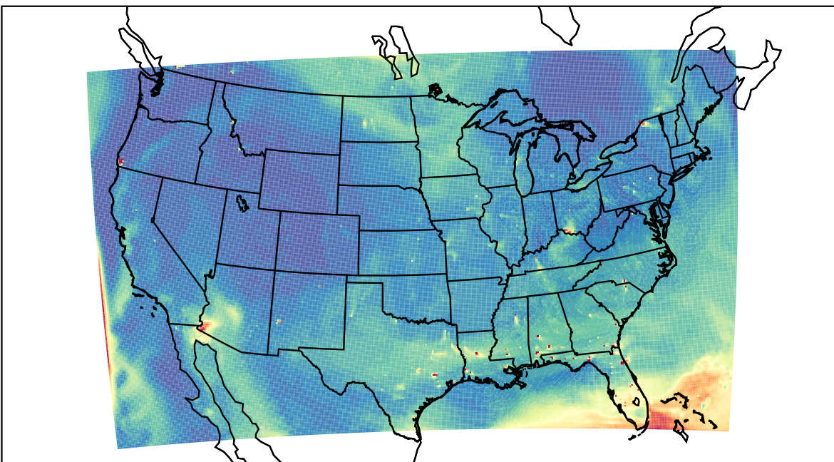
WRF 2023-07-22_22:00:00
