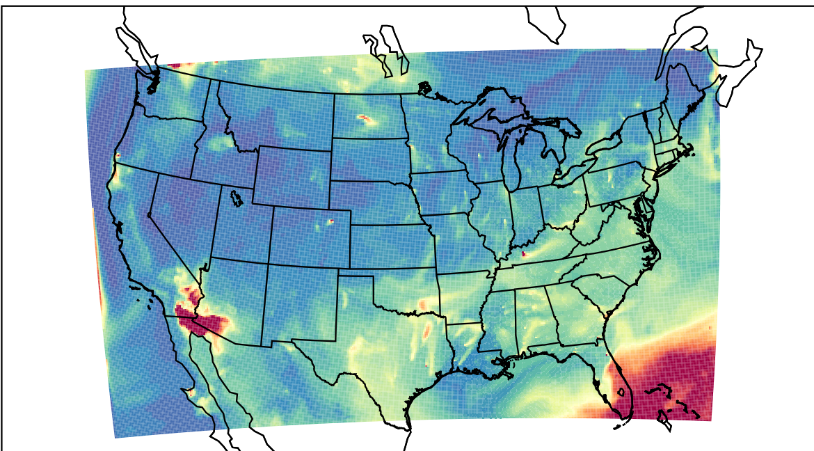
WRF 2023-07-21_09:00:00
