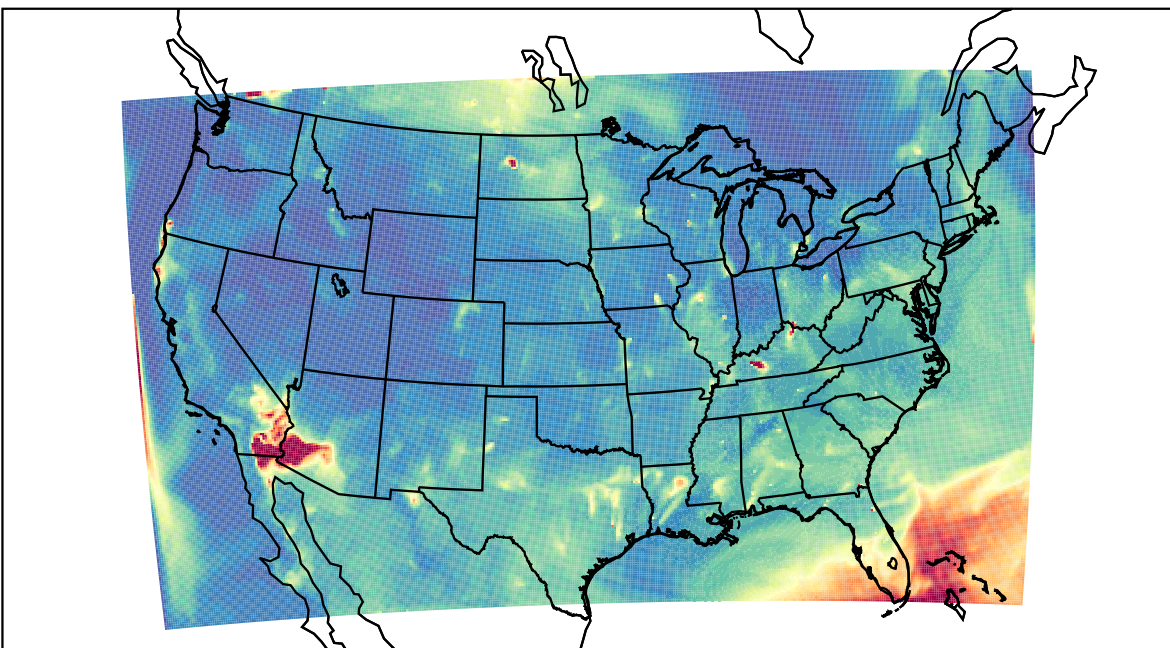
WRF 2023-07-22_07:00:00
