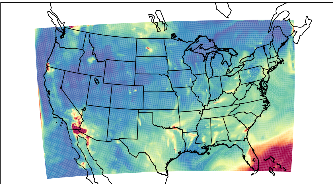
WRF 2023-07-21_07:00:00
