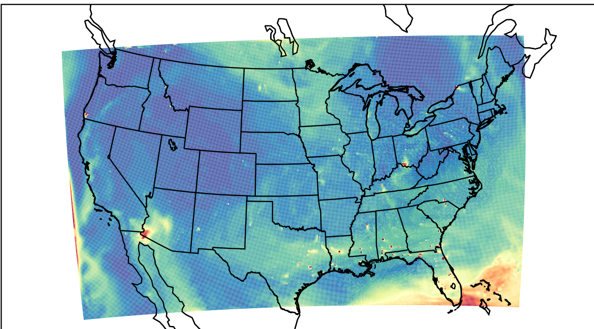
WRF 2023-07-22_21:00:00
