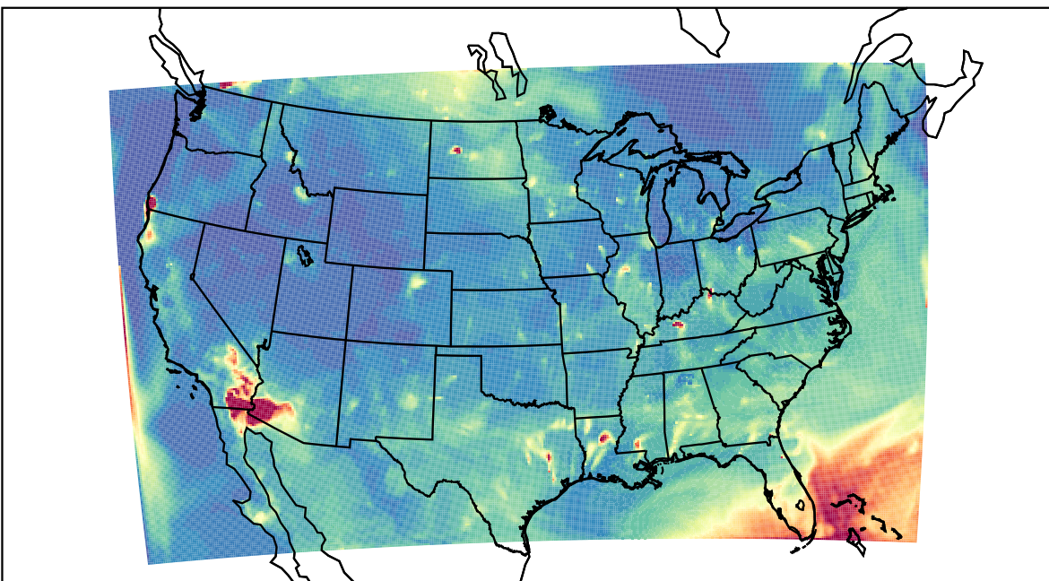
WRF 2023-07-22_05:00:00
