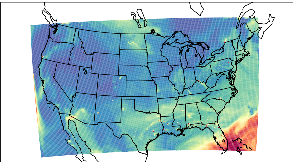
WRF 2023-07-21_21:00:00
