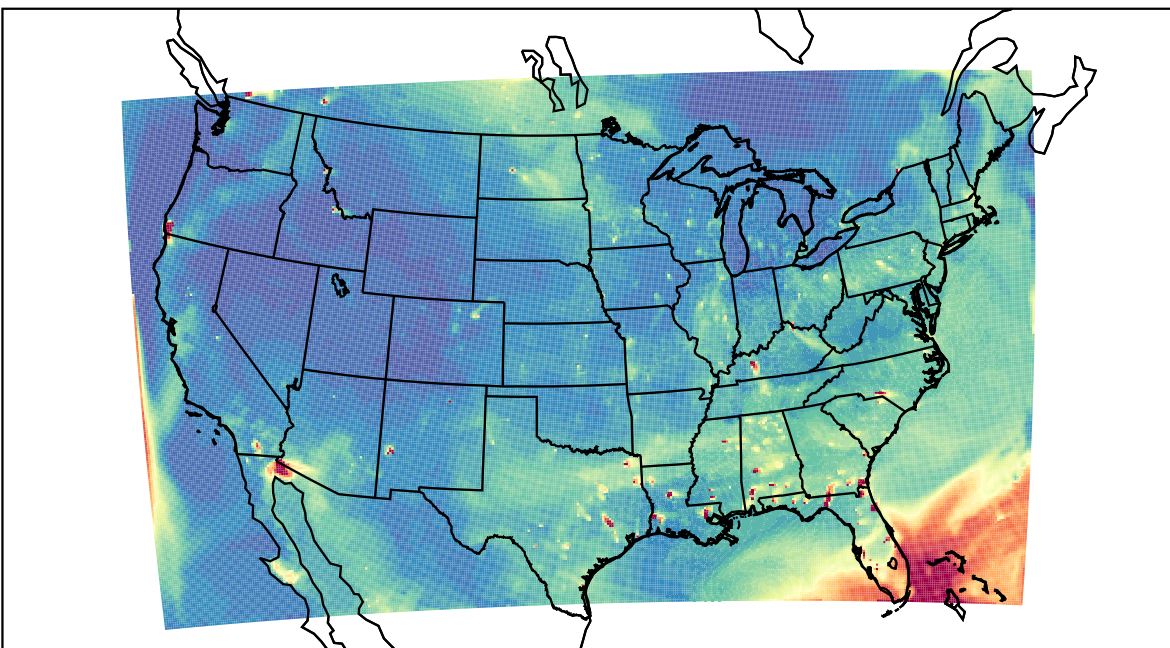
WRF 2023-07-22_01:00:00
