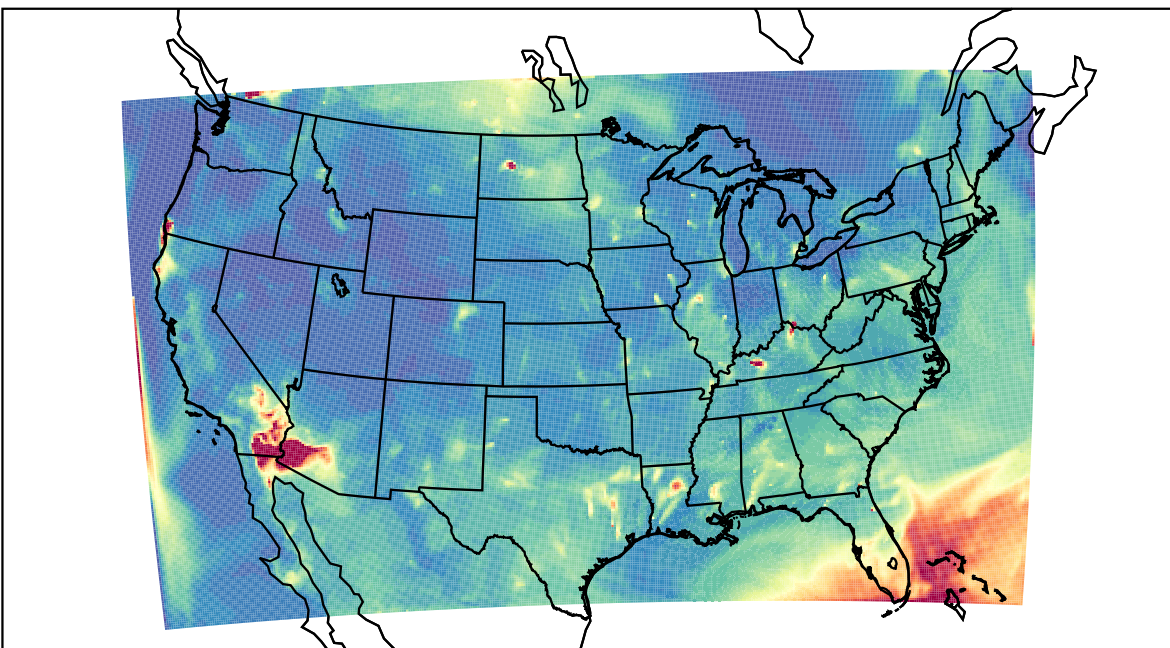
WRF 2023-07-22_06:00:00
