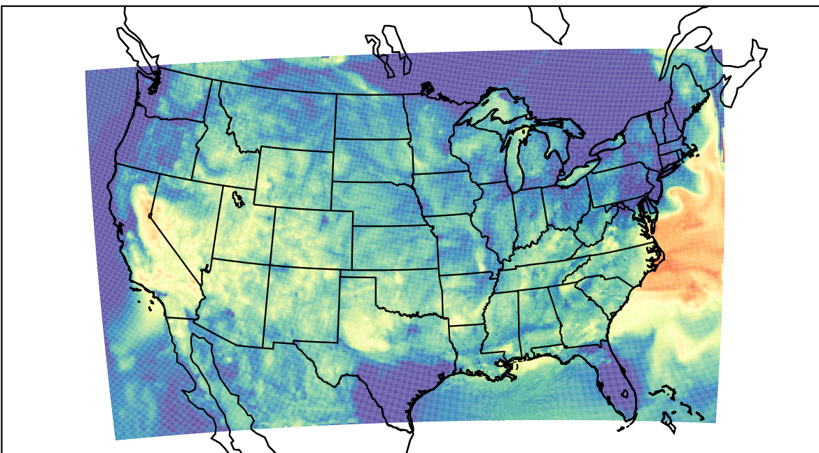
WRF (2023-07-23_12:00:00)
