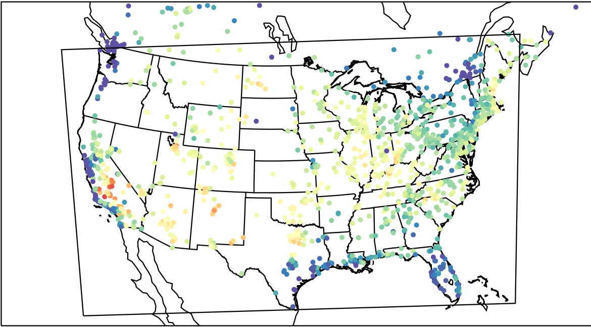
AirNOW (2023-07-22_16:00:00)
