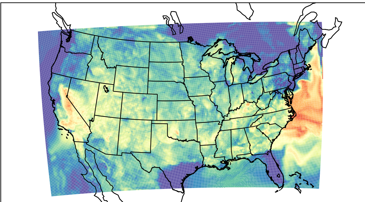
WRF (2023-07-23_08:00:00)
