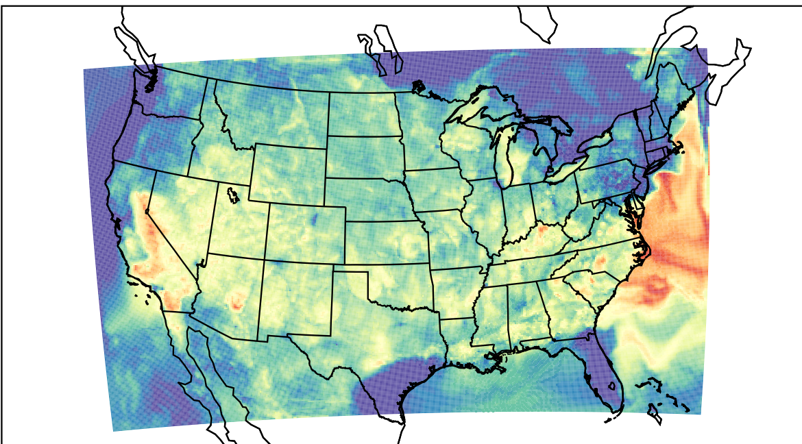
WRF (2023-07-23_06:00:00)
