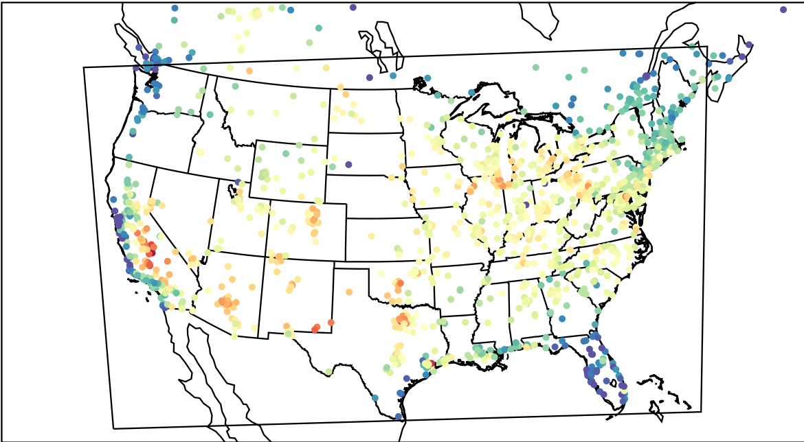
AirNOW (2023-07-23_17:00:00)
