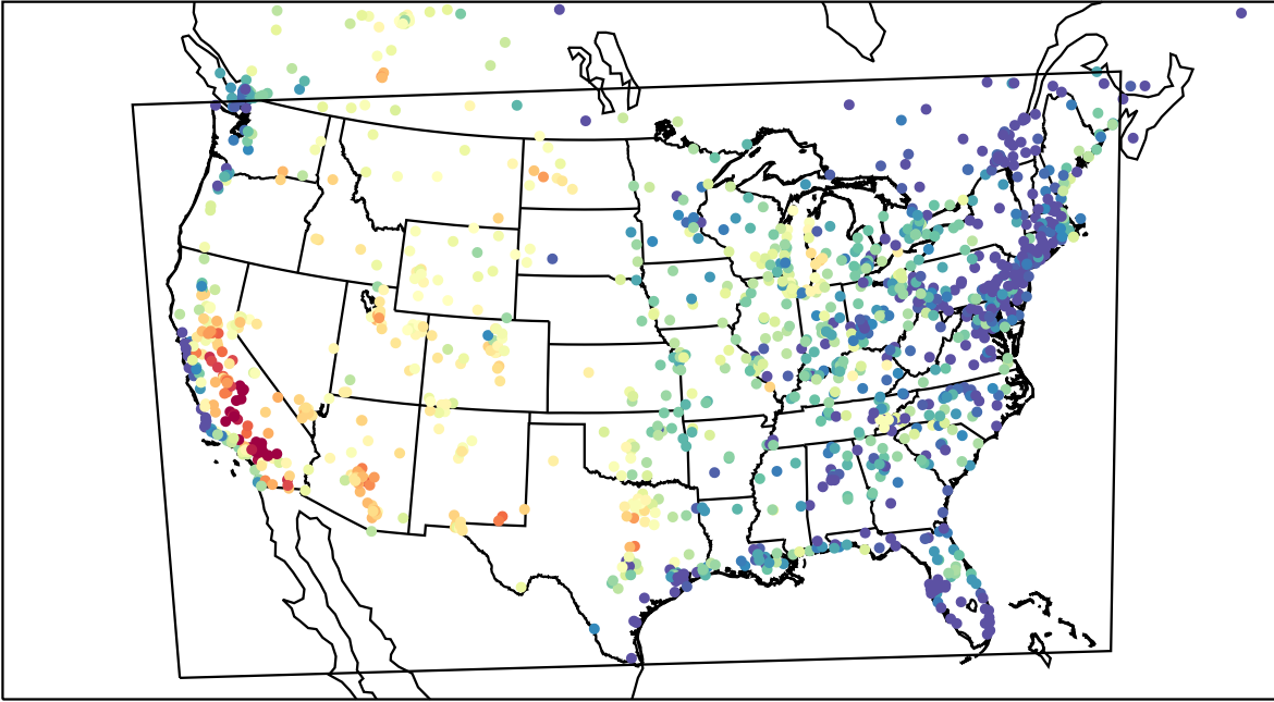
AirNOW (2023-07-23_01:00:00)
