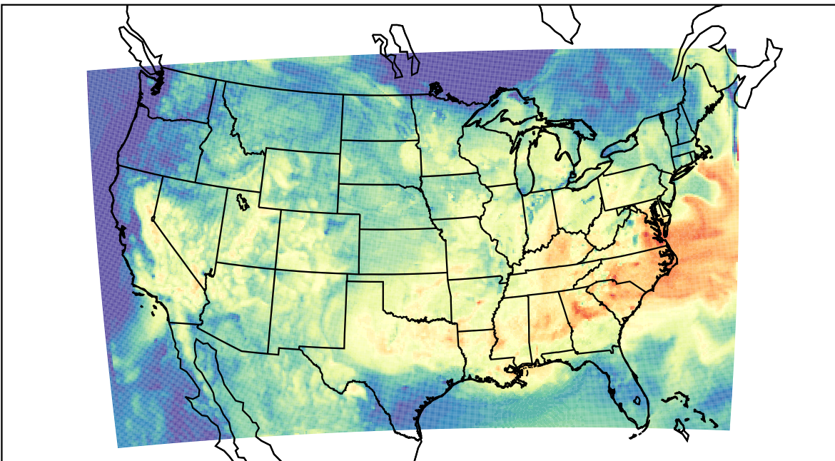
WRF (2023-07-23_15:00:00)
