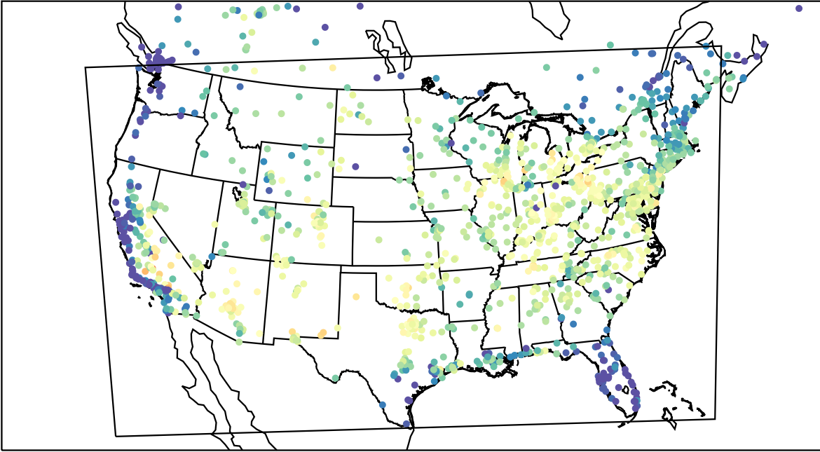
AirNOW (2023-07-23_15:00:00)
