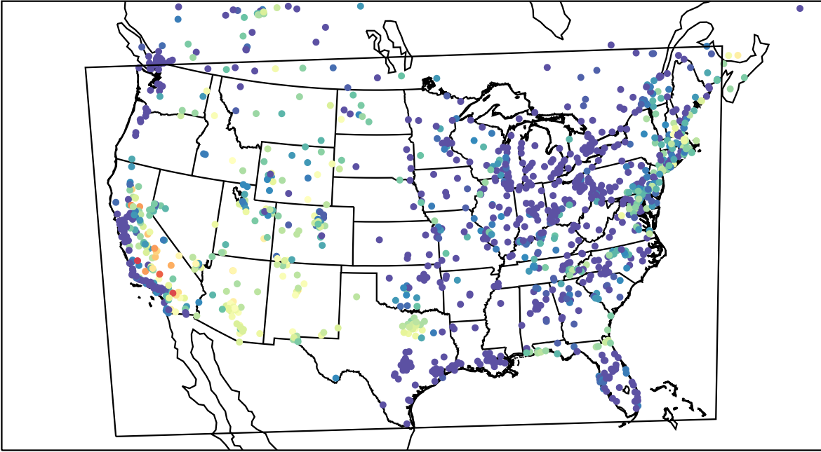
AirNOW (2023-07-22_07:00:00)
