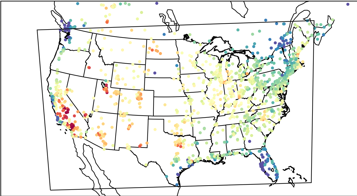
AirNOW (2023-07-22_19:00:00)
