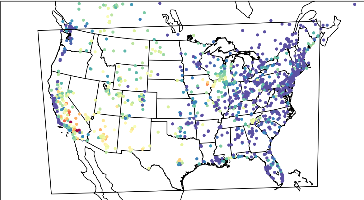
AirNOW (2023-07-23_04:00:00)
