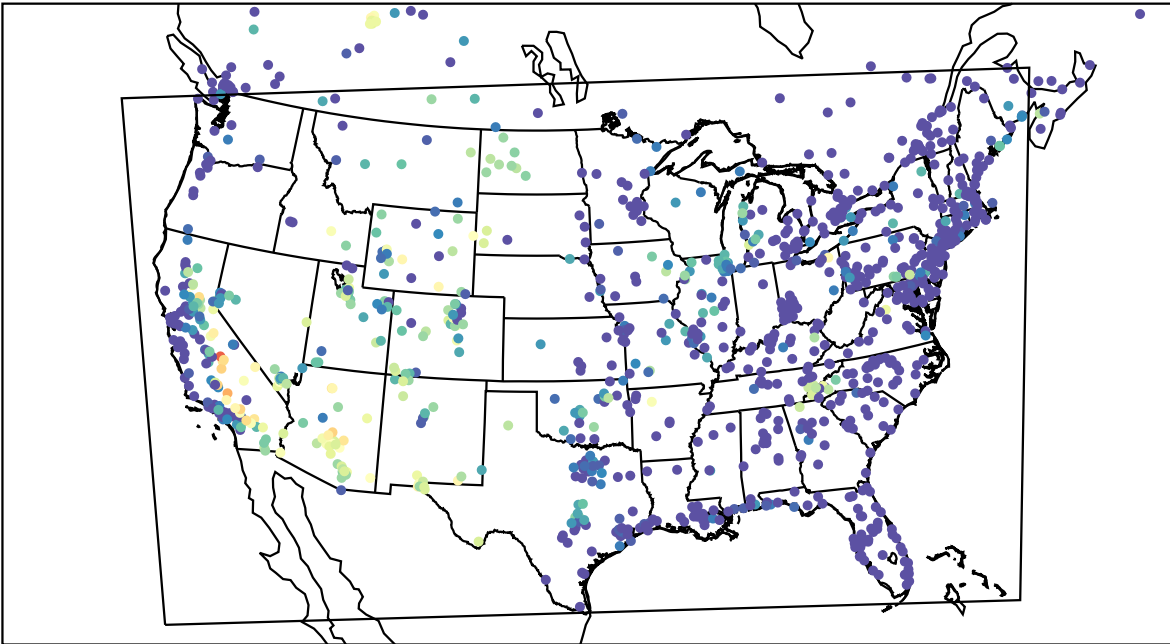
AirNOW (2023-07-23_10:00:00)
