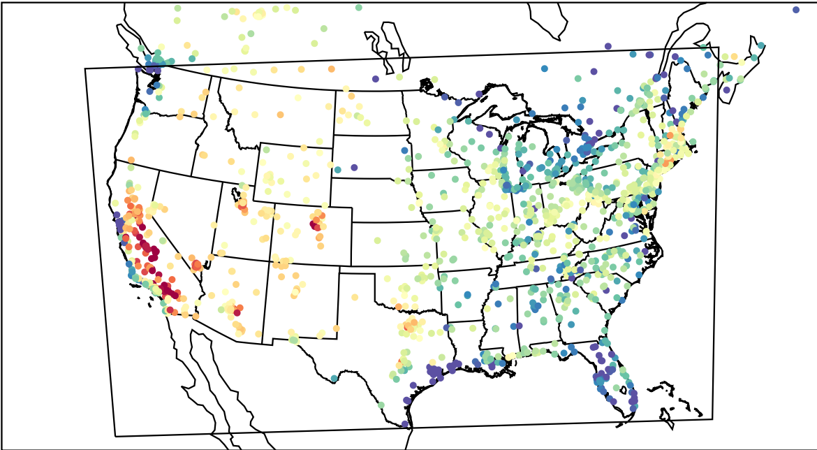
AirNOW (2023-07-22_00:00:00)
