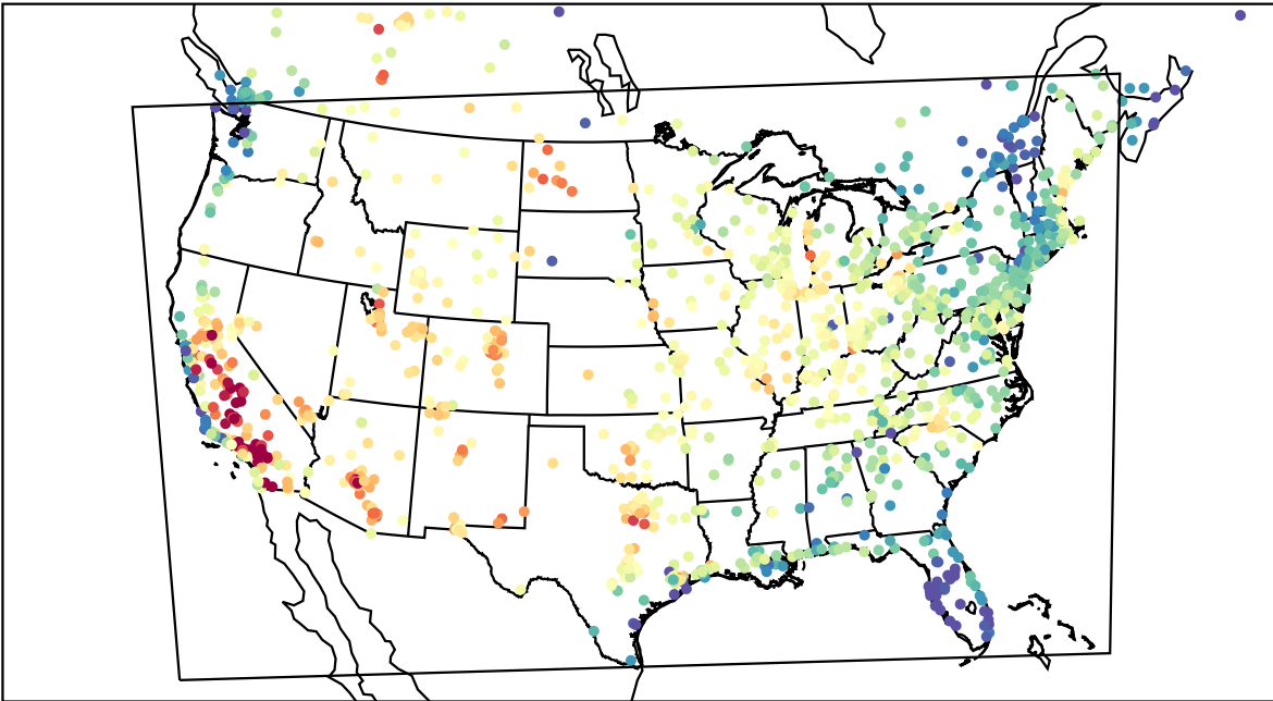
AirNOW (2023-07-22_22:00:00)
