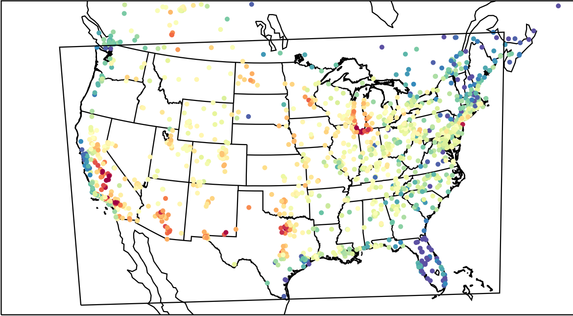
AirNOW (2023-07-23_23:00:00)
