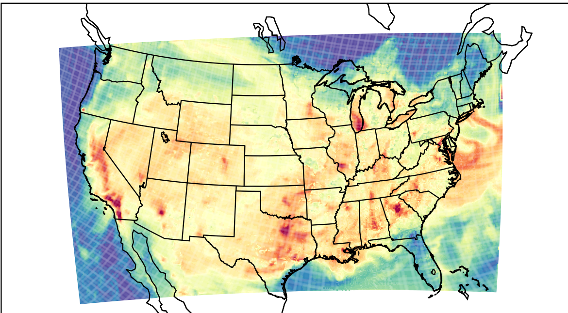
WRF (2023-07-23_23:00:00)
