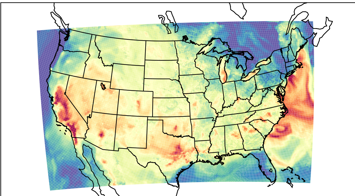
WRF (2023-07-23_00:00:00)
