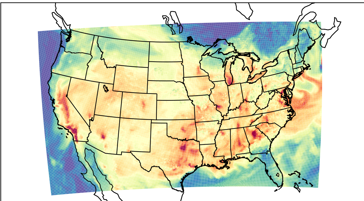
WRF (2023-07-23_22:00:00)
