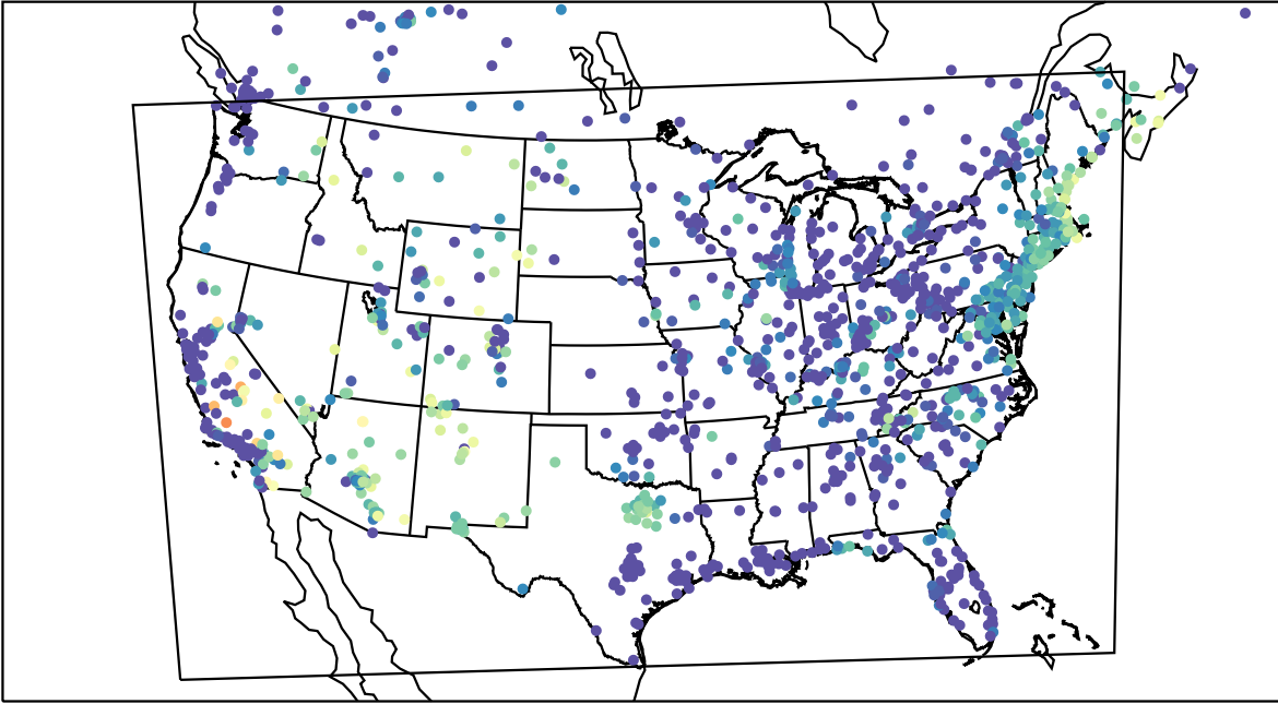
AirNOW (2023-07-22_12:00:00)
