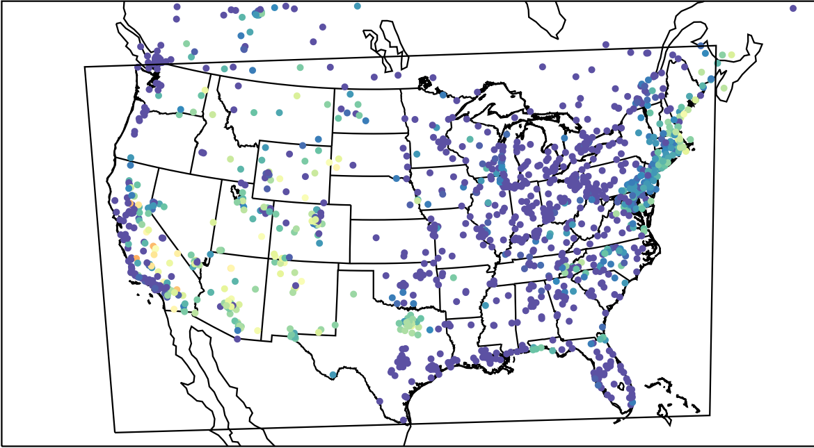
AirNOW (2023-07-22_11:00:00)
