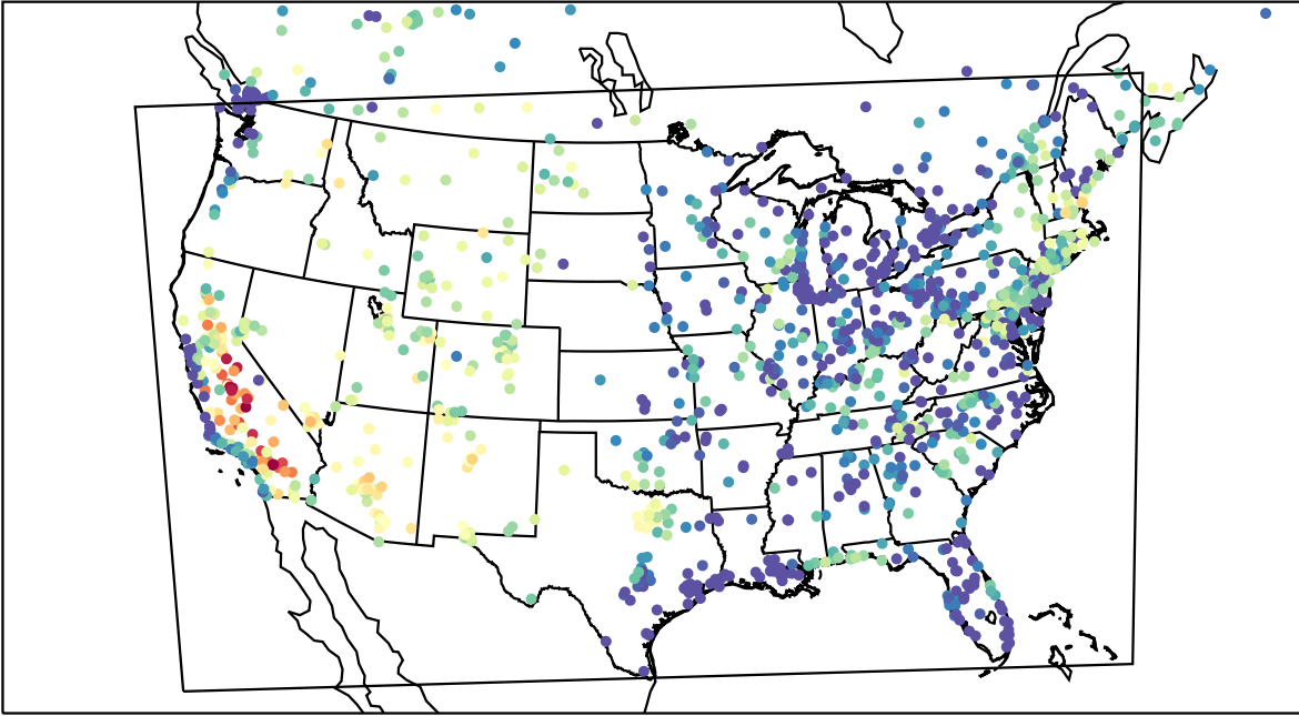
AirNOW (2023-07-22_03:00:00)
