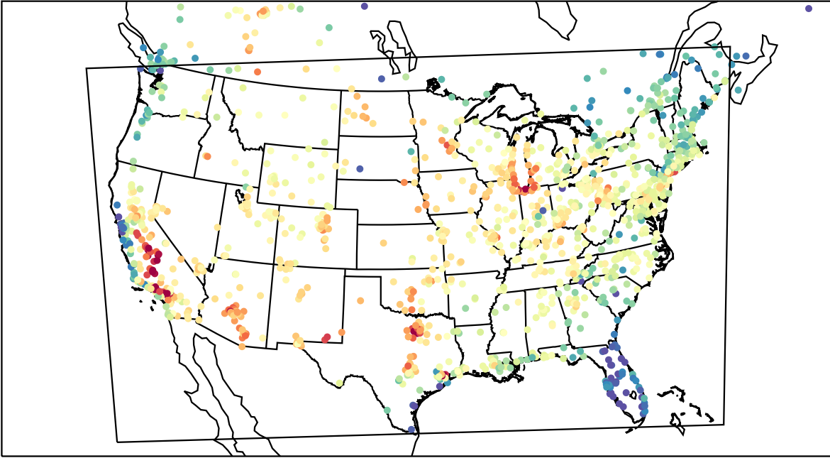
AirNOW (2023-07-23_21:00:00)
