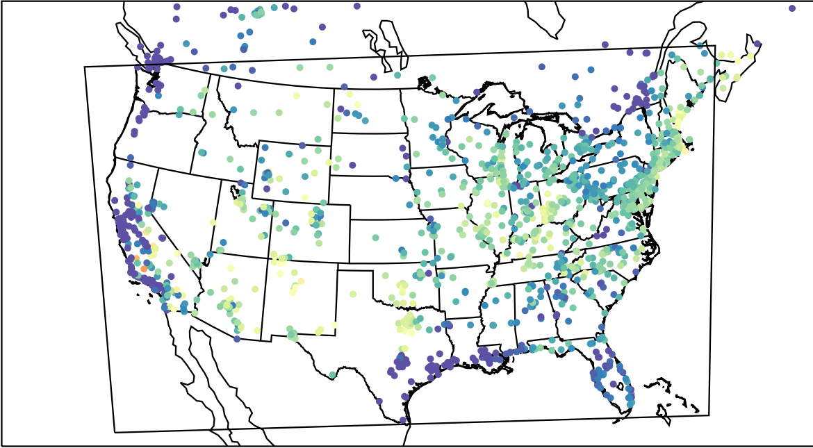
AirNOW (2023-07-22_14:00:00)
