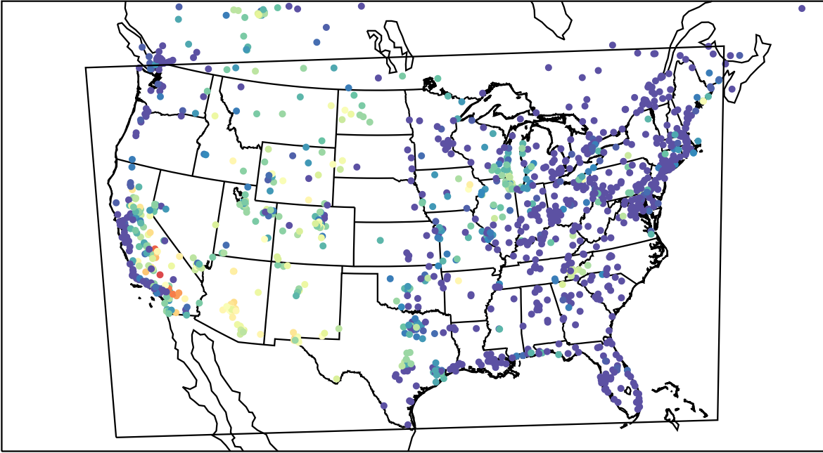
AirNOW (2023-07-23_08:00:00)
