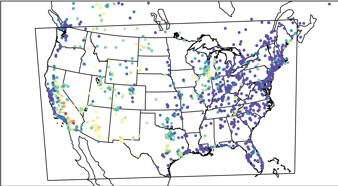
AirNOW (2023-07-23_06:00:00)
