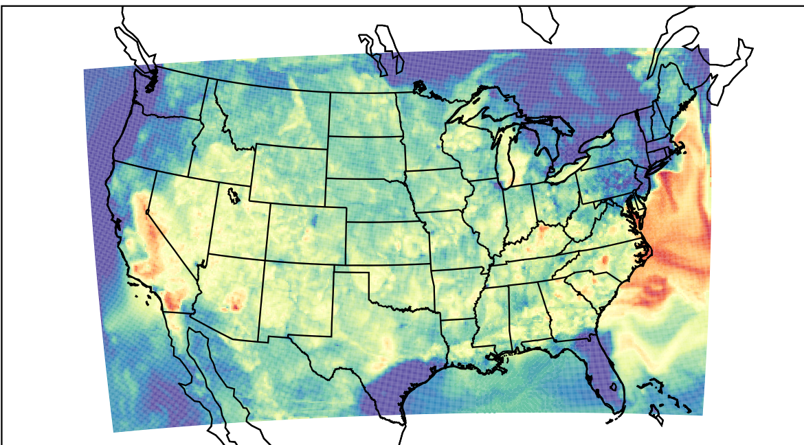
WRF (2023-07-23_05:00:00)
