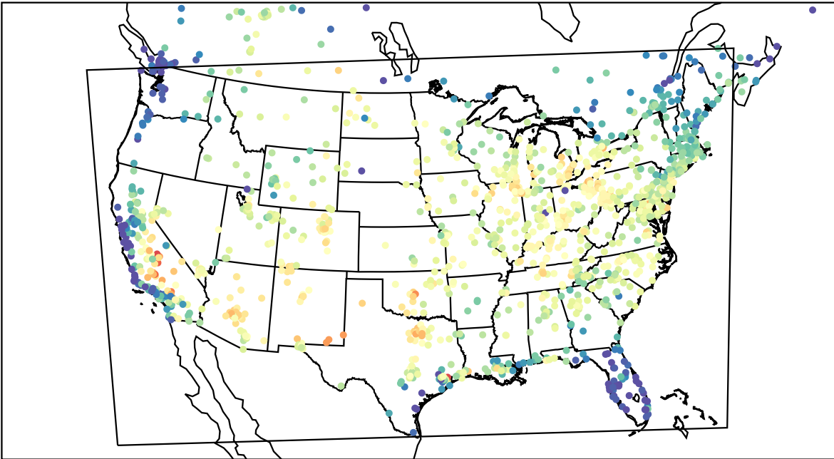
AirNOW (2023-07-23_16:00:00)
