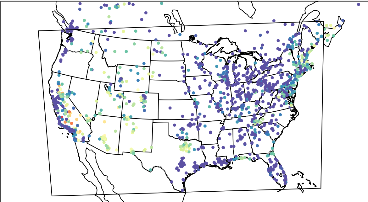
AirNOW (2023-07-22_08:00:00)
