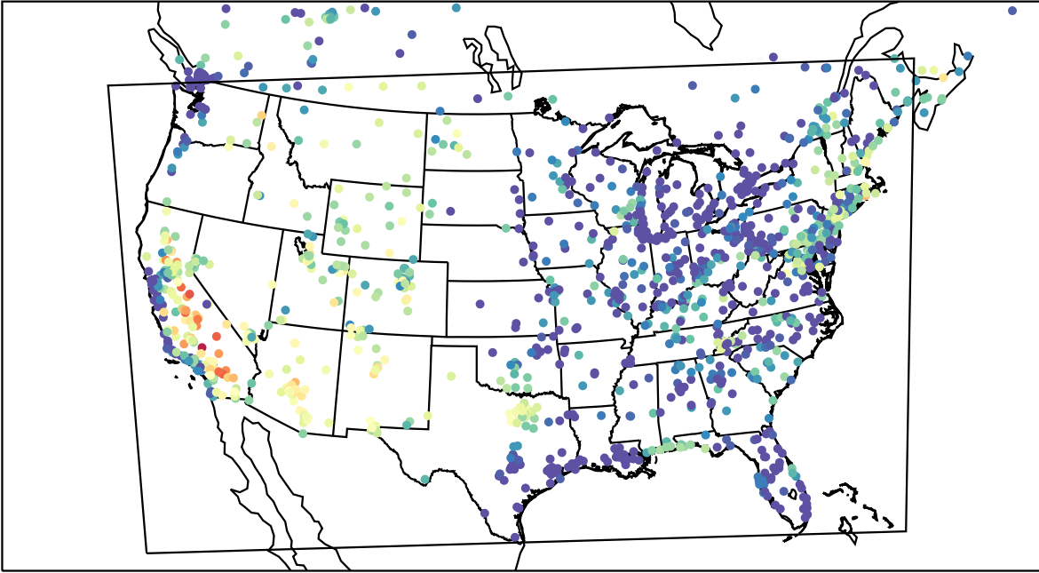
AirNOW (2023-07-22_04:00:00)
