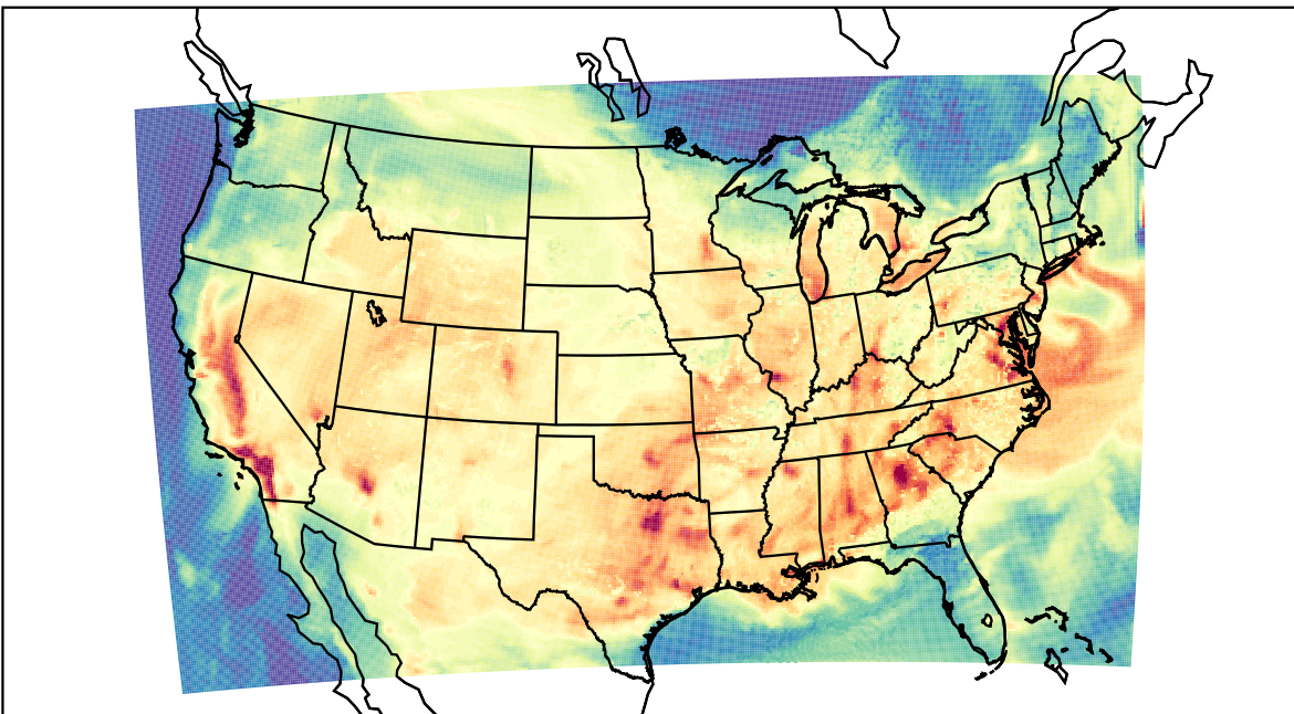
WRF (2023-07-23_21:00:00)
