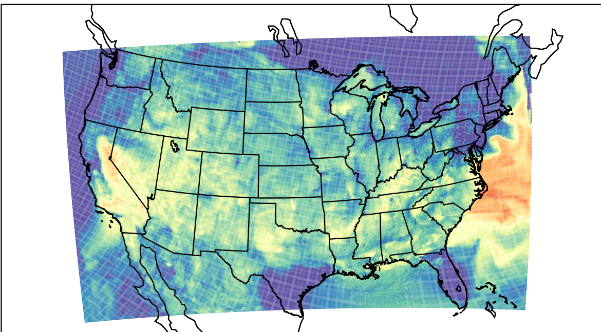
WRF (2023-07-23_11:00:00)
