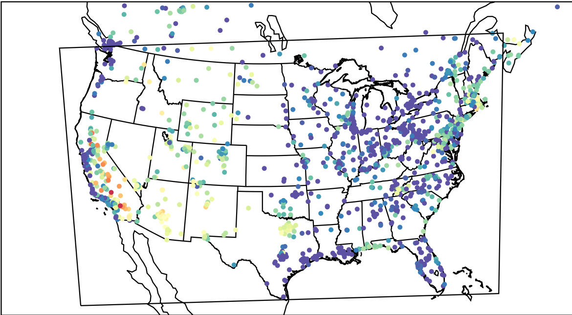
AirNOW (2023-07-22_05:00:00)
