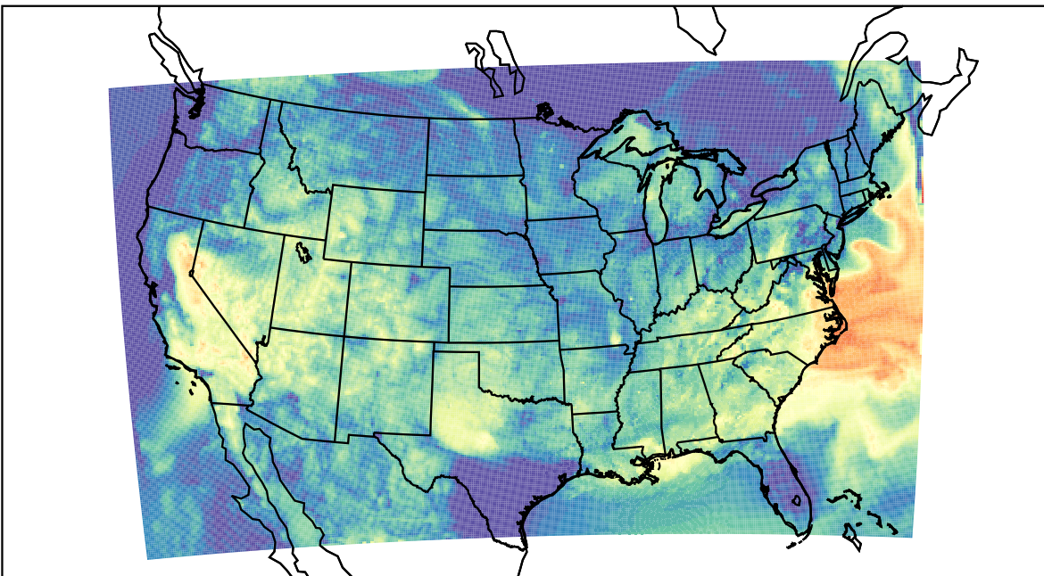
WRF (2023-07-23_13:00:00)
