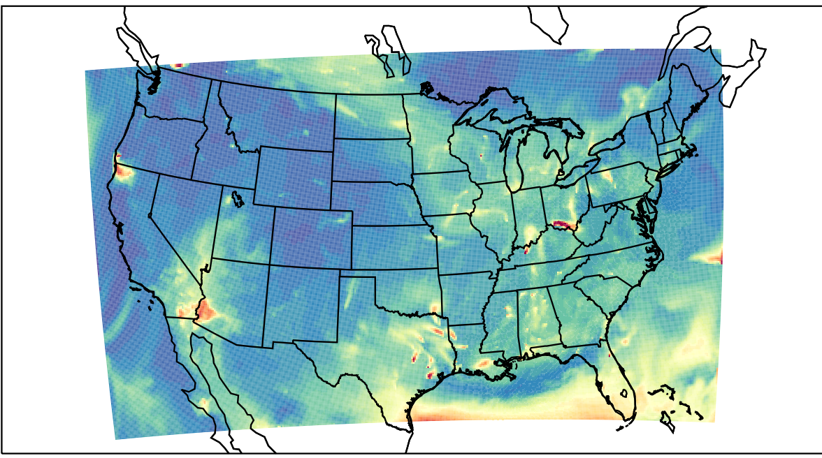
WRF 2023-07-24_09:00:00
