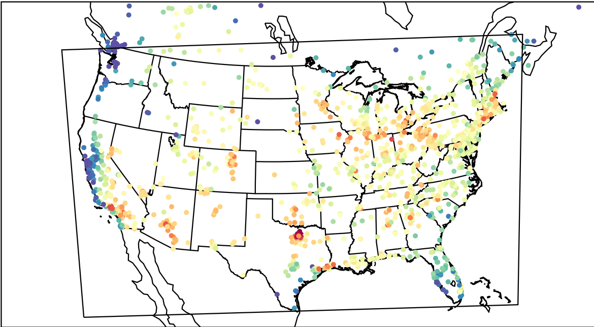
AirNOW (2023-07-24_17:00:00)
