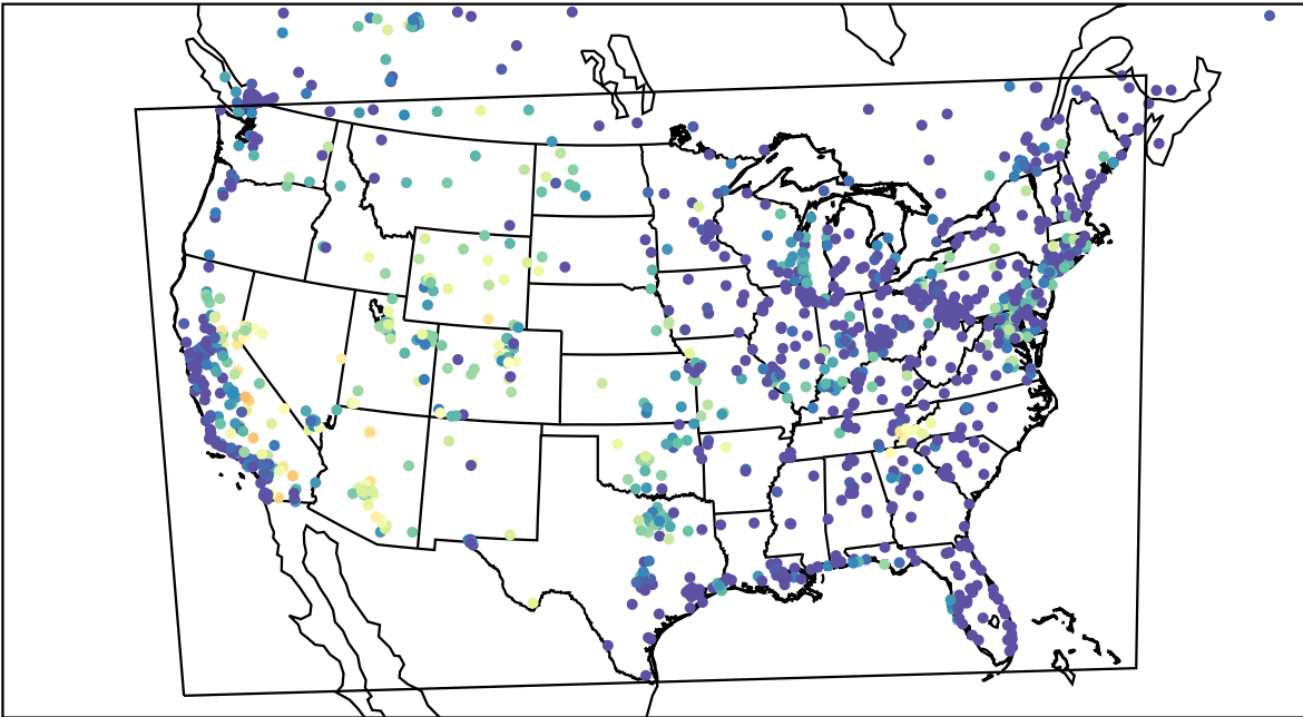
AirNOW (2023-07-24_08:00:00)
