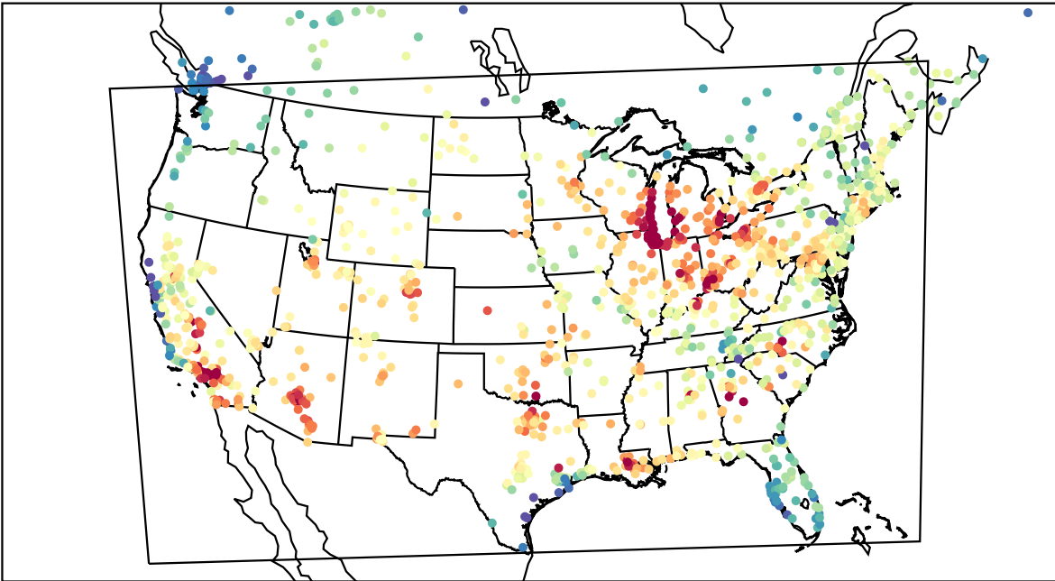
AirNOW (2023-07-25_22:00:00)
