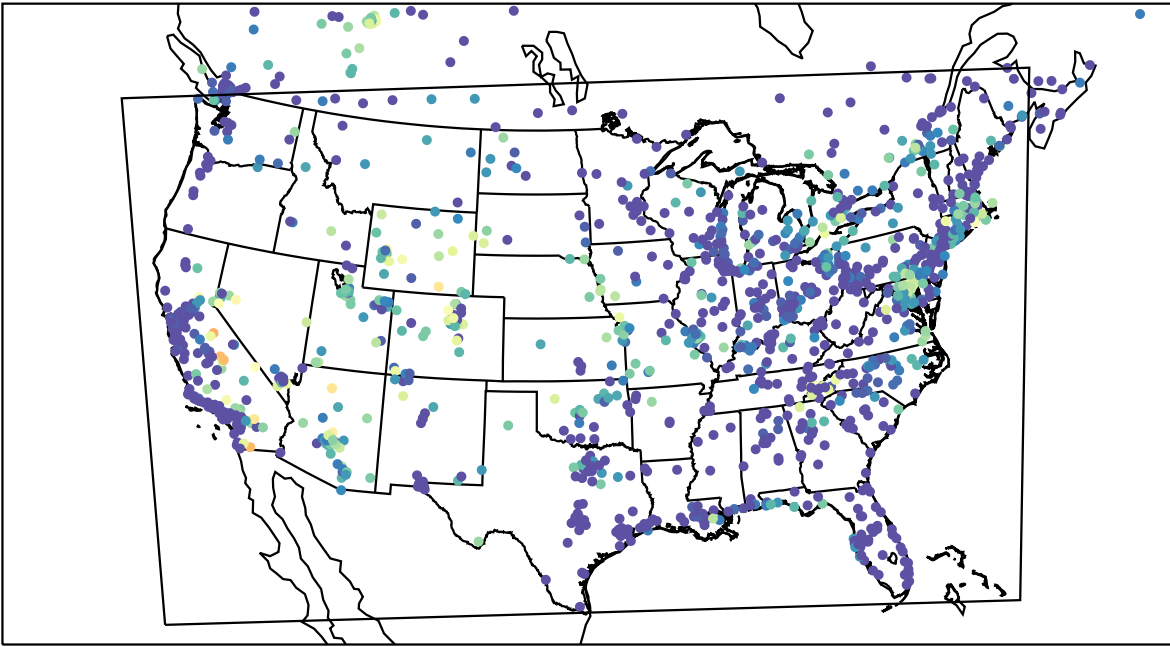
AirNOW (2023-07-24_12:00:00)
