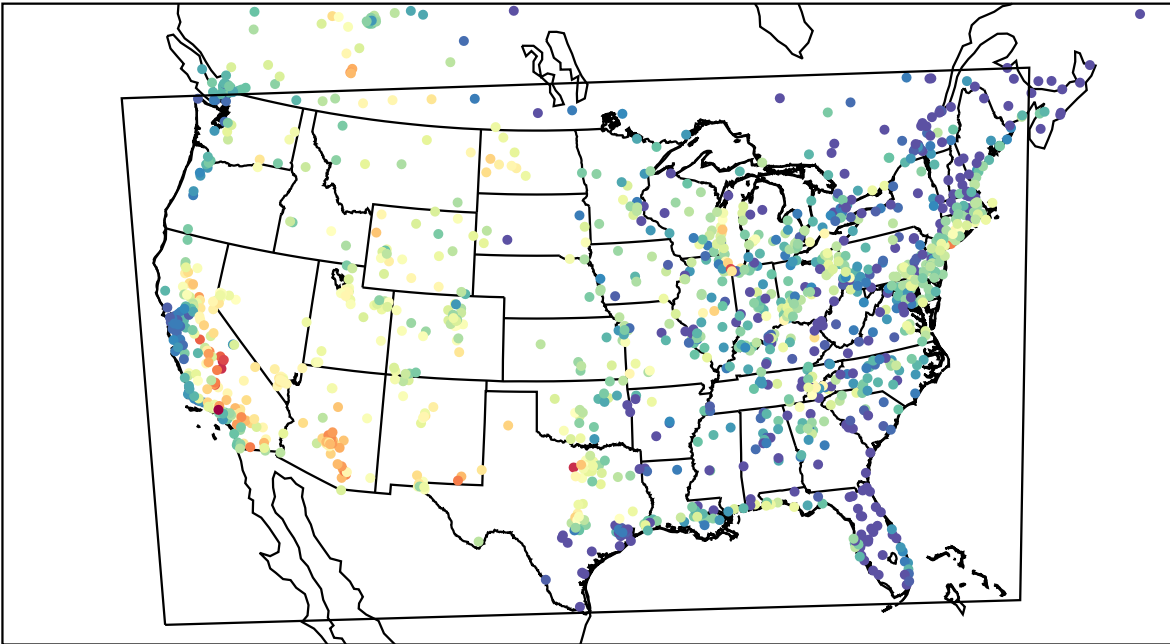
AirNOW (2023-07-24_02:00:00)
