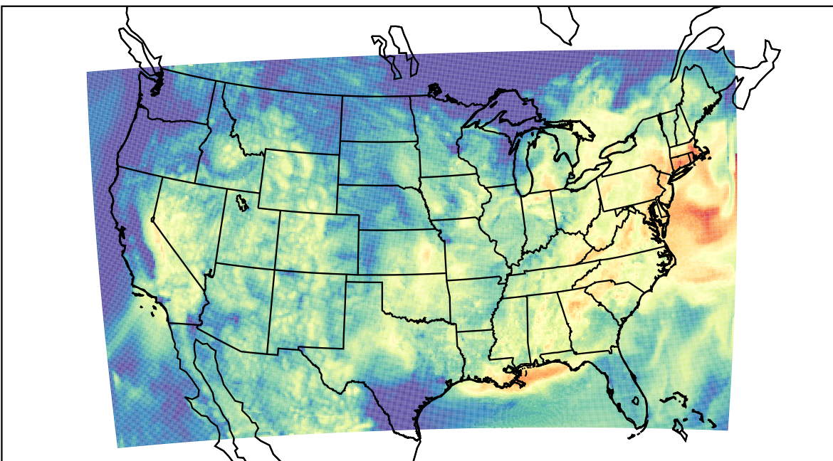
WRF (2023-07-24_14:00:00)
