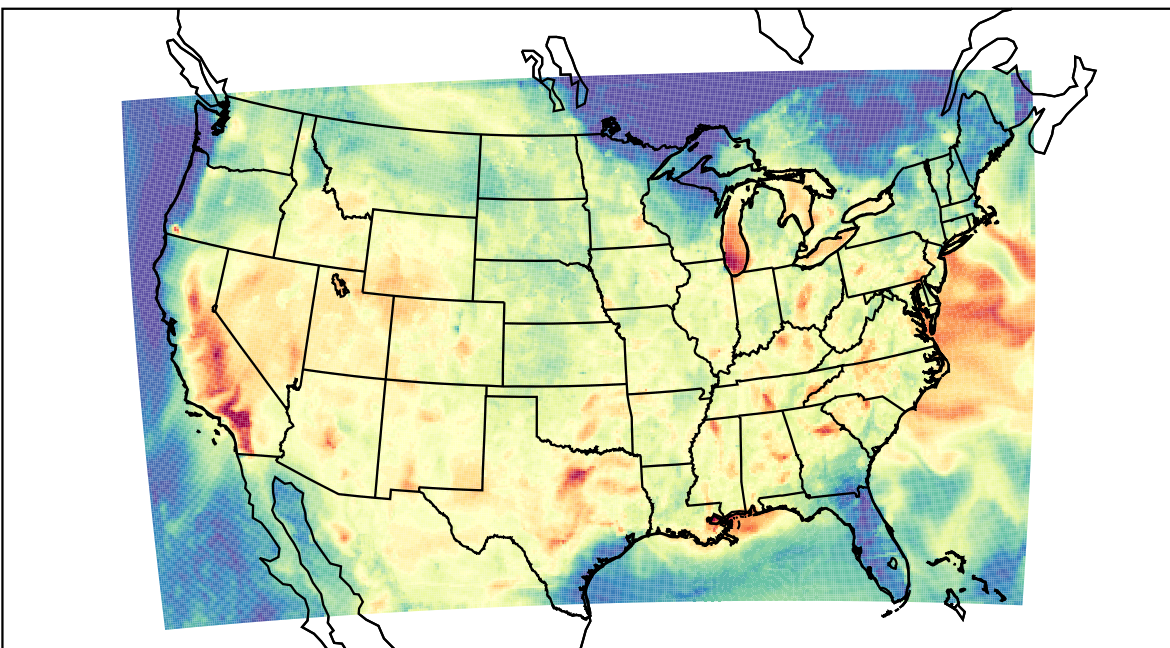
WRF (2023-07-24_01:00:00)
