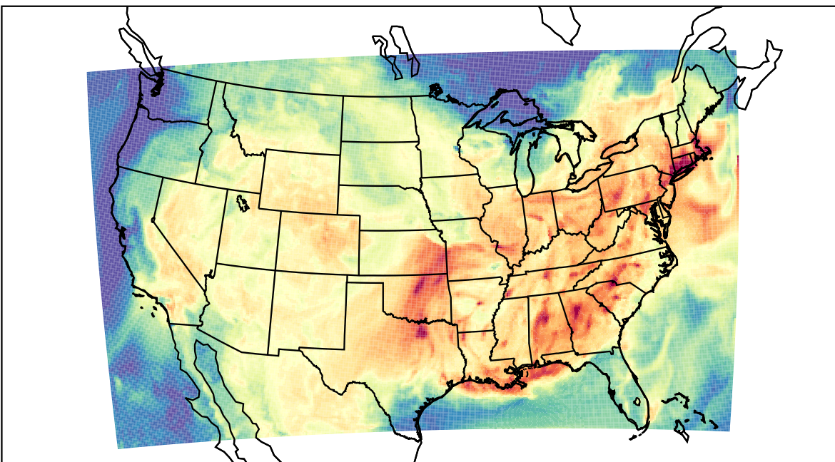
WRF (2023-07-24_17:00:00)
