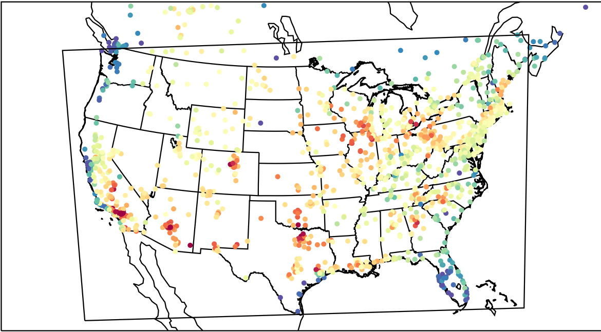
AirNOW (2023-07-24_22:00:00)
