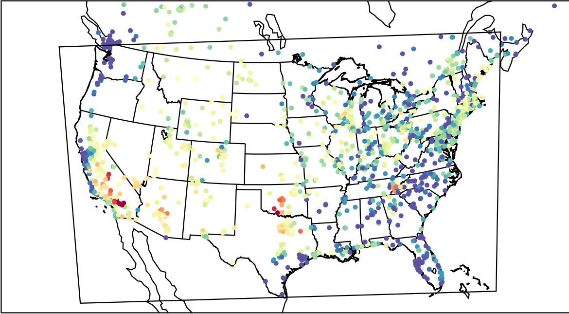
AirNOW (2023-07-25_02:00:00)
