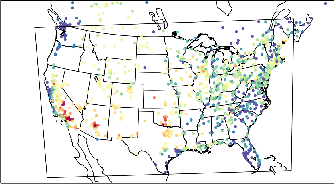
AirNOW (2023-07-25_01:00:00)
