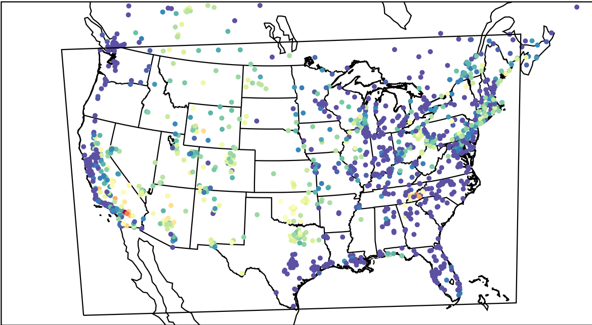
AirNOW (2023-07-25_07:00:00)
