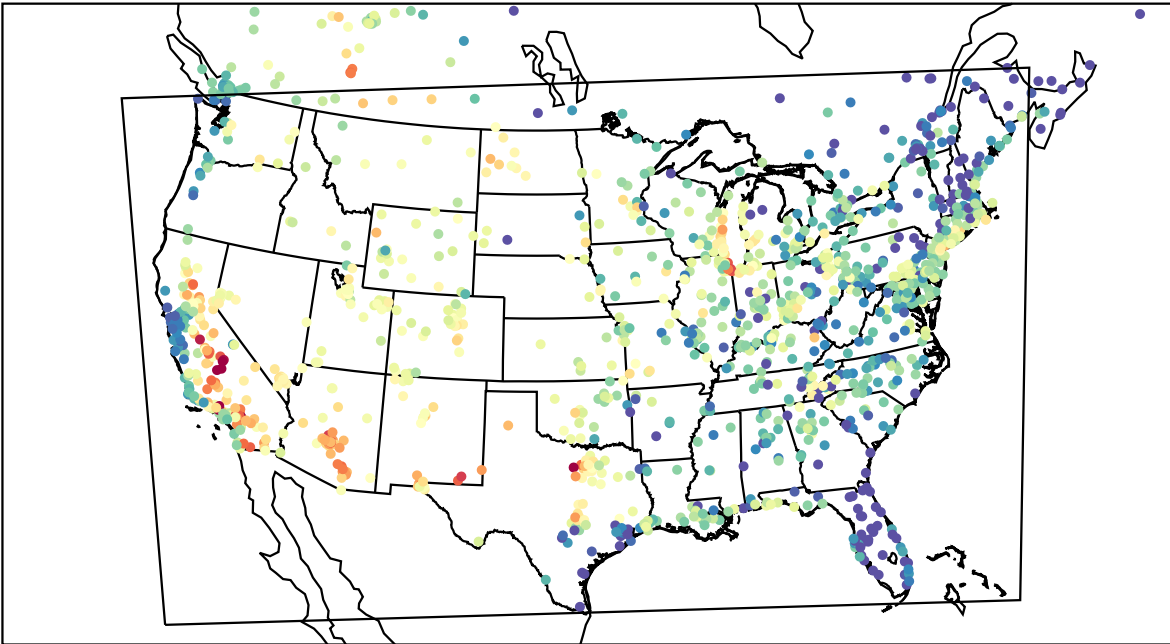
AirNOW (2023-07-24_01:00:00)
