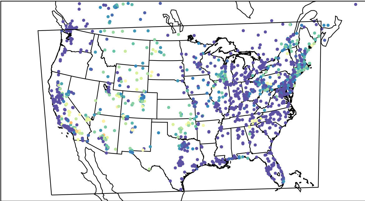
AirNOW (2023-07-25_11:00:00)
