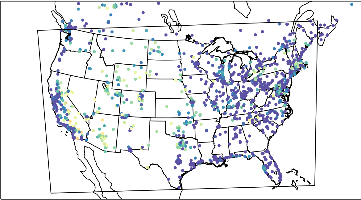
AirNOW (2023-07-24_09:00:00)
