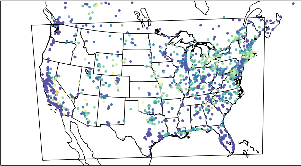
AirNOW (2023-07-24_13:00:00)
