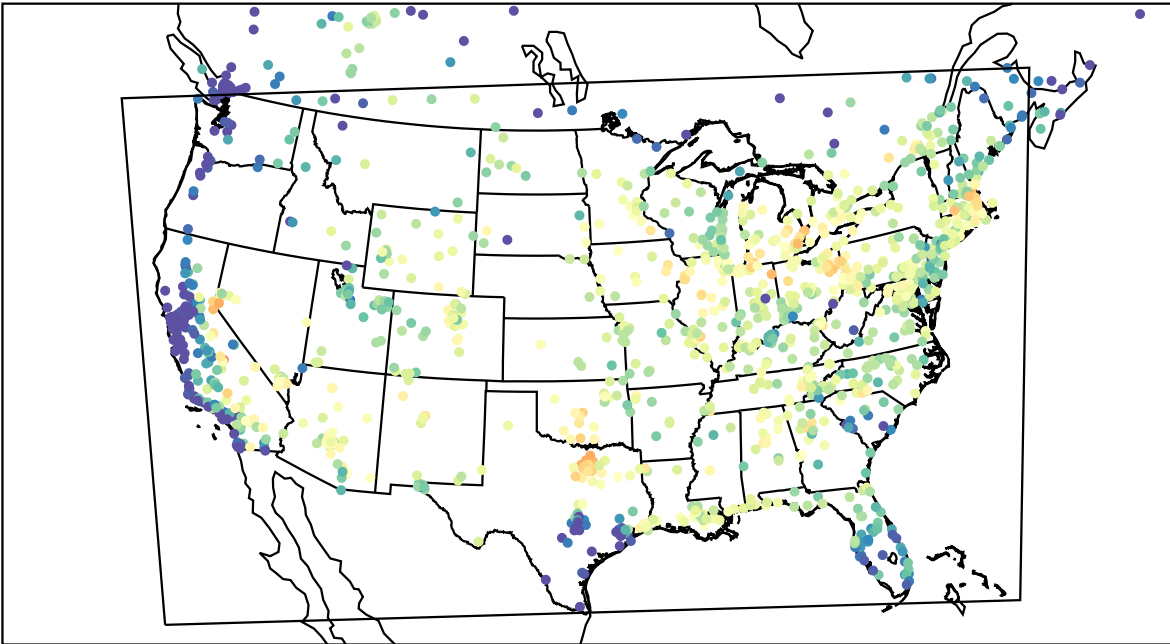
AirNOW (2023-07-24_15:00:00)
