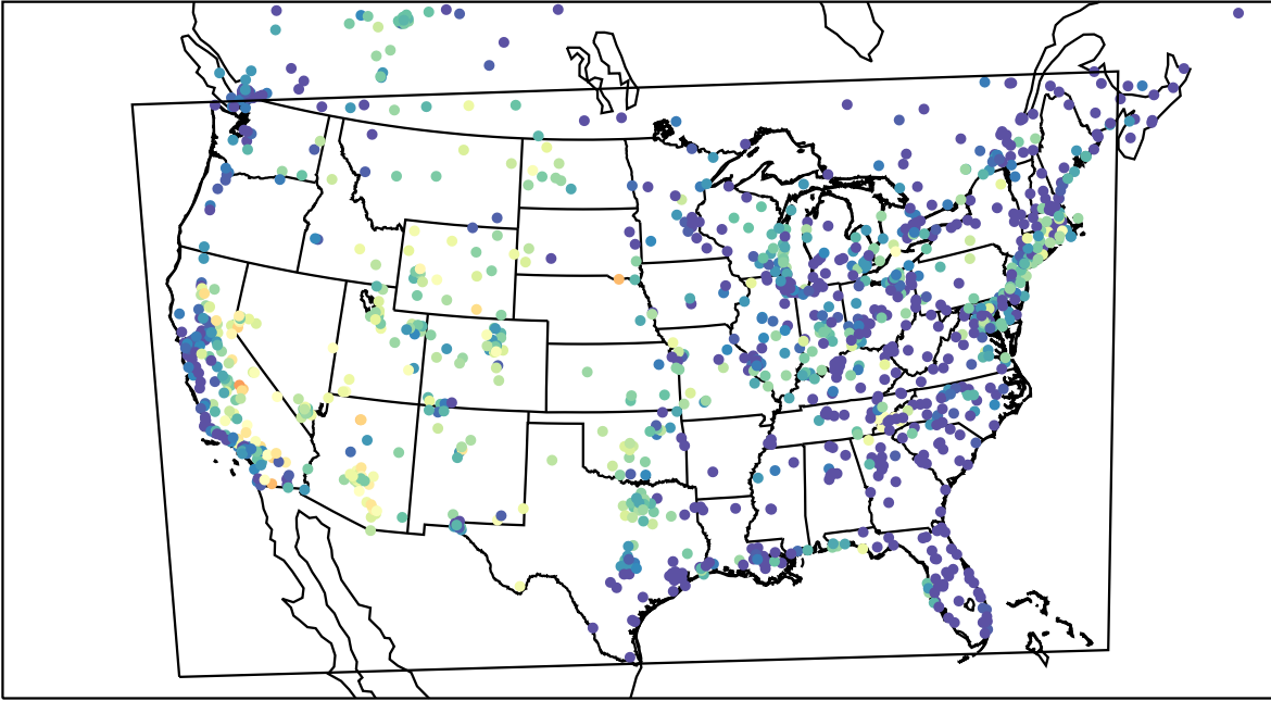
AirNOW (2023-07-24_06:00:00)
