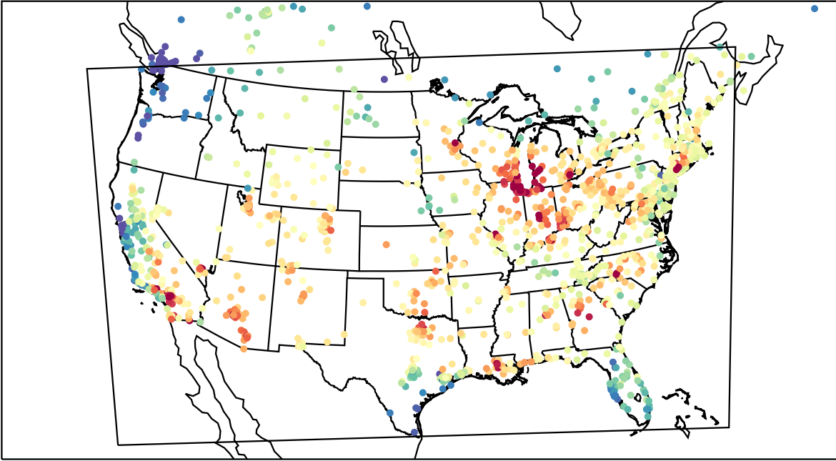
AirNOW (2023-07-25_18:00:00)
