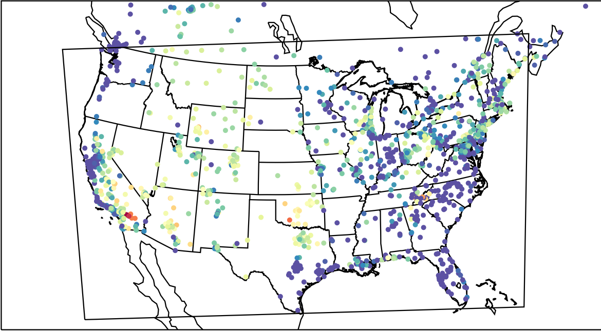
AirNOW (2023-07-25_05:00:00)
