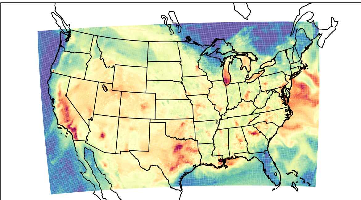
WRF (2023-07-24_00:00:00)
