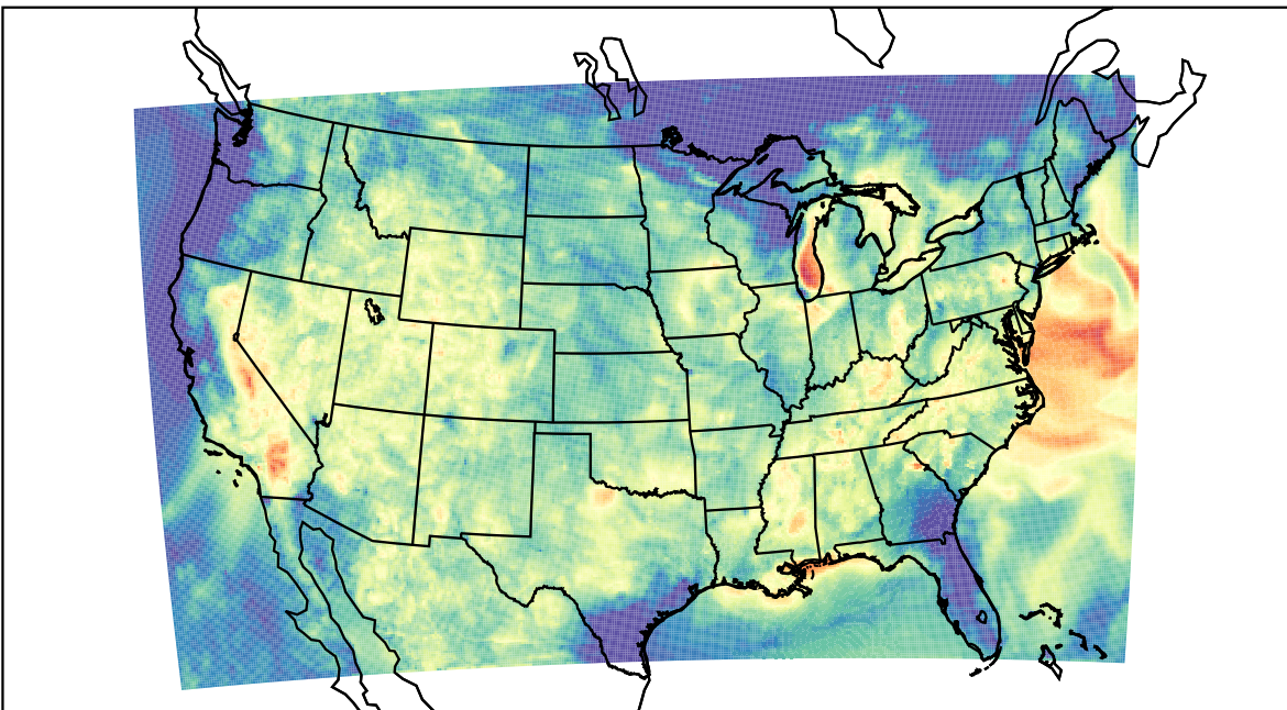
WRF (2023-07-24_06:00:00)
