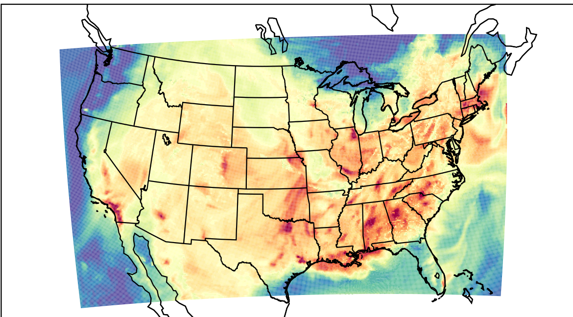
WRF (2023-07-24_22:00:00)
