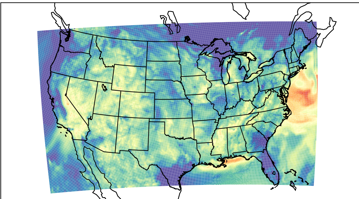
WRF (2023-07-24_11:00:00)
