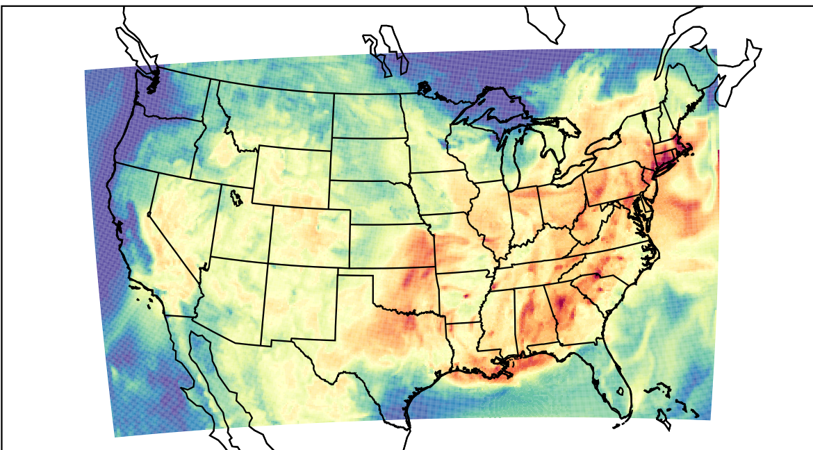
WRF (2023-07-24_16:00:00)
