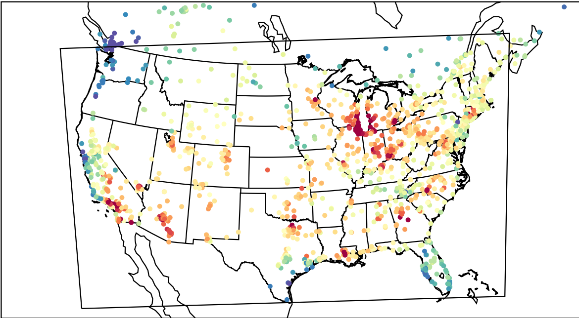
AirNOW (2023-07-25_19:00:00)
