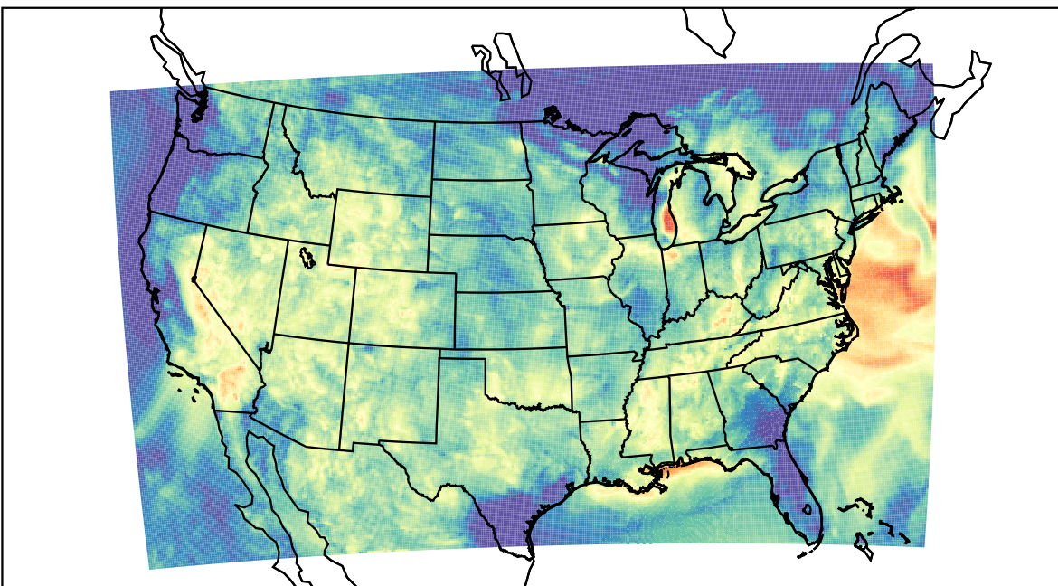
WRF (2023-07-24_08:00:00)
