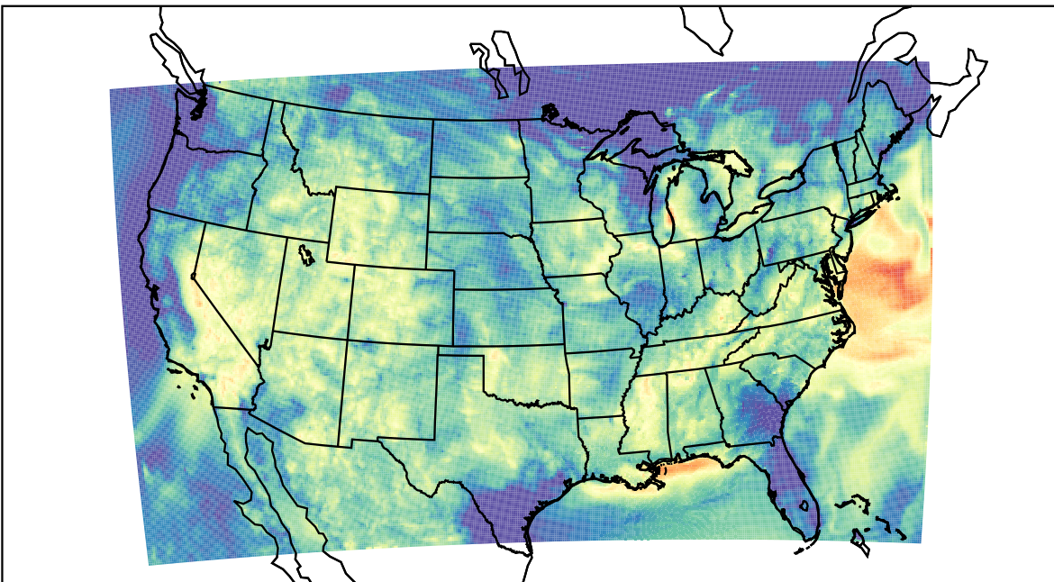
WRF (2023-07-24_10:00:00)
