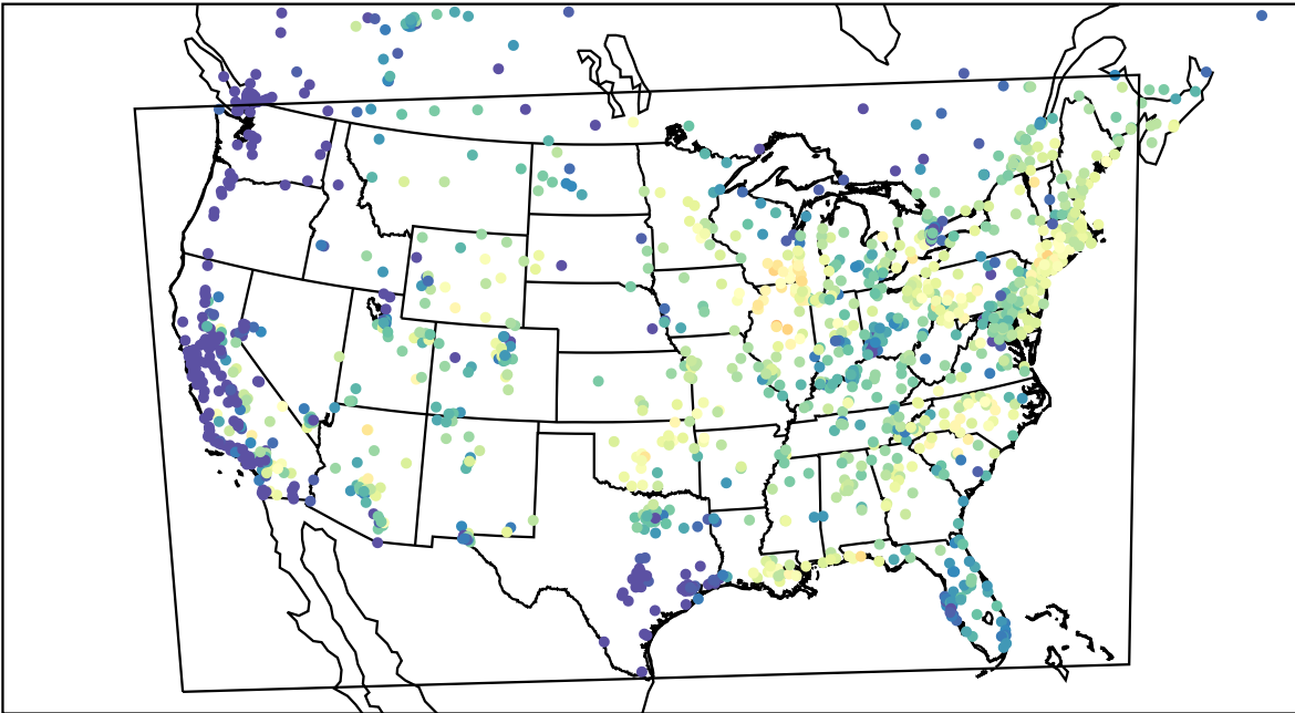
AirNOW (2023-07-25_14:00:00)
