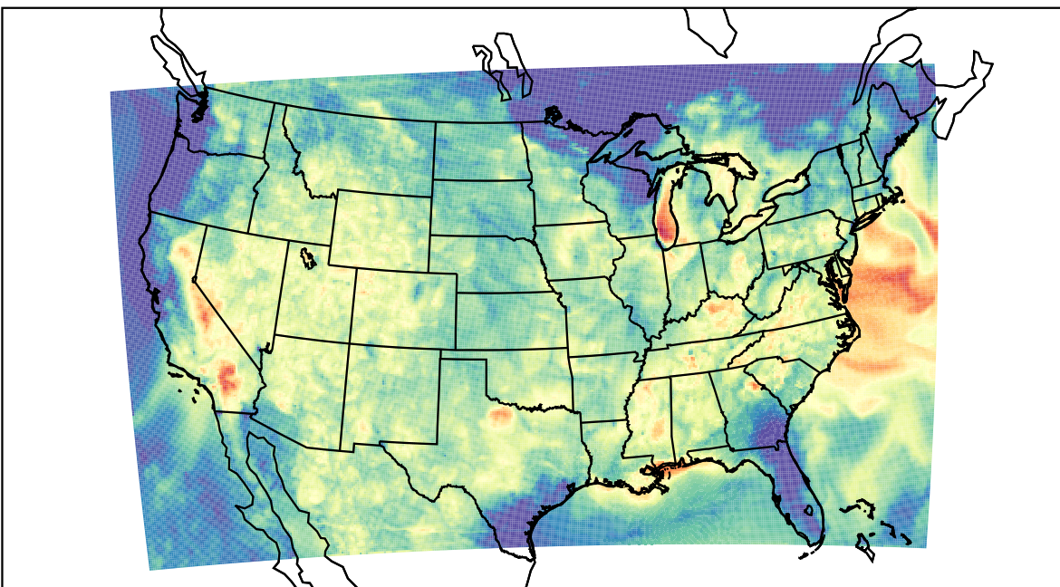
WRF (2023-07-24_05:00:00)
