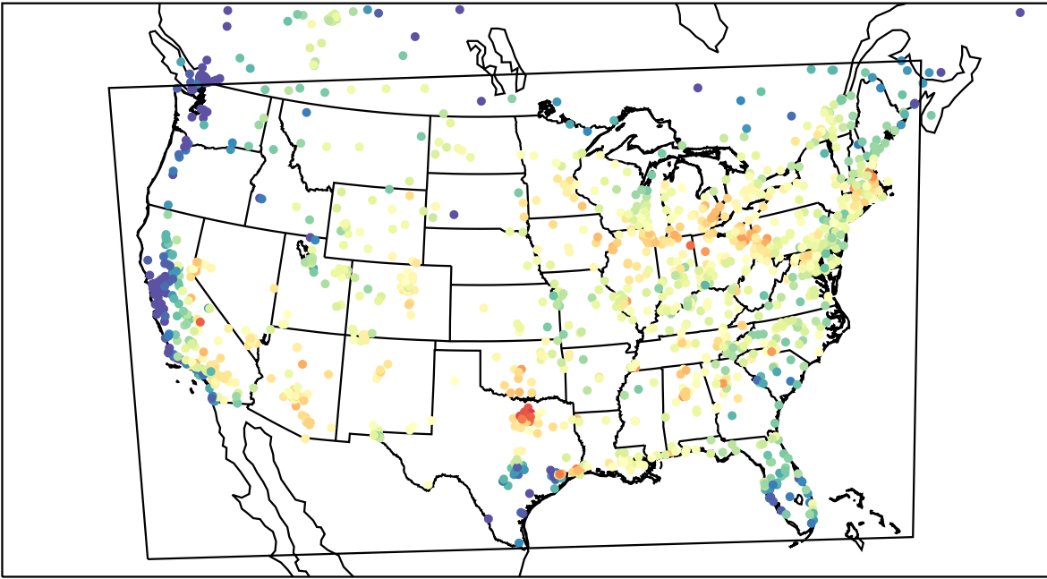
AirNOW (2023-07-24_16:00:00)
