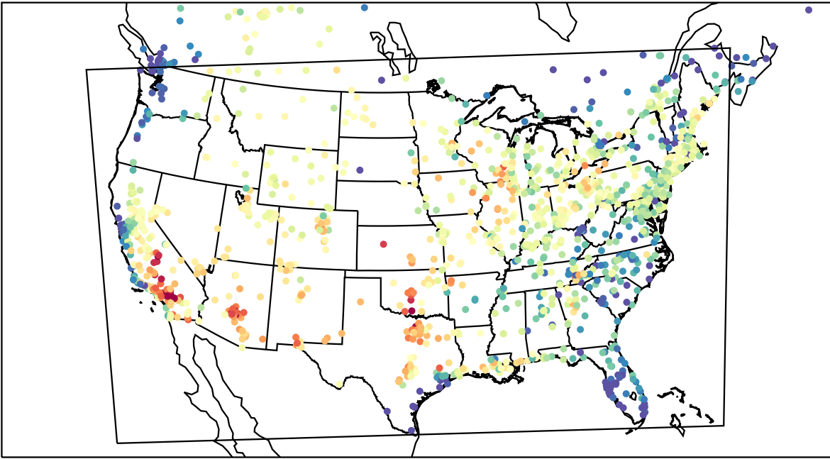
AirNOW (2023-07-25_00:00:00)
