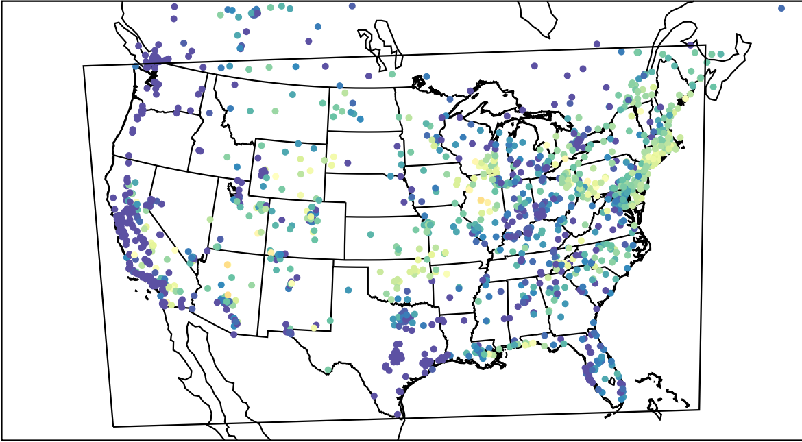
AirNOW (2023-07-25_13:00:00)
