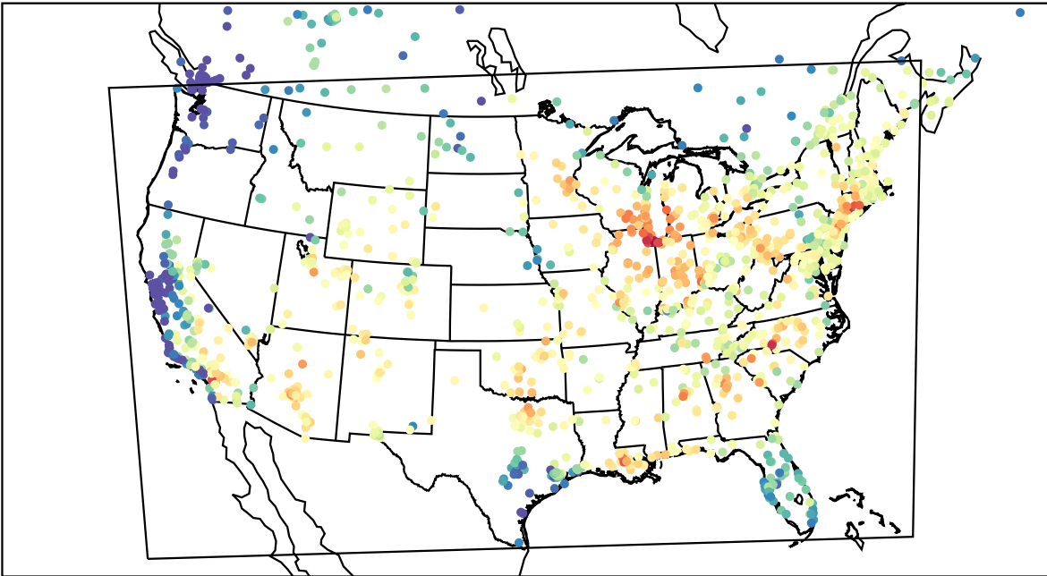
AirNOW (2023-07-25_16:00:00)
