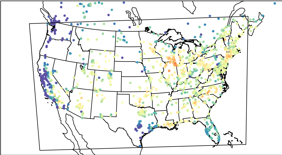
AirNOW (2023-07-25_15:00:00)
