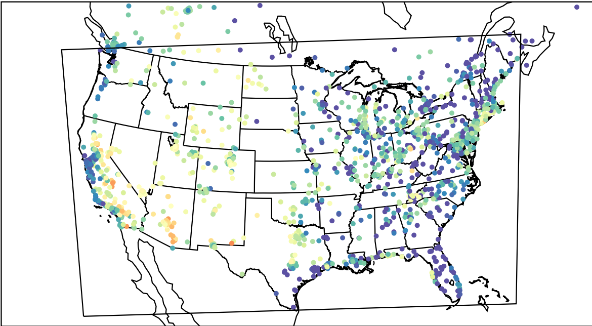
AirNOW (2023-07-24_03:00:00)
