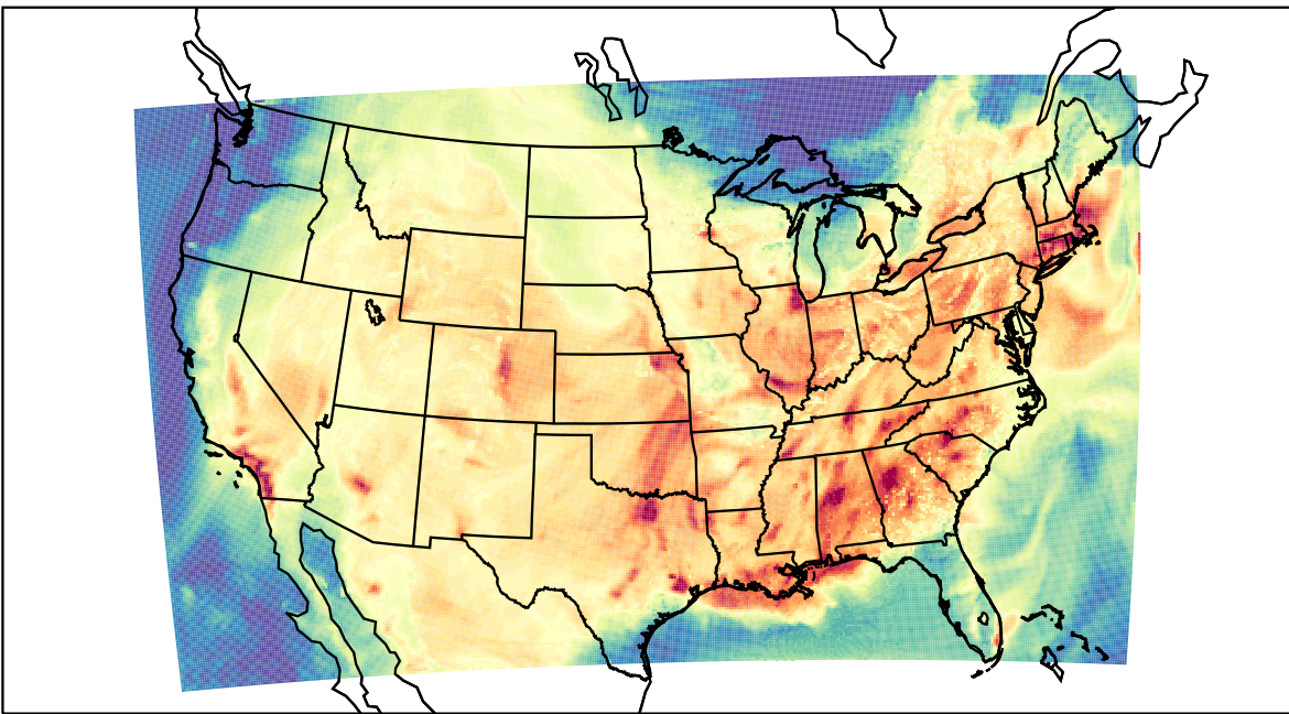
WRF (2023-07-24_21:00:00)
