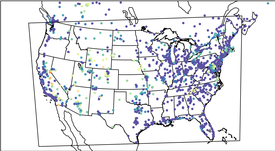
AirNOW (2023-07-24_11:00:00)
