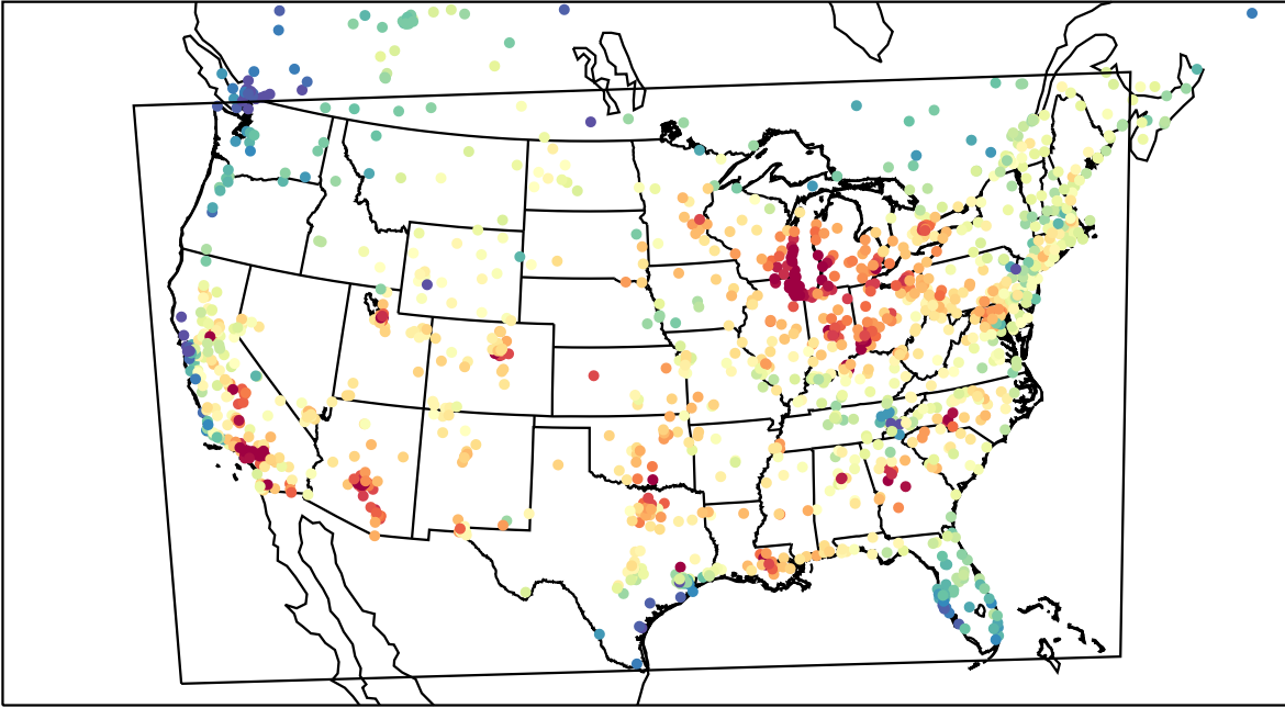
AirNOW (2023-07-25_21:00:00)
