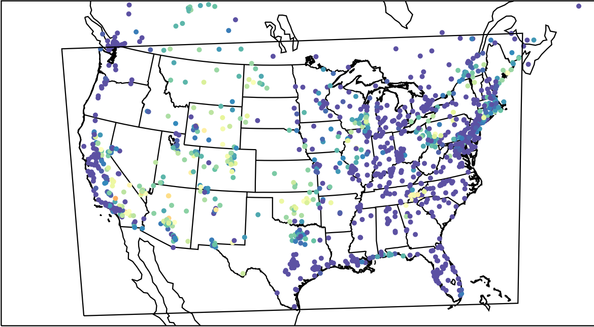
AirNOW (2023-07-25_10:00:00)
