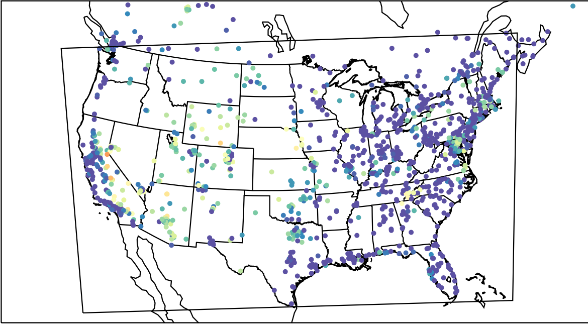
AirNOW (2023-07-24_10:00:00)
