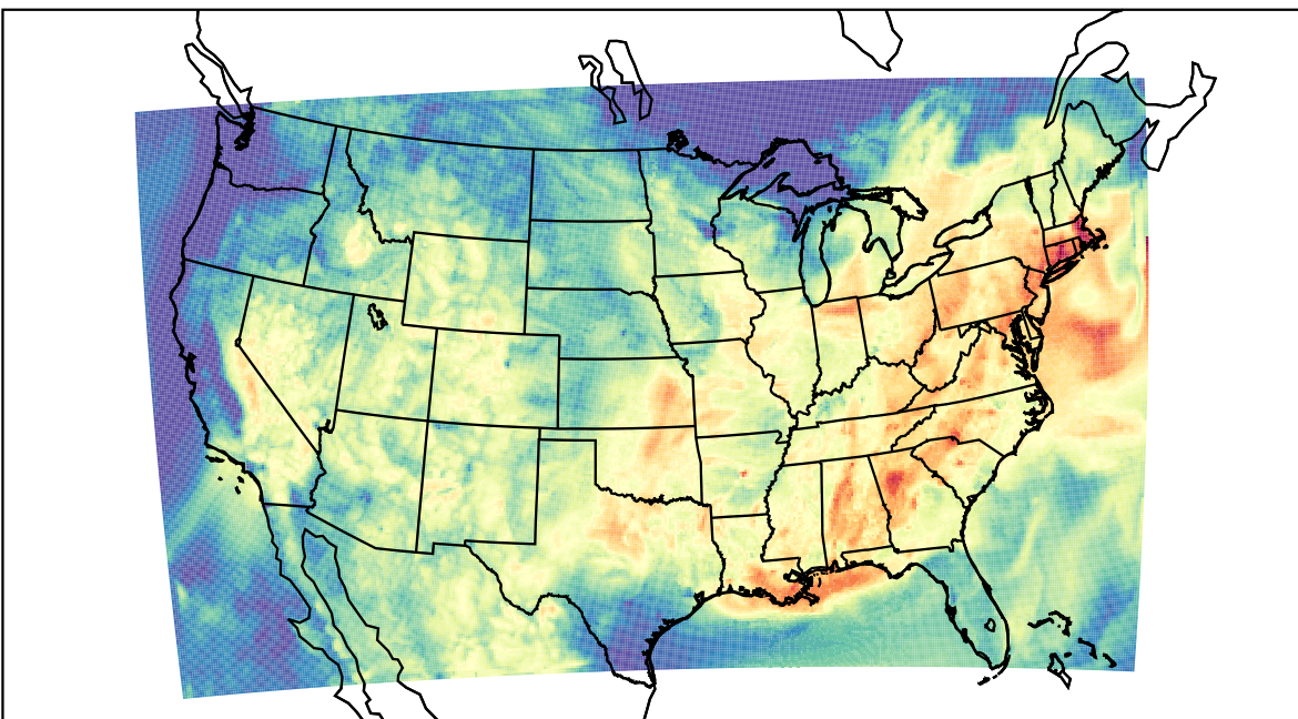
WRF (2023-07-24_15:00:00)
