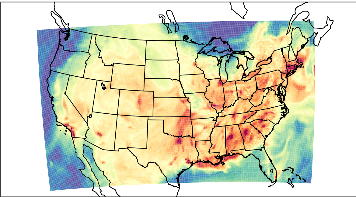
WRF (2023-07-24_20:00:00)
