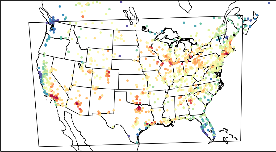
AirNOW (2023-07-24_19:00:00)
