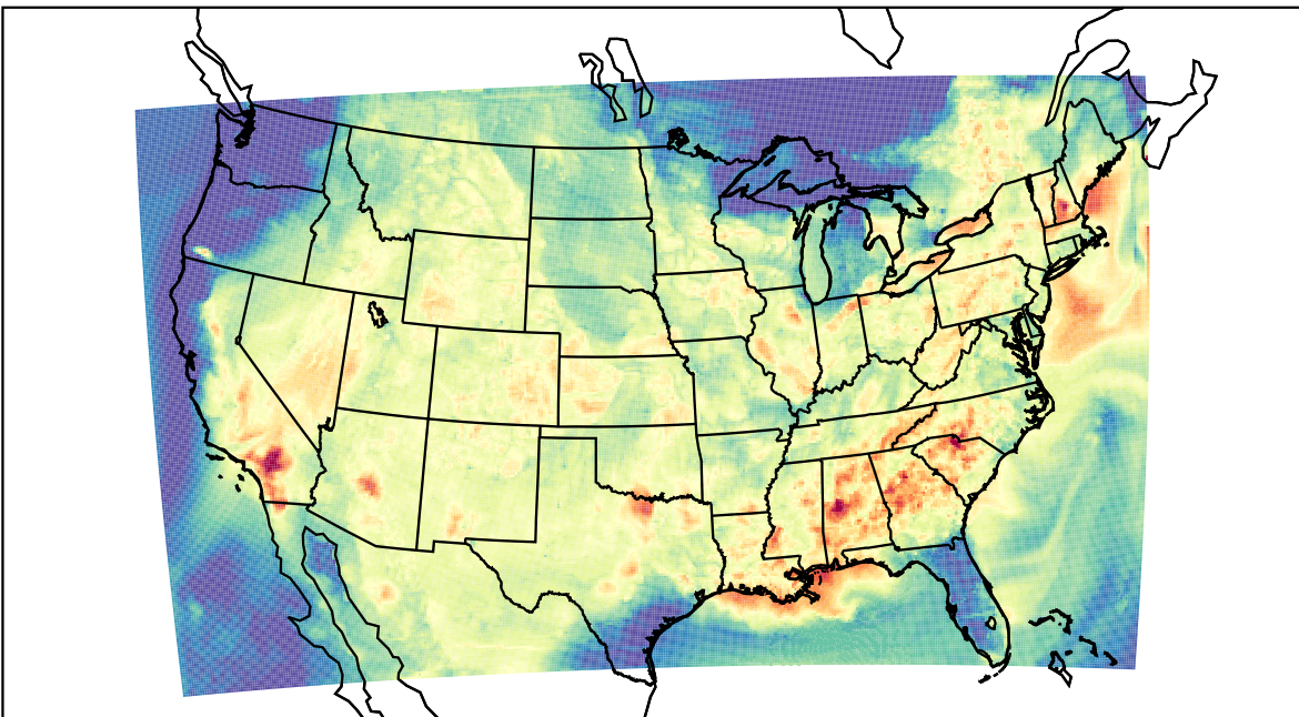
WRF (2023-07-25_02:00:00)
