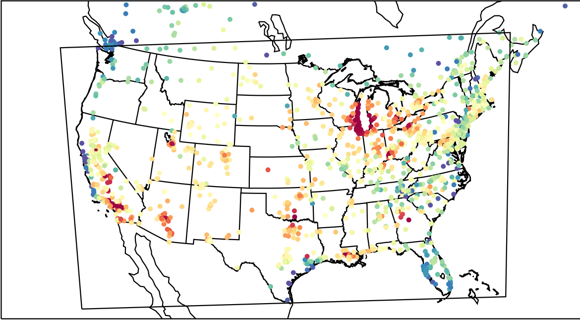
AirNOW (2023-07-25_23:00:00)
