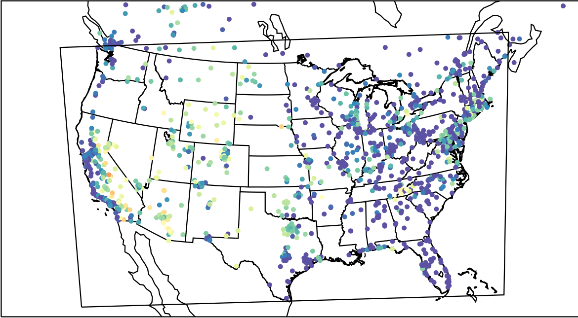
AirNOW (2023-07-24_07:00:00)
