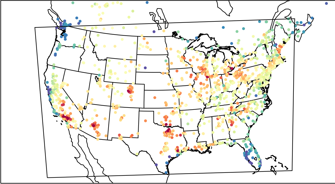
AirNOW (2023-07-24_21:00:00)
