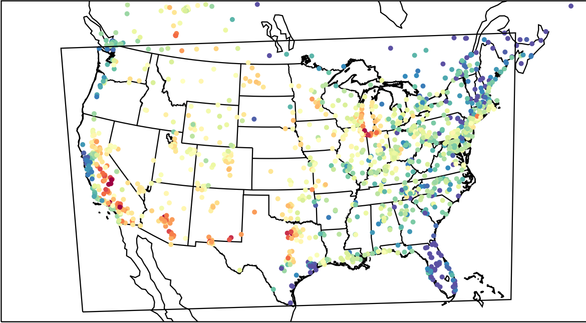
AirNOW (2023-07-24_00:00:00)
