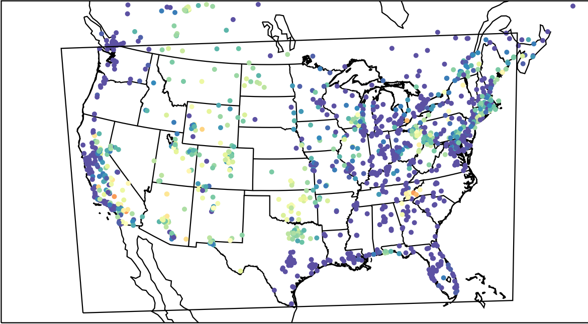
AirNOW (2023-07-25_08:00:00)
