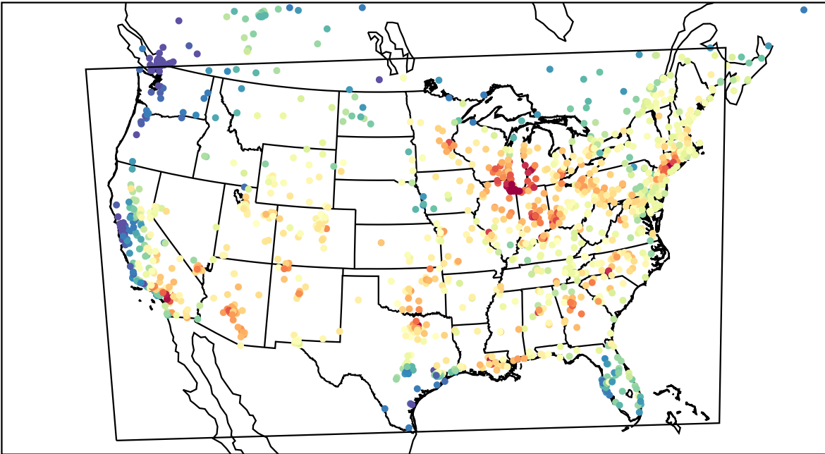
AirNOW (2023-07-25_17:00:00)
