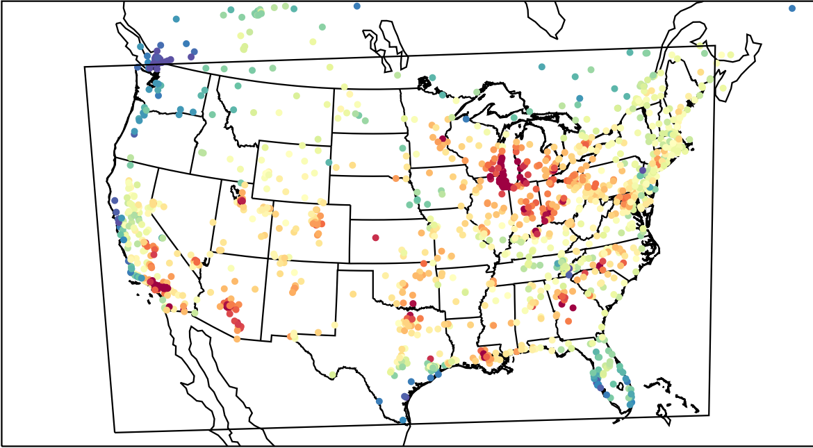
AirNOW (2023-07-25_20:00:00)
