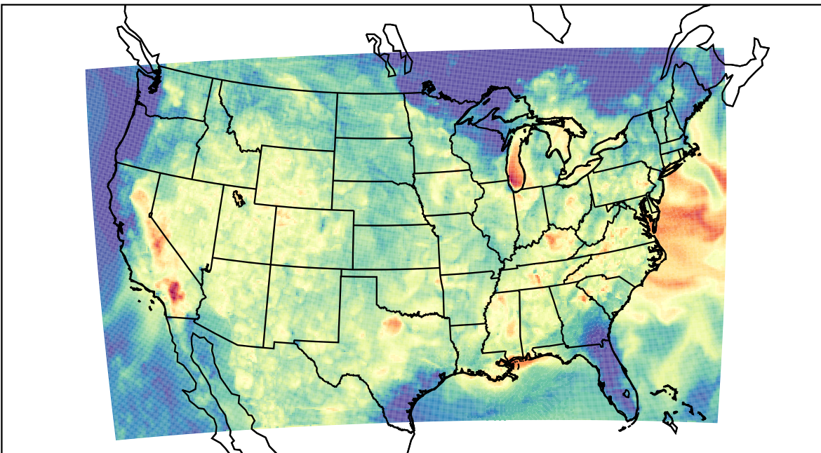
WRF (2023-07-24_04:00:00)
