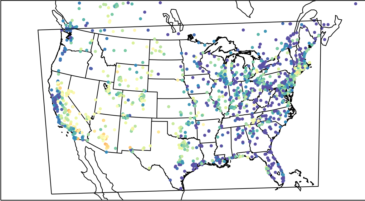
AirNOW (2023-07-24_04:00:00)
