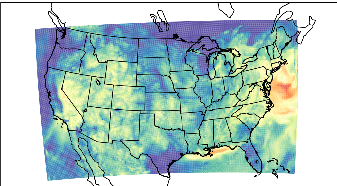
WRF (2023-07-24_13:00:00)
