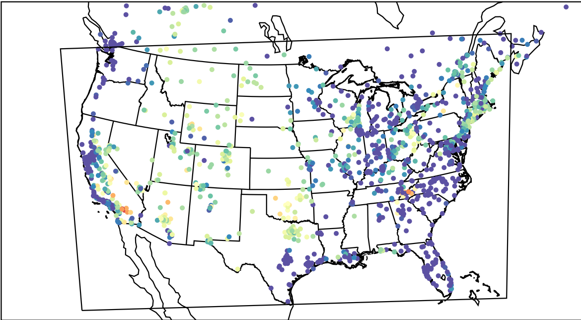
AirNOW (2023-07-25_06:00:00)
