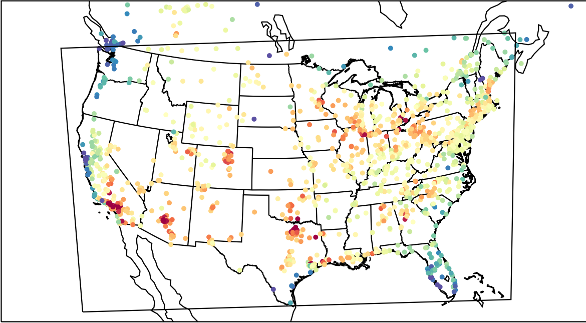
AirNOW (2023-07-24_20:00:00)
