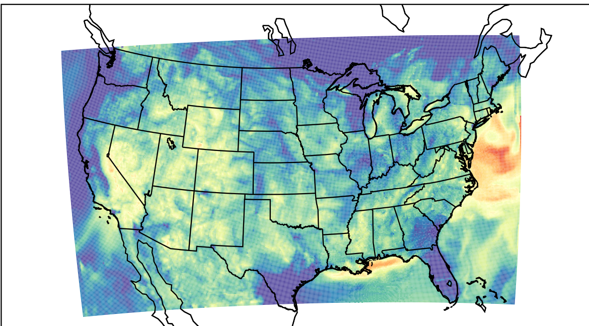
WRF (2023-07-24_12:00:00)
