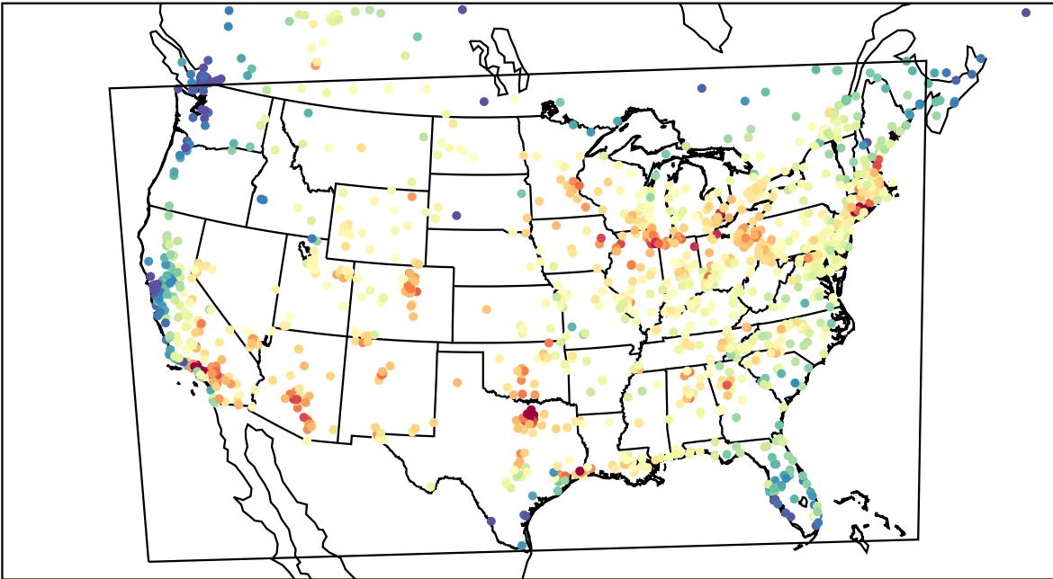
AirNOW (2023-07-24_18:00:00)
