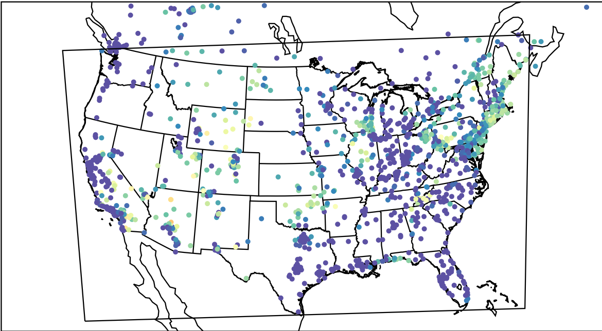
AirNOW (2023-07-25_12:00:00)
