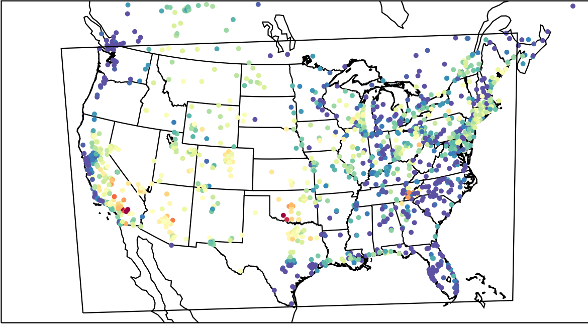
AirNOW (2023-07-25_03:00:00)
