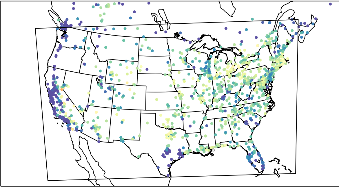
AirNOW (2023-07-24_14:00:00)
