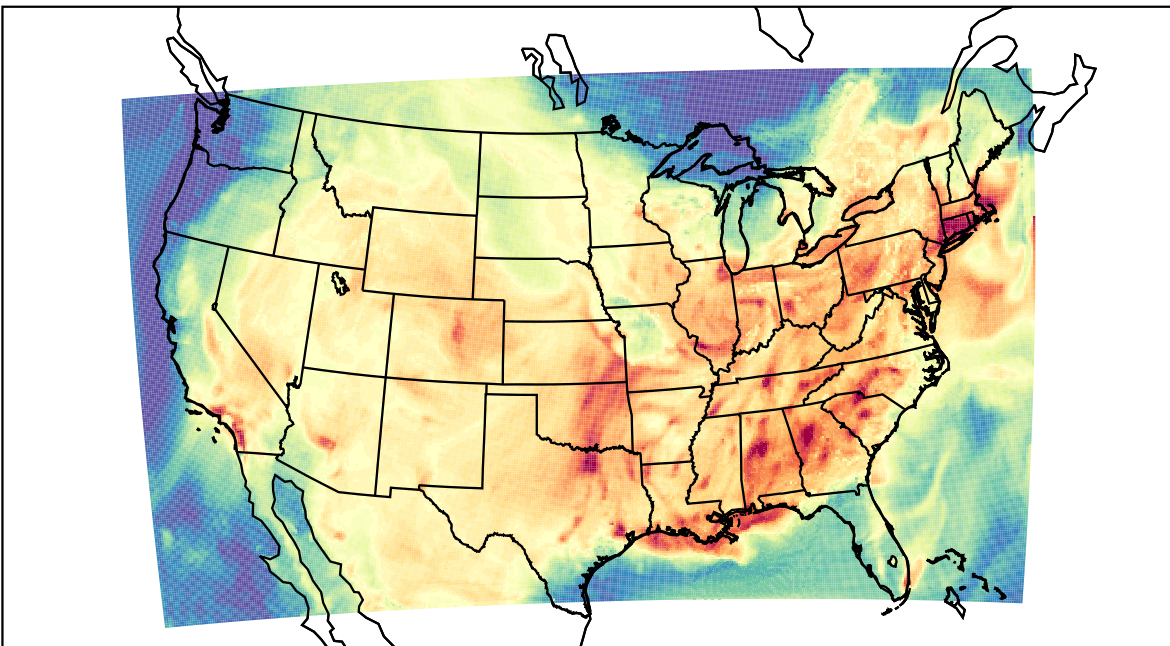
WRF (2023-07-24_19:00:00)
