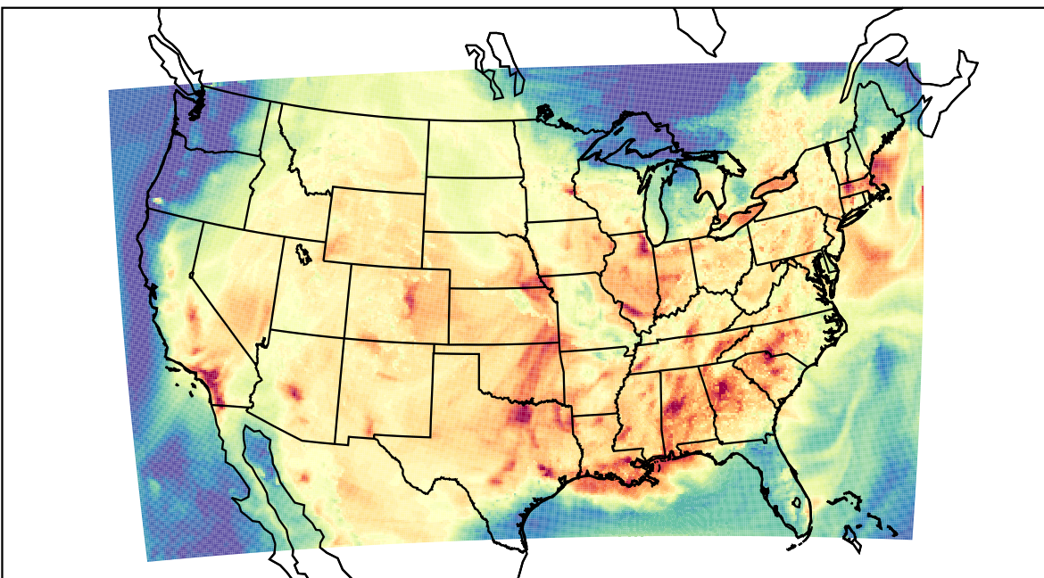
WRF (2023-07-24_23:00:00)
