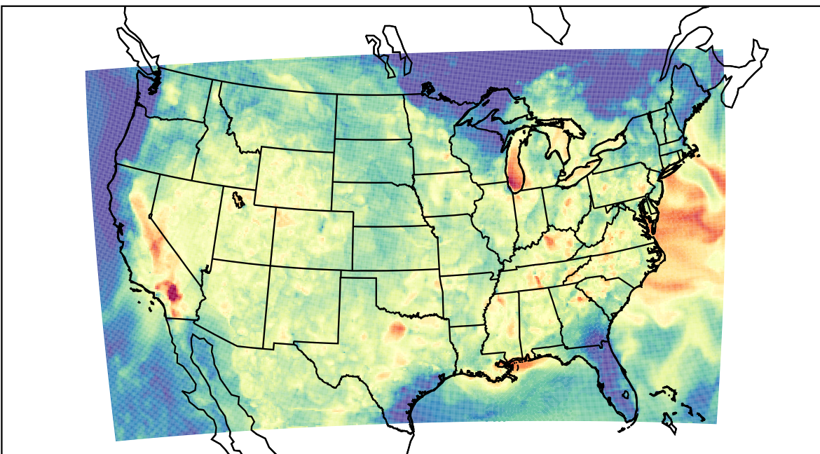
WRF (2023-07-24_03:00:00)
