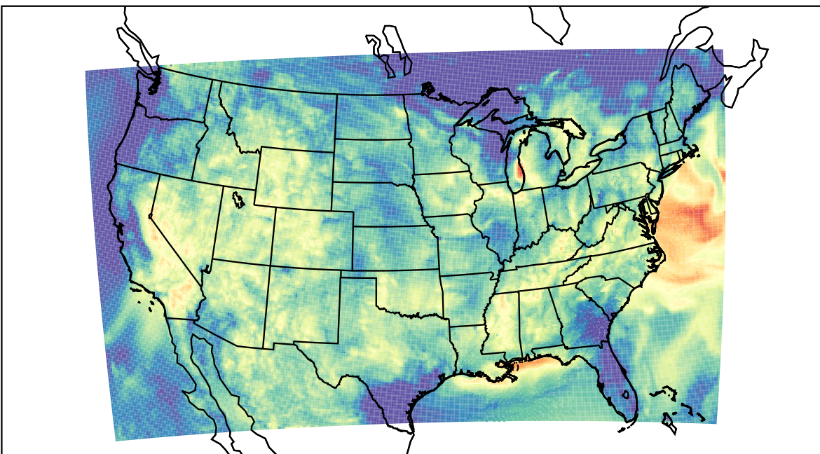
WRF (2023-07-24_09:00:00)
