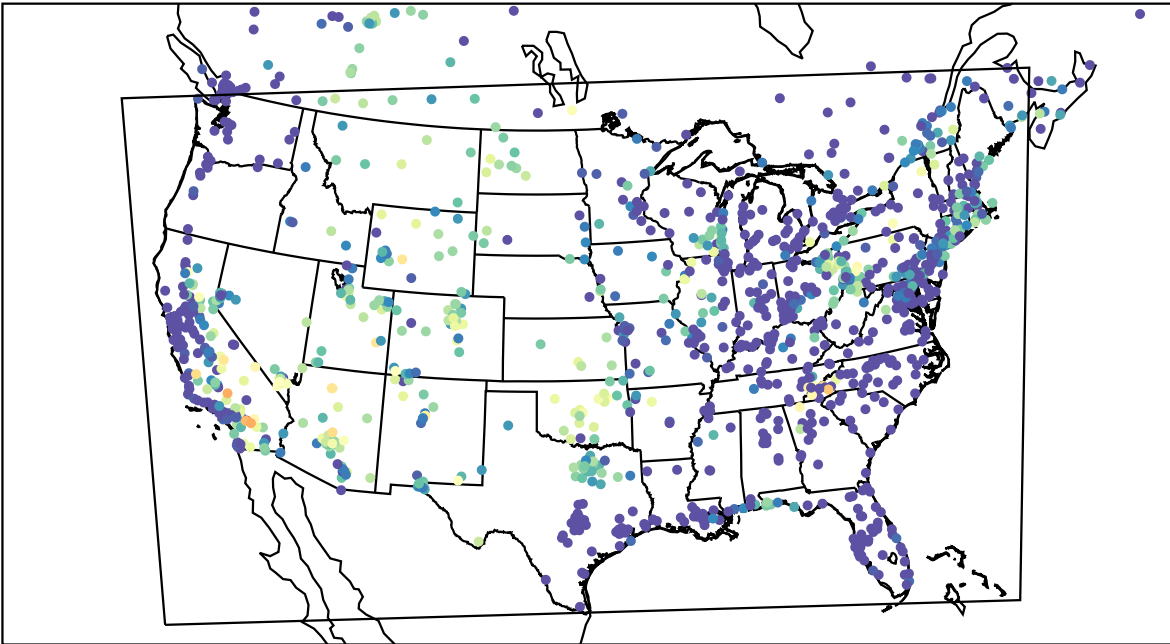
AirNOW (2023-07-25_09:00:00)
