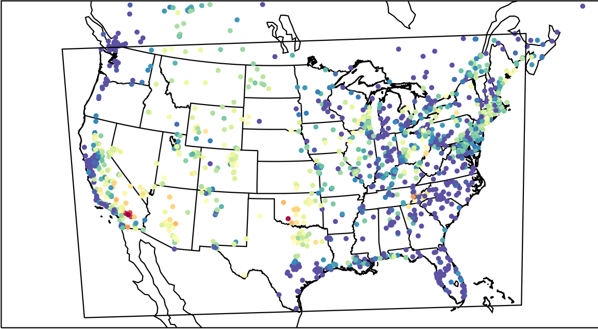
AirNOW (2023-07-25_04:00:00)
