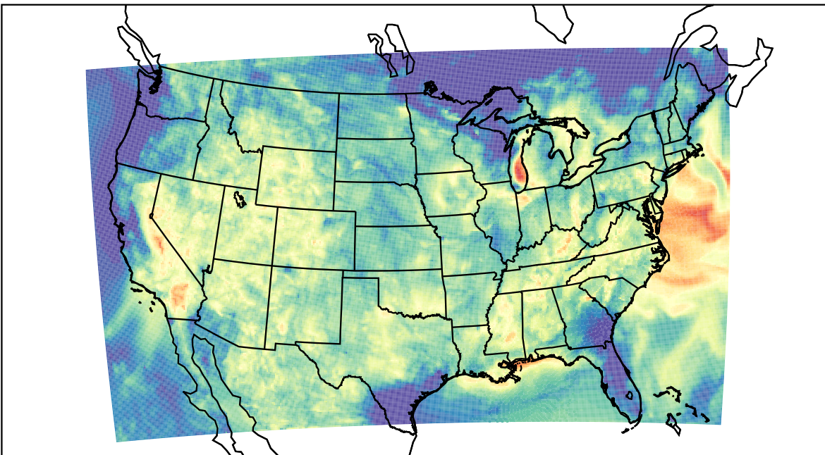
WRF (2023-07-24_07:00:00)
