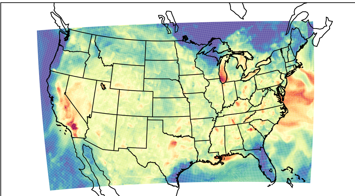
WRF (2023-07-24_02:00:00)
