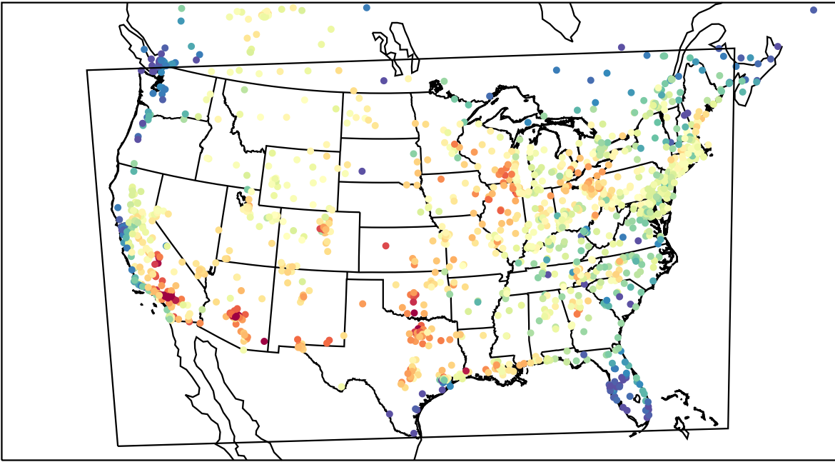
AirNOW (2023-07-24_23:00:00)
