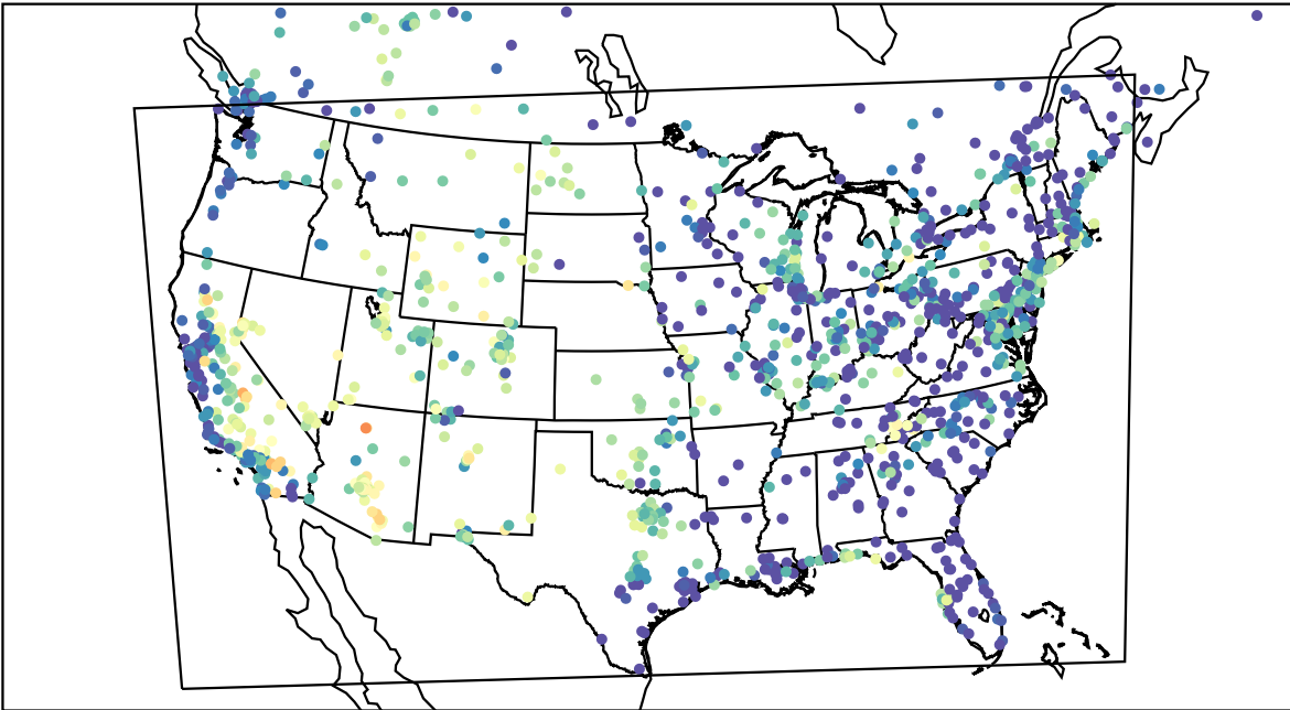
AirNOW (2023-07-24_05:00:00)
