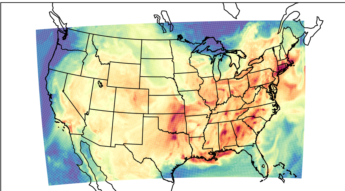
WRF (2023-07-24_18:00:00)
