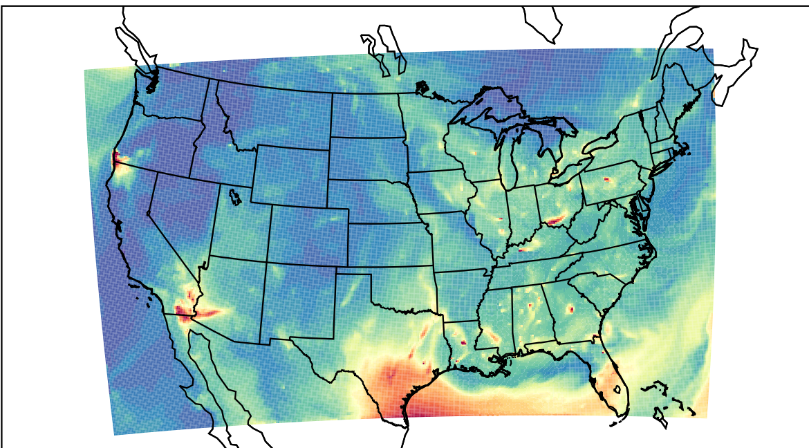
WRF 2023-07-25_11:00:00
