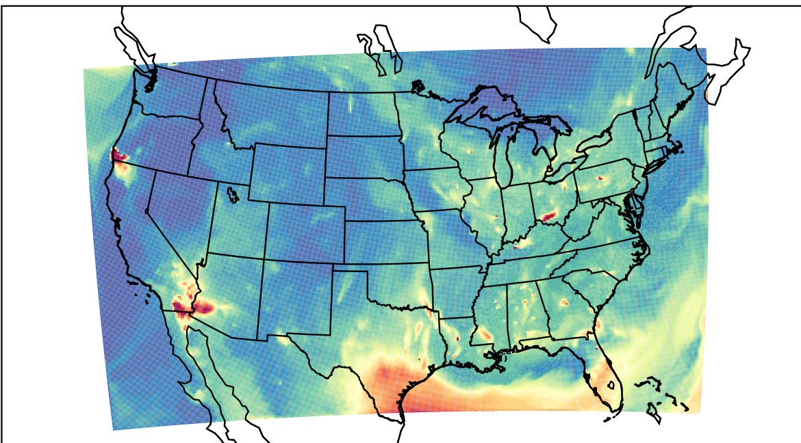
WRF 2023-07-25_09:00:00
