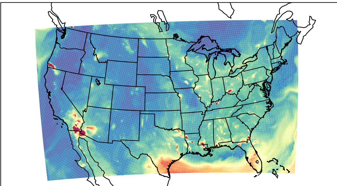
WRF 2023-07-25_05:00:00
