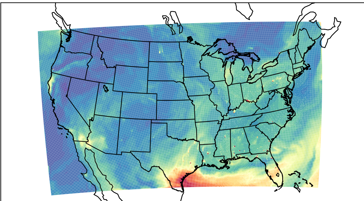
WRF 2023-07-25_19:00:00
