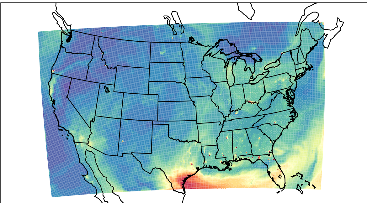
WRF 2023-07-25_21:00:00
