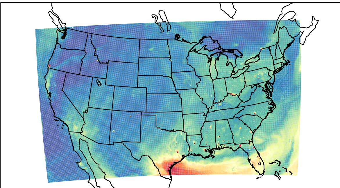
WRF 2023-07-25_22:00:00
