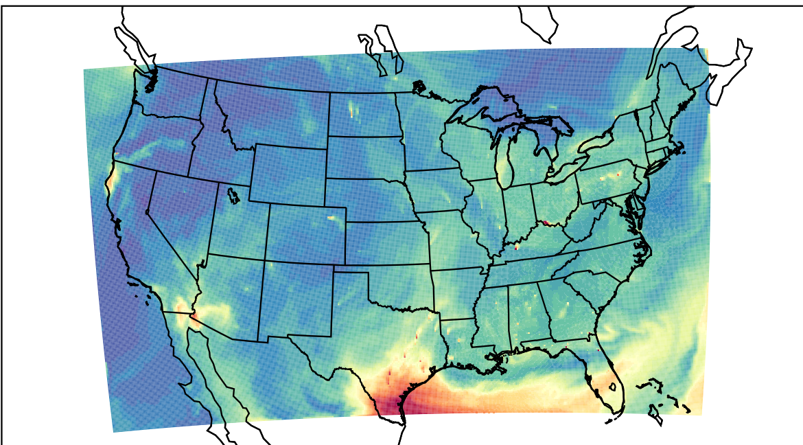
WRF 2023-07-25_17:00:00
