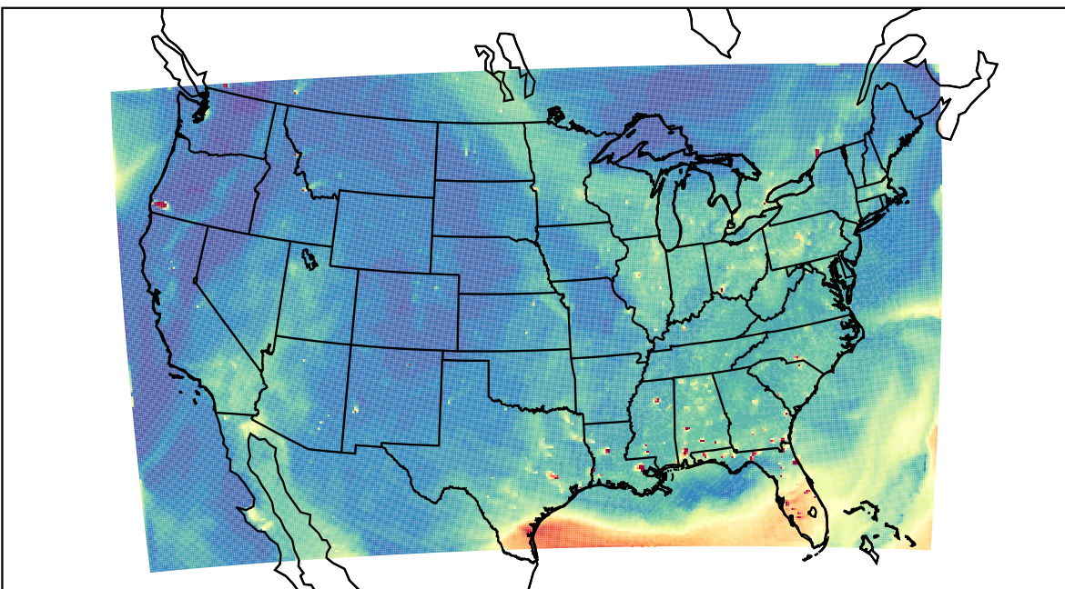
WRF 2023-07-25_00:00:00
