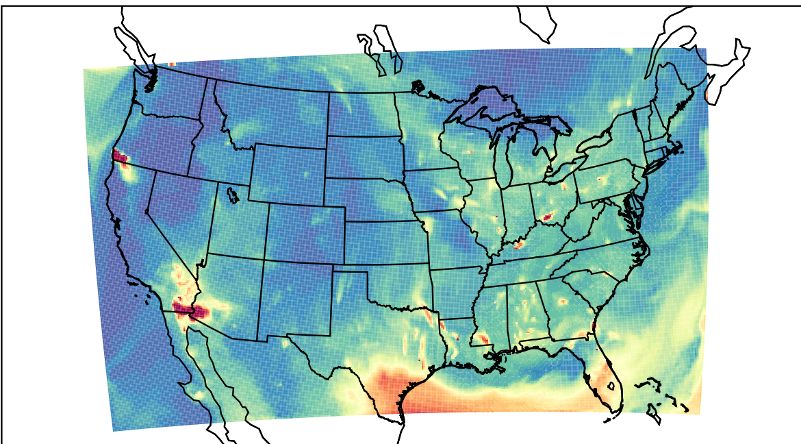
WRF 2023-07-25_07:00:00
