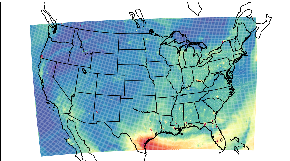
WRF 2023-07-25_23:00:00
