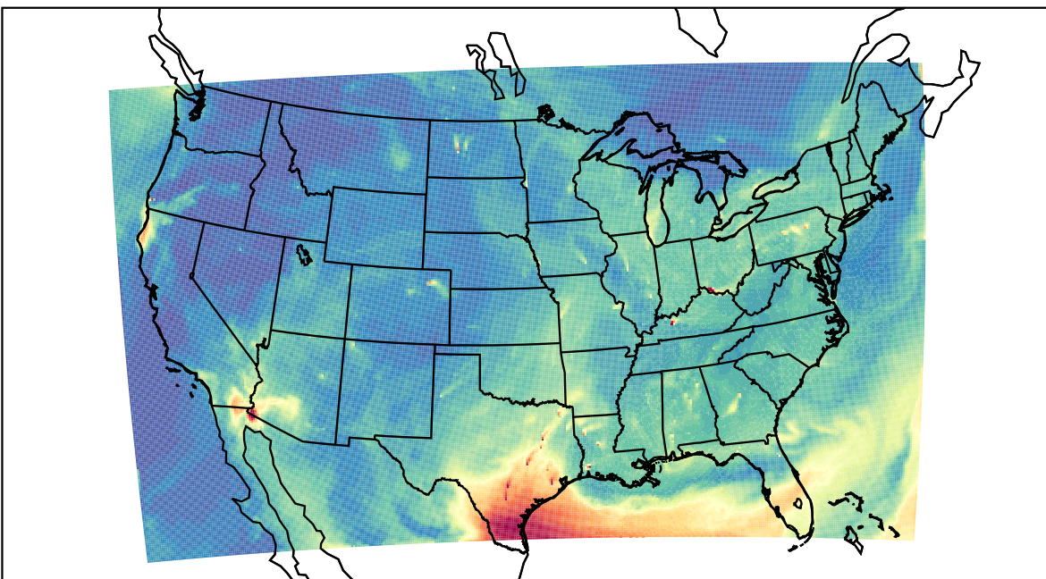
WRF 2023-07-25_16:00:00
