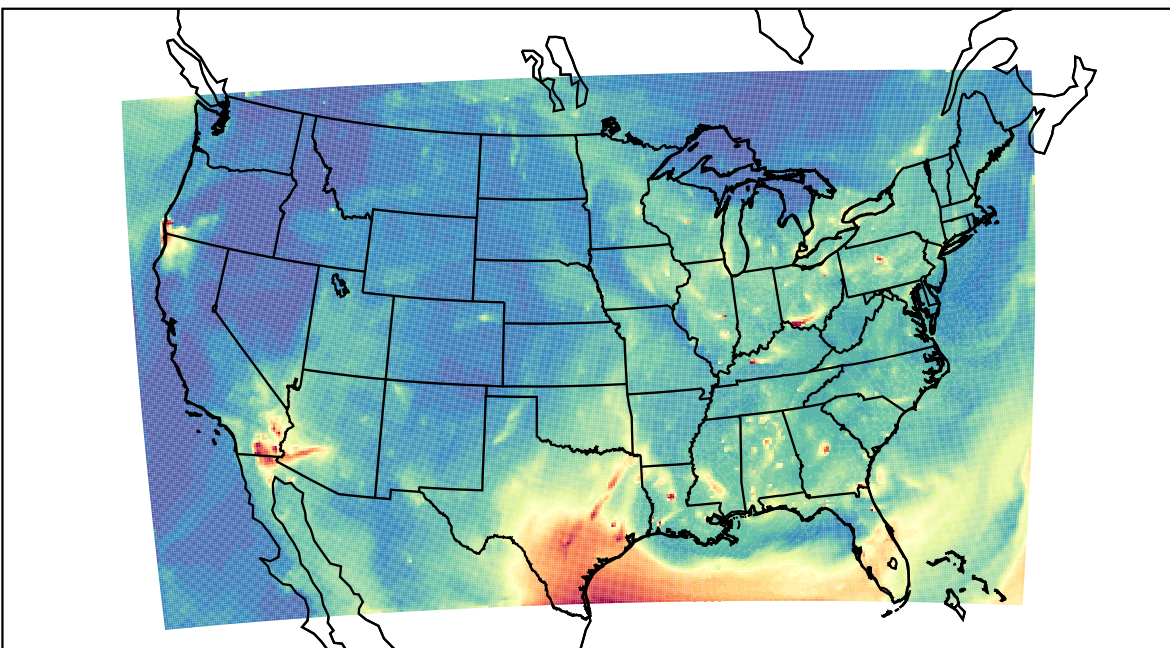
WRF 2023-07-25_12:00:00
