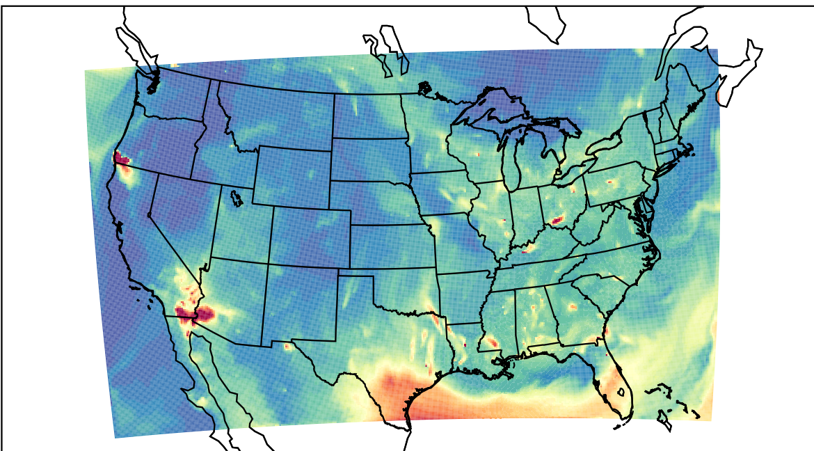
WRF 2023-07-25_08:00:00
