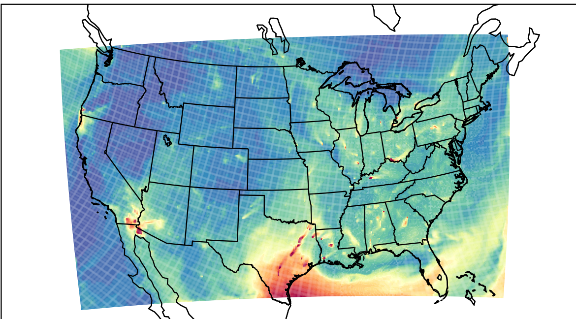
WRF 2023-07-25_14:00:00
