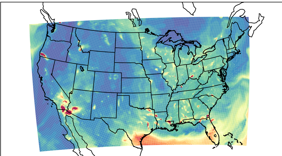
WRF 2023-07-25_04:00:00
