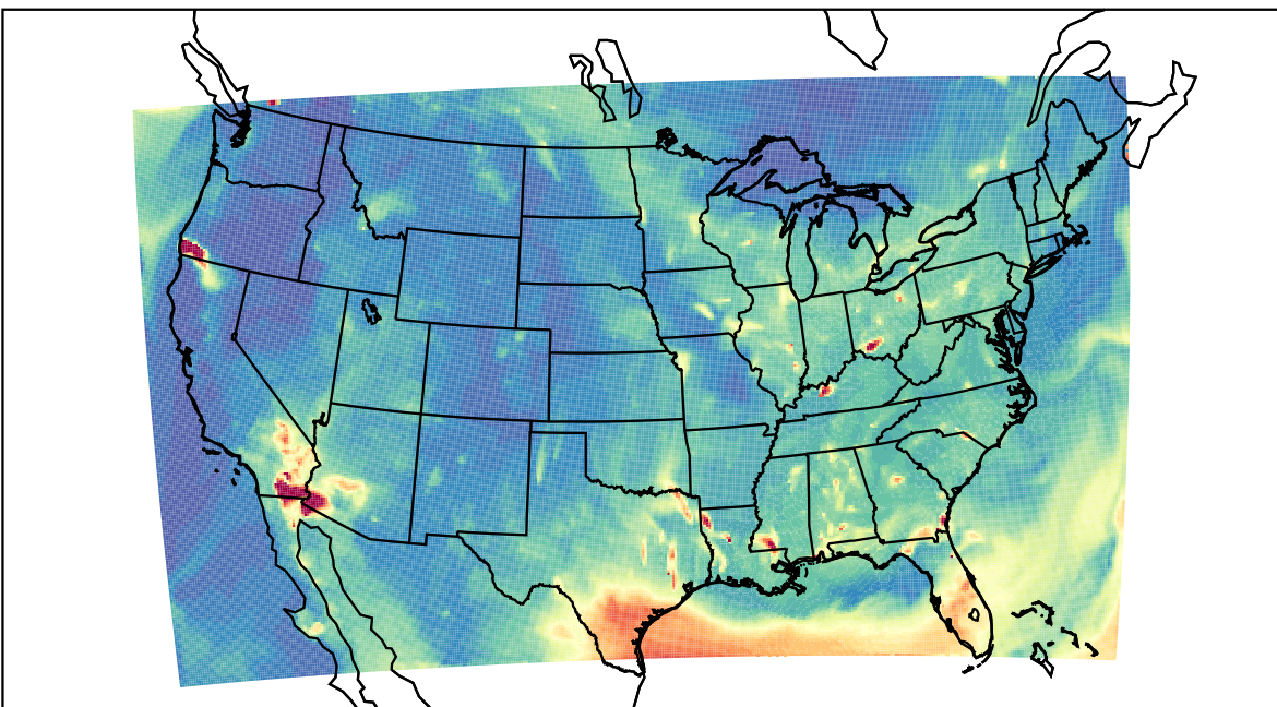
WRF 2023-07-25_06:00:00
