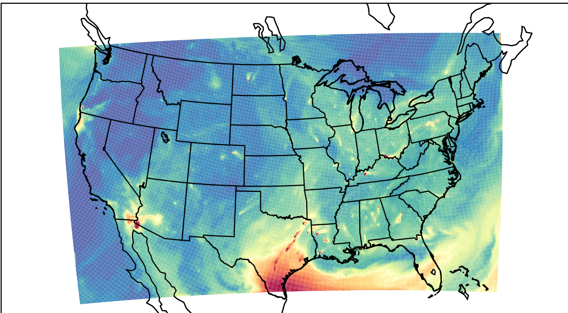
WRF 2023-07-25_15:00:00
