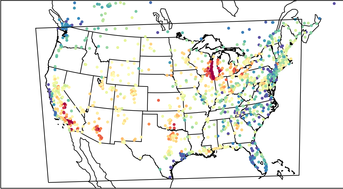
AirNOW (2023-07-26_00:00:00)
