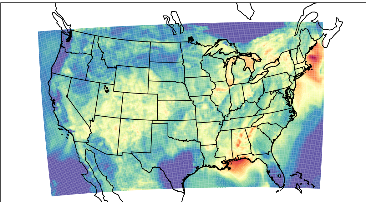
WRF (2023-07-27_07:00:00)
