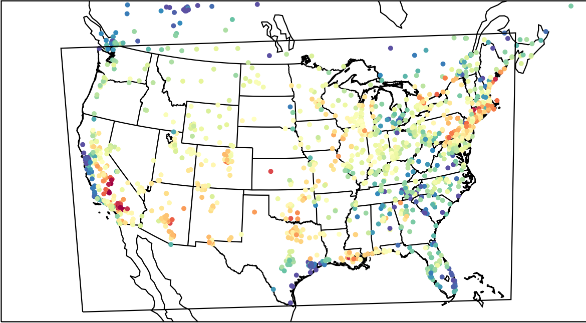
AirNOW (2023-07-27_00:00:00)
