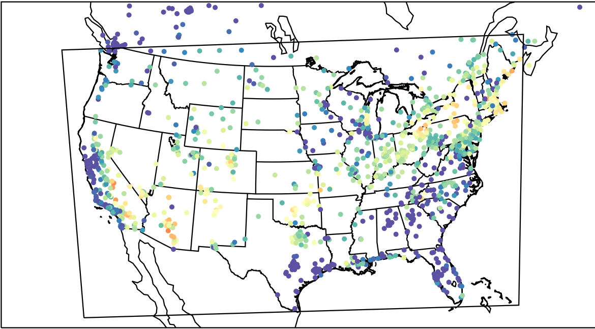
AirNOW (2023-07-27_05:00:00)
