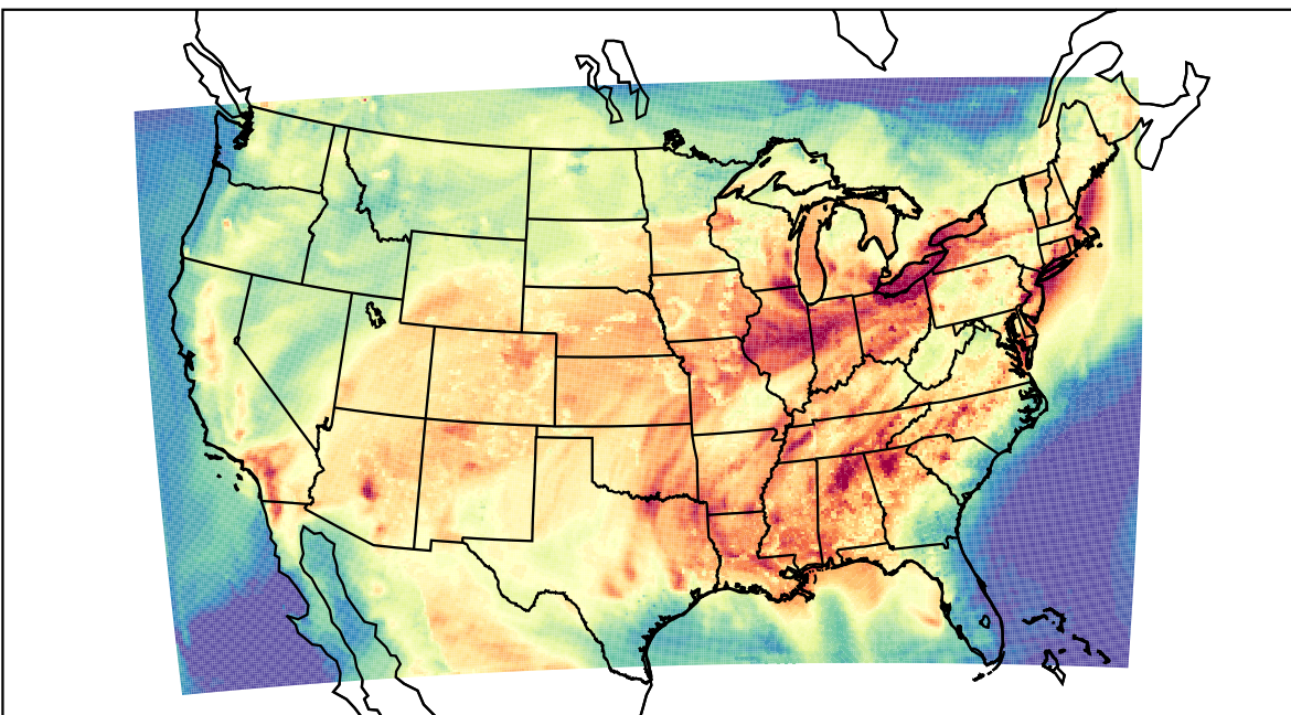
WRF (2023-07-27_23:00:00)
