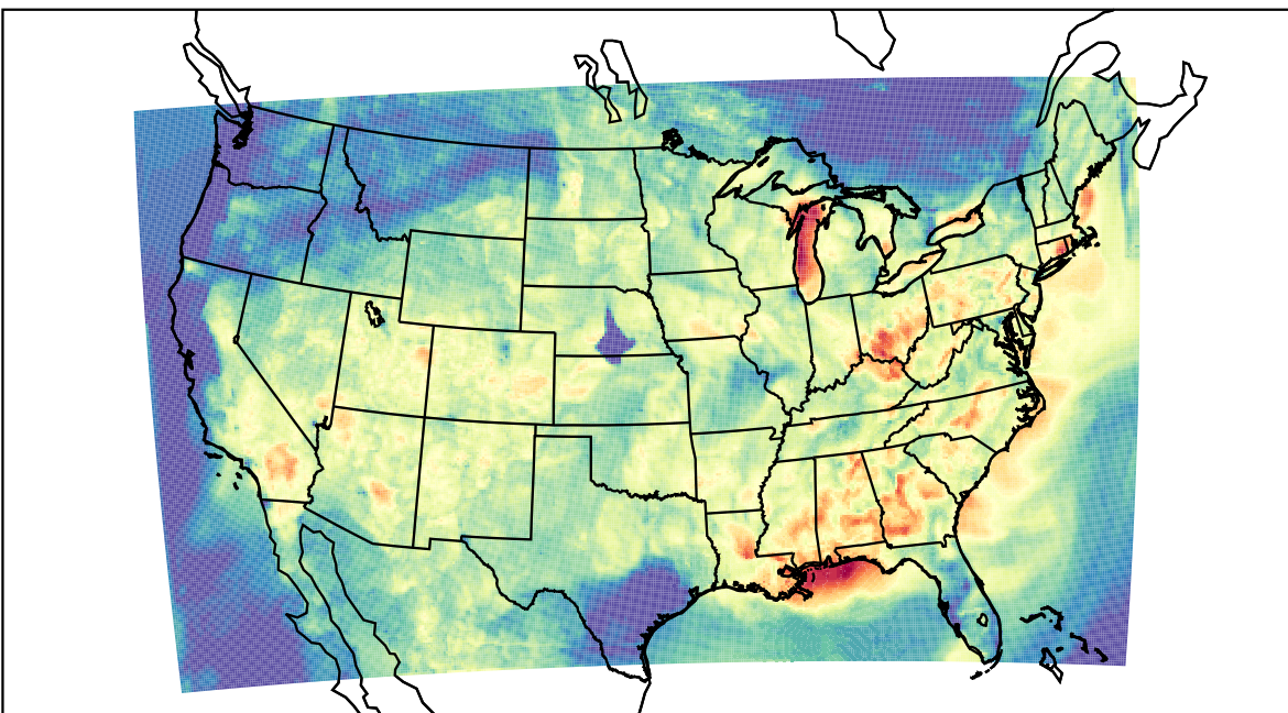
WRF (2023-07-26_04:00:00)
