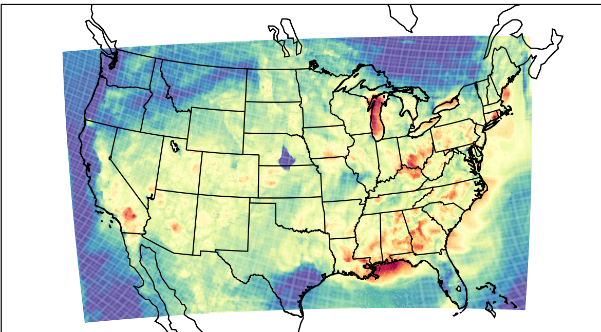
WRF (2023-07-26_03:00:00)
