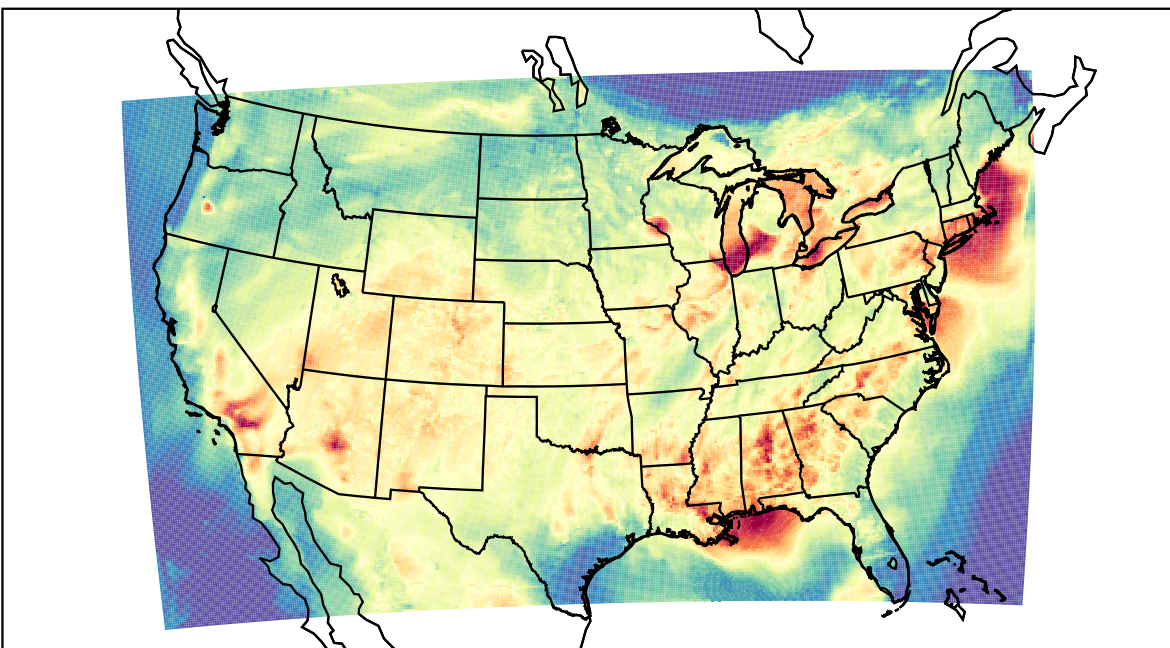
WRF (2023-07-27_01:00:00)
