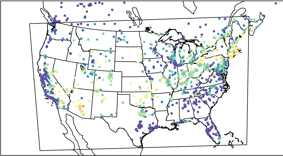
AirNOW (2023-07-27_07:00:00)
