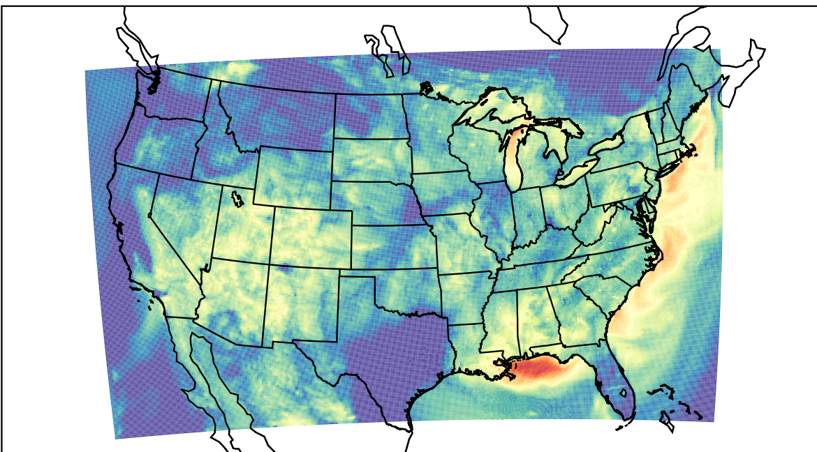
WRF (2023-07-26_12:00:00)
