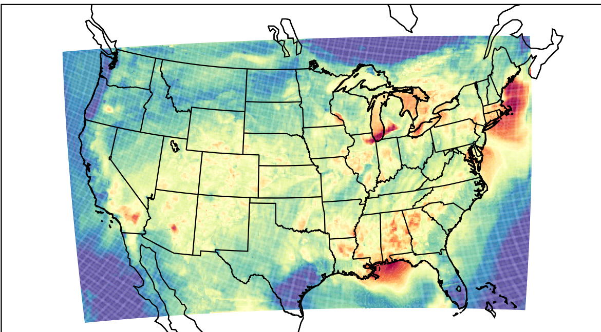
WRF (2023-07-27_03:00:00)
