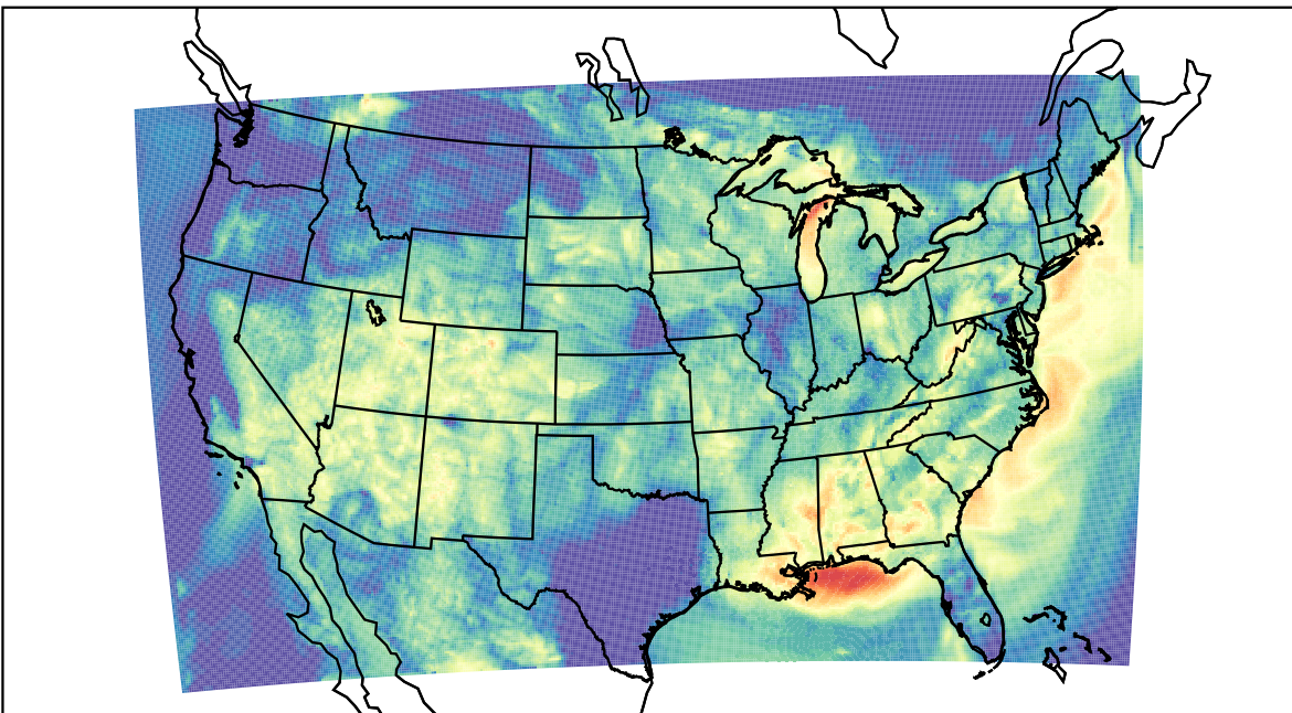
WRF (2023-07-26_11:00:00)
