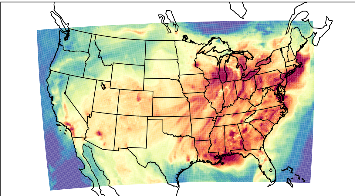
WRF (2023-07-26_20:00:00)
