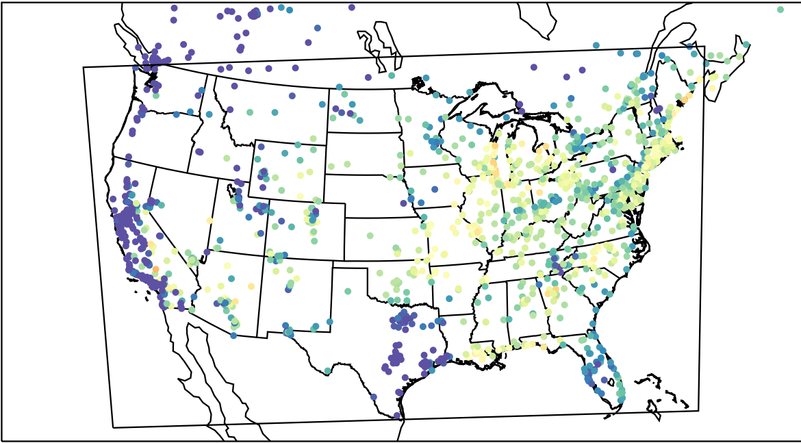
AirNOW (2023-07-27_14:00:00)
