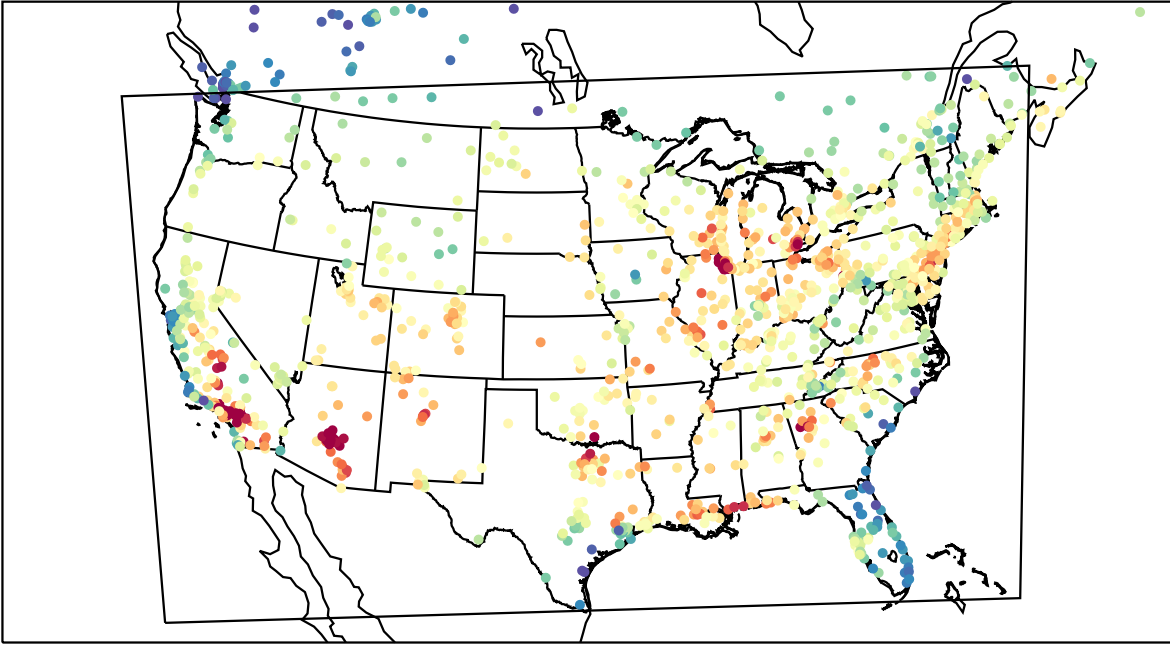
AirNOW (2023-07-27_21:00:00)
