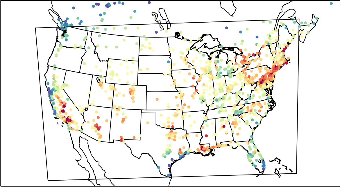
AirNOW (2023-07-26_21:00:00)
