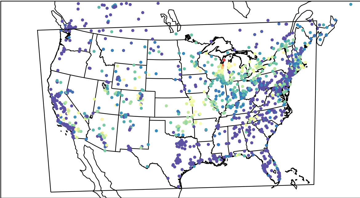
AirNOW (2023-07-26_12:00:00)
