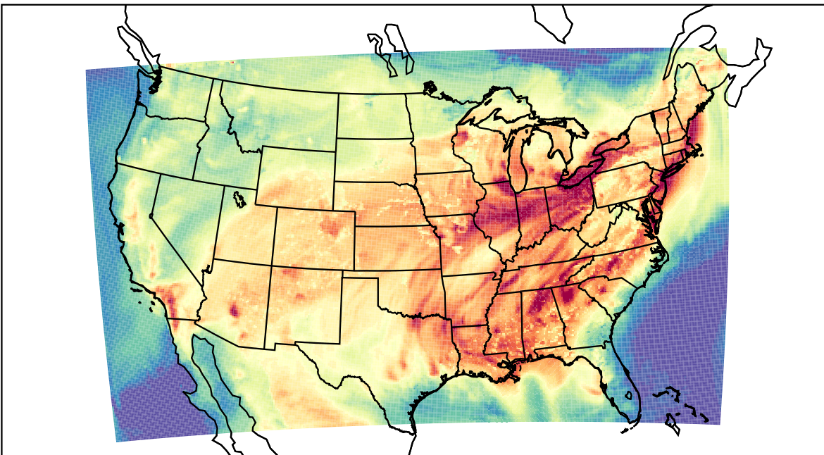
WRF (2023-07-27_22:00:00)
