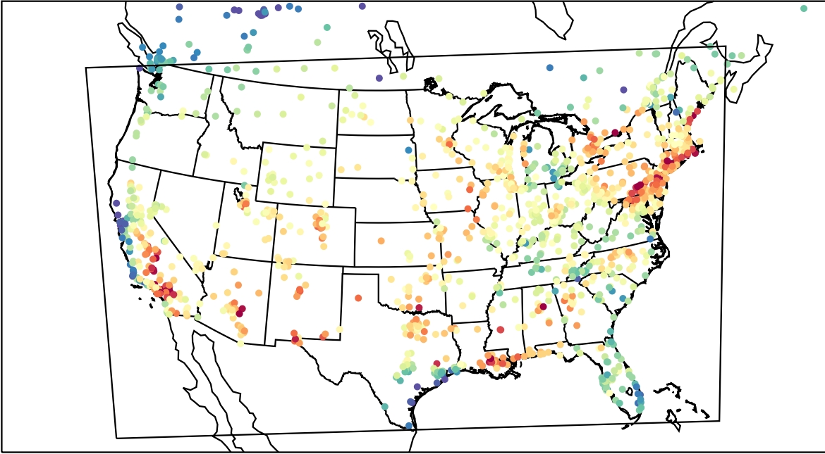
AirNOW (2023-07-26_22:00:00)
