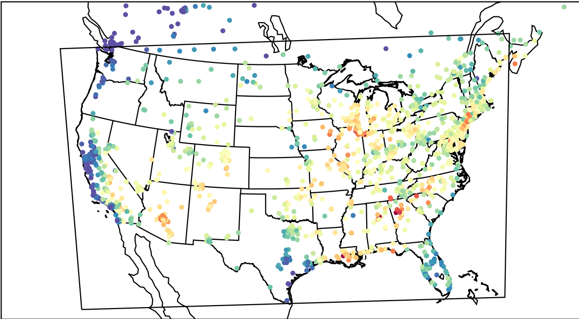
AirNOW (2023-07-27_16:00:00)
