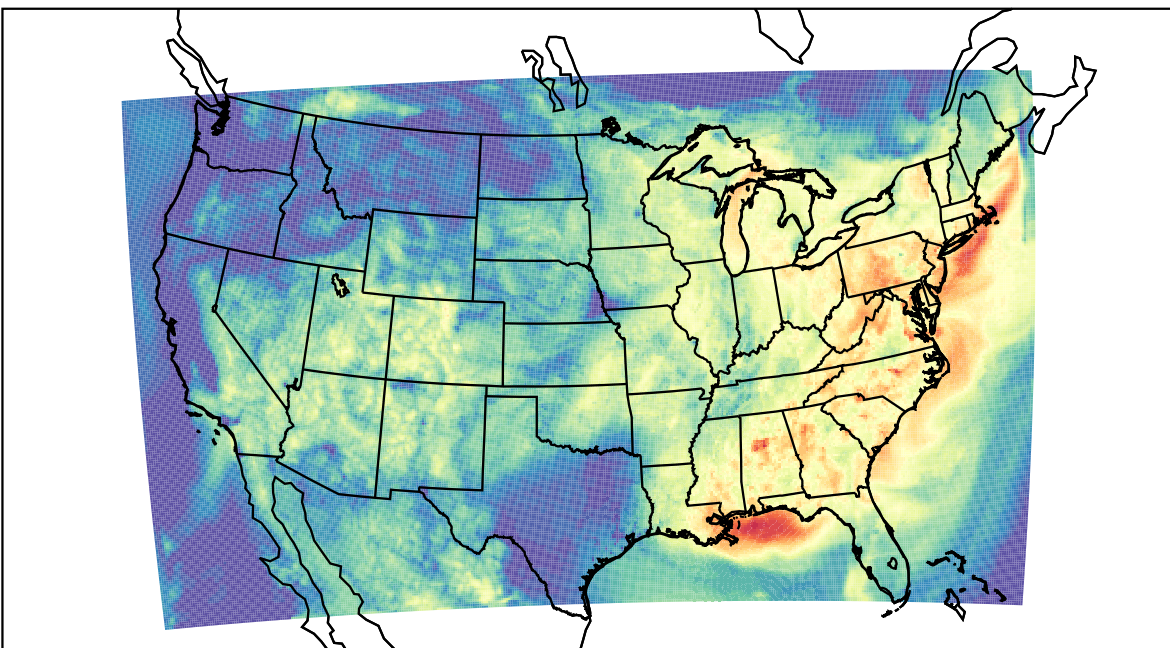
WRF (2023-07-26_14:00:00)
