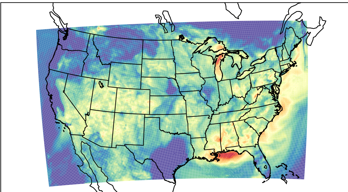
WRF (2023-07-26_09:00:00)
