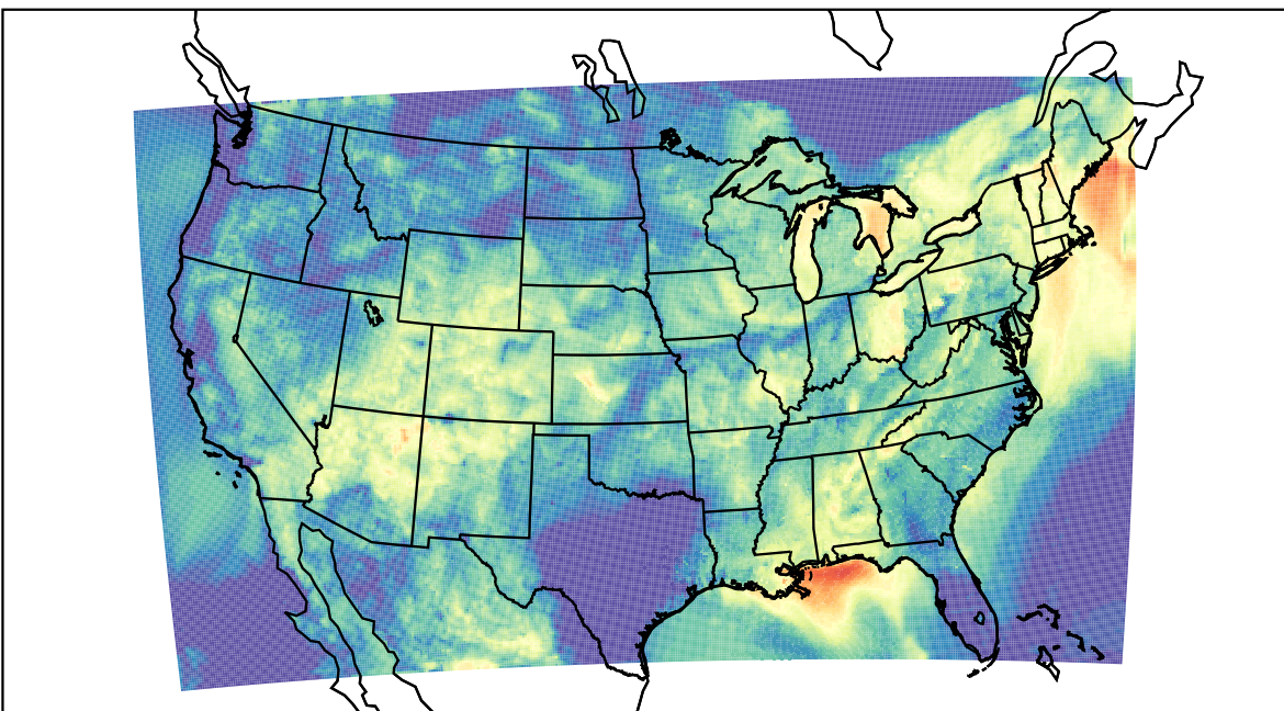
WRF (2023-07-27_12:00:00)
