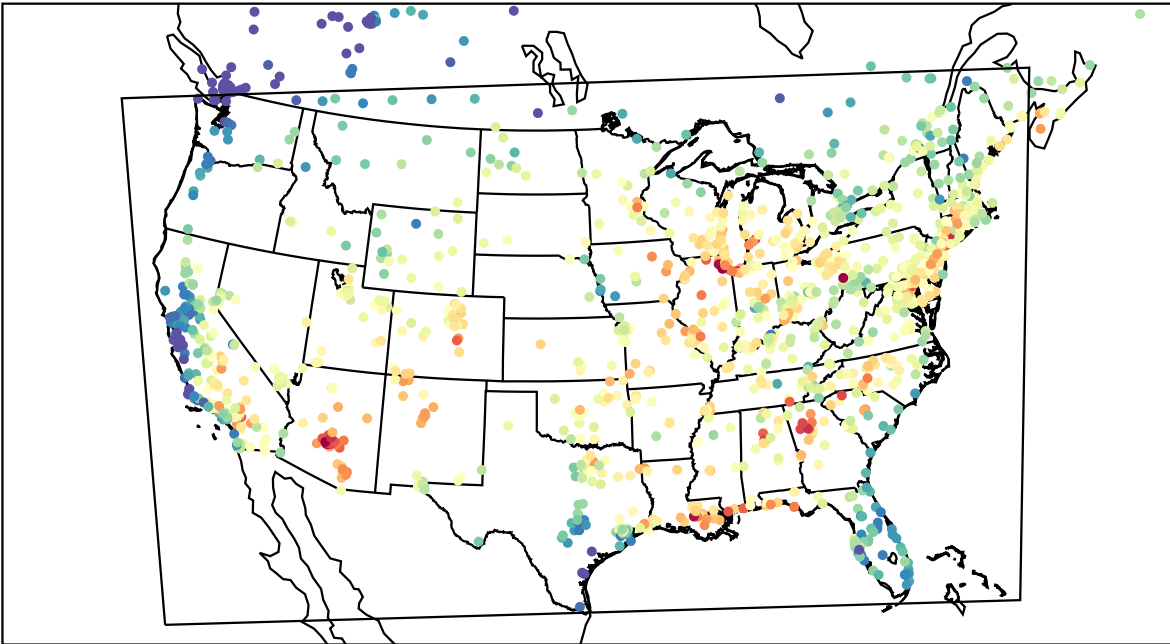
AirNOW (2023-07-27_17:00:00)
