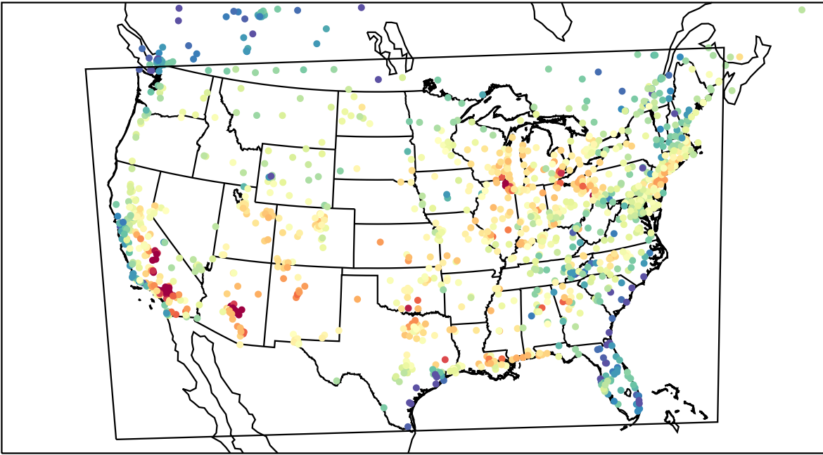
AirNOW (2023-07-27_23:00:00)
