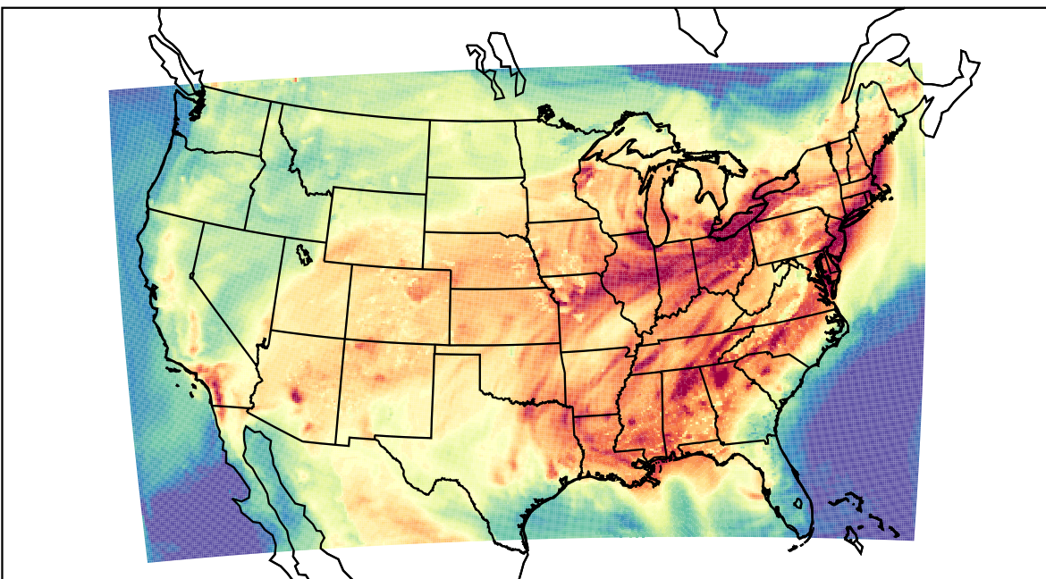
WRF (2023-07-27_21:00:00)
