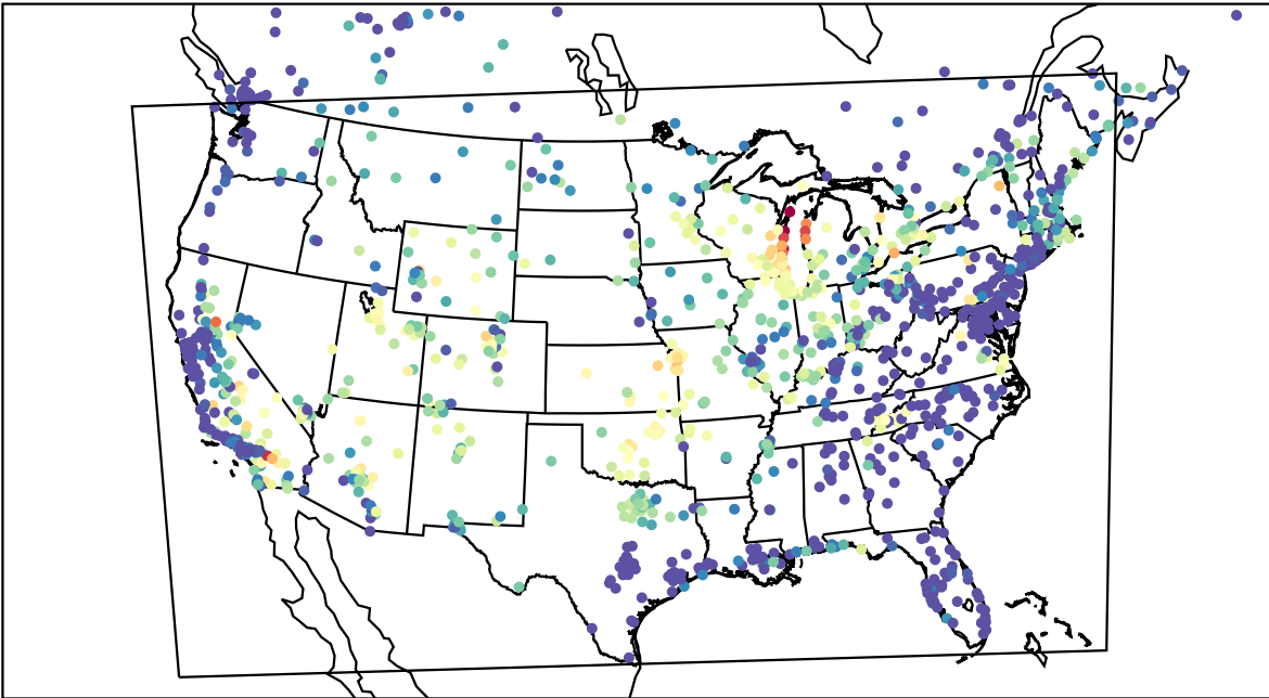
AirNOW (2023-07-26_07:00:00)
