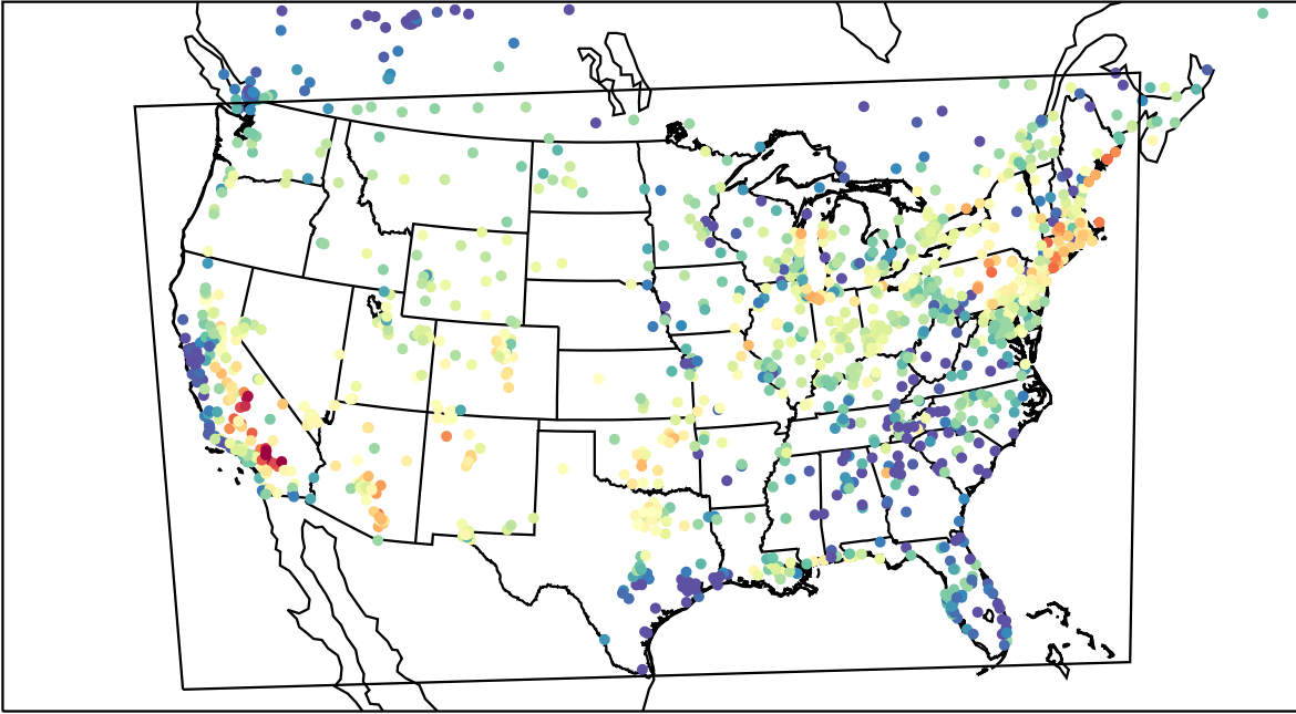
AirNOW (2023-07-27_02:00:00)
