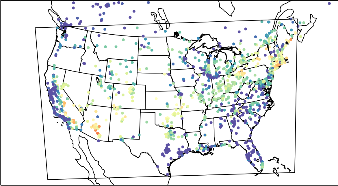
AirNOW (2023-07-27_06:00:00)
