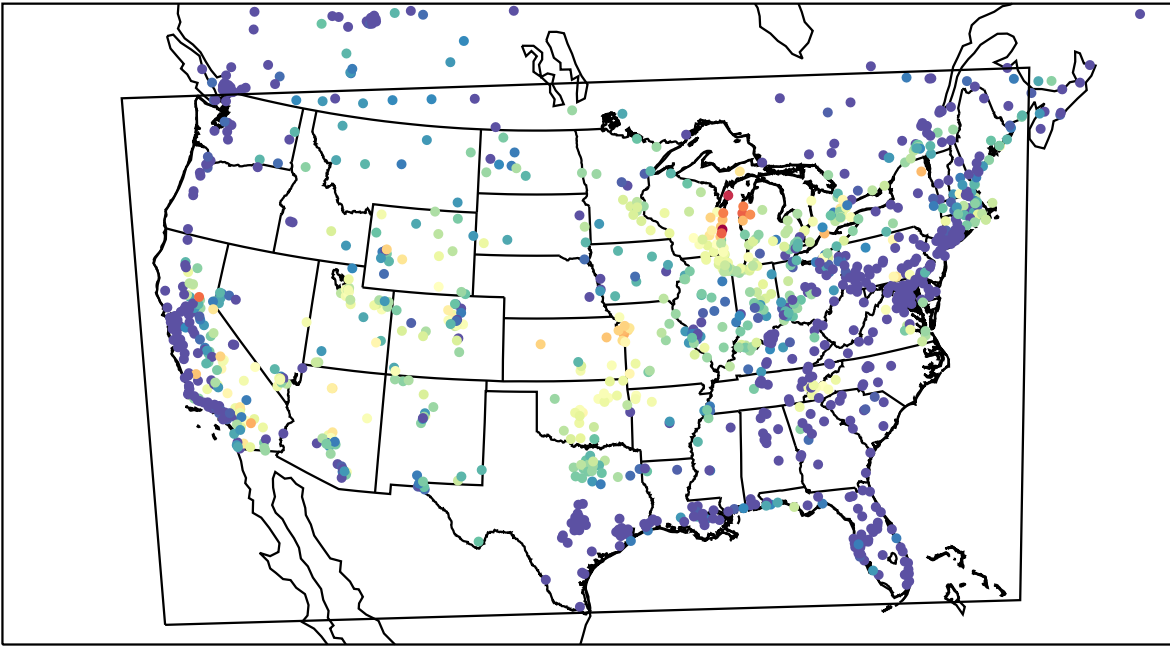
AirNOW (2023-07-26_08:00:00)
