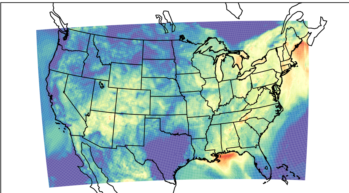
WRF (2023-07-27_13:00:00)
