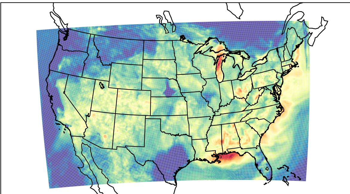
WRF (2023-07-26_07:00:00)
