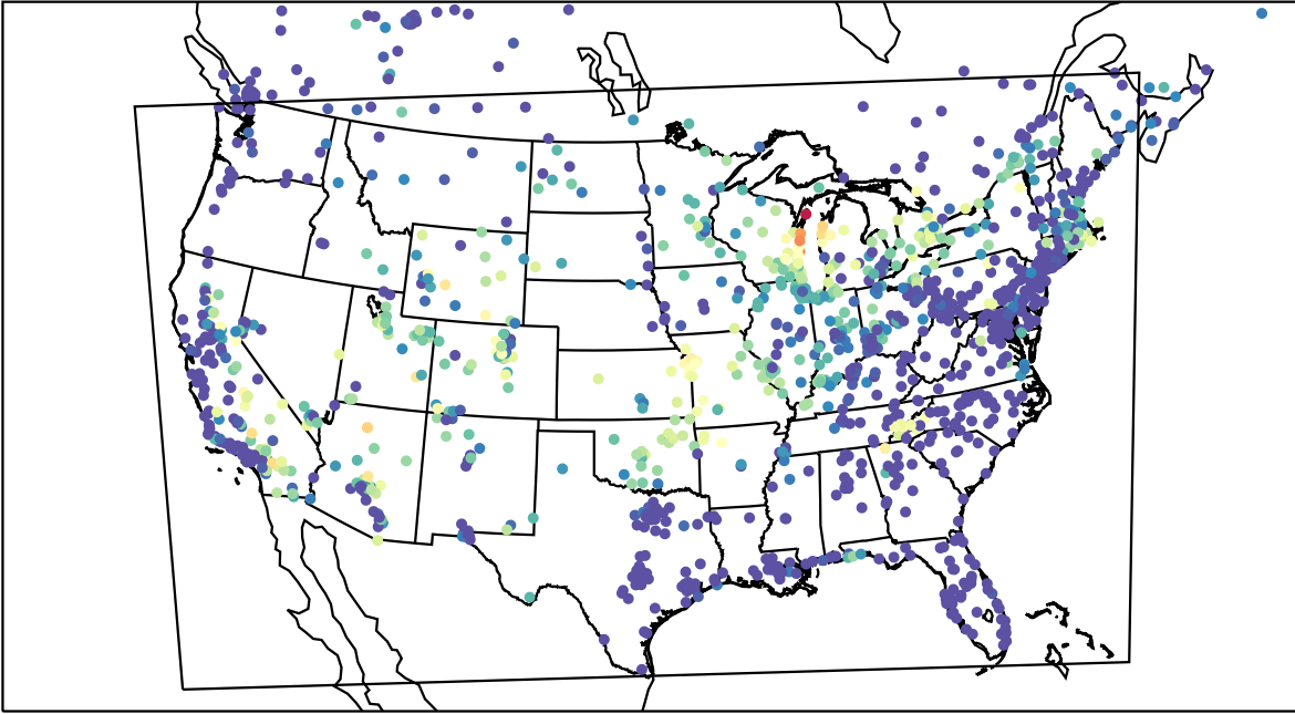
AirNOW (2023-07-26_11:00:00)
