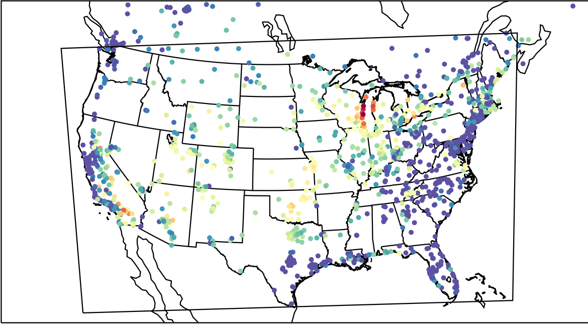
AirNOW (2023-07-26_06:00:00)
