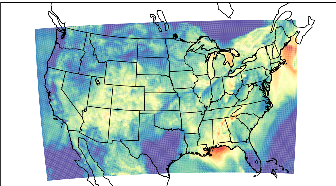
WRF (2023-07-27_10:00:00)
