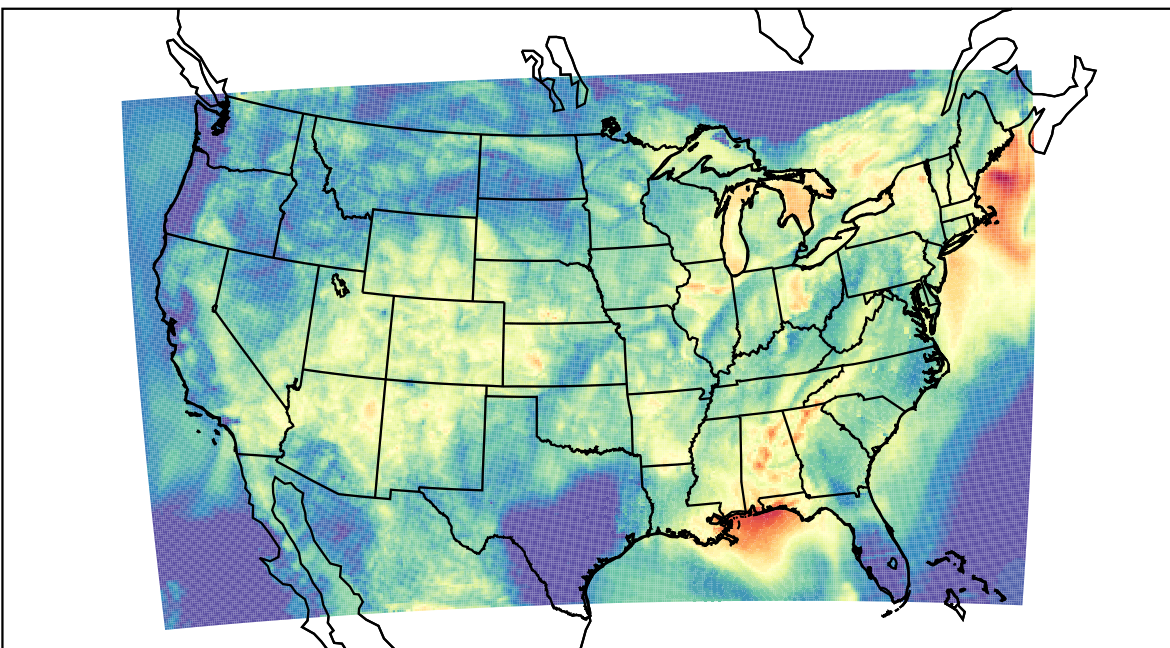
WRF (2023-07-27_08:00:00)
