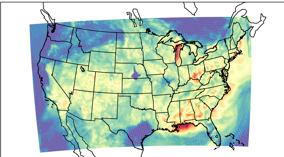
WRF (2023-07-26_05:00:00)
