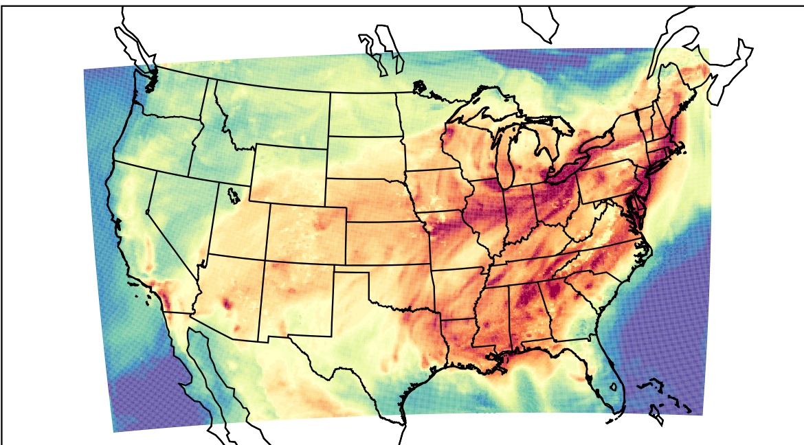
WRF (2023-07-27_20:00:00)
