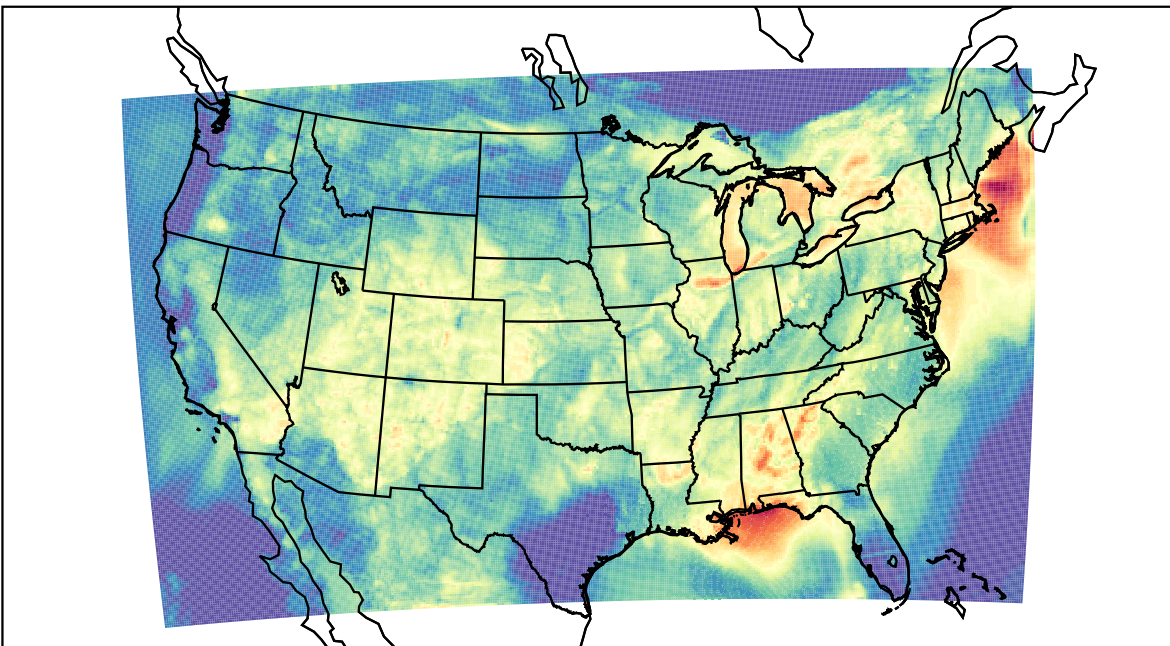
WRF (2023-07-27_06:00:00)
