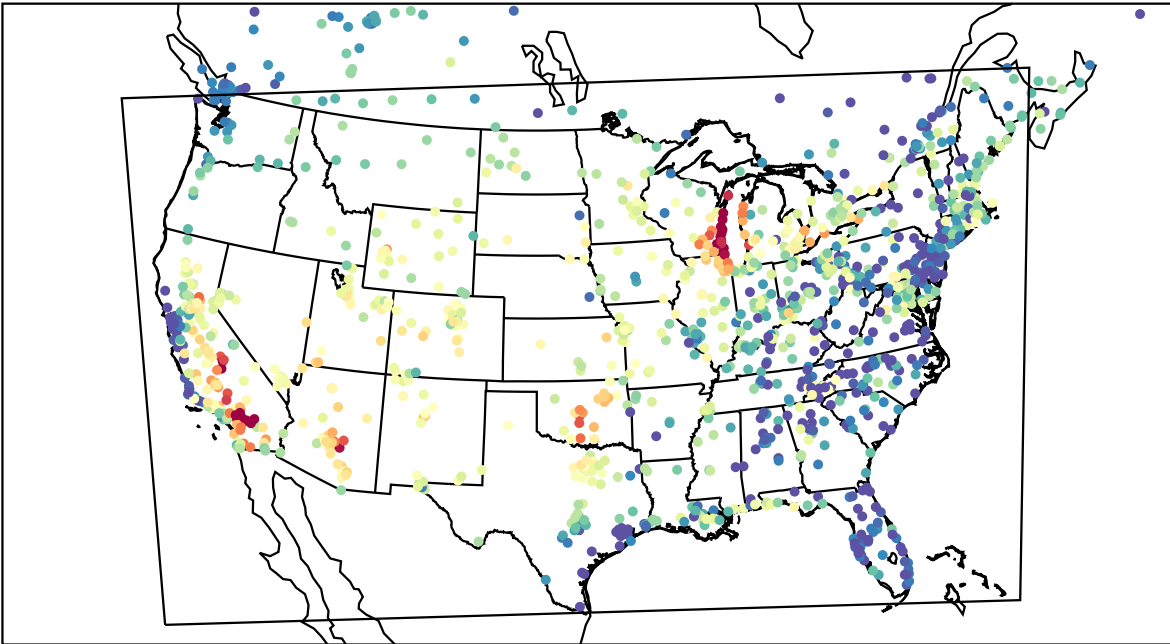
AirNOW (2023-07-26_02:00:00)
