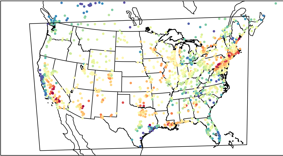
AirNOW (2023-07-26_23:00:00)
