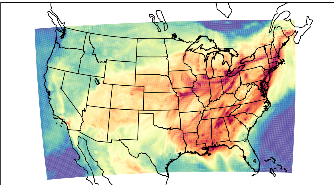
WRF (2023-07-27_18:00:00)
