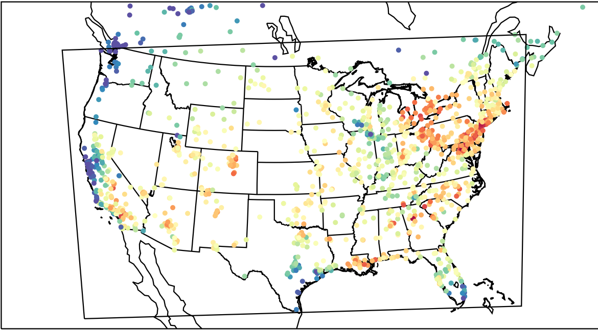
AirNOW (2023-07-26_17:00:00)
