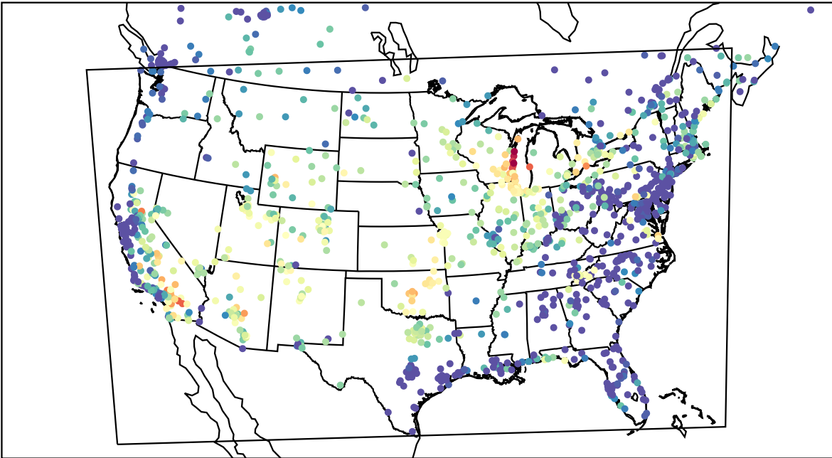
AirNOW (2023-07-26_05:00:00)
