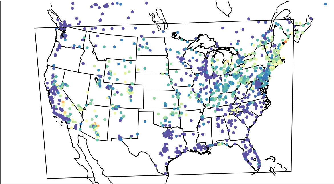
AirNOW (2023-07-27_11:00:00)
