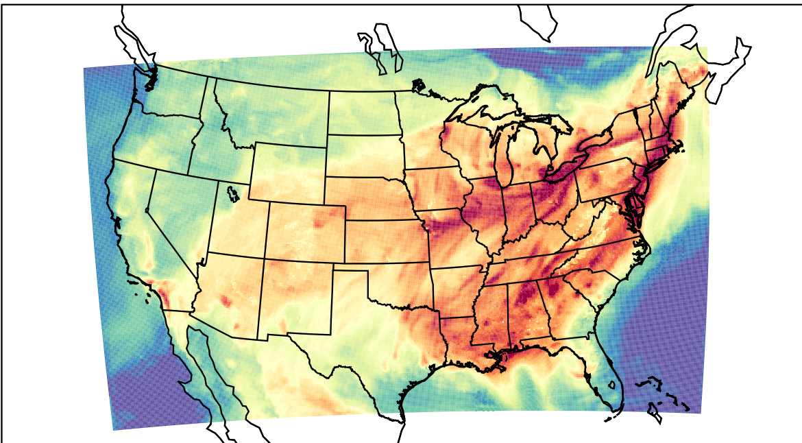
WRF (2023-07-27_19:00:00)
