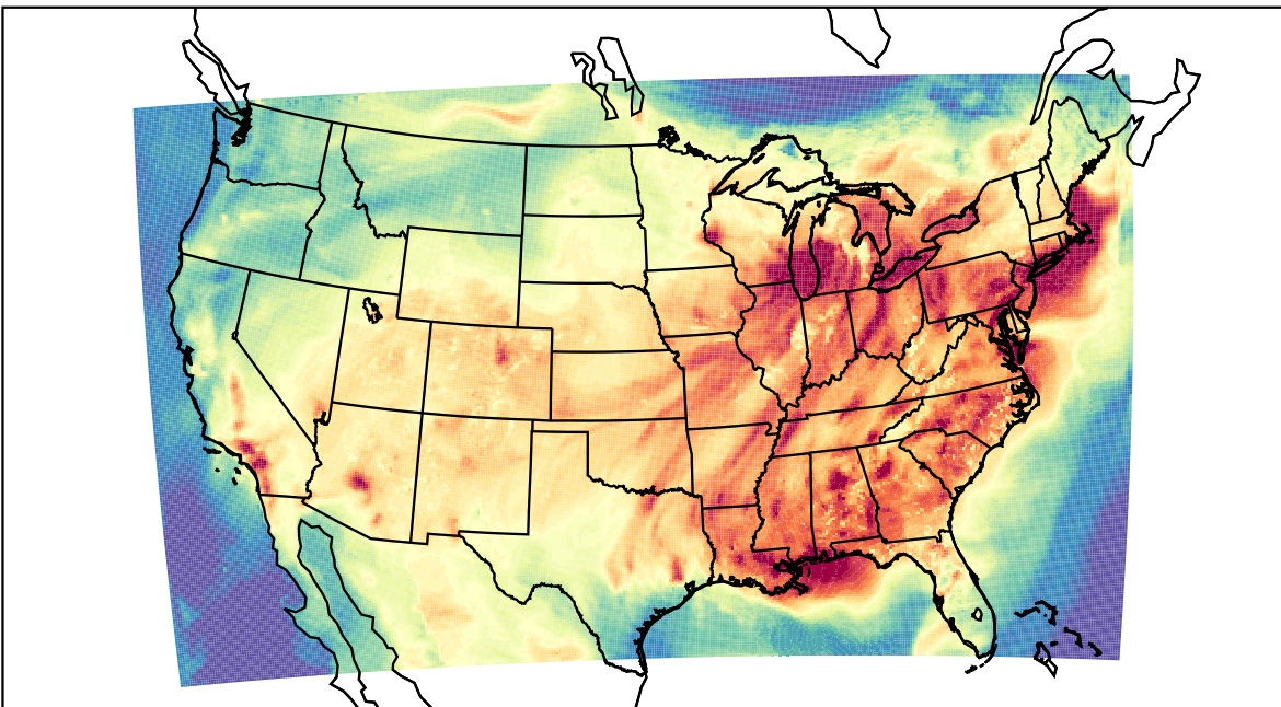
WRF (2023-07-26_21:00:00)
