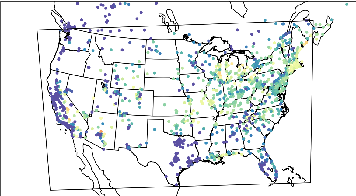
AirNOW (2023-07-27_13:00:00)
