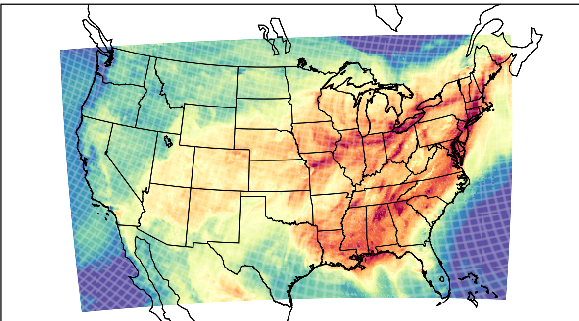
WRF (2023-07-27_17:00:00)
