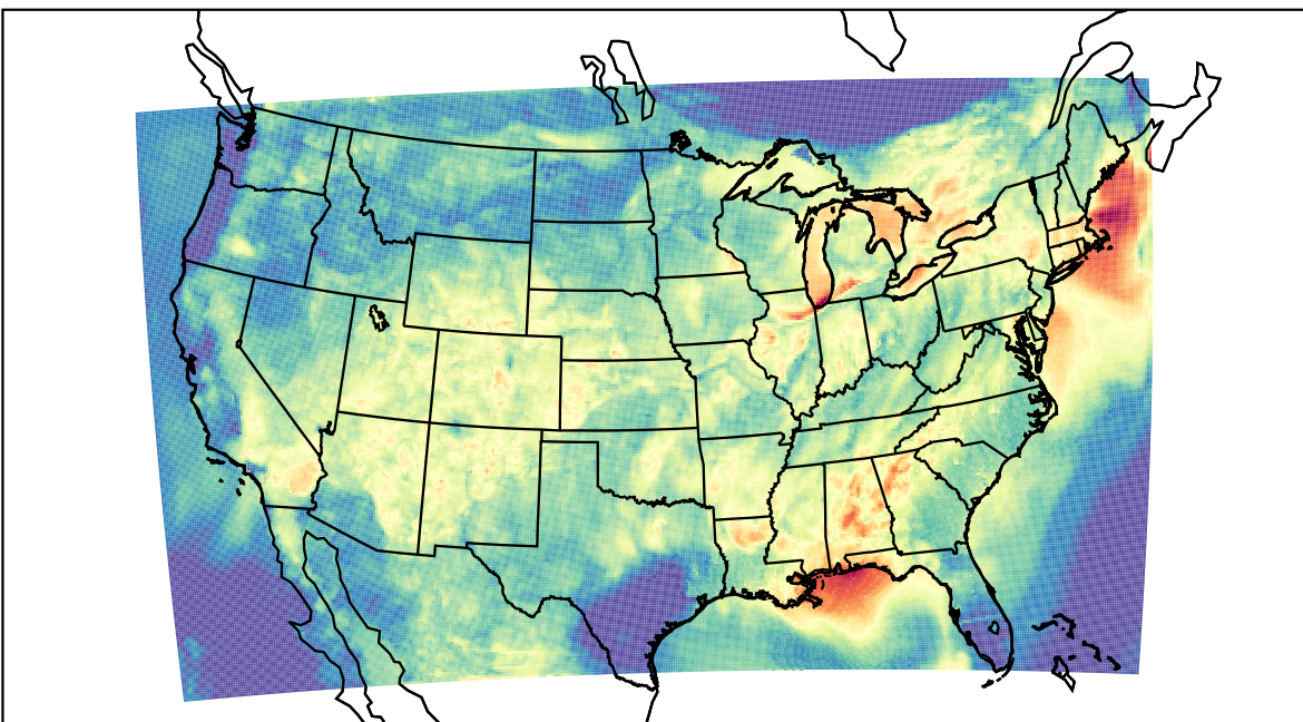
WRF (2023-07-27_05:00:00)
