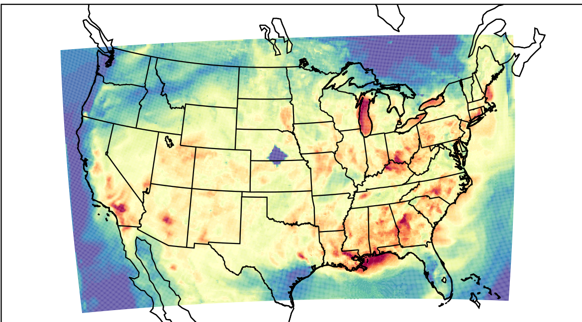
WRF (2023-07-26_01:00:00)
