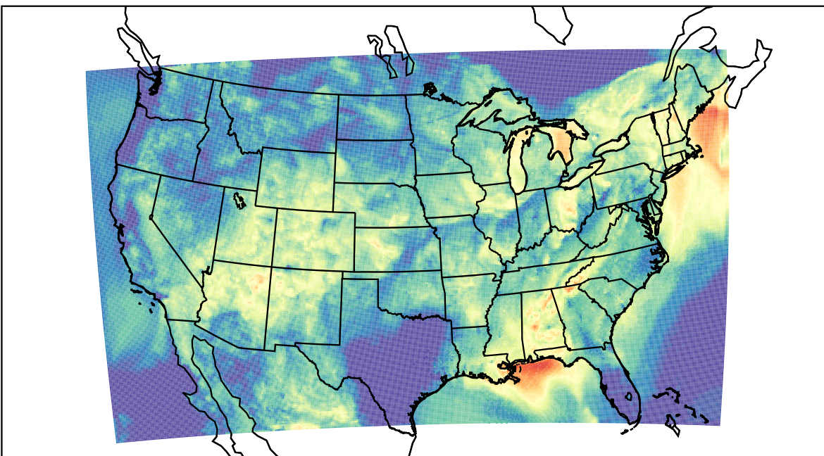
WRF (2023-07-27_11:00:00)
