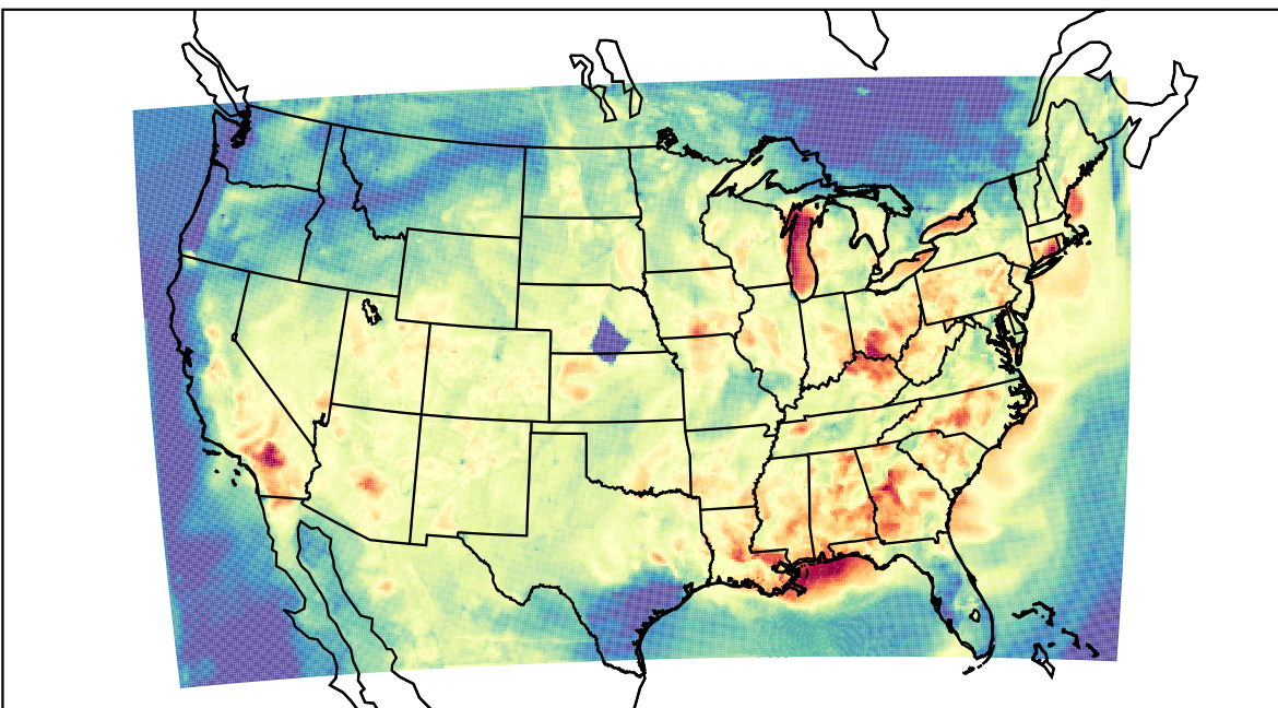
WRF (2023-07-26_02:00:00)
