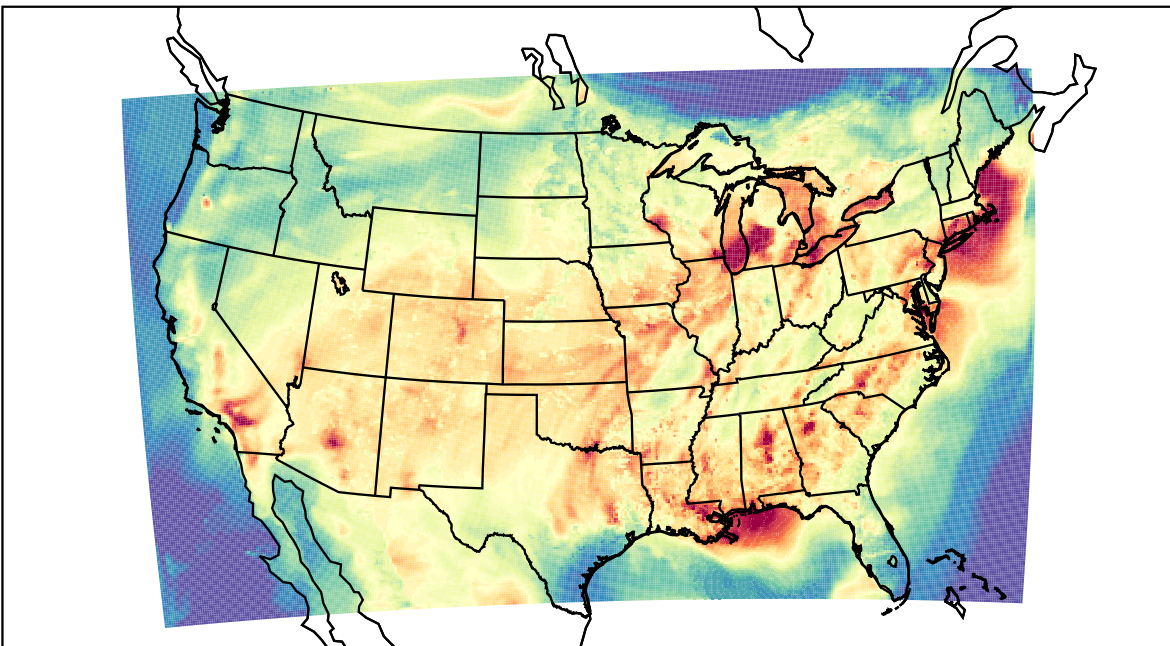
WRF (2023-07-27_00:00:00)
