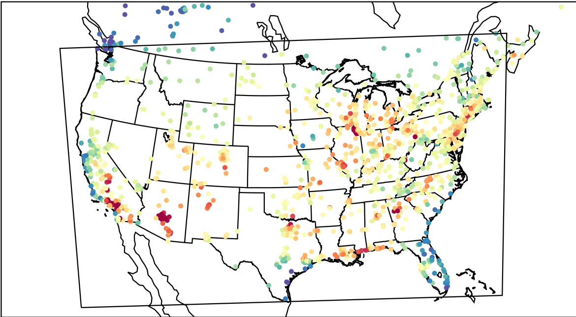
AirNOW (2023-07-27_20:00:00)
