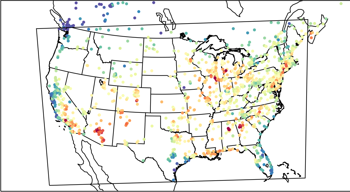
AirNOW (2023-07-27_18:00:00)
