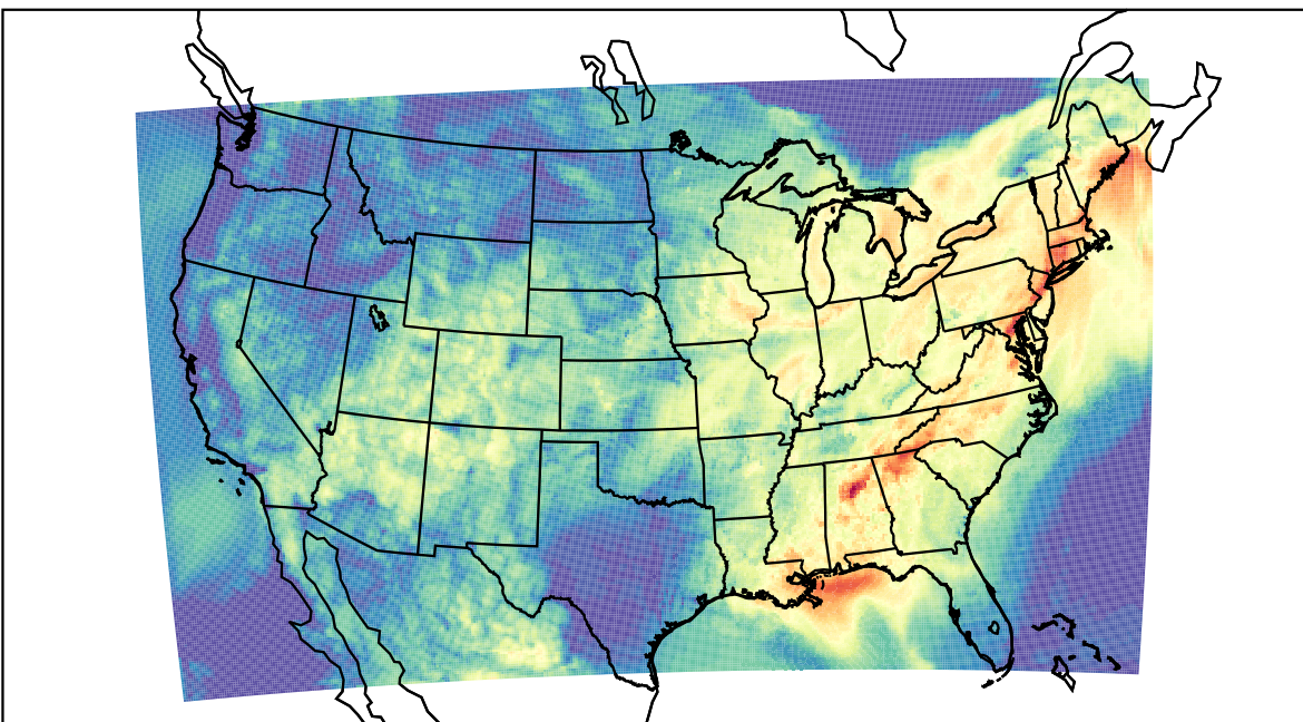
WRF (2023-07-27_14:00:00)
