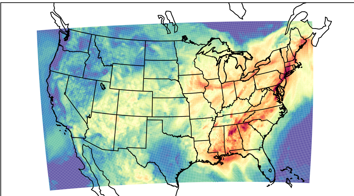
WRF (2023-07-27_15:00:00)
