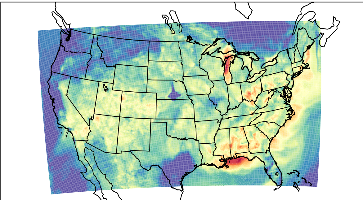
WRF (2023-07-26_06:00:00)
