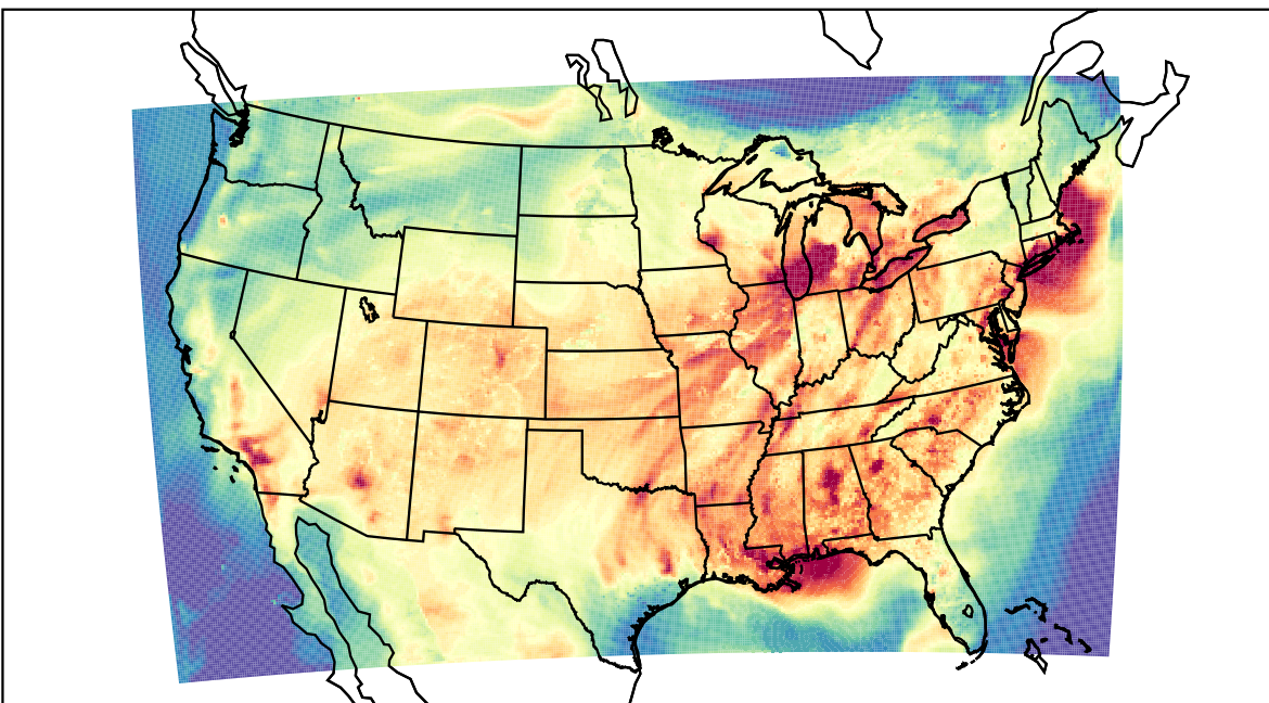
WRF (2023-07-26_23:00:00)
