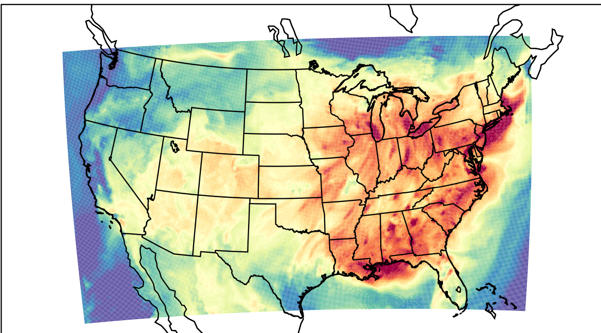
WRF (2023-07-26_17:00:00)
