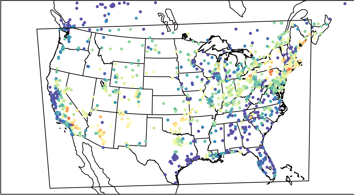
AirNOW (2023-07-27_04:00:00)
