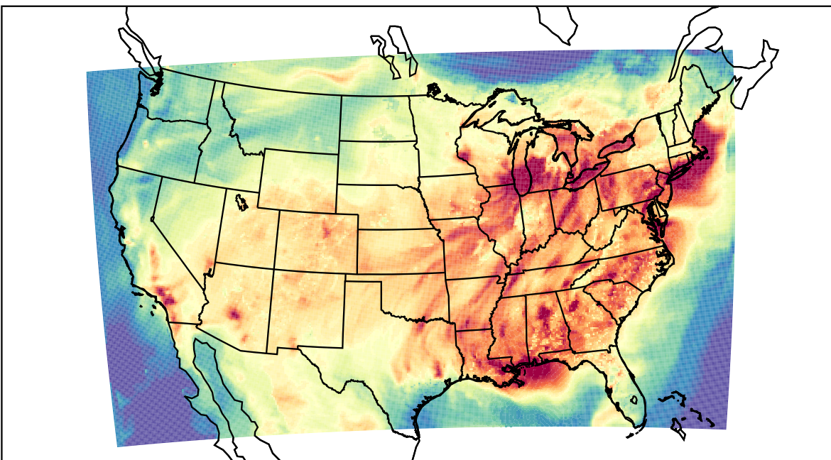
WRF (2023-07-26_22:00:00)
