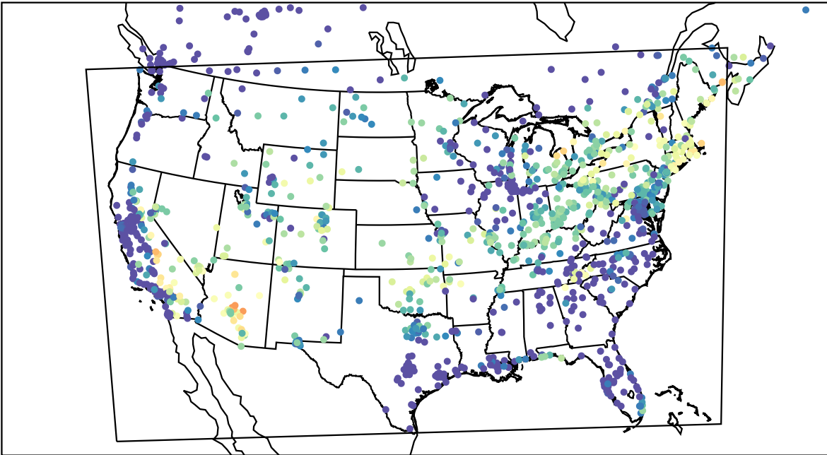
AirNOW (2023-07-27_09:00:00)
