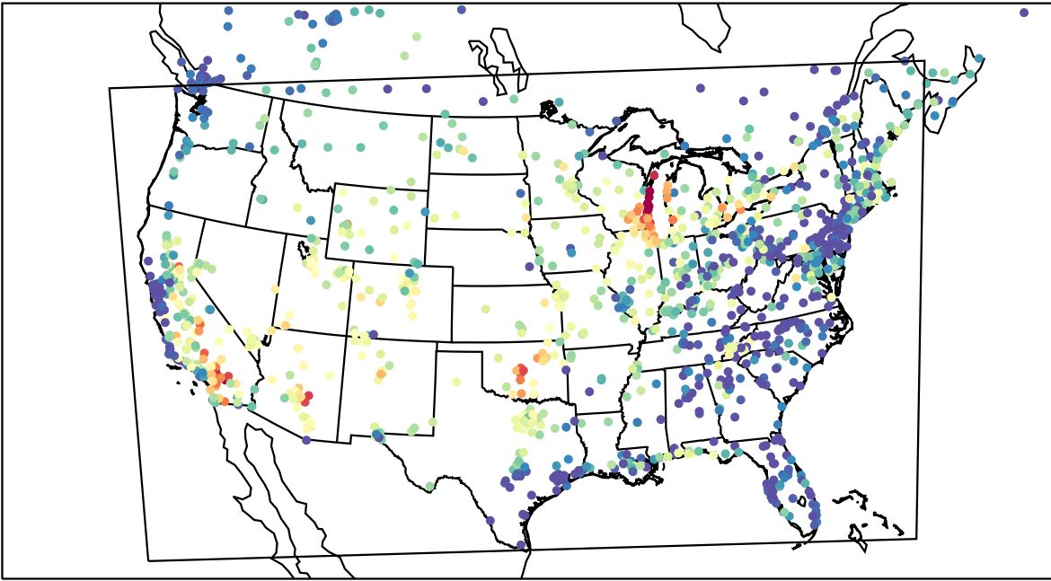
AirNOW (2023-07-26_03:00:00)
