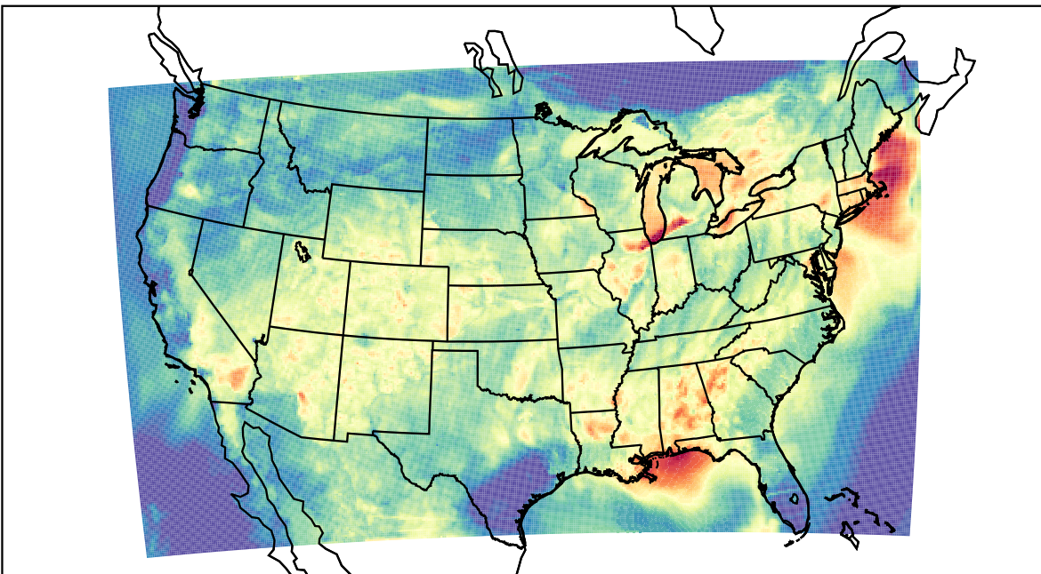
WRF (2023-07-27_04:00:00)
