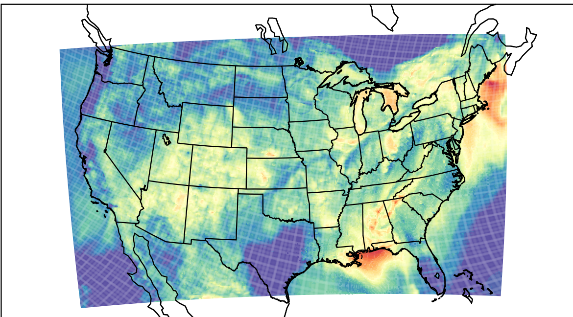
WRF (2023-07-27_09:00:00)
