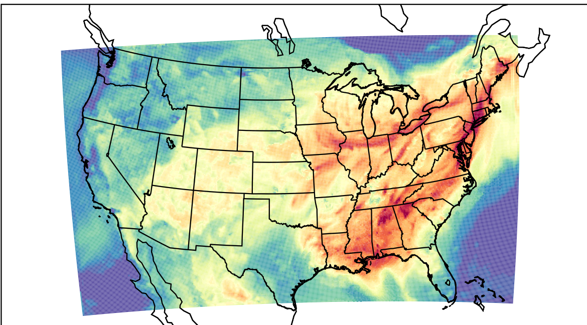
WRF (2023-07-27_16:00:00)
