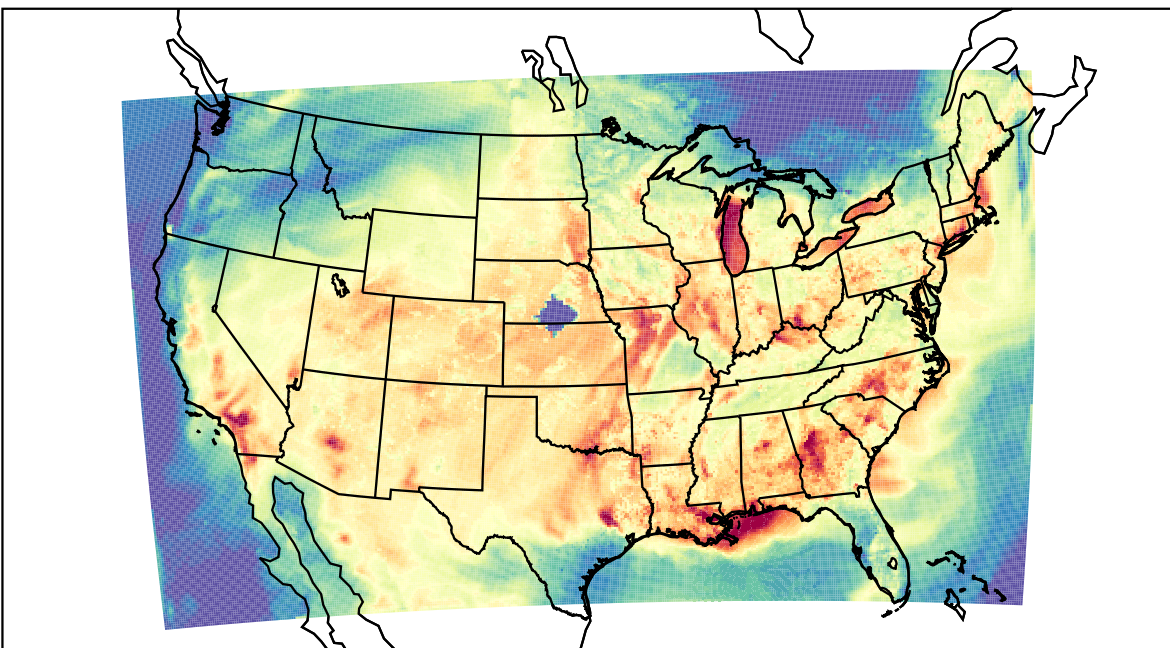
WRF (2023-07-26_00:00:00)
