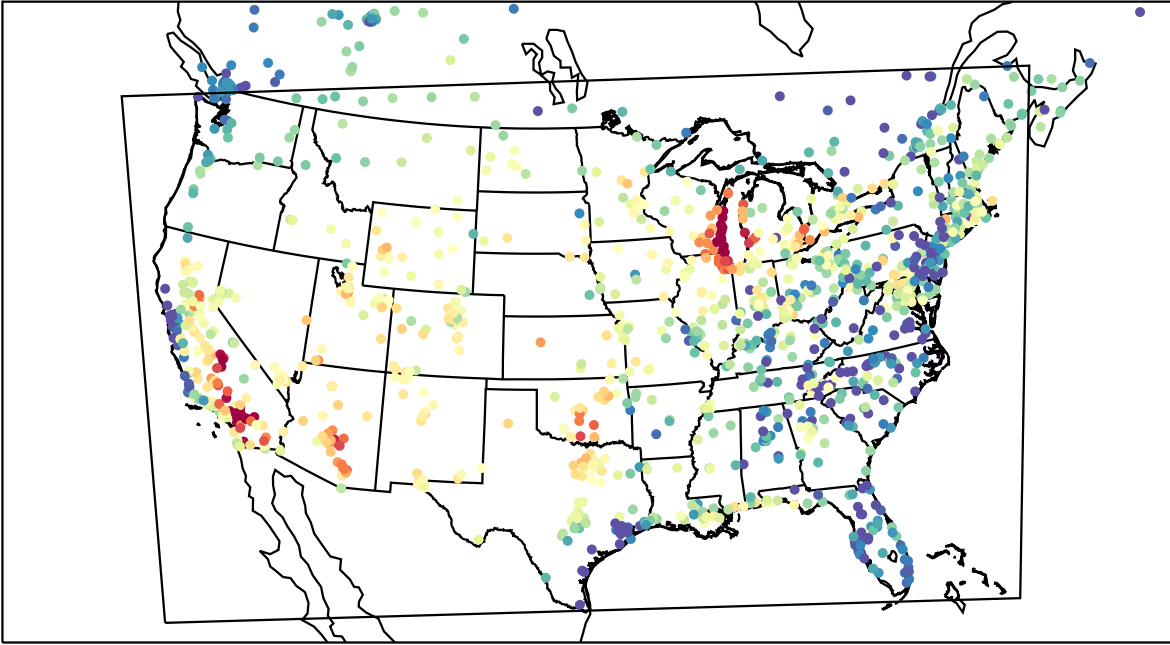
AirNOW (2023-07-26_01:00:00)
