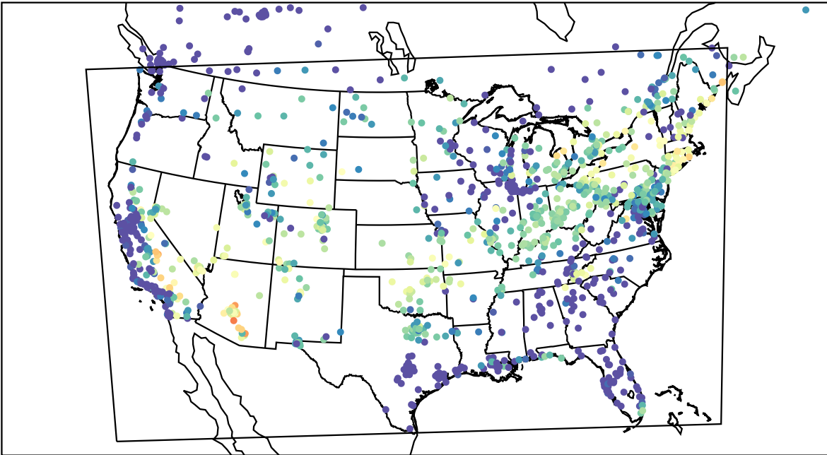
AirNOW (2023-07-27_08:00:00)
