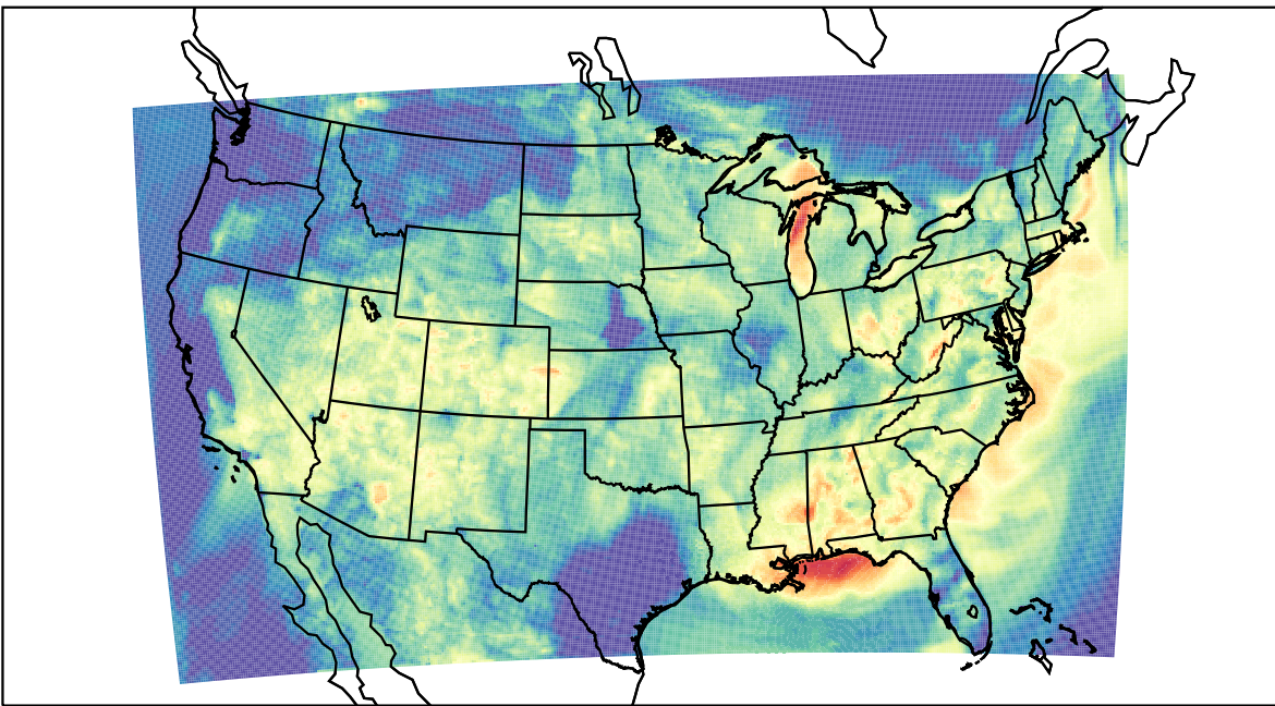
WRF (2023-07-26_08:00:00)
