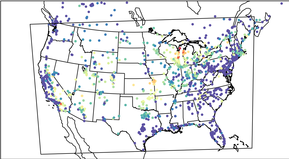
AirNOW (2023-07-26_09:00:00)
