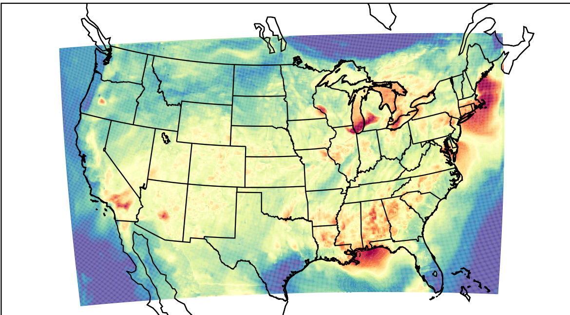
WRF (2023-07-27_02:00:00)
