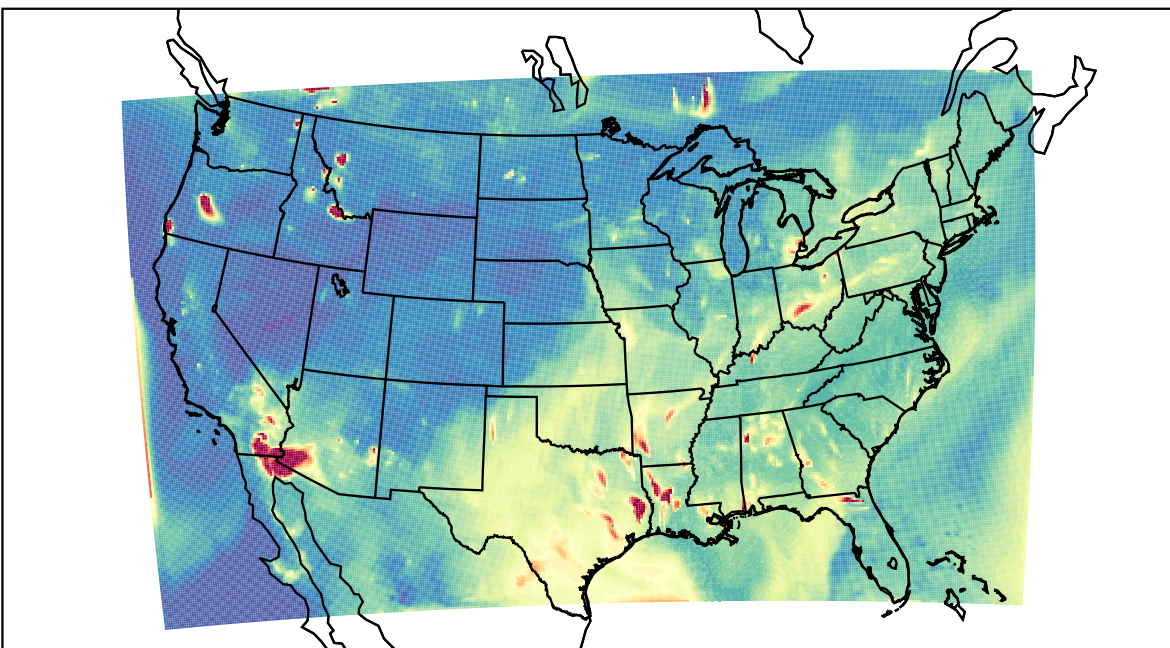
WRF 2023-07-28_04:00:00
