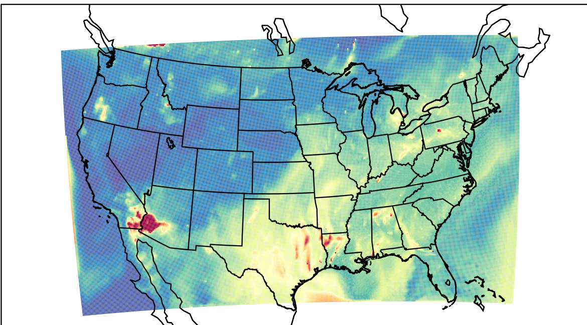
WRF 2023-07-28_09:00:00
