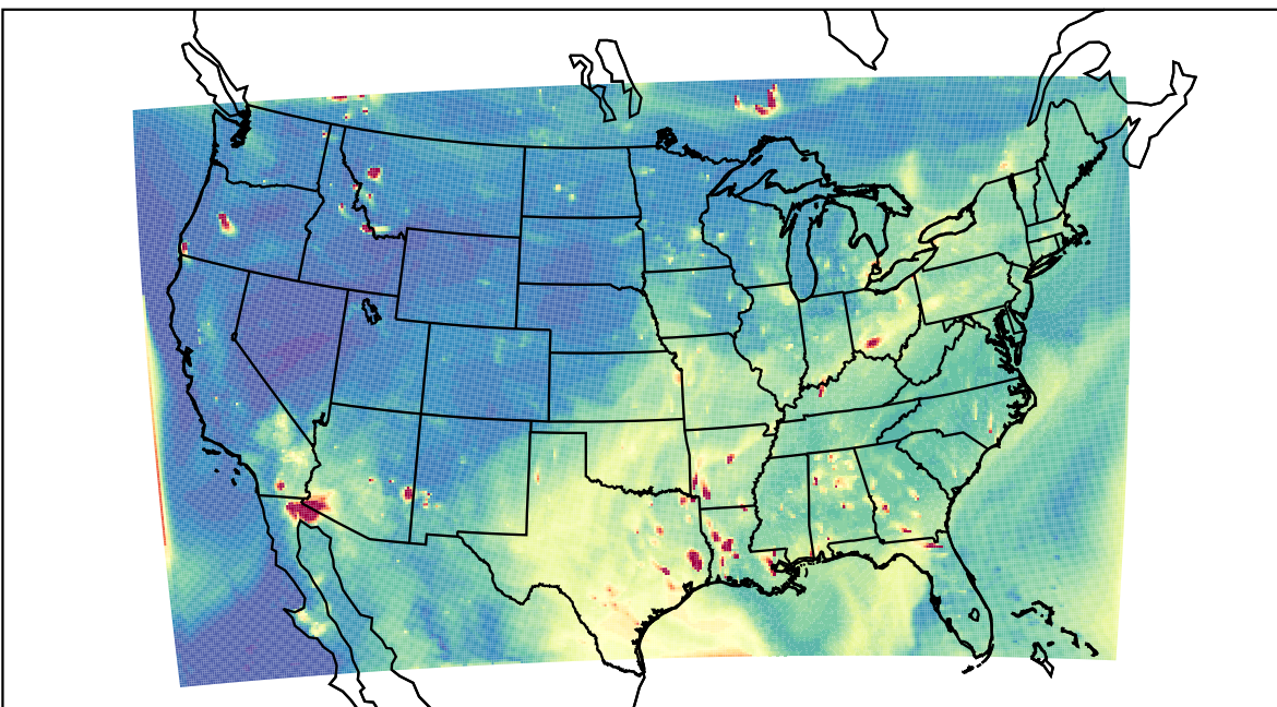
WRF 2023-07-28_02:00:00
