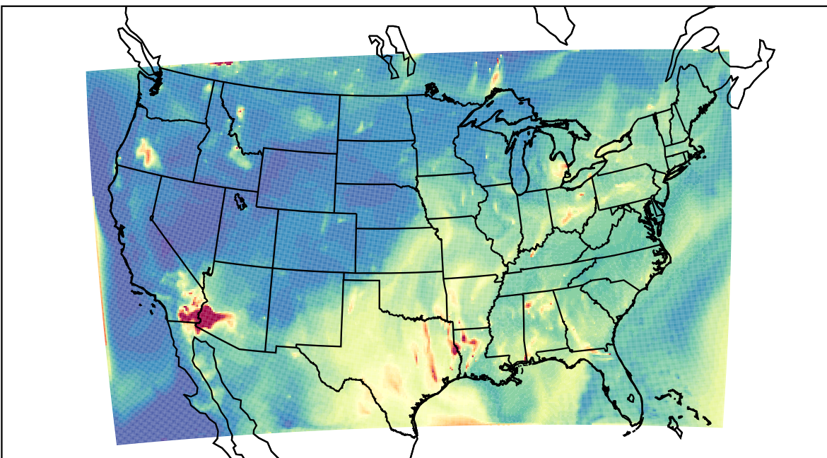
WRF 2023-07-28_07:00:00
