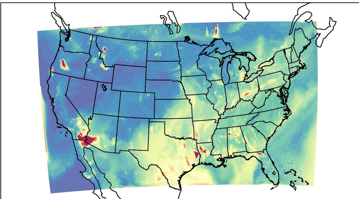
WRF 2023-07-28_05:00:00
