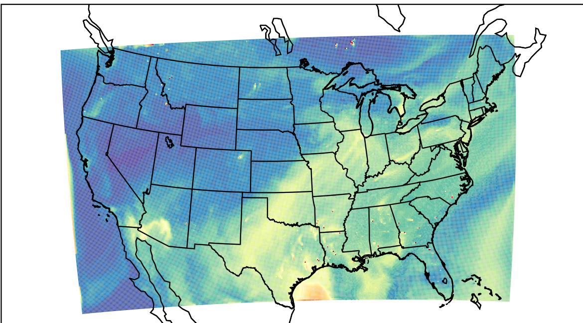
WRF 2023-07-28_19:00:00
