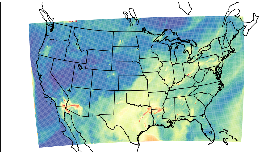
WRF 2023-07-28_15:00:00
