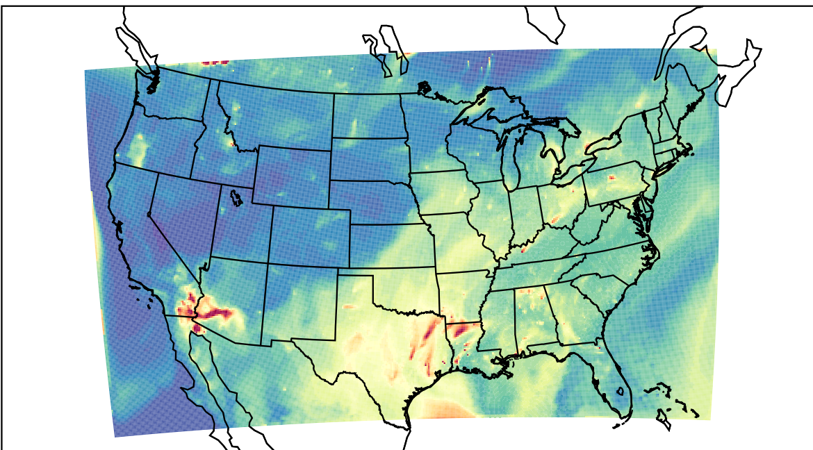
WRF 2023-07-28_12:00:00
