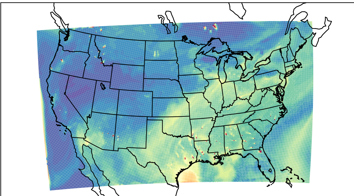
WRF 2023-07-28_22:00:00
