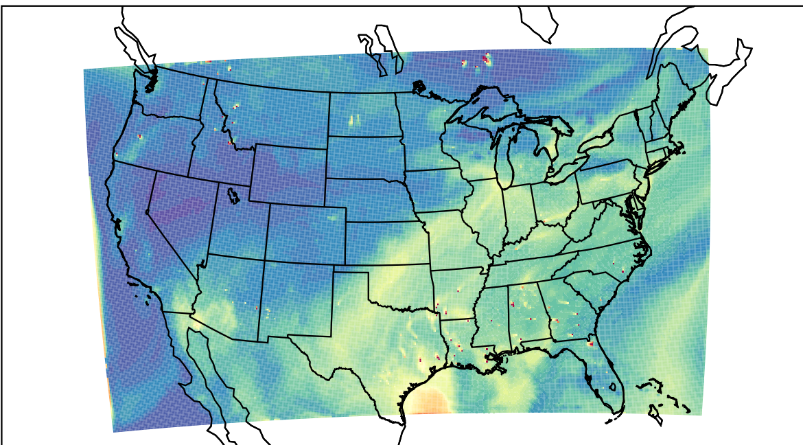
WRF 2023-07-28_21:00:00
