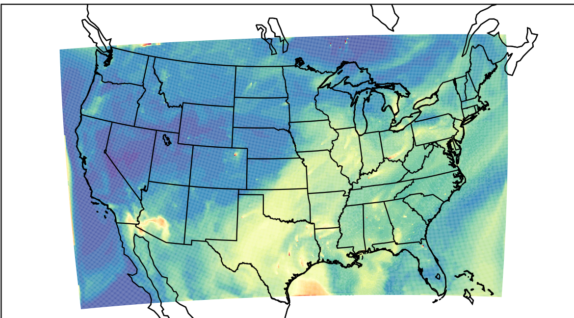
WRF 2023-07-28_17:00:00
