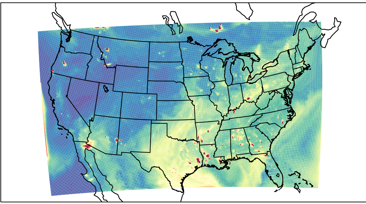
WRF 2023-07-28_01:00:00
