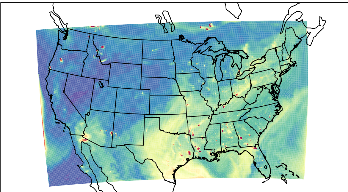
WRF 2023-07-28_00:00:00
