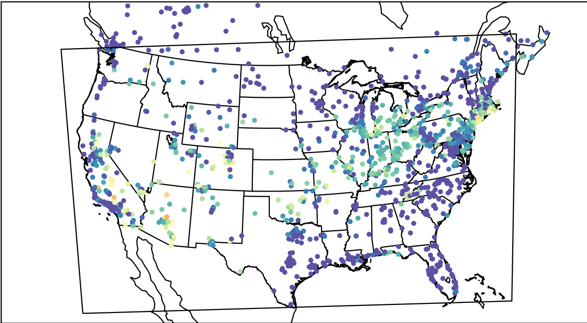
AirNOW (2023-07-29_11:00:00)
