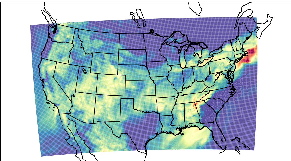
WRF (2023-07-29_11:00:00)
