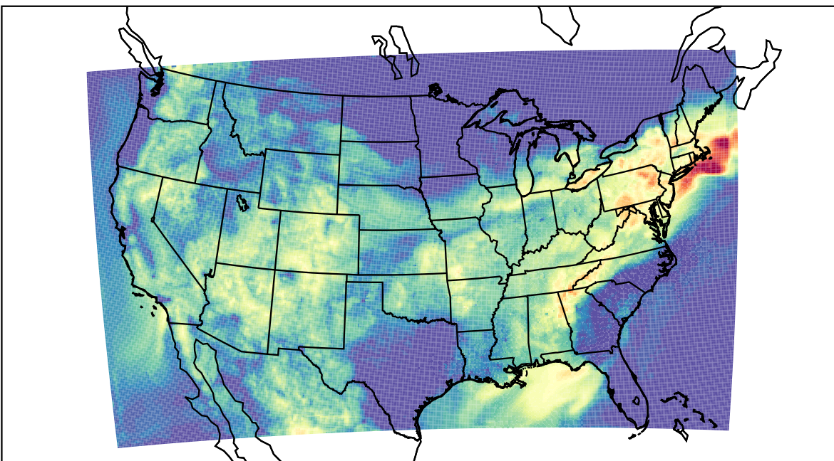
WRF (2023-07-29_13:00:00)
