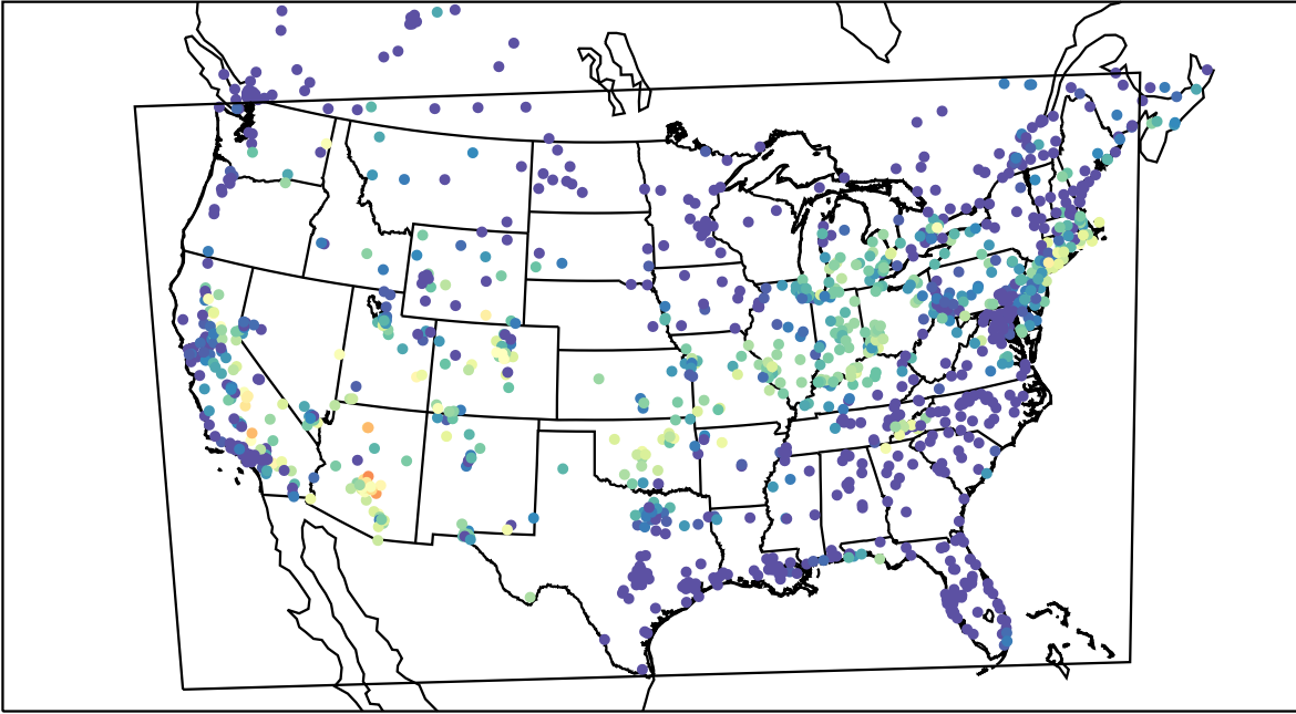
AirNOW (2023-07-29_10:00:00)
