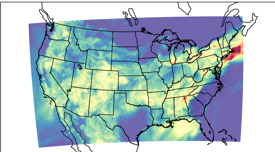
WRF (2023-07-29_09:00:00)
