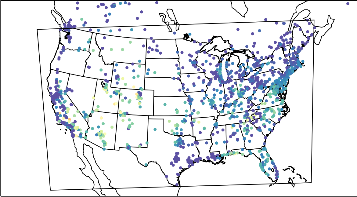
AirNOW (2023-07-30_13:00:00)
