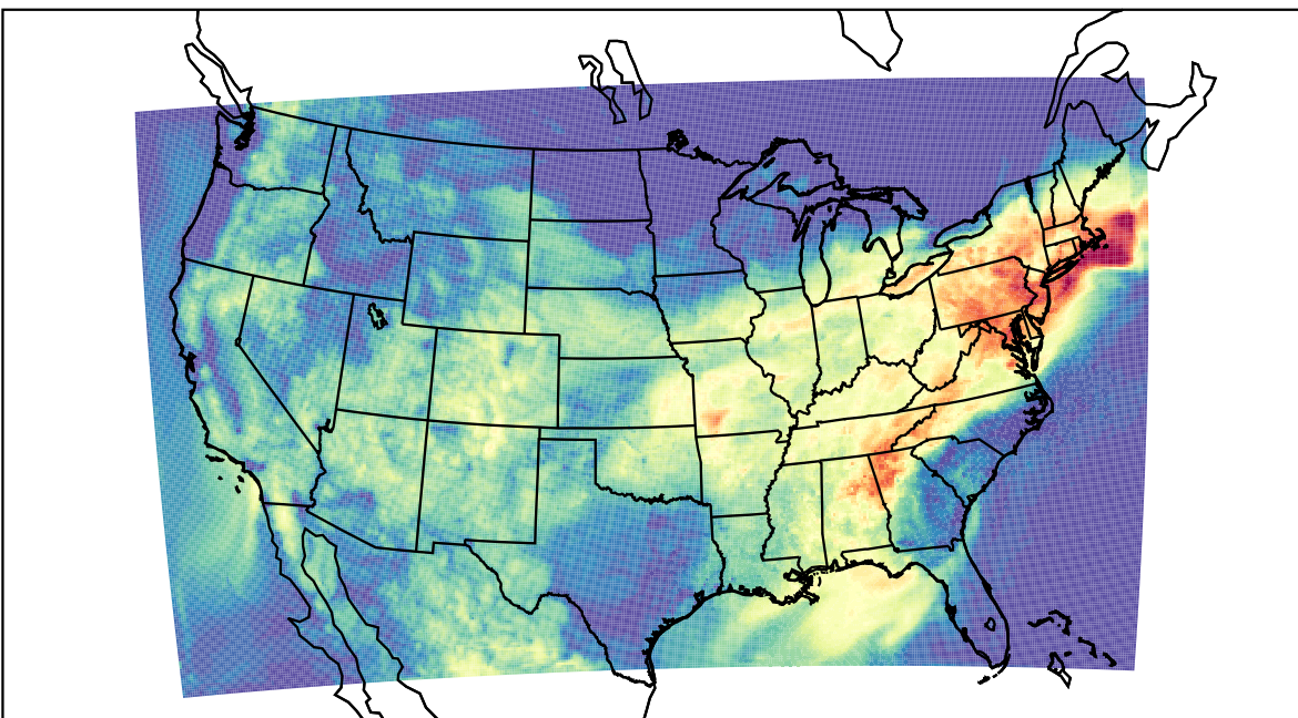
WRF (2023-07-29_14:00:00)
