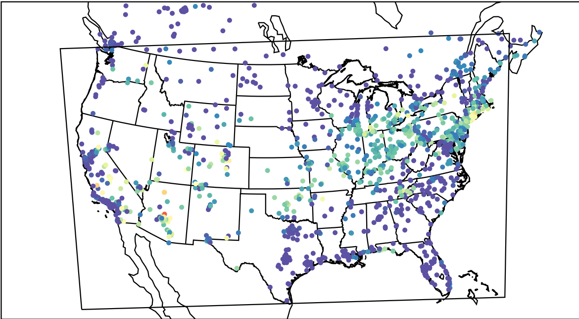
AirNOW (2023-07-29_12:00:00)
