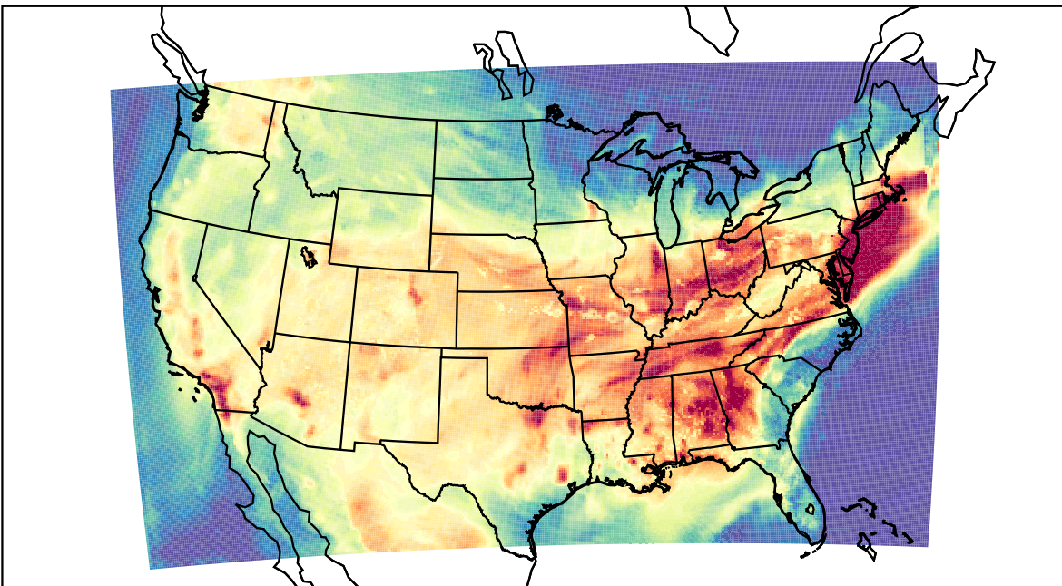
WRF (2023-07-29_22:00:00)
