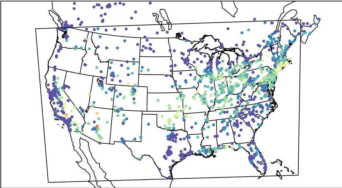
AirNOW (2023-07-29_13:00:00)
