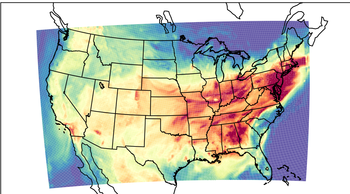
WRF (2023-07-29_19:00:00)
