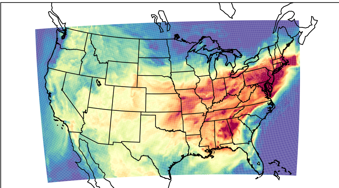
WRF (2023-07-29_17:00:00)
