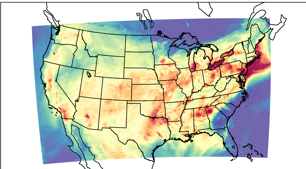
WRF (2023-07-29_00:00:00)
