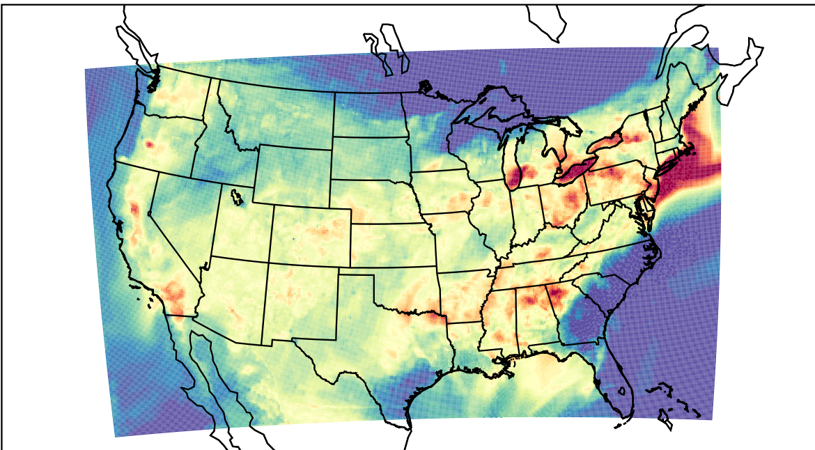
WRF (2023-07-29_02:00:00)
