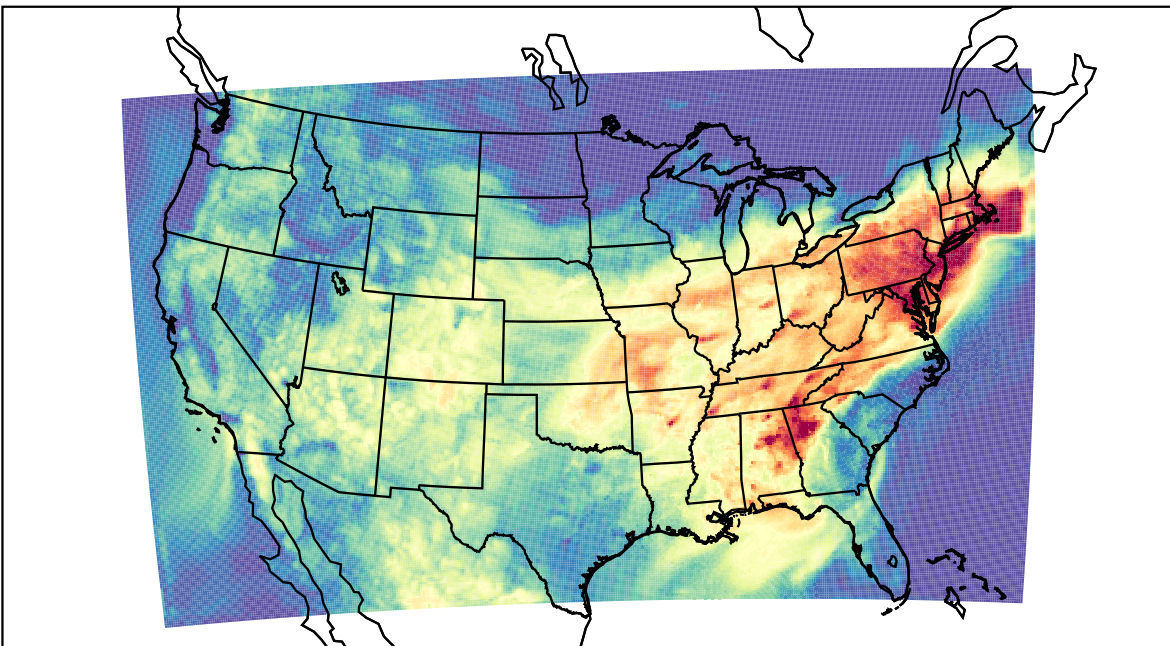
WRF (2023-07-29_15:00:00)
