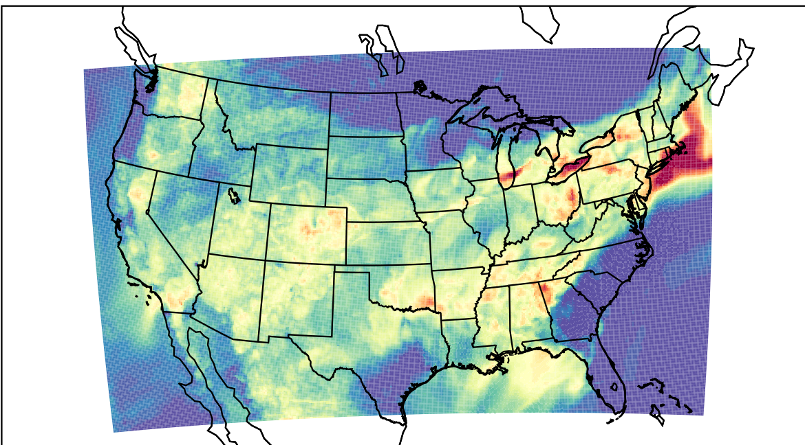
WRF (2023-07-29_05:00:00)
