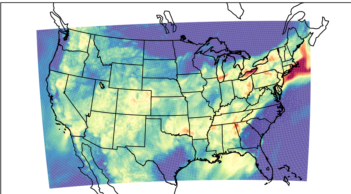
WRF (2023-07-29_06:00:00)
