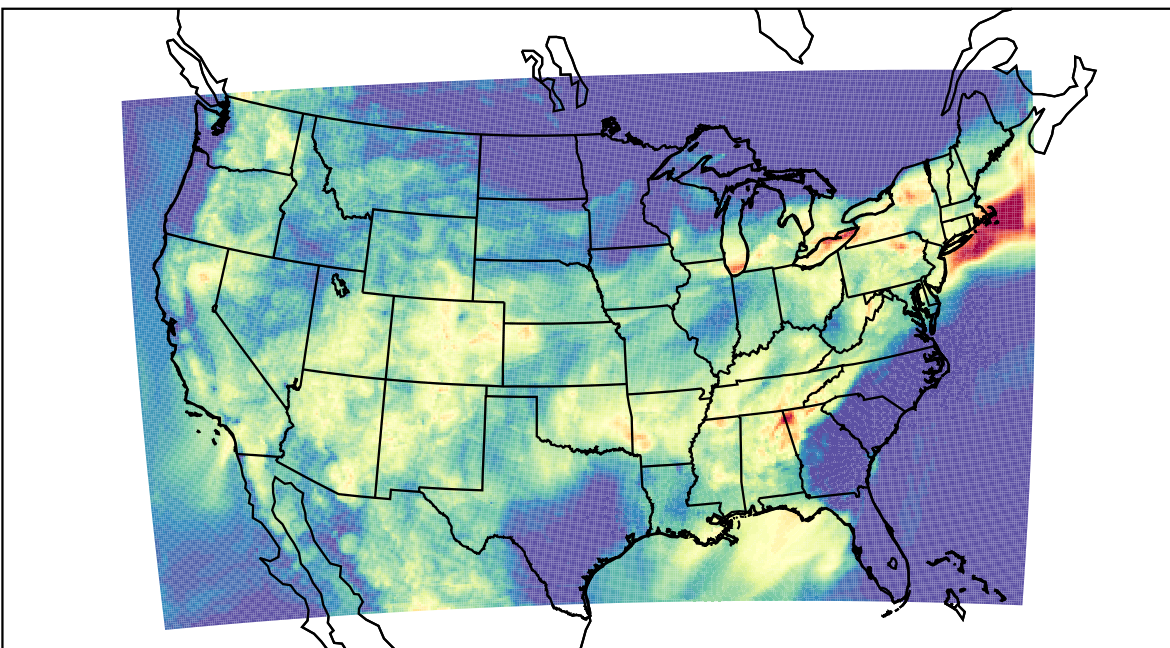
WRF (2023-07-29_08:00:00)
