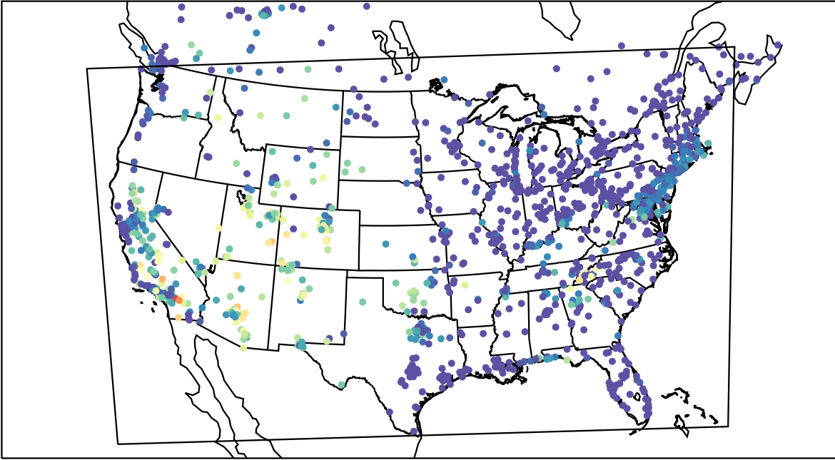
AirNOW (2023-07-30_09:00:00)
