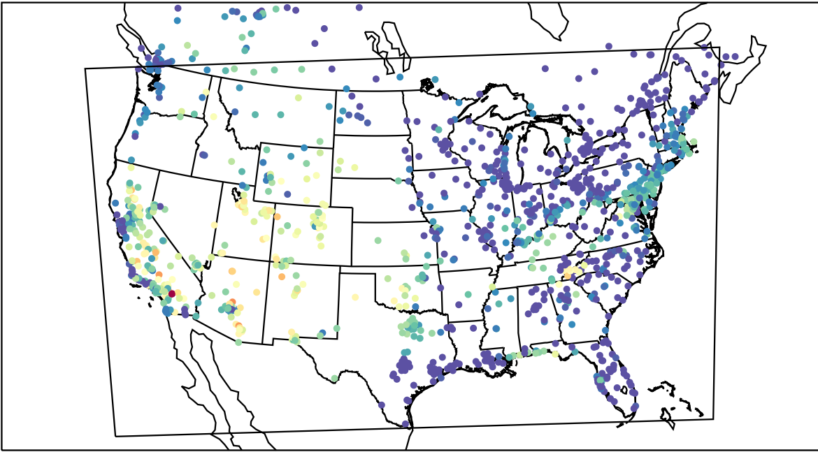
AirNOW (2023-07-30_05:00:00)
