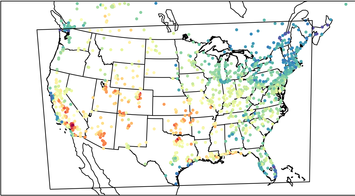
AirNOW (2023-07-30_21:00:00)
