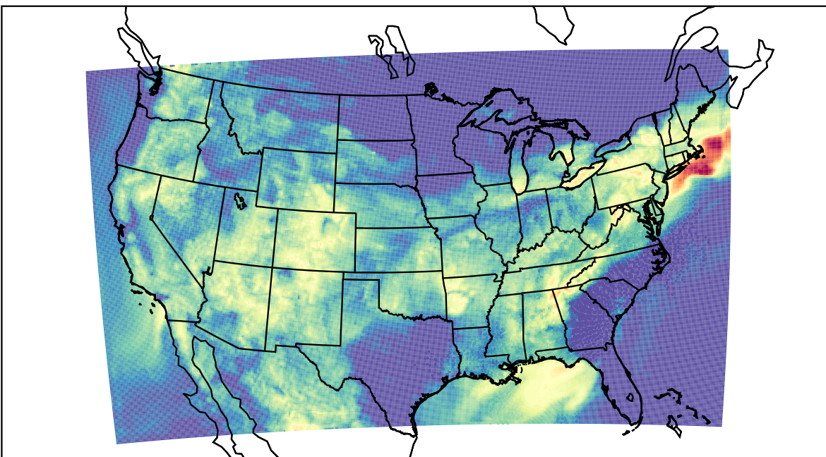
WRF (2023-07-29_12:00:00)
