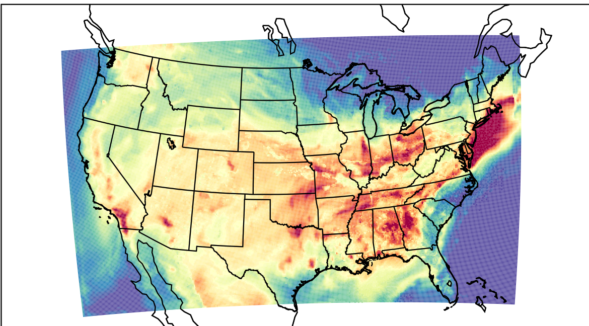
WRF (2023-07-29_23:00:00)
