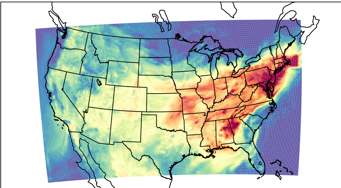
WRF (2023-07-29_16:00:00)
