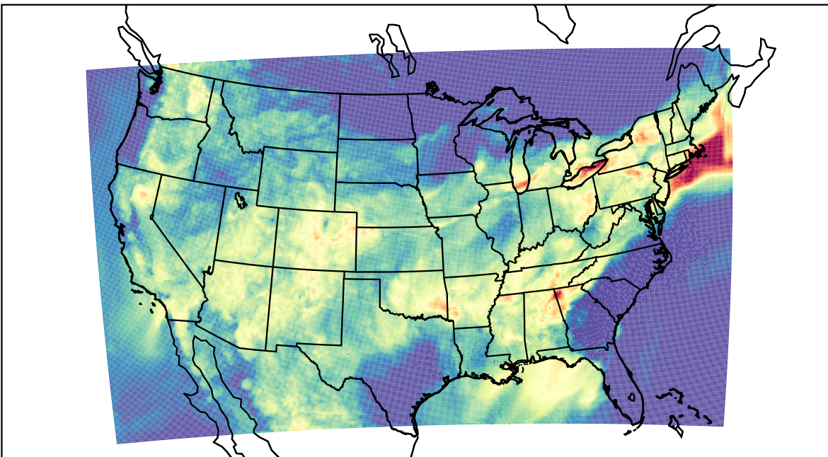
WRF (2023-07-29_07:00:00)
