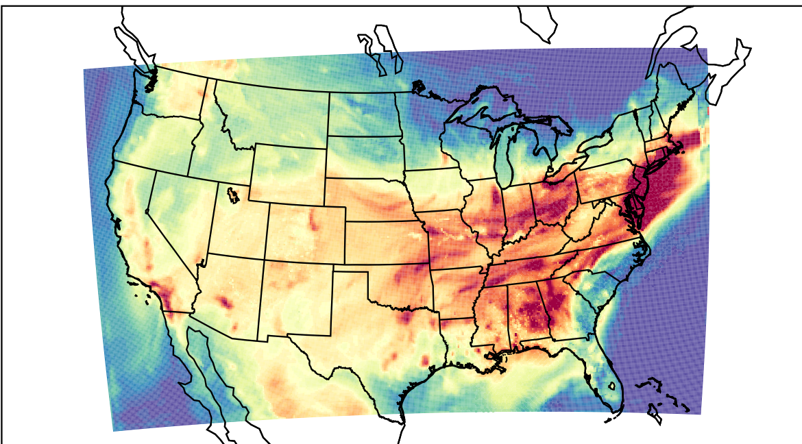
WRF (2023-07-29_21:00:00)
