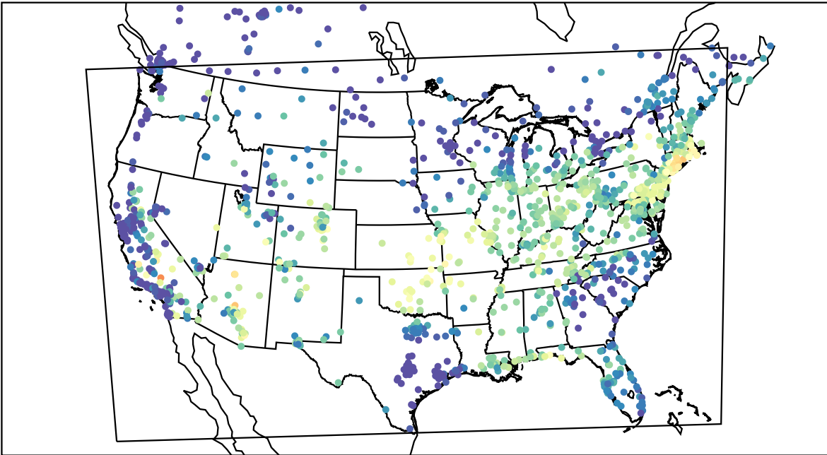
AirNOW (2023-07-29_14:00:00)
