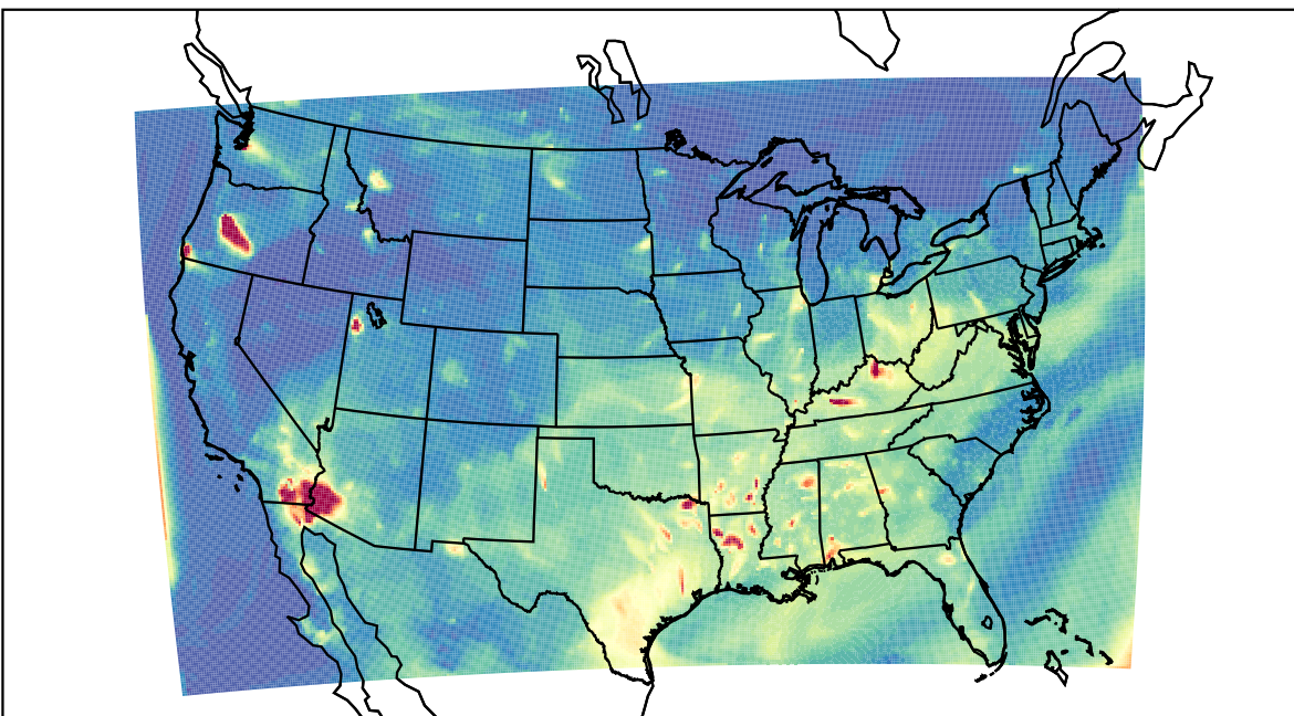
WRF 2023-07-30_05:00:00
