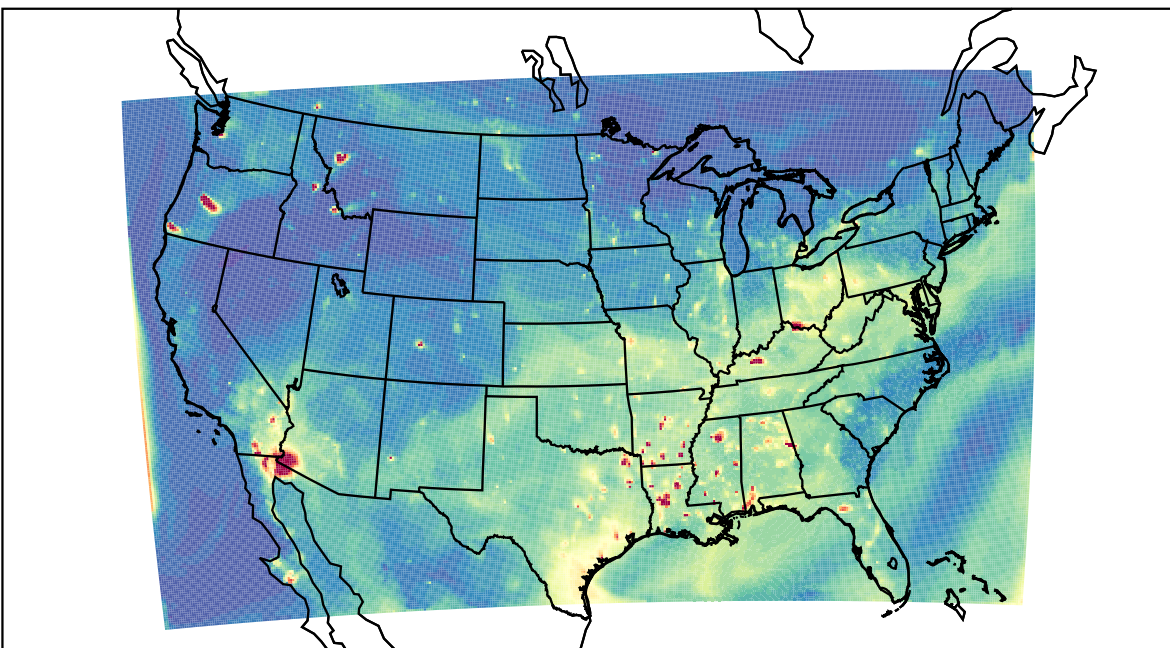
WRF 2023-07-30_02:00:00
