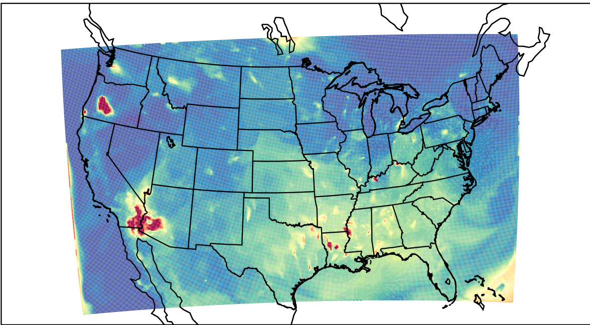
WRF 2023-07-31_05:00:00
