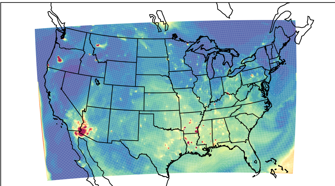
WRF 2023-07-31_02:00:00
