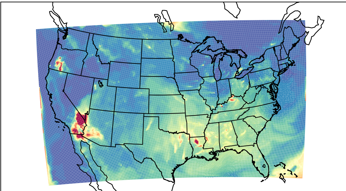
WRF 2023-07-31_09:00:00
