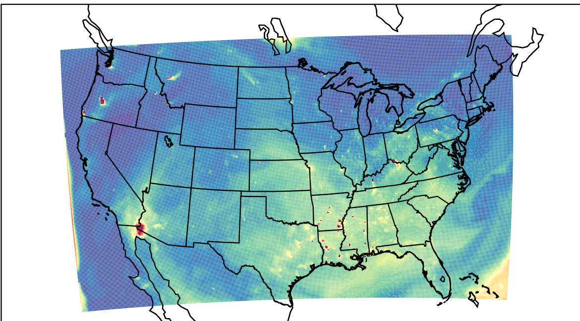
WRF 2023-07-31_00:00:00
