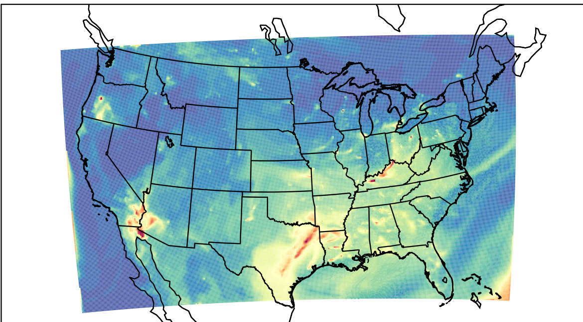
WRF 2023-07-30_12:00:00
