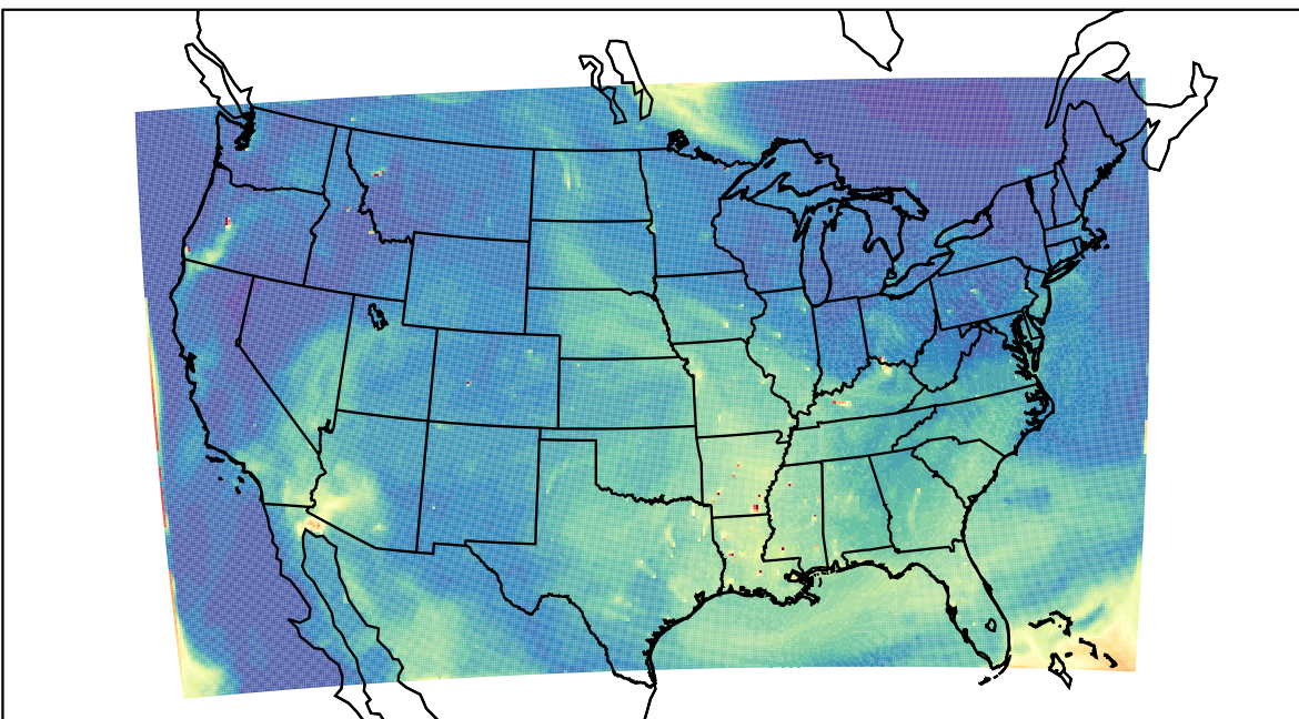
WRF 2023-07-31_21:00:00
