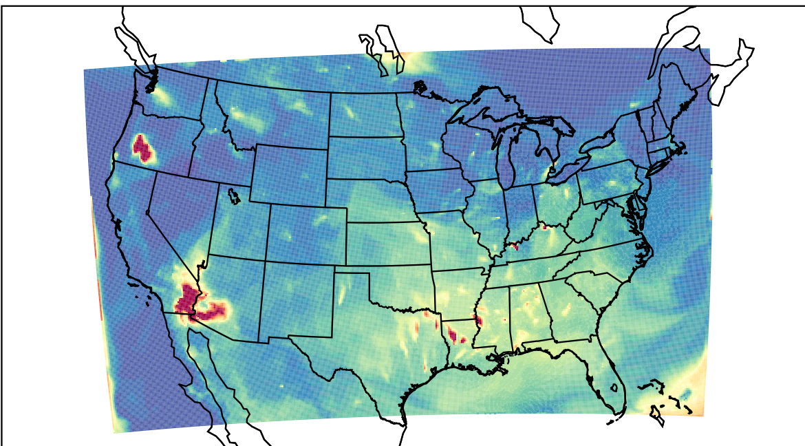
WRF 2023-07-31_06:00:00
