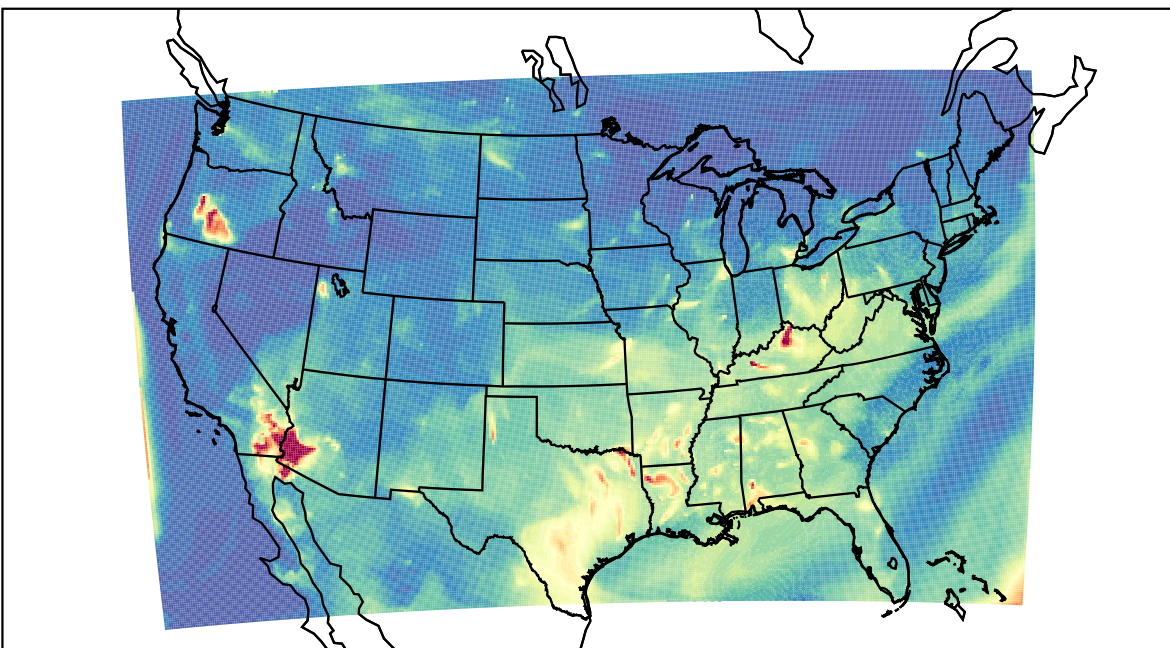
WRF 2023-07-30_07:00:00
