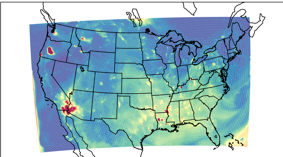
WRF 2023-07-31_04:00:00
